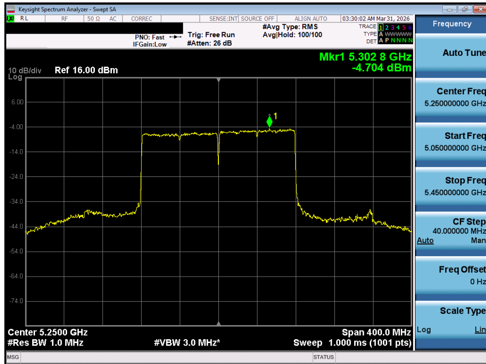
Plot 7-75. Power Spectral Density Plot MIMO ANT1 (160MHz BW 802.11be – 2x996 Tones (UNII Band 1/2A) – Ch. 50)
