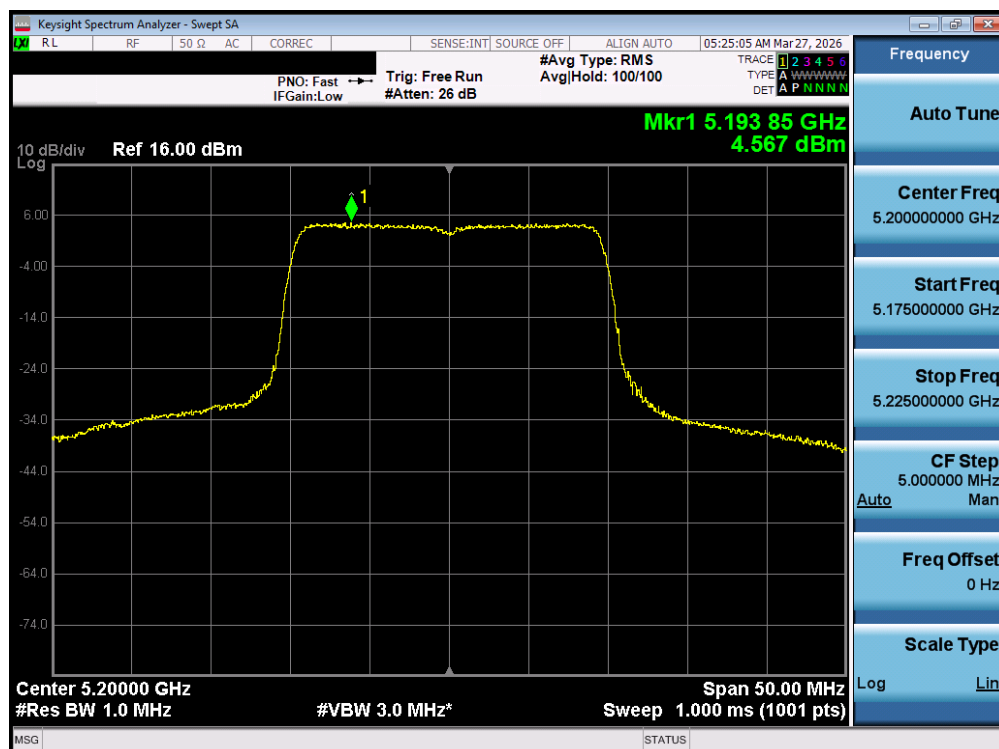
Plot 7-72. Power Spectral Density Plot MIMO ANT1 (20MHz BW 802.11be – 242 Tones (UNII Band 1) – Ch. 40)
