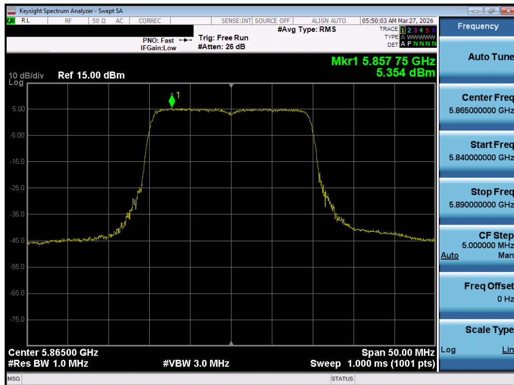
Plot 7-79. Power Spectral Density Plot MIMO ANT1 (20MHz BW 802.11be – 242 Tones (UNII Band 4) – Ch. 173)
