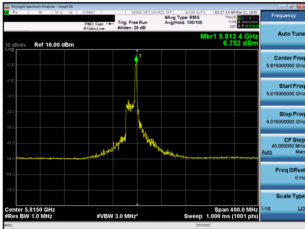
Plot 7-71. Power Spectral Density Plot MIMO ANT1 (160MHz BW 802.11be – 26 Tones (UNII Band 3/4) – Ch. 163)
