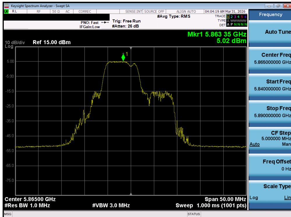
Plot 7-88. Power Spectral Density Plot MIMO ANT1 (20MHz BW 802.11be – 52+26 Tones (UNII Band 4) – Ch. 173)
