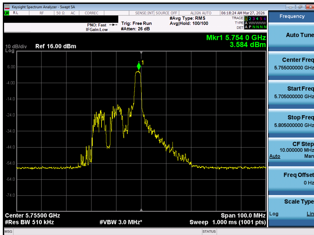
Plot 7-66. Power Spectral Density Plot MIMO ANT1 (40MHz BW 802.11be – 26 Tones (UNII Band 3) – Ch. 151)
