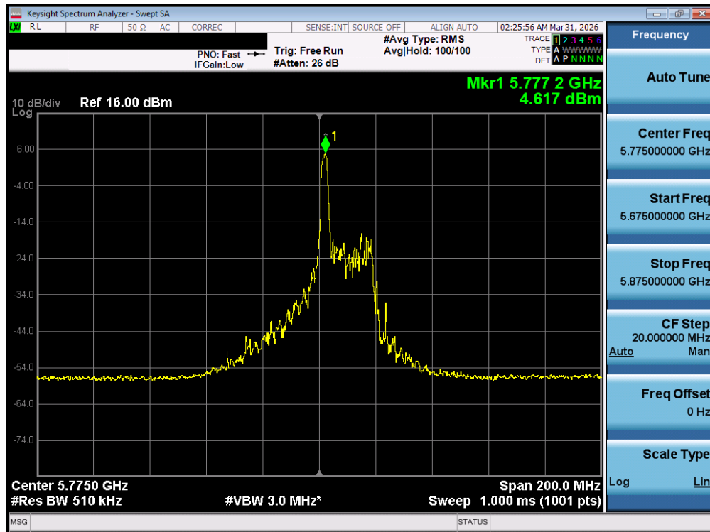
Plot 7-67. Power Spectral Density Plot MIMO ANT1 (80MHz BW 802.11be – 26 Tones (UNII Band 3) – Ch. 155)
