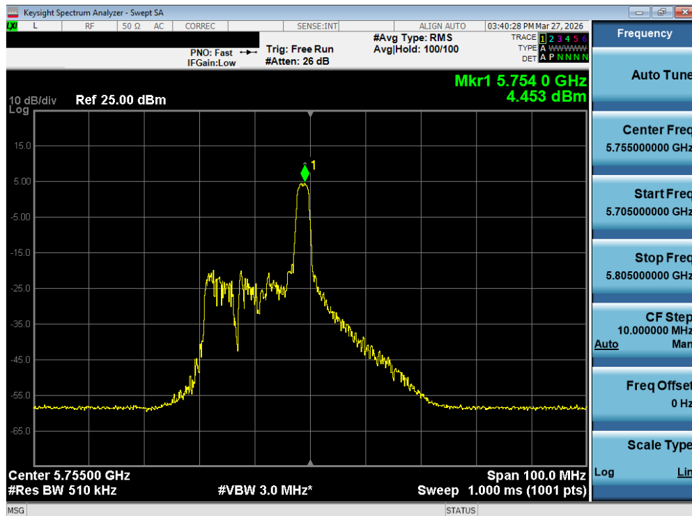
Plot 7-96. Power Spectral Density Plot MIMO ANT2 (40MHz BW 802.11be – 26 Tones (UNII Band 3) – Ch. 151)
