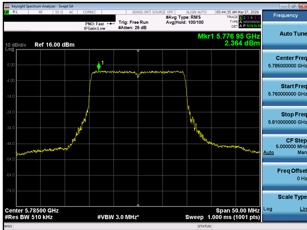
Plot 7-76. Power Spectral Density Plot MIMO ANT1 (20MHz BW 802.11be – 242 Tones (UNII Band 3) – Ch. 157)
