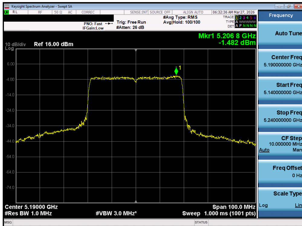
Plot 7-73. Power Spectral Density Plot MIMO ANT1 (40MHz BW 802.11be – 484 Tones (UNII Band 1) – Ch. 38)
