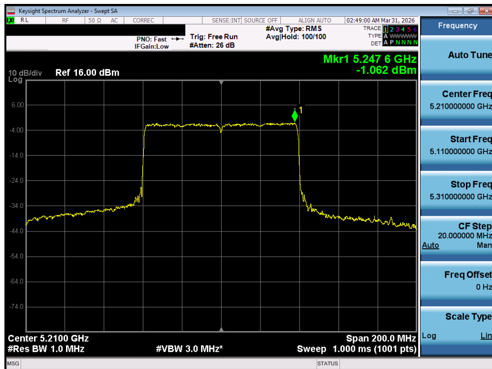
Plot 7-74. Power Spectral Density Plot MIMO ANT1 (80MHz BW 802.11be – 996 Tones (UNII Band 1) – Ch. 42)
