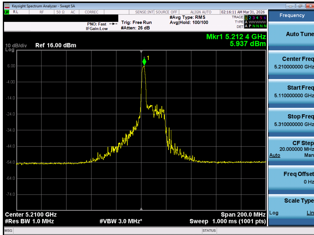
Plot 7-63. Power Spectral Density Plot MIMO ANT1 (80MHz BW 802.11be – 26 Tones (UNII Band 1) – Ch. 42)
