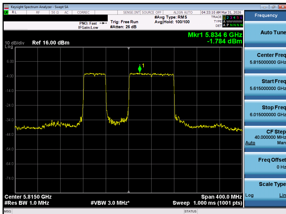
Plot 7-90. Power Spectral Density Plot MIMO ANT1 (160MHz BW 802.11be – 996+484 Tones (UNII Band 3/4) – Ch. 163)
