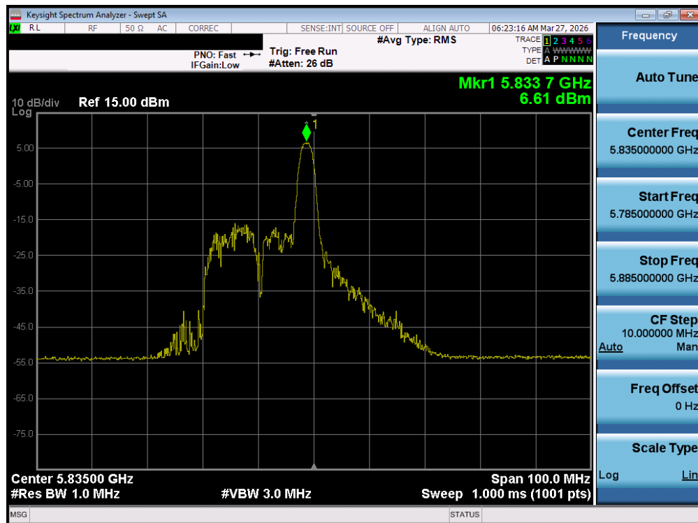
Plot 7-69. Power Spectral Density Plot MIMO ANT1 (40MHz BW 802.11be – 26 Tones (UNII Band 3/4) – Ch. 167)
