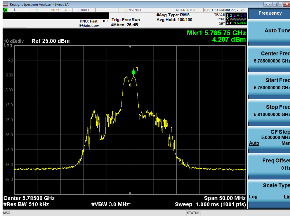
Plot 7-95. Power Spectral Density Plot MIMO ANT2 (20MHz BW 802.11be – 26 Tones (UNII Band 3) – Ch. 157)
