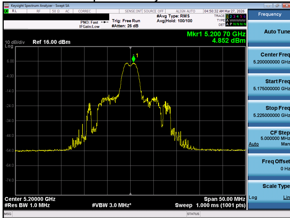
Plot 7-61. Power Spectral Density Plot MIMO ANT1 (20MHz BW 802.11be – 26 Tones (UNII Band 1) – Ch. 40)
