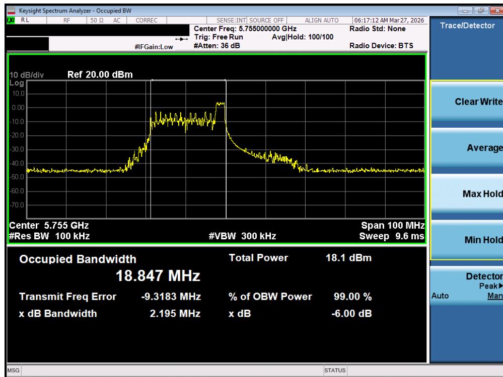
Plot 7-24. 6dB Bandwidth Plot MIMO ANT1 (40MHz BW 802.11be – 26 Tones (UNII Band 3) – Ch. 151)
