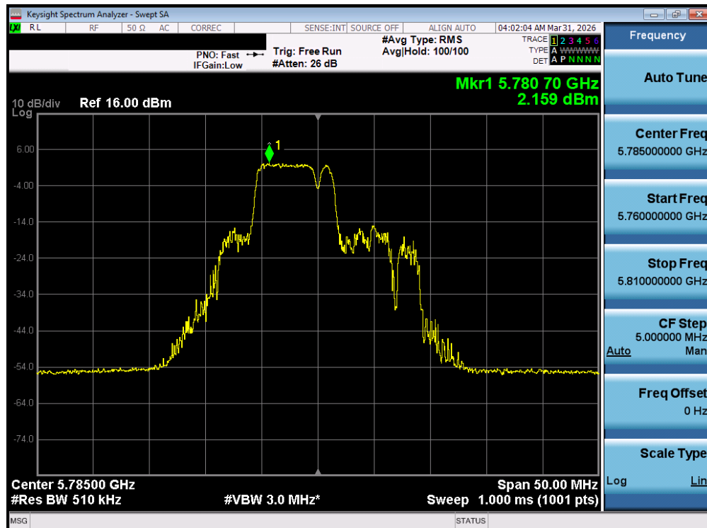
Plot 7-86. Power Spectral Density Plot MIMO ANT1 (20MHz BW 802.11be – 52+26 Tones (UNII Band 3) – Ch. 157)
