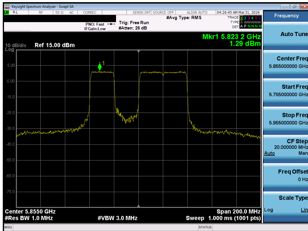
Plot 7-89. Power Spectral Density Plot MIMO ANT1 (80MHz BW 802.11be – 484+242 Tones (UNII Band 3/4) – Ch. 171)
