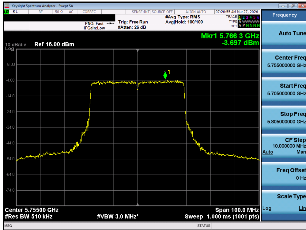
Plot 7-77. Power Spectral Density Plot MIMO ANT1 (40MHz BW 802.11be – 484 Tones (UNII Band 3) – Ch. 151)
