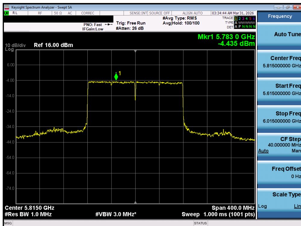
Plot 7-82. Power Spectral Density Plot MIMO ANT1 (160MHz BW 802.11be – 996*2 Tones (UNII Band 3/4) – Ch. 163)
