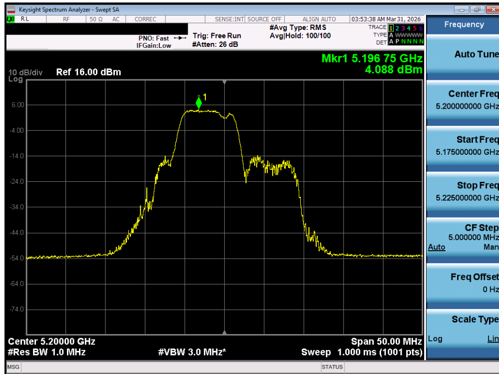
Plot 7-83. Power Spectral Density Plot MIMO ANT1 (20MHz BW 802.11be – 52+26 Tones (UNII Band 1) – Ch. 40)
