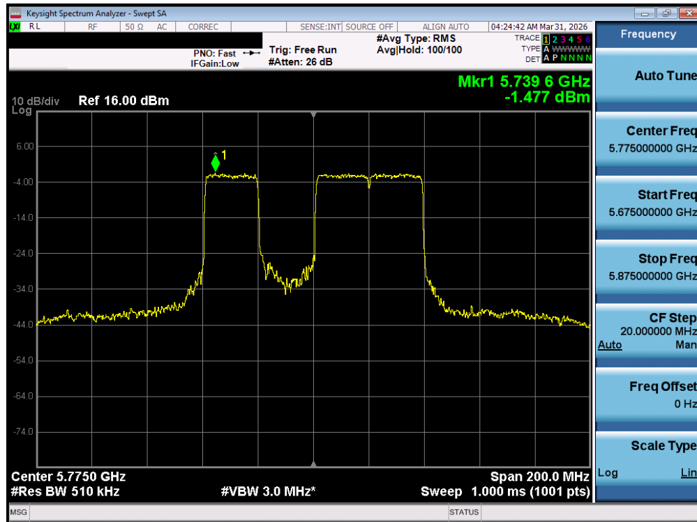
Plot 7-87. Power Spectral Density Plot MIMO ANT1 (80MHz BW 802.11be – 484+242 Tones (UNII Band 3) – Ch. 155)
