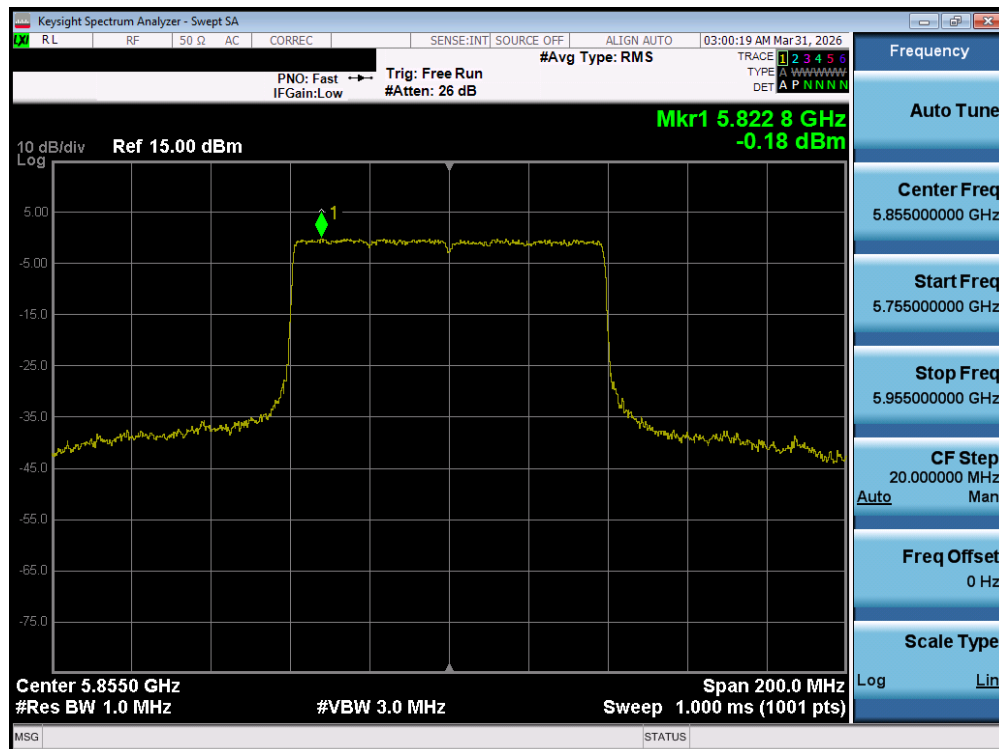
Plot 7-81. Power Spectral Density Plot MIMO ANT1 (80MHz BW 802.11be – 996 Tones (UNII Band 3/4) – Ch. 171)
