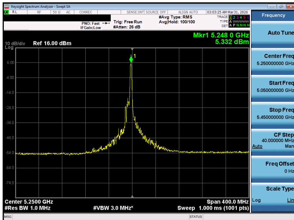
Plot 7-64. Power Spectral Density Plot MIMO ANT1 (160MHz BW 802.11be – 26 Tones (UNII Band 1/2A) – Ch. 50)
