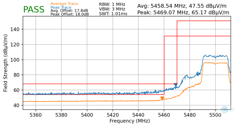
Plot 7-150. Radiated Lower Band Edge Plot MIMO (Average & Peak – UNII Band 2C – 242 Tones)
