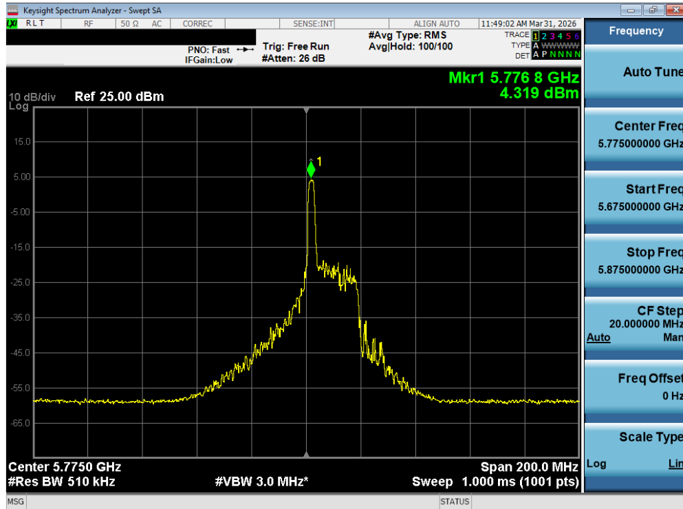
Plot 7-97. Power Spectral Density Plot MIMO ANT2 (80MHz BW 802.11be – 26 Tones (UNII Band 3) – Ch. 155)
