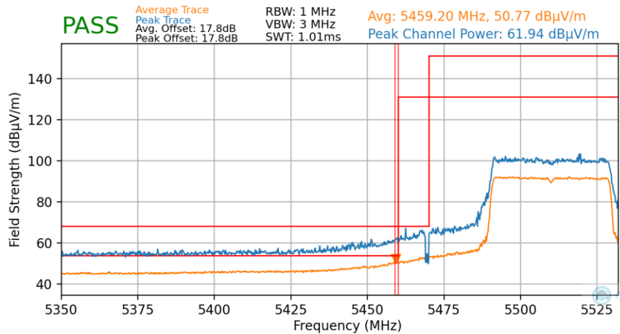
Plot 7-156. Radiated Lower Band Edge Plot MIMO (Average & Peak – UNII Band 2C – 484 Tones)
