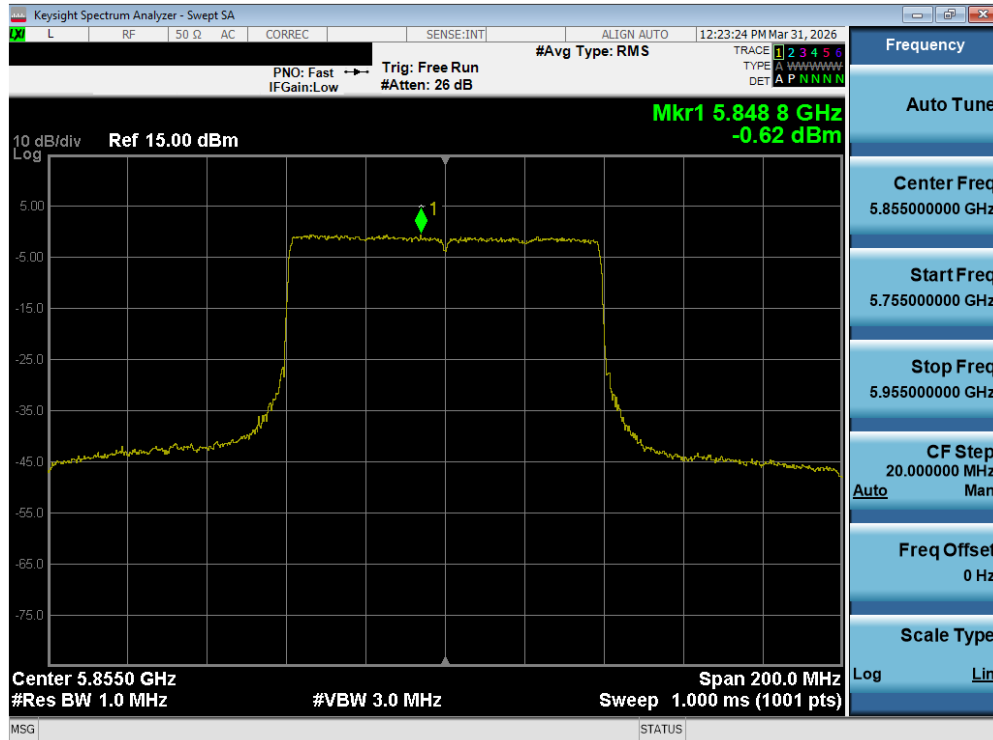
Plot 7-111. Power Spectral Density Plot MIMO ANT2 (80MHz BW 802.11be – 996 Tones (UNII Band 3/4) – Ch. 171)
