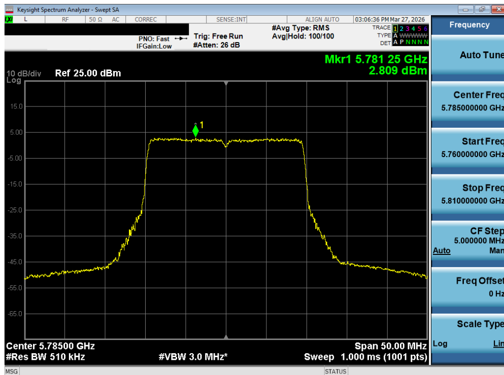
Plot 7-106. Power Spectral Density Plot MIMO ANT2 (20MHz BW 802.11be – 242 Tones (UNII Band 3) – Ch. 157)
