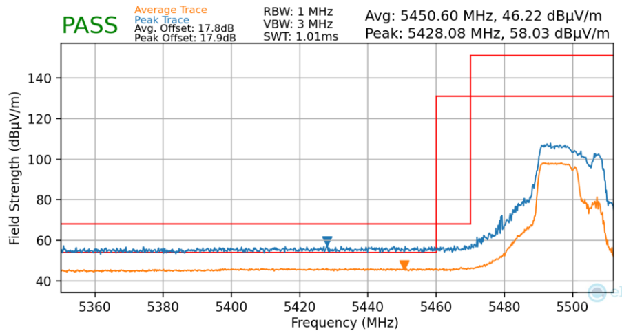
Plot 7-144. Radiated Lower Band Edge Plot MIMO (Average & Peak – UNII Band 2C – 106+26 Tones)
