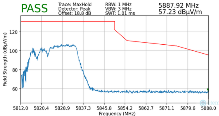
Plot 7-145. Radiated Upper Band Edge Plot MIMO (Peak – UNII Band 3 – 106+26 Tones)
