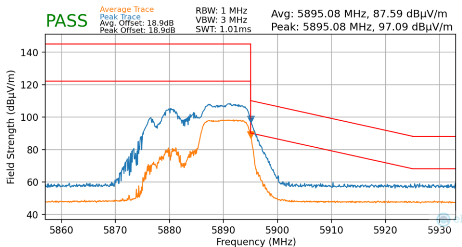
Plot 7-141. Radiated Upper Band Edge Plot MIMO (Average & Peak – UNII Band 4 – 106 Tones)
