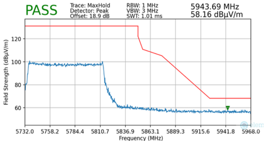
Plot 7-164. Radiated Upper Band Edge Plot MIMO (Peak – UNII Band 3 – 996 Tones)
