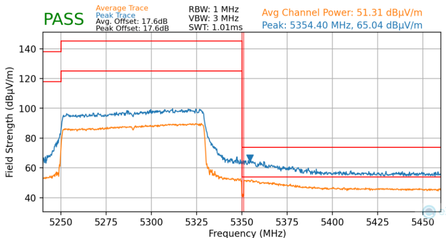
Plot 7-161. Radiated Upper Band Edge Plot MIMO (Average & Peak – UNII Band 2A – 996 Tones)
