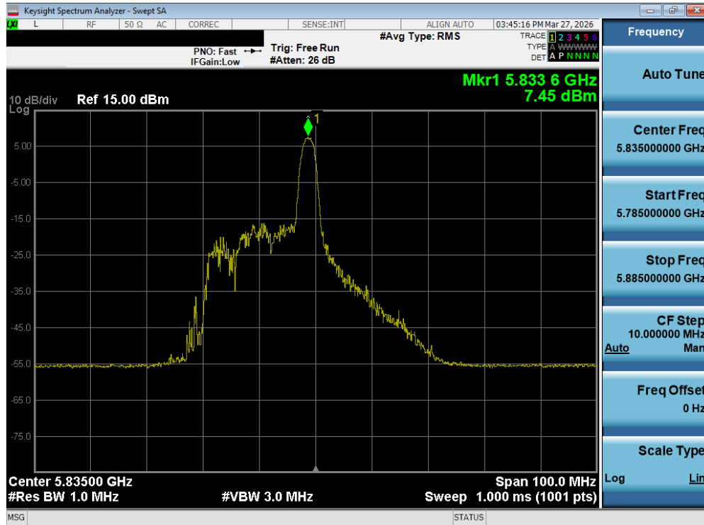
Plot 7-99. Power Spectral Density Plot MIMO ANT2 (40MHz BW 802.11be – 26 Tones (UNII Band 3/4) – Ch. 167)
