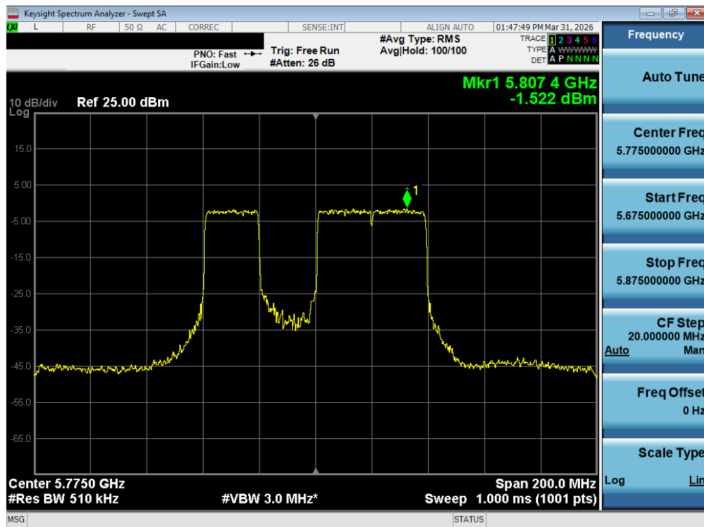
Plot 7-117. Power Spectral Density Plot MIMO ANT2 (80MHz BW 802.11be – 484+242 Tones (UNII Band 3) – Ch. 155)
