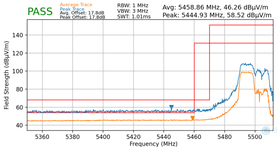
Plot 7-138. Radiated Lower Band Edge Plot MIMO (Average & Peak – UNII Band 2C – 106 Tones)
