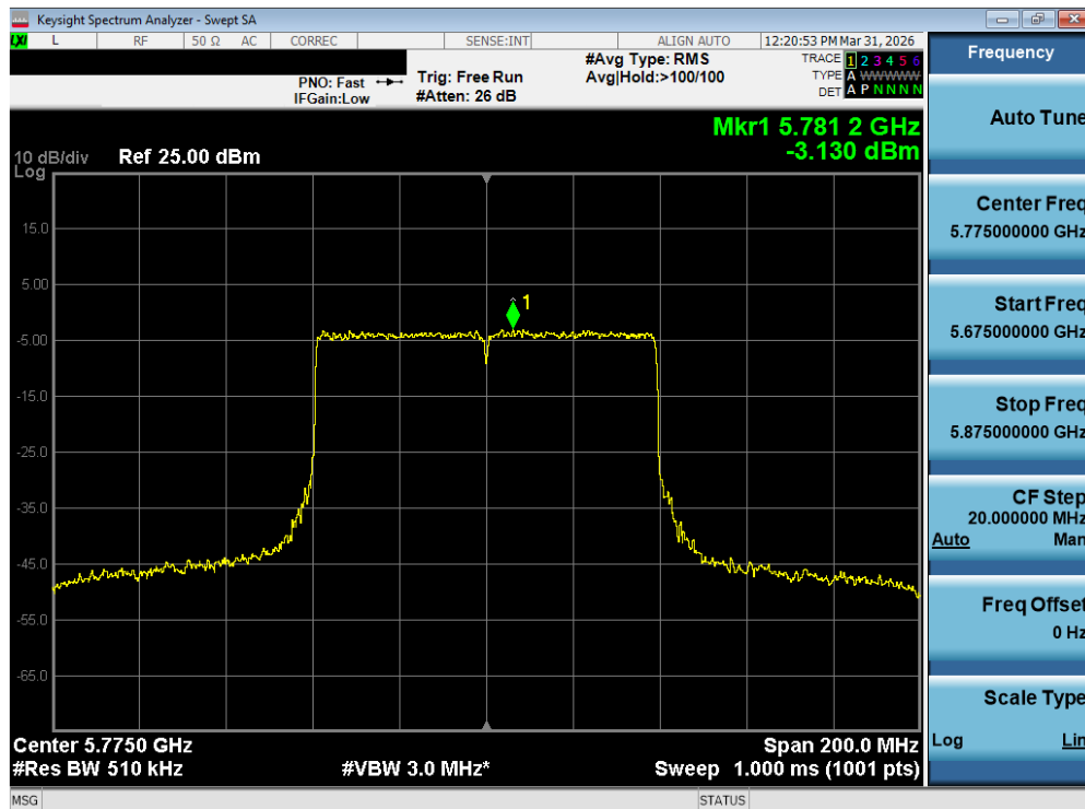
Plot 7-108. Power Spectral Density Plot MIMO ANT2 (80MHz BW 802.11be – 996 Tones (UNII Band 3) – Ch. 155)
