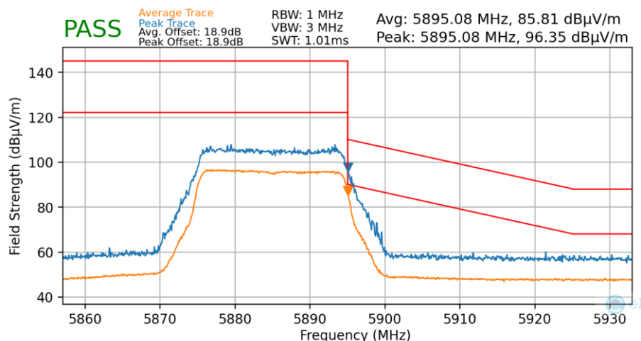
Plot 7-153. Radiated Upper Band Edge Plot MIMO (Average & Peak – UNII Band 4 – 242 Tones)
