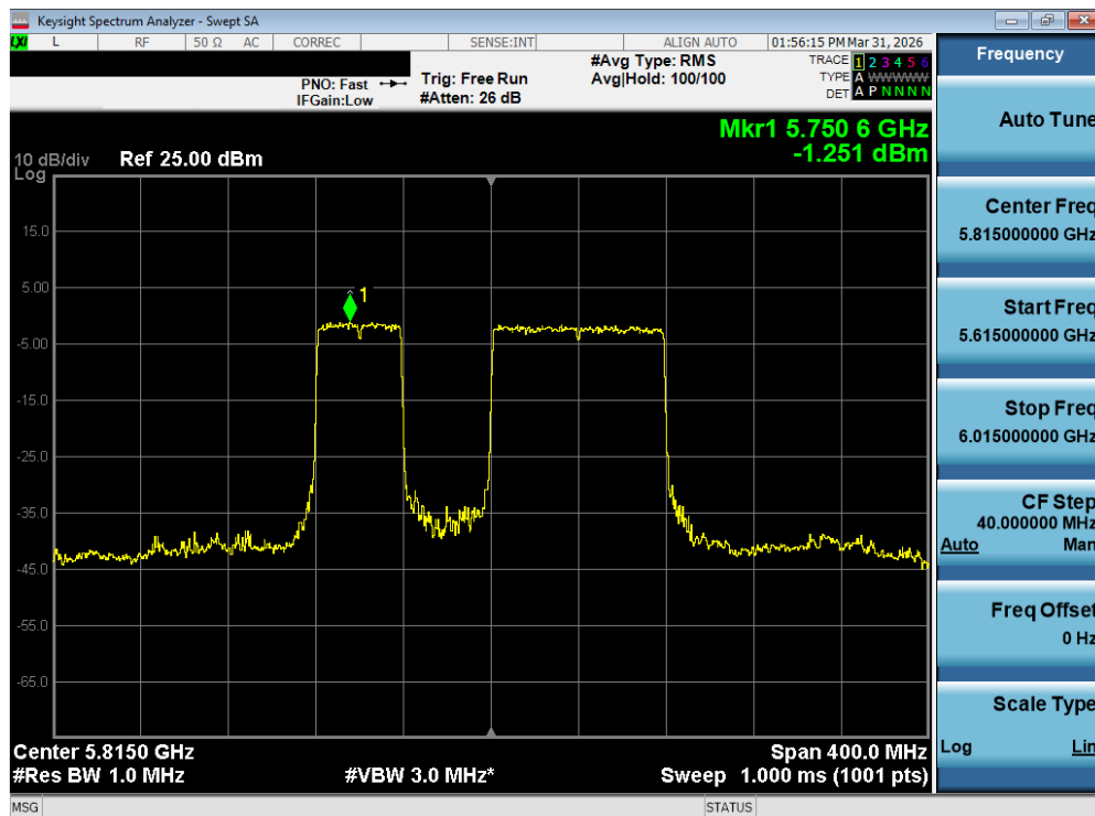
Plot 7-120. Power Spectral Density Plot MIMO ANT2 (160MHz BW 802.11be – 996+484 Tones (UNII Band 3/4) – Ch. 163)
