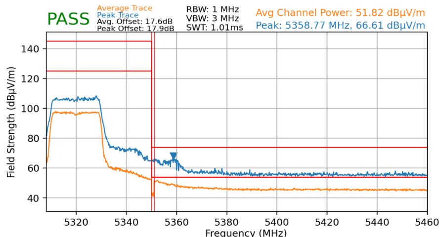
Plot 7-149. Radiated Upper Band Edge Plot MIMO (Average & Peak – UNII Band 2A – 242 Tones)
