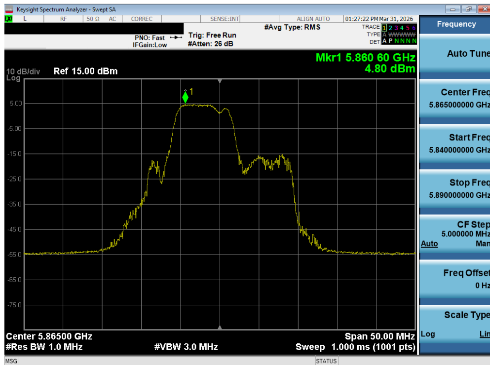
Plot 7-118. Power Spectral Density Plot MIMO ANT2 (20MHz BW 802.11be – 52+26 Tones (UNII Band 4) – Ch. 173)
