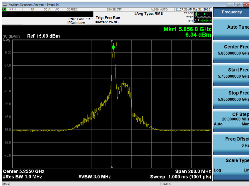
Plot 7-100. Power Spectral Density Plot MIMO ANT2 (80MHz BW 802.11be – 26 Tones (UNII Band 3/4) – Ch. 171)
