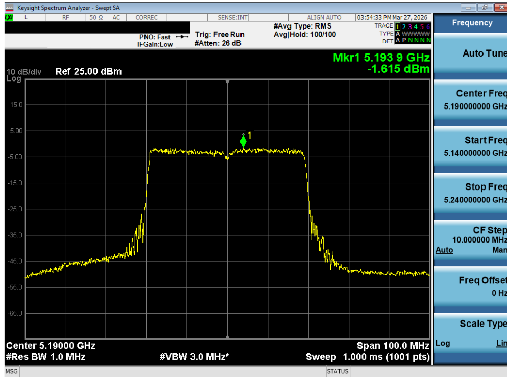
Plot 7-103. Power Spectral Density Plot MIMO ANT2 (40MHz BW 802.11be – 484 Tones (UNII Band 1) – Ch. 38)
