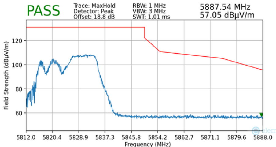
Plot 7-139. Radiated Upper Band Edge Plot MIMO (Peak – UNII Band 3 – 106 Tones)
