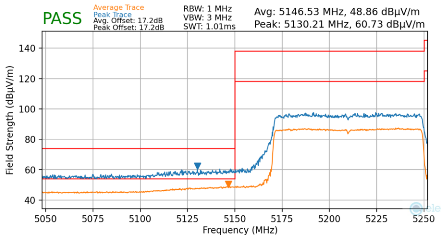
Plot 7-160. Radiated Lower Band Edge Plot MIMO (Average & Peak – UNII Band 1 – 996 Tones)
