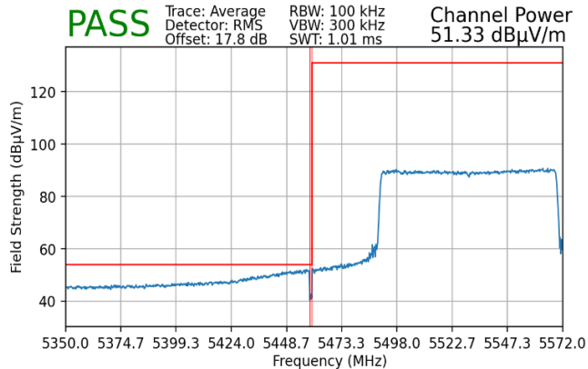
Plot 7-162. Radiated Lower Band Edge Plot MIMO (Average – UNII Band 2C – 996 Tones)
