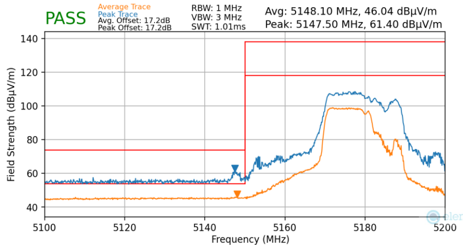
Plot 7-142. Radiated Lower Band Edge Plot MIMO (Average & Peak – UNII Band 1 – 106+26 Tones)
