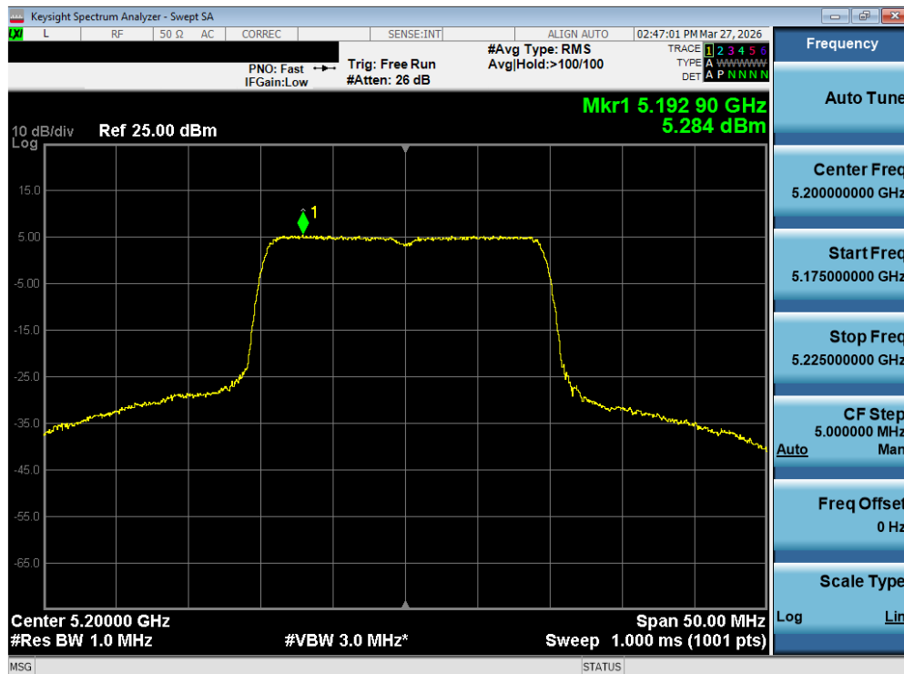
Plot 7-102. Power Spectral Density Plot MIMO ANT2 (20MHz BW 802.11be – 242 Tones (UNII Band 1) – Ch. 40)
