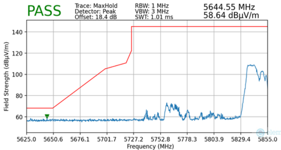
Plot 7-140. Radiated Lower Band Edge Plot MIMO (Peak – UNII Band 4 – 106 Tones)
