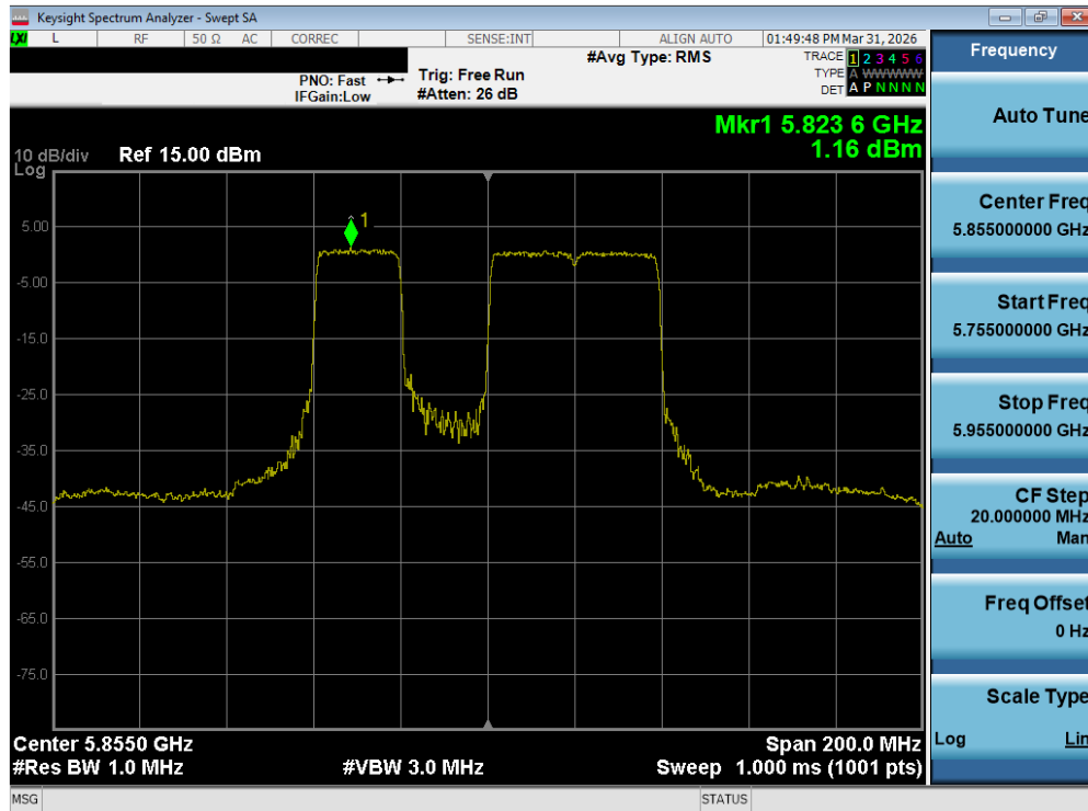
Plot 7-119. Power Spectral Density Plot MIMO ANT2 (80MHz BW 802.11be – 484+242 Tones (UNII Band 3/4) – Ch. 171)
