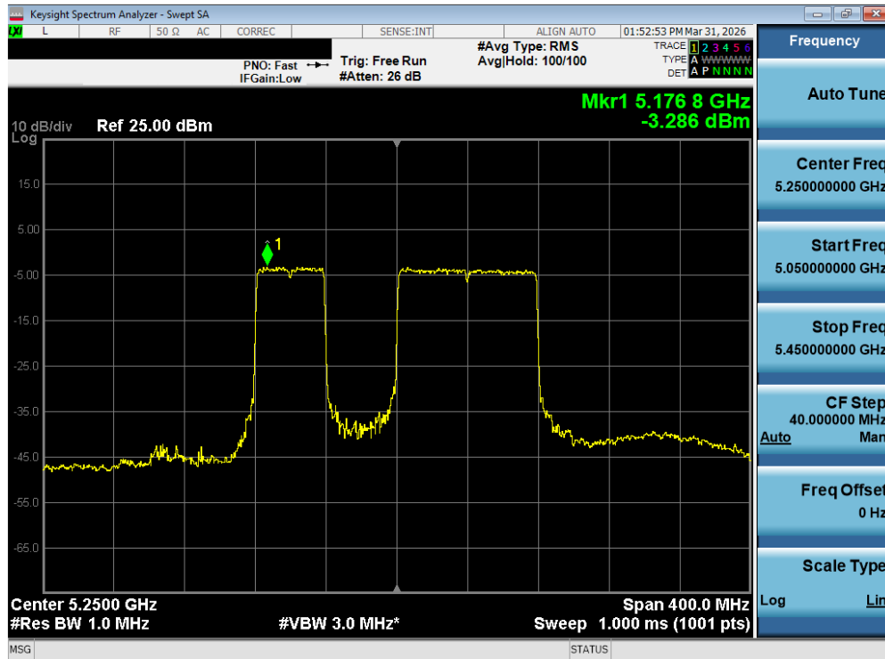
Plot 7-115. Power Spectral Density Plot MIMO ANT2 (160MHz BW 802.11be – 996+484 Tones (UNII Band 1/2A) – Ch. 50)
