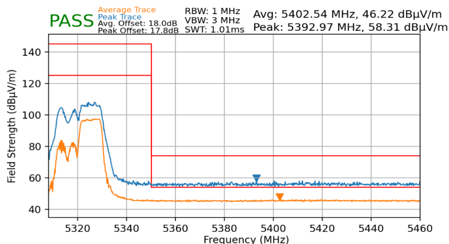
Plot 7-137. Radiated Upper Band Edge Plot MIMO (Average & Peak – UNII Band 2A – 106 Tones)
