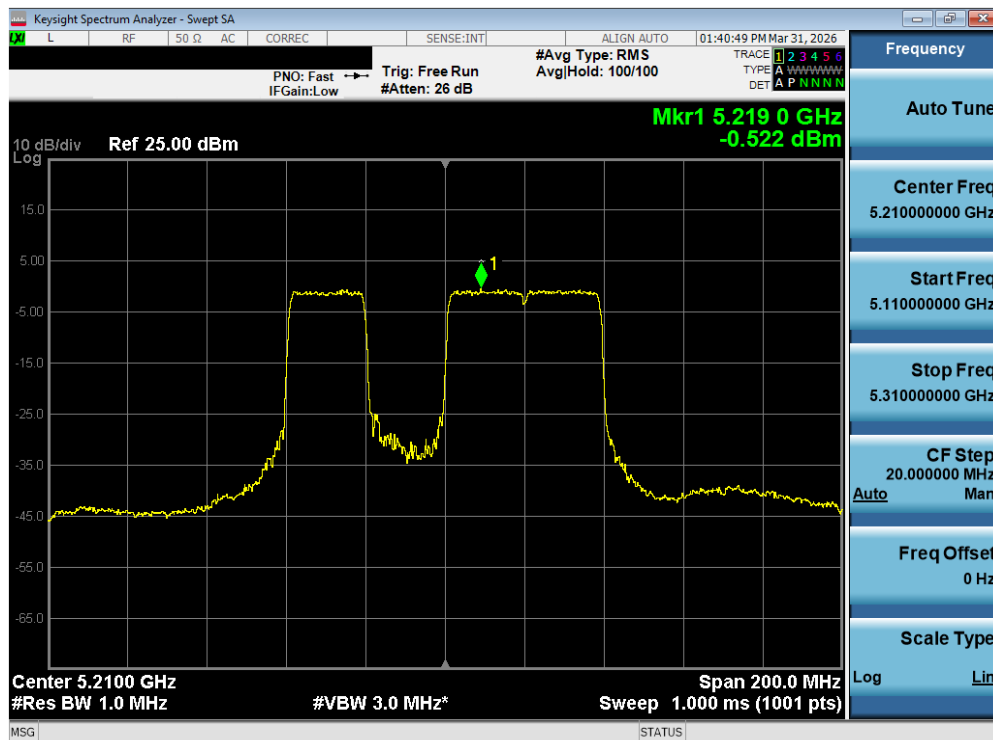
Plot 7-114. Power Spectral Density Plot MIMO ANT2 (80MHz BW 802.11be – 484+242 Tones (UNII Band 1) – Ch. 42)
