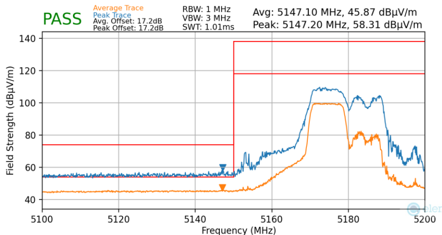
Plot 7-136. Radiated Lower Band Edge Plot MIMO (Average & Peak – UNII Band 1 – 106 Tones)
