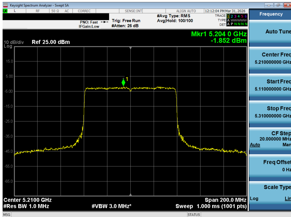
Plot 7-104. Power Spectral Density Plot MIMO ANT2 (80MHz BW 802.11be – 996 Tones (UNII Band 1) – Ch. 42)
