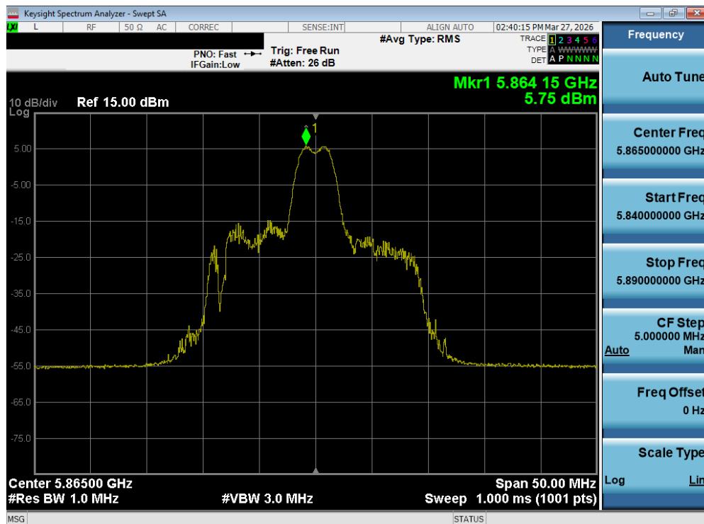
Plot 7-98. Power Spectral Density Plot MIMO ANT2 (20MHz BW 802.11be – 26 Tones (UNII Band 4) – Ch. 173)
