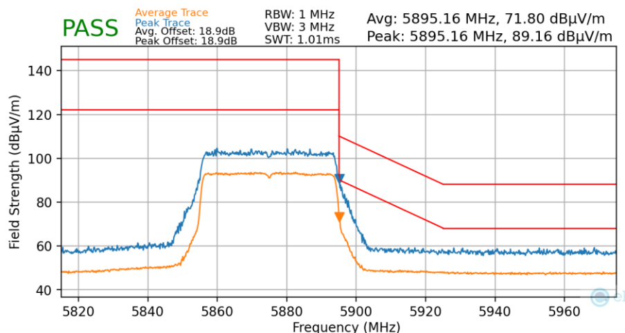
Plot 7-159. Radiated Upper Band Edge Plot MIMO (Average & Peak – UNII Band 4 – 484 Tones)
