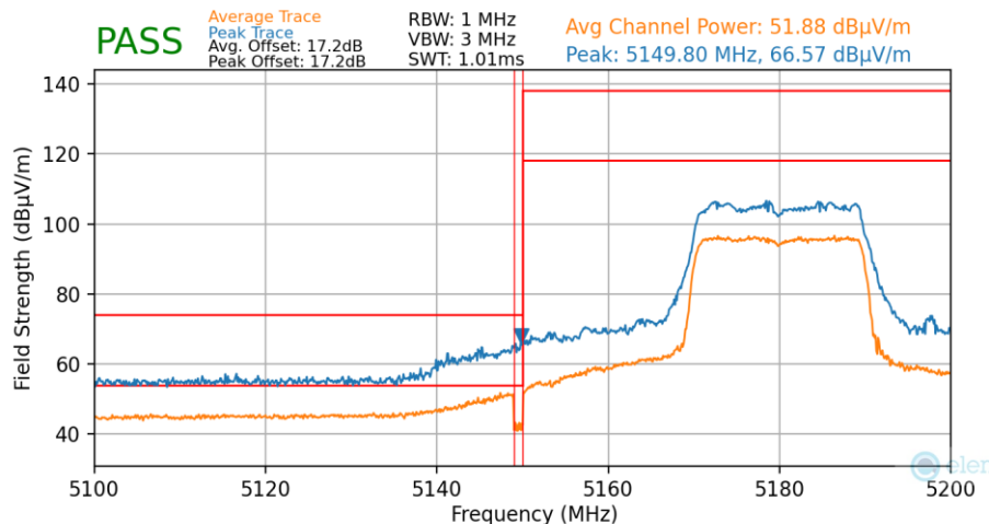
Plot 7-148. Radiated Lower Band Edge Plot MIMO (Average & Peak – UNII Band 1 – 242 Tones)
