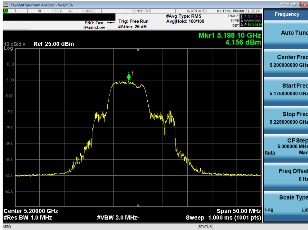
Plot 7-113. Power Spectral Density Plot MIMO ANT2 (20MHz BW 802.11be – 52+26 Tones (UNII Band 1) – Ch. 40)
