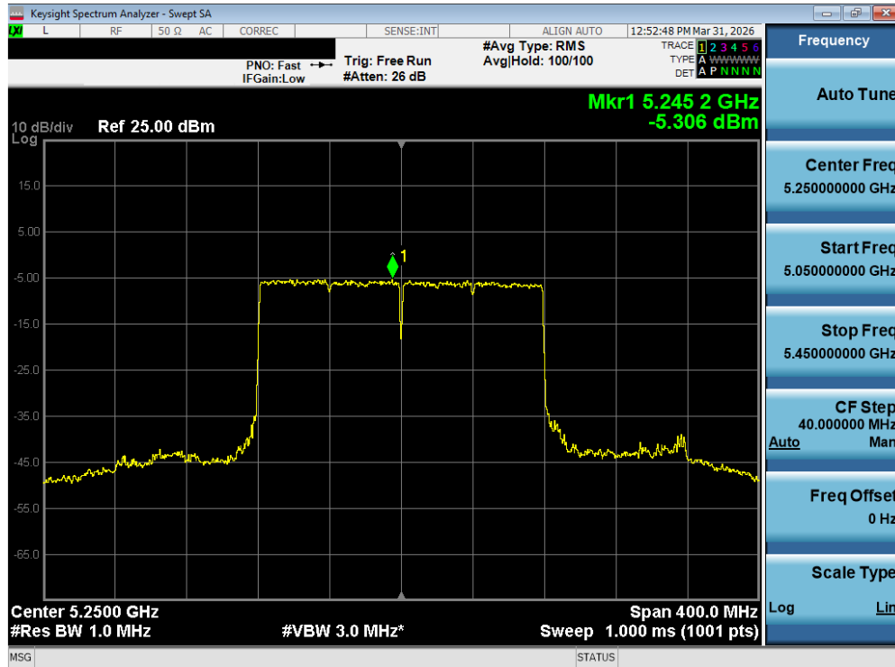
Plot 7-105. Power Spectral Density Plot MIMO ANT2 (160MHz BW 802.11be – 2x996 Tones (UNII Band 1/2A) – Ch. 50)
