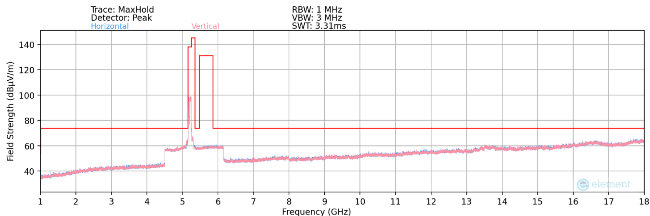
Plot 7-128. Radiated Spurious Plot above 1GHz MIMO (802.11be – MRU 484+242 Tones)
