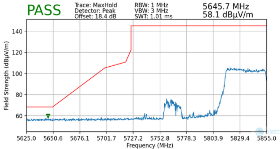
Plot 7-158. Radiated Lower Band Edge Plot MIMO (Peak – UNII Band 4 – 484 Tones)
