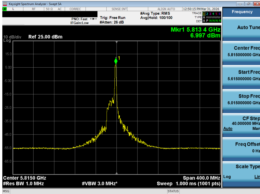
Plot 7-101. Power Spectral Density Plot MIMO ANT2 (160MHz BW 802.11be – 26 Tones (UNII Band 3/4) – Ch. 163)
