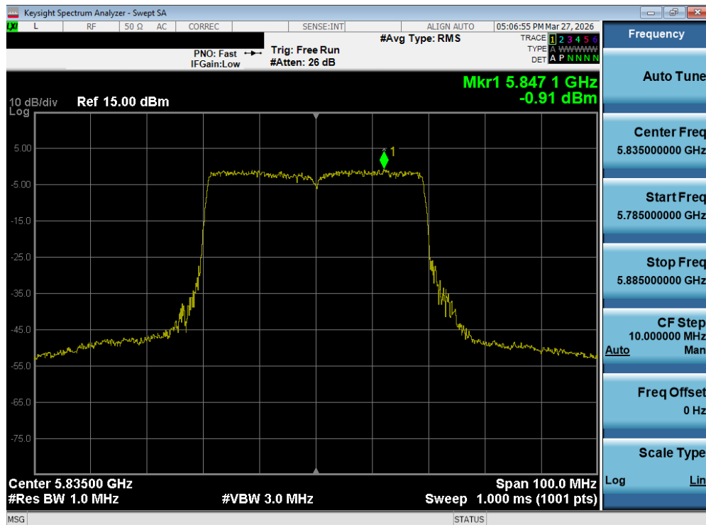
Plot 7-110. Power Spectral Density Plot MIMO ANT2 (40MHz BW 802.11be – 484 Tones (UNII Band 3/4) – Ch. 167)
