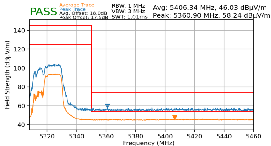
Plot 7-143. Radiated Upper Band Edge Plot MIMO (Average & Peak – UNII Band 2A – 106+26 Tones)
