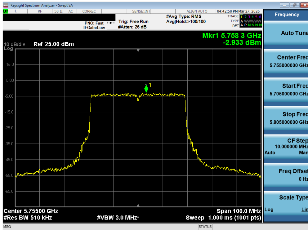
Plot 7-107. Power Spectral Density Plot MIMO ANT2 (40MHz BW 802.11be – 484 Tones (UNII Band 3) – Ch. 151)
