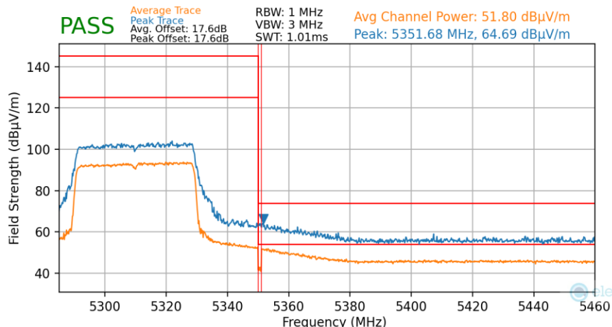
Plot 7-155. Radiated Upper Band Edge Plot MIMO (Average & Peak – UNII Band 2A – 484 Tones)
