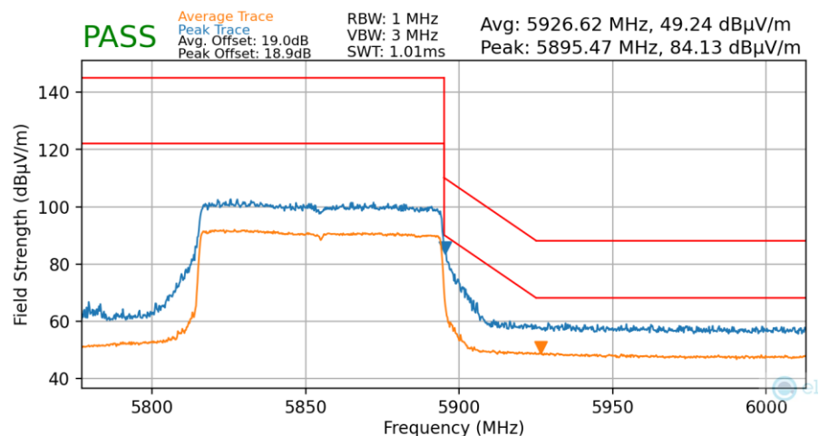
Plot 7-166. Radiated Upper Band Edge Plot MIMO (Average & Peak – UNII Band 4 – 996 Tones)
