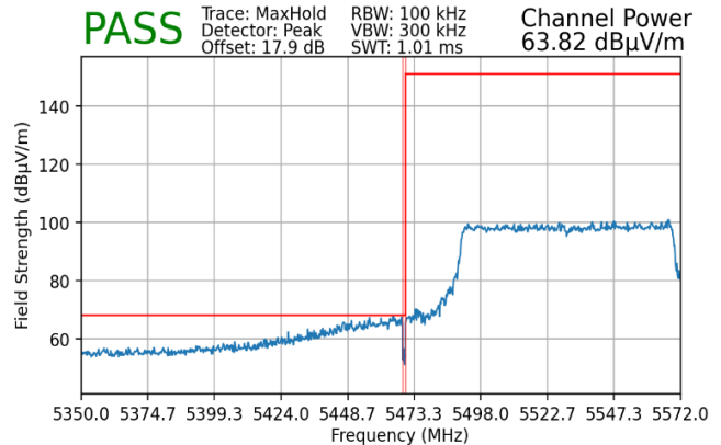
Plot 7-163. Radiated Lower Band Edge Plot MIMO (Peak – UNII Band 2C – 996 Tones)
