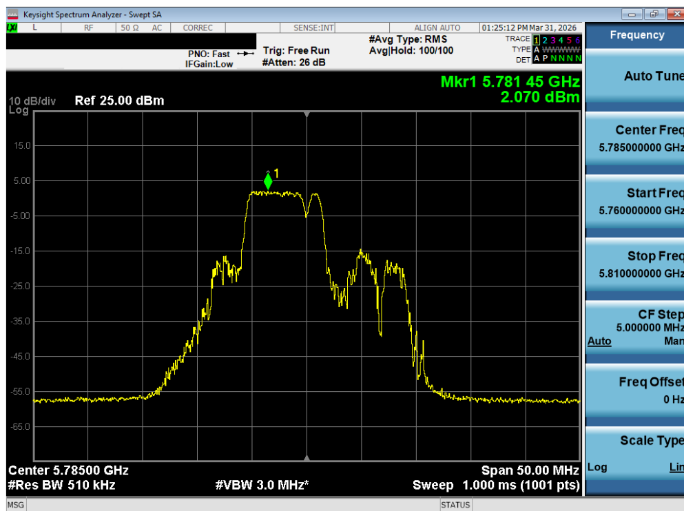
Plot 7-116. Power Spectral Density Plot MIMO ANT2 (20MHz BW 802.11be – 52+26 Tones (UNII Band 3) – Ch. 157)
