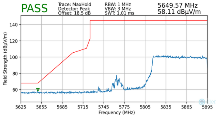
Plot 7-165. Radiated Lower Band Edge Plot MIMO (Peak – UNII Band 4 – 996 Tones)
