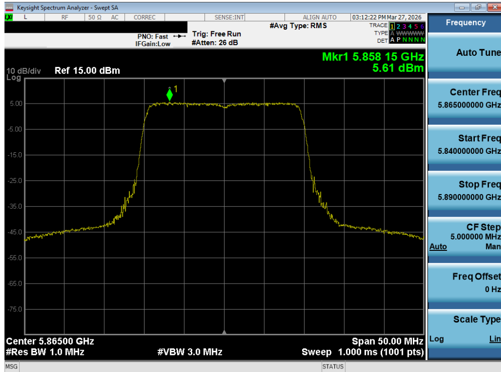
Plot 7-109. Power Spectral Density Plot MIMO ANT2 (20MHz BW 802.11be – 242 Tones (UNII Band 4) – Ch. 173)
