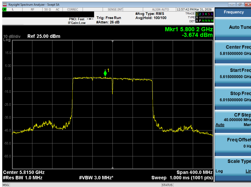
Plot 7-112. Power Spectral Density Plot MIMO ANT2 (160MHz BW 802.11be – 996*2 Tones (UNII Band 3/4) – Ch. 163)
