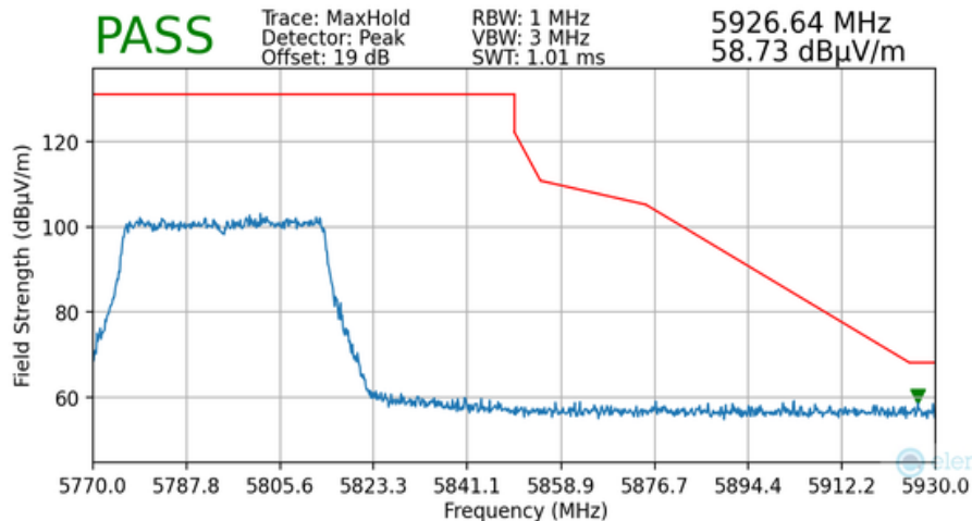
Plot 7-157. Radiated Upper Band Edge Plot MIMO (Peak – UNII Band 3 – 484 Tones)
