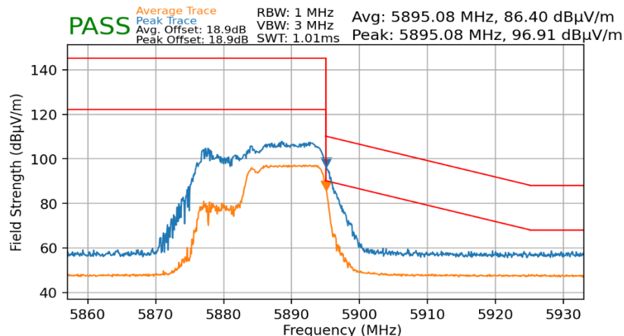
Plot 7-147. Radiated Upper Band Edge Plot MIMO (Average & Peak – UNII Band 4 – 106+26 Tones)
