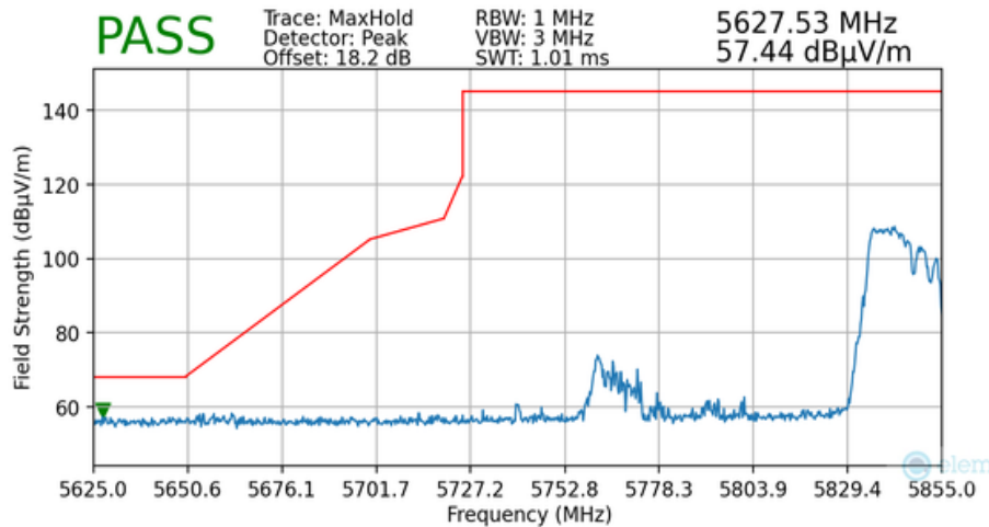
Plot 7-146. Radiated Lower Band Edge Plot MIMO (Peak – UNII Band 4 – 106+26 Tones)
