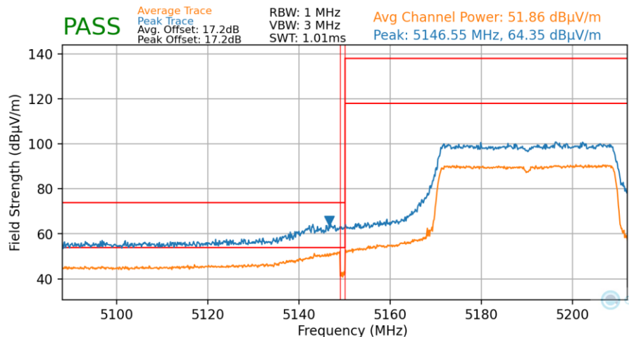
Plot 7-154. Radiated Lower Band Edge Plot MIMO (Average & Peak – UNII Band 1 – 484 Tones)
