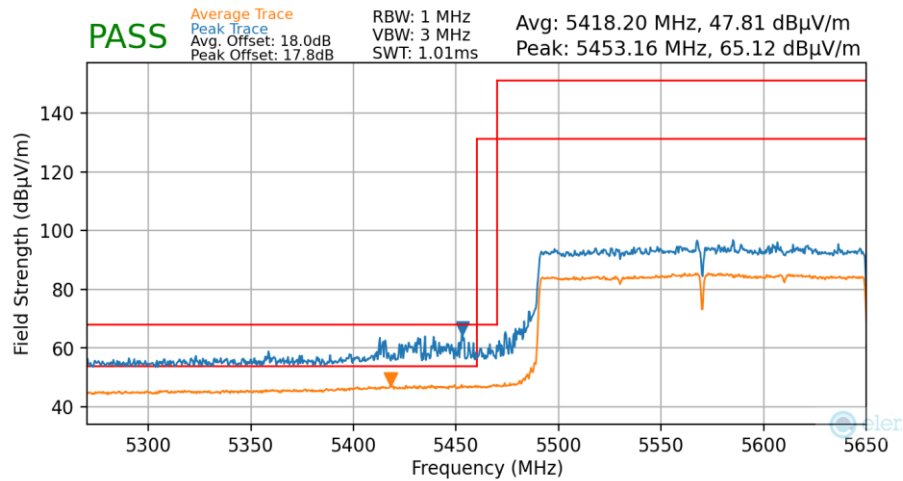
Plot 7-175. Radiated Lower Band Edge Plot MIMO (Average & Peak – UNII Band 2C – 2x996T)
