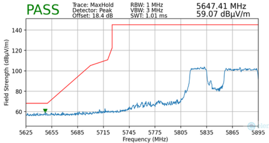
Plot 7-171. Radiated Lower Band Edge Plot MIMO (Peak – UNII Band 4 – 484+242 Tones)
