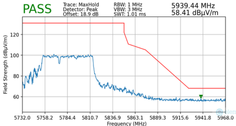
Plot 7-170. Radiated Upper Band Edge Plot MIMO (Peak – UNII Band 3 – 484+242 Tones)
