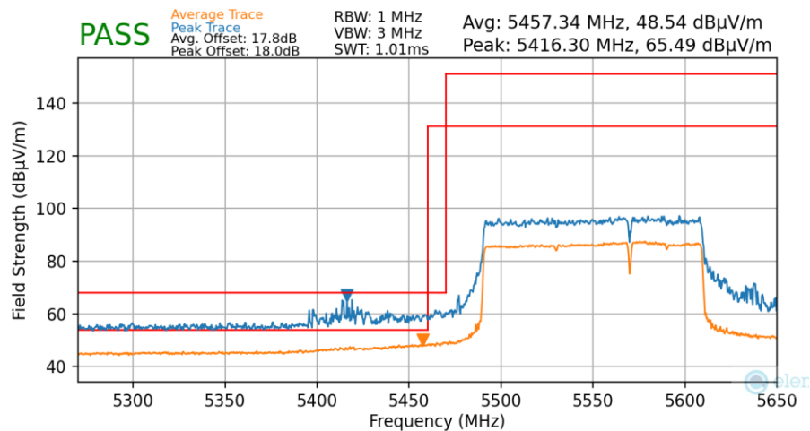
Plot 7-180. Radiated Lower Band Edge Plot MIMO (Average & Peak – UNII Band 2C – 996+484T)
