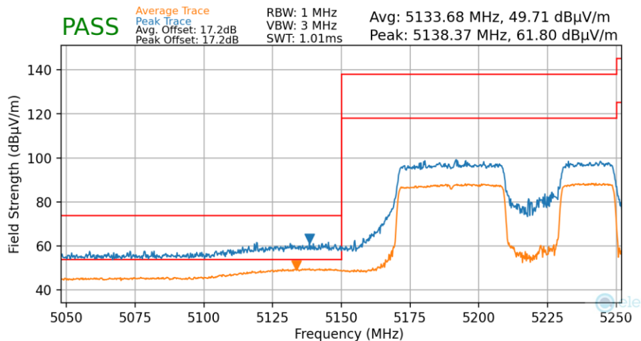
Plot 7-167. Radiated Lower Band Edge Plot MIMO (Average & Peak – UNII Band 1 – 484+242 Tones)
