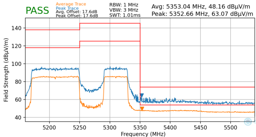
Plot 7-179. Radiated Upper Band Edge Plot MIMO (Average & Peak – UNII Band 2A – 996+484T)
