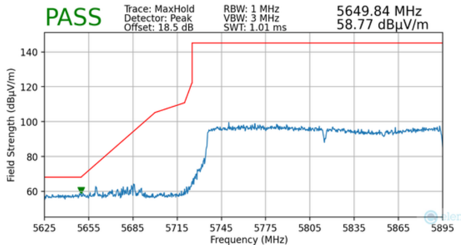
Plot 7-176. Radiated Lower Band Edge Plot MIMO (Peak – UNII Band 4 – 2x996T)
