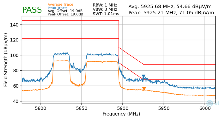
Plot 7-172. Radiated Upper Band Edge Plot MIMO (Average & Peak – UNII Band 4 – 484+242 Tones)
