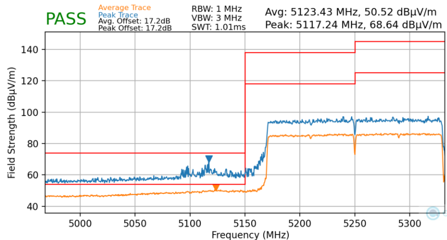
Plot 7-173. Radiated Lower Band Edge Plot MIMO (Average & Peak – UNII Band 1 – 2x996T)
