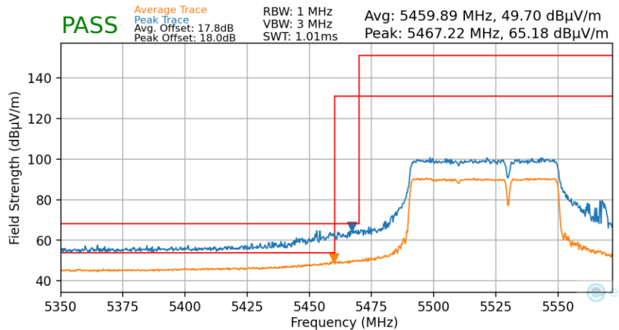
Plot 7-169. Radiated Lower Band Edge Plot MIMO (Average & Peak – UNII Band 2C – 484+242 Tones)
