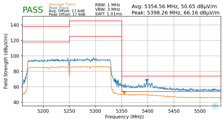
Plot 7-174. Radiated Upper Band Edge Plot MIMO (Average & Peak – UNII Band 2A – 2x996T)
