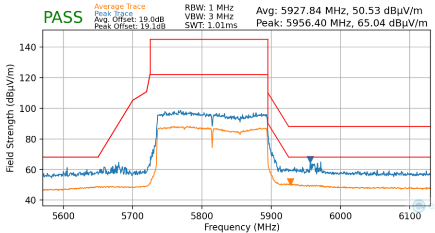
Plot 7-177. Radiated Upper Band Edge Plot MIMO (Average & Peak – UNII Band 4 – 2x996T)
