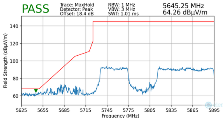
Plot 7-181. Radiated Lower Band Edge Plot MIMO (Peak – UNII Band 4 – 996+484T)
