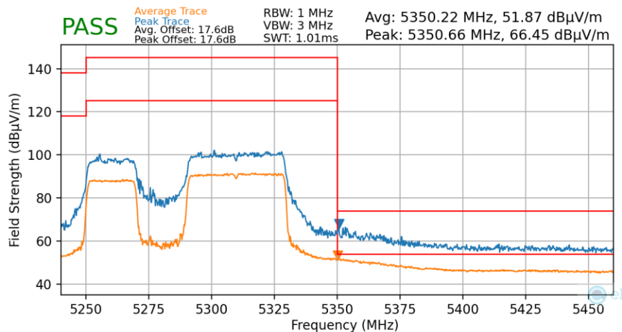
Plot 7-168. Radiated Upper Band Edge Plot MIMO (Average & Peak – UNII Band 2A – 484+242 Tones)
