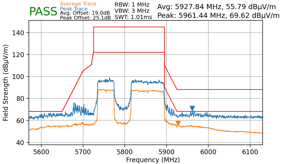
Plot 7-182. Radiated Upper Band Edge Plot MIMO (Average & Peak – UNII Band 4 – 996+484T)
