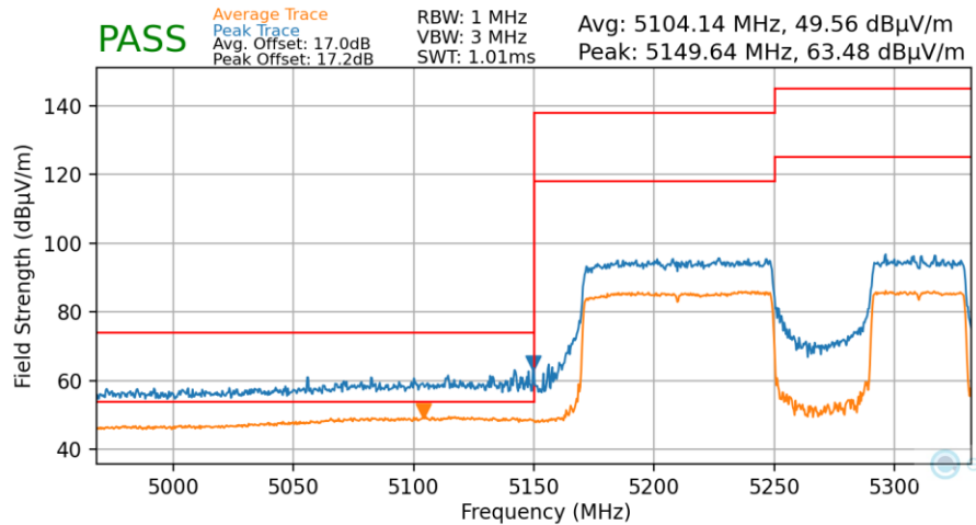
Plot 7-178. Radiated Lower Band Edge Plot MIMO (Average & Peak – UNII Band 1 – 996+484T)
