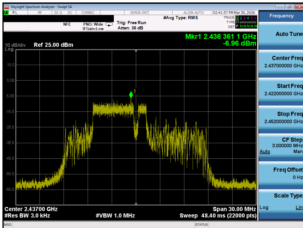
Plot 7-26. Power Spectral Density Plot MIMO ANT2 (802.11be OFDMA – 52+26 Tones – Ch. 6)
