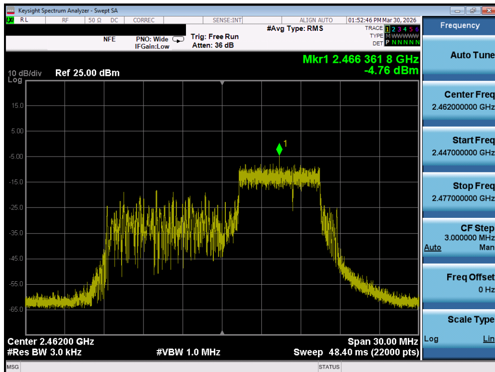
Plot 7-18. Power Spectral Density Plot MIMO ANT1 (802.11be OFDMA – 52+26 Tones – Ch. 11)
