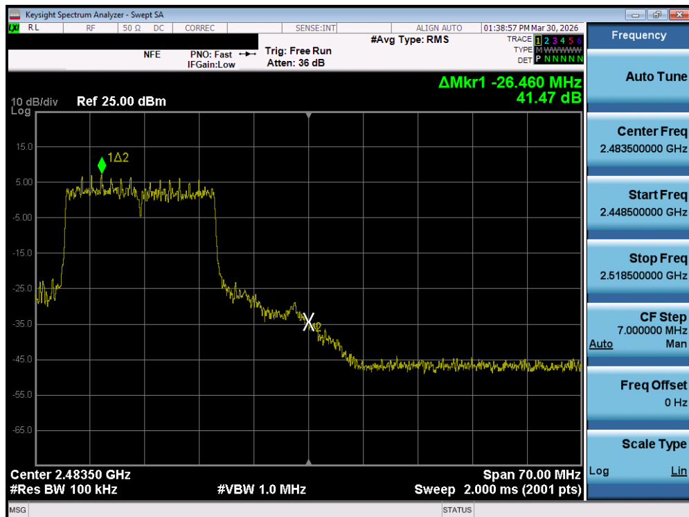
Plot 7-38. Band Edge Plot MIMO ANT1 (802.11ax/be OFDMA – 242 Tones – Ch. 11)
