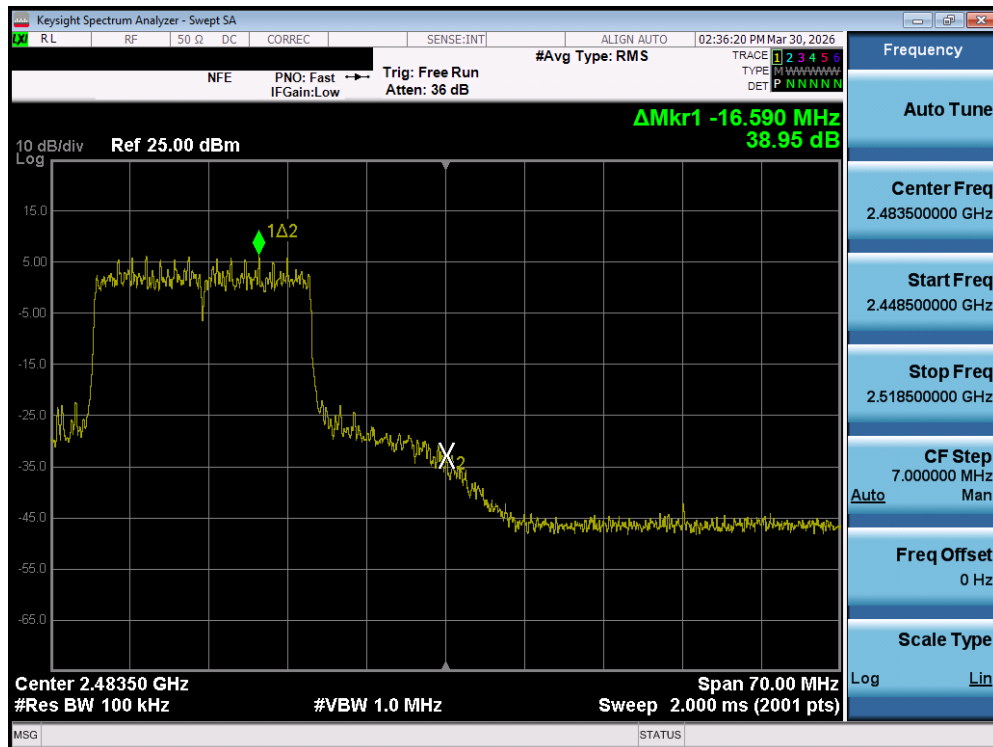
Plot 7-47. Band Edge Plot MIMO ANT2 (802.11ax/be OFDMA – 242 Tones – Ch. 11)
