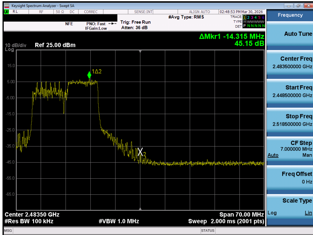
Plot 7-41. Band Edge Plot MIMO ANT2 (802.11ax/be OFDMA – 106 Tones – Ch. 11)
