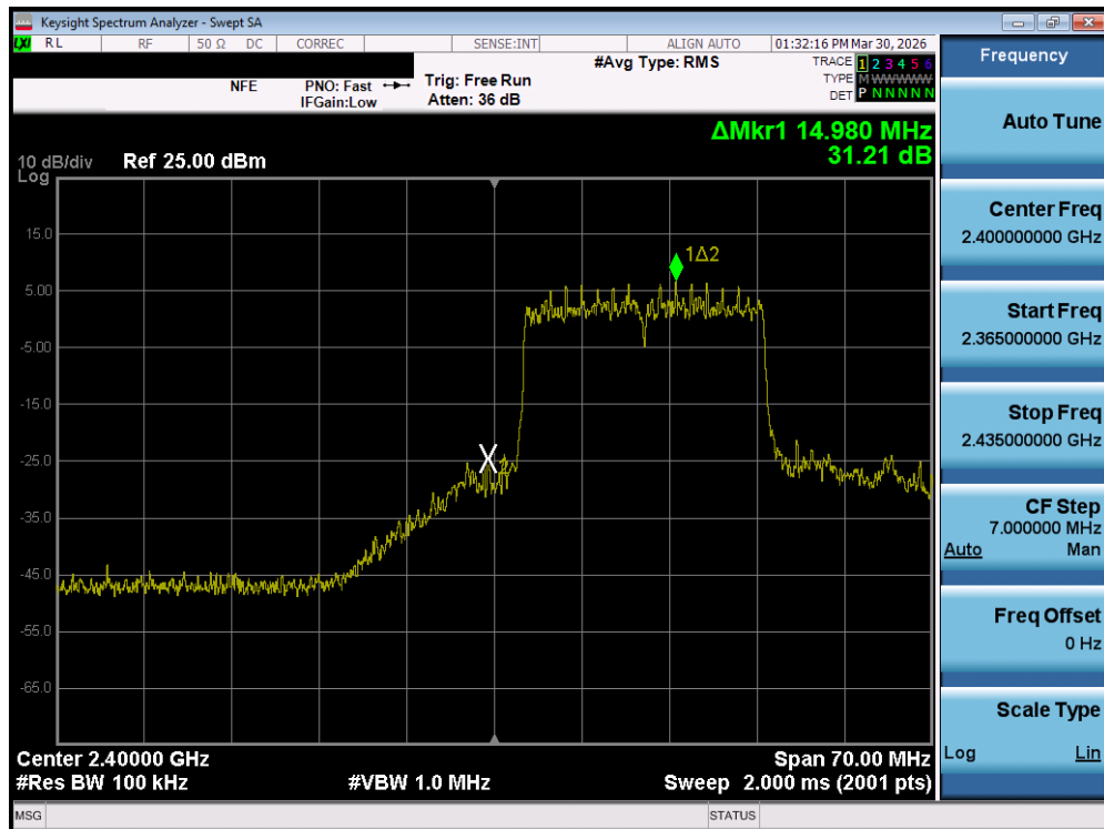
Plot 7-37. Band Edge Plot MIMO ANT1 (802.11ax/be OFDMA – 242 Tones – Ch. 1)
