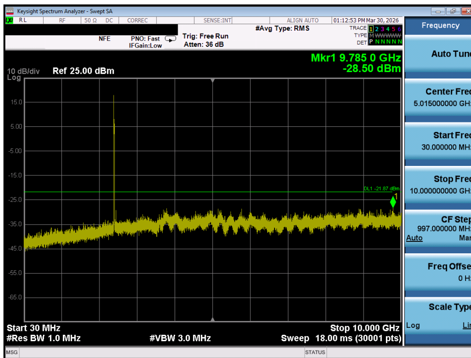
Plot 7-49. Conducted Spurious Plot MIMO ANT1 (802.11ax/be OFDMA – 26 Tones – Ch. 1)
