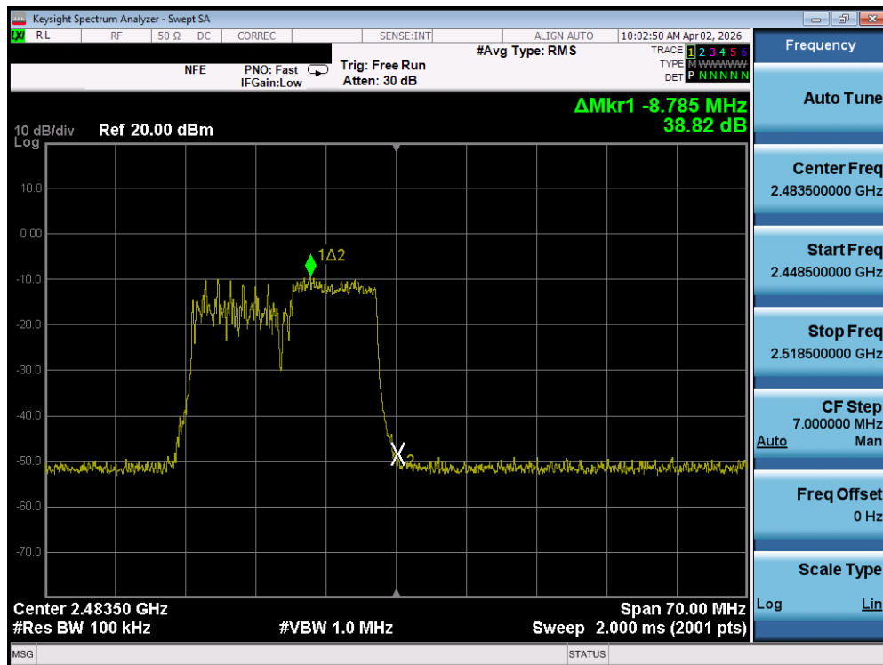
Plot 7-33. Band Edge Plot MIMO ANT1 (802.11ax/be OFDMA – 106 Tones – Ch. 13)
