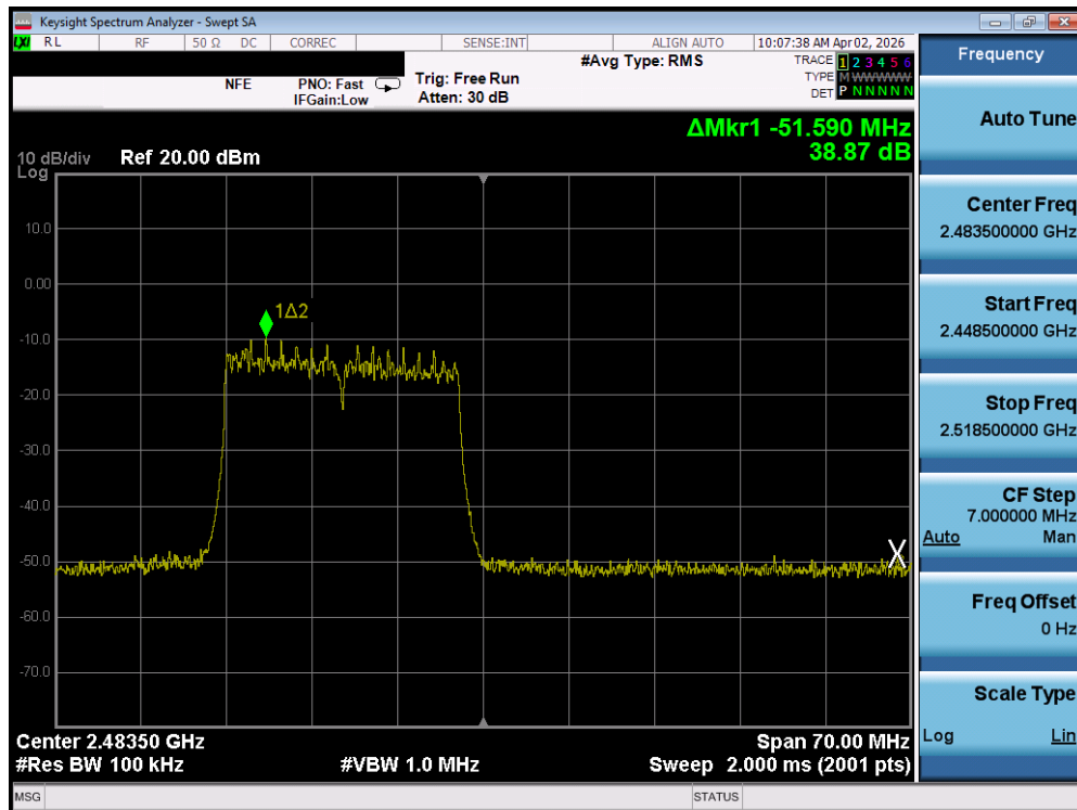
Plot 7-39. Band Edge Plot MIMO ANT1 (802.11ax/be OFDMA – 242 Tones – Ch. 13)
