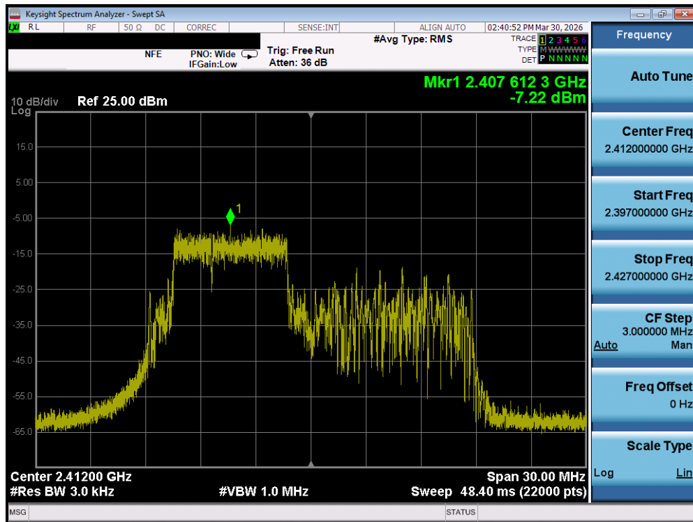
Plot 7-25. Power Spectral Density Plot MIMO ANT2 (802.11be OFDMA – 52+26 Tones – Ch. 1)
