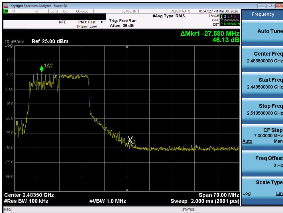
Plot 7-35. Band Edge Plot MIMO ANT1 (802.11be OFDMA – 106+26 Tones – Ch. 11)
