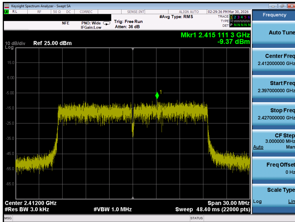
Plot 7-28. Power Spectral Density Plot MIMO ANT2 (802.11ax/be OFDMA – 242 Tones – Ch. 1)
