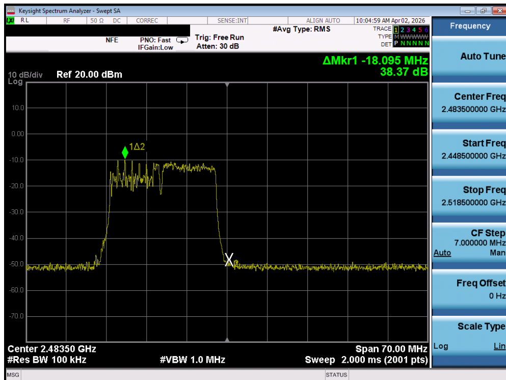
Plot 7-36. Band Edge Plot MIMO ANT1 (802.11be OFDMA – 106+26 Tones – Ch. 13)
