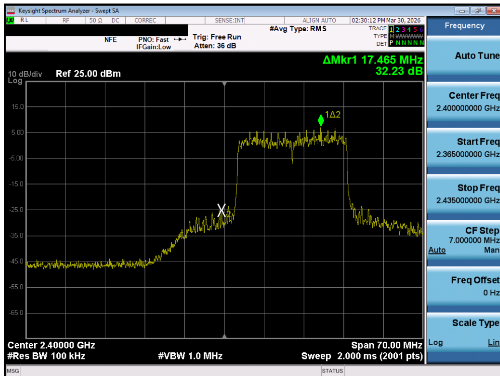
Plot 7-46. Band Edge Plot MIMO ANT2 (802.11ax/be OFDMA – 242 Tones – Ch. 1)
