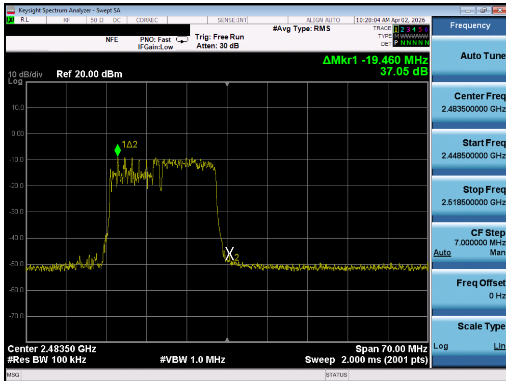
Plot 7-45. Band Edge Plot MIMO ANT2 (802.11be OFDMA – 106+26 Tones – Ch. 13)
