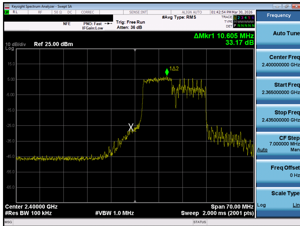
Plot 7-31. Band Edge Plot MIMO ANT1 (802.11ax/be OFDMA – 106 Tones – Ch. 1)
