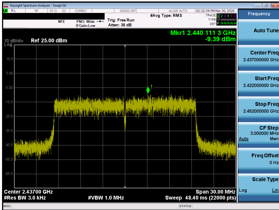
Plot 7-29. Power Spectral Density Plot MIMO ANT2 (802.11ax/be OFDMA – 242 Tones – Ch. 6)
