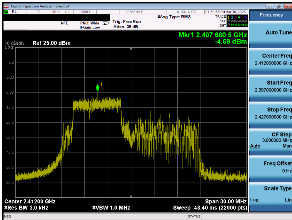
Plot 7-16. Power Spectral Density Plot MIMO ANT1 (802.11be OFDMA – 52+26 Tones – Ch. 1)
