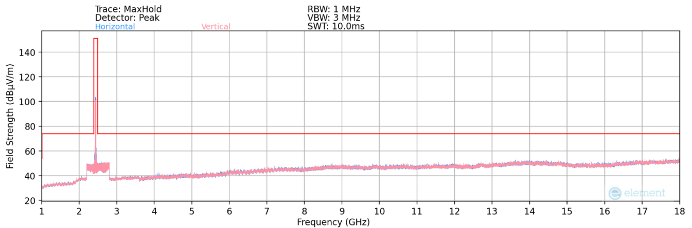
Plot 7-77. Radiated Spurious Plot above 1GHz MIMO (802.11be OFDMA – 106 + 26 Tones – Ch. 6)
