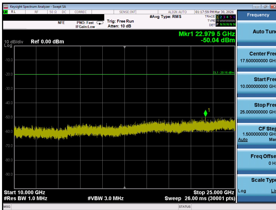
Plot 7-52. Conducted Spurious Plot MIMO ANT1 (802.11ax/be OFDMA – 26 Tones – Ch. 6)
