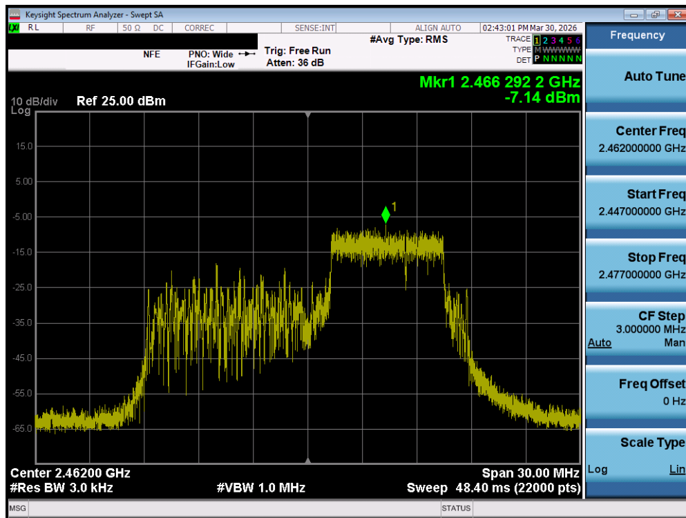
Plot 7-27. Power Spectral Density Plot MIMO ANT2 (802.11be OFDMA – 52+26 Tones – Ch. 11)
