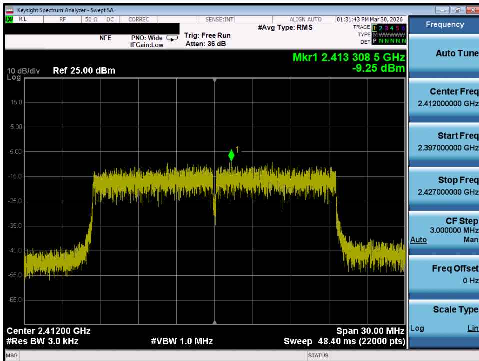
Plot 7-19. Power Spectral Density Plot MIMO ANT1 (802.11ax/be OFDMA – 242 Tones – Ch. 1)
