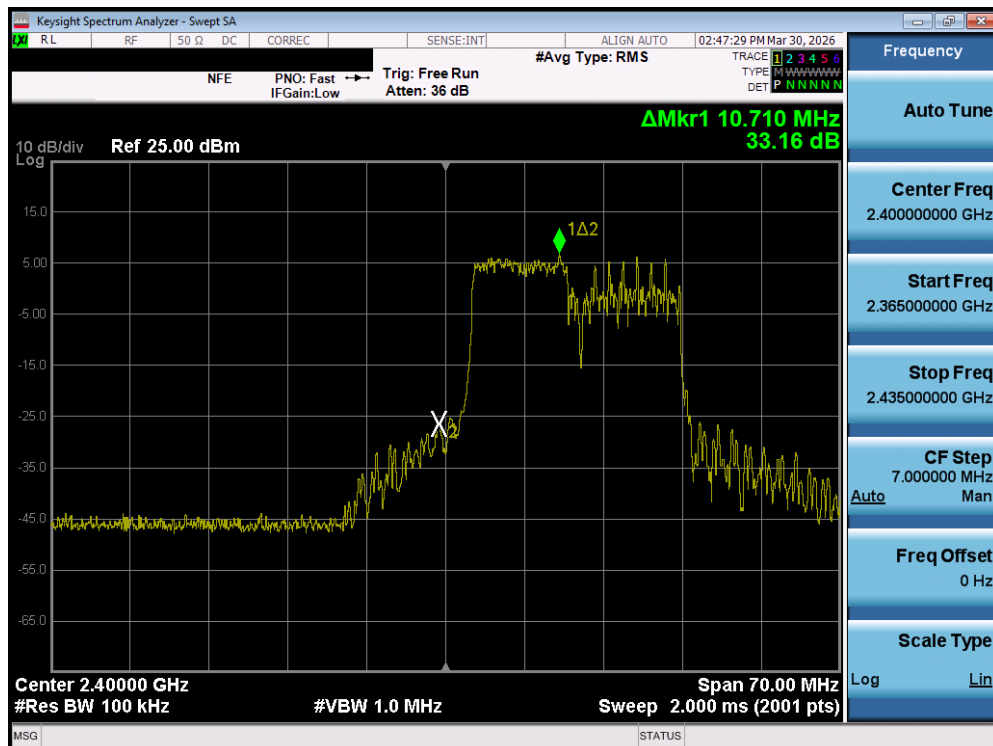
Plot 7-40. Band Edge Plot MIMO ANT2 (802.11ax/be OFDMA – 106 Tones – Ch. 1)
