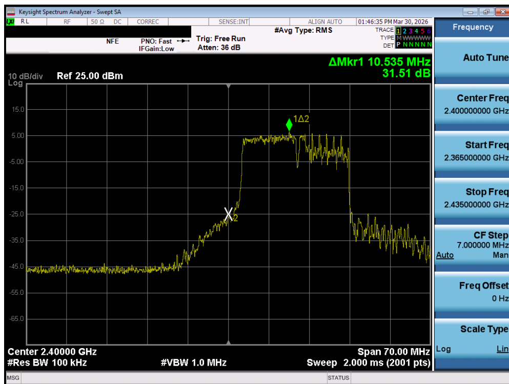
Plot 7-34. Band Edge Plot MIMO ANT1 (802.11be OFDMA – 106+26 Tones – Ch. 1)
