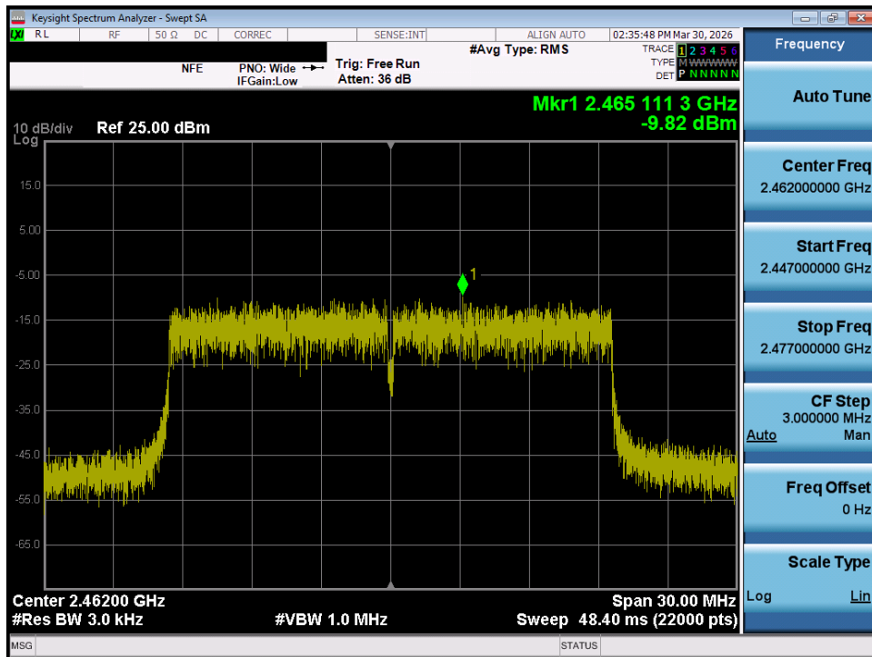
Plot 7-30. Power Spectral Density Plot MIMO ANT2 (802.11ax/be OFDMA – 242 Tones – Ch. 11)
