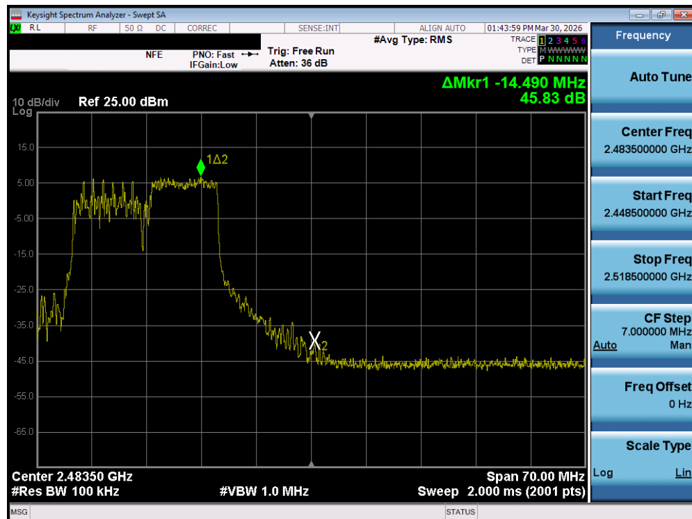
Plot 7-32. Band Edge Plot MIMO ANT1 (802.11ax/be OFDMA – 106 Tones – Ch. 11)
