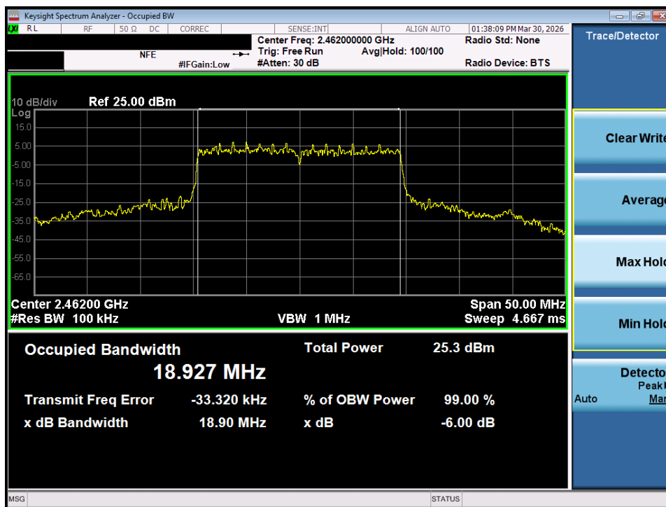
Plot 7-6. 6dB Bandwidth Plot MIMO ANT1 (802.11ax/be OFDMA – 242 Tones – Ch. 11)
