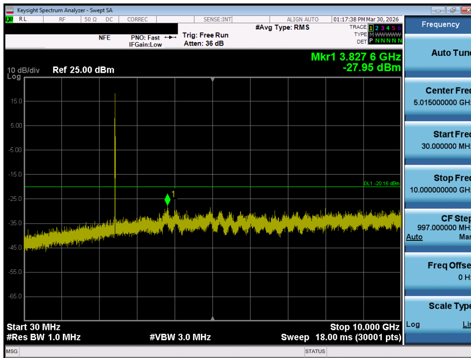
Plot 7-51. Conducted Spurious Plot MIMO ANT1 (802.11ax/be OFDMA – 26 Tones – Ch. 6)
