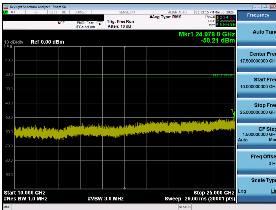
Plot 7-50. Conducted Spurious Plot MIMO ANT1 (802.11ax/be OFDMA – 26 Tones – Ch. 1)
