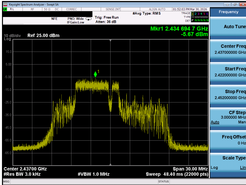
Plot 7-17. Power Spectral Density Plot MIMO ANT1 (802.11be OFDMA – 52+26 Tones – Ch. 6)
