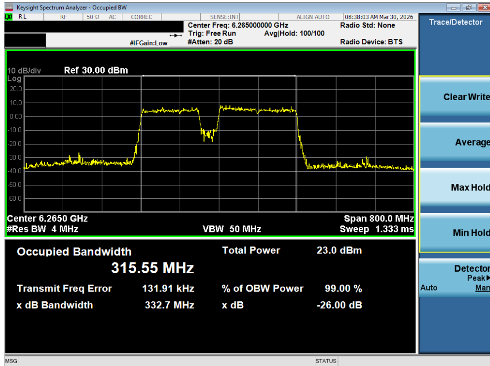
Plot 7-9. 26dB Bandwidth Plot MIMO ANT1 (320MHz 802.11be (UNII Band 5) – Ch. 63) – 40MHz Punctured – LPI/SP
