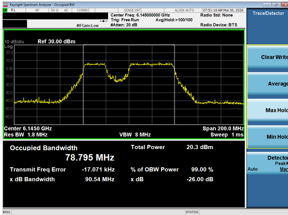
Plot 7-7. 26dB Bandwidth Plot MIMO ANT1 (80MHz 802.11be (UNII Band 5) – Ch. 39) – 20MHz Punctured - LPI
