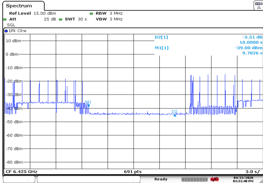
Plot 7-86. Contention Based Protocol Timing Plot (320MHz (UNII Band 6) – Ch. 95 Mid)
