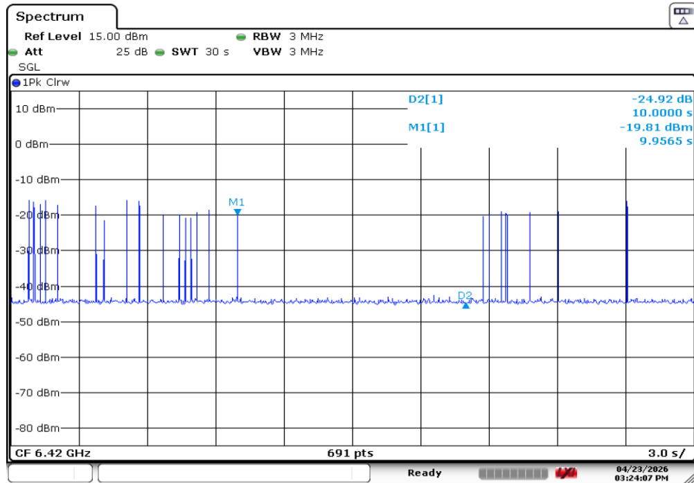
Plot 7-82. Contention Based Protocol Timing Plot (320MHz (UNII Band 5) – Ch. 63 Mid)
