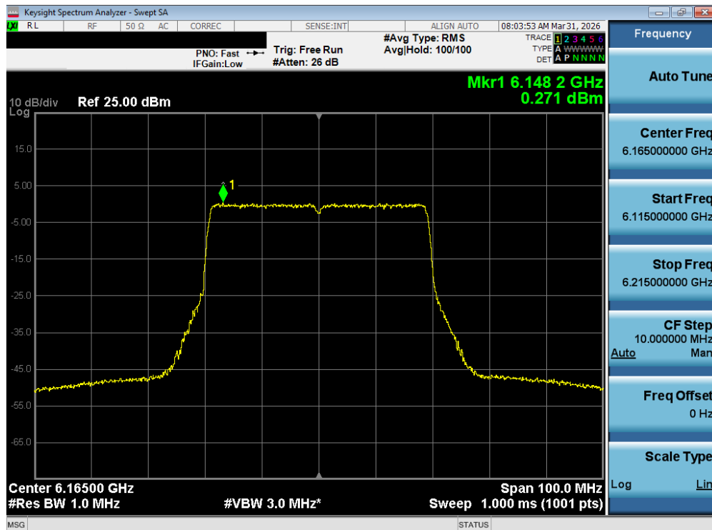
Plot 7-38. Power Spectral Density Plot MIMO ANT1 (40MHz 802.11ax/be (UNII Band 5) – Ch. 43) – SP
