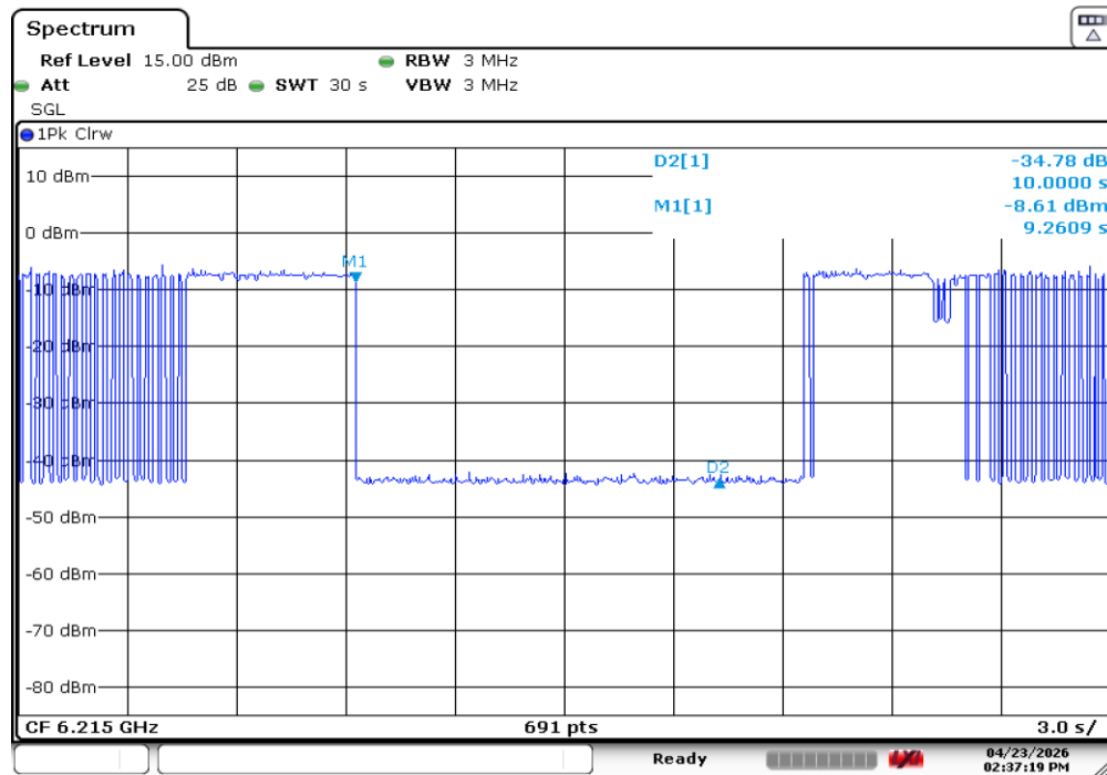
Plot 7-80. Contention Based Protocol Timing Plot (20MHz (UNII Band 5) – Ch. 53)
