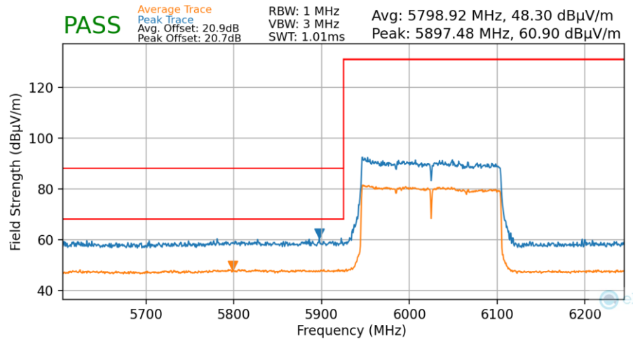
Plot 7-94. Radiated Lower Band Edge Plot MIMO (Average & Peak – UNII Band 5)
