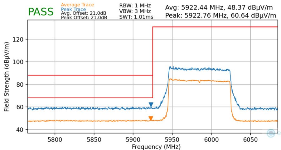
Plot 7-90. Radiated Lower Band Edge Plot MIMO (Average & Peak – UNII Band 5)
