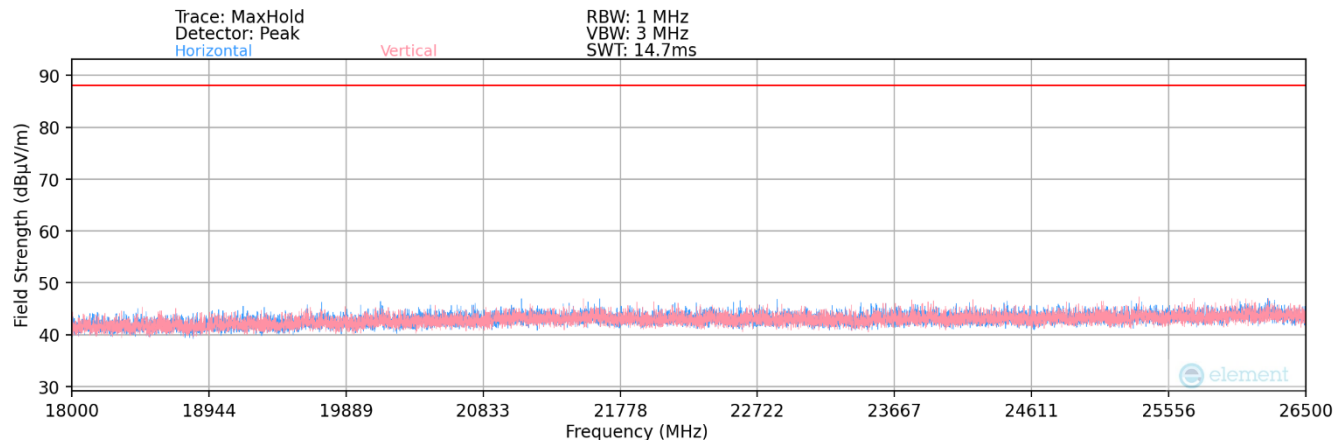
Plot 7-82. Radiated Spurious Plot 18GHz - 26.5GHz (802.11a) – Ch. 45
