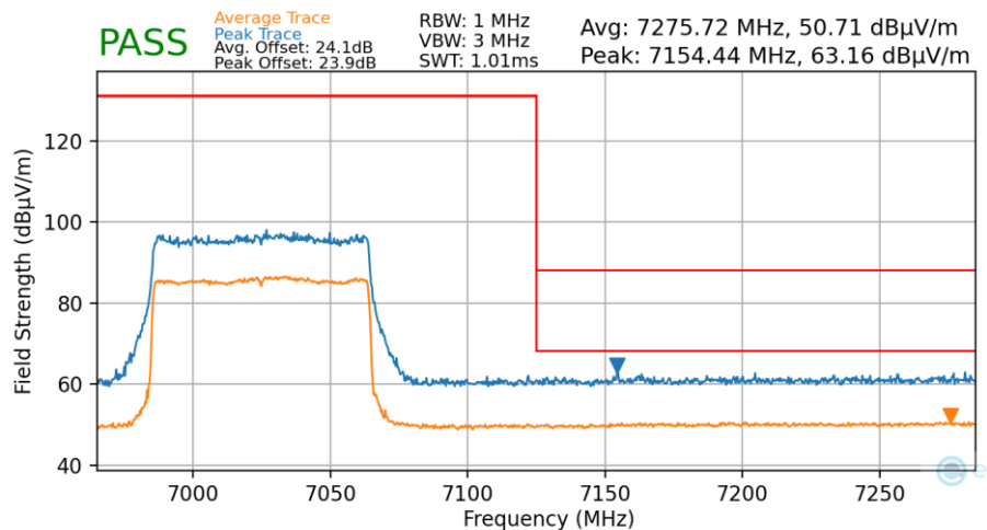
Plot 7-91. Radiated Upper Band Edge Plot MIMO (Average & Peak – UNII Band 8)
