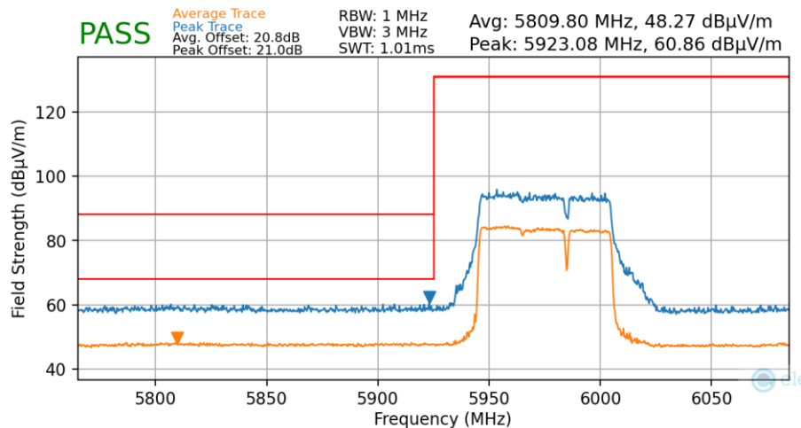
Plot 7-92. Radiated Lower Band Edge Plot MIMO (Average & Peak – UNII Band 5)
