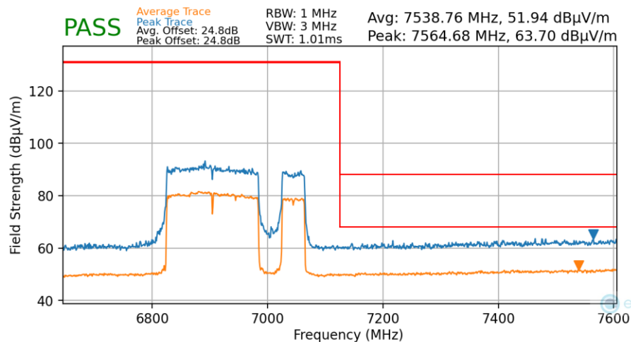
Plot 7-101. Radiated Upper Band Edge Plot MIMO (Average & Peak – UNII Band 8)
