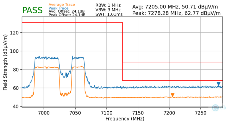
Plot 7-93. Radiated Upper Band Edge Plot MIMO (Average & Peak – UNII Band 8)
