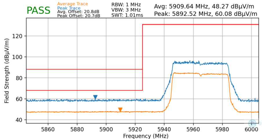
Plot 7-88. Radiated Lower Band Edge Plot MIMO (Average & Peak – UNII Band 5)
