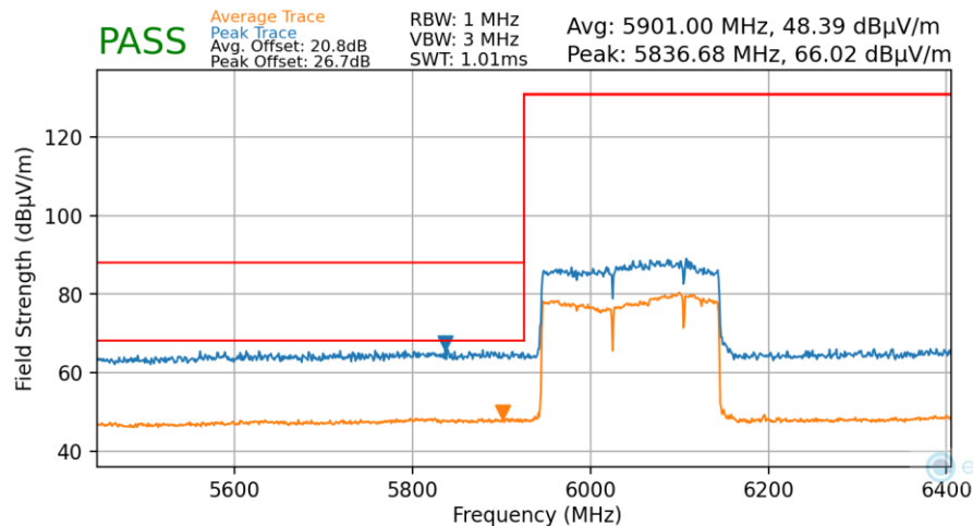
Plot 7-100. Radiated Lower Band Edge Plot MIMO (Average & Peak – UNII Band 5)
