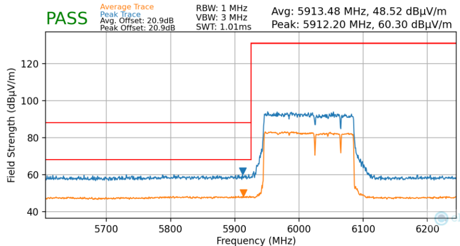
Plot 7-96. Radiated Lower Band Edge Plot MIMO (Average & Peak – UNII Band 5)
