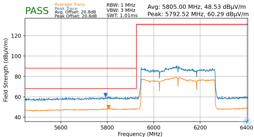
Plot 7-98. Radiated Lower Band Edge Plot MIMO (Average & Peak – UNII Band 5)
