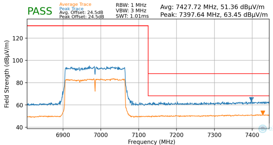
Plot 7-95. Radiated Upper Band Edge Plot MIMO (Average & Peak – UNII Band 8)
