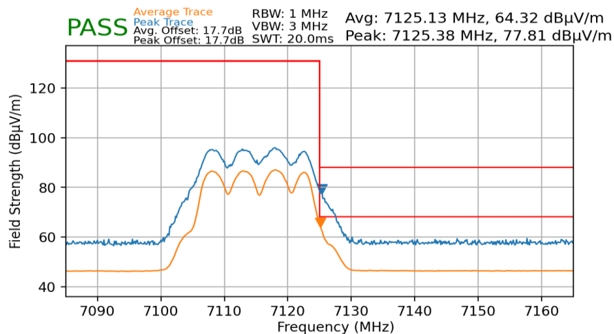
Plot 7-87. Radiated Upper Band Edge Plot MIMO (Average & Peak – UNII Band 8) – WCP
