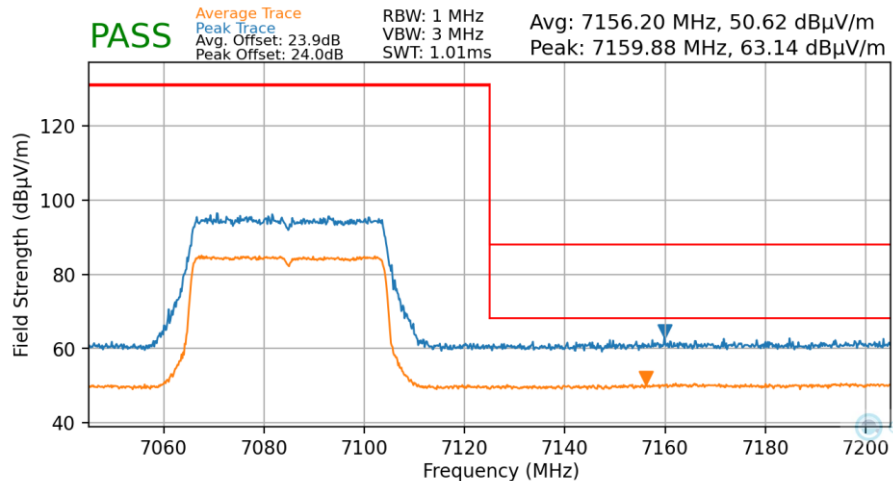
Plot 7-89. Radiated Upper Band Edge Plot MIMO (Average & Peak – UNII Band 8)
