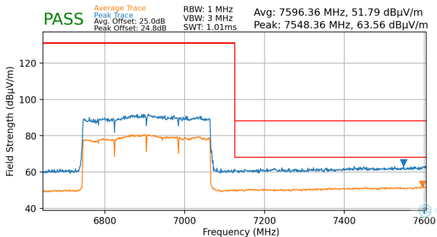
Plot 7-99. Radiated Upper Band Edge Plot MIMO (Average & Peak – UNII Band 8)
