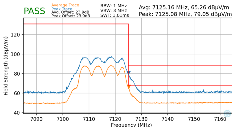
Plot 7-86. Radiated Upper Band Edge Plot MIMO (Average & Peak – UNII Band 8)
