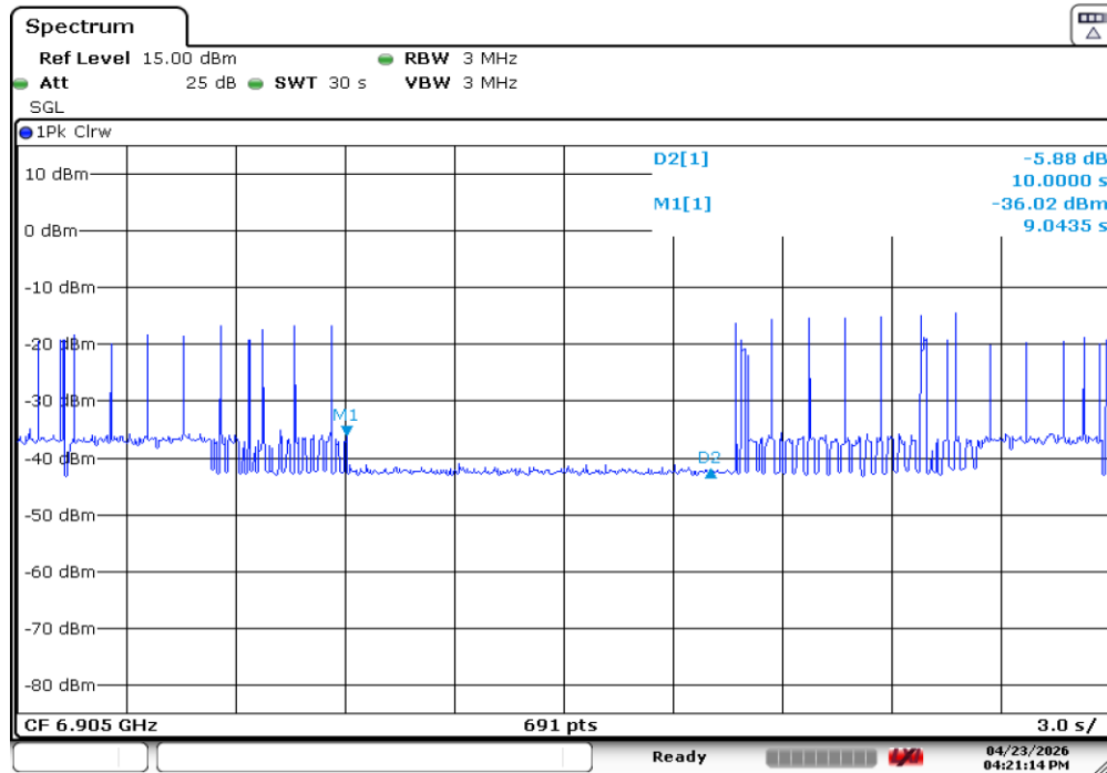
Plot 7-94. Contention Based Protocol Timing Plot (320MHz (UNII Band 8) – Ch. 191 Mid)
