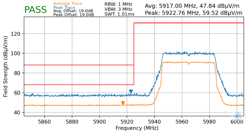
Plot 7-114. Radiated Lower Band Edge Plot MIMO (Average & Peak – UNII Band 5)
