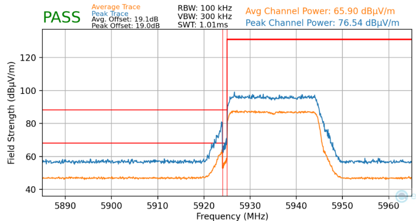
Plot 7-111. Radiated Lower Band Edge Plot MIMO (Average & Peak – UNII Band 5)
