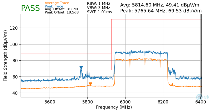
Plot 7-126. Radiated Lower Band Edge Plot MIMO (Average & Peak – UNII Band 5)
