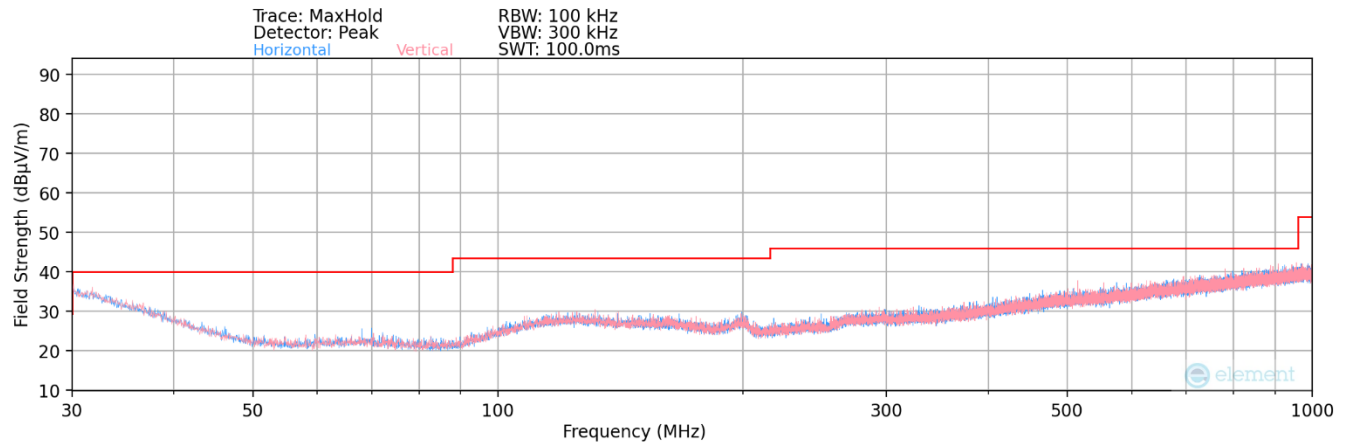
Plot 7-99. Radiated Spurious Plot below 1GHz MIMO (802.11a)
