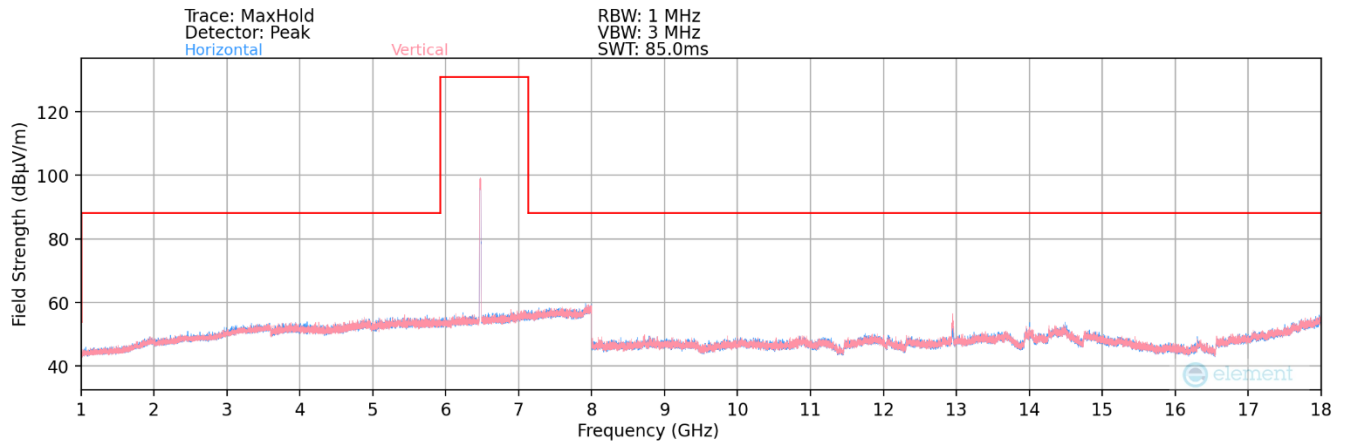
Plot 7-101. Radiated Spurious Plot 1GHz – 18GHz MIMO (802.11a – UNII Band 6 Ch. 105)
