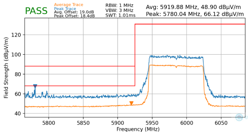
Plot 7-116. Radiated Lower Band Edge Plot MIMO (Average & Peak – UNII Band 5)
