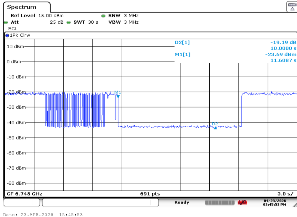
Plot 7-90. Contention Based Protocol Timing Plot (320MHz (UNII Band 7) – Ch. 159 Mid)
