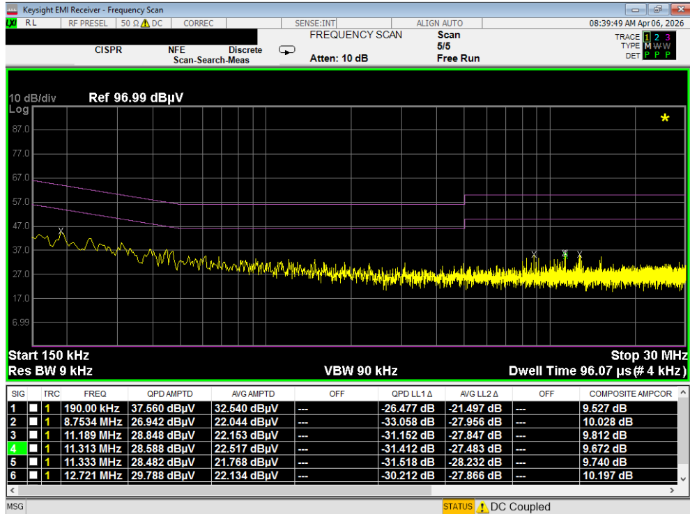
Plot 7-128. Line Conducted Plot with 802.11a UNII Band 5 (L1)
