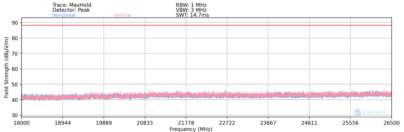
Plot 7-105. Radiated Spurious Plot 18GHz - 26.5GHz (802.11a) – Ch. 45
