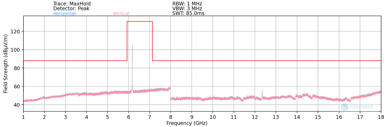
Plot 7-100. Radiated Spurious Plot 1GHz – 18GHz MIMO (802.11a – UNII Band 5 Ch. 45)
