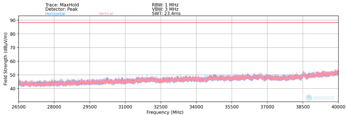
Plot 7-106. Radiated Spurious Plot 26.5GHz - 40GHz (802.11a) – Ch. 45
