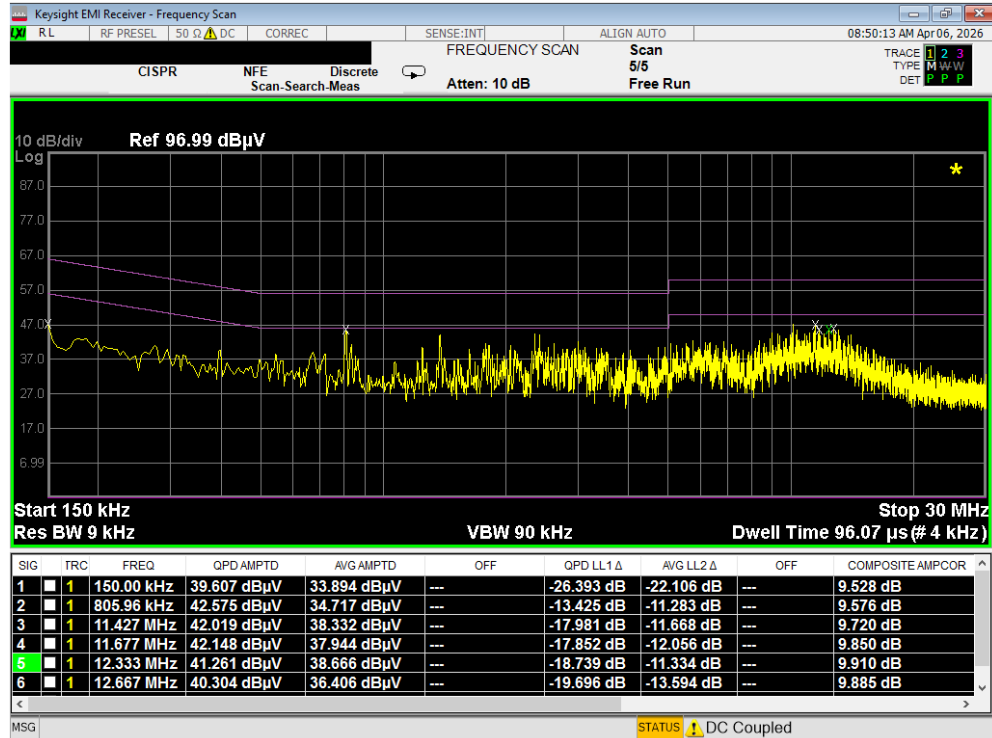
Plot 7-138. Line Conducted Plot with 802.11a UNII Band 6 (L1) with WCP
