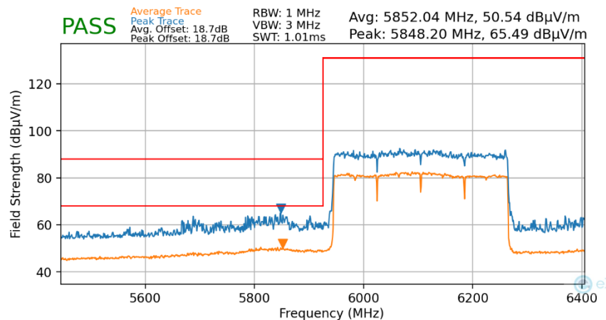
Plot 7-124. Radiated Lower Band Edge Plot MIMO (Average & Peak – UNII Band 5)
