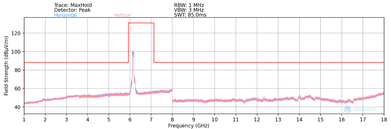
Plot 7-104. Radiated Spurious Plot above 1GHz MIMO (802.11be – UNII Band 5 Ch. 39 – Punctured)
