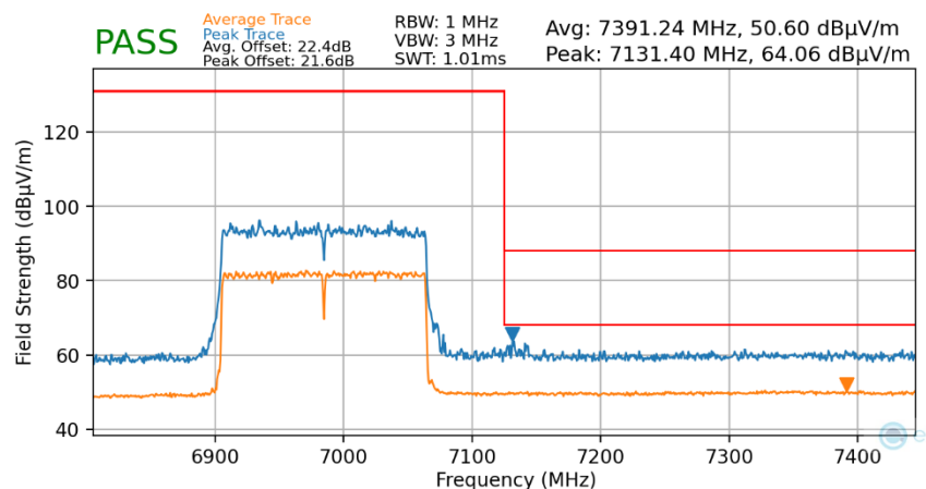
Plot 7-121. Radiated Upper Band Edge Plot MIMO (Average & Peak – UNII Band 8)
