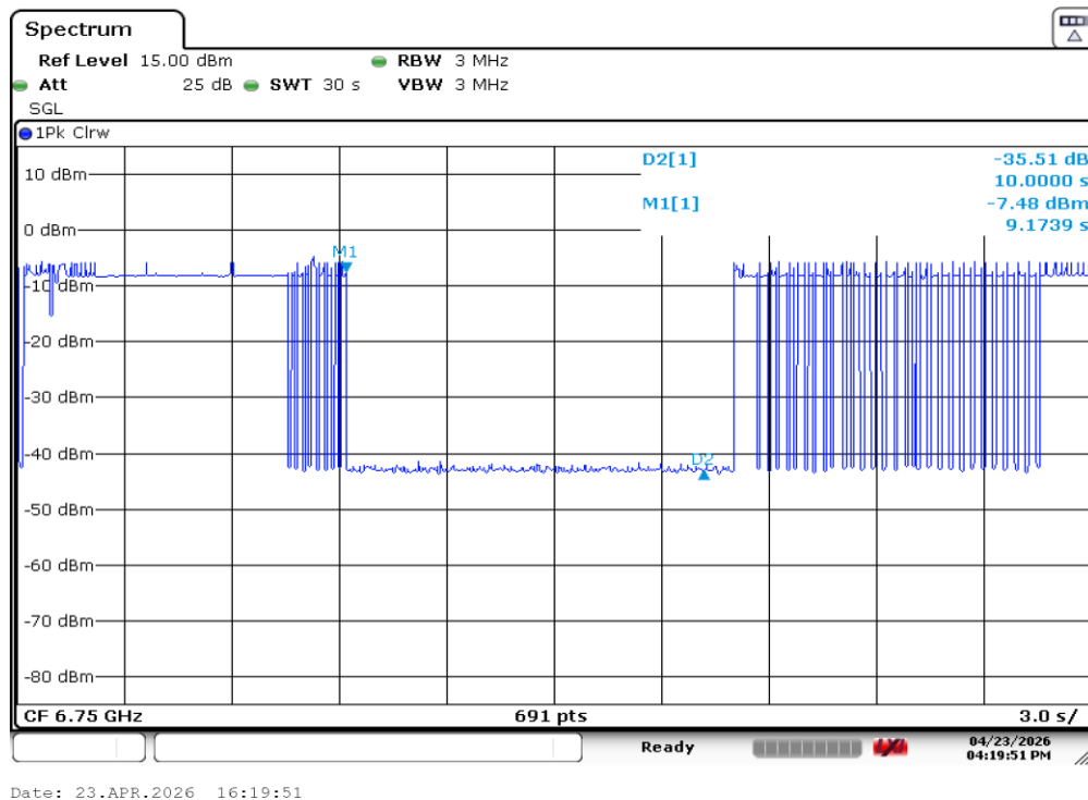
Plot 7-93. Contention Based Protocol Timing Plot (320MHz (UNII Band 8) – Ch. 191 Low)
