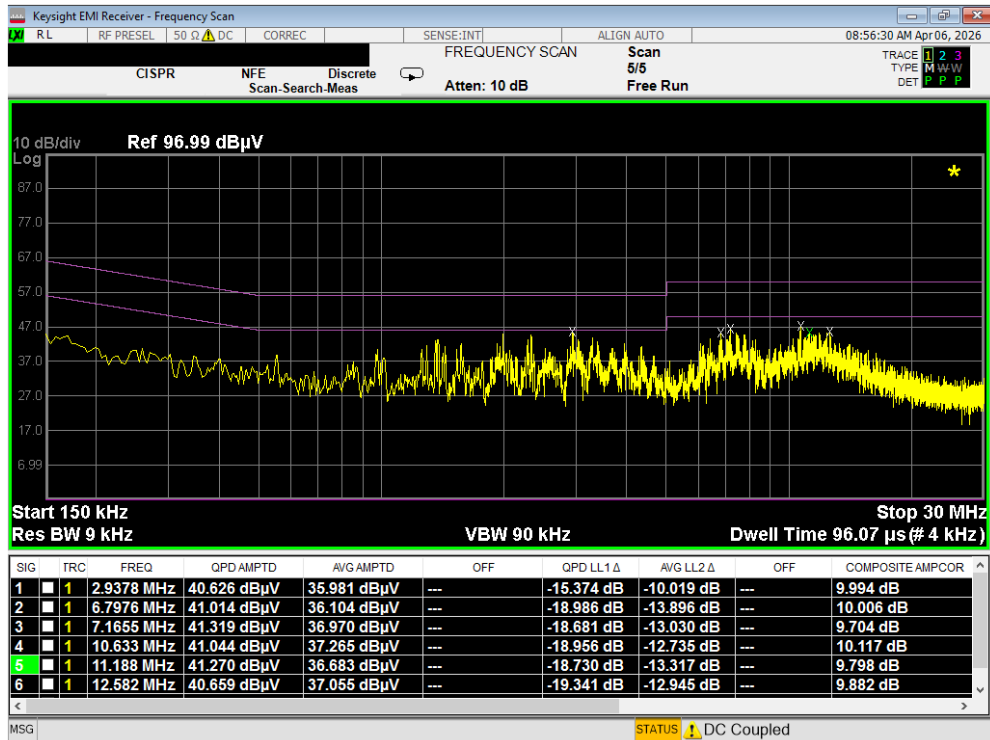
Plot 7-134. Line Conducted Plot with 802.11a UNII Band 8 (L1)
