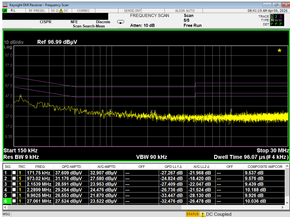
Plot 7-129. Line Conducted Plot with 802.11a UNII Band 5 (N)
