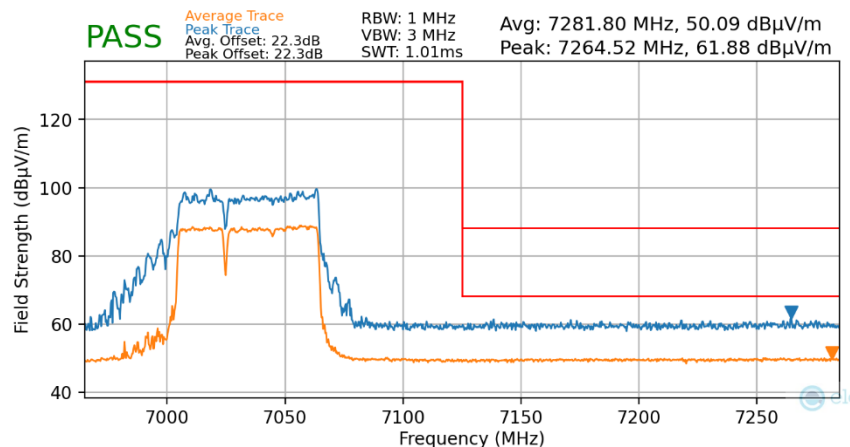
Plot 7-119. Radiated Upper Band Edge Plot MIMO (Average & Peak – UNII Band 8)
