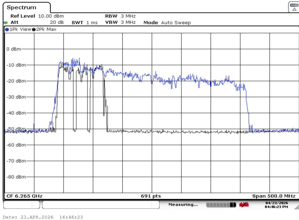
Plot 7-97. CBP 320MHz Channel - Injection Center – [6265 MHz]
