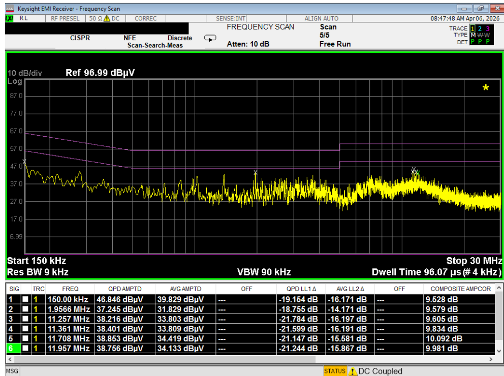
Plot 7-131. Line Conducted Plot with 802.11a UNII Band 6 (N)
