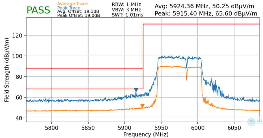
Plot 7-118. Radiated Lower Band Edge Plot MIMO (Average & Peak – UNII Band 5)
