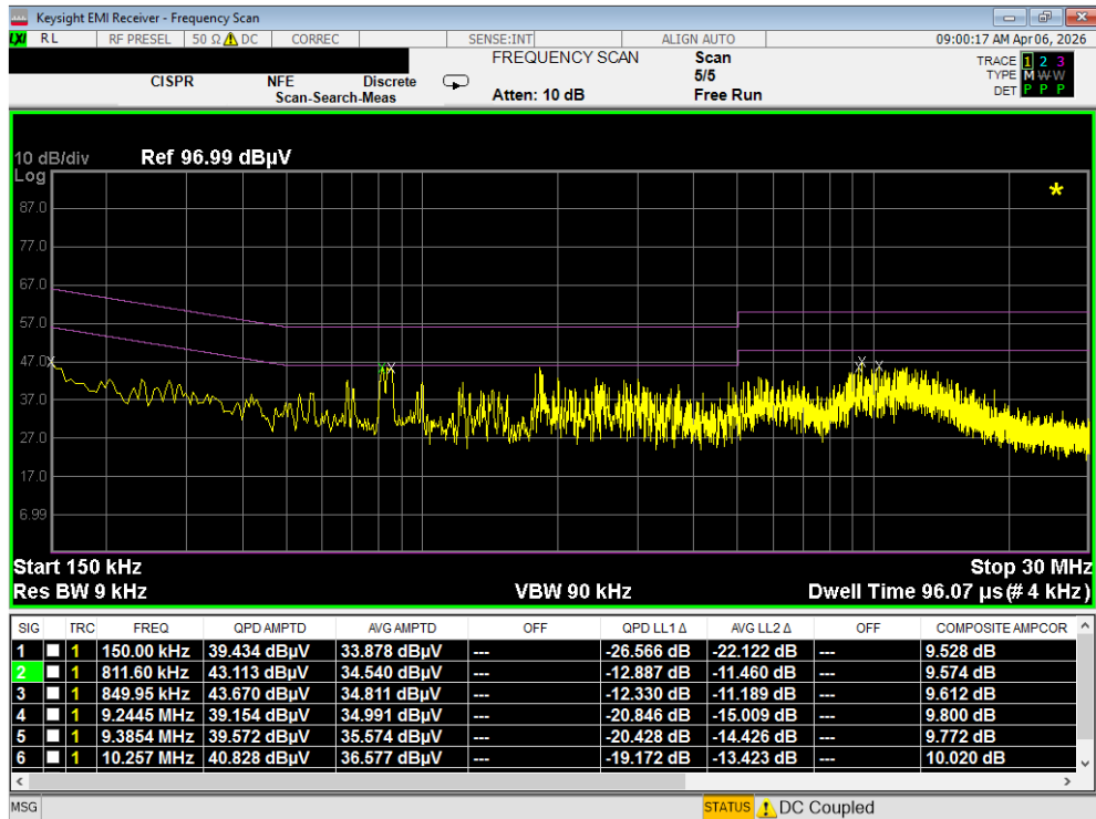
Plot 7-142. Line Conducted Plot with 802.11a UNII Band 8 (L1) with WCP
