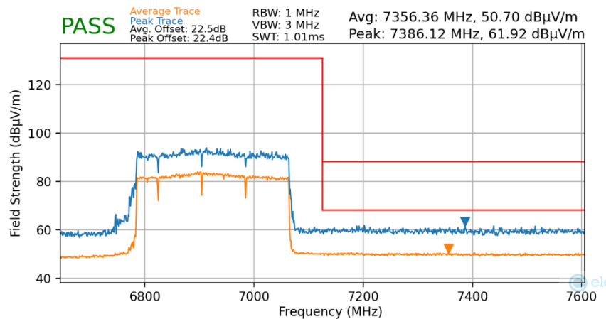
Plot 7-127. Radiated Upper Band Edge Plot MIMO (Average & Peak – UNII Band 8)
