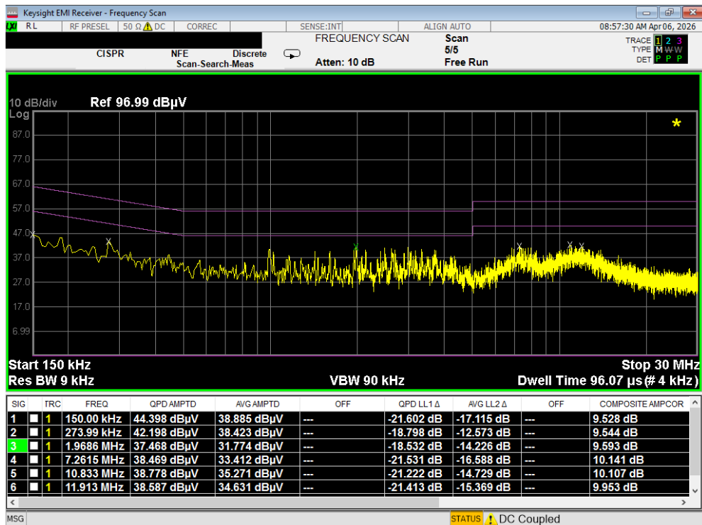
Plot 7-135. Line Conducted Plot with 802.11a UNII Band 8 (N)
