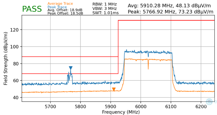
Plot 7-120. Radiated Lower Band Edge Plot MIMO (Average & Peak – UNII Band 5)
