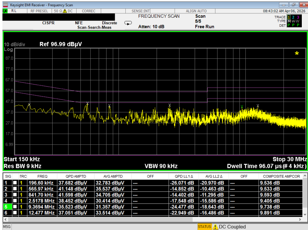
Plot 7-137. Line Conducted Plot with 802.11a UNII Band 5 (N) with WCP
