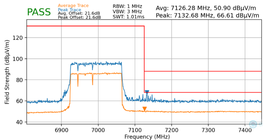
Plot 7-123. Radiated Upper Band Edge Plot MIMO (Average & Peak – UNII Band 8)
