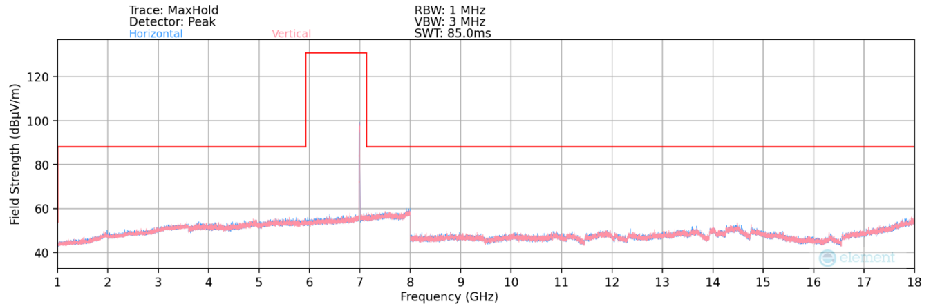
Plot 7-103. Radiated Spurious Plot 1GHz – 18GHz MIMO (802.11a – U Band 8 Ch. 209)
