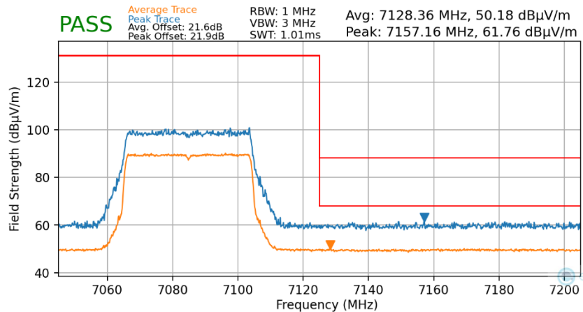
Plot 7-115. Radiated Upper Band Edge Plot MIMO (Average & Peak – UNII Band 8)
