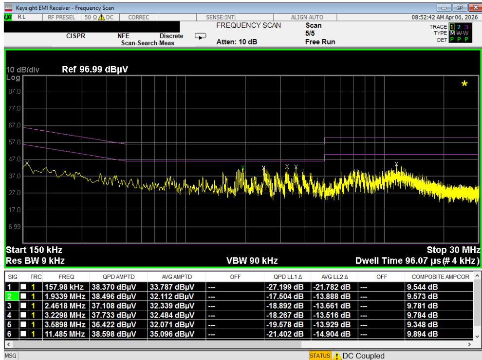
Plot 7-133. Line Conducted Plot with 802.11a UNII Band 7 (N)
