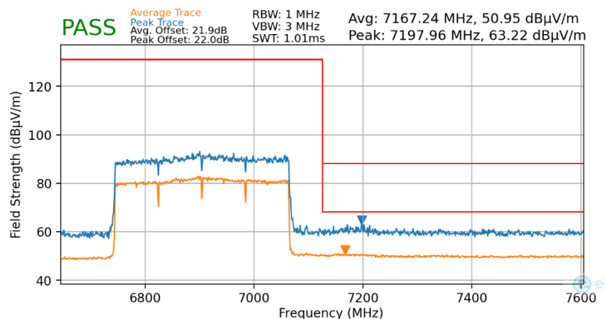
Plot 7-125. Radiated Upper Band Edge Plot MIMO (Average & Peak – UNII Band 8)
