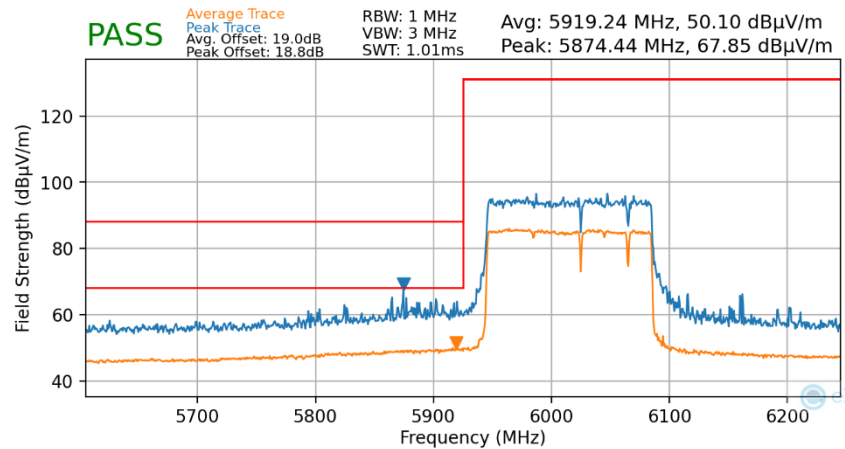
Plot 7-122. Radiated Lower Band Edge Plot MIMO (Average & Peak – UNII Band 5)
