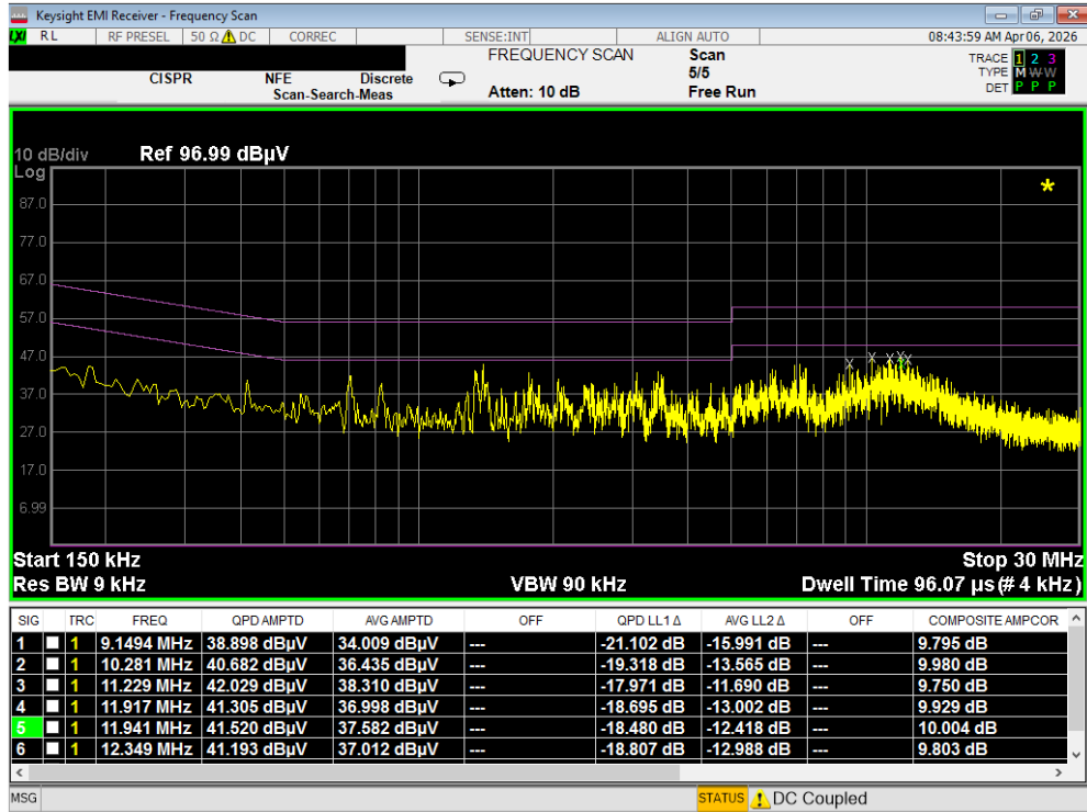
Plot 7-136. Line Conducted Plot with 802.11a UNII Band 5 (L1) with WCP
