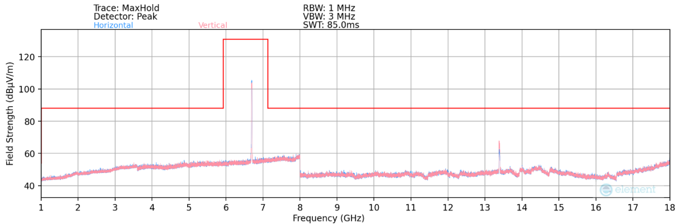
Plot 7-102. Radiated Spurious Plot 1GHz – 18GHz MIMO (802.11a – UNII Band 7 Ch. 149)
