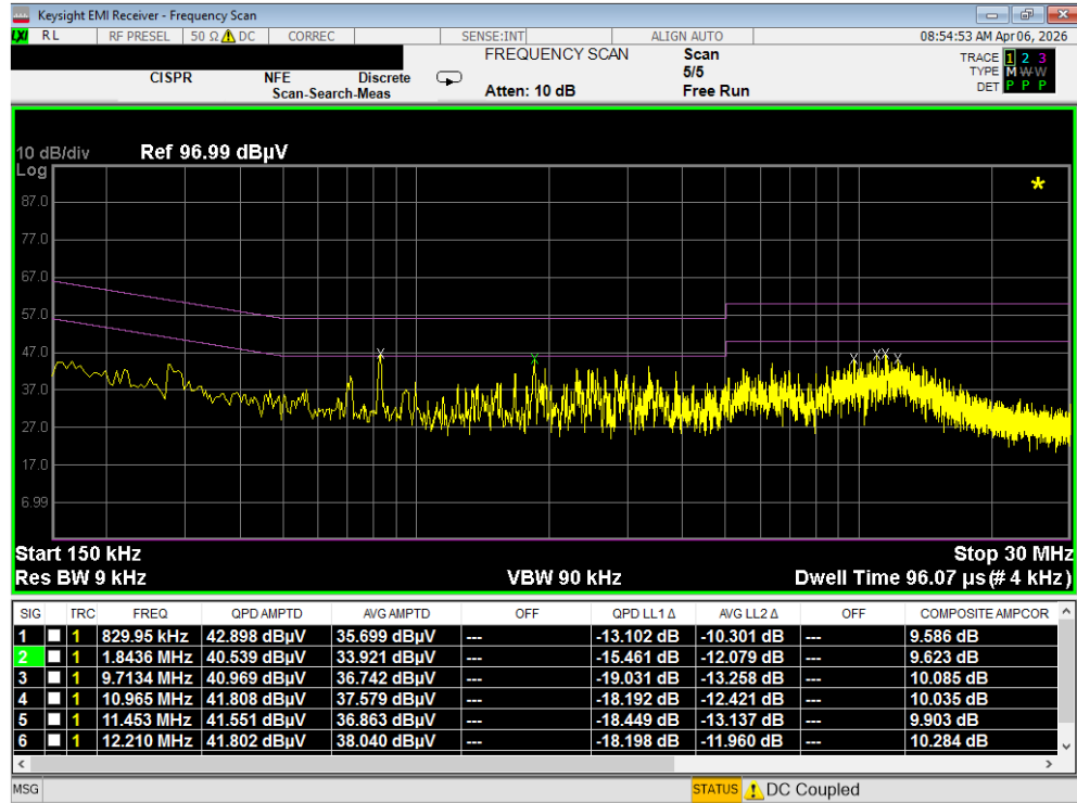
Plot 7-140. Line Conducted Plot with 802.11a UNII Band 7 (L1) with WCP
