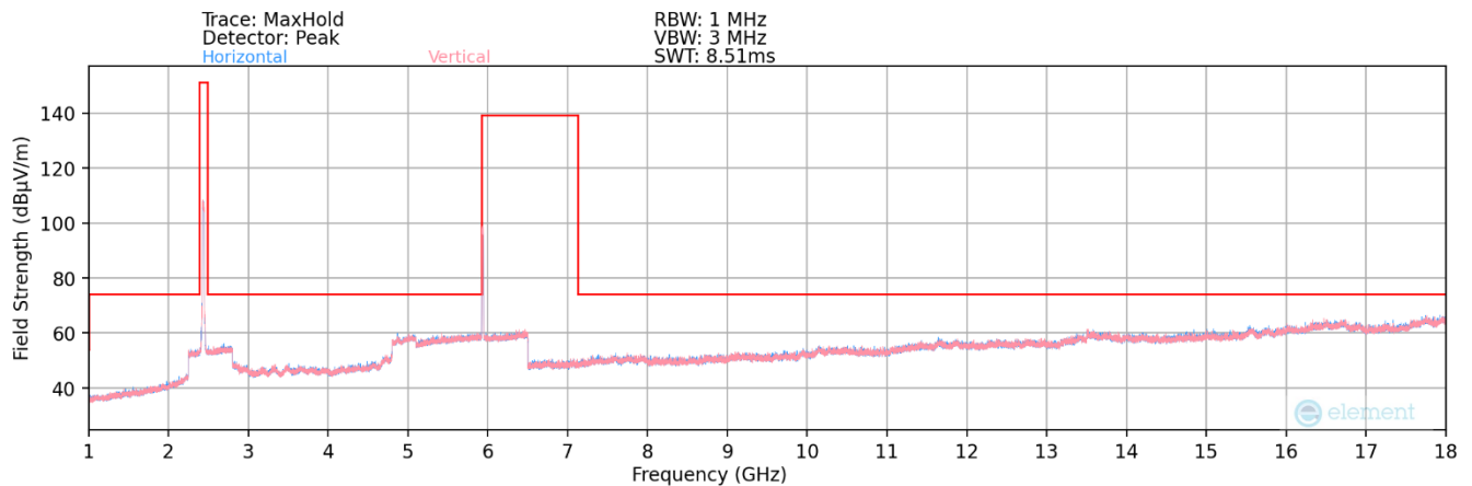
Plot 7-108. Radiated Spurious Plot above 1GHz MIMO 802.11b (2.4GHz – Ch.6) + MIMO 802.11a (6GHz – Ch.2)
