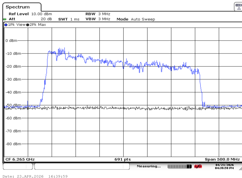
Plot 7-96. CBP 320MHz Channel - Injection Lower Edge – [6110 MHz]
