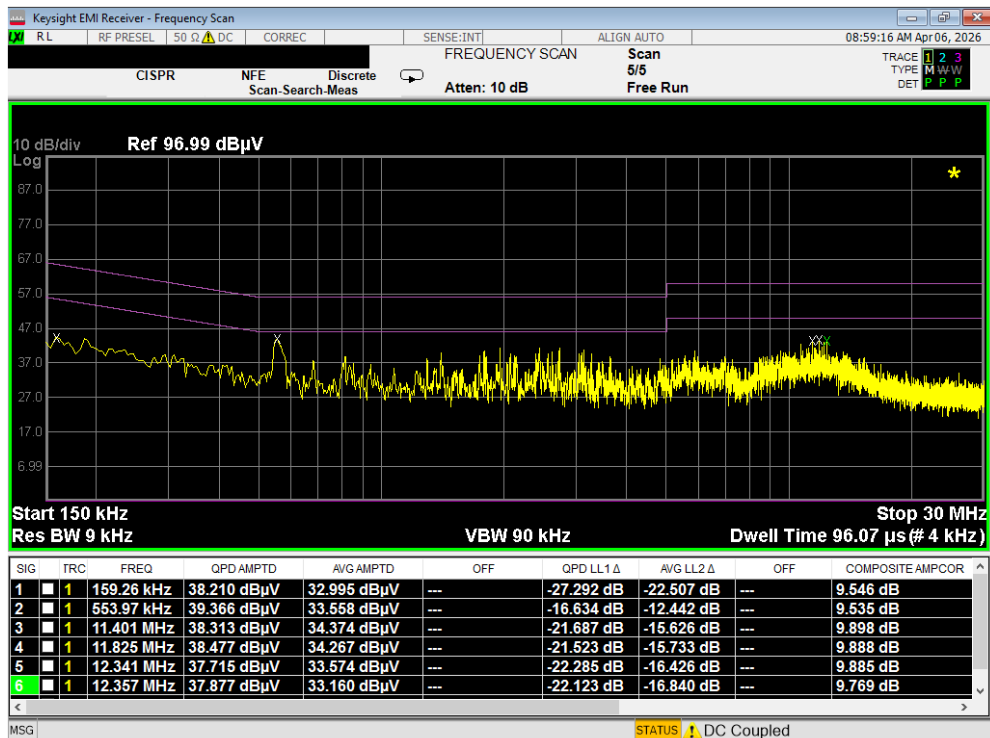
Plot 7-143. Line Conducted Plot with 802.11a UNII Band 8 (N) with WCP
