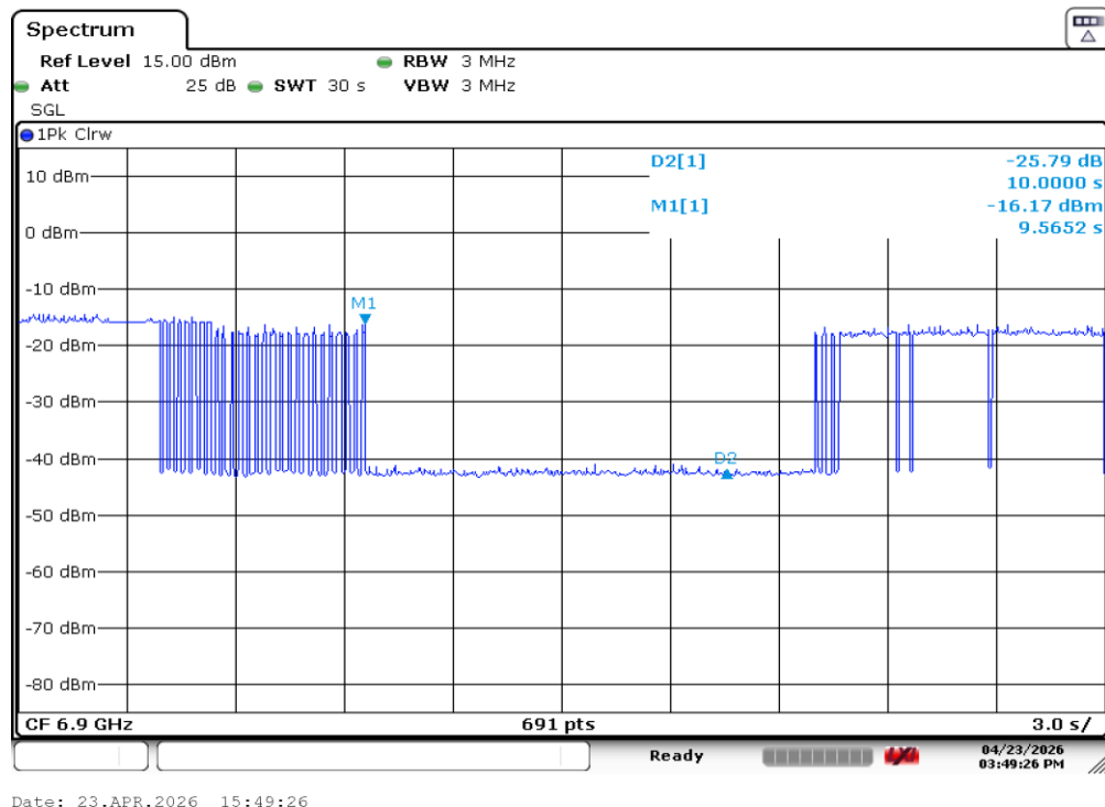
Plot 7-91. Contention Based Protocol Timing Plot (320MHz (UNII Band 7) – Ch. 159 High)
