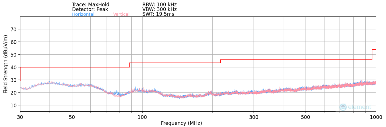
Plot 7-107. Radiated Spurious Plot below 1GHz MIMO 802.11b (2.4GHz – Ch.6) + MIMO 802.11a (6GHz – Ch.2)
