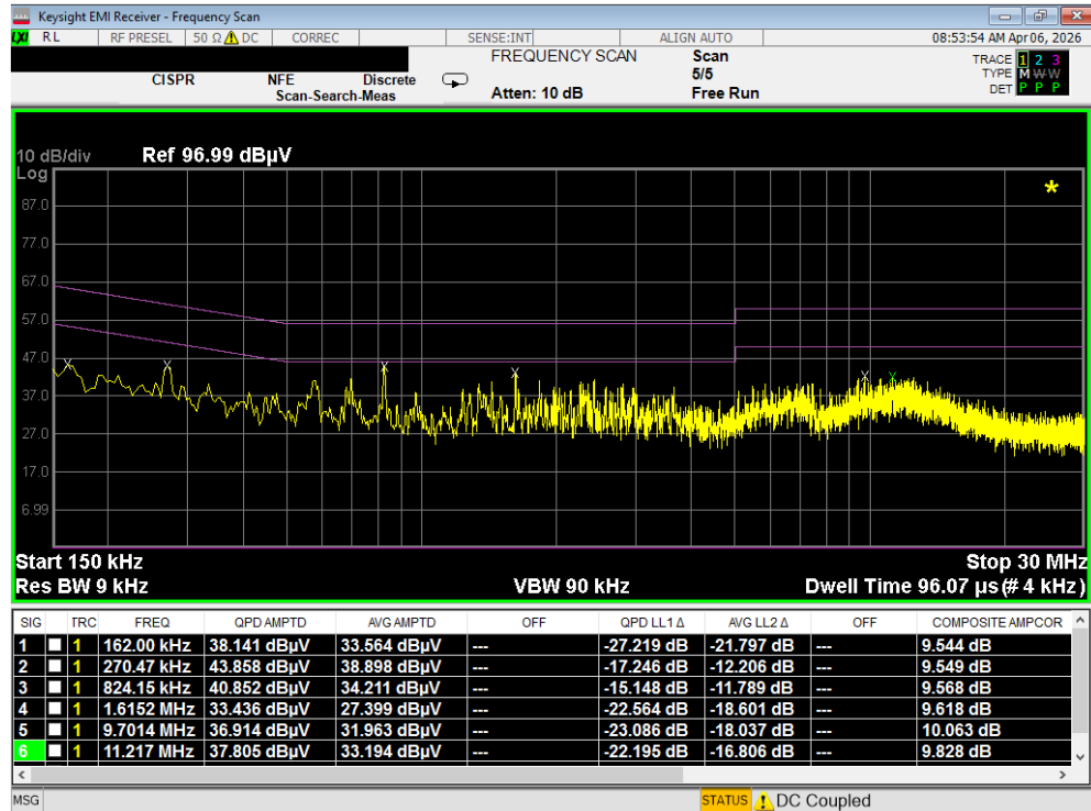
Plot 7-141. Line Conducted Plot with 802.11a UNII Band 7 (N) with WCP
