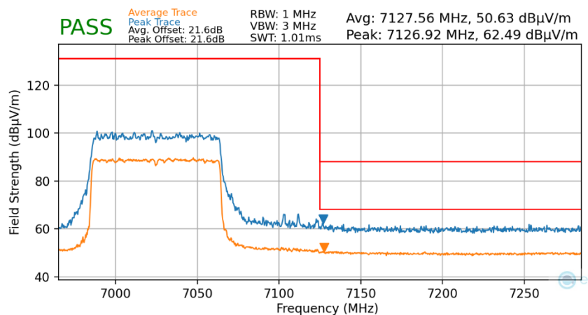
Plot 7-117. Radiated Upper Band Edge Plot MIMO (Average & Peak – UNII Band 8)
