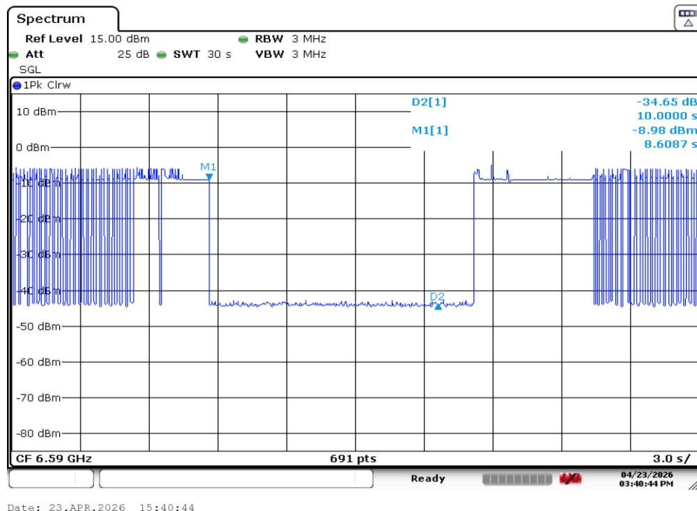
Plot 7-89. Contention Based Protocol Timing Plot (320MHz (UNII Band 7) – Ch. 159 Low)
