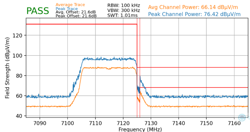
Plot 7-112. Radiated Upper Band Edge Plot MIMO (Average & Peak – UNII Band 8)
