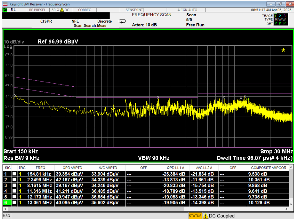
Plot 7-132. Line Conducted Plot with 802.11a UNII Band 7 (L1)
