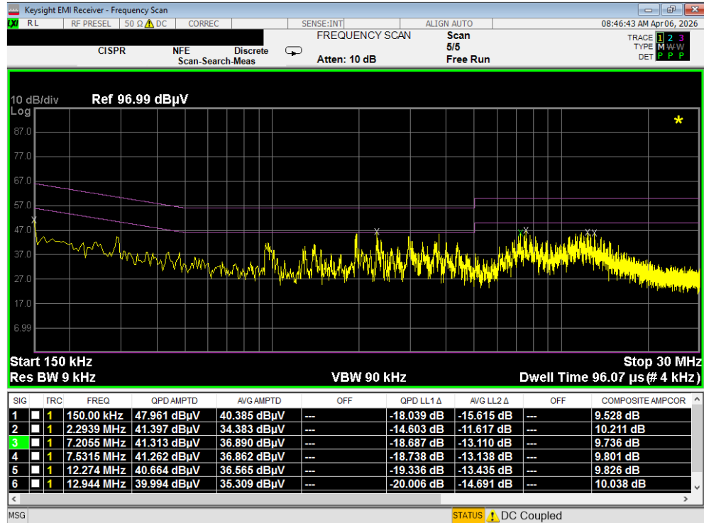
Plot 7-130. Line Conducted Plot with 802.11a UNII Band 6 (L1)
