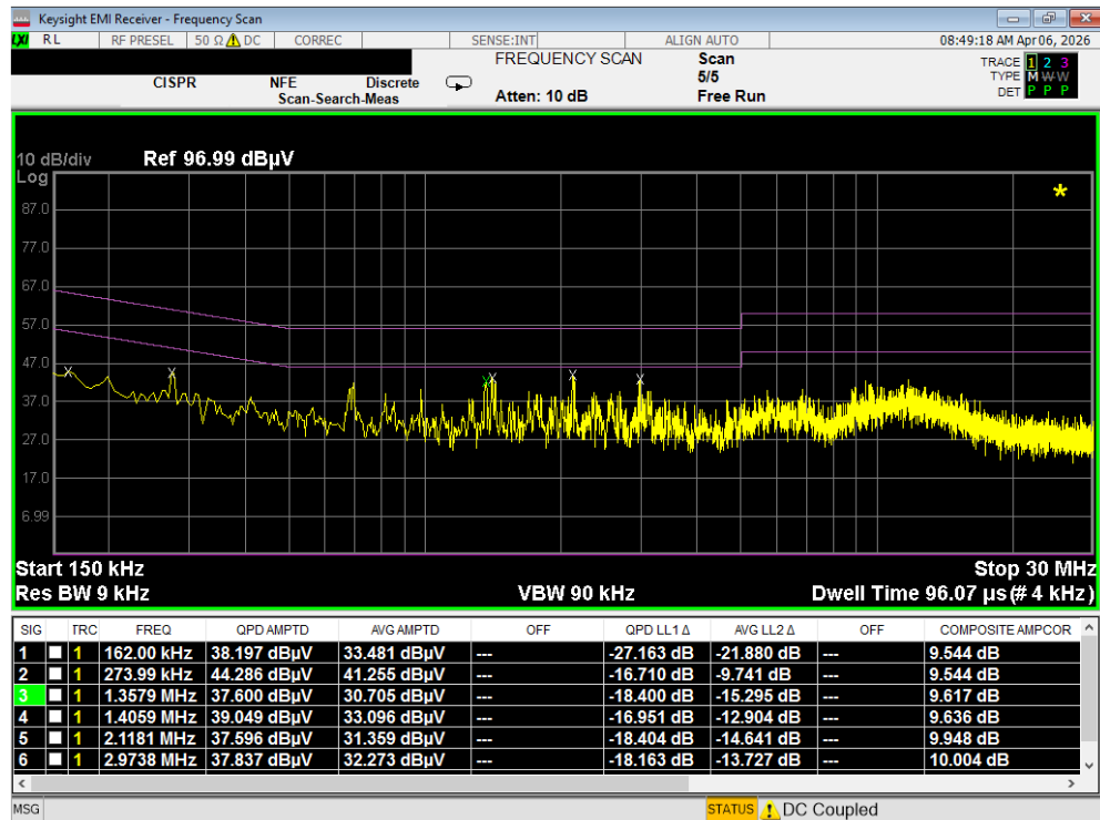
Plot 7-139. Line Conducted Plot with 802.11a UNII Band 6 (N) with WCP
