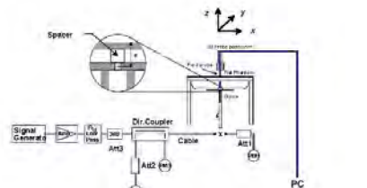
Figure 11-1 System Verification Setup Diagram
