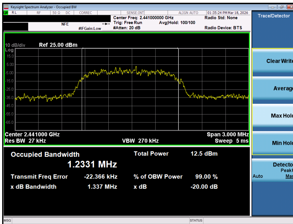
Plot 7-14. 20dB Bandwidth Plot (Bluetooth, 2Mbps – Ch. 39) – SISO ANT 2
