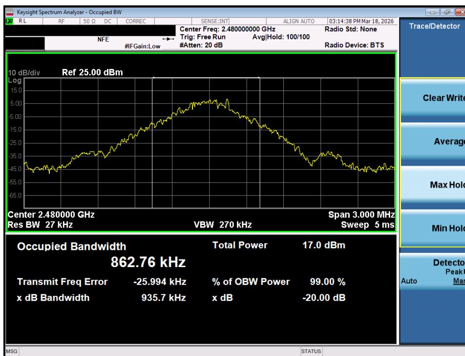
Plot 7-30. 20dB Bandwidth Plot (Bluetooth, 1Mbps – Ch. 78) – MIMO ANT 2
