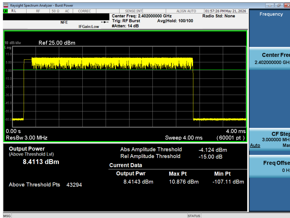
Plot 7-103. Average Conducted Power (2Mbps – Ch. 0) – MIMO ANT 2
