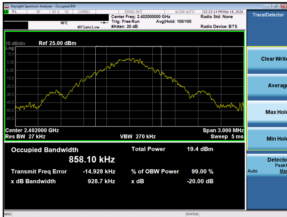
Plot 7-19. 20dB Bandwidth Plot (Bluetooth, 1Mbps – Ch. 0) – MIMO ANT 1
