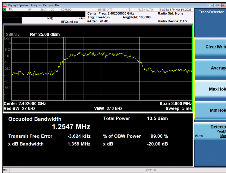
Plot 7-13. 20dB Bandwidth Plot (Bluetooth, 2Mbps – Ch. 0) – SISO ANT 2
