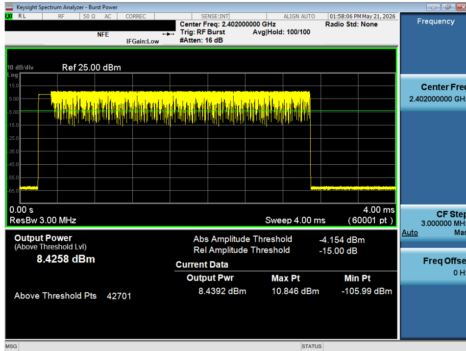
Plot 7-106. Average Conducted Power (3Mbps – Ch. 0) – MIMO ANT 2
