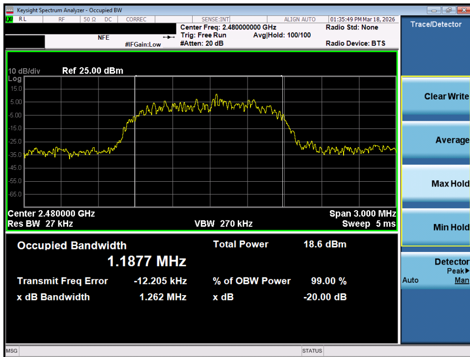
Plot 7-18. 20dB Bandwidth Plot (Bluetooth, 3Mbps – Ch. 78) – SISO ANT 2
