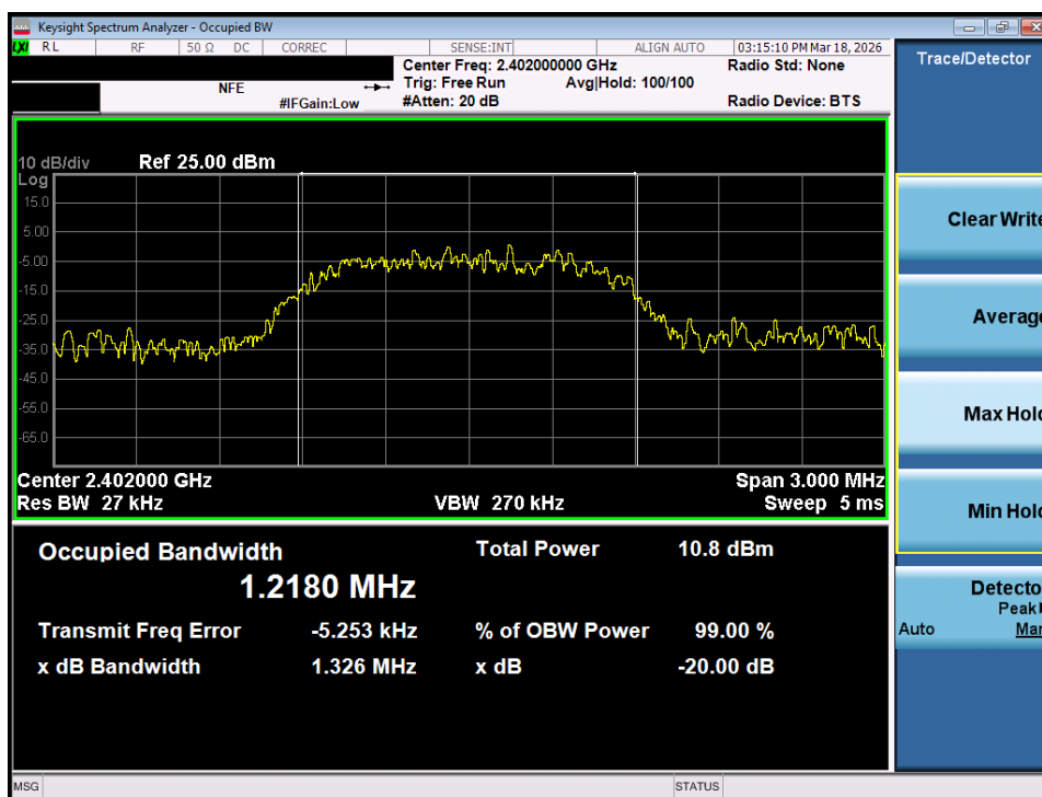
Plot 7-34. 20dB Bandwidth Plot (Bluetooth, 3Mbps – Ch. 0) – MIMO ANT 2
