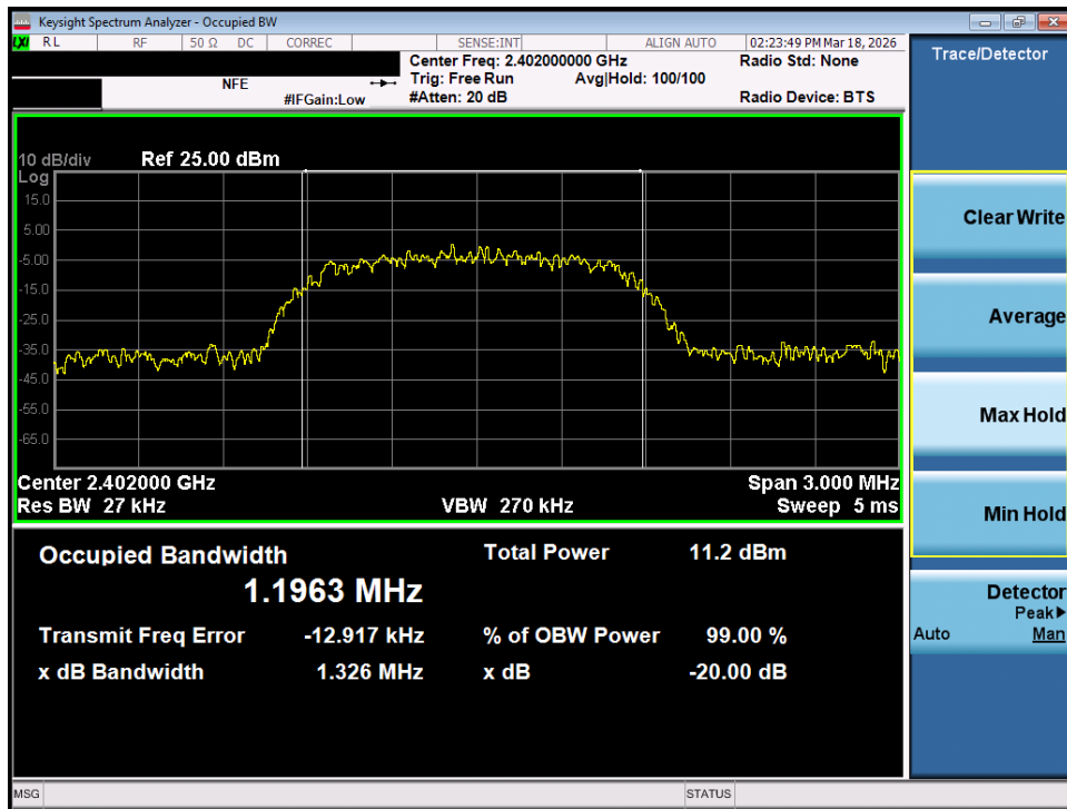
Plot 7-25. 20dB Bandwidth Plot (Bluetooth, 3Mbps – Ch. 0) – MIMO ANT 1
