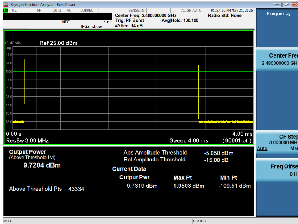
Plot 7-102. Average Conducted Power (1Mbps – Ch. 78) – MIMO ANT 2
