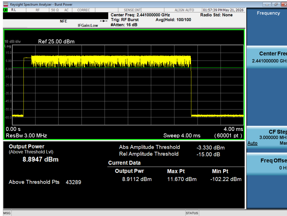
Plot 7-104. Average Conducted Power (2Mbps – Ch. 39) – MIMO ANT 2
