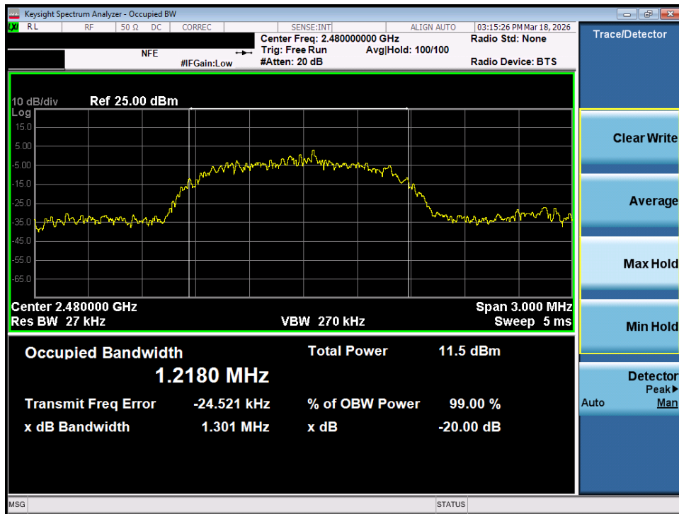
Plot 7-36. 20dB Bandwidth Plot (Bluetooth, 3Mbps – Ch. 78) – MIMO ANT 2
