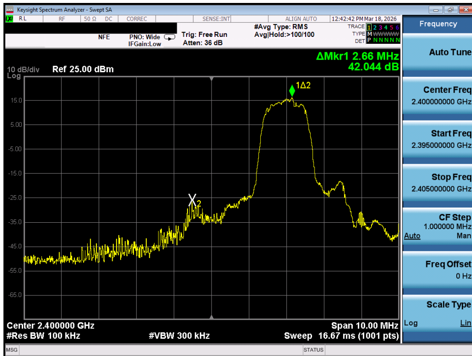
Plot 7-109. Band Edge Plot (Bluetooth with Hopping Disabled, 3 Mbps – Ch. 0) – SISO ANT 1
