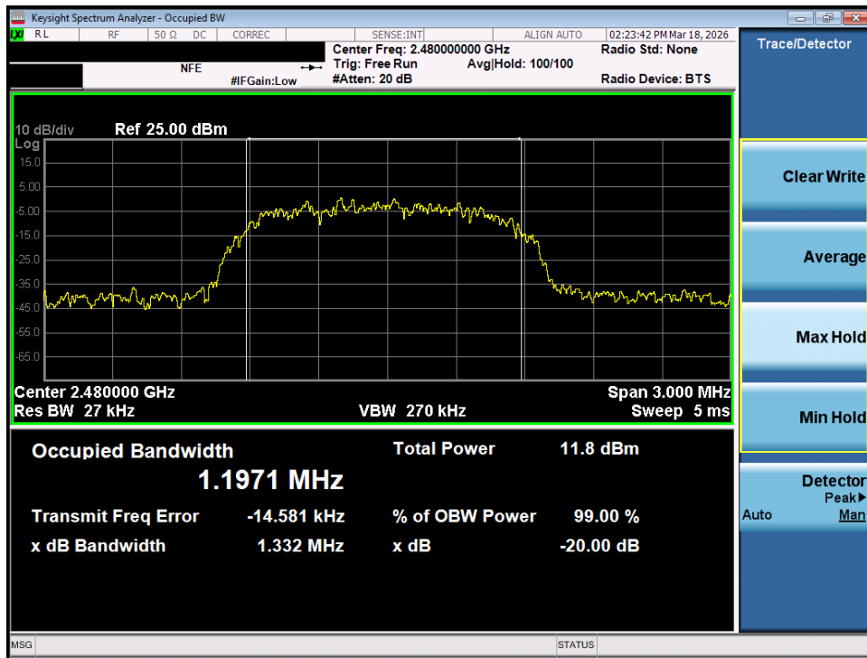
Plot 7-24. 20dB Bandwidth Plot (Bluetooth, 2Mbps – Ch. 78) – MIMO ANT 1
