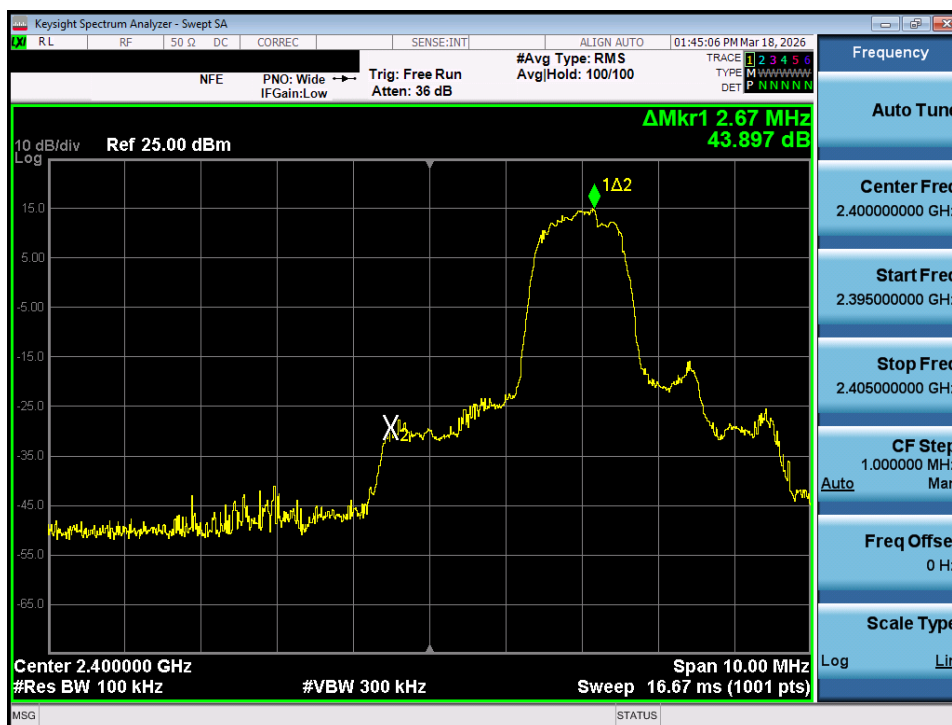
Plot 7-113. Band Edge Plot (Bluetooth with Hopping Disabled, 3 Mbps – Ch. 0) – SISO ANT 2
