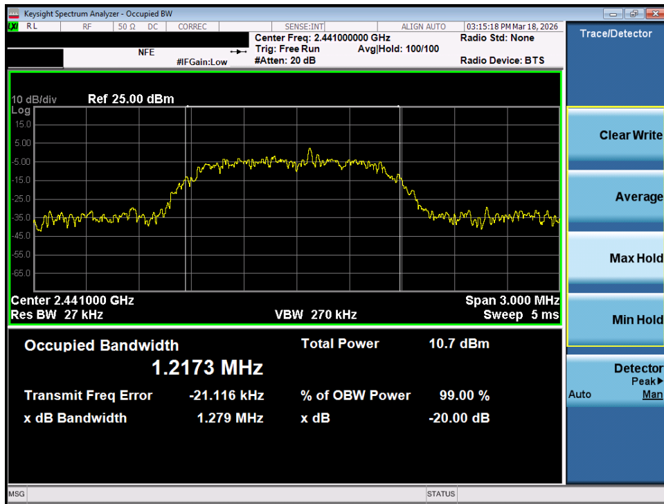
Plot 7-35. 20dB Bandwidth Plot (Bluetooth, 3Mbps – Ch. 39) – MIMO ANT 2
