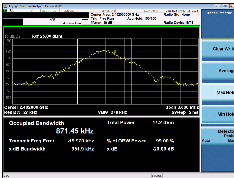
Plot 7-28. 20dB Bandwidth Plot (Bluetooth, 1Mbps – Ch. 0) – MIMO ANT 2
