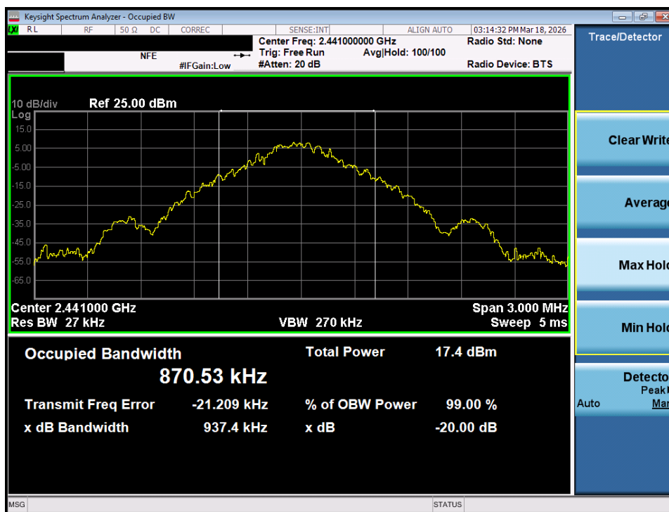
Plot 7-29. 20dB Bandwidth Plot (Bluetooth, 1Mbps – Ch. 39) – MIMO ANT 2
