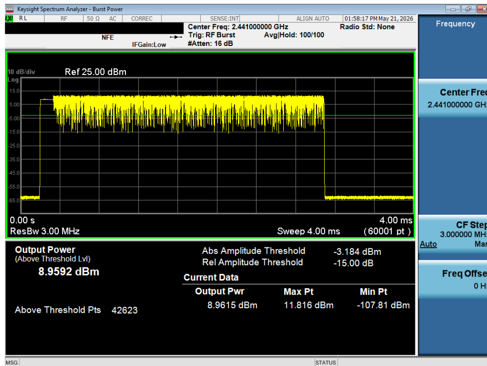
Plot 7-107. Average Conducted Power (3Mbps – Ch. 39) – MIMO ANT 2
