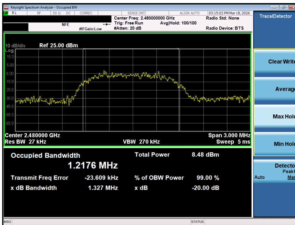
Plot 7-33. 20dB Bandwidth Plot (Bluetooth, 2Mbps – Ch. 78) – MIMO ANT 2
