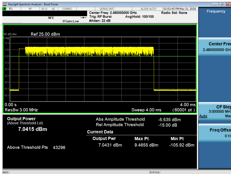
Plot 7-105. Average Conducted Power (2Mbps – Ch. 78) – MIMO ANT 2
