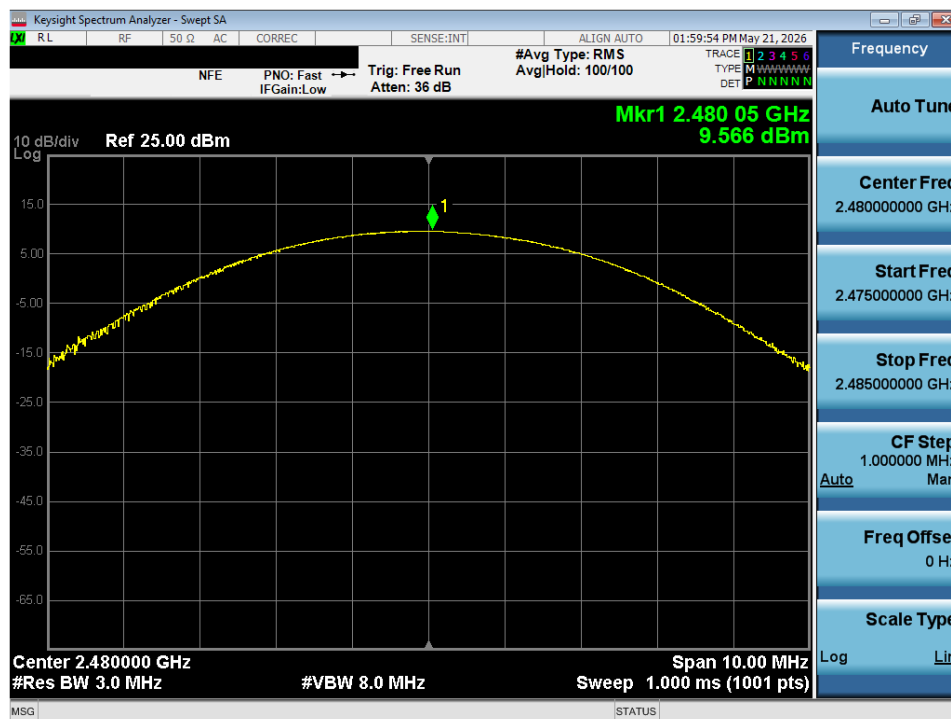
Plot 7-99. Peak Conducted Power (3Mbps – Ch. 78) – MIMO ANT 2
