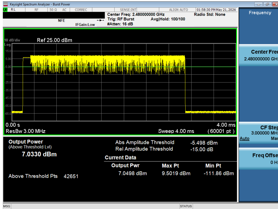
Plot 7-108. Average Conducted Power (3Mbps – Ch. 78) – MIMO ANT 2
