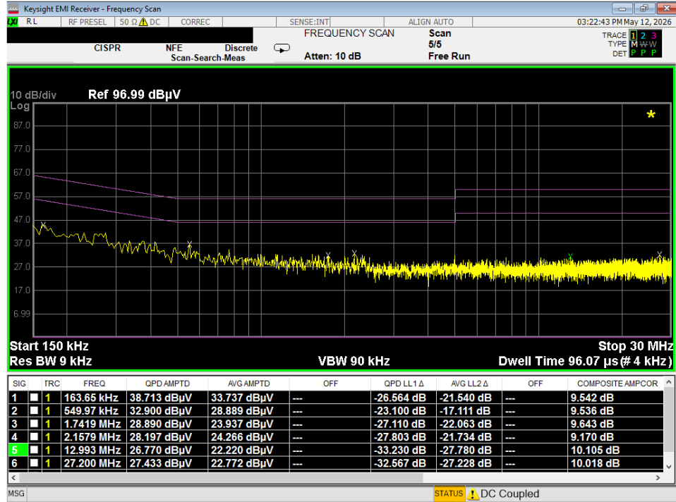
Plot 7-118. Line Conducted Plot with 802.11b (L1)
