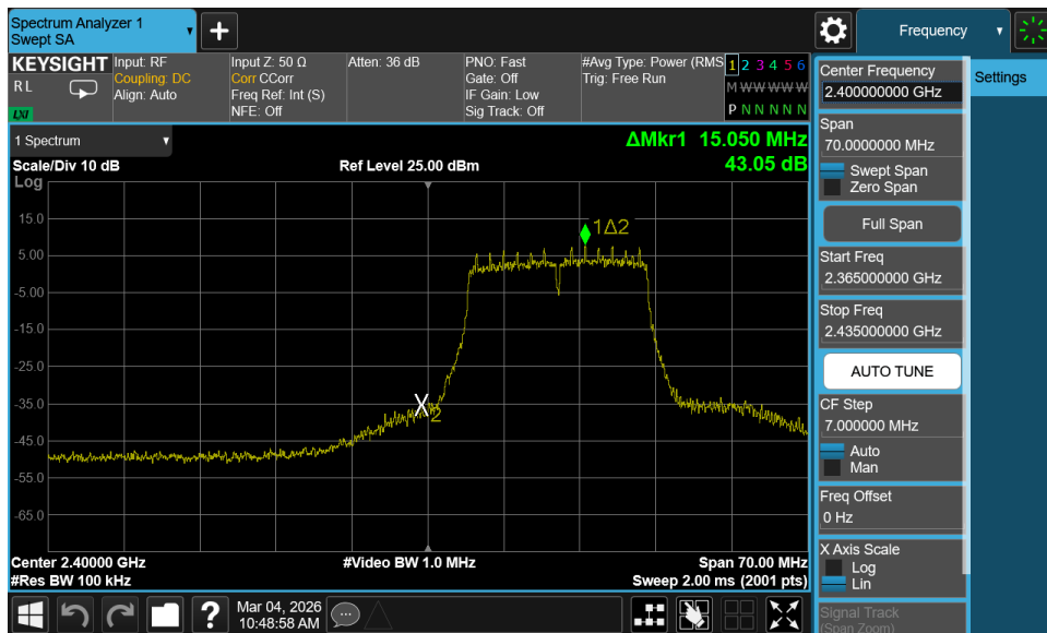
Plot 7-76. Band Edge Plot MIMO ANT1 (802.11g – Ch. 1)
