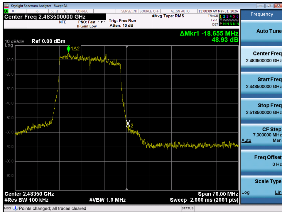
Plot 7-84. Band Edge Plot MIMO ANT1 (802.11ax/be – Ch. 13)
