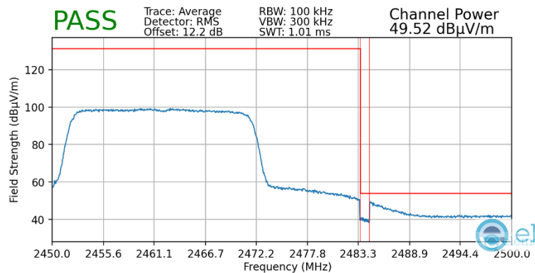
Plot 9-1. Radiated Restricted Upper Band Edge Measurement MIMO (Average)
