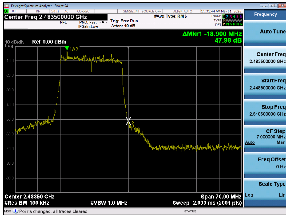
Plot 7-96. Band Edge Plot MIMO ANT2 (802.11ax/be – Ch. 13)
