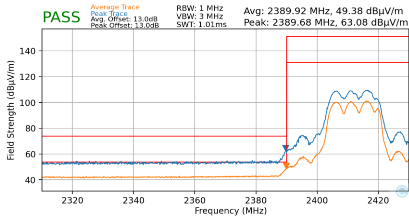
Plot 7-114. Radiated Restricted Lower Band Edge Measurement MIMO (Average & Peak)
