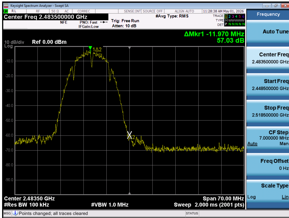
Plot 7-87. Band Edge Plot MIMO ANT2 (802.11b – Ch. 13)
