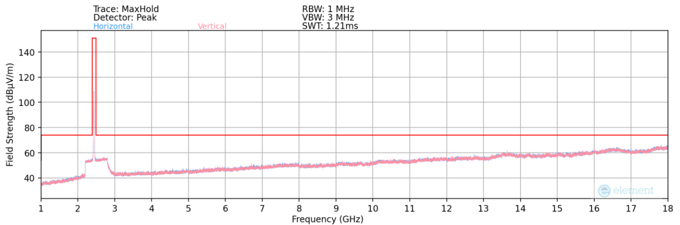
Plot 7-111. Radiated Spurious Plot above 1GHz MIMO (802.11b – Ch. OFDM 6)
