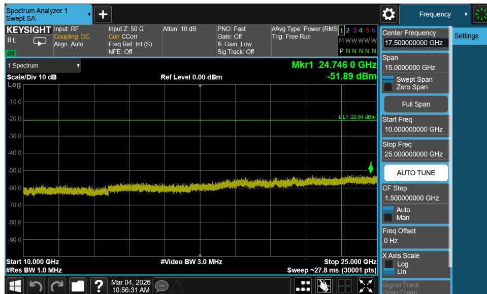
Plot 7-98. Conducted Spurious Plot MIMO ANT1 (802.11b – Ch. 1)
