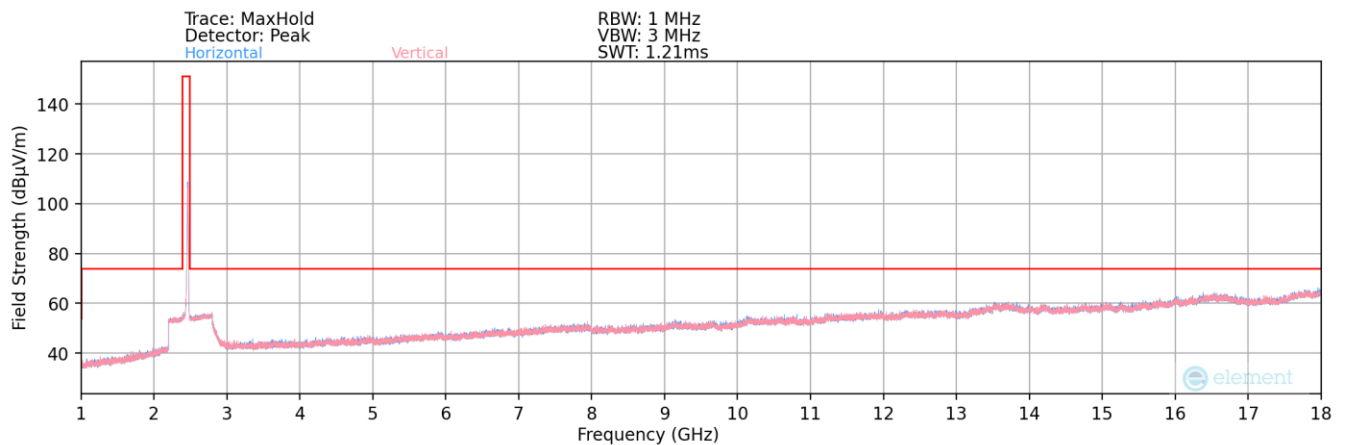
Plot 7-112. Radiated Spurious Plot above 1GHz MIMO (802.11b – Ch. OFDM 11)
