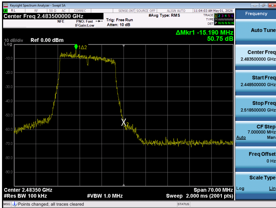
Plot 7-81. Band Edge Plot MIMO ANT1 (802.11n/ac – Ch. 13)
