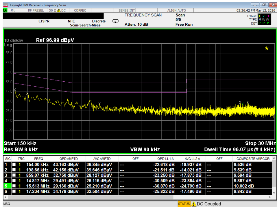
Plot 7-121. Line Conducted Plot with 802.11b (N) - WCP
