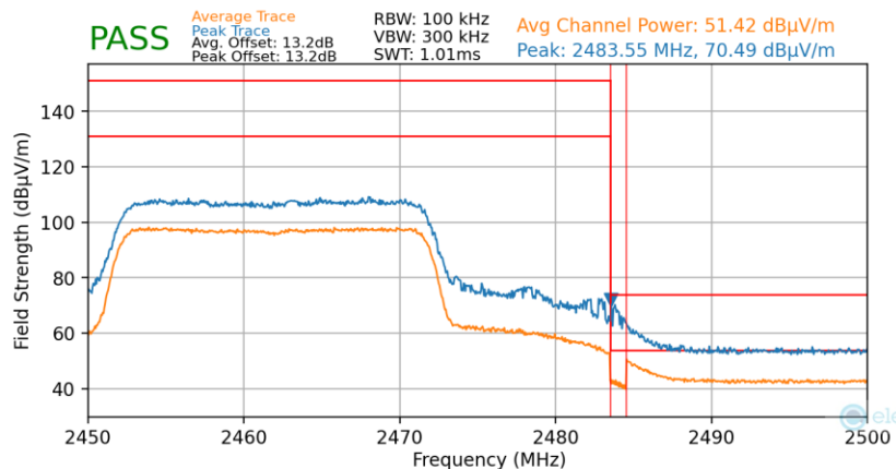
Plot 7-117. Radiated Restricted Upper Band Edge Measurement MIMO (Average & Peak) – with WCP
