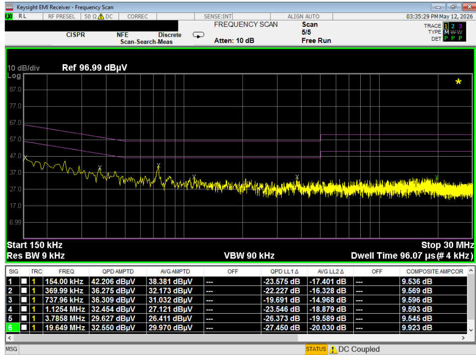
Plot 7-120. Line Conducted Plot with 802.11b (L1) - WCP
