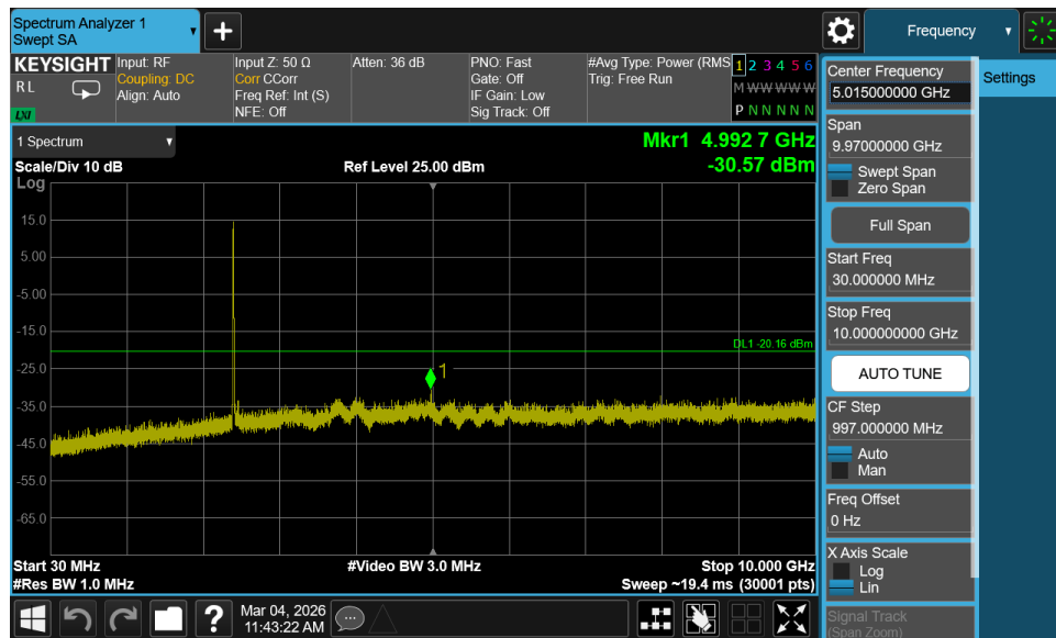
Plot 7-103. Conducted Spurious Plot MIMO ANT2 (802.11b – Ch. 1)
