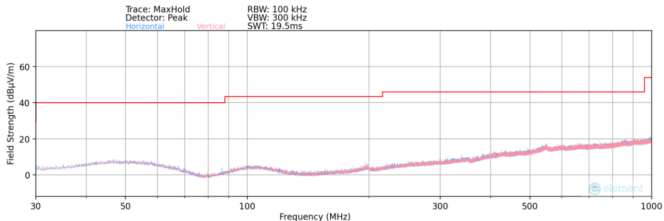
Plot 7-109. Radiated Spurious Plot below 1GHz MIMO
