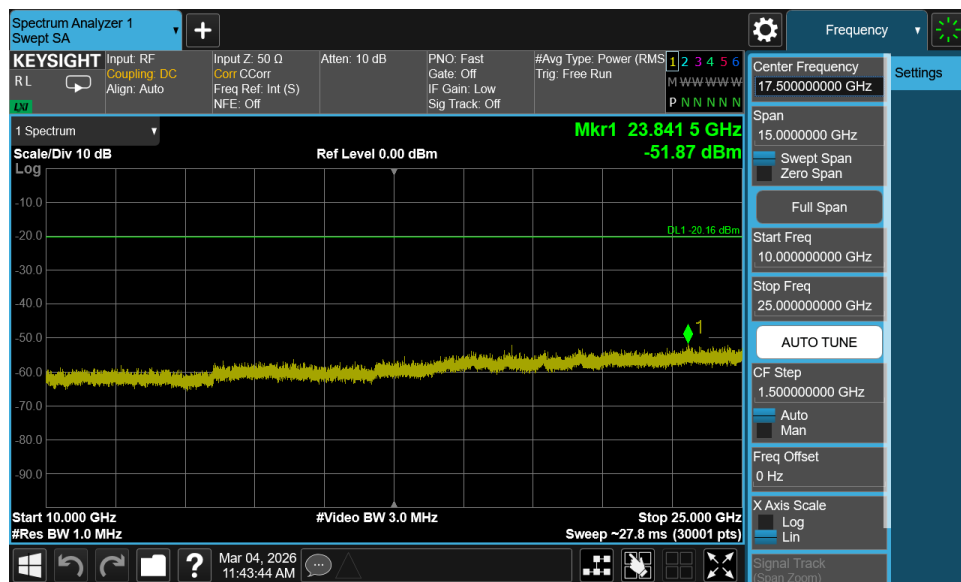
Plot 7-104. Conducted Spurious Plot MIMO ANT2 (802.11b – Ch. 1)
