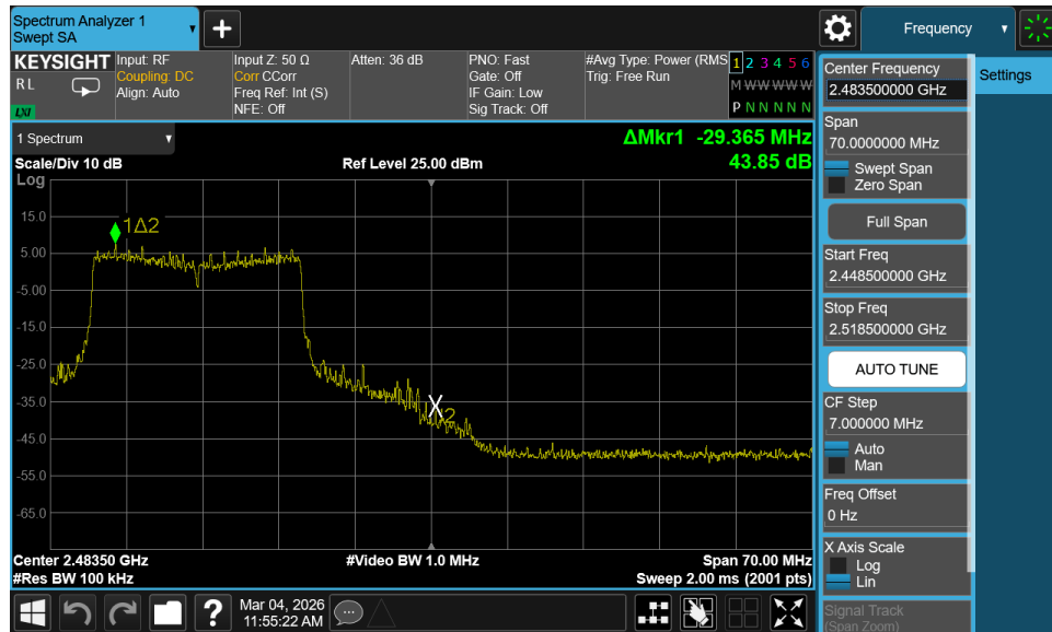
Plot 7-95. Band Edge Plot MIMO ANT2 (802.11ax/be – Ch. 11)
