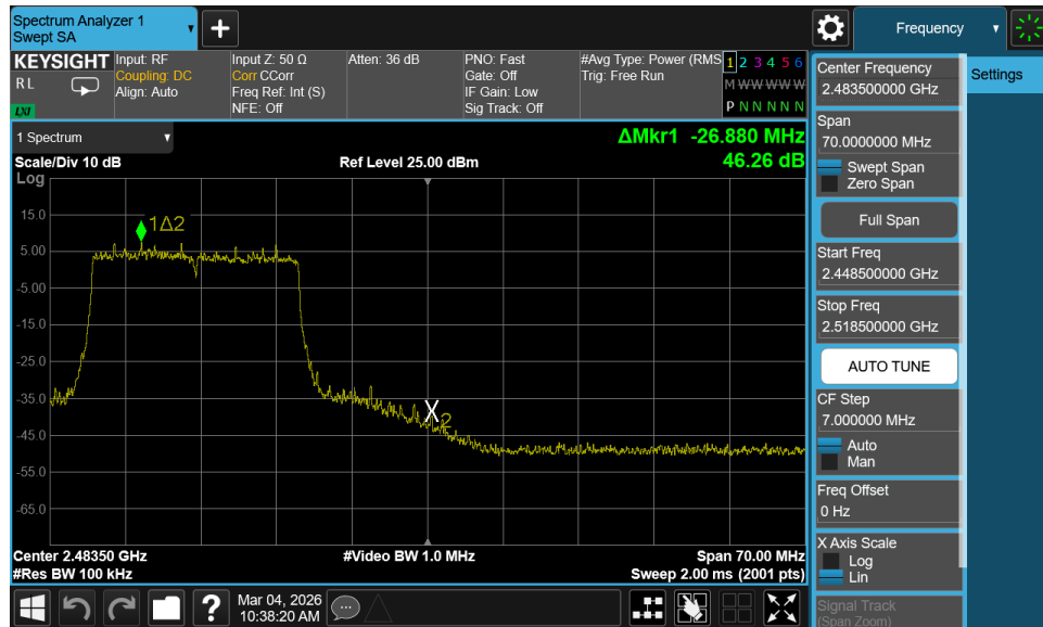
Plot 7-83. Band Edge Plot MIMO ANT1 (802.11ax/be – Ch. 11)
