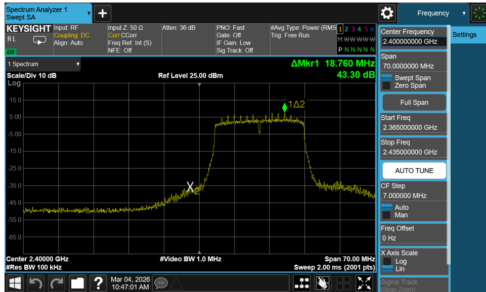
Plot 7-79. Band Edge Plot MIMO ANT1 (802.11n/ac – Ch. 1)
