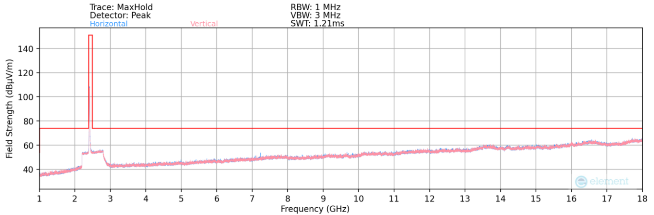
Plot 7-110. Radiated Spurious Plot above 1GHz MIMO (802.11b – Ch. OFDM 1)
