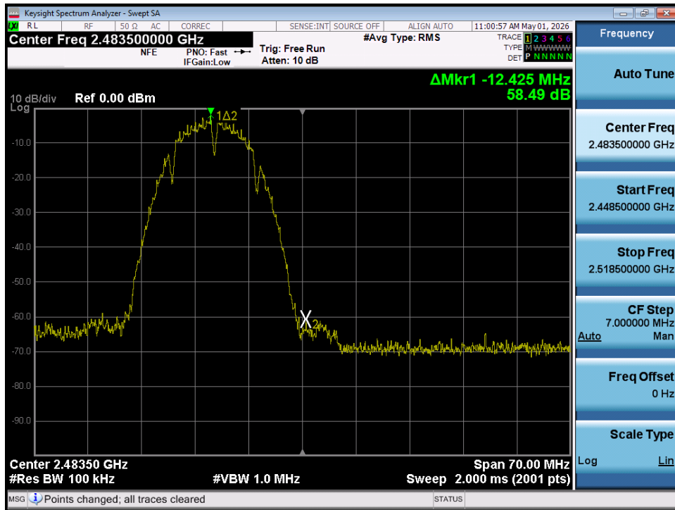
Plot 7-75. Band Edge Plot MIMO ANT1 (802.11b – Ch. 13)
