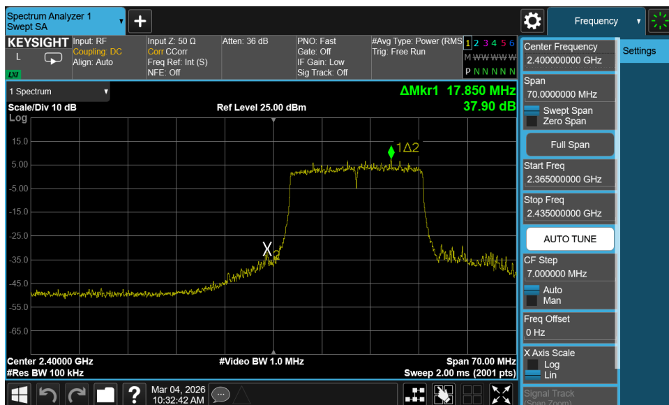
Plot 7-82. Band Edge Plot MIMO ANT1 (802.11ax/be – Ch. 1)
