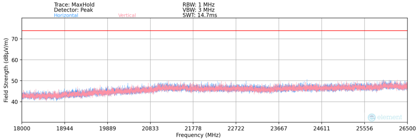
Plot 7-113. Radiated Spurious Plot above 18GHz MIMO
