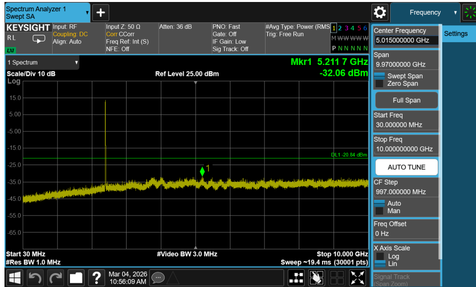
Plot 7-97. Conducted Spurious Plot MIMO ANT1 (802.11b – Ch. 1)
