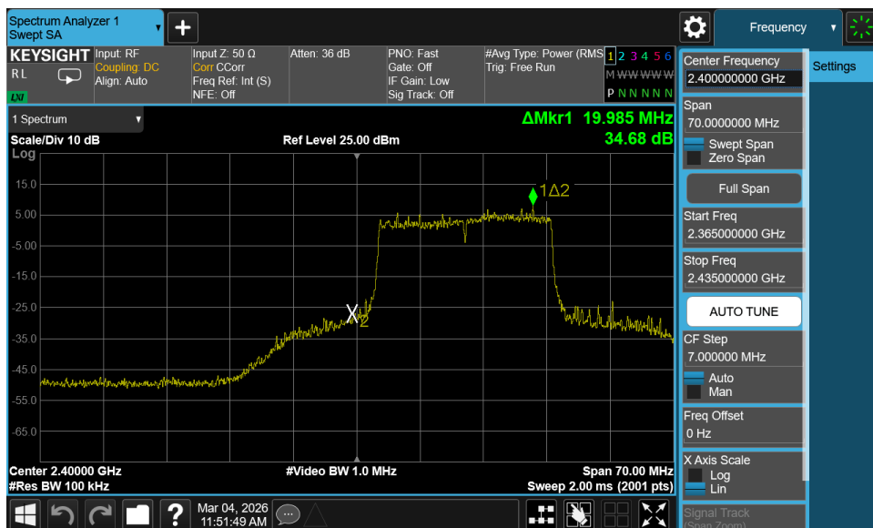
Plot 7-94. Band Edge Plot MIMO ANT2 (802.11ax/be – Ch. 1)
