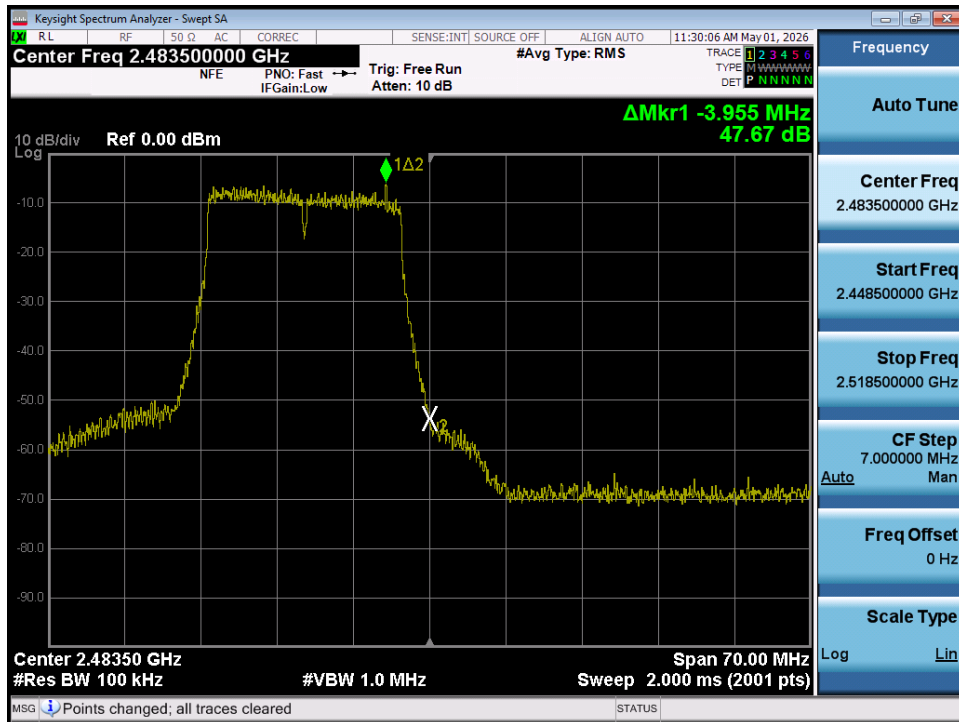
Plot 7-93. Band Edge Plot MIMO ANT2 (802.11n/ac – Ch. 13)
