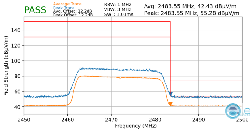
Plot 7-116. Radiated Restricted Upper Band Edge Measurement MIMO (Average & Peak)
