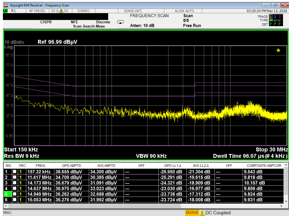
Plot 7-119. Line Conducted Plot with 802.11b (N)
