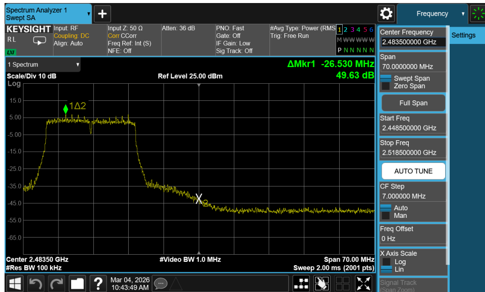
Plot 7-80. Band Edge Plot MIMO ANT1 (802.11n/ac – Ch. 11)
