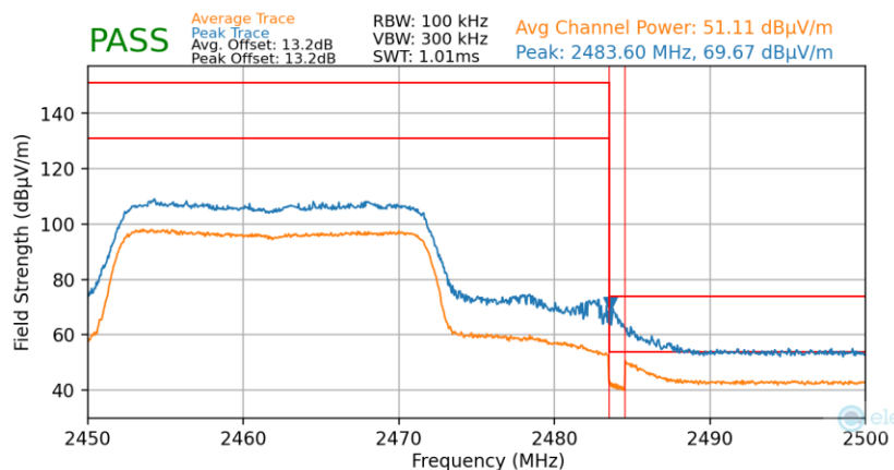
Plot 7-115. Radiated Restricted Upper Band Edge Measurement MIMO (Average & Peak)
