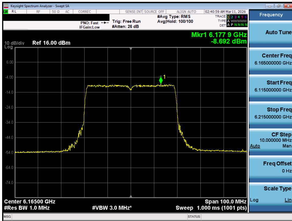
Plot 7-39. Power Spectral Density Plot MIMO ANT1 (40MHz 802.11ax/be (Full Tones) (UNII Band 5) – Ch. 43) - VLP
