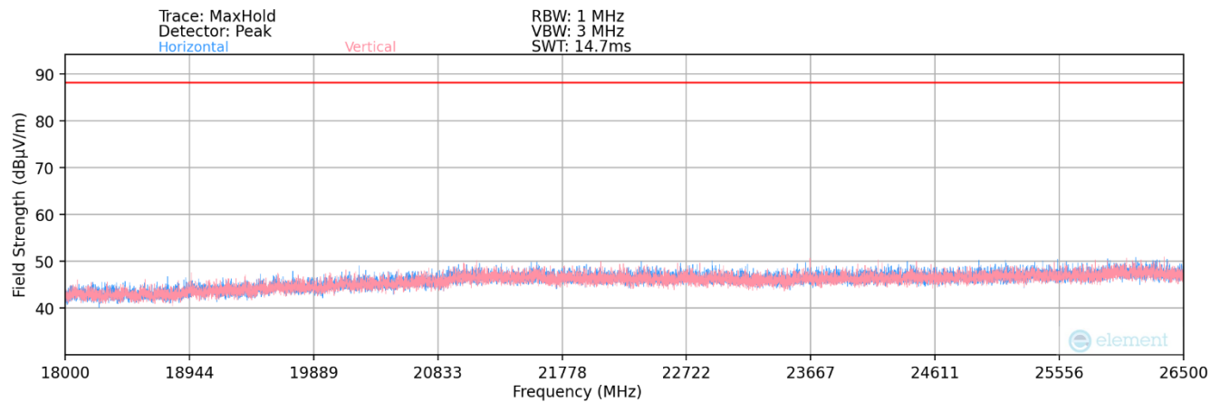
Plot 7-89. Radiated Spurious Plot 18GHz - 26.5GHz (802.11ax) – Ch. 45
