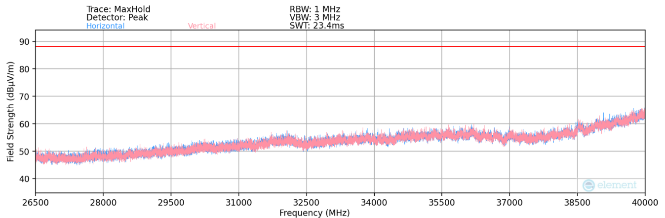
Plot 7-90. Radiated Spurious Plot 26.5GHz - 40GHz (802.11ax) – Ch. 45
