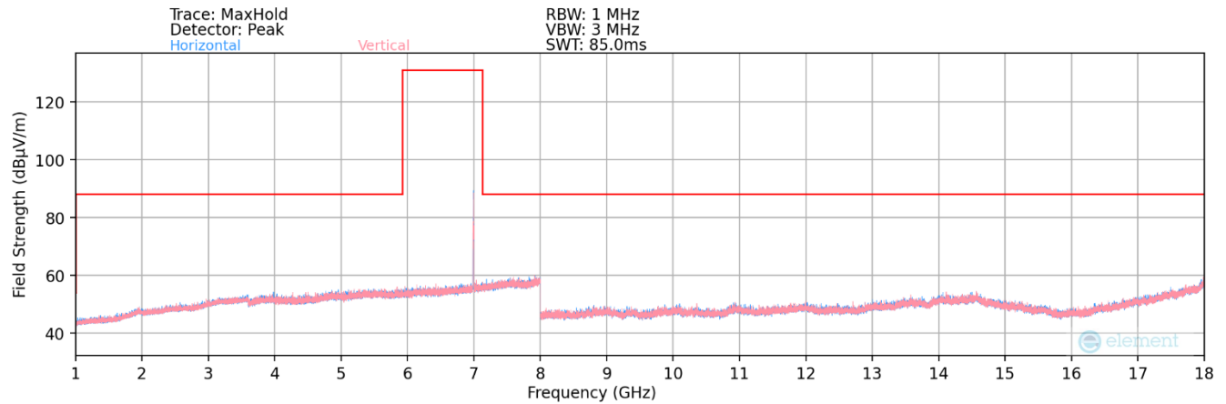
Plot 7-88. Radiated Spurious Plot 1GHz – 18GHz MIMO (802.11ax – UNII Band 8 Ch. 209)
