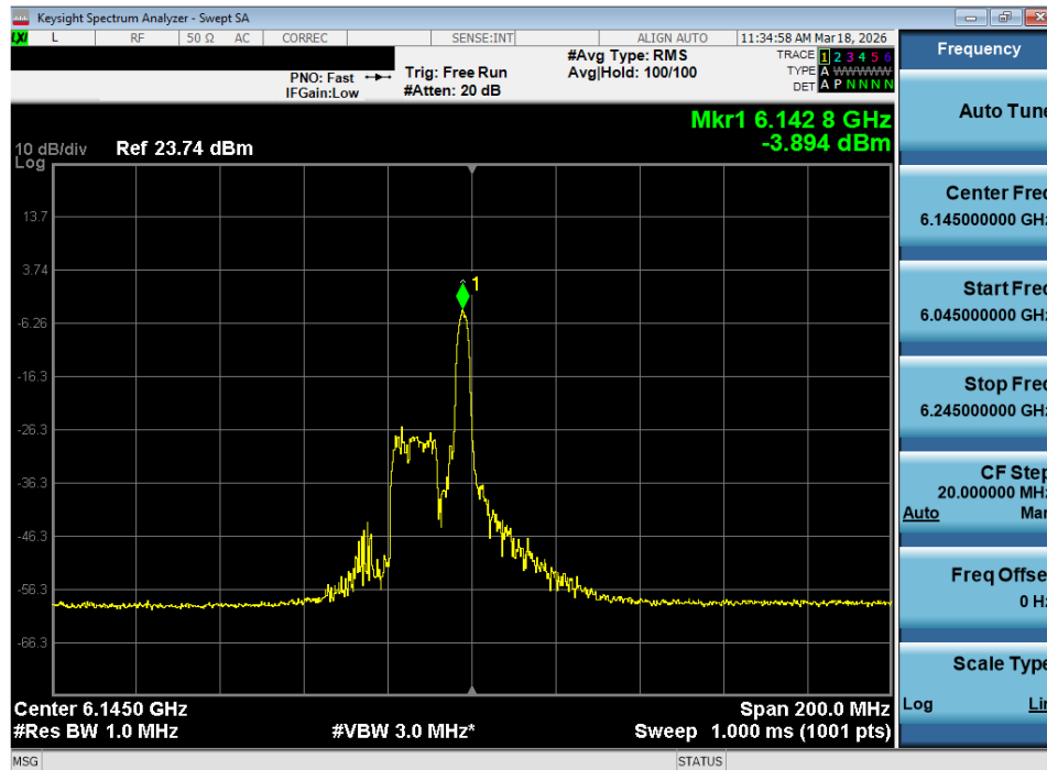
Plot 7-72. Power Spectral Density Plot MIMO ANT2 (80MHz 802.11ax/be (26 Tones) (UNII Band 5) – Ch. 39) - LPI
