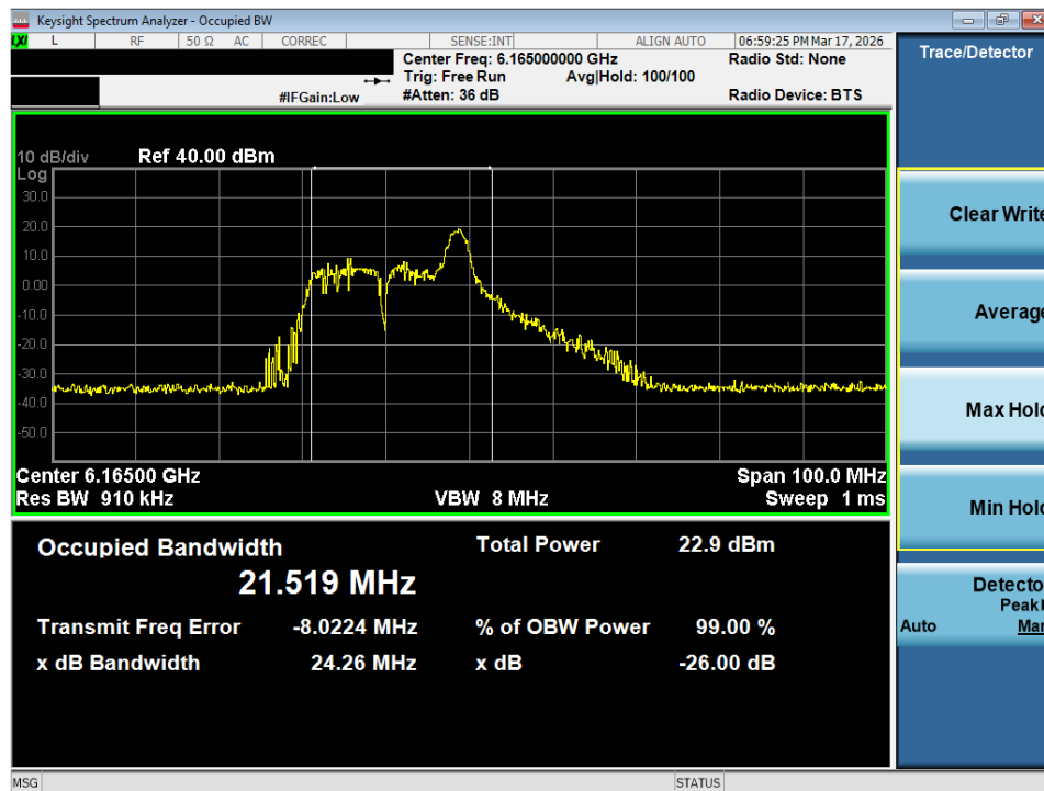
Plot 7-34. 26dB Bandwidth Plot MIMO ANT2 (40MHz 802.11ax/be (26 Tones) (UNII Band 5) – Ch. 43) - SP
