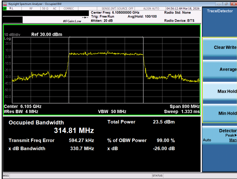
Plot 7-21. 26dB Bandwidth Plot MIMO ANT1 (320MHz 802.11be (Full Tones) (UNII Band 5) – Ch. 31) - LPI/SP
