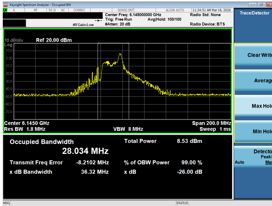
Plot 7-26. 26dB Bandwidth Plot MIMO ANT2 (80MHz 802.11ax/be (26 Tones) (UNII Band 5) – Ch. 39) - LPI
