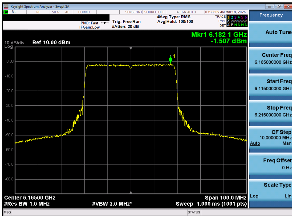
Plot 7-64. Power Spectral Density Plot MIMO ANT1 (40MHz 802.11ax/be (Full Tones) (UNII Band 5) – Ch. 43) - LPI
