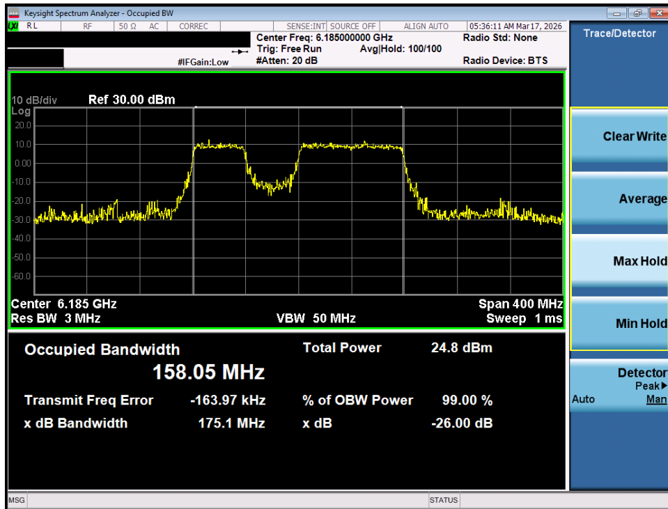
Plot 7-8. 26dB Bandwidth Plot MIMO ANT1 (160MHz 802.11be (996+484 Tones) (UNII Band 5) – Ch. 47) - LPI/SP
