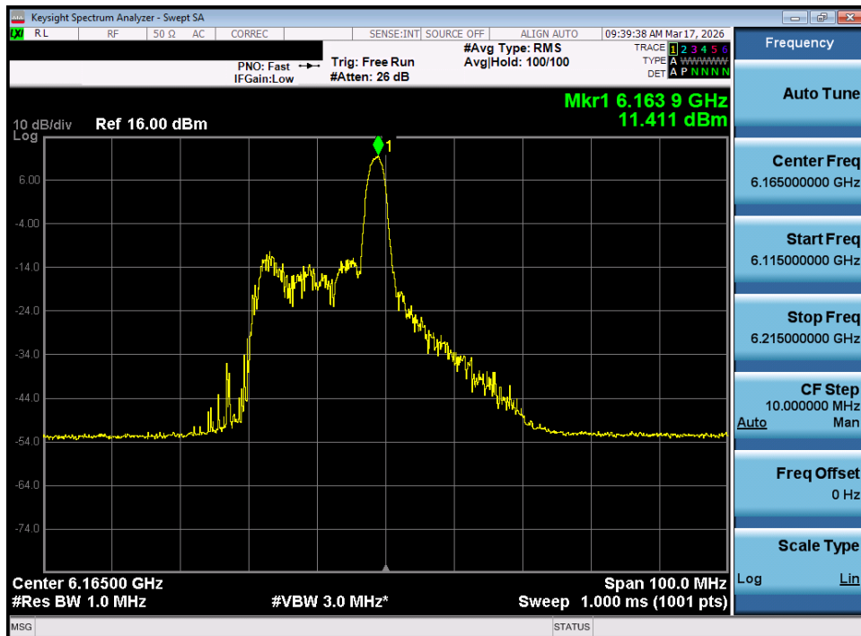
Plot 7-57. Power Spectral Density Plot MIMO ANT1 (40MHz 802.11ax/be (26 Tones) (UNII Band 5) – Ch. 43) - SP
