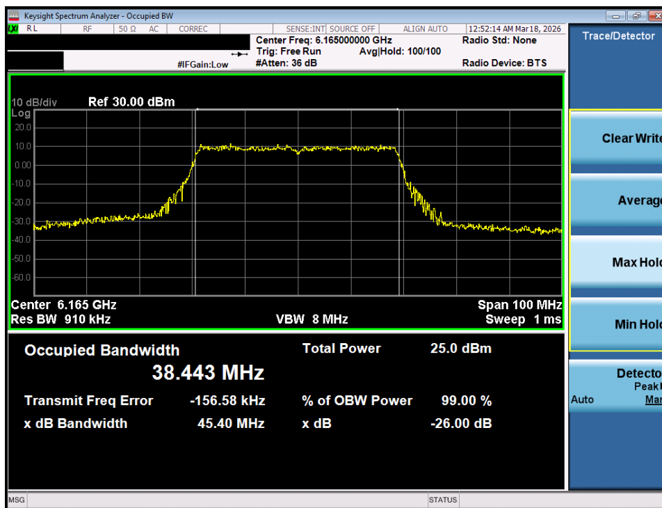
Plot 7-23. 26dB Bandwidth Plot MIMO ANT1 (40MHz 802.11ax/be (Full Tones) (UNII Band 5) – Ch. 43) – SP
