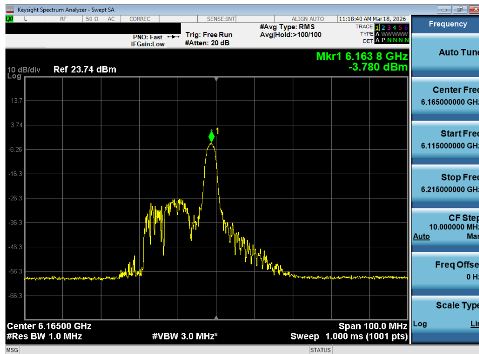
Plot 7-71. Power Spectral Density Plot MIMO ANT2 (40MHz 802.11ax/be (26 Tones) (UNII Band 5) – Ch. 43) - LPI
