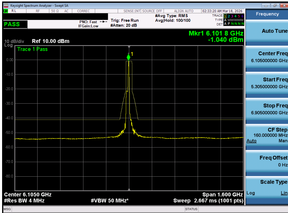
Plot 7-97. In Band Emissions Plot MIMO ANT1 (320MHz 802.11be (26 Tones) (UNII Band 5) – Ch. 31) - LPI
