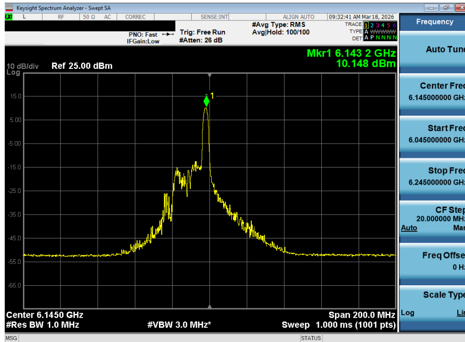
Plot 7-81. Power Spectral Density Plot MIMO ANT2 (80MHz 802.11ax/be (26 Tones) (UNII Band 5) – Ch. 39) - SP
