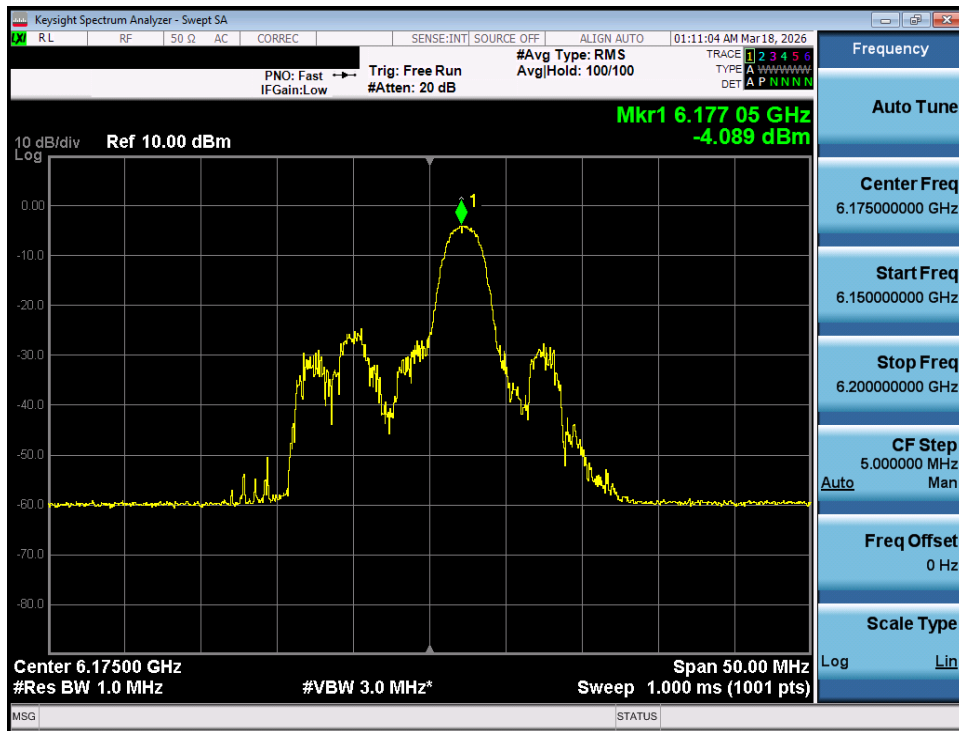
Plot 7-47. Power Spectral Density Plot MIMO ANT1 (20MHz 802.11ax/be (26 Tones) (UNII Band 5) – Ch. 45) - LPI
