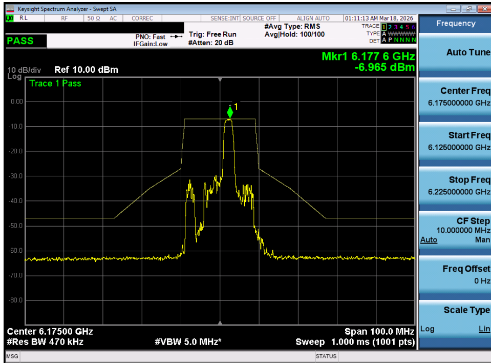
Plot 7-93. In Band Emissions Plot MIMO ANT1 (20MHz 802.11ax/be (26 Tones) (UNII Band 5) – Ch. 45) - LPI
