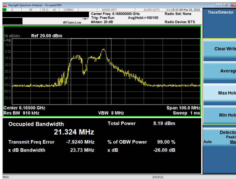
Plot 7-25. 26dB Bandwidth Plot MIMO ANT2 (40MHz 802.11ax/be (26 Tones) (UNII Band 5) – Ch. 43) - LPI
