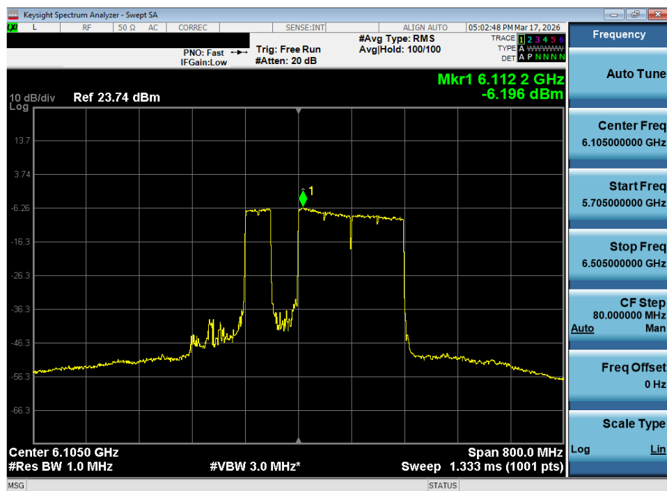
Plot 7-78. Power Spectral Density Plot MIMO ANT2 (320MHz 802.11be (2x996+484 Tones) (UNII Band 5) – Ch. 31) - LPI/SP
