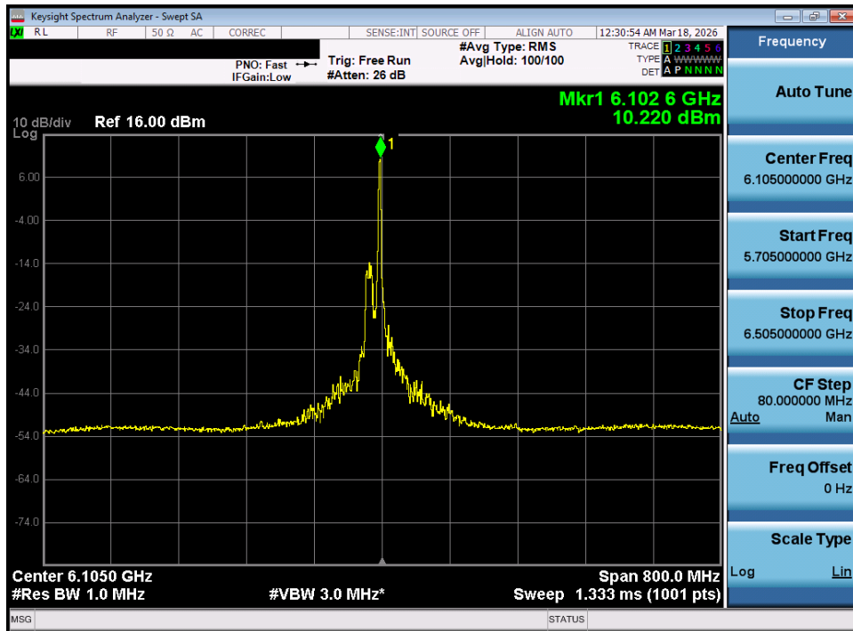
Plot 7-60. Power Spectral Density Plot MIMO ANT1 (320MHz 802.11be (26 Tones) (UNII Band 5) – Ch. 31) - SP
