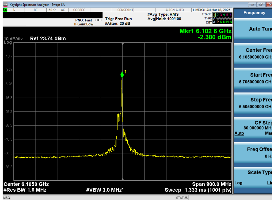
Plot 7-74. Power Spectral Density Plot MIMO ANT2 (320MHz 802.11be (26 Tones) (UNII Band 5) – Ch. 31) - LPI
