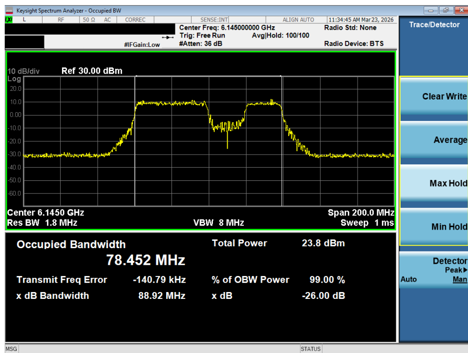
Plot 7-39. 26dB Bandwidth Plot MIMO ANT2 (80MHz 802.11be (484+242 Tones) (UNII Band 5) – Ch. 39) - SP
