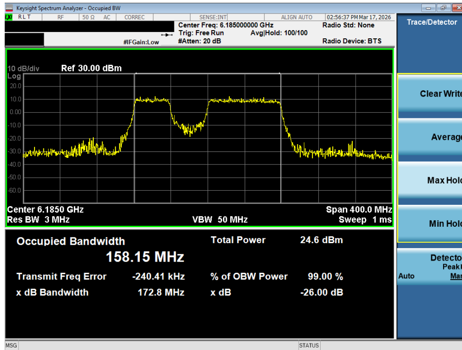
Plot 7-31. 26dB Bandwidth Plot MIMO ANT2 (160MHz 802.11be (996+484 Tones) (UNII Band 5) – Ch. 47) – LPI/SP
