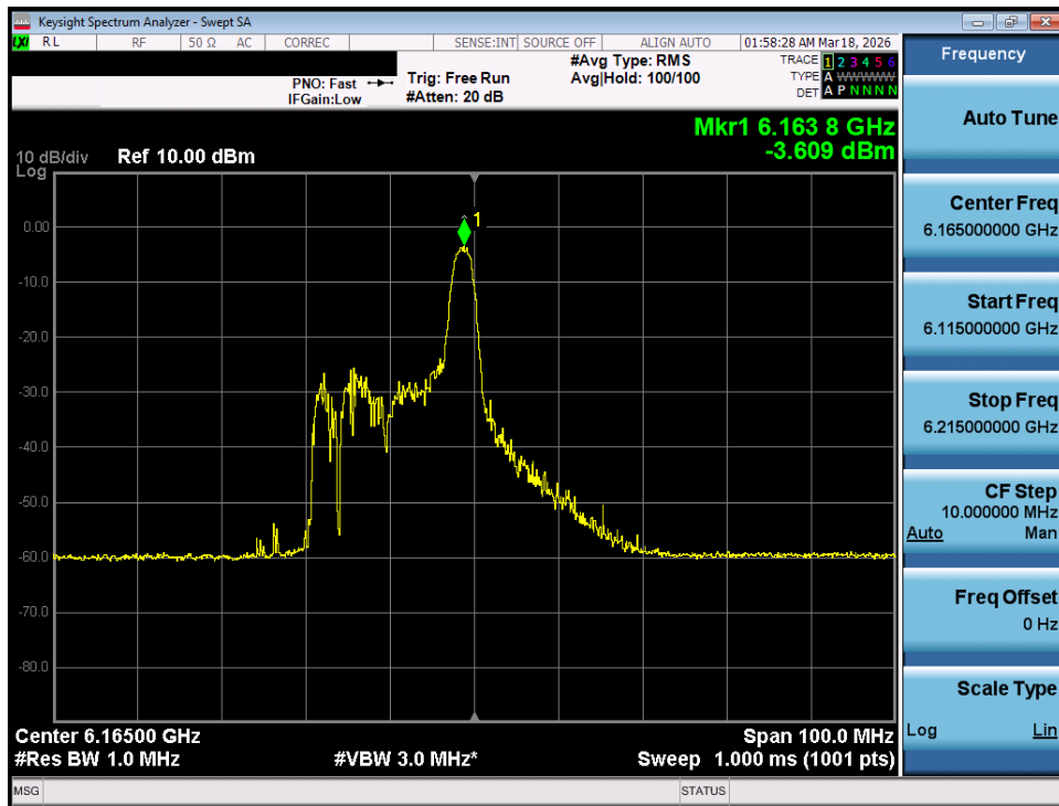
Plot 7-48. Power Spectral Density Plot MIMO ANT1 (40MHz 802.11ax/be (26 Tones) (UNII Band 5) – Ch. 43) - LPI
