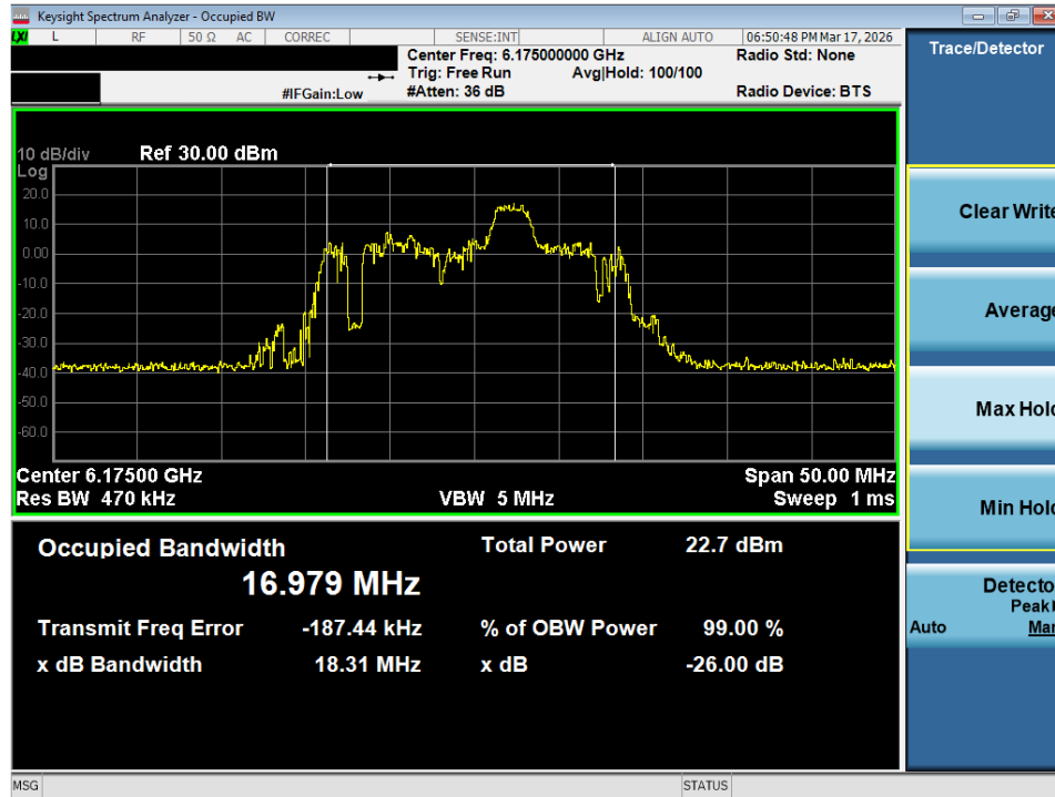
Plot 7-33. 26dB Bandwidth Plot MIMO ANT2 (20MHz 802.11ax/be (26 Tones) (UNII Band 5) – Ch. 45) - SP
