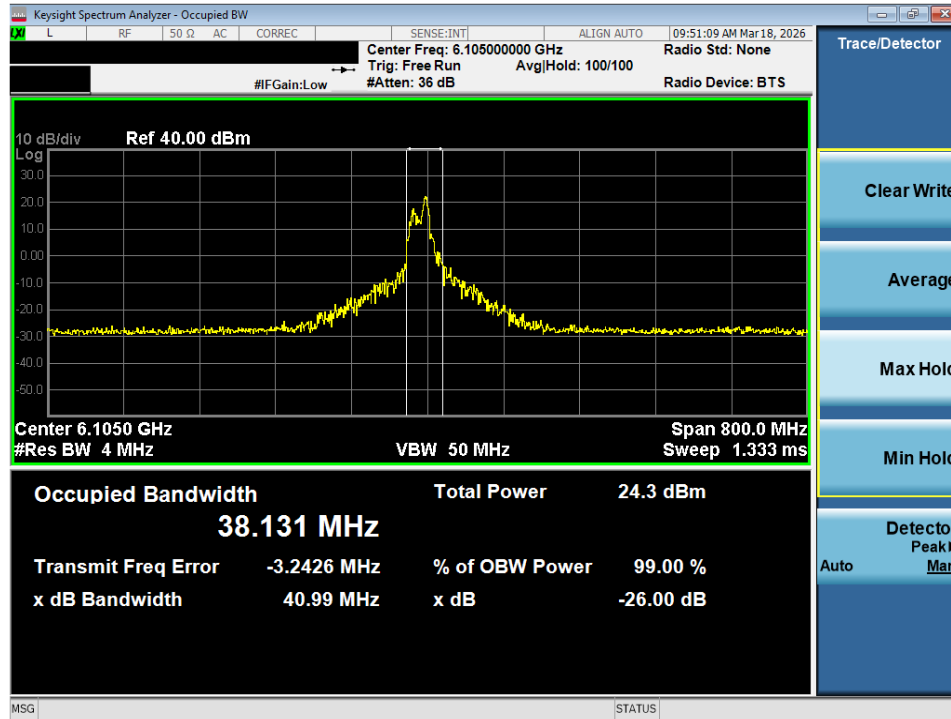
Plot 7-37. 26dB Bandwidth Plot MIMO ANT2 (320MHz 802.11be (26 Tones) (UNII Band 5) – Ch. 31) - SP
