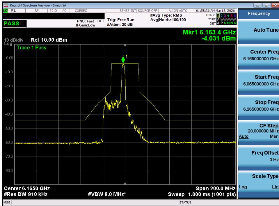
Plot 7-94. In Band Emissions Plot MIMO ANT1 (40MHz 802.11ax/be (26 Tones) (UNII Band 5) – Ch. 43) - LPI
