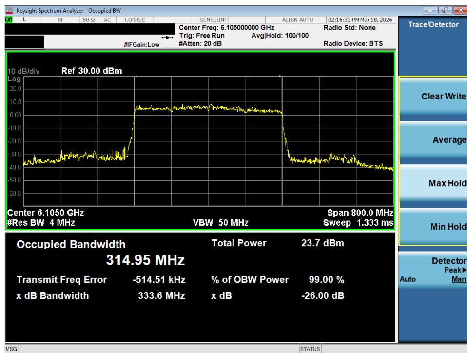
Plot 7-44. 26dB Bandwidth Plot MIMO ANT2 (320MHz 802.11be (Full Tones) (UNII Band 5) – Ch. 31) - LPI/SP
