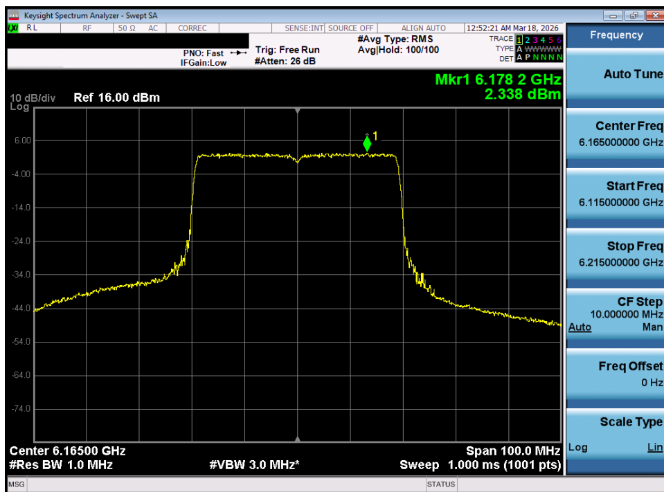
Plot 7-69. Power Spectral Density Plot MIMO ANT1 (40MHz 802.11ax/be (Full Tones) (UNII Band 5) – Ch. 43) – SP
