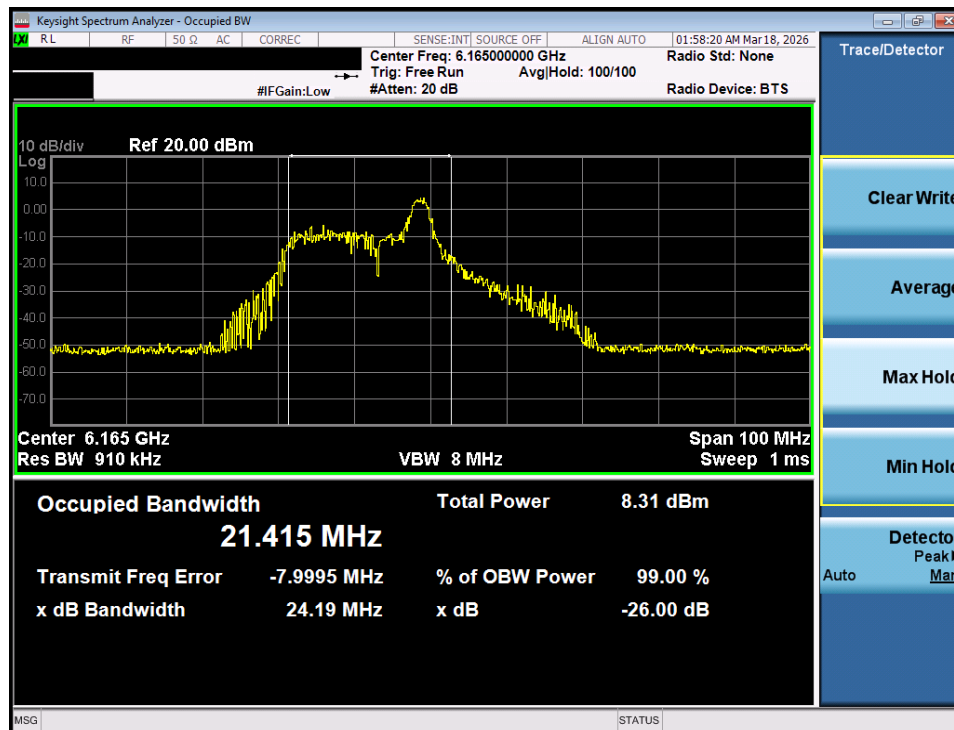
Plot 7-2. 26dB Bandwidth Plot MIMO ANT1 (40MHz 802.11ax/be (26 Tones) (UNII Band 5) – Ch. 43) - LPI
