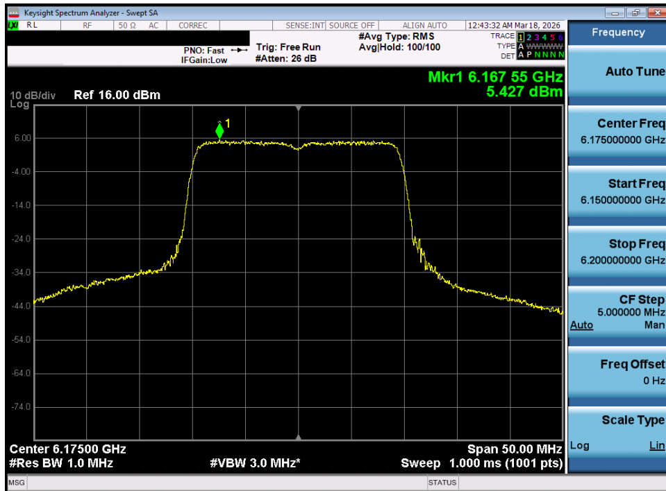
Plot 7-68. Power Spectral Density Plot MIMO ANT1 (20MHz 802.11ax/be (Full Tones) (UNII Band 5) – Ch. 45) - SP
