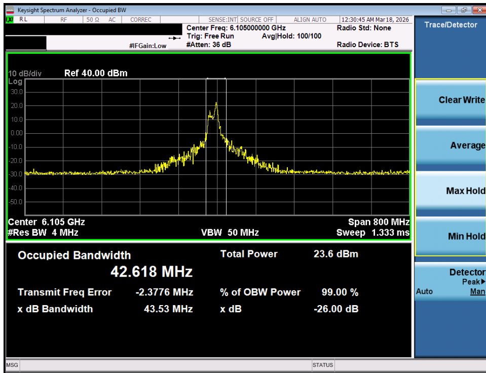
Plot 7-14. 26dB Bandwidth Plot MIMO ANT1 (320MHz 802.11be (26 Tones) (UNII Band 5) – Ch. 31) - SP
