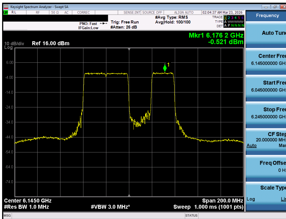
Plot 7-62. Power Spectral Density Plot MIMO ANT1 (80MHz 802.11be (484+242 Tones) (UNII Band 5) – Ch. 39) - SP
