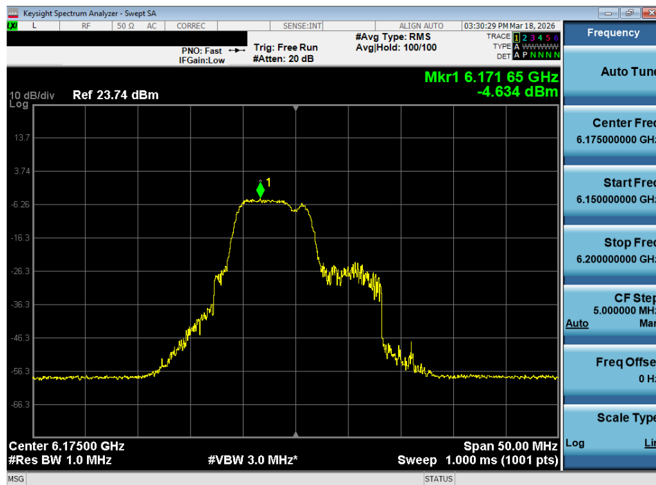
Plot 7-75. Power Spectral Density Plot MIMO ANT2 (20MHz 802.11be (52+26 Tones) (UNII Band 5) – Ch. 45) - LPI
