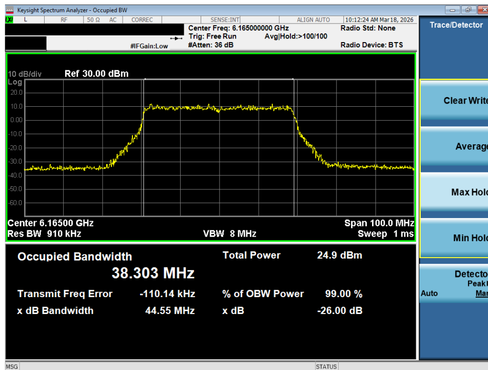
Plot 7-46. 26dB Bandwidth Plot MIMO ANT2 (40MHz 802.11ax/be (Full Tones) (UNII Band 5) – Ch. 43) - SP
