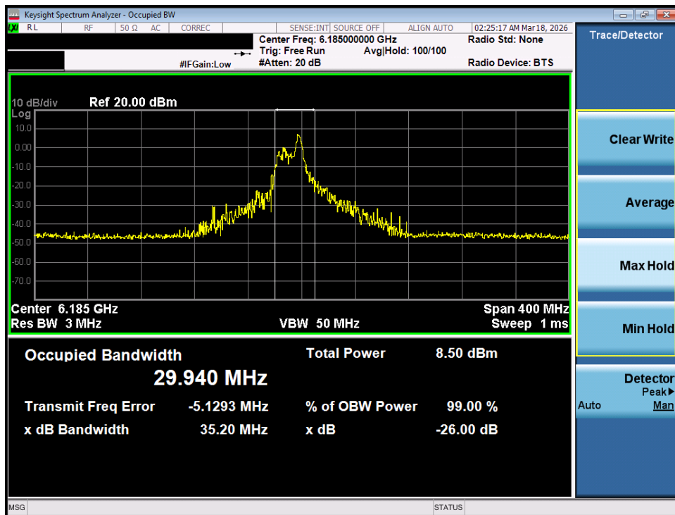
Plot 7-4. 26dB Bandwidth Plot MIMO ANT1 (160MHz 802.11ax/be (26 Tones) (UNII Band 5) – Ch. 47) - LPI
