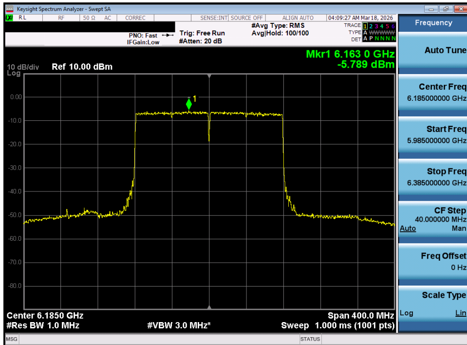
Plot 7-66. Power Spectral Density Plot MIMO ANT1 (160MHz 802.11ax/be (Full Tones) (UNII Band 5) – Ch. 47) - LPI/SP
