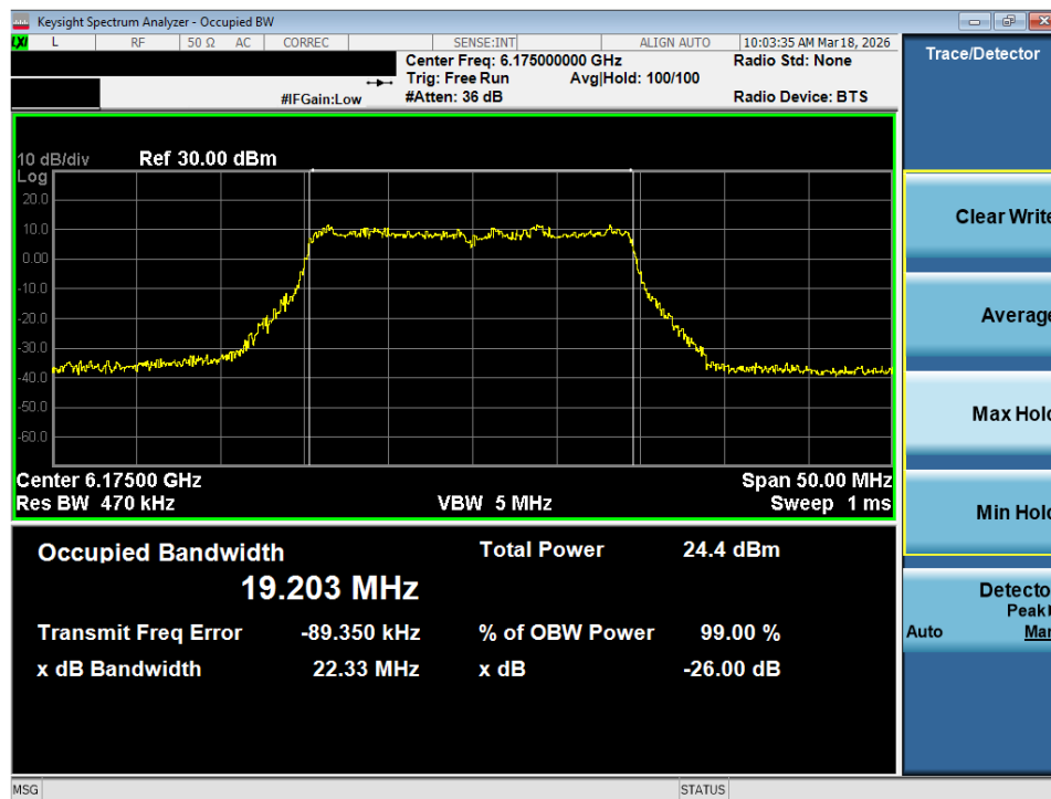
Plot 7-45. 26dB Bandwidth Plot MIMO ANT2 (20MHz 802.11ax/be (Full Tones) (UNII Band 5) – Ch. 45) - SP
