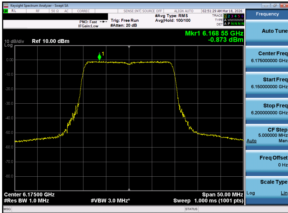
Plot 7-63. Power Spectral Density Plot MIMO ANT1 (20MHz 802.11ax/be (Full Tones) (UNII Band 5) – Ch. 45) - LPI
