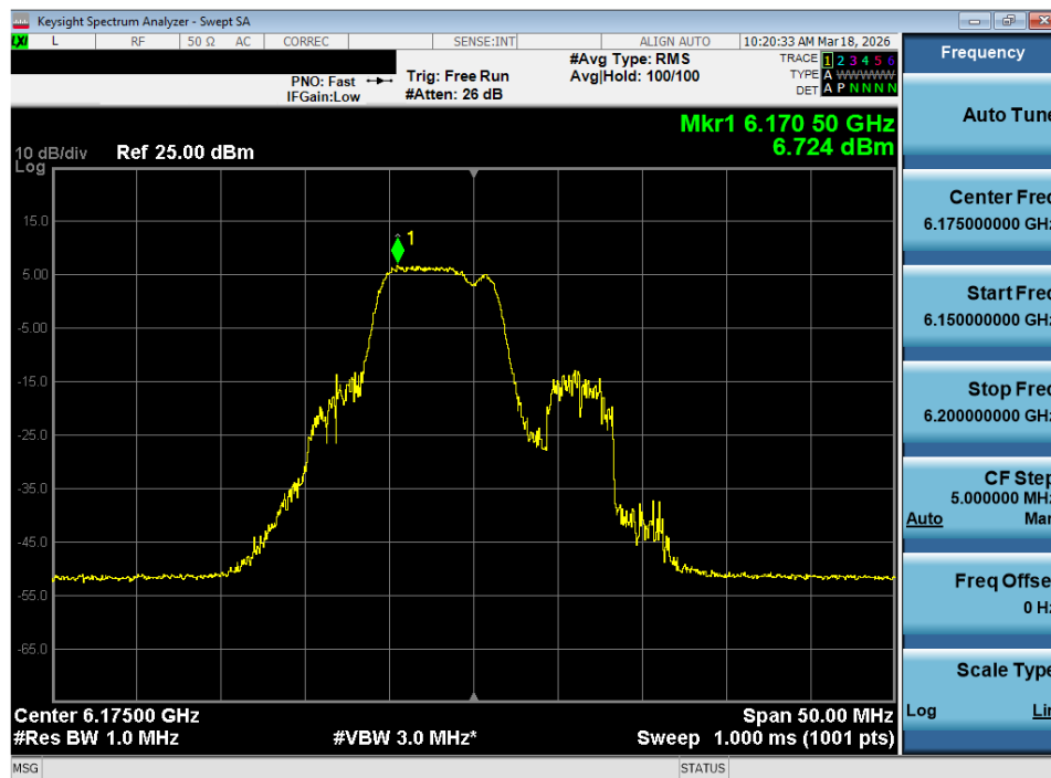
Plot 7-84. Power Spectral Density Plot MIMO ANT2 (20MHz 802.11be (52+26 Tones) (UNII Band 5) – Ch. 45) – SP
