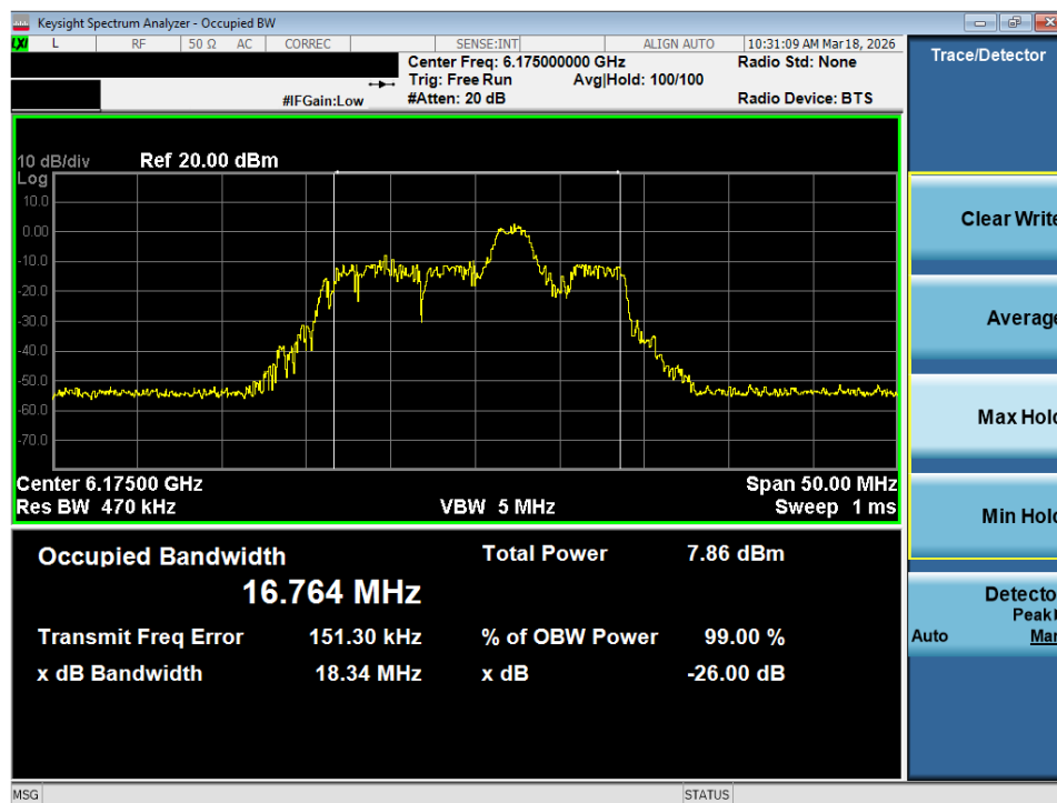
Plot 7-24. 26dB Bandwidth Plot MIMO ANT2 (20MHz 802.11ax/be (26 Tones) (UNII Band 5) – Ch. 45) - LPI
