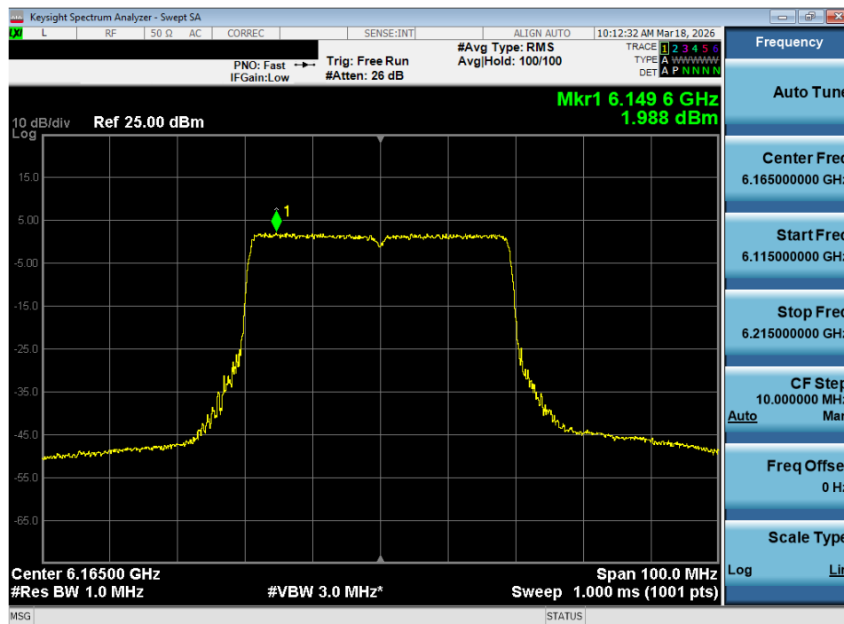
Plot 7-92. Power Spectral Density Plot MIMO ANT2 (40MHz 802.11ax/be (Full Tones) (UNII Band 5) – Ch. 43) - SP
