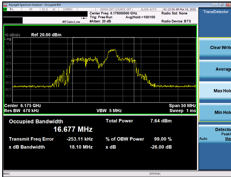
Plot 7-1. 26dB Bandwidth Plot MIMO ANT1 (20MHz 802.11ax/be (26 Tones) (UNII Band 5) – Ch. 45) - LPI
