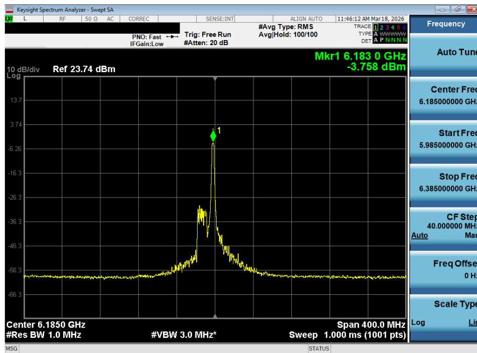
Plot 7-73. Power Spectral Density Plot MIMO ANT2 (160MHz 802.11ax/be (26 Tones) (UNII Band 5) – Ch. 47) - LPI
