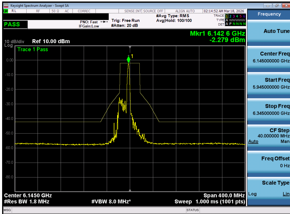
Plot 7-95. In Band Emissions Plot MIMO ANT1 (80MHz 802.11ax/be (26 Tones) (UNII Band 5) – Ch. 39) - LPI
