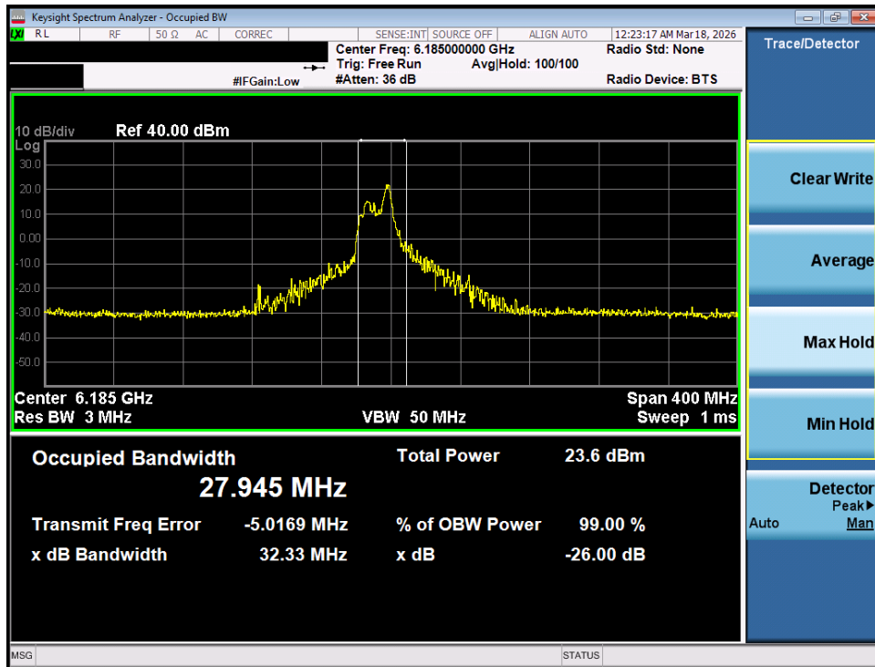
Plot 7-13. 26dB Bandwidth Plot MIMO ANT1 (160MHz 802.11ax/be (26 Tones) (UNII Band 5) – Ch. 47) - SP
