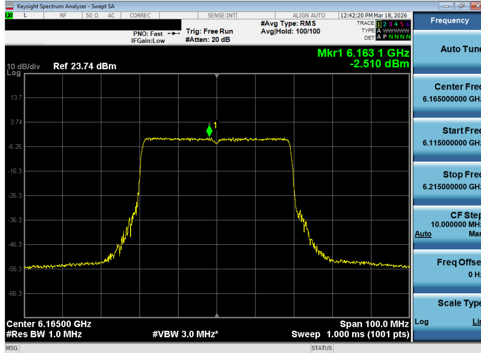
Plot 7-87. Power Spectral Density Plot MIMO ANT2 (40MHz 802.11ax/be (Full Tones) (UNII Band 5) – Ch. 43) - LPI
