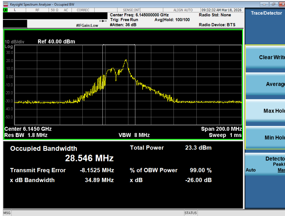
Plot 7-35. 26dB Bandwidth Plot MIMO ANT2 (80MHz 802.11ax/be (26 Tones) (UNII Band 5) – Ch. 39) - SP
