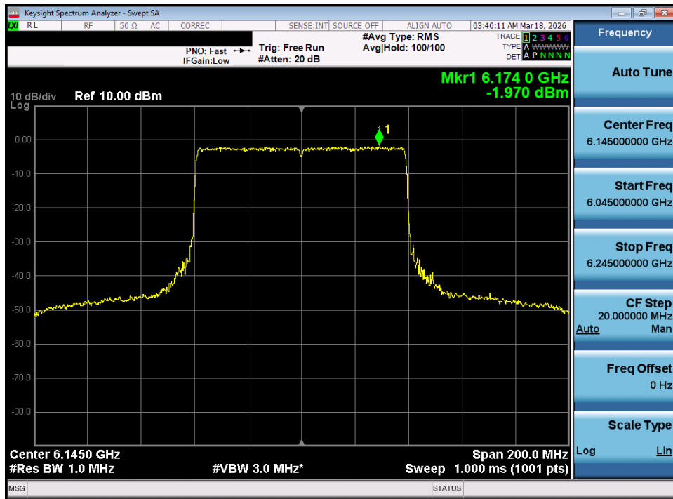
Plot 7-65. Power Spectral Density Plot MIMO ANT1 (80MHz 802.11ax/be (Full Tones) (UNII Band 5) – Ch. 39) - LPI/SP
