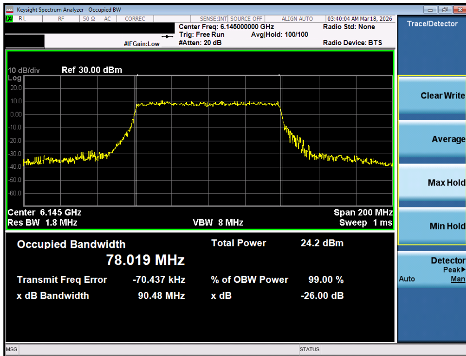
Plot 7-19. 26dB Bandwidth Plot MIMO ANT1 (80MHz 802.11ax/be (Full Tones) (UNII Band 5) – Ch. 39) - LPI/SP
