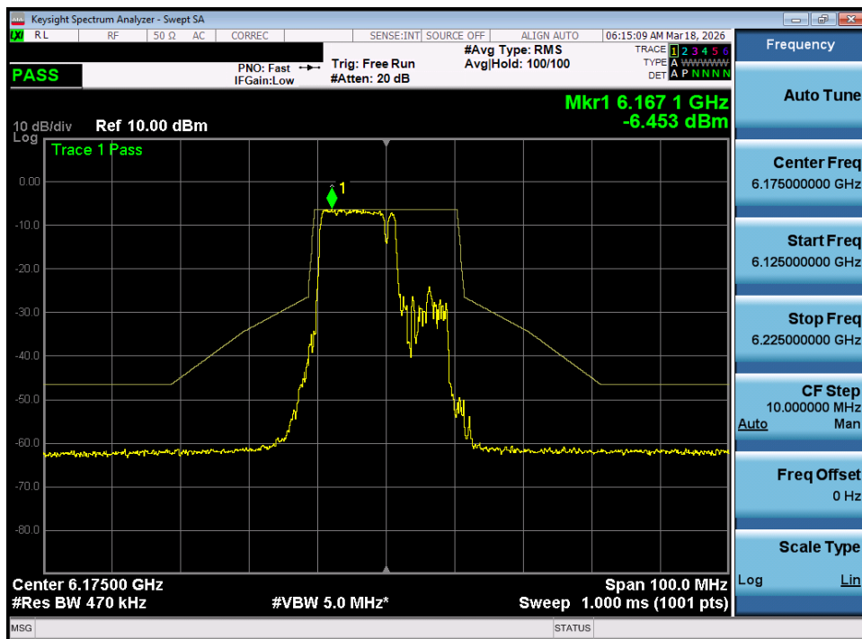
Plot 7-98. In Band Emissions Plot MIMO ANT1 (20MHz 802.11be (106+26 Tones) (UNII Band 5) – Ch. 45) - LPI
