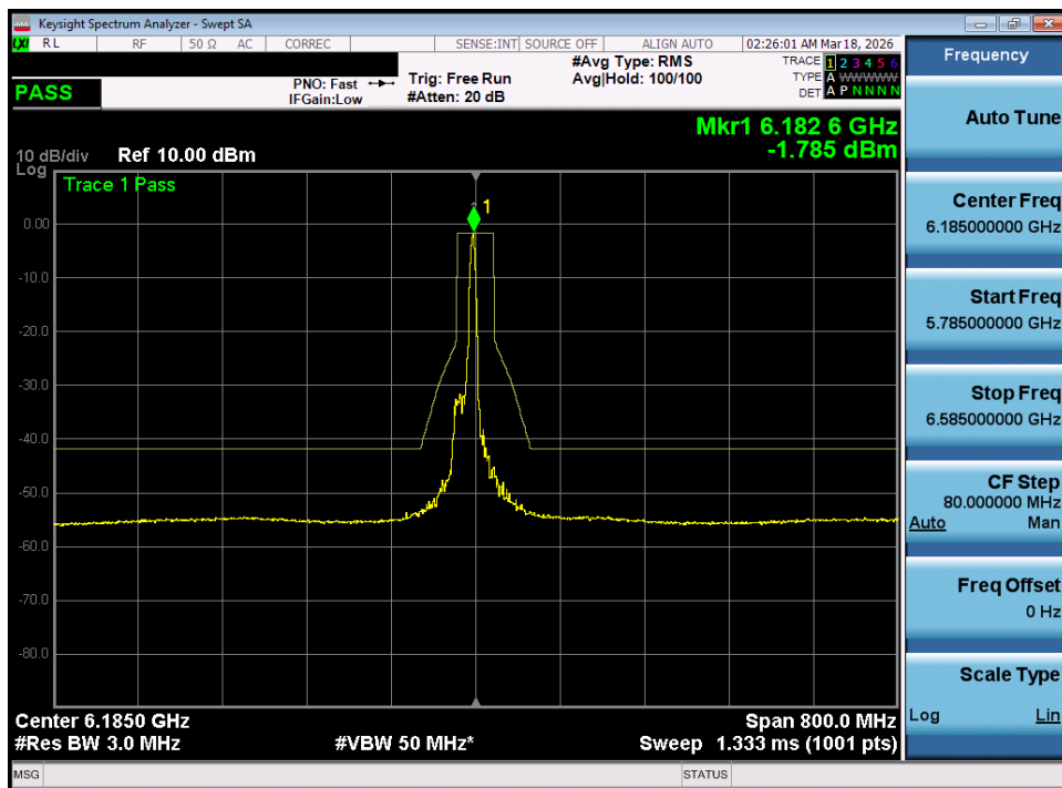
Plot 7-96. In Band Emissions Plot MIMO ANT1 (160MHz 802.11ax/be (26 Tones) (UNII Band 5) – Ch. 47) - LPI
