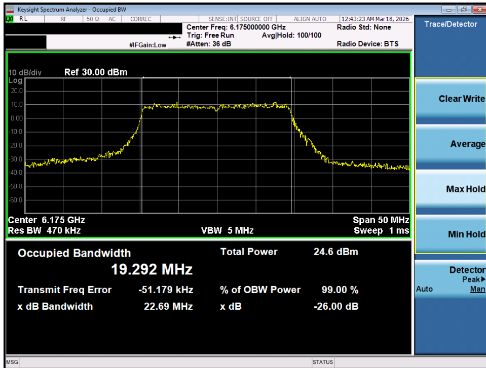
Plot 7-22. 26dB Bandwidth Plot MIMO ANT1 (20MHz 802.11ax/be (Full Tones) (UNII Band 5) – Ch. 45) - SP
