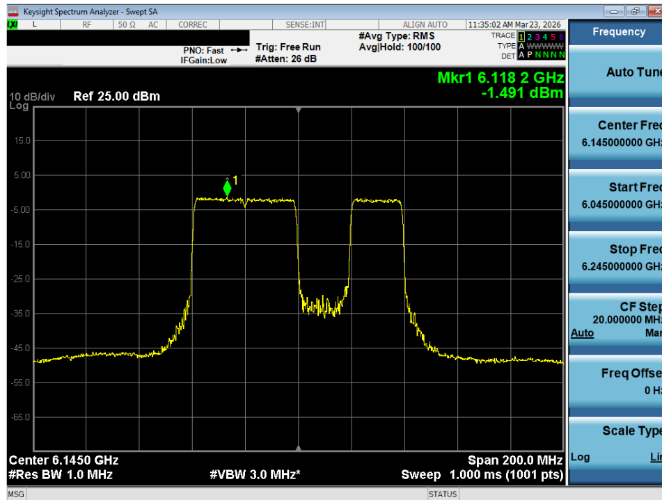
Plot 7-85. Power Spectral Density Plot MIMO ANT2 (80MHz 802.11be (484+242 Tones) (UNII Band 5) – Ch. 39) - SP
