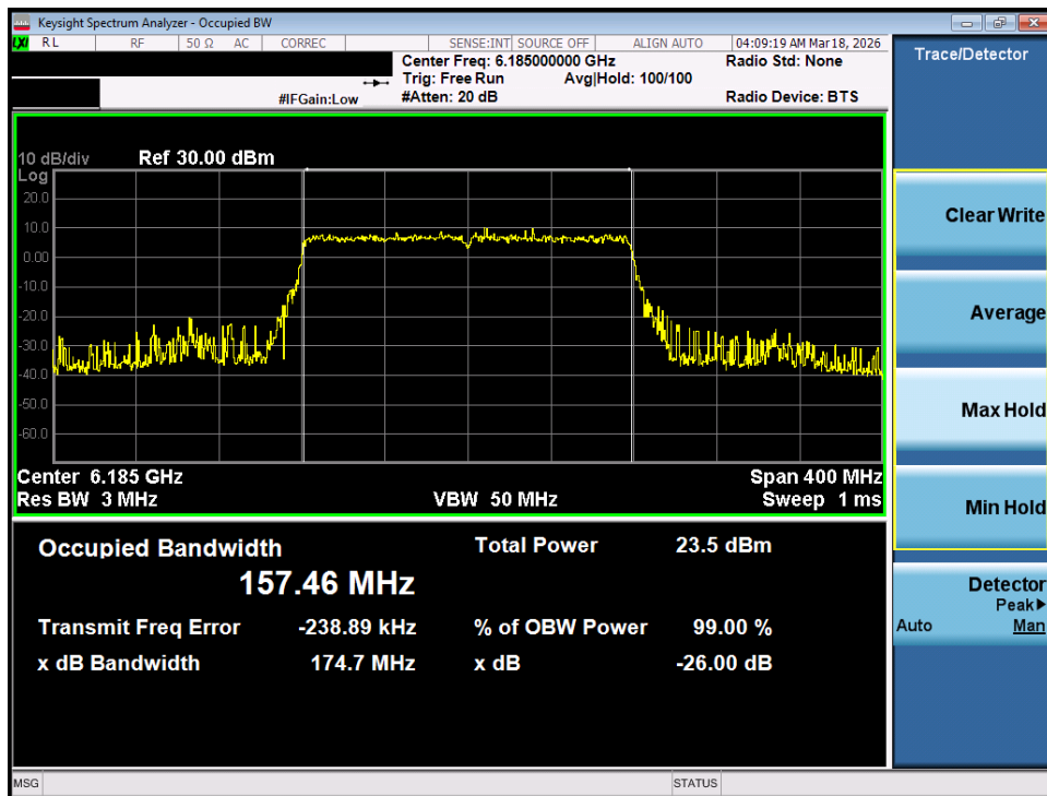
Plot 7-20. 26dB Bandwidth Plot MIMO ANT1 (160MHz 802.11ax/be (Full Tones) (UNII Band 5) – Ch. 47) - LPI/SP
