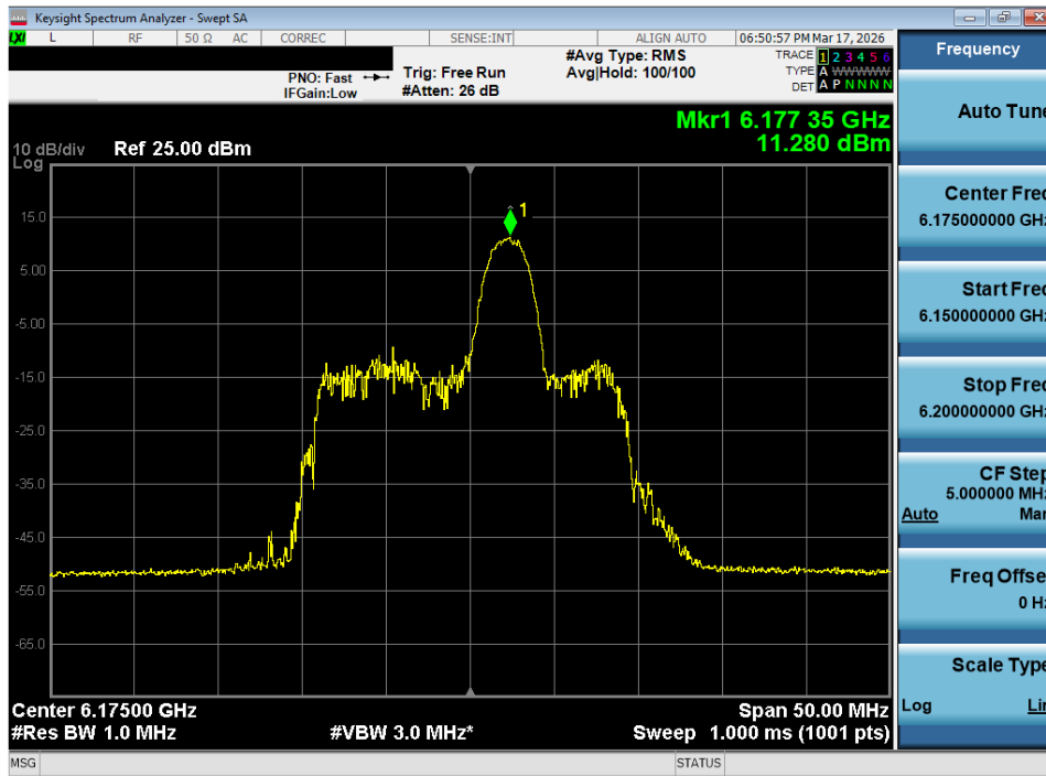
Plot 7-79. Power Spectral Density Plot MIMO ANT2 (20MHz 802.11ax/be (26 Tones) (UNII Band 5) – Ch. 45) - SP
