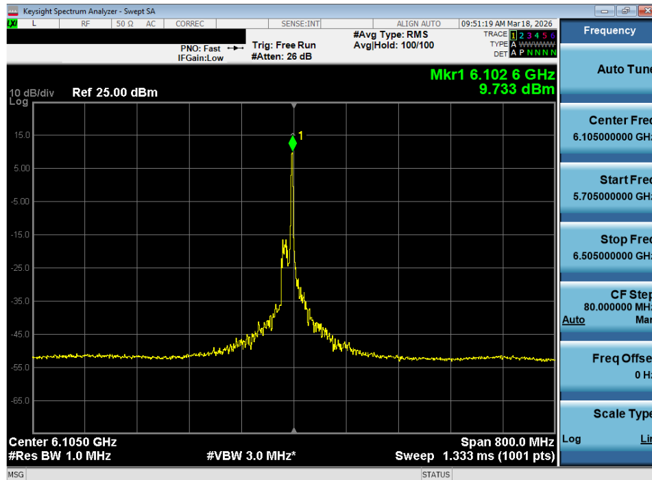
Plot 7-83. Power Spectral Density Plot MIMO ANT2 (320MHz 802.11be (26 Tones) (UNII Band 5) – Ch. 31) - SP
