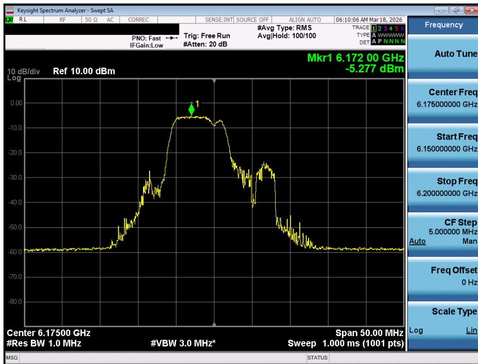
Plot 7-52. Power Spectral Density Plot MIMO ANT1 (20MHz 802.11be (52+26 Tones) (UNII Band 5) – Ch. 45) - LPI
