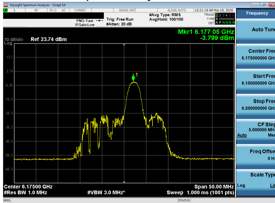
Plot 7-70. Power Spectral Density Plot MIMO ANT2 (20MHz 802.11ax/be (26 Tones) (UNII Band 5) – Ch. 45) - LPI
