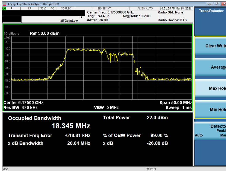
Plot 7-38. 26dB Bandwidth Plot MIMO ANT2 (20MHz 802.11be (106+26 Tones) (UNII Band 5) – Ch. 45) – SP
