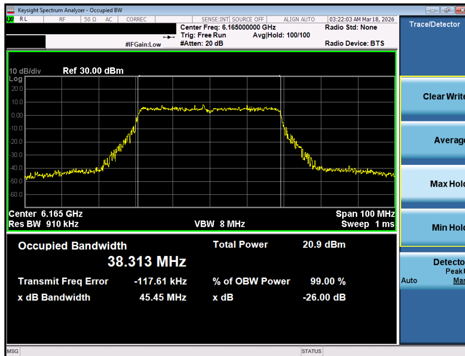
Plot 7-18. 26dB Bandwidth Plot MIMO ANT1 (40MHz 802.11ax/be (Full Tones) (UNII Band 5) – Ch. 43) - LPI
