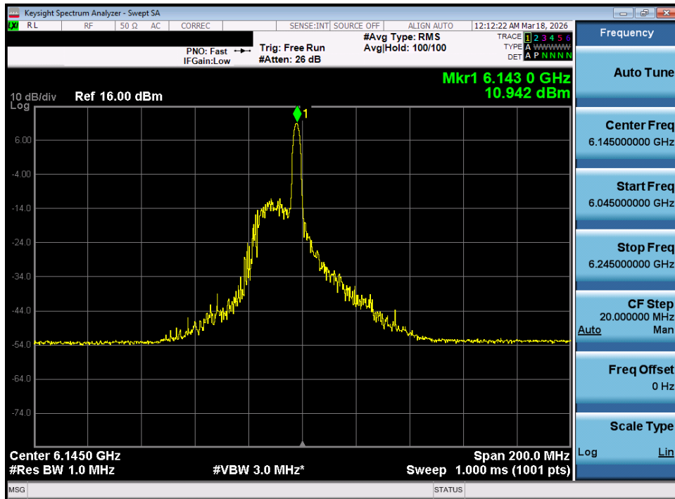
Plot 7-58. Power Spectral Density Plot MIMO ANT1 (80MHz 802.11ax/be (26 Tones) (UNII Band 5) – Ch. 39) - SP
