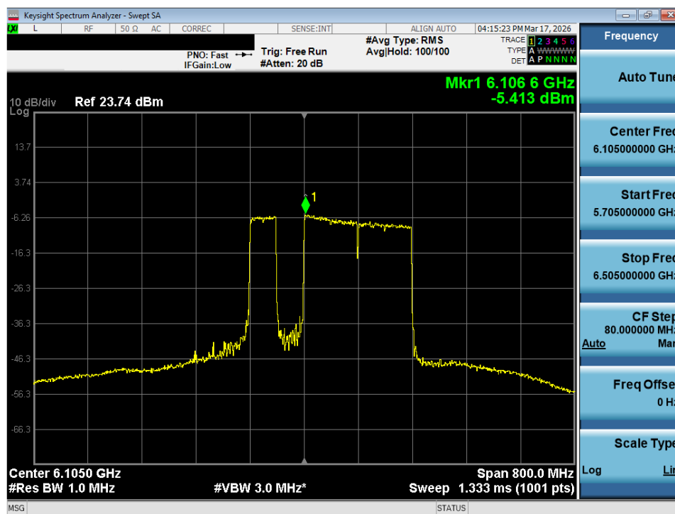
Plot 7-55. Power Spectral Density Plot MIMO ANT1 (320MHz 802.11be (2x996+484 Tones) (UNII Band 5) – Ch. 31) - LPI/SP
