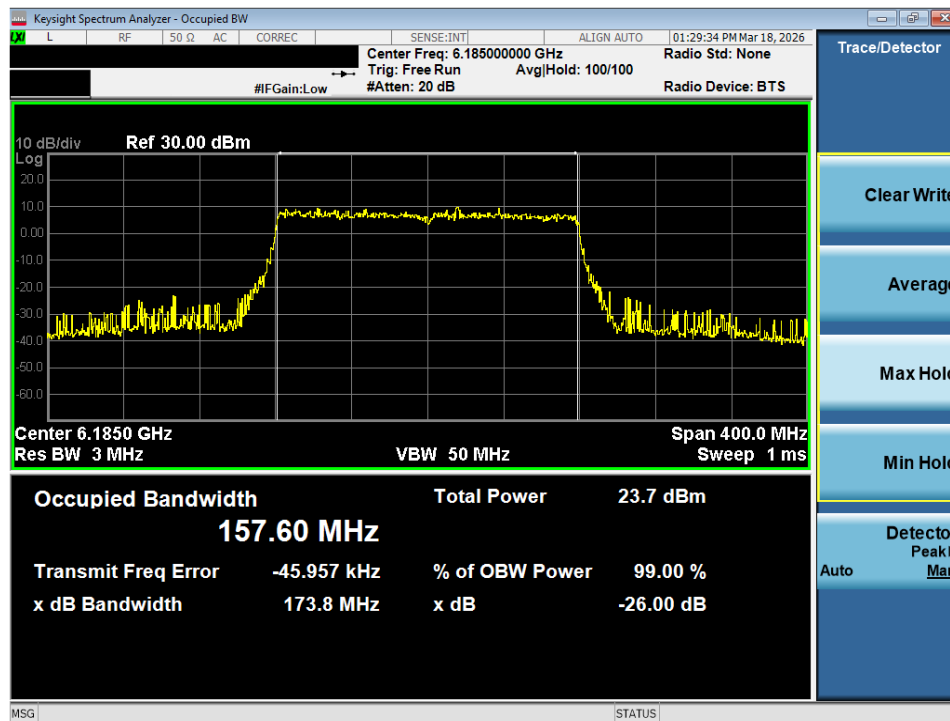
Plot 7-43. 26dB Bandwidth Plot MIMO ANT2 (160MHz 802.11ax/be (Full Tones) (UNII Band 5) – Ch. 47) - LPI/SP
