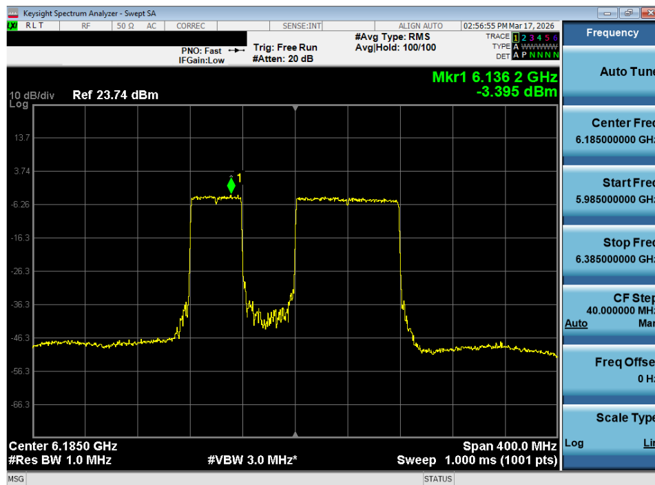
Plot 7-77. Power Spectral Density Plot MIMO ANT2 (160MHz 802.11be (996+484 Tones) (UNII Band 5) – Ch. 47) - LPI/SP
