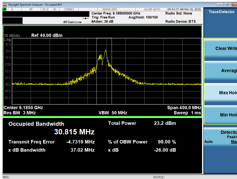
Plot 7-36. 26dB Bandwidth Plot MIMO ANT2 (160MHz 802.11ax/be (26 Tones) (UNII Band 5) – Ch. 47) - SP
