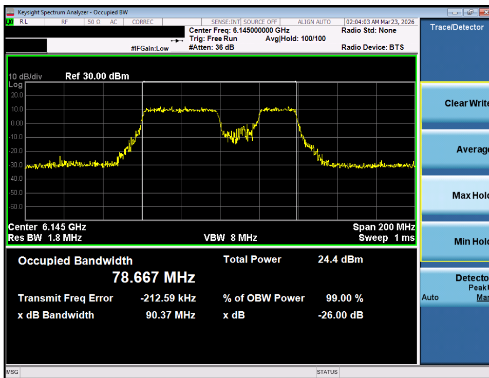
Plot 7-16. 26dB Bandwidth Plot MIMO ANT1 (80MHz 802.11be (484+242 Tones) (UNII Band 5) – Ch. 39) - SP
