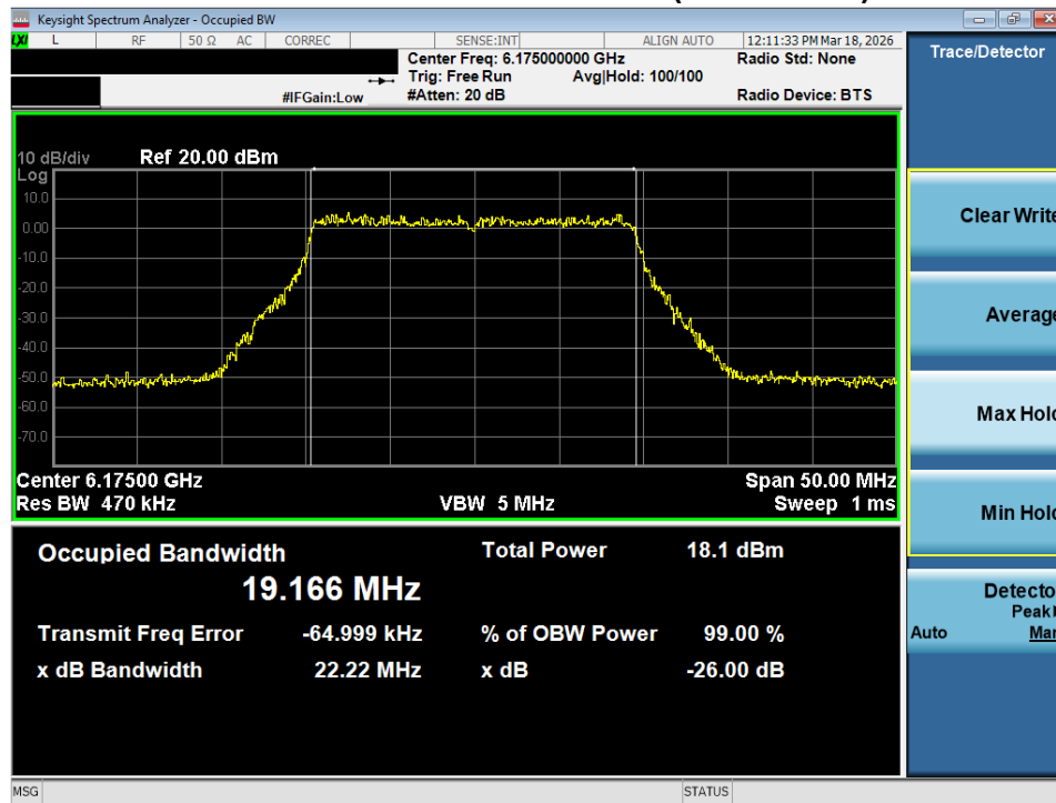
Plot 7-40. 26dB Bandwidth Plot MIMO ANT2 (20MHz 802.11ax/be (Full Tones) (UNII Band 5) – Ch. 45) - LPI
