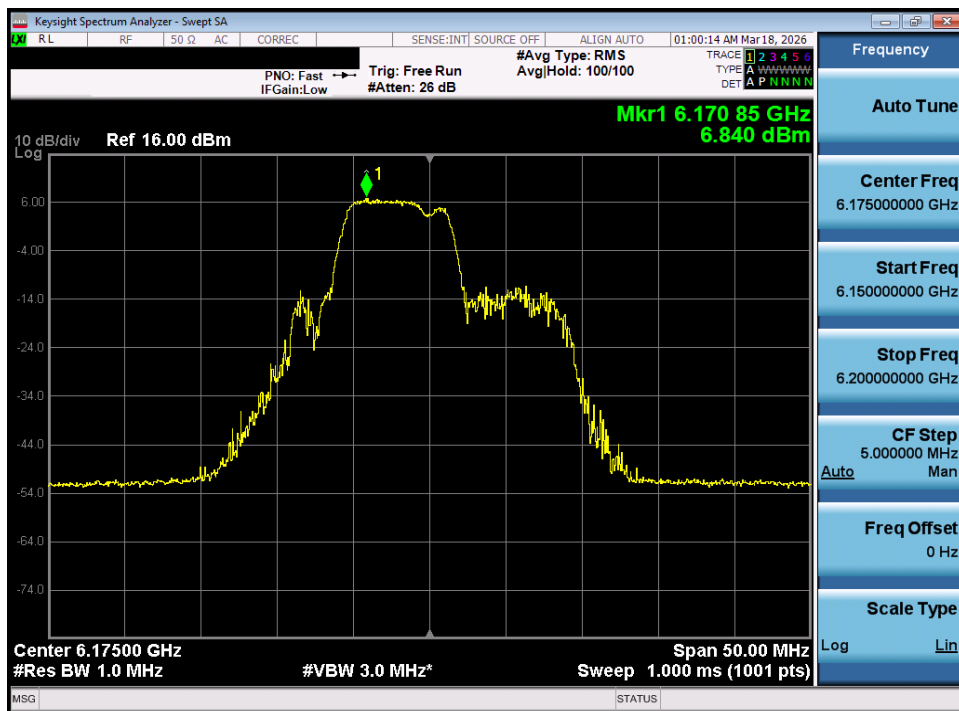
Plot 7-61. Power Spectral Density Plot MIMO ANT1 (20MHz 802.11be (52+26 Tones) (UNII Band 5) – Ch. 45) – SP
