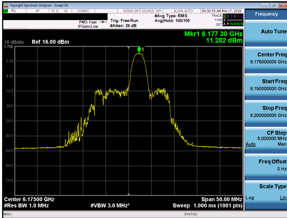
Plot 7-56. Power Spectral Density Plot MIMO ANT1 (20MHz 802.11ax/be (26 Tones) (UNII Band 5) – Ch. 45) - SP
