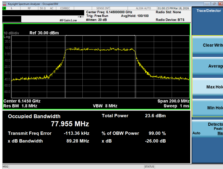
Plot 7-42. 26dB Bandwidth Plot MIMO ANT2 (80MHz 802.11ax/be (Full Tones) (UNII Band 5) – Ch. 39) - LPI/SP
