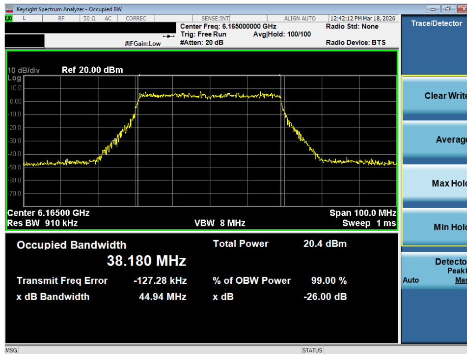
Plot 7-41. 26dB Bandwidth Plot MIMO ANT2 (40MHz 802.11ax/be (Full Tones) (UNII Band 5) – Ch. 43) - LPI
