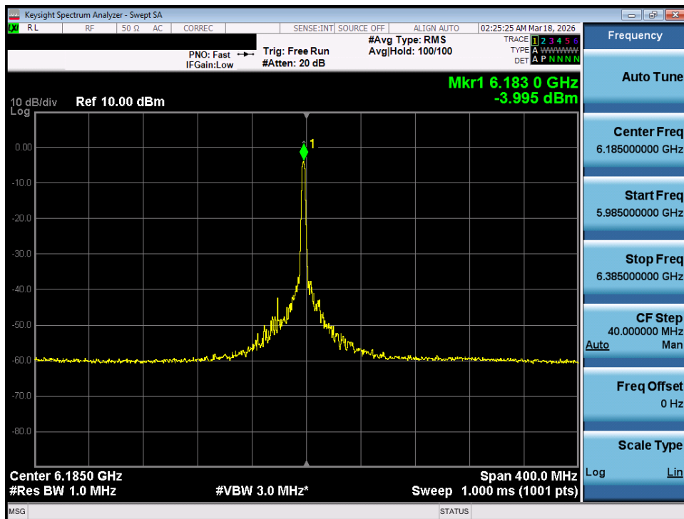
Plot 7-50. Power Spectral Density Plot MIMO ANT1 (160MHz 802.11ax/be (26 Tones) (UNII Band 5) – Ch. 47) - LPI
