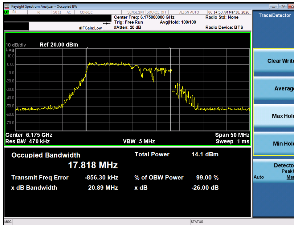
Plot 7-6. 26dB Bandwidth Plot MIMO ANT1 (20MHz 802.11be (106+26 Tones) (UNII Band 5) – Ch. 45) - LPI
