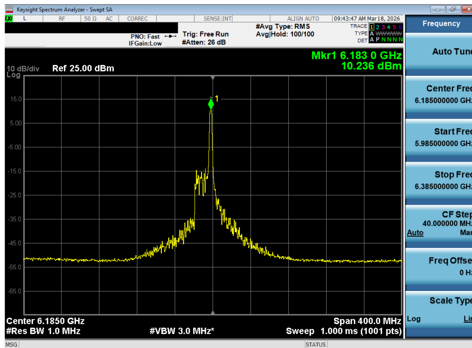
Plot 7-82. Power Spectral Density Plot MIMO ANT2 (160MHz 802.11ax/be (26 Tones) (UNII Band 5) – Ch. 47) - SP
