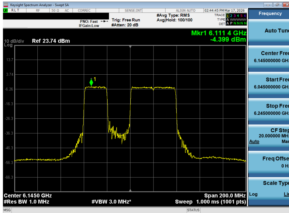
Plot 7-76. Power Spectral Density Plot MIMO ANT2 (80MHz 802.11be (484+242 Tones) (UNII Band 5) – Ch. 39) - LPI
