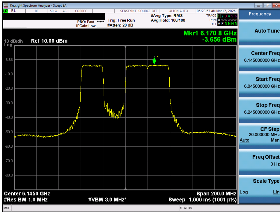
Plot 7-53. Power Spectral Density Plot MIMO ANT1 (80MHz 802.11be (484+242 Tones) (UNII Band 5) – Ch. 39) - LPI
