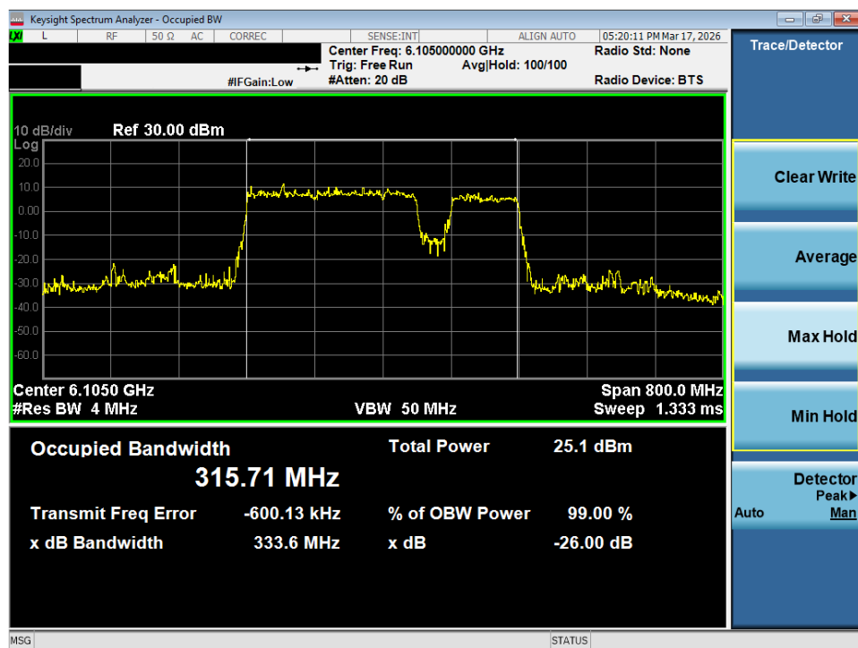
Plot 7-32. 26dB Bandwidth Plot MIMO ANT2 (320MHz 802.11be (3*996+484 Tones) (UNII Band 5) – Ch. 31) LPI/SP
