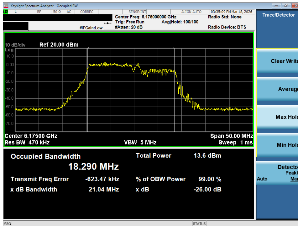
Plot 7-29. 26dB Bandwidth Plot MIMO ANT2 (20MHz 802.11be (106+26 Tones) (UNII Band 5) – Ch. 45) - LPI
