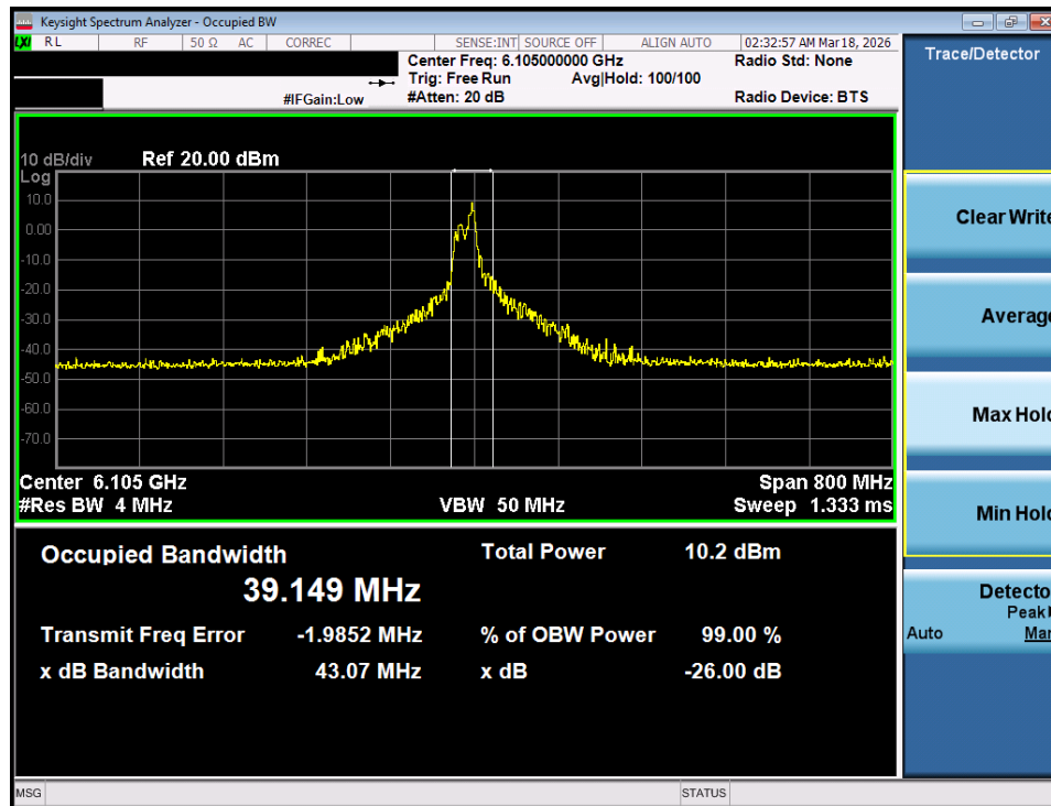
Plot 7-5. 26dB Bandwidth Plot MIMO ANT1 (320MHz 802.11be (26 Tones) (UNII Band 5) – Ch. 31) - LPI
