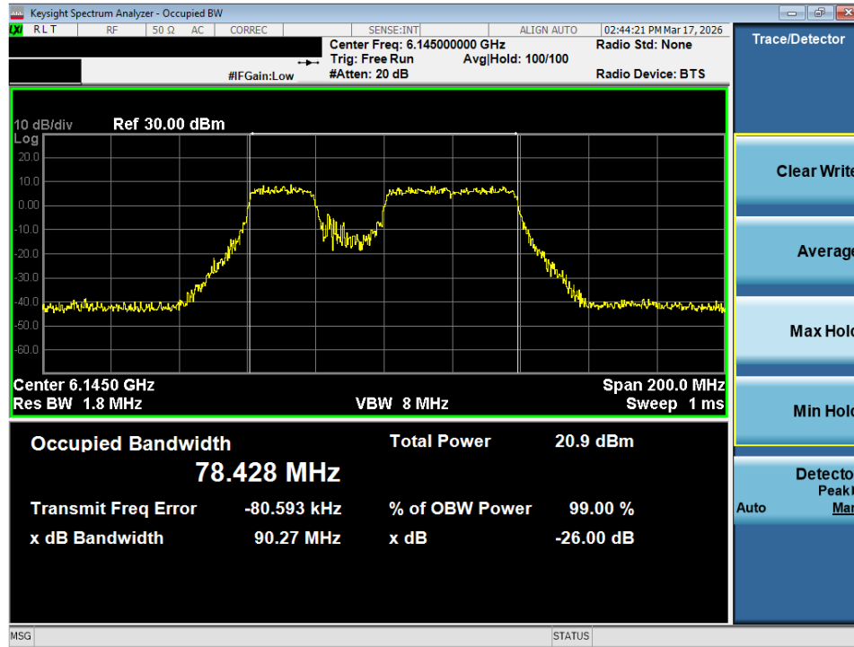
Plot 7-30. 26dB Bandwidth Plot MIMO ANT2 (80MHz 802.11be (484+242 Tones) (UNII Band 5) – Ch. 39) - LPI
