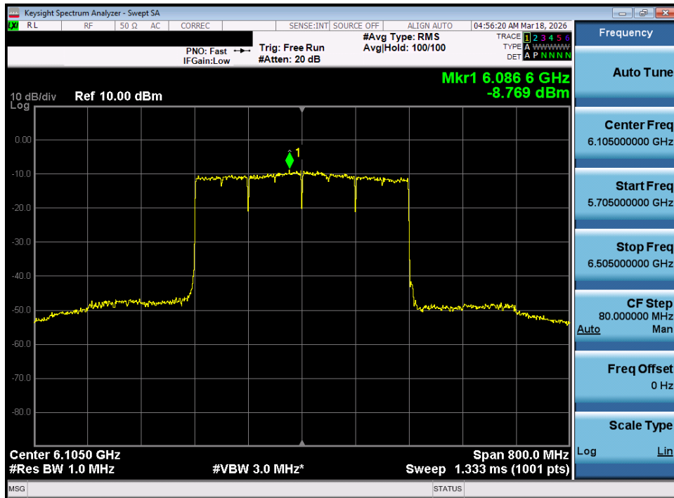
Plot 7-67. Power Spectral Density Plot MIMO ANT1 (320MHz 802.11be (Full Tones) (UNII Band 5) – Ch. 31) - LPI/SP
