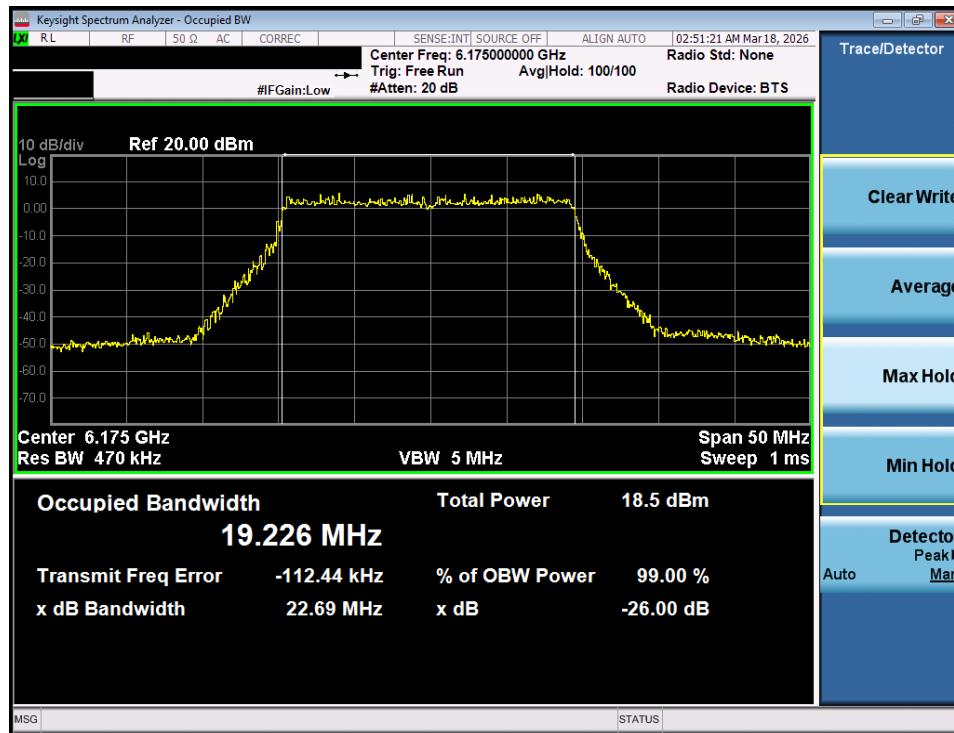
Plot 7-17. 26dB Bandwidth Plot MIMO ANT1 (20MHz 802.11ax/be (Full Tones) (UNII Band 5) – Ch. 45) – LPI
