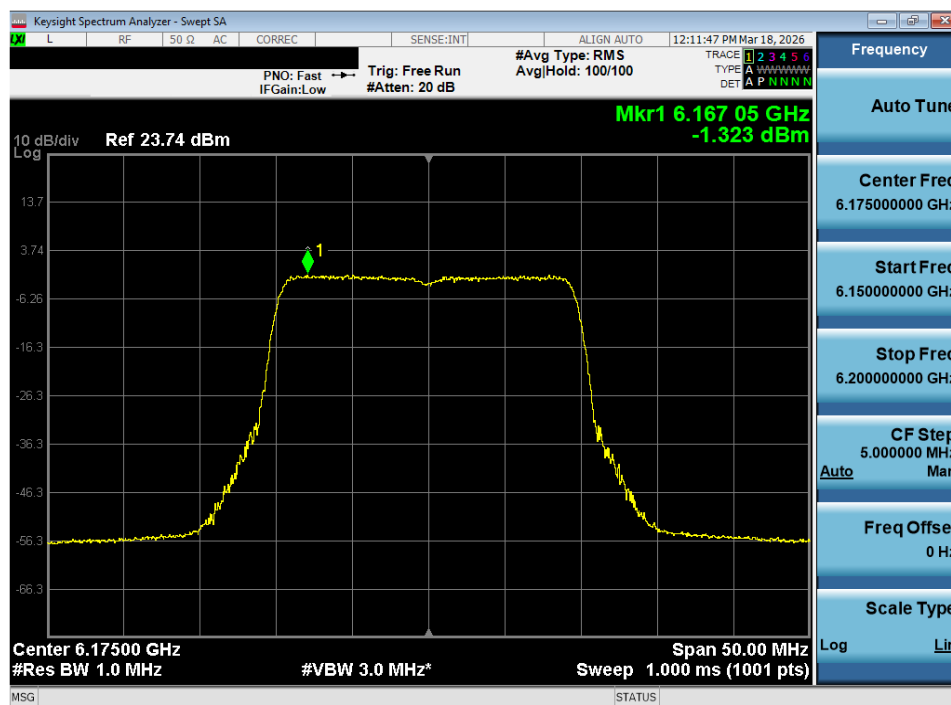
Plot 7-86. Power Spectral Density Plot MIMO ANT2 (20MHz 802.11ax/be (Full Tones) (UNII Band 5) – Ch. 45) - LPI
