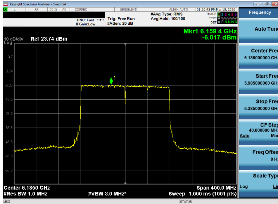
Plot 7-89. Power Spectral Density Plot MIMO ANT2 (160MHz 802.11ax/be (Full Tones) (UNII Band 5) – Ch. 47) - LPI/SP
