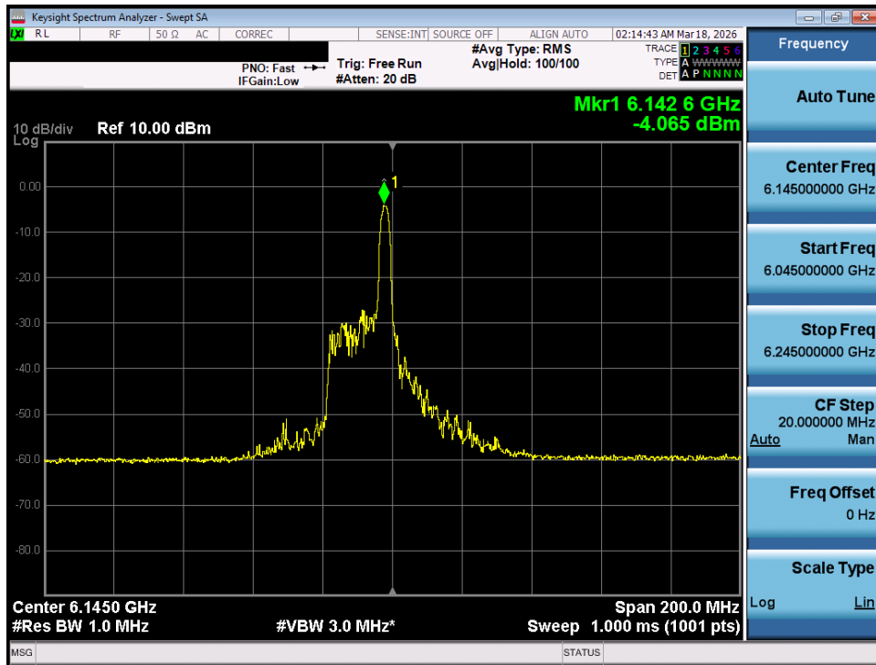
Plot 7-49. Power Spectral Density Plot MIMO ANT1 (80MHz 802.11ax/be (26 Tones) (UNII Band 5) – Ch. 39) - LPI
