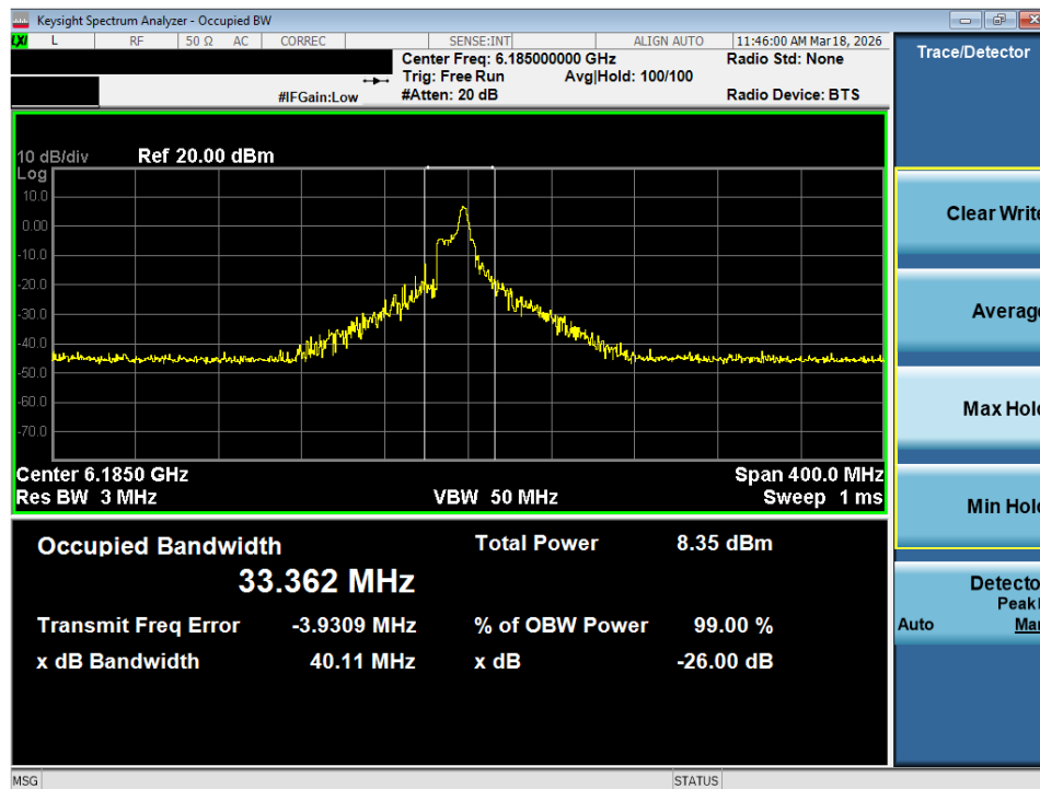
Plot 7-27. 26dB Bandwidth Plot MIMO ANT2 (160MHz 802.11ax/be (26 Tones) (UNII Band 5) – Ch. 47) - LPI
