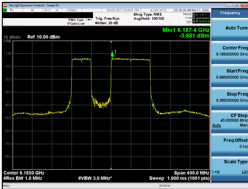
Plot 7-54. Power Spectral Density Plot MIMO ANT1 (160MHz 802.11be (996+484 Tones) (UNII Band 5) – Ch. 47) - LPI/SP
