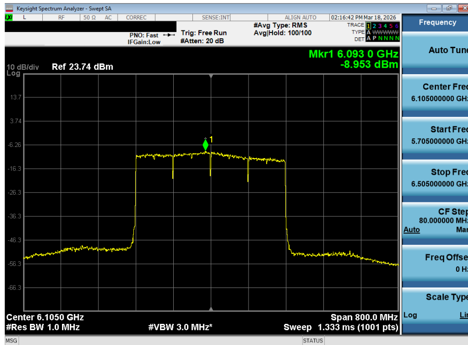
Plot 7-90. Power Spectral Density Plot MIMO ANT2 (320MHz 802.11be (Full Tones) (UNII Band 5) – Ch. 31) - LPI/SP
