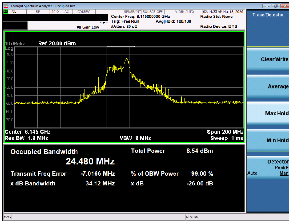
Plot 7-3. 26dB Bandwidth Plot MIMO ANT1 (80MHz 802.11ax/be (26 Tones) (UNII Band 5) – Ch. 39) - LPI
