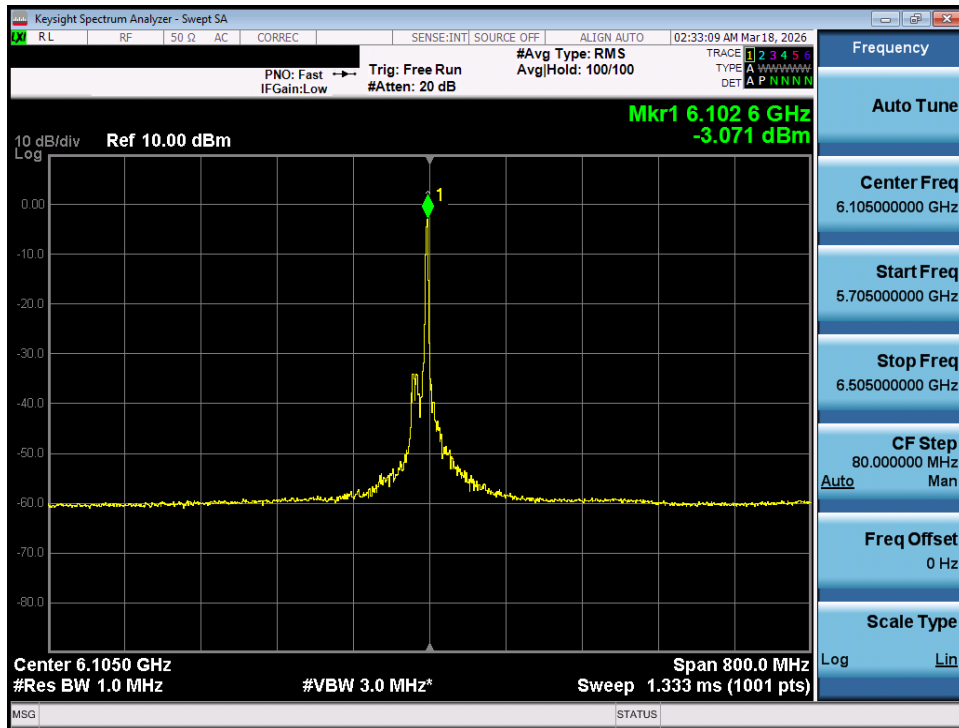
Plot 7-51. Power Spectral Density Plot MIMO ANT1 (320MHz 802.11be (26 Tones) (UNII Band 5) – Ch. 31) - LPI
