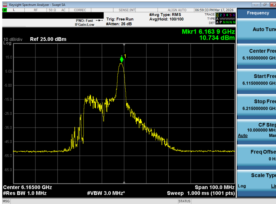
Plot 7-80. Power Spectral Density Plot MIMO ANT2 (40MHz 802.11ax/be (26 Tones) (UNII Band 5) – Ch. 43) - SP
