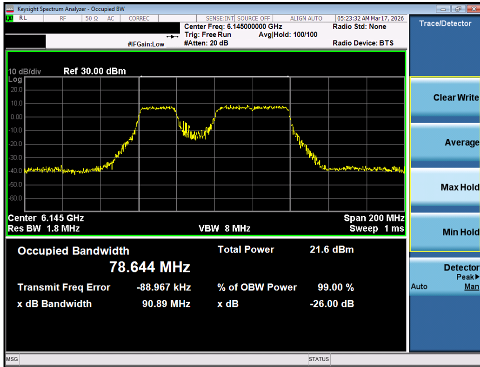
Plot 7-7. 26dB Bandwidth Plot MIMO ANT1 (80MHz 802.11be (484+242 Tones) (UNII Band 5) – Ch. 39) - LPI
