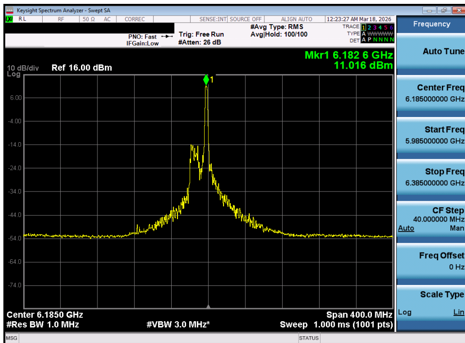
Plot 7-59. Power Spectral Density Plot MIMO ANT1 (160MHz 802.11ax/be (26 Tones) (UNII Band 5) – Ch. 47) - SP
