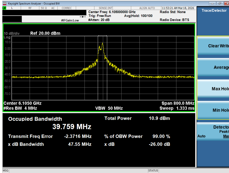
Plot 7-28. 26dB Bandwidth Plot MIMO ANT2 (320MHz 802.11be (26 Tones) (UNII Band 5) – Ch. 31) - LPI
