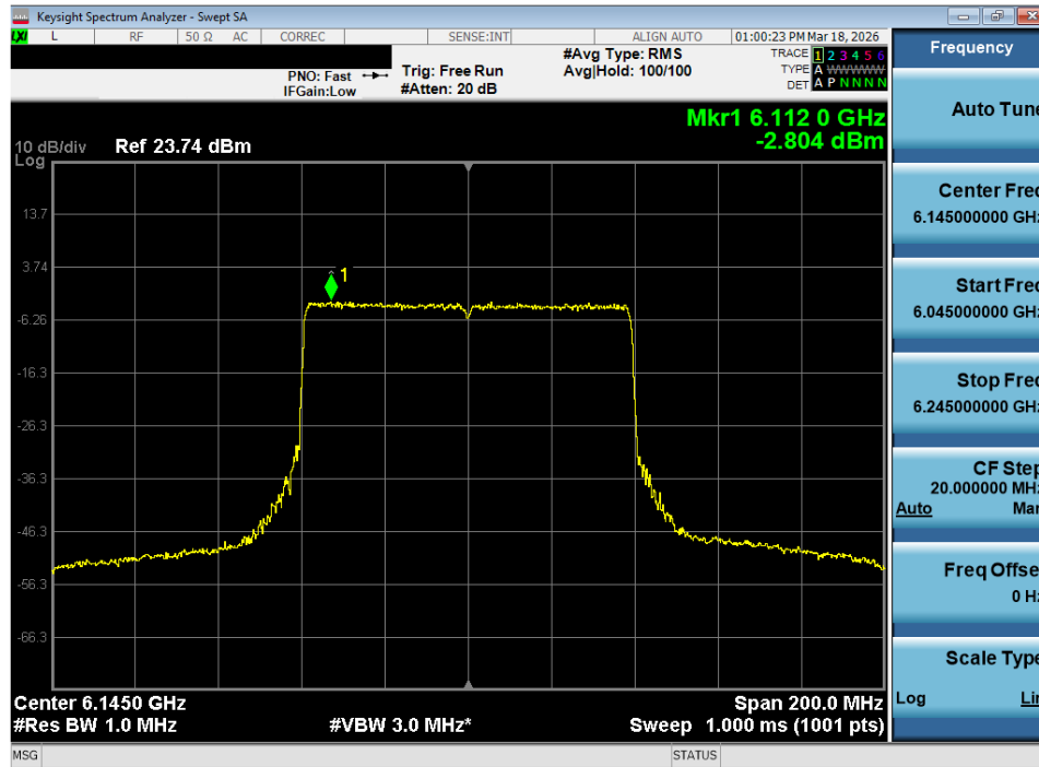
Plot 7-88. Power Spectral Density Plot MIMO ANT2 (80MHz 802.11ax/be (Full Tones) (UNII Band 5) – Ch. 39) - LPI/SP
