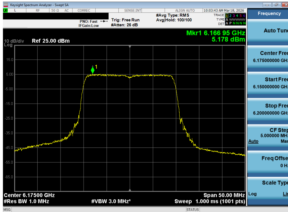
Plot 7-91. Power Spectral Density Plot MIMO ANT2 (20MHz 802.11ax/be (Full Tones) (UNII Band 5) – Ch. 45) - SP
