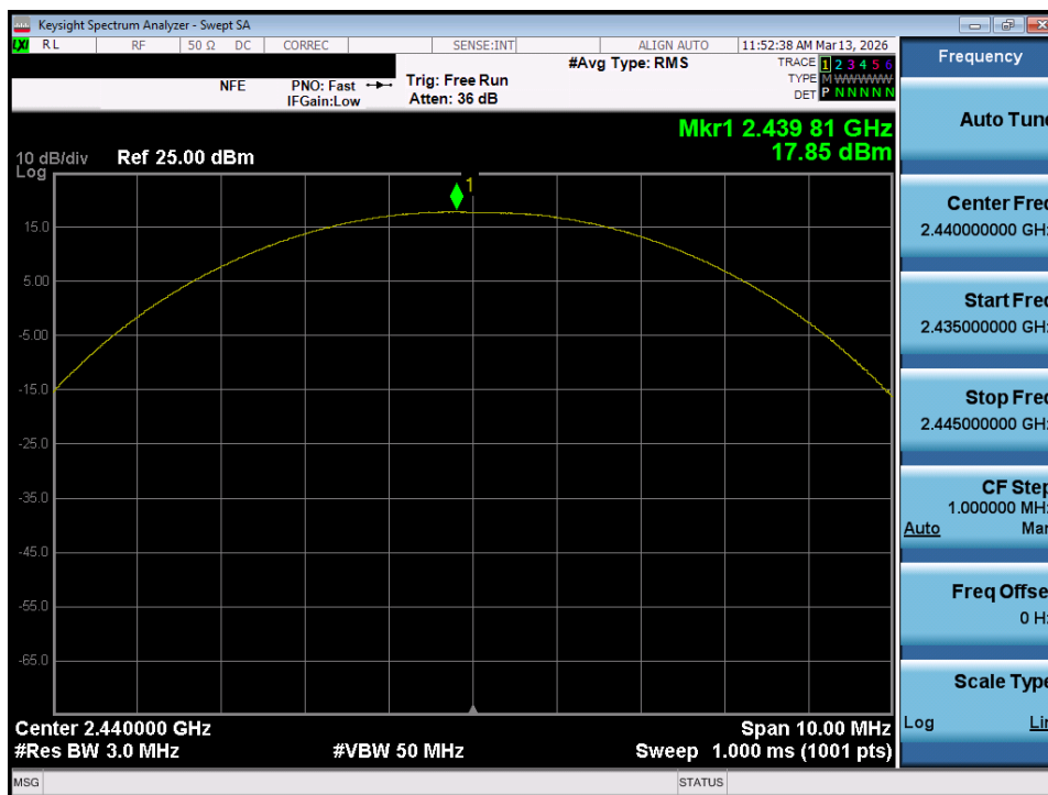
Plot 7-92. Peak Power Plot (Bluetooth (LE), 1Mbps – Ch. 17) – Ant 2
