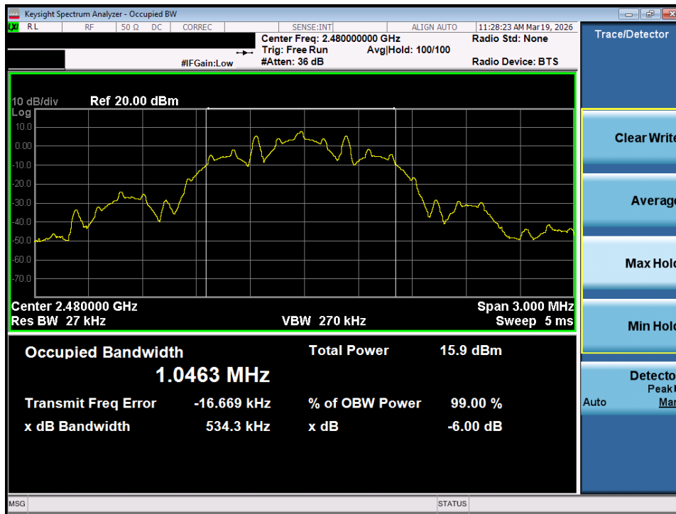
Plot 7-39. OBW Plot (Bluetooth (LE), 125kbps – Ch. 39) – SISO ANT1
