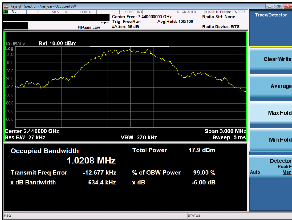
Plot 7-68. OBW Plot (Bluetooth (LE), 1Mbps – Ch. 17) – Dual ANT2
