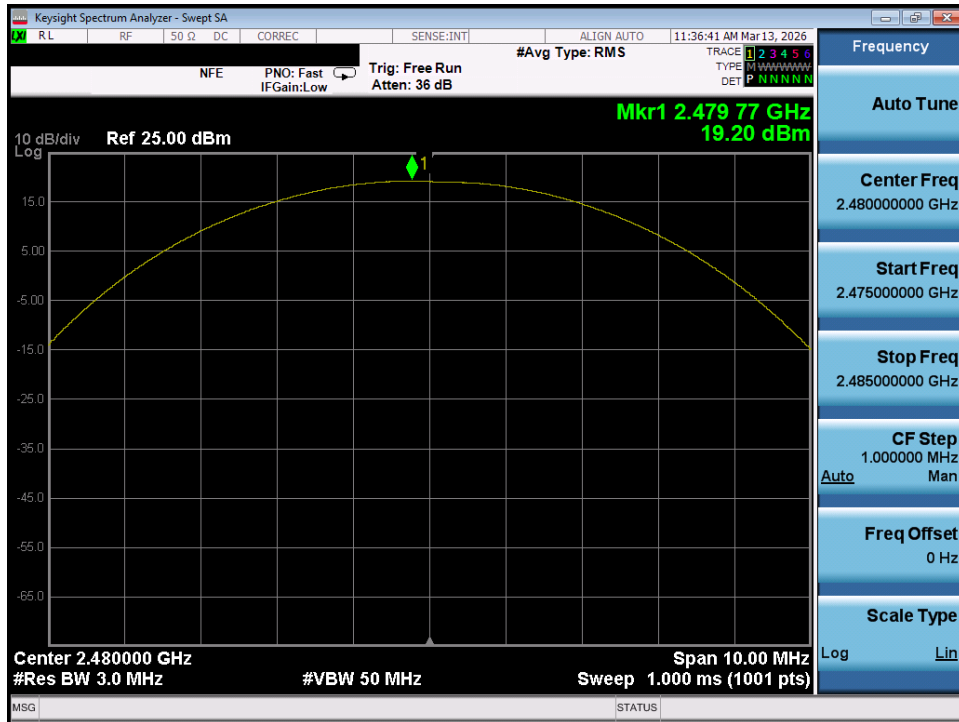
Plot 7-81. Peak Power Plot (Bluetooth (LE), 1Mbps – Ch. 39) – Ant 1
