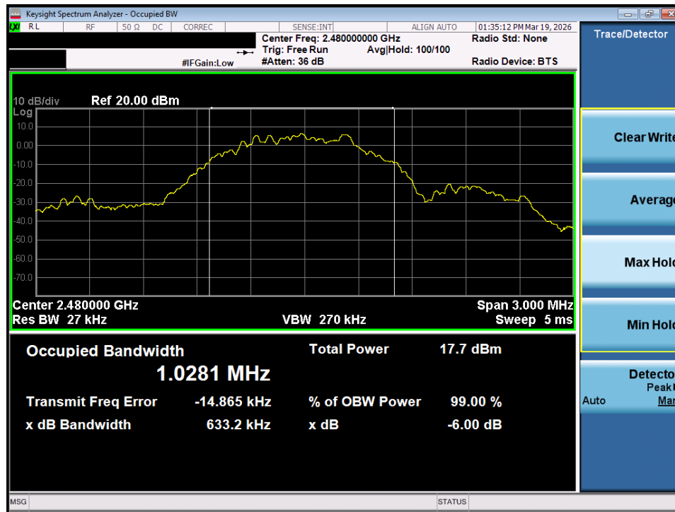
Plot 7-69. OBW Plot (Bluetooth (LE), 1Mbps – Ch. 39) – Dual ANT2
