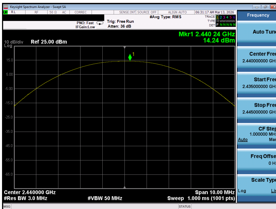
Plot 7-98. Peak Power Plot (Bluetooth (LE), 1Mbps – Ch. 17) – Dual Ant 1
