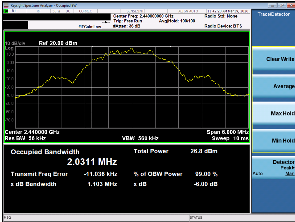
Plot 7-47. OBW Plot (Bluetooth (LE), 2Mbps – Ch. 17) – SISO ANT1
