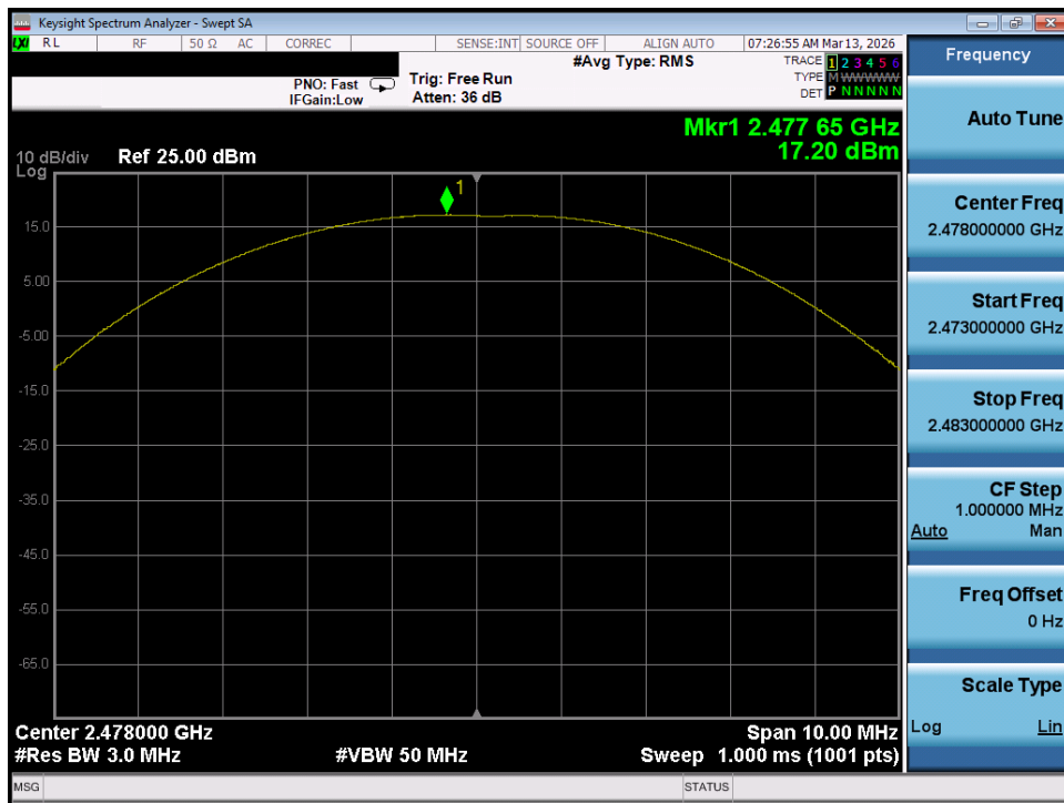
Plot 7-96. Peak Power Plot (Bluetooth (LE), 2Mbps – Ch. 36) – Ant 2
