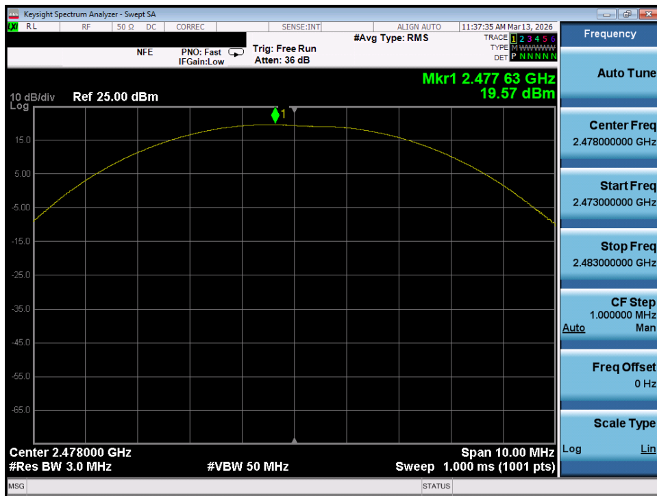
Plot 7-84. Peak Power Plot (Bluetooth (LE), 2Mbps – Ch. 36) – Ant 1
