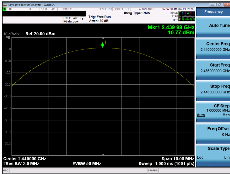
Plot 7-77. Peak Power Plot (Bluetooth (LE), 500kbps – Ch. 17) – Ant 1
