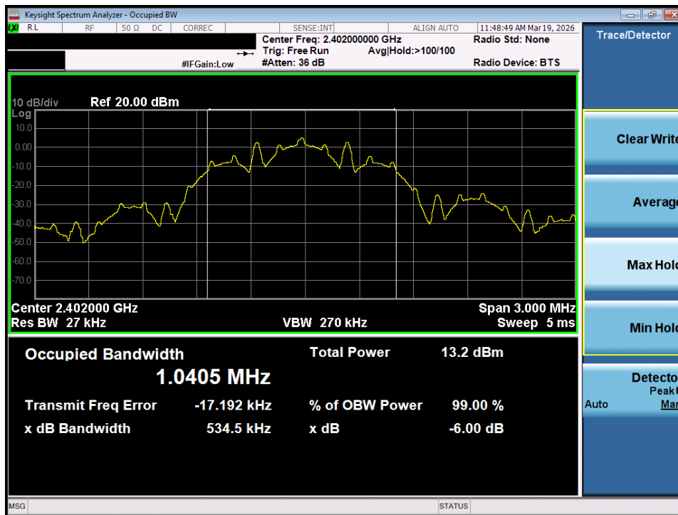
Plot 7-49. OBW Plot (Bluetooth (LE), 125kbps – Ch. 37) – SISO ANT2
