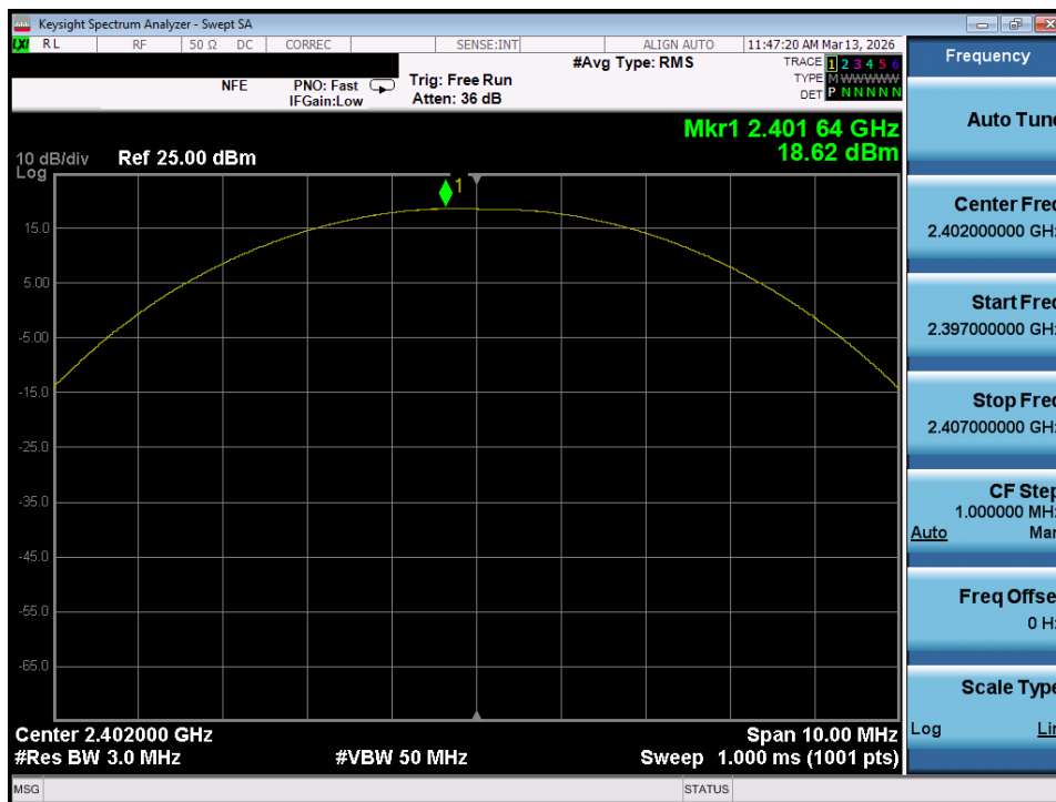
Plot 7-91. Peak Power Plot (Bluetooth (LE), 1Mbps – Ch. 37) – Ant 2
