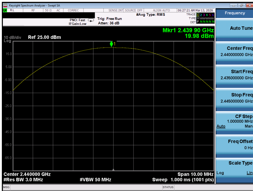
Plot 7-80. Peak Power Plot (Bluetooth (LE), 1Mbps - Ch. 17) - Ant 1
