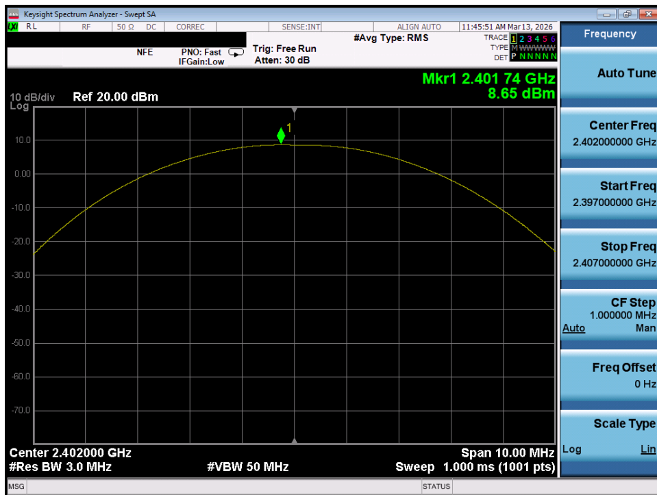
Plot 7-85. Peak Power Plot (Bluetooth (LE), 125kbps – Ch. 37) – Ant 2
