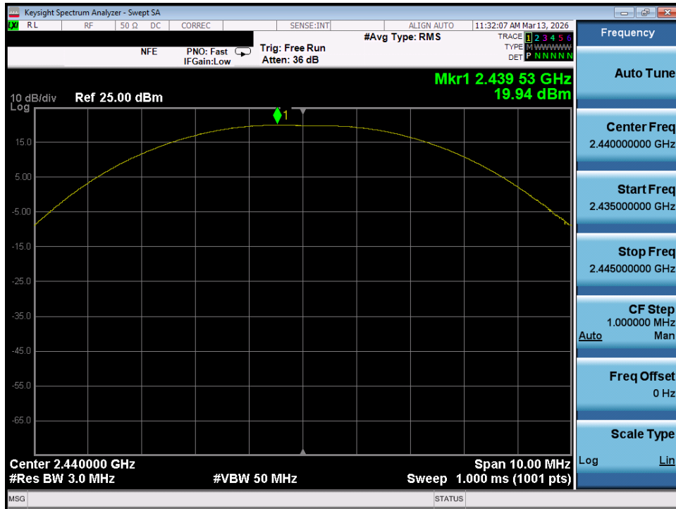
Plot 7-83. Peak Power Plot (Bluetooth (LE), 2Mbps – Ch. 17) – Ant 1
