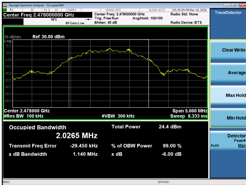
Plot 7-24. 6dB Bandwidth Plot (Bluetooth (LE), 2Mbps – Ch. 36) – Ant 2
