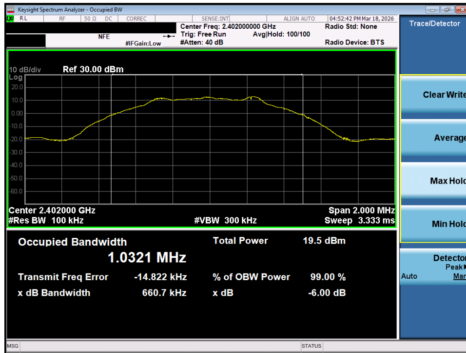
Plot 7-25. 6dB Bandwidth Plot (Bluetooth (LE), 1Mbps – Ch. 37) – Dual Ant 1
