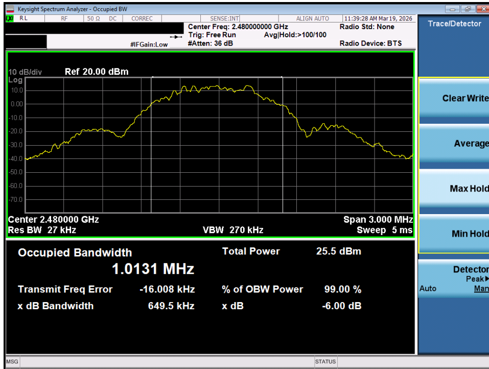
Plot 7-45. OBW Plot (Bluetooth (LE), 1Mbps – Ch. 39) – SISO ANT1
