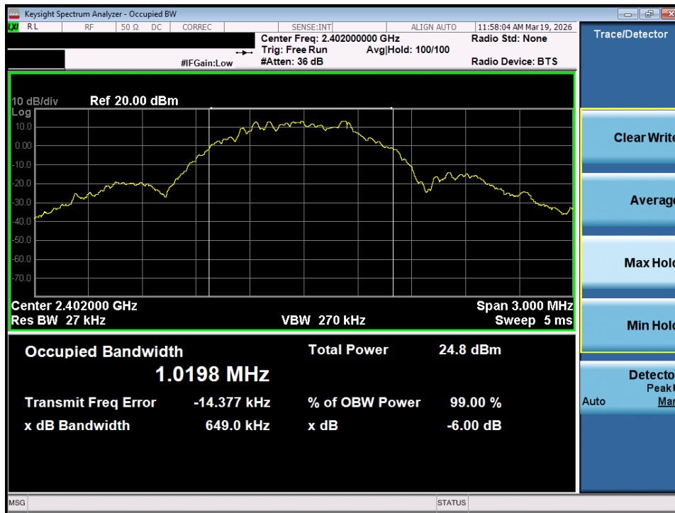
Plot 7-55. OBW Plot (Bluetooth (LE), 1Mbps – Ch. 37) – SISO ANT2
