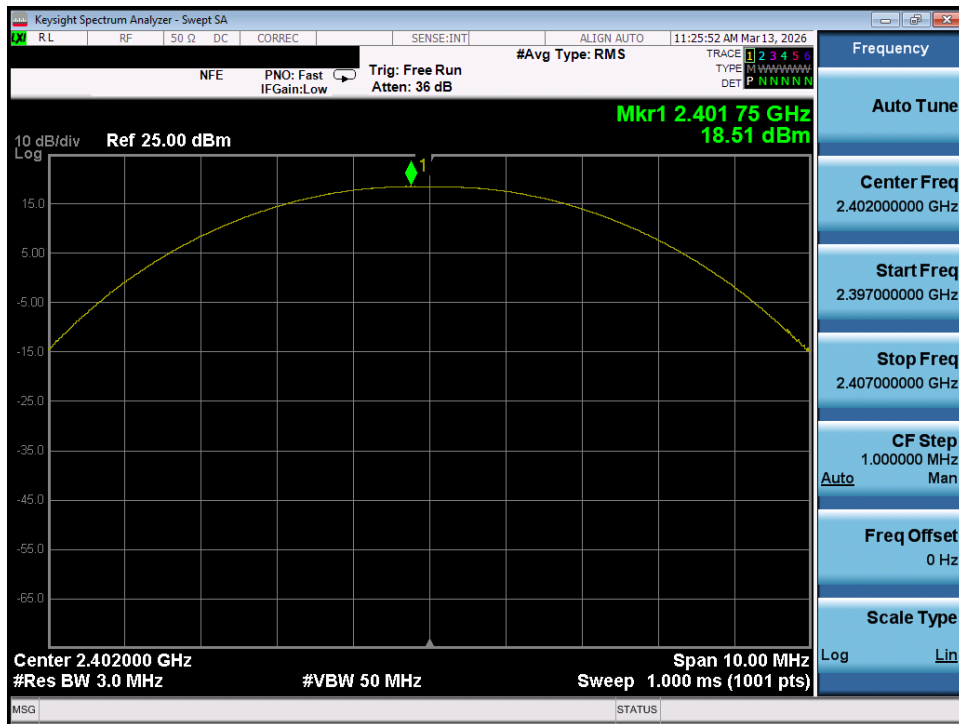
Plot 7-79. Peak Power Plot (Bluetooth (LE), 1Mbps - Ch. 37) - Ant 1
