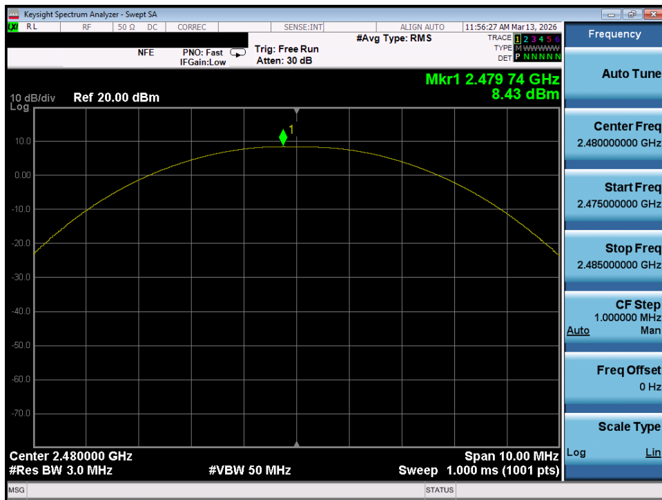
Plot 7-90. Peak Power Plot (Bluetooth (LE), 500kbps – Ch. 39) – Ant 2
