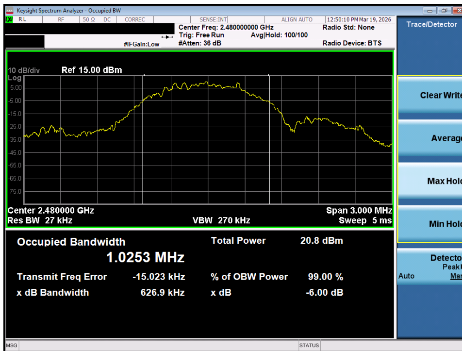
Plot 7-63. OBW Plot (Bluetooth (LE), 1Mbps – Ch. 39) – Dual ANT1
