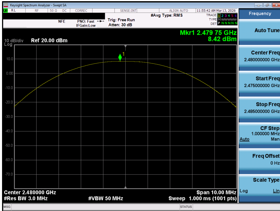
Plot 7-87. Peak Power Plot (Bluetooth (LE), 125kbps – Ch. 39) – Ant 2
