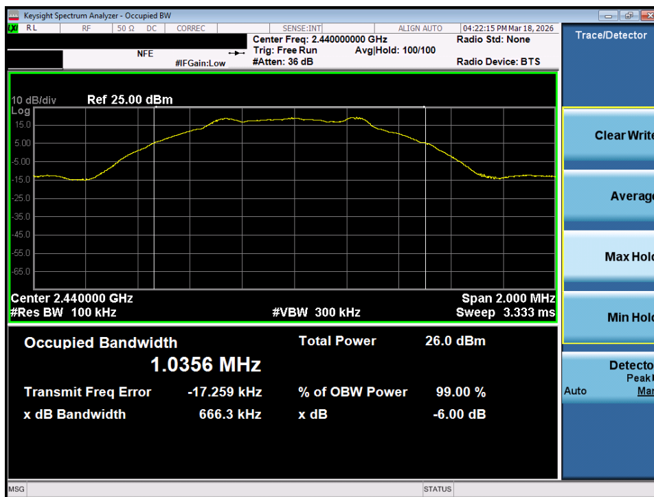
Plot 7-8. 6dB Bandwidth Plot (Bluetooth (LE), 1Mbps - Ch. 17) - Ant 1
