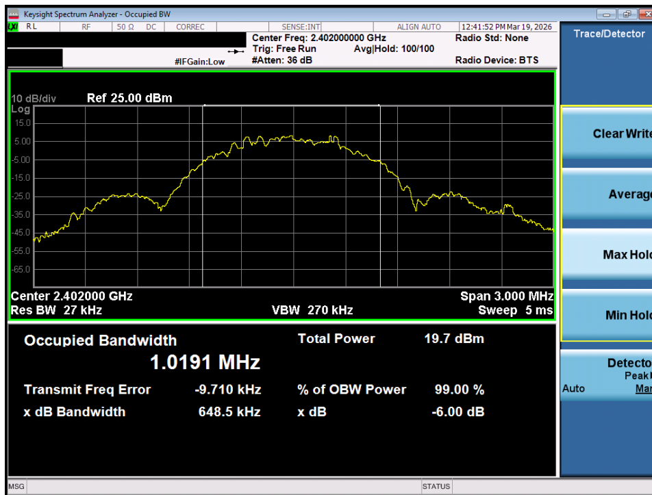
Plot 7-61. OBW Plot (Bluetooth (LE), 1Mbps – Ch. 37) – Dual ANT1
