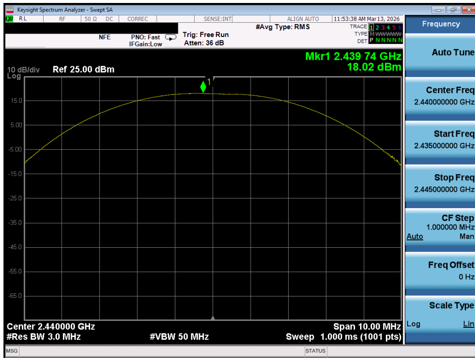
Plot 7-95. Peak Power Plot (Bluetooth (LE), 2Mbps – Ch. 17) – Ant 2
