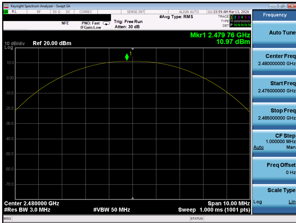
Plot 7-75. Peak Power Plot (Bluetooth (LE), 125kbps – Ch. 39) – Ant 1
