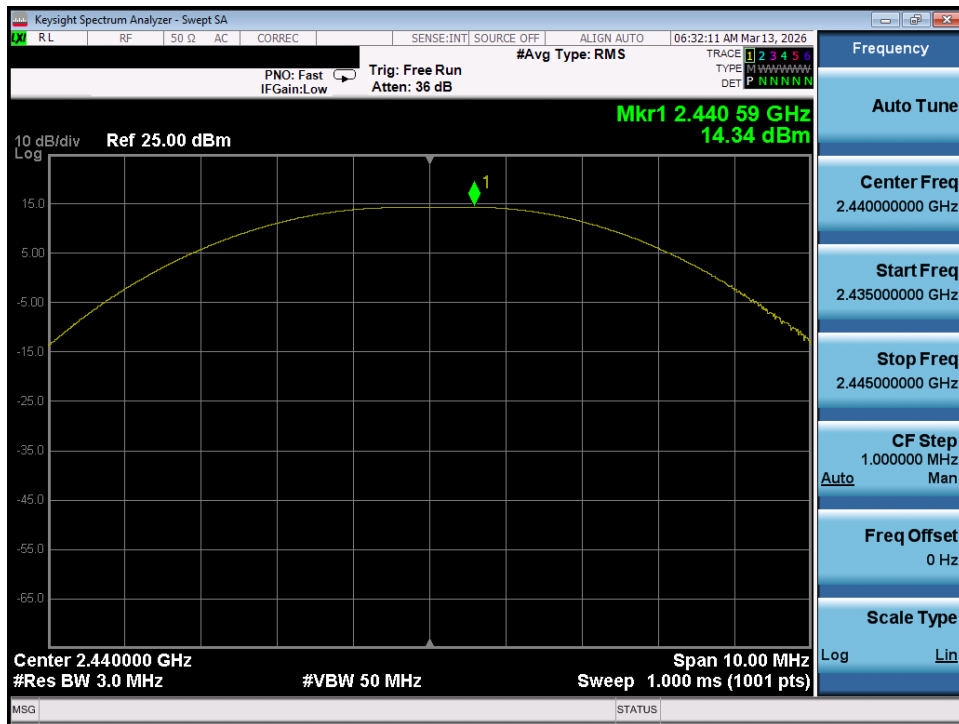
Plot 7-101. Peak Power Plot (Bluetooth (LE), 2Mbps - Ch. 17) - Dual Ant 1
