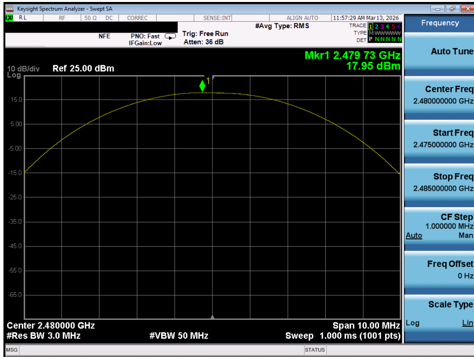
Plot 7-93. Peak Power Plot (Bluetooth (LE), 1Mbps – Ch. 39) – Ant 2
