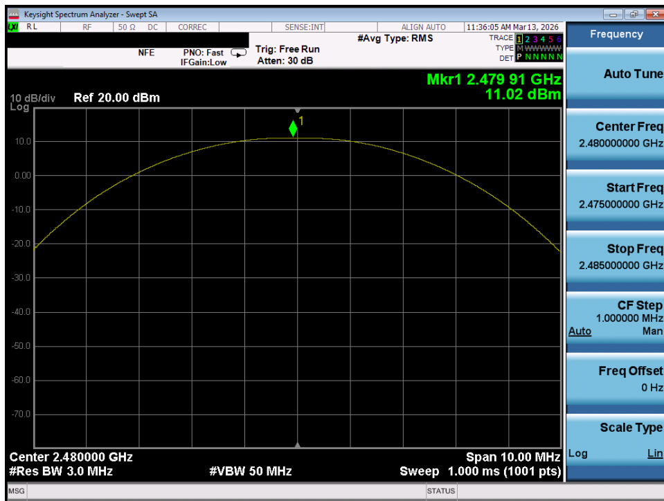
Plot 7-78. Peak Power Plot (Bluetooth (LE), 500kbps – Ch. 39) – Ant 1
