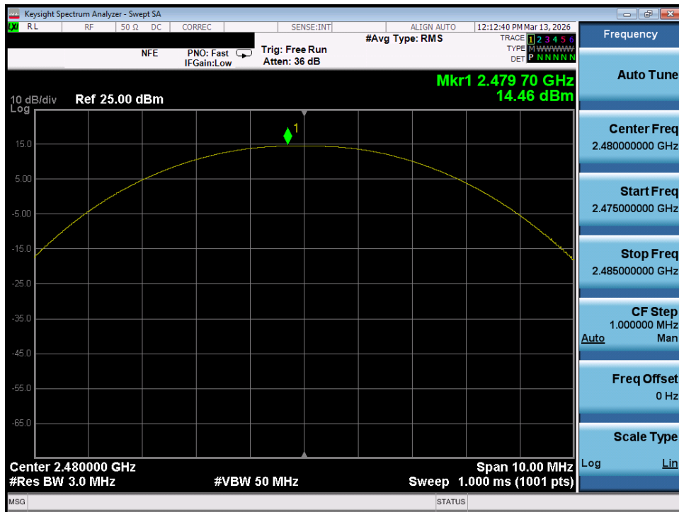
Plot 7-99. Peak Power Plot (Bluetooth (LE), 1Mbps – Ch. 39) – Dual Ant 1
