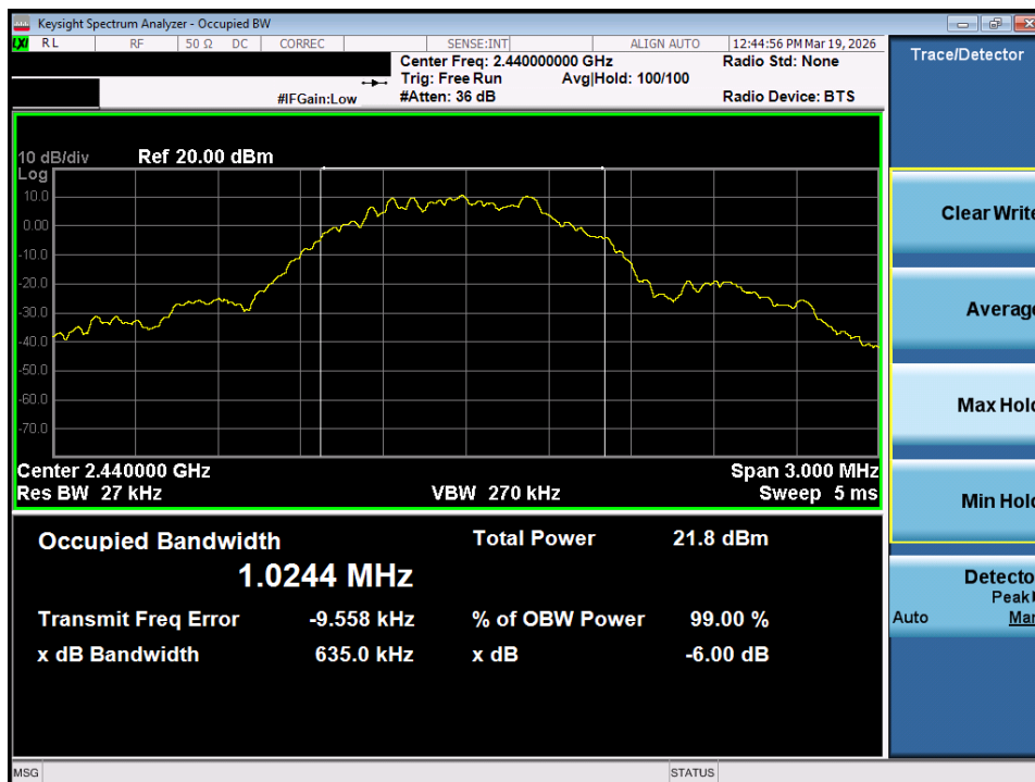
Plot 7-62. OBW Plot (Bluetooth (LE), 1Mbps – Ch. 17) – Dual ANT1
