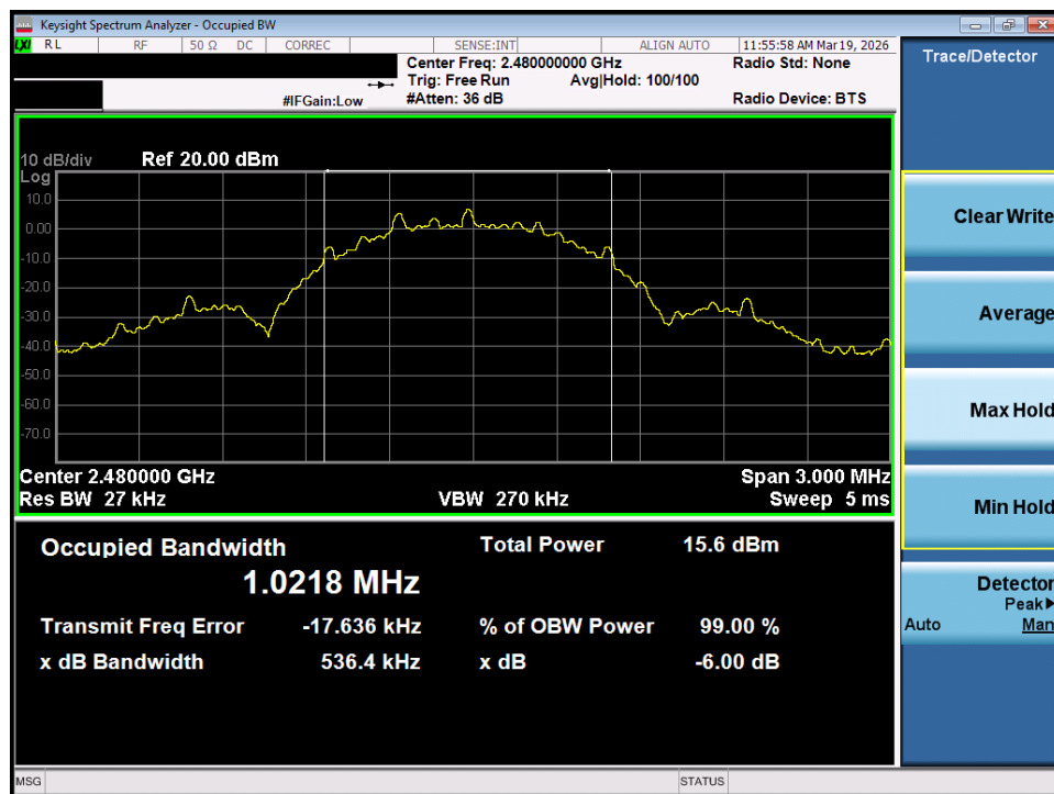
Plot 7-54. OBW Plot (Bluetooth (LE), 500kbps – Ch. 39) – SISO ANT2
