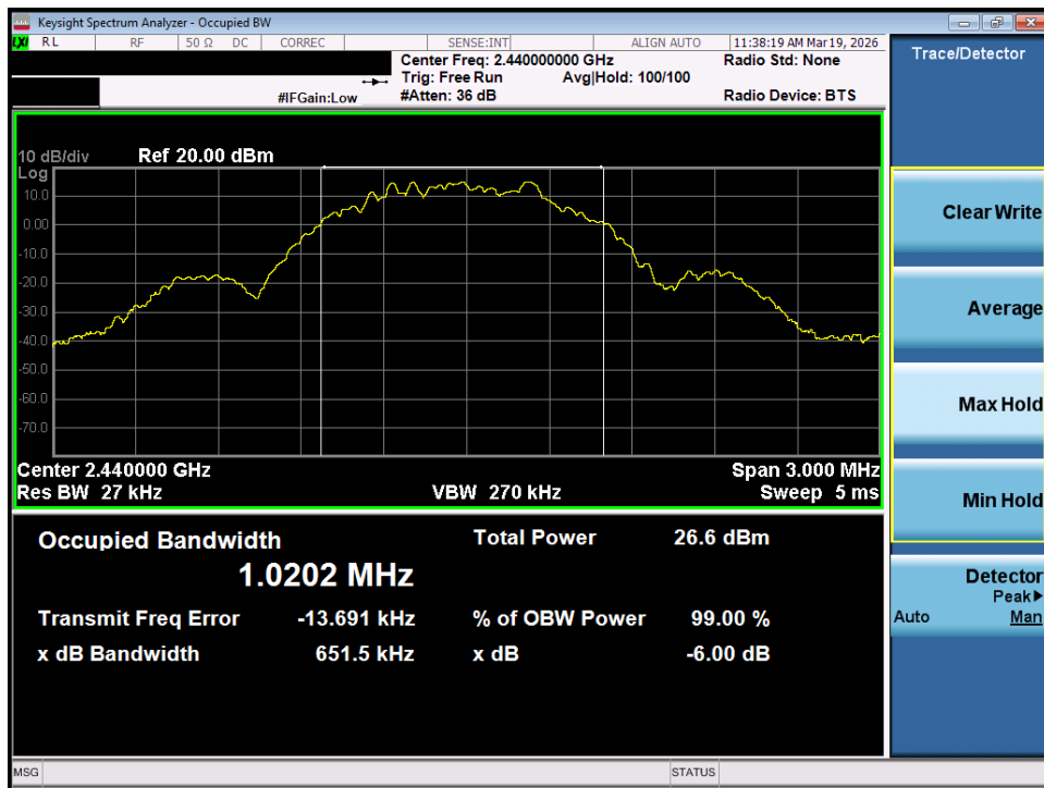
Plot 7-44. OBW Plot (Bluetooth (LE), 1Mbps – Ch. 17) – SISO ANT1
