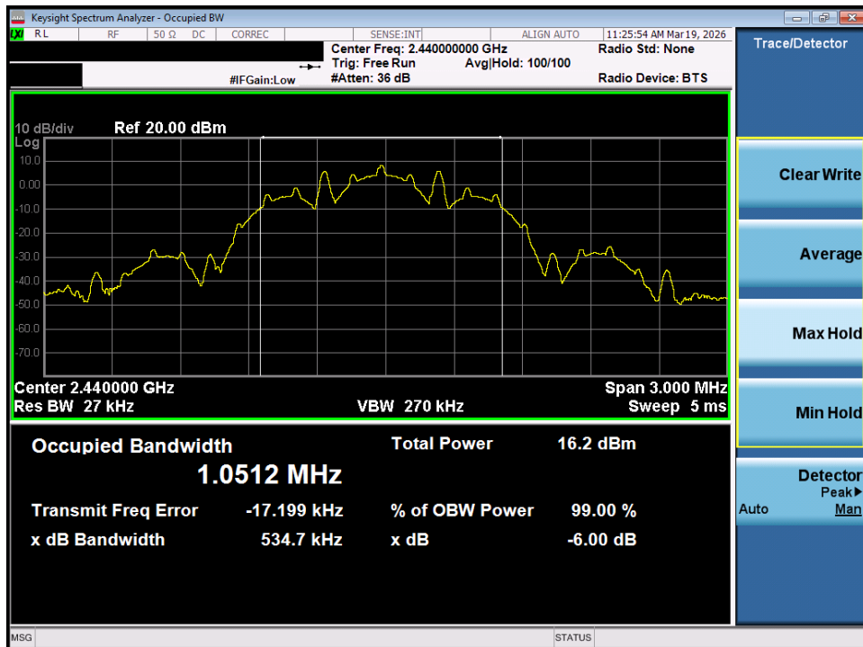
Plot 7-38. OBW Plot (Bluetooth (LE), 125kbps – Ch. 17) – SISO ANT1
