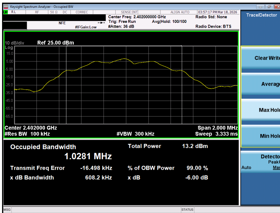
Plot 7-1. 6dB Bandwidth Plot (Bluetooth (LE), 125kbps – Ch. 37) – Ant 1
