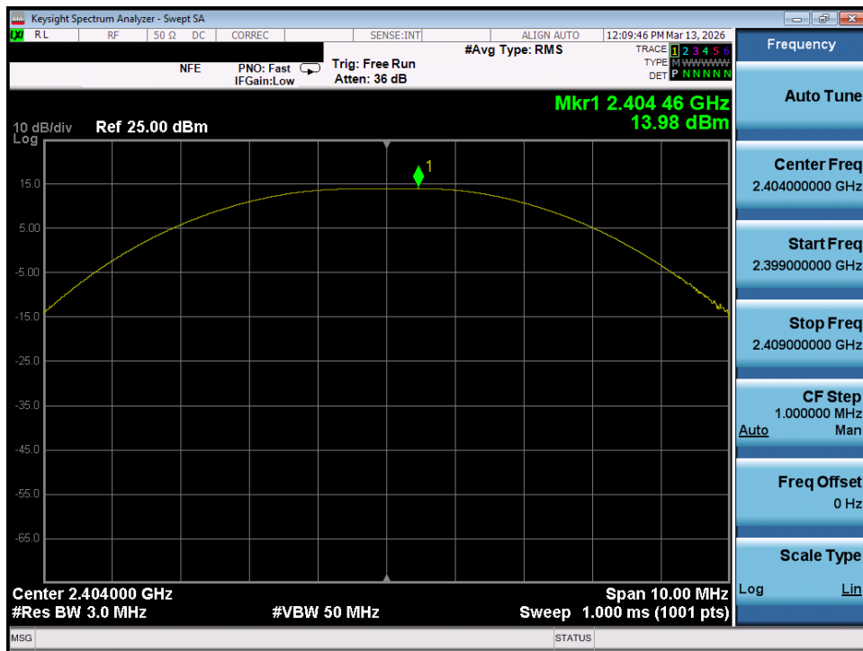
Plot 7-100. Peak Power Plot (Bluetooth (LE), 2Mbps – Ch. 0) – Dual Ant 1
