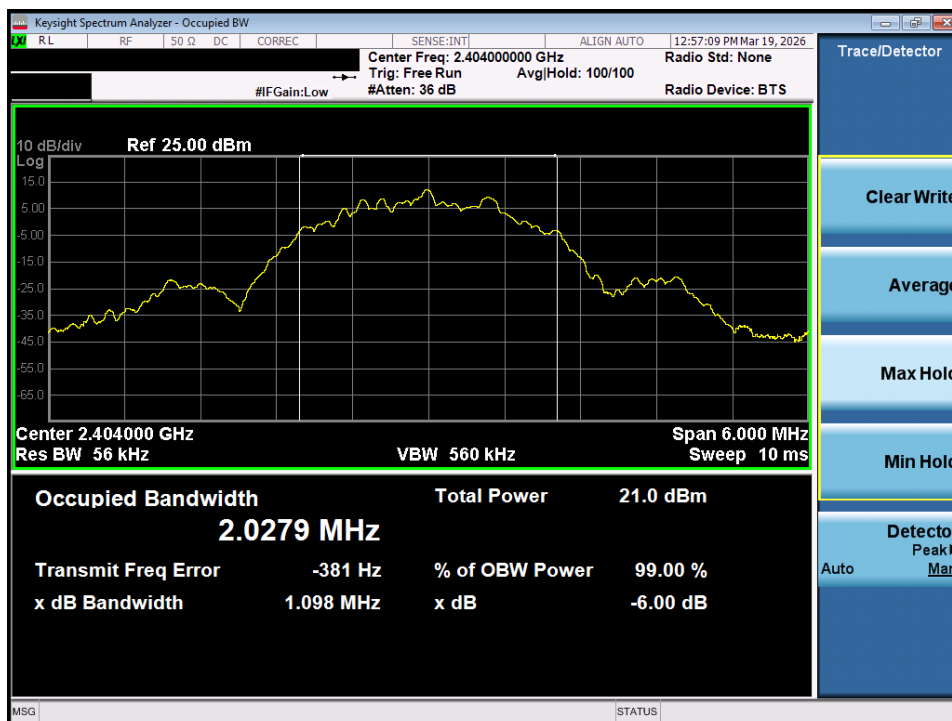
Plot 7-64. OBW Plot (Bluetooth (LE), 2Mbps – Ch. 0) – Dual ANT1
