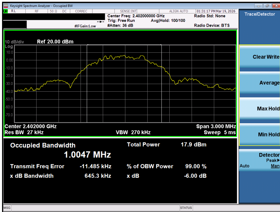
Plot 7-67. OBW Plot (Bluetooth (LE), 1Mbps – Ch. 37) – Dual ANT2
