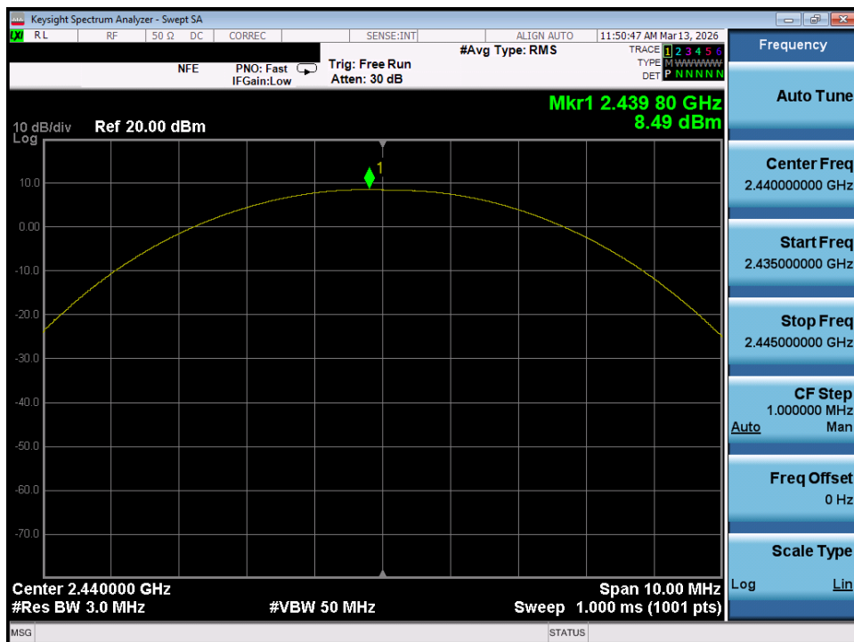
Plot 7-86. Peak Power Plot (Bluetooth (LE), 125kbps – Ch. 17) – Ant 2
