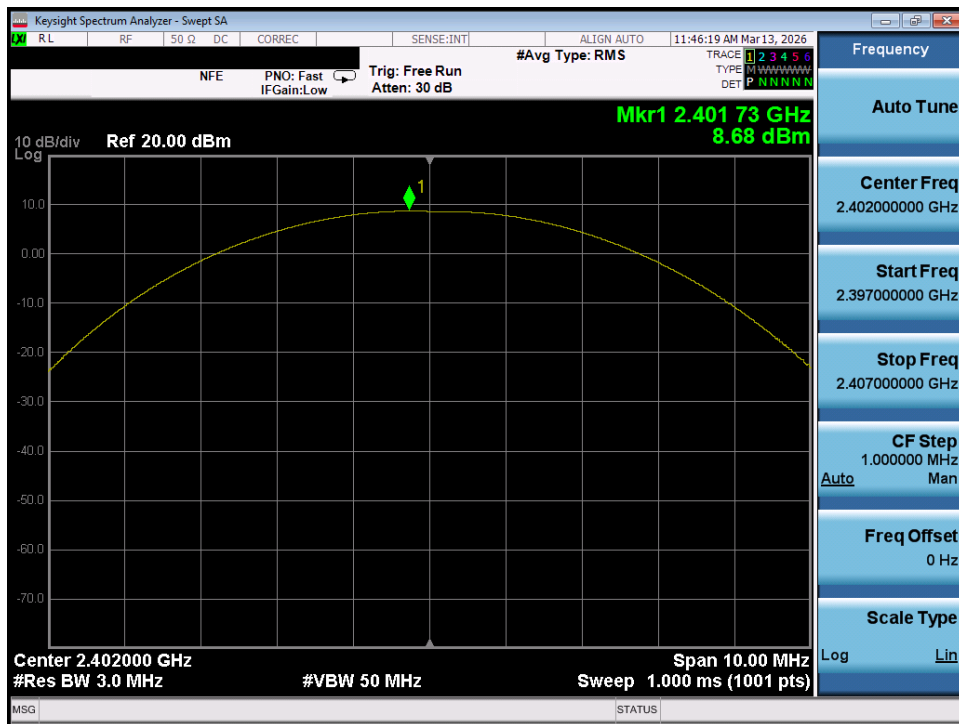
Plot 7-88. Peak Power Plot (Bluetooth (LE), 500kbps – Ch. 37) – Ant 2
