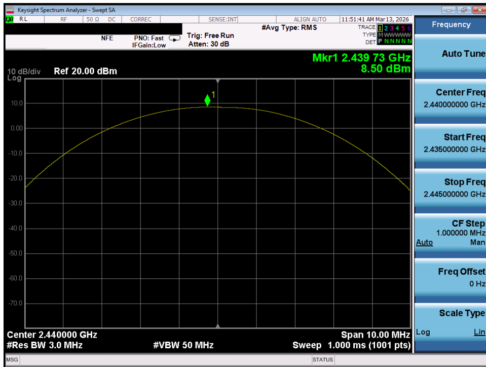
Plot 7-89. Peak Power Plot (Bluetooth (LE), 500kbps – Ch. 17) – Ant 2
