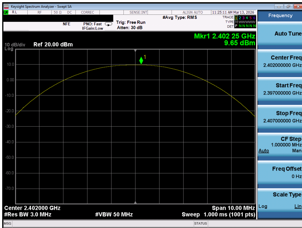
Plot 7-76. Peak Power Plot (Bluetooth (LE), 500kbps – Ch. 37) – Ant 1
