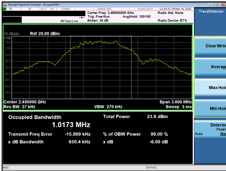
Plot 7-57. OBW Plot (Bluetooth (LE), 1Mbps – Ch. 39) – SISO ANT2
