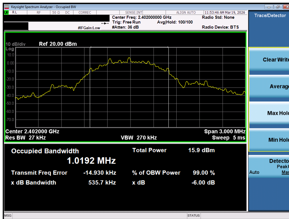
Plot 7-52. OBW Plot (Bluetooth (LE), 500kbps – Ch. 37) – SISO ANT2
