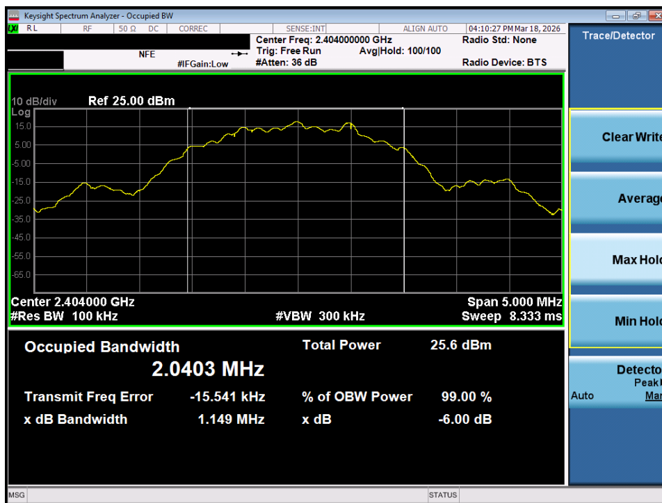
Plot 7-10. 6dB Bandwidth Plot (Bluetooth (LE), 2Mbps – Ch. 0) – Ant 1
