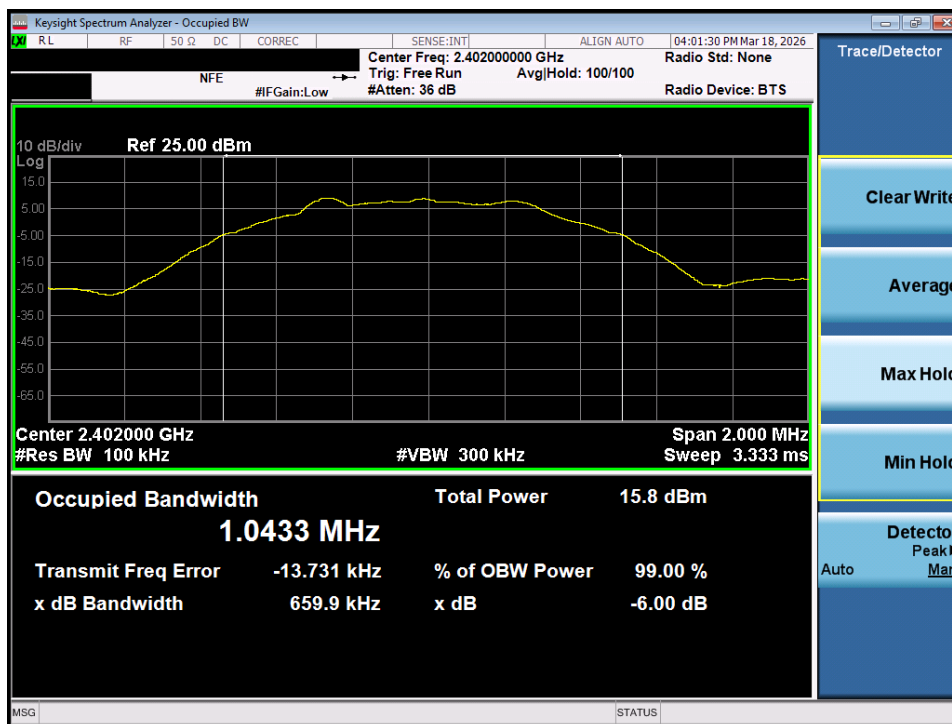
Plot 7-4. 6dB Bandwidth Plot (Bluetooth (LE), 500kbps – Ch. 37) – Ant 1
