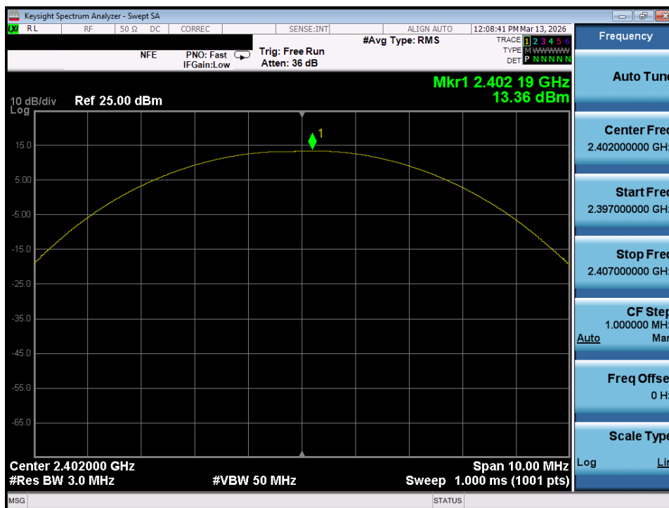
Plot 7-97. Peak Power Plot (Bluetooth (LE), 1Mbps – Ch. 37) – Dual Ant 1
