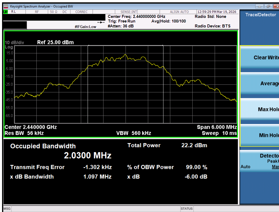
Plot 7-65. OBW Plot (Bluetooth (LE), 2Mbps - Ch. 17) - Dual ANT1
