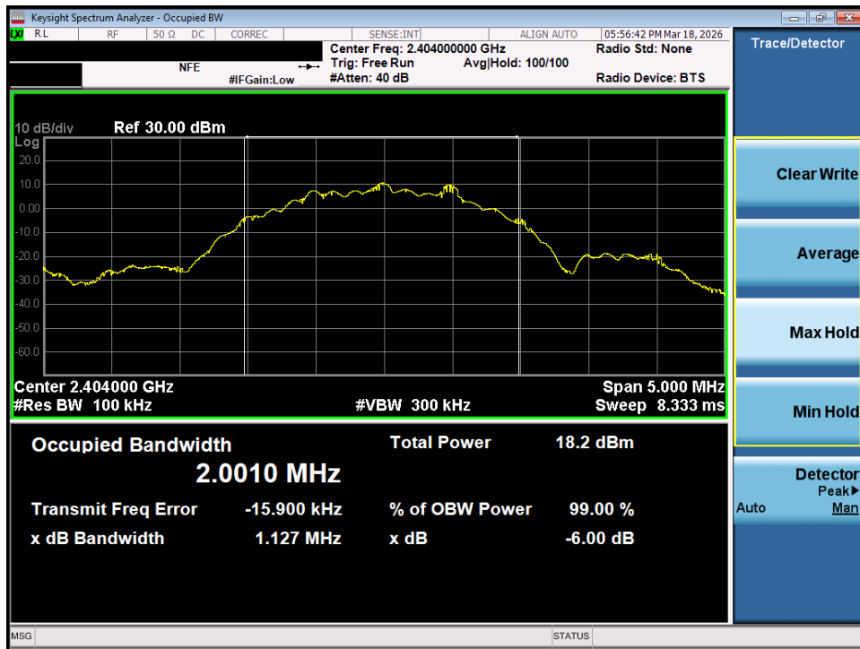
Plot 7-34. 6dB Bandwidth Plot (Bluetooth (LE), 2Mbps – Ch. 0) – Dual Ant 2
