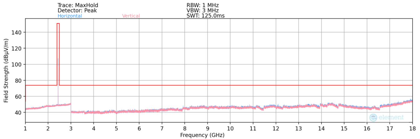
Plot 7-202. Radiated Spurious Plot above 1GHz (Bluetooth (LE) – Ch. 17) – Dual
