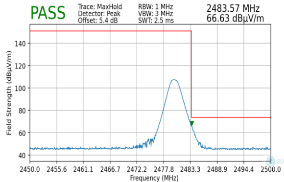
Plot 7-212. Radiated Restricted Upper Band Edge Measurement (Peak) – Ant 2 - WCP
