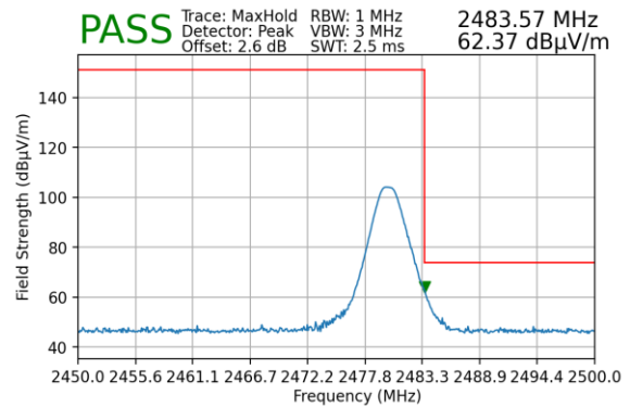
Plot 7-210. Radiated Restricted Upper Band Edge Measurement (Peak) – Ant 2
