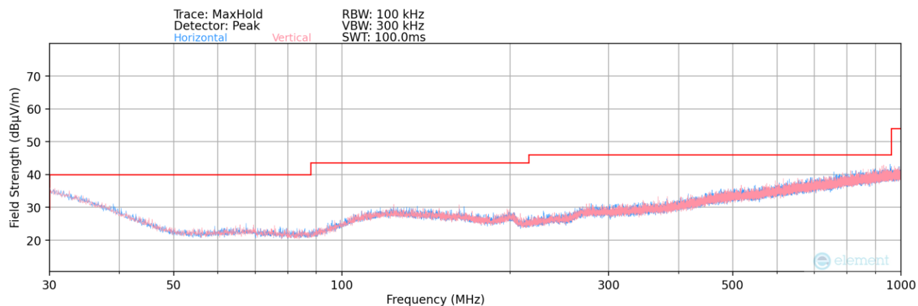
Plot 7-219. Radiated Spurious Plot below 1GHz – Dual
