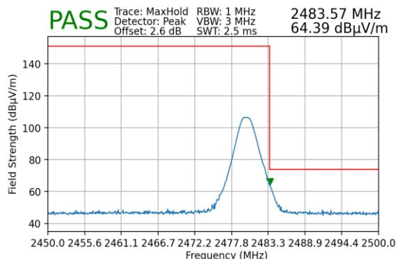
Plot 7-208. Radiated Restricted Upper Band Edge Measurement (Peak) – Ant 1 - WCP
