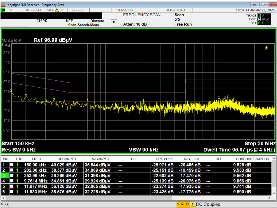
Plot 7-220. Line-Conducted Test Plot (L1)
