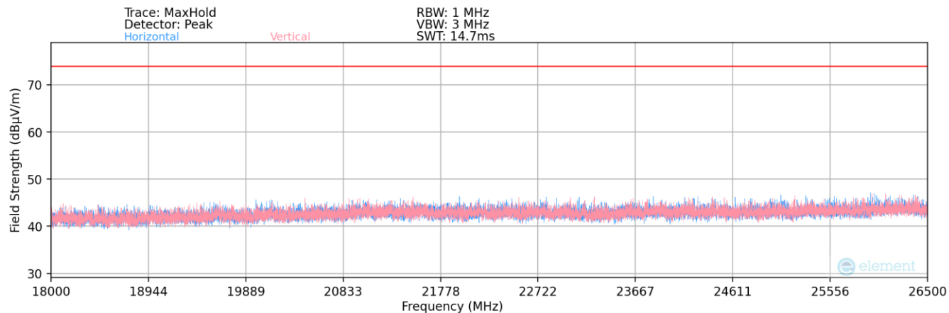
Plot 7-200. Radiated Spurious Plot above 18GHz (Bluetooth (LE)) – Ant 2
