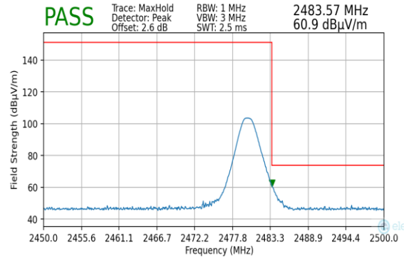
Plot 7-214. Radiated Restricted Upper Band Edge Measurement (Peak) – Dual
