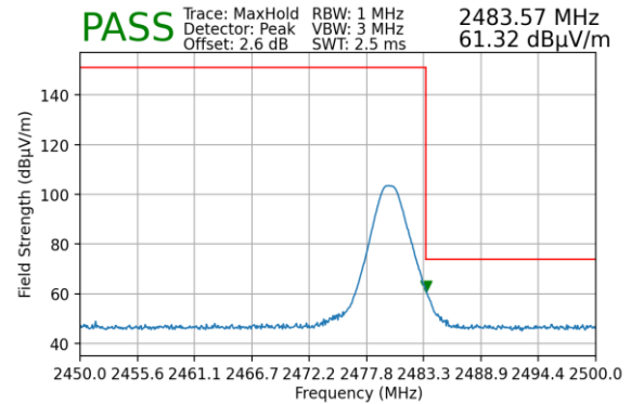
Plot 7-216. Radiated Restricted Upper Band Edge Measurement (Peak) – Dual - WCP
