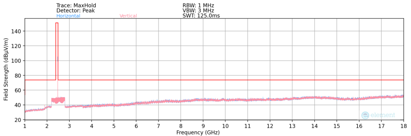
Plot 7-203. Radiated Spurious Plot above 1GHz (Bluetooth (LE) – Ch. 39) – Dual
