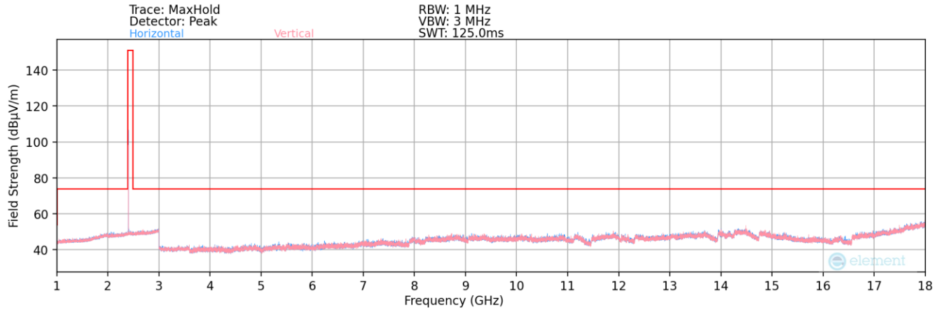
Plot 7-201. Radiated Spurious Plot above 1GHz (Bluetooth (LE) – Ch. 37) – Dual
