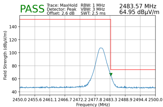
Plot 7-206. Radiated Restricted Upper Band Edge Measurement (Peak) – Ant 1
