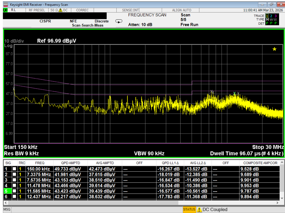
Plot 7-221. Line-Conducted Test Plot (L1) - WCP
