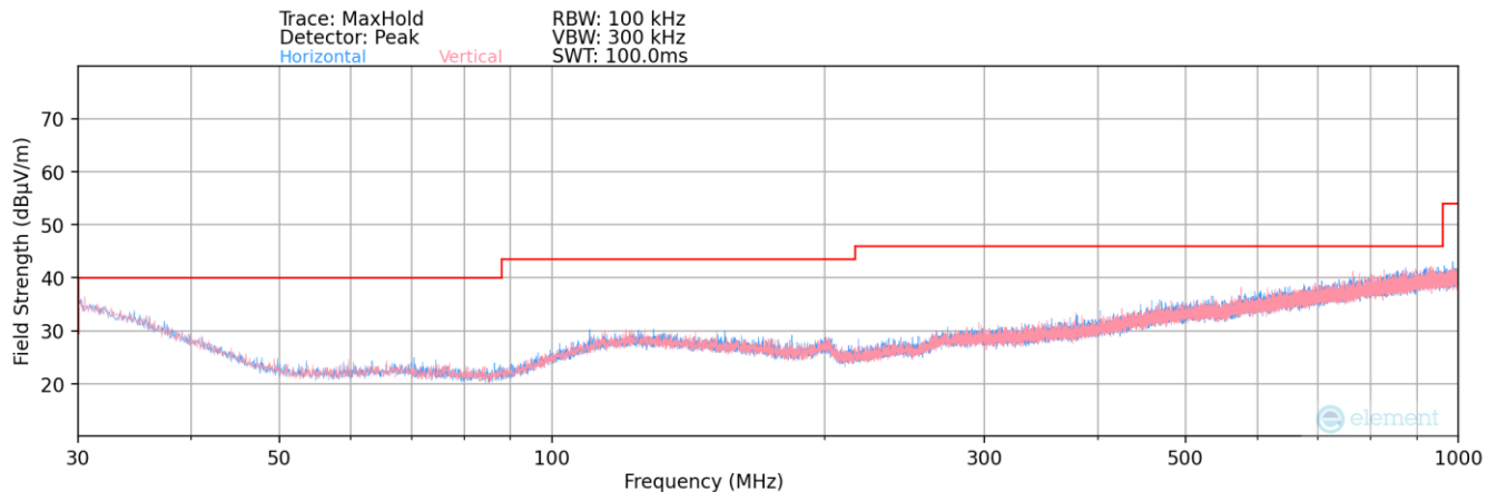
Plot 7-218. Radiated Spurious Plot below 1GHz – Ant 2
