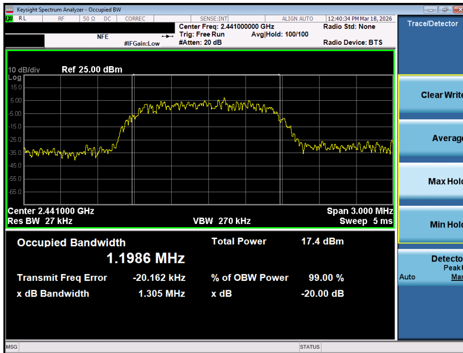
Plot 7-5. 20dB Bandwidth Plot (Bluetooth, 2Mbps - Ch. 39) - SISO ANT 1
