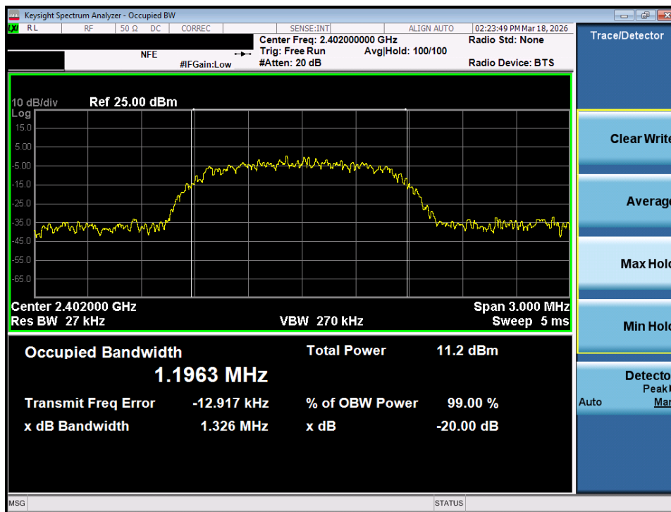
Plot 7-25. 20dB Bandwidth Plot (Bluetooth, 3Mbps – Ch. 0) – MIMO ANT 1
