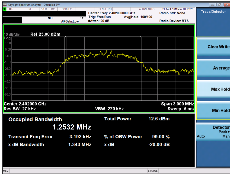
Plot 7-31. 20dB Bandwidth Plot (Bluetooth, 2Mbps – Ch. 0) – MIMO ANT 2
