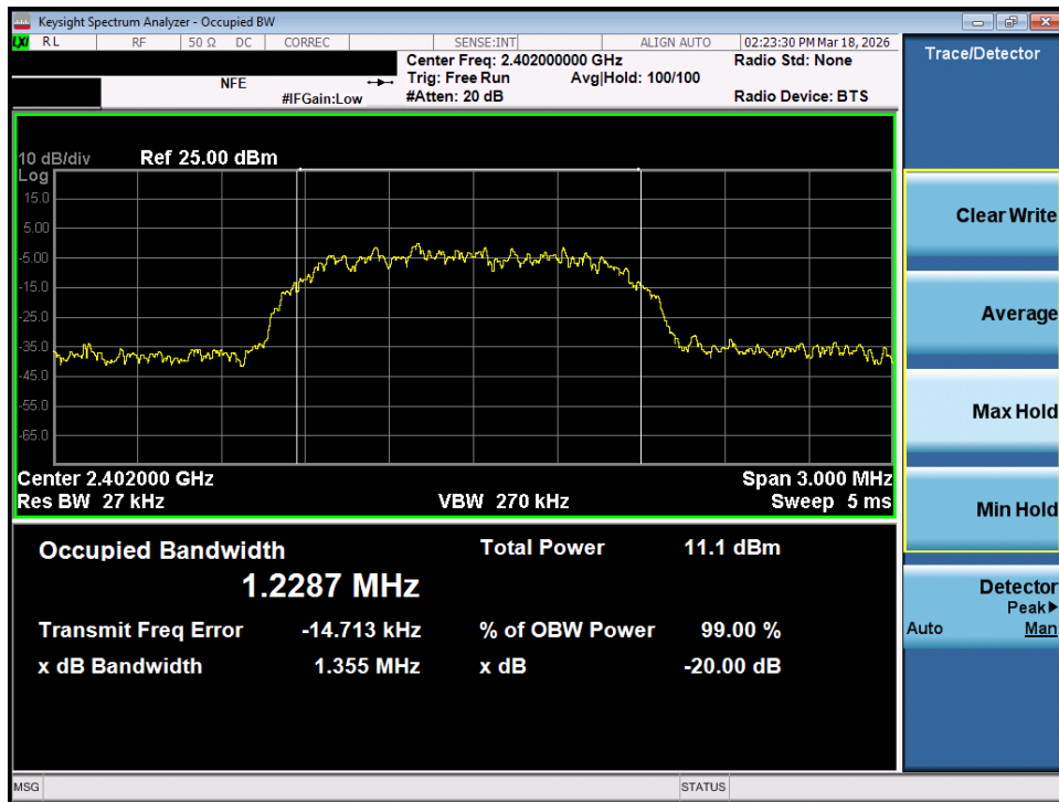
Plot 7-22. 20dB Bandwidth Plot (Bluetooth, 2Mbps - Ch. 0) - MIMO ANT 1
