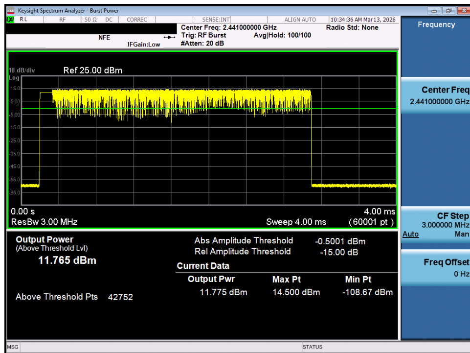
Plot 7-89. Average Conducted Power (3Mbps - Ch. 39) - MIMO ANT 1
