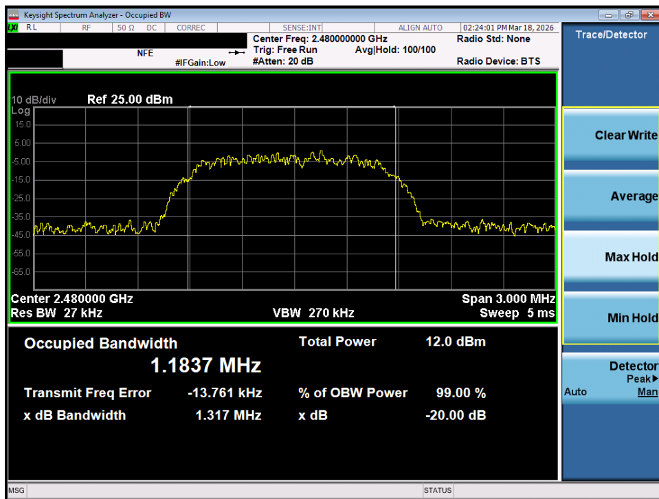
Plot 7-27. 20dB Bandwidth Plot (Bluetooth, 3Mbps – Ch. 78) – MIMO ANT 1
