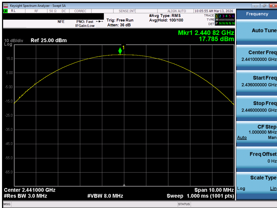
Plot 7-56. Peak Conducted Power (1Mbps – Ch. 39) – SISO ANT 2
