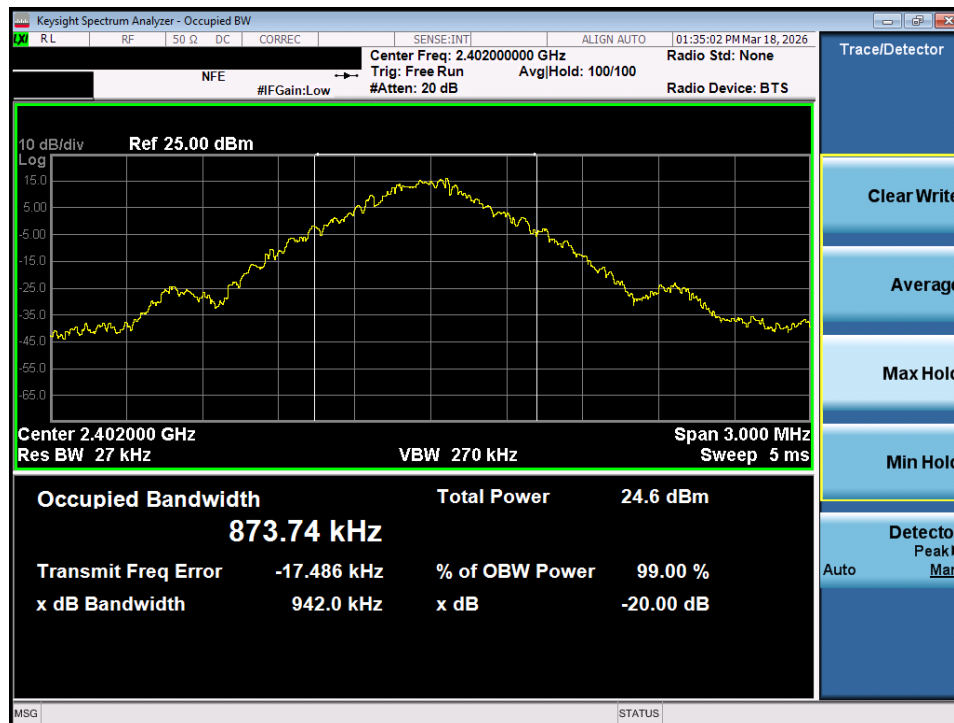
Plot 7-10. 20dB Bandwidth Plot (Bluetooth, 1Mbps – Ch. 0) – SISO ANT 2
