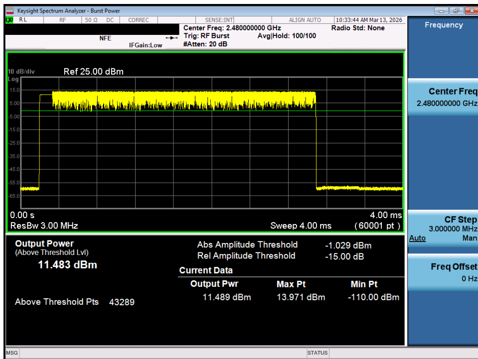
Plot 7-87. Average Conducted Power (2Mbps - Ch. 78) - MIMO ANT 1
