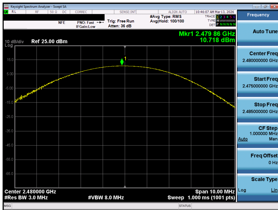
Plot 7-96. Peak Conducted Power (2Mbps – Ch. 78) – MIMO ANT 2
