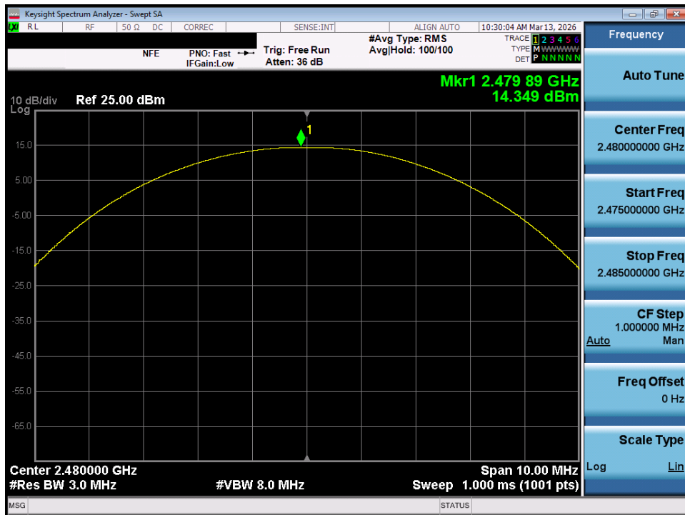
Plot 7-75. Peak Conducted Power (1Mbps – Ch. 78) – MIMO ANT 1
