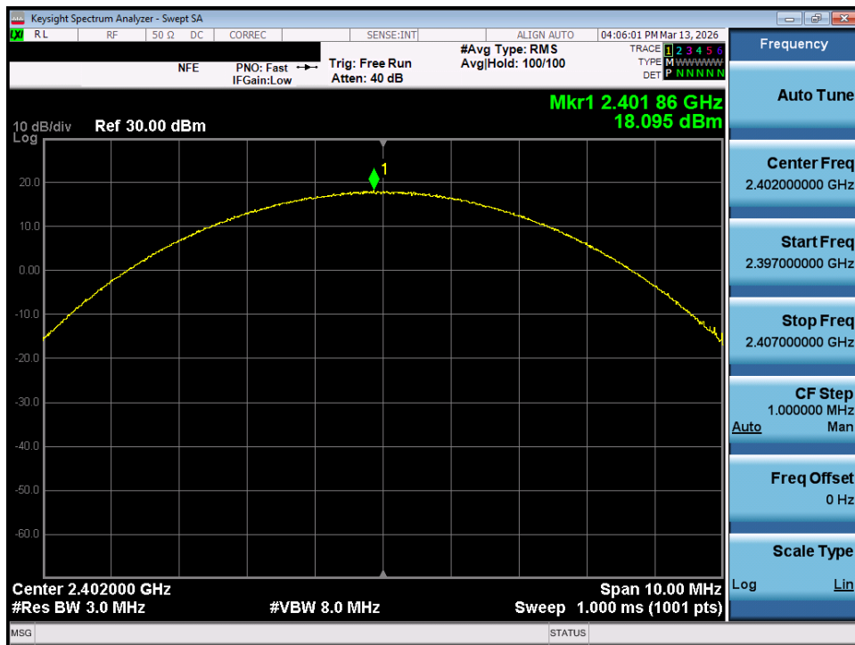
Plot 7-43. Peak Conducted Power (3Mbps – Ch. 0) – SISO ANT 1
