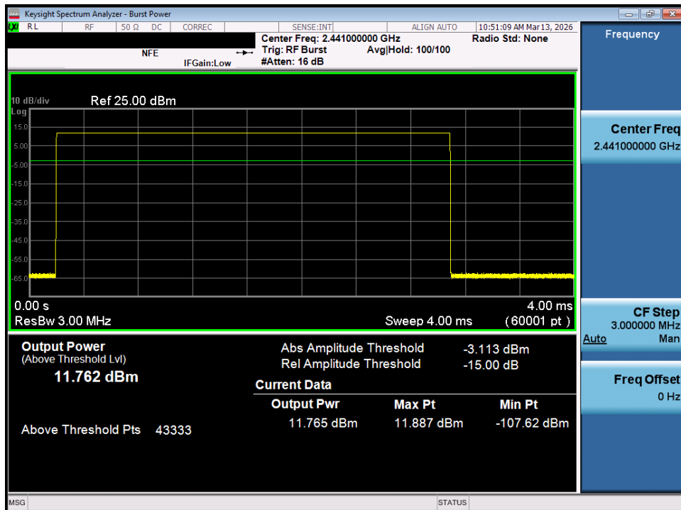
Plot 7-101. Average Conducted Power (1Mbps – Ch. 39) – MIMO ANT 2
