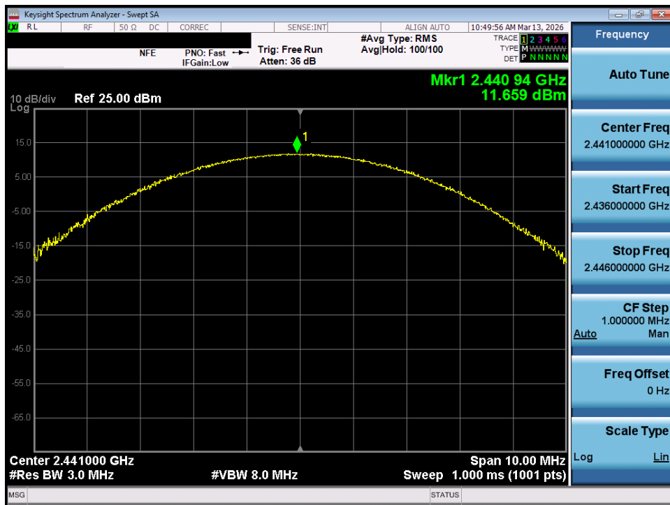
Plot 7-98. Peak Conducted Power (3Mbps – Ch. 39) – MIMO ANT 2
