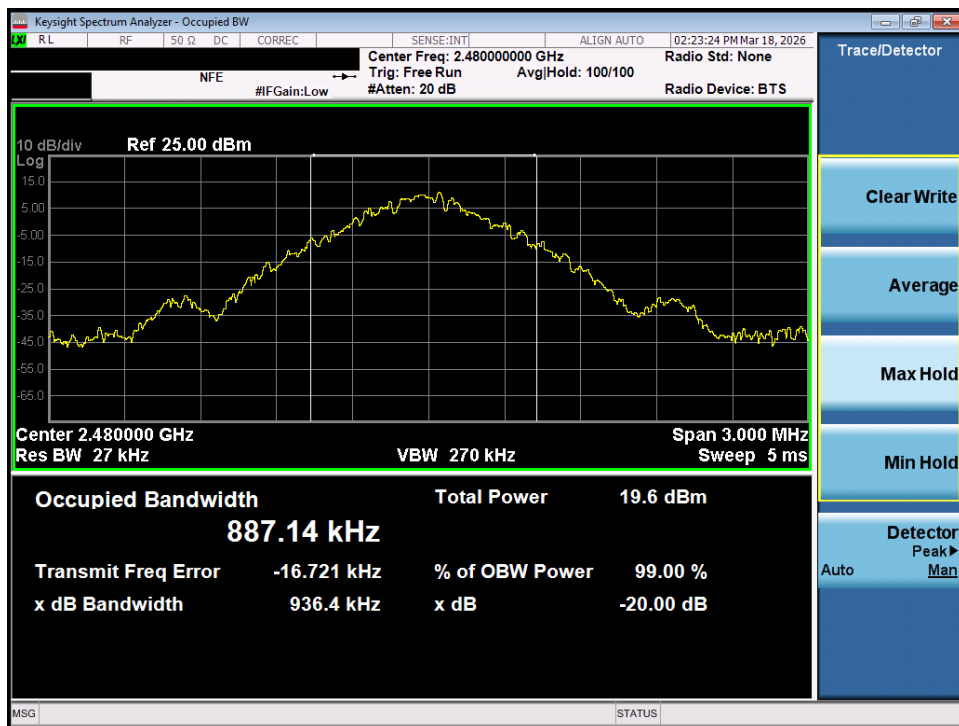
Plot 7-21. 20dB Bandwidth Plot (Bluetooth, 1Mbps – Ch. 78) – MIMO ANT 1
