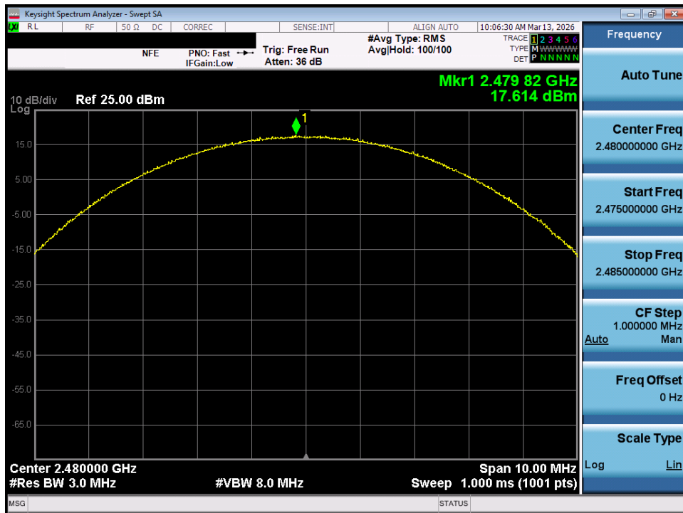
Plot 7-60. Peak Conducted Power (2Mbps – Ch. 78) – SISO ANT 2
