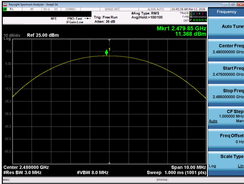
Plot 7-93. Peak Conducted Power (1Mbps – Ch. 78) – MIMO ANT 2
