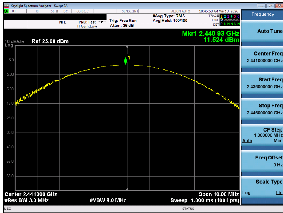
Plot 7-95. Peak Conducted Power (2Mbps – Ch. 39) – MIMO ANT 2
