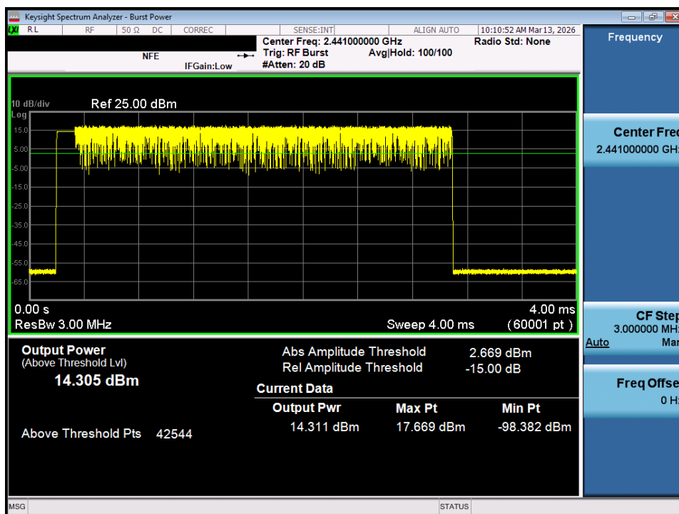
Plot 7-71. Average Conducted Power (3Mbps – Ch. 39) – SISO ANT 2
