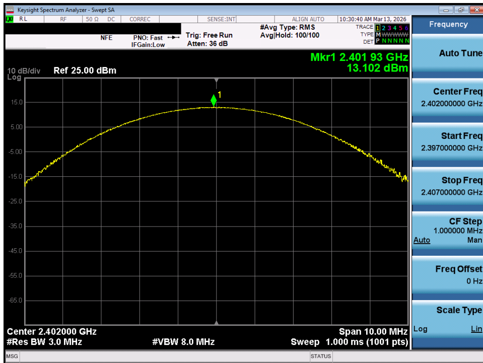
Plot 7-79. Peak Conducted Power (3Mbps – Ch. 0) – MIMO ANT 1
