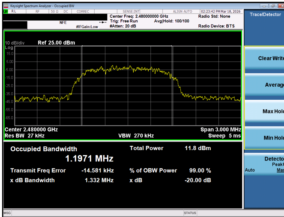
Plot 7-24. 20dB Bandwidth Plot (Bluetooth, 2Mbps – Ch. 78) – MIMO ANT 1
