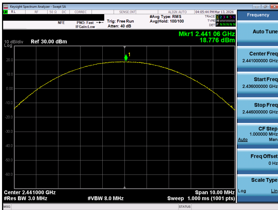
Plot 7-41. Peak Conducted Power (2Mbps – Ch. 39) – SISO ANT 1
