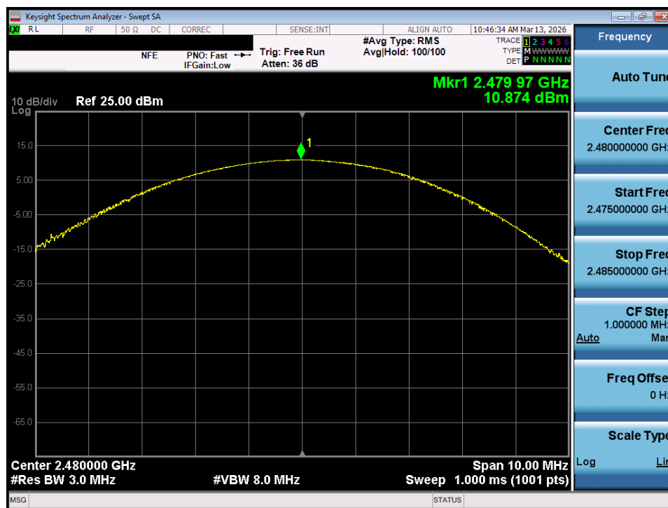
Plot 7-99. Peak Conducted Power (3Mbps – Ch. 78) – MIMO ANT 2
