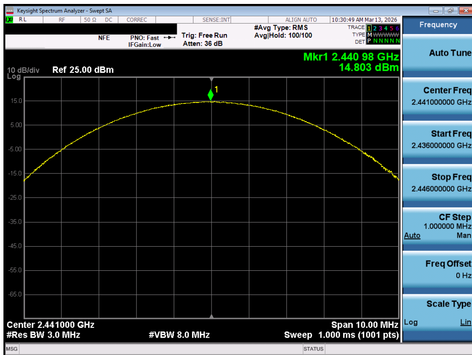
Plot 7-80. Peak Conducted Power (3Mbps – Ch. 39) – MIMO ANT 1
