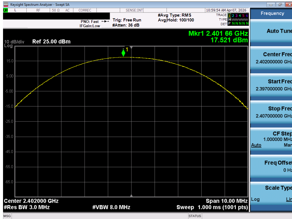
Plot 7-58. Peak Conducted Power (2Mbps – Ch. 0) – SISO ANT 2
