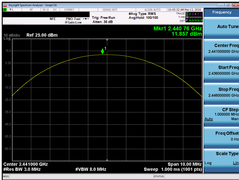
Plot 7-92. Peak Conducted Power (1Mbps – Ch. 39) – MIMO ANT 2
