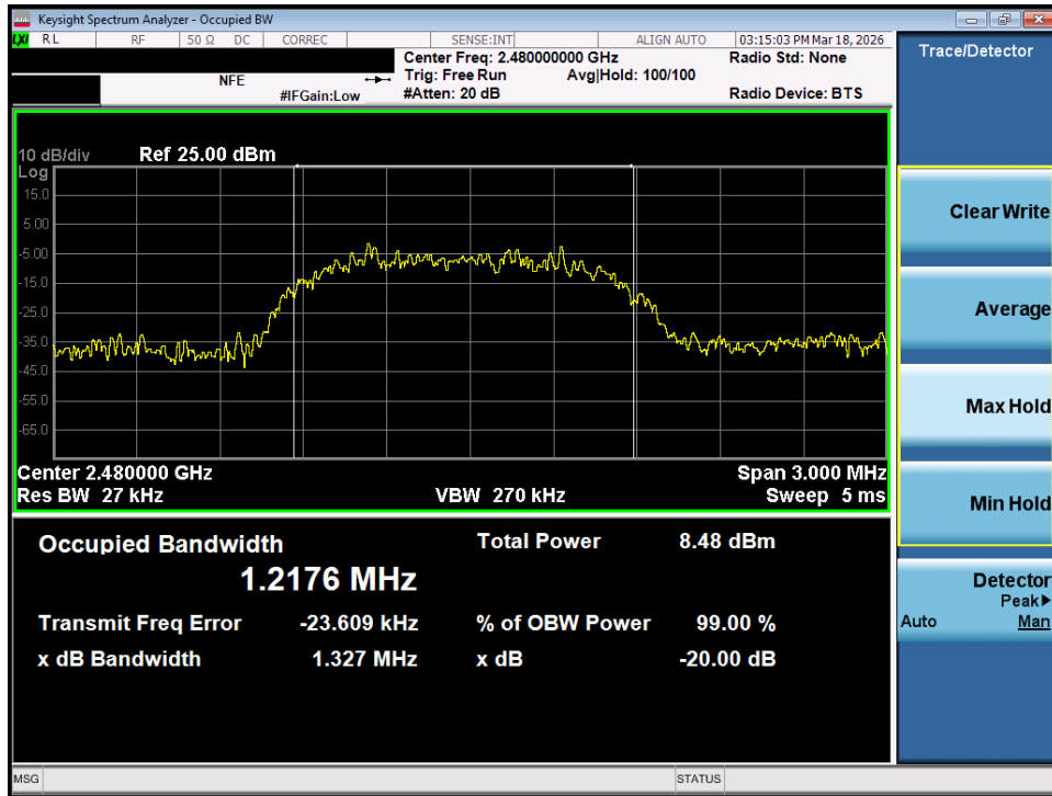
Plot 7-33. 20dB Bandwidth Plot (Bluetooth, 2Mbps – Ch. 78) – MIMO ANT 2
