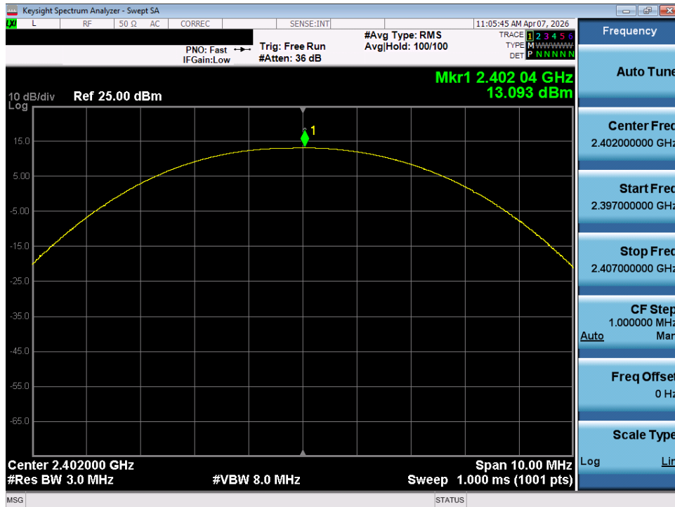
Plot 7-73. Peak Conducted Power (1Mbps – Ch. 0) – MIMO ANT 1
