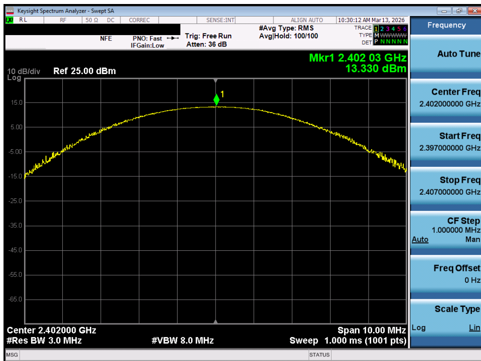
Plot 7-76. Peak Conducted Power (2Mbps – Ch. 0) – MIMO ANT 1
