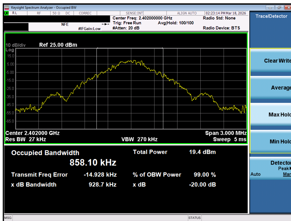
Plot 7-19. 20dB Bandwidth Plot (Bluetooth, 1Mbps – Ch. 0) – MIMO ANT 1
