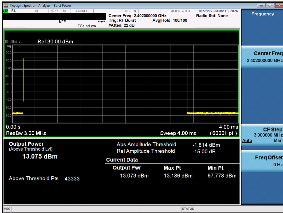
Plot 7-82. Average Conducted Power (1Mbps – Ch. 0) – MIMO ANT 1
