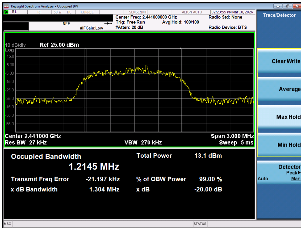
Plot 7-26. 20dB Bandwidth Plot (Bluetooth, 3Mbps – Ch. 39) – MIMO ANT 1
