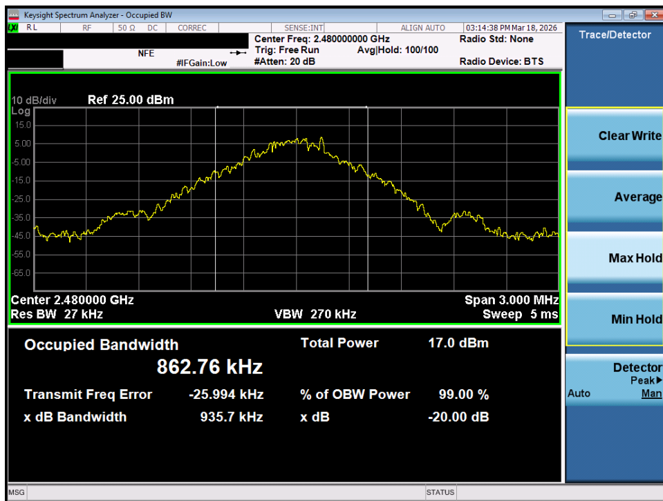
Plot 7-30. 20dB Bandwidth Plot (Bluetooth, 1Mbps – Ch. 78) – MIMO ANT 2
