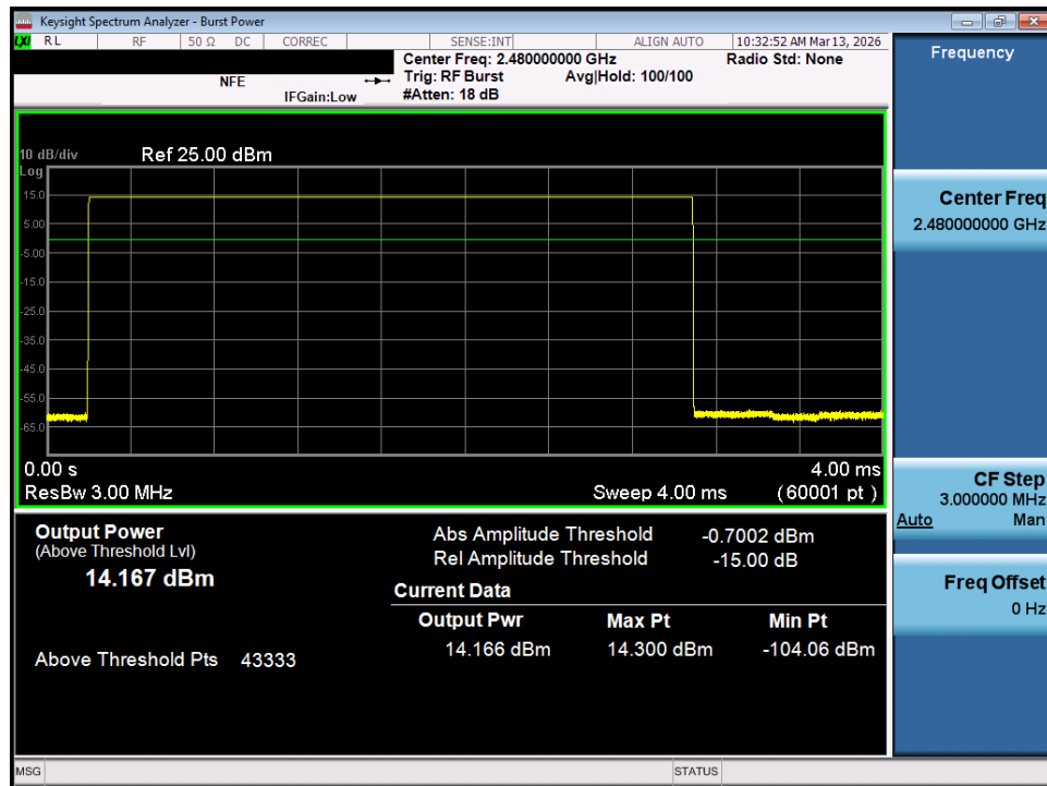
Plot 7-84. Average Conducted Power (1Mbps - Ch. 78) - MIMO ANT 1
