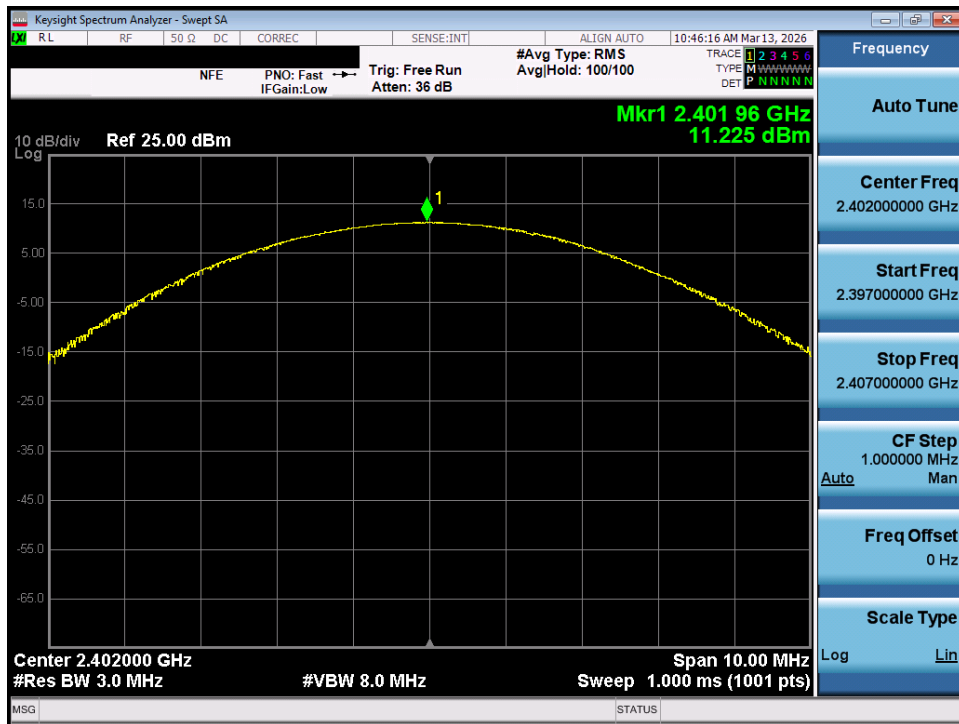
Plot 7-97. Peak Conducted Power (3Mbps – Ch. 0) – MIMO ANT 2
