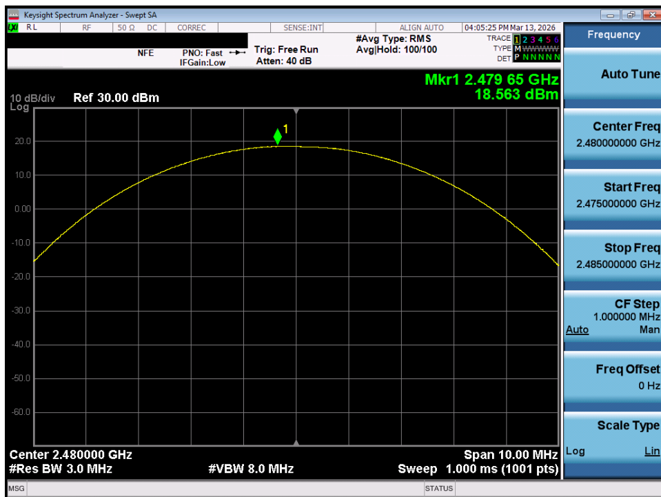
Plot 7-39. Peak Conducted Power (1Mbps - Ch. 78) – SISO ANT 1
