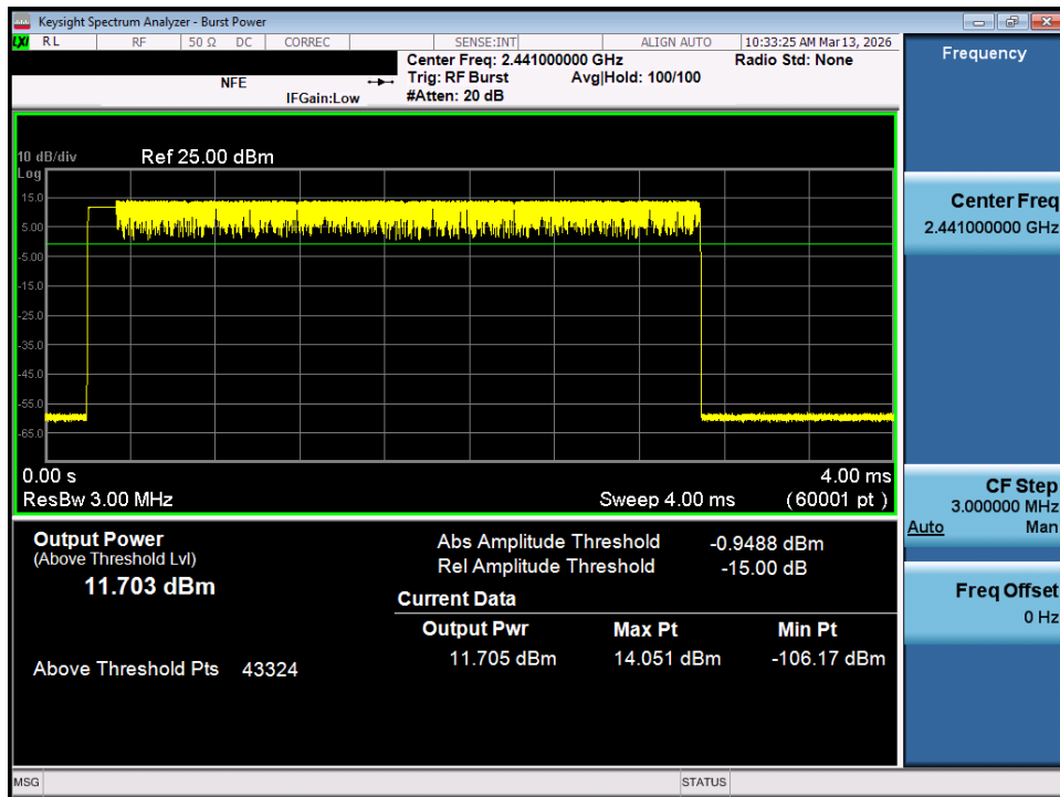
Plot 7-86. Average Conducted Power (2Mbps - Ch. 39) - MIMO ANT 1
