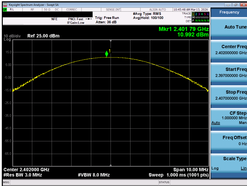
Plot 7-94. Peak Conducted Power (2Mbps – Ch. 0) – MIMO ANT 2
