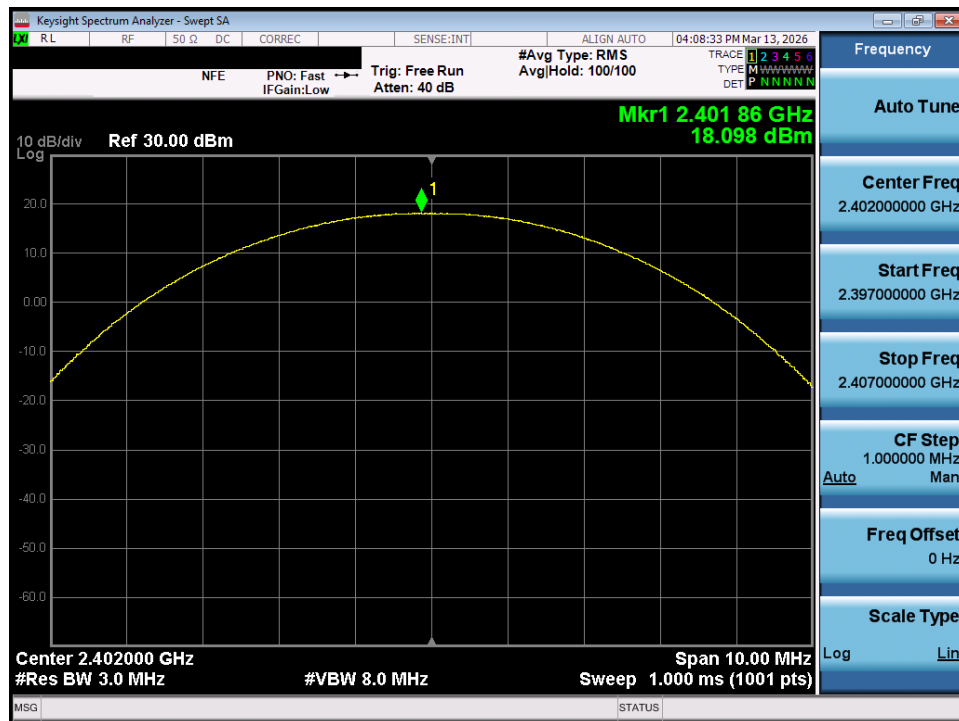
Plot 7-37. Peak Conducted Power (1Mbps – Ch. 0) – SISO ANT 1
