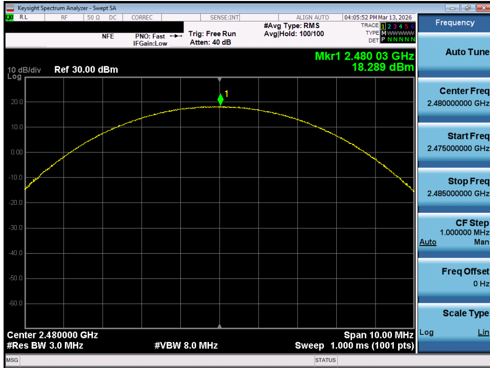
Plot 7-42. Peak Conducted Power (2Mbps – Ch. 78) – SISO ANT 1
