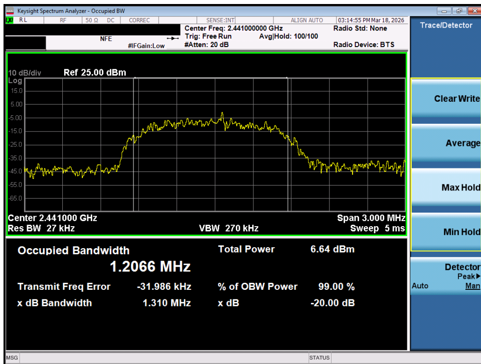
Plot 7-32. 20dB Bandwidth Plot (Bluetooth, 2Mbps – Ch. 39) – MIMO ANT 2
