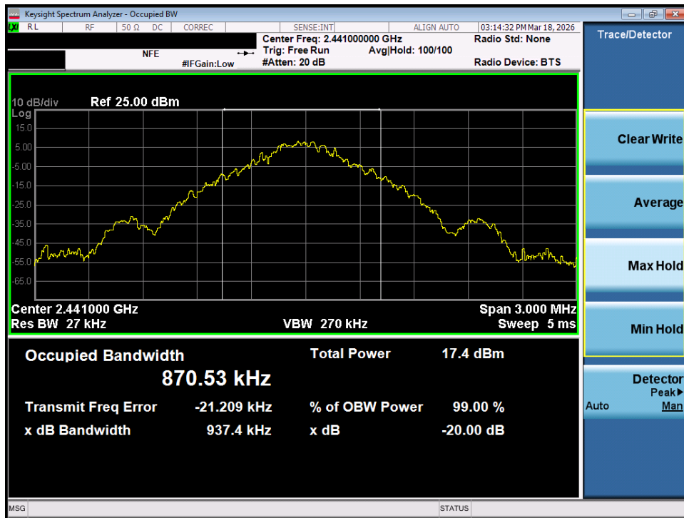
Plot 7-29. 20dB Bandwidth Plot (Bluetooth, 1Mbps – Ch. 39) – MIMO ANT 2
