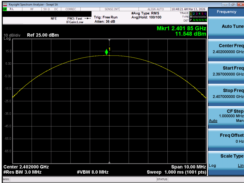
Plot 7-91. Peak Conducted Power (1Mbps – Ch. 0) – MIMO ANT 2
