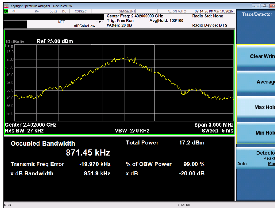
Plot 7-28. 20dB Bandwidth Plot (Bluetooth, 1Mbps – Ch. 0) – MIMO ANT 2
