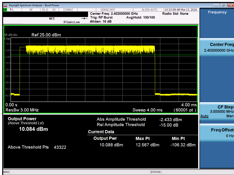
Plot 7-85. Average Conducted Power (2Mbps - Ch. 0) - MIMO ANT 1
