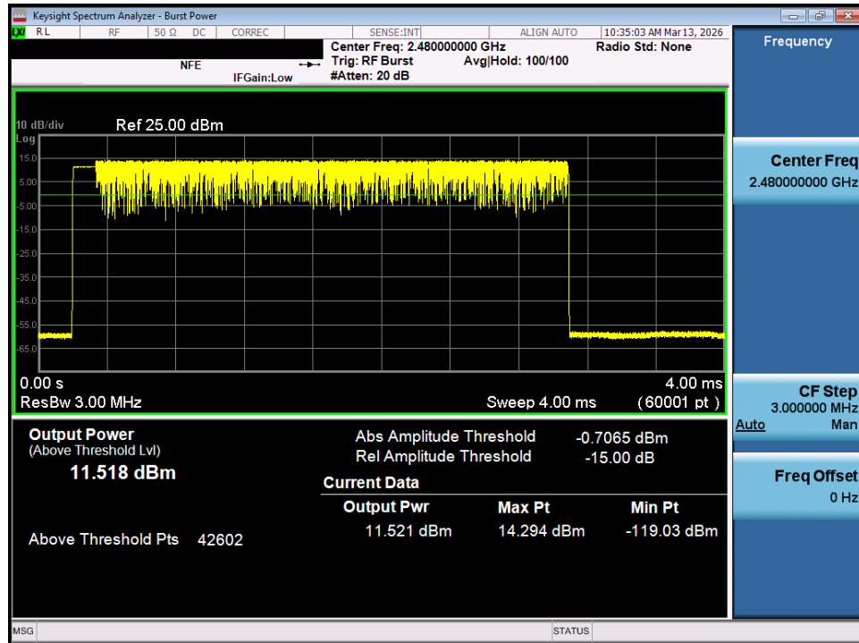
Plot 7-90. Average Conducted Power (3Mbps - Ch. 78) - MIMO ANT 1
