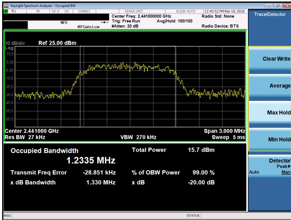
Plot 7-8. 20dB Bandwidth Plot (Bluetooth, 3Mbps – Ch. 39) – SISO ANT 1
