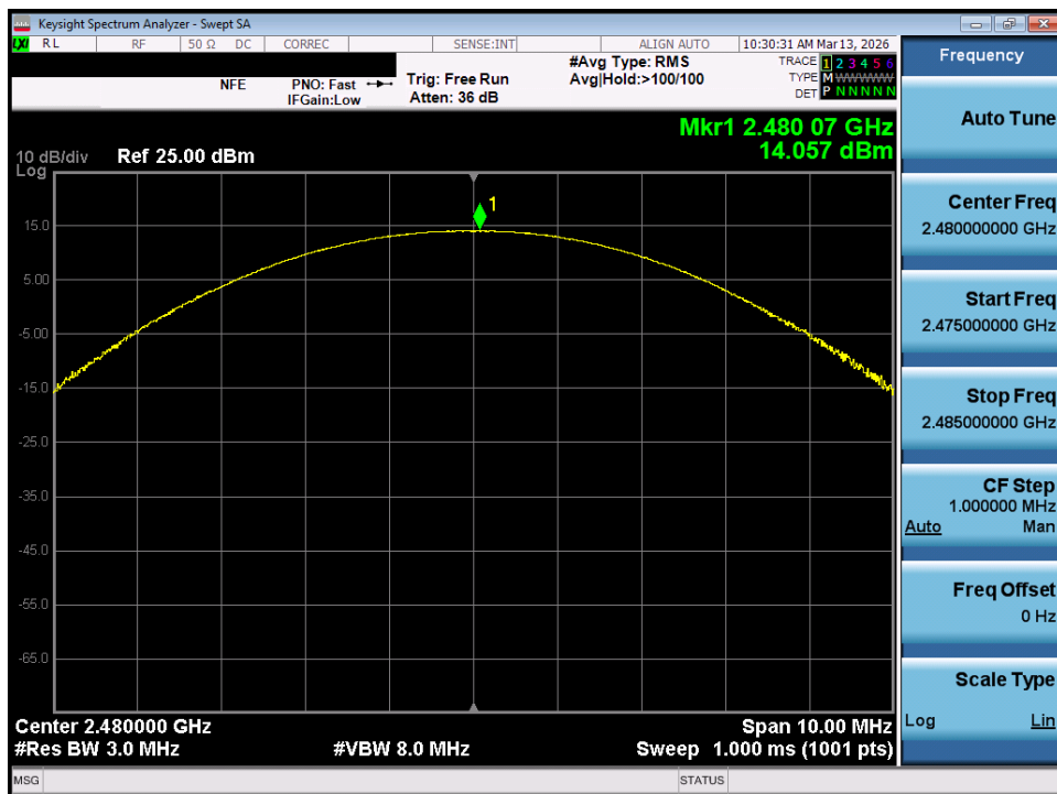
Plot 7-78. Peak Conducted Power (2Mbps – Ch. 78) – MIMO ANT 1
