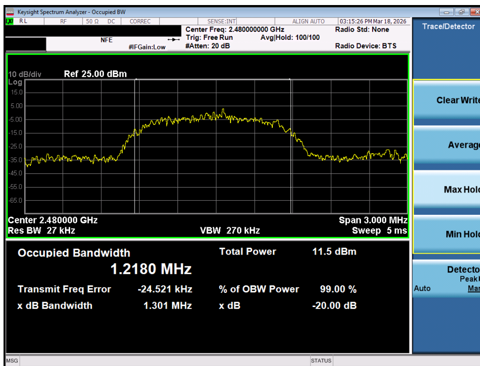
Plot 7-36. 20dB Bandwidth Plot (Bluetooth, 3Mbps – Ch. 78) – MIMO ANT 2
