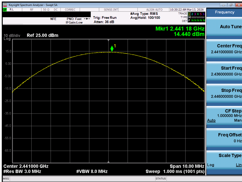
Plot 7-77. Peak Conducted Power (2Mbps – Ch. 39) – MIMO ANT 1
