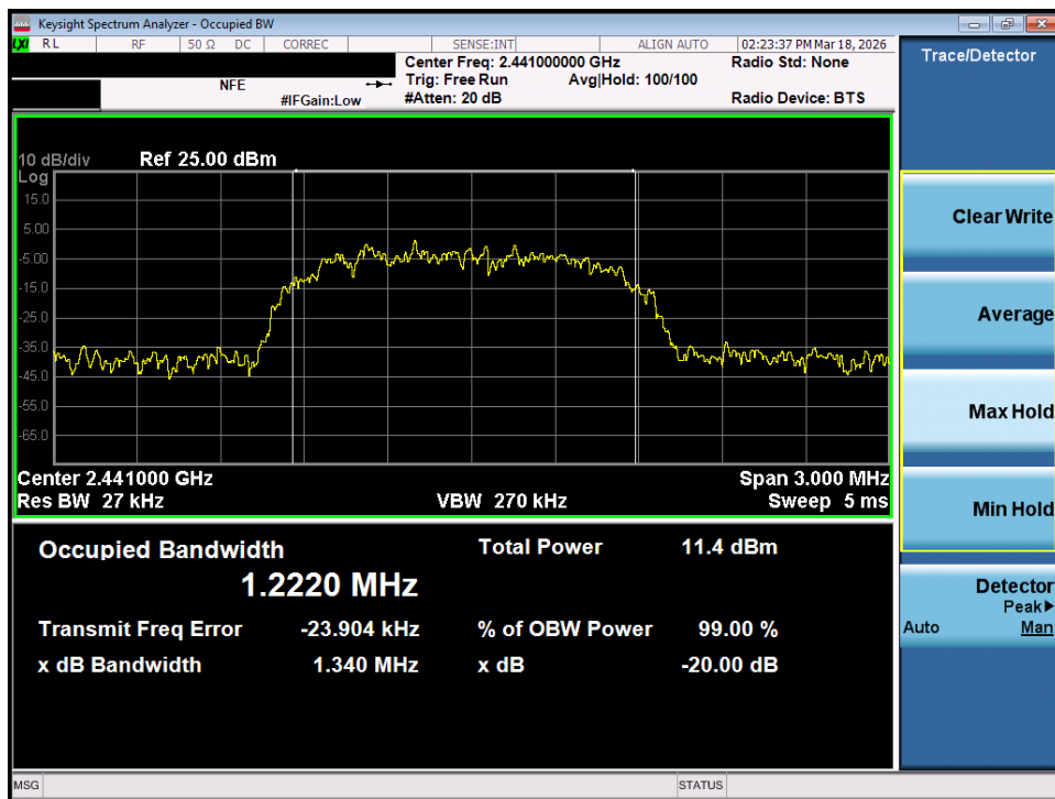
Plot 7-23. 20dB Bandwidth Plot (Bluetooth, 2Mbps - Ch. 39) - MIMO ANT 1
