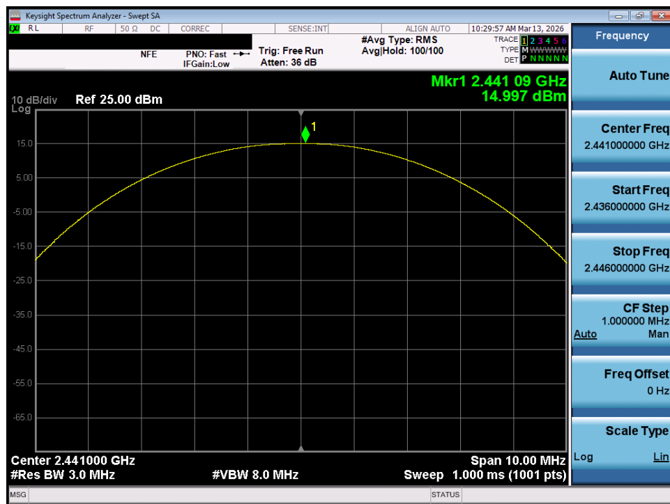
Plot 7-74. Peak Conducted Power (1Mbps – Ch. 39) – MIMO ANT 1
