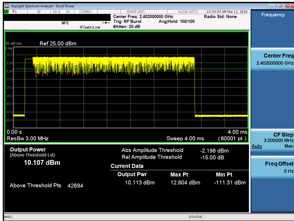
Plot 7-88. Average Conducted Power (3Mbps - Ch. 0) - MIMO ANT 1
