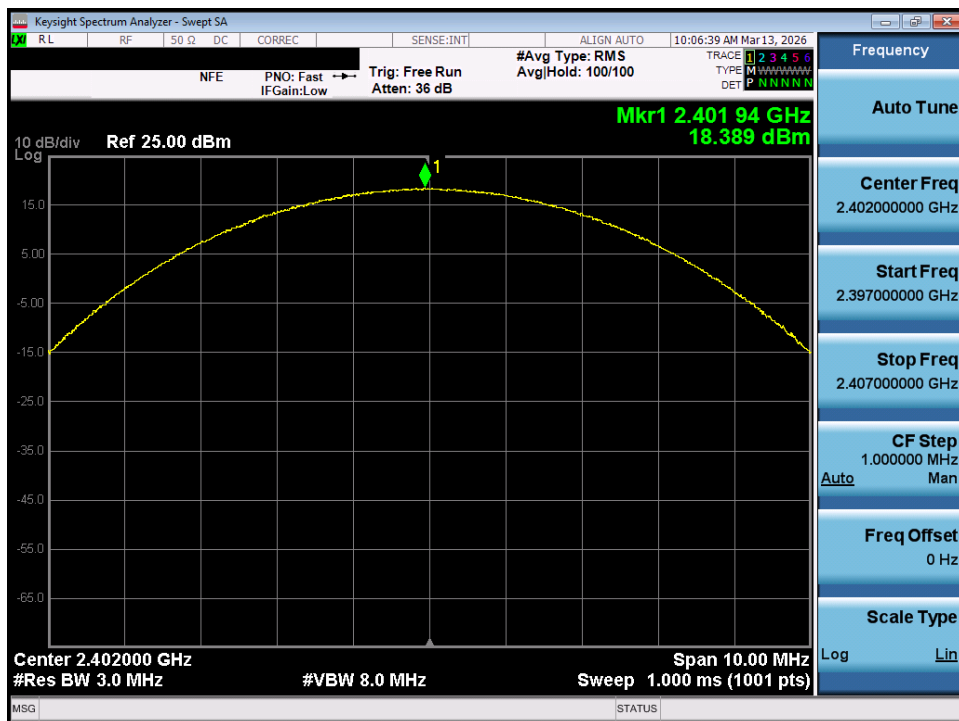
Plot 7-61. Peak Conducted Power (3Mbps – Ch. 0) – SISO ANT 2
