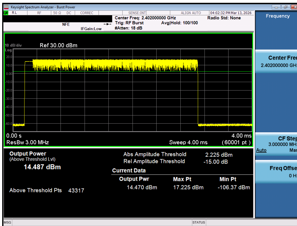
Plot 7-49. Average Conducted Power (2Mbps – Ch. 0) – SISO ANT 1
