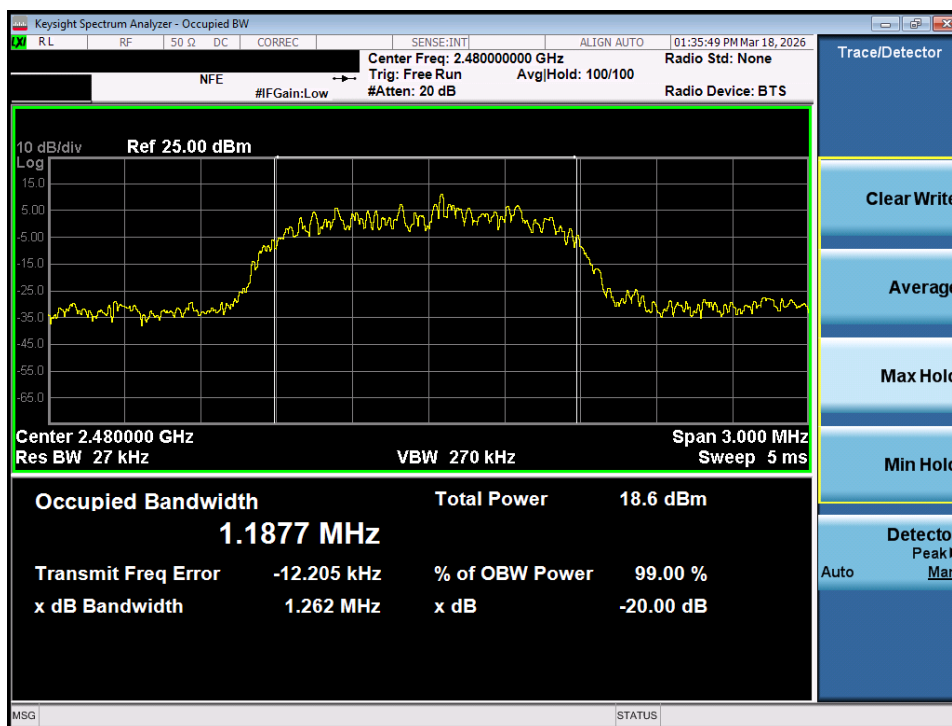
Plot 7-18. 20dB Bandwidth Plot (Bluetooth, 3Mbps – Ch. 78) – SISO ANT 2
