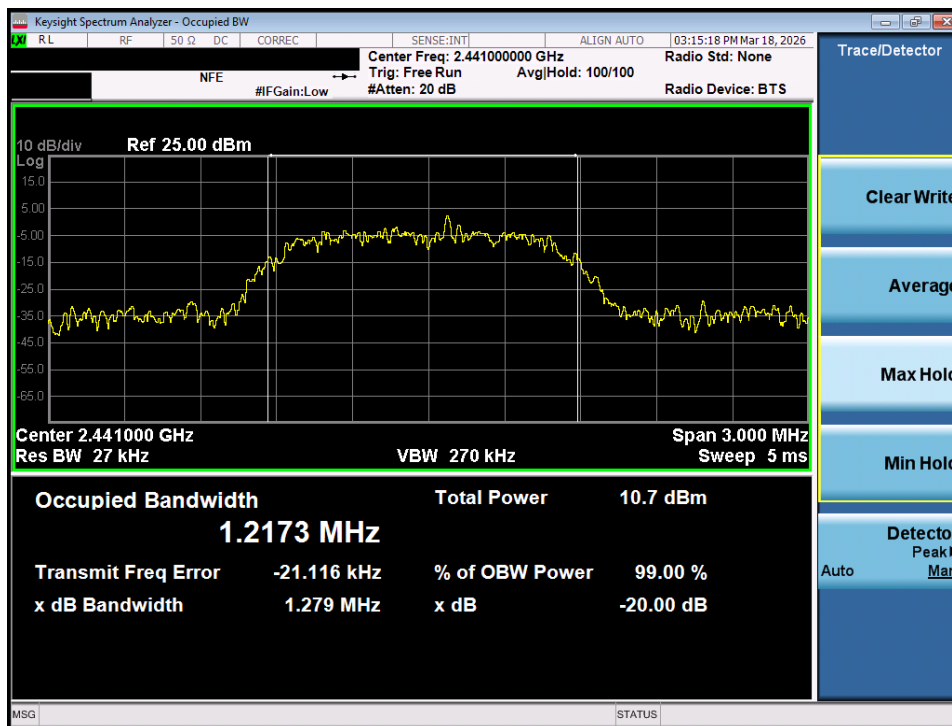
Plot 7-35. 20dB Bandwidth Plot (Bluetooth, 3Mbps – Ch. 39) – MIMO ANT 2
