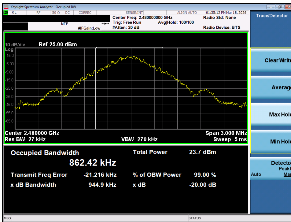
Plot 7-12. 20dB Bandwidth Plot (Bluetooth, 1Mbps – Ch. 78) – SISO ANT 2
