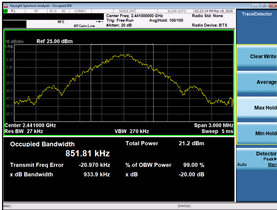
Plot 7-20. 20dB Bandwidth Plot (Bluetooth, 1Mbps – Ch. 39) – MIMO ANT 1
