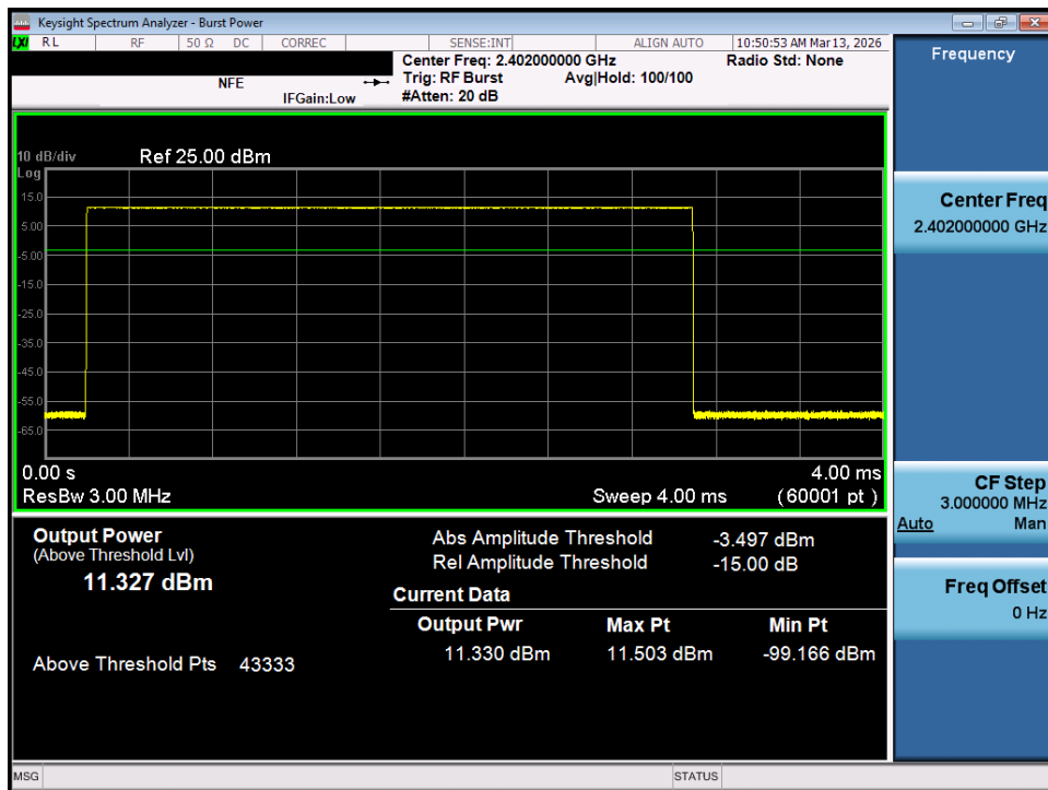
Plot 7-100. Average Conducted Power (1Mbps – Ch. 0) – MIMO ANT 2
