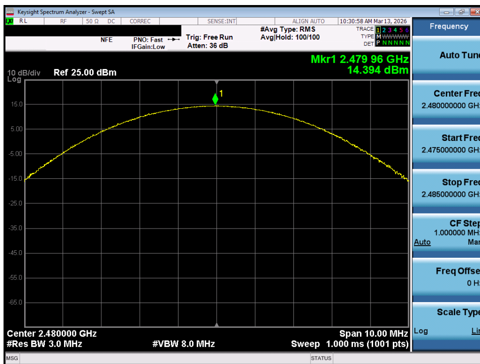
Plot 7-81. Peak Conducted Power (3Mbps – Ch. 78) – MIMO ANT 1
