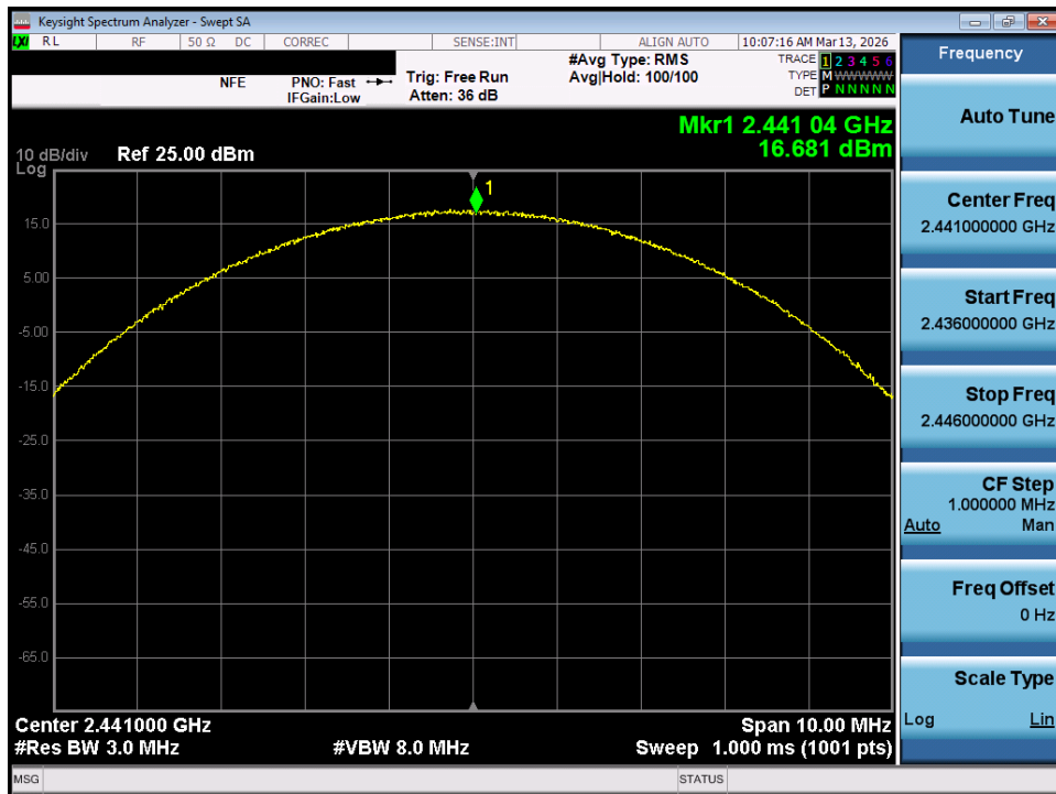
Plot 7-62. Peak Conducted Power (3Mbps – Ch. 39) – SISO ANT 2
