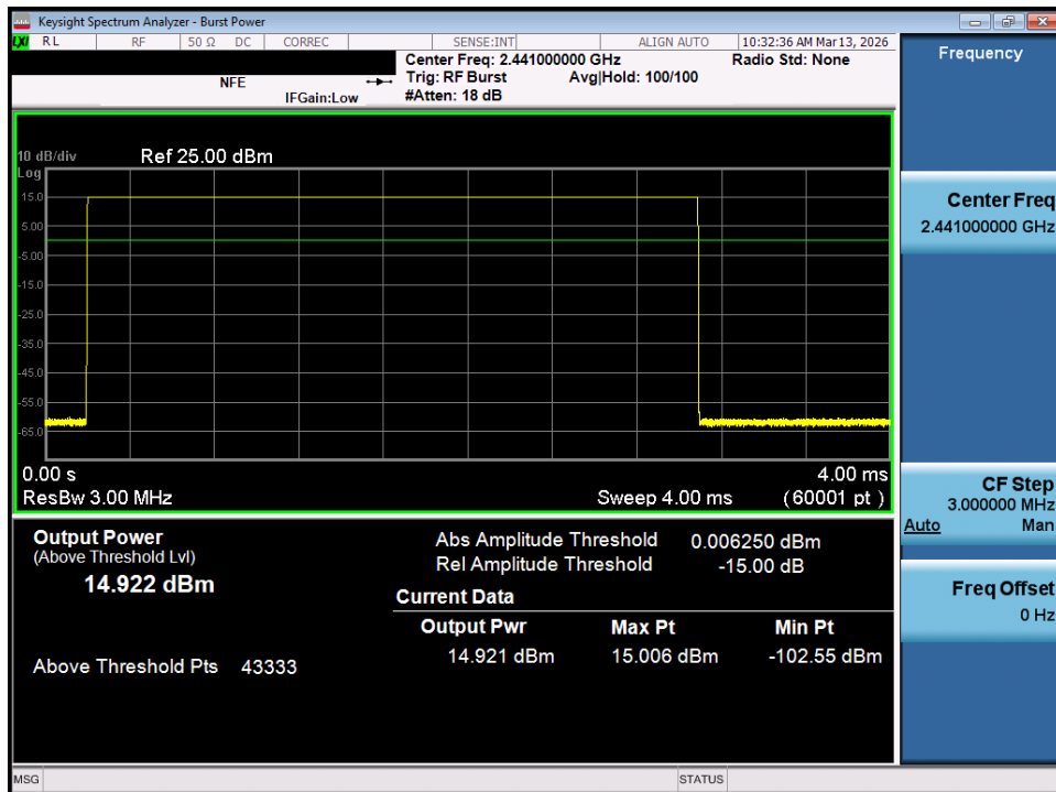
Plot 7-83. Average Conducted Power (1Mbps – Ch. 39) – MIMO ANT 1
