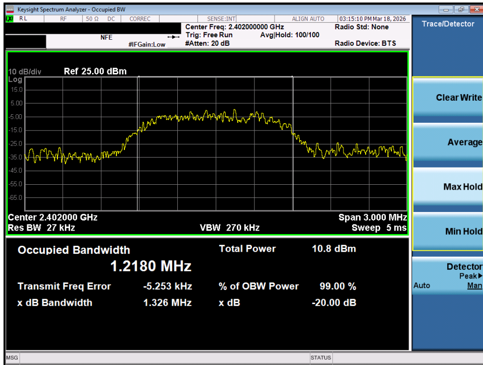
Plot 7-34. 20dB Bandwidth Plot (Bluetooth, 3Mbps – Ch. 0) – MIMO ANT 2
