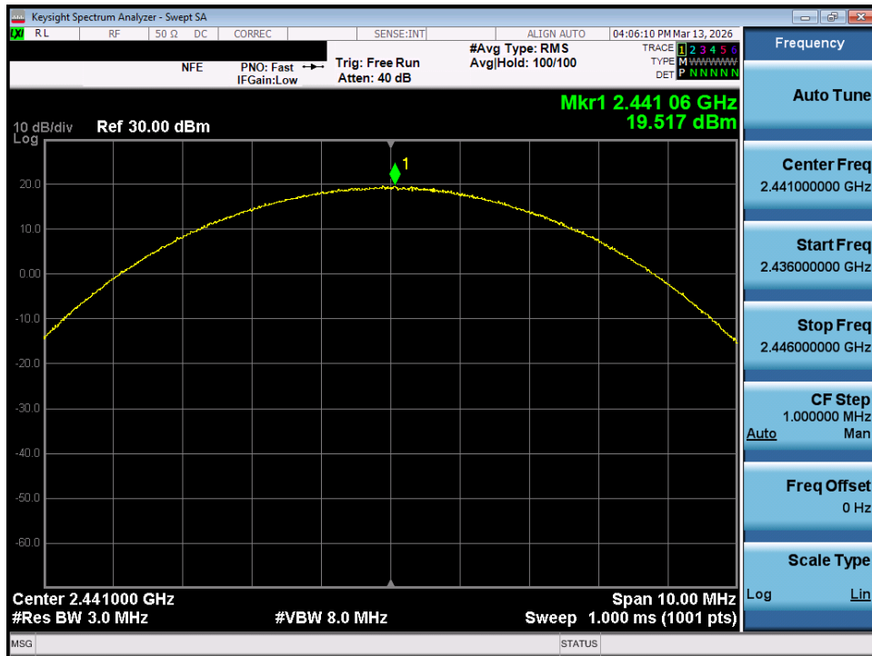
Plot 7-44. Peak Conducted Power (3Mbps – Ch. 39) – SISO ANT 1
