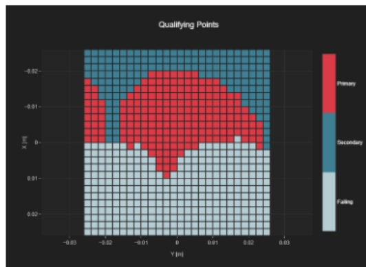
Figure 14-6 Worst-Case Scan Results for WIFI VoWIFI 2.4GHz, MIMO, IEEE 802.11n SU, CH.6, EVS WB 6.60KBPS
