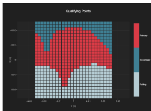
Figure 14-1 Worst-Case Scan Results for GSM GSM 1900, ANT B, CH.661, EFR: FR V2
