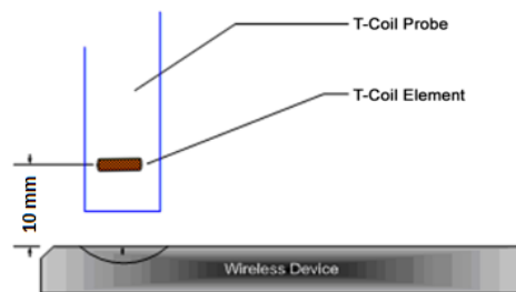
Figure 4-5 Measurement Distance
