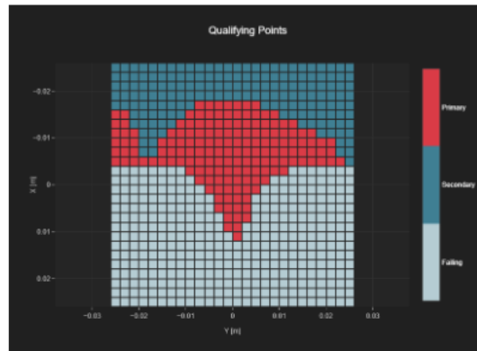
Figure 14-3 Worst-Case Scan Results for LTE VoLTE TDD Band 41 (PC3), ANT H, CH.40185, EVS WB 5.90KBPS
