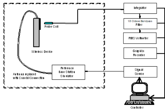
Figure 4-7 Audio Magnetic Field Test Setup
