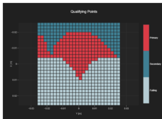
Figure 14-8 Worst-Case Scan Results for OTT VoIP TDD Band n38 (PC2), Ant H, PC2, CH.516500, OPUS 6KBPS
