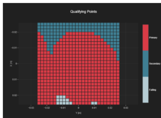
Figure 14-2 Worst-Case Scan Results for UMTS UMTS Band 5, Ant E, CH.4233, AMR WB 6.60KBPS
