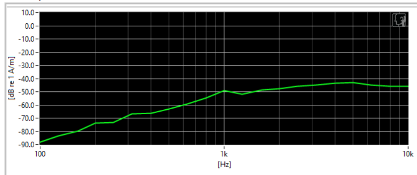
P 50 Frequency Response
