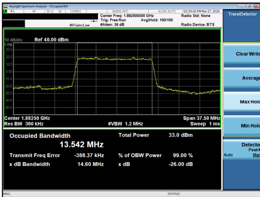
Plot 7-31. Occupied Bandwidth Plot (NR Band n25/2 - 15.0MHz DFT-s-OFDM BPSK - Full RB - ANT1)
