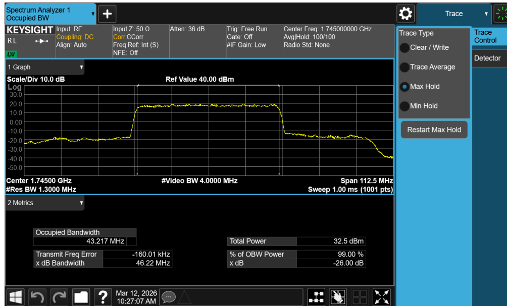
Plot 7-73. Occupied Bandwidth Plot (NR Band n66 - 45.0MHz DFT-s-OFDM BPSK - Full RB – ANT1)
