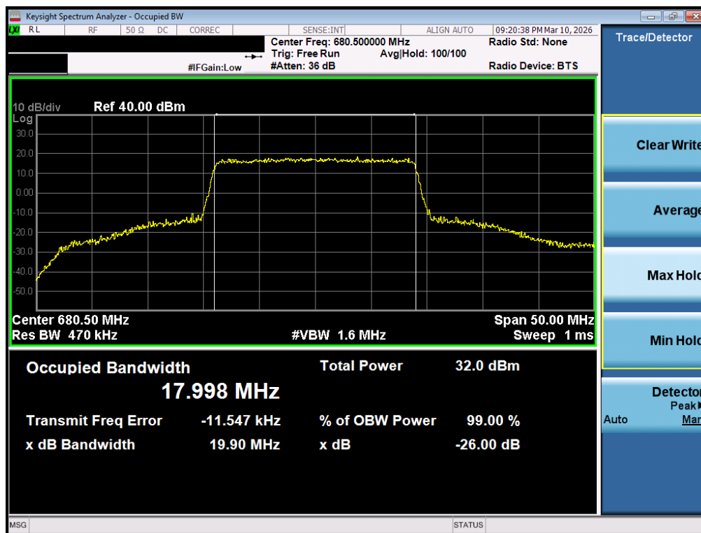
Plot 7-3. Occupied Bandwidth Plot (LTE Band 71 - 20MHz 16-QAM - Full RB – ANT1)
