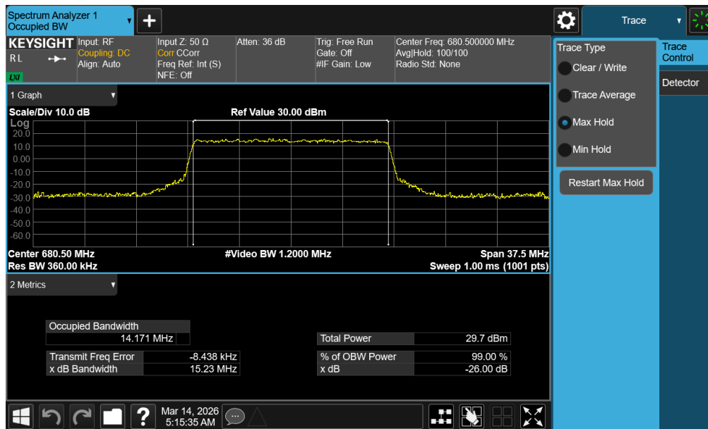
Plot 7-57. Occupied Bandwidth Plot (NR Band n71 - 15MHz CP-OFDM 16-QAM - Full RB – ANT1)
