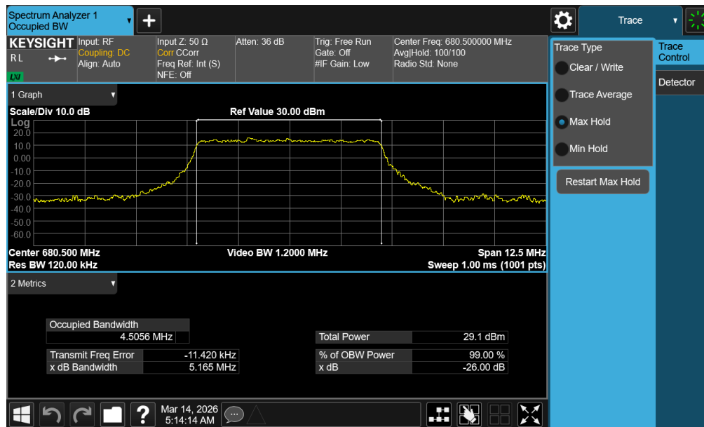
Plot 7-63. Occupied Bandwidth Plot (NR Band n71 - 5MHz CP-OFDM 16-QAM - Full RB – ANT1)
