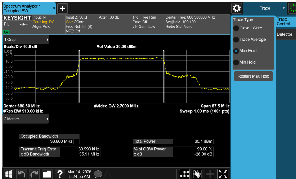
Plot 7-44. Occupied Bandwidth Plot (NR Band n71 - 35MHz CP-OFDM QPSK - Full RB – ANT1)
