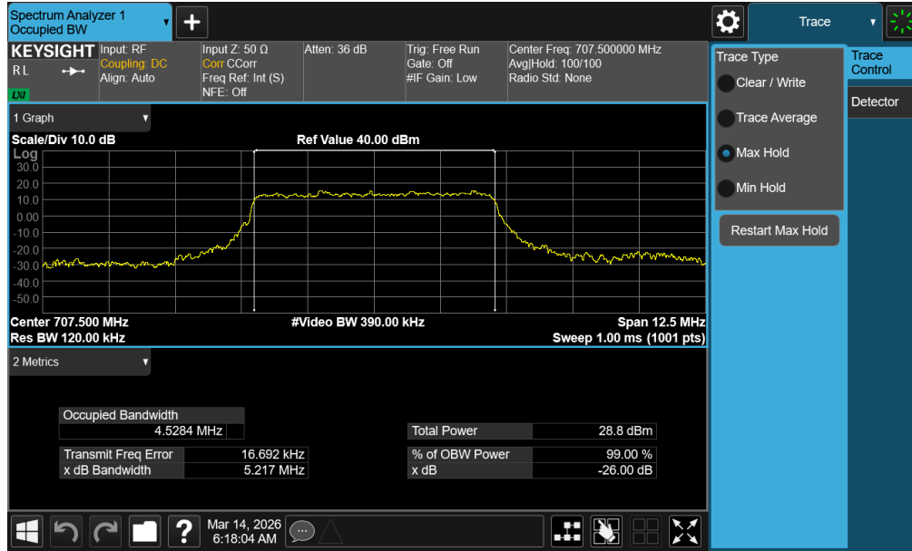
Plot 7-42. Occupied Bandwidth Plot (NR Band n12 - 5MHz CP-OFDM 16-QAM - Full RB – ANT1)
