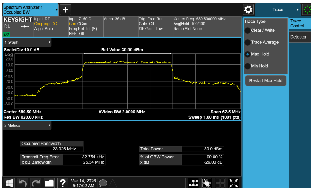
Plot 7-50. Occupied Bandwidth Plot (NR Band n71 – 25MHz CP-OFDM QPSK - Full RB – ANT1)
