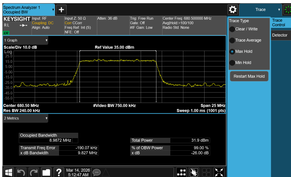
Plot 7-58. Occupied Bandwidth Plot (NR Band n71 - 10MHz DFT-s-OFDM BPSK - Full RB – ANT1)
