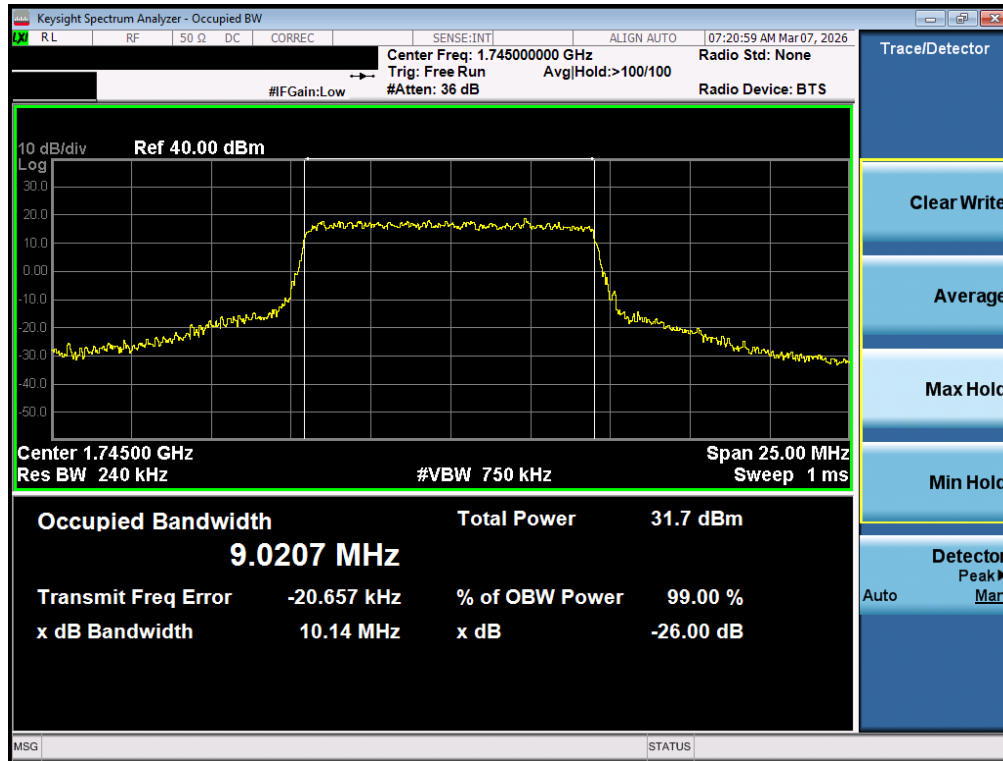
Plot 7-26. Occupied Bandwidth Plot (LTE Band 66/4 - 10MHz QPSK - Full RB - ANT1)
