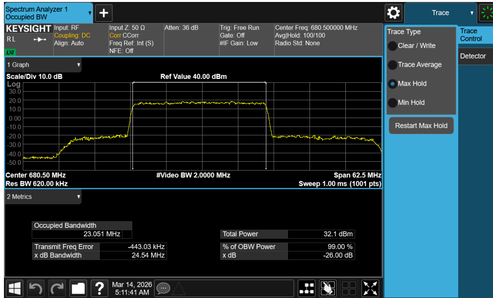
Plot 7-49. Occupied Bandwidth Plot (NR Band n71 - 25MHz DFT-s-OFDM BPSK - Full RB – ANT1)
