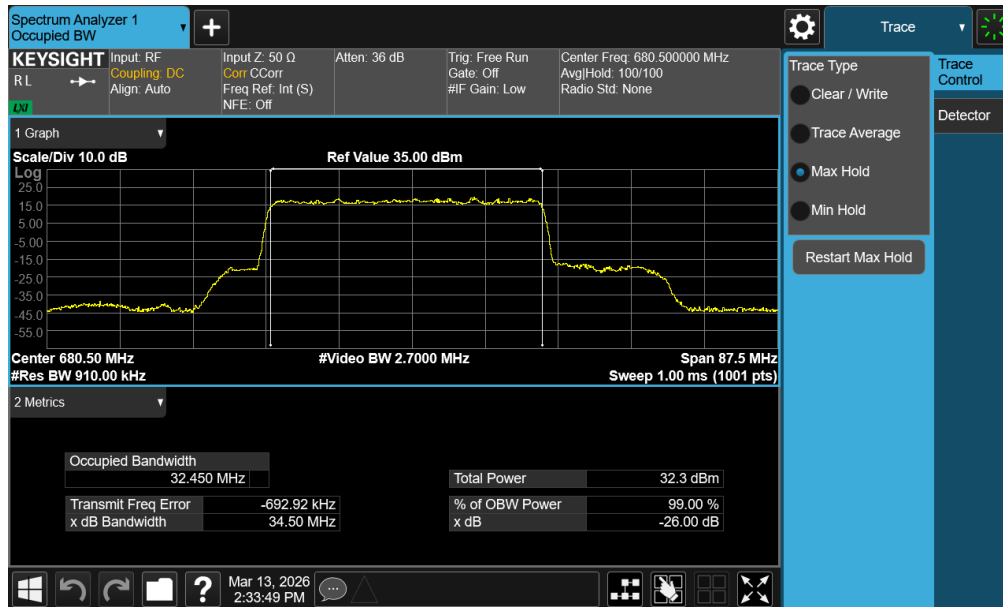
Plot 7-43. Occupied Bandwidth Plot (NR Band n71 - 35MHz DFT-s-OFDM BPSK - Full RB – ANT1)
