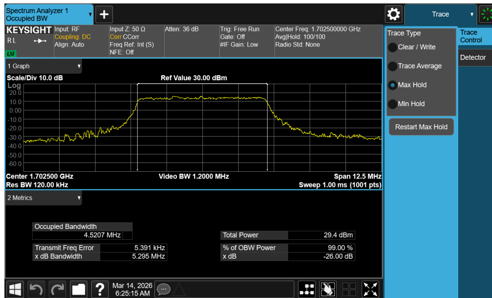
Plot 7-72. Occupied Bandwidth Plot (NR Band n70 - 5.0MHz CP-OFDM 16QAM - Full RB – ANT1)
