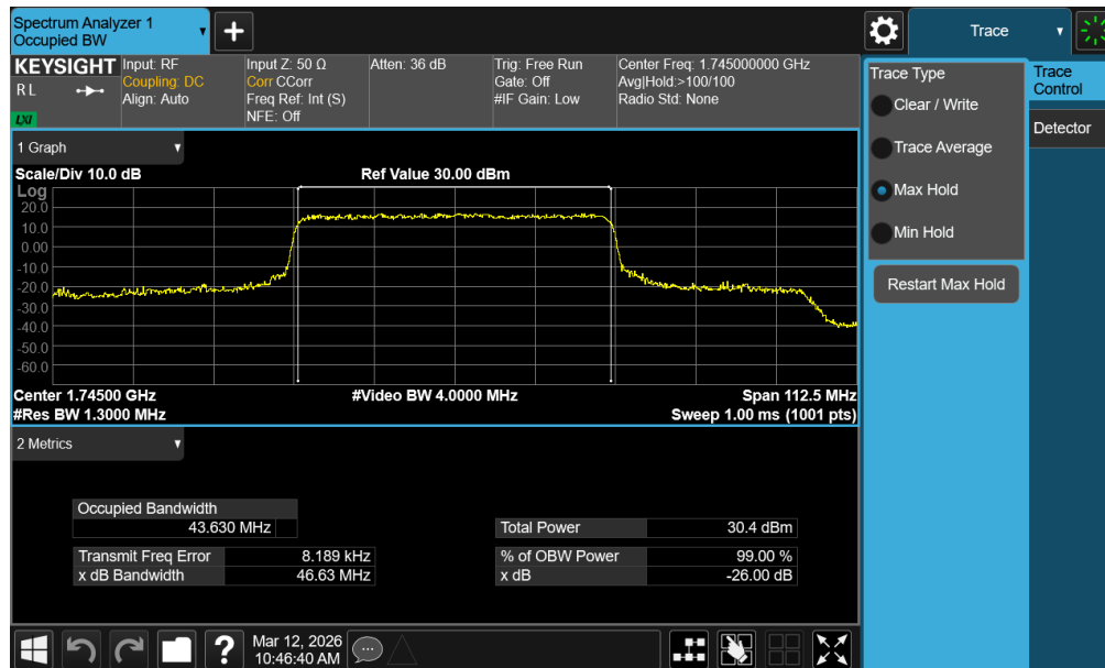
Plot 7-74. Occupied Bandwidth Plot (NR Band n66 - 45.0MHz CP-OFDM QPSK - Full RB – ANT1)
