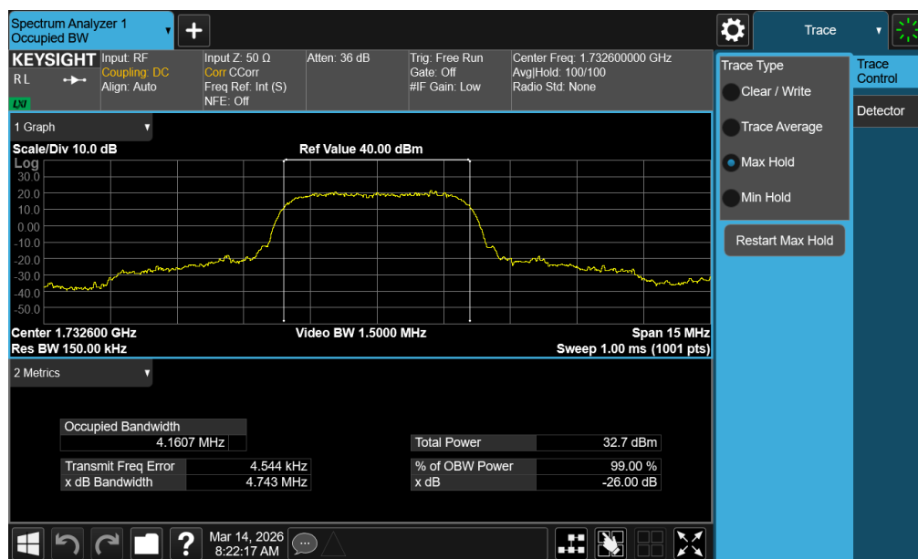
Plot 7-1. Occupied Bandwidth Plot (WCDMA, Ch. 1413 – ANT1)
