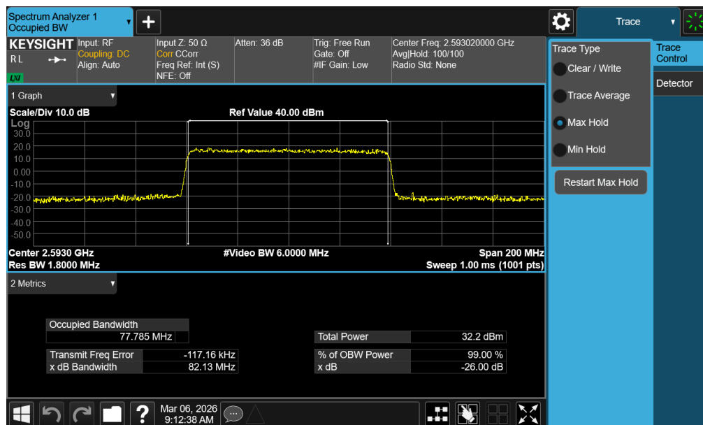
Plot 7-61. Occupied Bandwidth Plot (NR Band n41 PC2 – 80MHz QPSK – Full RB – Default – Ant1)
