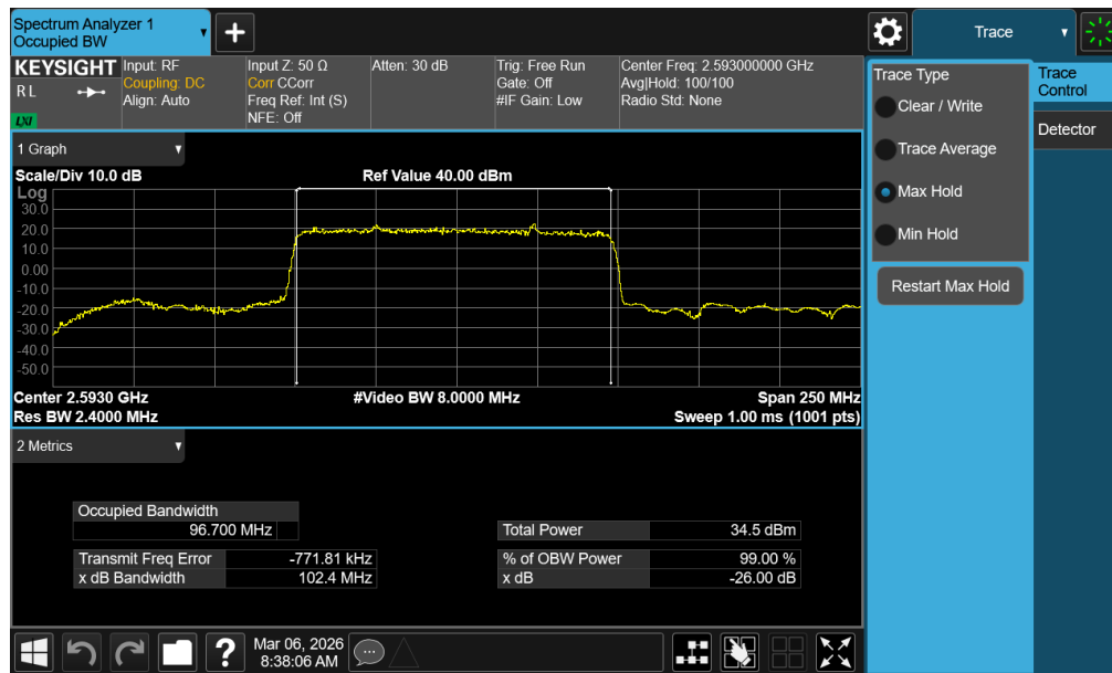
Plot 7-54. Occupied Bandwidth Plot (NR Band n41 PC2 – 100MHz \pi/2 BPSK – Full RB – Default – Ant1)
