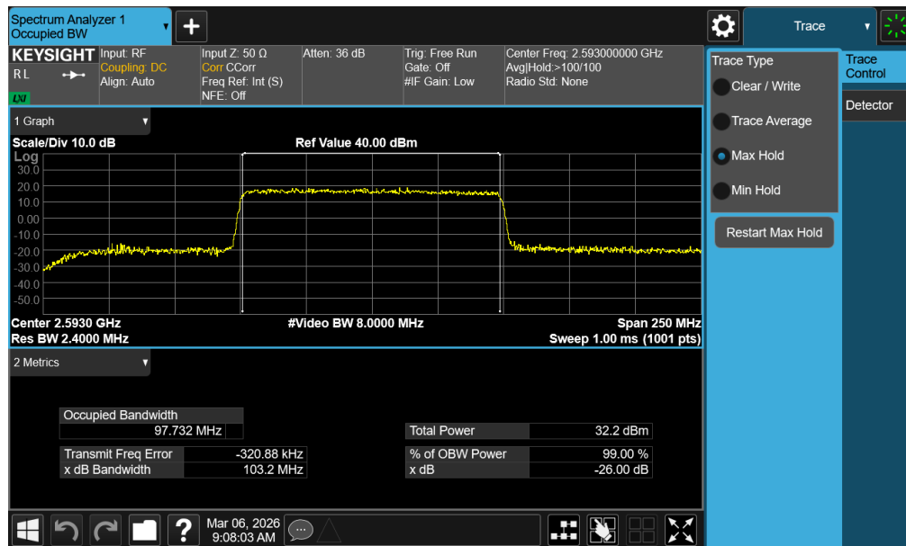
Plot 7-55. Occupied Bandwidth Plot (NR Band n41 PC2 – 100MHz QPSK – Full RB – Default – Ant1)
