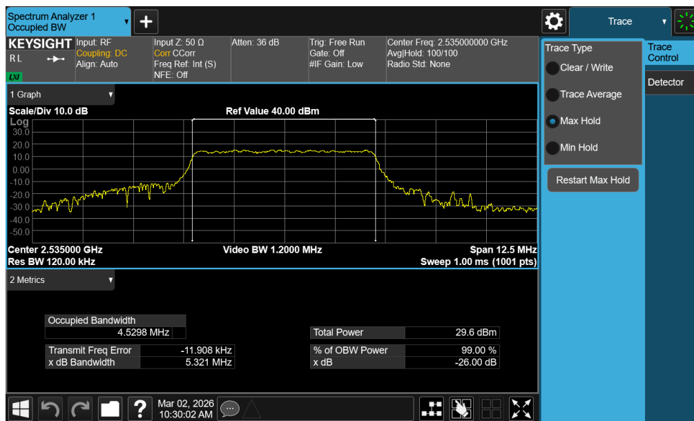
Plot 7-52. Occupied Bandwidth Plot (NR Band n7 - 5MHz QPSK - Full RB - Ant1)
