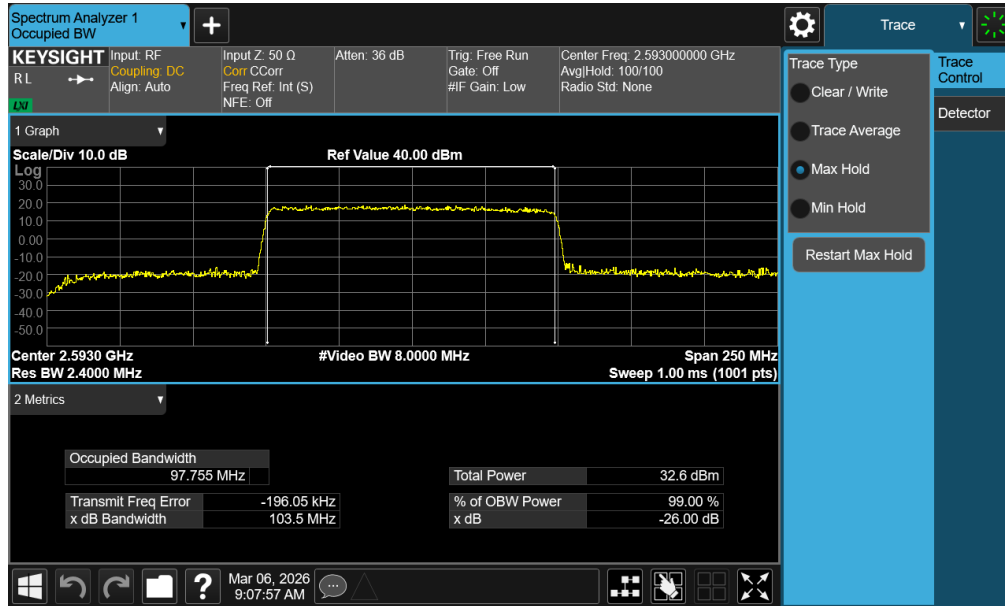
Plot 7-56. Occupied Bandwidth Plot (NR Band n41 PC2 – 100MHz 16-QAM – Full RB – Default – Ant1)
