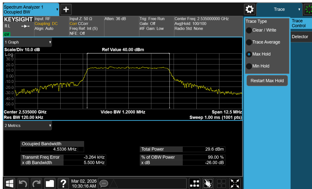
Plot 7-53. Occupied Bandwidth Plot (NR Band n7 - 5MHz 16-QAM - Full RB - Ant1)
