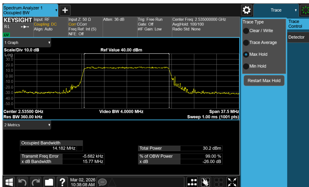
Plot 7-46. Occupied Bandwidth Plot (NR Band n7 - 15MHz QPSK - Full RB - Ant1)
