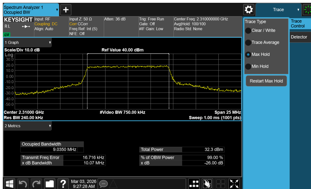
Plot 7-1. Occupied Bandwidth Plot (LTE Band 30 - 10MHz QPSK - Full RB - Ant1 – Ant1)
