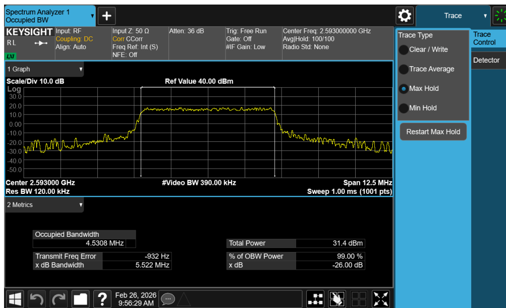
Plot 7-12. Occupied Bandwidth Plot (LTE Band 41(PC3)/38 - 5MHz 16-QAM - Full RB - Ant1)
