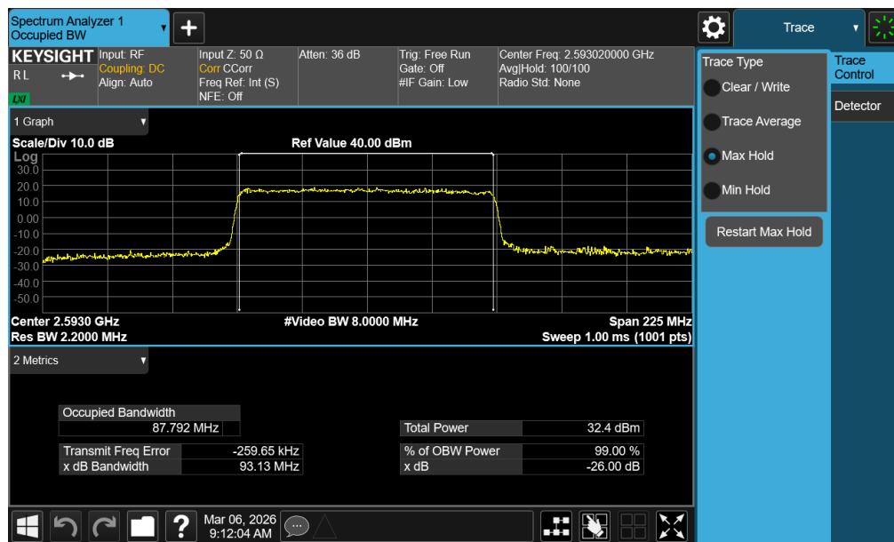
Plot 7-59. Occupied Bandwidth Plot (NR Band n41 PC2 – 90MHz 16-QAM – Full RB – Default – Ant1)
