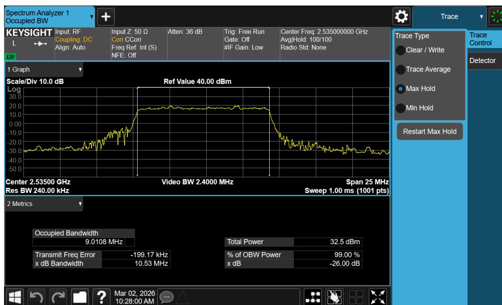
Plot 7-48. Occupied Bandwidth Plot (NR Band n7 - 10MHz \pi/2 BPSK - Full RB - Ant1)
