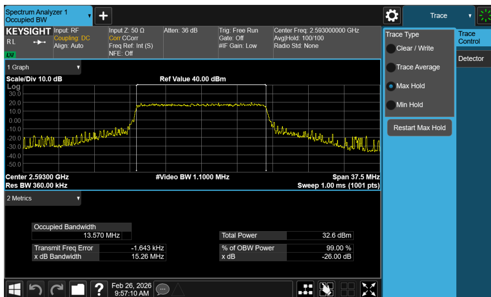
Plot 7-7. Occupied Bandwidth Plot (LTE Band 41(PC3)/38 - 15MHz QPSK - Full RB - Ant1)
