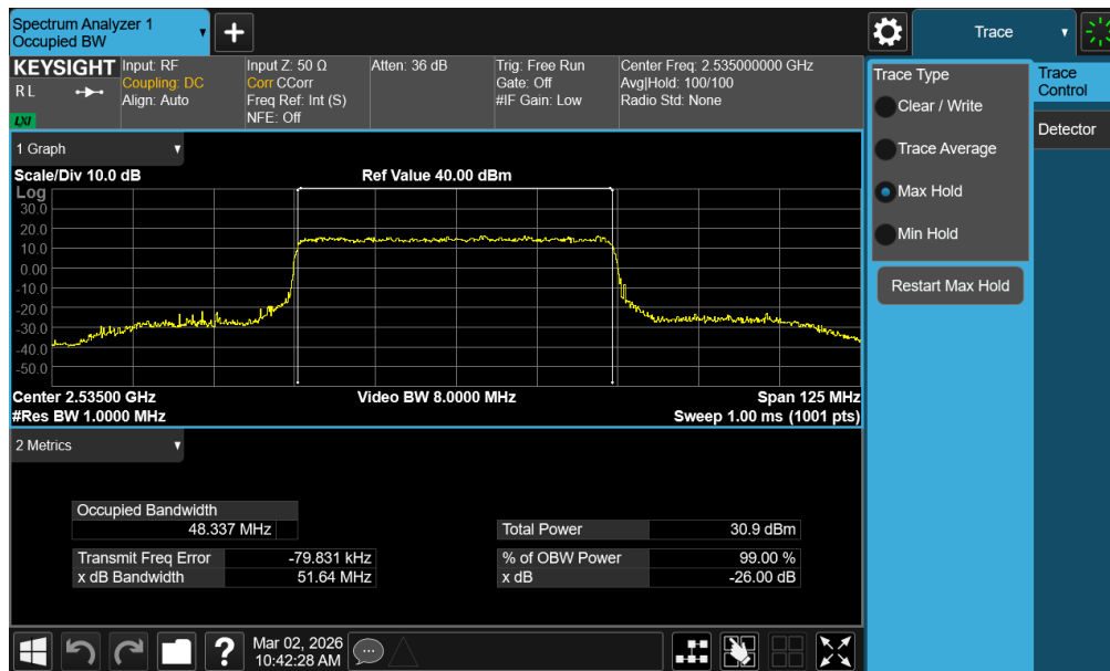
Plot 7-28. Occupied Bandwidth Plot (NR Band n7 - 50MHz QPSK - Full RB - Ant1)
