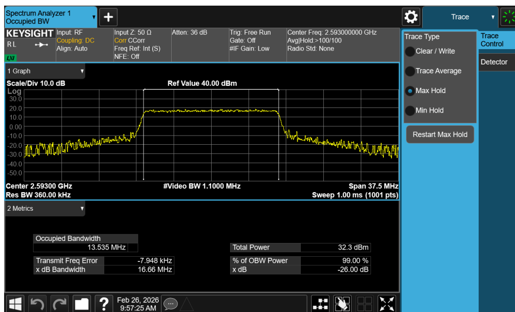
Plot 7-8. Occupied Bandwidth Plot (LTE Band 41(PC3)/38 - 15MHz 16-QAM - Full RB - Ant1)
