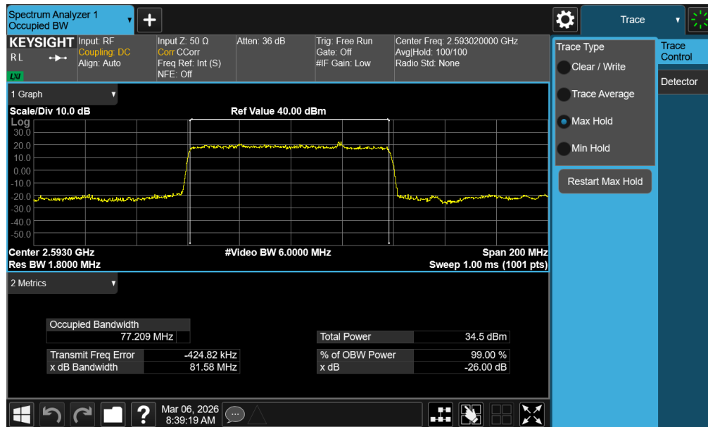
Plot 7-60. Occupied Bandwidth Plot (NR Band n41 PC2 – 80MHz \pi/2 BPSK – Full RB – Default – Ant1)
