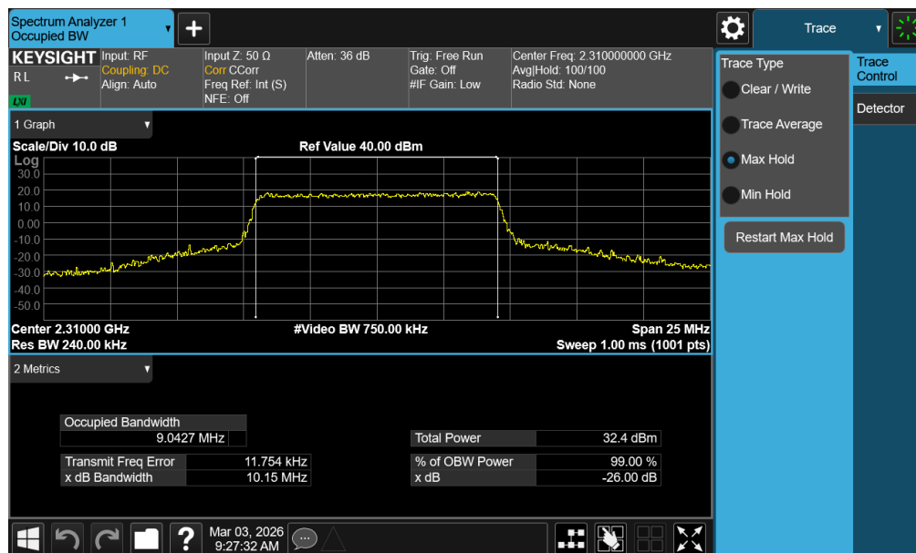
Plot 7-2. Occupied Bandwidth Plot (LTE Band 30 - 10MHz 16-QAM - Full RB - Ant1)
