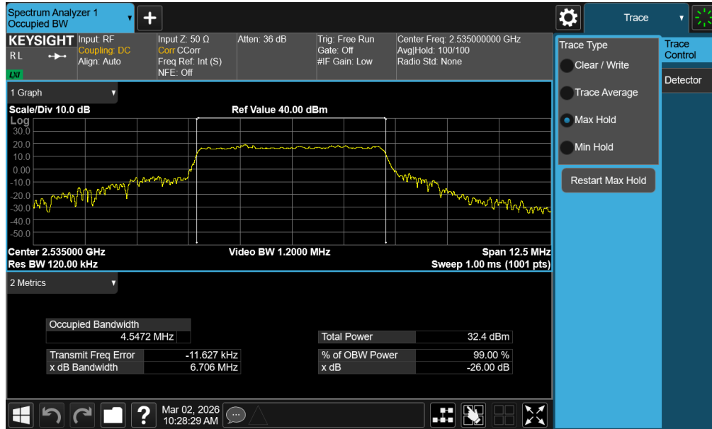
Plot 7-51. Occupied Bandwidth Plot (NR Band n7 - 5MHz \pi/2 BPSK - Full RB - Ant1)
