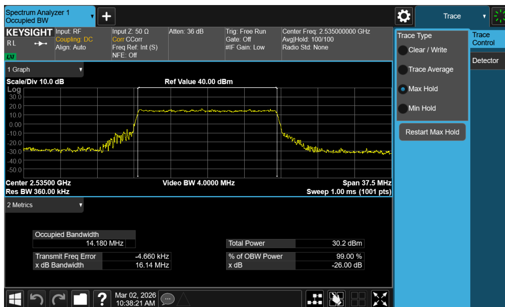
Plot 7-47. Occupied Bandwidth Plot (NR Band n7 - 15MHz 16-QAM - Full RB - Ant1)
