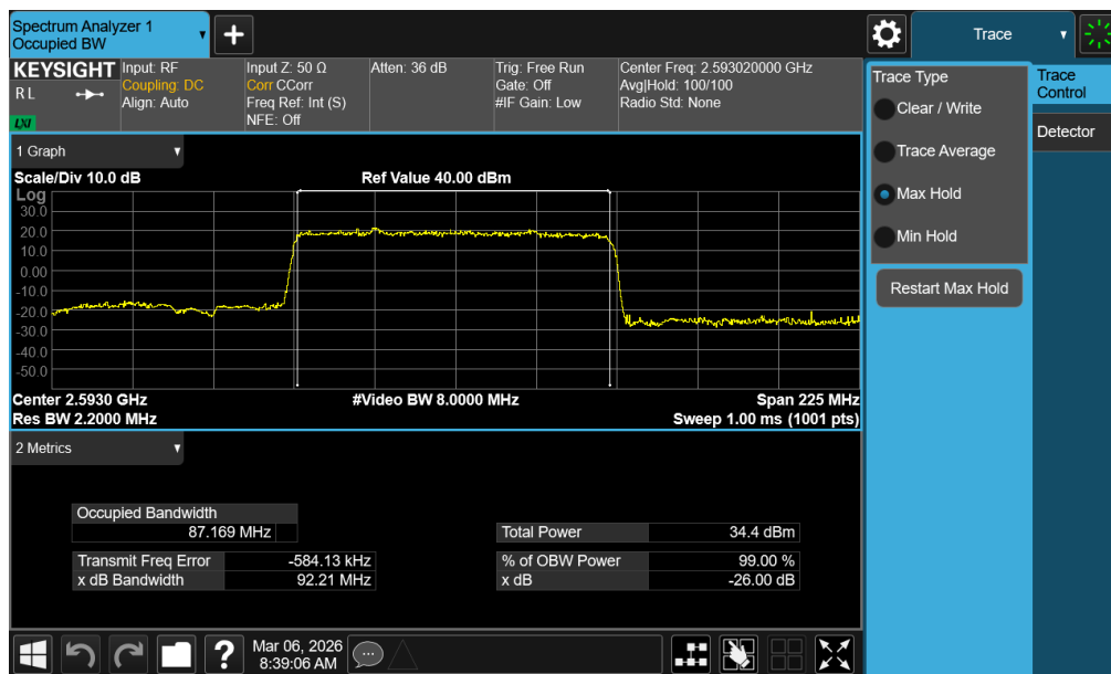
Plot 7-57. Occupied Bandwidth Plot (NR Band n41 PC2 – 90MHz \pi/2 BPSK – Full RB – Default – Ant1)
