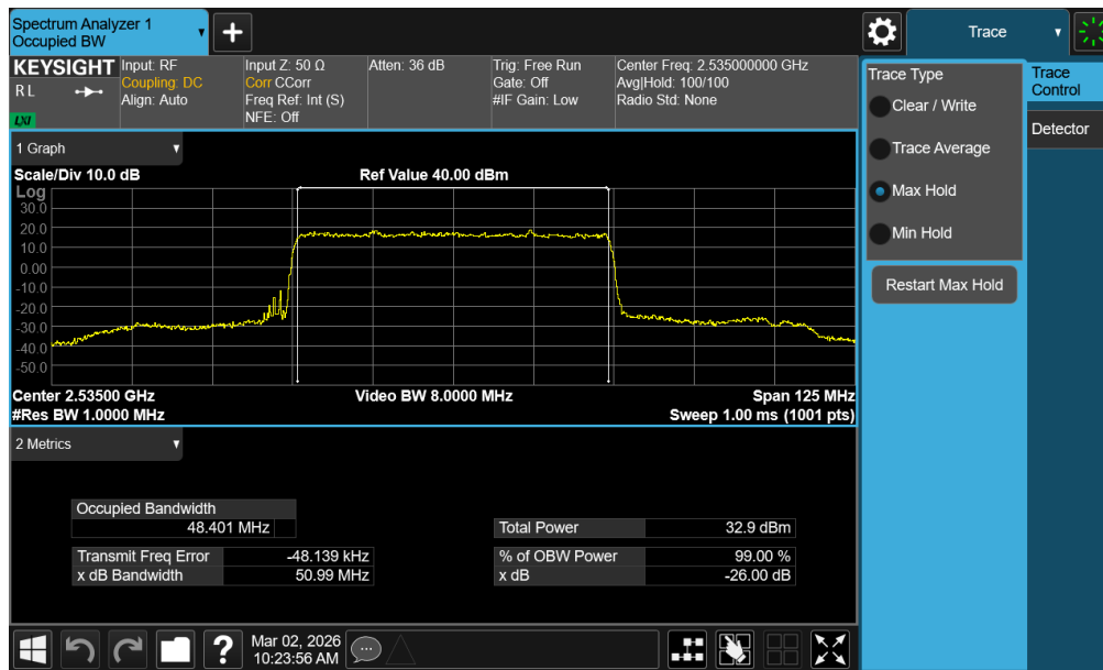
Plot 7-27. Occupied Bandwidth Plot (NR Band n7 - 50MHz \pi/2 BPSK - Full RB - Ant1)
