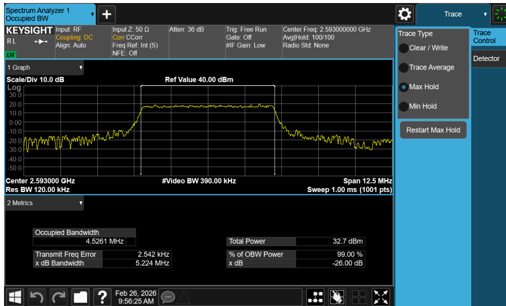
Plot 7-11. Occupied Bandwidth Plot (LTE Band 41(PC3)/38 - 5MHz QPSK - Full RB - Ant1)
