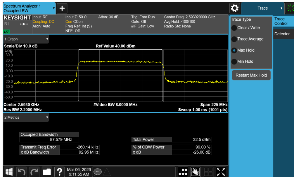
Plot 7-58. Occupied Bandwidth Plot (NR Band n41 PC2 – 90MHz QPSK – Full RB – Default – Ant1)
