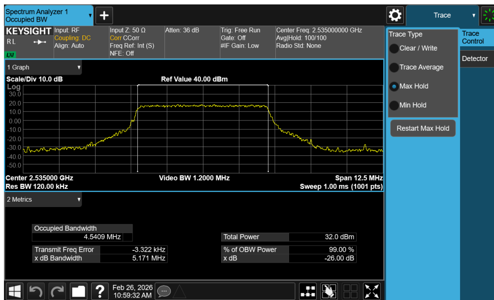
Plot 7-20. Occupied Bandwidth Plot (LTE Band 7 - 5MHz 16-QAM - Full RB - Ant1)
