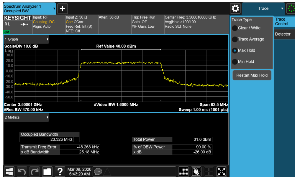
Plot 7-26. Occupied Bandwidth Plot (NR Band n77 - 25MHz QPSK - Full RB - Ant1 - DoD Band - Main)
