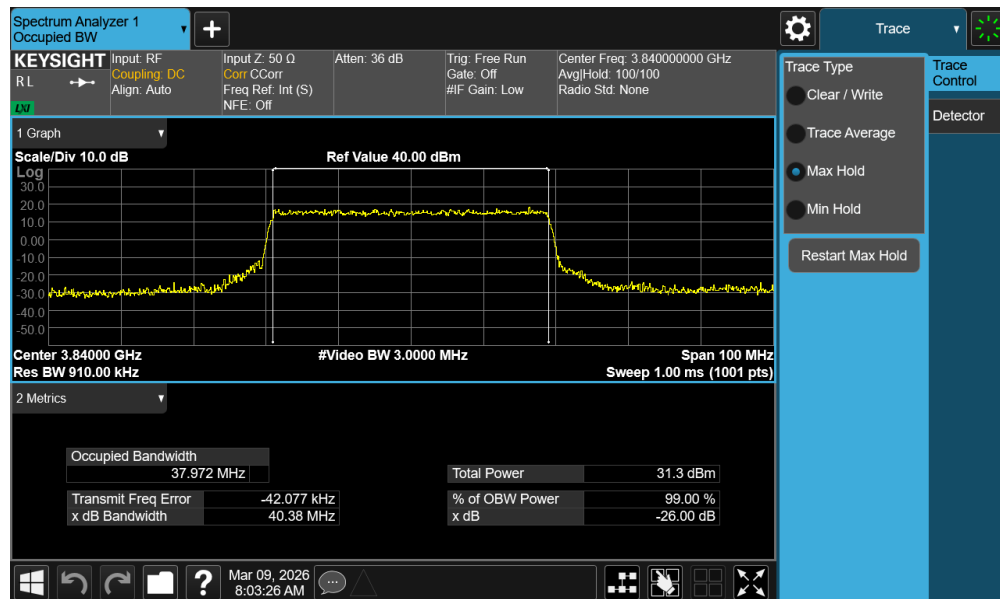
Plot 7-56. Occupied Bandwidth Plot (NR Band n77 - 40MHz QPSK - Full RB - Ant1 - C-Band - Main)
