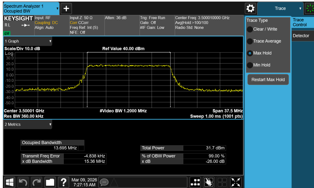
Plot 7-32. Occupied Bandwidth Plot (NR Band n77 - 15MHz QPSK - Full RB - Ant1 - DoD Band - Main)
