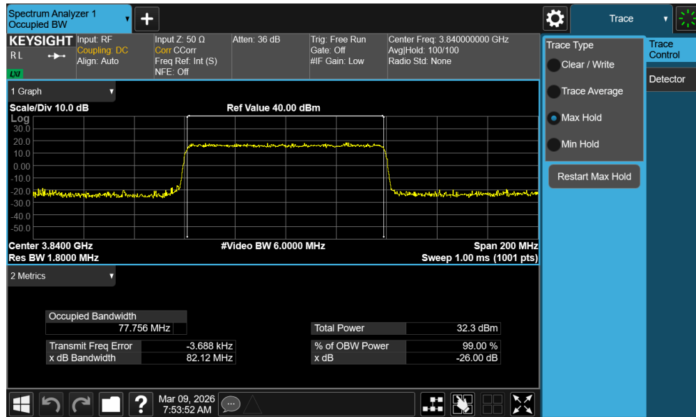
Plot 7-44. Occupied Bandwidth Plot (NR Band n77 - 80MHz QPSK - Full RB - Ant1 - C-Band - Main)
