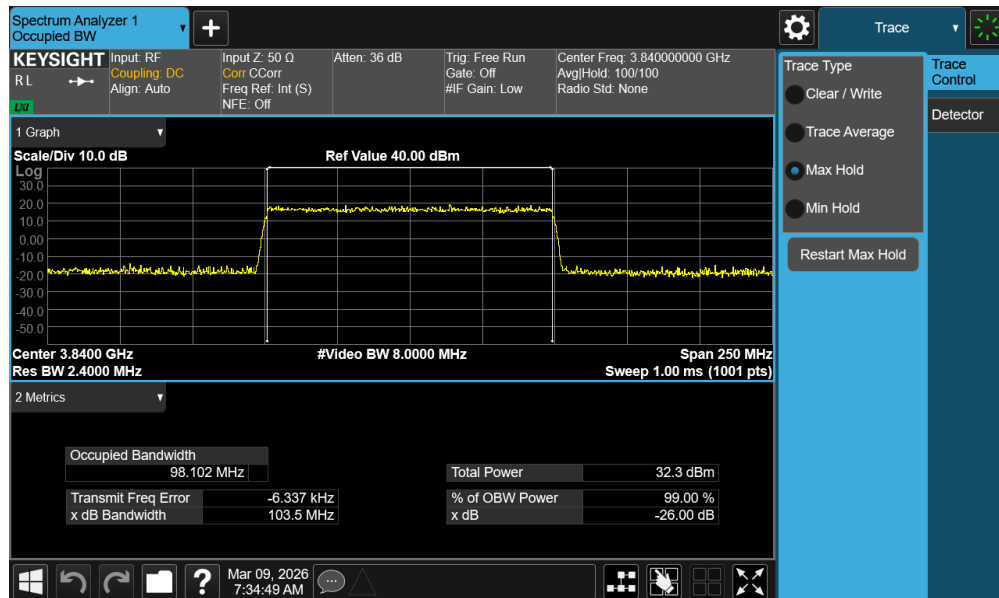
Plot 7-38. Occupied Bandwidth Plot (NR Band n77PC2 - 100MHz QPSK - Full RB - Ant1 - C-Band - Main)
