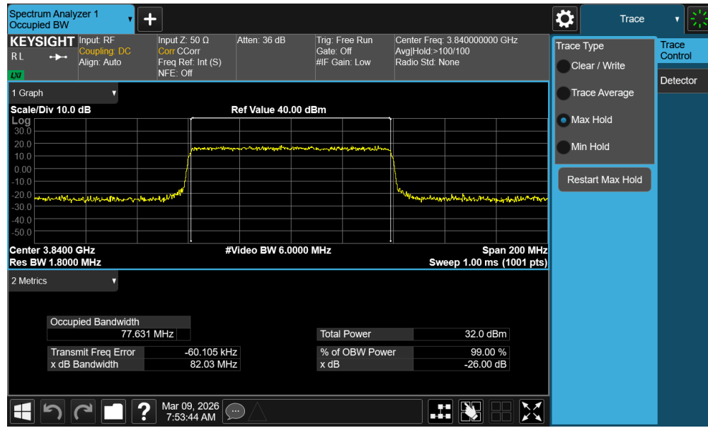
Plot 7-45. Occupied Bandwidth Plot (NR Band n77 - 80MHz 16-QAM - Full RB - Ant1 - C-Band - Main)
