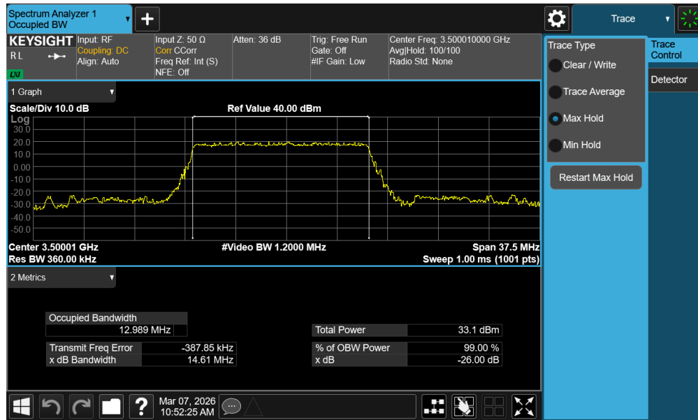
Plot 7-31. Occupied Bandwidth Plot (NR Band n77 - 15MHz \pi/2 BPSK - Full RB - Ant1 - DoD Band - Main)
