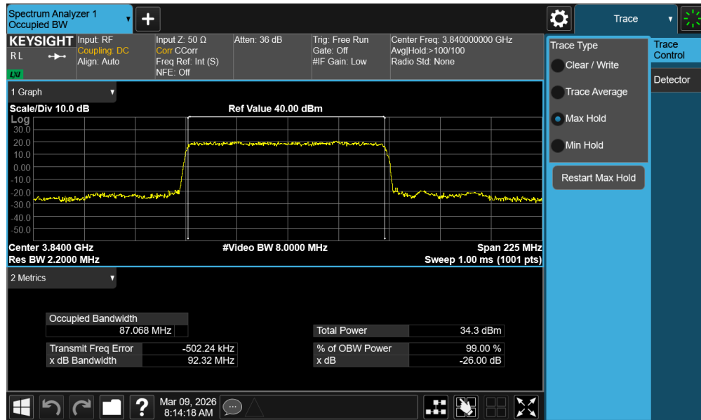
Plot 7-40. Occupied Bandwidth Plot (NR Band n77 - 90MHz \pi/2 BPSK - Full RB - Ant1 - C-Band - Main)
