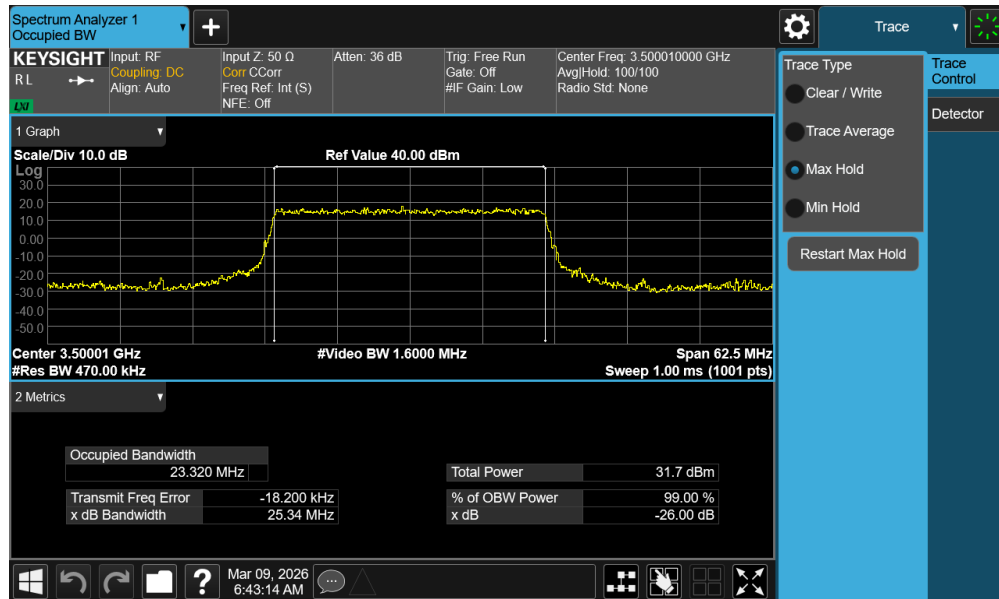
Plot 7-27. Occupied Bandwidth Plot (NR Band n77 - 25MHz 16-QAM - Full RB - Ant1 - DoD Band - Main)
