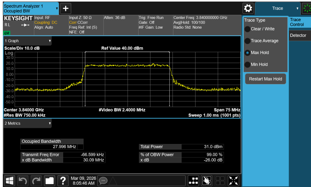
Plot 7-60. Occupied Bandwidth Plot (NR Band n77 - 30MHz 16-QAM - Full RB - Ant1 - C-Band - Main)
