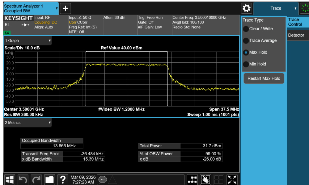
Plot 7-33. Occupied Bandwidth Plot (NR Band n77 - 15MHz 16-QAM - Full RB - Ant1 - DoD Band - Main)
