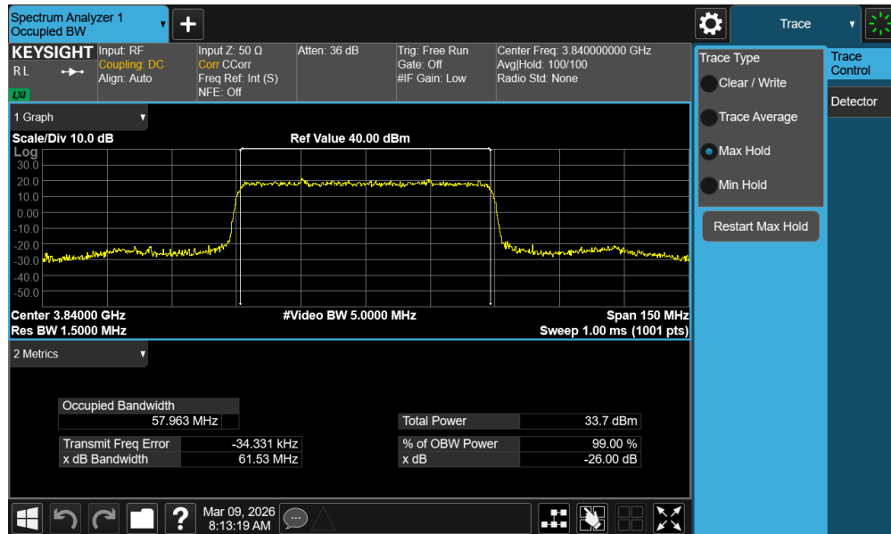
Plot 7-49. Occupied Bandwidth Plot (NR Band n77 - 60MHz \pi/2 BPSK - Full RB - Ant1 - C-Band - Main)
