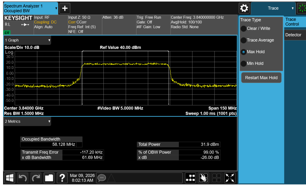
Plot 7-51. Occupied Bandwidth Plot (NR Band n77 - 60MHz 16-QAM - Full RB - Ant1 - C-Band - Main)
