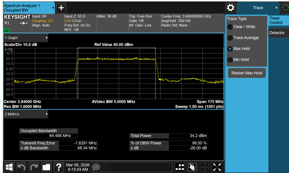
Plot 7-46. Occupied Bandwidth Plot (NR Band n77 - 70MHz \pi/2 BPSK - Full RB - Ant1 - C-Band - Main)
