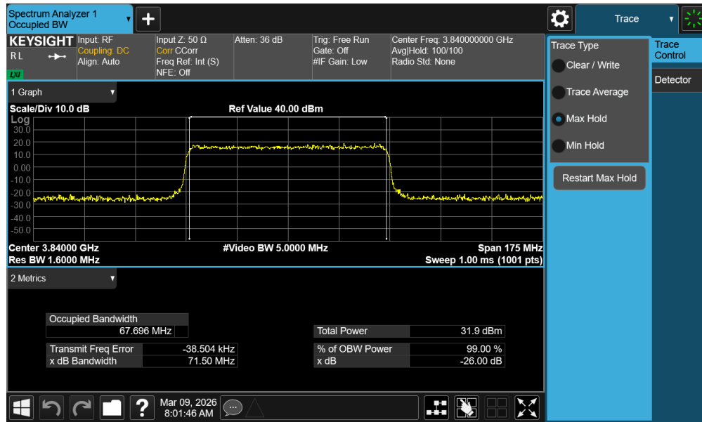
Plot 7-48. Occupied Bandwidth Plot (NR Band n77 - 70MHz 16-QAM - Full RB - Ant1 - C-Band - Main)
