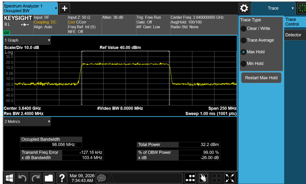
Plot 7-39. Occupied Bandwidth Plot (NR Band n77PC2 - 100MHz 16-QAM - Full RB - Ant1 - C-Band - Main)
