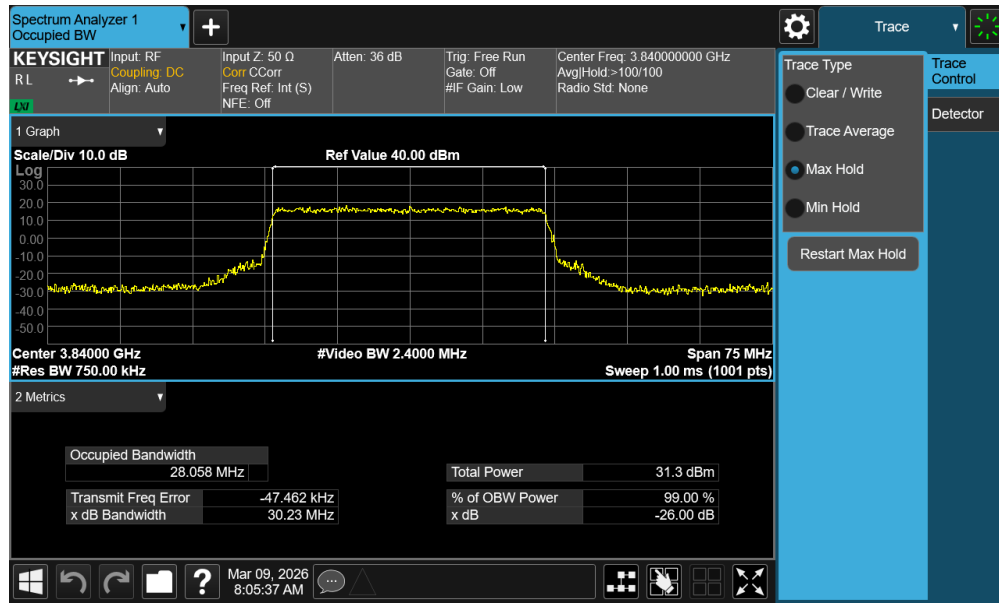
Plot 7-59. Occupied Bandwidth Plot (NR Band n77 - 30MHz QPSK - Full RB - Ant1 - C-Band - Main)
