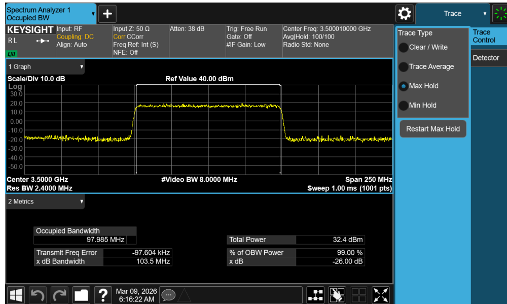
Plot 7-3. Occupied Bandwidth Plot (NR Band n77PC2 - 100MHz 16-QAM - Full RB - Ant1 - DoD Band - Main)
