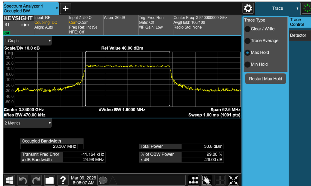
Plot 7-62. Occupied Bandwidth Plot (NR Band n77 - 25MHz QPSK - Full RB - Ant1 - C-Band - Main)
