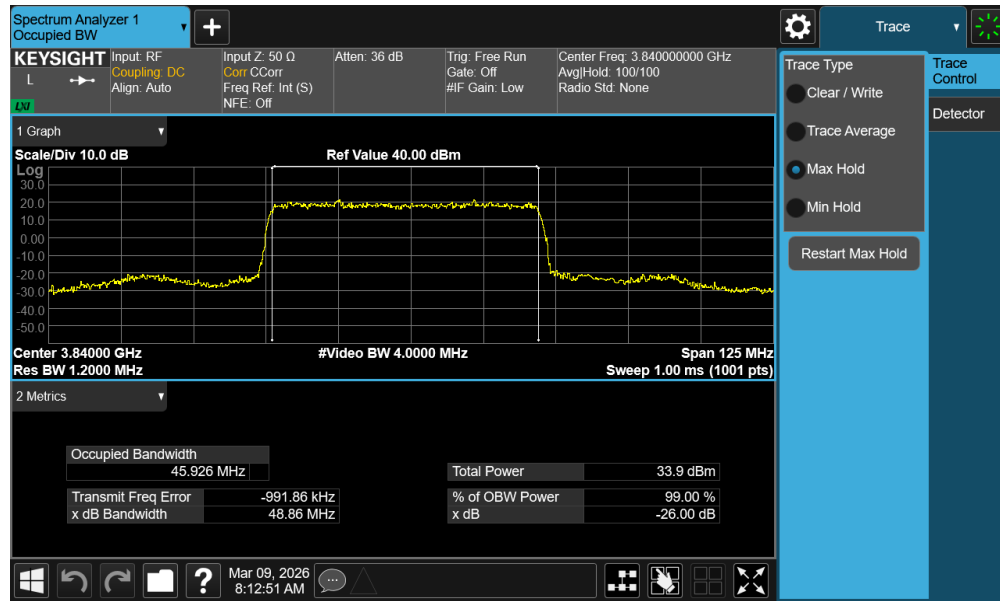
Plot 7-52. Occupied Bandwidth Plot (NR Band n77 - 50MHz \pi/2 BPSK - Full RB - Ant1 - C-Band - Main)
