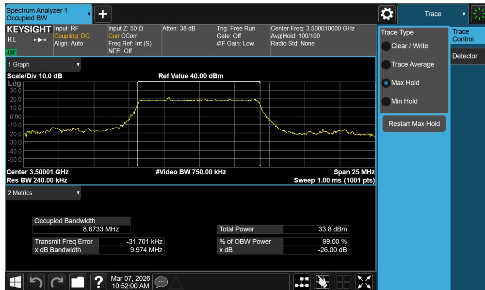
Plot 7-34. Occupied Bandwidth Plot (NR Band n77 - 10MHz \pi/2 BPSK - Full RB - Ant1 - DoD Band - Main)
