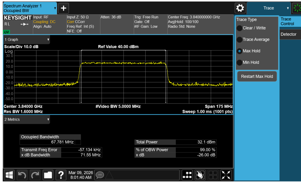
Plot 7-47. Occupied Bandwidth Plot (NR Band n77 - 70MHz QPSK - Full RB - Ant1 - C-Band - Main)
