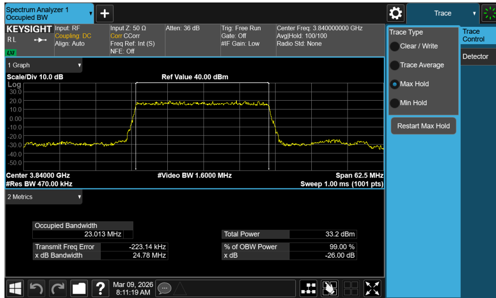
Plot 7-61. Occupied Bandwidth Plot (NR Band n77 - 25MHz \pi/2 BPSK - Full RB - Ant1 - C-Band - Main)
