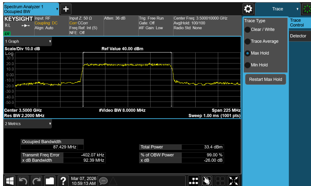
Plot 7-4. Occupied Bandwidth Plot (NR Band n77 - 90MHz \pi/2 BPSK - Full RB - Ant1 - DoD Band - Main)
