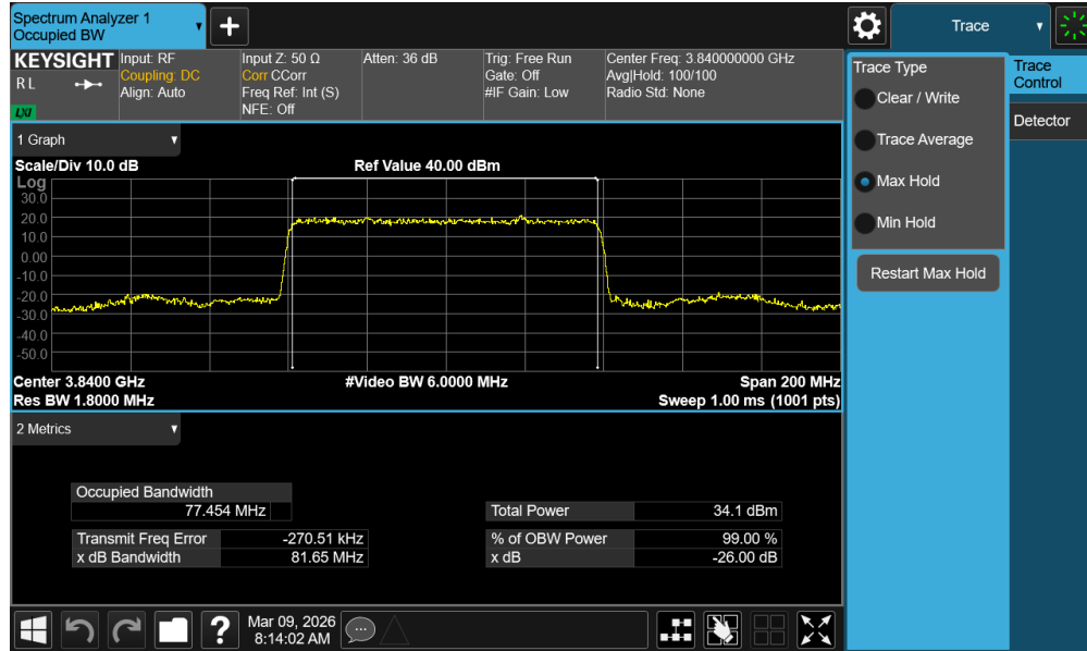
Plot 7-43. Occupied Bandwidth Plot (NR Band n77 - 80MHz \pi/2 BPSK - Full RB - Ant1 - C-Band - Main)
