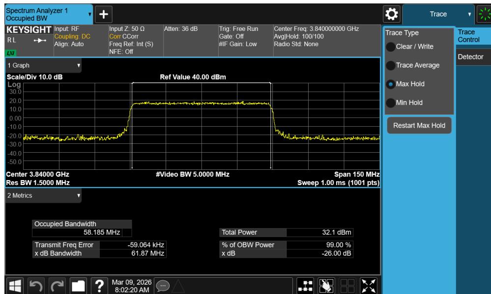
Plot 7-50. Occupied Bandwidth Plot (NR Band n77 - 60MHz QPSK - Full RB - Ant1 - C-Band - Main)
