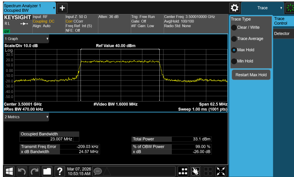
Plot 7-25. Occupied Bandwidth Plot (NR Band n77 - 25MHz \pi/2 BPSK - Full RB - Ant1 - DoD Band - Main)
