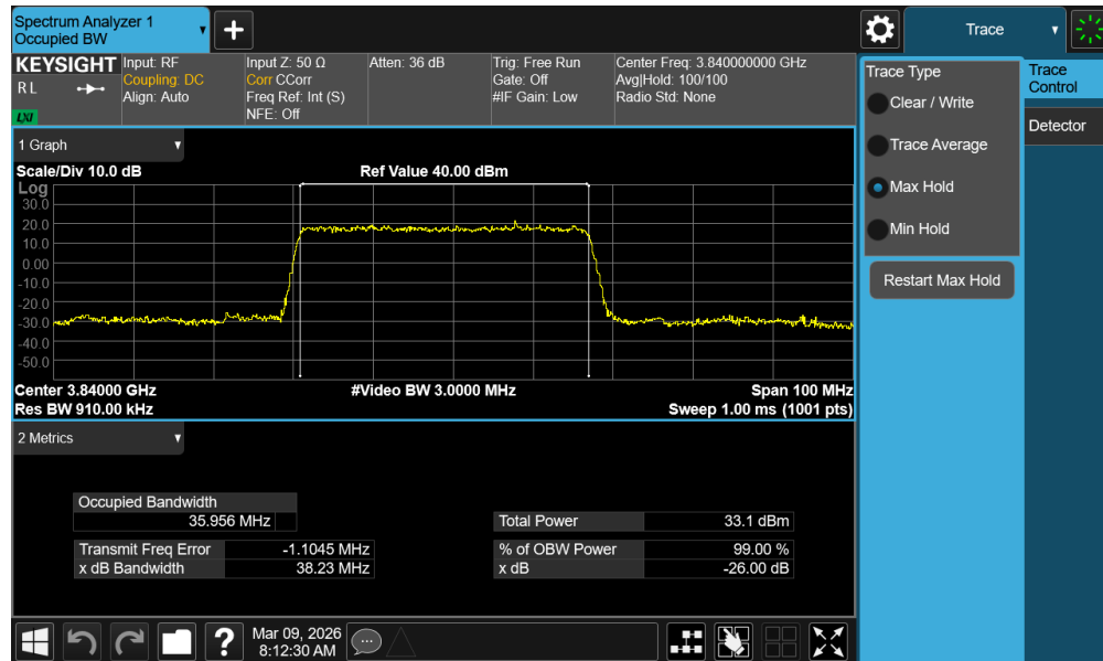
Plot 7-55. Occupied Bandwidth Plot (NR Band n77 - 40MHz \pi/2 BPSK - Full RB - Ant1 - C-Band - Main)
