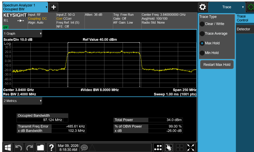
Plot 7-37. Occupied Bandwidth Plot (NR Band n77PC2 - 100MHz \pi/2 BPSK - Full RB - Ant1 - C-Band - Main)
