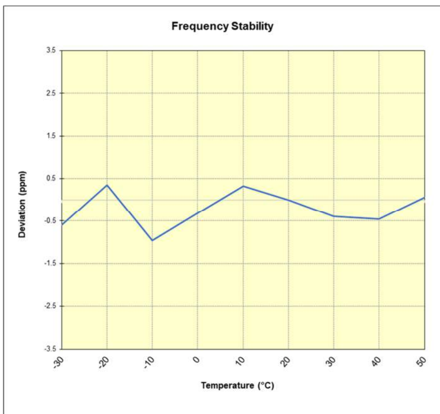
Plot 7-54. NR Band n48 Frequency Stability Chart
