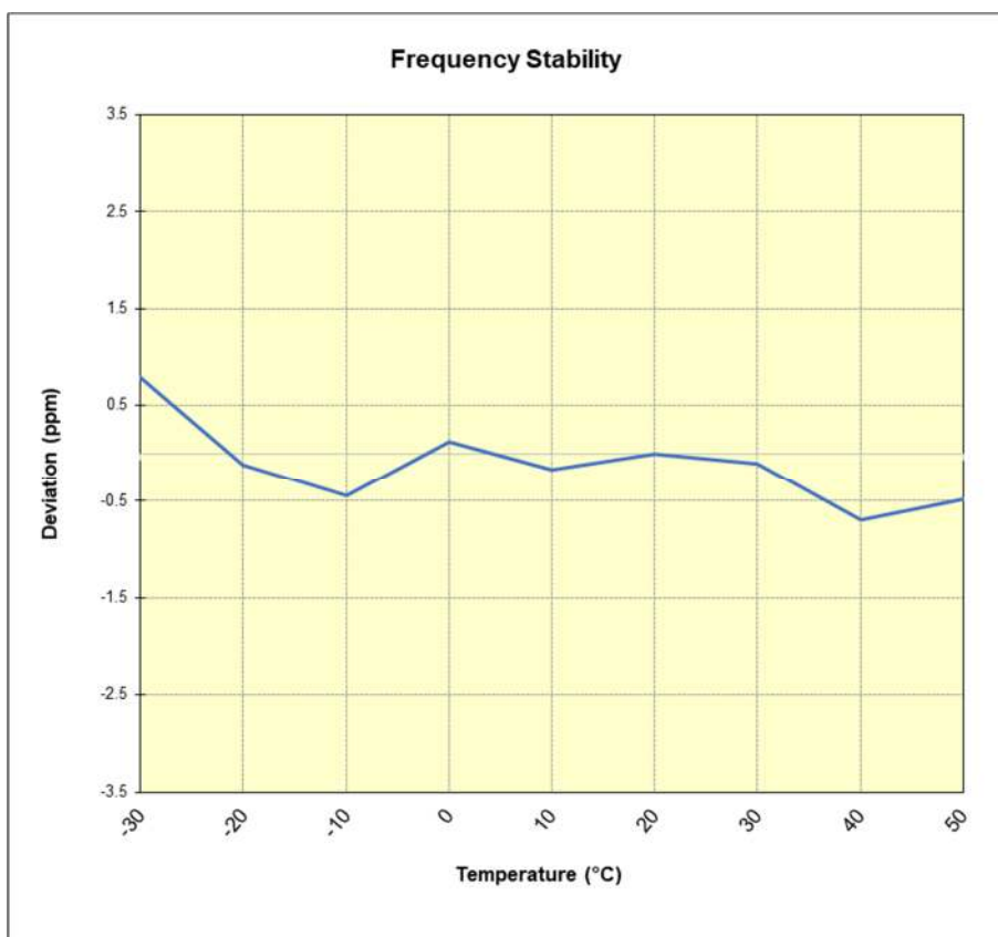
Plot 7-53. LTE Band 48 Frequency Stability Chart
