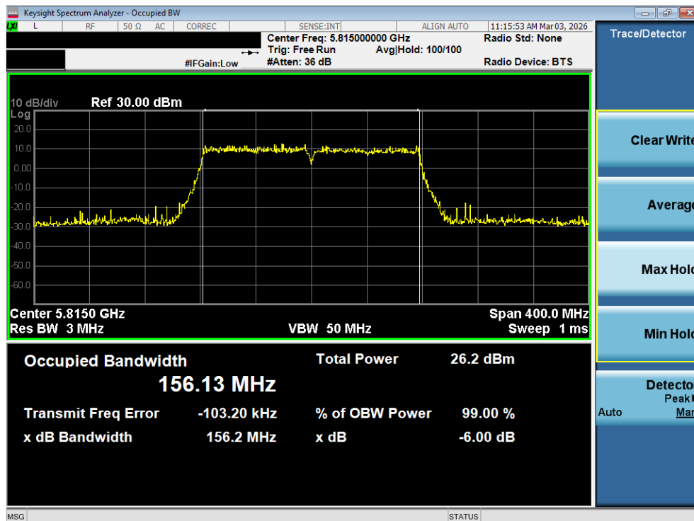
Plot 7-95. OBW Plot MIMO ANT2 (160MHz BW 802.11ac (UNII Band 3/4) – Ch. 163)
