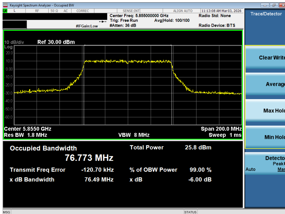
Plot 7-93. OBW Plot MIMO ANT2 (80MHz BW 802.11ac (UNII Band 3/4) – Ch. 171)
