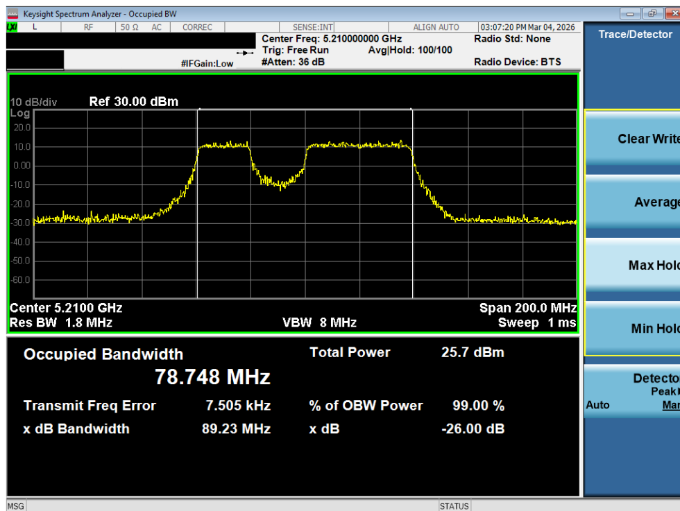
Plot 7-21. 26dB Bandwidth Plot MIMO ANT2 (80MHz BW 802.11be (20MHz Punct.) (UNII Band 1) – Ch. 42)
