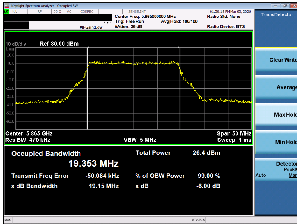
Plot 7-71. OBW Plot MIMO ANT1 (20MHz BW 802.11be (UNII Band 4) – Ch. 173)
