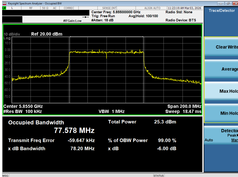
Plot 7-56. 6dB Bandwidth Plot MIMO ANT2 (80MHz BW 802.11be (UNII Band 3/4) – Ch. 171)
