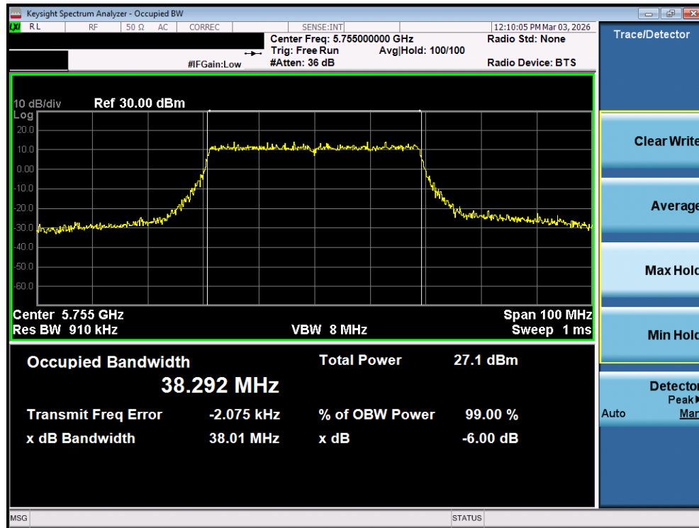
Plot 7-65. OBW Plot MIMO ANT1 (40MHz BW 802.11be (UNII Band 3) – Ch. 151)
