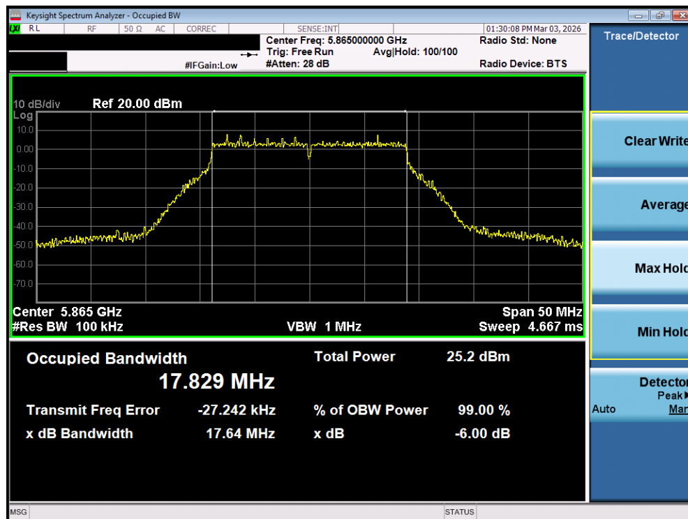
Plot 7-32. 6dB Bandwidth Plot MIMO ANT1 (20MHz BW 802.11n (UNII Band 4) – Ch. 173)
