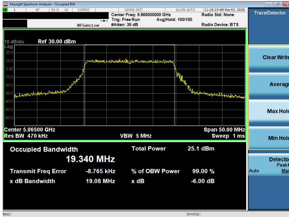
Plot 7-90. OBW Plot MIMO ANT2 (20MHz BW 802.11be (UNII Band 3/4) – Ch. 173)
