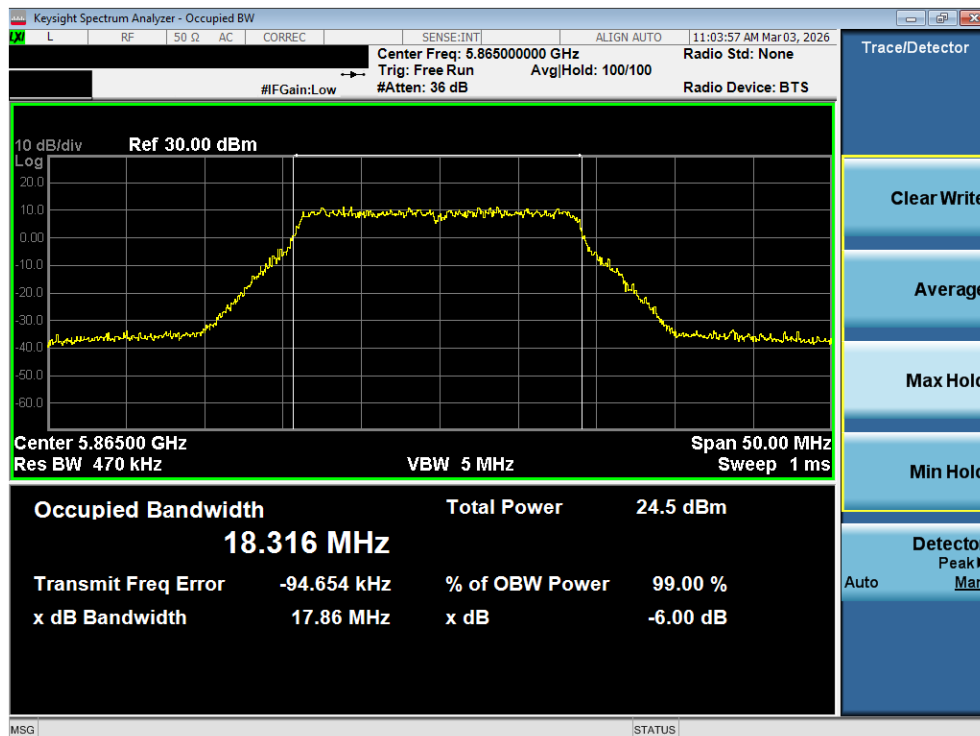
Plot 7-89. OBW Plot MIMO ANT2 (20MHz BW 802.11n (UNII Band 3/4) – Ch. 173)
