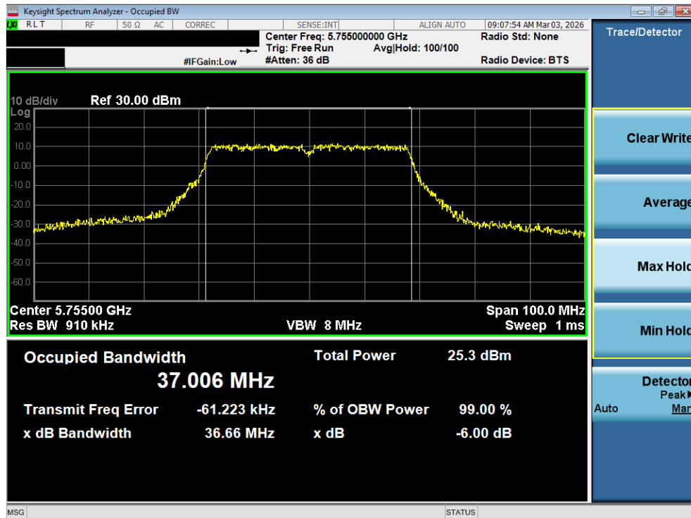
Plot 7-83. OBW Plot MIMO ANT2 (40MHz BW 802.11n (UNII Band 3) – Ch. 151)
