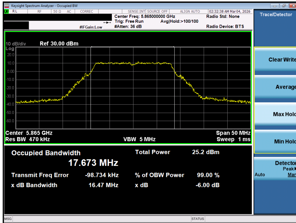
Plot 7-69. OBW Plot MIMO ANT1 (802.11a (UNII Band 4) – Ch. 173)
