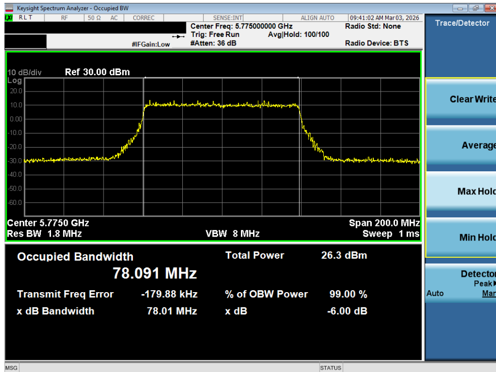
Plot 7-87. OBW Plot MIMO ANT2 (80MHz BW 802.11be (UNII Band 3) – Ch. 155)
