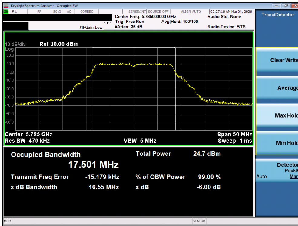
Plot 7-61. OBW Plot MIMO ANT1 (802.11a (UNII Band 3) – Ch. 157)
