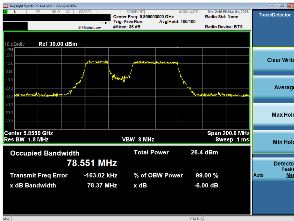
Plot 7-97. OBW Plot MIMO ANT2 (80MHz BW 802.11be (20MHz Punct.) (UNII Band 3/4) – Ch. 171)
