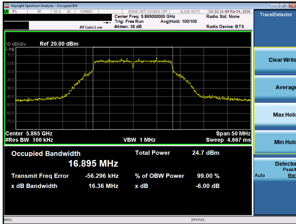
Plot 7-31. 6dB Bandwidth Plot MIMO ANT1 (802.11a (UNII Band 4) – Ch. 173)
