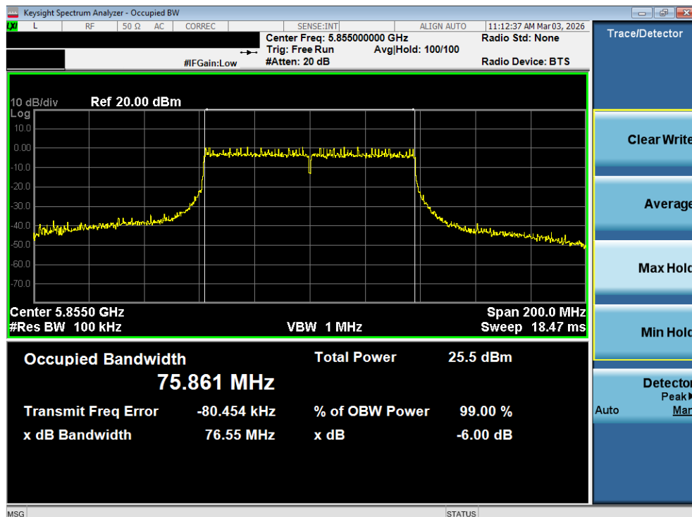
Plot 7-55. 6dB Bandwidth Plot MIMO ANT2 (80MHz BW 802.11ac (UNII Band 3/4) – Ch. 171)
