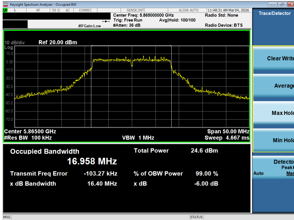
Plot 7-50. 6dB Bandwidth Plot MIMO ANT2 (802.11a (UNII Band 3/4) – Ch. 173)
