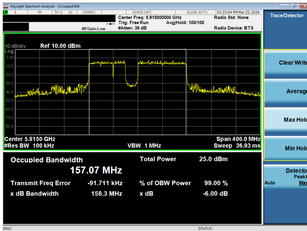
Plot 7-60. 6dB Bandwidth Plot MIMO ANT2 (160MHz BW 802.11be (20MHz Punct.) (UNII Band 3/4) – Ch. 163)
