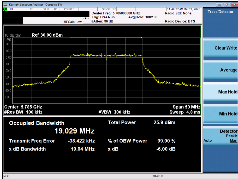
Plot 7-25. 6dB Bandwidth Plot MIMO ANT1 (20MHz BW 802.11be (UNII Band 3) – Ch. 157)
