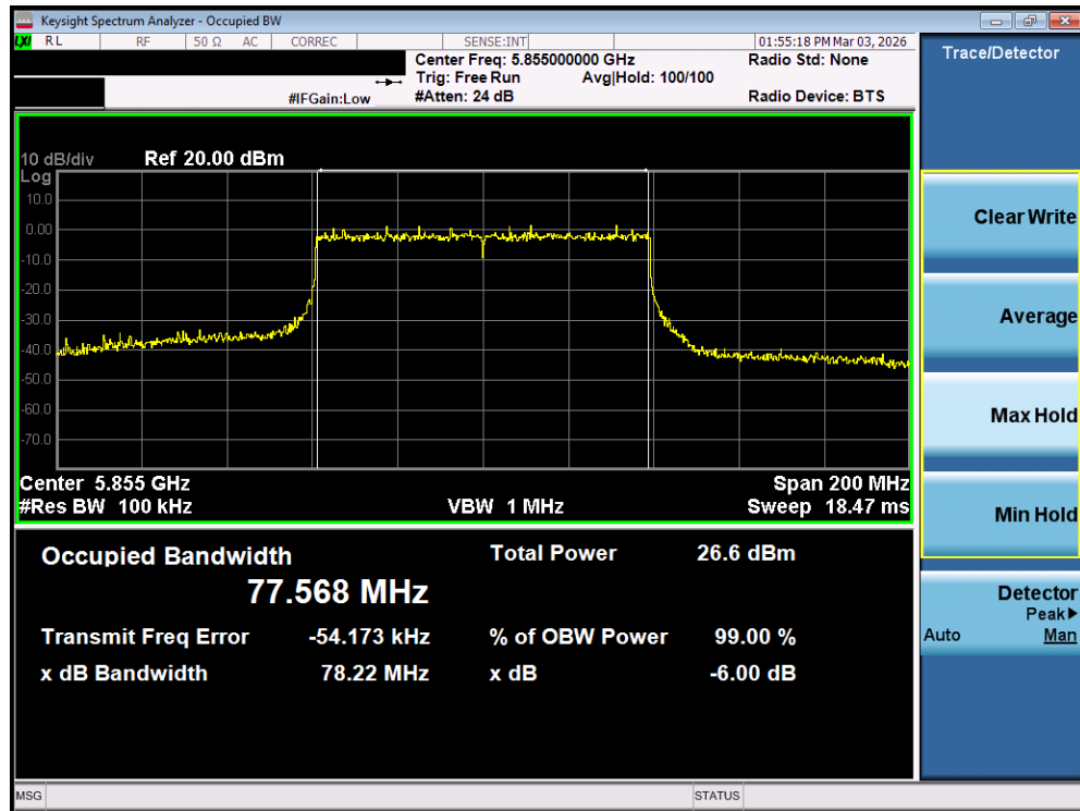
Plot 7-37. 6dB Bandwidth Plot MIMO ANT1 (80MHz BW 802.11be (UNII Band 3/4) – Ch. 171)
