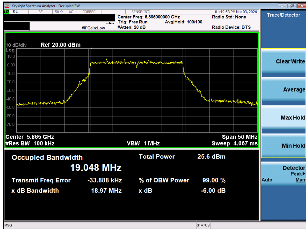
Plot 7-33. 6dB Bandwidth Plot MIMO ANT1 (20MHz BW 802.11be (UNII Band 4) – Ch. 173)
