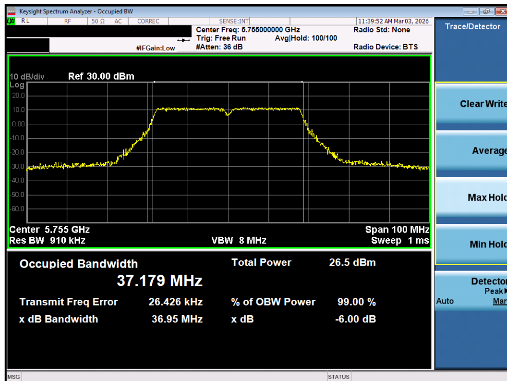
Plot 7-64. OBW Plot MIMO ANT1 (40MHz BW 802.11n (UNII Band 3) – Ch. 151)
