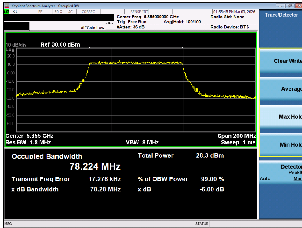
Plot 7-75. OBW Plot MIMO ANT1 (80MHz BW 802.11be (UNII Band 3/4) – Ch. 171)
