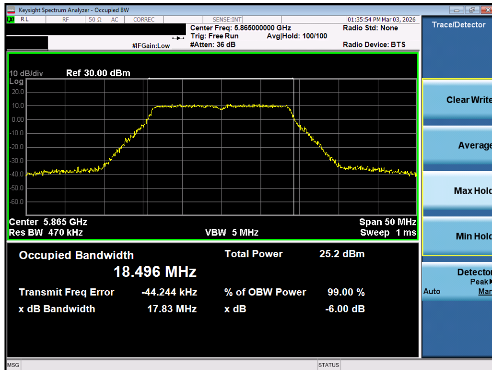
Plot 7-70. OBW Plot MIMO ANT1 (20MHz BW 802.11n (UNII Band 4) – Ch. 173)
