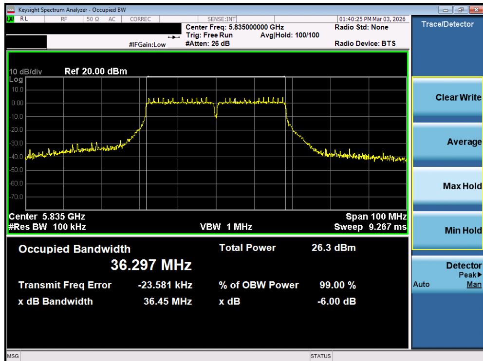
Plot 7-34. 6dB Bandwidth Plot MIMO ANT1 (40MHz BW 802.11n (UNII Band 3/4) – Ch. 167)
