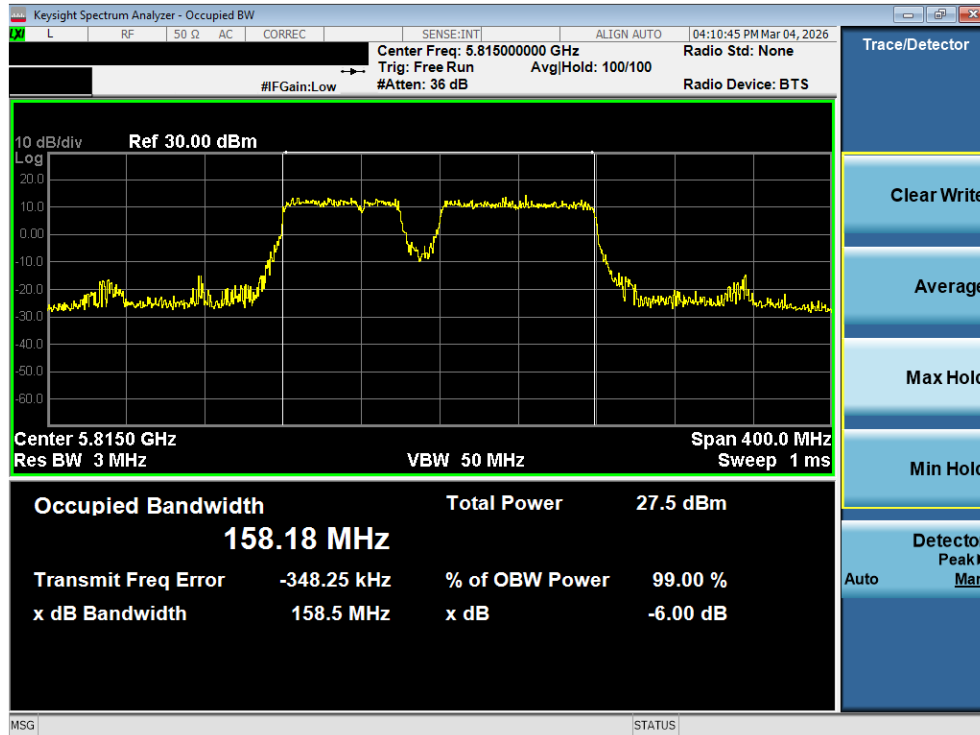
Plot 7-98. OBW Plot MIMO ANT2 (160MHz BW 802.11be (20MHz Punct.) (UNII Band 3/4) – Ch. 163)
