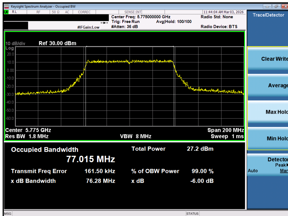
Plot 7-66. OBW Plot MIMO ANT1 (80MHz BW 802.11ac (UNII Band 3) – Ch. 155)
