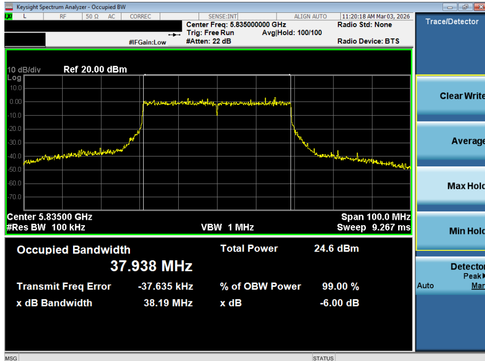
Plot 7-54. 6dB Bandwidth Plot MIMO ANT2 (40MHz BW 802.11be (UNII Band 3/4) – Ch. 167)
