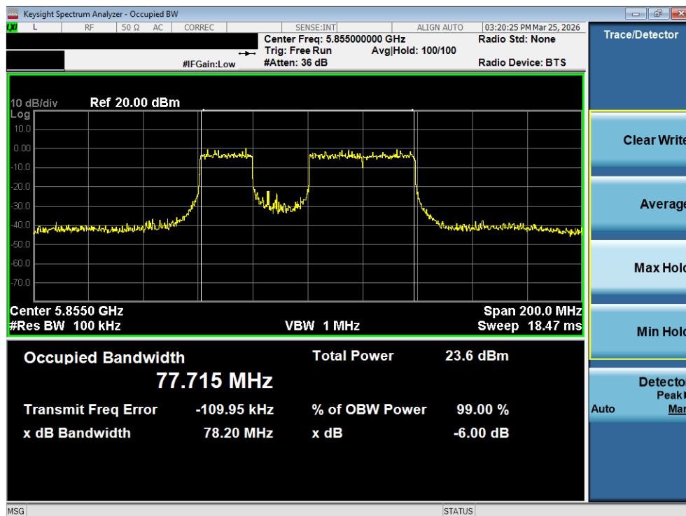
Plot 7-59. 6dB Bandwidth Plot MIMO ANT2 (80MHz BW 802.11be (20MHz Punct.) (UNII Band 3/4) – Ch. 171)
