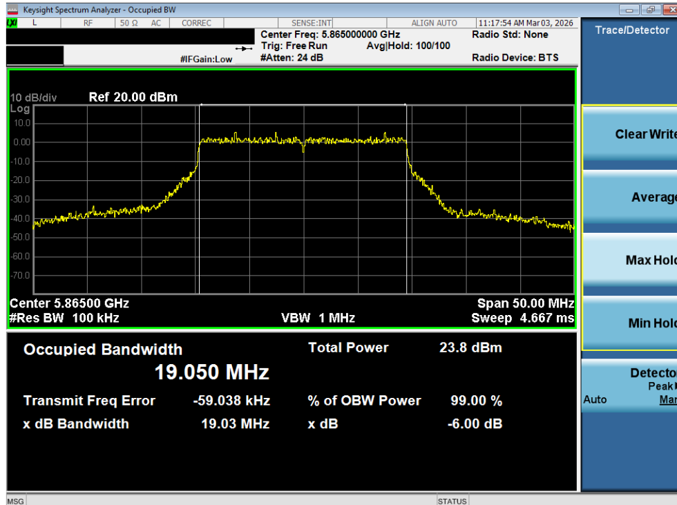
Plot 7-52. 6dB Bandwidth Plot MIMO ANT2 (20MHz BW 802.11be (UNII Band 3/4) – Ch. 173)
