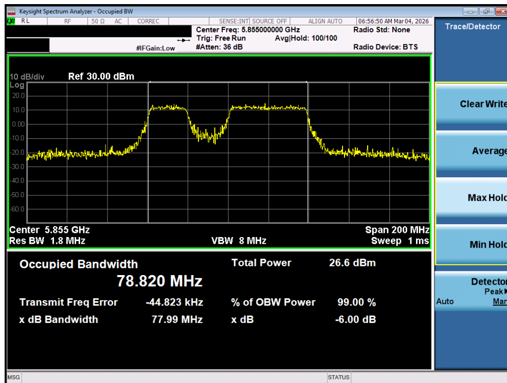
Plot 7-78. OBW Plot MIMO ANT1 (80MHz BW 802.11be (20MHz Punct.) (UNII Band 3/4) – Ch. 171)
