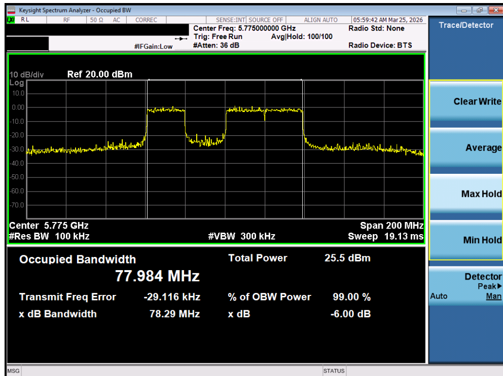
Plot 7-30. 6dB Bandwidth Plot MIMO ANT1 (80MHz BW 802.11be (20MHz Punct.) (UNII Band 3) – Ch. 155)
