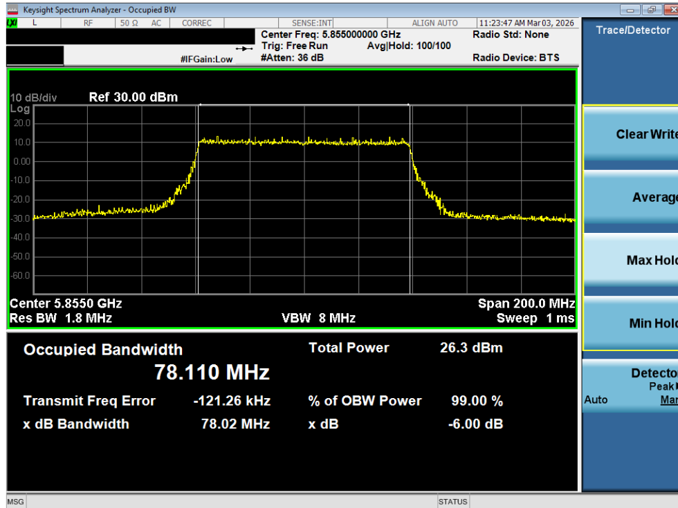
Plot 7-94. OBW Plot MIMO ANT2 (80MHz BW 802.11be (UNII Band 3/4) – Ch. 171)
