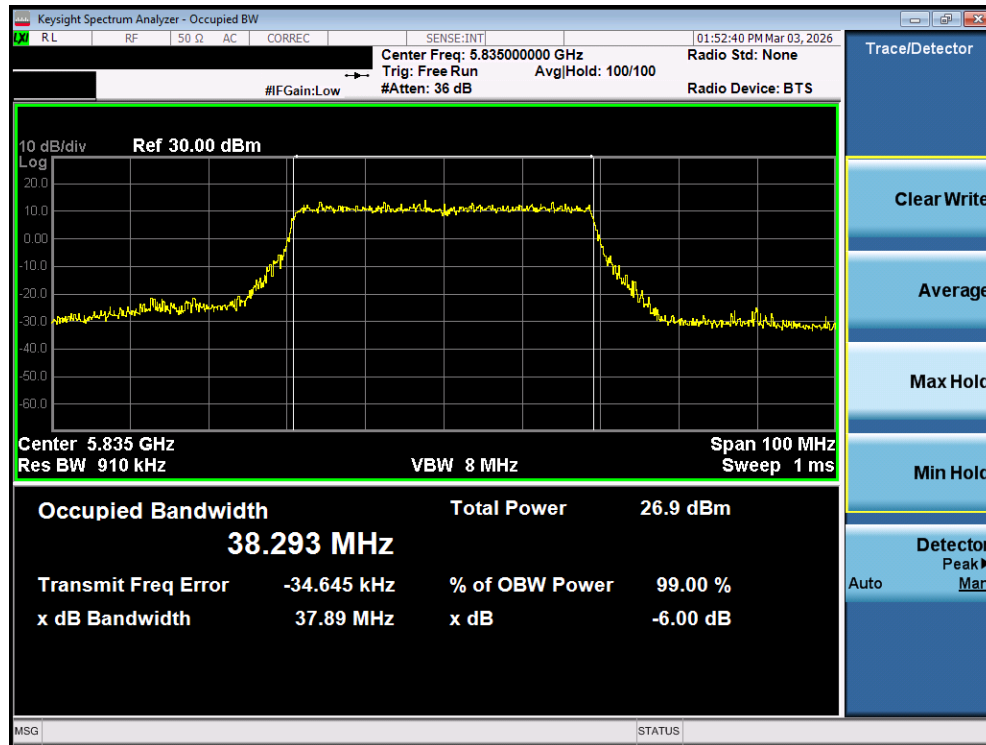
Plot 7-73. OBW Plot MIMO ANT1 (40MHz BW 802.11be (UNII Band 3/4) – Ch. 167)
