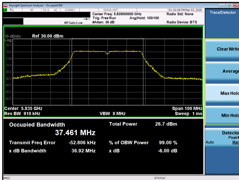
Plot 7-72. OBW Plot MIMO ANT1 (40MHz BW 802.11n (UNII Band 3/4) – Ch. 167)
