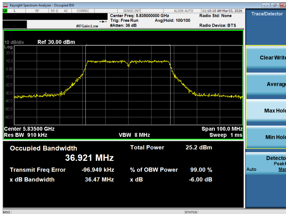
Plot 7-91. OBW Plot MIMO ANT2 (40MHz BW 802.11n (UNII Band 3/4) – Ch. 167)
