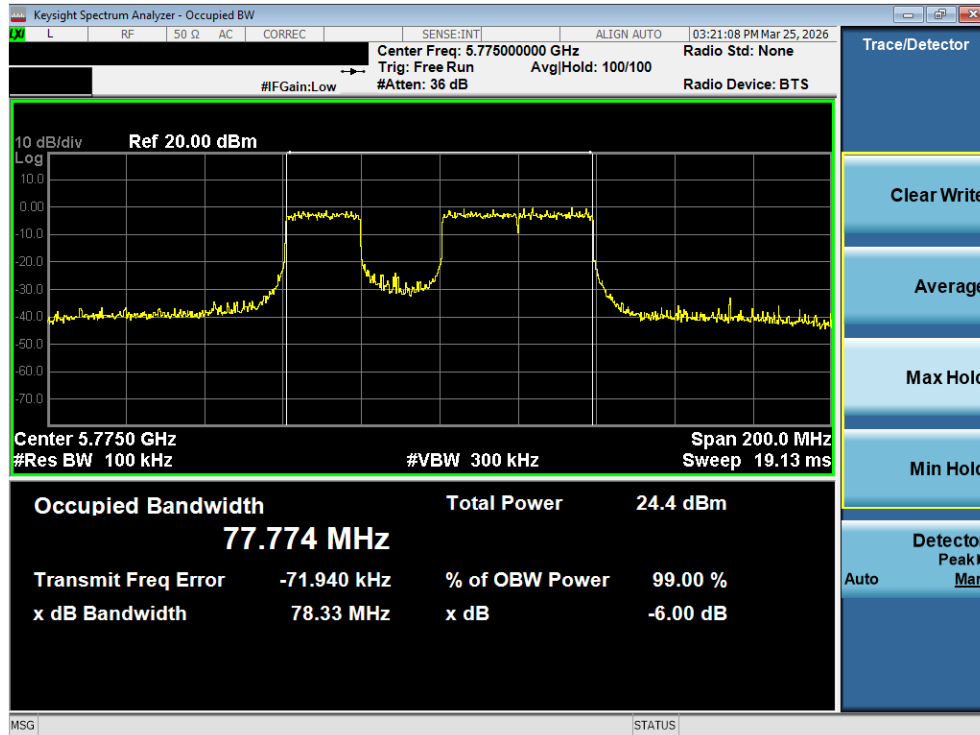
Plot 7-48. 6dB Bandwidth Plot MIMO ANT2 (80MHz BW 802.11be (20MHz Punct.) (UNII Band 3) – Ch. 155)
