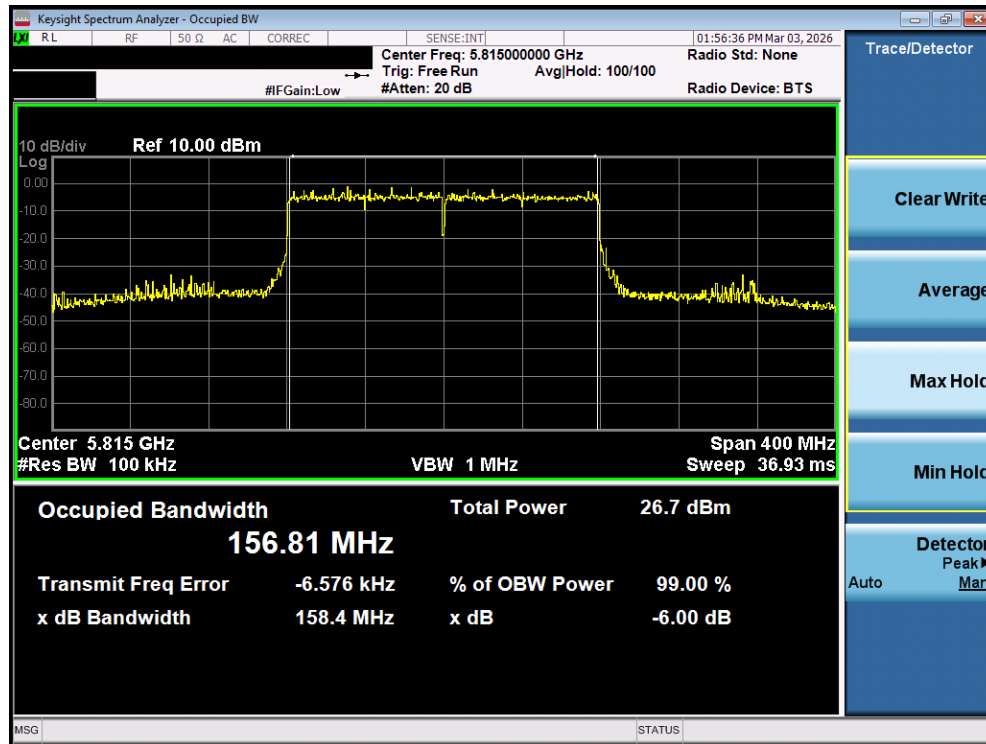
Plot 7-39. 6dB Bandwidth Plot MIMO ANT1 (160MHz BW 802.11be (UNII Band 3/4) – Ch. 163)
