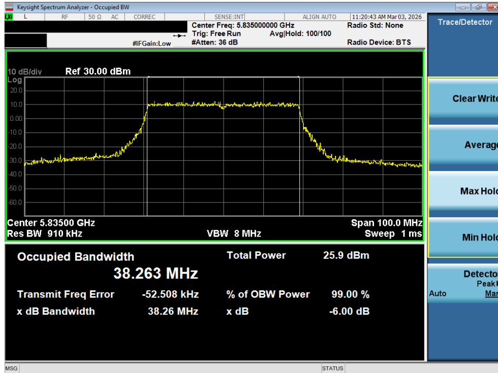
Plot 7-92. OBW Plot MIMO ANT2 (40MHz BW 802.11be (UNII Band 3/4) – Ch. 167)
