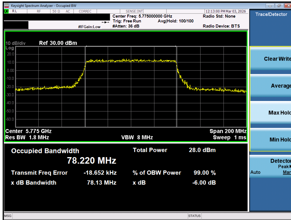
Plot 7-67. OBW Plot MIMO ANT1 (80MHz BW 802.11be (UNII Band 3) – Ch. 155)
