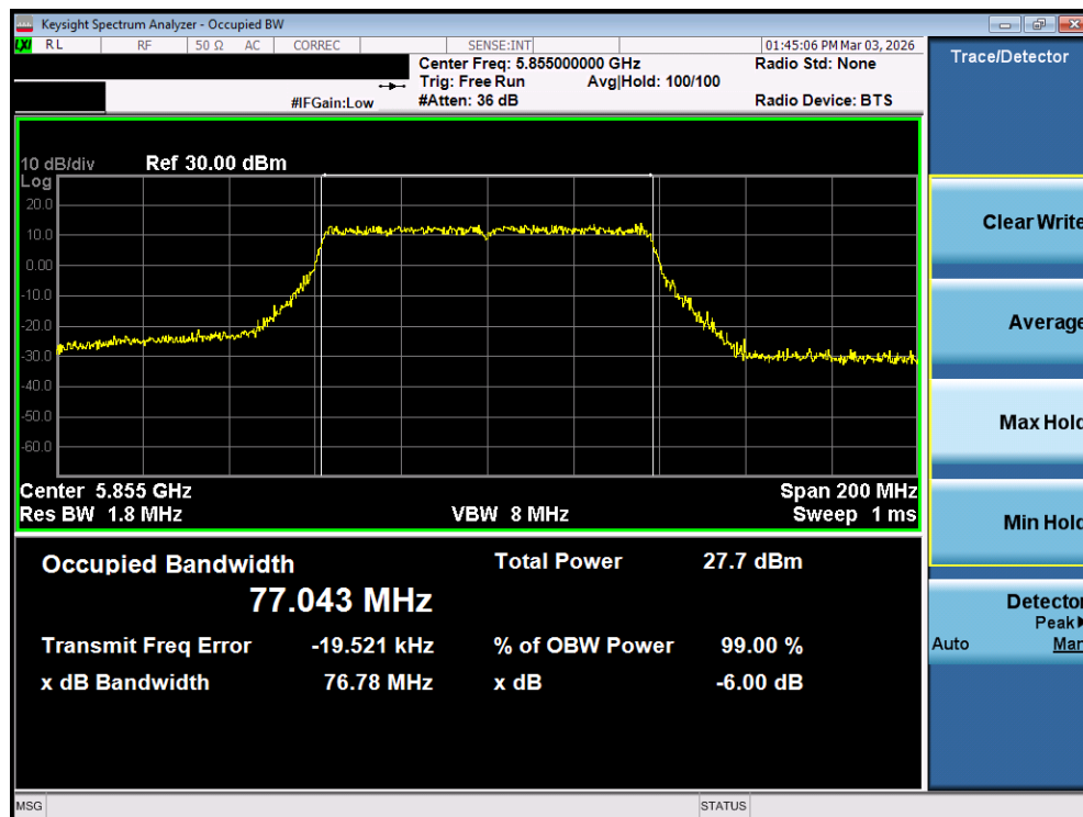
Plot 7-74. OBW Plot MIMO ANT1 (80MHz BW 802.11ac (UNII Band 3/4) – Ch. 171)
