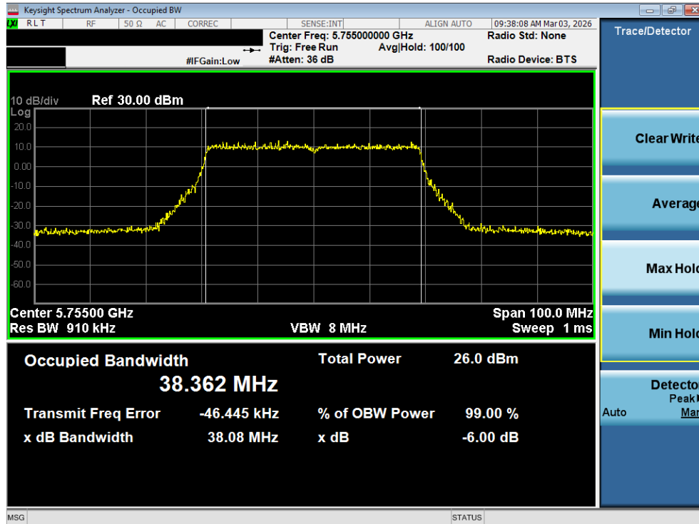
Plot 7-84. OBW Plot MIMO ANT2 (40MHz BW 802.11be (UNII Band 3) – Ch. 151)
