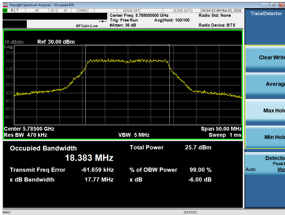
Plot 7-81. OBW Plot MIMO ANT2 (20MHz BW 802.11n (UNII Band 3) – Ch. 157)
