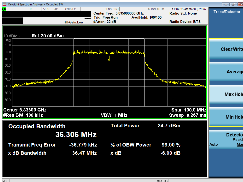
Plot 7-53. 6dB Bandwidth Plot MIMO ANT2 (40MHz BW 802.11n (UNII Band 3/4) – Ch. 167)
