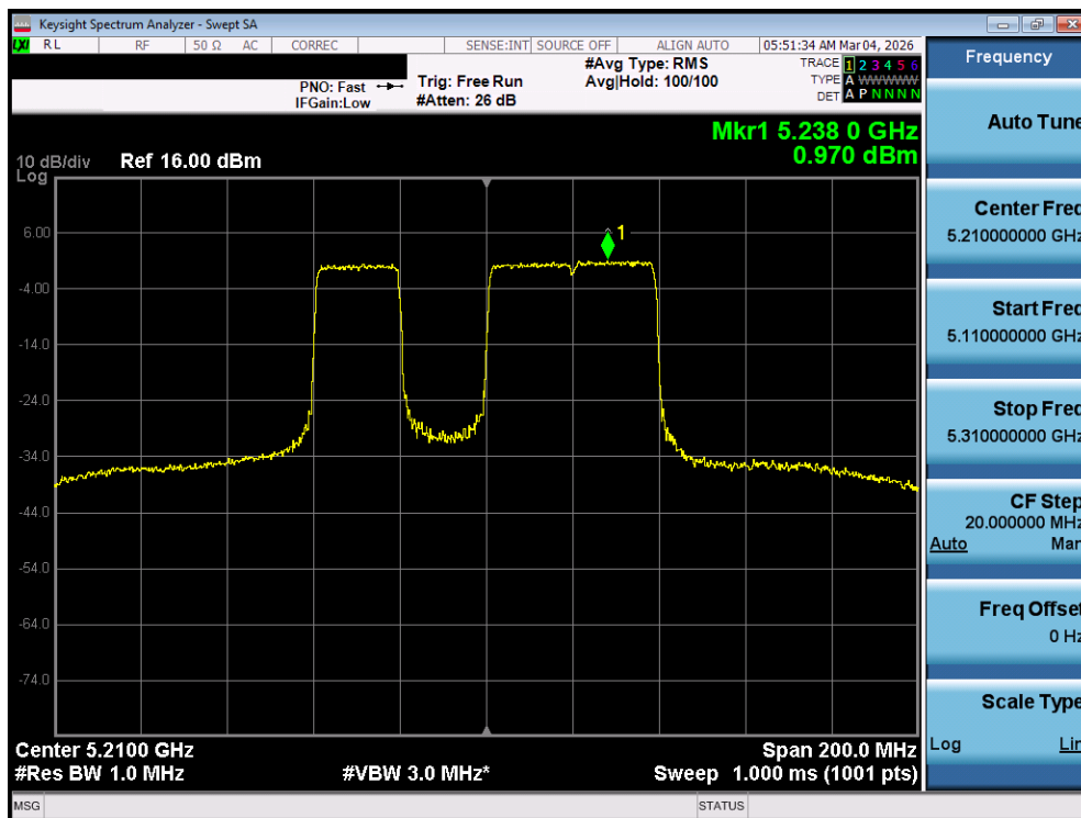
Plot 7-106. Power Spectral Density Plot MIMO ANT1 (80MHz BW 802.11be (20MHz Punct.) (UNII Band 1) – Ch. 42)
