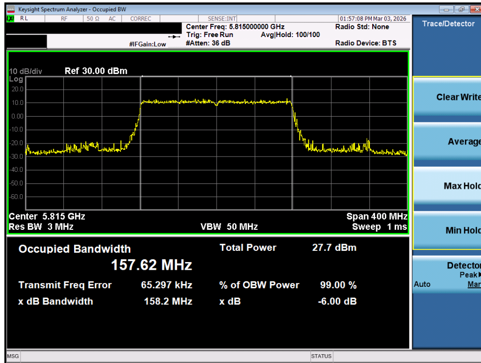
Plot 7-77. OBW Plot MIMO ANT1 (160MHz BW 802.11be (UNII Band 3/4) – Ch. 163)
