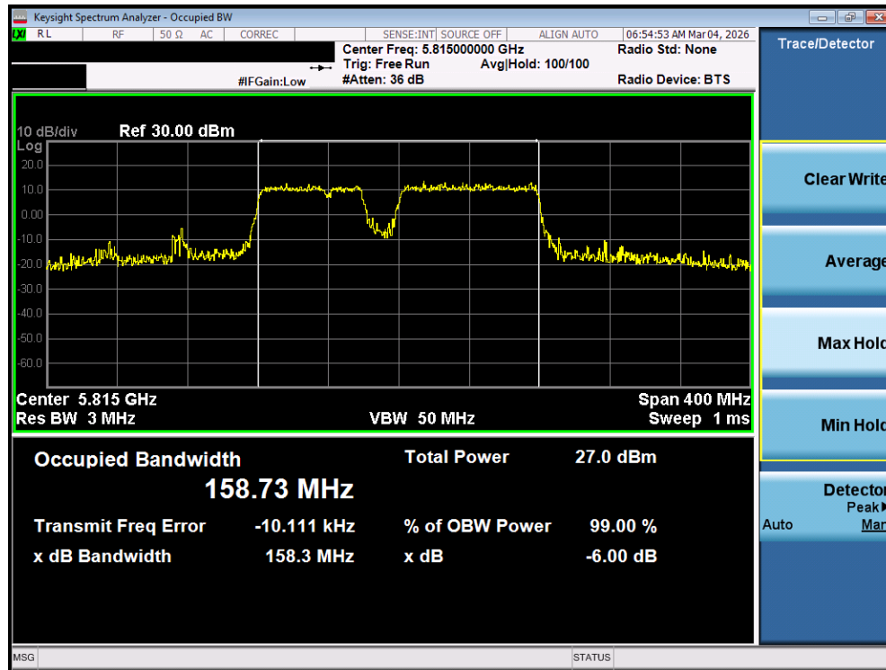
Plot 7-79. OBW Plot MIMO ANT1 (160MHz BW 802.11be (20MHz Punct.) (UNII Band 3/4) – Ch. 163)
