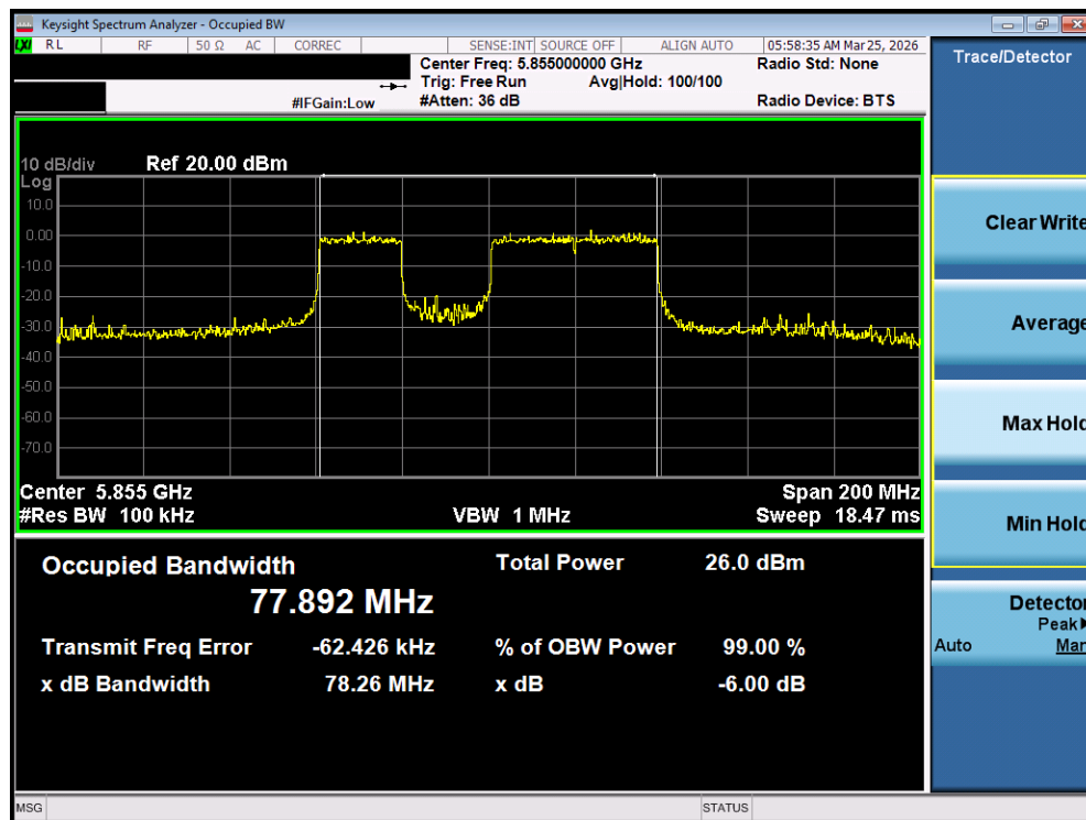
Plot 7-40. 6dB BW Bandwidth Plot MIMO ANT1 (80MHz BW 802.11be (20MHz Punct.) (UNII Band 3/4) – Ch. 171)
