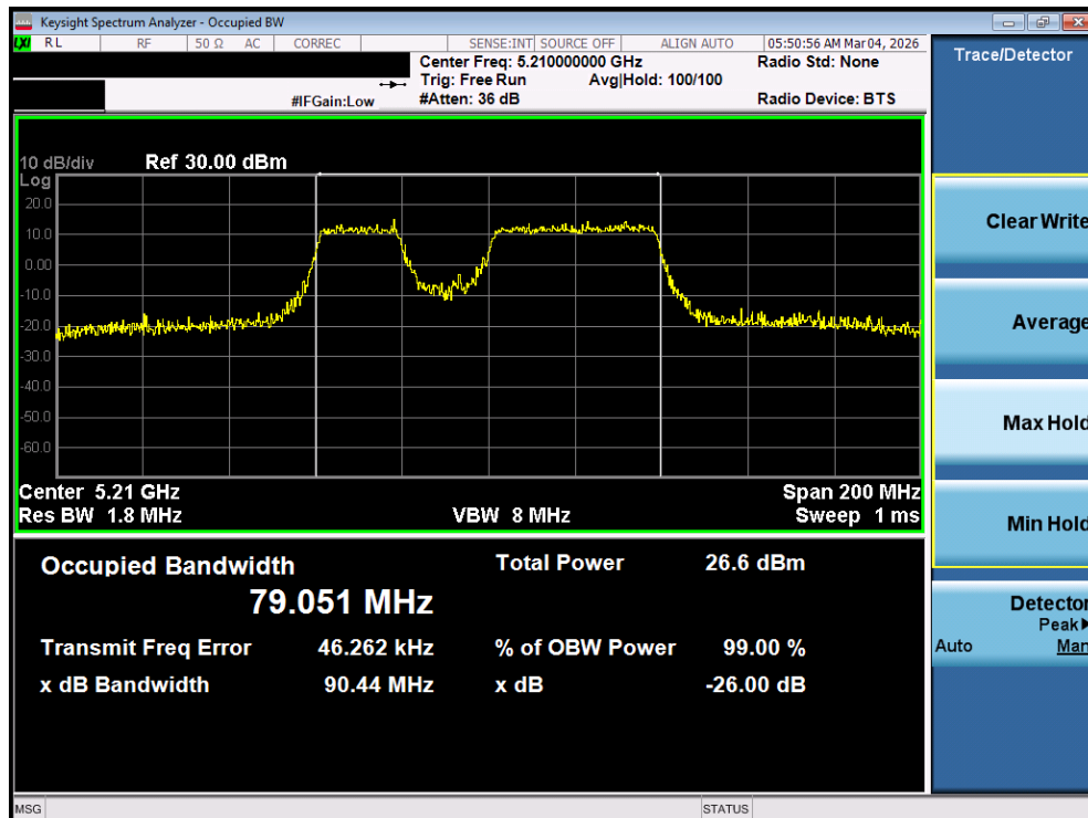
Plot 7-10. 26dB Bandwidth Plot MIMO ANT1 (80MHz BW 802.11be (20MHz Punct.) (UNII Band 1) – Ch. 42)
