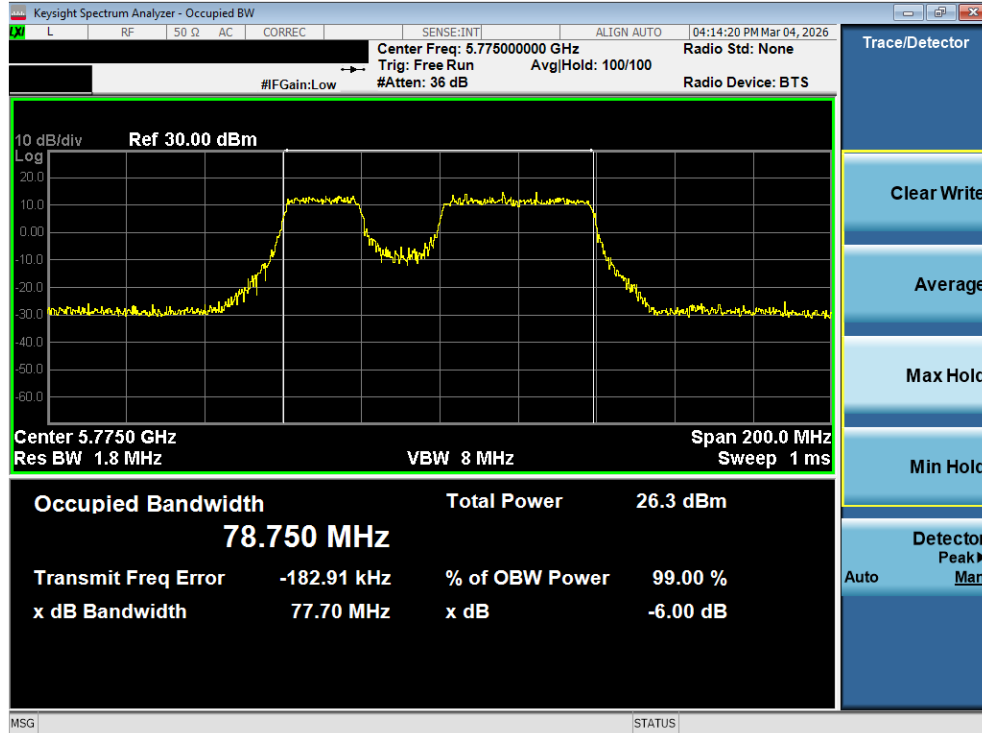
Plot 7-86. OBW Plot MIMO ANT2 (80MHz BW 802.11be (20MHz Punct.) (UNII Band 3) – Ch. 155)
