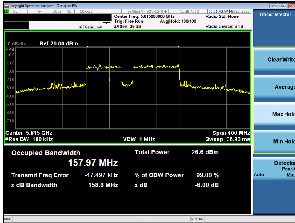
Plot 7-41. 6dB Bandwidth Plot MIMO ANT1 (160MHz BW 802.11be (20MHz Punct.) (UNII Band 3/4) – Ch. 163)
