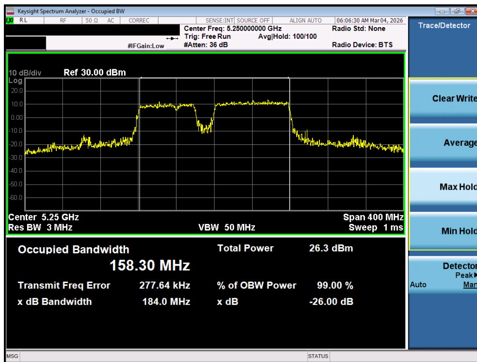
Plot 7-11. 26dB Bandwidth Plot MIMO ANT1 (160MHz BW 802.11be (20MHz Punct.) (UNII Band 1/2A) – Ch. 50)
