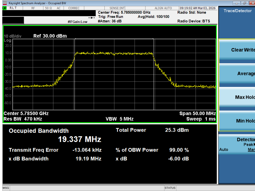
Plot 7-82. OBW Plot MIMO ANT2 (20MHz BW 802.11be (UNII Band 3) – Ch. 157)
