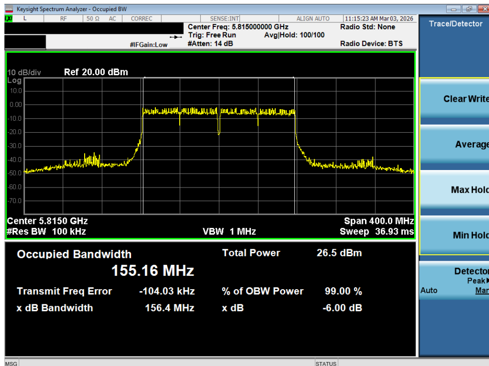
Plot 7-57. 6dB Bandwidth Plot MIMO ANT2 (160MHz BW 802.11ac (UNII Band 3/4) – Ch. 163)
