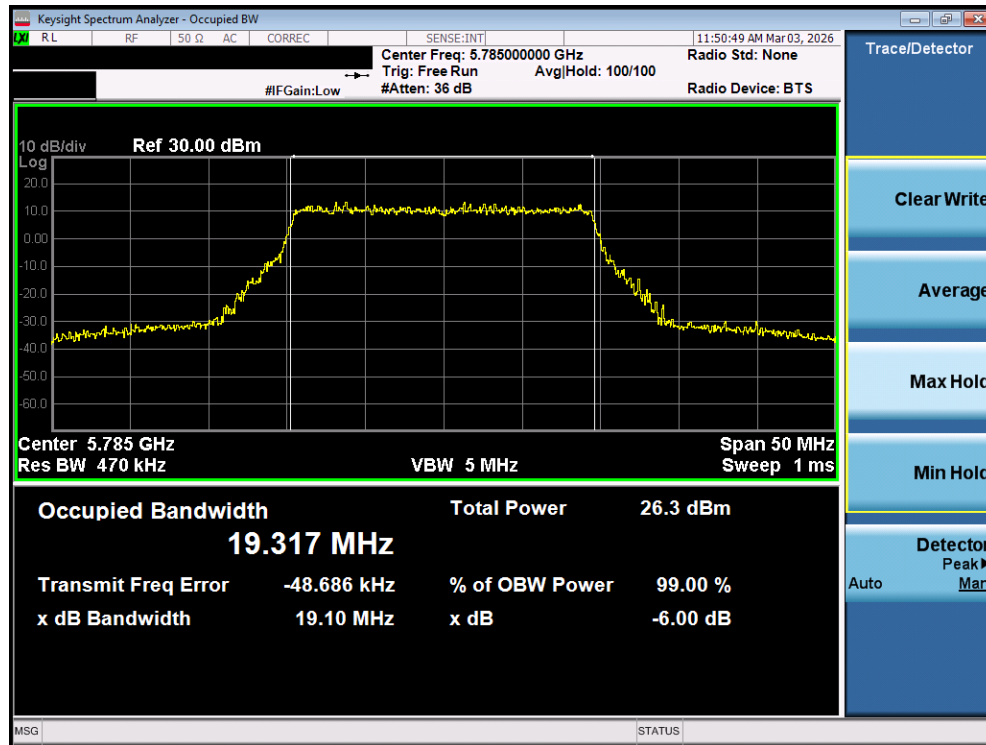
Plot 7-63. OBW Plot MIMO ANT1 (20MHz BW 802.11be (UNII Band 3) – Ch. 157)
