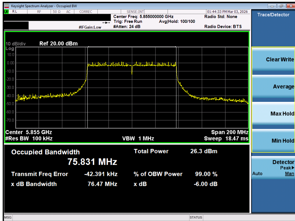
Plot 7-36. 6dB Bandwidth Plot MIMO ANT1 (80MHz BW 802.11ac (UNII Band 3/4) – Ch. 171)
