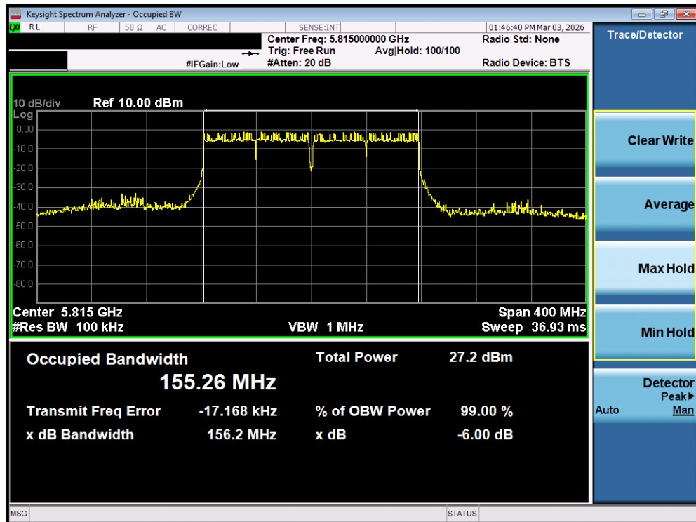
Plot 7-38. 6dB Bandwidth Plot MIMO ANT1 (160MHz BW 802.11ac (UNII Band 3/4) – Ch. 163)
