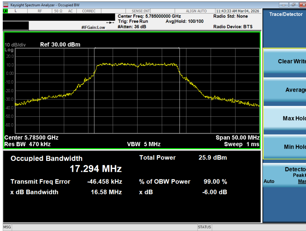
Plot 7-80. OBW Plot MIMO ANT2 (802.11a (UNII Band 3) – Ch. 157)
