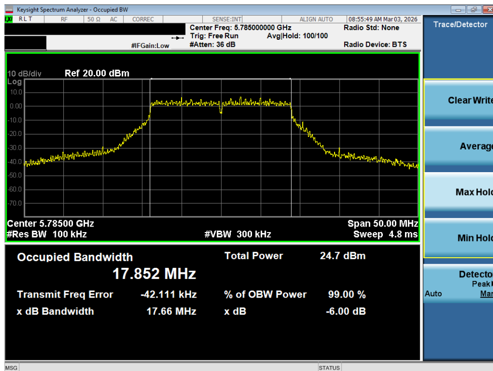
Plot 7-43. 6dB Bandwidth Plot MIMO ANT2 (20MHz BW 802.11n (UNII Band 3) – Ch. 157)
