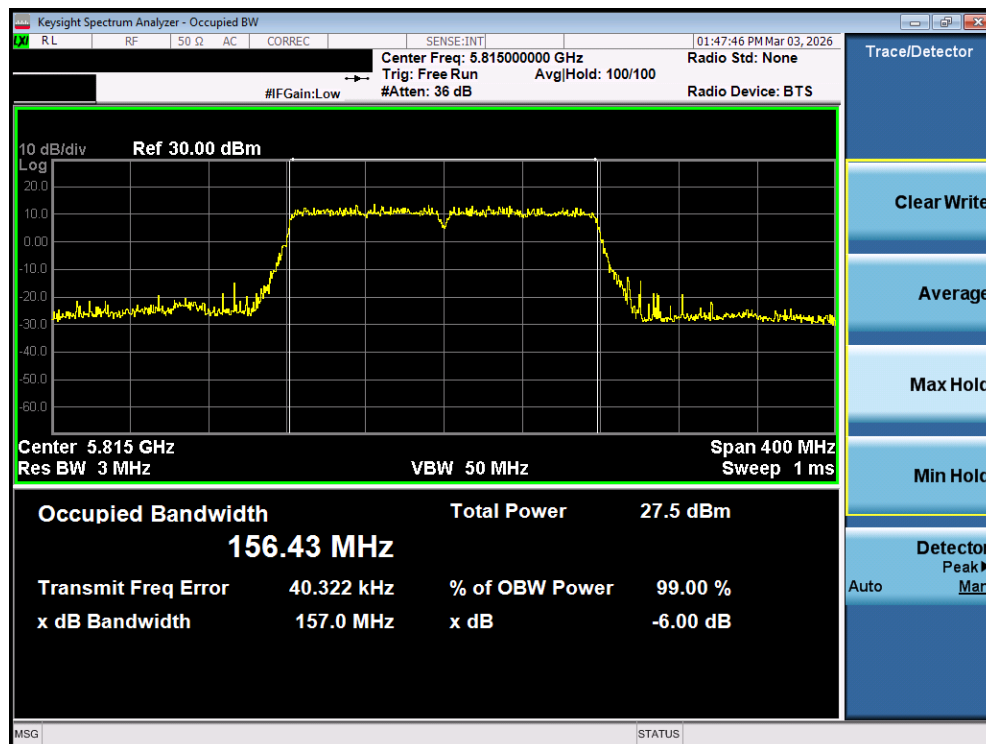
Plot 7-76. OBW Plot MIMO ANT1 (160MHz BW 802.11ac (UNII Band 3/4) – Ch. 163)
