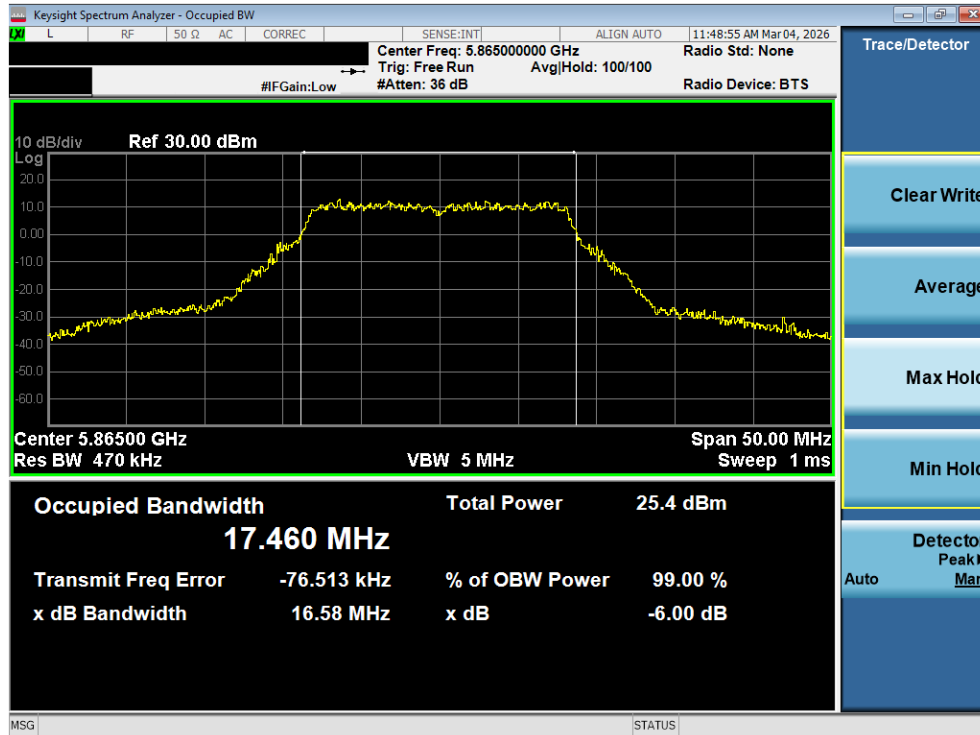
Plot 7-88. OBW Plot MIMO ANT2 (802.11a (UNII Band 3/4) – Ch. 173)
