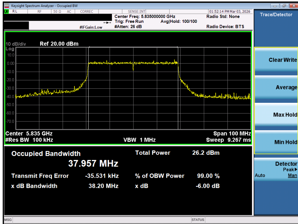
Plot 7-35. 6dB Bandwidth Plot MIMO ANT1 (40MHz BW 802.11be (UNII Band 3/4) – Ch. 167)
