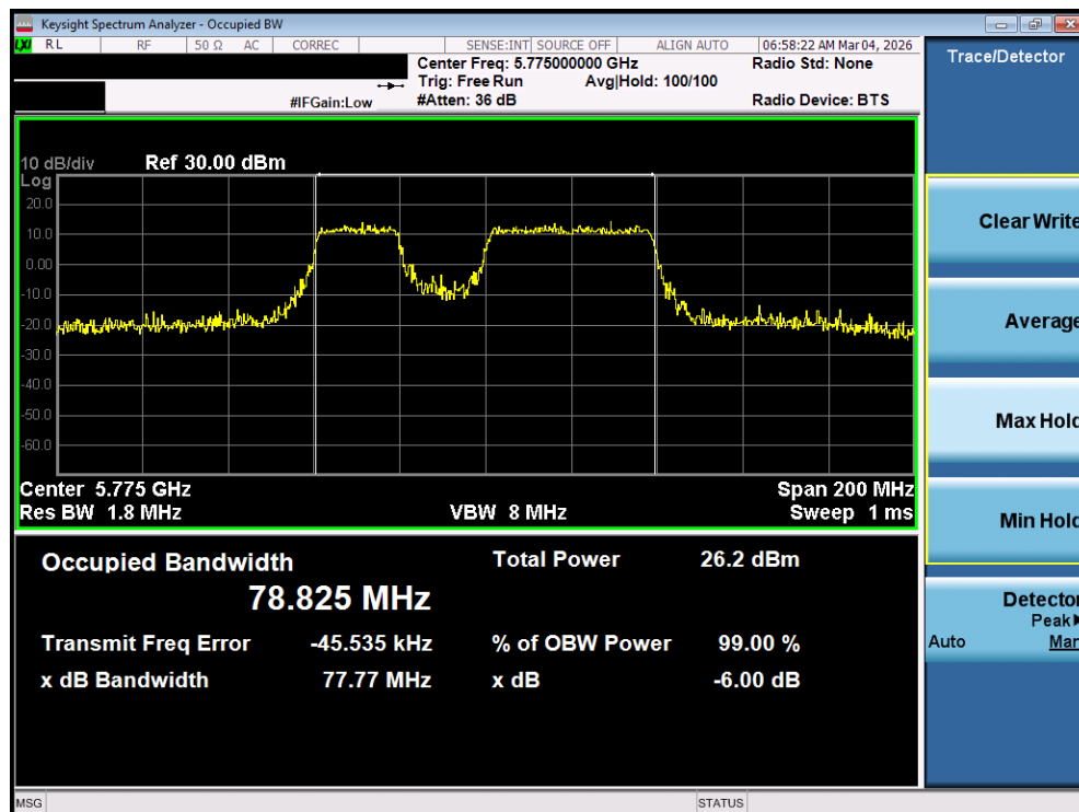
Plot 7-68. OBW Plot MIMO ANT1 (80MHz BW 802.11be (20MHz Punct.) (UNII Band 3) – Ch. 155)
