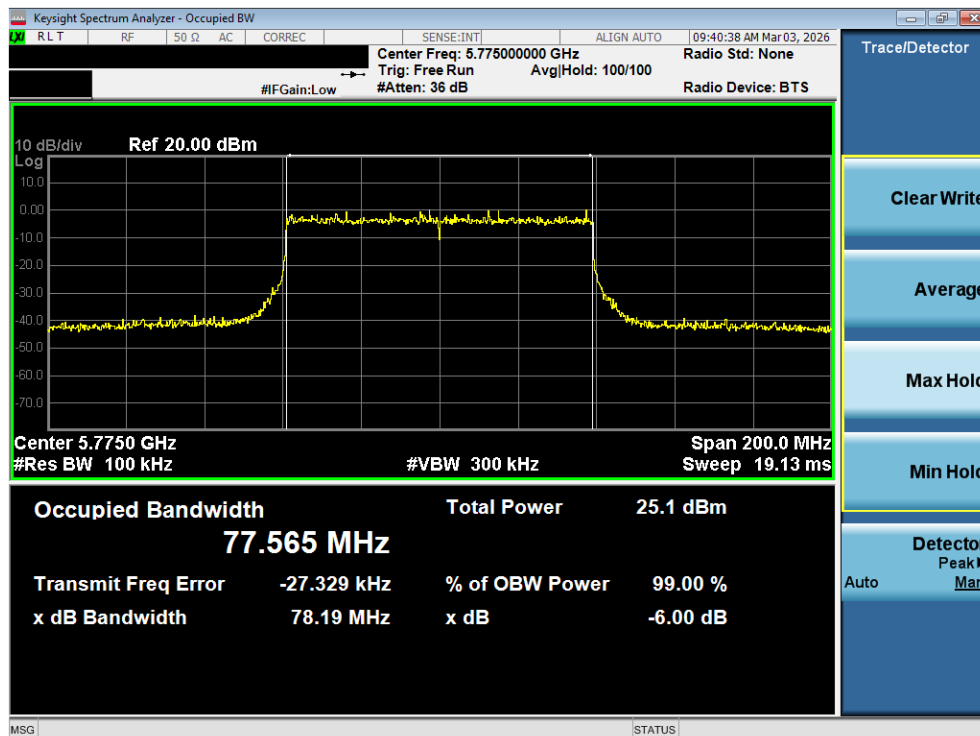
Plot 7-49. 6dB Bandwidth Plot MIMO ANT2 (80MHz BW 802.11be (UNII Band 3) – Ch. 155)
