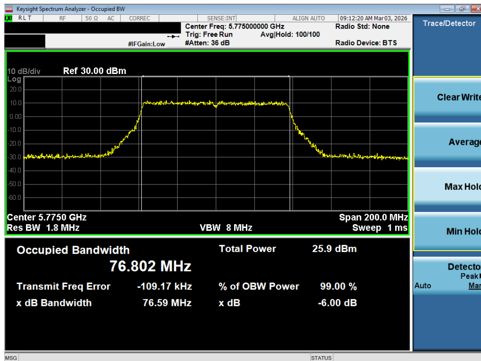
Plot 7-85. OBW Plot MIMO ANT2 (80MHz BW 802.11ac (UNII Band 3) – Ch. 155)
