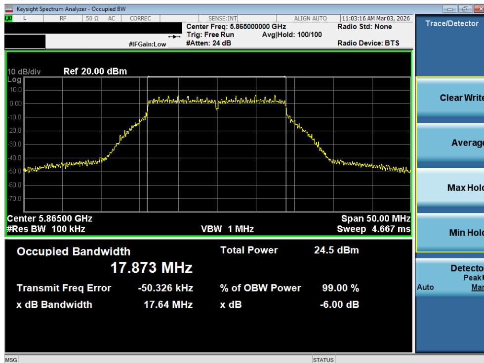
Plot 7-51. 6dB Bandwidth Plot MIMO ANT2 (20MHz BW 802.11n (UNII Band 3/4) – Ch. 173)
