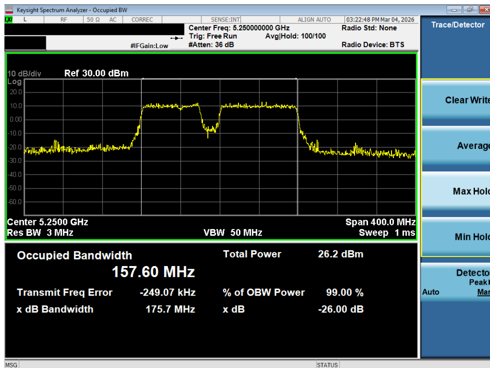
Plot 7-22. 26dB Bandwidth Plot MIMO ANT2 (160MHz BW 802.11be (20MHz Punct.) (UNII Band 1/2A) – Ch. 50)
