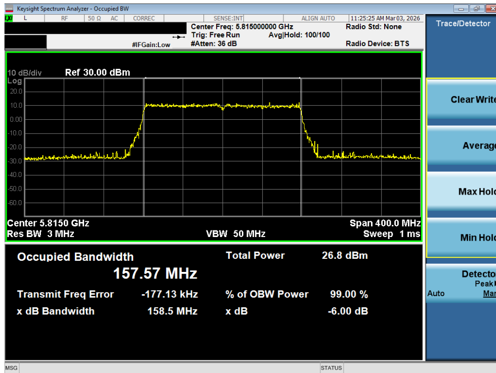
Plot 7-96. OBW Plot MIMO ANT2 (160MHz BW 802.11be (UNII Band 3/4) – Ch. 163)
