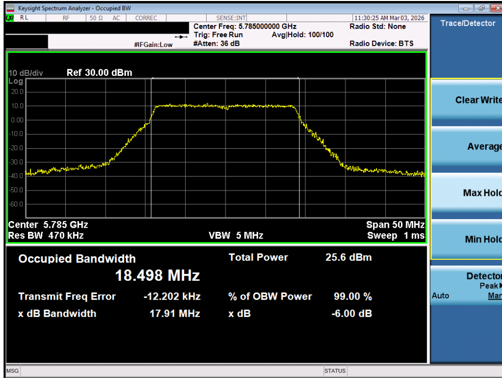
Plot 7-62. OBW Plot MIMO ANT1 (20MHz BW 802.11n (UNII Band 3) – Ch. 157)
