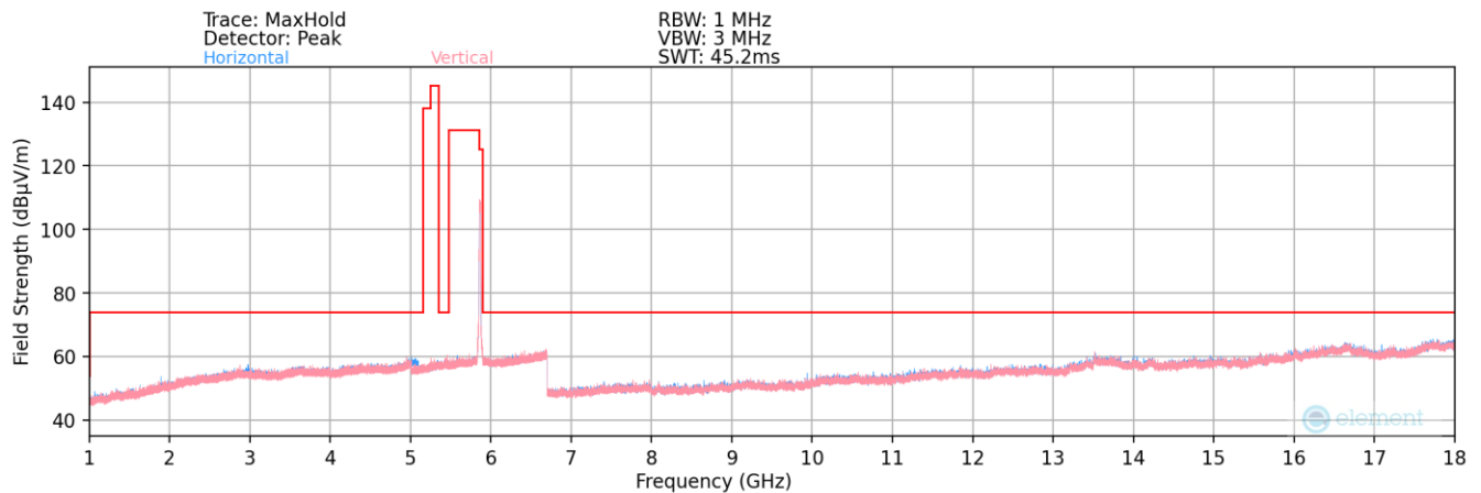
Plot 7-164. Radiated Spurious Plot above 1GHz MIMO (802.11a – UNII Band 4 Ch. 173)
