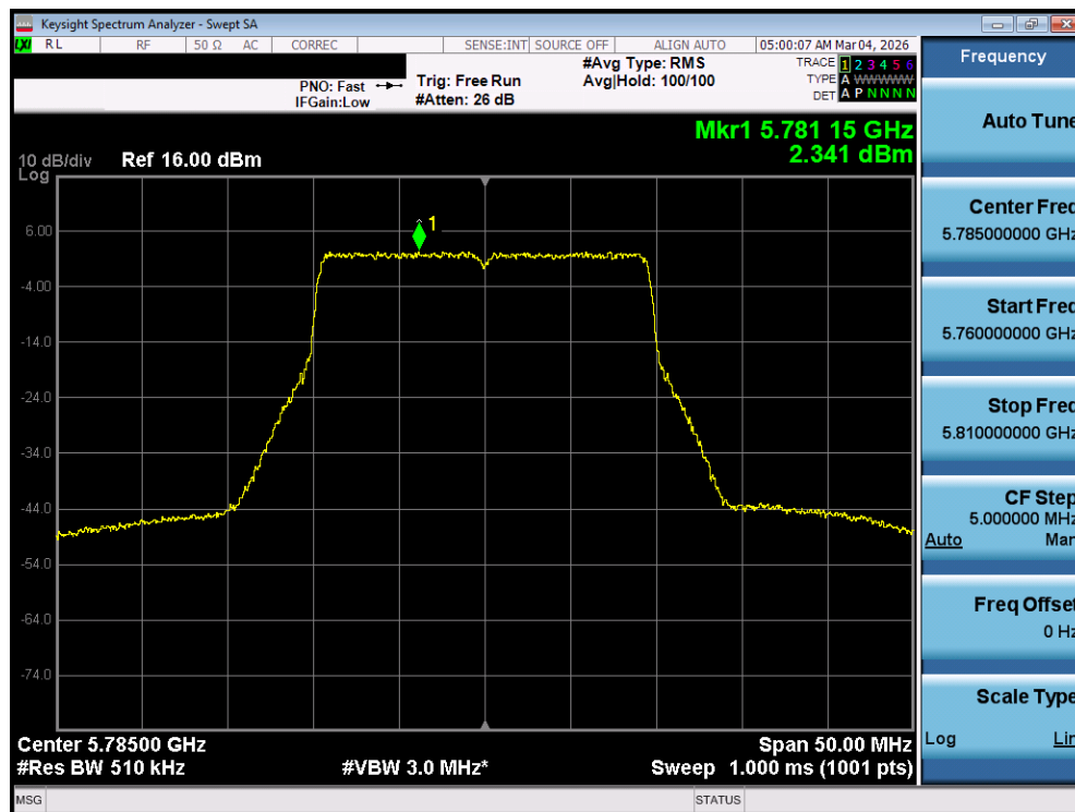
Plot 7-112. Power Spectral Density Plot MIMO ANT1 (20MHz BW 802.11be (UNII Band 3) – Ch. 157)
