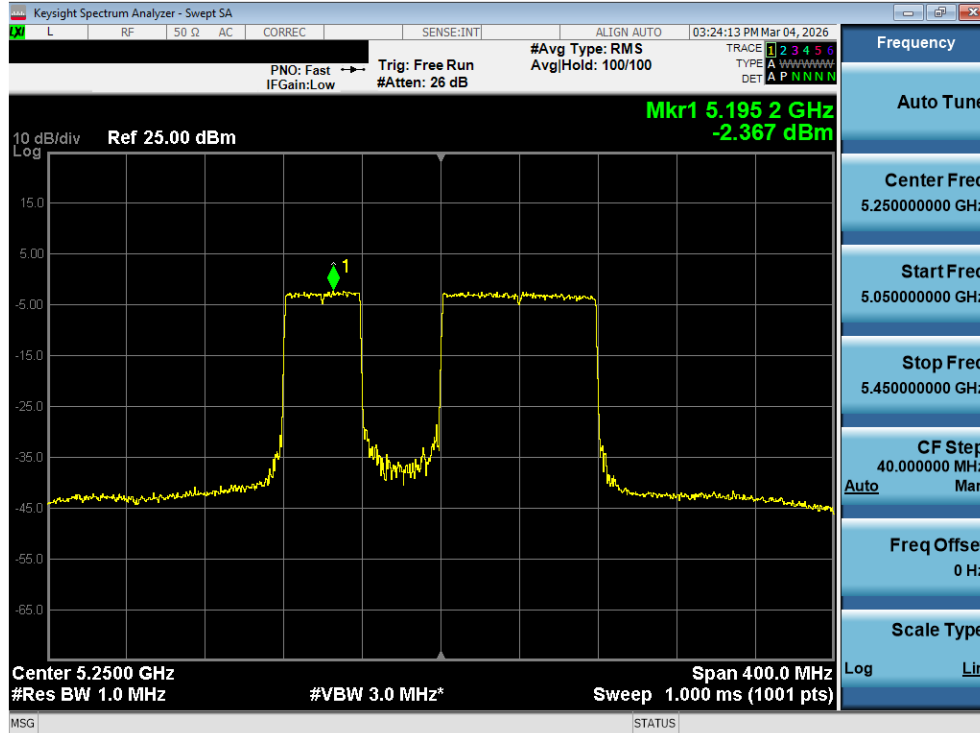
Plot 7-139. Power Spectral Density Plot MIMO ANT2 (160MHz BW 802.11be (40MHz Punct.) (UNII Band 1/2A) – Ch. 50)
