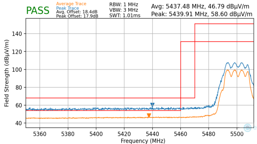
Plot 7-174. Radiated Lower Band Edge Plot MIMO (Average & Peak – UNII Band 2C)
