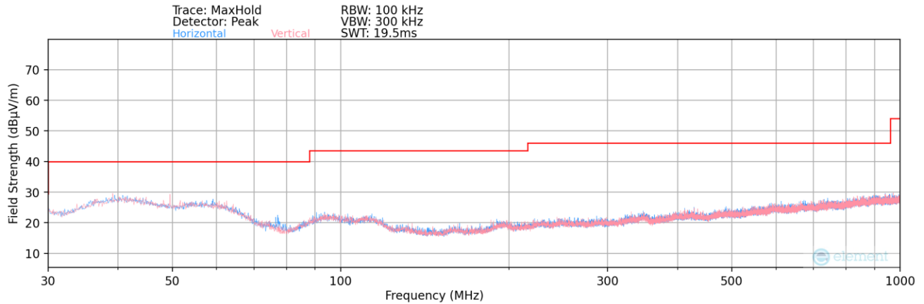
Plot 7-168. Radiated Spurious Plot below 1GHz MIMO 802.11b (2.4GHz – Ch. 6) + MIMO 802.11a (5GHz – Ch. 44)
