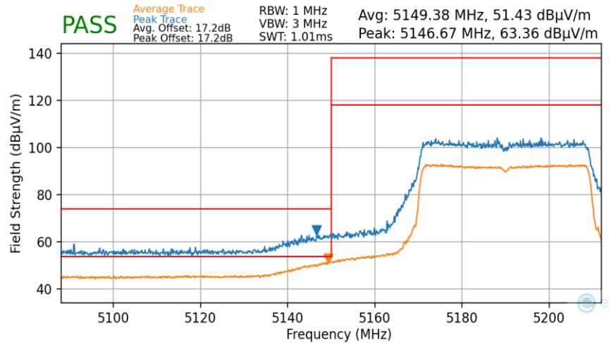
Plot 7-178. Radiated Lower Band Edge Plot MIMO (Average & Peak – UNII Band 1)
