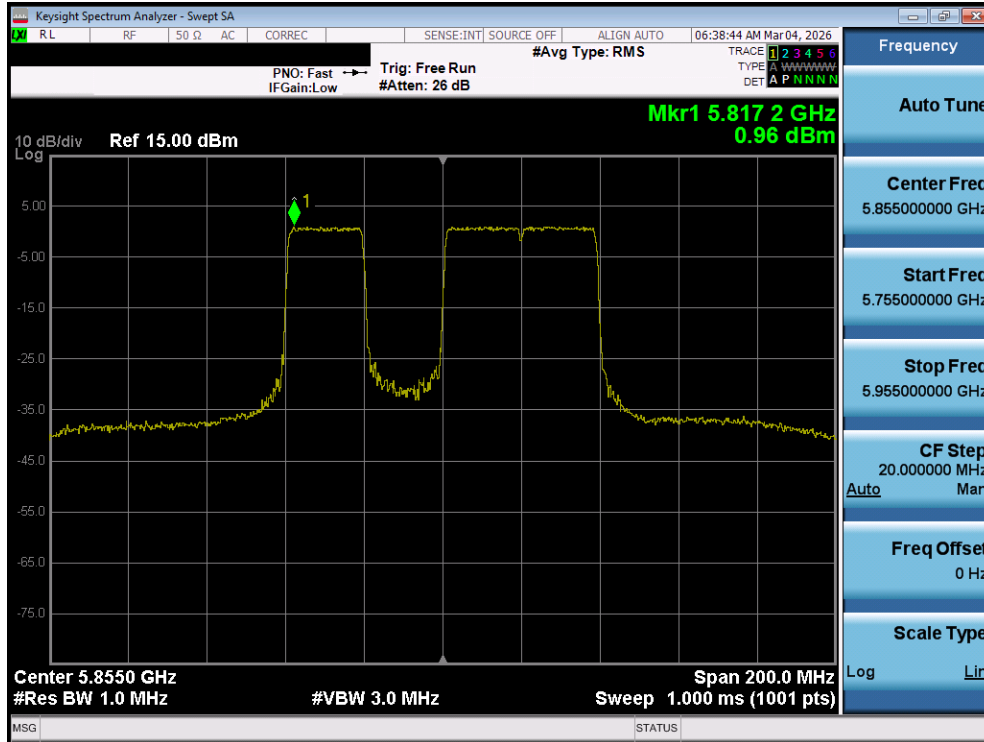
Plot 7-125. Power Spectral Density Plot MIMO ANT1 (80MHz BW 802.11be (20MHz Punct.) (UNII Band 3/4) – Ch. 171)
