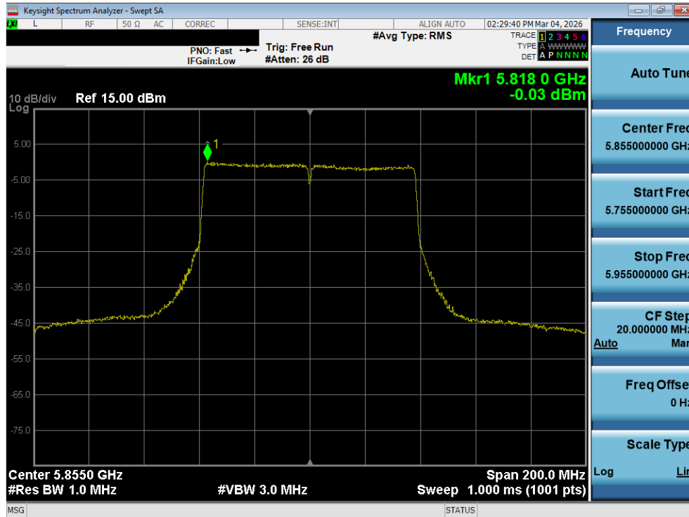
Plot 7-153. Power Spectral Density Plot MIMO ANT2 (80MHz BW 802.11ac (UNII Band 3/4) – Ch. 171)
