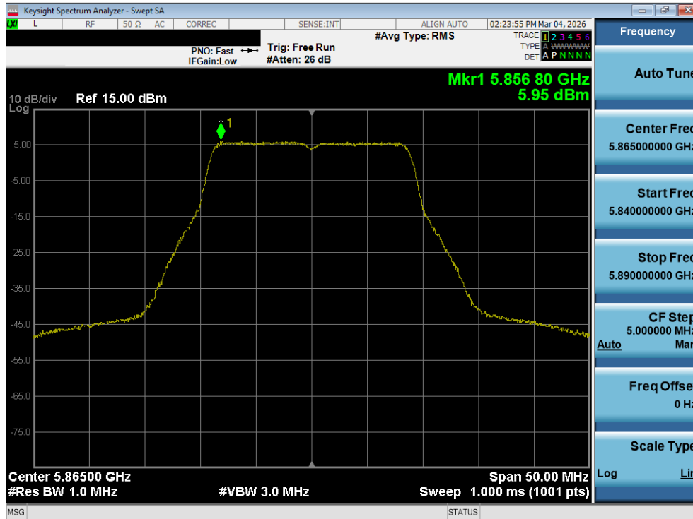
Plot 7-149. Power Spectral Density Plot MIMO ANT2 (20MHz BW 802.11n (UNII Band 4) – Ch. 173)
