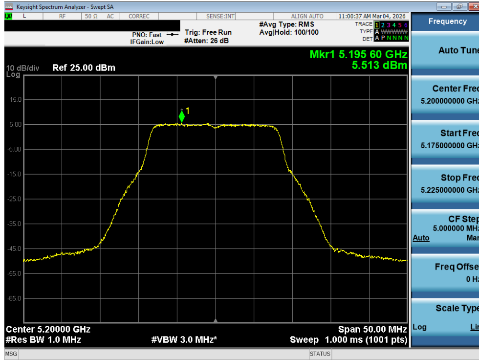
Plot 7-129. Power Spectral Density Plot MIMO ANT2 (802.11a (UNII Band 1) – Ch. 40)
