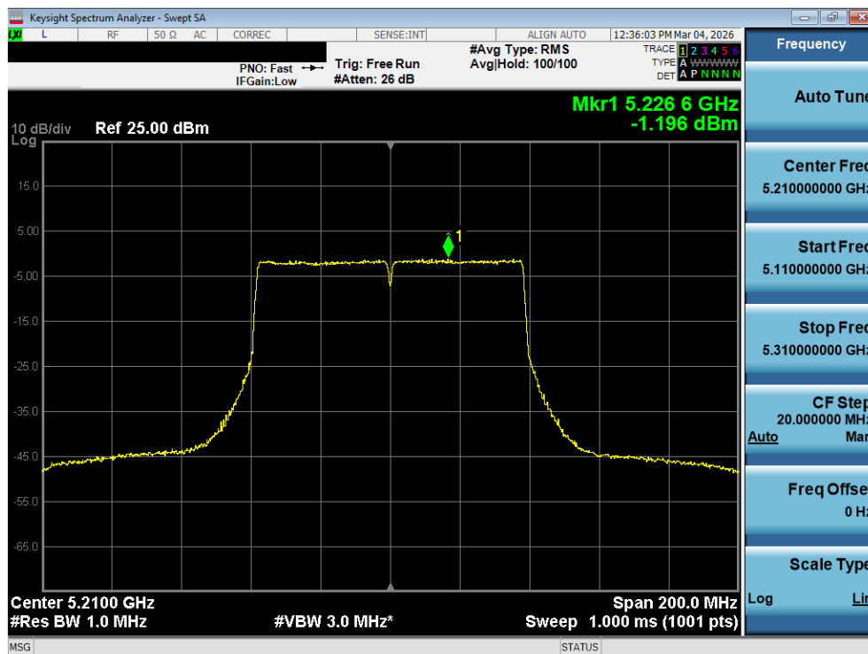
Plot 7-134. Power Spectral Density Plot MIMO ANT2 (80MHz BW 802.11ac (UNII Band 1) – Ch. 42)
