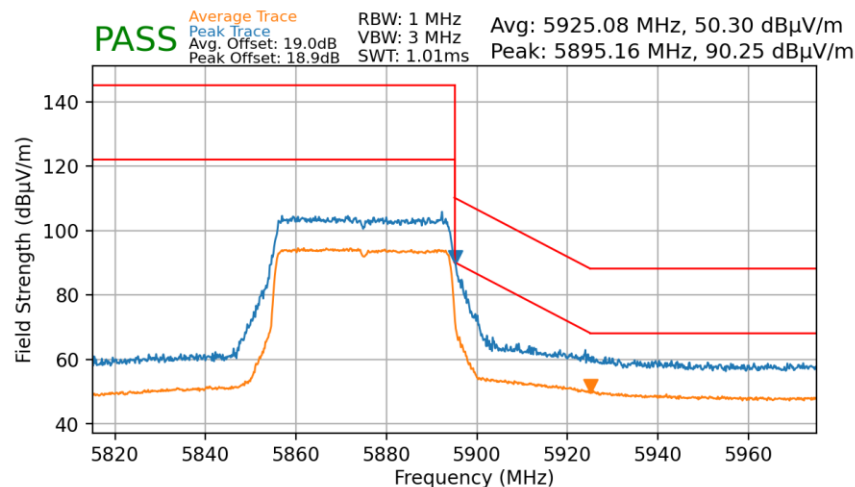
Plot 7-183. Radiated Upper Band Edge Plot MIMO (Average & Peak – UNII Band 4)
