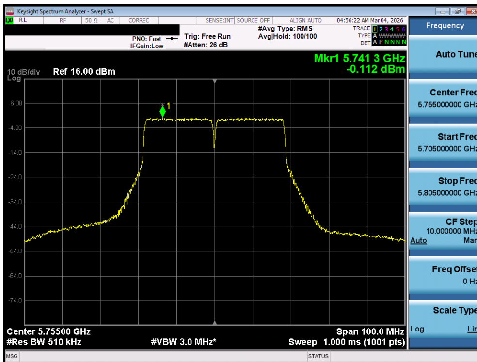
Plot 7-113. Power Spectral Density Plot MIMO ANT1 (40MHz BW 802.11n (UNII Band 3) – Ch. 151)
