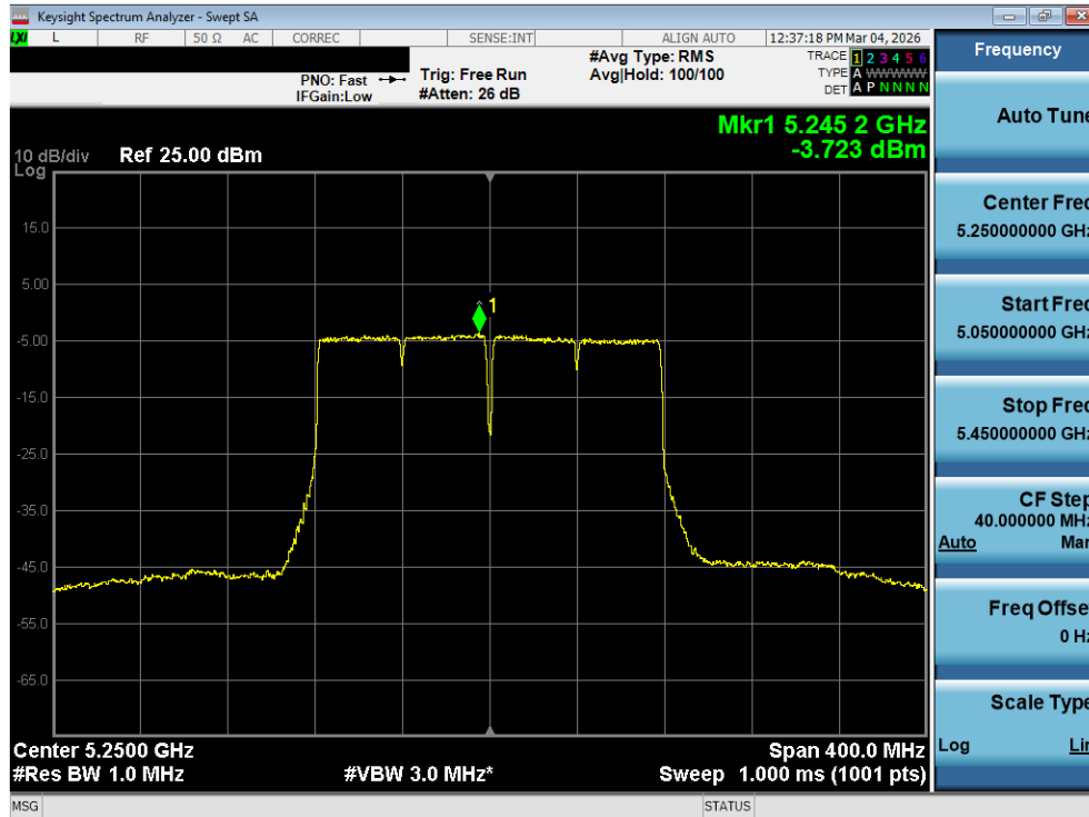
Plot 7-137. Power Spectral Density Plot MIMO ANT2 (160MHz BW 802.11ac (UNII Band 1/2A) – Ch. 50)
