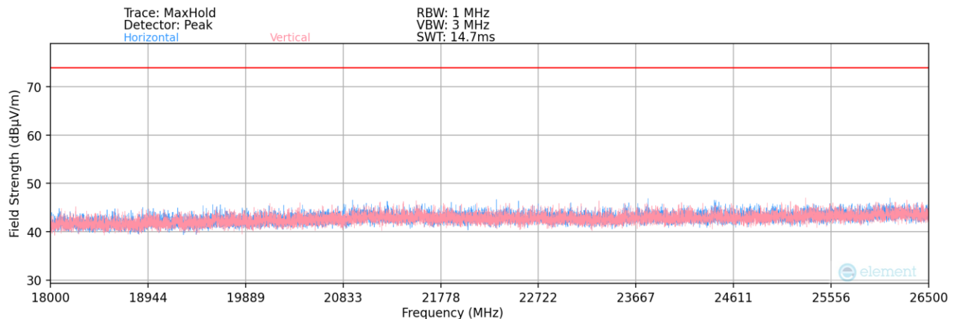
Plot 7-170. Radiated Spurious Plot below 18-26.5GHz MIMO 802.11b (2.4GHz – Ch.6) + MIMO 802.11a (5GHz – Ch. 44)
