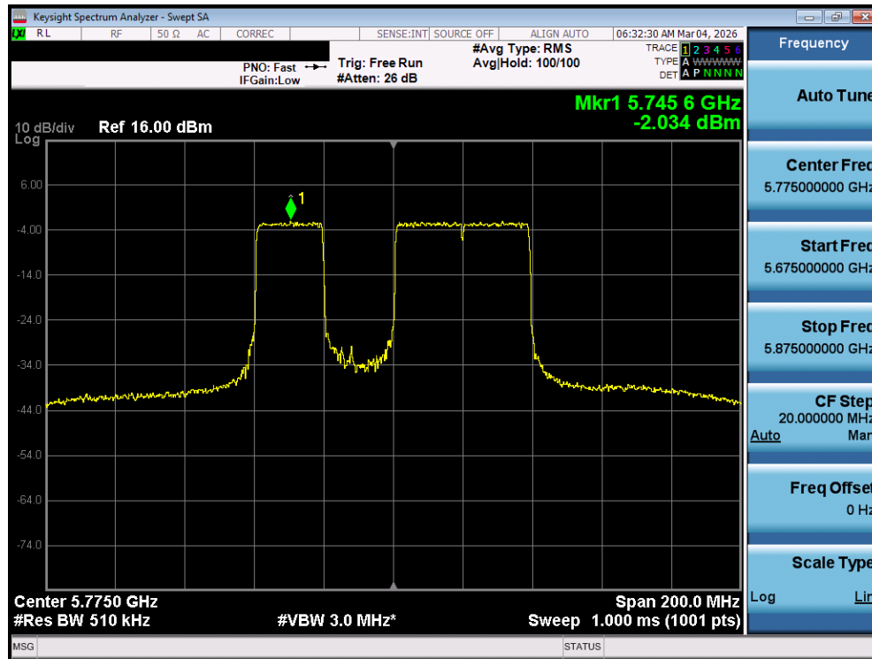
Plot 7-117. Power Spectral Density Plot MIMO ANT1 (80MHz BW 802.11be (20MHz Punct.) (UNII Band 3) – Ch. 155)
