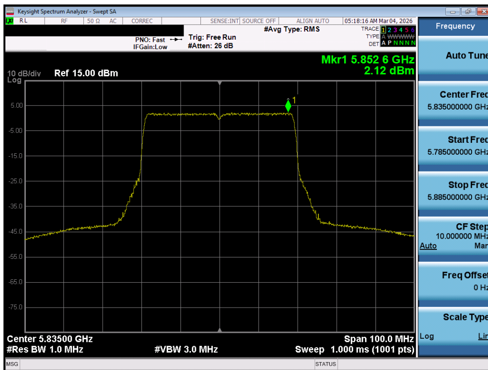
Plot 7-122. Power Spectral Density Plot MIMO ANT1 (40MHz BW 802.11be (UNII Band 3/4) – Ch. 167)
