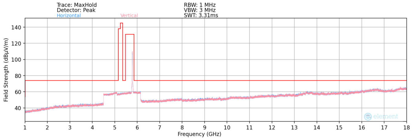
Plot 7-163. Radiated Spurious Plot above 1GHz MIMO (802.11a – UNII Band 3 Ch. 157)
