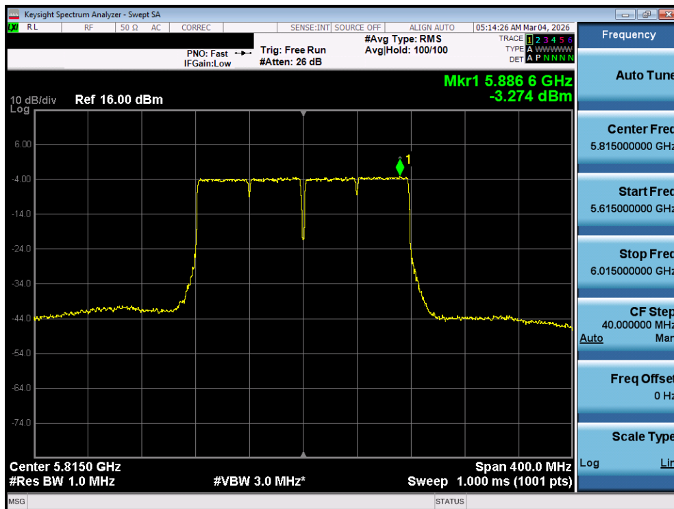
Plot 7-126. Power Spectral Density Plot MIMO ANT1 (160MHz BW 802.11ac (UNII Band 3/4) – Ch. 163)
