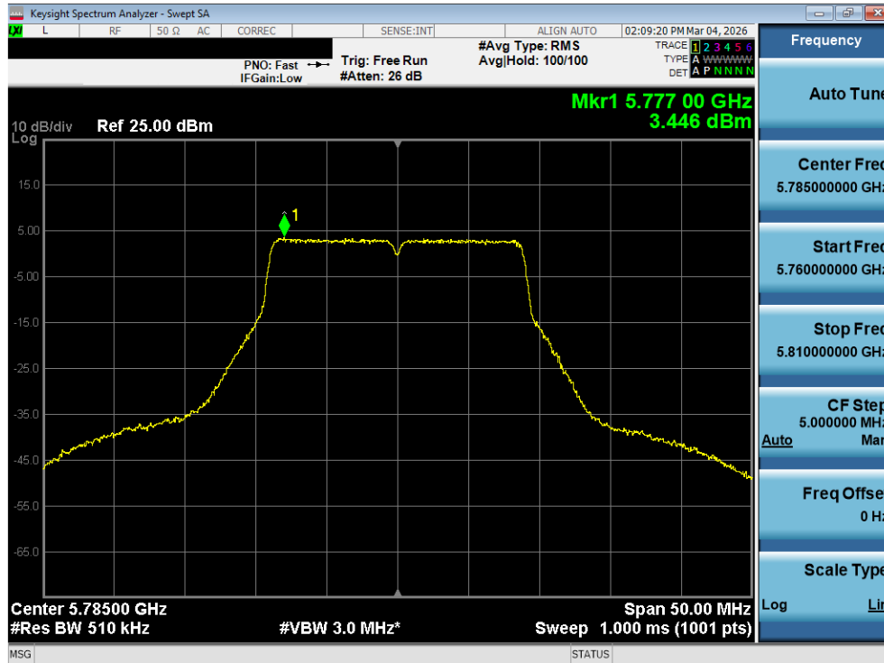
Plot 7-141. Power Spectral Density Plot MIMO ANT2 (20MHz BW 802.11n (UNII Band 3) – Ch. 157)
