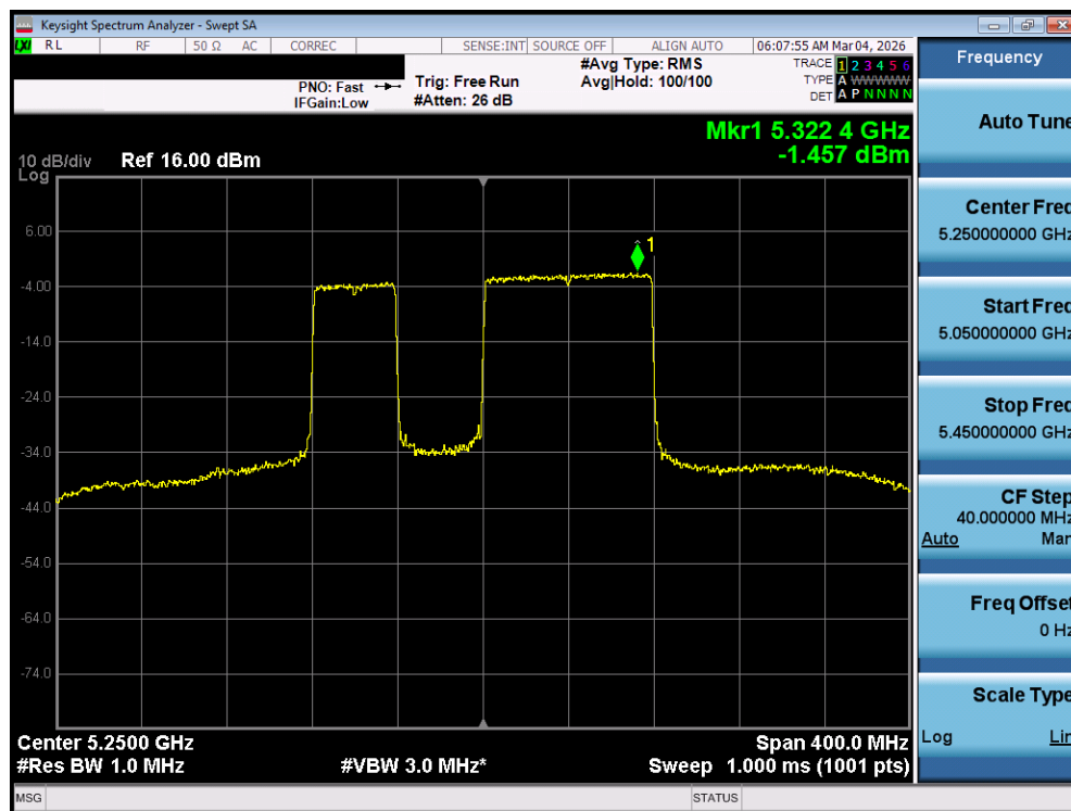
Plot 7-109. Power Spectral Density Plot MIMO ANT1 (160MHz BW 802.11be (40MHz Punct.) (UNII Band 1/2A) – Ch. 50)
