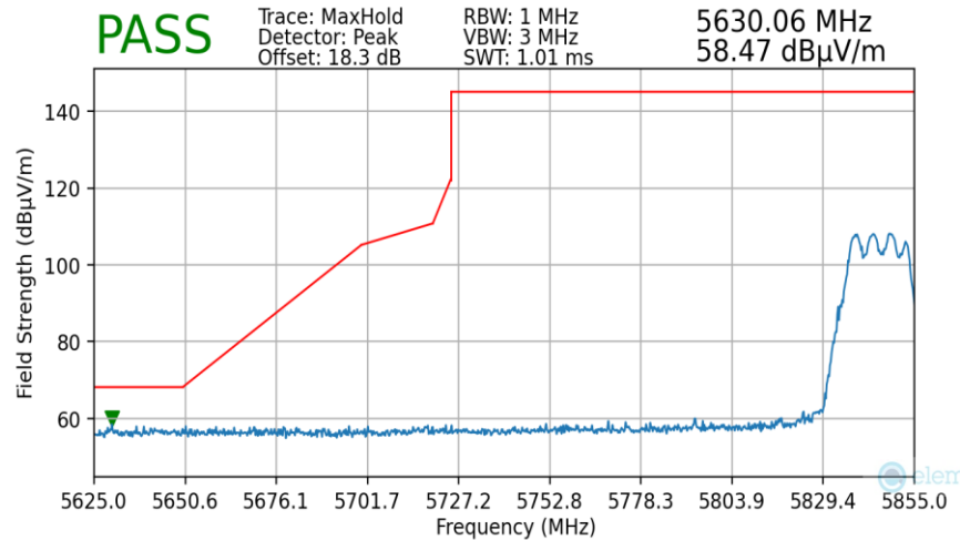
Plot 7-176. Radiated Lower Band Edge Plot MIMO (Peak – UNII Band 4)
