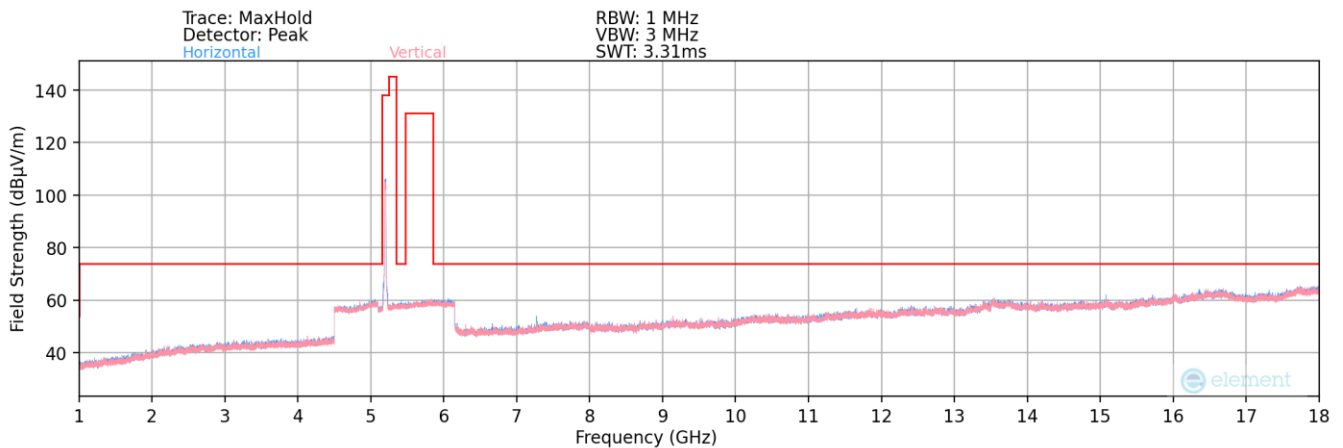
Plot 7-160. Radiated Spurious Plot above 1GHz MIMO (802.11a – UNII Band 1 Ch. 40)
