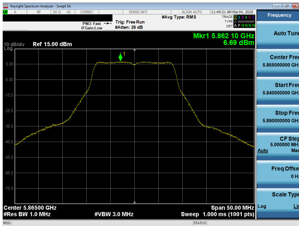
Plot 7-148. Power Spectral Density Plot MIMO ANT2 (802.11a (UNII Band 4) – Ch. 173)
