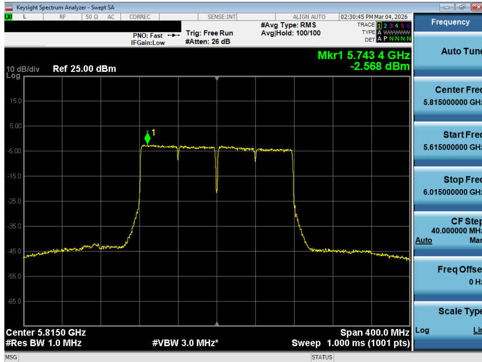
Plot 7-157. Power Spectral Density Plot MIMO ANT2 (160MHz BW 802.11ac (UNII Band 3/4) – Ch. 163)
