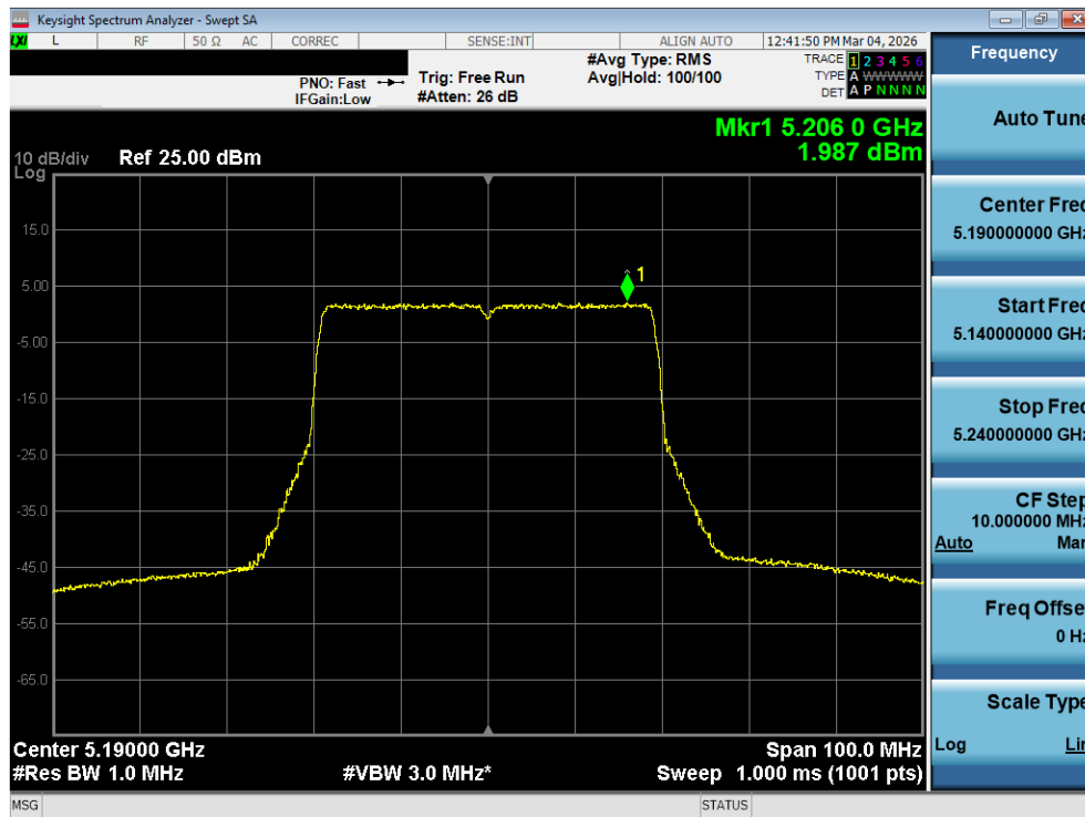
Plot 7-133. Power Spectral Density Plot MIMO ANT2 (40MHz BW 802.11be (UNII Band 1) – Ch. 38)
