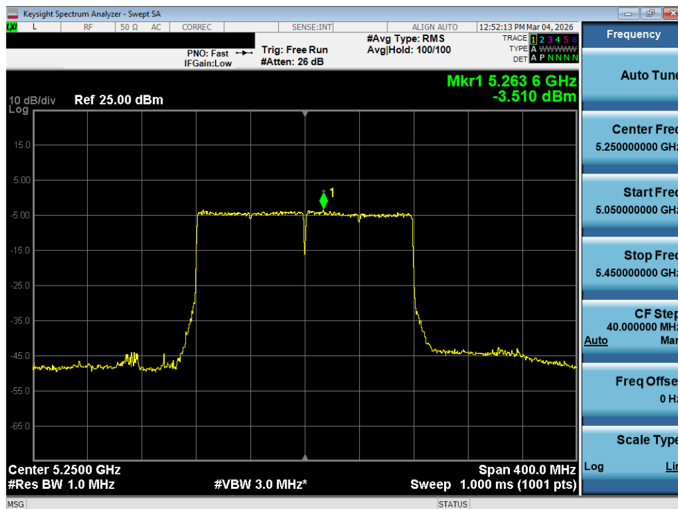
Plot 7-138. Power Spectral Density Plot MIMO ANT2 (160MHz BW 802.11be (UNII Band 1/2A) – Ch. 50)
