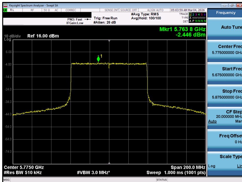
Plot 7-116. Power Spectral Density Plot MIMO ANT1 (80MHz BW 802.11be (UNII Band 3) – Ch. 155)
