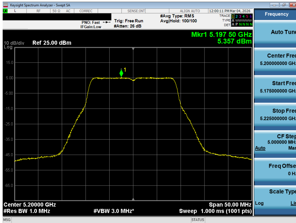
Plot 7-130. Power Spectral Density Plot MIMO ANT2 (20MHz BW 802.11n (UNII Band 1) – Ch. 40)
