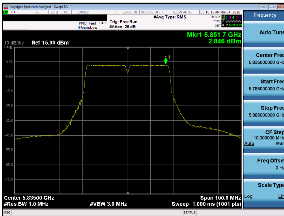
Plot 7-121. Power Spectral Density Plot MIMO ANT1 (40MHz BW 802.11n (UNII Band 3/4) – Ch. 167)
