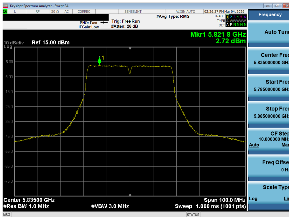
Plot 7-151. Power Spectral Density Plot MIMO ANT2 (40MHz BW 802.11n (UNII Band 3/4) – Ch. 167)
