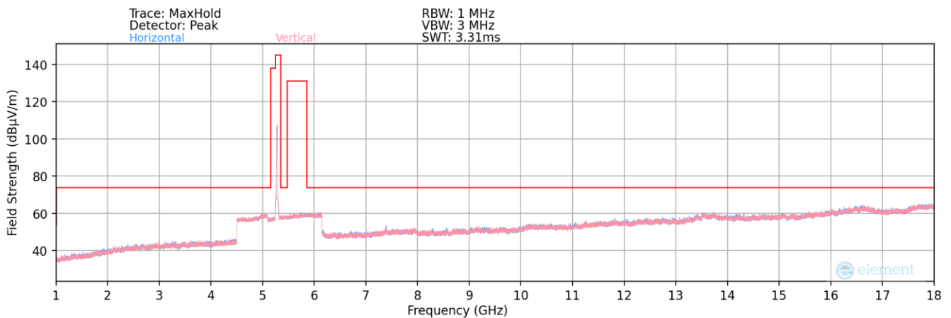
Plot 7-161. Radiated Spurious Plot above 1GHz MIMO (802.11a – UNII Band 2A Ch. 56)
