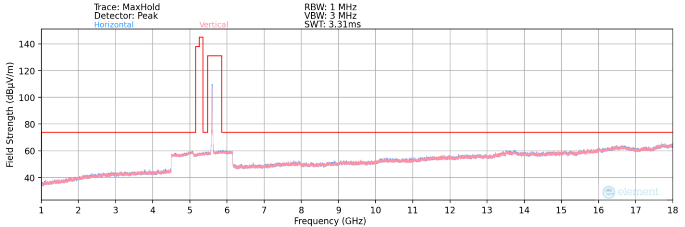
Plot 7-162. Radiated Spurious Plot above 1GHz MIMO (802.11a – UNII Band 2C Ch. 120)
