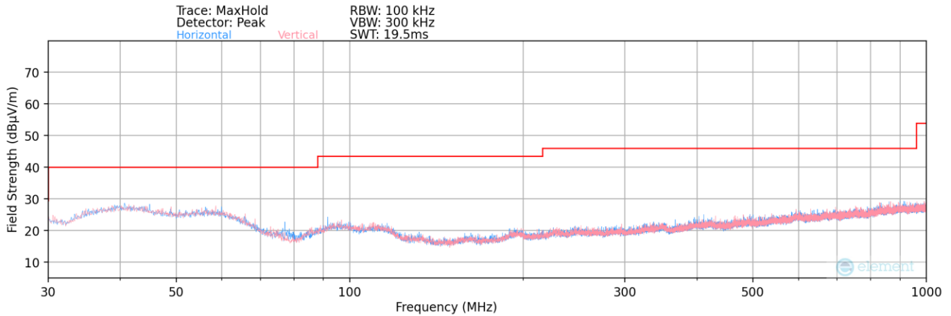
Plot 7-159. Radiated Spurious Plot below 1GHz MIMO (802.11a)
