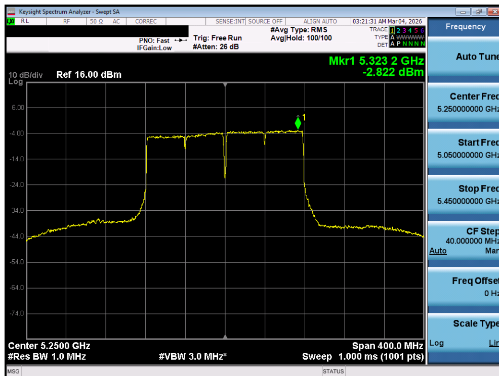
Plot 7-107. Power Spectral Density Plot MIMO ANT1 (160MHz BW 802.11ac (UNII Band 1/2A) – Ch. 50)
