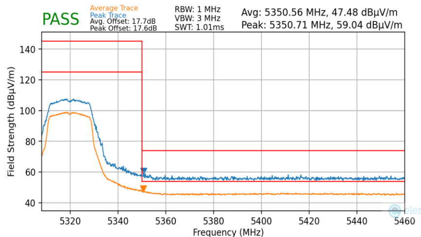
Plot 7-173. Radiated Upper Band Edge Plot MIMO (Average & Peak – UNII Band 2A)
