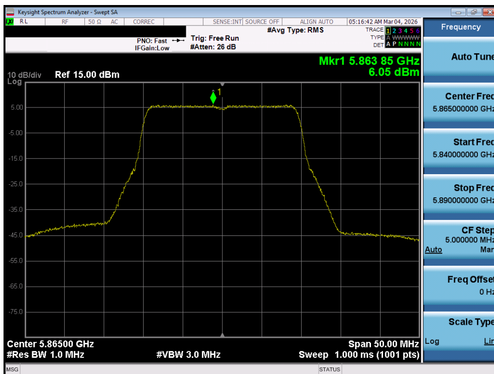
Plot 7-120. Power Spectral Density Plot MIMO ANT1 (20MHz BW 802.11be (UNII Band 4) – Ch. 173)
