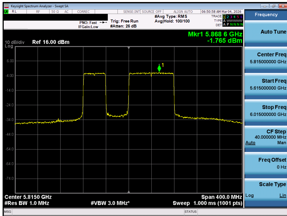
Plot 7-128. Power Spectral Density Plot MIMO ANT1 (160MHz BW 802.11be (40MHz Punct.) (UNII Band 3/4) – Ch. 163)
