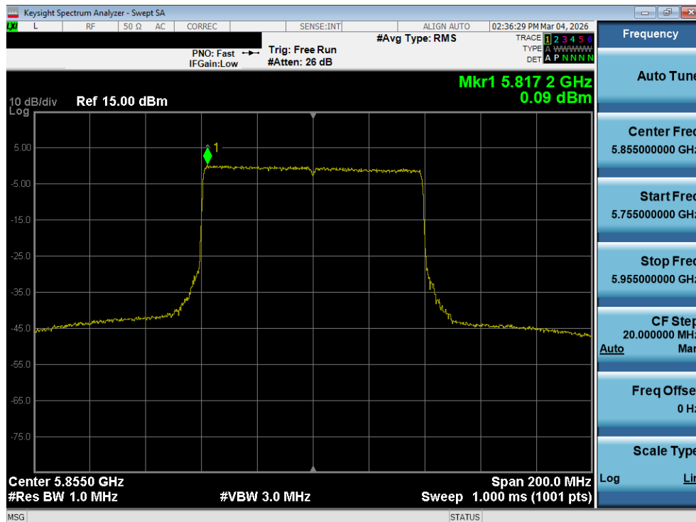
Plot 7-154. Power Spectral Density Plot MIMO ANT2 (80MHz BW 802.11be (UNII Band 3/4) – Ch. 171)
