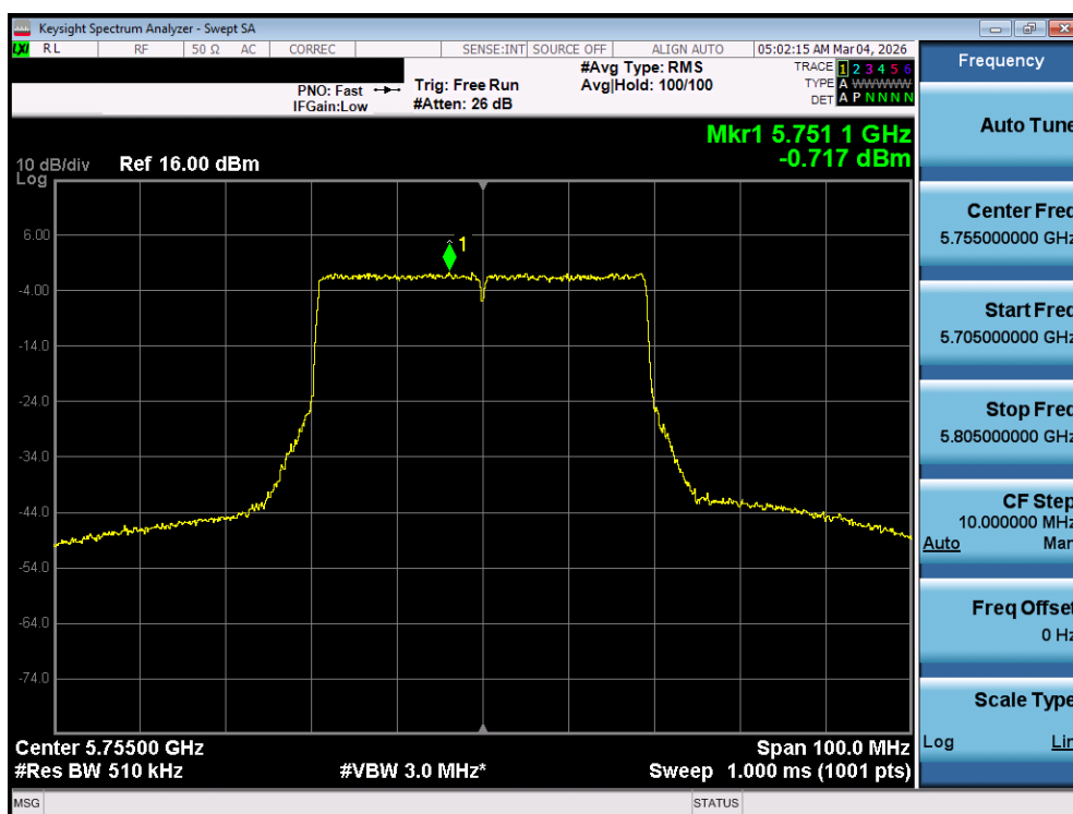
Plot 7-114. Power Spectral Density Plot MIMO ANT1 (40MHz BW 802.11be (UNII Band 3) – Ch. 151)
