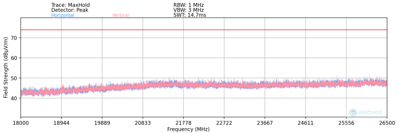
Plot 7-166. Radiated Spurious Plot 18GHz – 26.5GHz MIMO (802.11a)
