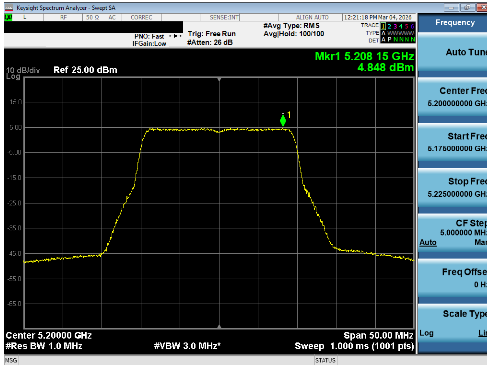
Plot 7-131. Power Spectral Density Plot MIMO ANT2 (20MHz BW 802.11be (UNII Band 1) – Ch. 40)
