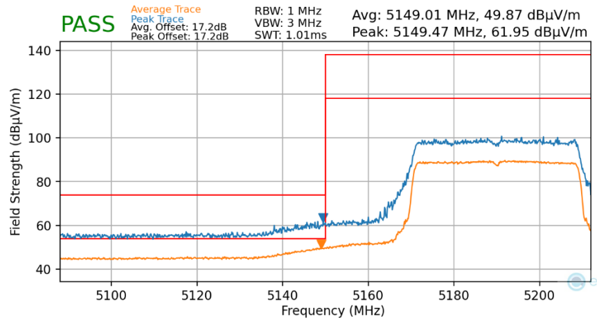
Plot 7-184. Radiated Band Edge Plot MIMO with WCP (Average & Peak – UNII Band 1)
