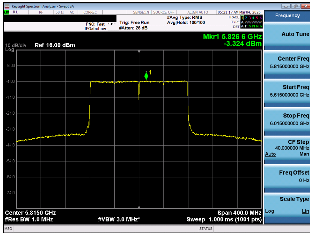
Plot 7-127. Power Spectral Density Plot MIMO ANT1 (160MHz BW 802.11be (UNII Band 3/4) – Ch. 163)
