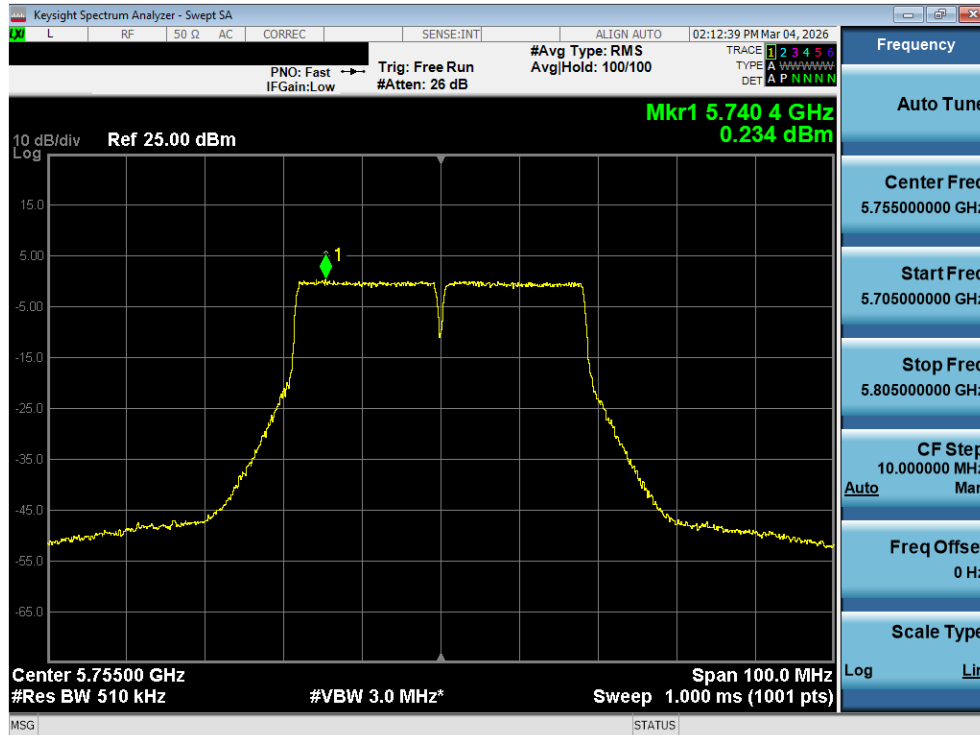
Plot 7-143. Power Spectral Density Plot MIMO ANT2 (40MHz BW 802.11n (UNII Band 3) – Ch. 151)
