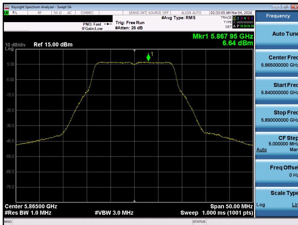
Plot 7-118. Power Spectral Density Plot MIMO ANT1 (802.11a (UNII Band 4) – Ch. 173)
