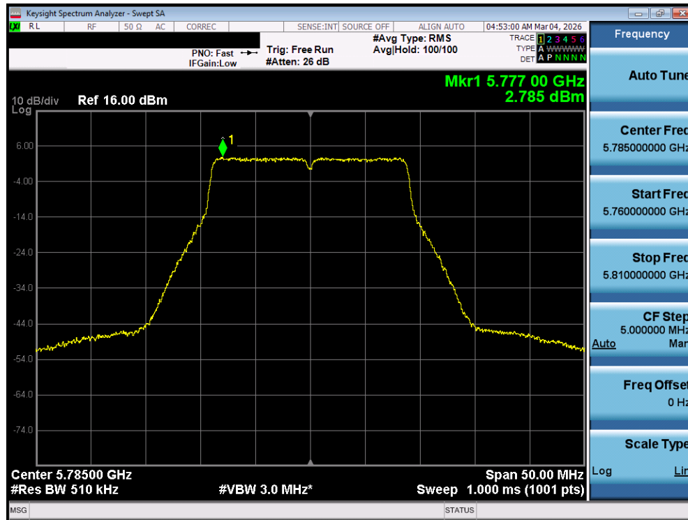
Plot 7-111. Power Spectral Density Plot MIMO ANT1 (20MHz BW 802.11n (UNII Band 3) – Ch. 157)
