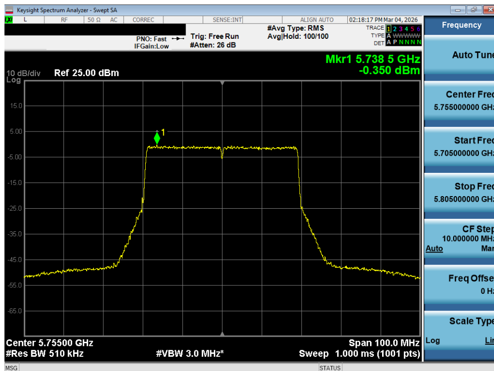
Plot 7-144. Power Spectral Density Plot MIMO ANT2 (40MHz BW 802.11be (UNII Band 3) – Ch. 151)
