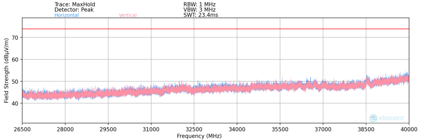
Plot 7-171. Radiated Spurious Plot below 26.5-40GHz MIMO 802.11b (2.4GHz – Ch.6) + MIMO 802.11a (5GHz – Ch. 44)
