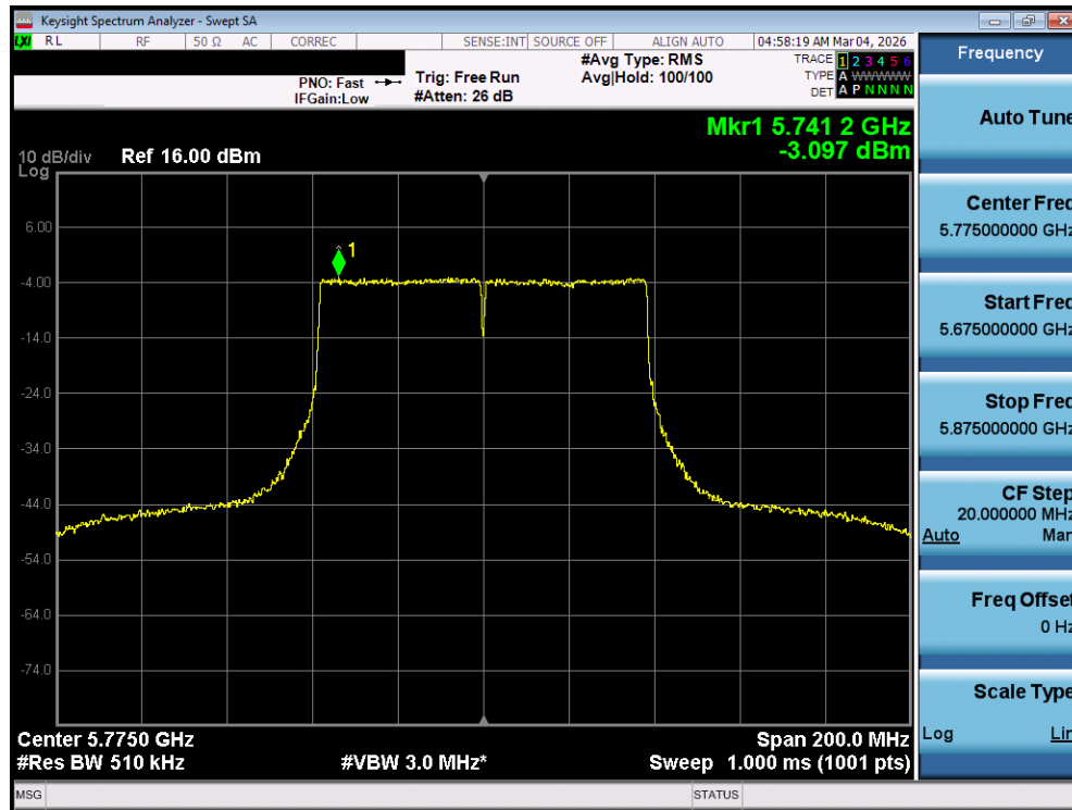
Plot 7-115. Power Spectral Density Plot MIMO ANT1 (80MHz BW 802.11ac (UNII Band 3) – Ch. 155)
