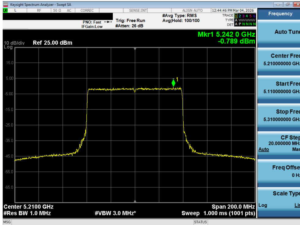
Plot 7-135. Power Spectral Density Plot MIMO ANT2 (80MHz BW 802.11be (UNII Band 1) – Ch. 42)
