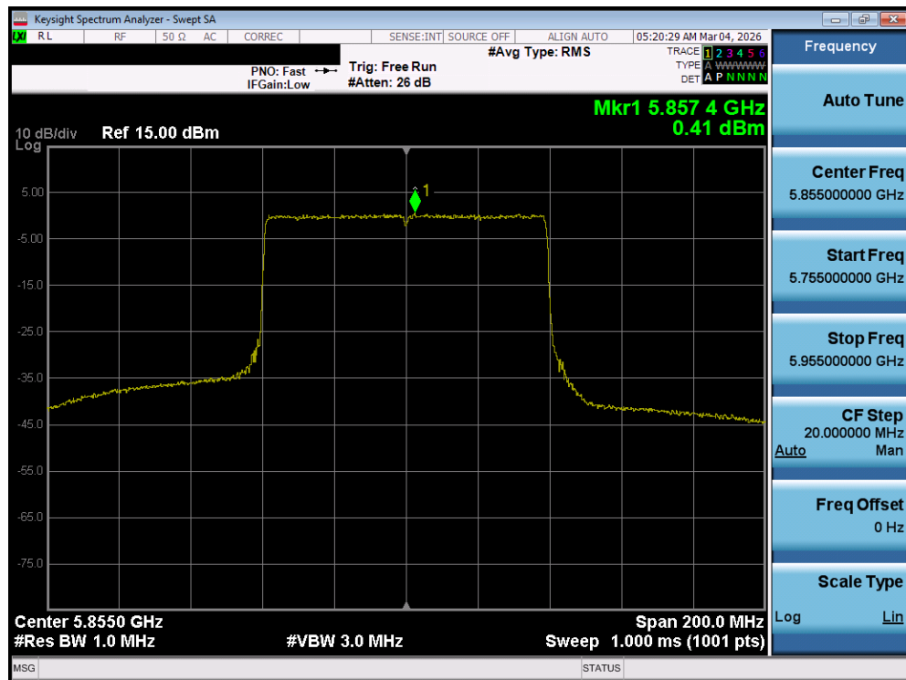
Plot 7-124. Power Spectral Density Plot MIMO ANT1 (80MHz BW 802.11be (UNII Band 3/4) – Ch. 171)
