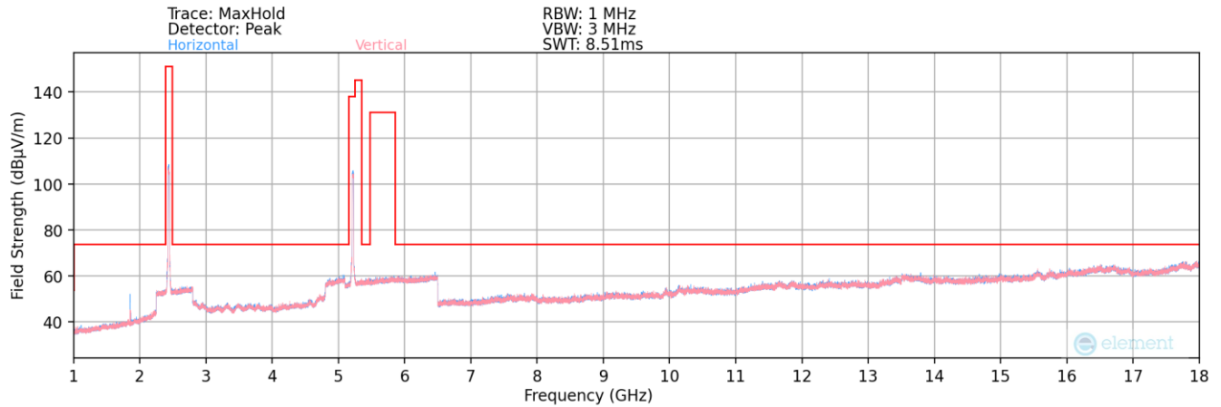
Plot 7-169. Radiated Spurious Plot below 1-18GHz MIMO 802.11b (2.4GHz – Ch.6) + MIMO 802.11a (5GHz – Ch. 44)
