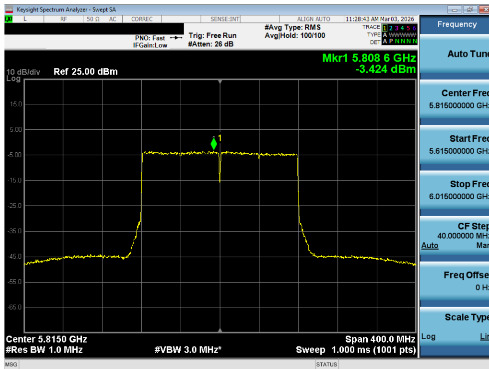
Plot 7-156. Power Spectral Density Plot MIMO ANT2 (160MHz BW 802.11be (UNII Band 3/4) – Ch. 163)
