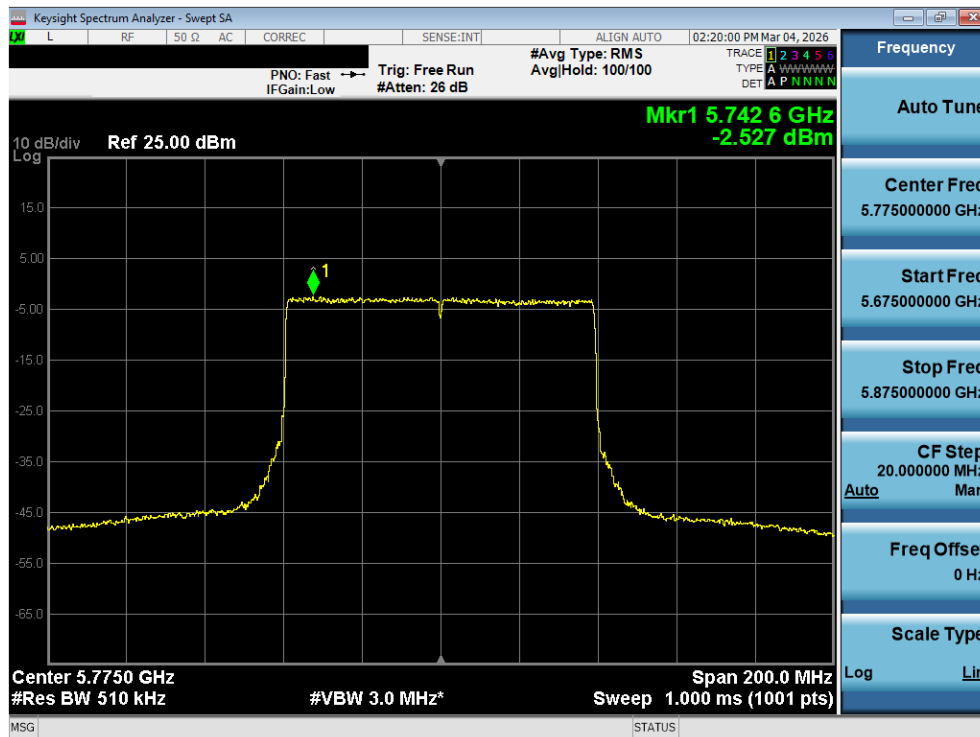
Plot 7-146. Power Spectral Density Plot MIMO ANT2 (80MHz BW 802.11be (UNII Band 3) – Ch. 155)
