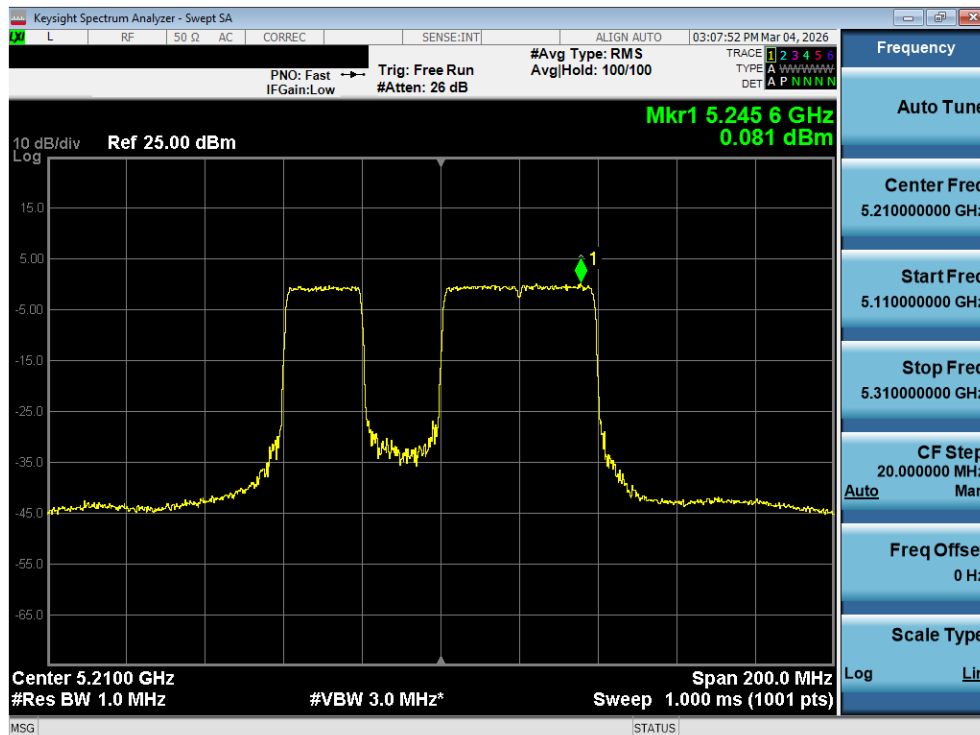
Plot 7-136. Power Spectral Density Plot MIMO ANT2 (80MHz BW 802.11be (20MHz Punct.) (UNII Band 1) – Ch. 42)
