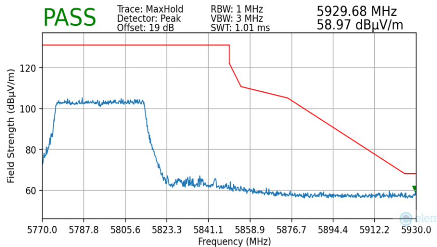
Plot 7-181. Radiated Upper Band Edge Plot MIMO (Peak – UNII Band 3)
