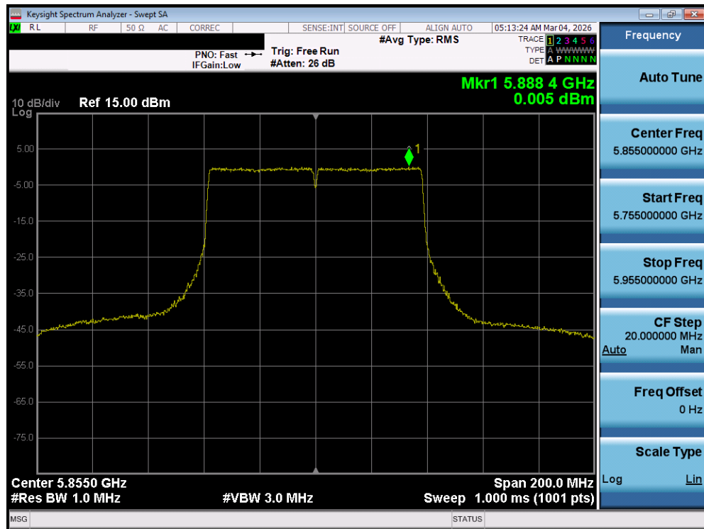
Plot 7-123. Power Spectral Density Plot MIMO ANT1 (80MHz BW 802.11ac (UNII Band 3/4) – Ch. 171)
