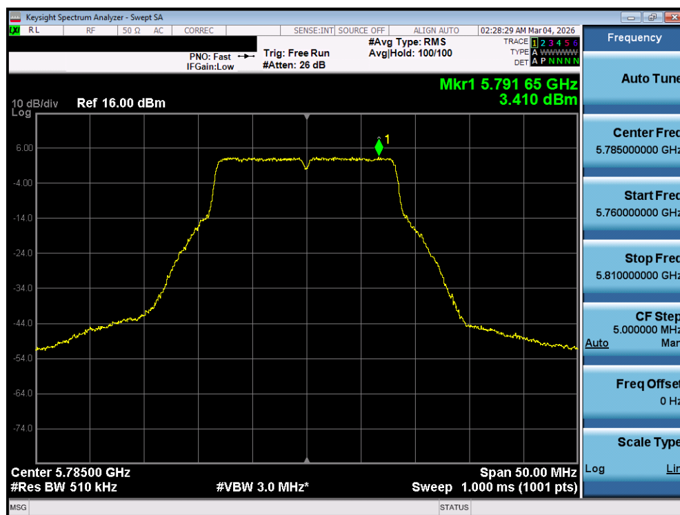
Plot 7-110. Power Spectral Density Plot MIMO ANT1 (802.11a (UNII Band 3) – Ch. 157)
