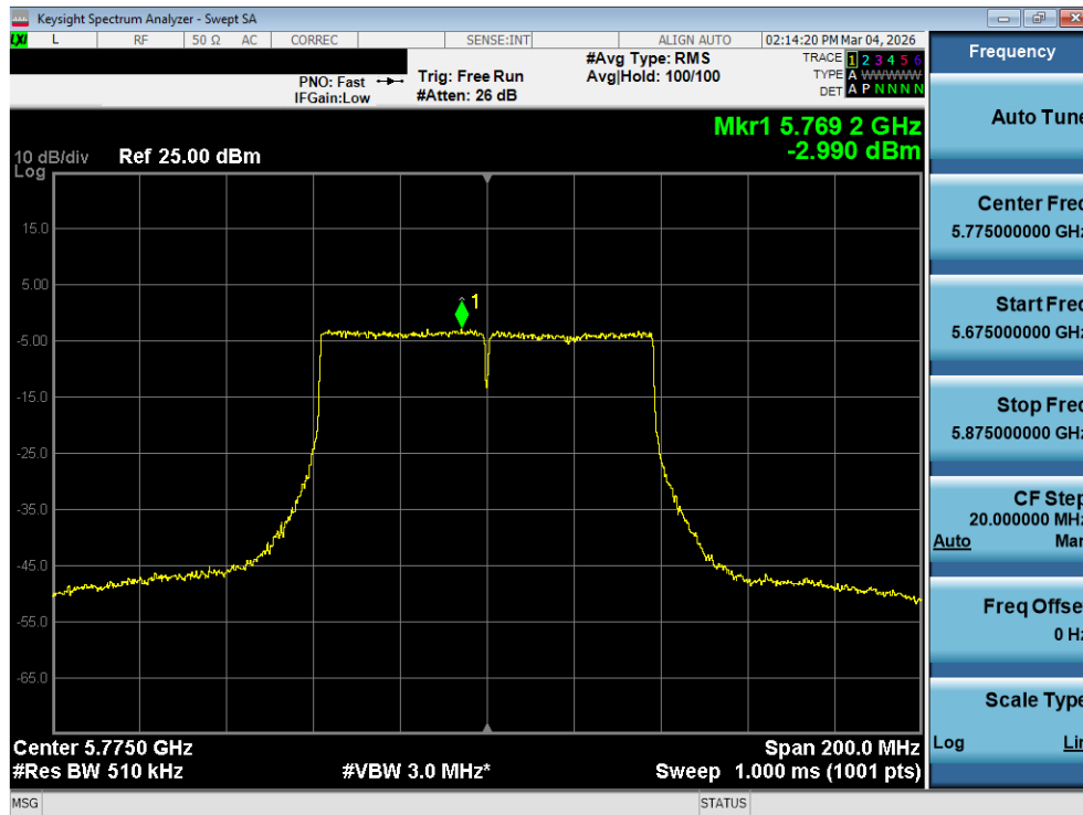
Plot 7-145. Power Spectral Density Plot MIMO ANT2 (80MHz BW 802.11ac (UNII Band 3) – Ch. 155)
