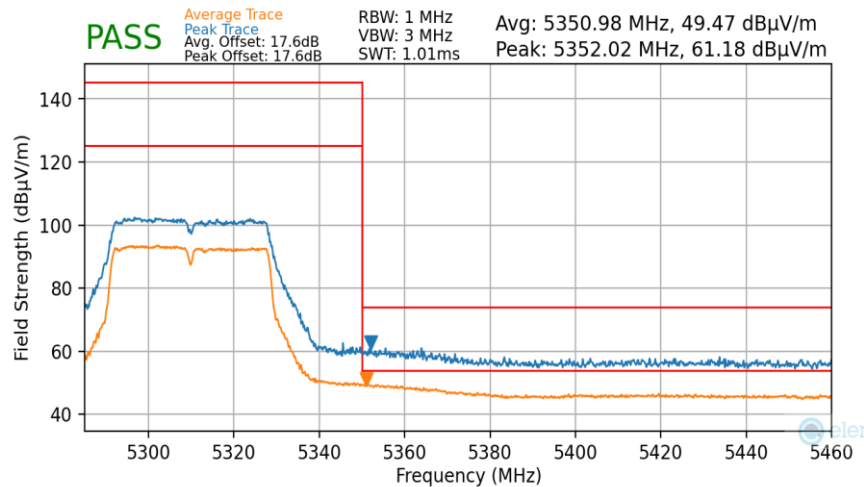
Plot 7-179. Radiated Upper Band Edge Plot MIMO (Average & Peak – UNII Band 2A)
