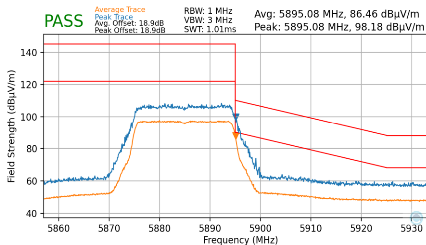
Plot 7-177. Radiated Upper Band Edge Plot MIMO (Average & Peak – UNII Band 4)
