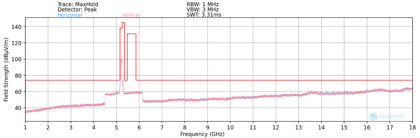
Plot 7-165. Radiated Spurious Plot above 1GHz MIMO (802.11be – UNII Band 1 Ch. 42 – Punctured)
