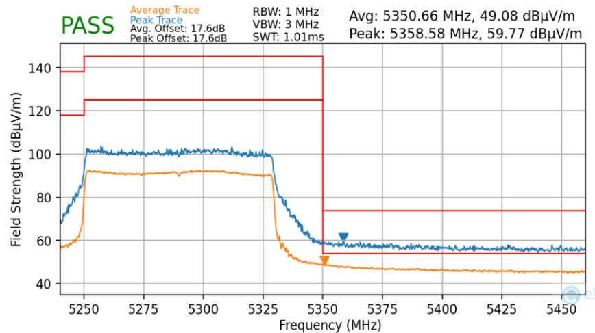
Plot 7-186. Radiated Upper Band Edge Plot MIMO (Average & Peak – UNII Band 2A)
