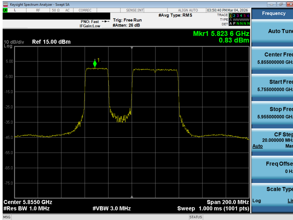
Plot 7-155. Power Spectral Density Plot MIMO ANT2 (80MHz BW 802.11be (20MHz Punct.) (UNII Band 3/4) – Ch. 171)
