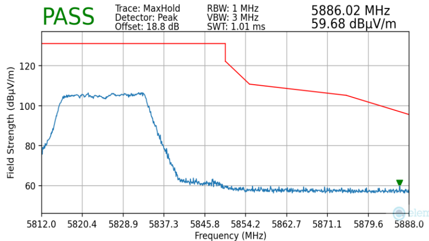
Plot 7-175. Radiated Upper Band Edge Plot MIMO (Peak – UNII Band 3)
