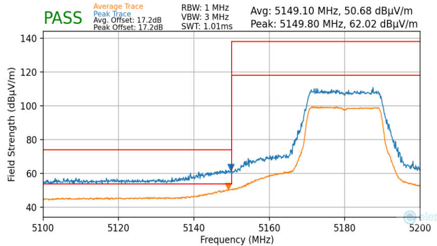
Plot 7-172. Radiated Lower Band Edge Plot MIMO (Average & Peak – UNII Band 1)
