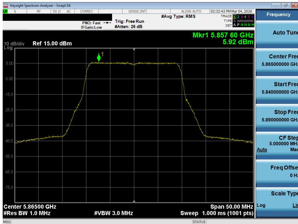
Plot 7-150. Power Spectral Density Plot MIMO ANT2 (20MHz BW 802.11be (UNII Band 4) – Ch. 173)
