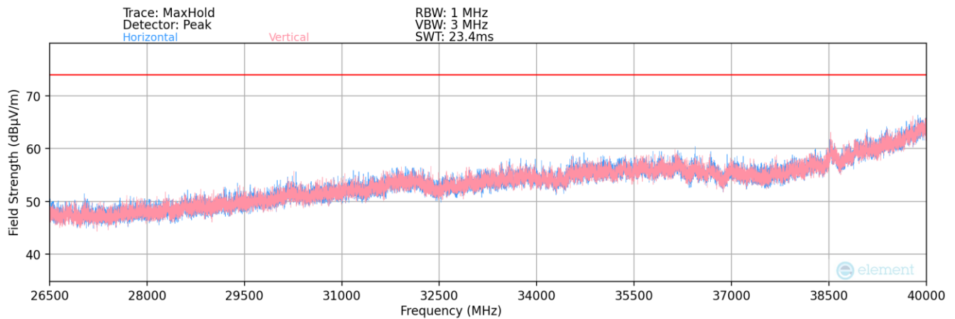
Plot 7-167. Radiated Spurious Plot 26.5GHz – 40GHz MIMO (802.11a)
