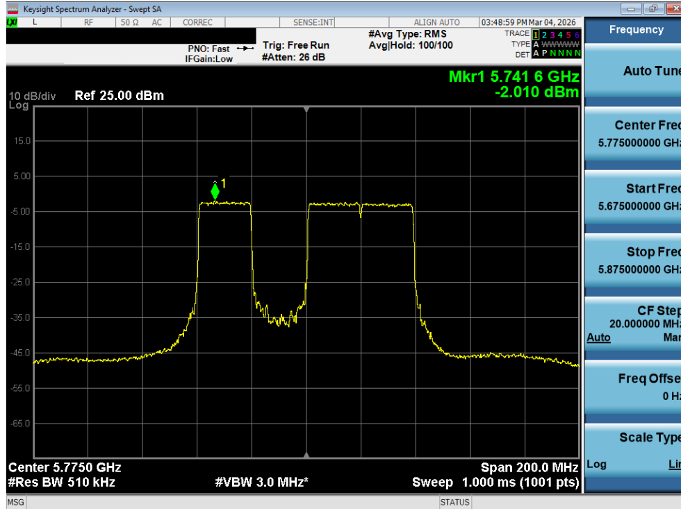
Plot 7-147. Power Spectral Density Plot MIMO ANT2 (80MHz BW 802.11be (20MHz Punct.) (UNII Band 3) – Ch. 155)
