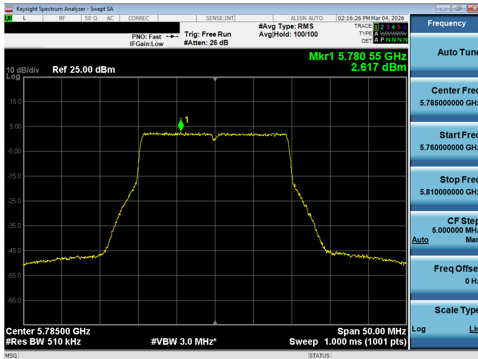
Plot 7-142. Power Spectral Density Plot MIMO ANT2 (20MHz BW 802.11be (UNII Band 3) – Ch. 157)
