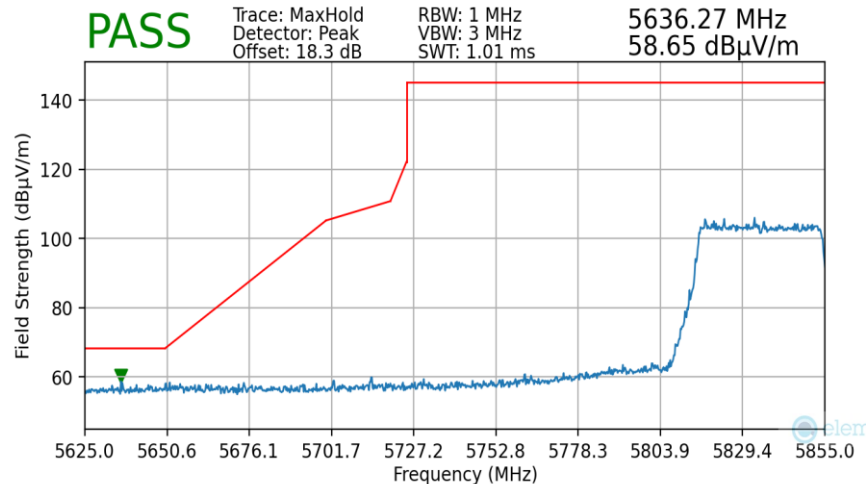
Plot 7-182. Radiated Lower Band Edge Plot MIMO (Peak – UNII Band 4)
