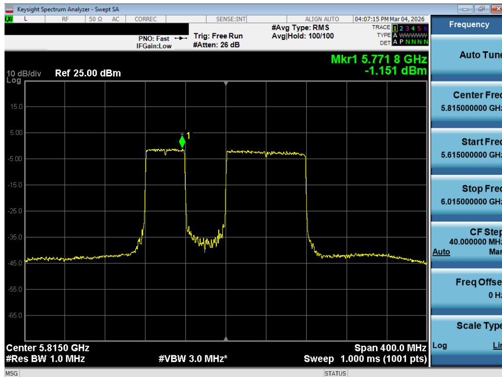
Plot 7-158. Power Spectral Density Plot MIMO ANT2 (160MHz BW 802.11be (40MHz Punct.) (UNII Band 3/4) – Ch. 163)
