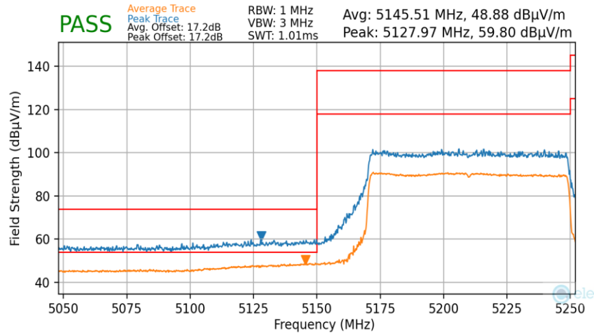
Plot 7-185. Radiated Lower Band Edge Plot MIMO (Average & Peak – UNII Band 1)
