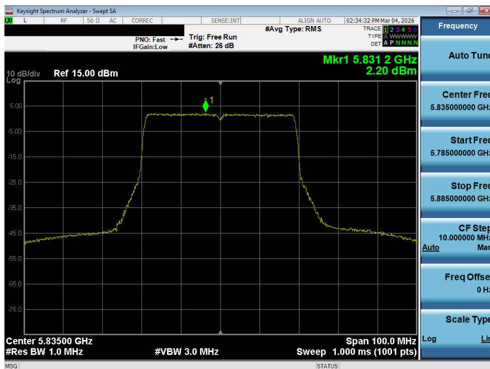
Plot 7-152. Power Spectral Density Plot MIMO ANT2 (40MHz BW 802.11be (UNII Band 3/4) – Ch. 167)
