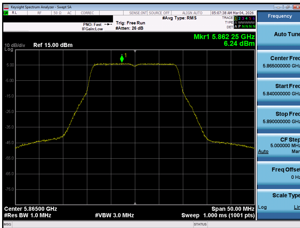
Plot 7-119. Power Spectral Density Plot MIMO ANT1 (20MHz BW 802.11n (UNII Band 4) – Ch. 173)
