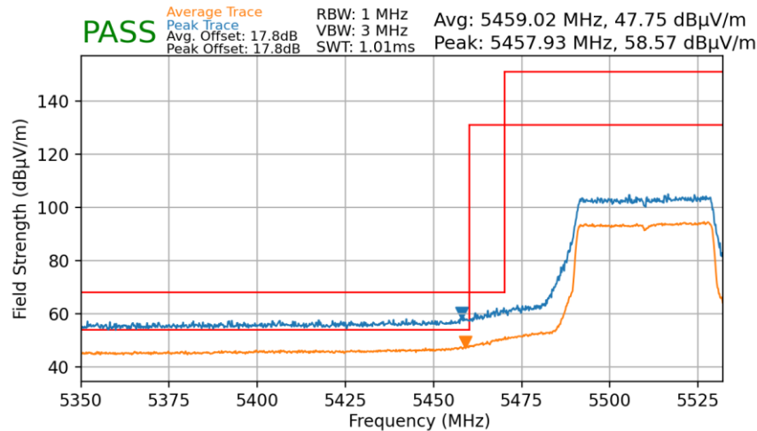
Plot 7-180. Radiated Lower Band Edge Plot MIMO (Average & Peak – UNII Band 2C)
