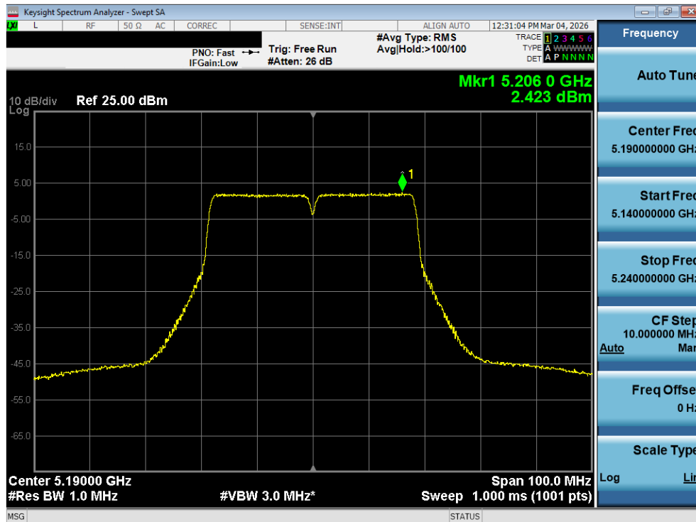
Plot 7-132. Power Spectral Density Plot MIMO ANT2 (40MHz BW 802.11n (UNII Band 1) – Ch. 38)
