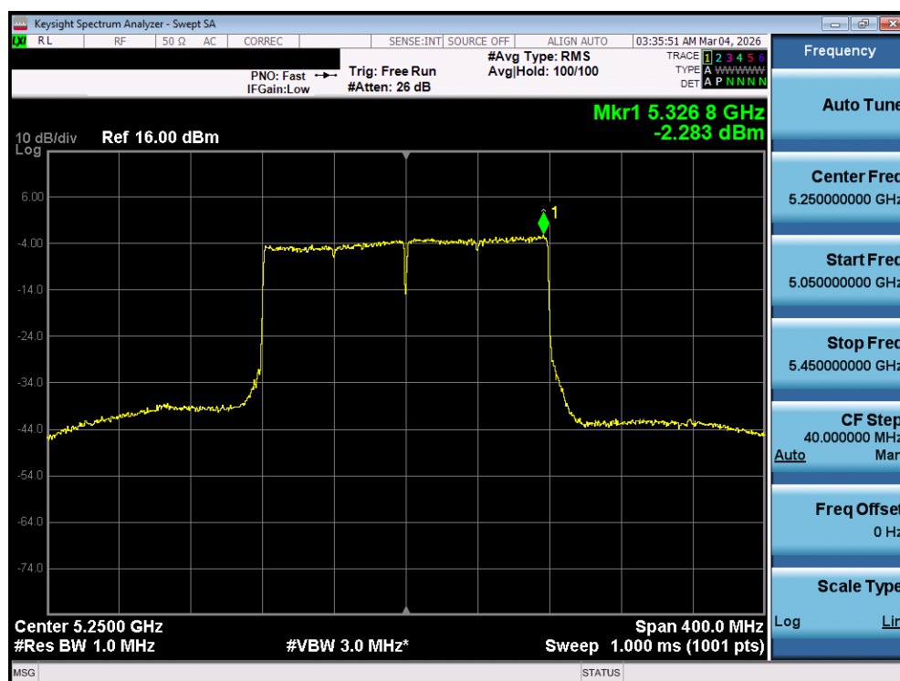
Plot 7-108. Power Spectral Density Plot MIMO ANT1 (160MHz BW 802.11be (UNII Band 1/2A) – Ch. 50)
