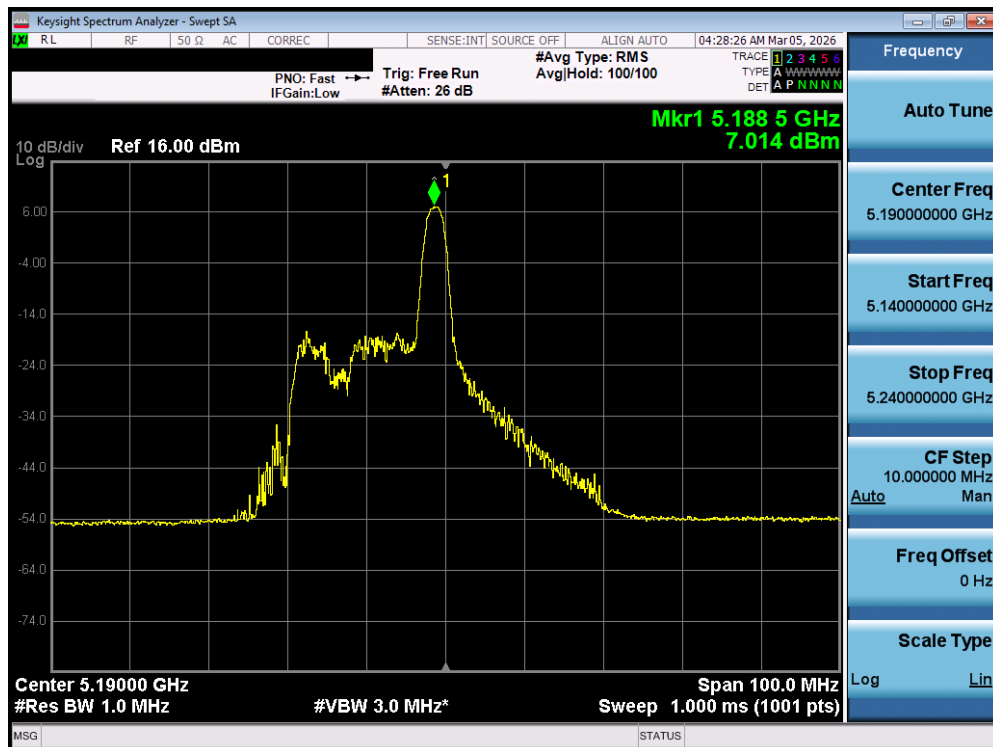
Plot 7-100. Power Spectral Density Plot MIMO ANT1 (40MHz BW 802.11be – 26 Tones (UNII Band 1) – Ch. 38)
