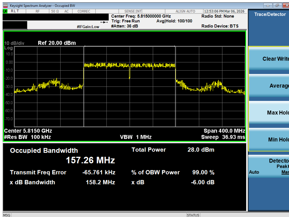
Plot 7-36. 6dB Bandwidth Plot MIMO ANT1 (160MHz BW 802.11be – 996*2 Tones (UNII Band 3/4) – Ch. 163)
