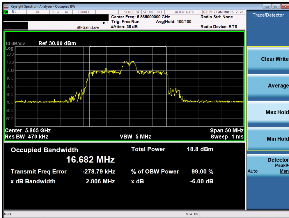
Plot 7-83. OBW Plot MIMO ANT2 (20MHz BW 802.11be – 26 Tones (UNII Band 4) – Ch. 173)
