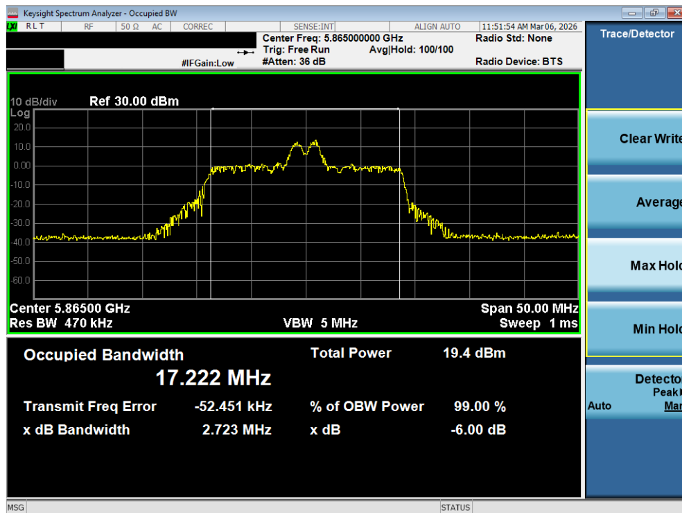
Plot 7-64. OBW Plot MIMO ANT1 (20MHz BW 802.11be – 26 Tones (UNII Band 4) – Ch. 173)
