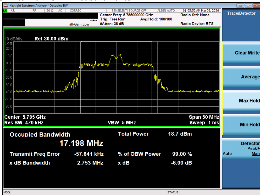
Plot 7-80. OBW Plot MIMO ANT2 (20MHz BW 802.11be – 26 Tones (UNII Band 3) – Ch. 157)
