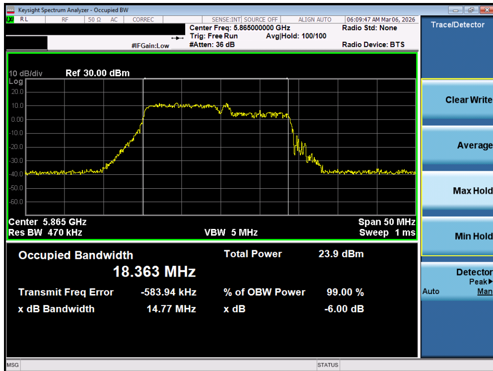
Plot 7-96. OBW Plot MIMO ANT2 (20MHz BW 802.11be – 106+26 Tones (UNII Band 4) – Ch. 173)
