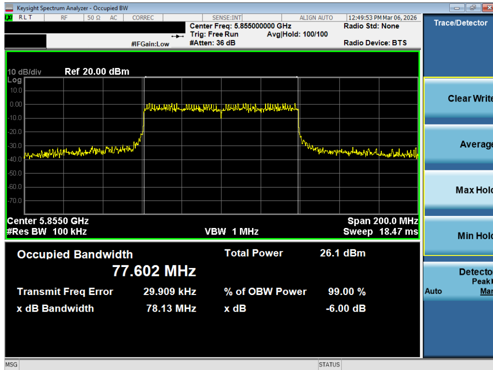
Plot 7-35. 6dB Bandwidth Plot MIMO ANT1 (80MHz BW 802.11be – 996 Tones (UNII Band 3/4) – Ch. 171)
