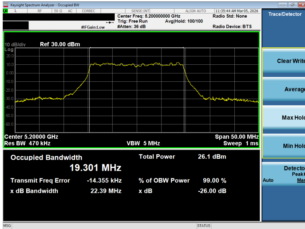
Plot 7-16. 26dB Bandwidth Plot MIMO ANT2 (20MHz BW 802.11be – 242 Tones (UNII Band 1) – Ch. 40)
