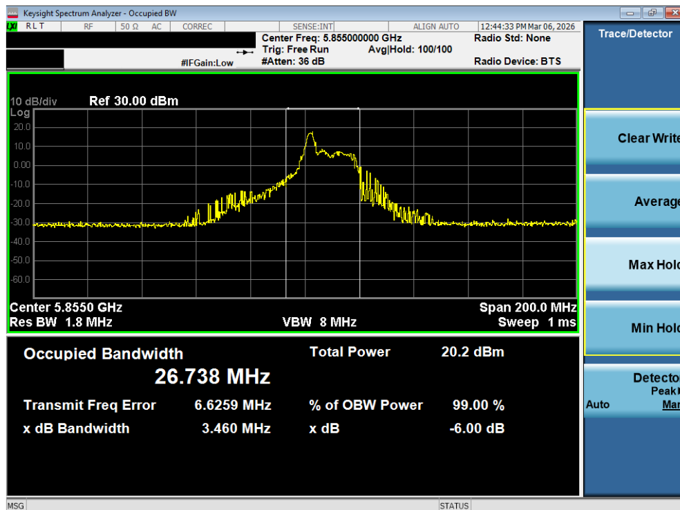
Plot 7-66. OBW Plot MIMO ANT1 (80MHz BW 802.11be – 26 Tones (UNII Band 3/4) – Ch. 171)
