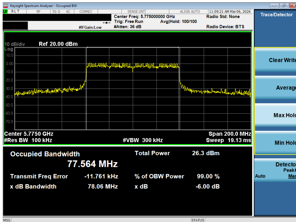
Plot 7-32. 6dB Bandwidth Plot MIMO ANT1 (80MHz BW 802.11be – 996 Tones (UNII Band 3) – Ch. 155)
