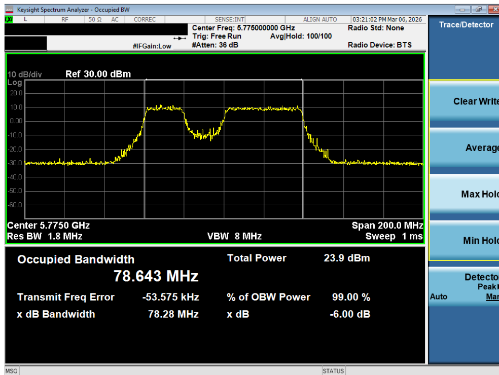
Plot 7-76. OBW Plot MIMO ANT1 (80MHz BW 802.11be – 484+242 Tones (UNII Band 3) – Ch. 155)
