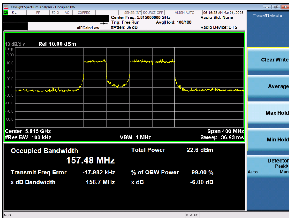
Plot 7-60. 6dB Bandwidth Plot MIMO ANT2 (160MHz BW 802.11be – 996+484 Tones (UNII Band 3/4) – Ch. 163)
