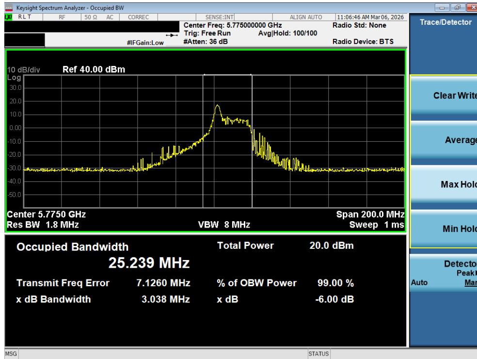
Plot 7-63. OBW Plot MIMO ANT1 (80MHz BW 802.11be – 26 Tones (UNII Band 3) – Ch. 155)
