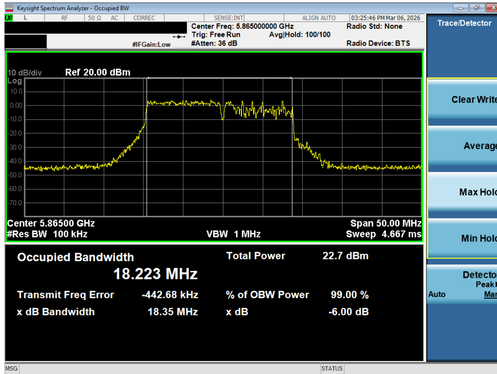
Plot 7-39. 6dB Bandwidth Plot MIMO ANT1 (20MHz BW 802.11be – 106+26 Tones (UNII Band 4) – Ch. 173)
