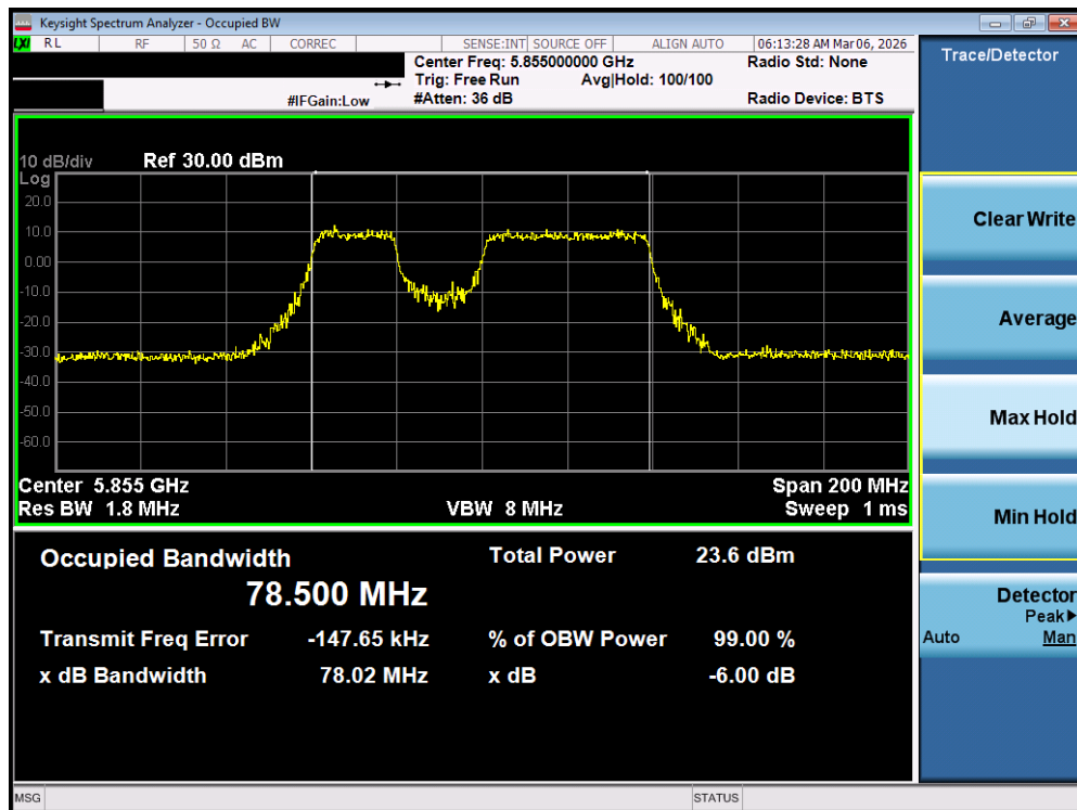
Plot 7-97. OBW Plot MIMO ANT2 (80MHz BW 802.11be – 484+242 Tones (UNII Band 3/4) – Ch. 171)
