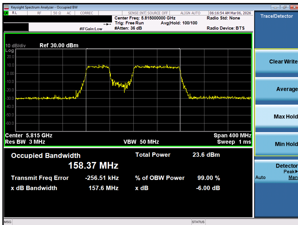
Plot 7-98. OBW Plot MIMO ANT2 (160MHz BW 802.11be – 996+484 Tones (UNII Band 3/4) – Ch. 163)
