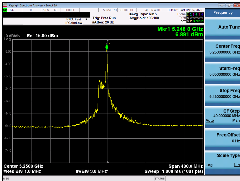
Plot 7-102. Power Spectral Density Plot MIMO ANT1 (160MHz BW 802.11be – 26 Tones (UNII Band 1/2A) – Ch. 50)
