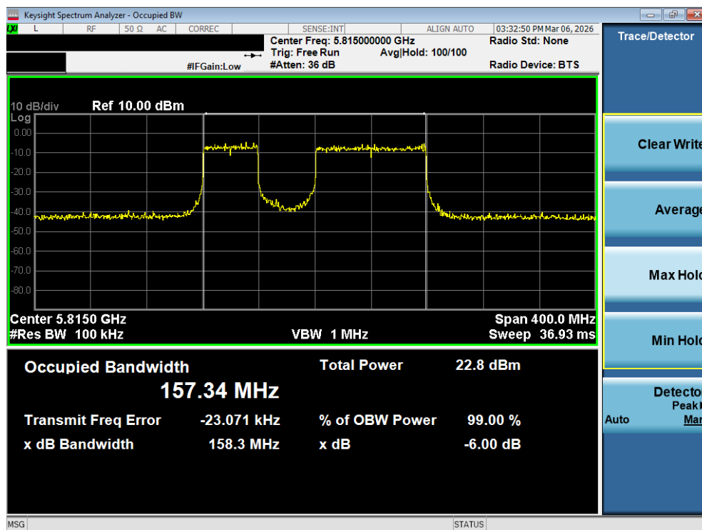
Plot 7-41. 6dB Bandwidth Plot MIMO ANT1 (160MHz BW 802.11be – 996+484 Tones (UNII Band 3/4) – Ch. 163)
