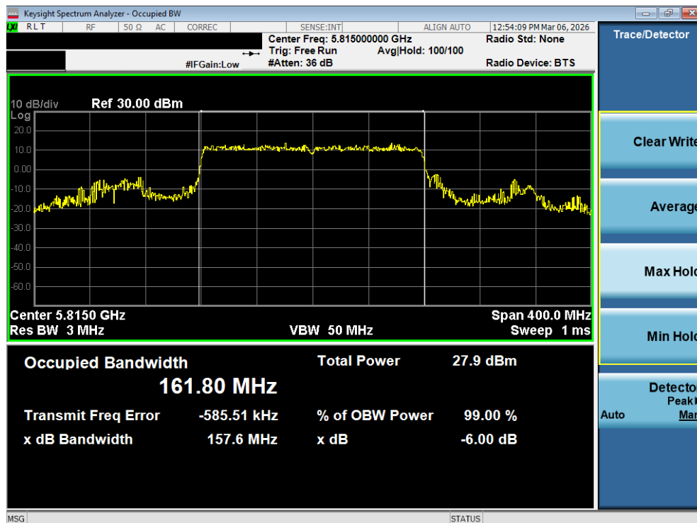
Plot 7-74. OBW Plot MIMO ANT1 (160MHz BW 802.11be – 996*2 Tones (UNII Band 3/4) – Ch. 163)
