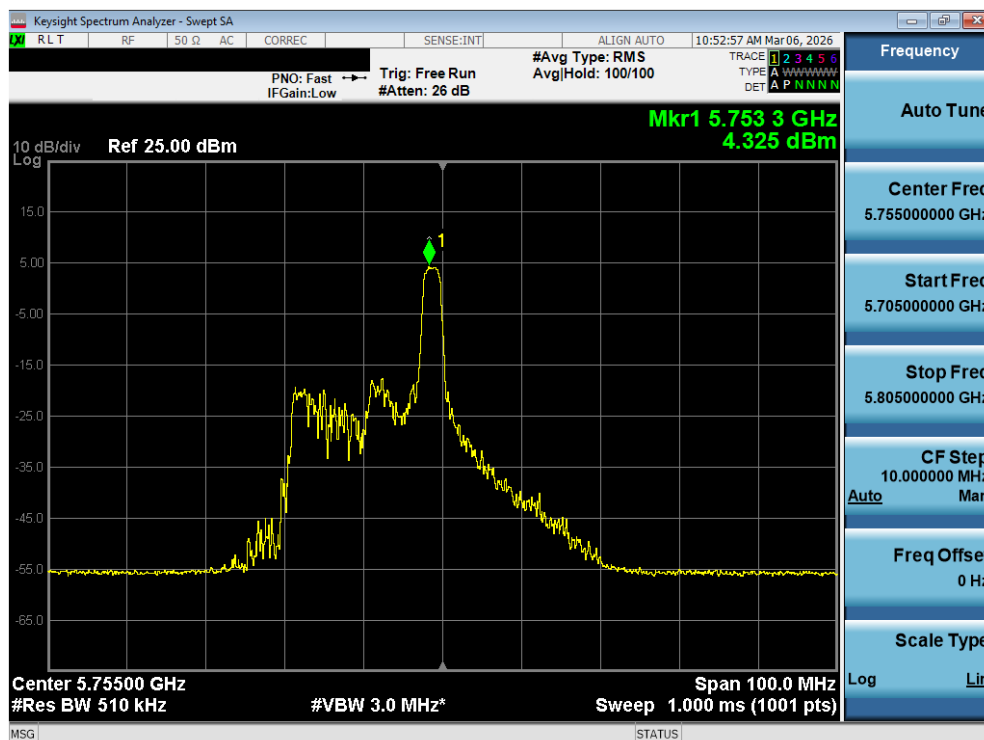
Plot 7-104. Power Spectral Density Plot MIMO ANT1 (40MHz BW 802.11be – 26 Tones (UNII Band 3) – Ch. 151)
