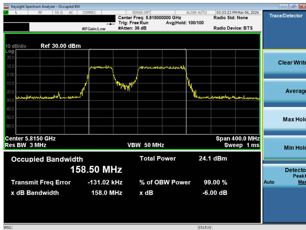
Plot 7-79. OBW Plot MIMO ANT1 (160MHz BW 802.11be – 996+484 Tones (UNII Band 3/4) – Ch. 163)
