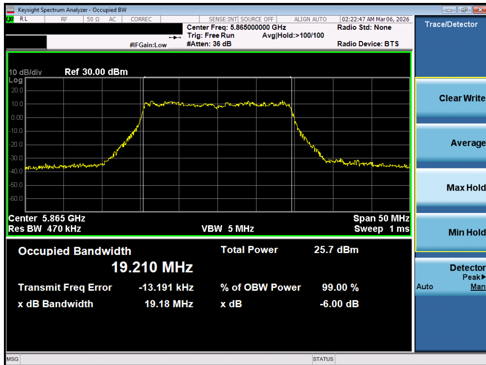
Plot 7-90. OBW Plot MIMO ANT2 (20MHz BW 802.11be – 242 Tones (UNII Band 4) – Ch. 173)
