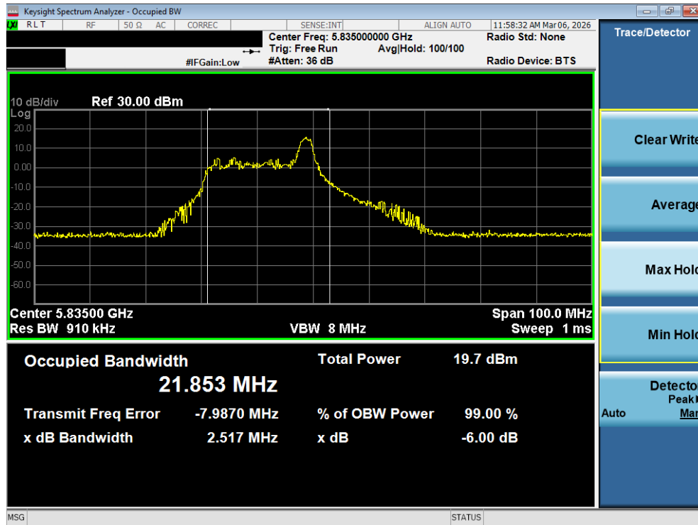
Plot 7-65. OBW Plot MIMO ANT1 (40MHz BW 802.11be – 26 Tones (UNII Band 3/4) – Ch. 167)
