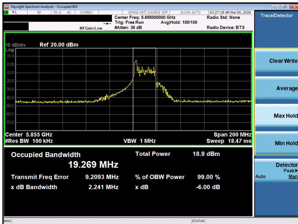
Plot 7-47. 6dB Bandwidth Plot MIMO ANT2 (80MHz BW 802.11be – 26 Tones (UNII Band 3/4) – Ch. 171)
