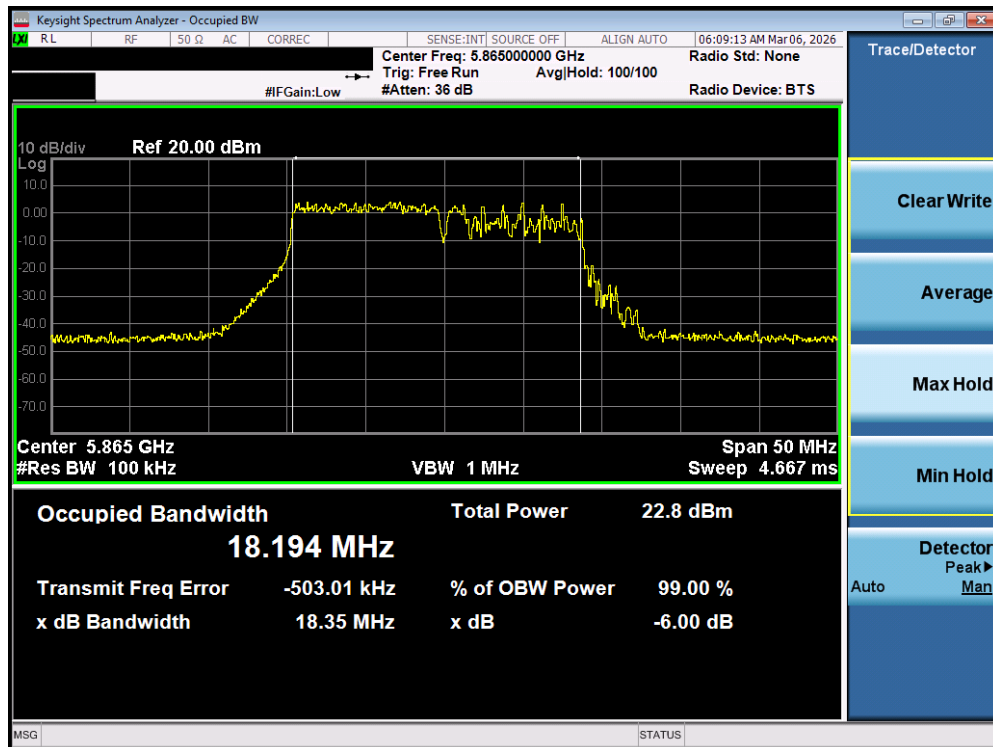
Plot 7-58. 6dB Bandwidth Plot MIMO ANT2 (20MHz BW 802.11be – 106+26 Tones (UNII Band 4) – Ch. 173)
