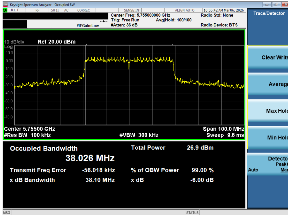
Plot 7-31. 6dB Bandwidth Plot MIMO ANT1 (40MHz BW 802.11be – 484 Tones (UNII Band 3) – Ch. 151)
