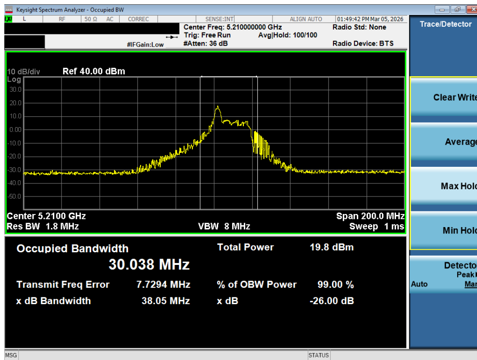
Plot 7-14. 26dB Bandwidth Plot MIMO ANT2 (80MHz BW 802.11be – 26 Tones (UNII Band 1) – Ch. 42)
