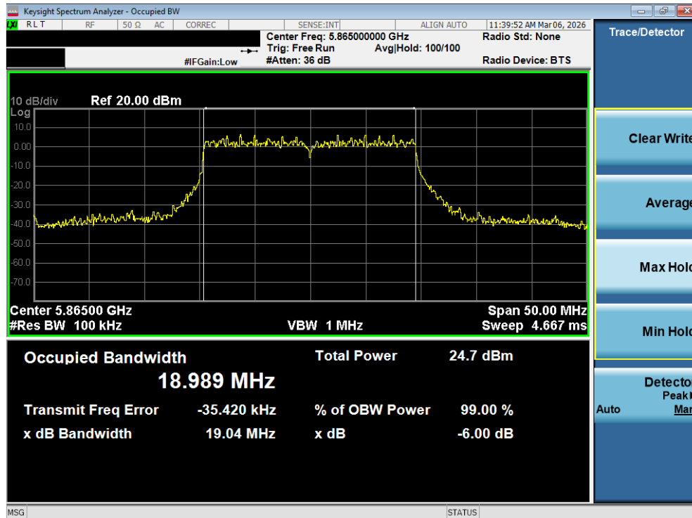
Plot 7-33. 6dB Bandwidth Plot MIMO ANT1 (20MHz BW 802.11be – 242 Tones (UNII Band 4) – Ch. 173)
