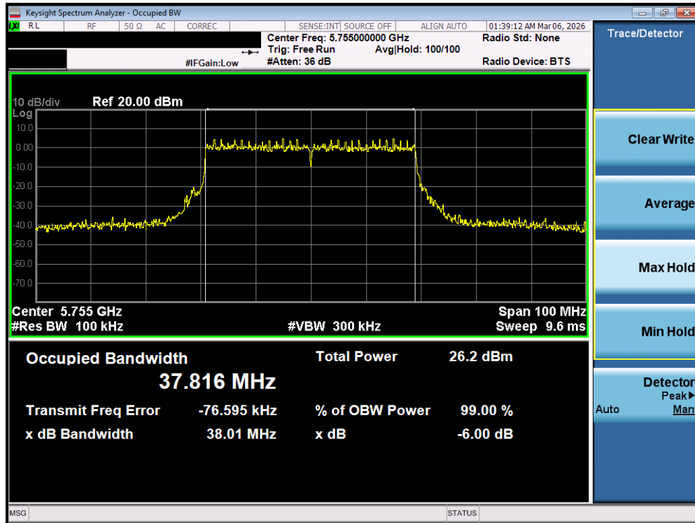
Plot 7-50. 6dB Bandwidth Plot MIMO ANT2 (40MHz BW 802.11be – 484 Tones (UNII Band 3) – Ch. 151)
