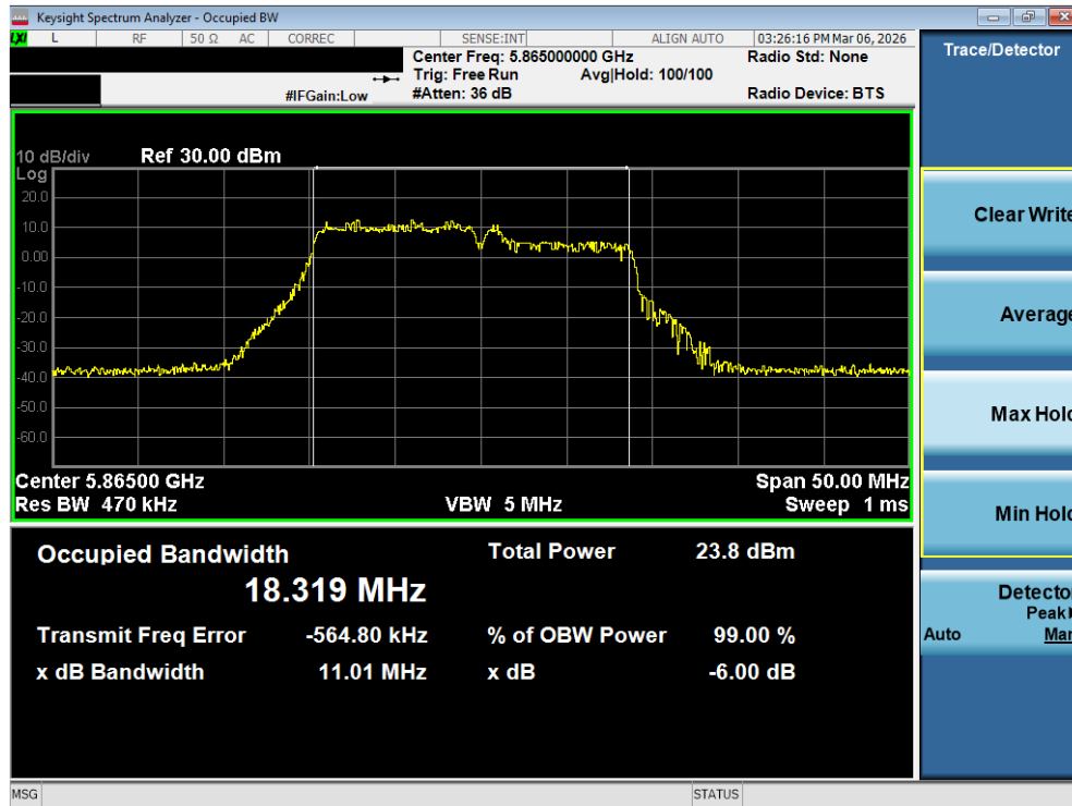
Plot 7-77. OBW Plot MIMO ANT1 (20MHz BW 802.11be – 106+26 Tones (UNII Band 4) – Ch. 173)
