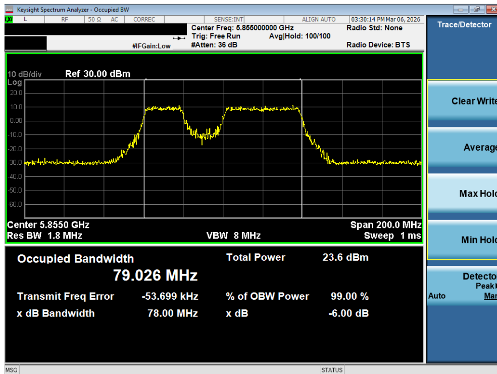
Plot 7-78. OBW Plot MIMO ANT1 (80MHz BW 802.11be – 484+242 Tones (UNII Band 3/4) – Ch. 171)
