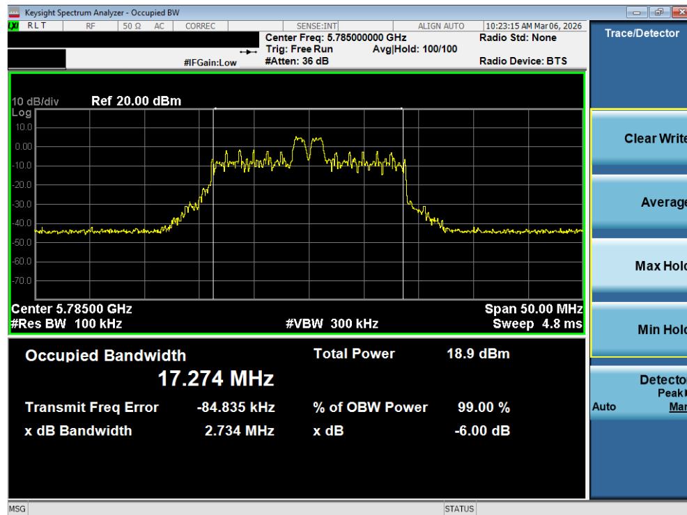
Plot 7-23. 6dB Bandwidth Plot MIMO ANT1 (20MHz BW 802.11be – 26 Tones (UNII Band 3) – Ch. 157)
