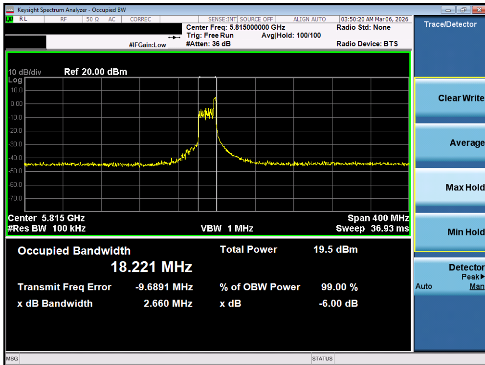
Plot 7-48. 6dB Bandwidth Plot MIMO ANT2 (160MHz BW 802.11be – 26 Tones (UNII Band 3/4) – Ch. 163)
