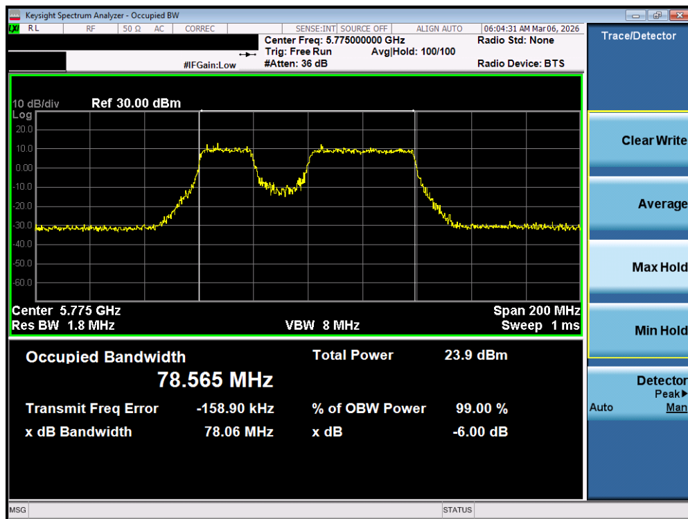
Plot 7-95. OBW Plot MIMO ANT2 (80MHz BW 802.11be – 484+242 Tones (UNII Band 3) – Ch. 155)
