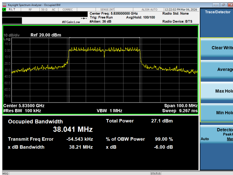
Plot 7-34. 6dB Bandwidth Plot MIMO ANT1 (40MHz BW 802.11be – 484 Tones (UNII Band 3/4) – Ch. 167)
