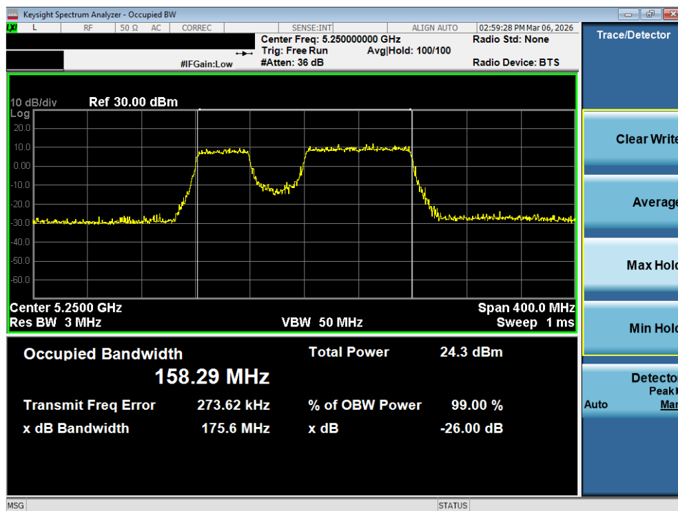
Plot 7-11. 26dB Bandwidth Plot MIMO ANT1 (160MHz BW 802.11be – 996+484 Tones (UNII Band 1/2A) – Ch. 50)
