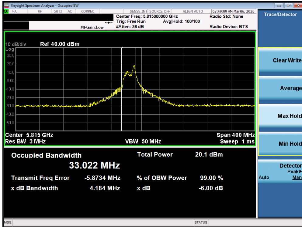
Plot 7-86. OBW Plot MIMO ANT2 (160MHz BW 802.11be – 26 Tones (UNII Band 3/4) – Ch. 163)
