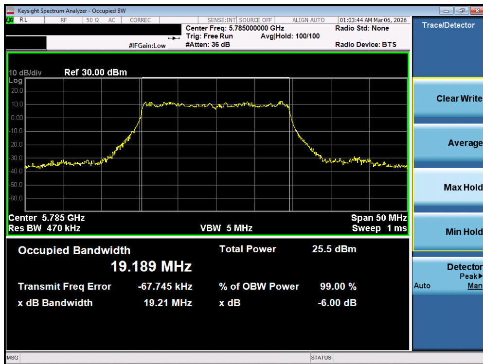
Plot 7-87. OBW Plot MIMO ANT2 (20MHz BW 802.11be – 242 Tones (UNII Band 3) – Ch. 157)
