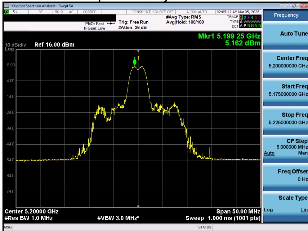
Plot 7-99. Power Spectral Density Plot MIMO ANT1 (20MHz BW 802.11be – 26 Tones (UNII Band 1) – Ch. 40)
