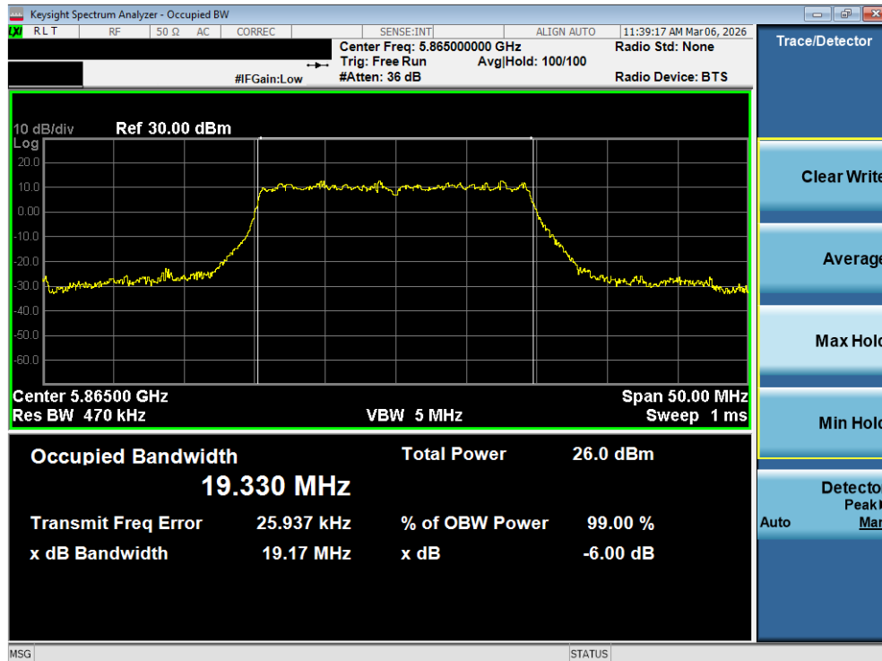
Plot 7-71. OBW Plot MIMO ANT1 (20MHz BW 802.11be – 242 Tones (UNII Band 4) – Ch. 173)
