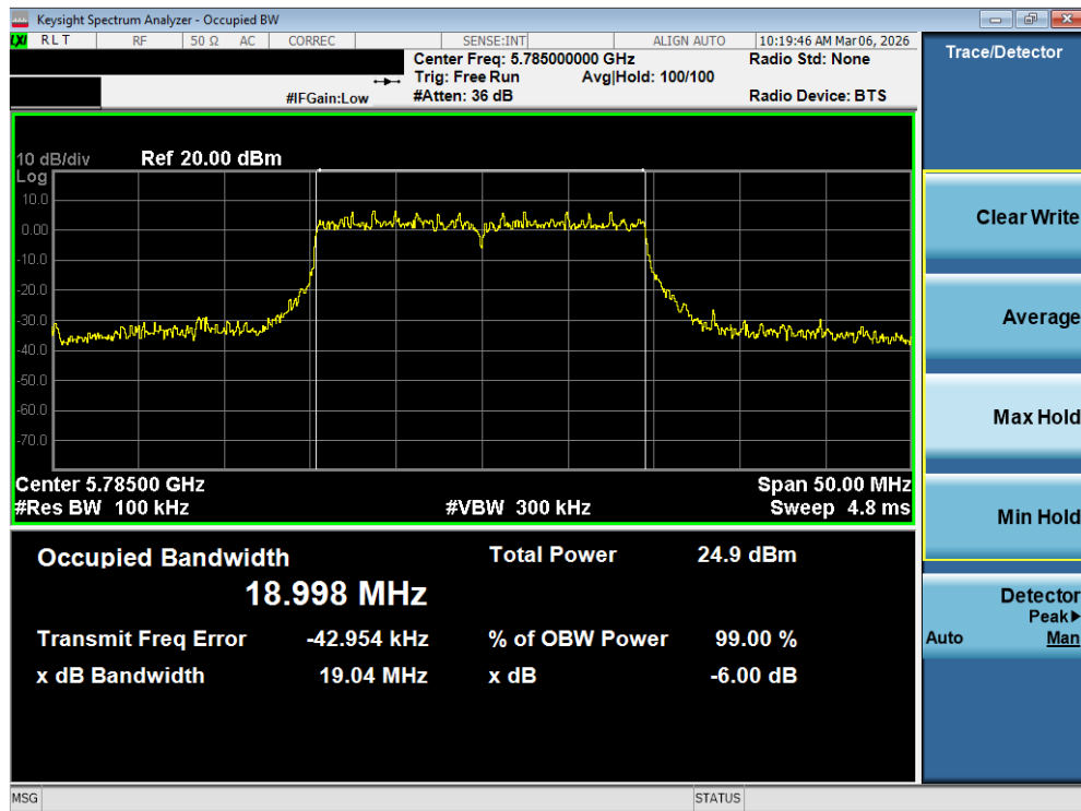
Plot 7-30. 6dB Bandwidth Plot MIMO ANT1 (20MHz BW 802.11be – 242 Tones (UNII Band 3) – Ch. 157)
