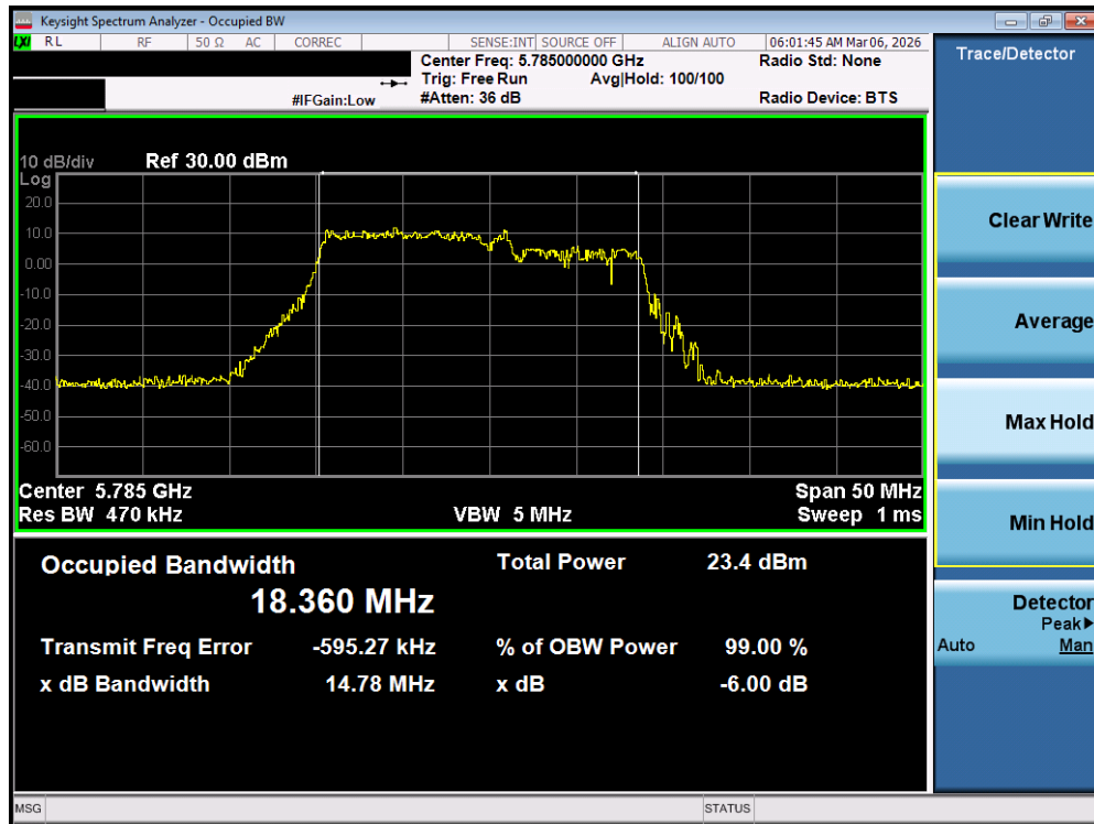
Plot 7-94. OBW Plot MIMO ANT2 (20MHz BW 802.11be – 106+26 Tones (UNII Band 3) – Ch. 157)
