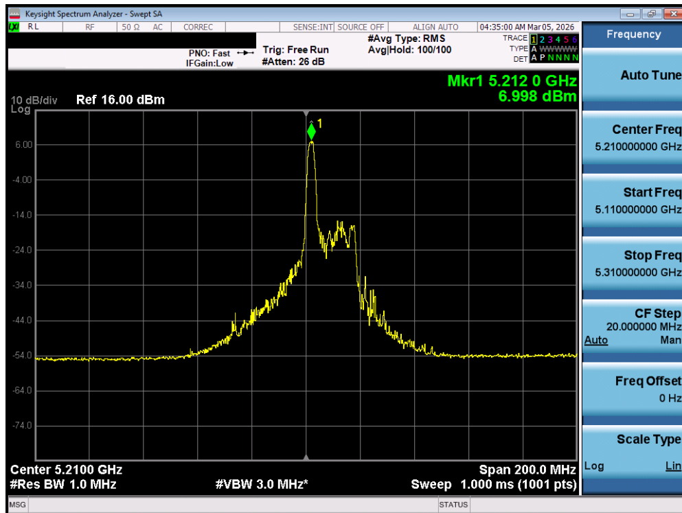
Plot 7-101. Power Spectral Density Plot MIMO ANT1 (80MHz BW 802.11be – 26 Tones (UNII Band 1) – Ch. 42)
