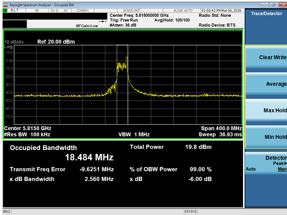
Plot 7-29. 6dB Bandwidth Plot MIMO ANT1 (160MHz BW 802.11be – 26 Tones (UNII Band 3/4) – Ch. 163)
