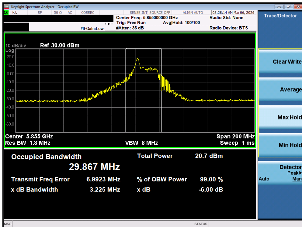
Plot 7-85. OBW Plot MIMO ANT2 (80MHz BW 802.11be – 26 Tones (UNII Band 3/4) – Ch. 171)
