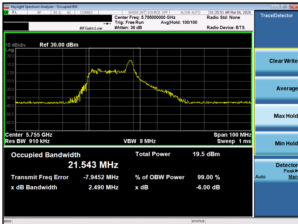
Plot 7-81. OBW Plot MIMO ANT2 (40MHz BW 802.11be – 26 Tones (UNII Band 3) – Ch. 151)
