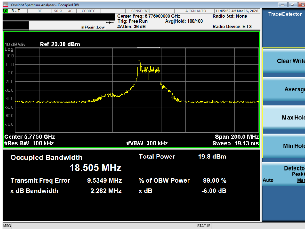
Plot 7-25. 6dB Bandwidth Plot MIMO ANT1 (80MHz BW 802.11be – 26 Tones (UNII Band 3) – Ch. 155)
