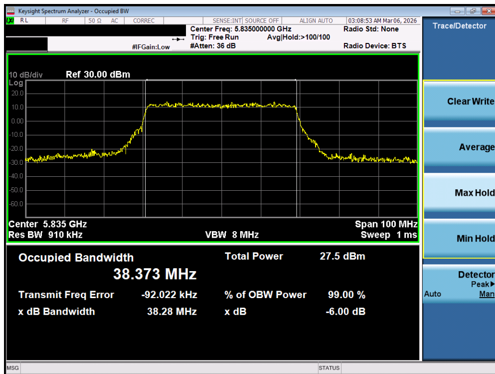
Plot 7-91. OBW Plot MIMO ANT2 (40MHz BW 802.11be – 484 Tones (UNII Band 3/4) – Ch. 167)
