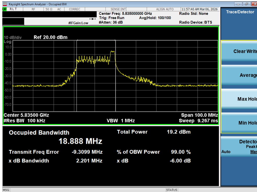
Plot 7-27. 6dB Bandwidth Plot MIMO ANT1 (40MHz BW 802.11be – 26 Tones (UNII Band 3/4) – Ch. 167)
