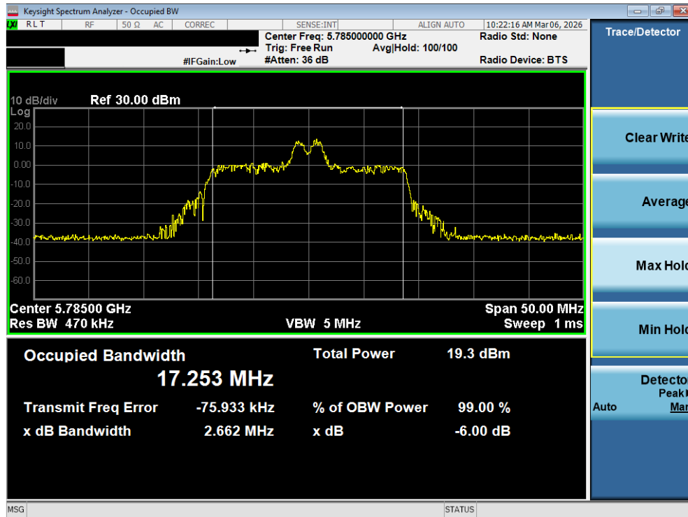
Plot 7-61. OBW Plot MIMO ANT1 (20MHz BW 802.11be – 26 Tones (UNII Band 3) – Ch. 157)
