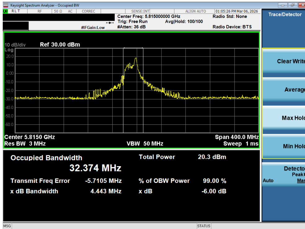
Plot 7-67. OBW Plot MIMO ANT1 (160MHz BW 802.11be – 26 Tones (UNII Band 3/4) – Ch. 163)
