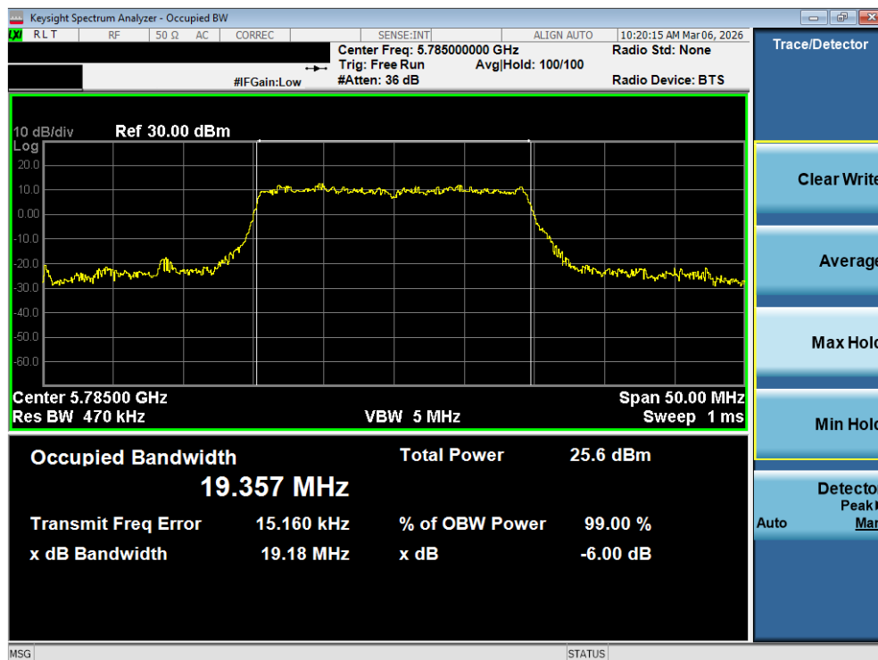
Plot 7-68. OBW Plot MIMO ANT1 (20MHz BW 802.11be – 242 Tones (UNII Band 3) – Ch. 157)
