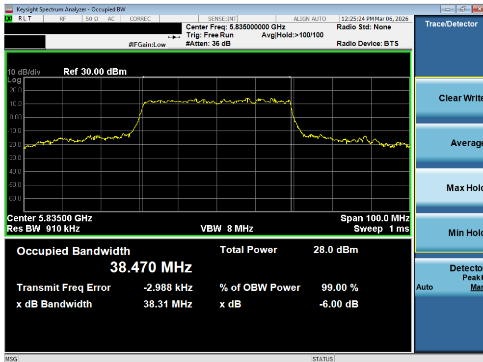
Plot 7-72. OBW Plot MIMO ANT1 (40MHz BW 802.11be – 484 Tones (UNII Band 3/4) – Ch. 167)
