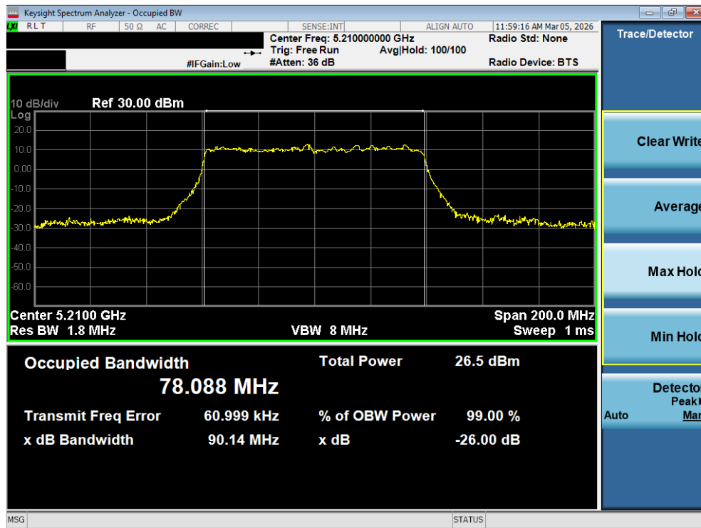
Plot 7-18. 26dB Bandwidth Plot MIMO ANT2 (80MHz BW 802.11be – 996 Tones (UNII Band 1) – Ch. 42)
