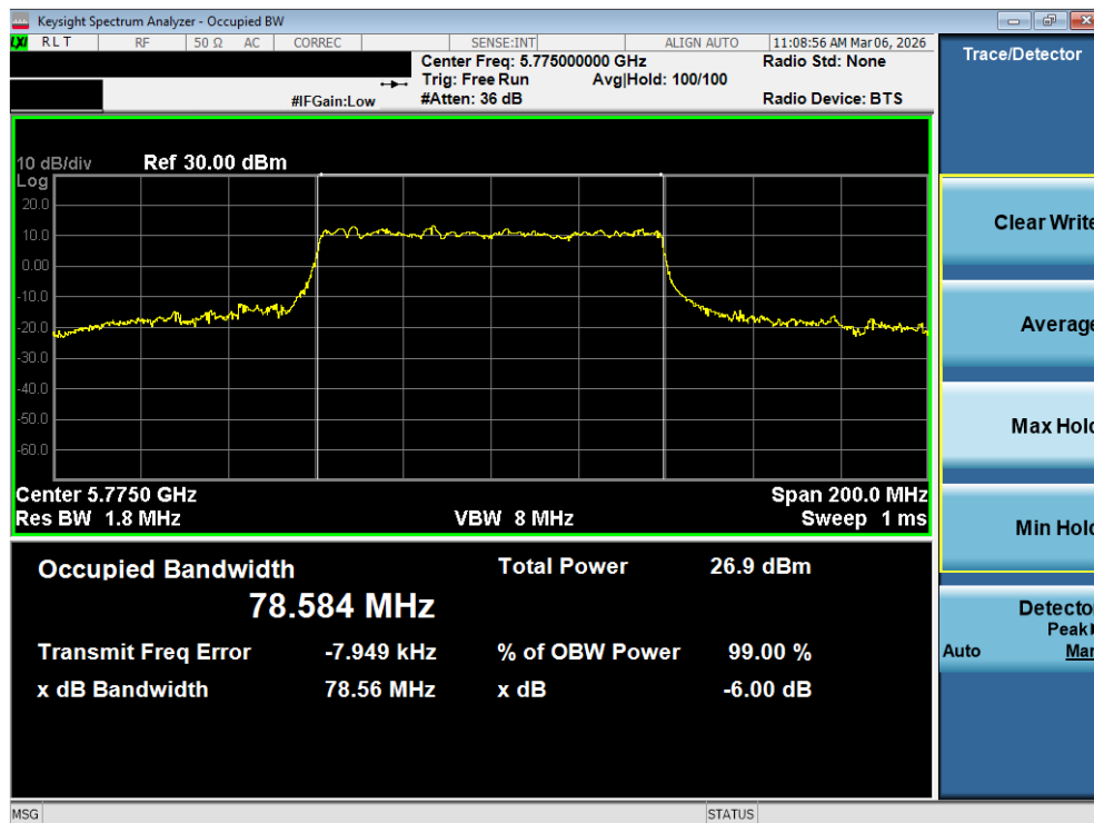
Plot 7-70. OBW Plot MIMO ANT1 (80MHz BW 802.11be – 996 Tones (UNII Band 3) – Ch. 155)
