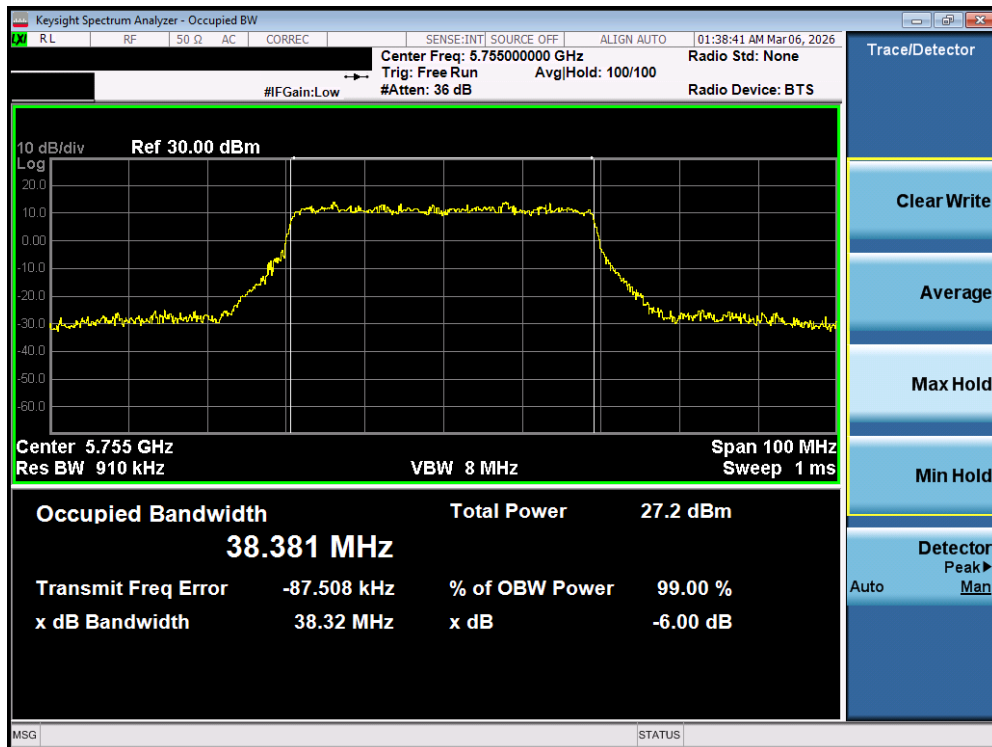
Plot 7-88. OBW Plot MIMO ANT2 (40MHz BW 802.11be – 484 Tones (UNII Band 3) – Ch. 151)
