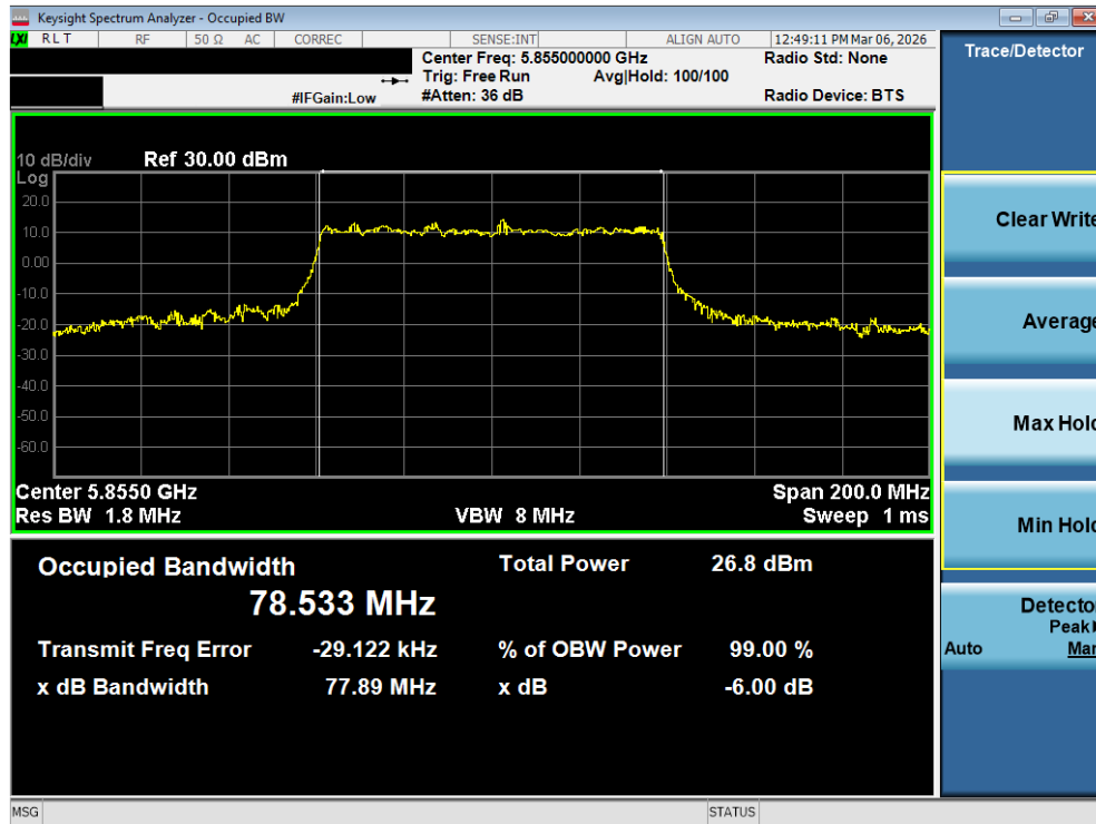
Plot 7-73. OBW Plot MIMO ANT1 (80MHz BW 802.11be – 996 Tones (UNII Band 3/4) – Ch. 171)
