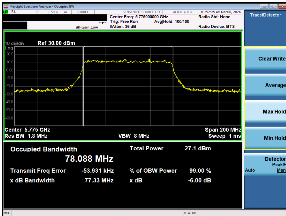
Plot 7-89. OBW Plot MIMO ANT2 (80MHz BW 802.11be – 996 Tones (UNII Band 3) – Ch. 155)
