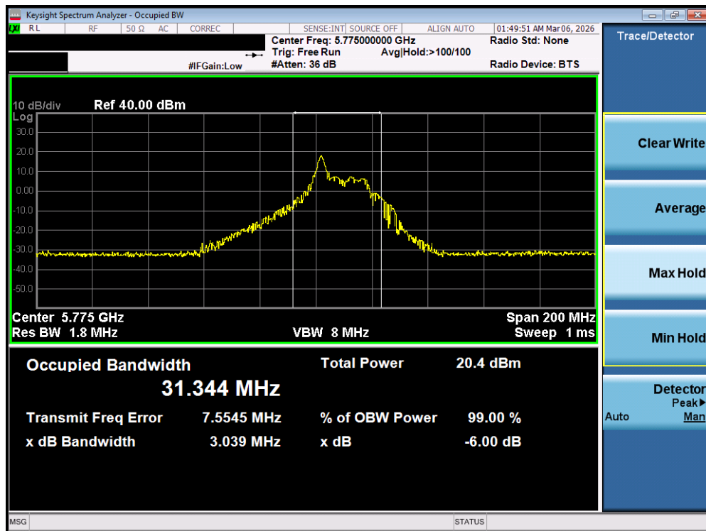
Plot 7-82. OBW Plot MIMO ANT2 (80MHz BW 802.11be – 26 Tones (UNII Band 3) – Ch. 155)
