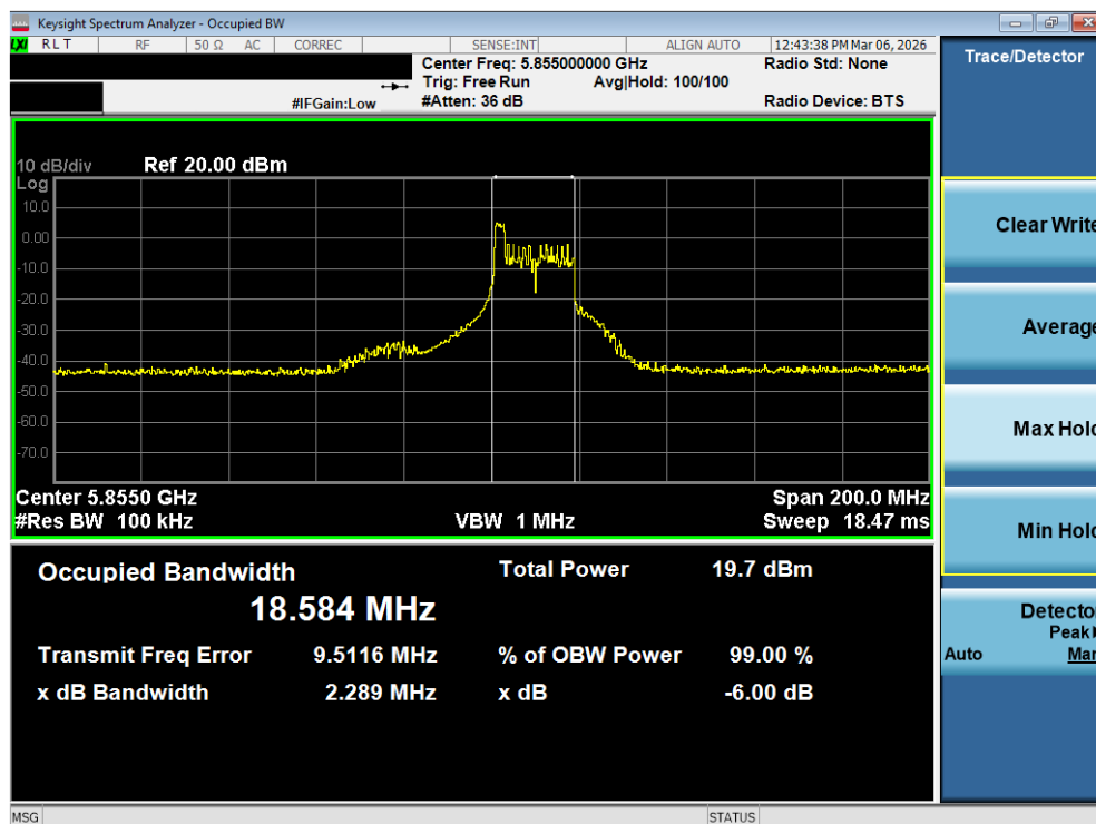
Plot 7-28. 6dB Bandwidth Plot MIMO ANT1 (80MHz BW 802.11be – 26 Tones (UNII Band 3/4) – Ch. 171)
