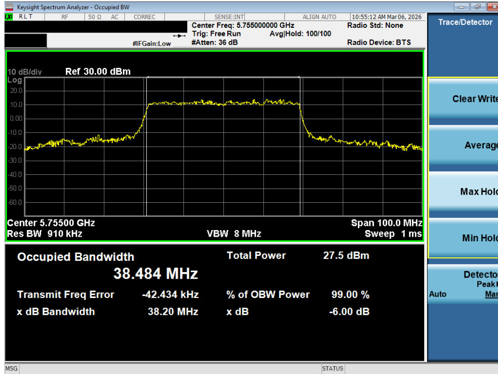
Plot 7-69. OBW Plot MIMO ANT1 (40MHz BW 802.11be – 484 Tones (UNII Band 3) – Ch. 151)
