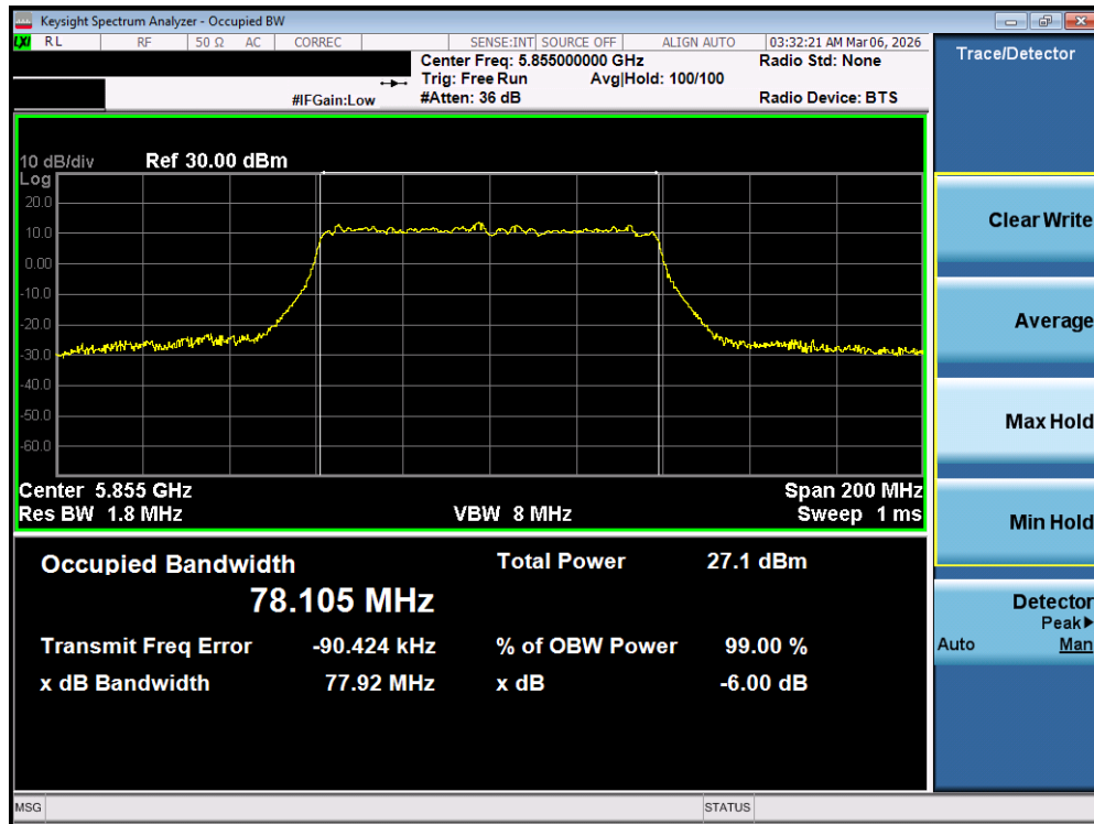
Plot 7-92. OBW Plot MIMO ANT2 (80MHz BW 802.11be – 996 Tones (UNII Band 3/4) – Ch. 171)
