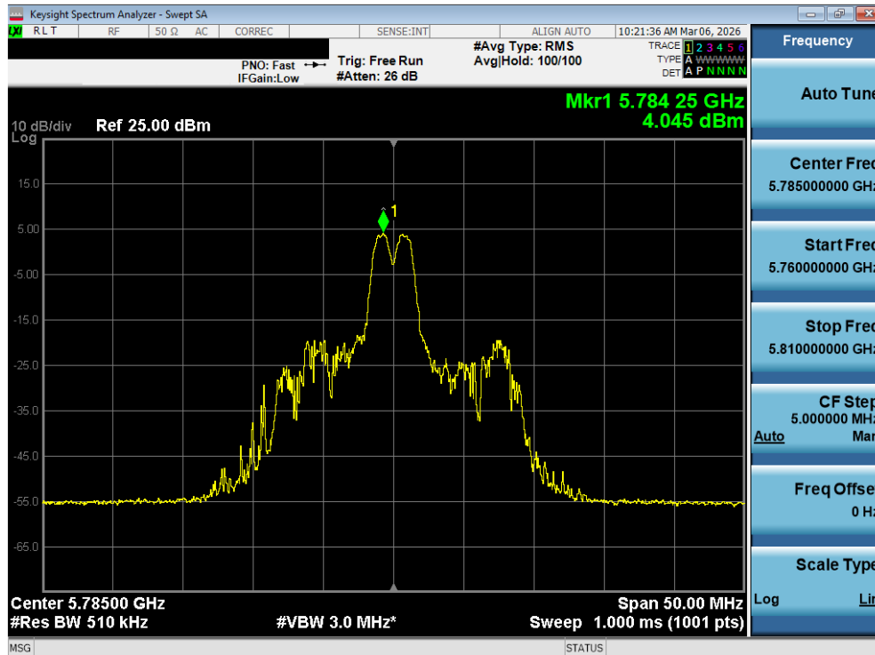
Plot 7-103. Power Spectral Density Plot MIMO ANT1 (20MHz BW 802.11be – 26 Tones (UNII Band 3) – Ch. 157)
