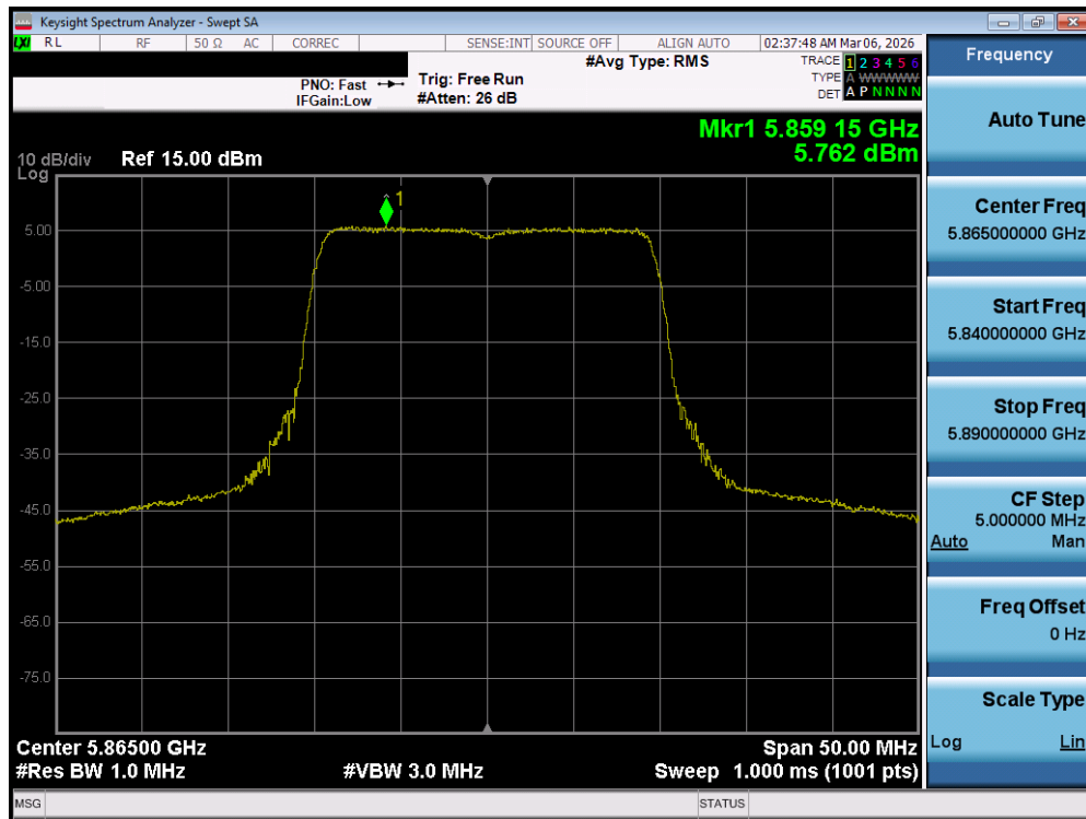
Plot 7-147. Power Spectral Density Plot MIMO ANT2 (20MHz BW 802.11be – 242 Tones (UNII Band 4) – Ch. 173)
