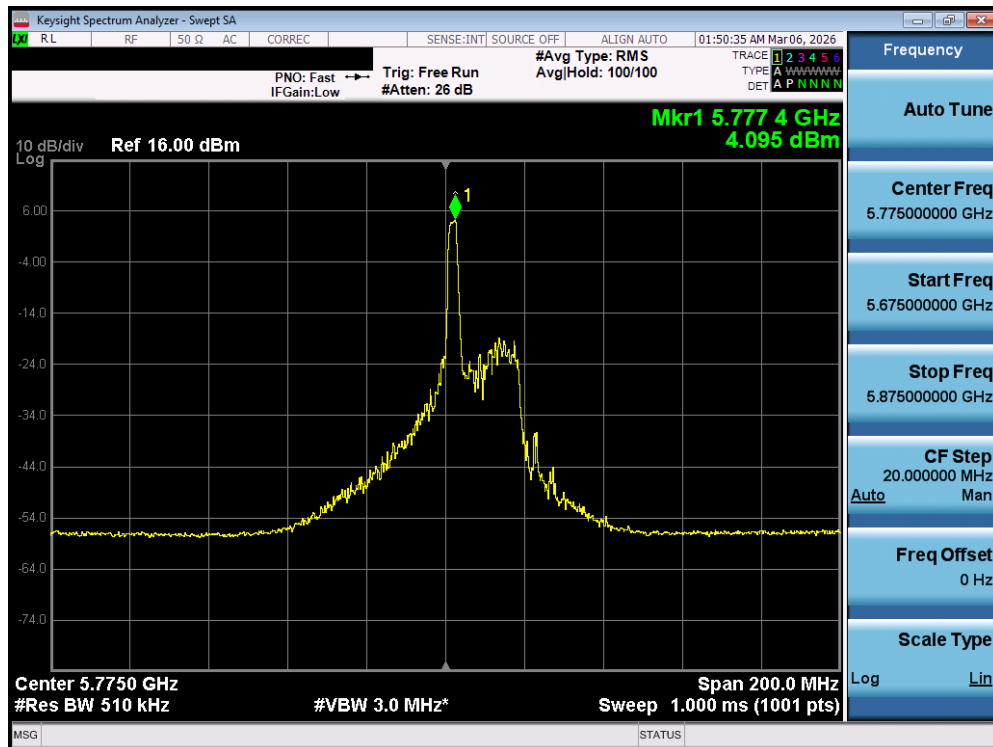
Plot 7-135. Power Spectral Density Plot MIMO ANT2 (80MHz BW 802.11be – 26 Tones (UNII Band 3) – Ch. 155)
