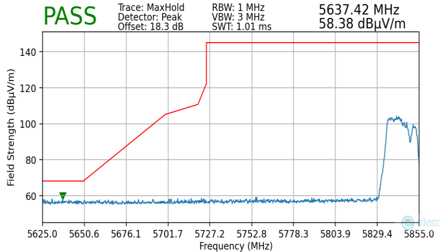
Plot 7-184. Radiated Lower Band Edge Plot MIMO (Peak - UNII Band 4 - 106+26 Tones)
