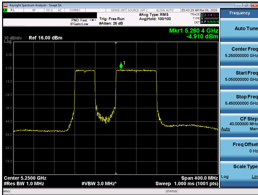
Plot 7-153. Power Spectral Density Plot MIMO ANT2 (160MHz BW 802.11be – 996+484 Tones (UNII Band 1/2A) – Ch. 50)
