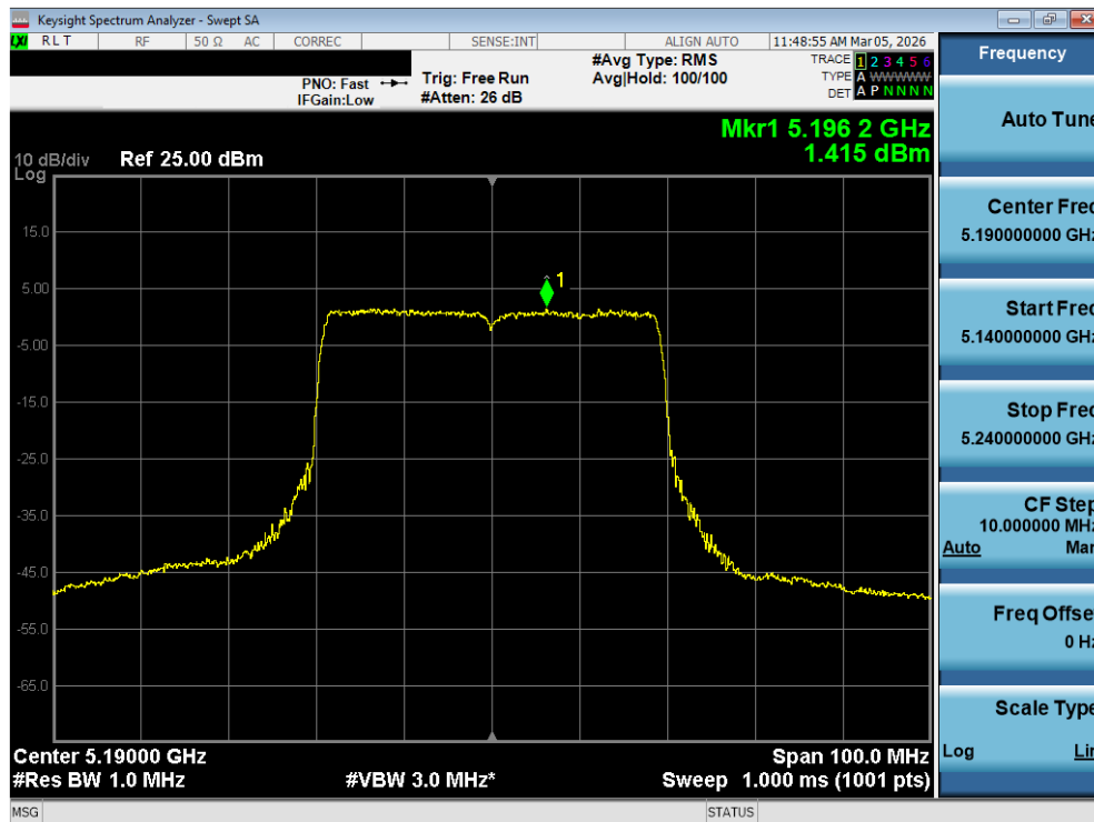
Plot 7-141. Power Spectral Density Plot MIMO ANT2 (40MHz BW 802.11be – 484 Tones (UNII Band 1) – Ch. 38)
