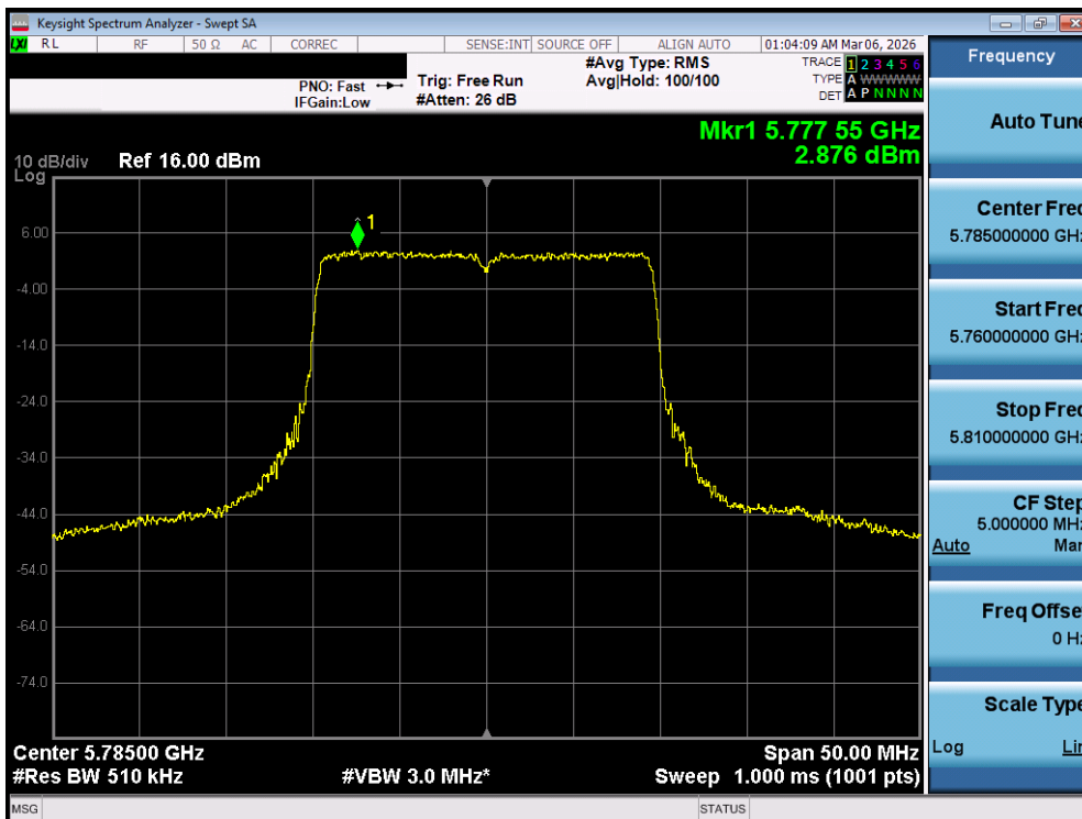
Plot 7-144. Power Spectral Density Plot MIMO ANT2 (20MHz BW 802.11be – 242 Tones (UNII Band 3) – Ch. 157)
