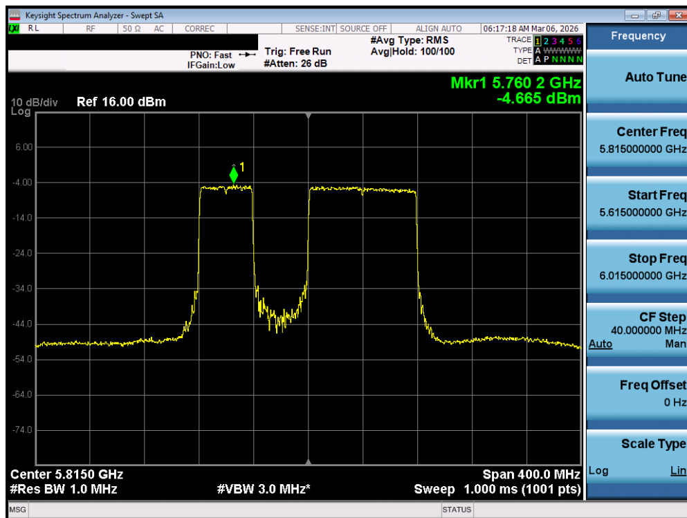
Plot 7-158. Power Spectral Density Plot MIMO ANT2 (160MHz BW 802.11be – 996+484 Tones (UNII Band 3/4) – Ch. 163)
