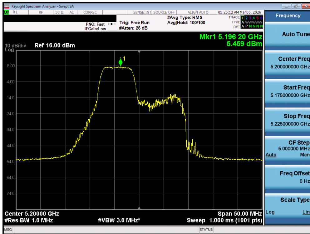
Plot 7-151. Power Spectral Density Plot MIMO ANT2 (20MHz BW 802.11be – 52+26 Tones (UNII Band 1) – Ch. 40)
