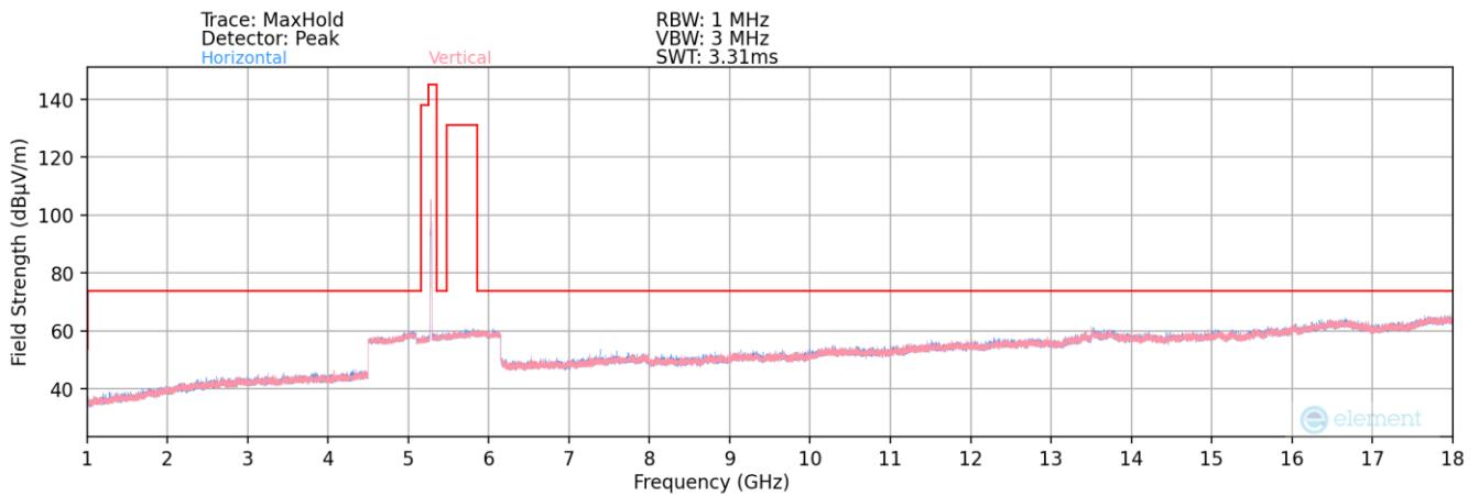
Plot 7-160. Radiated Spurious Plot above 1GHz MIMO (802.11ax – UNII 2A Ch. 56)
