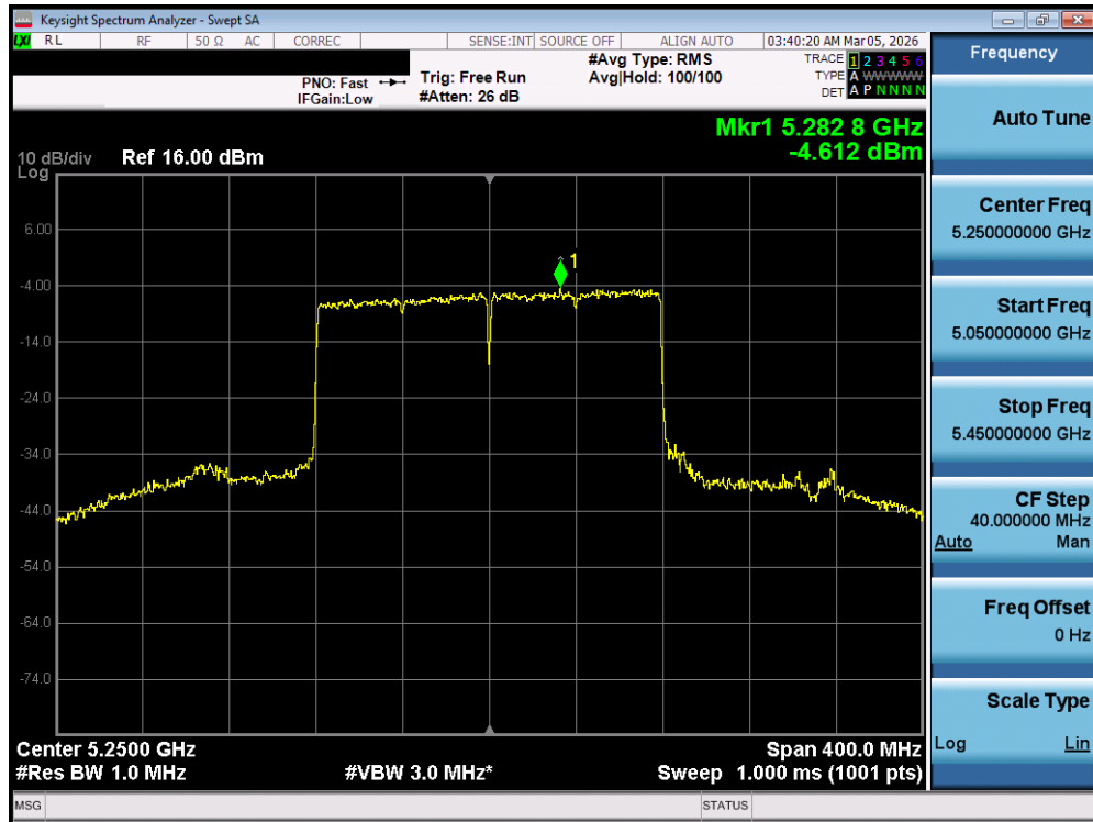
Plot 7-113. Power Spectral Density Plot MIMO ANT1 (160MHz BW 802.11be – 2x996 Tones (UNII Band 1/2A) – Ch. 50)
