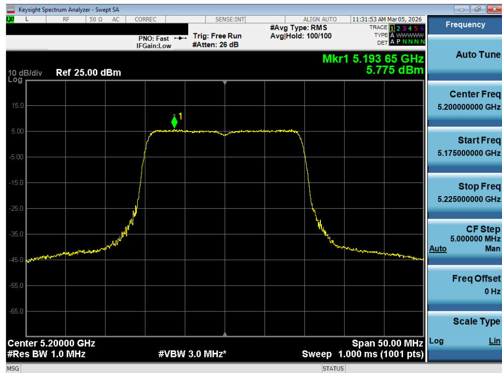
Plot 7-140. Power Spectral Density Plot MIMO ANT2 (20MHz BW 802.11be – 242 Tones (UNII Band 1) – Ch. 40)
