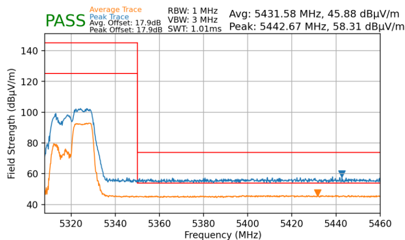
Plot 7-175. Radiated Upper Band Edge Plot MIMO (Average & Peak – UNII Band 2A – 106 Tones)
