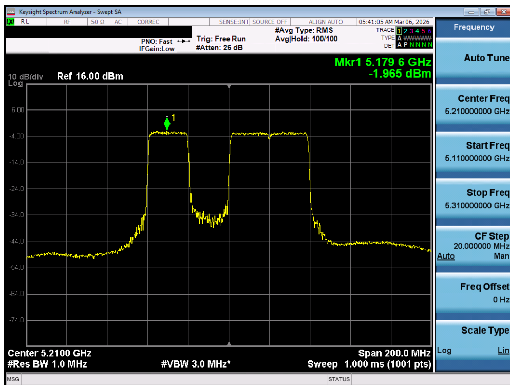
Plot 7-152. Power Spectral Density Plot MIMO ANT2 (80MHz BW 802.11be – 484+242 Tones (UNII Band 1) – Ch. 42)
