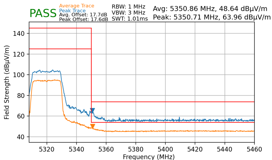
Plot 7-187. Radiated Upper Band Edge Plot MIMO (Average & Peak – UNII Band 2A – 242 Tones)
