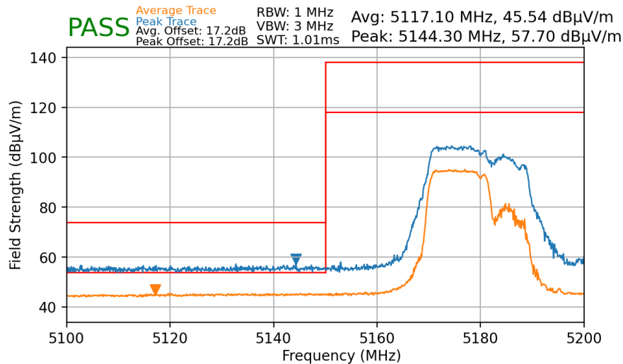
Plot 7-180. Radiated Lower Band Edge Plot MIMO (Average & Peak – UNII Band 1 – 106+26 Tones)
