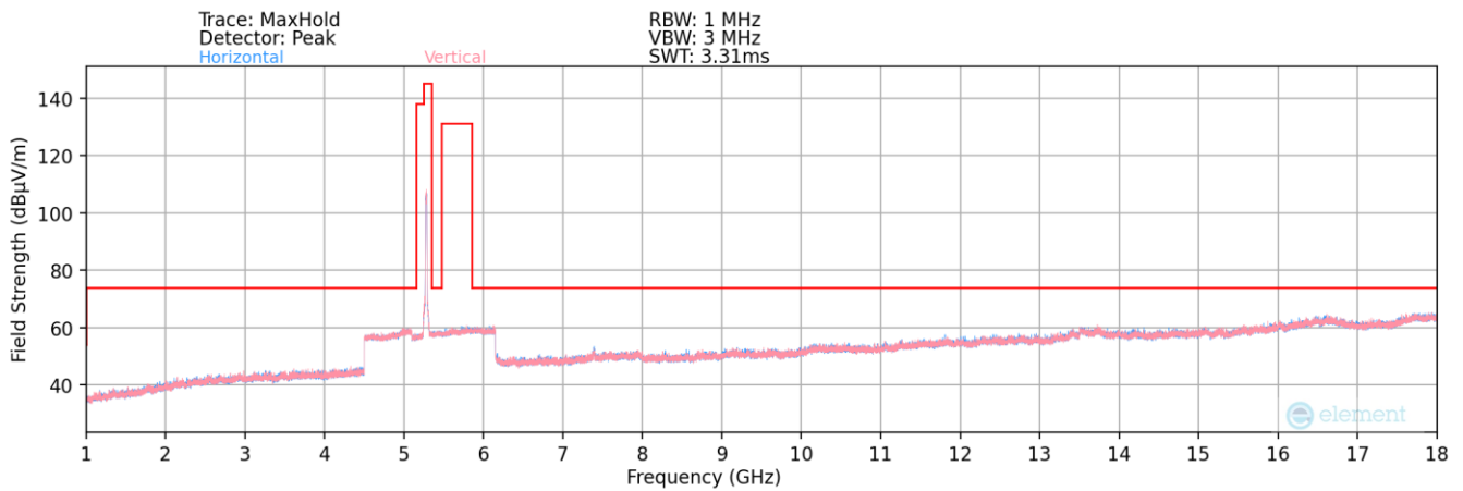
Plot 7-168. Radiated Spurious Plot above 1GHz MIMO (802.11ax – UNII 2A Ch. 56)
