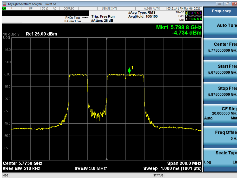
Plot 7-125. Power Spectral Density Plot MIMO ANT1 (80MHz BW 802.11be – 484+242 Tones (UNII Band 3) – Ch. 155)
