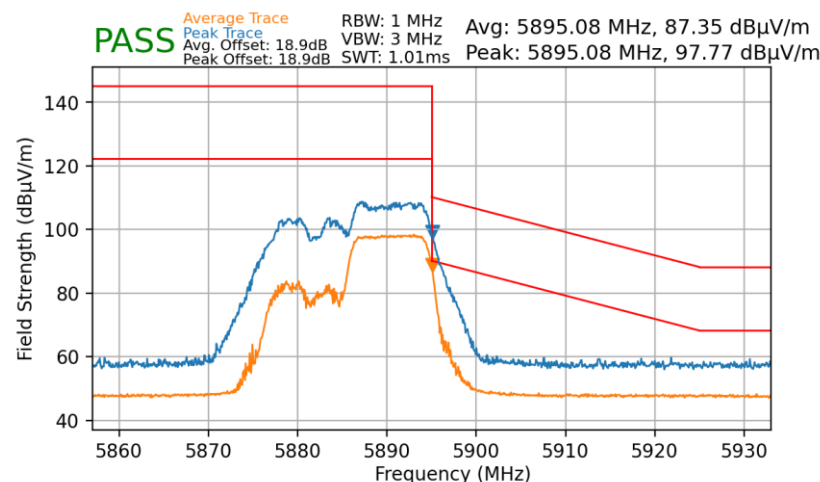
Plot 7-179. Radiated Upper Band Edge Plot MIMO (Average & Peak – UNII Band 4 – 106 Tones)
