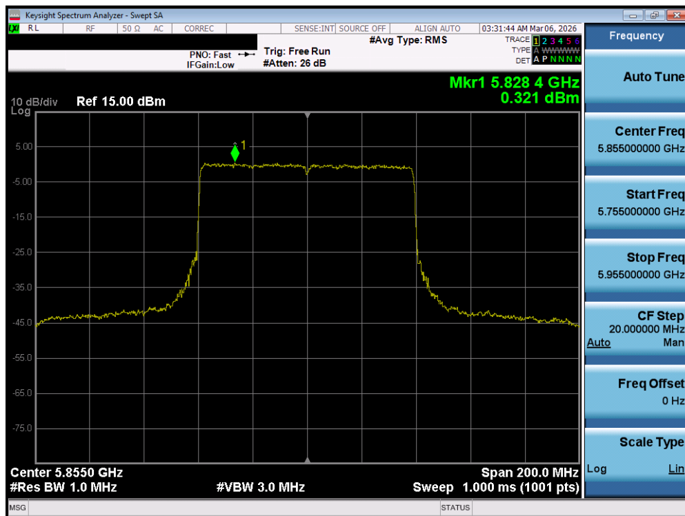
Plot 7-149. Power Spectral Density Plot MIMO ANT2 (80MHz BW 802.11be – 996 Tones (UNII Band 3/4) – Ch. 171)
