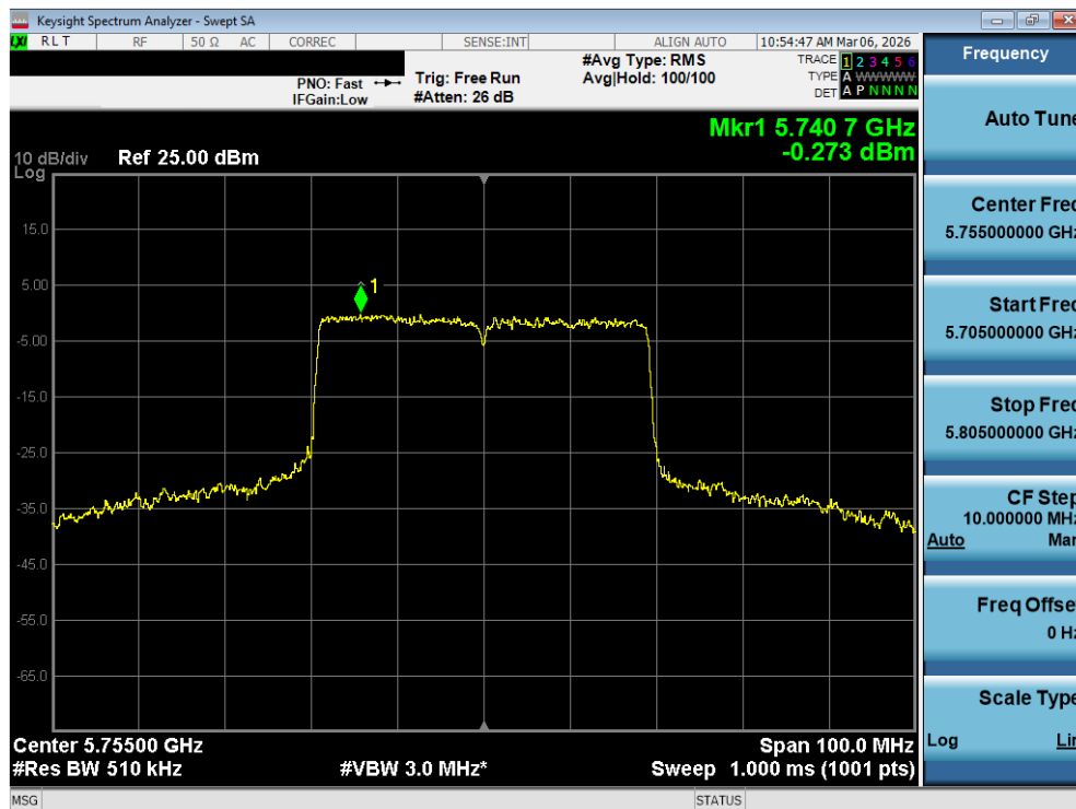
Plot 7-115. Power Spectral Density Plot MIMO ANT1 (40MHz BW 802.11be – 484 Tones (UNII Band 3) – Ch. 151)
