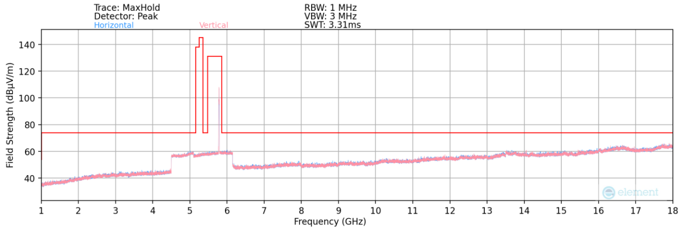
Plot 7-162. Radiated Spurious Plot above 1GHz MIMO (802.11ax – UNII 3 Ch. 157)
