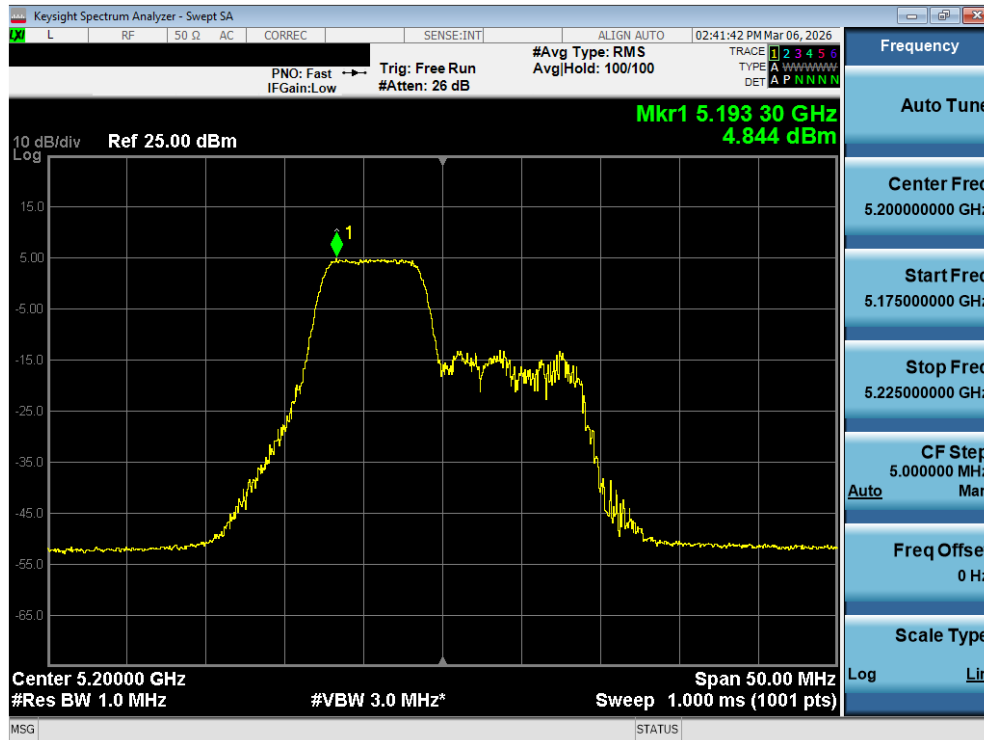
Plot 7-121. Power Spectral Density Plot MIMO ANT1 (20MHz BW 802.11be – 52+26 Tones (UNII Band 1) – Ch. 40)
