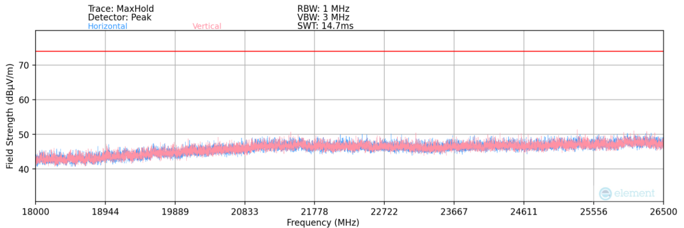
Plot 7-172. Radiated Spurious Plot 18GHz - 26.5GHz (802.11ax)
