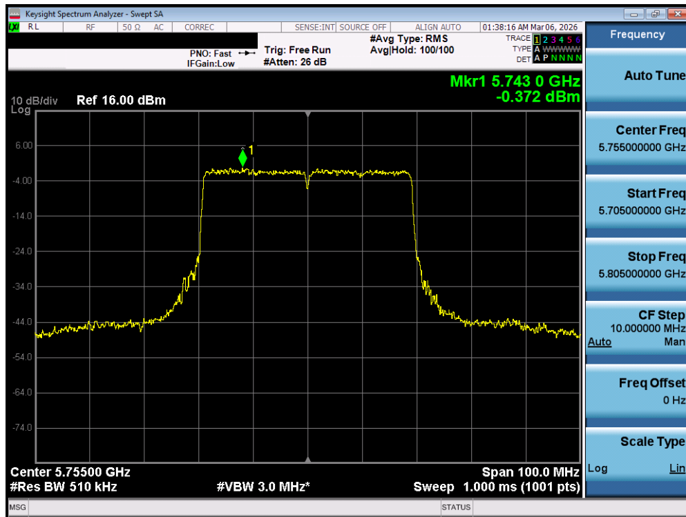
Plot 7-145. Power Spectral Density Plot MIMO ANT2 (40MHz BW 802.11be – 484 Tones (UNII Band 3) – Ch. 151)
