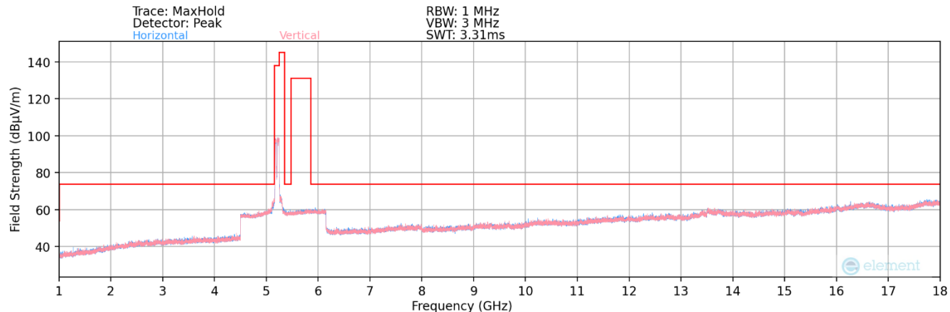
Plot 7-166. Radiated Spurious Plot above 1GHz MIMO (802.11be – MRU 484+242 Tones)
