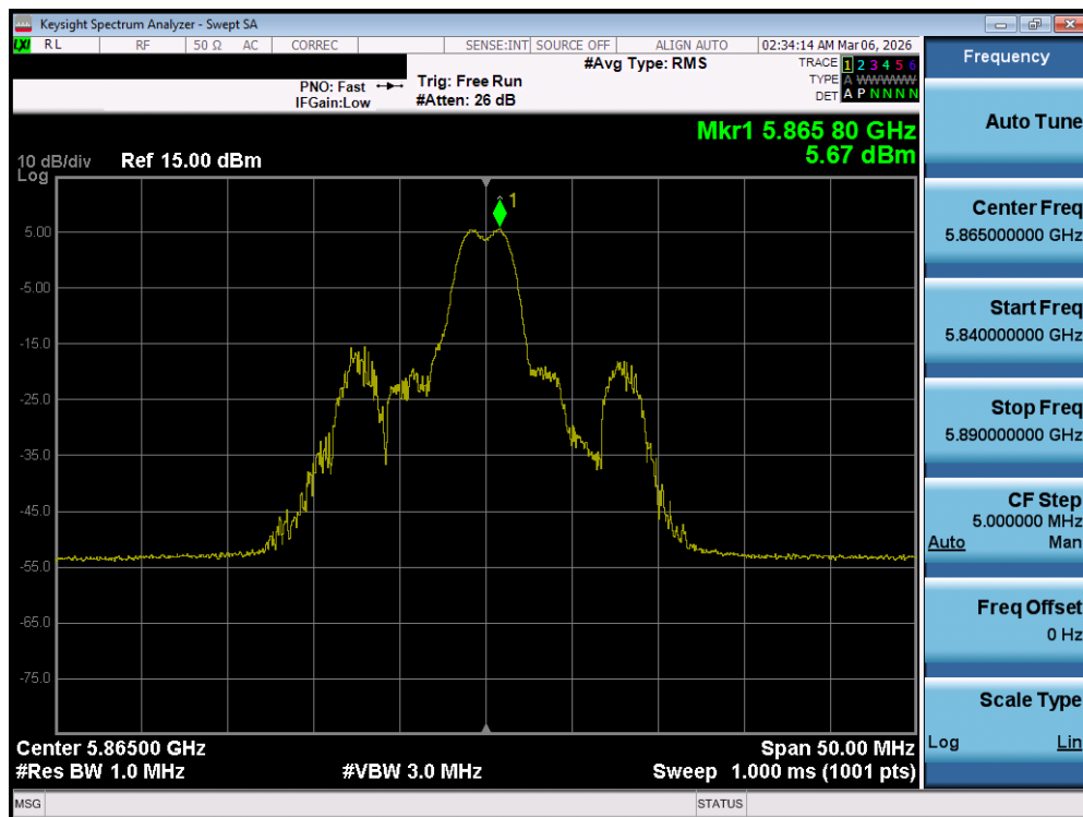
Plot 7-136. Power Spectral Density Plot MIMO ANT2 (20MHz BW 802.11be – 26 Tones (UNII Band 4) – Ch. 173)
