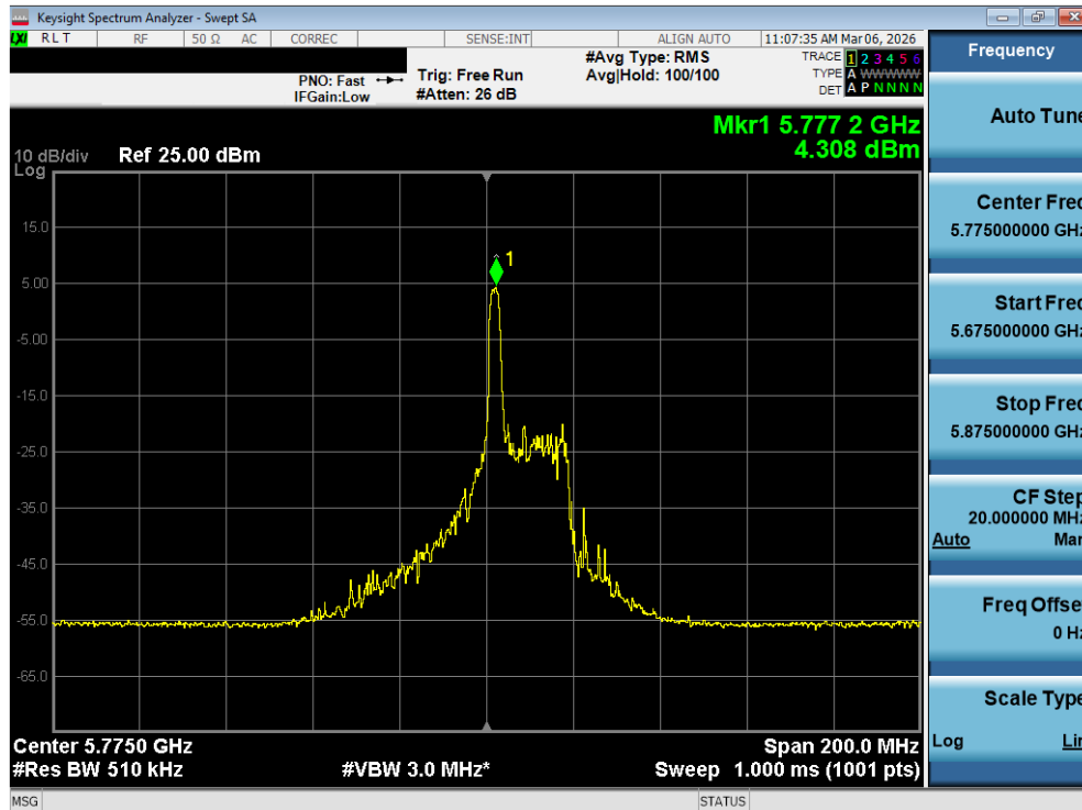
Plot 7-105. Power Spectral Density Plot MIMO ANT1 (80MHz BW 802.11be – 26 Tones (UNII Band 3) – Ch. 155)
