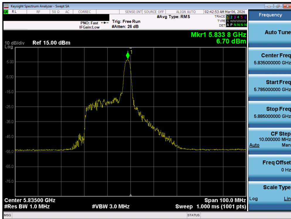
Plot 7-137. Power Spectral Density Plot MIMO ANT2 (40MHz BW 802.11be – 26 Tones (UNII Band 3/4) – Ch. 167)
