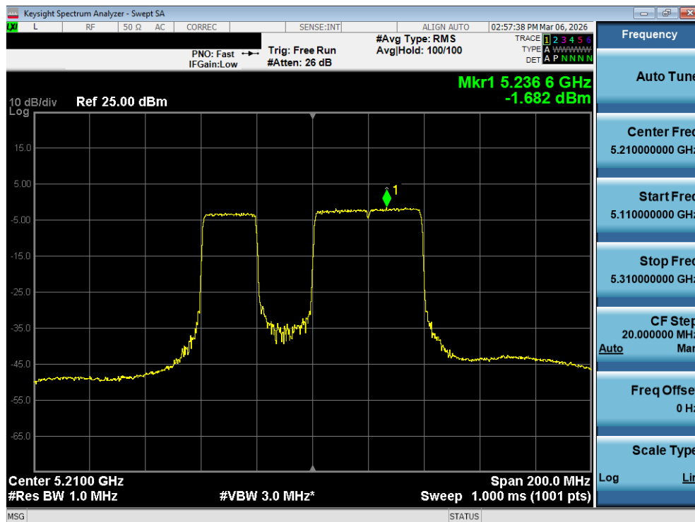
Plot 7-122. Power Spectral Density Plot MIMO ANT1 (80MHz BW 802.11be – 484+242 Tones (UNII Band 1) – Ch. 42)
