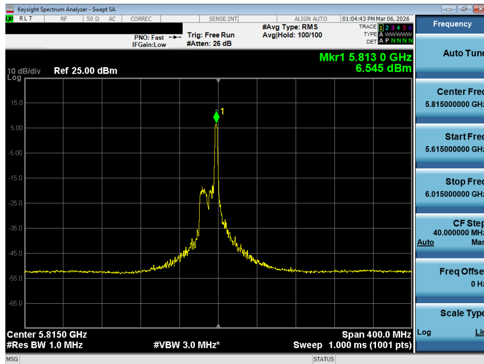
Plot 7-109. Power Spectral Density Plot MIMO ANT1 (160MHz BW 802.11be – 26 Tones (UNII Band 3/4) – Ch. 163)
