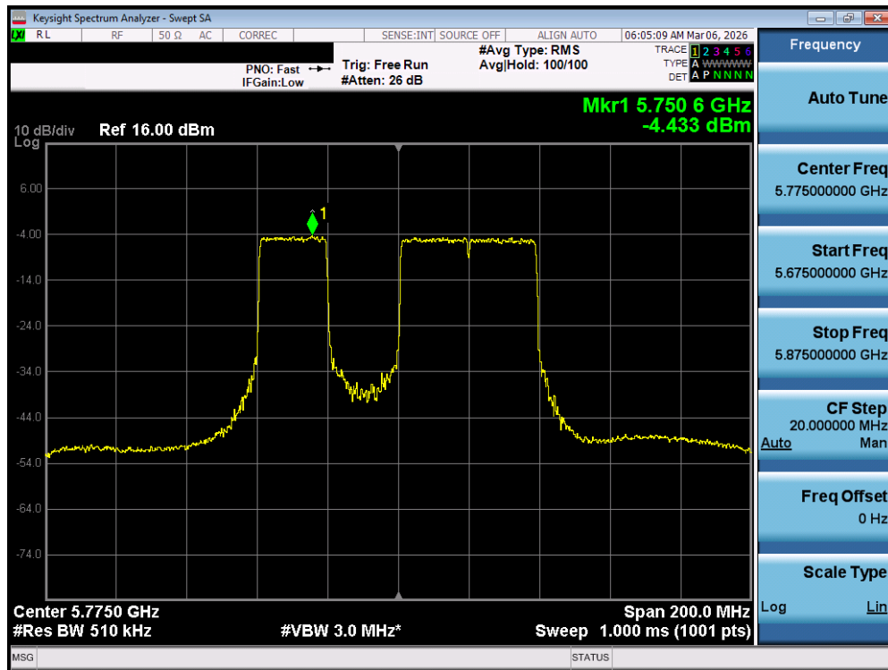
Plot 7-155. Power Spectral Density Plot MIMO ANT2 (80MHz BW 802.11be – 484+242 Tones (UNII Band 3) – Ch. 155)
