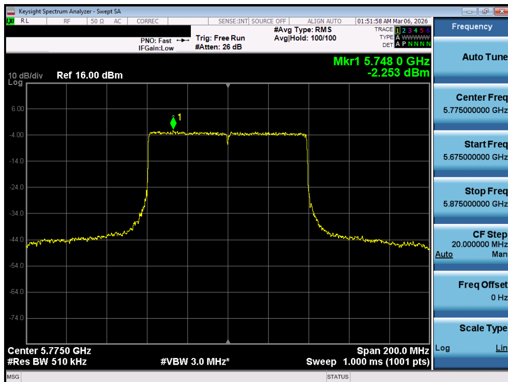
Plot 7-146. Power Spectral Density Plot MIMO ANT2 (80MHz BW 802.11be – 996 Tones (UNII Band 3) – Ch. 155)
