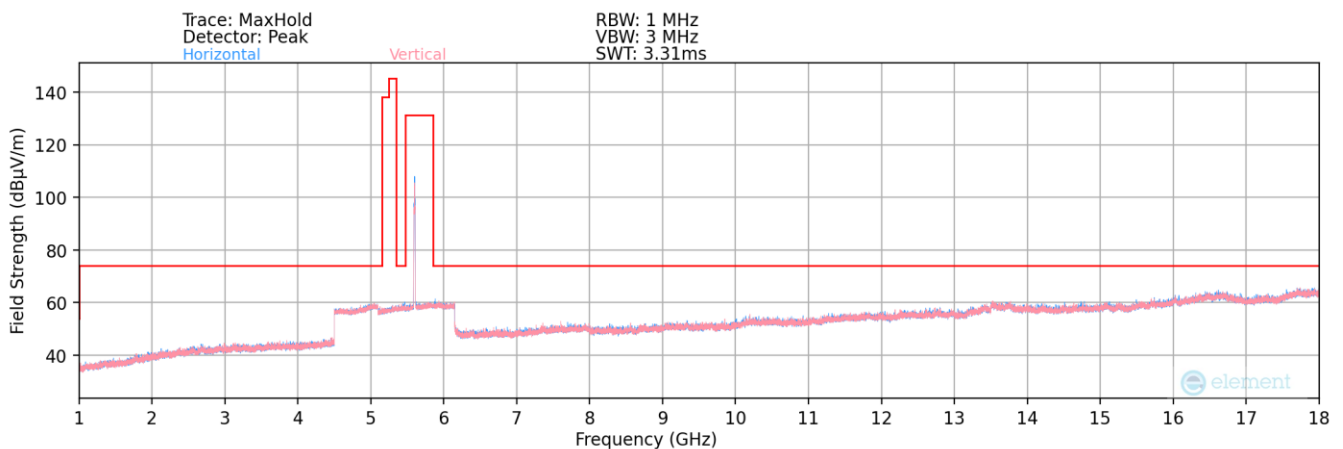
Plot 7-161. Radiated Spurious Plot above 1GHz MIMO (802.11ax – UNII 2C Ch. 120)
