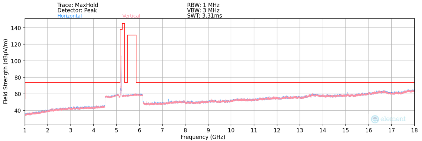
Plot 7-167. Radiated Spurious Plot above 1GHz MIMO (802.11ax – UNII 1 Ch. 40)
