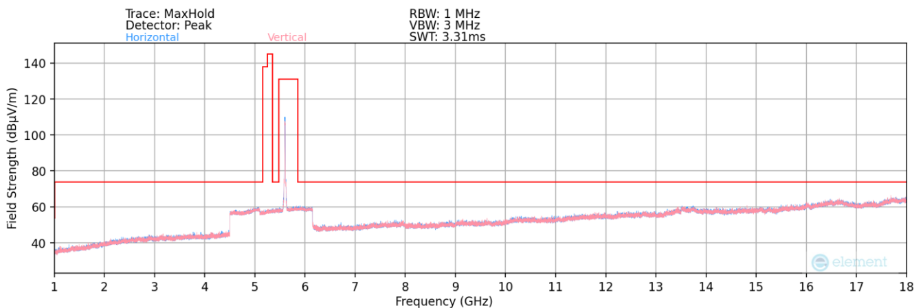
Plot 7-169. Radiated Spurious Plot above 1GHz MIMO (802.11ax – UNII 2C Ch. 120)
