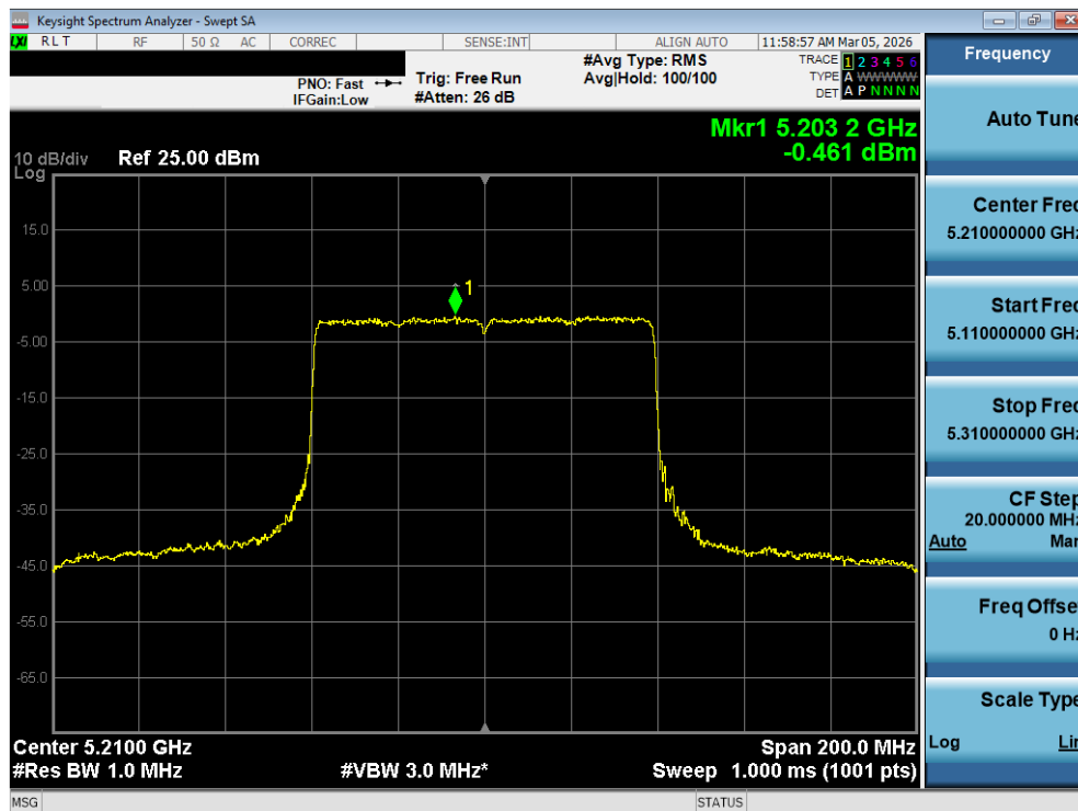
Plot 7-142. Power Spectral Density Plot MIMO ANT2 (80MHz BW 802.11be – 996 Tones (UNII Band 1) – Ch. 42)
