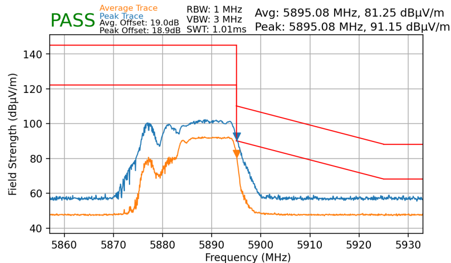
Plot 7-185. Radiated Upper Band Edge Plot MIMO (Average & Peak - UNII Band 4 - 106+26 Tones)
