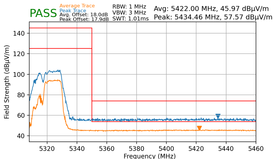
Plot 7-181. Radiated Upper Band Edge Plot MIMO (Average & Peak – UNII Band 2A – 106+26 Tones)
