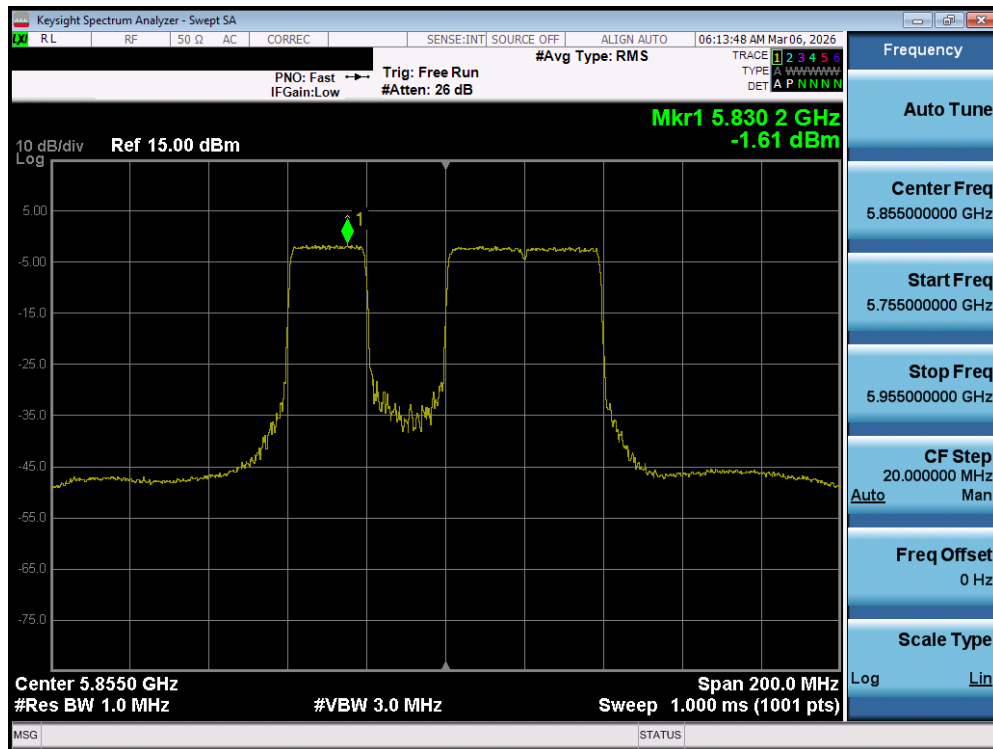
Plot 7-157. Power Spectral Density Plot MIMO ANT2 (80MHz BW 802.11be – 484+242 Tones (UNII Band 3/4) – Ch. 171)
