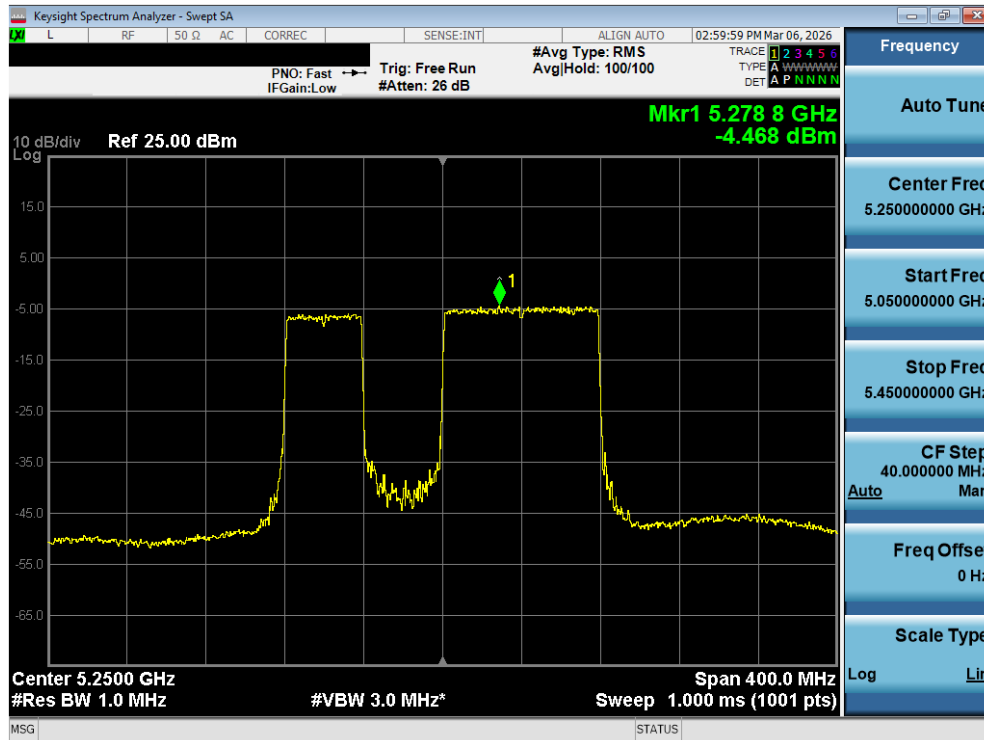
Plot 7-123. Power Spectral Density Plot MIMO ANT1 (160MHz BW 802.11be – 996+484 Tones (UNII Band 1/2A) – Ch. 50)
