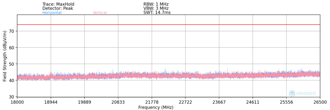
Plot 7-164. Radiated Spurious Plot 18GHz - 26.5GHz (802.11ax)
