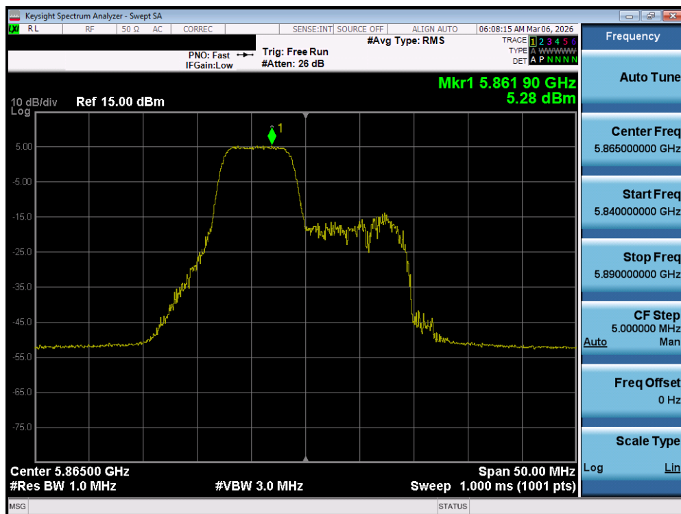
Plot 7-156. Power Spectral Density Plot MIMO ANT2 (20MHz BW 802.11be – 52+26 Tones (UNII Band 4) – Ch. 173)
