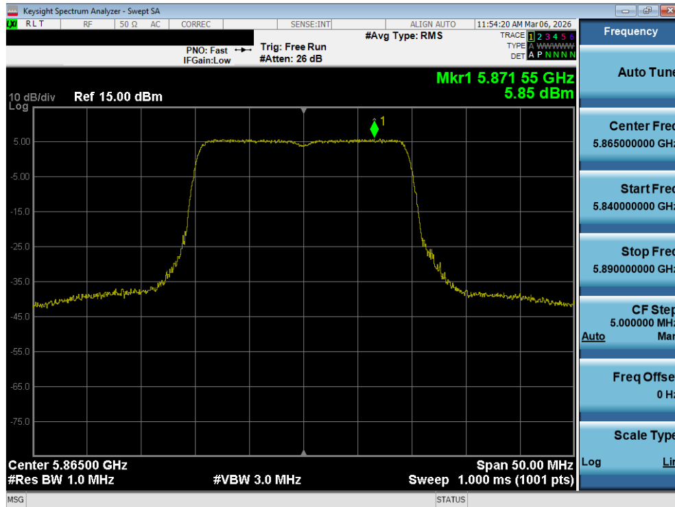
Plot 7-117. Power Spectral Density Plot MIMO ANT1 (20MHz BW 802.11be – 242 Tones (UNII Band 4) – Ch. 173)
