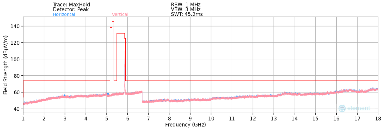
Plot 7-171. Radiated Spurious Plot above 1GHz MIMO (802.11ax – UNII 4 Ch. 173)
