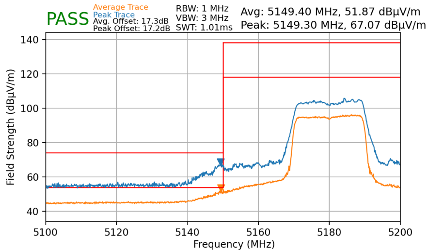
Plot 7-186. Radiated Lower Band Edge Plot MIMO (Average & Peak – UNII Band 1 – 242 Tones)
