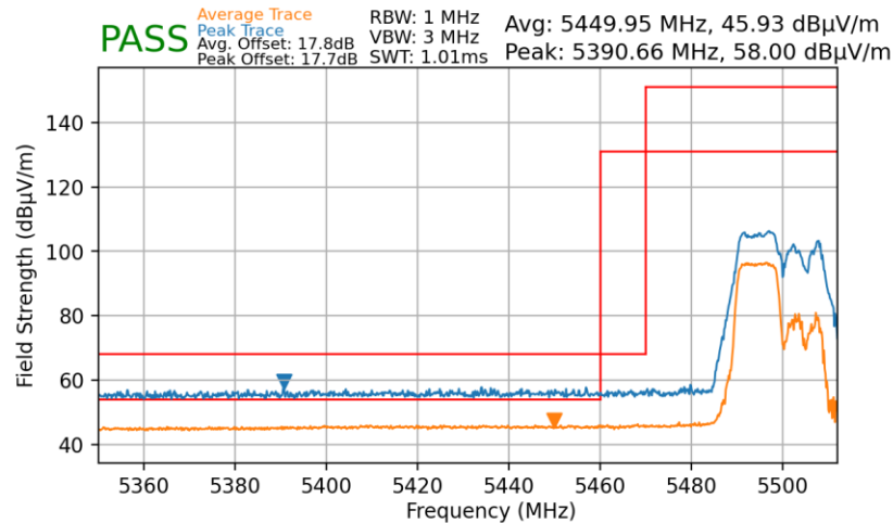
Plot 7-176. Radiated Lower Band Edge Plot MIMO (Average & Peak – UNII Band 2C – 106 Tones)
