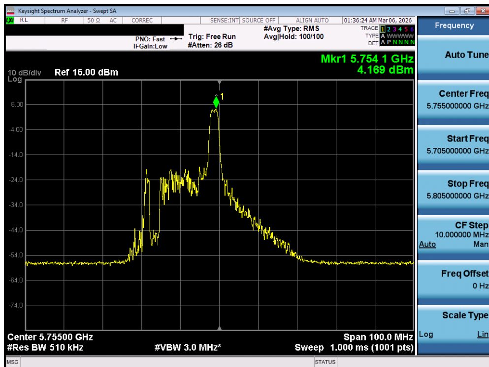
Plot 7-134. Power Spectral Density Plot MIMO ANT2 (40MHz BW 802.11be – 26 Tones (UNII Band 3) – Ch. 151)
