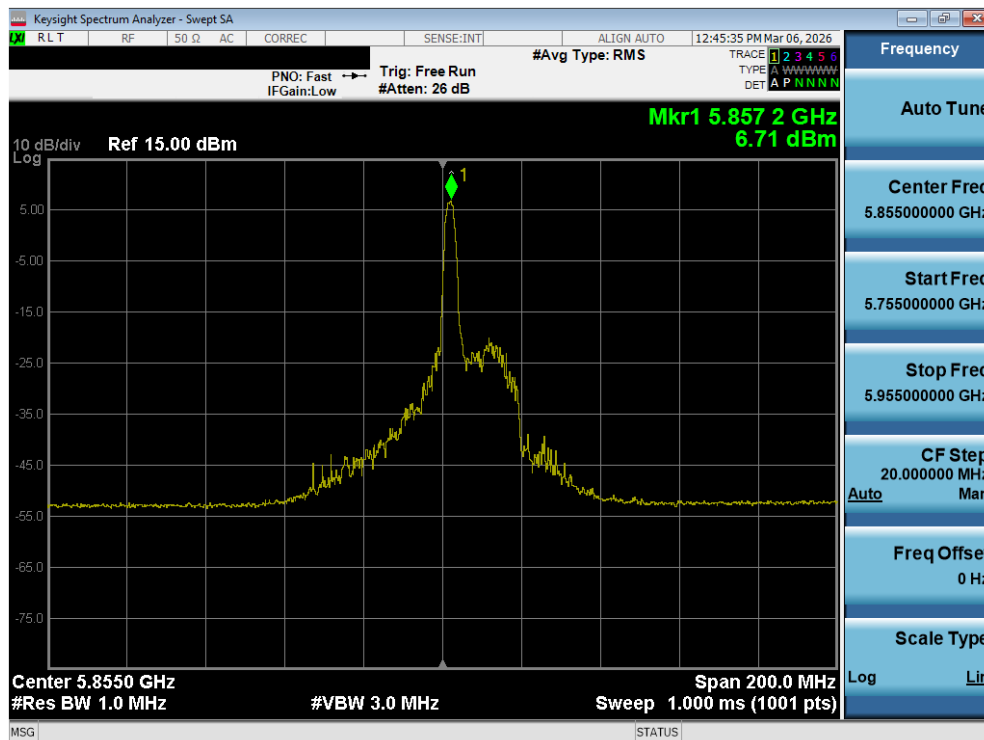
Plot 7-108. Power Spectral Density Plot MIMO ANT1 (80MHz BW 802.11be – 26 Tones (UNII Band 3/4) – Ch. 171)
