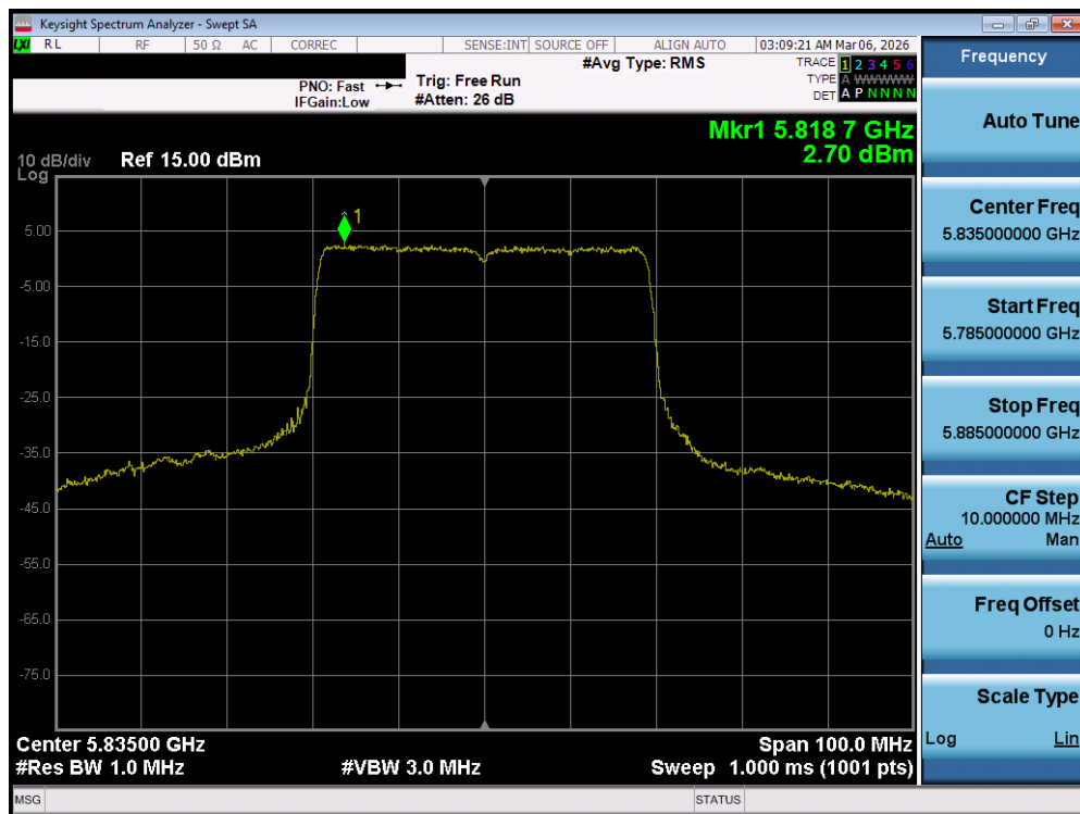
Plot 7-148. Power Spectral Density Plot MIMO ANT2 (40MHz BW 802.11be – 484 Tones (UNII Band 3/4) – Ch. 167)
