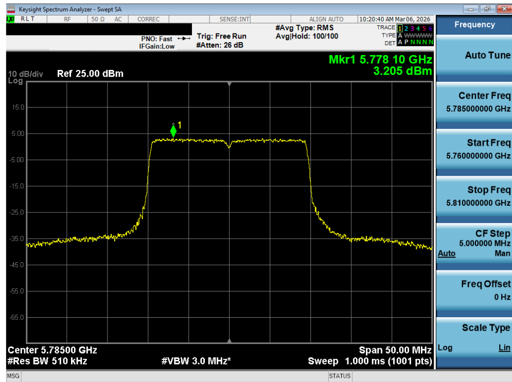
Plot 7-114. Power Spectral Density Plot MIMO ANT1 (20MHz BW 802.11be – 242 Tones (UNII Band 3) – Ch. 157)
