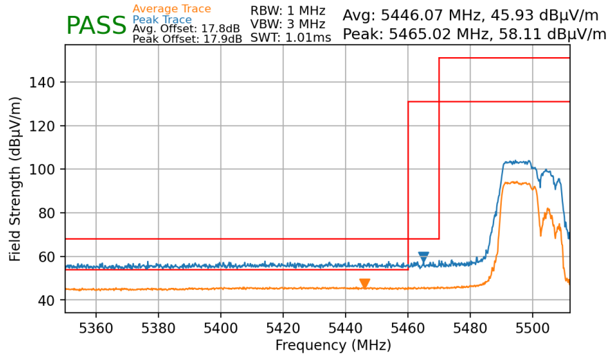
Plot 7-182. Radiated Lower Band Edge Plot MIMO (Average & Peak – UNII Band 2C – 106+26 Tones)
