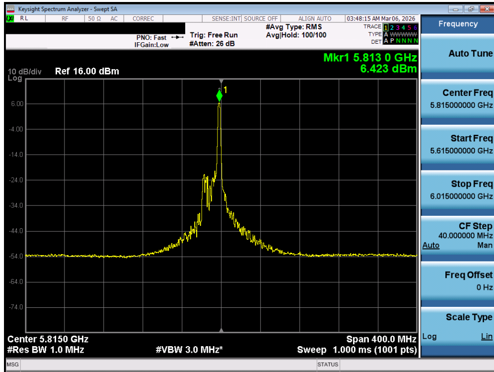
Plot 7-139. Power Spectral Density Plot MIMO ANT2 (160MHz BW 802.11be – 26 Tones (UNII Band 3/4) – Ch. 163)
