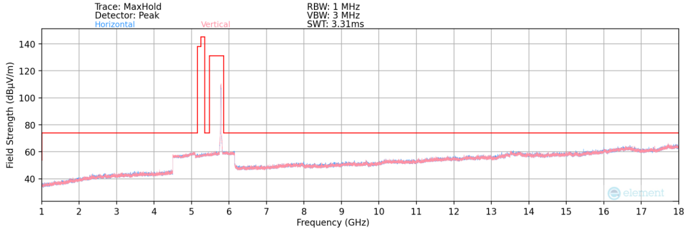
Plot 7-170. Radiated Spurious Plot above 1GHz MIMO (802.11ax – UNII 3 Ch. 157)
