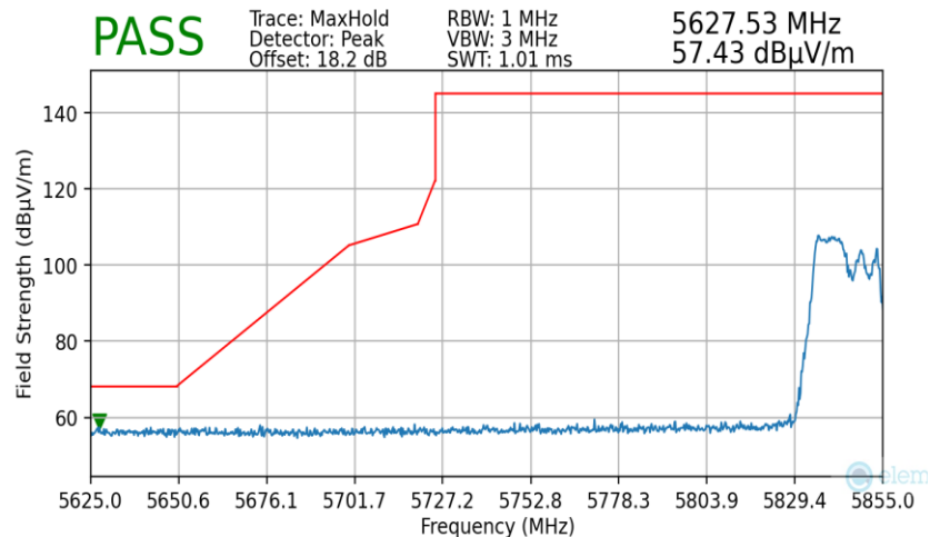
Plot 7-178. Radiated Lower Band Edge Plot MIMO (Peak – UNII Band 4 – 106 Tones)
