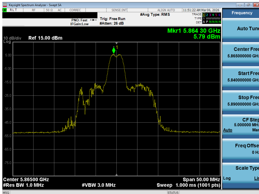
Plot 7-106. Power Spectral Density Plot MIMO ANT1 (20MHz BW 802.11be – 26 Tones (UNII Band 4) – Ch. 173)
