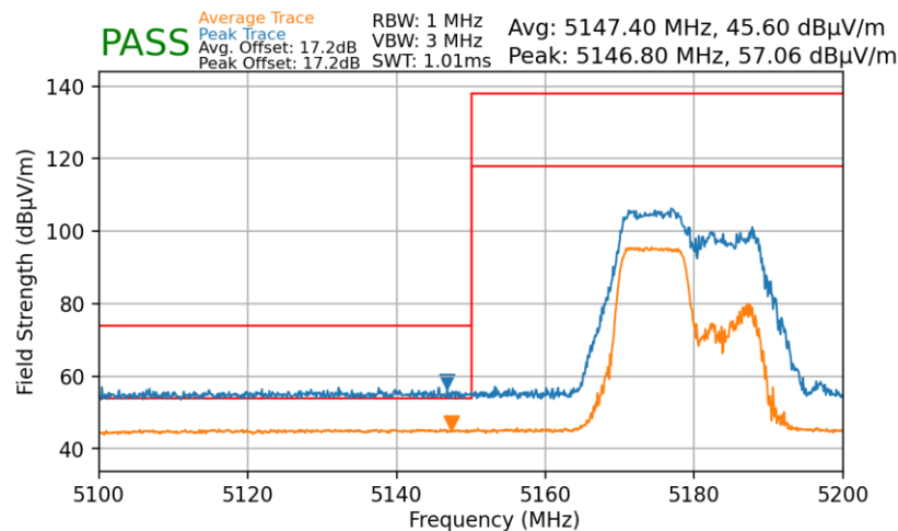
Plot 7-174. Radiated Lower Band Edge Plot MIMO (Average & Peak – UNII Band 1 – 106 Tones)
