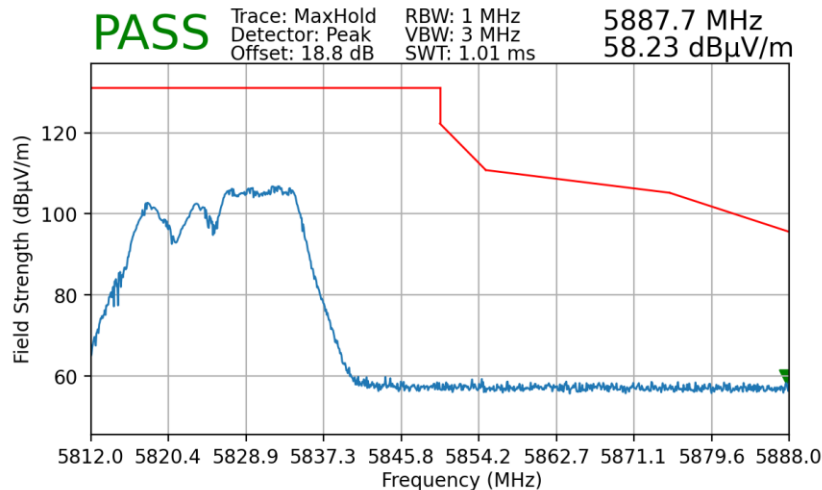
Plot 7-177. Radiated Upper Band Edge Plot MIMO (Peak – UNII Band 3 – 106 Tones)
