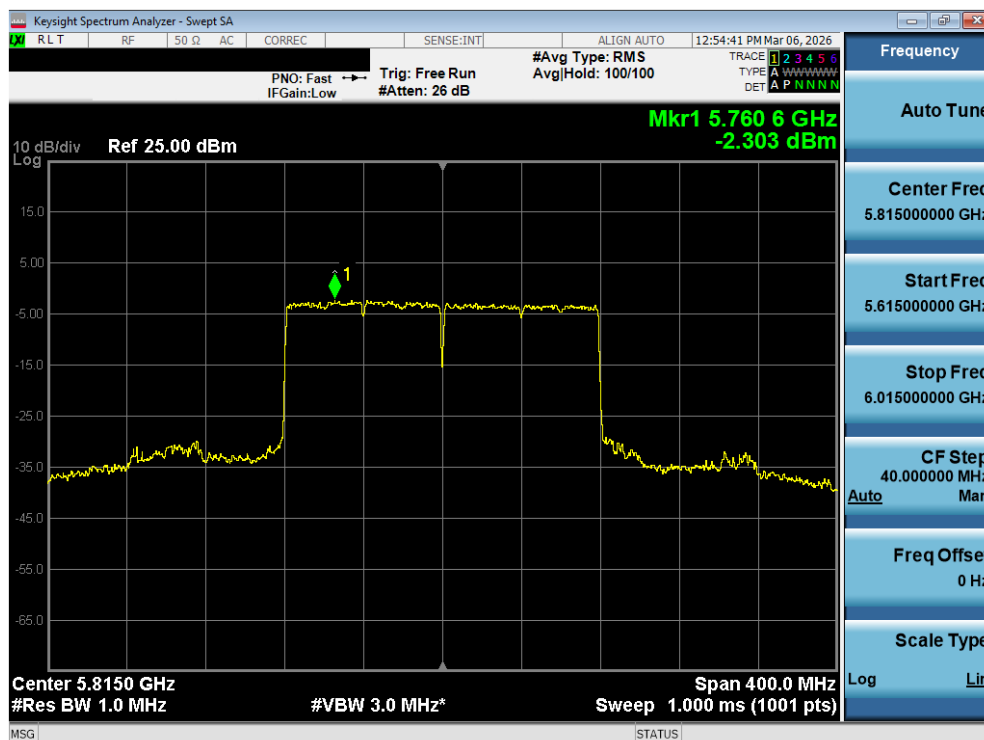
Plot 7-120. Power Spectral Density Plot MIMO ANT1 (160MHz BW 802.11be – 996*2 Tones (UNII Band 3/4) – Ch. 163)
