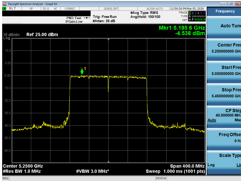
Plot 7-143. Power Spectral Density Plot MIMO ANT2 (160MHz BW 802.11be – 2x996 Tones (UNII Band 1/2A) – Ch. 50)
