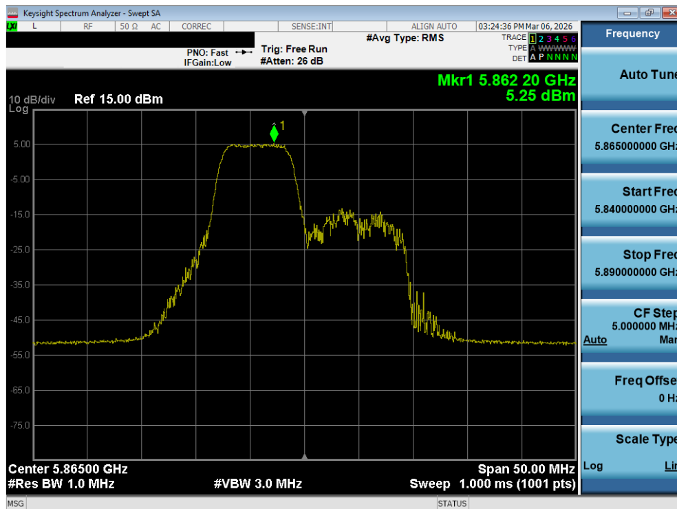
Plot 7-126. Power Spectral Density Plot MIMO ANT1 (20MHz BW 802.11be – 52+26 Tones (UNII Band 4) – Ch. 173)
