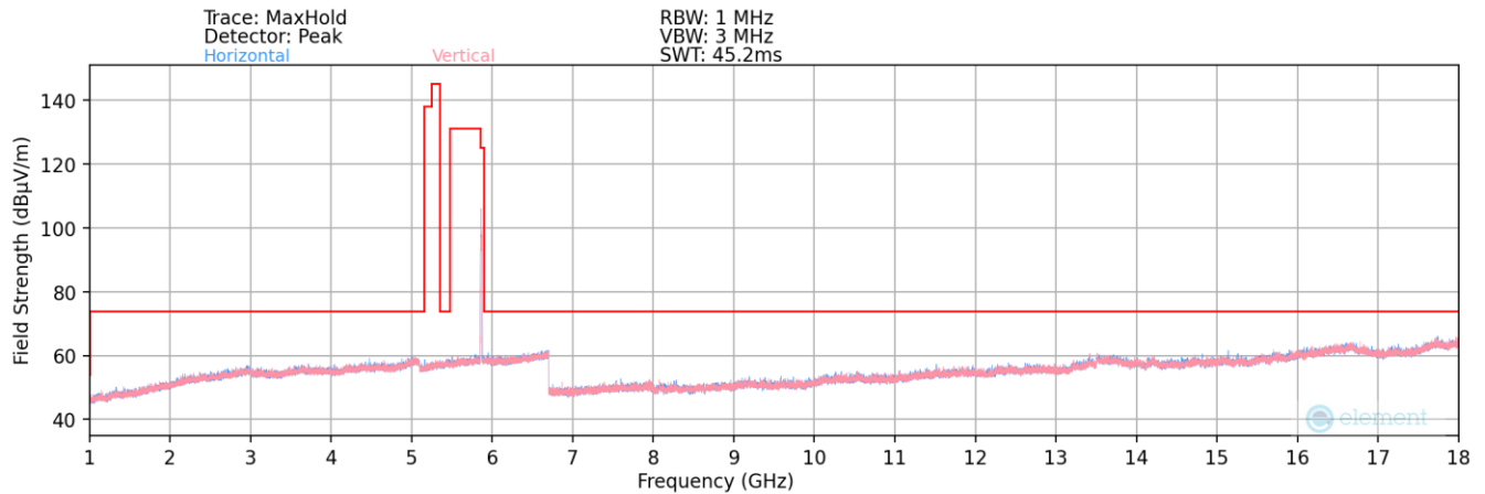
Plot 7-163. Radiated Spurious Plot above 1GHz MIMO (802.11ax – UNII 4 Ch. 173)
