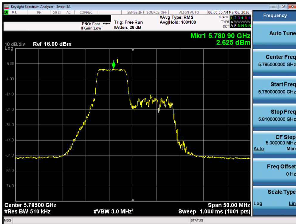
Plot 7-154. Power Spectral Density Plot MIMO ANT2 (20MHz BW 802.11be – 52+26 Tones (UNII Band 3) – Ch. 157)
