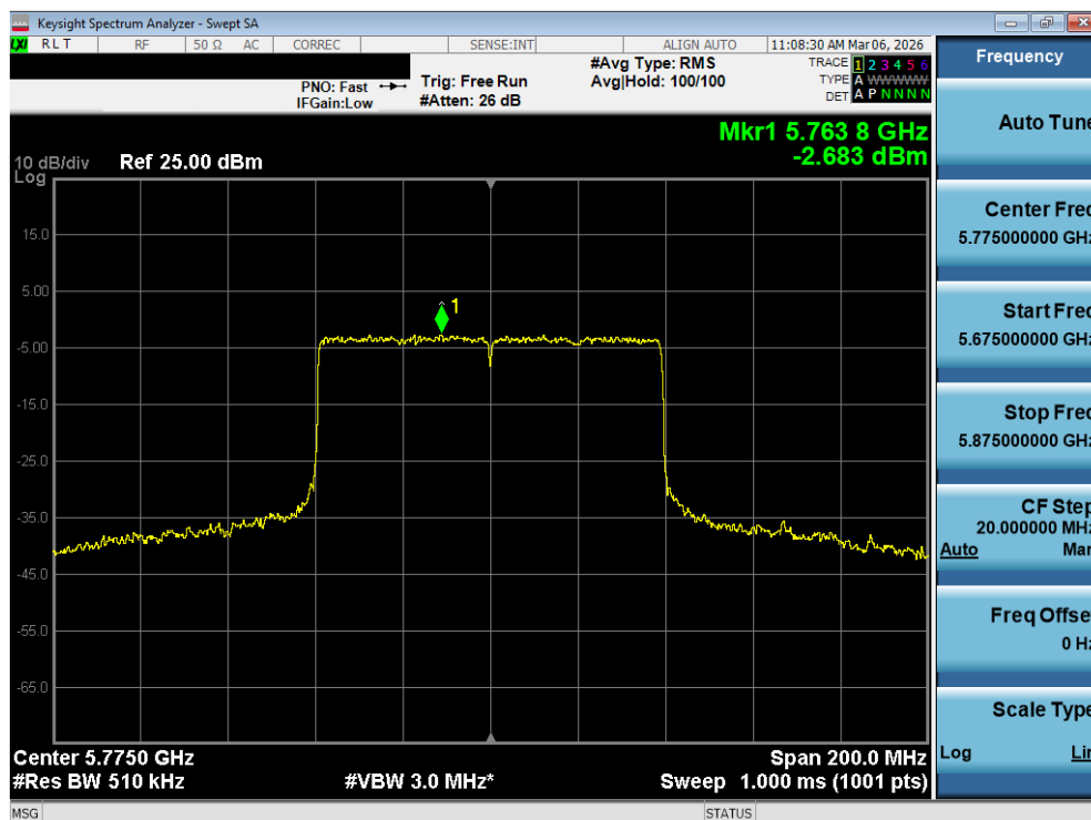
Plot 7-116. Power Spectral Density Plot MIMO ANT1 (80MHz BW 802.11be – 996 Tones (UNII Band 3) – Ch. 155)
