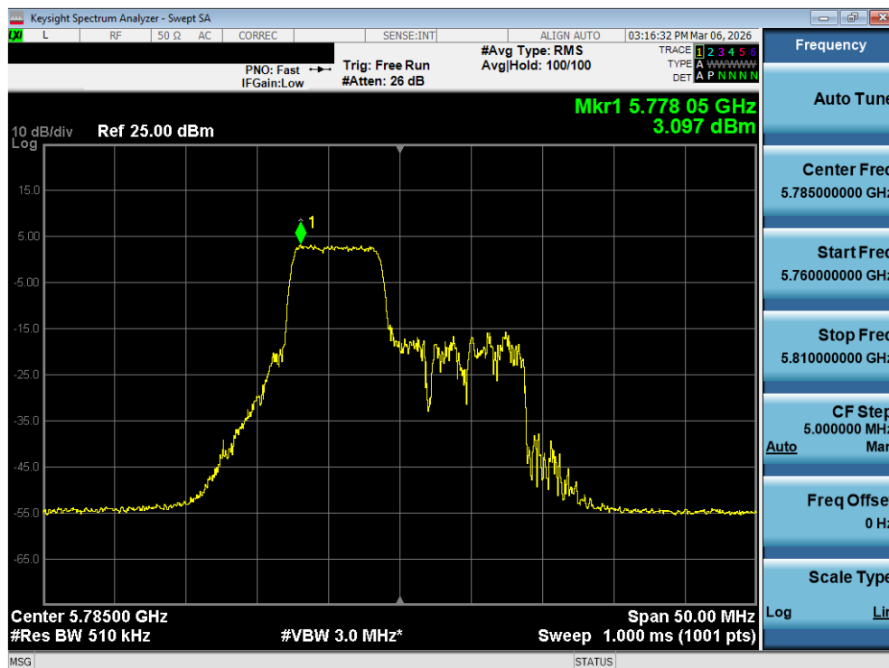
Plot 7-124. Power Spectral Density Plot MIMO ANT1 (20MHz BW 802.11be – 52+26 Tones (UNII Band 3) – Ch. 157)
