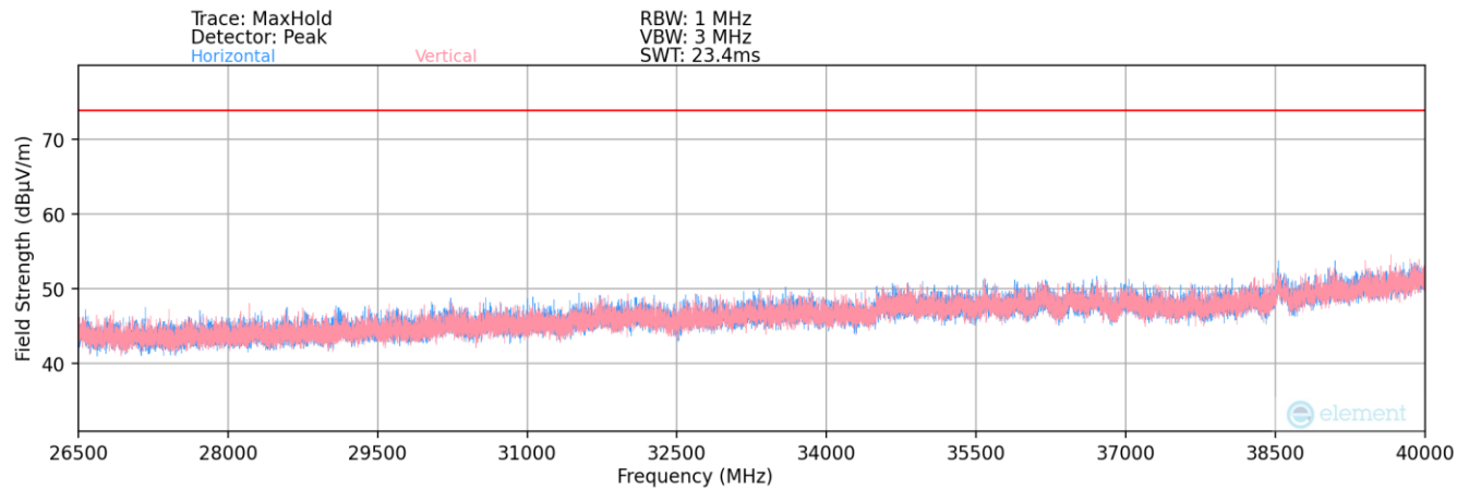
Plot 7-165. Radiated Spurious Plot 26.5GHz - 40GHz (802.11ax)
