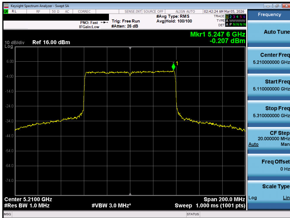
Plot 7-112. Power Spectral Density Plot MIMO ANT1 (80MHz BW 802.11be – 996 Tones (UNII Band 1) – Ch. 42)
