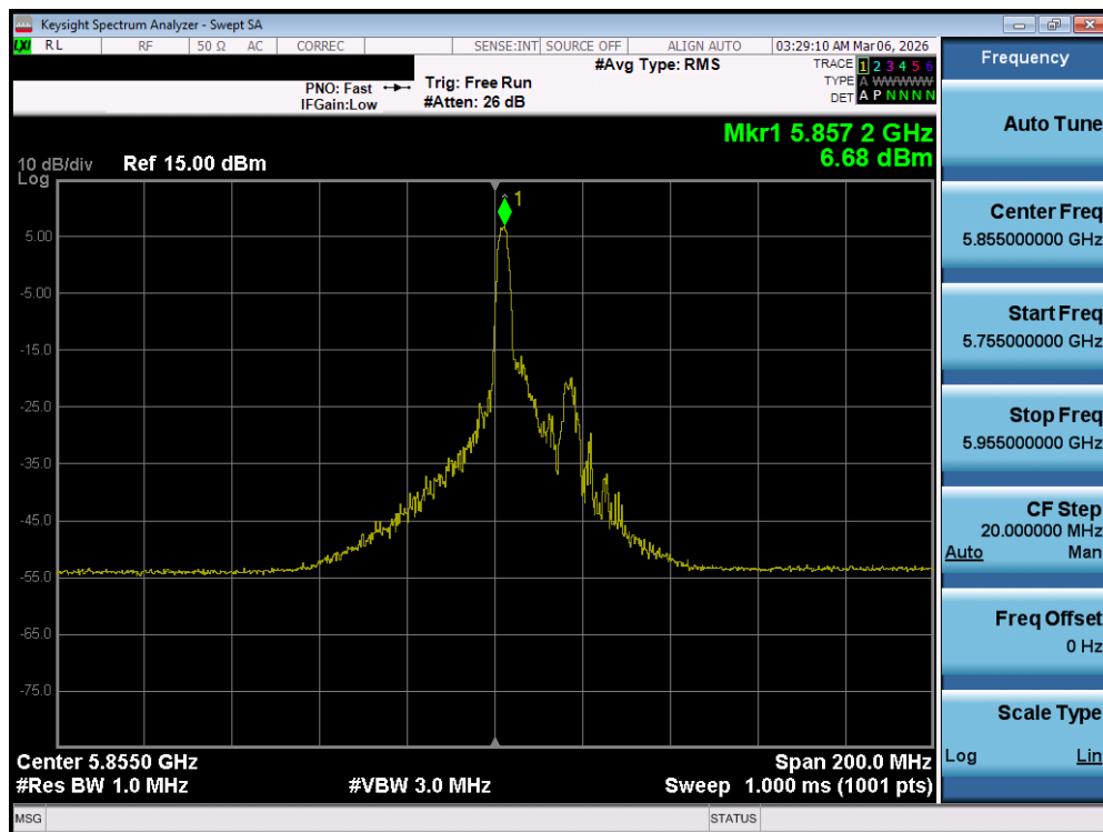
Plot 7-138. Power Spectral Density Plot MIMO ANT2 (80MHz BW 802.11be – 26 Tones (UNII Band 3/4) – Ch. 171)
