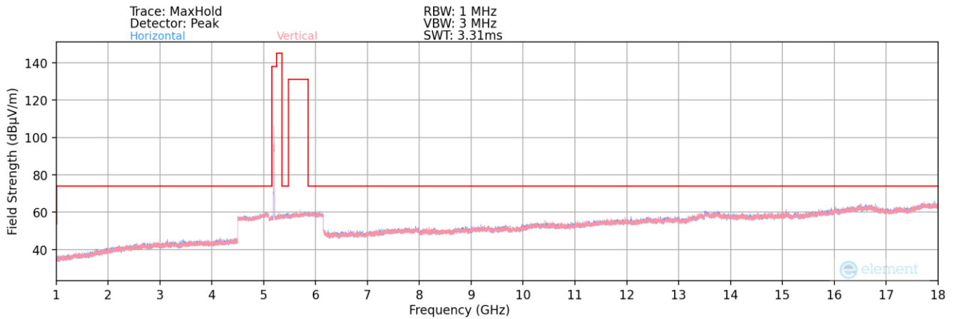
Plot 7-159. Radiated Spurious Plot above 1GHz MIMO (802.11ax – UNII 1 Ch. 40)
