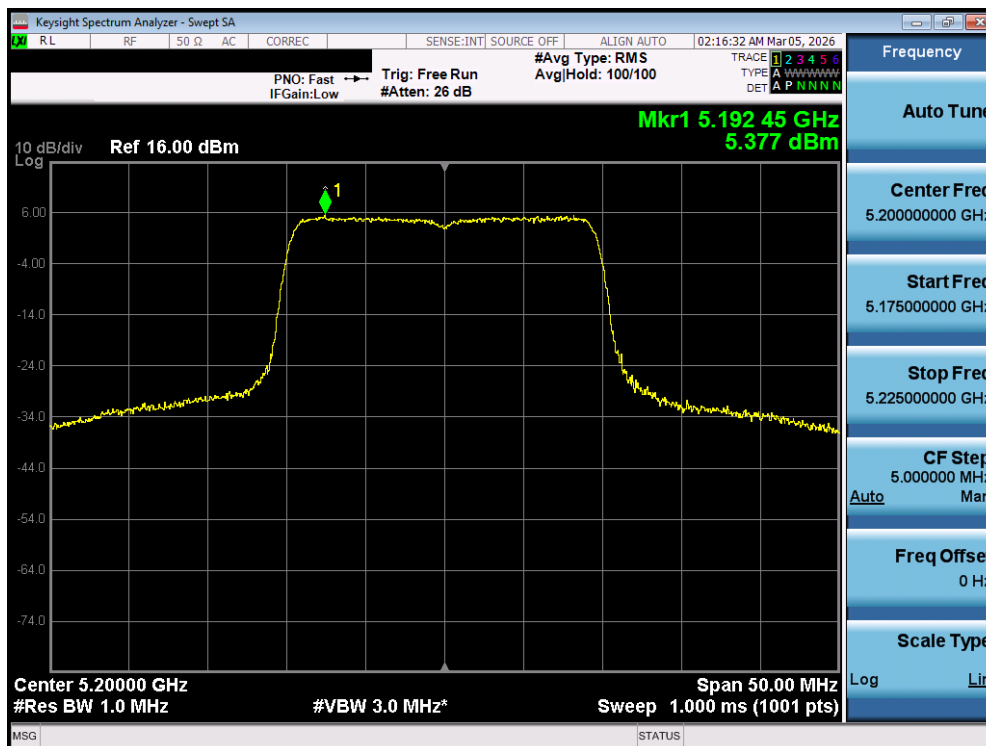
Plot 7-110. Power Spectral Density Plot MIMO ANT1 (20MHz BW 802.11be – 242 Tones (UNII Band 1) – Ch. 40)
