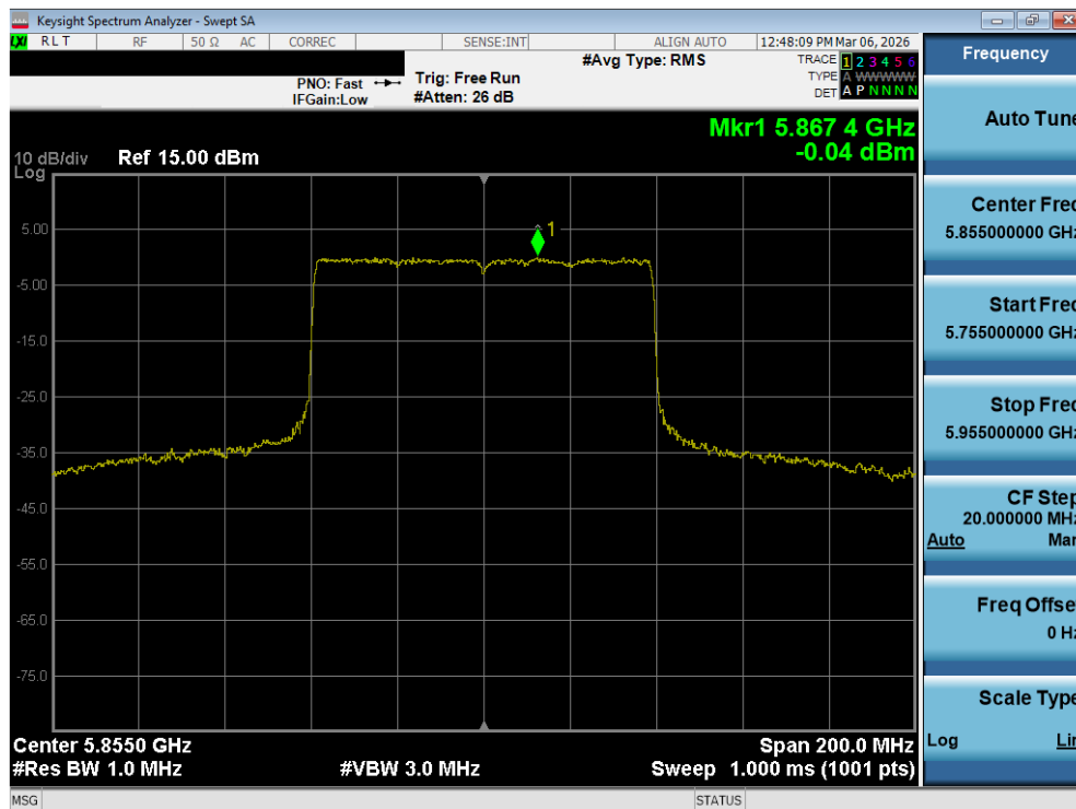
Plot 7-119. Power Spectral Density Plot MIMO ANT1 (80MHz BW 802.11be – 996 Tones (UNII Band 3/4) – Ch. 171)
