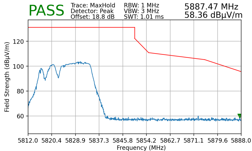
Plot 7-183. Radiated Upper Band Edge Plot MIMO (Peak – UNII Band 3 – 106+26 Tones)
