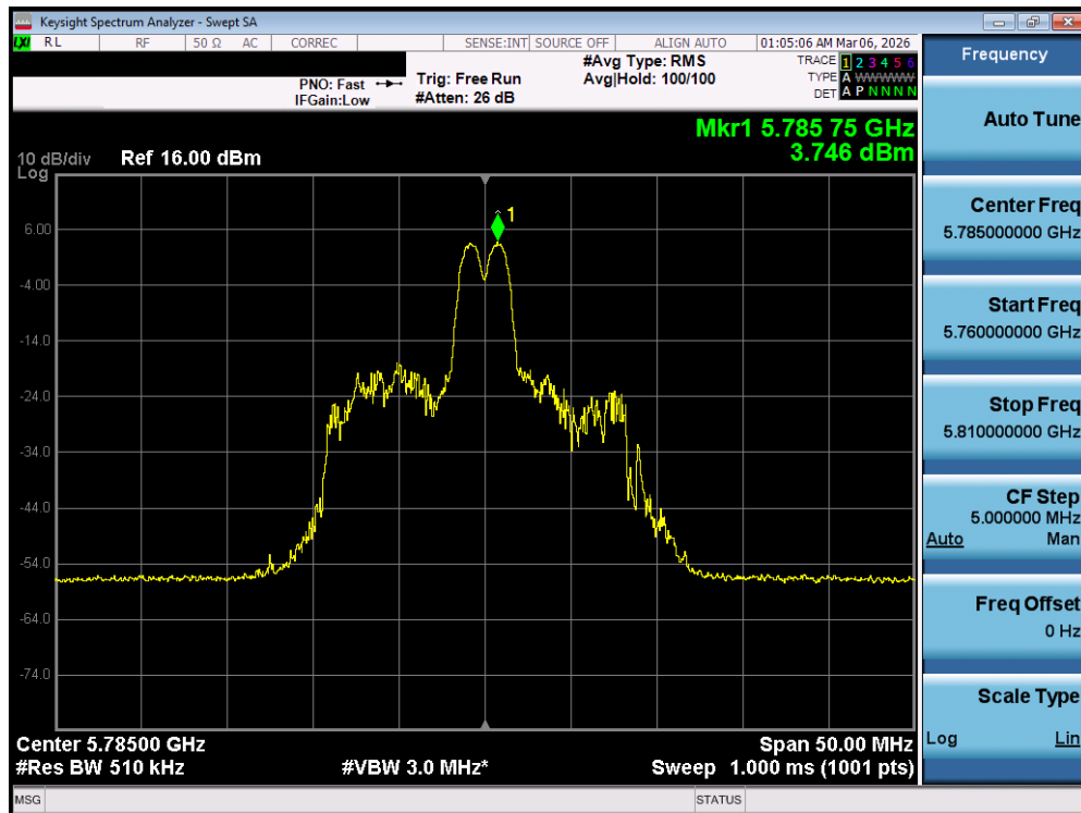
Plot 7-133. Power Spectral Density Plot MIMO ANT2 (20MHz BW 802.11be – 26 Tones (UNII Band 3) – Ch. 157)
