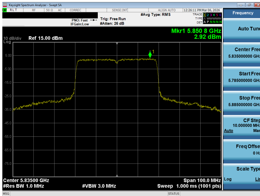
Plot 7-118. Power Spectral Density Plot MIMO ANT1 (40MHz BW 802.11be – 484 Tones (UNII Band 3/4) – Ch. 167)
