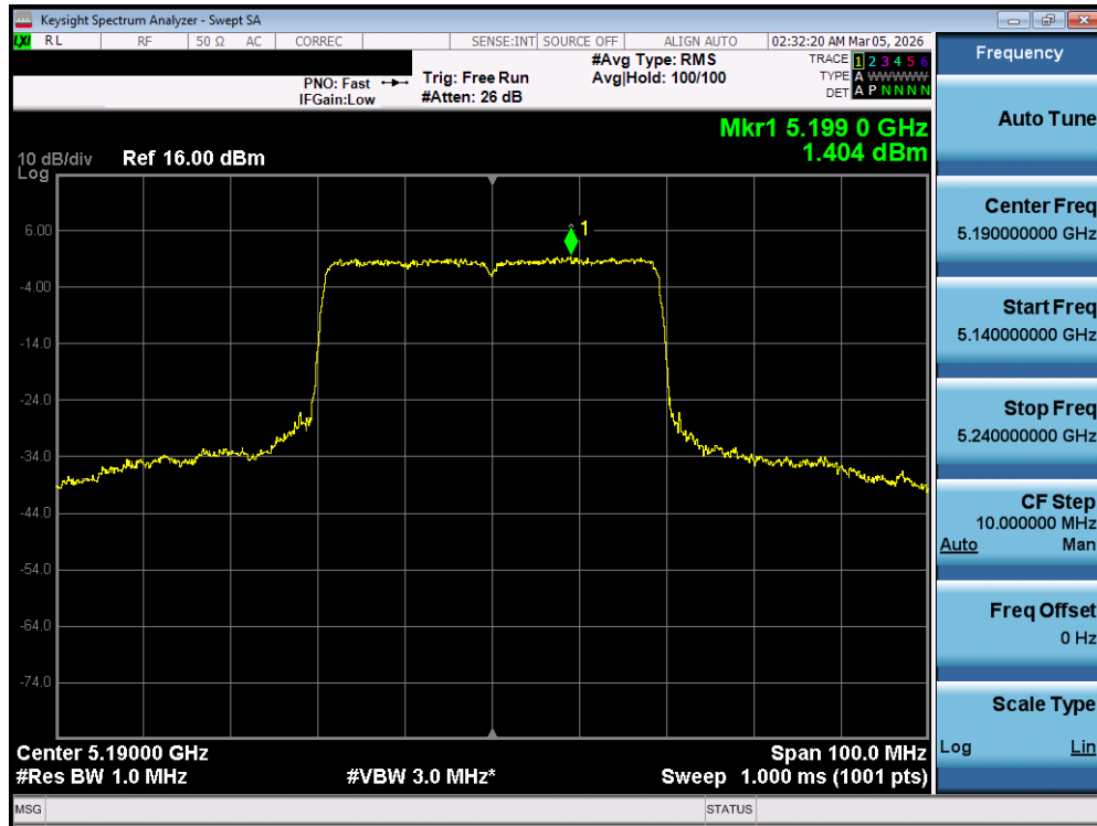
Plot 7-111. Power Spectral Density Plot MIMO ANT1 (40MHz BW 802.11be – 484 Tones (UNII Band 1) – Ch. 38)
