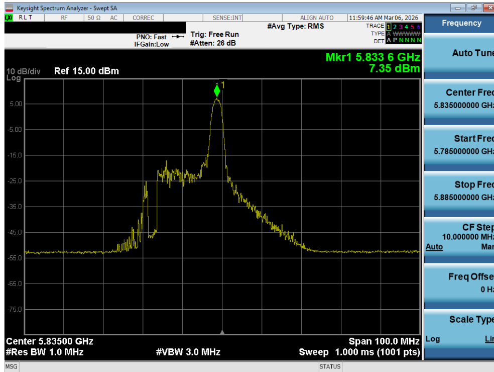
Plot 7-107. Power Spectral Density Plot MIMO ANT1 (40MHz BW 802.11be – 26 Tones (UNII Band 3/4) – Ch. 167)
