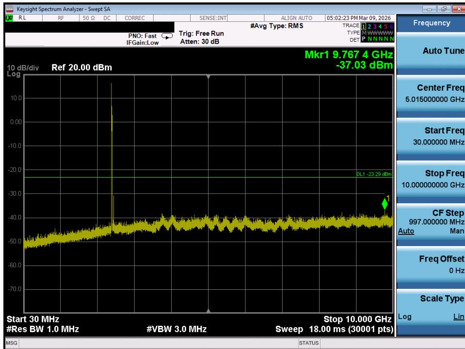
Plot 7-81. Conducted Spurious Plot MIMO ANT1 (802.11ax/be OFDMA – 26 Tones – Ch. 1)
