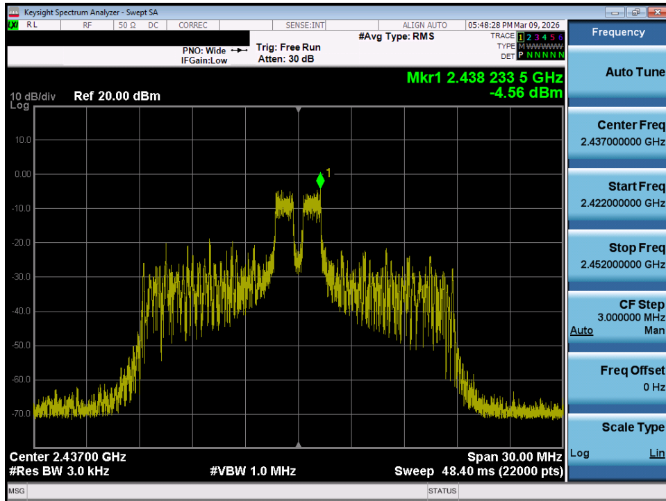
Plot 7-47. Power Spectral Density Plot MIMO ANT2 (802.11ax/be OFDMA – 26 Tones – Ch. 6)
