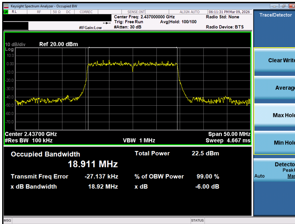
Plot 7-5. 6dB Bandwidth Plot MIMO ANT1 (802.11ax/be OFDMA – 242 Tones – Ch. 6)
