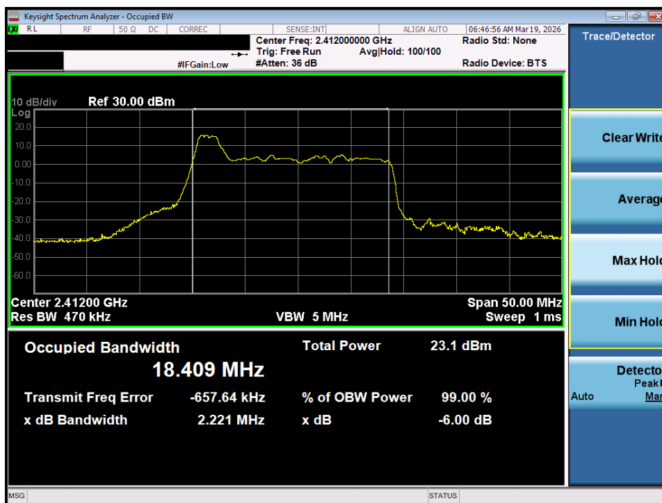
Plot 7-13. OBW Plot MIMO ANT1 (802.11ax/be OFDMA – 26 Tones – Ch. 1)
