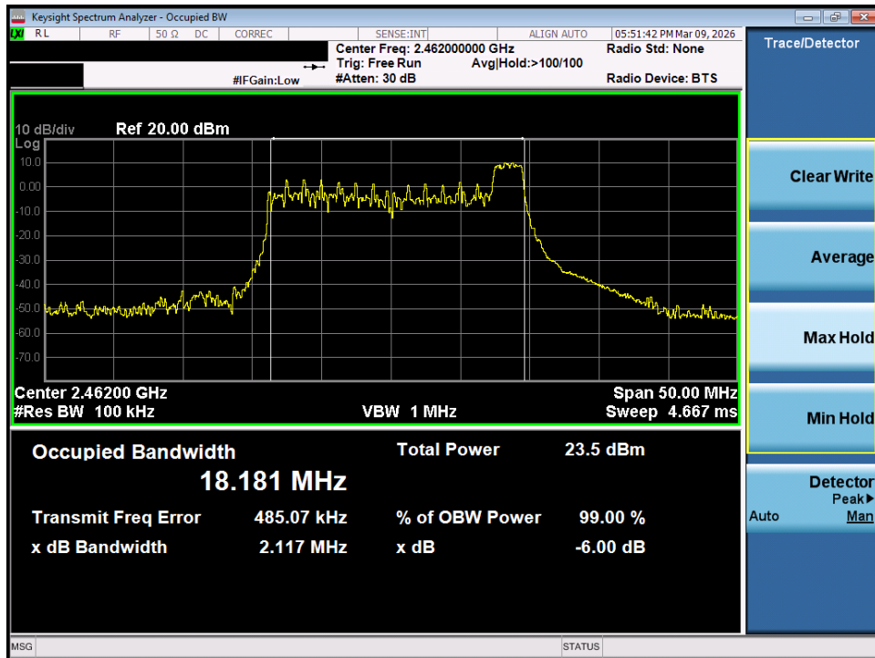
Plot 7-9. 6dB Bandwidth Plot MIMO ANT2 (802.11ax/be OFDMA – 26 Tones – Ch. 11)
