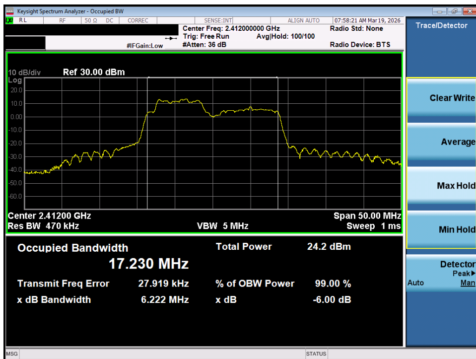
Plot 7-28. OBW Plot MIMO ANT2 (802.11be OFDMA – 52+26 Tones – Ch. 1)
