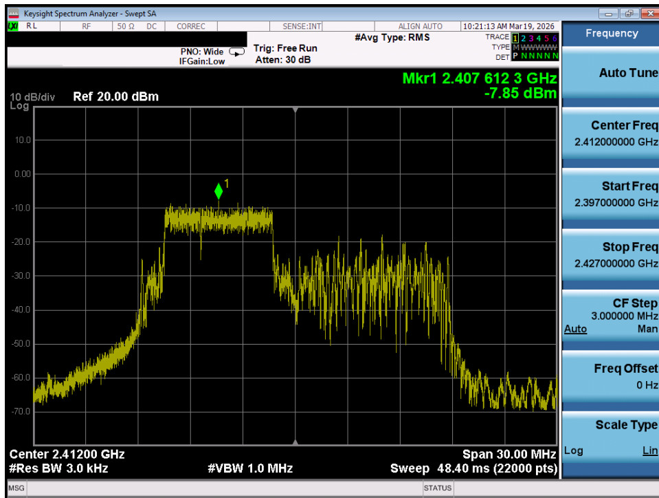
Plot 7-49. Power Spectral Density Plot MIMO ANT2 (802.11be OFDMA – 52+26 Tones – Ch. 1)
