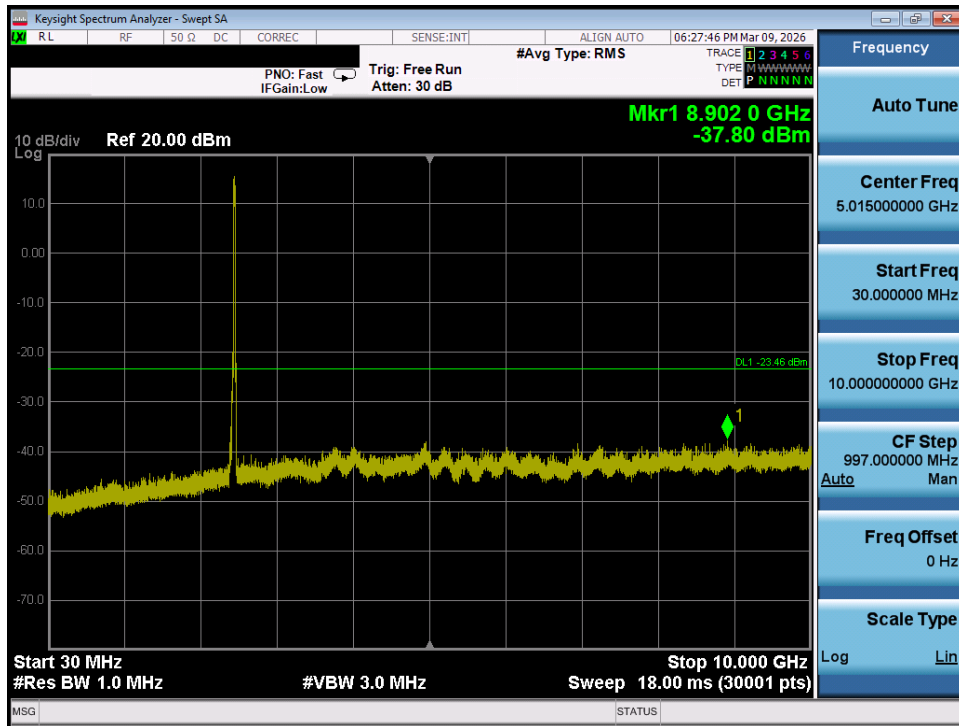
Plot 7-91. Conducted Spurious Plot MIMO ANT2 (802.11ax/be OFDMA – 242 Tones – Ch. 11)
