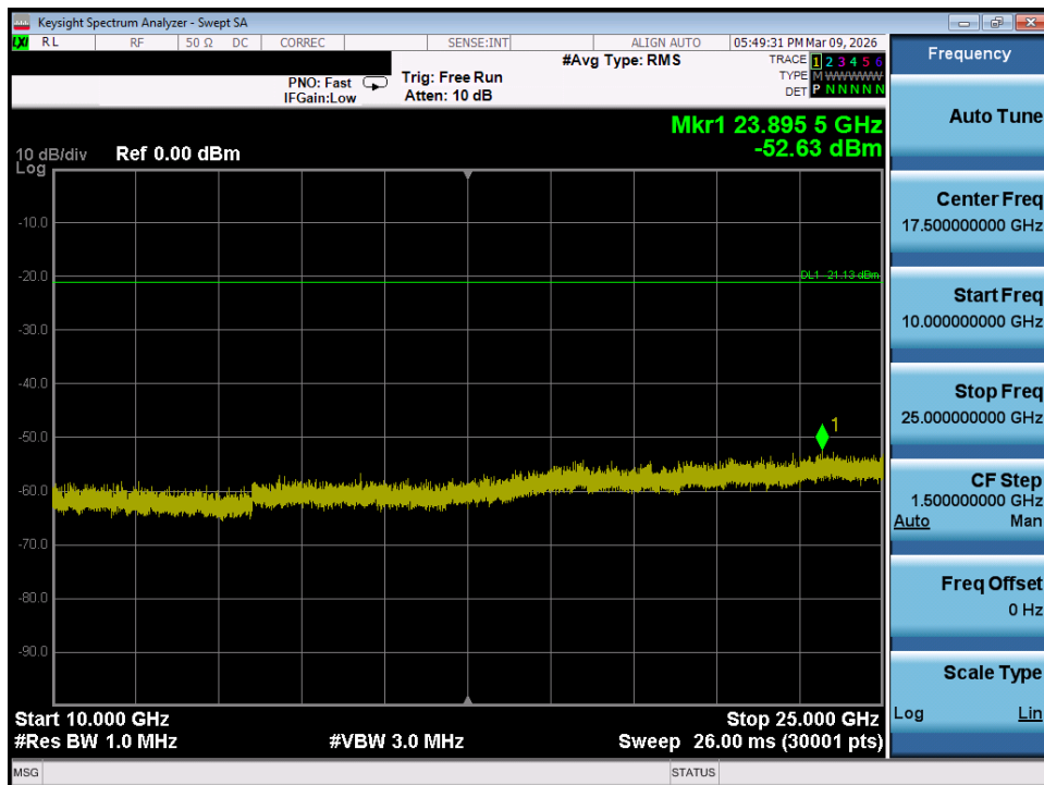
Plot 7-84. Conducted Spurious Plot MIMO ANT2 (802.11ax/be OFDMA – 26 Tones – Ch. 6)
