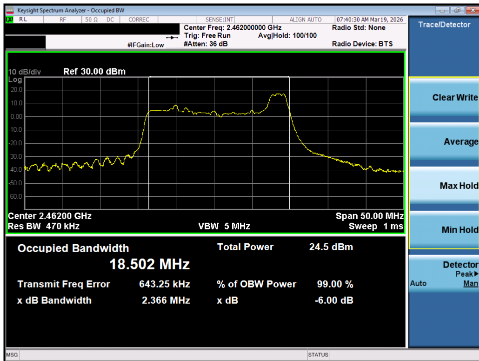
Plot 7-27. OBW Plot MIMO ANT2 (802.11ax/be OFDMA – 26 Tones – Ch. 11)
