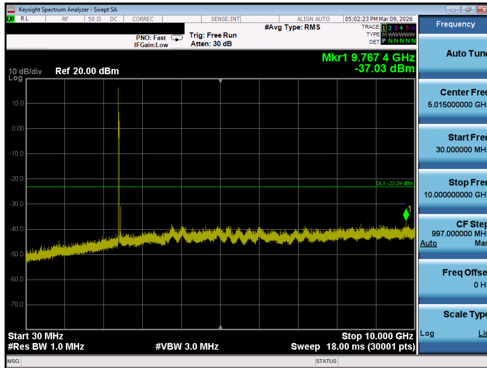
Plot 7-69. Conducted Spurious Plot MIMO ANT1 (802.11ax/be OFDMA – 26 Tones – Ch. 1)
