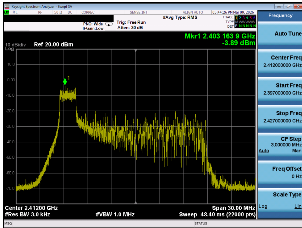
Plot 7-46. Power Spectral Density Plot MIMO ANT2 (802.11ax/be OFDMA – 26 Tones – Ch. 1)
