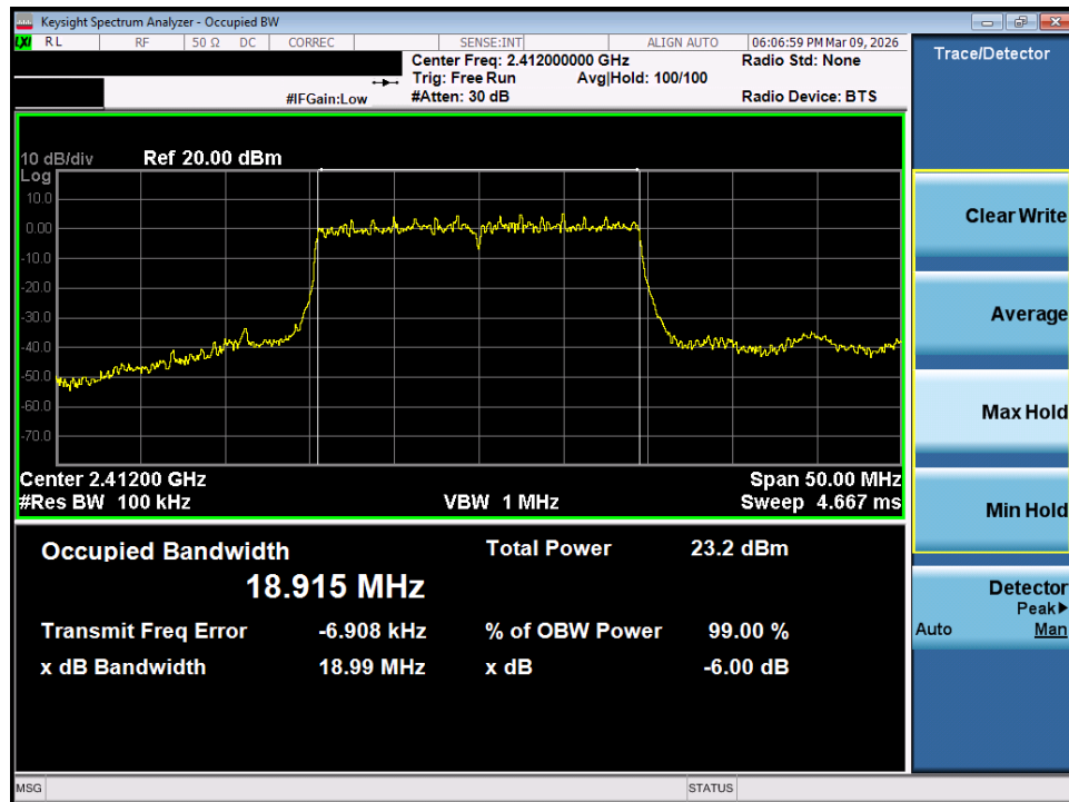
Plot 7-4. 6dB Bandwidth Plot MIMO ANT1 (802.11ax/be OFDMA – 242 Tones – Ch. 1)
