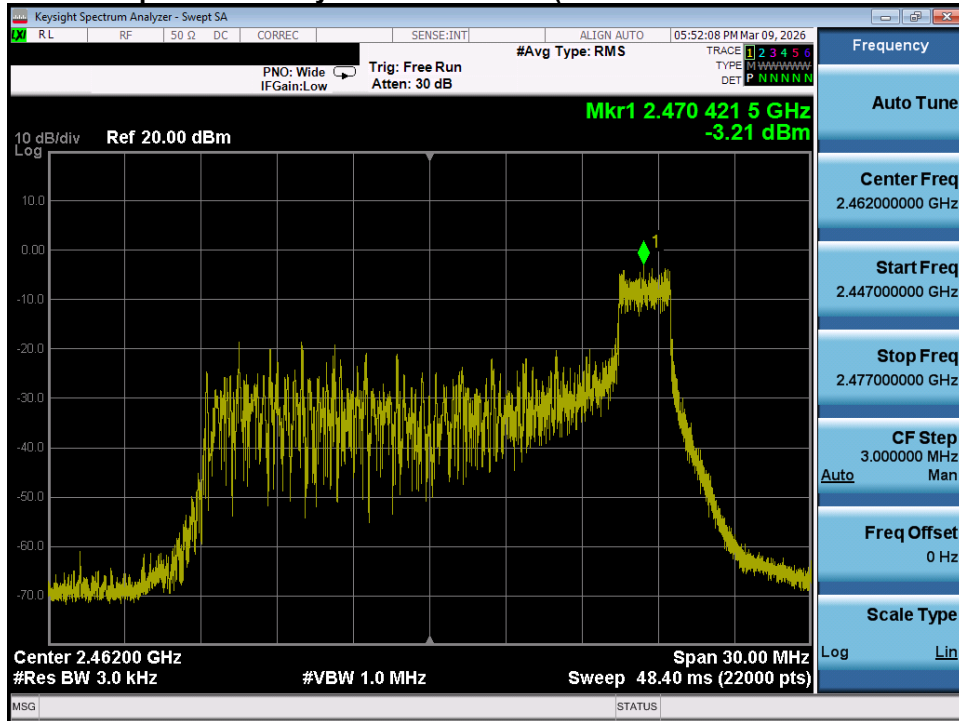
Plot 7-48. Power Spectral Density Plot MIMO ANT2 (802.11ax/be OFDMA – 26 Tones – Ch. 11)
