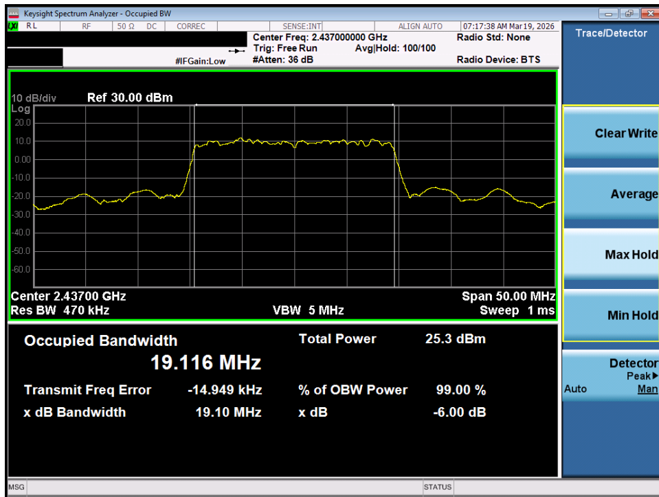
Plot 7-23. OBW Plot MIMO ANT1 (802.11ax/be OFDMA – 242 Tones – Ch. 6)
