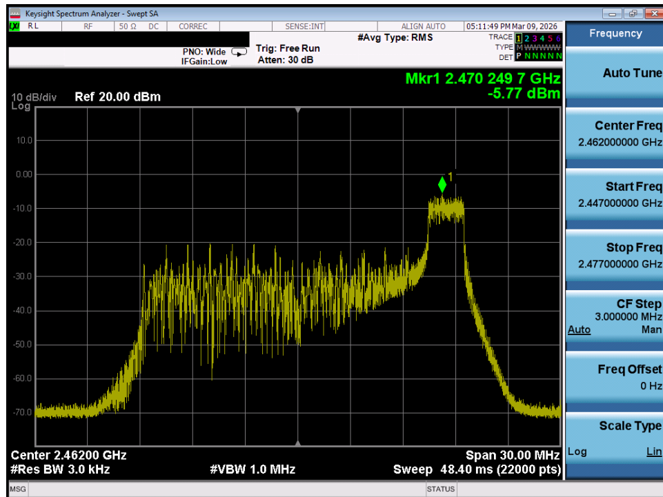
Plot 7-39. Power Spectral Density Plot MIMO ANT1 (802.11ax/be OFDMA – 26 Tones – Ch. 11)
