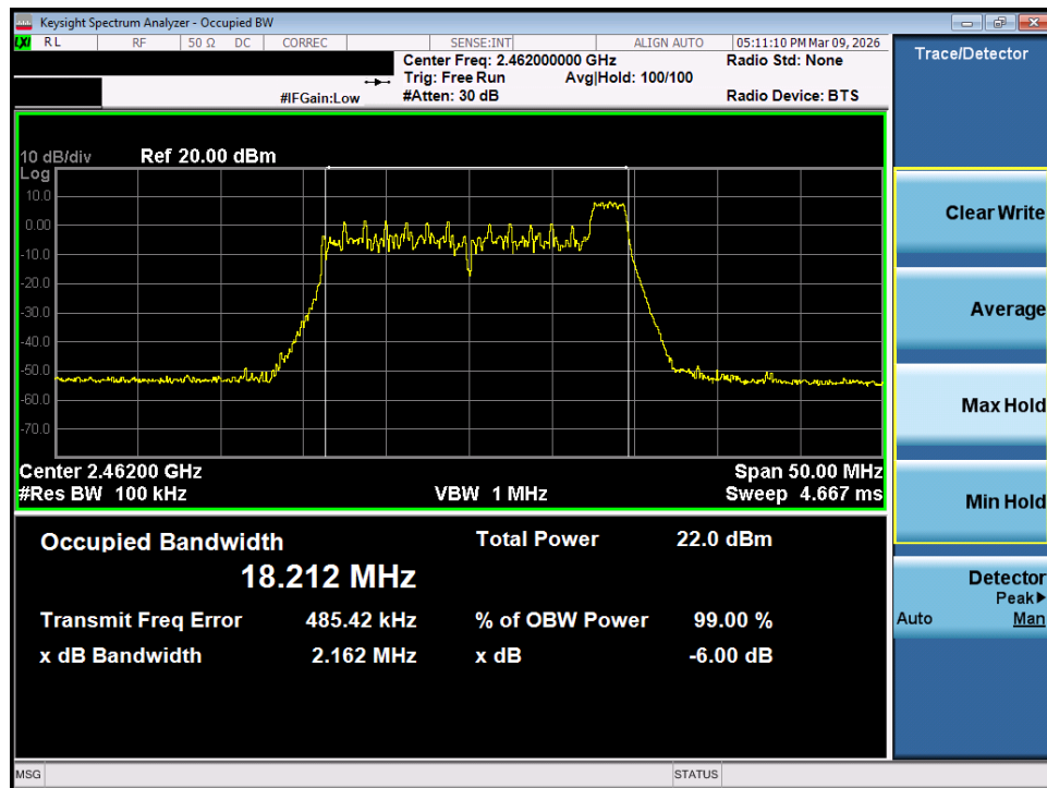
Plot 7-3. 6dB Bandwidth Plot MIMO ANT1 (802.11ax/be OFDMA – 26 Tones – Ch. 11)
