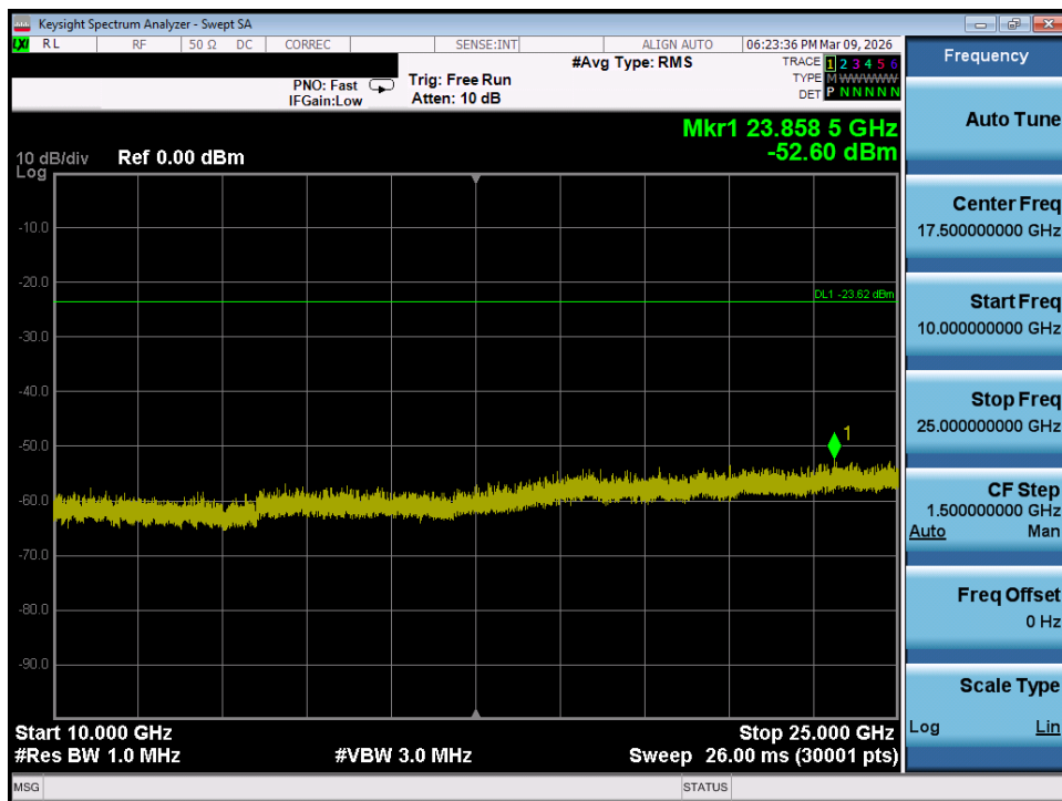
Plot 7-88. Conducted Spurious Plot MIMO ANT2 (802.11ax/be OFDMA – 242 Tones – Ch. 1)
