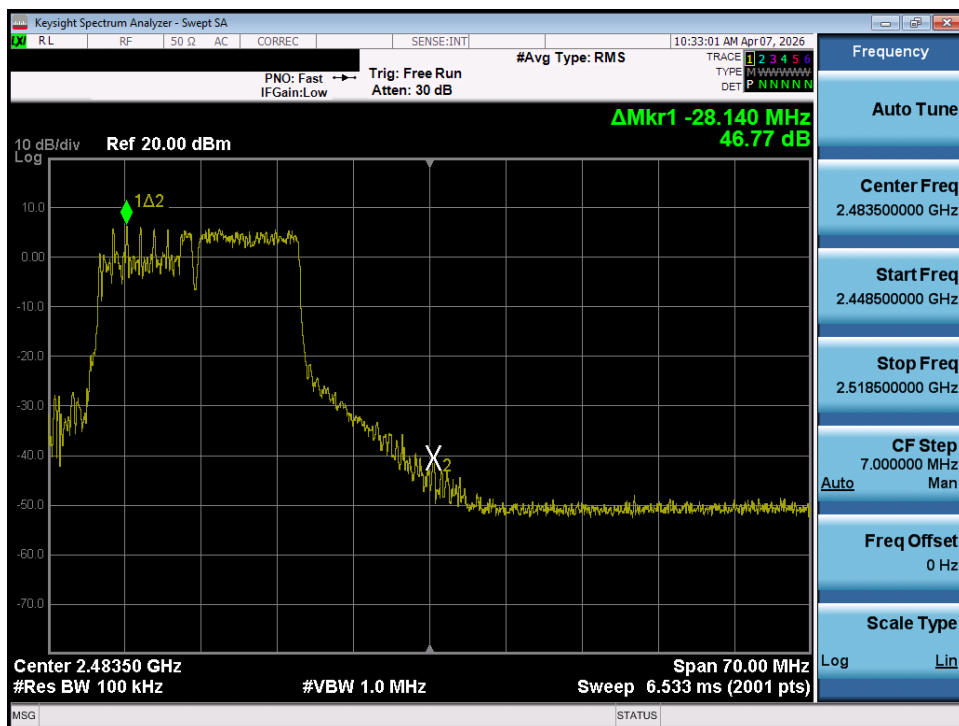
Plot 7-58. Band Edge Plot MIMO ANT1 (802.11be OFDMA – 106+26 Tones – Ch. 11)
