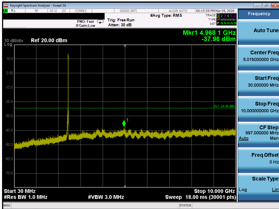
Plot 7-79. Conducted Spurious Plot MIMO ANT1 (802.11ax/be OFDMA – 242 Tones – Ch. 11)
