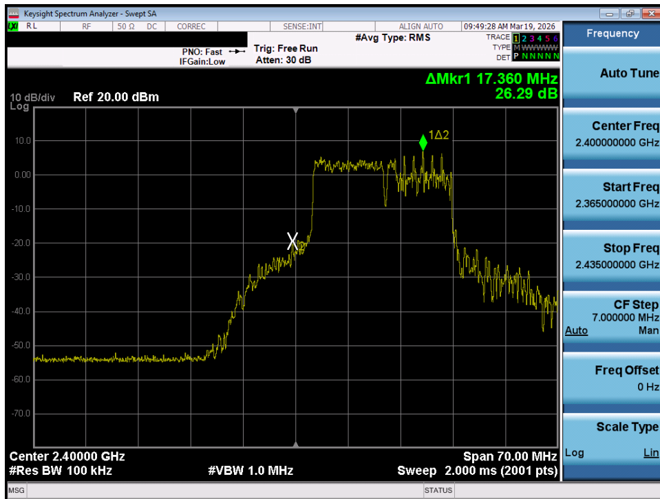
Plot 7-64. Band Edge Plot MIMO ANT2 (802.11be OFDMA – 106 Tones – Ch. 1)
