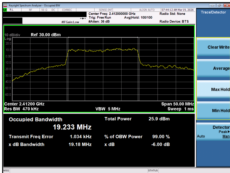
Plot 7-34. OBW Plot MIMO ANT2 (802.11ax/be OFDMA – 242 Tones – Ch. 1)
