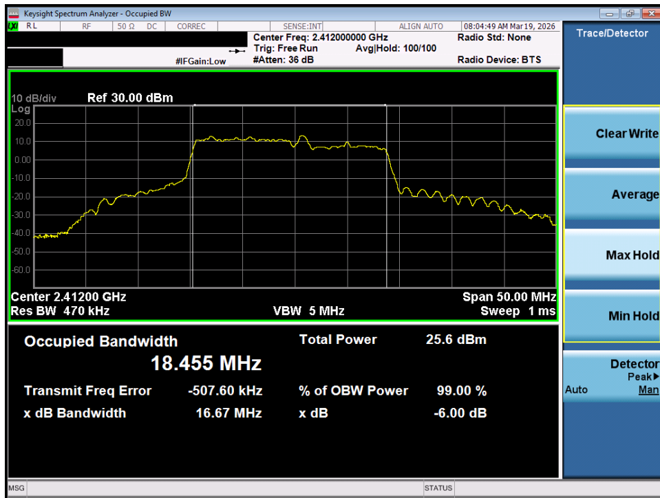
Plot 7-31. OBW Plot MIMO ANT2 (802.11be OFDMA – 106+26 Tones – Ch. 1)
