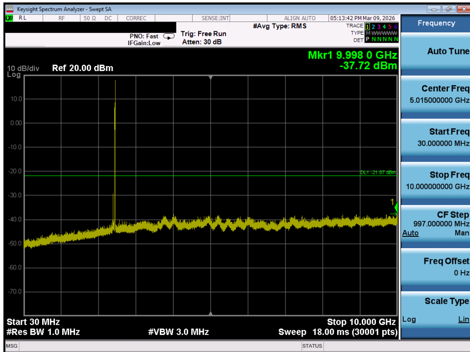
Plot 7-73. Conducted Spurious Plot MIMO ANT1 (802.11ax/be OFDMA – 26 Tones – Ch. 11)
