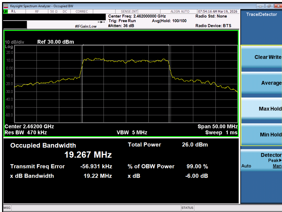
Plot 7-36. OBW Plot MIMO ANT2 (802.11ax/be OFDMA – 242 Tones – Ch. 11)
