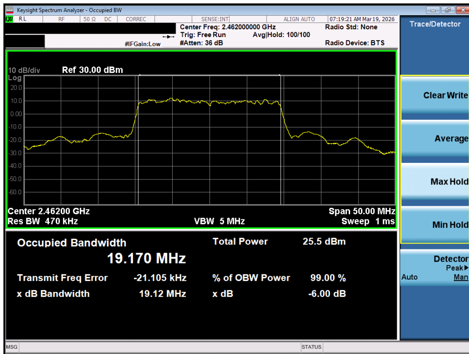
Plot 7-24. OBW Plot MIMO ANT1 (802.11ax/be OFDMA – 242 Tones – Ch. 11)
