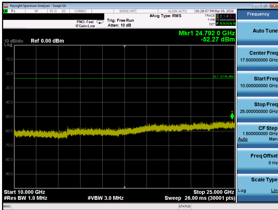
Plot 7-92. Conducted Spurious Plot MIMO ANT2 (802.11ax/be OFDMA – 242 Tones – Ch. 11)
