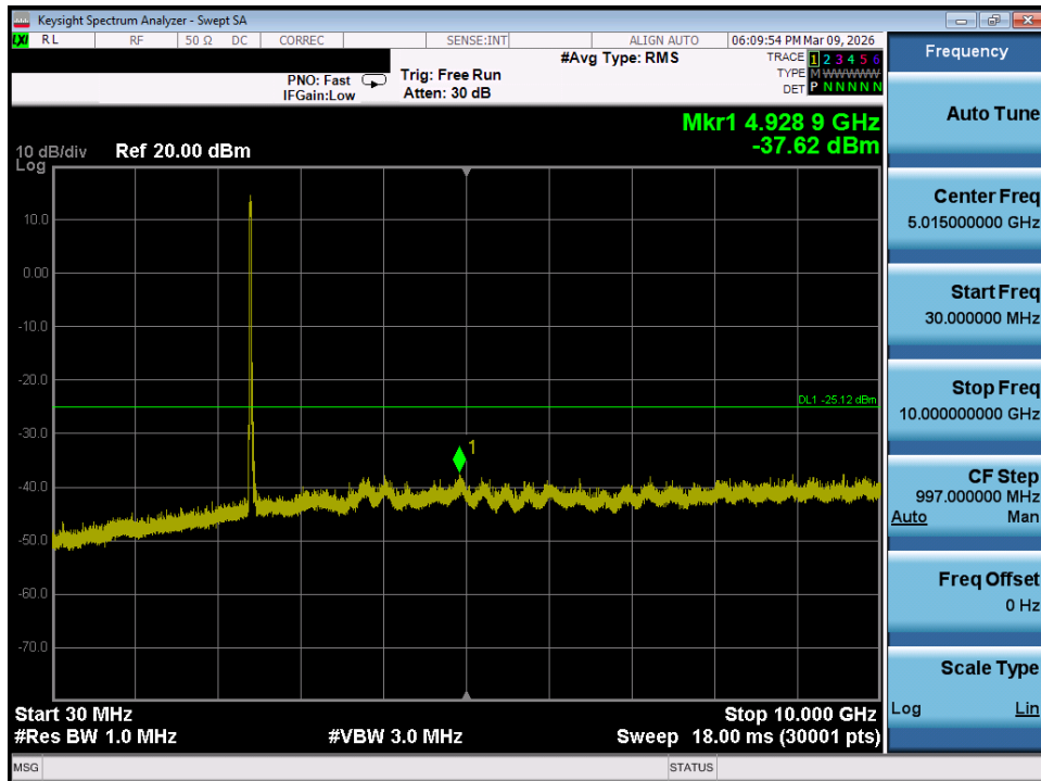
Plot 7-75. Conducted Spurious Plot MIMO ANT1 (802.11ax/be OFDMA – 242 Tones – Ch. 1)
