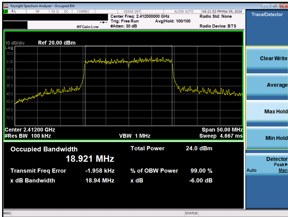
Plot 7-10. 6dB Bandwidth Plot MIMO ANT2 (802.11ax/be OFDMA – 242 Tones – Ch. 1)
