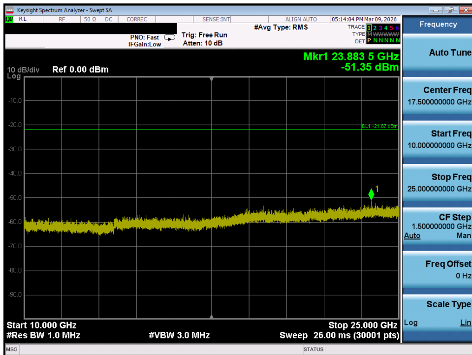
Plot 7-74. Conducted Spurious Plot MIMO ANT1 (802.11ax/be OFDMA – 26 Tones – Ch. 11)
