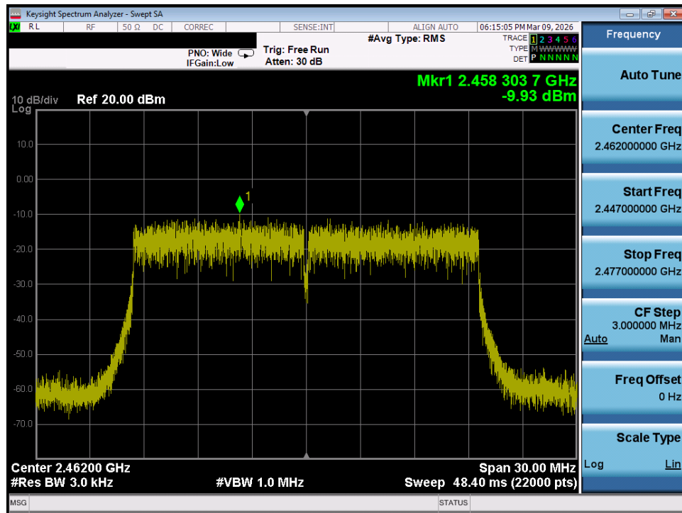
Plot 7-45. Power Spectral Density Plot MIMO ANT1 (802.11ax/be OFDMA – 242 Tones – Ch. 11)
