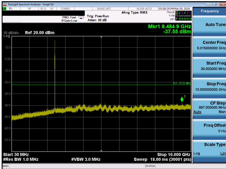
Plot 7-71. Conducted Spurious Plot MIMO ANT1 (802.11ax/be OFDMA – 26 Tones – Ch. 6)
