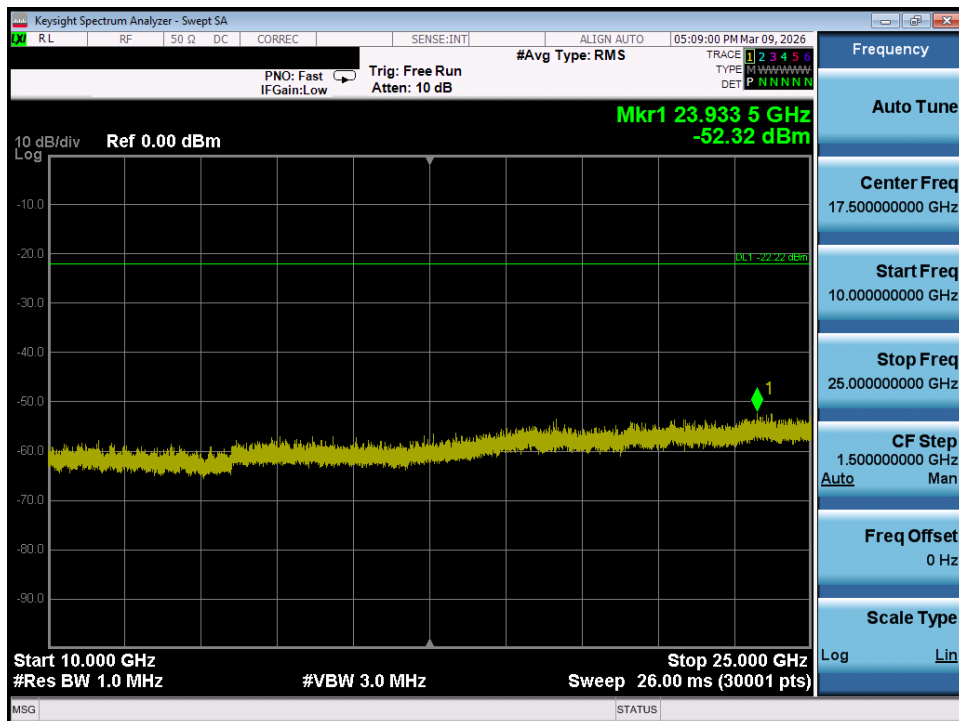
Plot 7-72. Conducted Spurious Plot MIMO ANT1 (802.11ax/be OFDMA – 26 Tones – Ch. 6)
