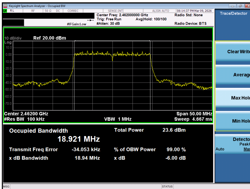
Plot 7-6. 6dB Bandwidth Plot MIMO ANT1 (802.11ax/be OFDMA – 242 Tones – Ch. 11)
