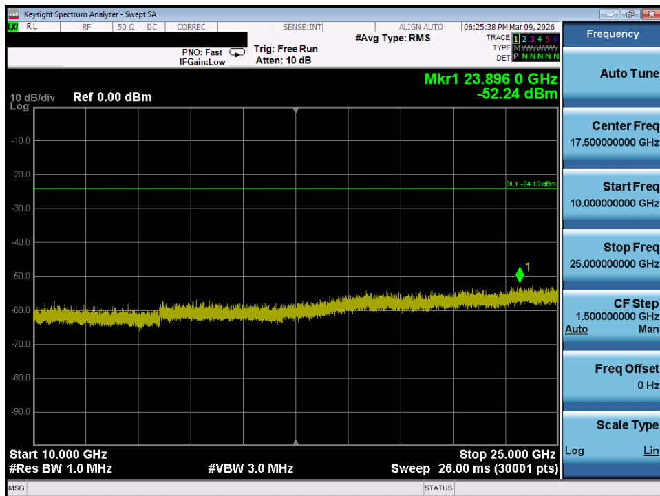
Plot 7-90. Conducted Spurious Plot MIMO ANT2 (802.11ax/be OFDMA – 242 Tones – Ch. 6)
