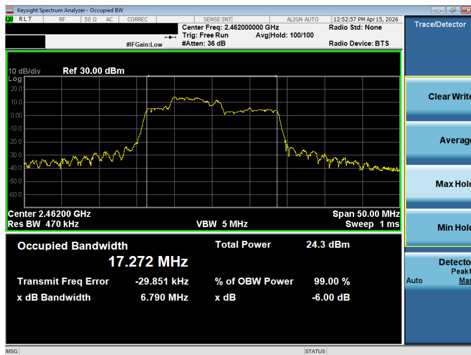
Plot 7-30. OBW Plot MIMO ANT2 (802.11be OFDMA – 52+26 Tones – Ch. 11)
