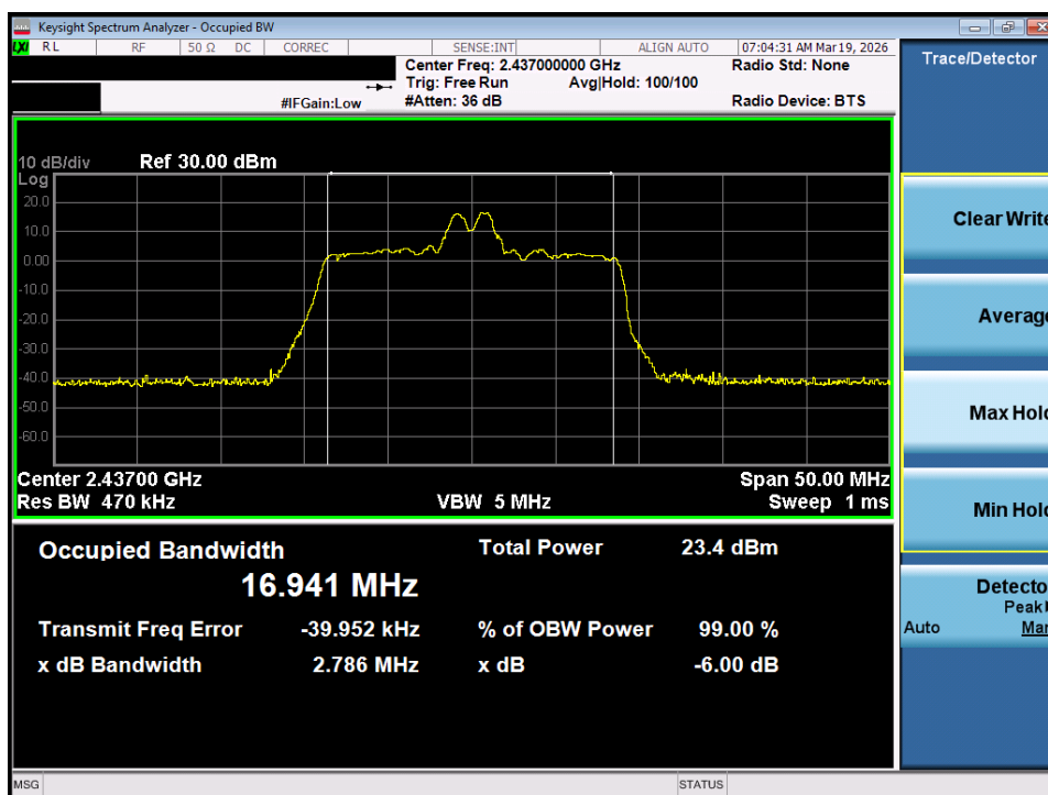
Plot 7-14. OBW Plot MIMO ANT1 (802.11ax/be OFDMA – 26 Tones – Ch. 6)
