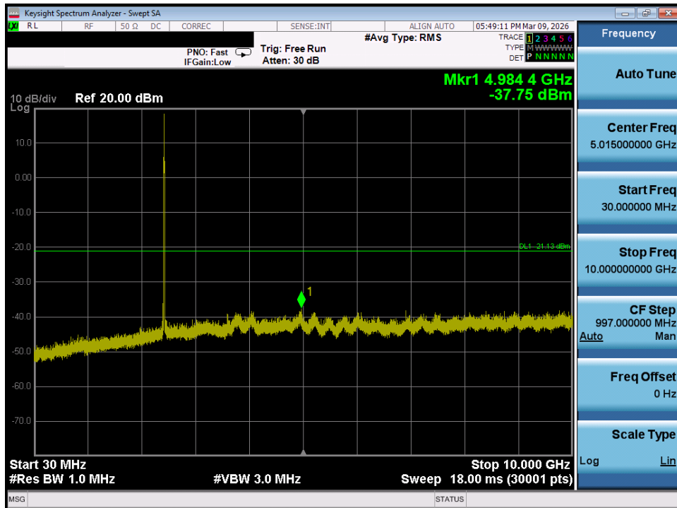
Plot 7-83. Conducted Spurious Plot MIMO ANT2 (802.11ax/be OFDMA – 26 Tones – Ch. 6)
