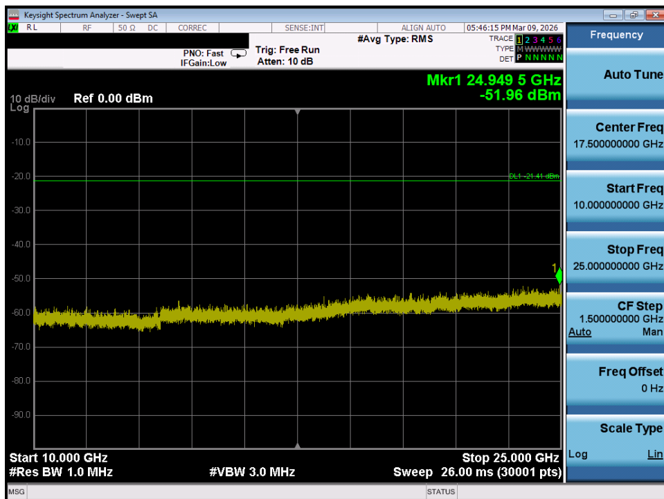
Plot 7-82. Conducted Spurious Plot MIMO ANT2 (802.11ax/be OFDMA – 26 Tones – Ch. 1)
