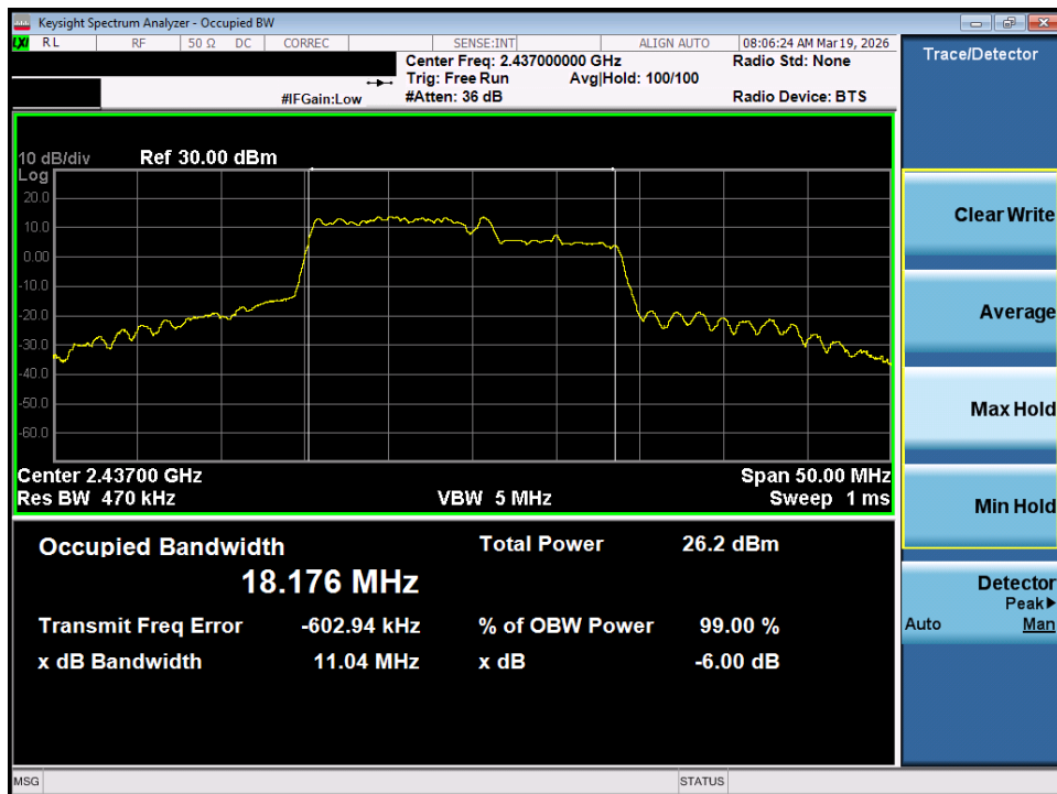
Plot 7-32. OBW Plot MIMO ANT2 (802.11be OFDMA – 106+26 Tones – Ch. 6)
