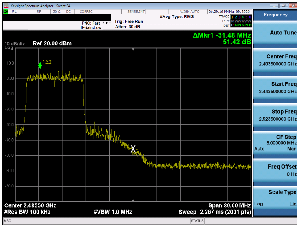
Plot 7-67. Band Edge Plot MIMO ANT2 (802.11ax/be OFDMA – 242 Tones – Ch. 10)
