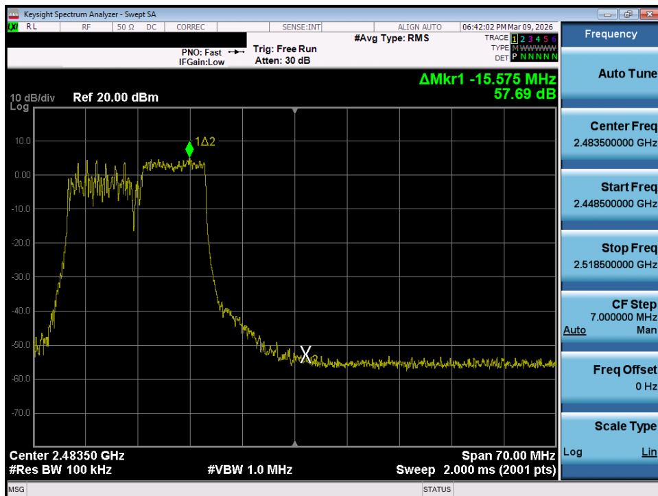
Plot 7-56. Band Edge Plot MIMO ANT1 (802.11ax/be OFDMA – 106 Tones – Ch. 11)
