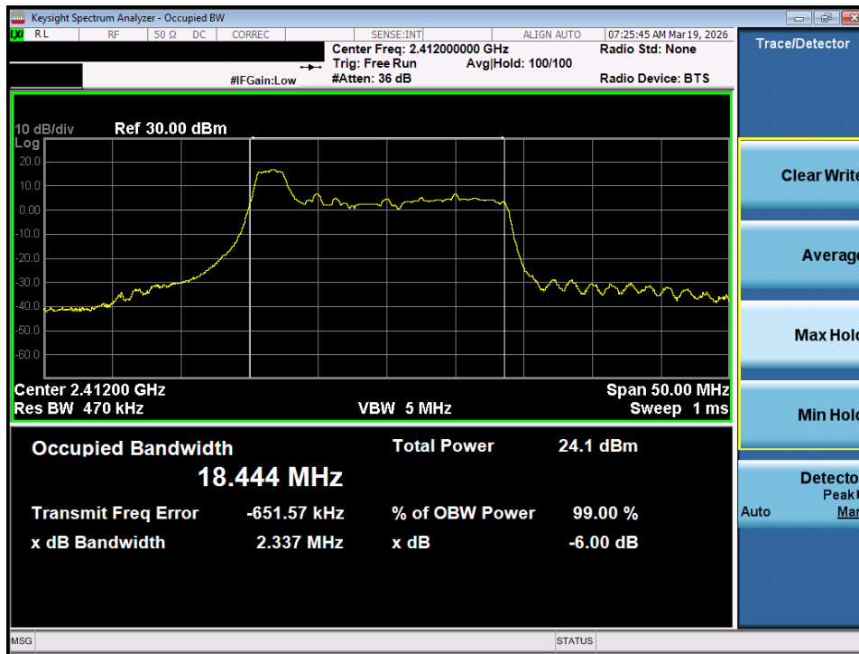
Plot 7-25. OBW Plot MIMO ANT2 (802.11ax/be OFDMA – 26 Tones – Ch. 1)
