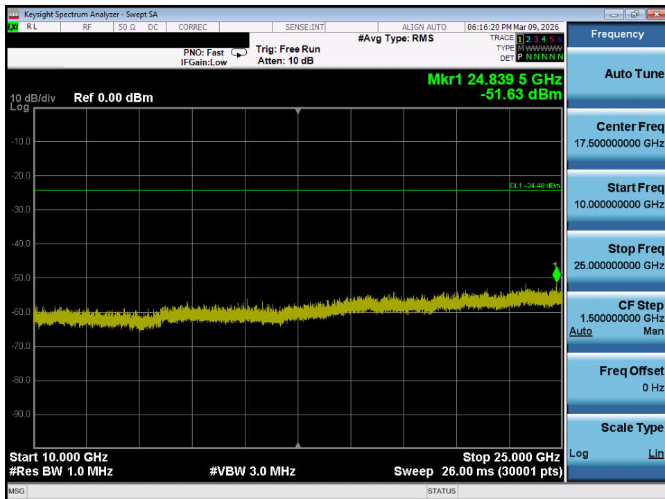
Plot 7-80. Conducted Spurious Plot MIMO ANT1 (802.11ax/be OFDMA – 242 Tones – Ch. 11)
