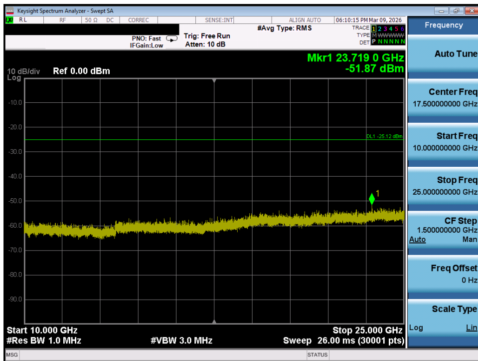
Plot 7-76. Conducted Spurious Plot MIMO ANT1 (802.11ax/be OFDMA – 242 Tones – Ch. 1)
