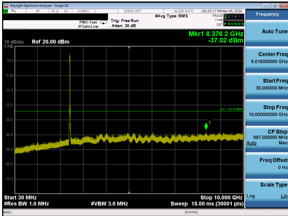
Plot 7-89. Conducted Spurious Plot MIMO ANT2 (802.11ax/be OFDMA – 242 Tones – Ch. 6)
