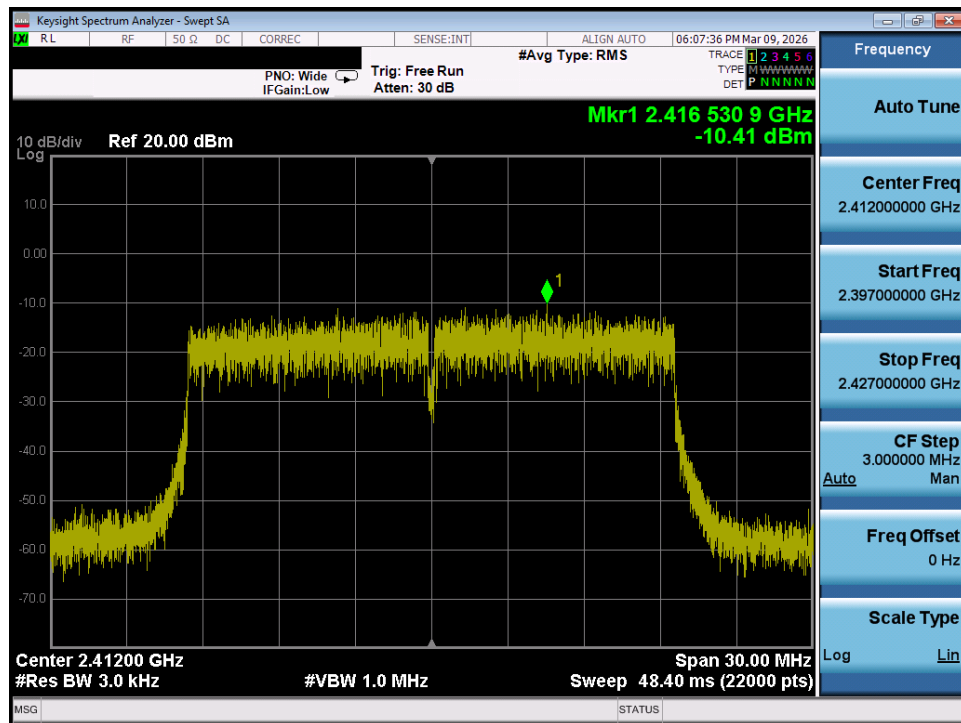
Plot 7-43. Power Spectral Density Plot MIMO ANT1 (802.11ax/be OFDMA – 242 Tones – Ch. 1)
