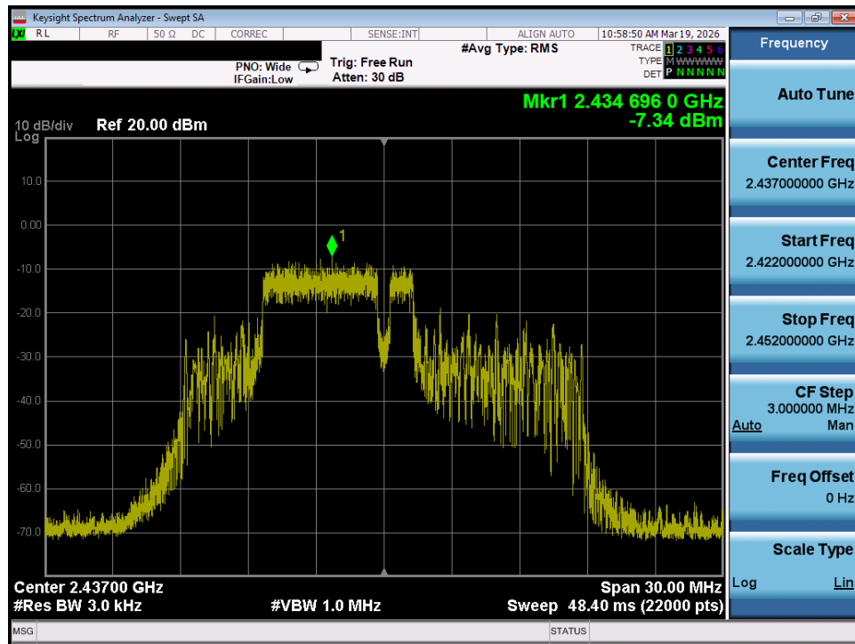
Plot 7-41. Power Spectral Density Plot MIMO ANT1 (802.11be OFDMA – 52+26 Tones – Ch. 6)
