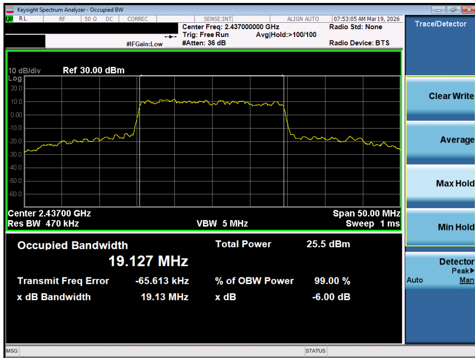
Plot 7-35. OBW Plot MIMO ANT2 (802.11ax/be OFDMA – 242 Tones – Ch. 6)
