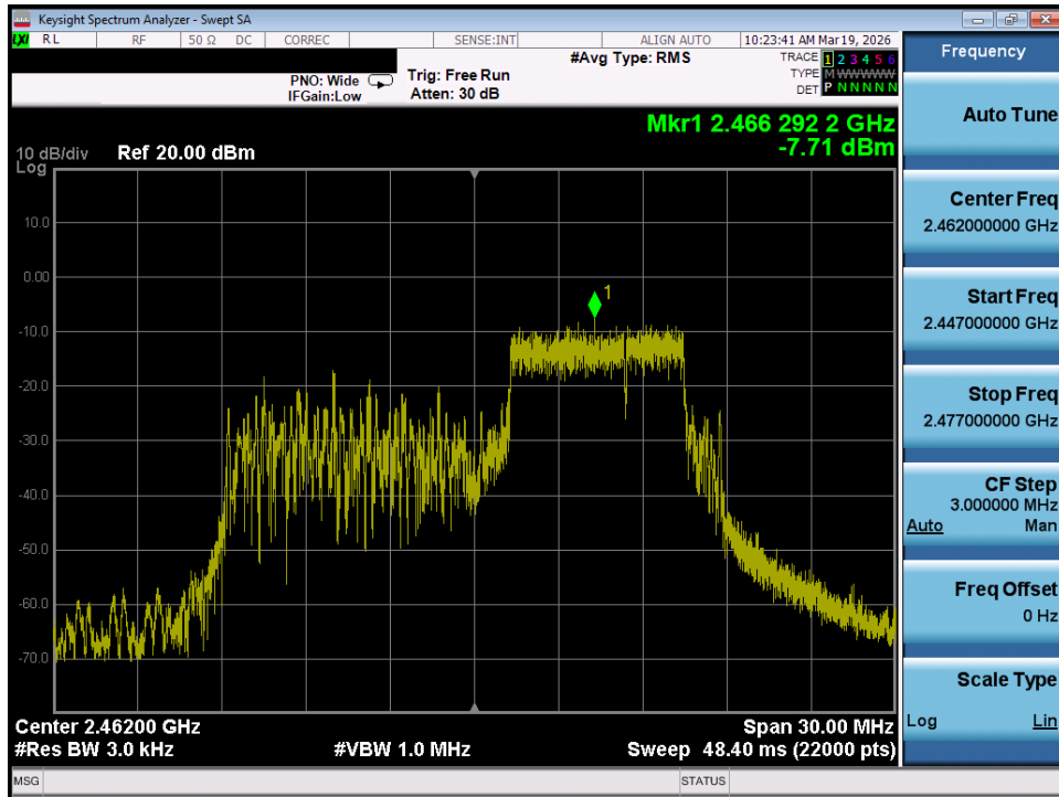
Plot 7-51. Power Spectral Density Plot MIMO ANT2 (802.11be OFDMA – 52+26 Tones – Ch. 11)
