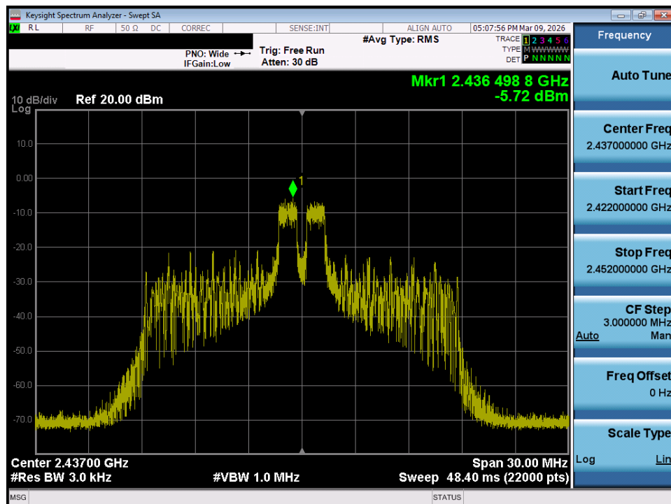
Plot 7-38. Power Spectral Density Plot MIMO ANT1 (802.11ax/be OFDMA – 26 Tones – Ch. 6)
