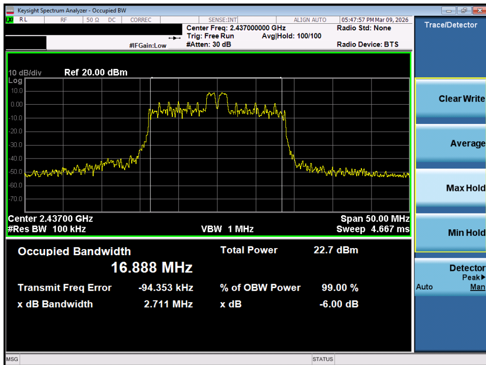
Plot 7-8. 6dB Bandwidth Plot MIMO ANT2 (802.11ax/be OFDMA – 26 Tones – Ch. 6)
