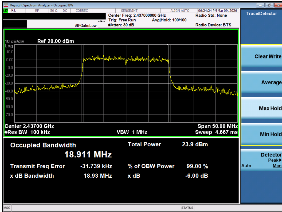
Plot 7-11. 6dB Bandwidth Plot MIMO ANT2 (802.11ax/be OFDMA – 242 Tones – Ch. 6)
