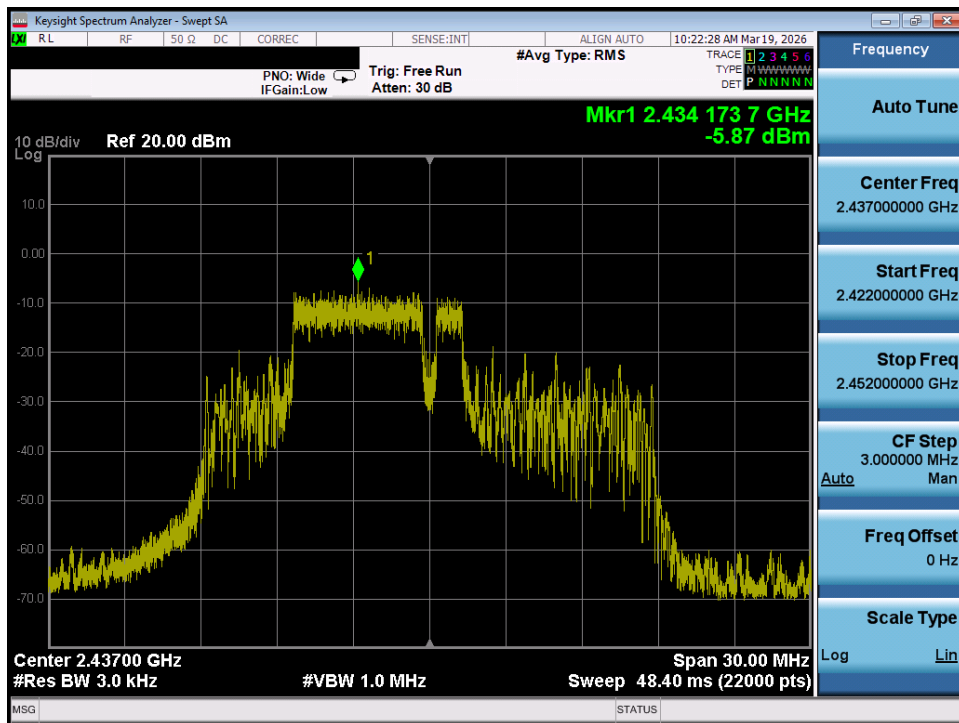
Plot 7-50. Power Spectral Density Plot MIMO ANT2 (802.11be OFDMA – 52+26 Tones – Ch. 6)
