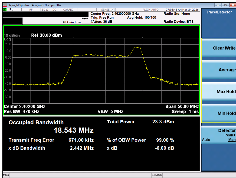
Plot 7-15. OBW Plot MIMO ANT1 (802.11ax/be OFDMA – 26 Tones – Ch. 11)
