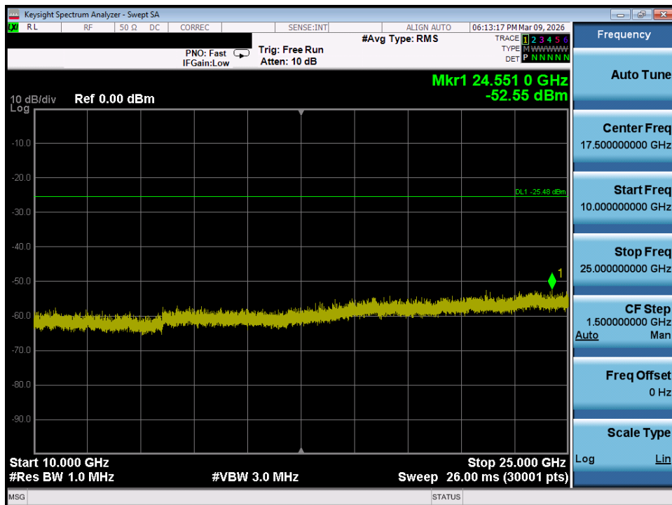
Plot 7-78. Conducted Spurious Plot MIMO ANT1 (802.11ax/be OFDMA – 242 Tones – Ch. 6)
