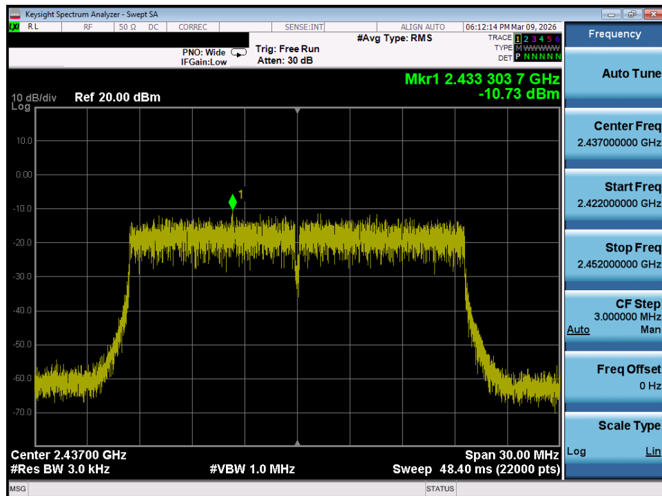
Plot 7-44. Power Spectral Density Plot MIMO ANT1 (802.11ax/be OFDMA – 242 Tones – Ch. 6)
