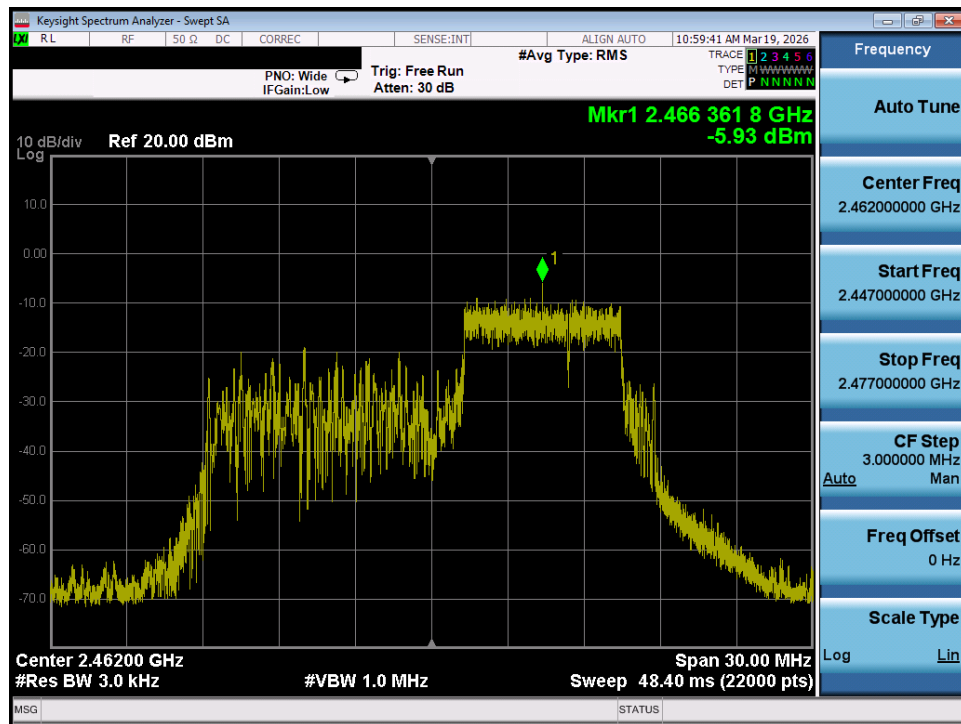
Plot 7-42. Power Spectral Density Plot MIMO ANT1 (802.11be OFDMA – 52+26 Tones – Ch. 11)
