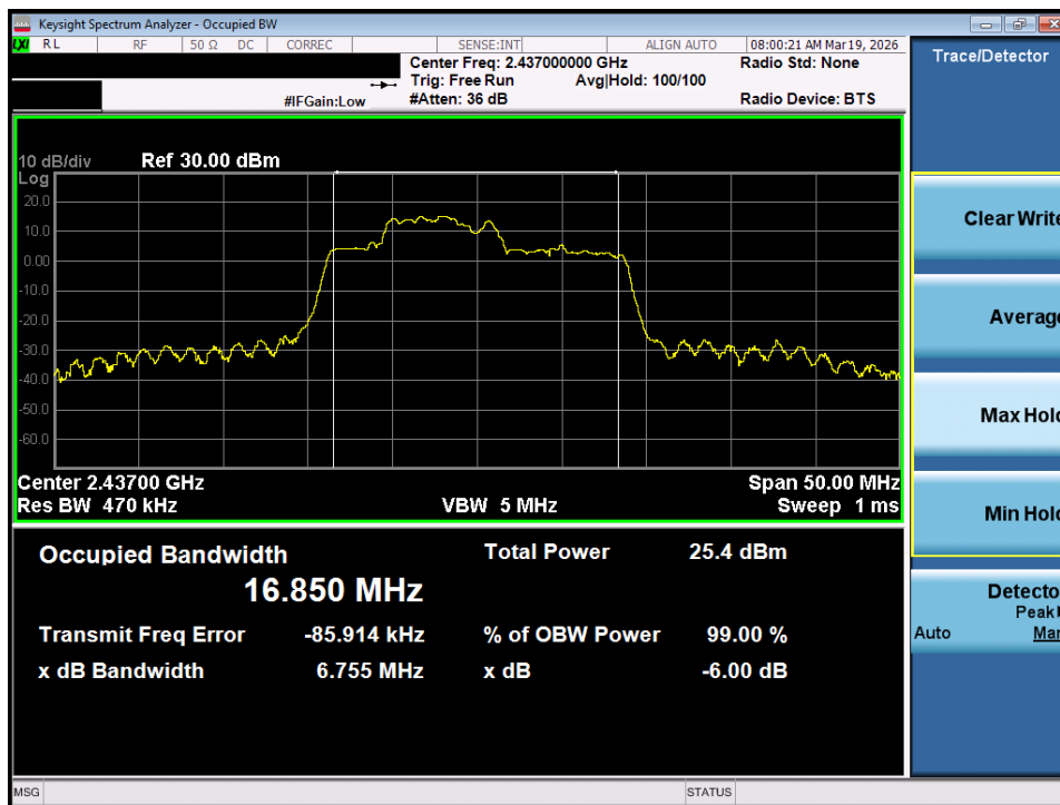
Plot 7-29. OBW Plot MIMO ANT2 (802.11be OFDMA – 52+26 Tones – Ch. 6)
