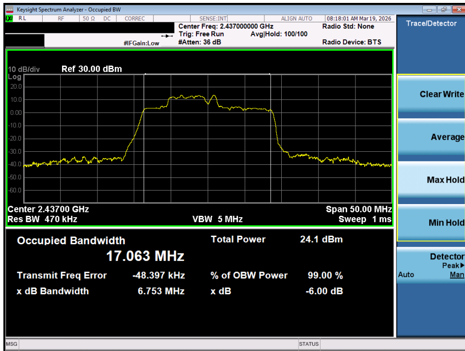
Plot 7-17. OBW Plot MIMO ANT1 (802.11be OFDMA – 52+26 Tones – Ch. 6)
