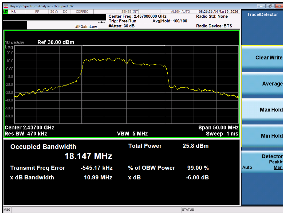
Plot 7-20. OBW Plot MIMO ANT1 (802.11be OFDMA – 106+26 Tones – Ch. 6)
