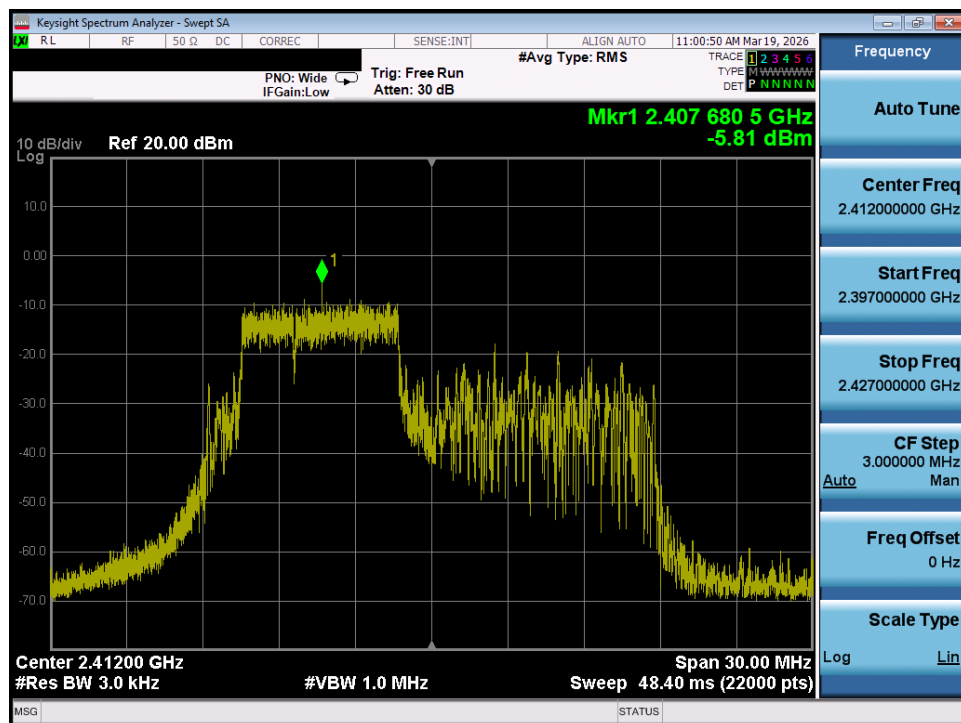
Plot 7-40. Power Spectral Density Plot MIMO ANT1 (802.11be OFDMA – 52+26 Tones – Ch. 1)
