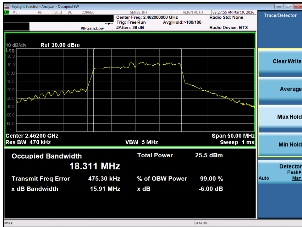
Plot 7-21. OBW Plot MIMO ANT1 (802.11be OFDMA – 106+26 Tones – Ch. 11)
