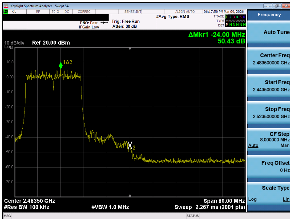
Plot 7-60. Band Edge Plot MIMO ANT1 (802.11ax/be OFDMA – 242 Tones – Ch. 10)
