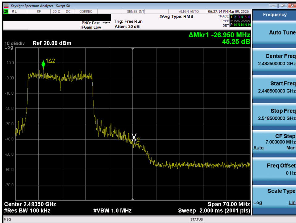
Plot 7-68. Band Edge Plot MIMO ANT2 (802.11ax/be OFDMA – 242 Tones – Ch. 11)
