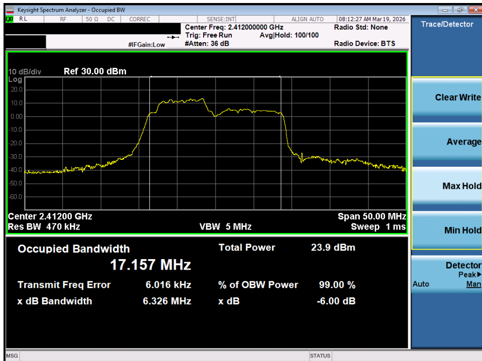
Plot 7-16. OBW Plot MIMO ANT1 (802.11be OFDMA – 52+26 Tones – Ch. 1)
