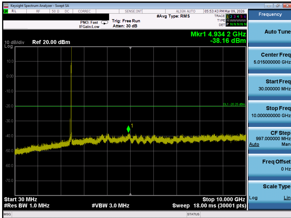
Plot 7-85. Conducted Spurious Plot MIMO ANT2 (802.11ax/be OFDMA – 26 Tones – Ch. 11)
