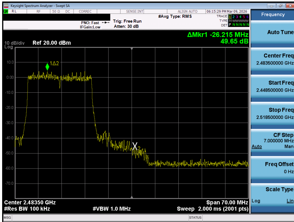
Plot 7-61. Band Edge Plot MIMO ANT1 (802.11ax/be OFDMA – 242 Tones – Ch. 11)
