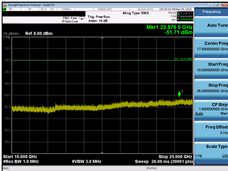
Plot 7-86. Conducted Spurious Plot MIMO ANT2 (802.11ax/be OFDMA – 26 Tones – Ch. 11)
