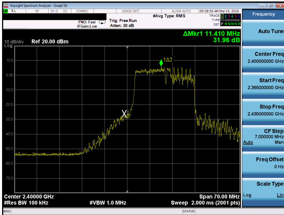
Plot 7-57. Band Edge Plot MIMO ANT1 (802.11be OFDMA – 106+26 Tones – Ch. 1)
