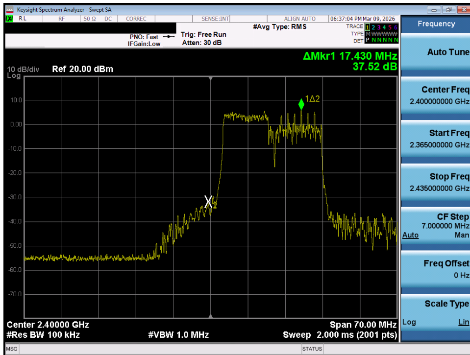
Plot 7-62. Band Edge Plot MIMO ANT2 (802.11ax/be OFDMA – 106 Tones – Ch. 1)
