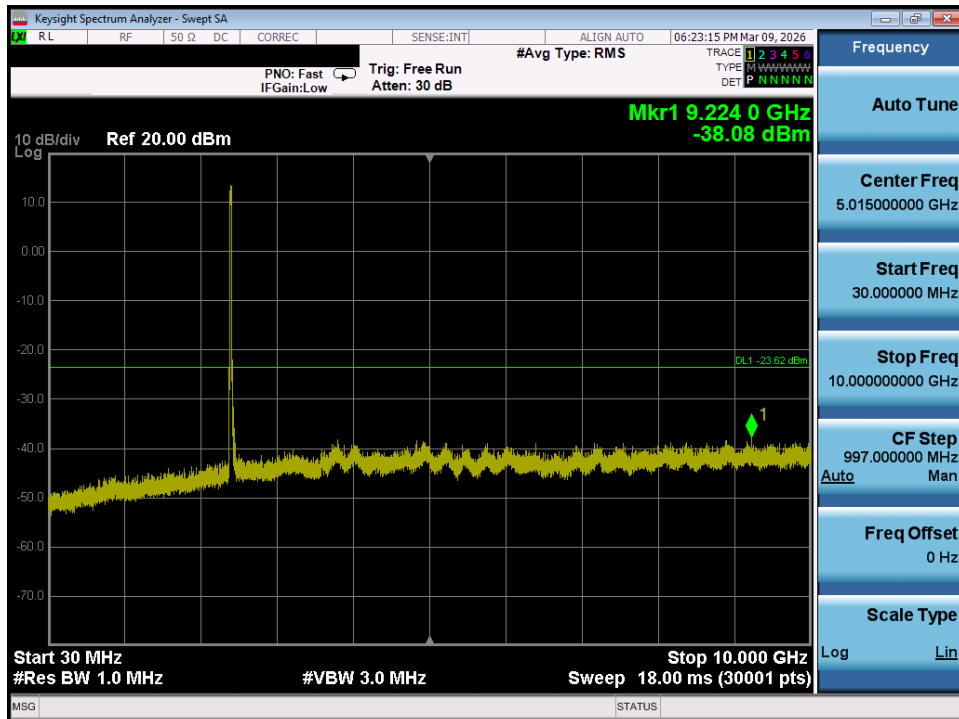
Plot 7-87. Conducted Spurious Plot MIMO ANT2 (802.11ax/be OFDMA – 242 Tones – Ch. 1)
