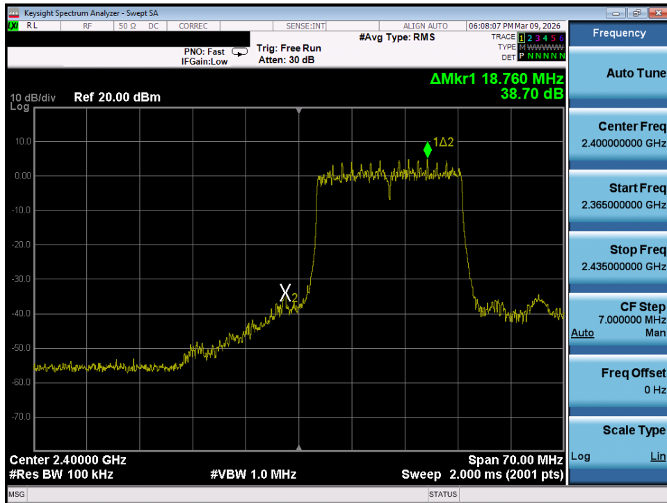
Plot 7-59. Band Edge Plot MIMO ANT1 (802.11ax/be OFDMA – 242 Tones – Ch. 1)
