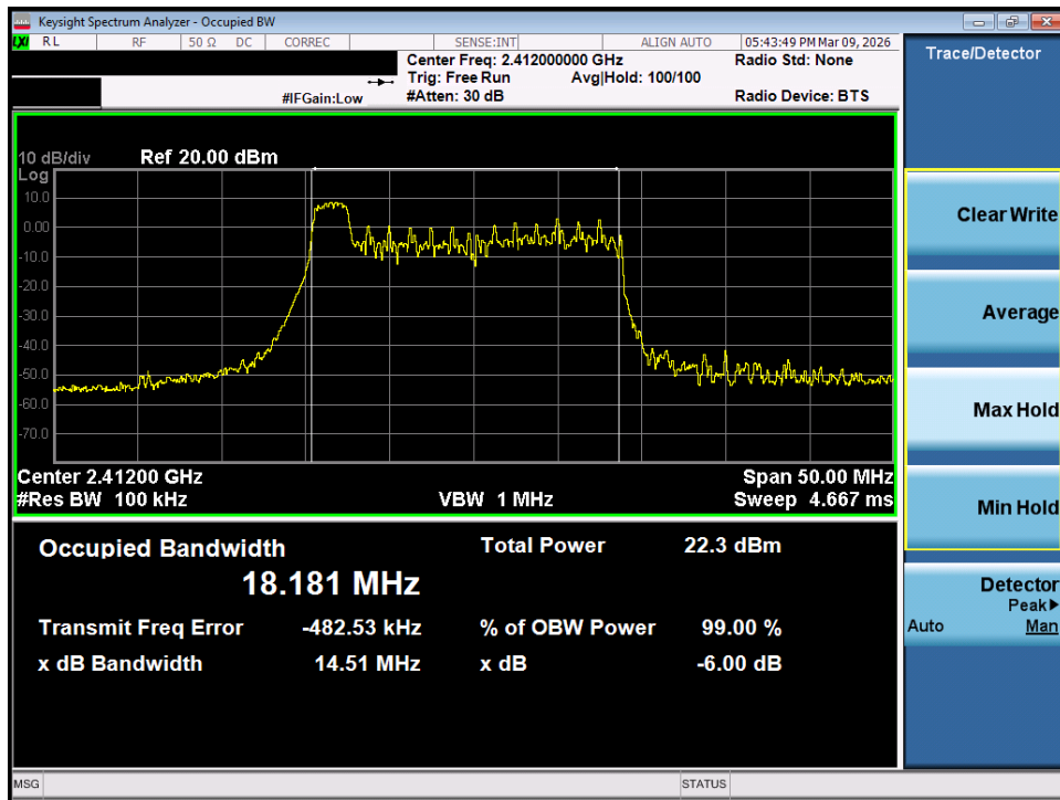
Plot 7-7. 6dB Bandwidth Plot MIMO ANT2 (802.11ax/be OFDMA – 26 Tones – Ch. 1)
