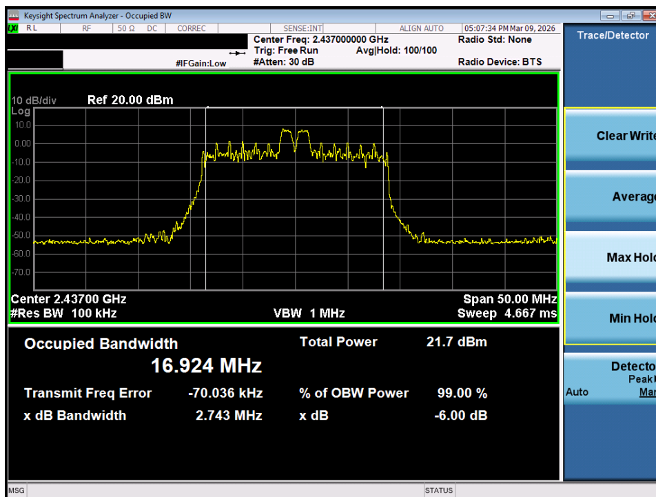
Plot 7-2. 6dB Bandwidth Plot MIMO ANT1 (802.11ax/be OFDMA – 26 Tones – Ch. 6)
