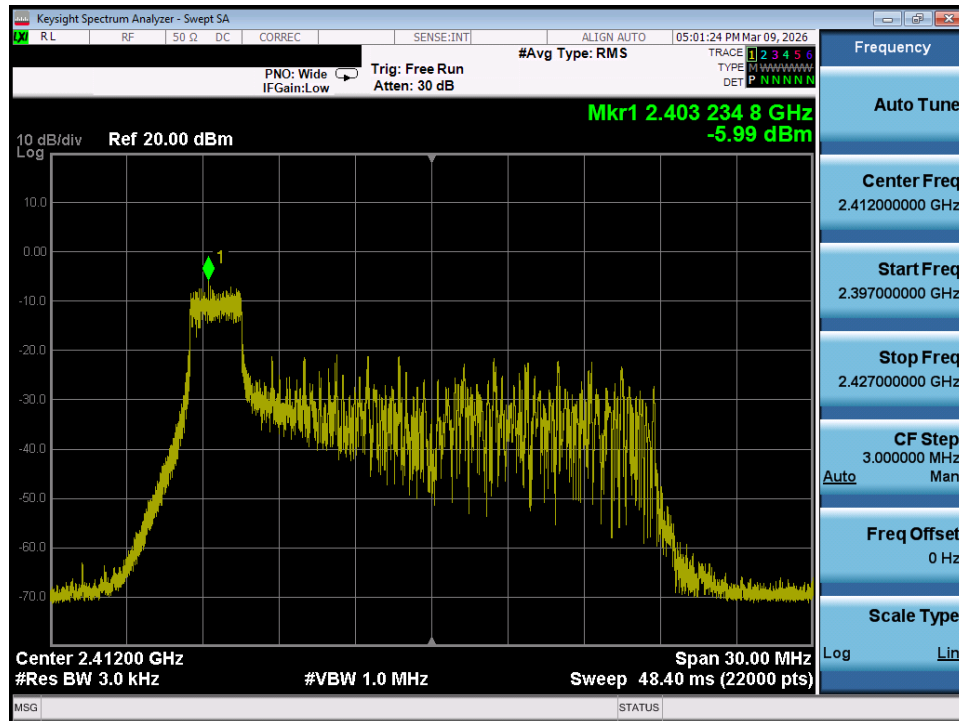
Plot 7-37. Power Spectral Density Plot MIMO ANT1 (802.11ax/be OFDMA – 26 Tones – Ch. 1)
