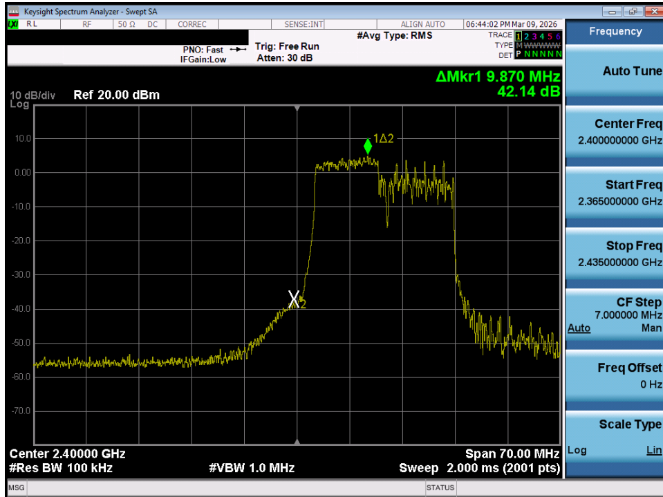
Plot 7-55. Band Edge Plot MIMO ANT1 (802.11ax/be OFDMA – 106 Tones – Ch. 1)
