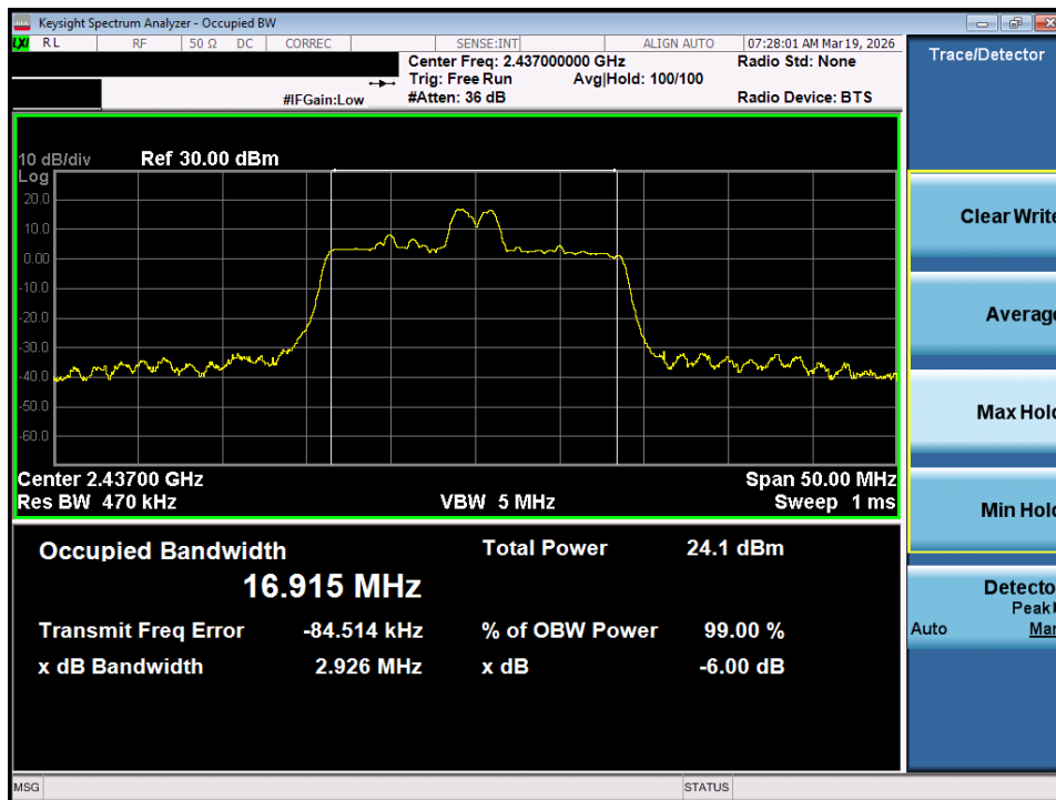
Plot 7-26. OBW Plot MIMO ANT2 (802.11ax/be OFDMA – 26 Tones – Ch. 6)
