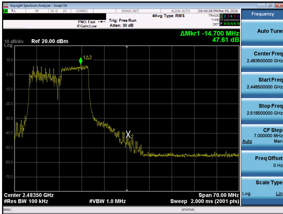
Plot 7-63. Band Edge Plot MIMO ANT2 (802.11ax/be OFDMA – 106 Tones – Ch. 11)
