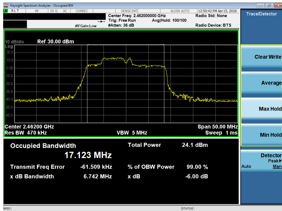
Plot 7-18. OBW Plot MIMO ANT1 (802.11be OFDMA – 52+26 Tones – Ch. 11)
