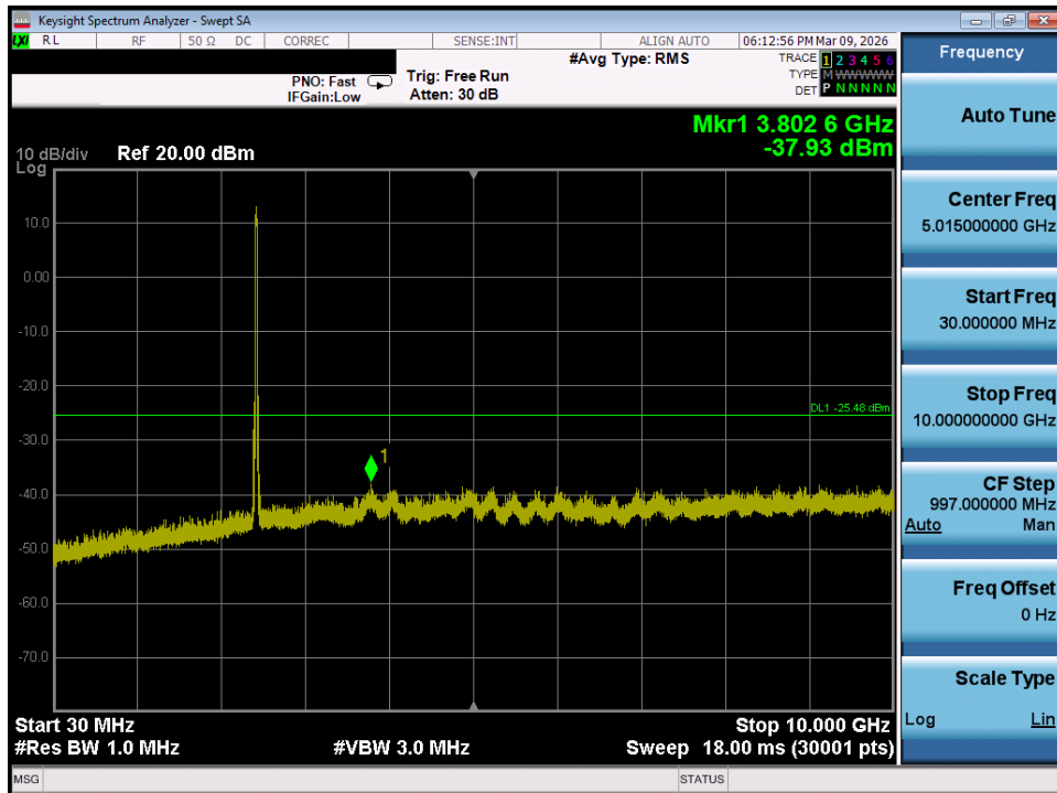
Plot 7-77. Conducted Spurious Plot MIMO ANT1 (802.11ax/be OFDMA – 242 Tones – Ch. 6)
