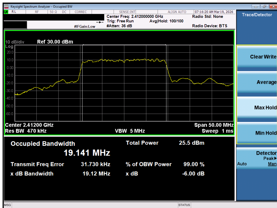
Plot 7-22. OBW Plot MIMO ANT1 (802.11ax/be OFDMA – 242 Tones – Ch. 1)
