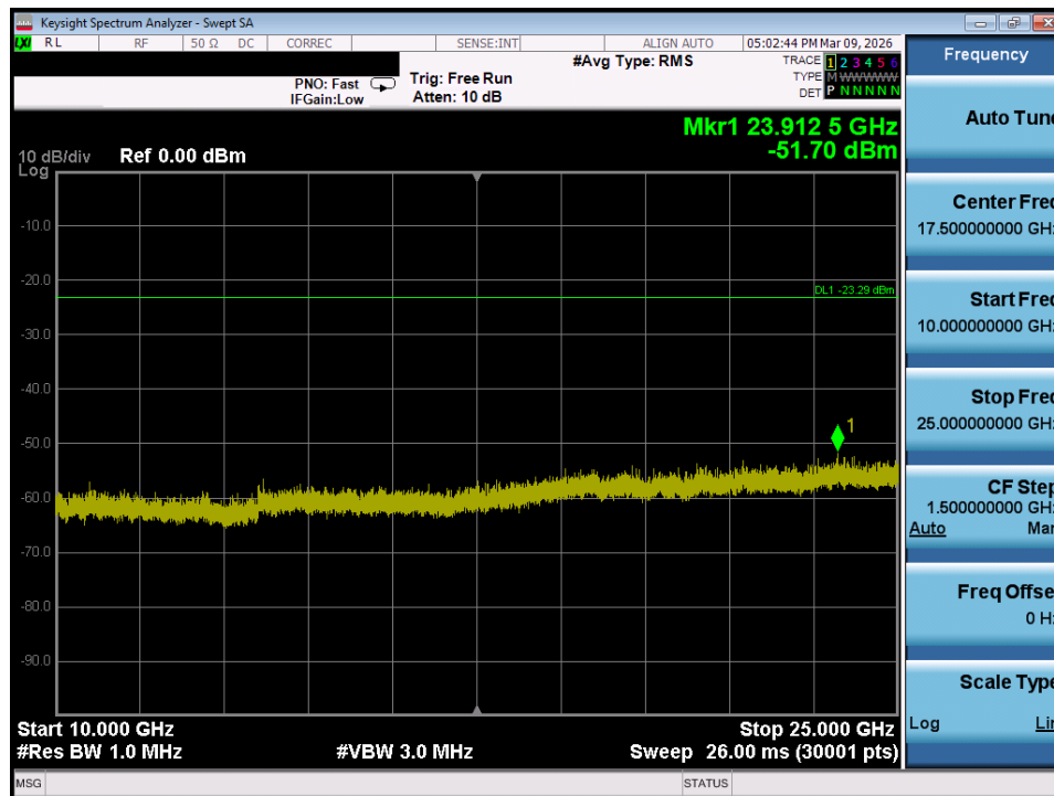
Plot 7-70. Conducted Spurious Plot MIMO ANT1 (802.11ax/be OFDMA – 26 Tones – Ch. 1)
