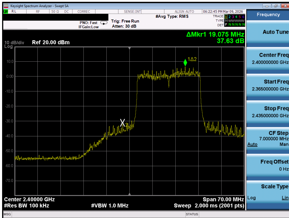
Plot 7-66. Band Edge Plot MIMO ANT2 (802.11ax/be OFDMA – 242 Tones – Ch. 1)
