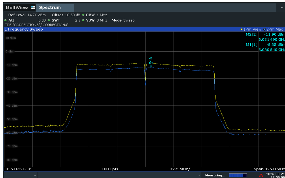
Plot 7-76. Power Spectral Density Plot – ANT2 (160MHz Bandwidth, RSSI level at -84dBm (yellow) and -34dBm (blue))
