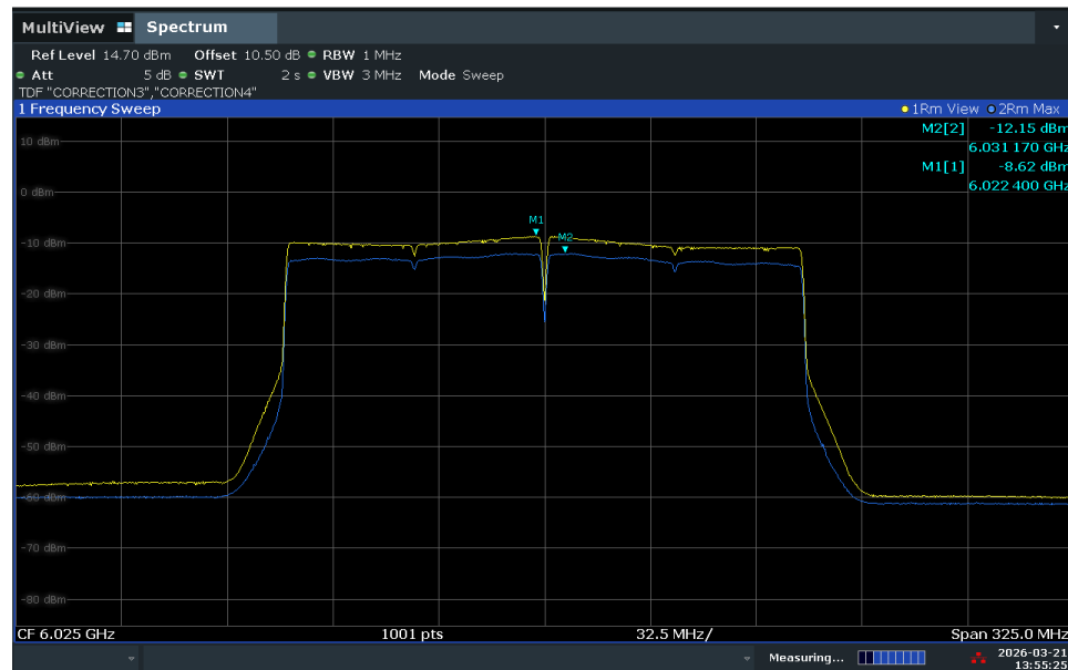
Plot 7-75. Power Spectral Density Plot – ANT1 (160MHz Bandwidth, RSSI level at -84dBm (yellow) and -34dBm (blue))
