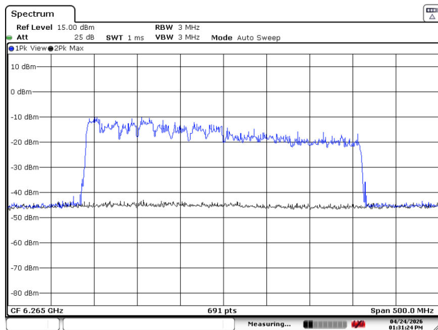
Plot 7-73. CBP 320MHz Channel - Injection Center – [6265 MHz]
