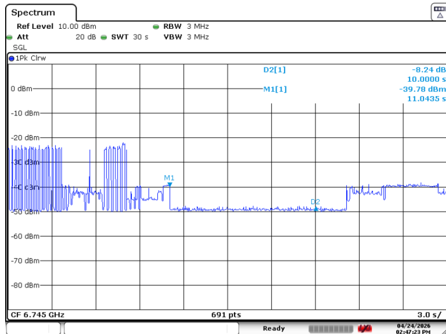
Plot 7-66. Contention Based Protocol Timing Plot (320MHz (UNII Band 7) – Ch. 159 Mid)
