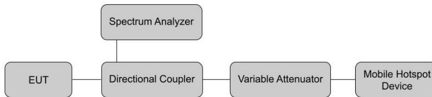
Figure 7-6. Test Instrument & Measurement Setup
