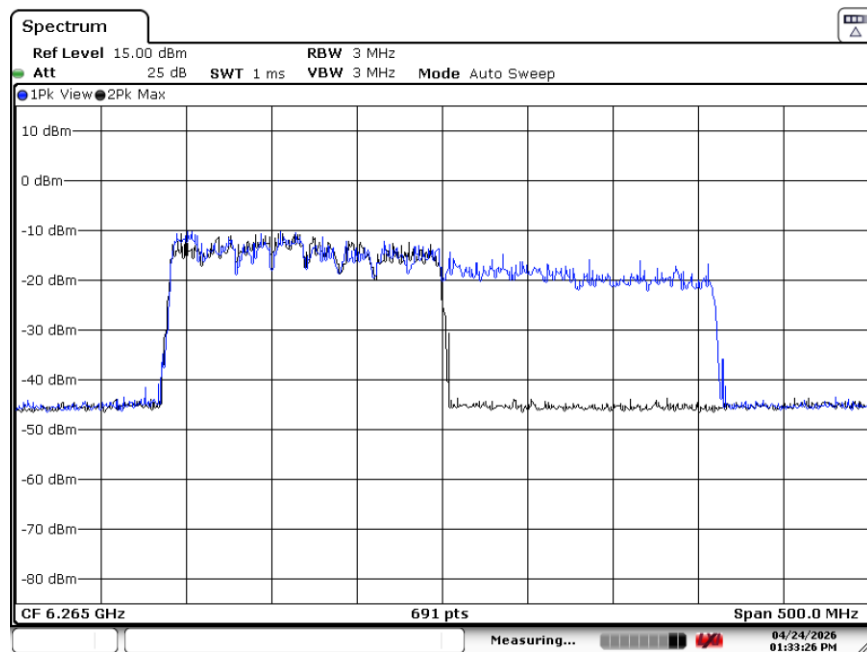
Plot 7-74. CBP 320MHz Channel - Injection Upper Edge – [6420 MHz]
