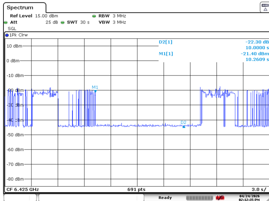
Plot 7-62. Contention Based Protocol Timing Plot (320MHz (UNII Band 6) – Ch. 95 Mid)
