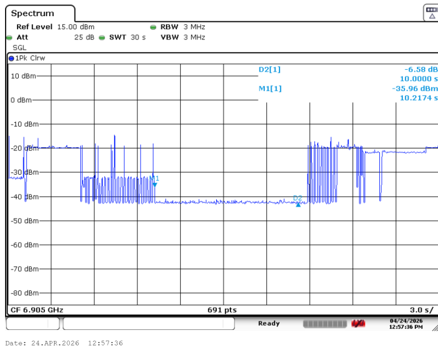
Plot 7-94. Contention Based Protocol Timing Plot (320MHz (UNII Band 8) – Ch. 191 Mid)
