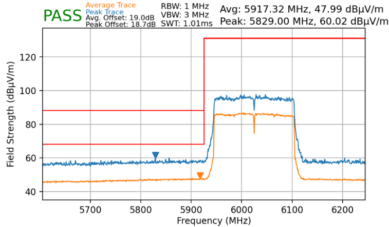
Plot 7-120. Radiated Lower Band Edge Plot MIMO (Average & Peak – UNII Band 5)
