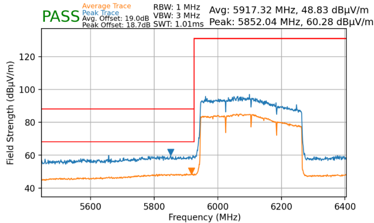
Plot 7-124. Radiated Lower Band Edge Plot MIMO (Average & Peak – UNII Band 5)
