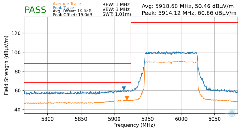
Plot 7-116. Radiated Lower Band Edge Plot MIMO (Average & Peak – UNII Band 5)
