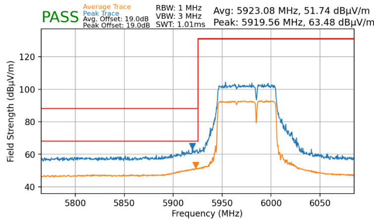
Plot 7-118. Radiated Lower Band Edge Plot MIMO (Average & Peak – UNII Band 5)
