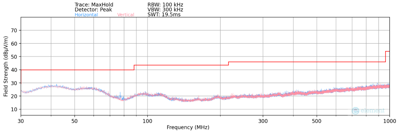
Plot 7-107. Radiated Spurious Plot below 1GHz MIMO 802.11g (2.4GHz – Ch.6) + MIMO 802.11a (6GHz – Ch.1)
