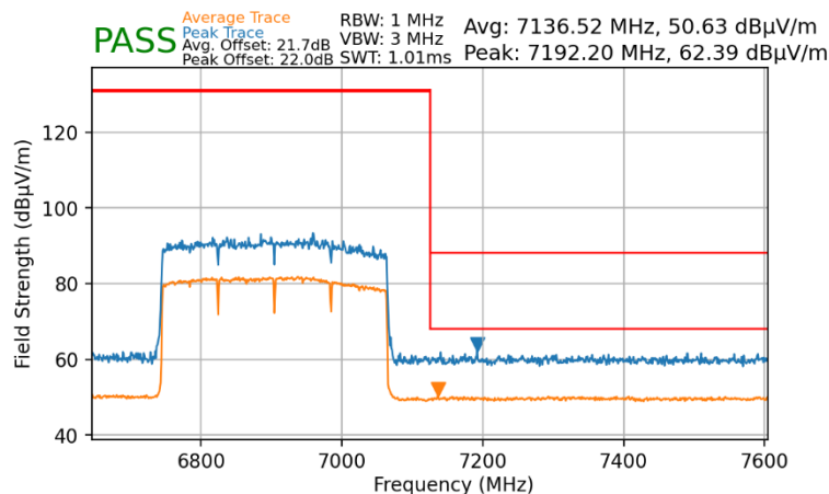
Plot 7-125. Radiated Upper Band Edge Plot MIMO (Average & Peak – UNII Band 8)
