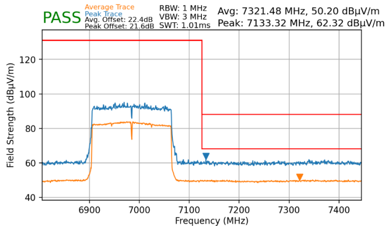
Plot 7-121. Radiated Upper Band Edge Plot MIMO (Average & Peak – UNII Band 8)
