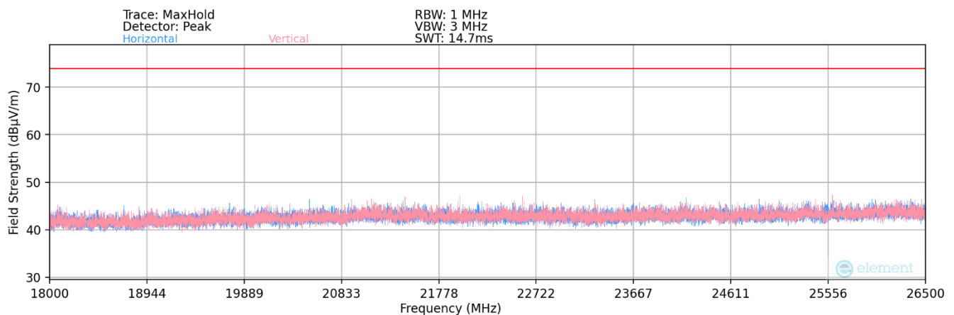
Plot 7-109. Radiated Spurious Plot 18GHz – 26.6GHz MIMO 802.11g (2.4GHz – Ch.6) + MIMO 802.11a (6GHz – Ch.1)
