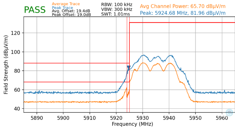
Plot 7-113. Radiated Lower Band Edge Plot MIMO (Average & Peak – UNII Band 5) – WCP
