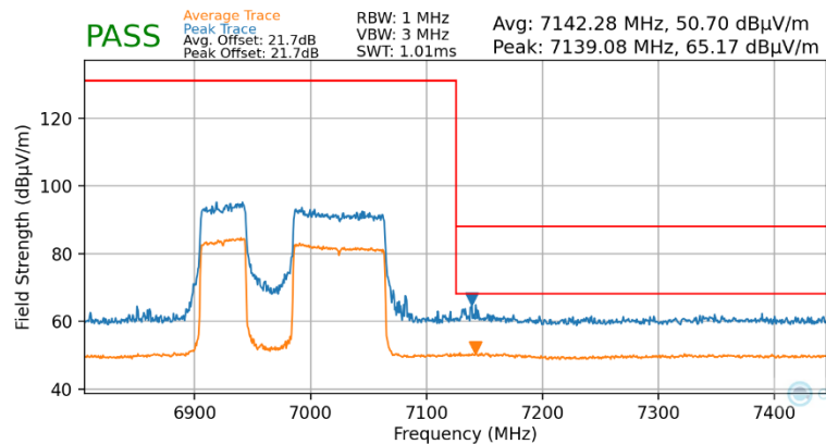
Plot 7-123. Radiated Upper Band Edge Plot MIMO (Average & Peak – UNII Band 8)
