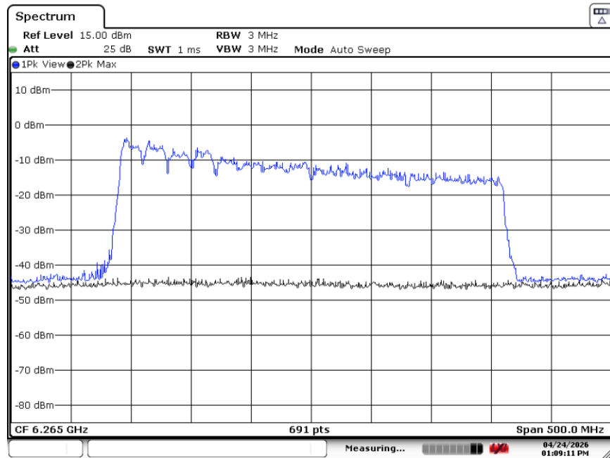
Plot 7-97. CBP 320MHz Channel - Injection Center – [6265 MHz]
