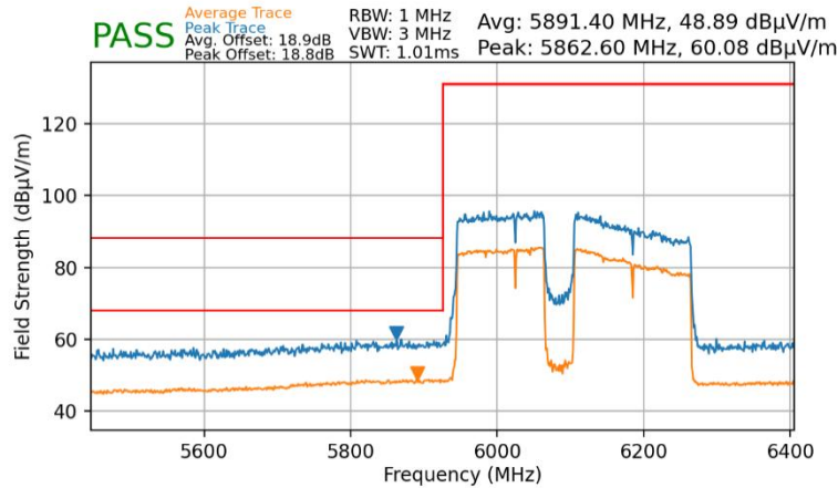
Plot 7-126. Radiated Lower Band Edge Plot MIMO (Average & Peak – UNII Band 5)
