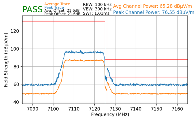
Plot 7-112. Radiated Upper Band Edge Plot MIMO (Average & Peak – UNII Band 8)
