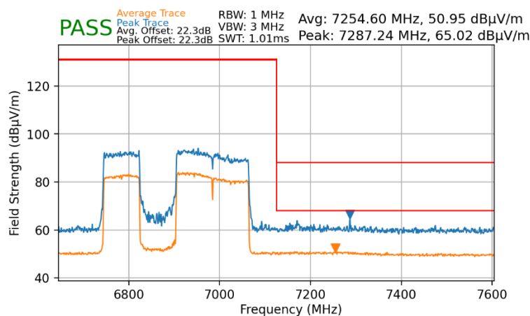
Plot 7-127. Radiated Upper Band Edge Plot MIMO (Average & Peak – UNII Band 8)
