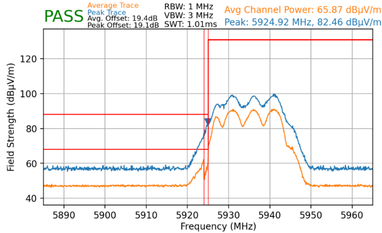
Plot 7-111. Radiated Lower Band Edge Plot MIMO (Average & Peak – UNII Band 5)
