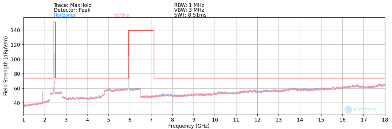
Plot 7-108. Radiated Spurious Plot above 1GHz MIMO 802.11g (2.4GHz – Ch.6) + MIMO 802.11a (6GHz – Ch.1)
