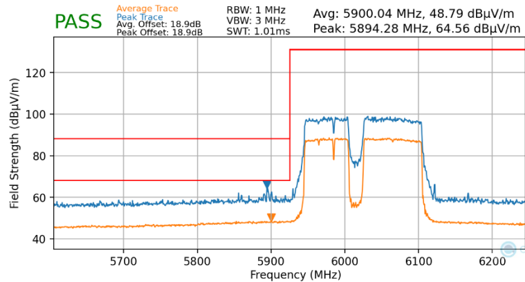
Plot 7-122. Radiated Lower Band Edge Plot MIMO (Average & Peak – UNII Band 5)
