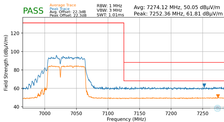
Plot 7-119. Radiated Upper Band Edge Plot MIMO (Average & Peak – UNII Band 8)
