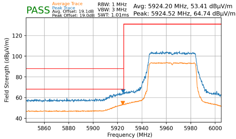
Plot 7-114. Radiated Lower Band Edge Plot MIMO (Average & Peak – UNII Band 5)
