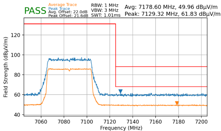
Plot 7-115. Radiated Upper Band Edge Plot MIMO (Average & Peak – UNII Band 8)
