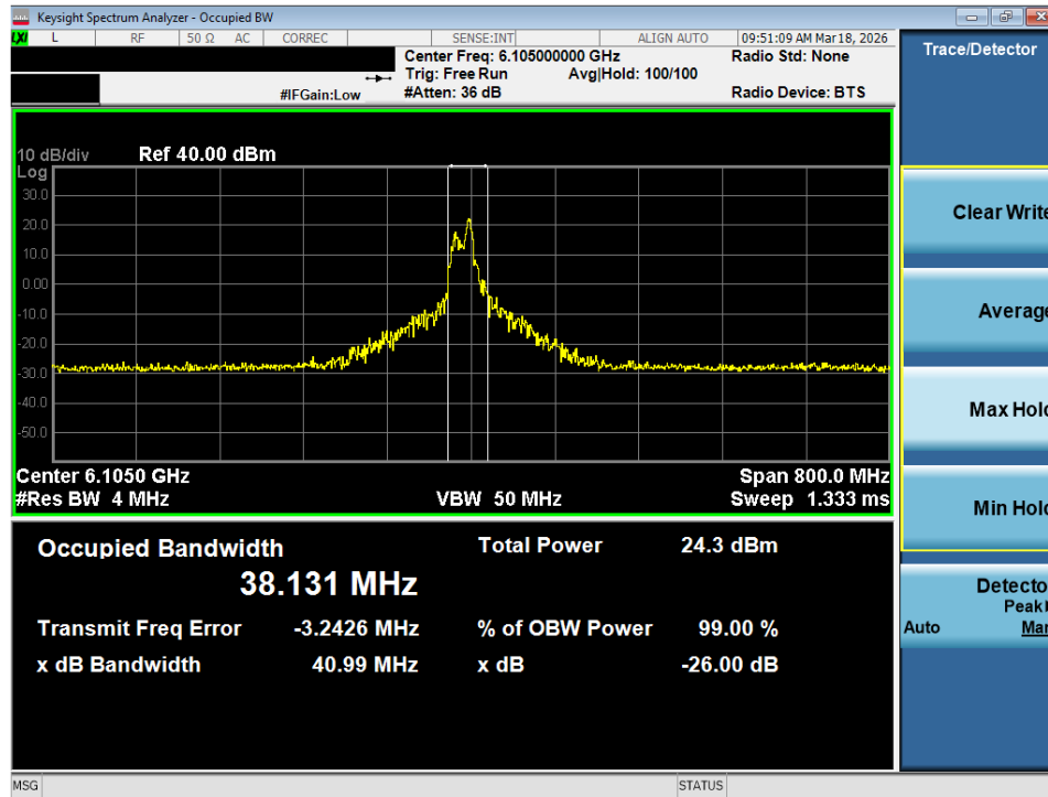
Plot 7-37. 26dB Bandwidth Plot MIMO ANT2 (320MHz 802.11be (26 Tones) (UNII Band 5) – Ch. 31) - SP
