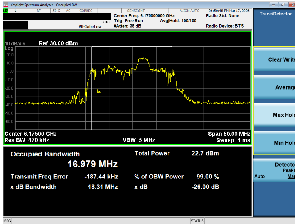
Plot 7-33. 26dB Bandwidth Plot MIMO ANT2 (20MHz 802.11ax/be (26 Tones) (UNII Band 5) – Ch. 45) - SP
