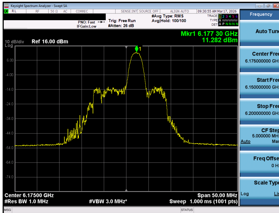
Plot 7-56. Power Spectral Density Plot MIMO ANT1 (20MHz 802.11ax/be (26 Tones) (UNII Band 5) – Ch. 45) - SP
