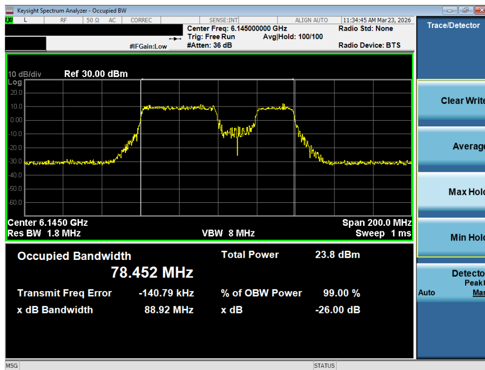
Plot 7-39. 26dB Bandwidth Plot MIMO ANT2 (80MHz 802.11be (484+242 Tones) (UNII Band 5) – Ch. 39) - SP
