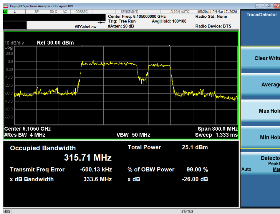
Plot 7-32. 26dB Bandwidth Plot MIMO ANT2 (320MHz 802.11be (3*996+484 Tones) (UNII Band 5) – Ch. 31) LPI/SP
