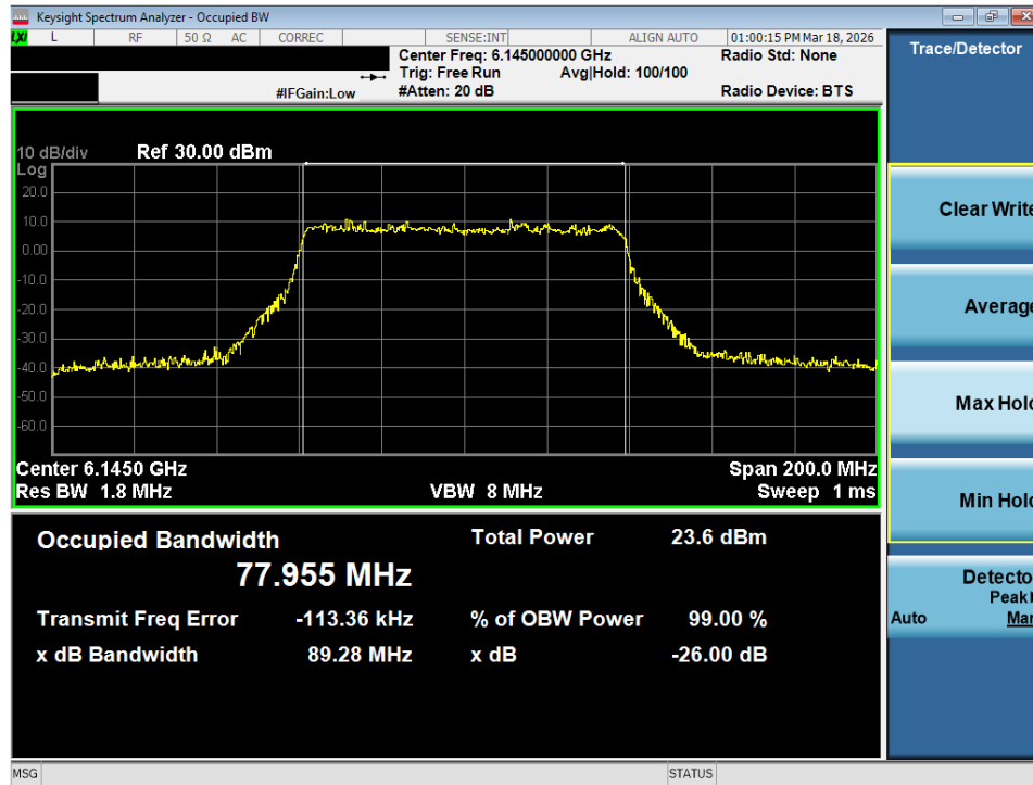
Plot 7-42. 26dB Bandwidth Plot MIMO ANT2 (80MHz 802.11ax/be (Full Tones) (UNII Band 5) – Ch. 39) - LPI/SP
