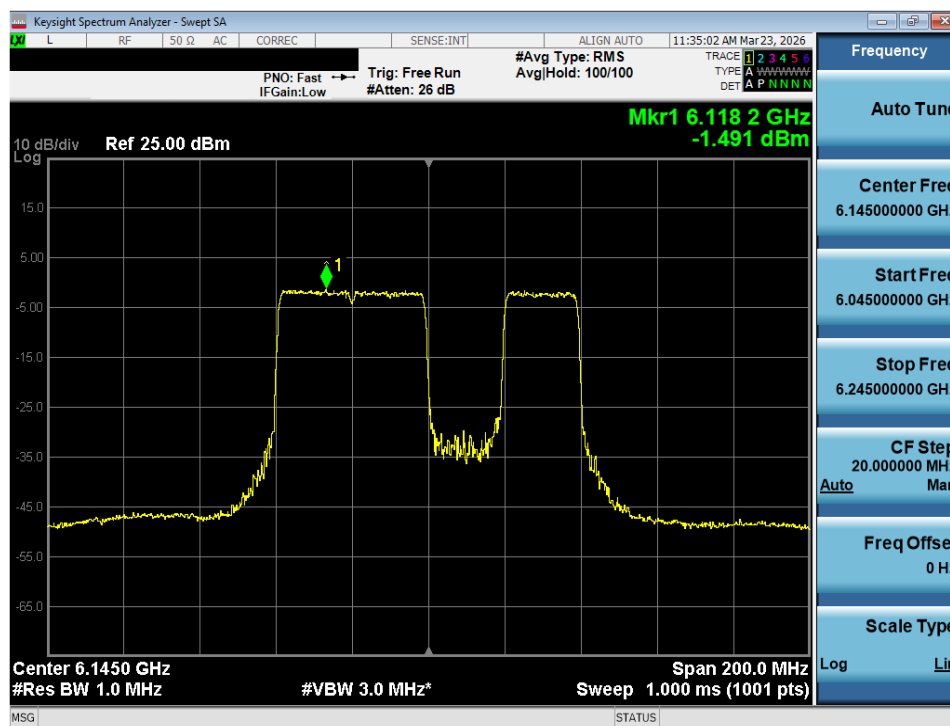
Plot 7-85. Power Spectral Density Plot MIMO ANT2 (80MHz 802.11be (484+242 Tones) (UNII Band 5) – Ch. 39) - SP
