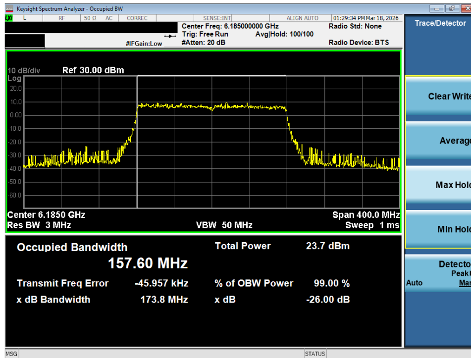
Plot 7-43. 26dB Bandwidth Plot MIMO ANT2 (160MHz 802.11ax/be (Full Tones) (UNII Band 5) – Ch. 47) - LPI/SP
