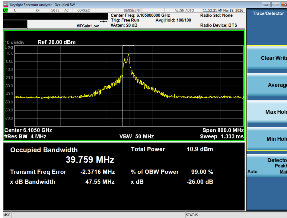
Plot 7-28. 26dB Bandwidth Plot MIMO ANT2 (320MHz 802.11be (26 Tones) (UNII Band 5) – Ch. 31) - LPI
