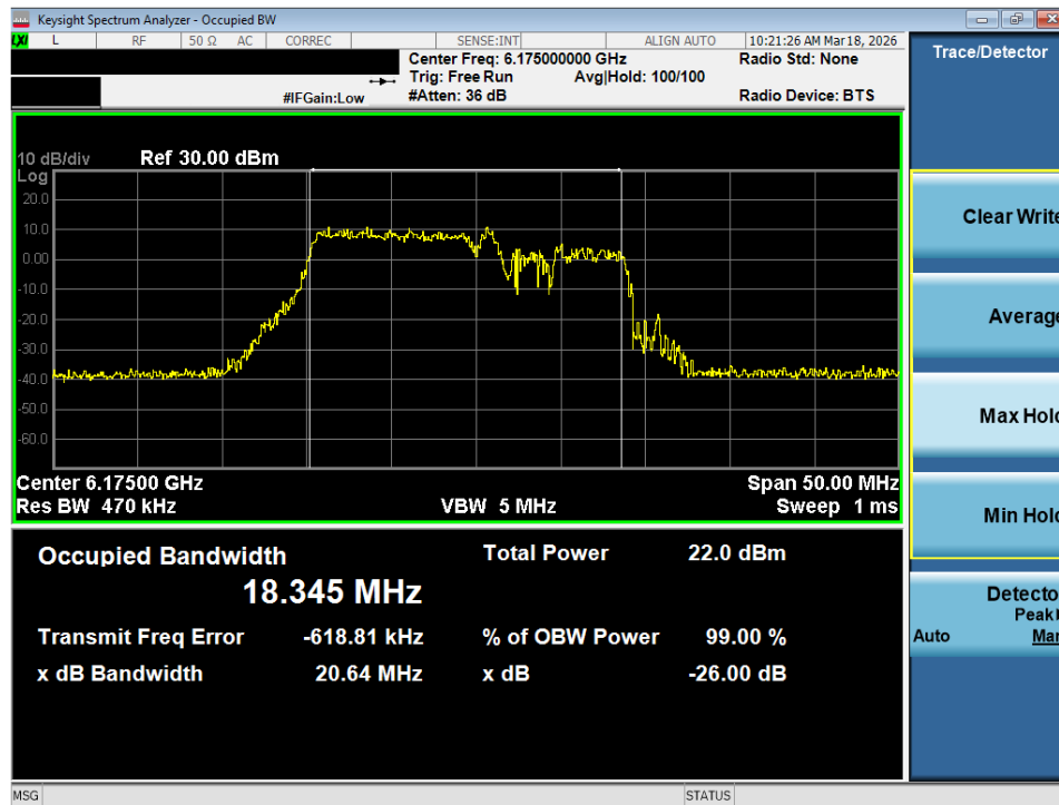
Plot 7-38. 26dB Bandwidth Plot MIMO ANT2 (20MHz 802.11be (106+26 Tones) (UNII Band 5) – Ch. 45) – SP
