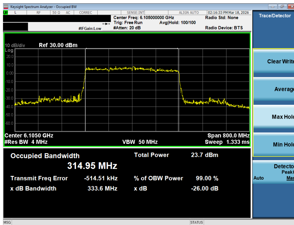
Plot 7-44. 26dB Bandwidth Plot MIMO ANT2 (320MHz 802.11be (Full Tones) (UNII Band 5) – Ch. 31) - LPI/SP
