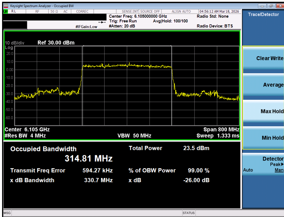
Plot 7-21. 26dB Bandwidth Plot MIMO ANT1 (320MHz 802.11be (Full Tones) (UNII Band 5) – Ch. 31) - LPI/SP
