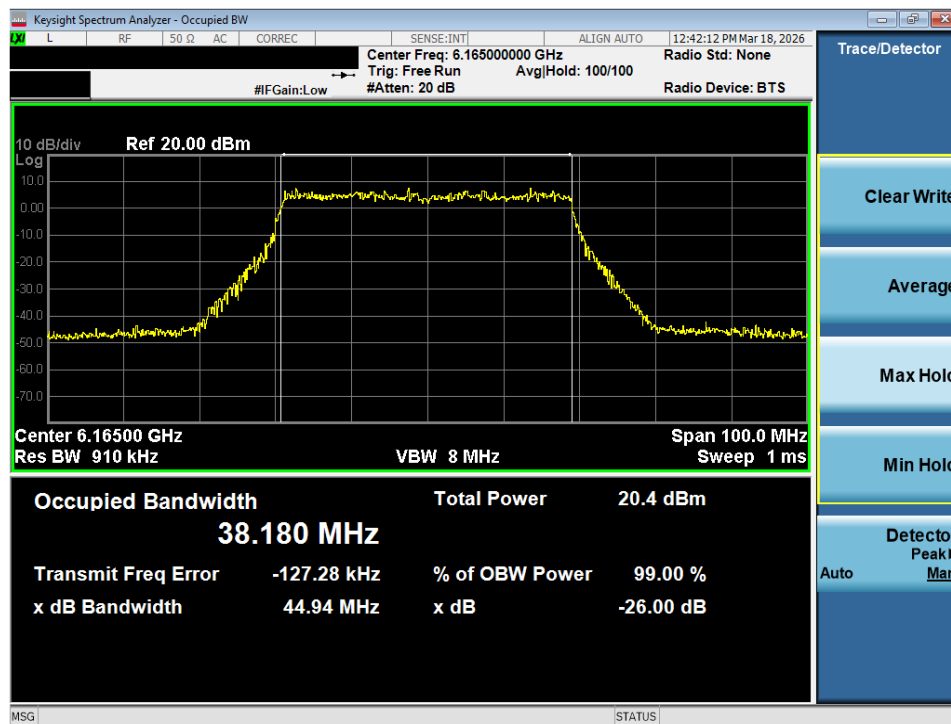
Plot 7-41. 26dB Bandwidth Plot MIMO ANT2 (40MHz 802.11ax/be (Full Tones) (UNII Band 5) – Ch. 43) - LPI
