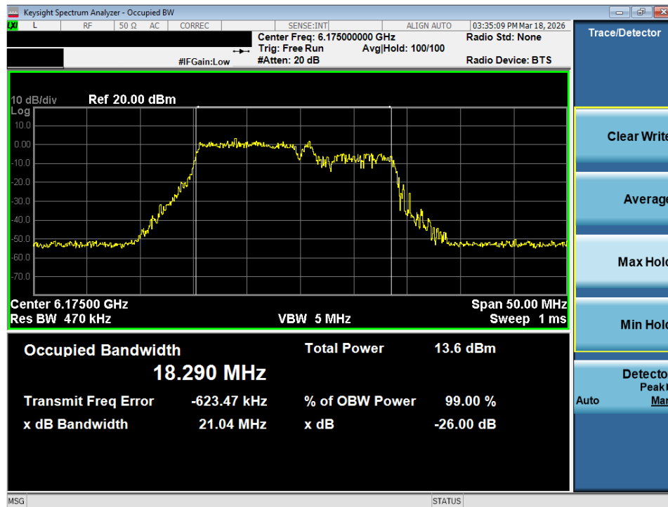
Plot 7-29. 26dB Bandwidth Plot MIMO ANT2 (20MHz 802.11be (106+26 Tones) (UNII Band 5) – Ch. 45) - LPI
