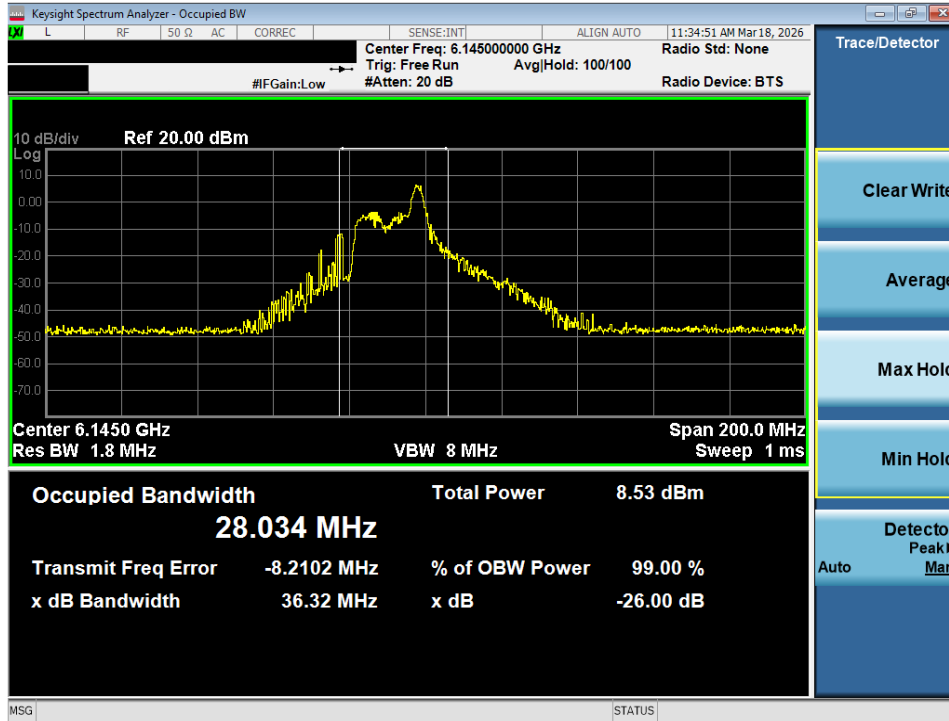
Plot 7-26. 26dB Bandwidth Plot MIMO ANT2 (80MHz 802.11ax/be (26 Tones) (UNII Band 5) – Ch. 39) - LPI
