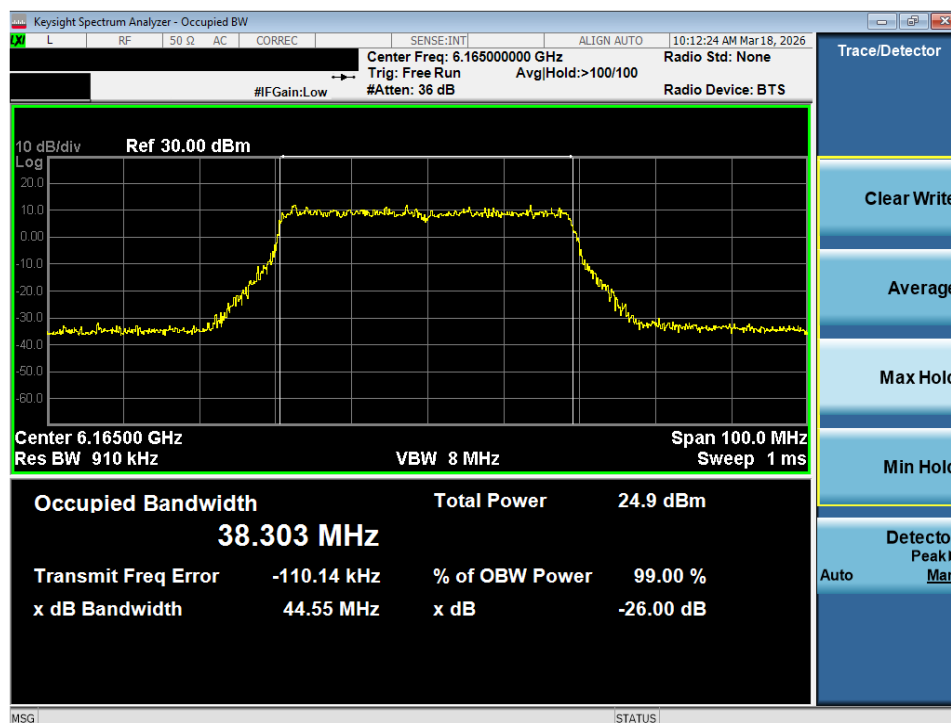
Plot 7-46. 26dB Bandwidth Plot MIMO ANT2 (40MHz 802.11ax/be (Full Tones) (UNII Band 5) – Ch. 43) - SP
