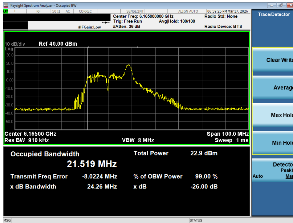
Plot 7-34. 26dB Bandwidth Plot MIMO ANT2 (40MHz 802.11ax/be (26 Tones) (UNII Band 5) – Ch. 43) - SP
