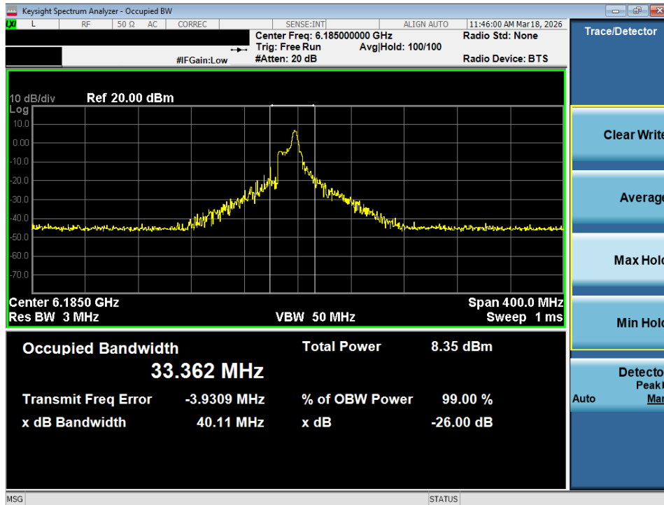
Plot 7-27. 26dB Bandwidth Plot MIMO ANT2 (160MHz 802.11ax/be (26 Tones) (UNII Band 5) – Ch. 47) - LPI
