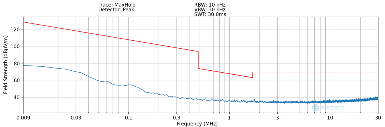
Plot 7-4 Radiated Spurious Plot 9kHz – 30MHz (Pol. Y – Device to Device)
