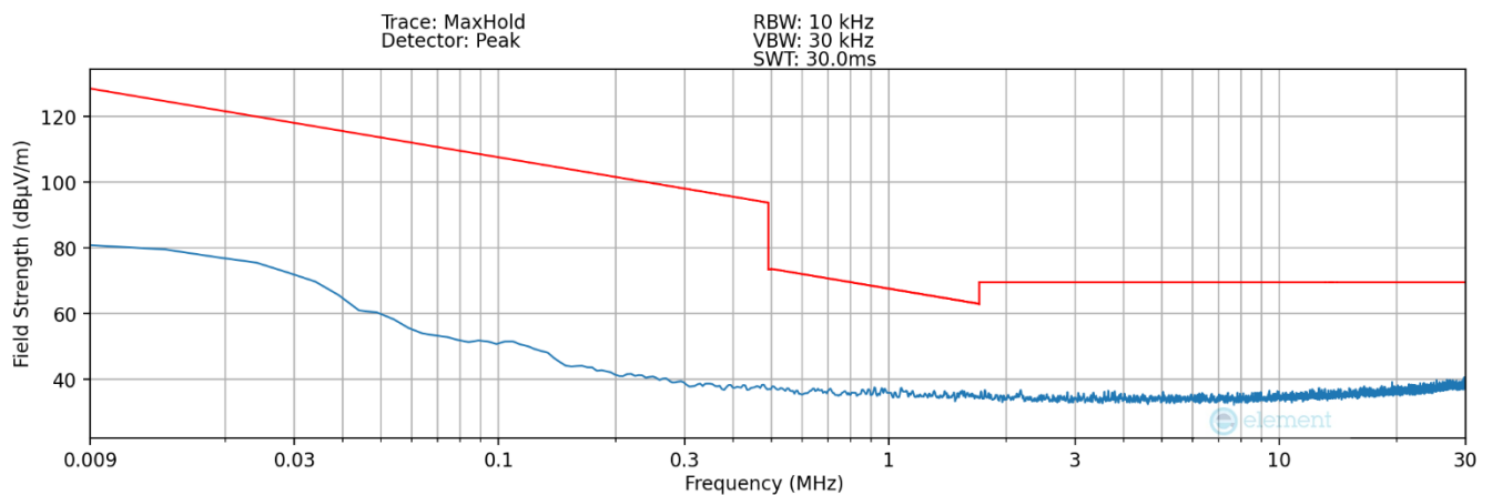
Plot 7-5. Radiated Spurious Plot 9kHz – 30MHz (Pol. Z – Device to Device)
