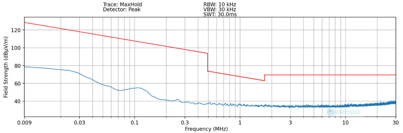
Plot 7-3. Radiated Spurious Plot 9kHz – 30MHz (Pol. X – Device to Device)
