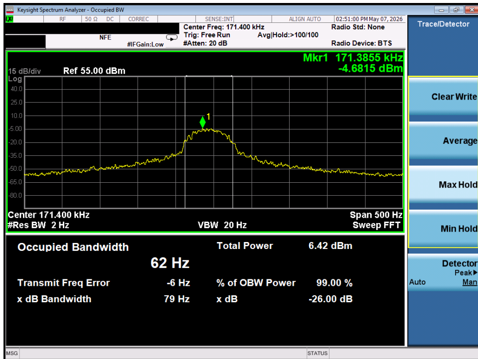
Plot 7-2. Occupied Bandwidth Measurement – Device to Device (Ping)
