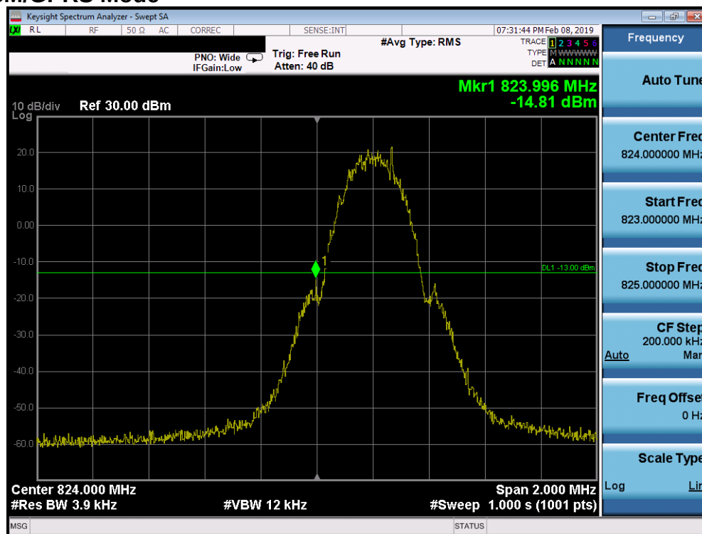
Plot 7-53. Band Edge Plot (Cellular GSM Mode - Low Channel)
