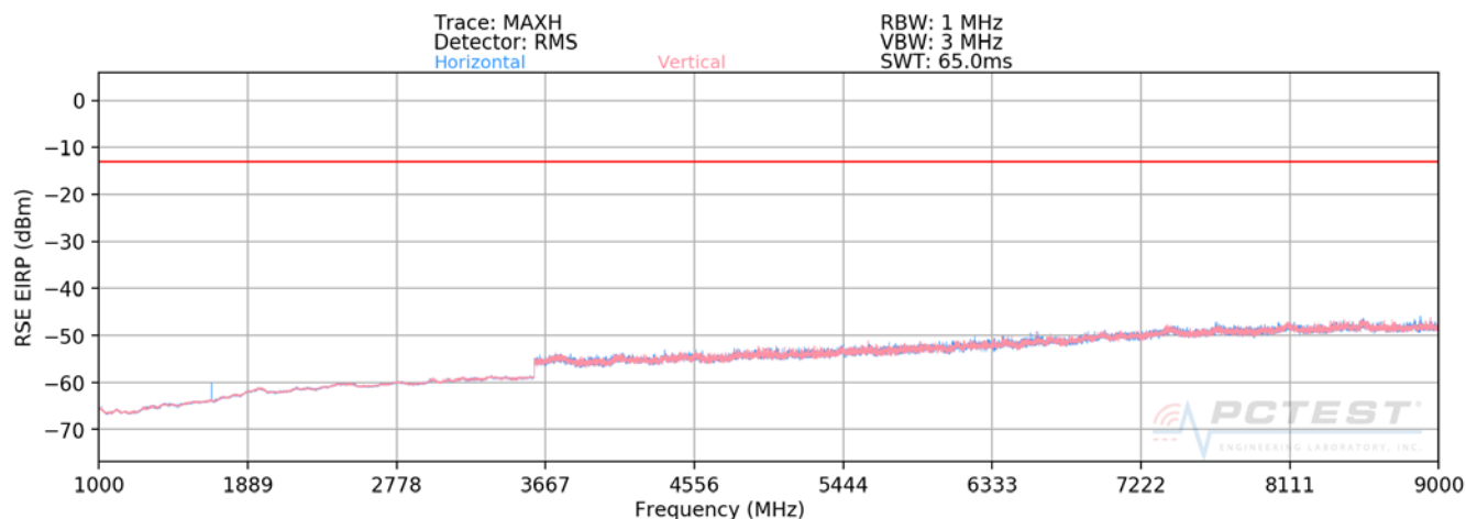
Plot 7-76. Radiated Spurious Plot above 1GHz (Cellular GPRS Mode - CLOSED)
