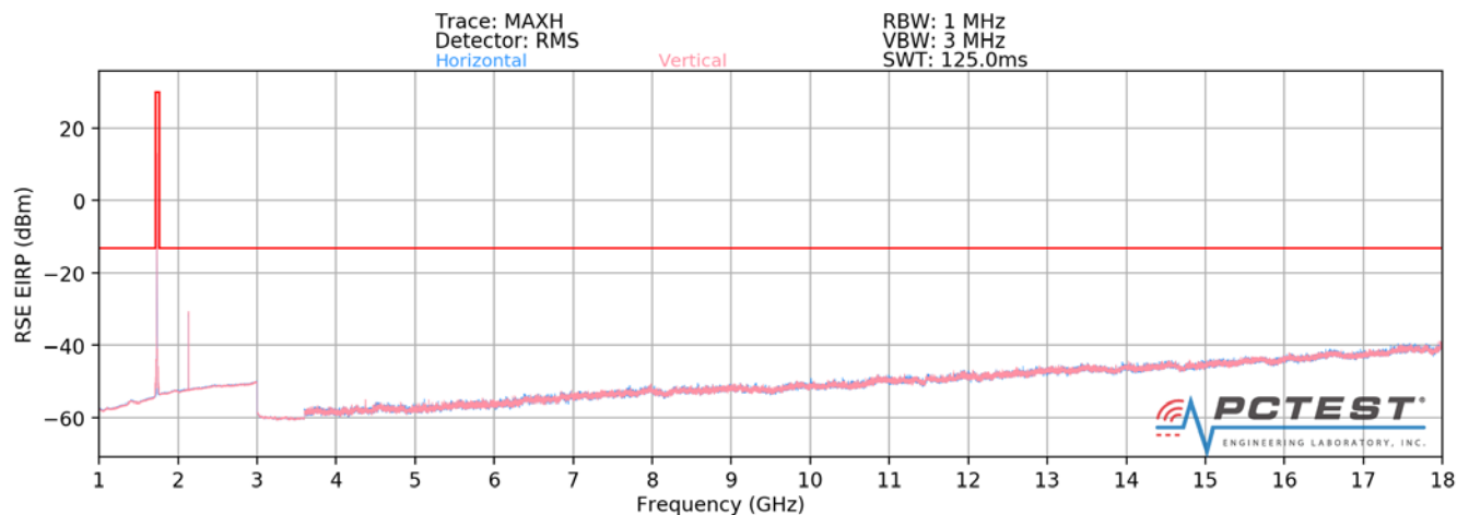
Plot 7-81. Radiated Spurious Plot above 1GHz (AWS WCDMA Mode - OPEN)
