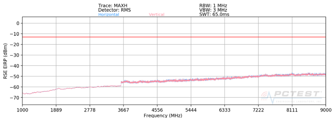
Plot 7-77. Radiated Spurious Plot above 1GHz (Cellular GPRS Mode - OPEN)
