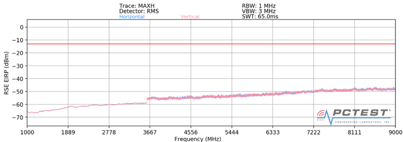
Plot 7-79. Radiated Spurious Plot above 1GHz (Cellular WCDMA Mode - OPEN)
