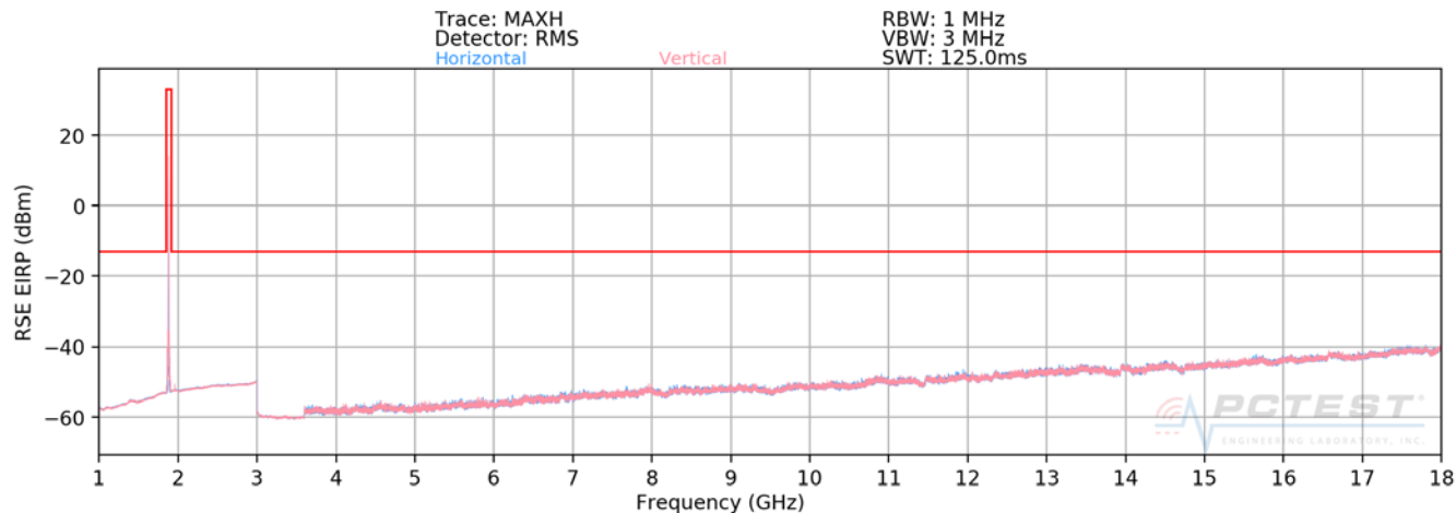
Plot 7-84. Radiated Spurious Plot above 1GHz (PCS WCDMA Mode - CLOSED)
