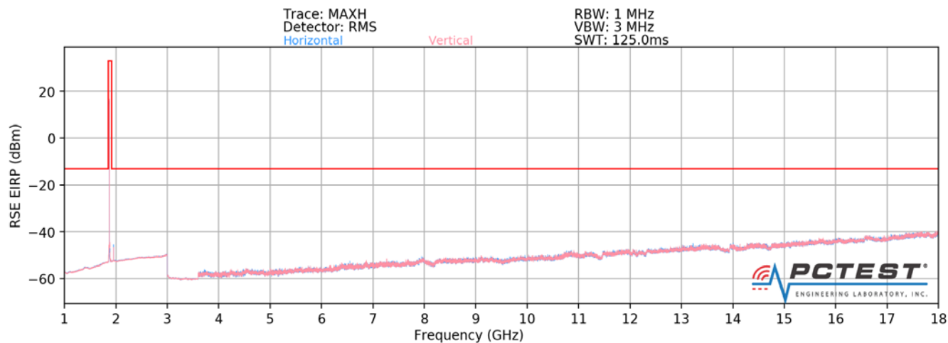
Plot 7-85. Radiated Spurious Plot above 1GHz (PCS WCDMA Mode - OPEN)
