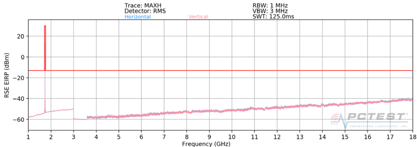
Plot 7-80. Radiated Spurious Plot above 1GHz (AWS WCDMA Mode - CLOSED)
