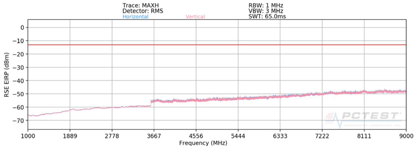
Plot 7-78. Radiated Spurious Plot above 1GHz (Cellular WCDMA Mode - CLOSED)
