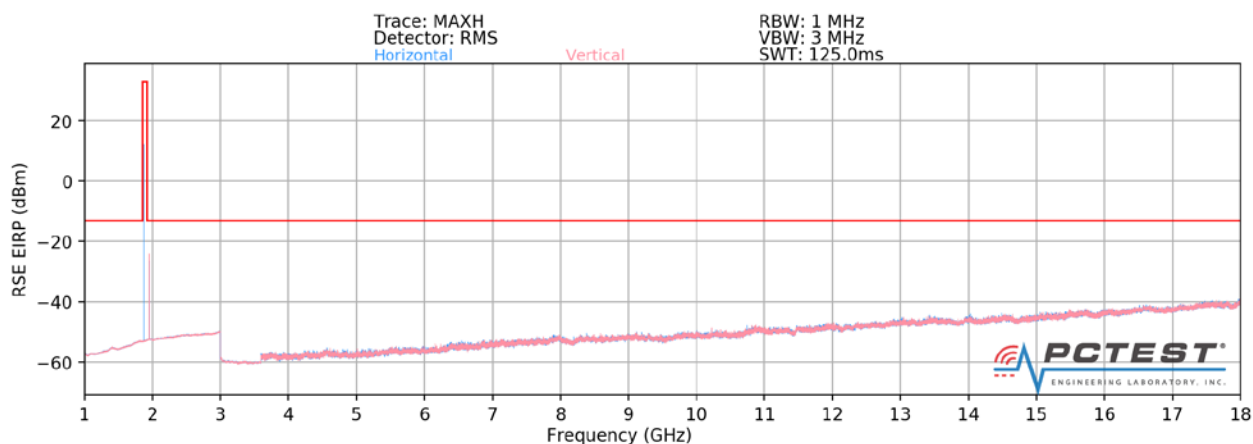
Plot 7-83. Radiated Spurious Plot above 1GHz (PCS GPRS Mode - OPEN)
