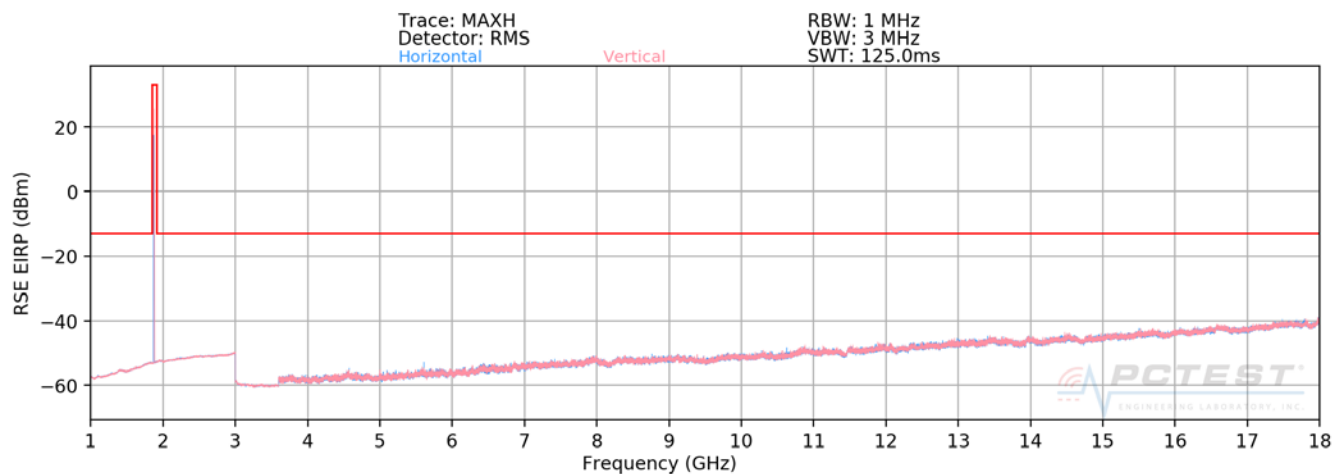
Plot 7-82. Radiated Spurious Plot above 1GHz (PCS GPRS Mode - CLOSED)
