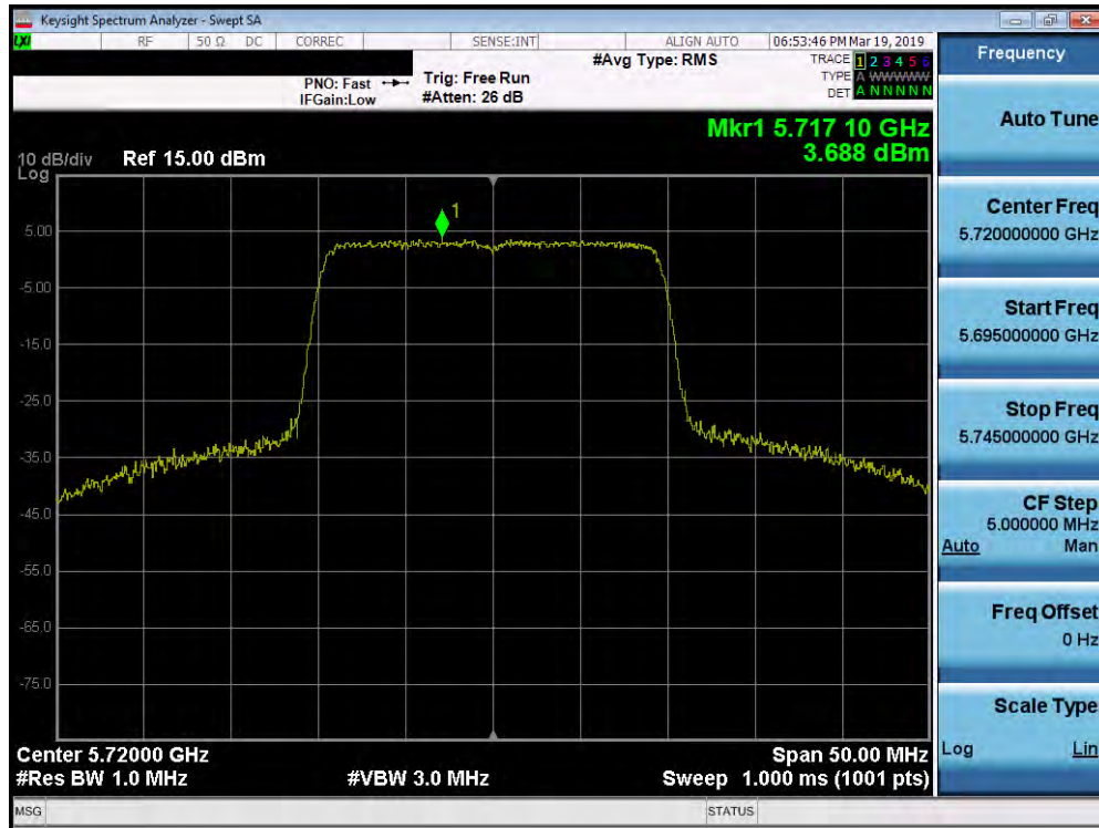
Plot 7-204. Power Spectral Density Plot SISO ANT2 (20MHz BW 802.11ax – 242 Tones (UNII Band 2C) – Ch. 144)
