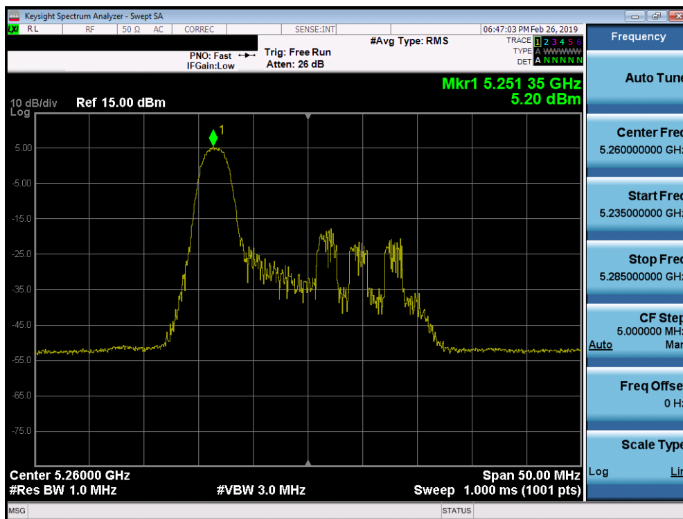
Plot 7-250. Power Spectral Density Plot MIMO ANT2 (20MHz BW 802.11ax – 26 Tones (UNII Band 2A) – Ch. 52)
