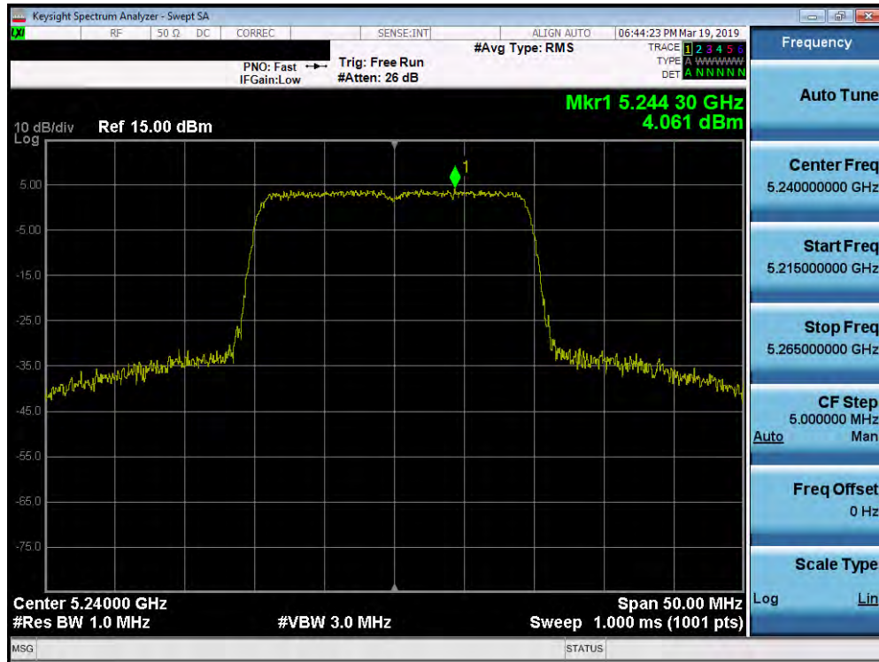
Plot 7-192. Power Spectral Density Plot SISO ANT2 (20MHz BW 802.11ax – 242 Tones (UNII Band 1) – Ch. 48)
