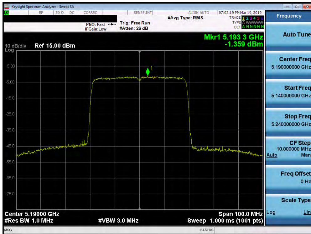
Plot 7-193. Power Spectral Density Plot SISO ANT2 (40MHz BW 802.11ax – 484 Tones (UNII Band 1) – Ch. 38)
