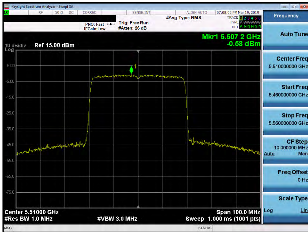
Plot 7-205. Power Spectral Density Plot SISO ANT2 (40MHz BW 802.11ax – 484 Tones (UNII Band 2C) – Ch. 102)
