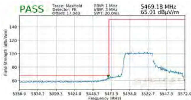
Plot 7-479. Radiated Lower Band Edge Plot SISO ANT2 (Peak – UNII Band 2C – 484 Tones)
