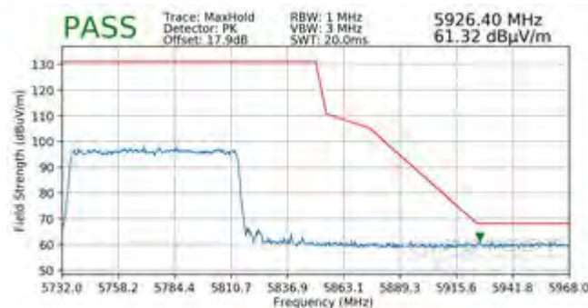
Plot 7-515. Radiated Upper Band Edge Plot MIMO (Peak – UNII Band 3 – 996 Tones)
