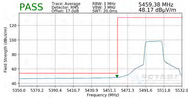
Plot 7-422. Radiated Lower Band Edge Plot SISO ANT1 (Average - UNII Band 2C - 242 Tones)
