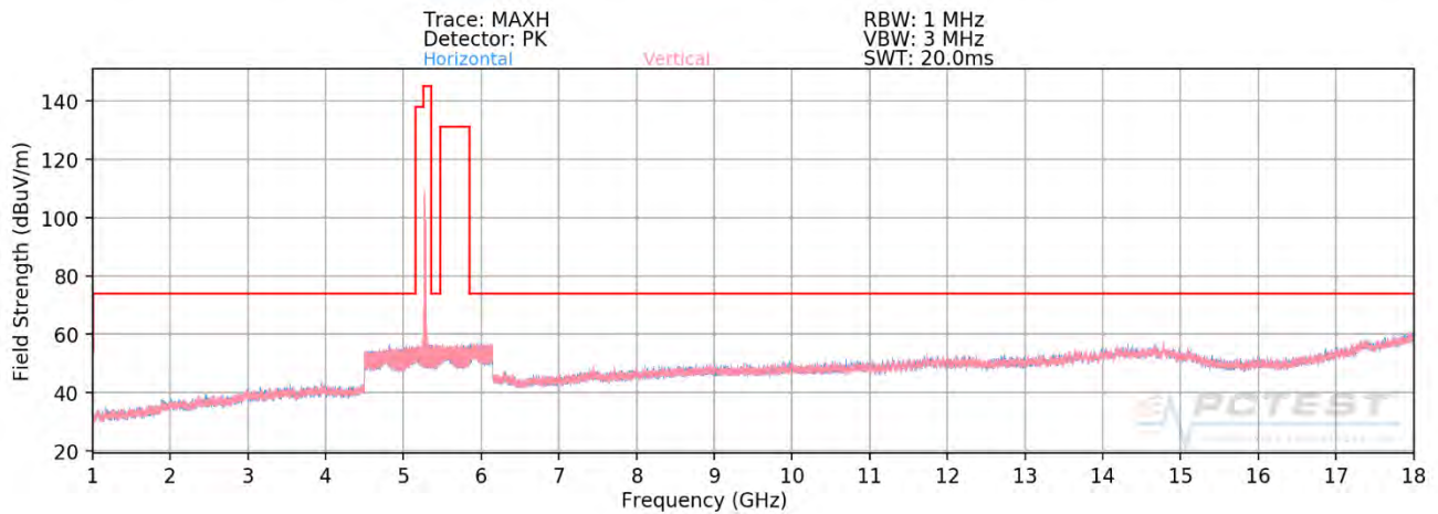
Plot 7-328. Radiated Spurious Plot above 1GHz SISO ANT1 (802.11ax – U2A Ch. 56 – 106 Tones - CLOSED)
