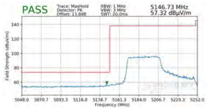
Plot 7-517. Radiated Lower Band Edge Plot MIMO (Peak - UNII Band 1 - 484 Tones)
