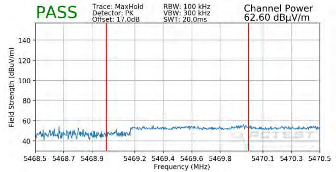
Plot 7-430. Radiated Lower Band Edge Plot SISO ANT1 (Peak – UNII Band 2C – 996 Tones)
