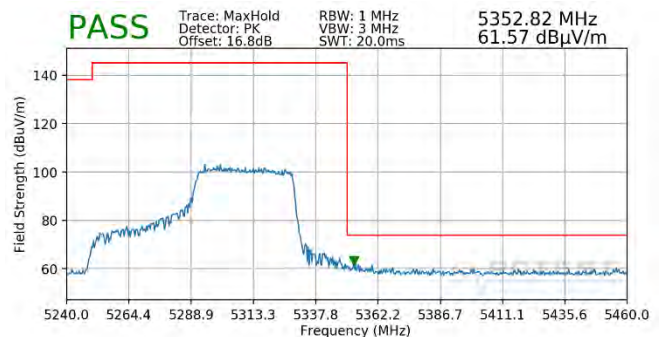
Plot 7-435. Radiated Upper Band Edge Plot SISO ANT1 (Peak - UNII Band 2A - 484 Tones)
