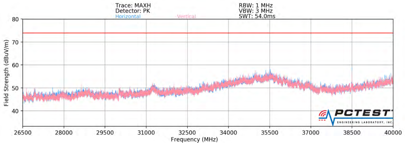
Plot 7-384. Radiated Spurious Plot 26.5GHz - 40GHz MIMO (802.11ax – 106 Tones – CLOSED)
