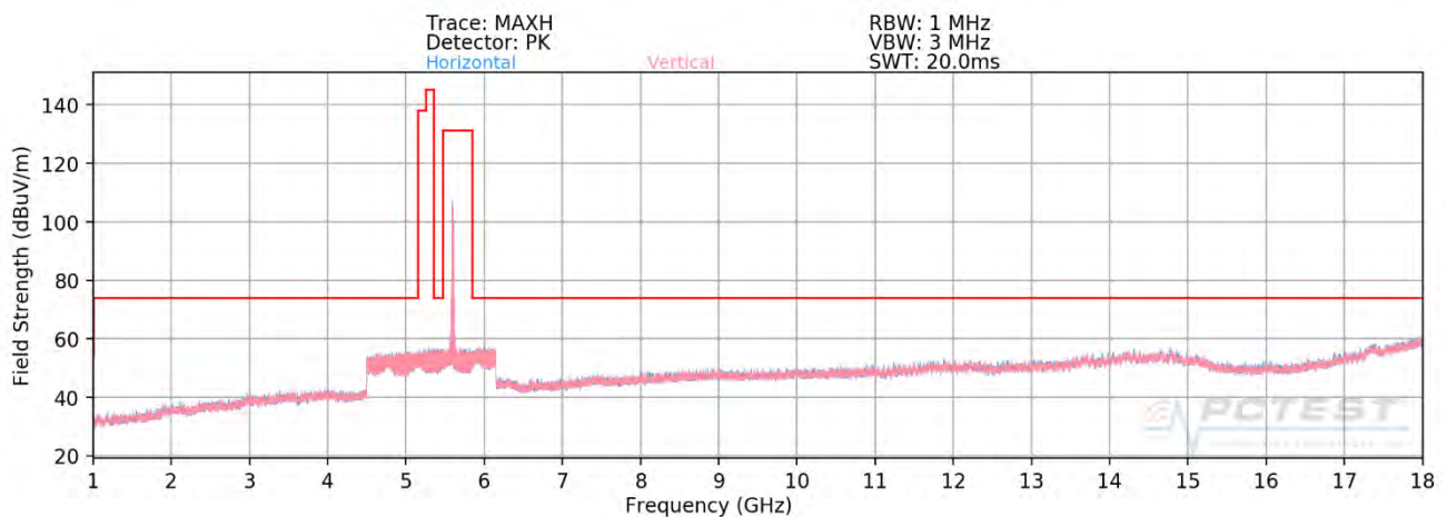
Plot 7-329. Radiated Spurious Plot above 1GHz SISO ANT1 (802.11ax – U2C Ch. 120 – 106 Tones - OPEN)
