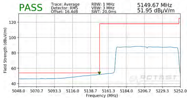
Plot 7-425. Radiated Lower Band Edge Plot SISO ANT1 (Average - UNII Band 1 - 996 Tones)
