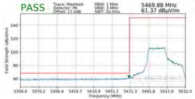
Plot 7-465. Radiated Lower Band Edge Plot SISO ANT2 (Peak – UNII Band 2C – 242 Tones)
