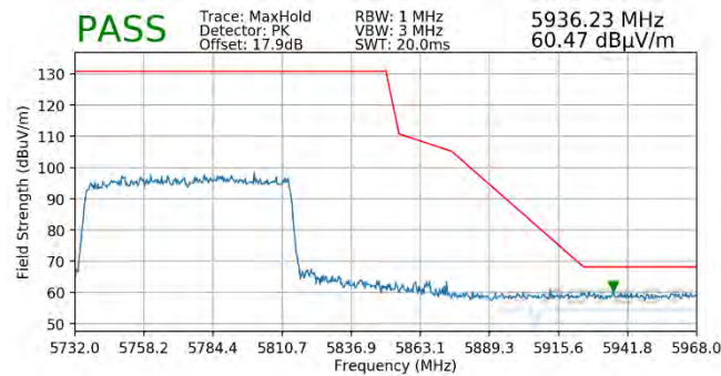
Plot 7-431. Radiated Upper Band Edge Plot SISO ANT1 (Peak – UNII Band 3 – 996 Tones)
