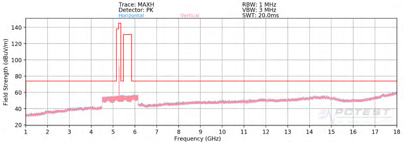
Plot 7-351. Radiated Spurious Plot above 1GHz SISO ANT2 (802.11ax - U2A Ch. 56 - 106 Tones - OPEN)
