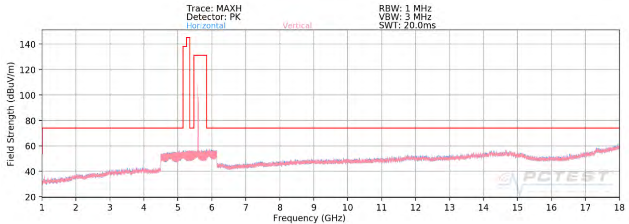
Plot 7-378. Radiated Spurious Plot above 1GHz MIMO (802.11ax – U2C Ch. 120 – 106 Tones - CLOSED)
