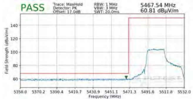
Plot 7-507. Radiated Lower Band Edge Plot MIMO (Peak - UNII Band 2C - 242 Tones)
