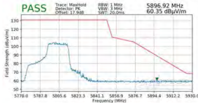
Plot 7-466. Radiated Upper Band Edge Plot SISO ANT2 (Peak – UNII Band 3 – 242 Tones)
