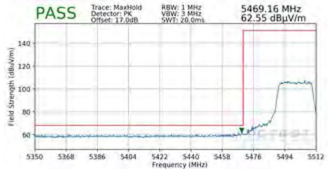
Plot 7-486. Radiated Lower Band Edge Plot MIMO (Peak - UNII Band 2C - 242 Tones)
