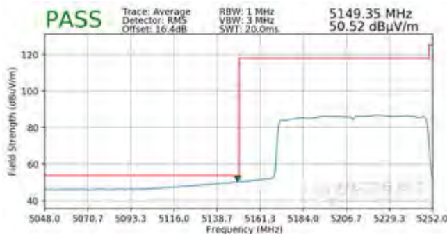
Plot 7-509. Radiated Lower Band Edge Plot MIMO (Average - UNII Band 1 - 996 Tones)
