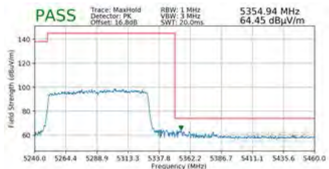
Plot 7-470. Radiated Upper Band Edge Plot SISO ANT2 (Peak - UNII Band 2A - 996 Tones)
