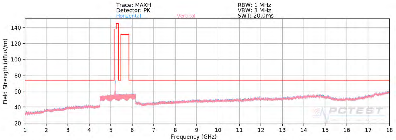
Plot 7-326. Radiated Spurious Plot above 1GHz SISO ANT1 (802.11ax – U1 Ch. 40 – 106 Tones - CLOSED)
