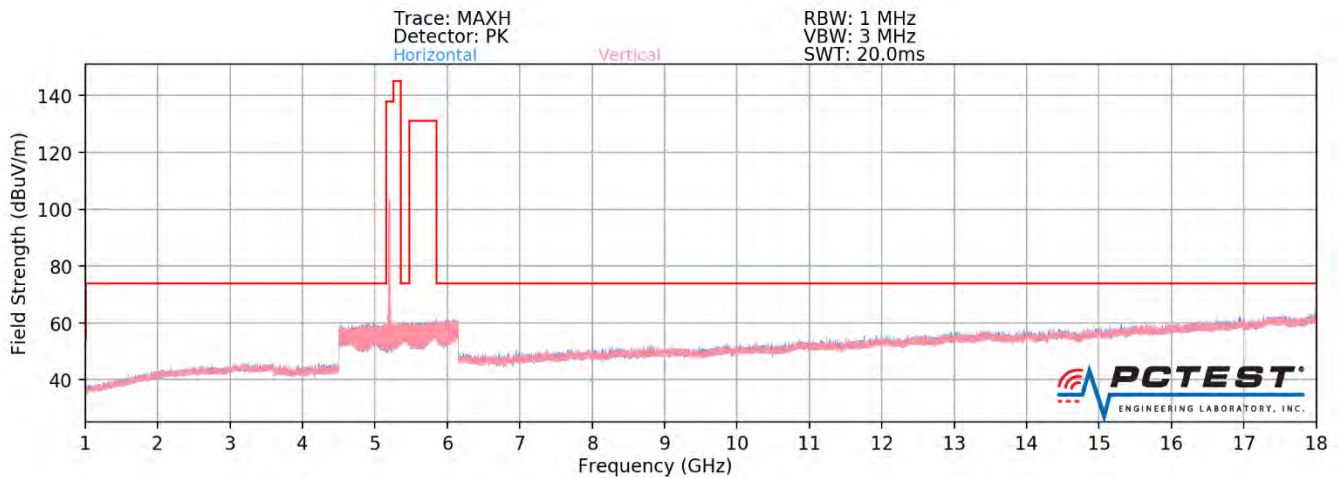
Plot 7-386. Radiated Spurious Plot above 1GHz MIMO (802.11ax - U1 Ch. 40 - 242 Tones - CLOSED)
