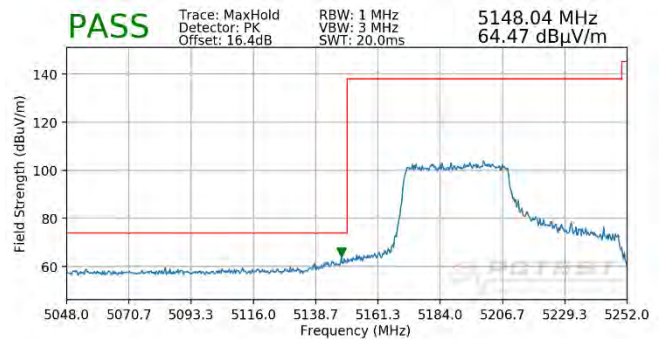
Plot 7-433. Radiated Lower Band Edge Plot SISO ANT1 (Peak - UNII Band 1 - 484 Tones)
