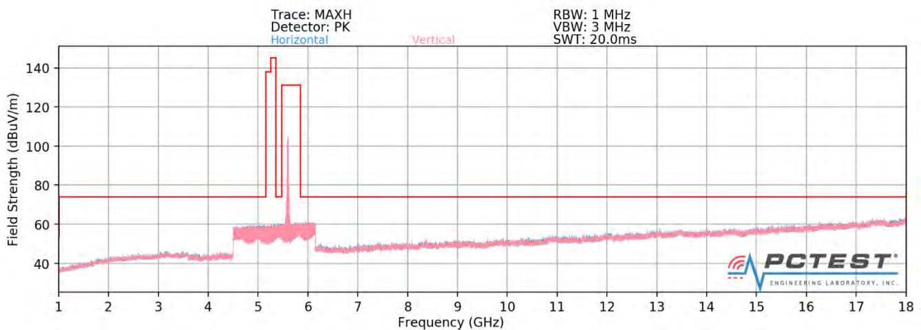
Plot 7-341. Radiated Spurious Plot above 1GHz SISO ANT1 (802.11ax - U2C Ch. 120 - 242 Tones - OPEN)
