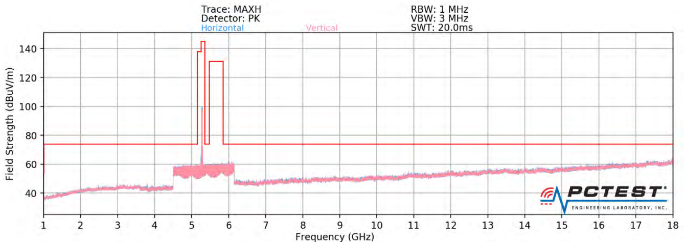
Plot 7-364. Radiated Spurious Plot above 1GHz SISO ANT2 (802.11ax - U2A Ch. 56 - 242 Tones - CLOSED)
