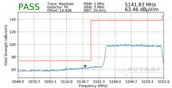
Plot 7-426. Radiated Lower Band Edge Plot SISO ANT1 (Peak - UNII Band 1 - 996 Tones)
