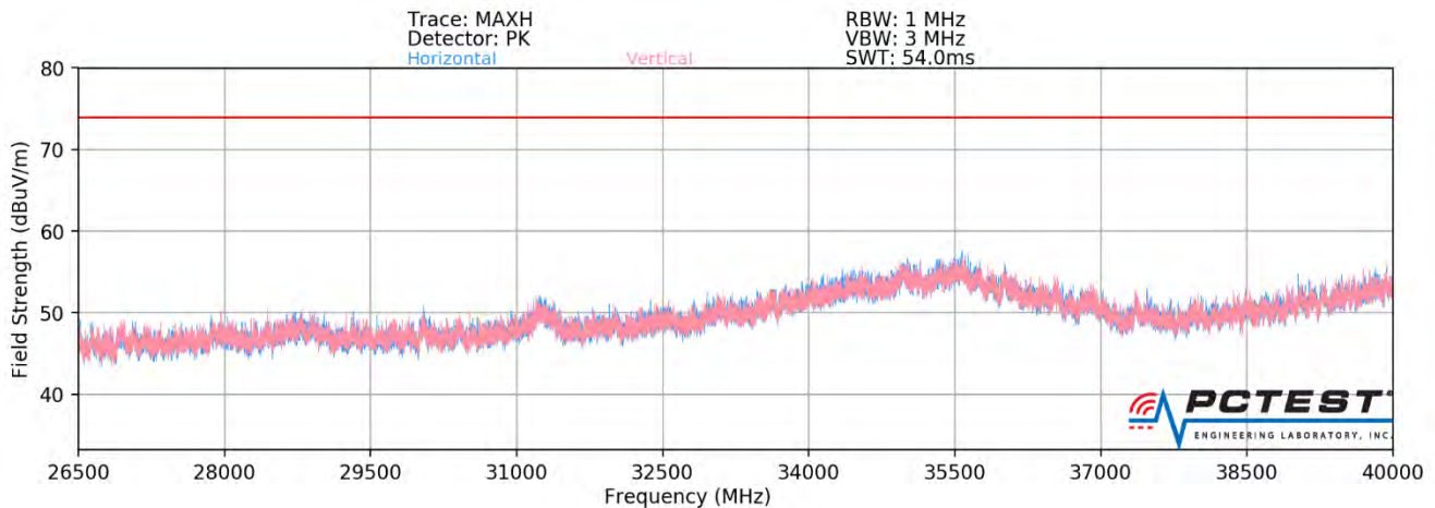
Plot 7-383. Radiated Spurious Plot 26.5GHz - 40GHz MIMO (802.11ax - 106 Tones - OPEN)
