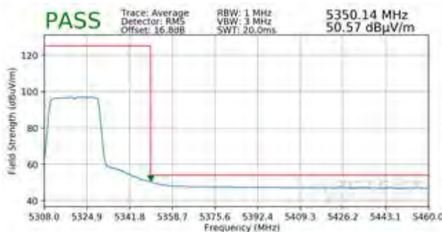
Plot 7-441. Radiated Upper Band Edge Plot SISO ANT2 (Average - UNII Band 2A - 242 Tones)
