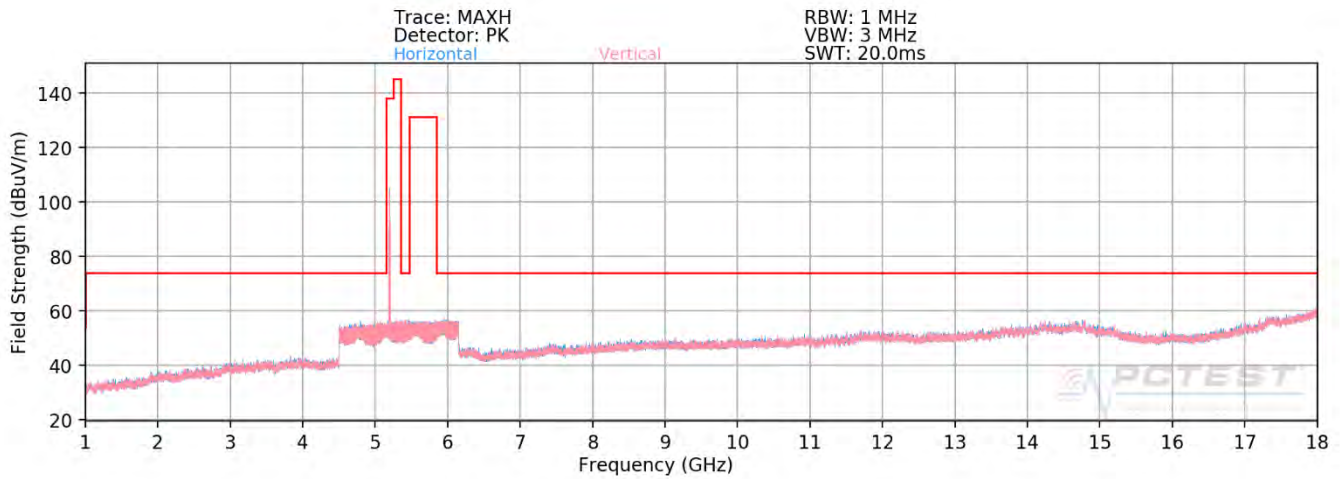
Plot 7-373. Radiated Spurious Plot above 1GHz MIMO (802.11ax – U1 Ch. 40 – 106 Tones - OPEN)
