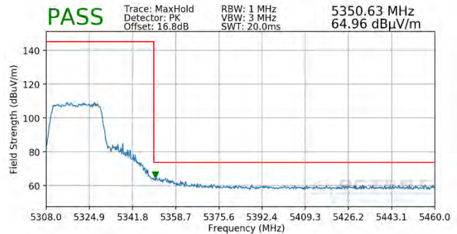
Plot 7-400. Radiated Upper Band Edge Plot SISO ANT1 (Peak - UNII Band 2A - 242 Tones)
