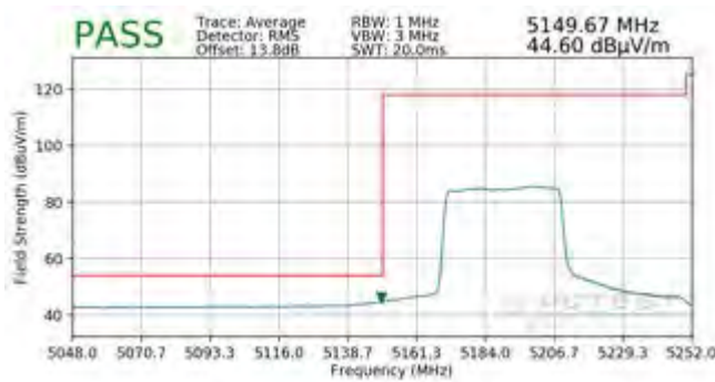
Plot 7-516. Radiated Lower Band Edge Plot MIMO (Average - UNII Band 1 - 484 Tones)
