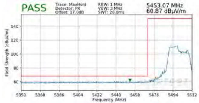
Plot 7-451. Radiated Lower Band Edge Plot SISO ANT2 (Peak – UNII Band 2C – 106 Tones)
