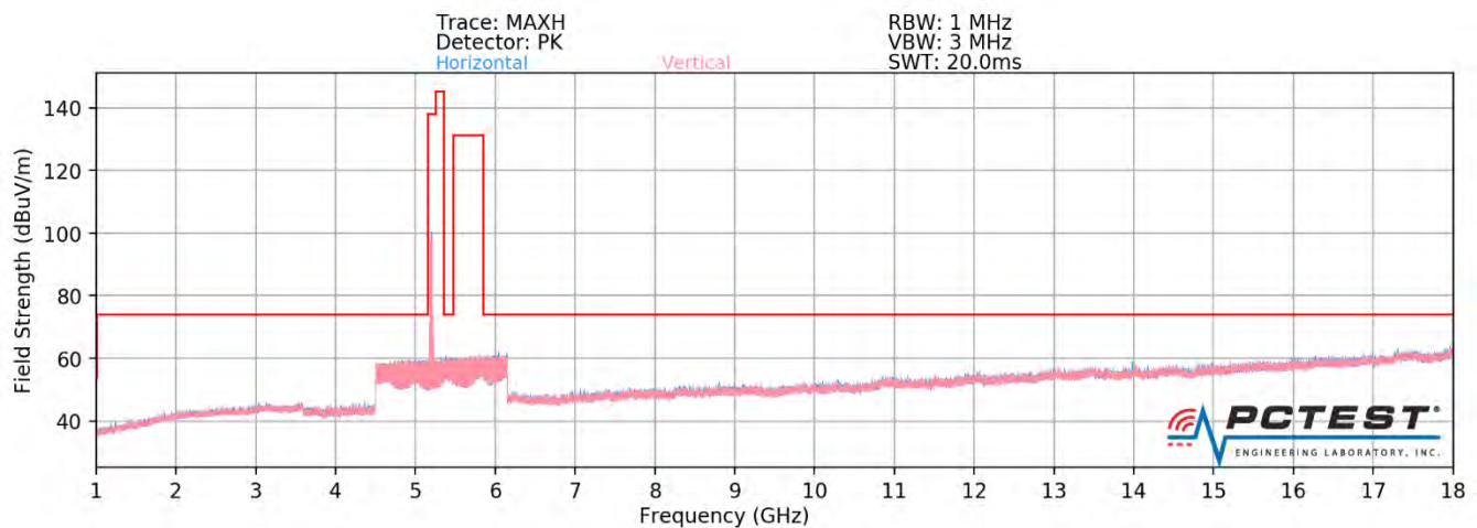
Plot 7-362. Radiated Spurious Plot above 1GHz SISO ANT2 (802.11ax - U1 Ch. 40 - 242 Tones - CLOSED)
