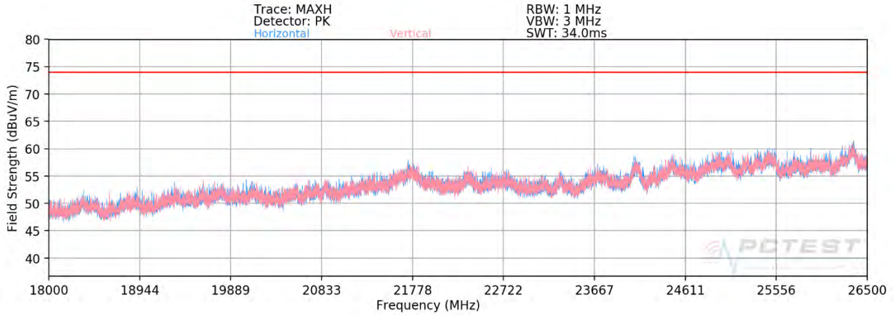
Plot 7-345. Radiated Spurious Plot 18GHz - 26.5GHz SISO ANT1 (802.11ax - 242 Tones - OPEN)
