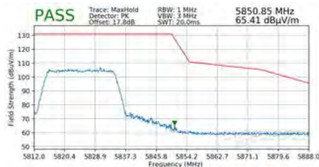
Plot 7-487. Radiated Upper Band Edge Plot MIMO (Peak - UNII Band 3 - 242 Tones)
