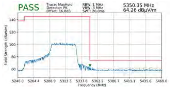
Plot 7-477. Radiated Upper Band Edge Plot SISO ANT2 (Peak - UNII Band 2A - 484 Tones)
