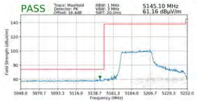
Plot 7-475. Radiated Lower Band Edge Plot SISO ANT2 (Peak - UNII Band 1 - 484 Tones)
