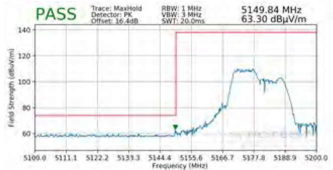
Plot 7-447. Radiated Lower Band Edge Plot SISO ANT2 (Peak - UNII Band 1 - 106 Tones)
