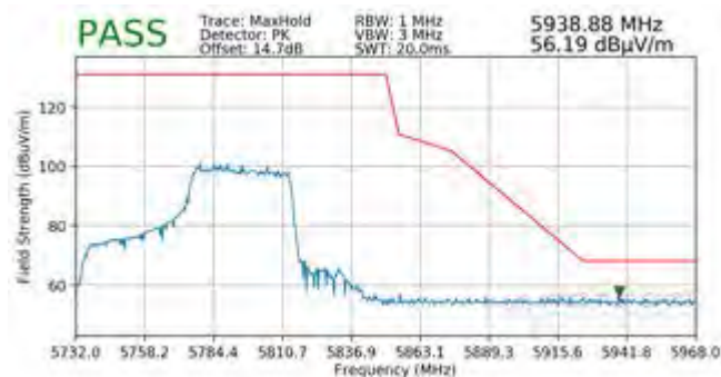
Plot 7-480. Radiated Upper Band Edge Plot SISO ANT2 (Peak – UNII Band 3 – 484 Tones)
