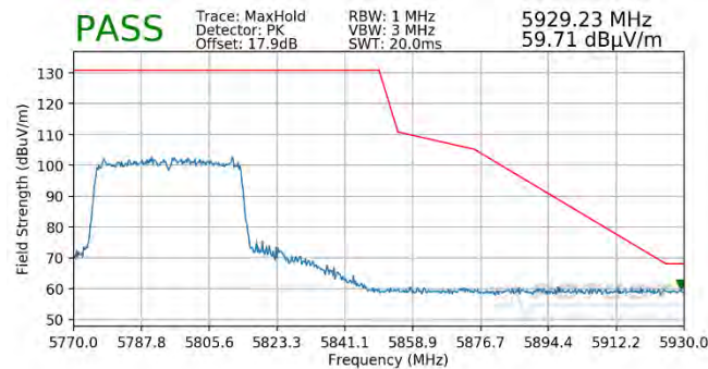
Plot 7-417. Radiated Upper Band Edge Plot SISO ANT1 (Peak – UNII Band 3 – 484 Tones)
