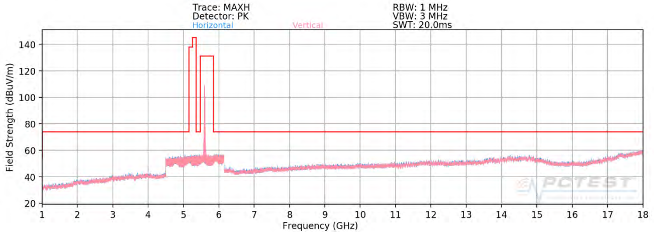
Plot 7-330. Radiated Spurious Plot above 1GHz SISO ANT1 (802.11ax – U2C Ch. 120 – 106 Tones - CLOSED)
