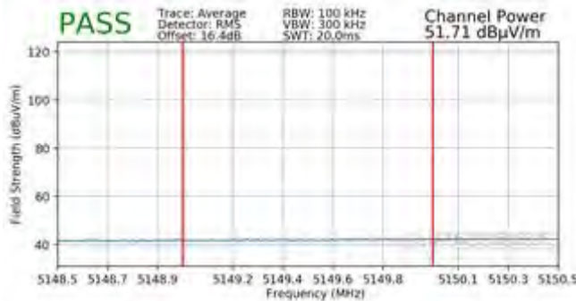
Plot 7-411. Radiated Lower Band Edge Plot SISO ANT1 (Average - UNII Band 1 - 484 Tones)
