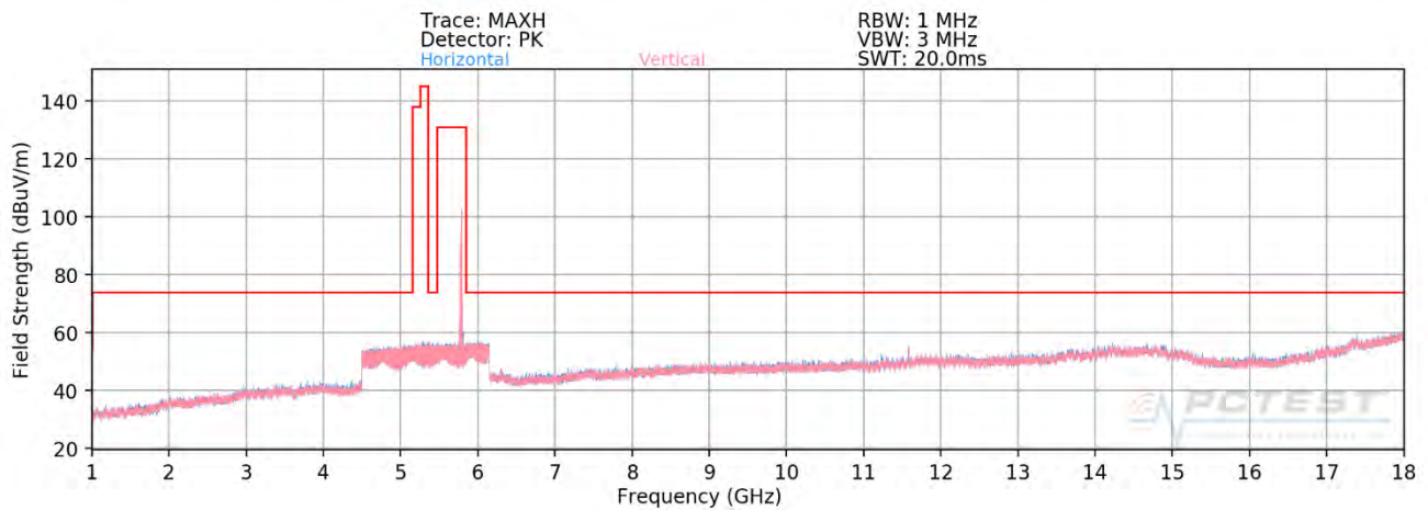
Plot 7-331. Radiated Spurious Plot above 1GHz SISO ANT1 (802.11ax – U3 Ch. 157 – 106 Tones - OPEN)
