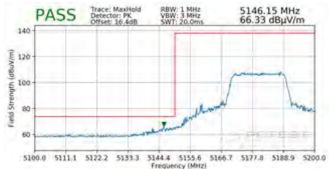
Plot 7-440. Radiated Lower Band Edge Plot SISO ANT2 (Peak - UNII Band 1 - 242 Tones)
