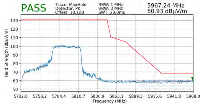
Plot 7-438. Radiated Upper Band Edge Plot SISO ANT1 (Peak – UNII Band 3 – 484 Tones)
