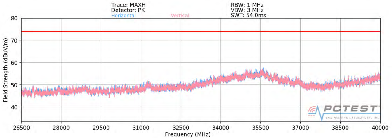
Plot 7-347. Radiated Spurious Plot 26.5GHz - 40GHz SISO ANT1 (802.11ax - 242 Tones - OPEN)
