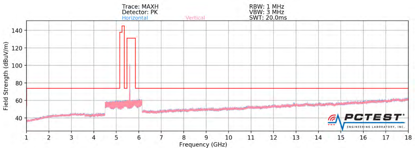
Plot 7-365. Radiated Spurious Plot above 1GHz SISO ANT2 (802.11ax - U2C Ch. 120 - 242 Tones - OPEN)
