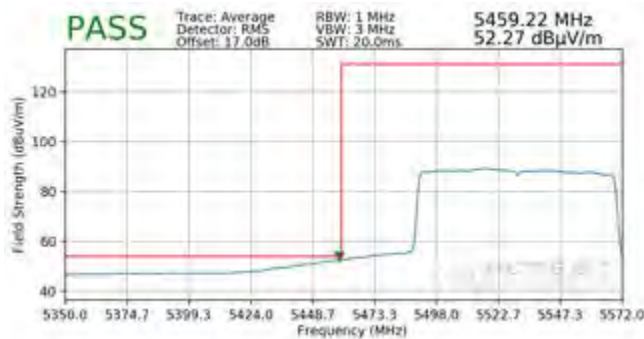
Plot 7-471. Radiated Lower Band Edge Plot SISO ANT2 (Average – UNII Band 2C – 996 Tones)
