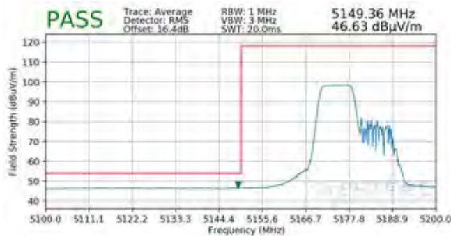
Plot 7-446. Radiated Lower Band Edge Plot SISO ANT2 (Average - UNII Band 1 - 106 Tones)
