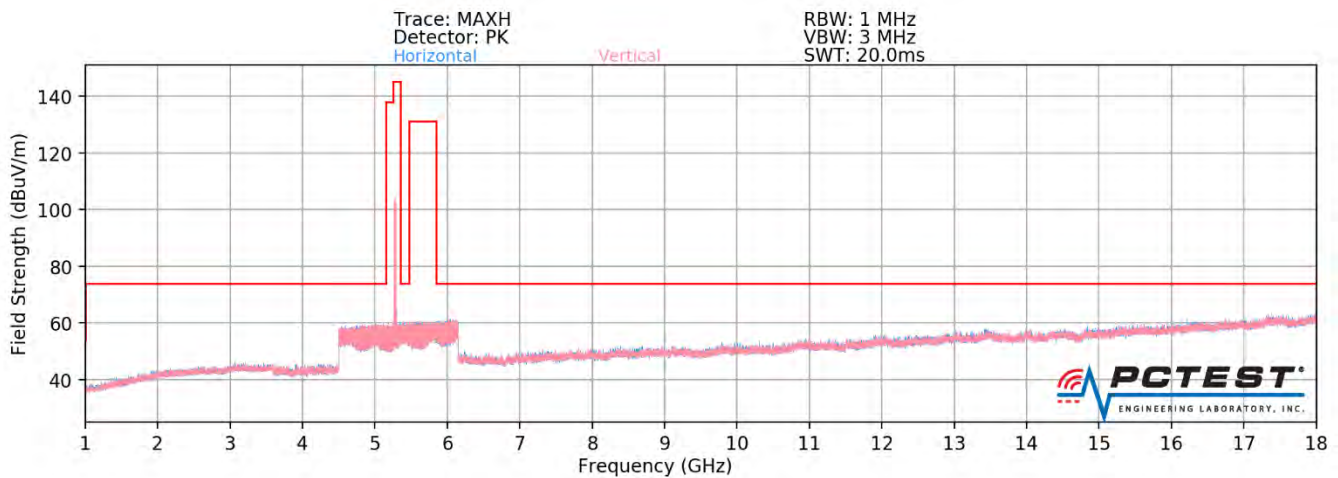
Plot 7-388. Radiated Spurious Plot above 1GHz MIMO (802.11ax – U2A Ch. 56 – 242 Tones – CLOSED)
