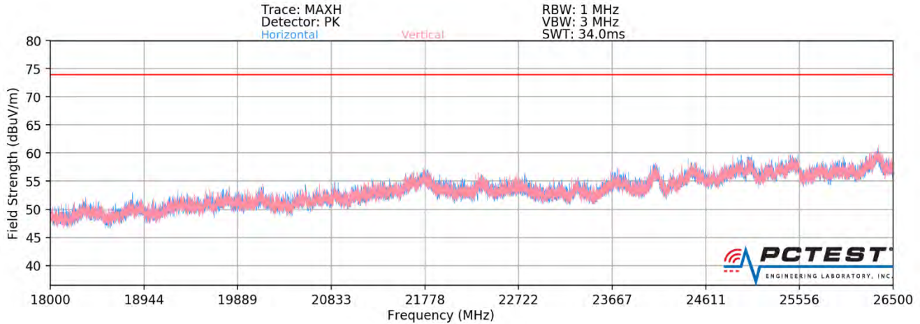
Plot 7-381. Radiated Spurious Plot above 18GHz - 26.5GHz MIMO (802.11ax - 106 Tones - OPEN)
