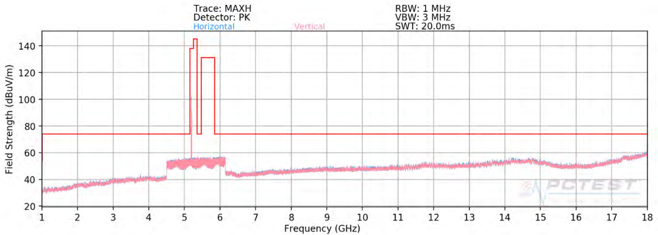
Plot 7-350. Radiated Spurious Plot above 1GHz SISO ANT2 (802.11ax - U1 Ch. 40 - 106 Tones - CLOSED)
