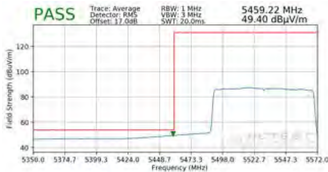
Plot 7-513. Radiated Lower Band Edge Plot MIMO (Average – UNII Band 2C – 996 Tones)
