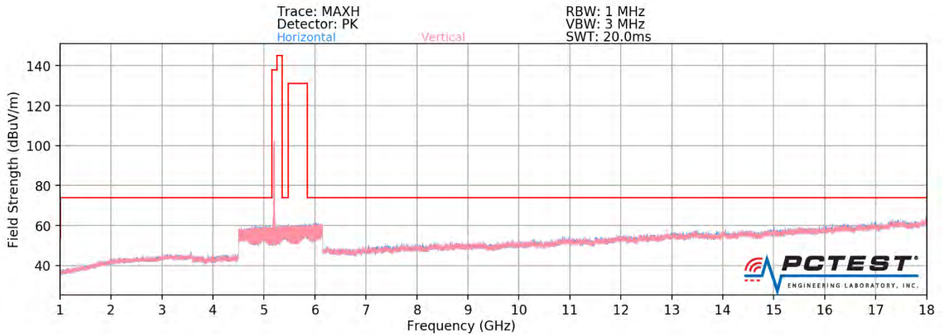
Plot 7-385. Radiated Spurious Plot above 1GHz MIMO (802.11ax - U1 Ch. 40 - 242 Tones - OPEN)
