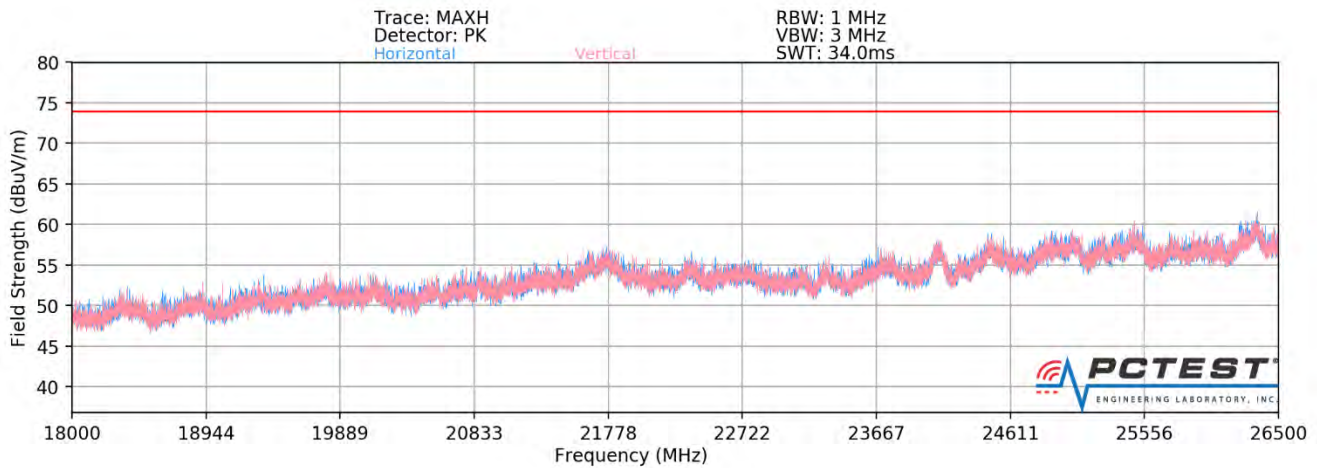
Plot 7-358. Radiated Spurious Plot above 18GHz - 26.5GHz SISO ANT2 (802.11ax - 106 Tones - CLOSED)
