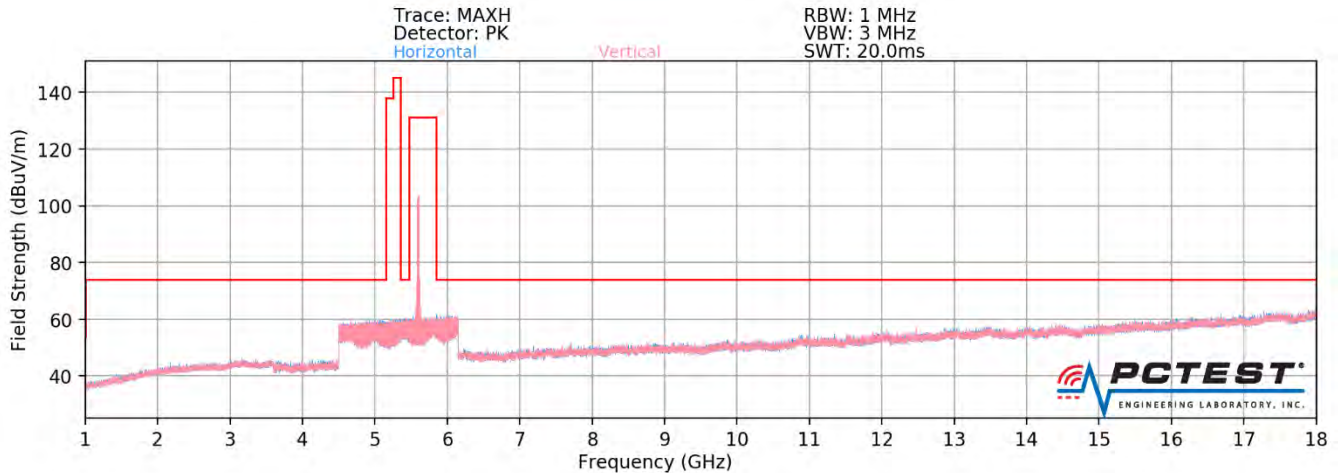
Plot 7-390. Radiated Spurious Plot above 1GHz MIMO (802.11ax – U2C Ch. 120 – 242 Tones – CLOSED)
