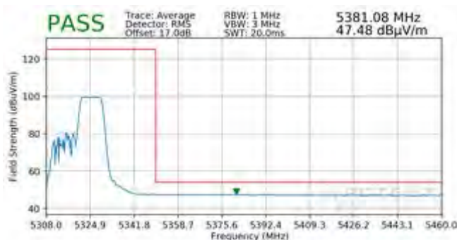
Plot 7-448. Radiated Upper Band Edge Plot SISO ANT2 (Average - UNII Band 2A - 106 Tones)
