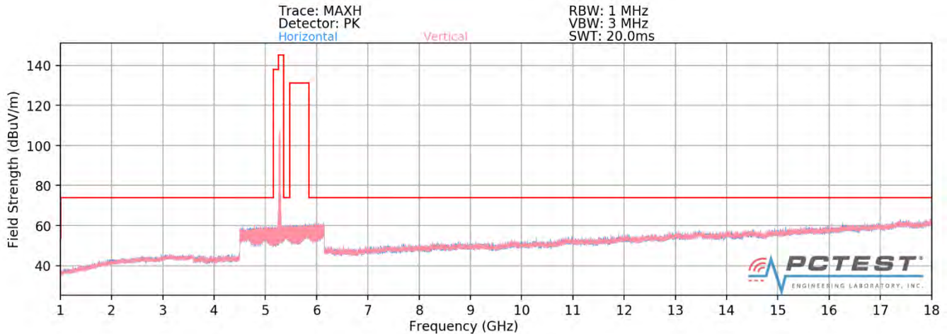
Plot 7-339. Radiated Spurious Plot above 1GHz SISO ANT1 (802.11ax - U2A Ch. 56 - 242 Tones - OPEN)
