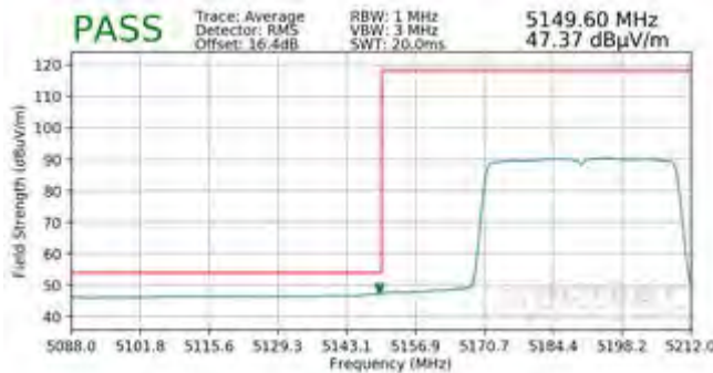
Plot 7-453. Radiated Lower Band Edge Plot SISO ANT2 (Average - UNII Band 1 - 484 Tones)
