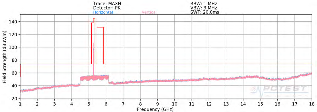
Plot 7-375. Radiated Spurious Plot above 1GHz MIMO (802.11ax – U2A Ch. 56 – 106 Tones - OPEN)
