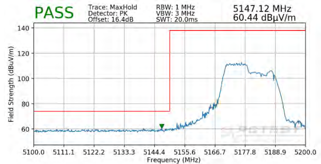
Plot 7-405. Radiated Lower Band Edge Plot SISO ANT1 (Peak - UNII Band 1 - 106 Tones)
