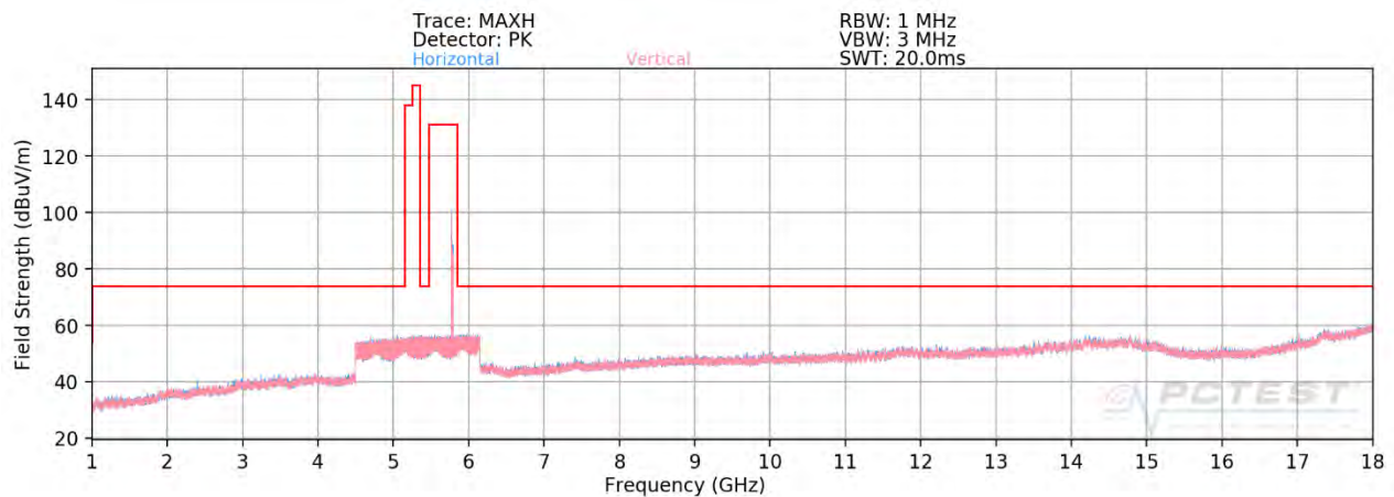
Plot 7-355. Radiated Spurious Plot above 1GHz SISO ANT2 (802.11ax – U3 Ch. 157 – 106 Tones - OPEN)
