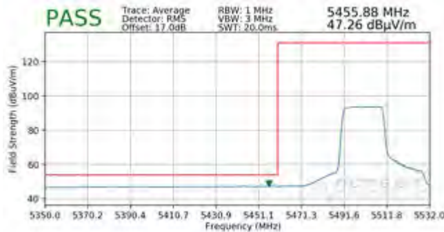
Plot 7-506. Radiated Lower Band Edge Plot MIMO (Average - UNII Band 2C - 242 Tones)
