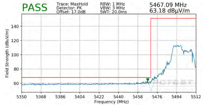
Plot 7-409. Radiated Lower Band Edge Plot SISO ANT1 (Peak - UNII Band 2C - 106 Tones)
