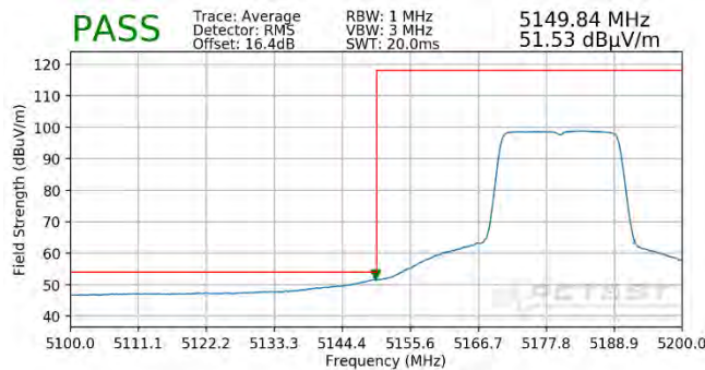
Plot 7-397. Radiated Lower Band Edge Plot SISO ANT1 (Average - UNII Band 1 - 242 Tones)
