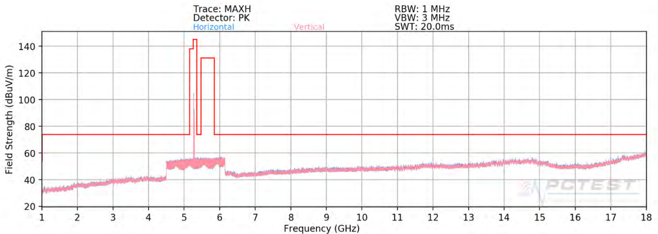
Plot 7-352. Radiated Spurious Plot above 1GHz SISO ANT2 (802.11ax - U2A Ch. 56 - 106 Tones - CLOSED)
