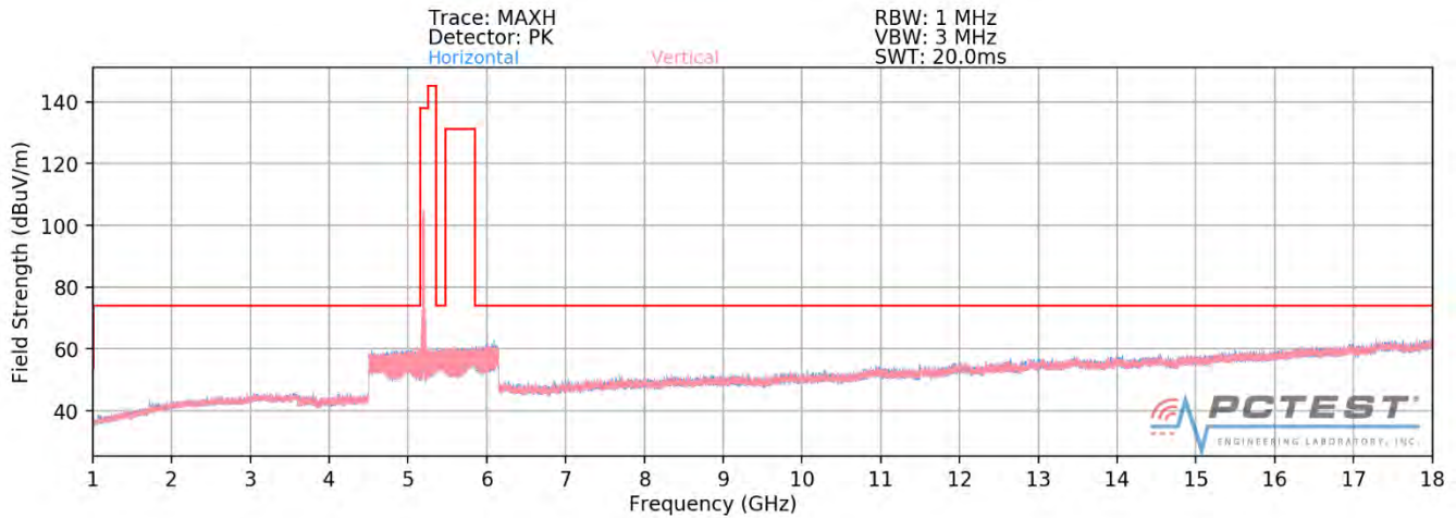
Plot 7-337. Radiated Spurious Plot above 1GHz SISO ANT1 (802.11ax - U1 Ch. 40 - 242 Tones - OPEN)
