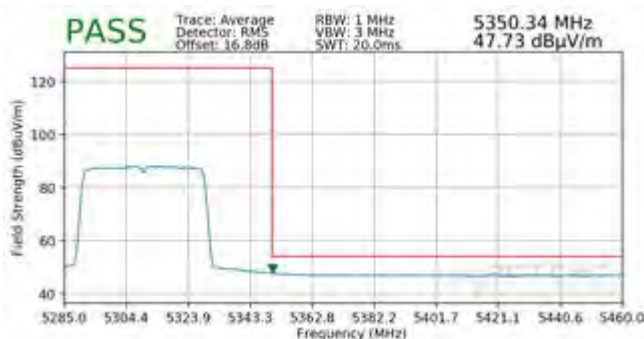
Plot 7-497. Radiated Upper Band Edge Plot MIMO (Average - UNII Band 2A - 484 Tones)
