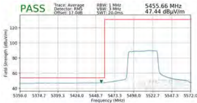
Plot 7-520. Radiated Lower Band Edge Plot MIMO (Average - UNII Band 2C - 484 Tones)
