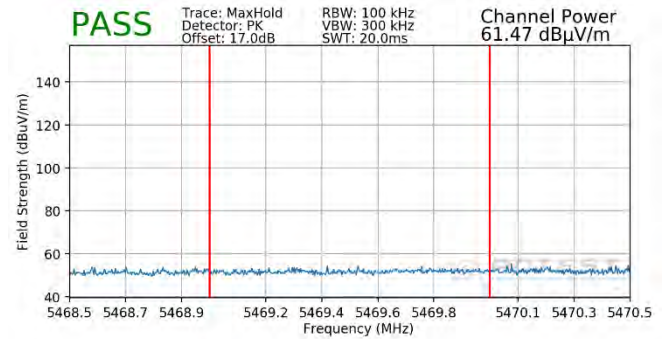
Plot 7-437. Radiated Lower Band Edge Plot SISO ANT1 (Peak – UNII Band 2C – 484 Tones)
