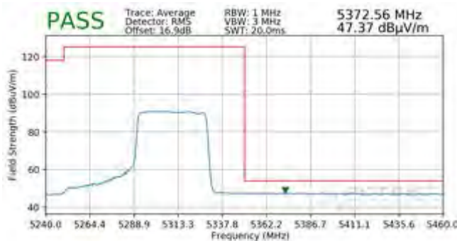
Plot 7-476. Radiated Upper Band Edge Plot SISO ANT2 (Average - UNII Band 2A - 484 Tones)
