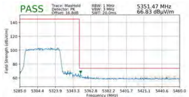
Plot 7-456. Radiated Upper Band Edge Plot SISO ANT2 (Peak - UNII Band 2A - 484 Tones)
