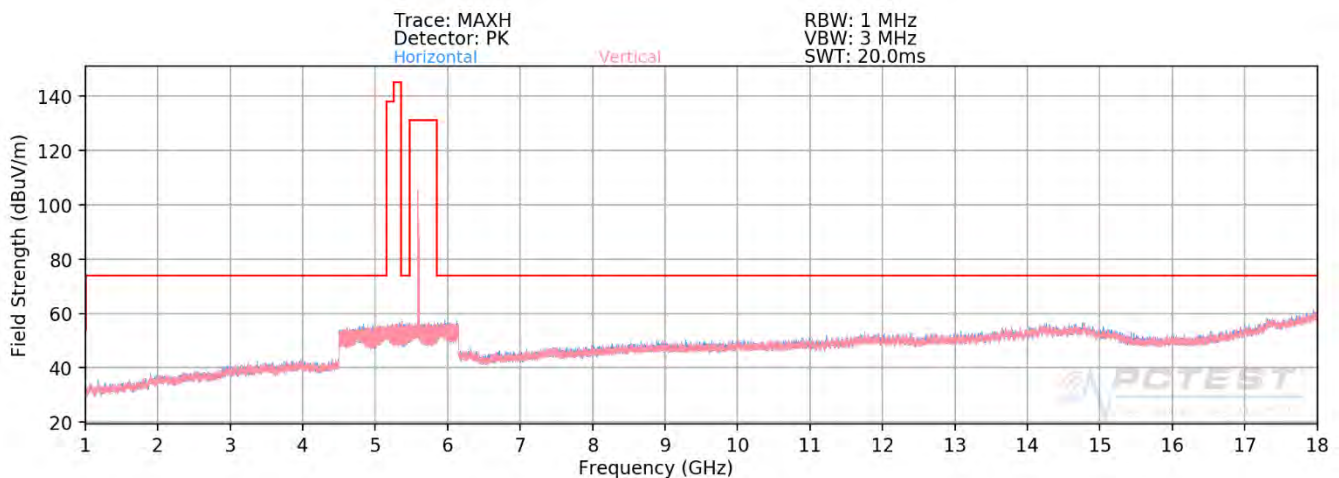
Plot 7-377. Radiated Spurious Plot above 1GHz MIMO (802.11ax – U2C Ch. 120 – 106 Tones - OPEN)
