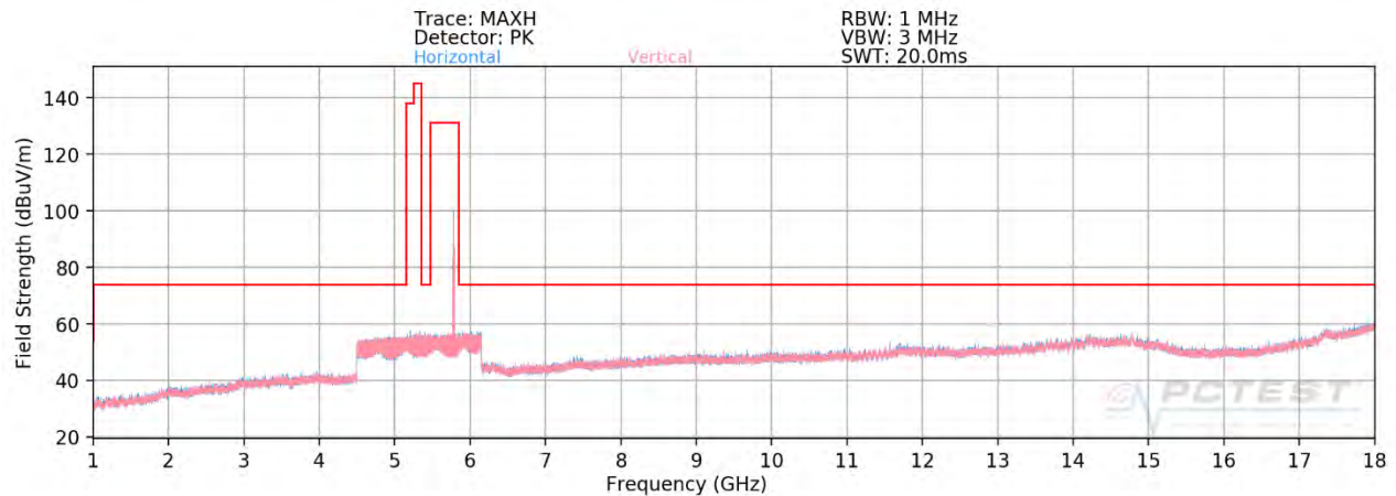
Plot 7-379. Radiated Spurious Plot above 1GHz MIMO (802.11ax – U3 Ch. 157 – 106 Tones - OPEN)
