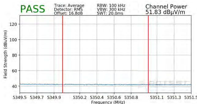
Plot 7-413. Radiated Upper Band Edge Plot SISO ANT1 (Average - UNII Band 2A - 484 Tones)
