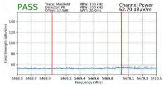
Plot 7-458. Radiated Lower Band Edge Plot SISO ANT2 (Peak – UNII Band 2C – 484 Tones)
