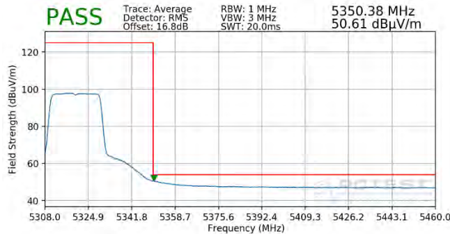
Plot 7-399. Radiated Upper Band Edge Plot SISO ANT1 (Average - UNII Band 2A - 242 Tones)
