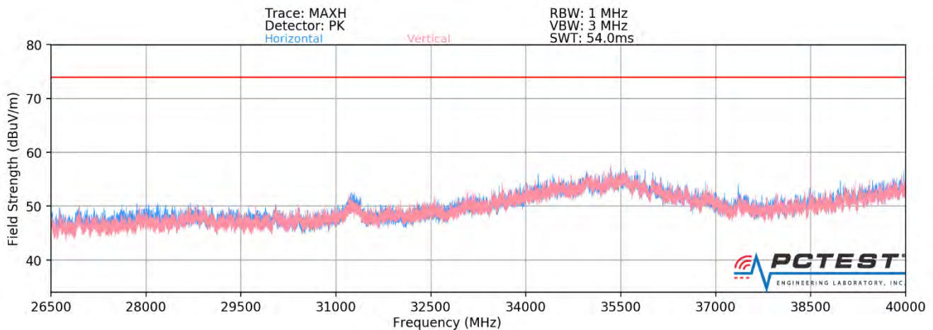
Plot 7-359. Radiated Spurious Plot 26.5GHz - 40GHz SISO ANT2 (802.11ax - 106 Tones - OPEN)
