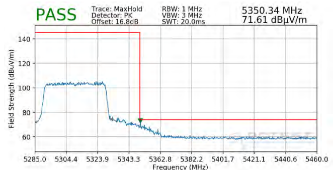
Plot 7-414. Radiated Upper Band Edge Plot SISO ANT1 (Peak - UNII Band 2A - 484 Tones)
