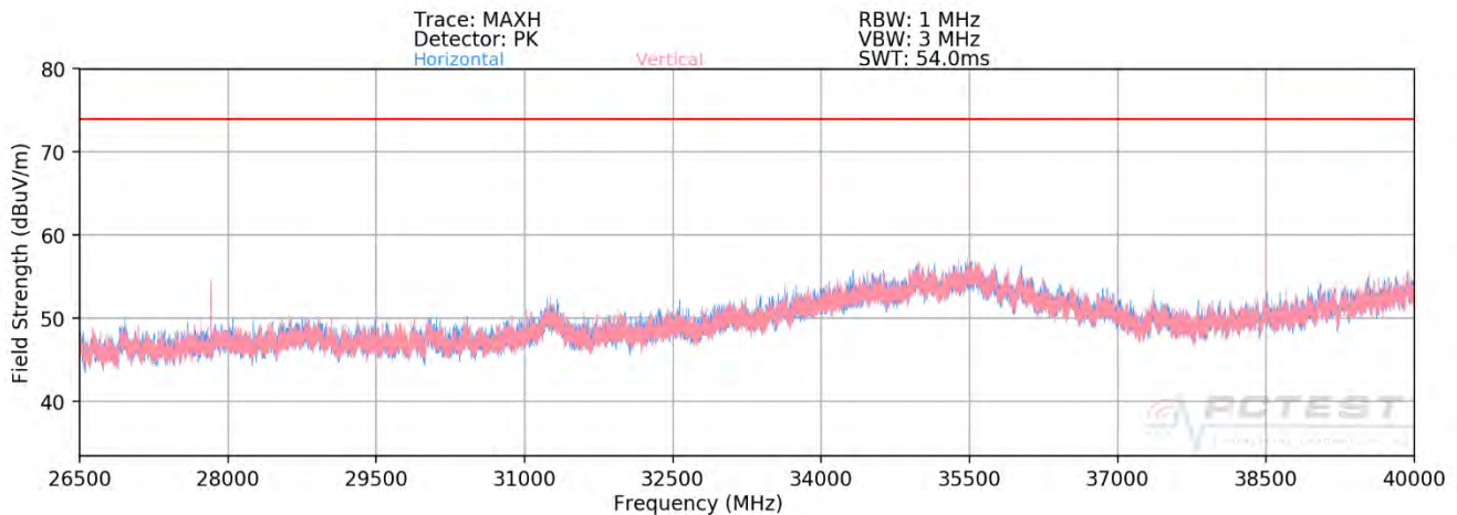
Plot 7-335. Radiated Spurious Plot 26.5GHz - 40GHz SISO ANT1 (802.11ax - 106 Tones - OPEN)
