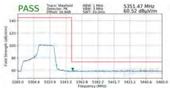
Plot 7-505. Radiated Upper Band Edge Plot MIMO (Peak - UNII Band 2A - 242 Tones)
