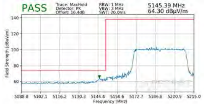
Plot 7-454. Radiated Lower Band Edge Plot SISO ANT2 (Peak - UNII Band 1 - 484 Tones)
