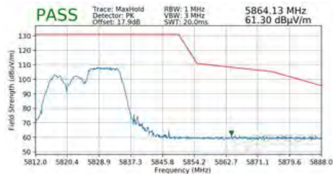
Plot 7-494. Radiated Upper Band Edge Plot MIMO (Peak - UNII Band 3 - 106 Tones)
