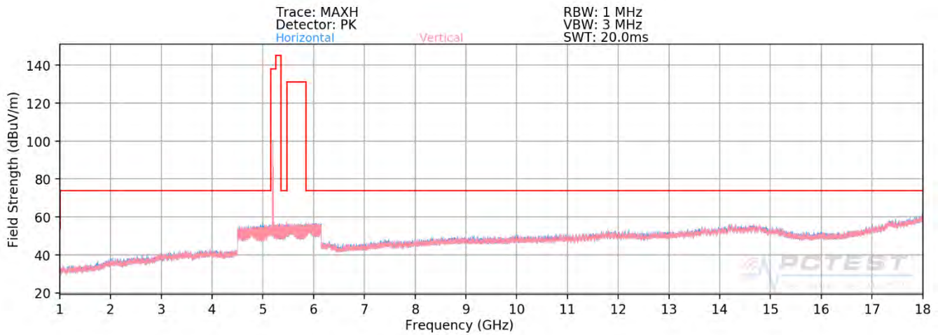
Plot 7-349. Radiated Spurious Plot above 1GHz SISO ANT2 (802.11ax - U1 Ch. 40 - 106 Tones - OPEN)
