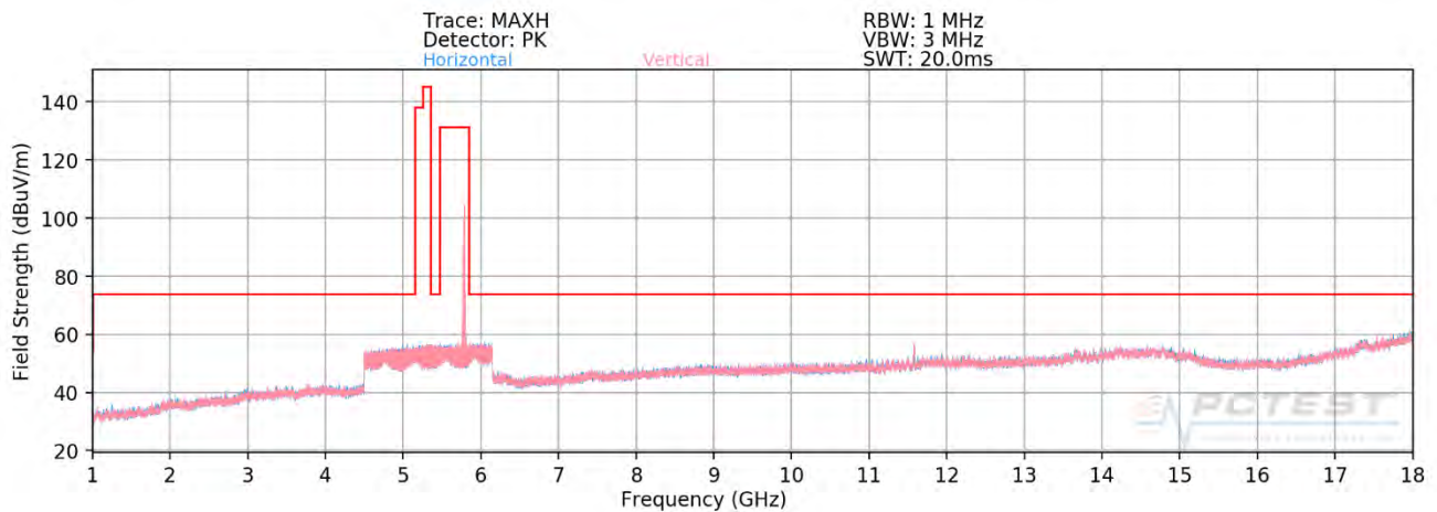
Plot 7-332. Radiated Spurious Plot above 1GHz SISO ANT1 (802.11ax – U3 Ch. 157 – 106 Tones - CLOSED)
