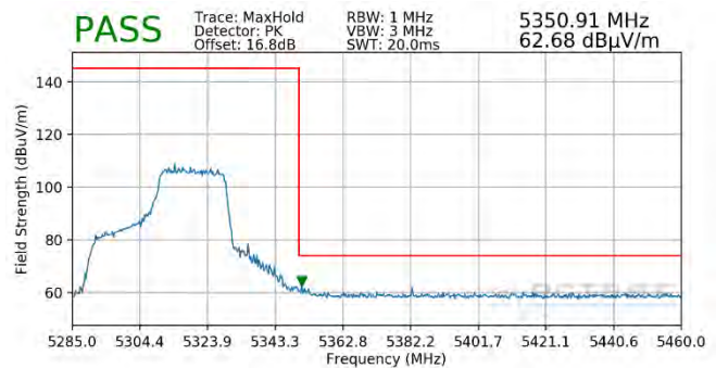
Plot 7-421. Radiated Upper Band Edge Plot SISO ANT1 (Peak - UNII Band 2A - 242 Tones)
