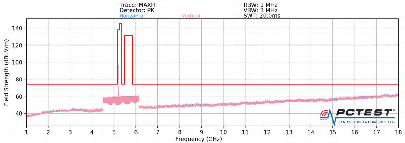
Plot 7-361. Radiated Spurious Plot above 1GHz SISO ANT2 (802.11ax - U1 Ch. 40 - 242 Tones - OPEN)
