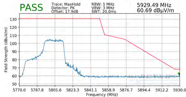
Plot 7-424. Radiated Upper Band Edge Plot SISO ANT1 (Peak - UNII Band 3 - 242 Tones)
