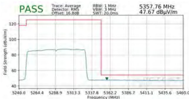
Plot 7-469. Radiated Upper Band Edge Plot SISO ANT2 (Average - UNII Band 2A - 996 Tones)
