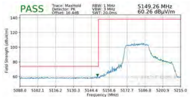
Plot 7-461. Radiated Lower Band Edge Plot SISO ANT2 (Peak - UNII Band 1 - 242 Tones)
