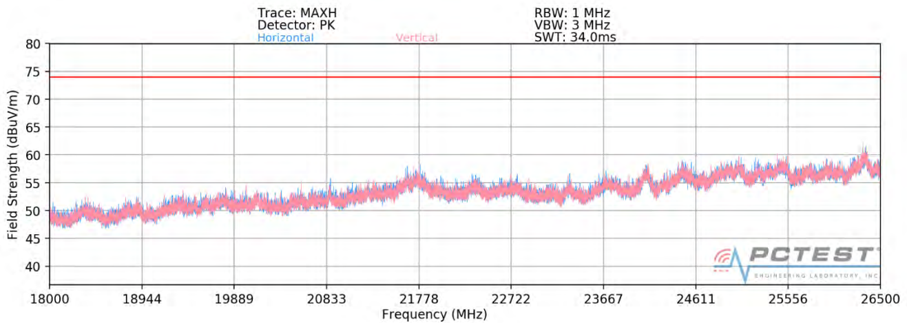
Plot 7-334. Radiated Spurious Plot 18GHz - 26.5GHz SISO ANT1 (802.11ax - 106 Tones - CLOSED)
