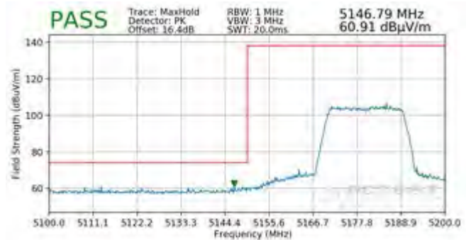
Plot 7-482. Radiated Lower Band Edge Plot MIMO (Peak – UNII Band 1 – 242 Tones)
