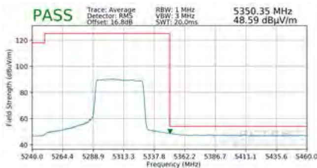
Plot 7-518. Radiated Upper Band Edge Plot MIMO (Average - UNII Band 2A - 484 Tones)
