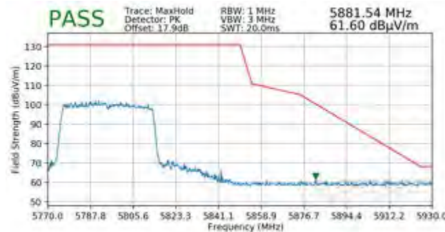
Plot 7-459. Radiated Upper Band Edge Plot SISO ANT2 (Peak – UNII Band 3 – 484 Tones)
