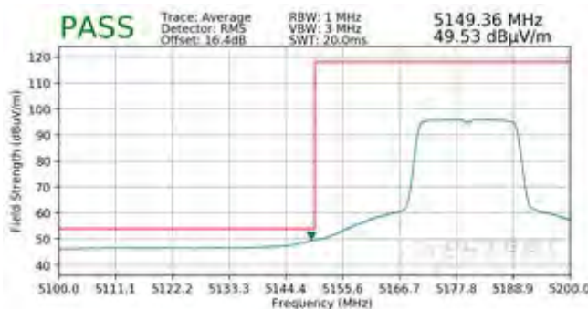
Plot 7-439. Radiated Lower Band Edge Plot SISO ANT2 (Average - UNII Band 1 - 242 Tones)
