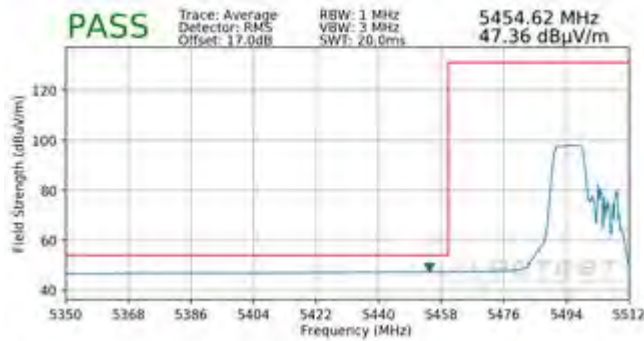
Plot 7-492. Radiated Lower Band Edge Plot MIMO (Average - UNII Band 2C - 106 Tones)
