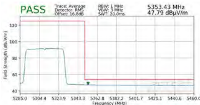
Plot 7-455. Radiated Upper Band Edge Plot SISO ANT2 (Average - UNII Band 2A - 484 Tones)
