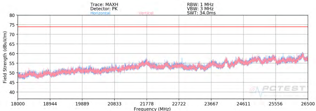
Plot 7-370. Radiated Spurious Plot above 18GHz - 26.5GHz SISO ANT2 (802.11ax - 242 Tones - CLOSED)
