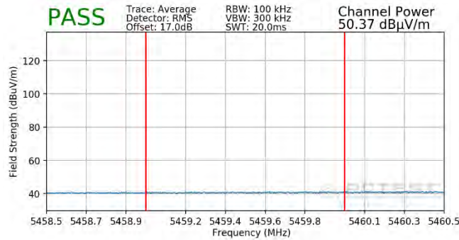
Plot 7-401. Radiated Lower Band Edge Plot SISO ANT1 (Average - UNII Band 2C - 242 Tones)
