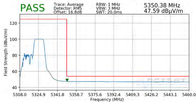
Plot 7-406. Radiated Upper Band Edge Plot SISO ANT1 (Average - UNII Band 2A - 106 Tones)
