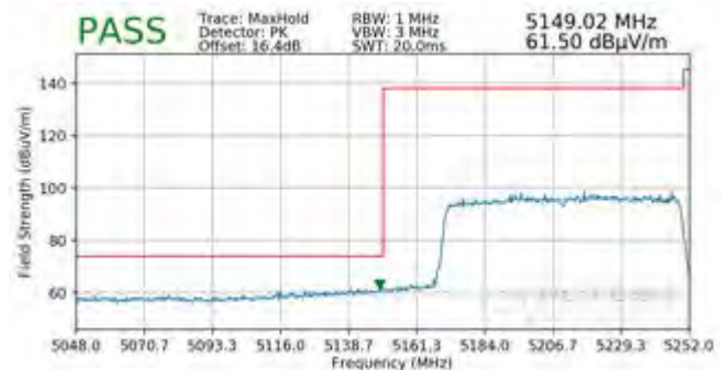
Plot 7-510. Radiated Lower Band Edge Plot MIMO (Peak - UNII Band 1 - 996 Tones)
