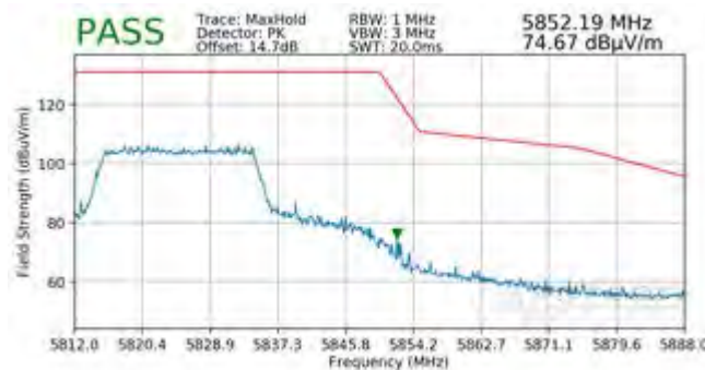
Plot 7-445. Radiated Upper Band Edge Plot SISO ANT2 (Peak – UNII Band 3 – 242 Tones)
