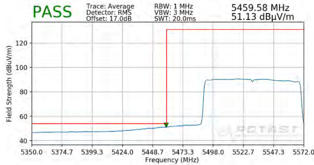
Plot 7-429. Radiated Lower Band Edge Plot SISO ANT1 (Average – UNII Band 2C – 996 Tones)
