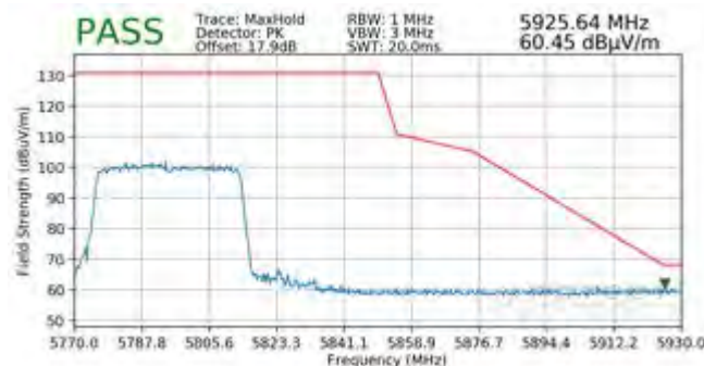
Plot 7-501. Radiated Upper Band Edge Plot MIMO (Peak - UNII Band 3 - 484 Tones)
