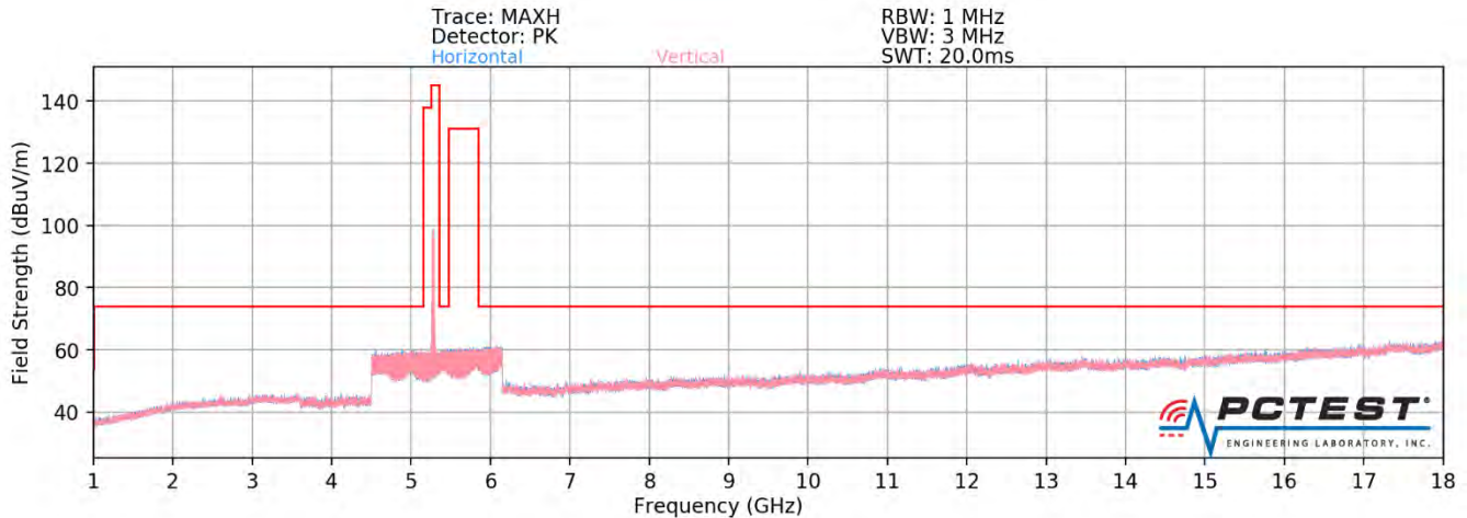
Plot 7-363. Radiated Spurious Plot above 1GHz SISO ANT2 (802.11ax - U2A Ch. 56 - 242 Tones - OPEN)
