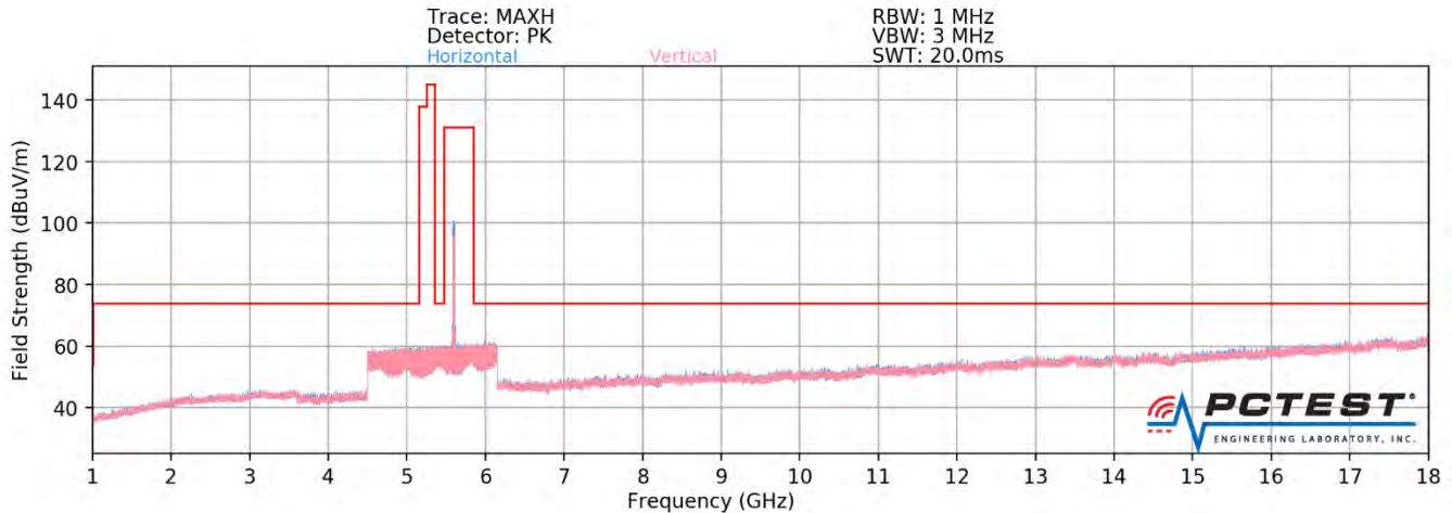
Plot 7-366. Radiated Spurious Plot above 1GHz SISO ANT2 (802.11ax – U2C Ch. 120 – 242 Tones – CLOSED)
