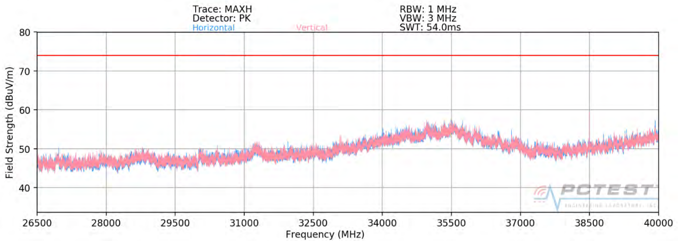
Plot 7-336. Radiated Spurious Plot 26.5GHz - 40GHz SISO ANT1 (802.11ax – 106 Tones – CLOSED)
