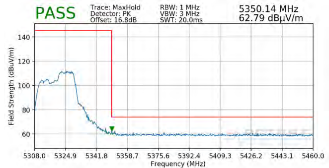
Plot 7-407. Radiated Upper Band Edge Plot SISO ANT1 (Peak - UNII Band 2A - 106 Tones)
