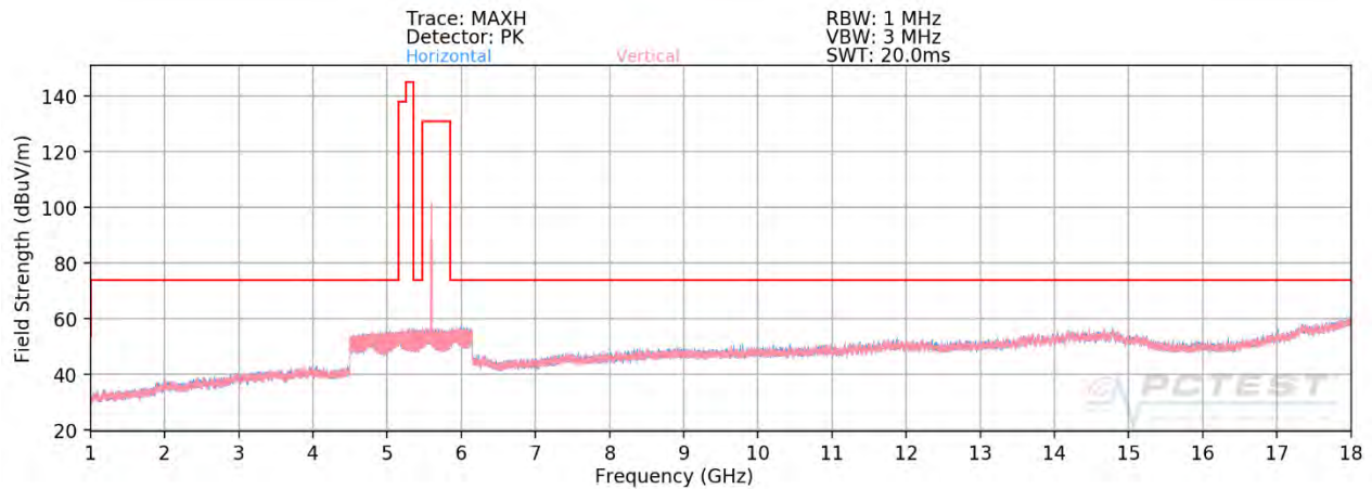
Plot 7-354. Radiated Spurious Plot above 1GHz SISO ANT2 (802.11ax – U2C Ch. 120 – 106 Tones - CLOSED)
