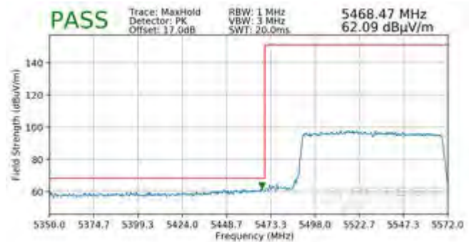
Plot 7-514. Radiated Lower Band Edge Plot MIMO (Peak – UNII Band 2C – 996 Tones)
