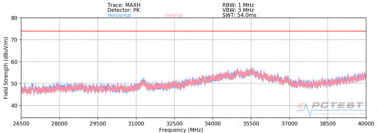
Plot 7-395. Radiated Spurious Plot 26.5GHz - 40GHz MIMO (802.11ax - 242 Tones - OPEN)
