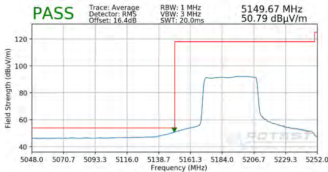
Plot 7-432. Radiated Lower Band Edge Plot SISO ANT1 (Average - UNII Band 1 - 484 Tones)
