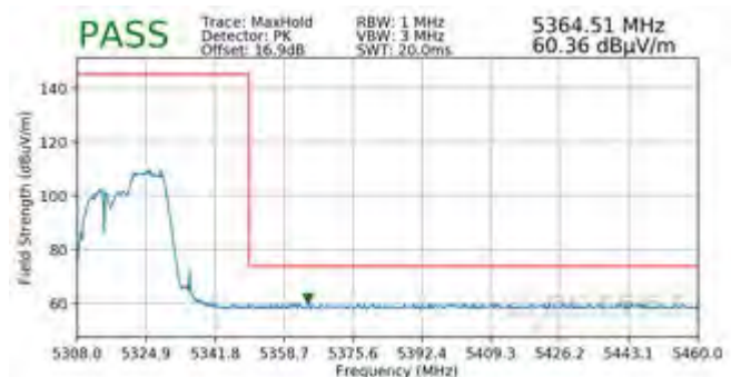
Plot 7-491. Radiated Upper Band Edge Plot MIMO (Peak – UNII Band 2A – 106 Tones)
