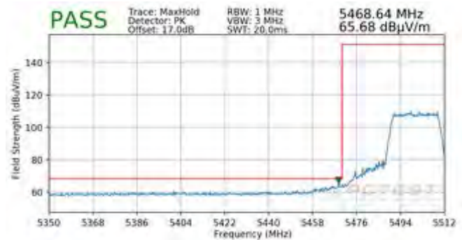
Plot 7-444. Radiated Lower Band Edge Plot SISO ANT2 (Peak – UNII Band 2C – 242 Tones)
