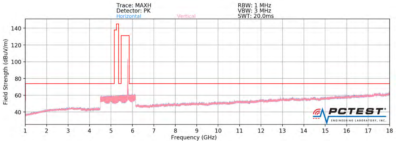
Plot 7-367. Radiated Spurious Plot above 1GHz SISO ANT2 (802.11ax – U3 Ch. 157 – 242 Tones – OPEN)
