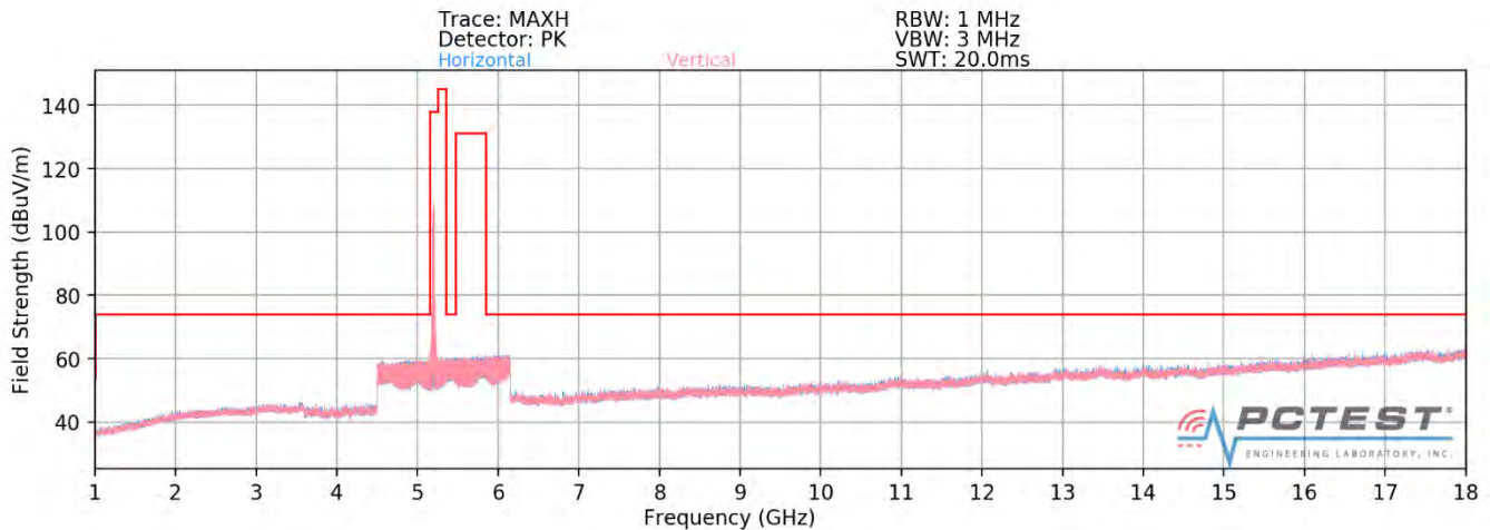
Plot 7-338. Radiated Spurious Plot above 1GHz SISO ANT1 (802.11ax - U1 Ch. 40 - 242 Tones - CLOSED)
