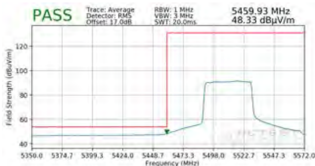
Plot 7-478. Radiated Lower Band Edge Plot SISO ANT2 (Average – UNII Band 2C – 484 Tones)
