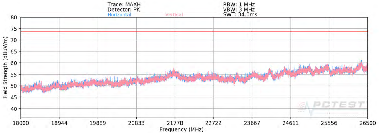
Plot 7-346. Radiated Spurious Plot 18GHz - 26.5GHz SISO ANT1 (802.11ax - 242 Tones - CLOSED)
