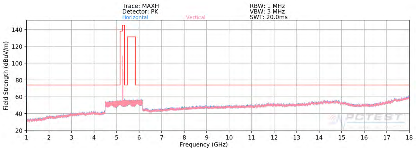
Plot 7-376. Radiated Spurious Plot above 1GHz MIMO (802.11ax – U2A Ch. 56 – 106 Tones - CLOSED)
