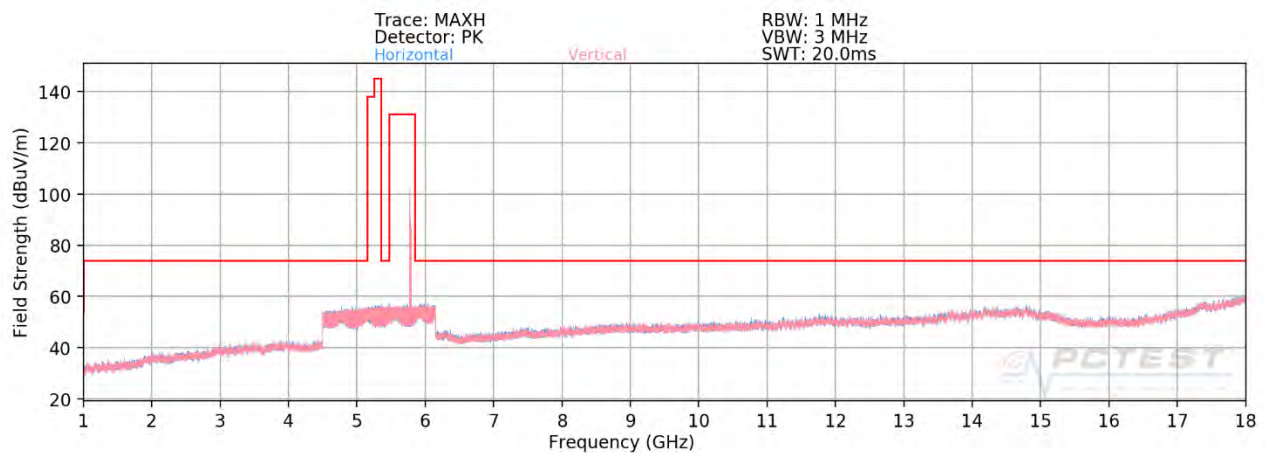
Plot 7-356. Radiated Spurious Plot above 1GHz SISO ANT2 (802.11ax – U3 Ch. 157 – 106 Tones - CLOSED)
