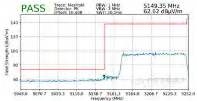
Plot 7-468. Radiated Lower Band Edge Plot SISO ANT2 (Peak - UNII Band 1 - 996 Tones)
