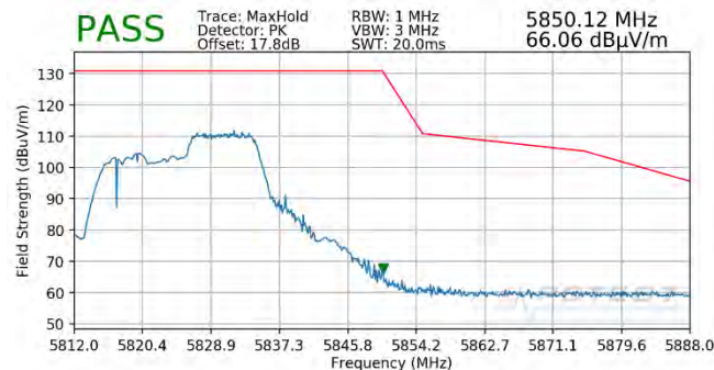
Plot 7-410. Radiated Upper Band Edge Plot SISO ANT1 (Peak - UNII Band 3 - 106 Tones)
