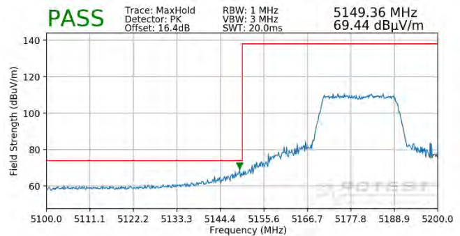
Plot 7-398. Radiated Lower Band Edge Plot SISO ANT1 (Peak - UNII Band 1 - 242 Tones)
