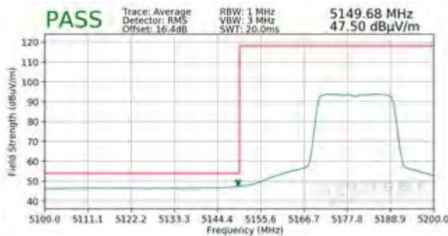
Plot 7-481. Radiated Lower Band Edge Plot MIMO (Average – UNII Band 1 – 242 Tones)
