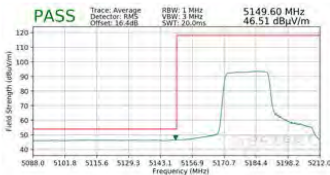
Plot 7-460. Radiated Lower Band Edge Plot SISO ANT2 (Average - UNII Band 1 - 242 Tones)
