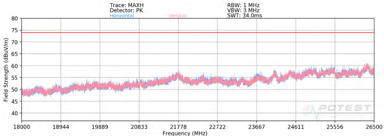
Plot 7-369. Radiated Spurious Plot above 18GHz - 26.5GHz SISO ANT2 (802.11ax - 242 Tones - OPEN)
