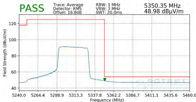
Plot 7-434. Radiated Upper Band Edge Plot SISO ANT1 (Average - UNII Band 2A - 484 Tones)
