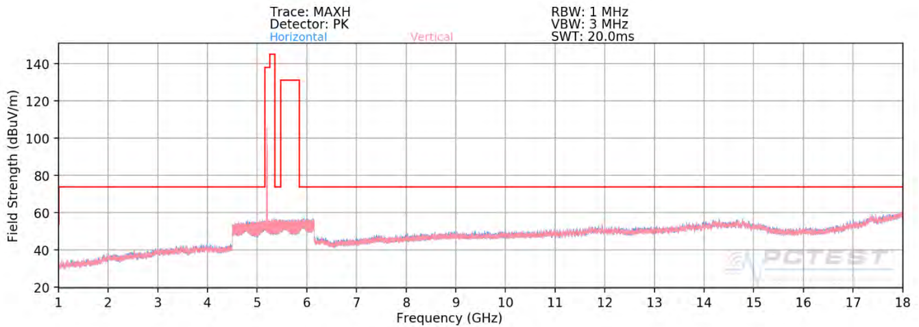
Plot 7-374. Radiated Spurious Plot above 1GHz MIMO (802.11ax – U1 Ch. 40 – 106 Tones - CLOSED)
