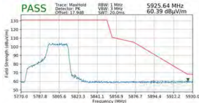
Plot 7-508. Radiated Upper Band Edge Plot MIMO (Peak - UNII Band 3 - 242 Tones)
