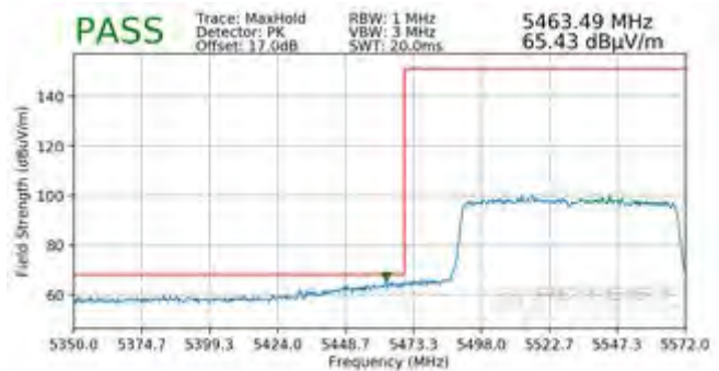
Plot 7-472. Radiated Lower Band Edge Plot SISO ANT2 (Peak – UNII Band 2C – 996 Tones)
