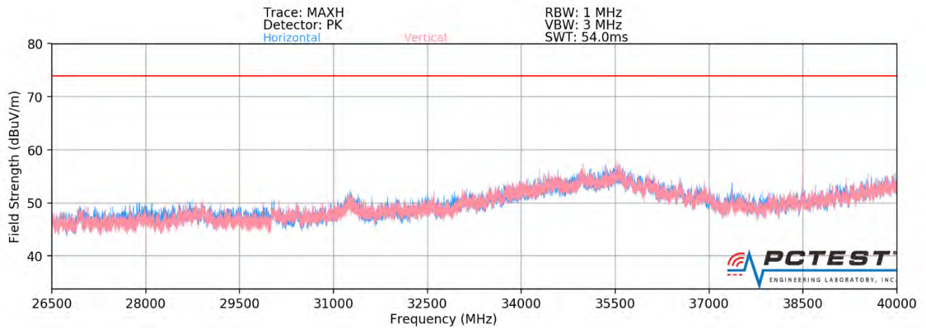
Plot 7-360. Radiated Spurious Plot 26.5GHz - 40GHz SISO ANT2 (802.11ax – 106 Tones – CLOSED)
