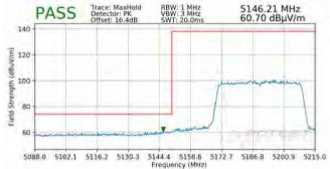
Plot 7-496. Radiated Lower Band Edge Plot MIMO (Peak - UNII Band 1 - 484 Tones)
