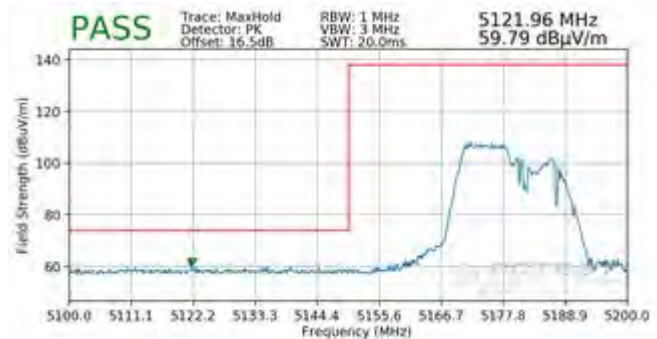
Plot 7-489. Radiated Lower Band Edge Plot MIMO (Peak – UNII Band 1 – 106 Tones)
