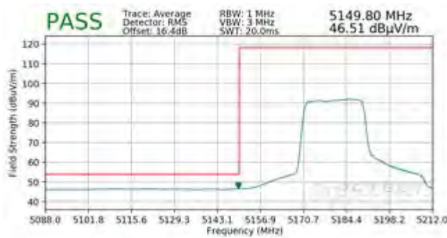
Plot 7-502. Radiated Lower Band Edge Plot MIMO (Average - UNII Band 1 - 242 Tones)
