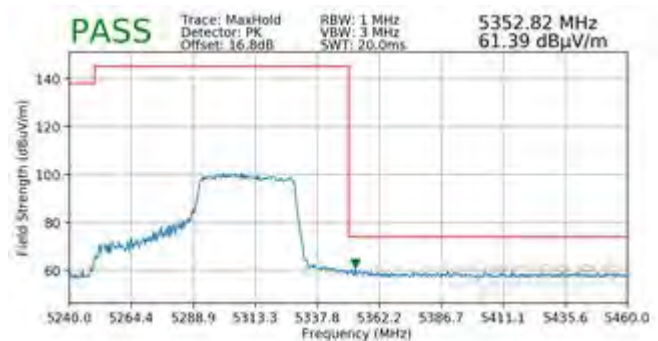
Plot 7-519. Radiated Upper Band Edge Plot MIMO (Peak - UNII Band 2A - 484 Tones)
