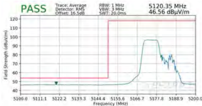
Plot 7-488. Radiated Lower Band Edge Plot MIMO (Average – UNII Band 1 – 106 Tones)
