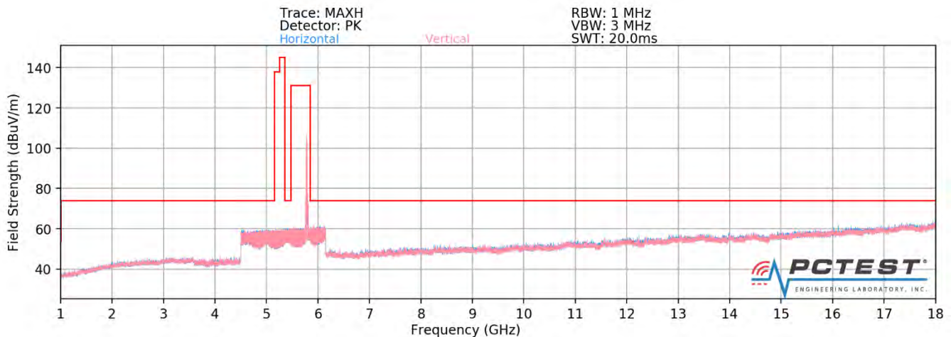
Plot 7-343. Radiated Spurious Plot above 1GHz SISO ANT1 (802.11ax – U3 Ch. 157 – 242 Tones – OPEN)
