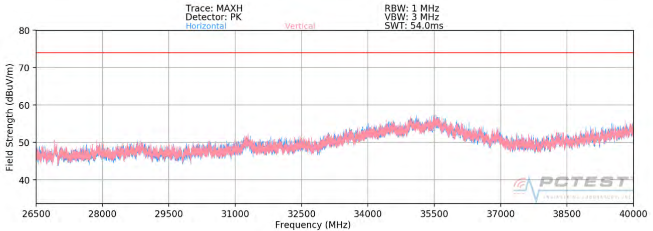
Plot 7-348. Radiated Spurious Plot 26.5GHz - 40GHz SISO ANT1 (802.11ax – 242 Tones – CLOSED)
