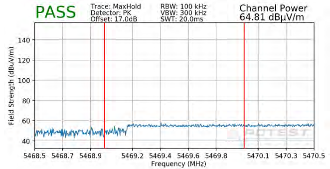
Plot 7-402. Radiated Lower Band Edge Plot SISO ANT1 (Peak - UNII Band 2C - 242 Tones)
