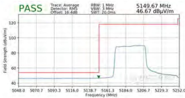
Plot 7-474. Radiated Lower Band Edge Plot SISO ANT2 (Average - UNII Band 1 - 484 Tones)
