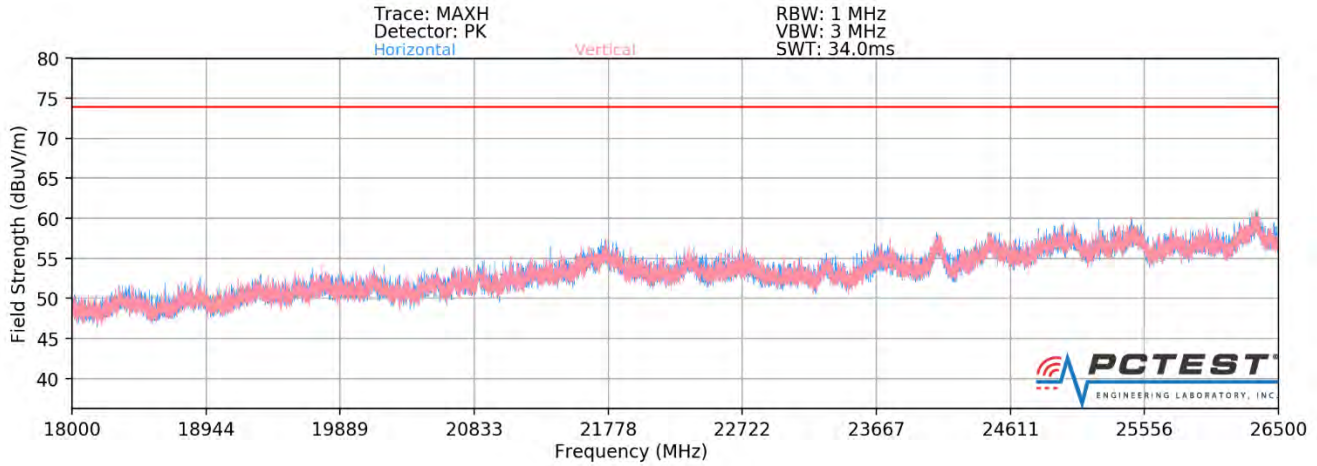
Plot 7-357. Radiated Spurious Plot above 18GHz - 26.5GHz SISO ANT2 (802.11ax - 106 Tones - OPEN)
