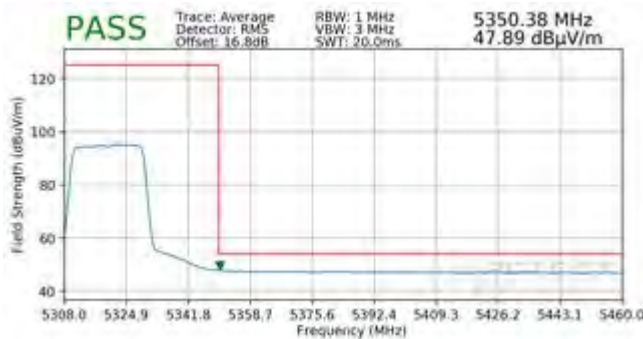
Plot 7-483. Radiated Upper Band Edge Plot MIMO (Average – UNII Band 2A – 242 Tones)
