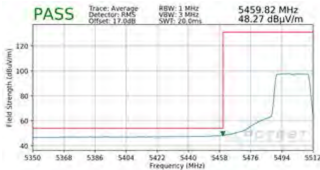
Plot 7-443. Radiated Lower Band Edge Plot SISO ANT2 (Average – UNII Band 2C – 242 Tones)
