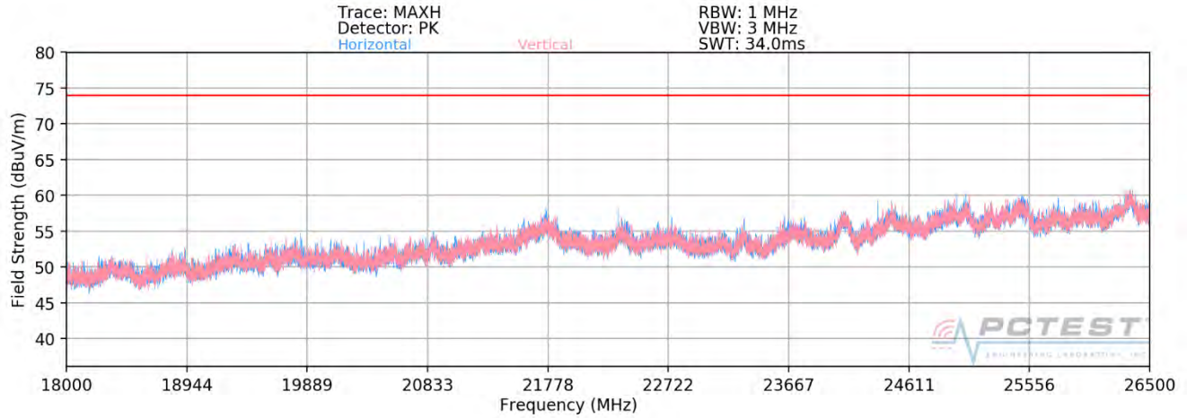
Plot 7-393. Radiated Spurious Plot above 18GHz - 26.5GHz MIMO (802.11ax - 242 Tones - OPEN)
