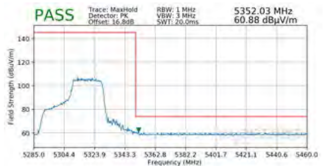
Plot 7-463. Radiated Upper Band Edge Plot SISO ANT2 (Peak - UNII Band 2A - 242 Tones)
