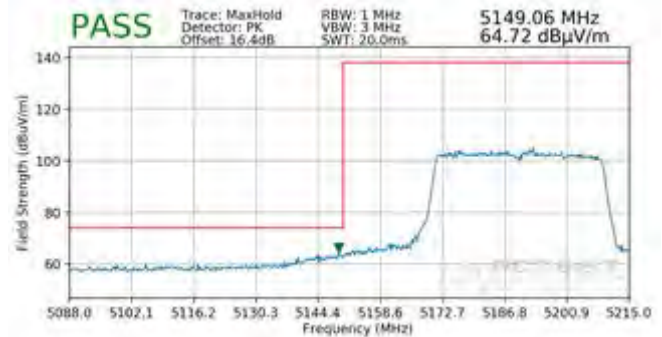
Plot 7-412. Radiated Lower Band Edge Plot SISO ANT1 (Peak - UNII Band 1 - 484 Tones)
