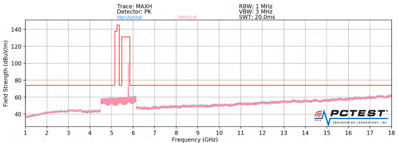
Plot 7-368. Radiated Spurious Plot above 1GHz SISO ANT2 (802.11ax – U3 Ch. 157 – 242 Tones – CLOSED)
