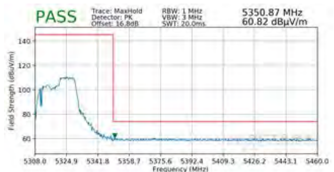
Plot 7-449. Radiated Upper Band Edge Plot SISO ANT2 (Peak - UNII Band 2A - 106 Tones)
