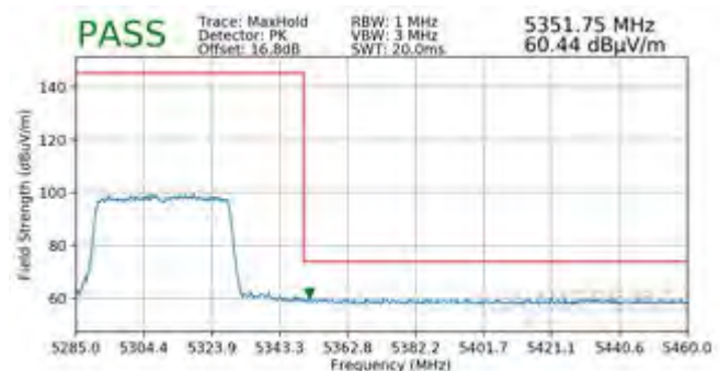
Plot 7-498. Radiated Upper Band Edge Plot MIMO (Peak - UNII Band 2A - 484 Tones)
