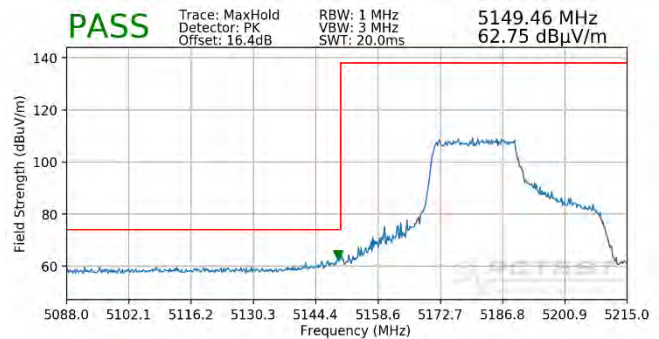
Plot 7-419. Radiated Lower Band Edge Plot SISO ANT1 (Peak - UNII Band 1 - 242 Tones)
