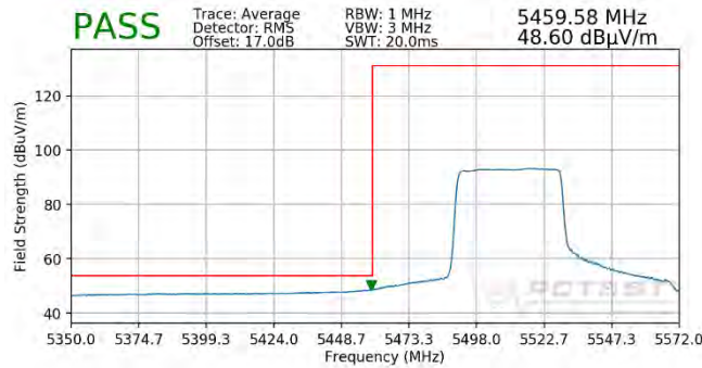
Plot 7-436. Radiated Lower Band Edge Plot SISO ANT1 (Average – UNII Band 2C – 484 Tones)
