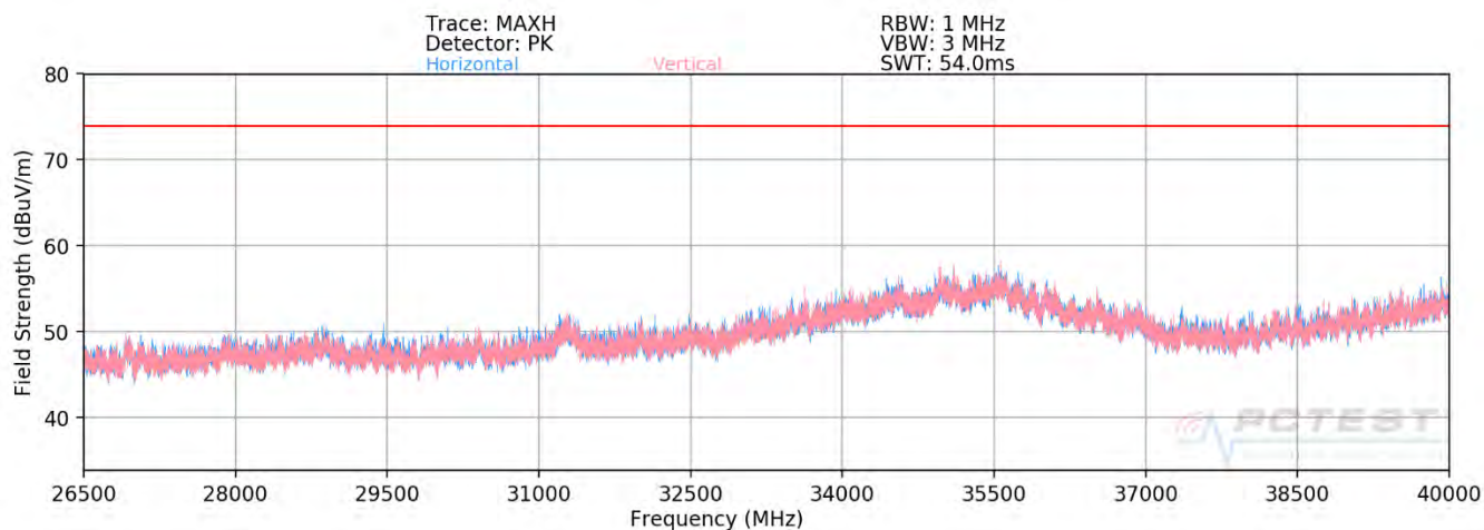
Plot 7-372. Radiated Spurious Plot 26.5GHz - 40GHz SISO ANT2 (802.11ax – 242 Tones – CLOSED)
