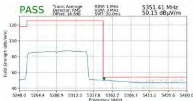
Plot 7-511. Radiated Upper Band Edge Plot MIMO (Average - UNII Band 2A - 996 Tones)
