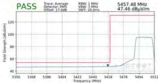
Plot 7-485. Radiated Lower Band Edge Plot MIMO (Average - UNII Band 2C - 242 Tones)
