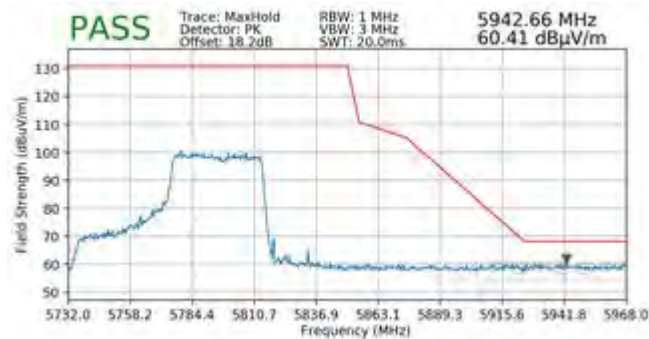
Plot 7-522. Radiated Upper Band Edge Plot MIMO (Peak - UNII Band 3 - 484 Tones)
