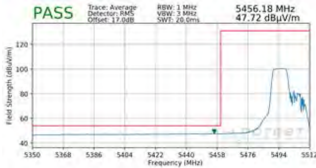
Plot 7-450. Radiated Lower Band Edge Plot SISO ANT2 (Average – UNII Band 2C – 106 Tones)
