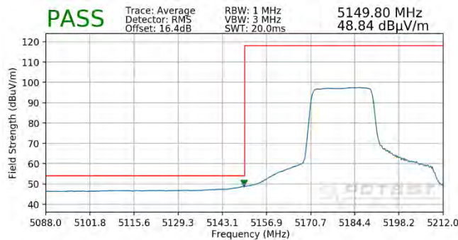
Plot 7-418. Radiated Lower Band Edge Plot SISO ANT1 (Average - UNII Band 1 - 242 Tones)
