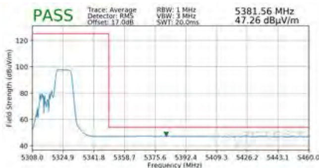
Plot 7-490. Radiated Upper Band Edge Plot MIMO (Average – UNII Band 2A – 106 Tones)
