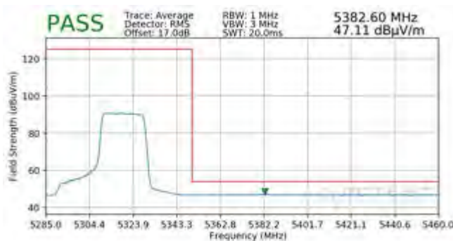
Plot 7-504. Radiated Upper Band Edge Plot MIMO (Average - UNII Band 2A - 242 Tones)
