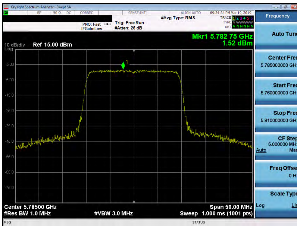
Plot 7-320. Power Spectral Density Plot MIMO ANT2 (20MHz BW 802.11ax – 242 Tones (UNII Band 3) – Ch. 157)
