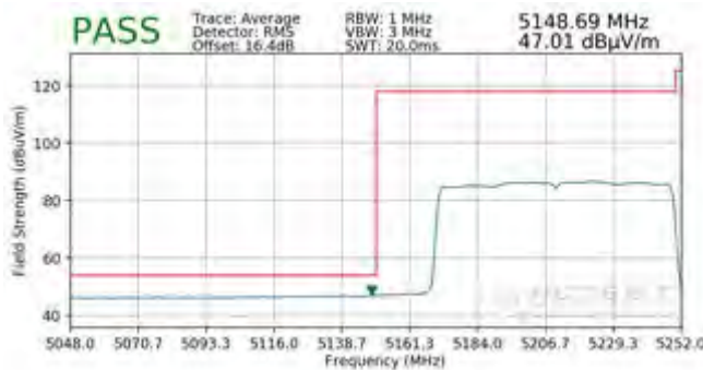
Plot 7-467. Radiated Lower Band Edge Plot SISO ANT2 (Average - UNII Band 1 - 996 Tones)
