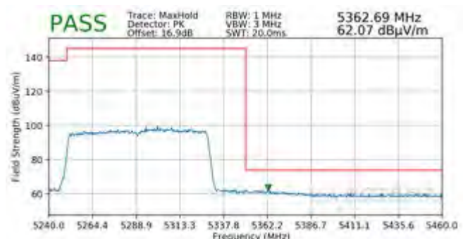
Plot 7-512. Radiated Upper Band Edge Plot MIMO (Peak - UNII Band 2A - 996 Tones)
