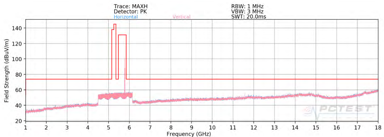
Plot 7-380. Radiated Spurious Plot above 1GHz MIMO (802.11ax – U3 Ch. 157 – 106 Tones - CLOSED)
