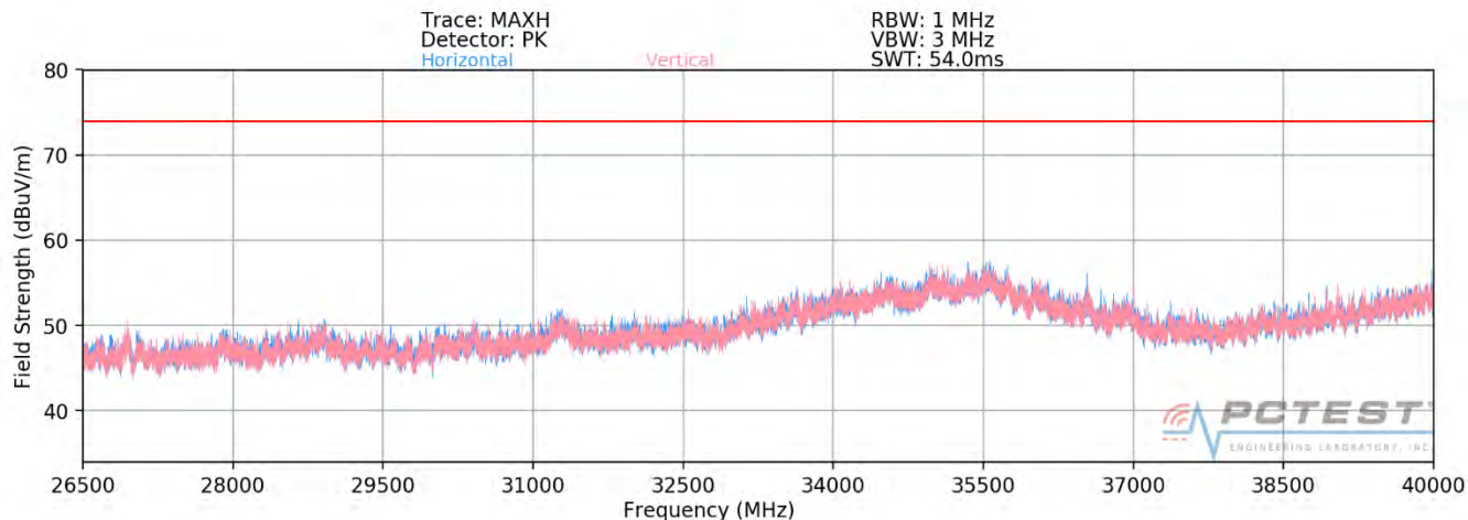
Plot 7-371. Radiated Spurious Plot 26.5GHz - 40GHz SISO ANT2 (802.11ax - 242 Tones - OPEN)
