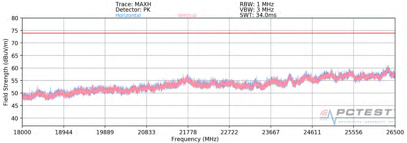
Plot 7-333. Radiated Spurious Plot 18GHz - 26.5GHz SISO ANT1 (802.11ax - 106 Tones - OPEN)
