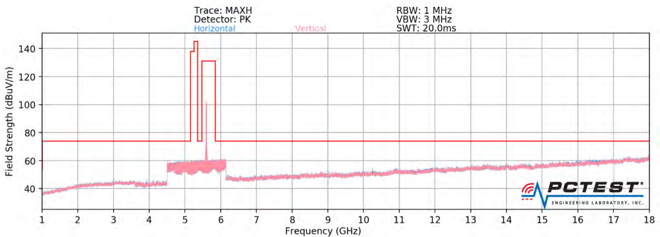
Plot 7-389. Radiated Spurious Plot above 1GHz MIMO (802.11ax – U2C Ch. 120 – 242 Tones – OPEN)
