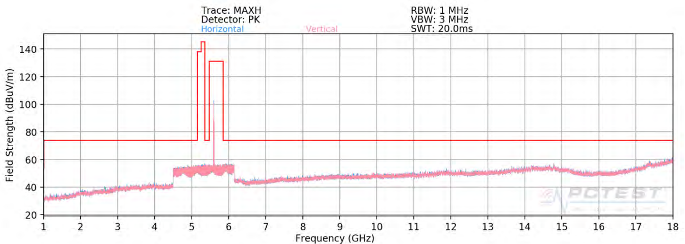
Plot 7-353. Radiated Spurious Plot above 1GHz SISO ANT2 (802.11ax - U2C Ch. 120 - 106 Tones - OPEN)
