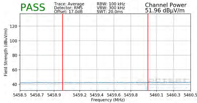
Plot 7-415. Radiated Lower Band Edge Plot SISO ANT1 (Average – UNII Band 2C – 484 Tones)
