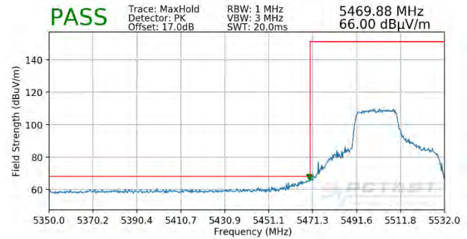
Plot 7-423. Radiated Lower Band Edge Plot SISO ANT1 (Peak - UNII Band 2C - 242 Tones)
