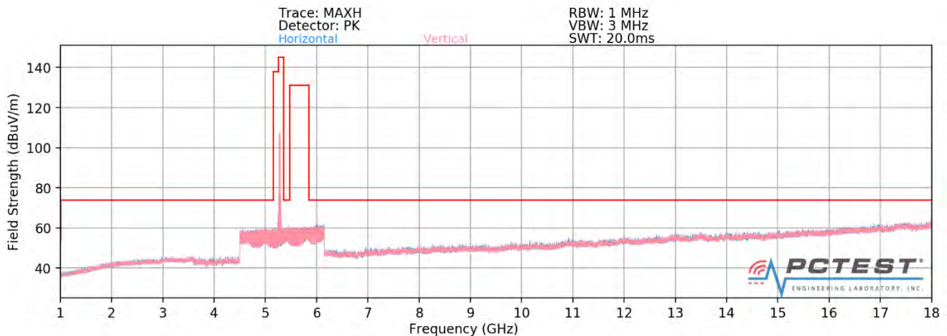
Plot 7-340. Radiated Spurious Plot above 1GHz SISO ANT1 (802.11ax - U2A Ch. 56 - 242 Tones - CLOSED)
