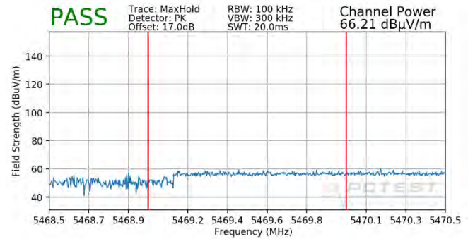
Plot 7-416. Radiated Lower Band Edge Plot SISO ANT1 (Peak – UNII Band 2C – 484 Tones)
