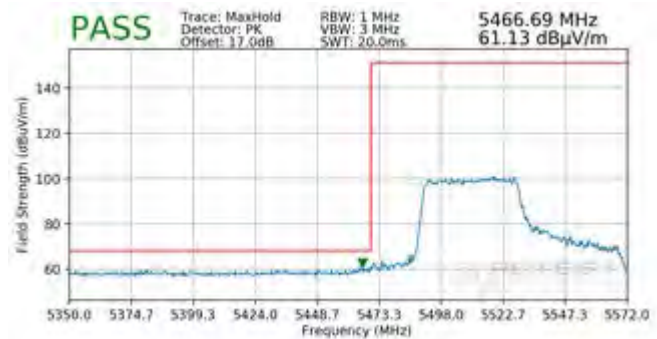
Plot 7-521. Radiated Lower Band Edge Plot MIMO (Peak - UNII Band 2C - 484 Tones)
