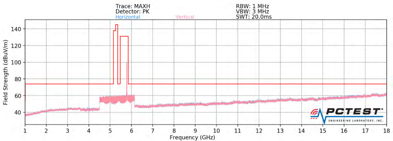
Plot 7-392. Radiated Spurious Plot above 1GHz MIMO (802.11ax – U3 Ch. 157 – 242 Tones – CLOSED)
