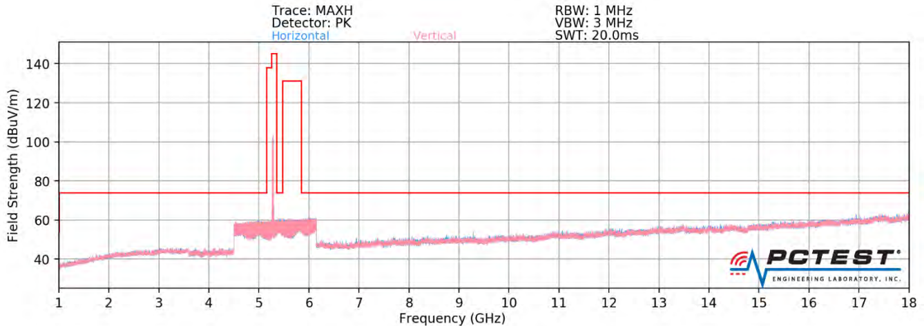
Plot 7-387. Radiated Spurious Plot above 1GHz MIMO (802.11ax – U2A Ch. 56 – 242 Tones – OPEN)
