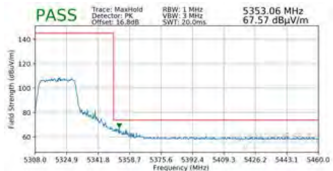
Plot 7-442. Radiated Upper Band Edge Plot SISO ANT2 (Peak - UNII Band 2A - 242 Tones)
