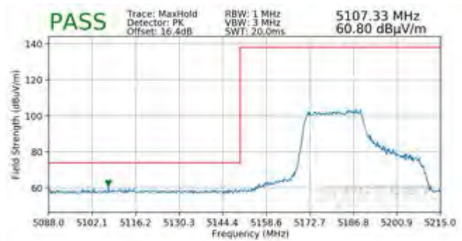
Plot 7-503. Radiated Lower Band Edge Plot MIMO (Peak - UNII Band 1 - 242 Tones)
