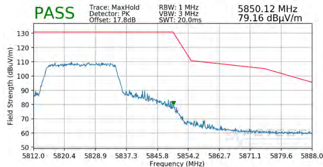
Plot 7-403. Radiated Upper Band Edge Plot SISO ANT1 (Peak - UNII Band 3 - 242 Tones)
