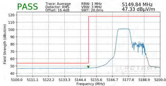
Plot 7-404. Radiated Lower Band Edge Plot SISO ANT1 (Average - UNII Band 1 - 106 Tones)
