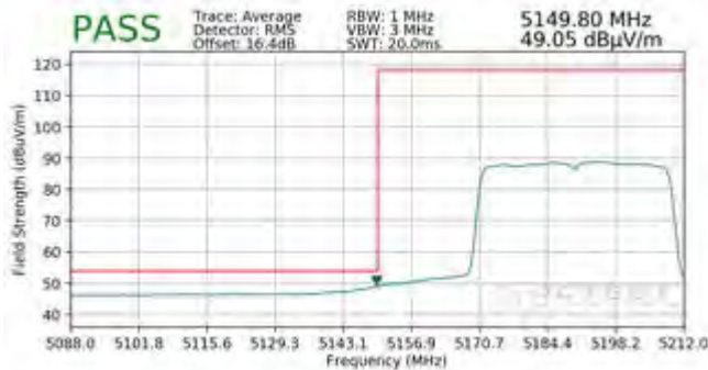
Plot 7-495. Radiated Lower Band Edge Plot MIMO (Average - UNII Band 1 - 484 Tones)
