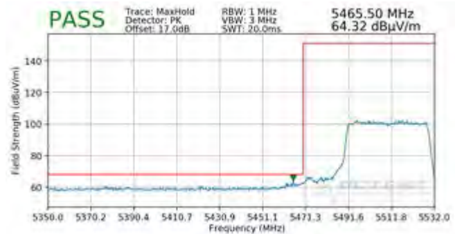
Plot 7-500. Radiated Lower Band Edge Plot MIMO (Peak - UNII Band 2C - 484 Tones)
