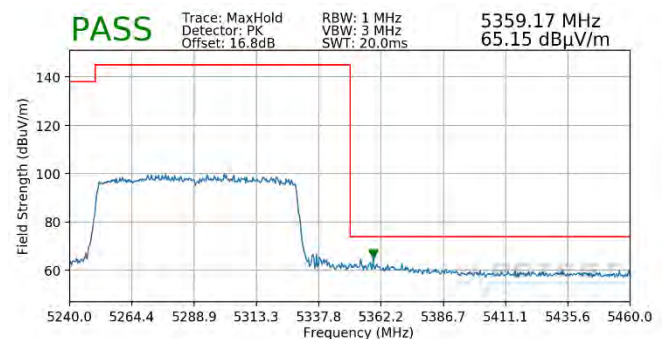
Plot 7-428. Radiated Upper Band Edge Plot SISO ANT1 (Peak - UNII Band 2A - 996 Tones)
