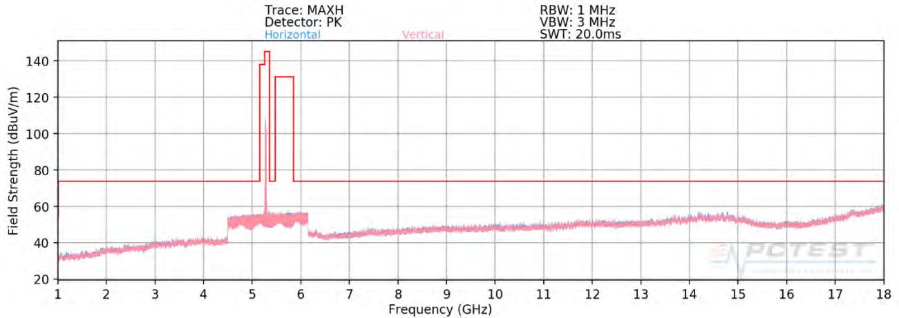
Plot 7-327. Radiated Spurious Plot above 1GHz SISO ANT1 (802.11ax – U2A Ch. 56 – 106 Tones - OPEN)
