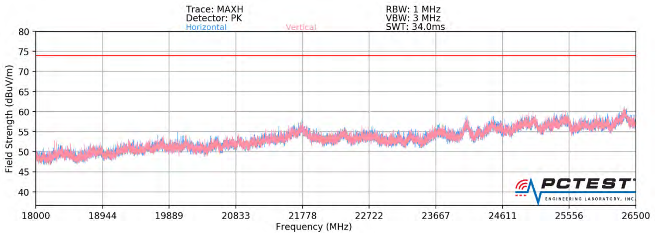
Plot 7-382. Radiated Spurious Plot above 18GHz - 26.5GHz MIMO (802.11ax - 106 Tones - CLOSED)
