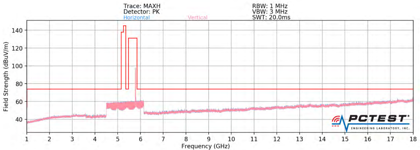
Plot 7-391. Radiated Spurious Plot above 1GHz MIMO (802.11ax – U3 Ch. 157 – 242 Tones – OPEN)
