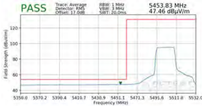
Plot 7-464. Radiated Lower Band Edge Plot SISO ANT2 (Average – UNII Band 2C – 242 Tones)
