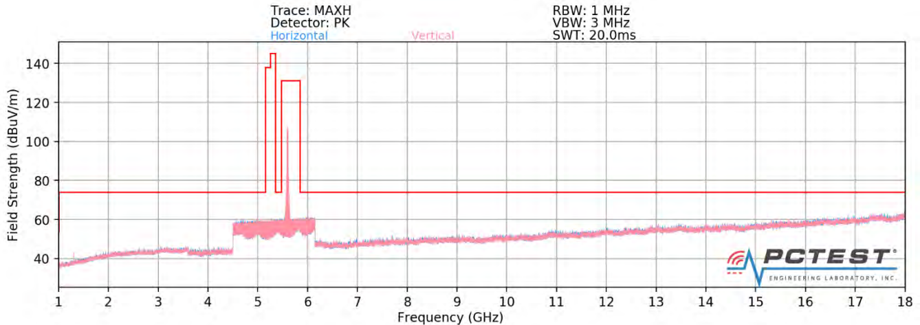
Plot 7-342. Radiated Spurious Plot above 1GHz SISO ANT1 (802.11ax – U2C Ch. 120 – 242 Tones – CLOSED)
