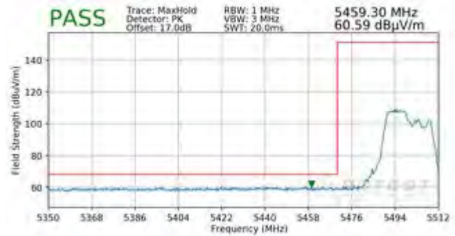
Plot 7-493. Radiated Lower Band Edge Plot MIMO (Peak - UNII Band 2C - 106 Tones)
