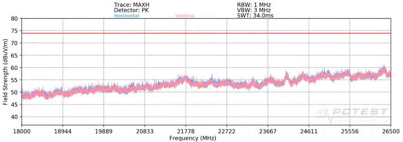
Plot 7-394. Radiated Spurious Plot above 18GHz - 26.5GHz MIMO (802.11ax - 242 Tones - CLOSED)
