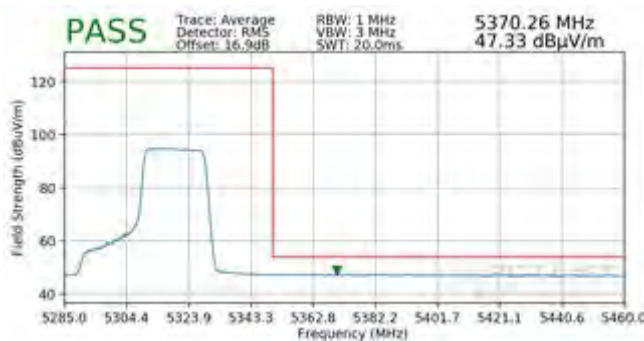
Plot 7-462. Radiated Upper Band Edge Plot SISO ANT2 (Average - UNII Band 2A - 242 Tones)
