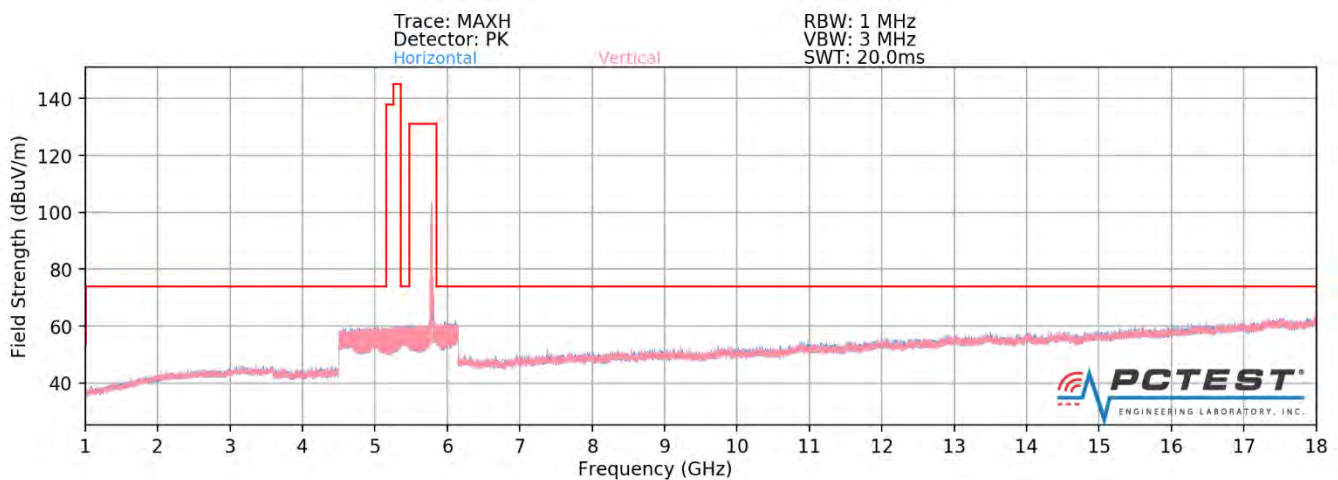
Plot 7-344. Radiated Spurious Plot above 1GHz SISO ANT1 (802.11ax – U3 Ch. 157 – 242 Tones – CLOSED)
