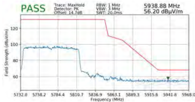
Plot 7-473. Radiated Upper Band Edge Plot SISO ANT2 (Peak – UNII Band 3 – 996 Tones)
