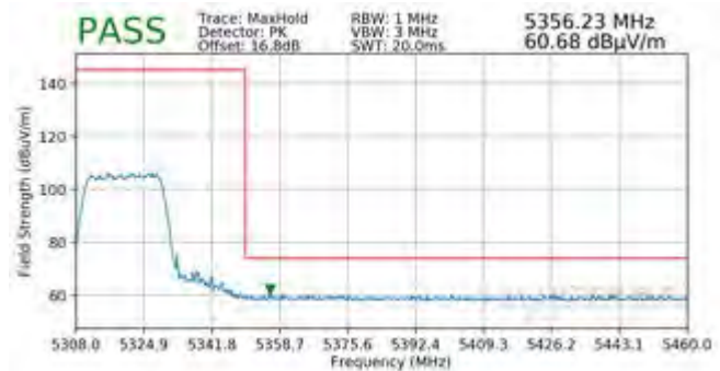
Plot 7-484. Radiated Upper Band Edge Plot MIMO (Peak – UNII Band 2A – 242 Tones)
