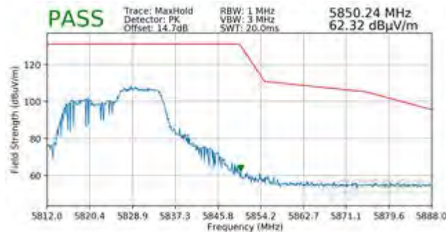
Plot 7-452. Radiated Upper Band Edge Plot SISO ANT2 (Peak – UNII Band 3 – 106 Tones)
