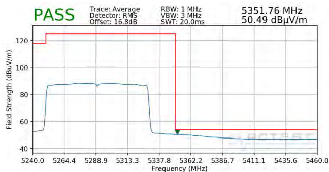
Plot 7-427. Radiated Upper Band Edge Plot SISO ANT1 (Average - UNII Band 2A - 996 Tones)
