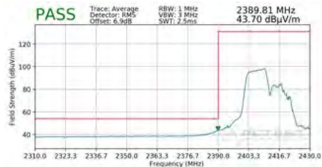
Plot 7-139. Radiated Restricted Lower Band Edge Measurement MIMO (Average - 106 Tones)
