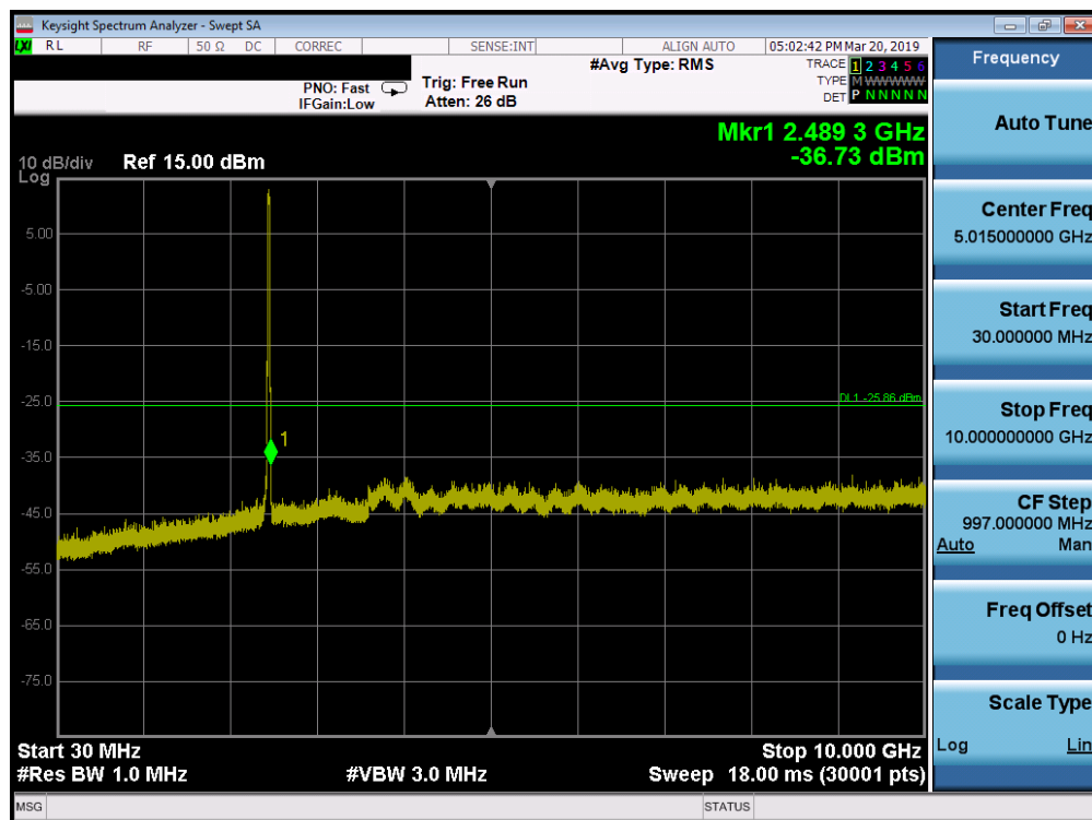
Plot 7-63. Conducted Spurious Plot SISO ANT2 (802.11ax OFDMA- 242 Tones - Ch. 11)
