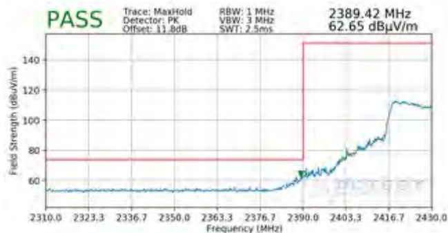
Plot 7-104. Radiated Restricted Lower Band Edge Measurement SISO ANT1 (Peak – 242 Tones)
