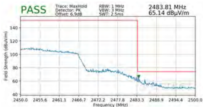
Plot 7-156. Radiated Restricted Upper Band Edge Measurement MIMO (Peak - 242 Tones)
