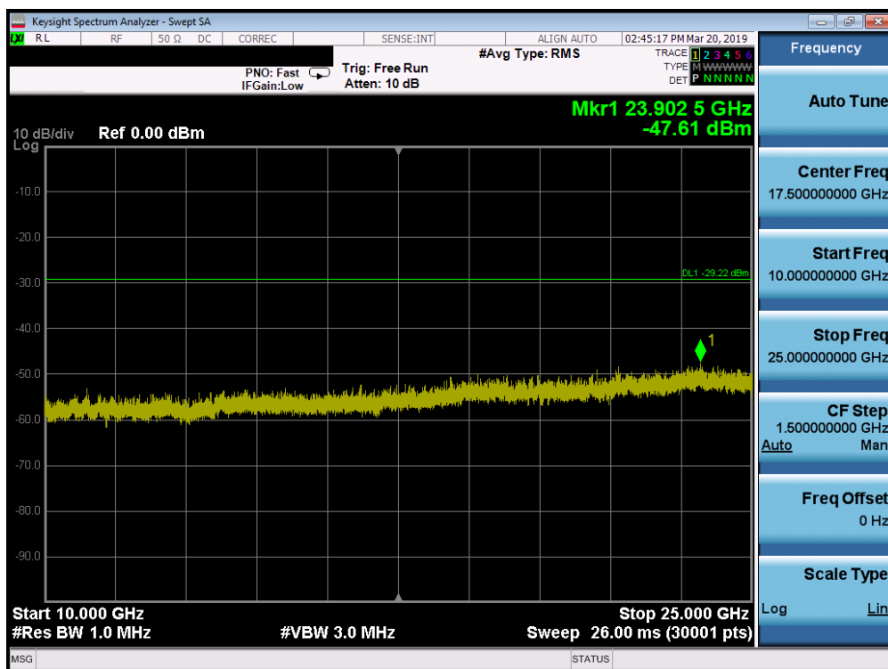
Plot 7-52. Conducted Spurious Plot SISO ANT1 (802.11ax OFDMA- 242 Tones - Ch. 11)
