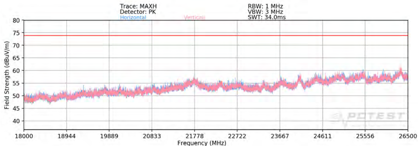
Plot 7-87. Radiated Spurious Plot above 18GHz MIMO (802.11ax OFDMA – 26 Tones – CLOSED)
