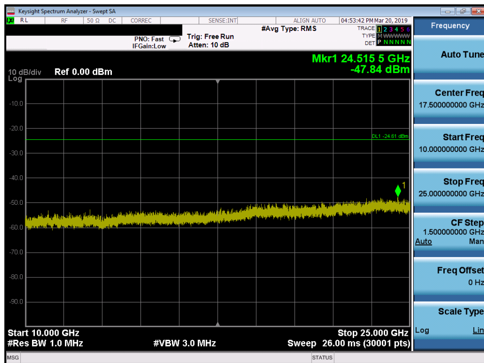
Plot 7-62. Conducted Spurious Plot SISO ANT2 (802.11ax OFDMA- 242 Tones - Ch. 6)
