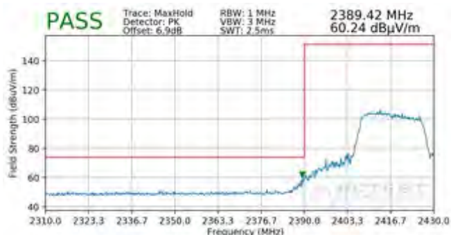
Plot 7-128. Radiated Restricted Lower Band Edge Measurement SISO ANT2 (Peak - 242 Tones)
