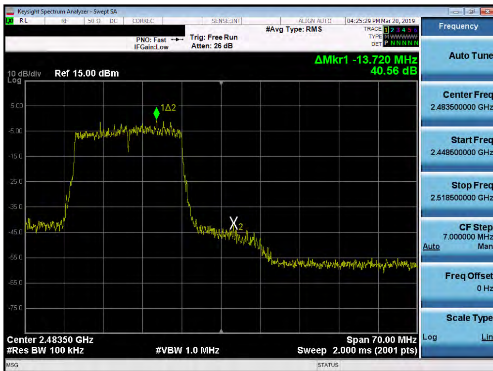
Plot 7-31. Band Edge Plot SISO ANT1 (802.11ax OFDMA - 242 Tones - Ch. 12)
