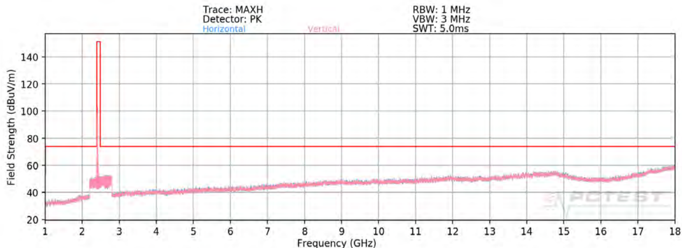
Plot 7-68. Radiated Spurious Plot above 1GHz SISO ANT1 (802.11ax OFDMA – 242 Tones – Ch. 1 – CLOSED)
