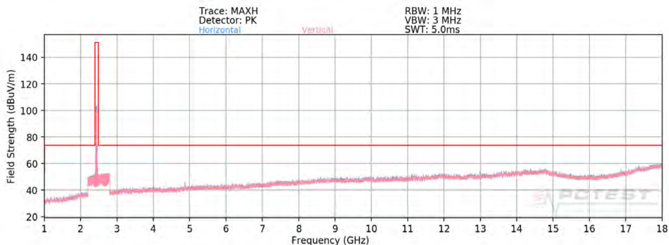
Plot 7-85. Radiated Spurious Plot above 1GHz MIMO (802.11ax OFDMA – 242 Tones – Ch. 6 – CLOSED)
