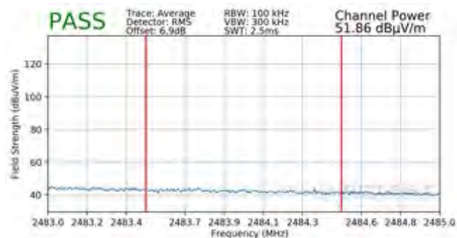
Plot 7-131. Radiated Restricted Upper Band Edge Measurement SISO ANT2 (Average - 242 Tones)
