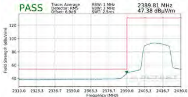
Plot 7-125. Radiated Restricted Lower Band Edge Measurement SISO ANT2 (Average - 242 Tones)
