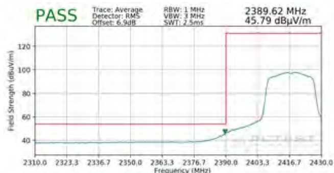
Plot 7-153. Radiated Restricted Lower Band Edge Measurement MIMO (Average - 242 Tones)
