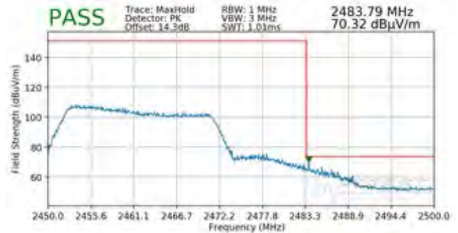
Plot 7-164. Radiated Restricted Band Edge Measurement MIMO with WCP (Peak – 242 Tones)
