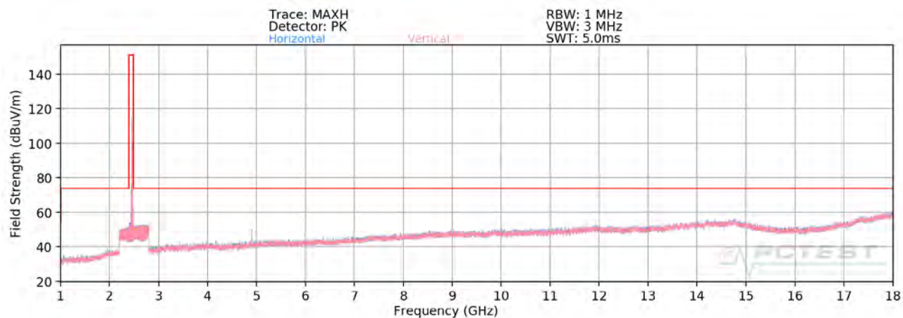
Plot 7-83. Radiated Spurious Plot above 1GHz MIMO (802.11ax OFDMA – 26 Tones – Ch. 11 – CLOSED)
