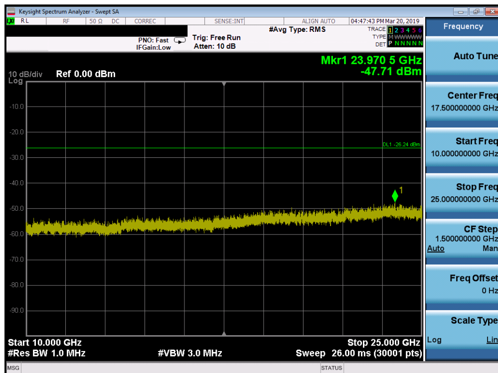
Plot 7-60. Conducted Spurious Plot SISO ANT2 (802.11ax OFDMA– 242 Tones – Ch. 1)
