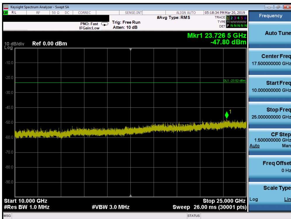
Plot 7-58. Conducted Spurious Plot SISO ANT2 (802.11ax OFDMA- 106 Tones - Ch. 11)
