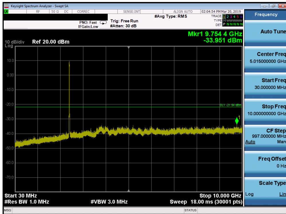
Plot 7-47. Conducted Spurious Plot SISO ANT1 (802.11ax OFDMA – 242 Tones – Ch. 1)
