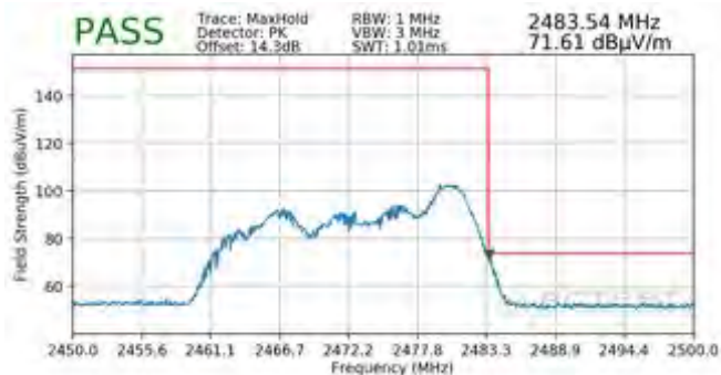
Plot 7-150. Radiated Restricted Upper Band Edge Measurement MIMO (Peak – 26 Tones)
