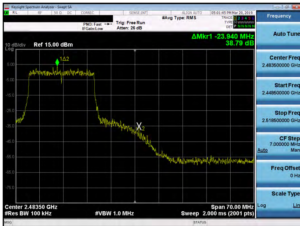
Plot 7-38. Band Edge Plot SISO ANT2 (802.11ax OFDMA - 242 Tones - Ch. 11)
