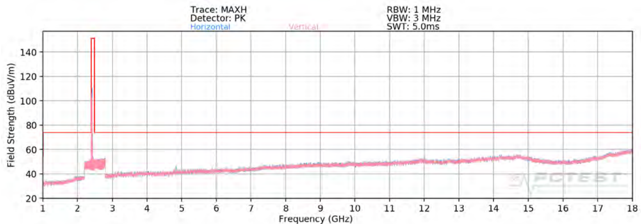
Plot 7-65. Radiated Spurious Plot above 1GHz SISO ANT1 (802.11ax OFDMA – 26 Tones – Ch. 1 – CLOSED)
