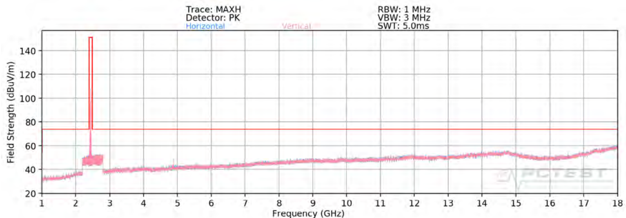
Plot 7-66. Radiated Spurious Plot above 1GHz SISO ANT1 (802.11ax OFDMA – 26 Tones – Ch. 6 – CLOSED)
