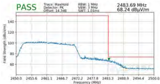
Plot 7-138. Radiated Restricted Band Edge Measurement SISO ANT2 with WCP (Peak – 242 Tones)
