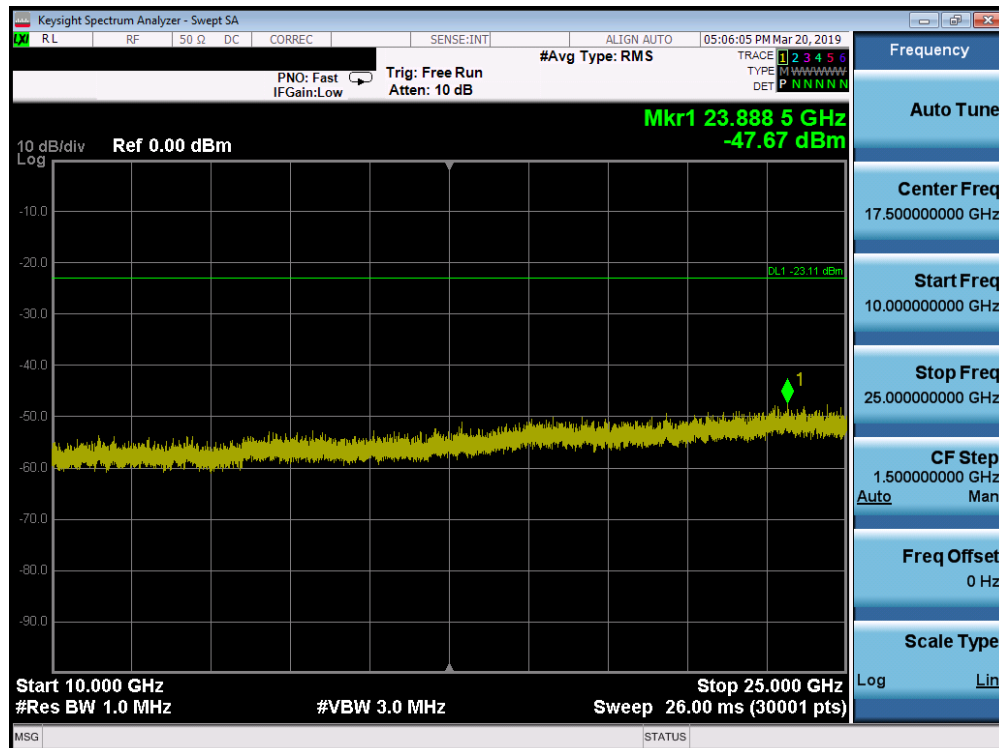
Plot 7-54. Conducted Spurious Plot SISO ANT2 (802.11ax OFDMA– 106 Tones – Ch. 1)
