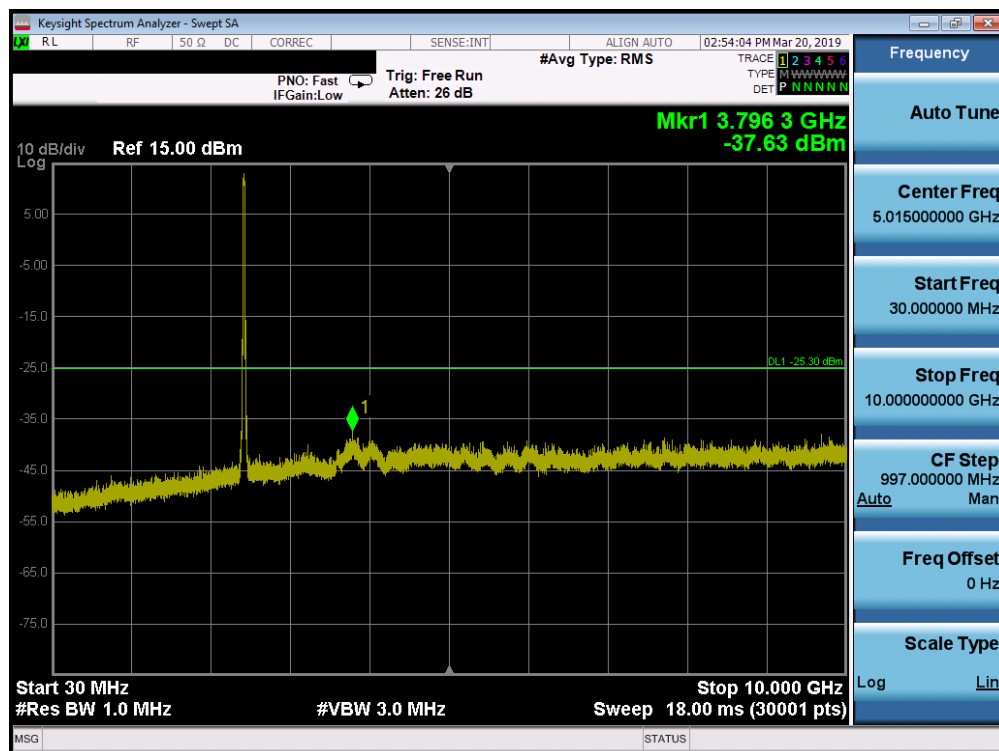
Plot 7-49. Conducted Spurious Plot SISO ANT1 (802.11ax OFDMA- 242 Tones - Ch. 6)
