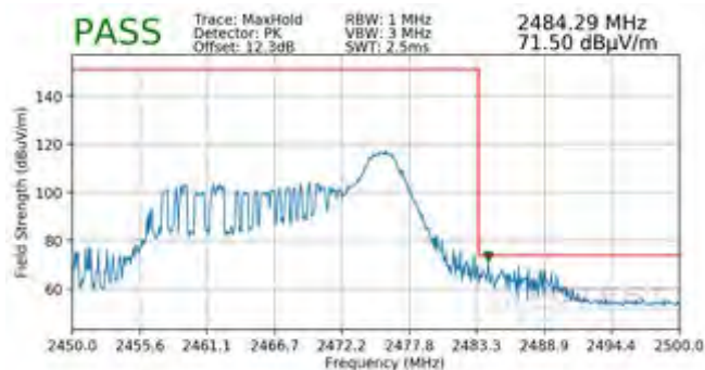
Plot 7-94. Radiated Restricted Upper Band Edge Measurement SISO ANT1 (Peak – 26 Tones)
