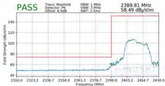
Plot 7-118. Radiated Restricted Lower Band Edge Measurement SISO ANT2 (Peak - 106 Tones)
