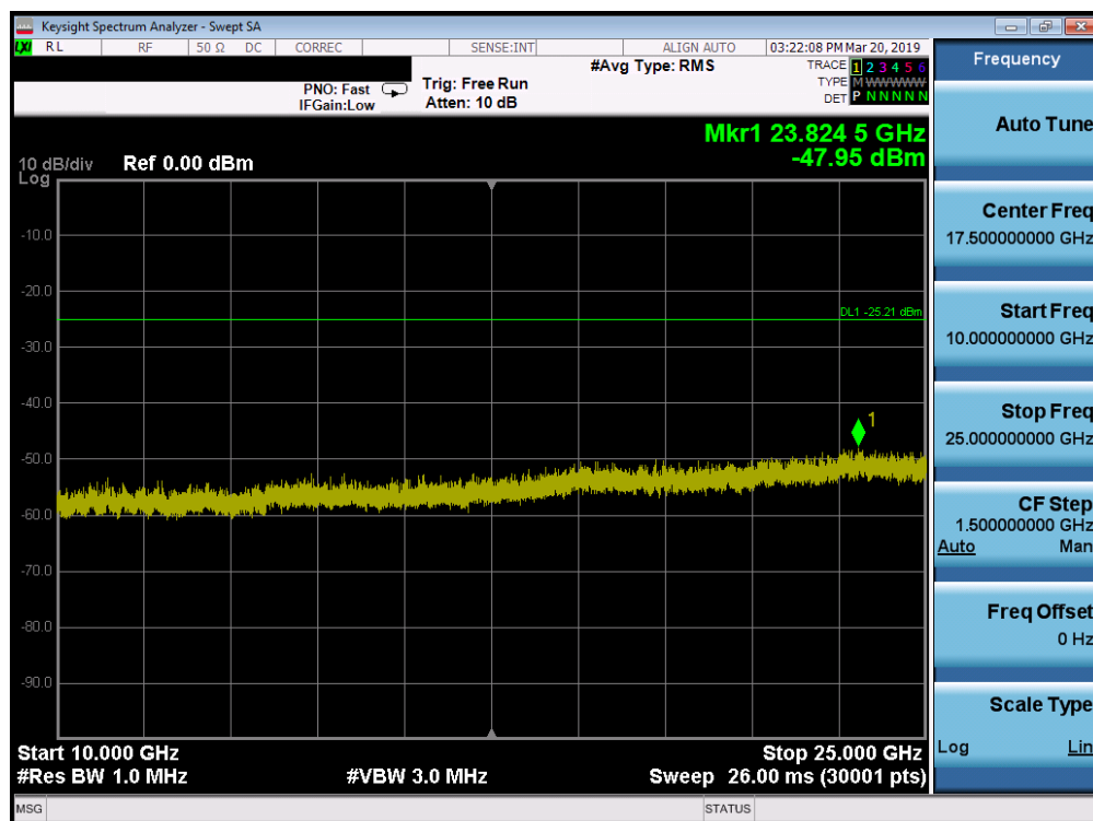
Plot 7-46. Conducted Spurious Plot SISO ANT1 (802.11ax OFDMA- 106 Tones - Ch. 11)
