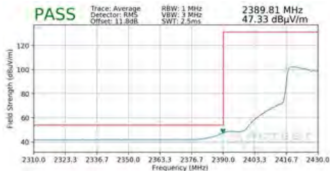
Plot 7-103. Radiated Restricted Lower Band Edge Measurement SISO ANT1 (Average – 242 Tones)
