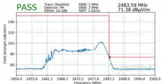
Plot 7-124. Radiated Restricted Upper Band Edge Measurement SISO ANT2 (Peak – 26 Tones)
