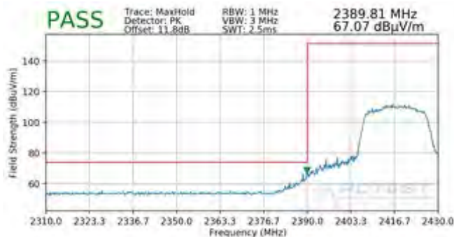
Plot 7-100. Radiated Restricted Lower Band Edge Measurement SISO ANT1 (Peak - 242 Tones)
