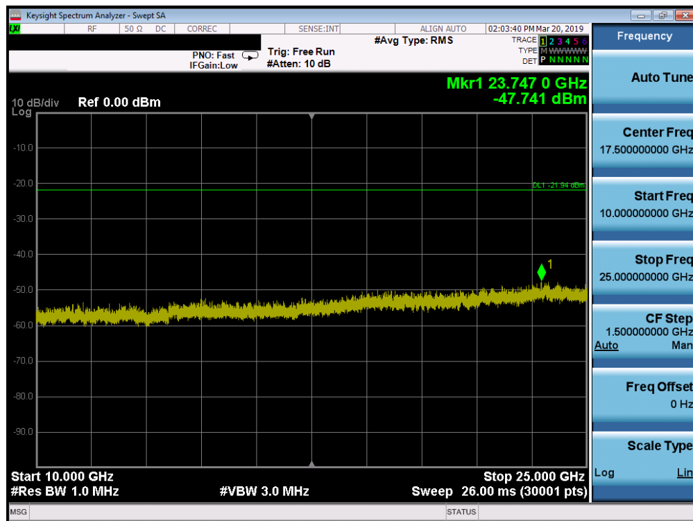
Plot 7-48. Conducted Spurious Plot SISO ANT1 (802.11ax OFDMA– 242 Tones – Ch. 1)
