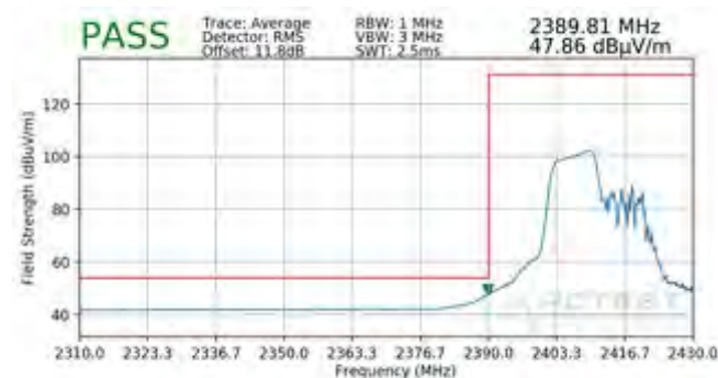
Plot 7-89. Radiated Restricted Lower Band Edge Measurement SISO ANT1 (Average - 106 Tones)
