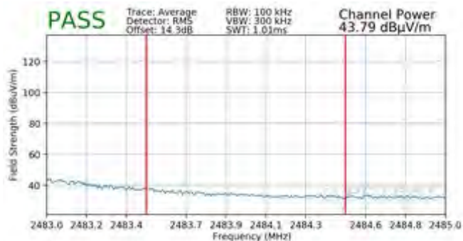
Plot 7-149. Radiated Restricted Upper Band Edge Measurement MIMO (Average – 26 Tones)
