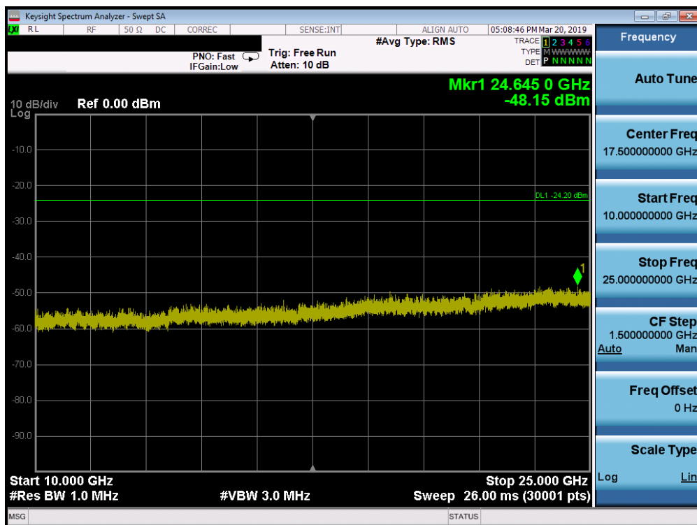
Plot 7-56. Conducted Spurious Plot SISO ANT2 (802.11ax OFDMA– 106 Tones – Ch. 6)
