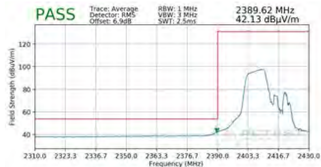
Plot 7-117. Radiated Restricted Lower Band Edge Measurement SISO ANT2 (Average - 106 Tones)
