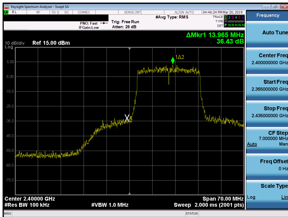
Plot 7-37. Band Edge Plot SISO ANT2 (802.11ax OFDMA - 242 Tones - Ch. 1)
