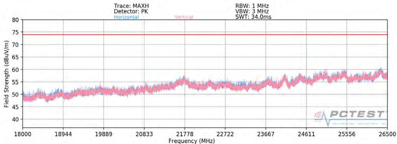
Plot 7-80. Radiated Spurious Plot above 18GHz SISO ANT2 (802.11ax OFDMA – 242 Tones – CLOSED)
