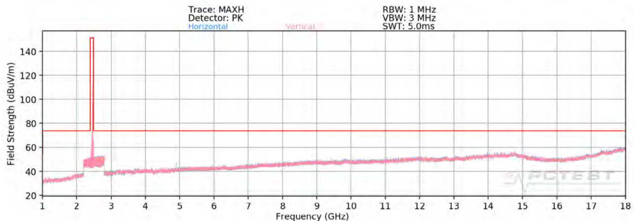
Plot 7-67. Radiated Spurious Plot above 1GHz SISO ANT1 (802.11ax OFDMA – 26 Tones – Ch. 11 – CLOSED)
