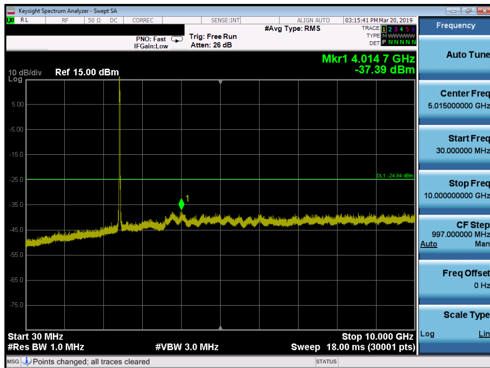
Plot 7-43. Conducted Spurious Plot SISO ANT1 (802.11ax OFDMA- 106 Tones – Ch. 6)
