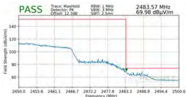
Plot 7-108. Radiated Restricted Upper Band Edge Measurement SISO ANT1 (Peak – 242 Tones)
