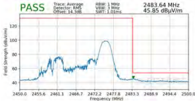
Plot 7-121. Radiated Restricted Upper Band Edge Measurement SISO ANT2 (Average – 26 Tones)
