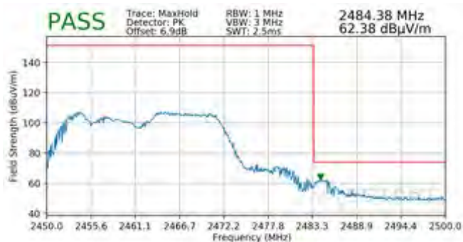
Plot 7-146. Radiated Restricted Upper Band Edge Measurement MIMO (Peak - 106 Tones)
