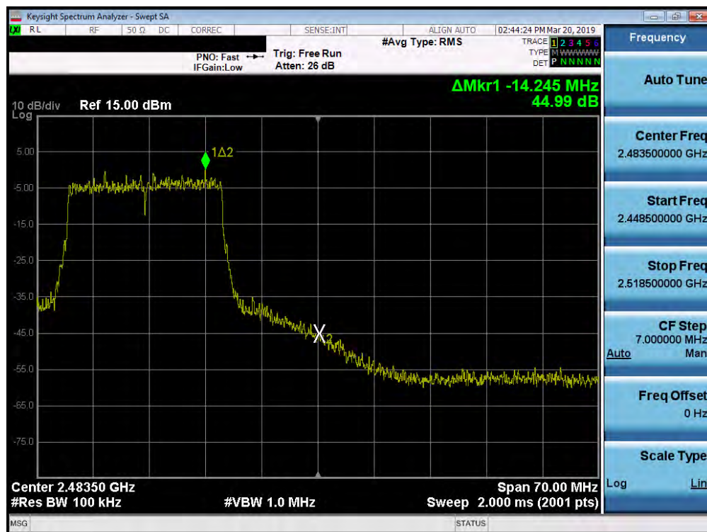
Plot 7-30. Band Edge Plot SISO ANT1 (802.11ax OFDMA – 242 Tones – Ch. 11)
