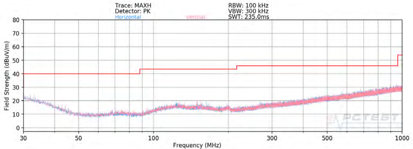
Plot 7-168. Radiated Spurious Plot below 1GHz SISO ANT2 (242 Tones - CLOSED)
