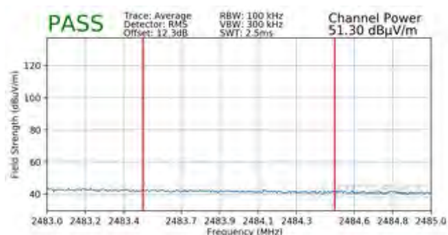
Plot 7-111. Radiated Restricted Upper Band Edge Measurement SISO ANT1 (Average - 242 Tones)
