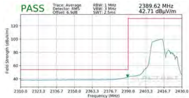
Plot 7-141. Radiated Restricted Lower Band Edge Measurement MIMO (Average - 106 Tones)
