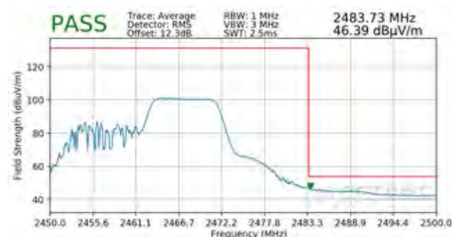
Plot 7-91. Radiated Restricted Upper Band Edge Measurement SISO ANT1 (Average - 106 Tones)
