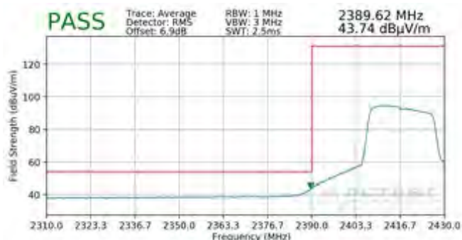
Plot 7-127. Radiated Restricted Lower Band Edge Measurement SISO ANT2 (Average - 242 Tones)
