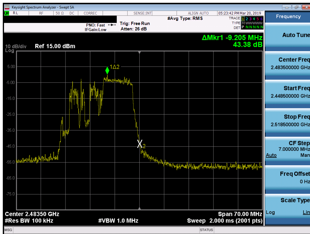
Plot 7-36. Band Edge Plot SISO ANT2 (802.11ax OFDMA - 106 Tones - Ch. 13)
