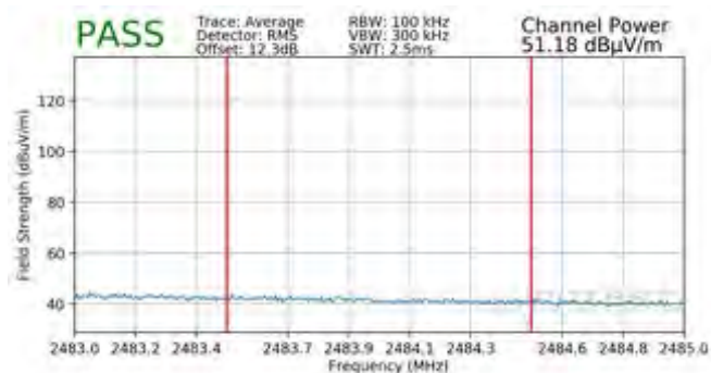
Plot 7-109. Radiated Restricted Upper Band Edge Measurement SISO ANT1 (Average - 242 Tones)
