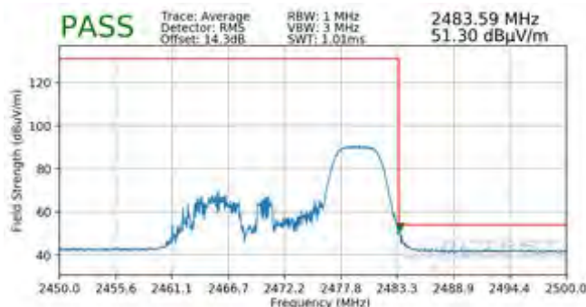
Plot 7-123. Radiated Restricted Upper Band Edge Measurement SISO ANT2 (Average – 52 Tones)
