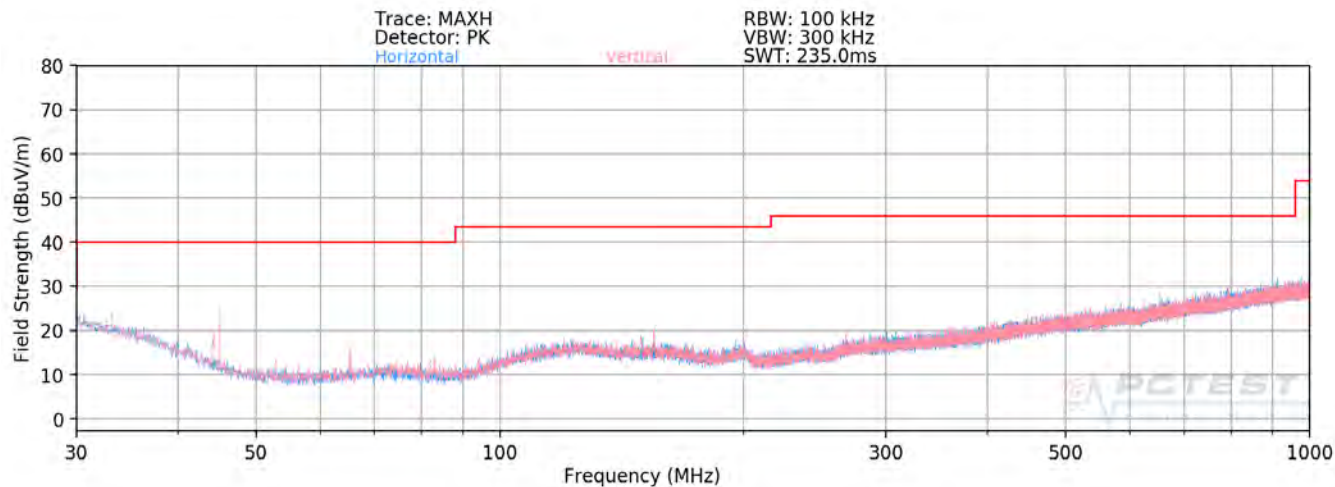
Plot 7-165. Radiated Spurious Plot below 1GHz SISO ANT1 (106 Tones - CLOSED)
