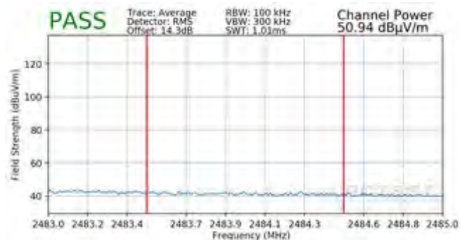
Plot 7-137. Radiated Restricted Band Edge Measurement SISO ANT2 with WCP (Average – 242 Tones)
