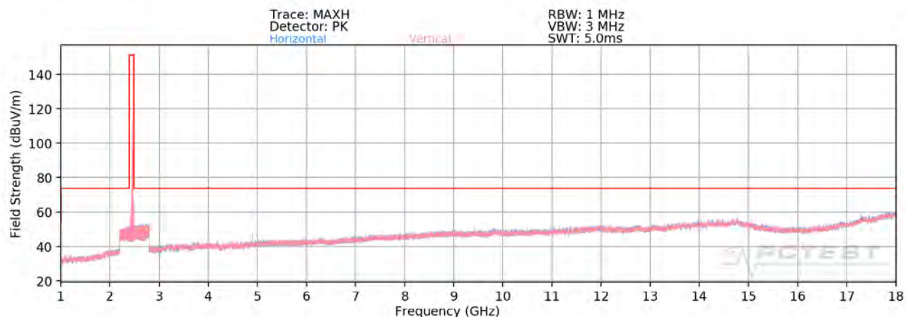
Plot 7-75. Radiated Spurious Plot above 1GHz SISO ANT2 (802.11ax OFDMA – 26 Tones – Ch. 11 – CLOSED)
