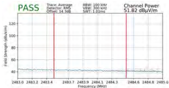
Plot 7-115. Radiated Restricted Band Edge Measurement SISO ANT1 with WCP (Average – 242 Tones)
