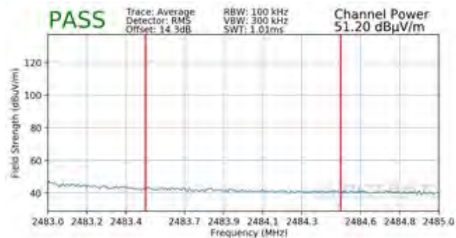
Plot 7-135. Radiated Restricted Upper Band Edge Measurement SISO ANT2 (Average – 242 Tones)
