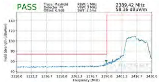
Plot 7-142. Radiated Restricted Lower Band Edge Measurement MIMO (Peak - 106 Tones)
