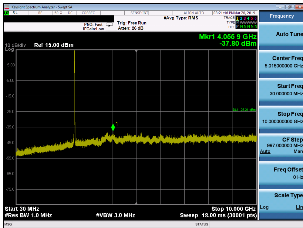
Plot 7-45. Conducted Spurious Plot SISO ANT1 (802.11ax OFDMA- 106 Tones - Ch. 11)
