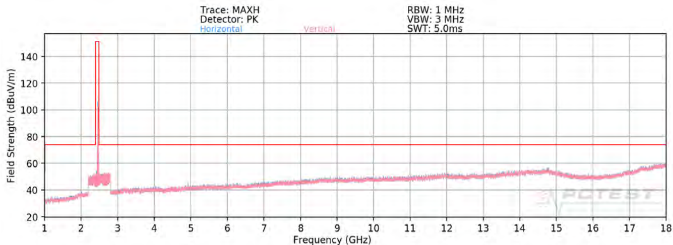
Plot 7-86. Radiated Spurious Plot above 1GHz MIMO (802.11ax OFDMA – 242 Tones – Ch. 11 – CLOSED)
