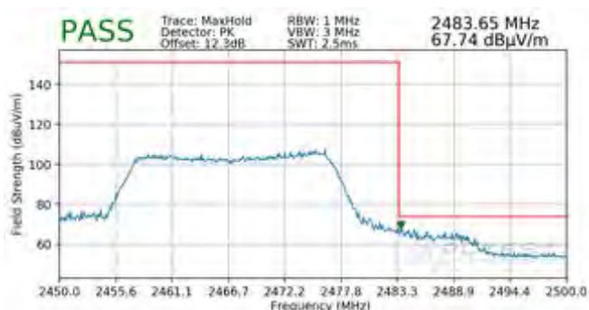
Plot 7-112. Radiated Restricted Upper Band Edge Measurement SISO ANT1 (Peak - 242 Tones)
