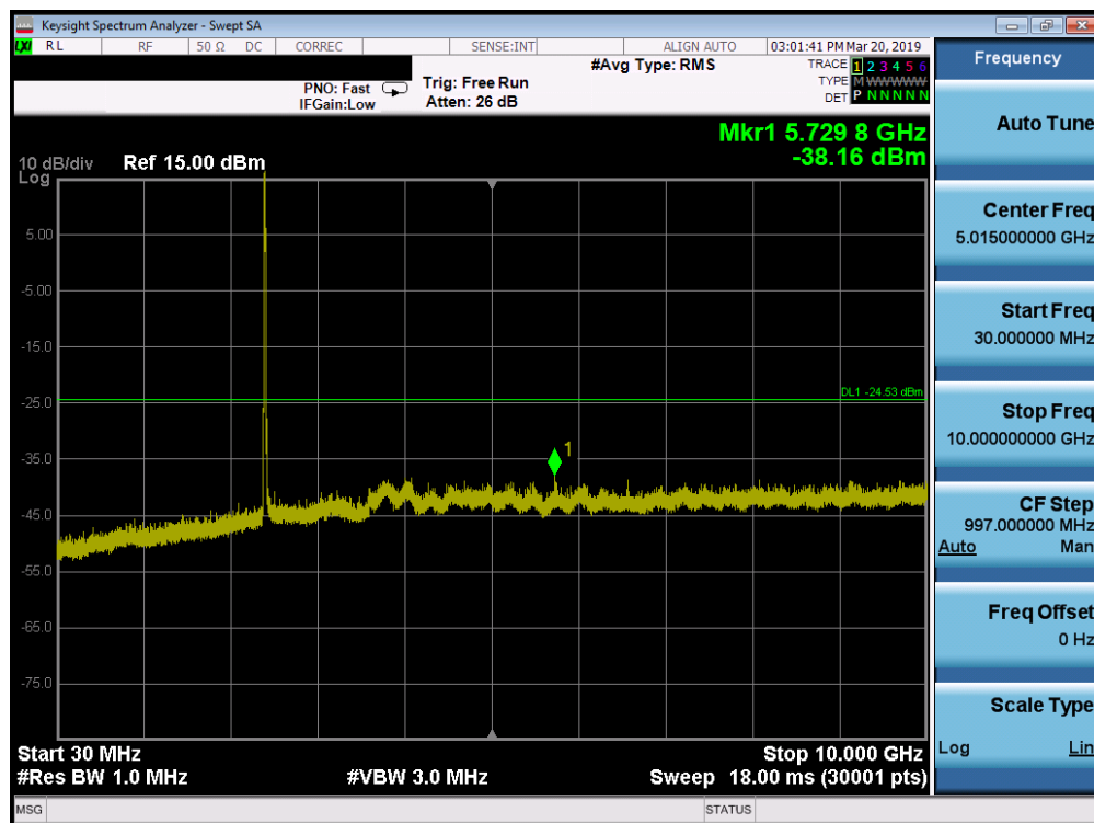
Plot 7-41. Conducted Spurious Plot SISO ANT1 (802.11ax OFDMA – 106 Tones – Ch. 1)
