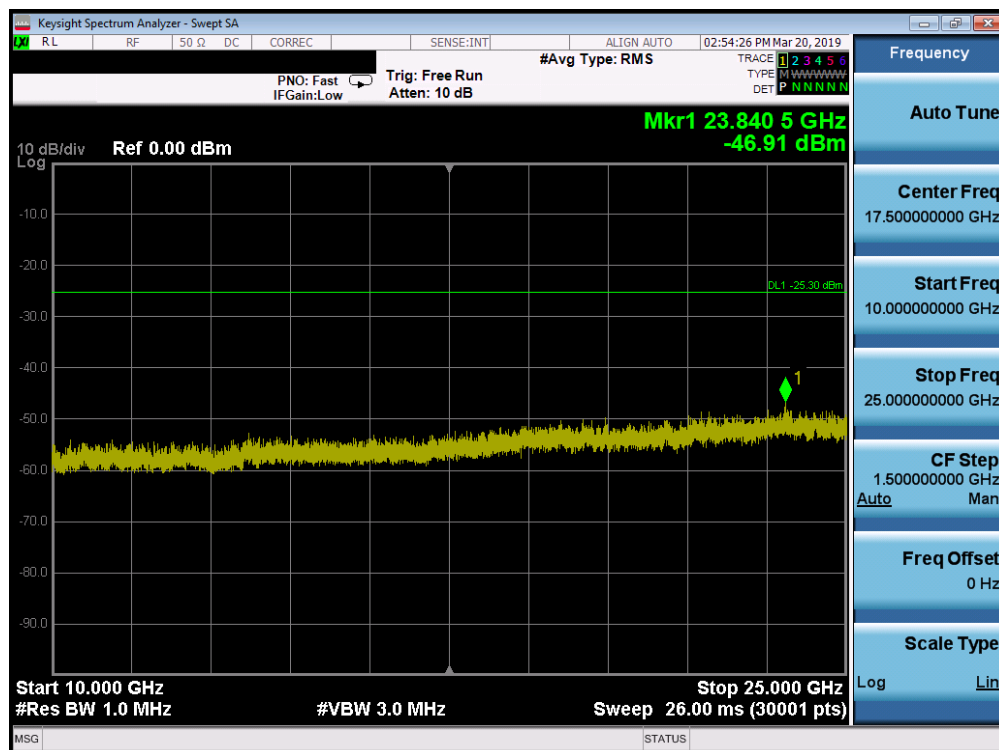
Plot 7-50. Conducted Spurious Plot SISO ANT1 (802.11ax OFDMA- 242 Tones - Ch. 6)
