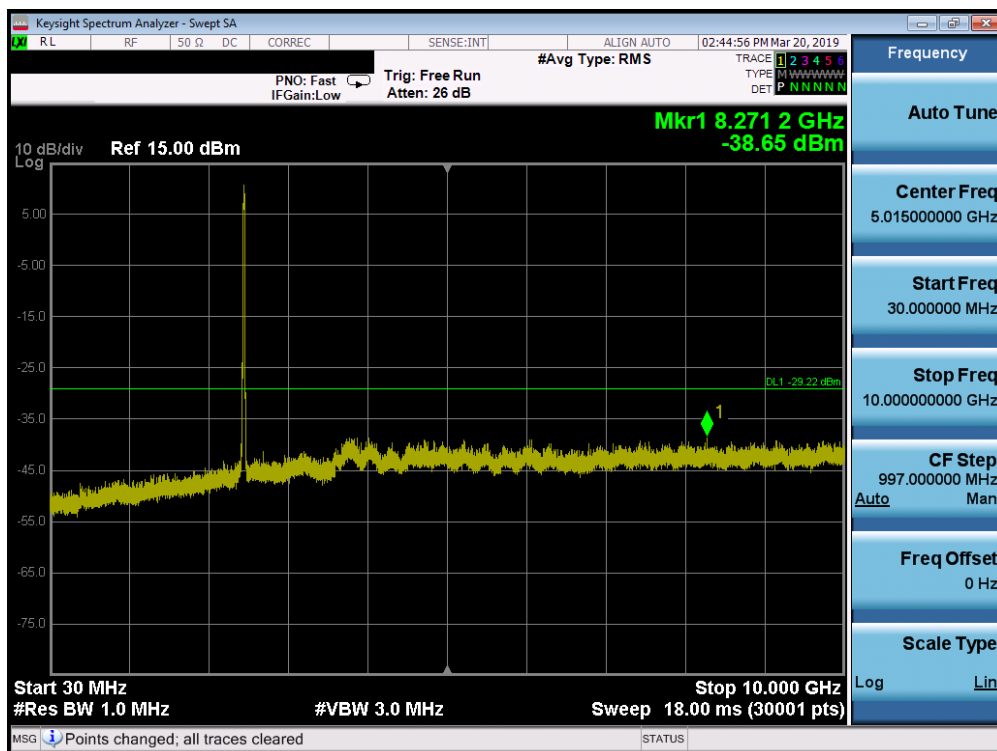
Plot 7-51. Conducted Spurious Plot SISO ANT1 (802.11ax OFDMA- 242 Tones - Ch. 11)
