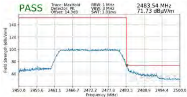
Plot 7-136. Radiated Restricted Upper Band Edge Measurement SISO ANT2 (Peak – 242 Tones)
