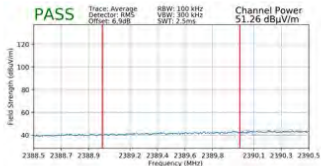
Plot 7-151. Radiated Restricted Lower Band Edge Measurement MIMO (Average - 242 Tones)
