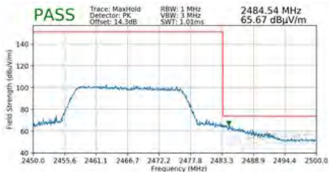
Plot 7-134. Radiated Restricted Upper Band Edge Measurement SISO ANT2 (Peak – 242 Tones)
