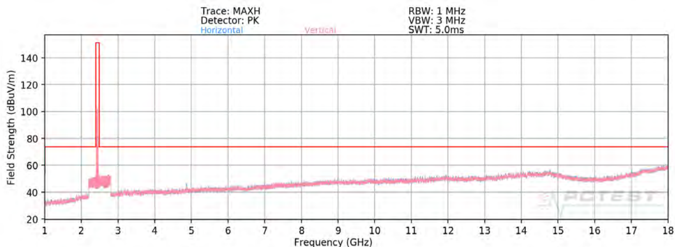
Plot 7-77. Radiated Spurious Plot above 1GHz SISO ANT2 (802.11ax OFDMA – 242 Tones – Ch. 6 – CLOSED)
