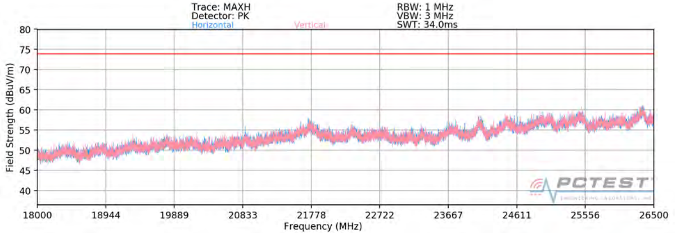
Plot 7-71. Radiated Spurious Plot above 18GHz SISO ANT1 (802.11ax OFDMA – 26 Tones – CLOSED)
