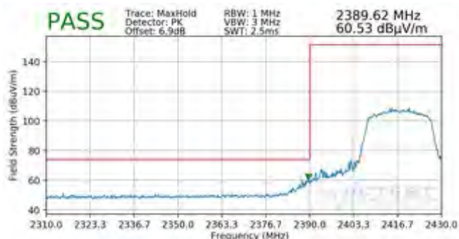
Plot 7-154. Radiated Restricted Lower Band Edge Measurement MIMO (Peak - 242 Tones)
