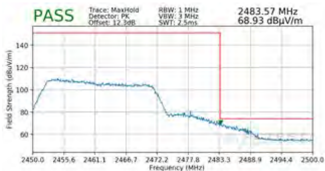
Plot 7-110. Radiated Restricted Upper Band Edge Measurement SISO ANT1 (Peak - 242 Tones)
