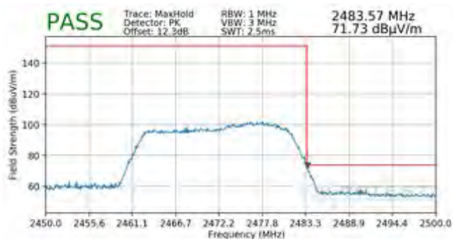
Plot 7-114. Radiated Restricted Upper Band Edge Measurement SISO ANT1 (Peak – 242 Tones)
