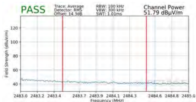
Plot 7-161. Radiated Restricted Upper Band Edge Measurement MIMO (Average – 242 Tones)
