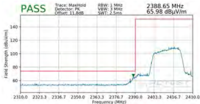
Plot 7-98. Radiated Restricted Lower Band Edge Measurement SISO ANT1 (Peak - 242 Tones)
