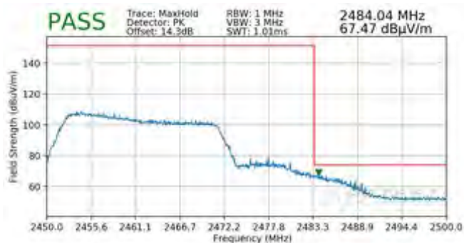
Plot 7-116. Radiated Restricted Band Edge Measurement SISO ANT1 with WCP (Peak – 242 Tones)
