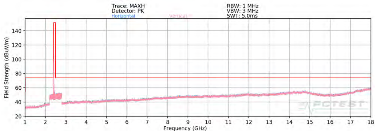
Plot 7-81. Radiated Spurious Plot above 1GHz MIMO (802.11ax OFDMA – 26 Tones – Ch. 1 – CLOSED)
