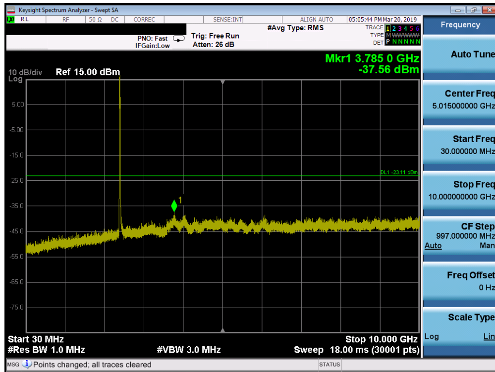
Plot 7-53. Conducted Spurious Plot SISO ANT2 (802.11ax OFDMA – 106 Tones – Ch. 1)
