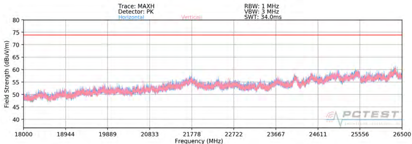
Plot 7-79. Radiated Spurious Plot above 18GHz SISO ANT2 (802.11ax OFDMA – 26 Tones – CLOSED)
