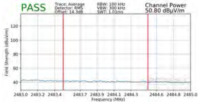
Plot 7-163. Radiated Restricted Band Edge Measurement MIMO with WCP (Average – 242 Tones)
