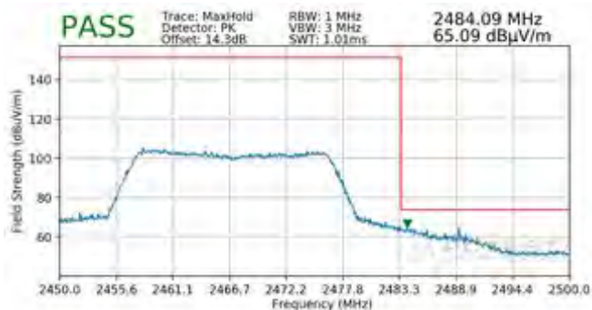
Plot 7-160. Radiated Restricted Upper Band Edge Measurement MIMO (Peak – 242 Tones)
