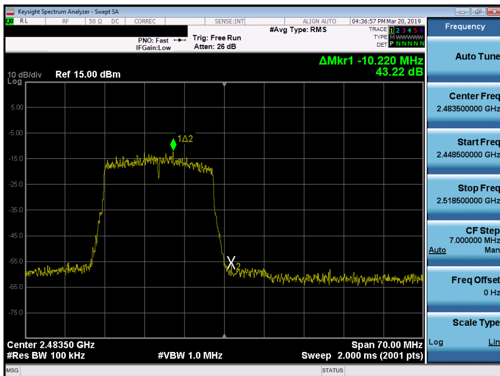
Plot 7-32. Band Edge Plot SISO ANT1 (802.11ax OFDMA - 242 Tones - Ch. 13)
