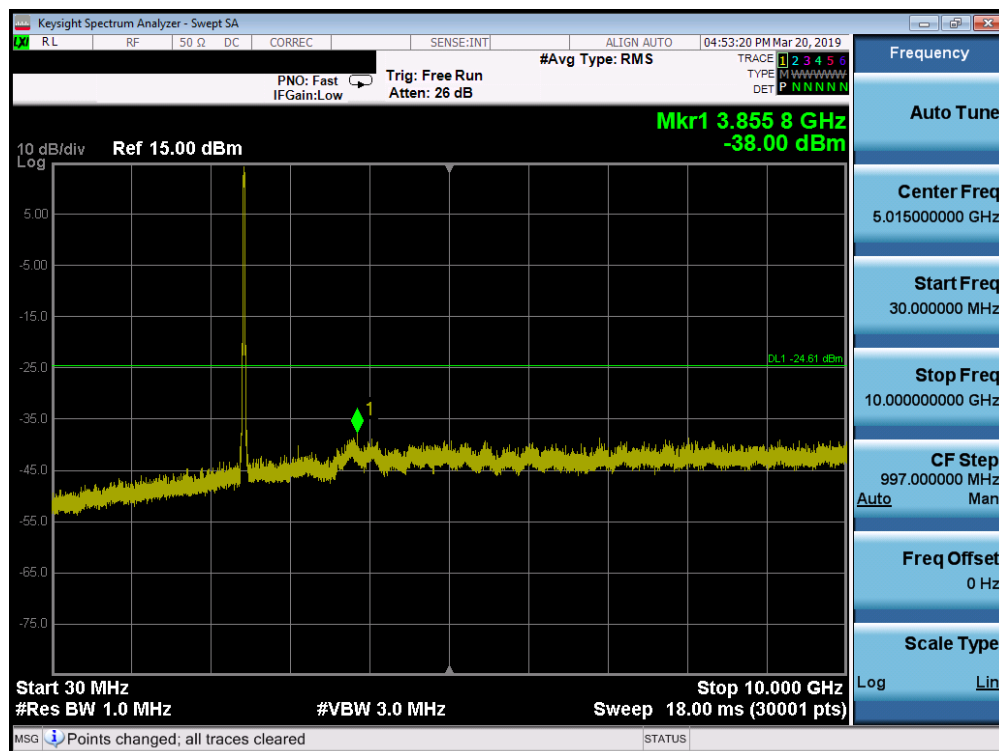
Plot 7-61. Conducted Spurious Plot SISO ANT2 (802.11ax OFDMA- 242 Tones - Ch. 6)
