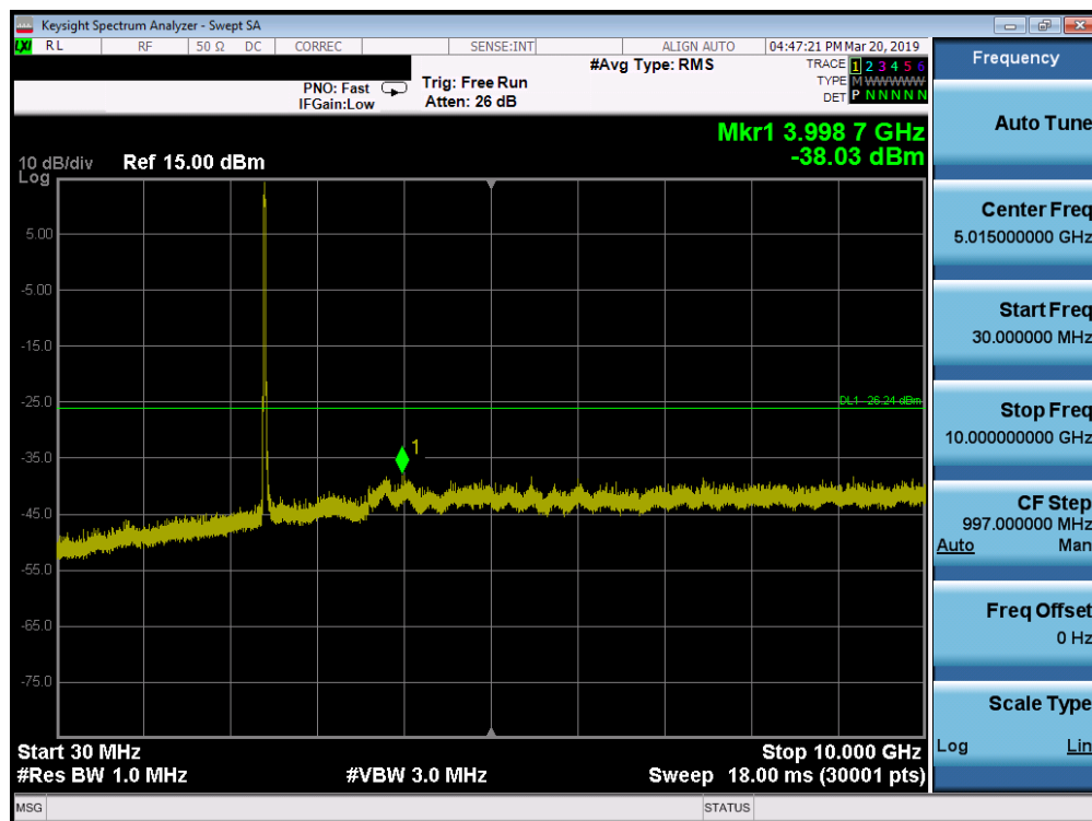
Plot 7-59. Conducted Spurious Plot SISO ANT2 (802.11ax OFDMA – 106 Tones – Ch. 1)
