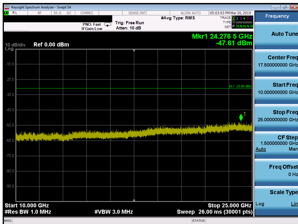
Plot 7-64. Conducted Spurious Plot SISO ANT2 (802.11ax OFDMA- 242 Tones - Ch. 11)
