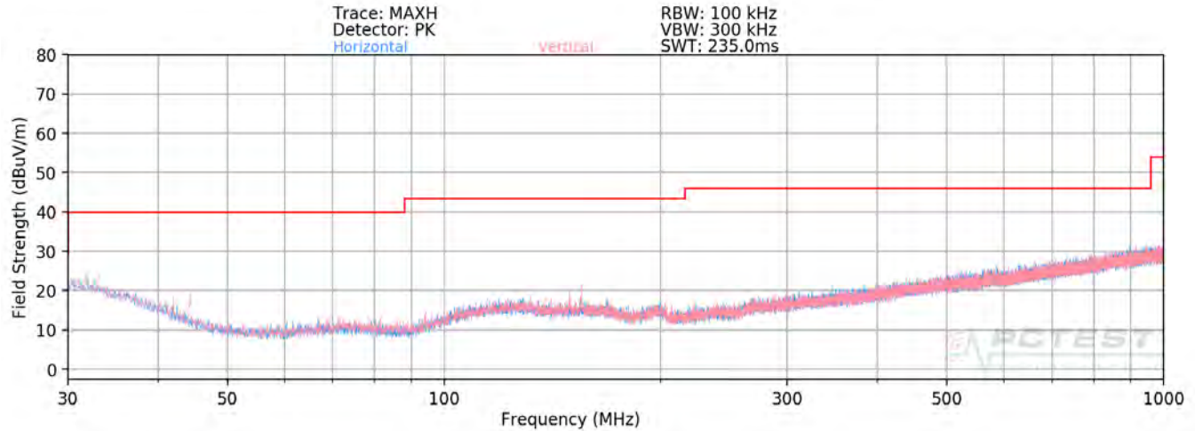
Plot 7-167. Radiated Spurious Plot below 1GHz SISO ANT2 (106 Tones - CLOSED)
