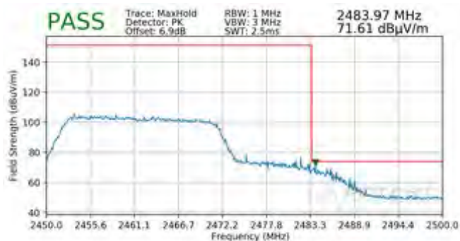
Plot 7-132. Radiated Restricted Upper Band Edge Measurement SISO ANT2 (Peak - 242 Tones)
