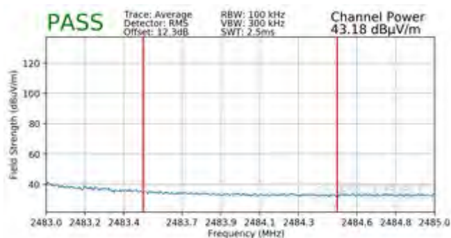
Plot 7-95. Radiated Restricted Upper Band Edge Measurement SISO ANT1 (Average – 26 Tones)
