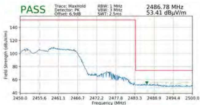
Plot 7-144. Radiated Restricted Upper Band Edge Measurement MIMO (Peak - 106 Tones)
