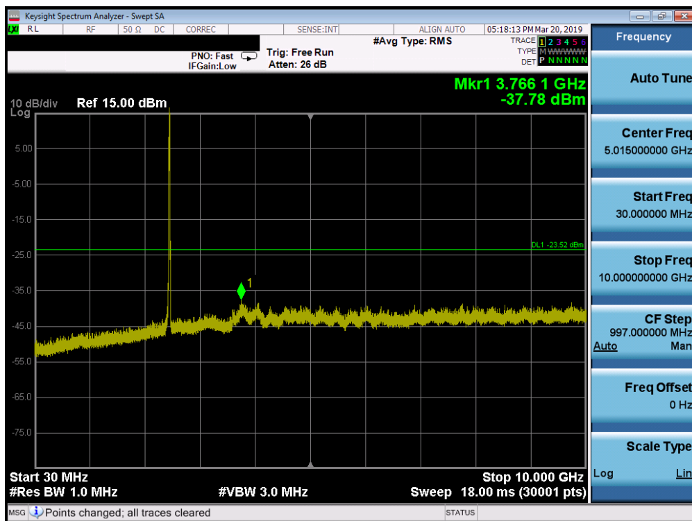
Plot 7-57. Conducted Spurious Plot SISO ANT2 (802.11ax OFDMA- 106 Tones - Ch. 11)
