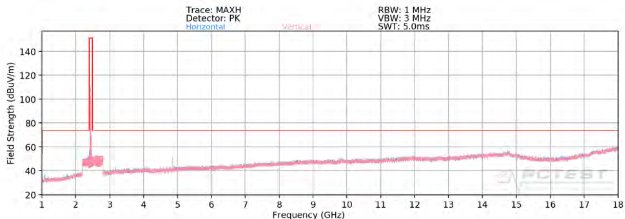
Plot 7-82. Radiated Spurious Plot above 1GHz MIMO (802.11ax OFDMA – 26 Tones – Ch. 6 – CLOSED)
