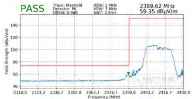
Plot 7-140. Radiated Restricted Lower Band Edge Measurement MIMO (Peak - 106 Tones)
