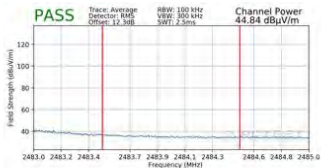
Plot 7-113. Radiated Restricted Upper Band Edge Measurement SISO ANT1 (Average – 242 Tones)
