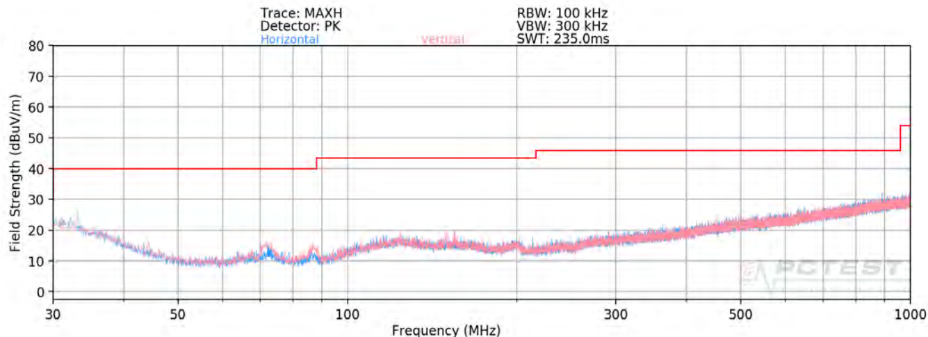
Plot 7-169. Radiated Spurious Plot below 1GHz MIMO (26 Tones - CLOSED)
