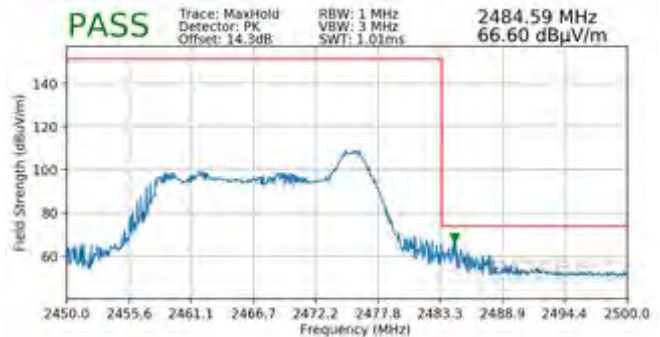
Plot 7-122. Radiated Restricted Upper Band Edge Measurement SISO ANT2 (Peak – 26 Tones)
