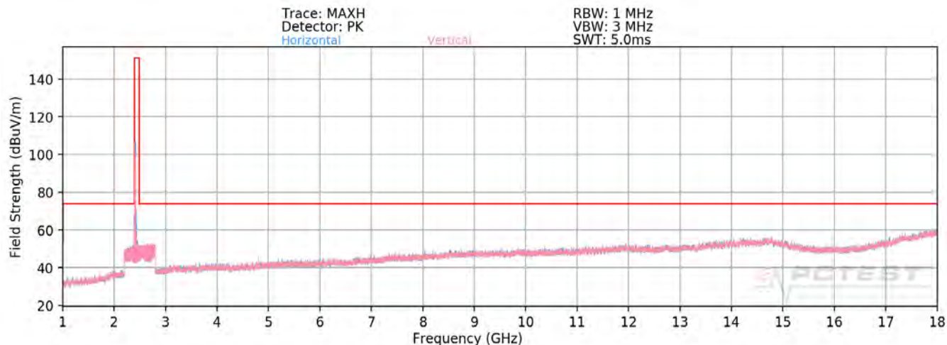
Plot 7-84. Radiated Spurious Plot above 1GHz MIMO (802.11ax OFDMA – 242 Tones – Ch. 1 – CLOSED)
