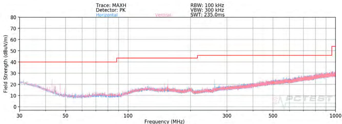
Plot 7-166. Radiated Spurious Plot below 1GHz SISO ANT1 (242 Tones - CLOSED)
