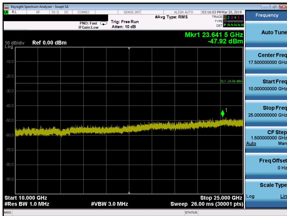
Plot 7-44. Conducted Spurious Plot SISO ANT1 (802.11ax OFDMA- 106 Tones – Ch. 6)
