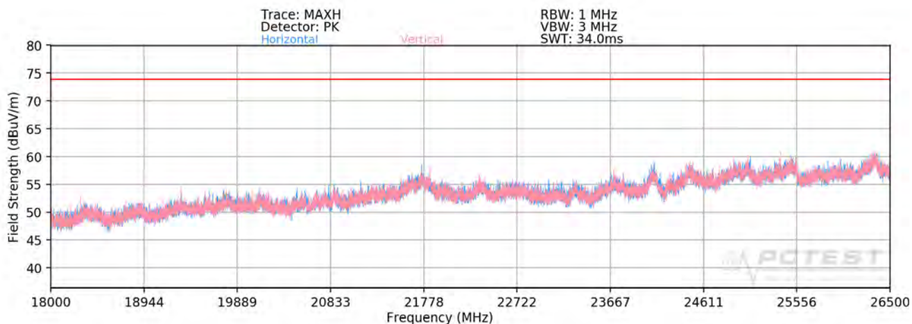
Plot 7-88. Radiated Spurious Plot above 18GHz MIMO (802.11ax OFDMA – 242 Tones – CLOSED)
