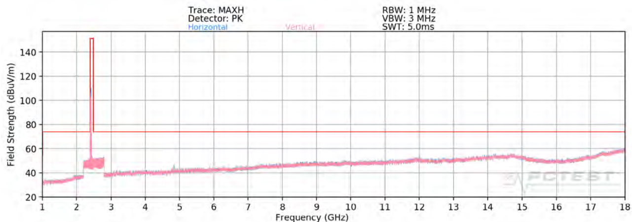
Plot 7-73. Radiated Spurious Plot above 1GHz SISO ANT2 (802.11ax OFDMA – 26 Tones – Ch. 1 – CLOSED)
