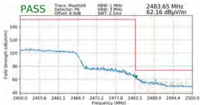
Plot 7-130. Radiated Restricted Upper Band Edge Measurement SISO ANT2 (Peak - 242 Tones)
