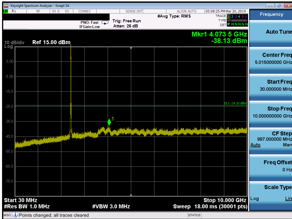
Plot 7-55. Conducted Spurious Plot SISO ANT2 (802.11ax OFDMA- 106 Tones – Ch. 6)
