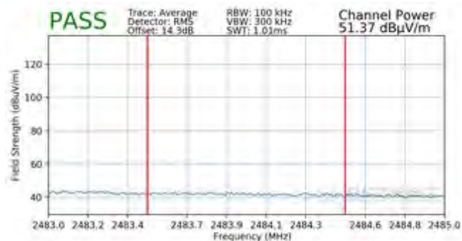
Plot 7-159. Radiated Restricted Upper Band Edge Measurement MIMO (Average – 242 Tones)
