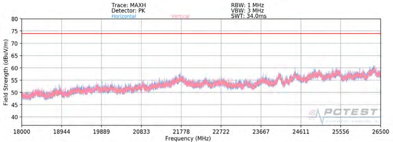
Plot 7-72. Radiated Spurious Plot above 18GHz SISO ANT1 (802.11ax OFDMA – 242 Tones – CLOSED)
