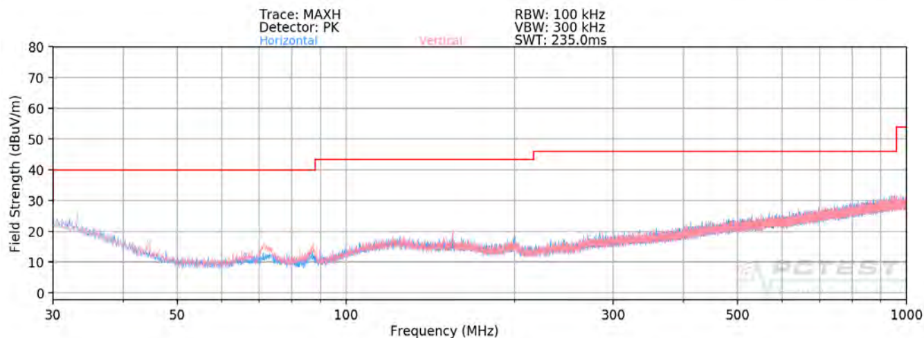
Plot 7-170. Radiated Spurious Plot below 1GHz MIMO (242 Tones - CLOSED)
