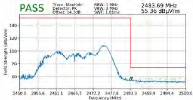
Plot 7-148. Radiated Restricted Upper Band Edge Measurement MIMO (Peak – 26 Tones)
