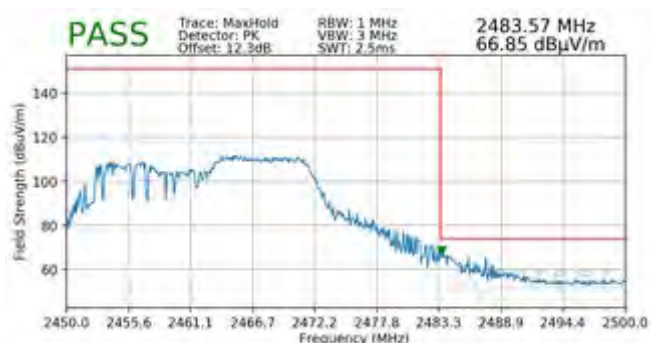
Plot 7-92. Radiated Restricted Upper Band Edge Measurement SISO ANT1 (Peak - 106 Tones)
