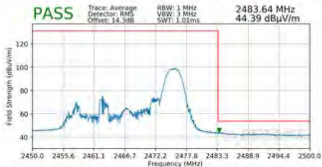
Plot 7-147. Radiated Restricted Upper Band Edge Measurement MIMO (Average – 26 Tones)
