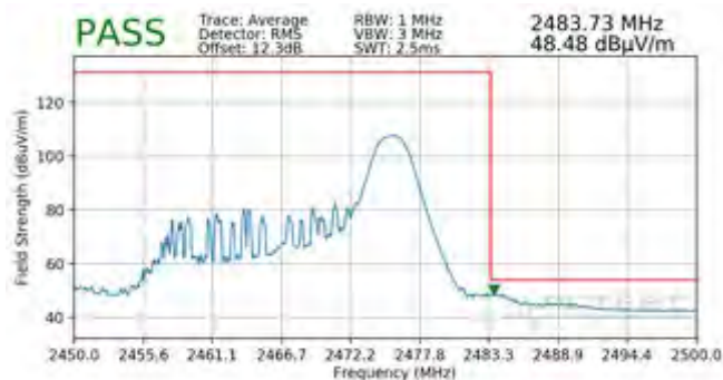
Plot 7-93. Radiated Restricted Upper Band Edge Measurement SISO ANT1 (Average – 26 Tones)
