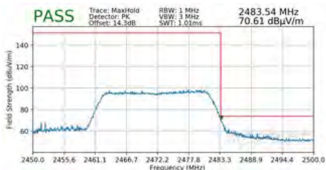
Plot 7-162. Radiated Restricted Upper Band Edge Measurement MIMO (Peak – 242 Tones)
