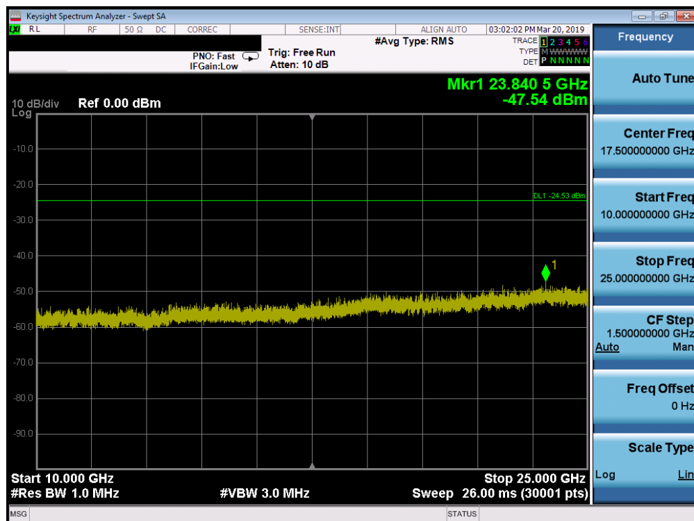
Plot 7-42. Conducted Spurious Plot SISO ANT1 (802.11ax OFDMA– 106 Tones – Ch. 1)
