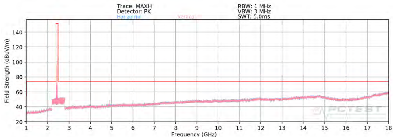
Plot 7-74. Radiated Spurious Plot above 1GHz SISO ANT2 (802.11ax OFDMA – 26 Tones – Ch. 6 – CLOSED)
