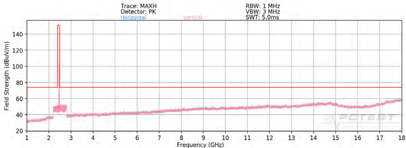
Plot 7-70. Radiated Spurious Plot above 1GHz SISO ANT1 (802.11ax OFDMA – 242 Tones – Ch. 11 – CLOSED)
