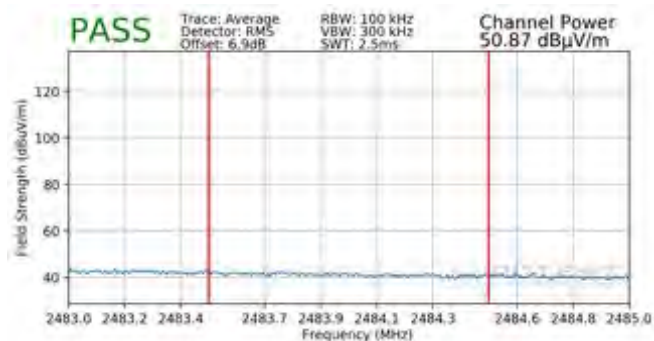
Plot 7-157. Radiated Restricted Upper Band Edge Measurement MIMO (Average - 242 Tones)
