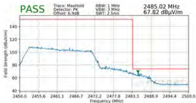
Plot 7-158. Radiated Restricted Upper Band Edge Measurement MIMO (Peak - 242 Tones)
