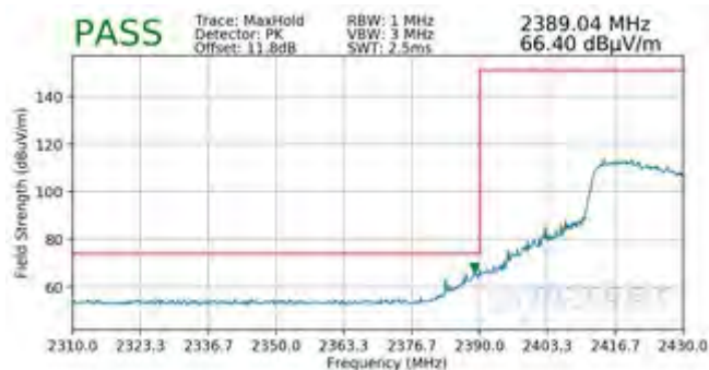
Plot 7-102. Radiated Restricted Lower Band Edge Measurement SISO ANT1 (Peak – 242 Tones)
