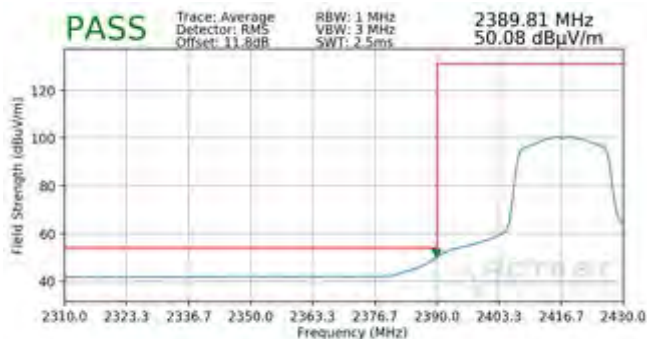
Plot 7-99. Radiated Restricted Lower Band Edge Measurement SISO ANT1 (Average - 242 Tones)
