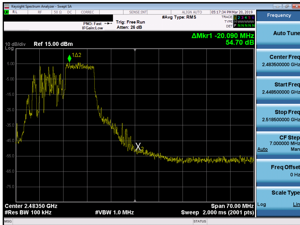
Plot 7-34. Band Edge Plot SISO ANT2 (802.11ax OFDMA - 106 Tones - Ch. 11)
