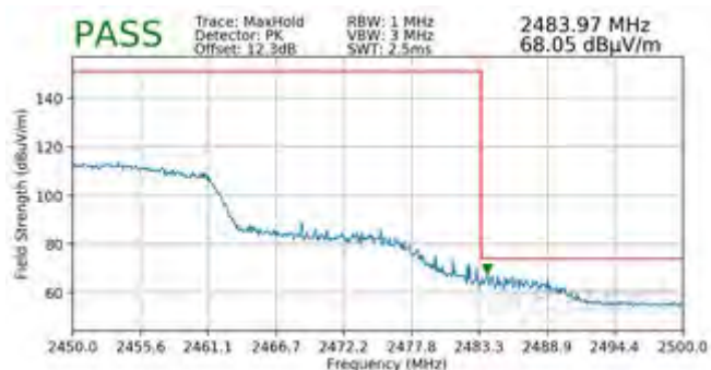
Plot 7-106. Radiated Restricted Upper Band Edge Measurement SISO ANT1 (Peak – 242 Tones)
