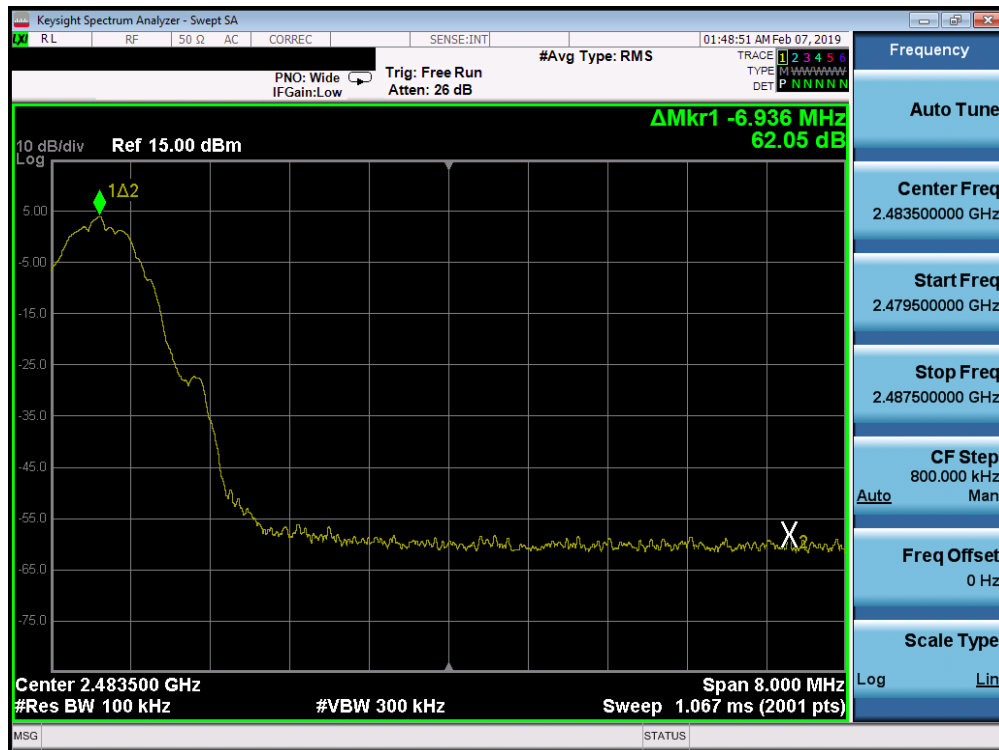
Plot 7-38. Band Edge Plot (Bluetooth (LE), 1Mbps – Ch. 39)
