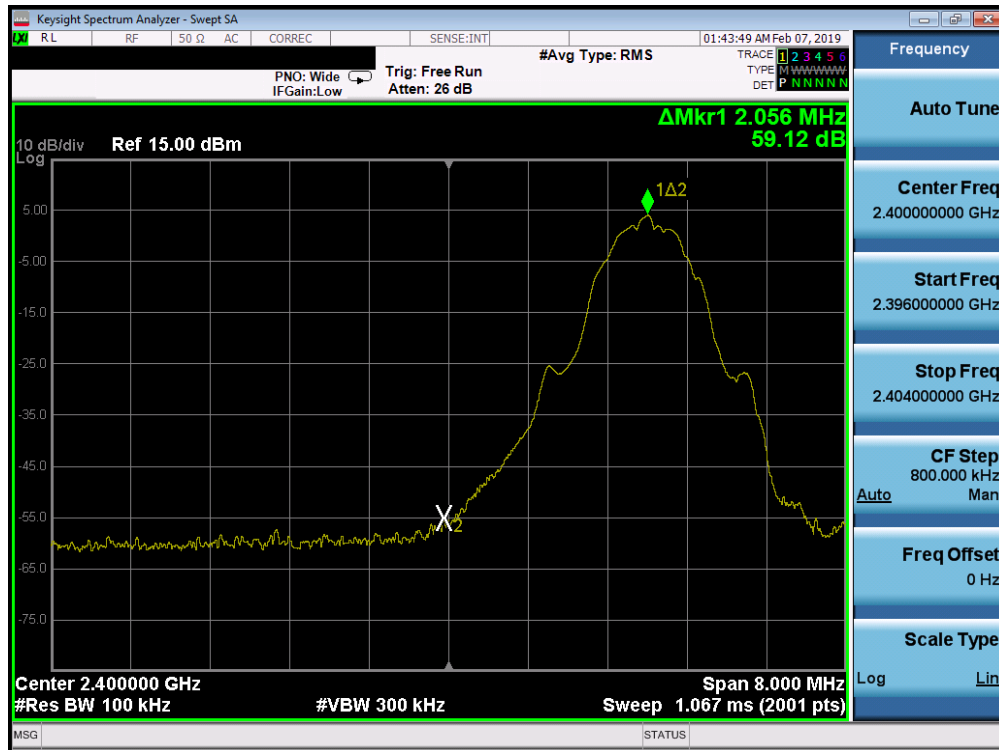
Plot 7-37. Band Edge Plot (Bluetooth (LE), 1Mbps – Ch. 0)
