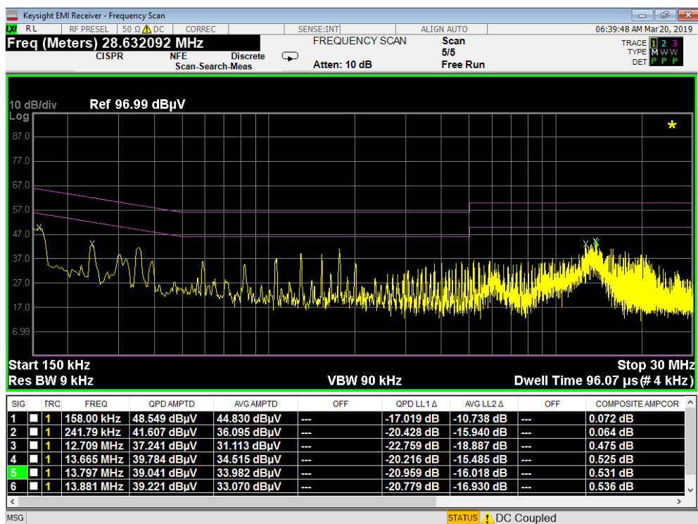
Plot 7-52. Line Conducted Plot with Bluetooth LE (N with WCP)
