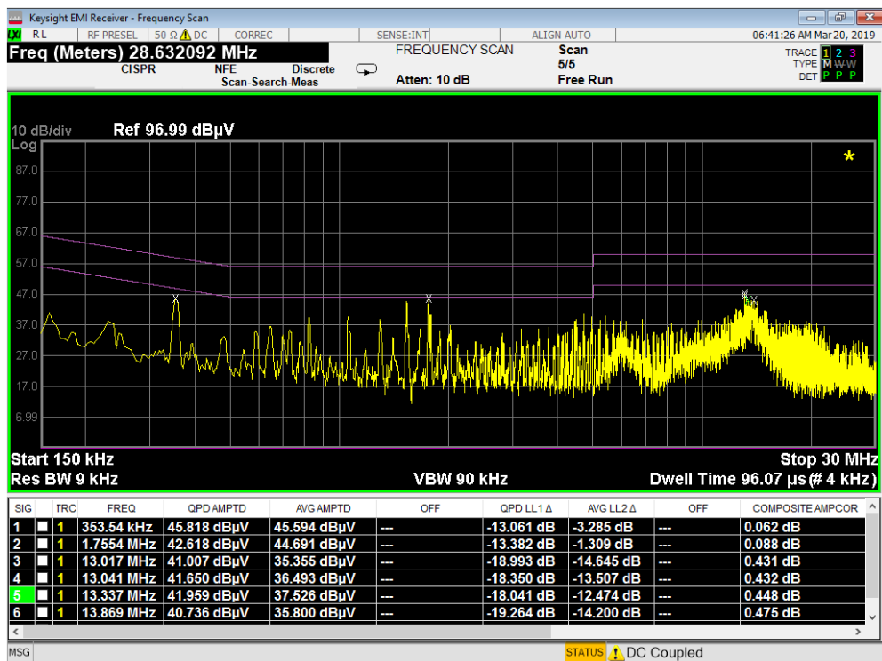
Plot 7-51. Line Conducted Plot with Bluetooth LE (L1 with WCP)
