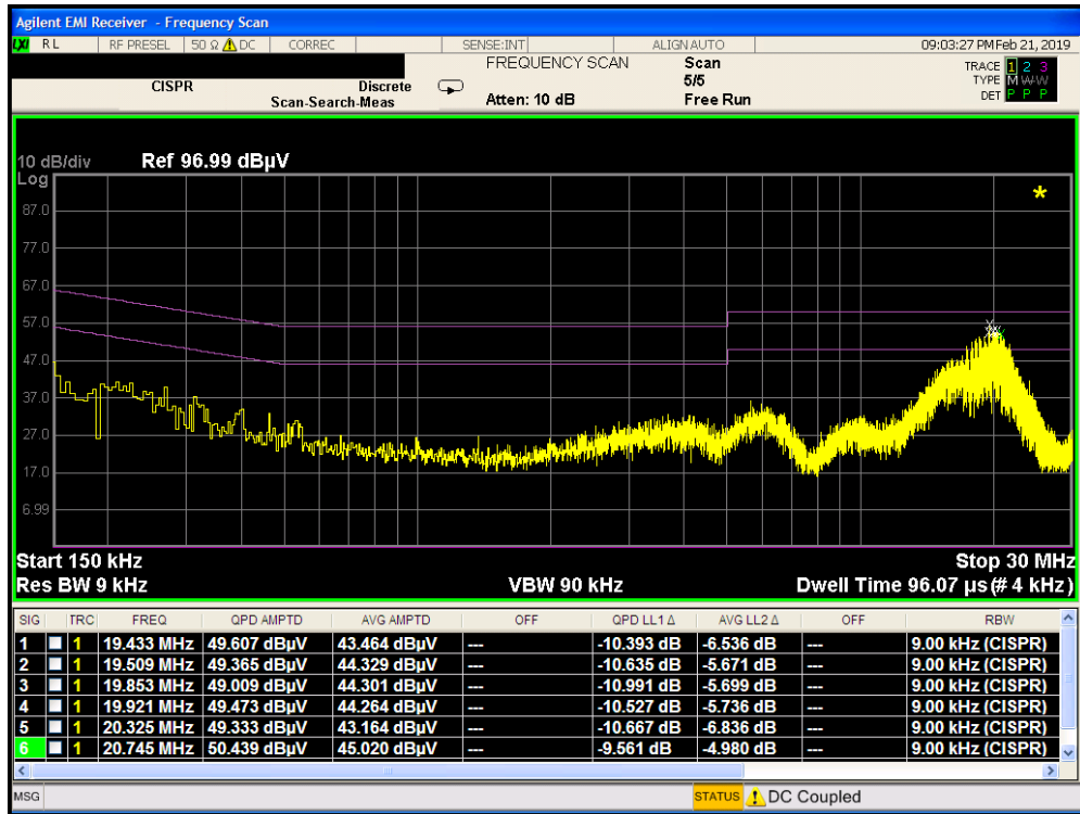
Plot 7-49. Line Conducted Plot with Bluetooth LE (L1)
