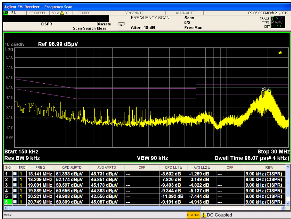
Plot 7-50. Line Conducted Plot with Bluetooth LE (N)
