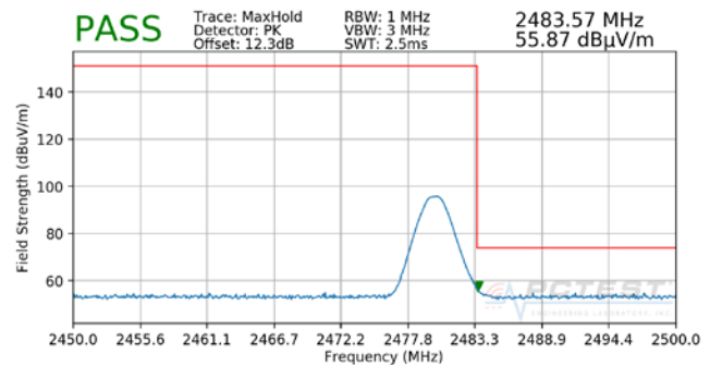
Plot 7-46. Radiated Restricted Upper Band Edge Measurement (Peak) - OPEN
