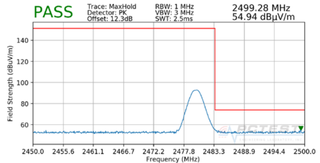
Plot 7-48. Radiated Restricted Upper Band Edge Measurement with WCP (Peak) - OPEN
