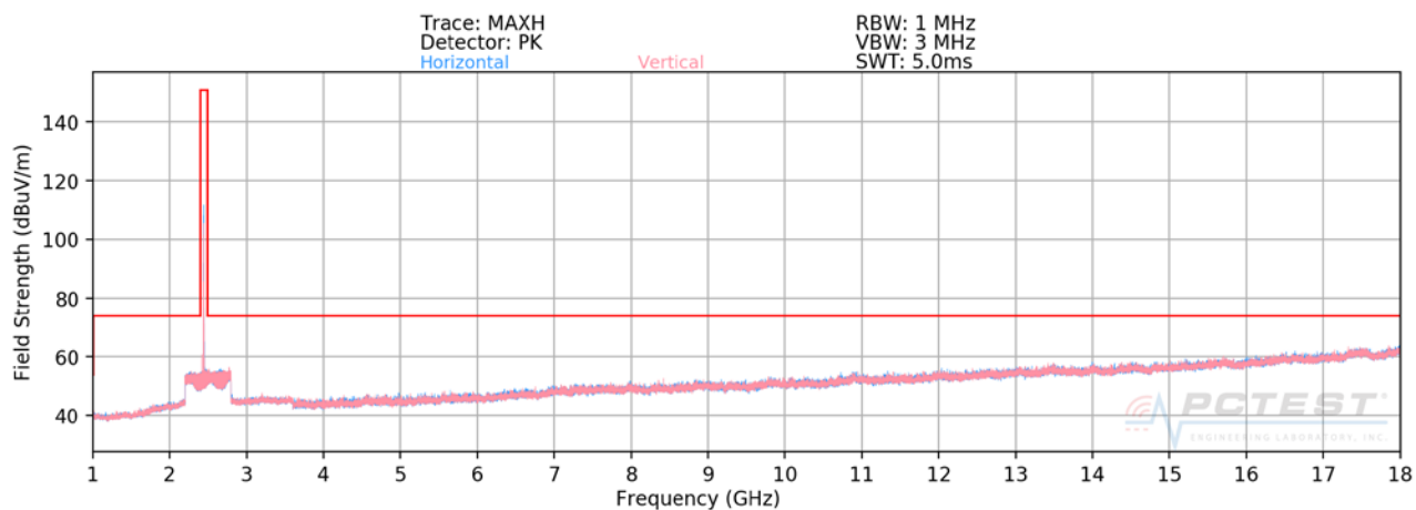
Plot 7-44. Radiated Spurious Plot above 1GHz (BT- Ch. 39 - OPEN)
