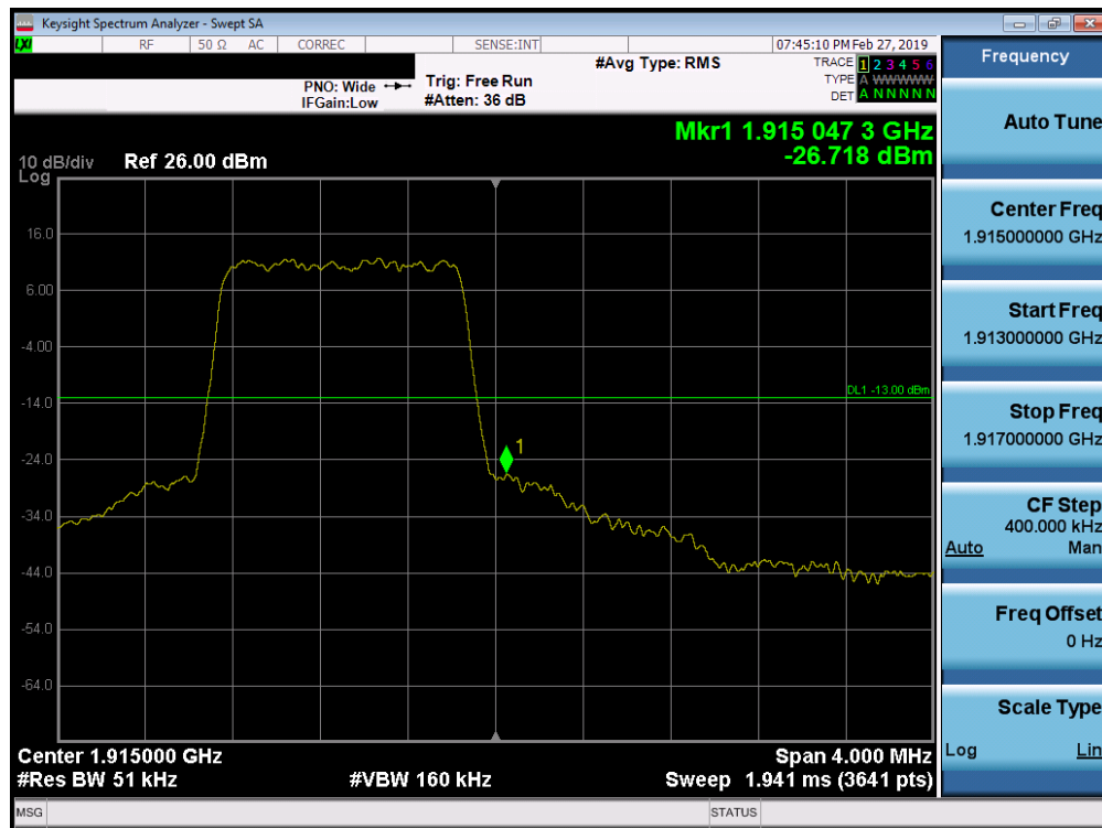
Plot 7-267. Upper Band Edge Plot (Band 25 - 1.4MHz QPSK - Full RB Configuration)
