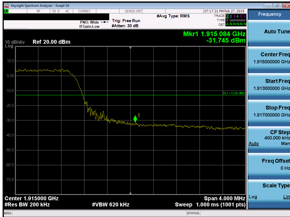
Plot 7-297. Upper Band Edge Plot (Band 25 - 20.0MHz QPSK - Full RB Configuration)
