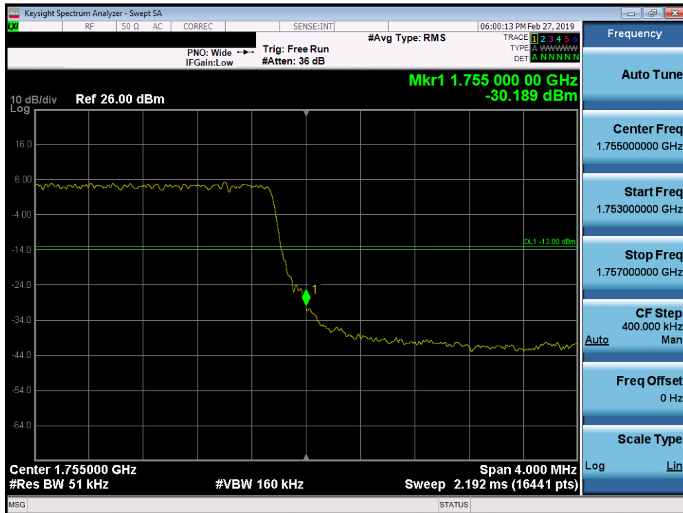
Plot 7-241. Upper Band Edge Plot (Band 4 – 5.0MHz QPSK - Full RB Configuration)
