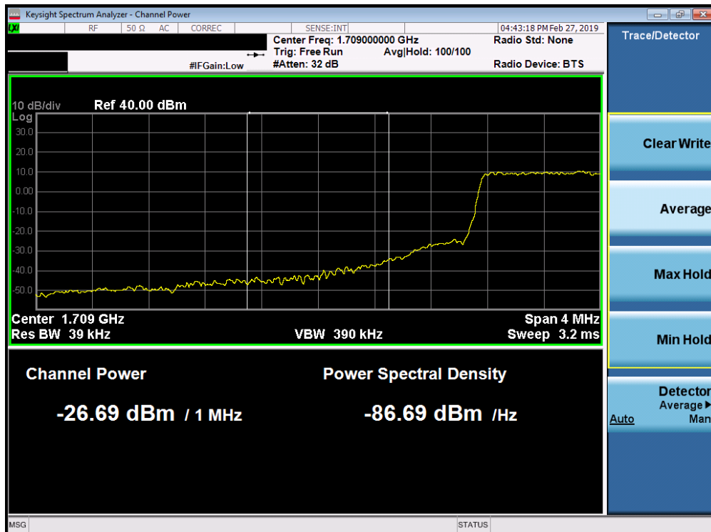
Plot 7-228. Lower Extended Band Edge Plot (Band 66/4 - 1.4MHz QPSK - Full RB Configuration)
