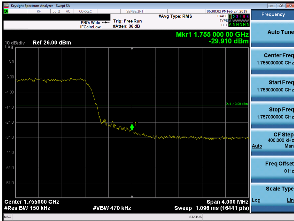
Plot 7-253. Upper Band Edge Plot (Band 4 – 15.0MHz QPSK - Full RB Configuration)
