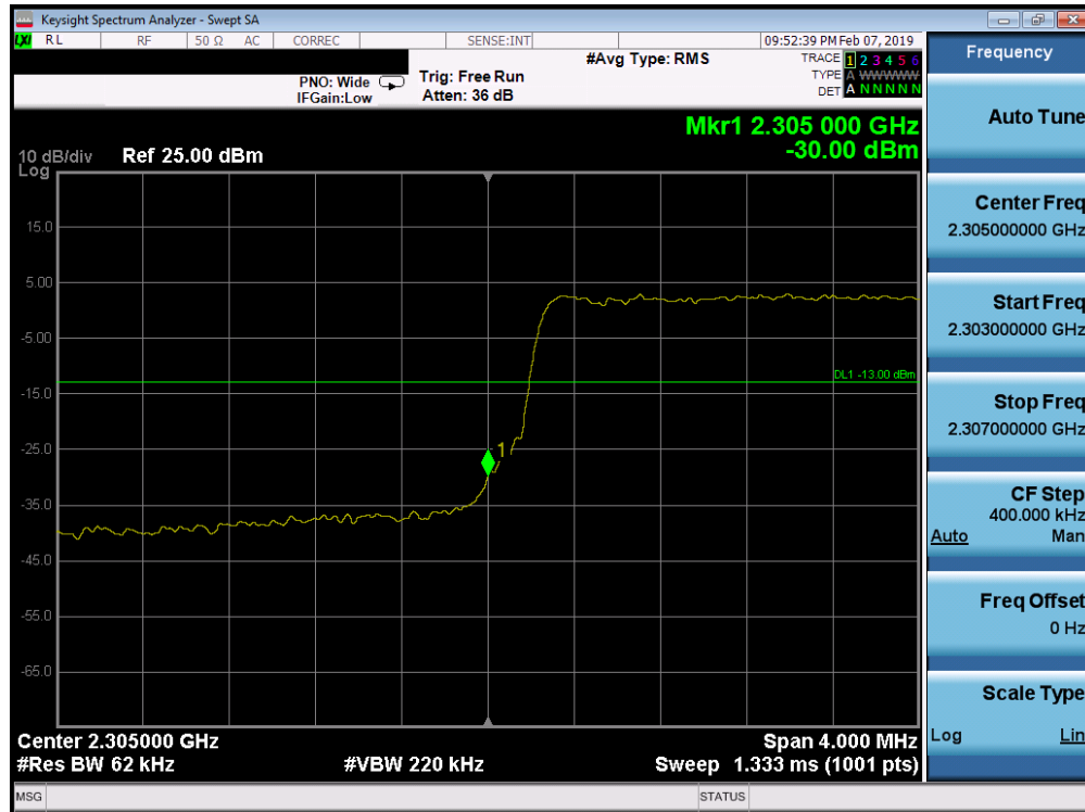
Plot 7-299. Lower Band Edge Plot (Band 30 - 5.0MHz QPSK - Full RB Configuration)
