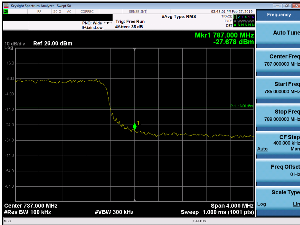
Plot 7-215. Upper Band Edge Plot (Band 13 - 10.0MHz QPSK - Full RB Configuration)
