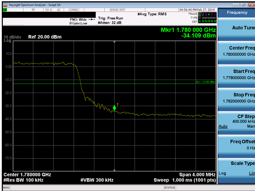
Plot 7-255. Upper Band Edge Plot (Band 66 - 15.0MHz QPSK - Full RB Configuration)
