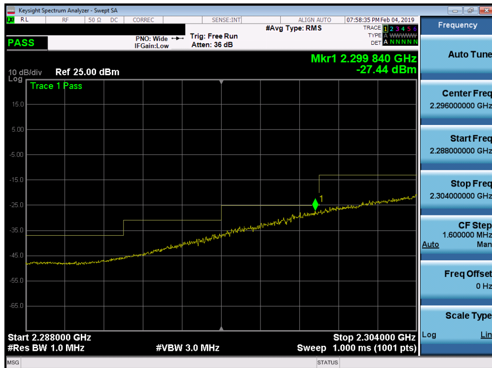
Plot 7-304. Lower Extended Band Edge Plot (Band 30 - 10.0MHz QPSK - Full RB Configuration)
