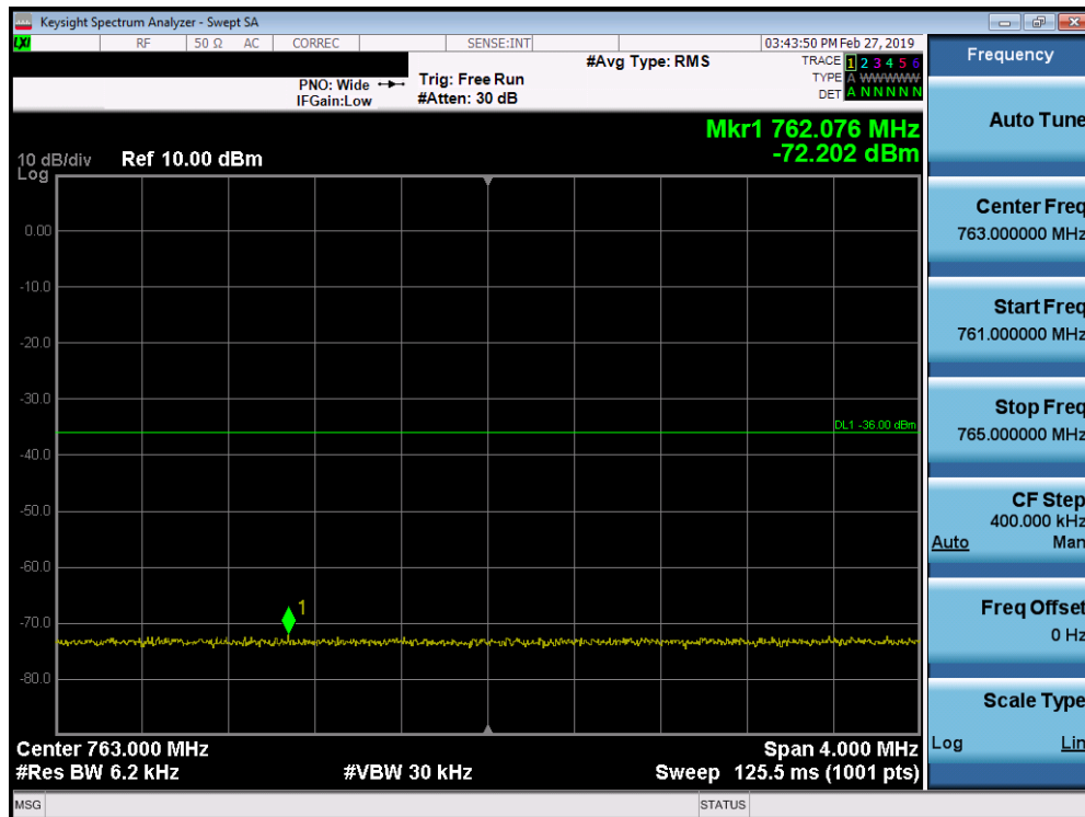
Plot 7-210. Lower Emission Mask Plot (Band 13 - 5.0MHz QPSK - Full RB Configuration)
