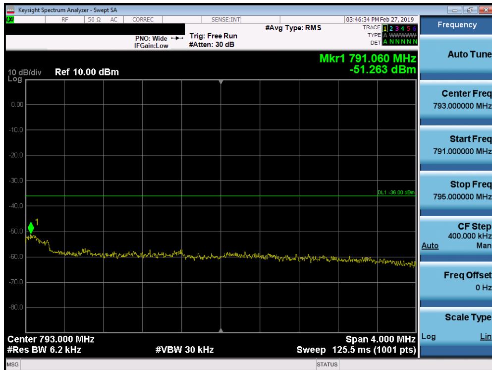
Plot 7-212. Upper Emission Mask Plot (Band 13 - 5.0MHz QPSK - Full RB Configuration)
