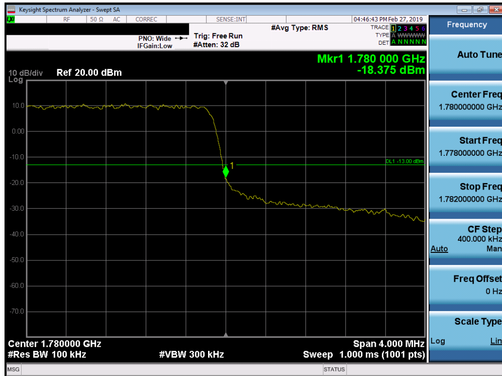
Plot 7-237. Upper Band Edge Plot (Band 66 - 3.0MHz QPSK - Full RB Configuration)
