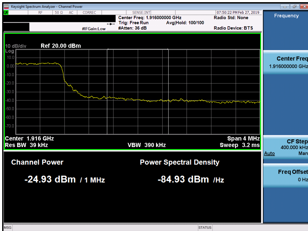
Plot 7-280. Upper Extended Band Edge Plot (Band 25 - 5.0MHz QPSK - Full RB Configuration)
