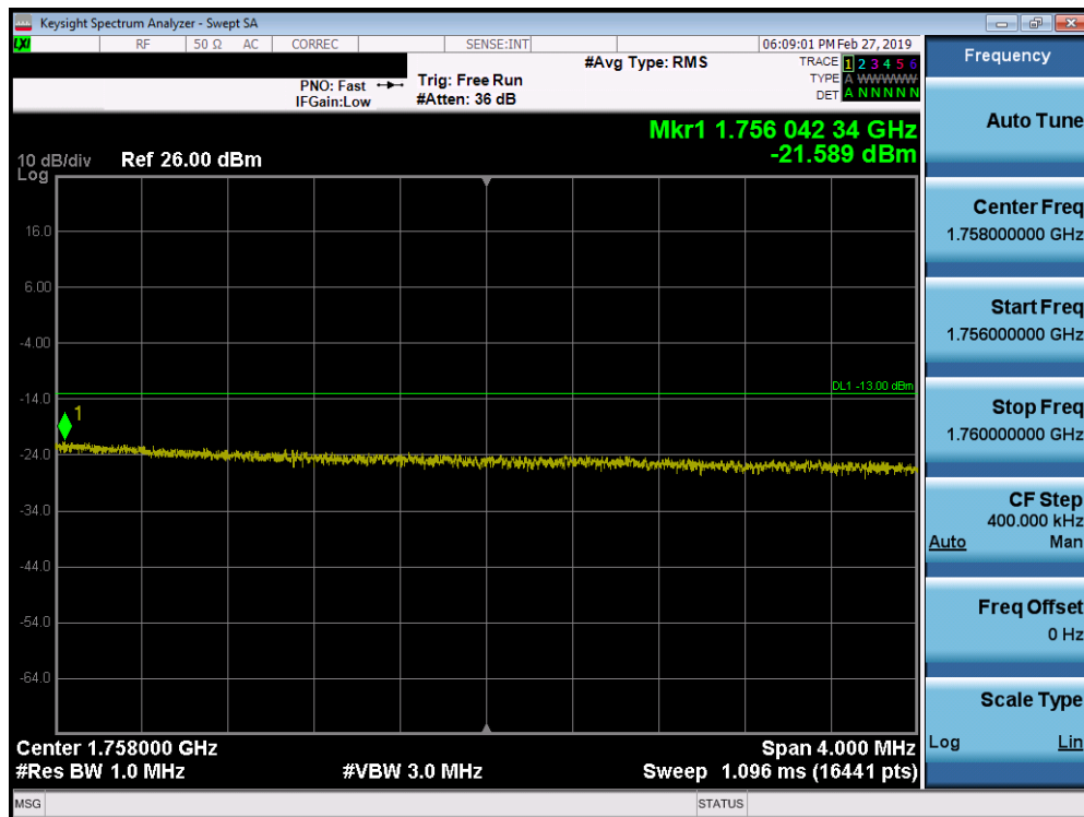
Plot 7-260. Upper Extended Band Edge Plot (Band 4 – 20.0MHz QPSK - Full RB Configuration)
