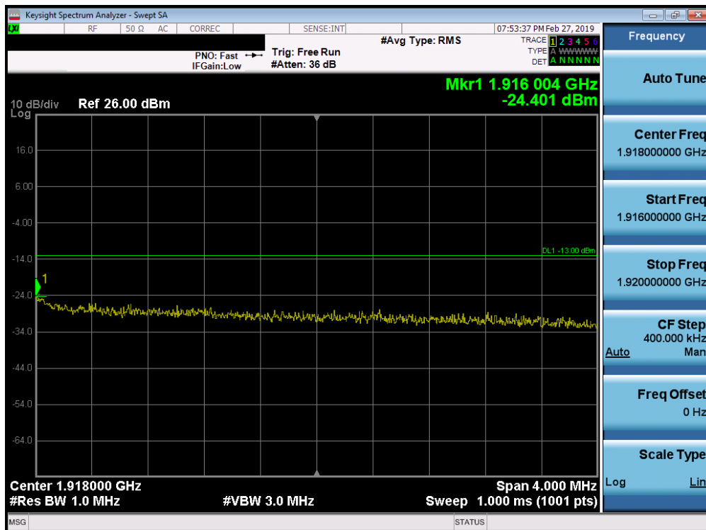
Plot 7-286. Upper Extended Band Edge Plot (Band 25/2 - 10.0MHz QPSK - Full RB Configuration)
