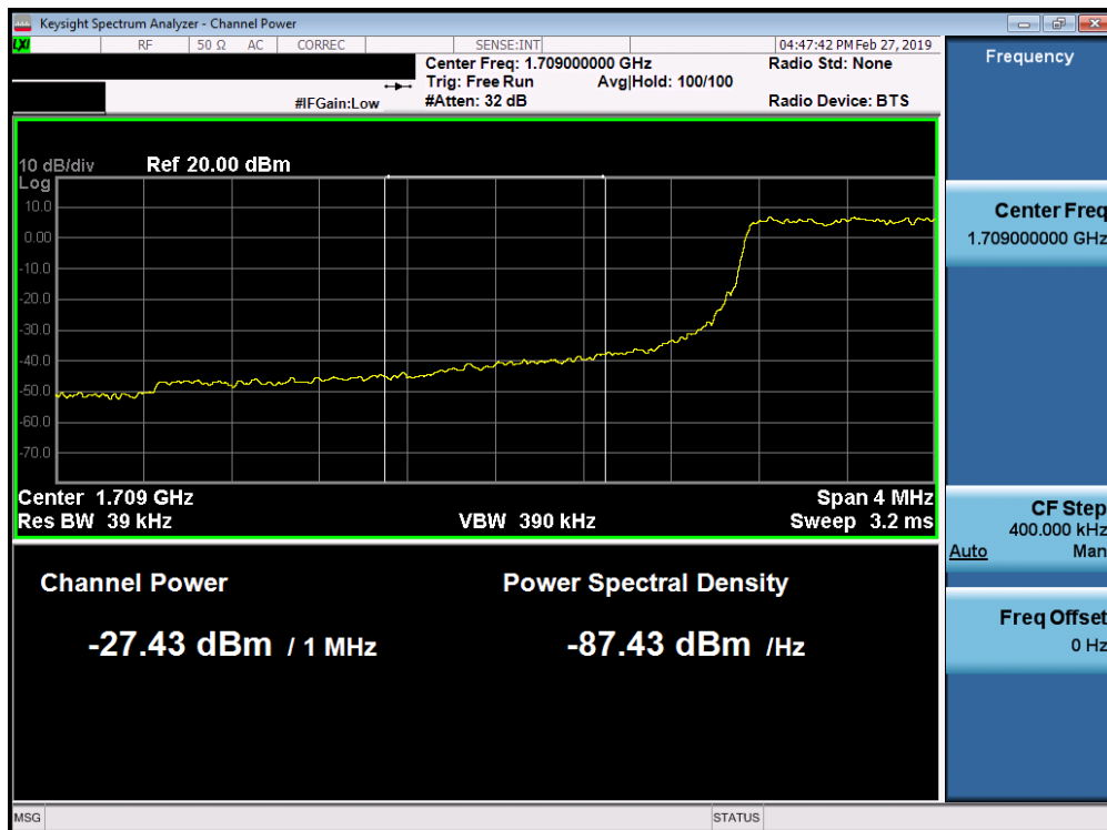
Plot 7-234. Lower Extended Band Edge Plot (Band 66/4 - 3.0MHz QPSK - Full RB Configuration)
