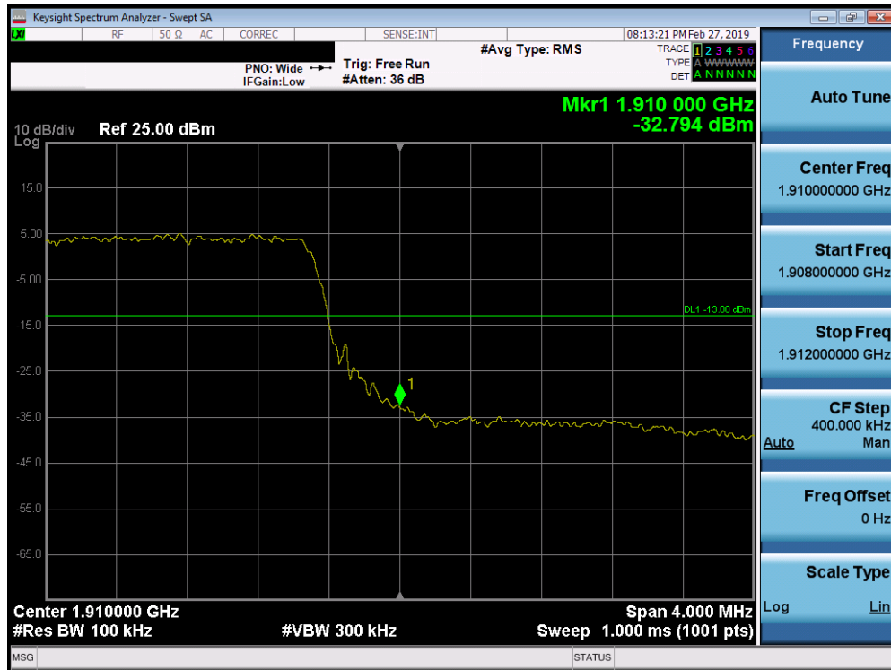
Plot 7-283. Upper Band Edge Plot (Band 2 – 10.0MHz QPSK - Full RB Configuration)
