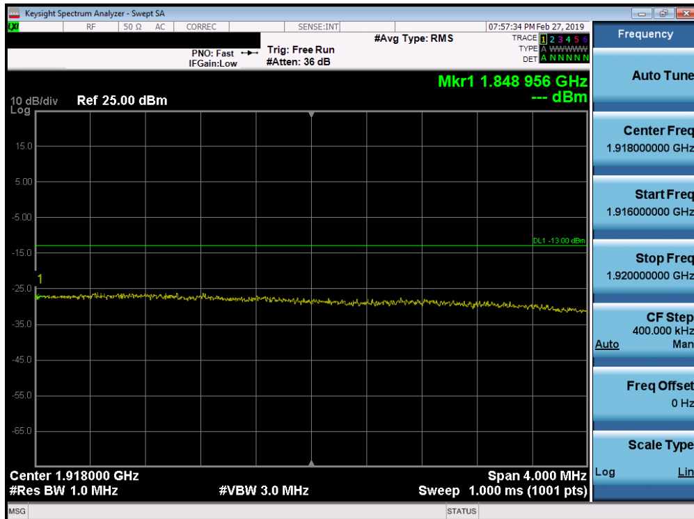
Plot 7-292. Upper Extended Band Edge Plot (Band 25 - 15.0MHz QPSK - Full RB Configuration)
