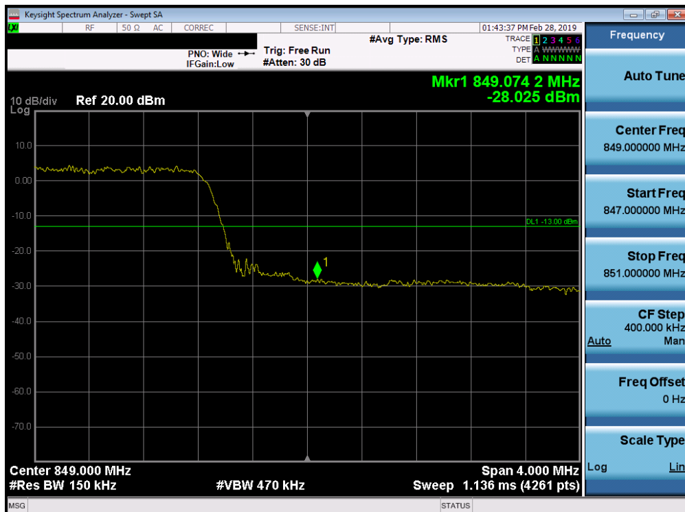
Plot 7-226. Upper Band Edge Plot (Band 26 - 15.0MHz QPSK - Full RB Configuration)
