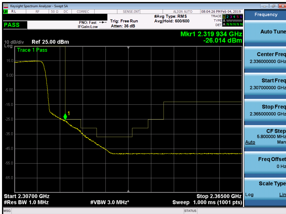
Plot 7-306. Upper Extended Band Edge Plot (Band 30 - 10.0MHz QPSK - Full RB Configuration)
