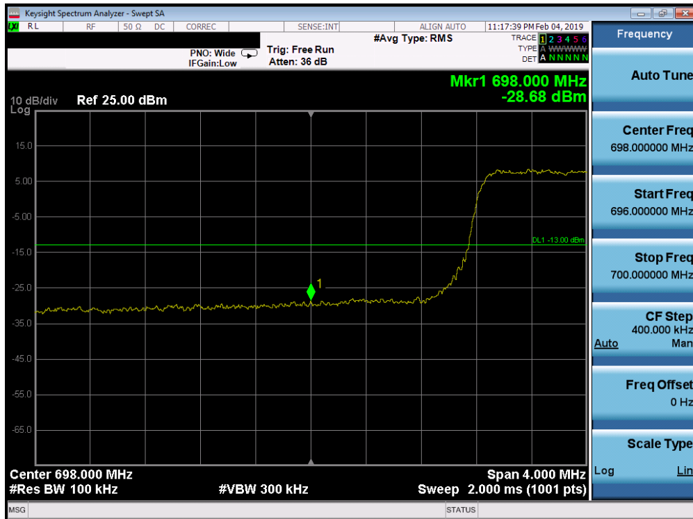
Plot 7-205. Lower Band Edge Plot (Band 12 - 5.0MHz QPSK - Full RB Configuration)
