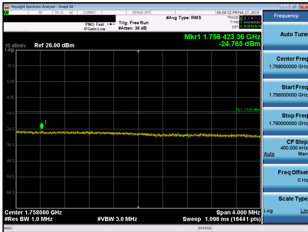
Plot 7-254. Upper Extended Band Edge Plot (Band 4 – 15.0MHz QPSK - Full RB Configuration)
