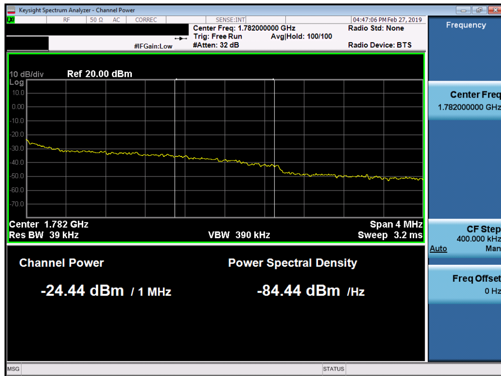
Plot 7-238. Upper Extended Band Edge Plot (Band 66 - 3.0MHz QPSK - Full RB Configuration)
