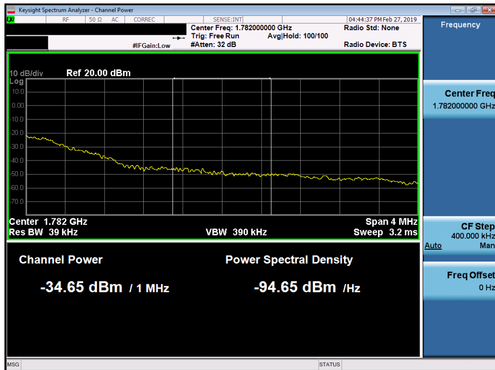
Plot 7-232. Upper Extended Band Edge Plot (Band 66 - 1.4MHz QPSK - Full RB Configuration)
