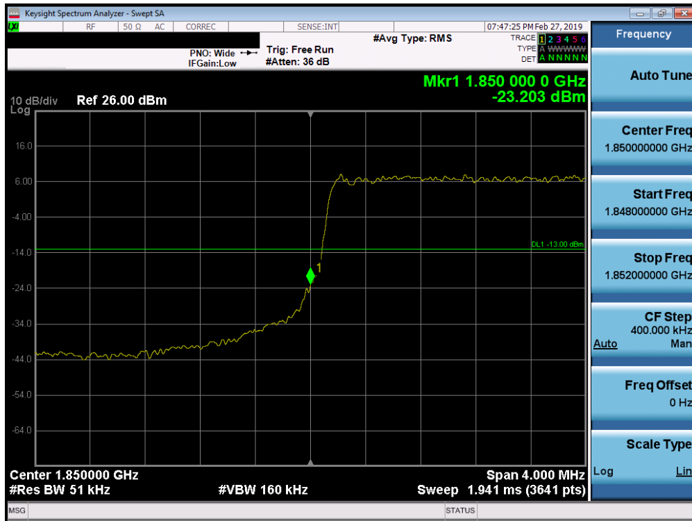
Plot 7-269. Lower Band Edge Plot (Band 25/2 - 3.0MHz QPSK - Full RB Configuration)
