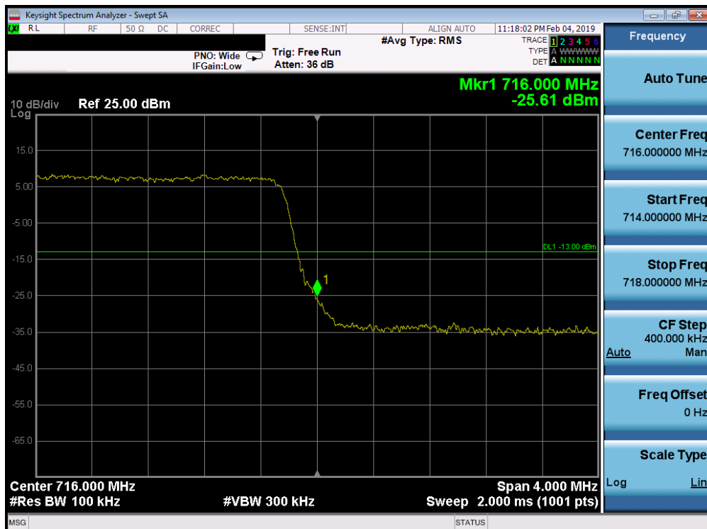
Plot 7-206. Upper Band Edge Plot (Band 12 - 5.0MHz QPSK - Full RB Configuration)
