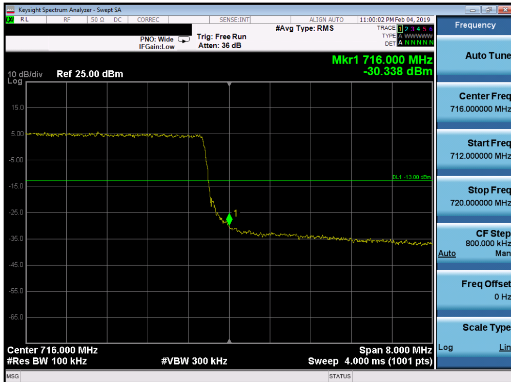
Plot 7-208. Upper Band Edge Plot (Band 12 - 10.0MHz QPSK - Full RB Configuration)
