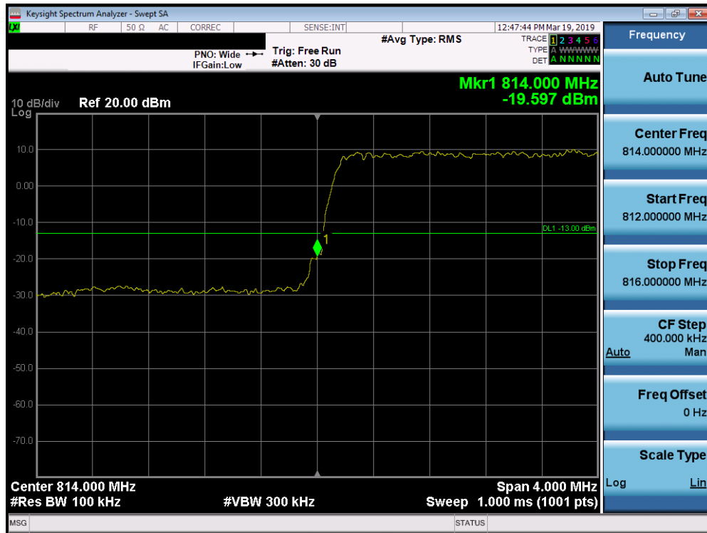
Plot 7-219. Lower Band Edge Plot (Band 26/5 - 3.0MHz QPSK - Full RB Configuration)
