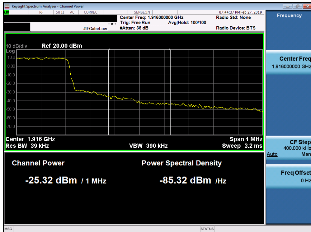
Plot 7-268. Upper Extended Band Edge Plot (Band 25 - 1.4MHz QPSK - Full RB Configuration)
