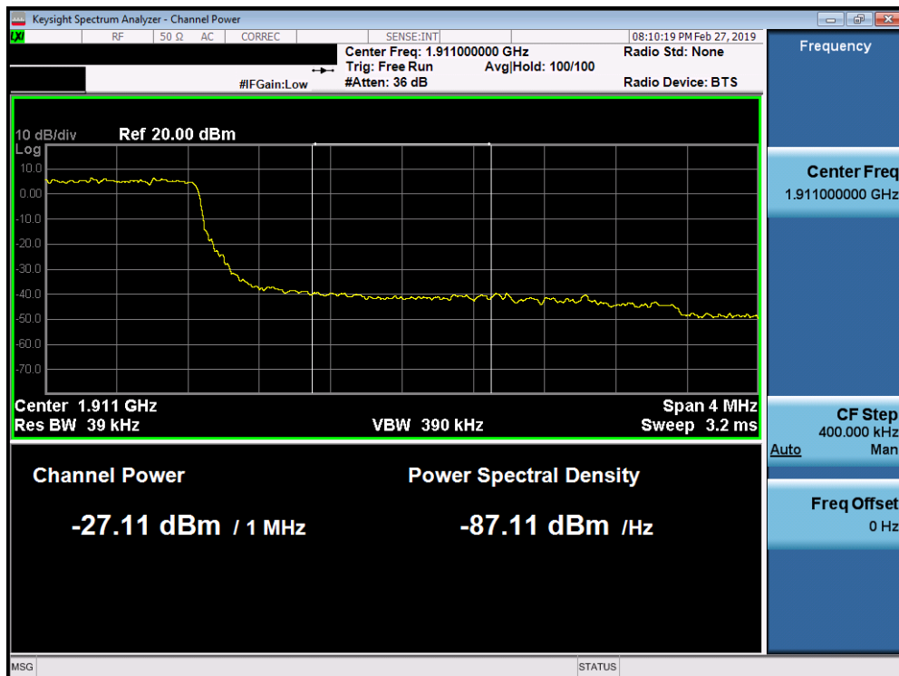
Plot 7-272. Upper Extended Band Edge Plot (Band 2 – 3.0MHz QPSK - Full RB Configuration)
