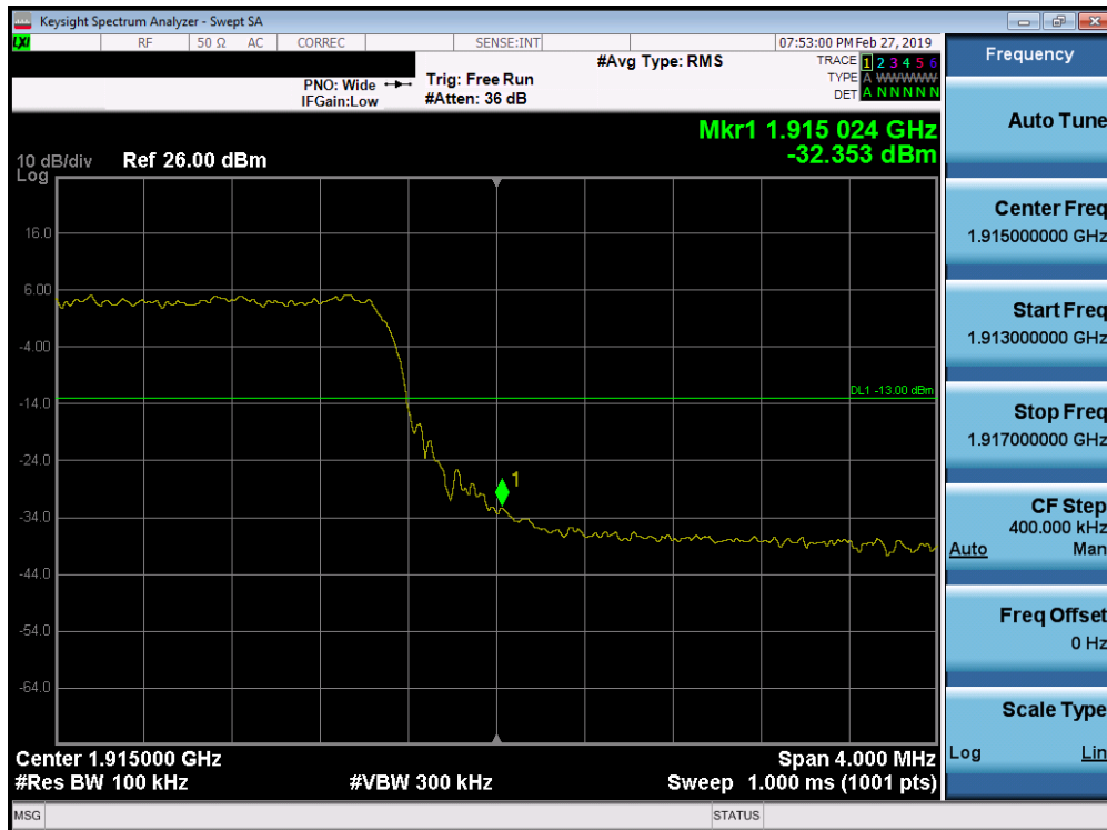
Plot 7-285. Upper Band Edge Plot (Band 25/2 - 10.0MHz QPSK - Full RB Configuration)
