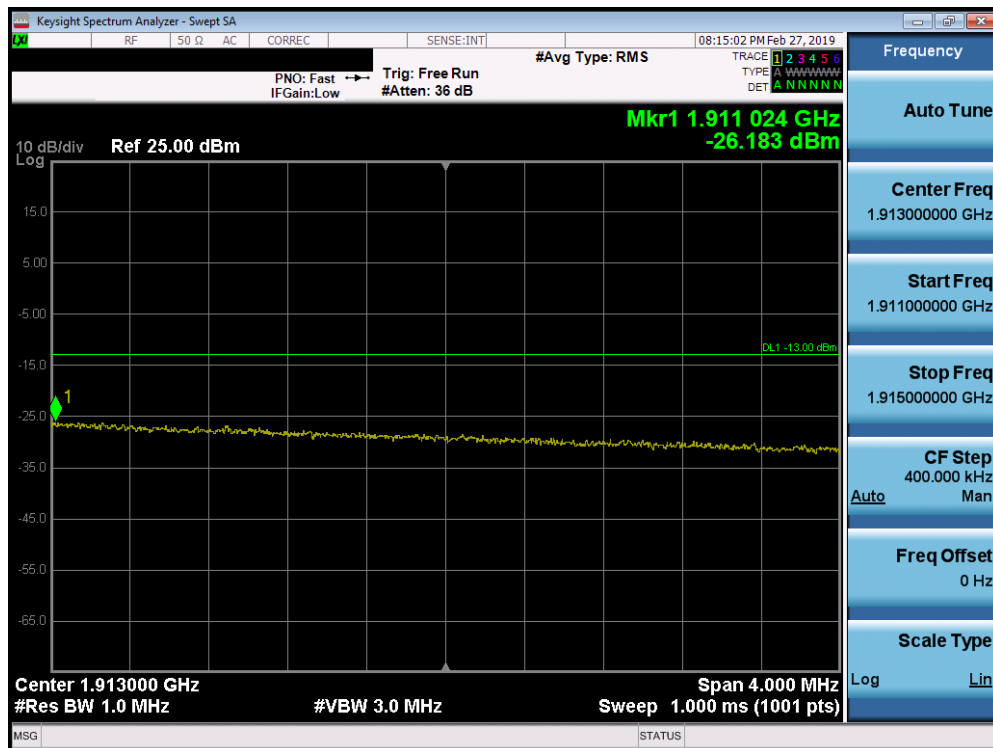
Plot 7-290. Upper Extended Band Edge Plot (Band 2 – 15.0MHz QPSK - Full RB Configuration)
