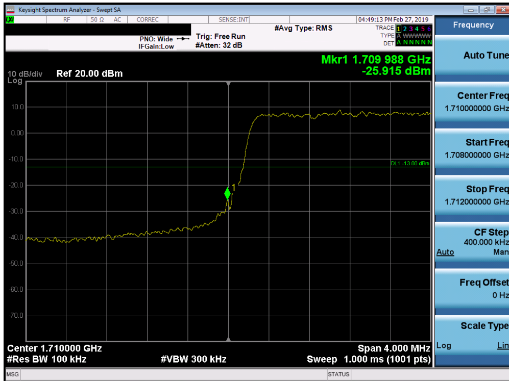
Plot 7-239. Lower Band Edge Plot (Band 66/4 - 5.0MHz QPSK - Full RB Configuration)
