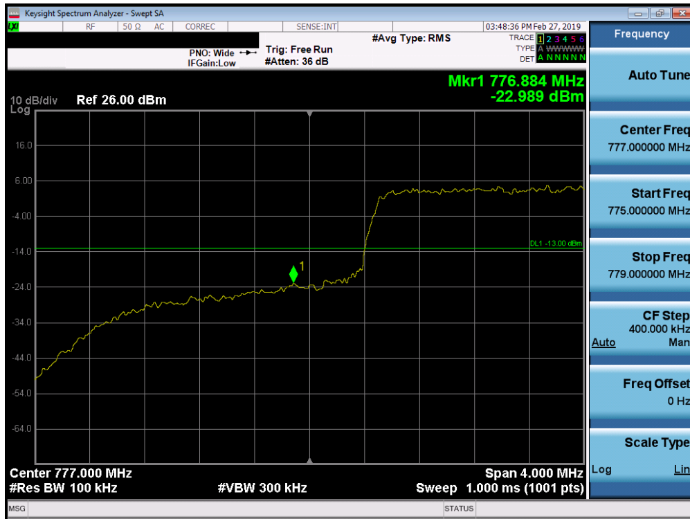
Plot 7-213. Lower Band Edge Plot (Band 13 - 10.0MHz QPSK - Full RB Configuration)
