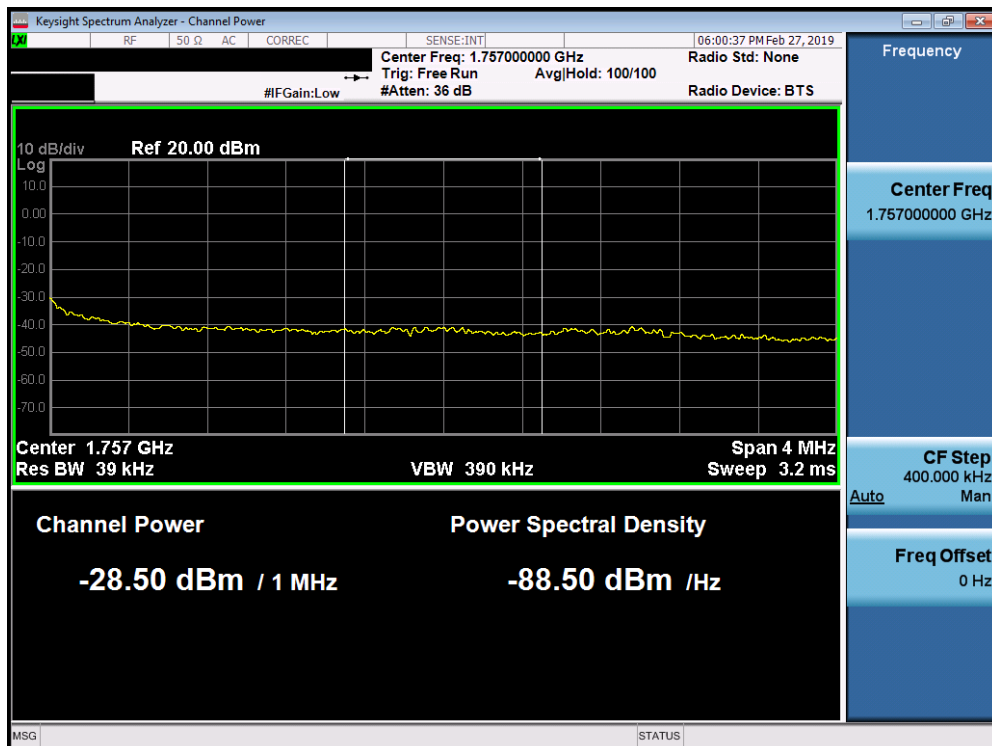
Plot 7-242. Upper Extended Band Edge Plot (Band 4 – 5.0MHz QPSK - Full RB Configuration)
