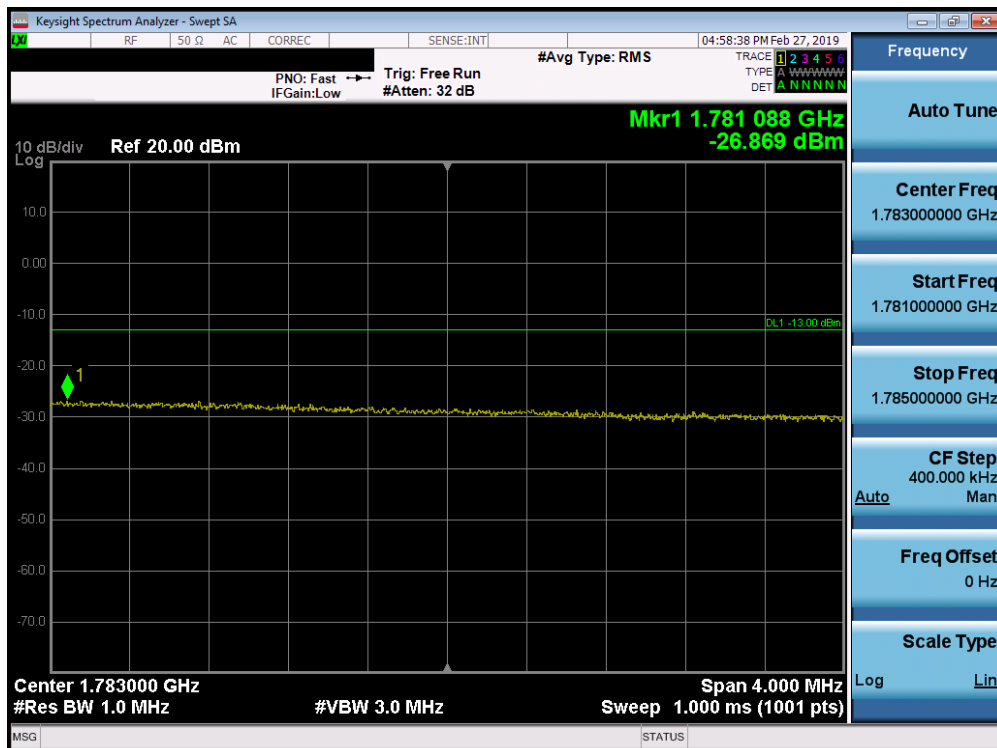
Plot 7-262. Upper Extended Band Edge Plot (Band 66 - 20.0MHz QPSK - Full RB Configuration)
