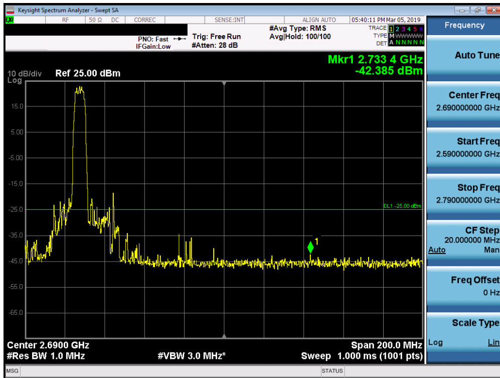
Plot 7-308. Upper ACP Plot (Band 38 - 5.0MHz QPSK - Full RB Configuration)
