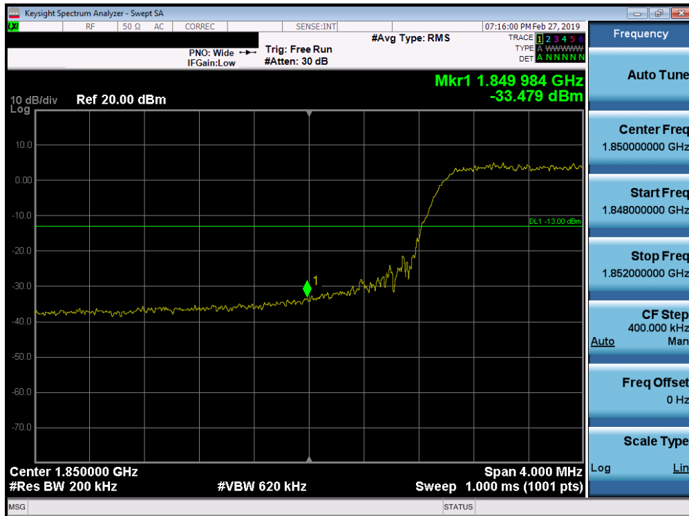
Plot 7-293. Lower Band Edge Plot (Band 25/2 - 20.0MHz QPSK - Full RB Configuration)
