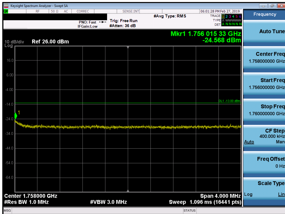
Plot 7-248. Upper Extended Band Edge Plot (Band 4 – 10.0MHz QPSK - Full RB Configuration)
