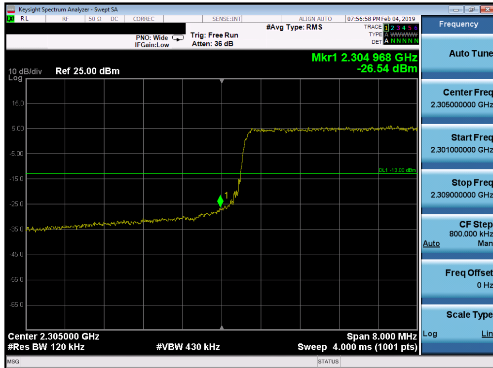
Plot 7-303. Lower Band Edge Plot (Band 30 - 10.0MHz QPSK - Full RB Configuration)
