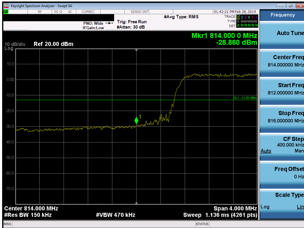
Plot 7-225. Lower Band Edge Plot (Band 26 - 15.0MHz QPSK - Full RB Configuration)
