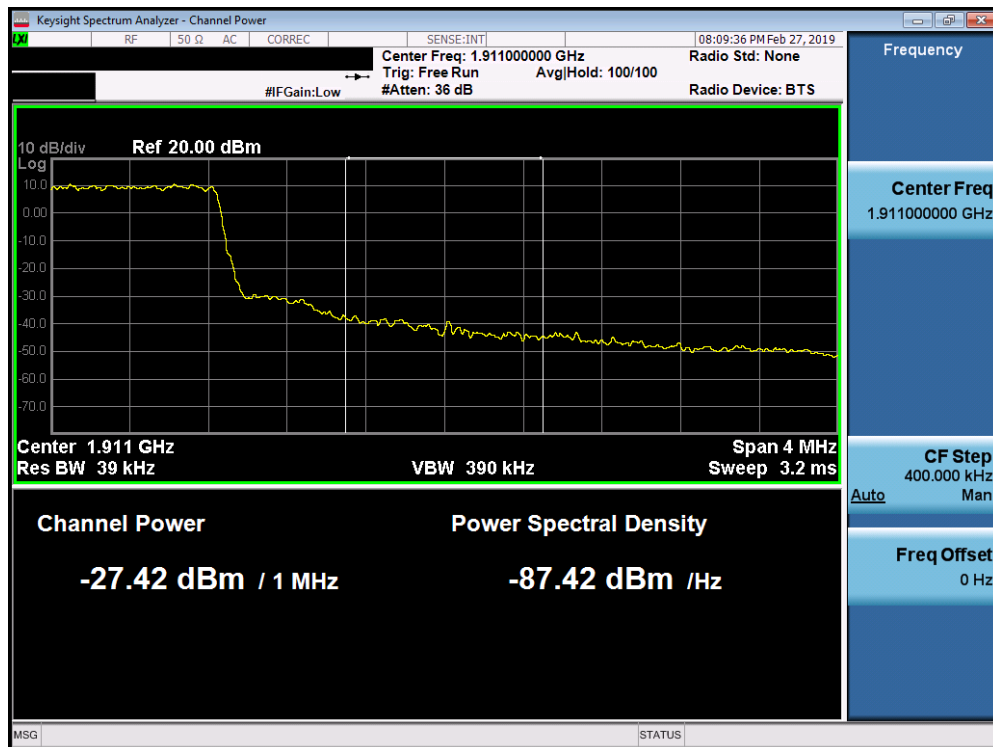
Plot 7-266. Upper Extended Band Edge Plot (Band 2 - 1.4MHz QPSK - Full RB Configuration)
