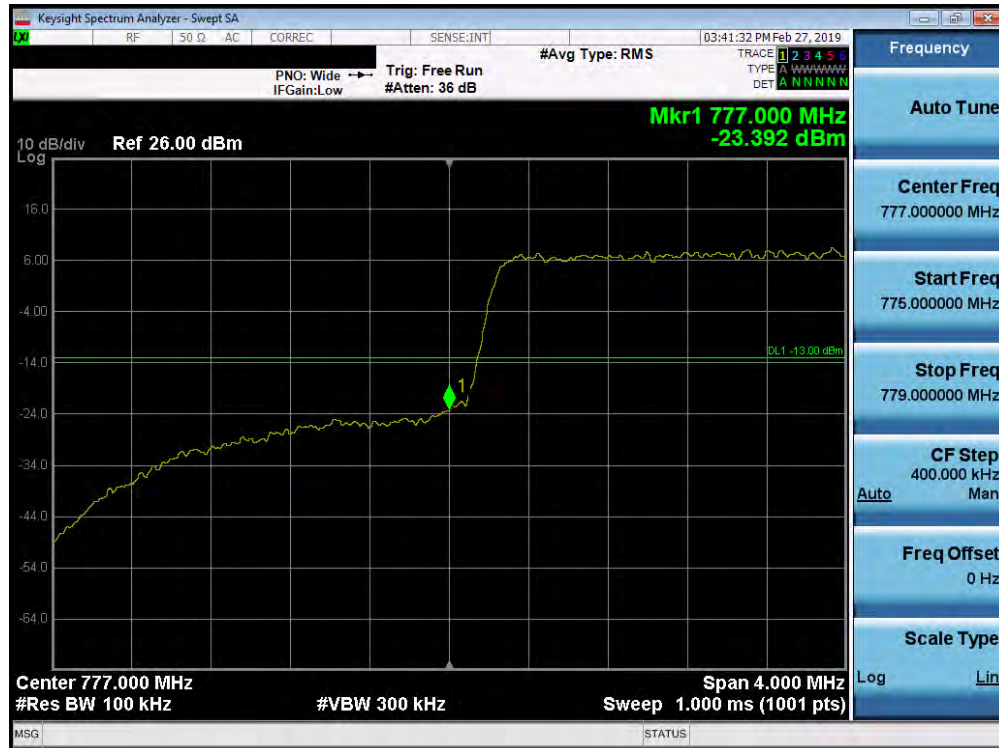
Plot 7-209. Lower Band Edge Plot (Band 13 - 5.0MHz QPSK - Full RB Configuration)
