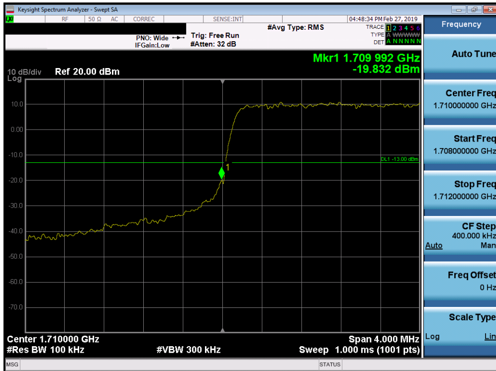
Plot 7-233. Lower Band Edge Plot (Band 66/4 - 3.0MHz QPSK - Full RB Configuration)
