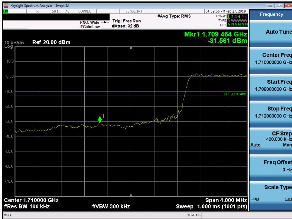
Plot 7-257. Lower Band Edge Plot (Band 66/4 - 20.0MHz QPSK - Full RB Configuration)
