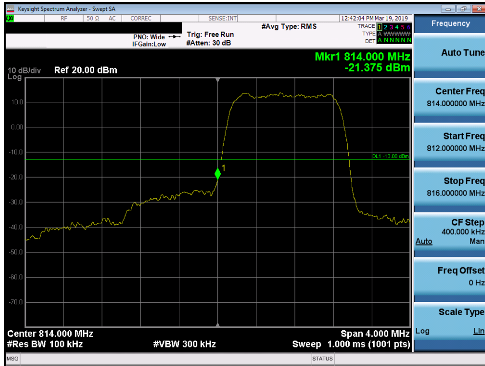
Plot 7-217. Lower Band Edge Plot (Band 26/5 - 1.4MHz QPSK - Full RB Configuration)
