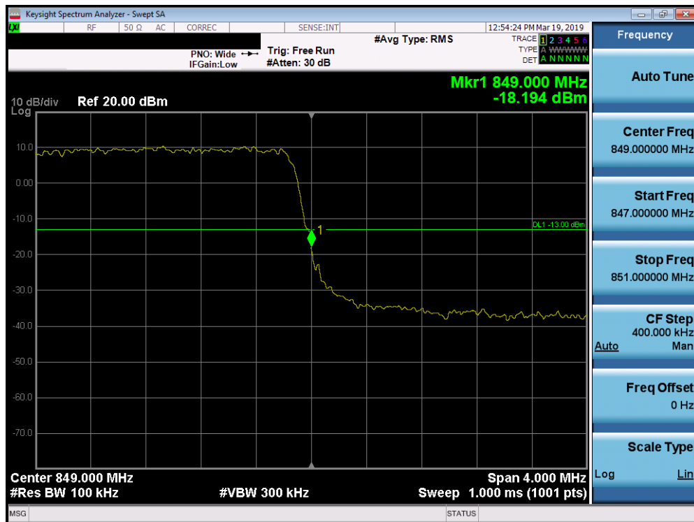
Plot 7-220. Upper Band Edge Plot (Band 26/5 - 3.0MHz QPSK - Full RB Configuration)
