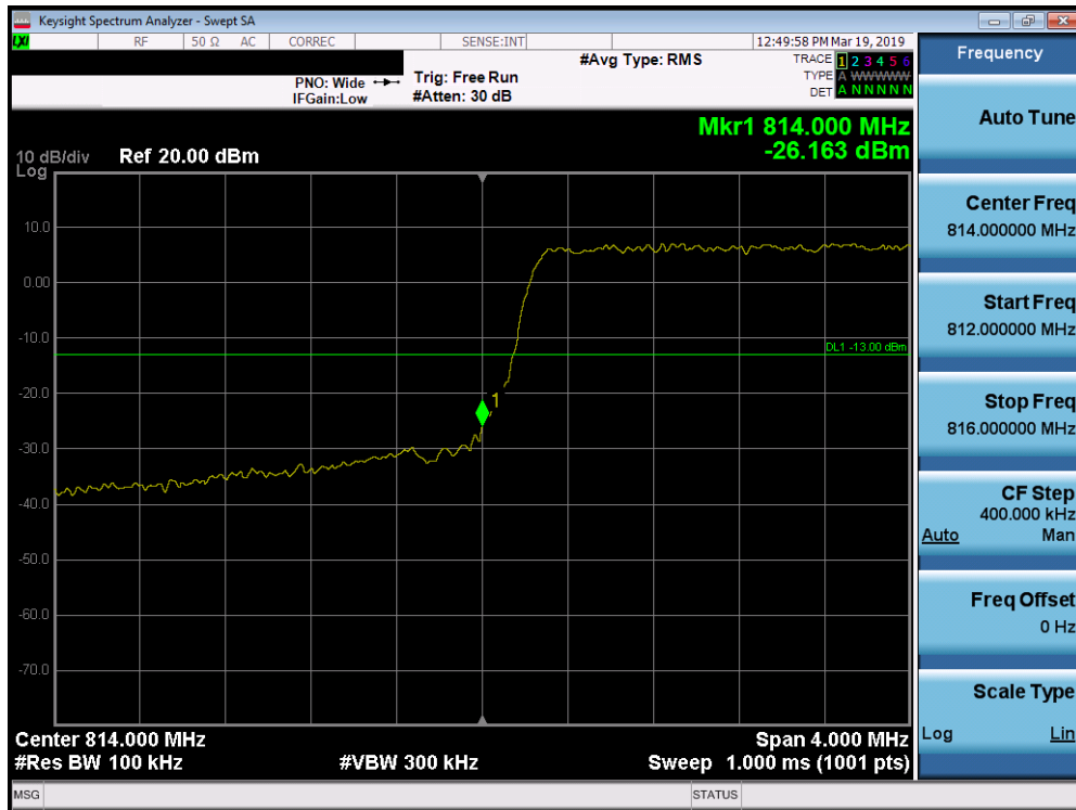
Plot 7-221. Lower Band Edge Plot (Band 26/5 - 5.0MHz QPSK - Full RB Configuration)
