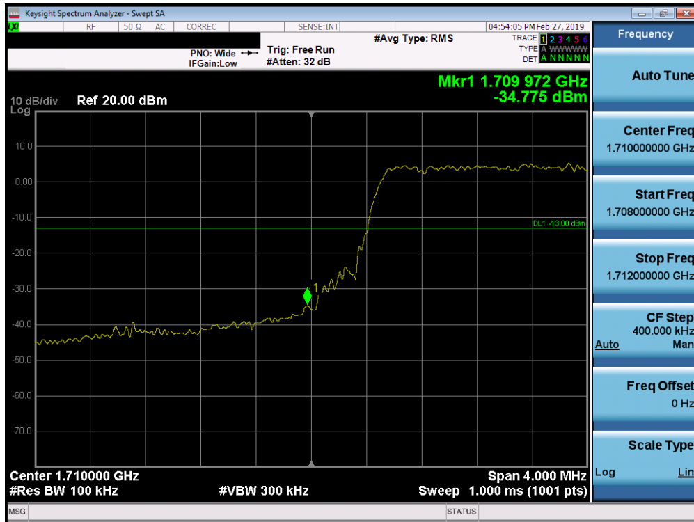
Plot 7-245. Lower Band Edge Plot (Band 66/4 - 10.0MHz QPSK - Full RB Configuration)
