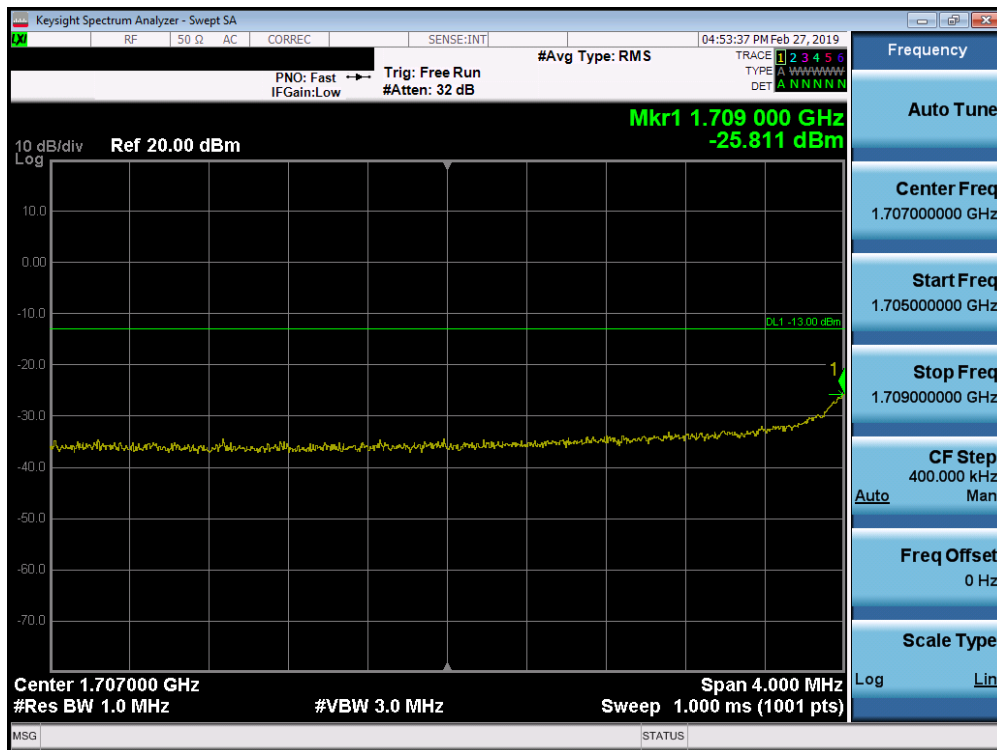
Plot 7-246. Lower Extended Band Edge Plot (Band 66/4 - 10.0MHz QPSK - Full RB Configuration)
