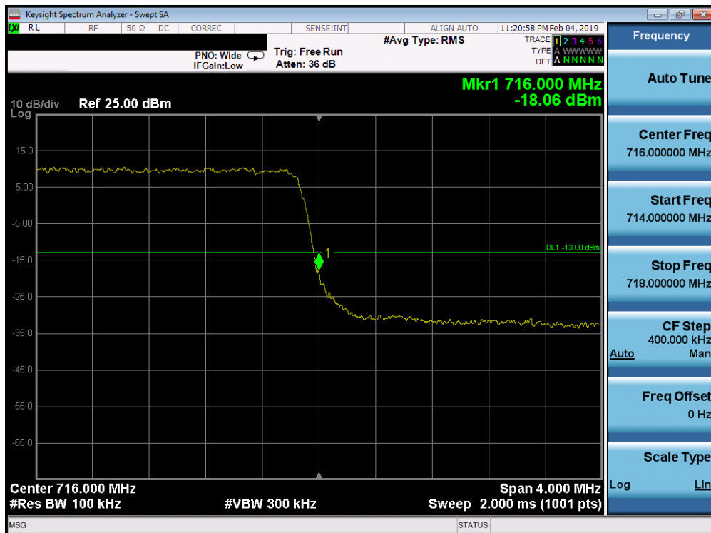
Plot 7-204. Upper Band Edge Plot (Band 12 - 3.0MHz QPSK - Full RB Configuration)
