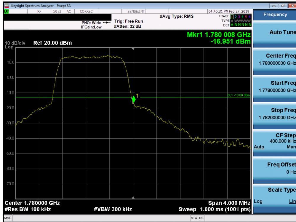
Plot 7-231. Upper Band Edge Plot (Band 66 - 1.4MHz QPSK - Full RB Configuration)
