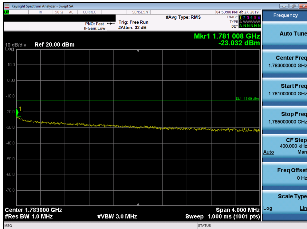
Plot 7-250. Upper Extended Band Edge Plot (Band 66 - 10.0MHz QPSK - Full RB Configuration)
