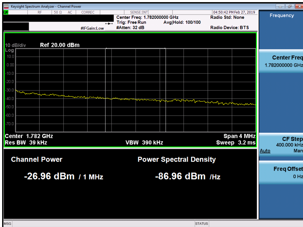
Plot 7-244. Upper Extended Band Edge Plot (Band 66 - 5.0MHz QPSK - Full RB Configuration)
