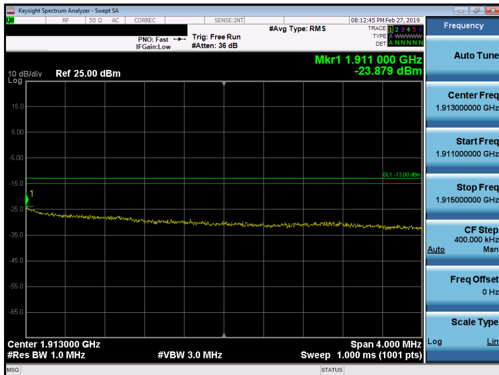
Plot 7-284. Upper Extended Band Edge Plot (Band 2 – 10.0MHz QPSK - Full RB Configuration)
