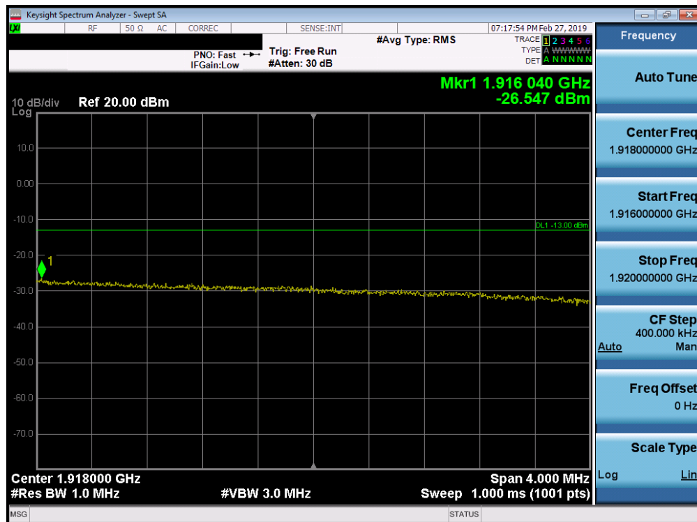
Plot 7-298. Upper Extended Band Edge Plot (Band 25 - 20.0MHz QPSK - Full RB Configuration)
