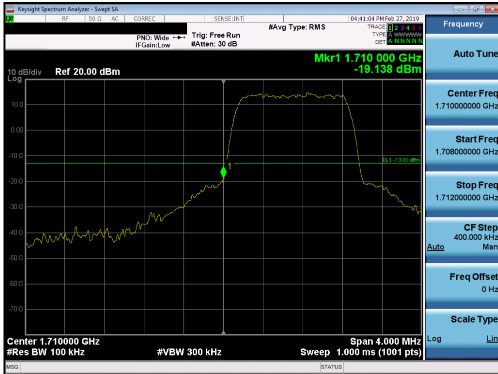
Plot 7-227. Lower Band Edge Plot (Band 66/4 - 1.4MHz QPSK - Full RB Configuration)
