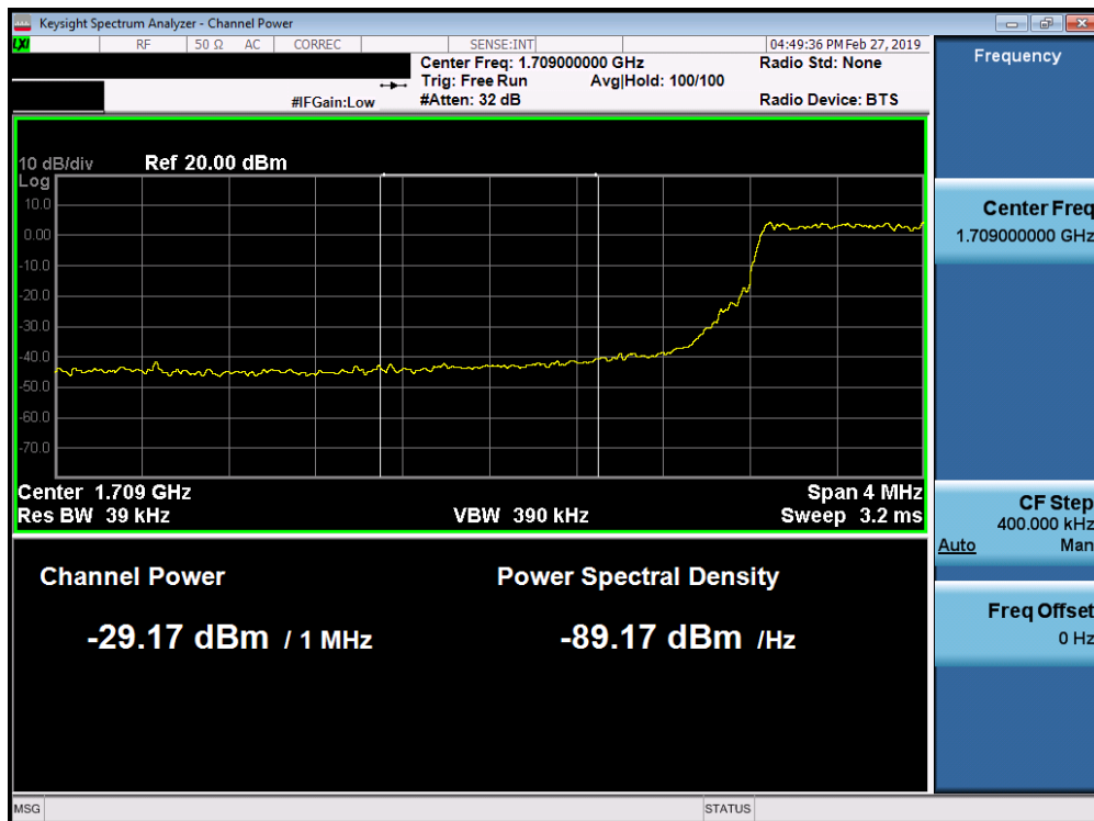
Plot 7-240. Lower Extended Band Edge Plot (Band 66/4 - 5.0MHz QPSK - Full RB Configuration)
