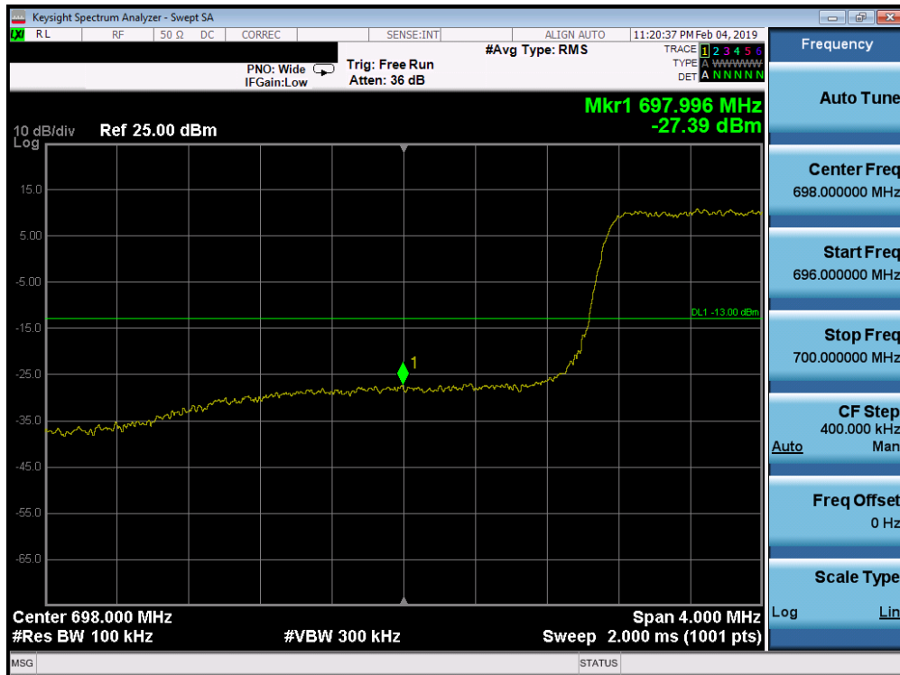
Plot 7-203. Lower Band Edge Plot (Band 12 - 3.0MHz QPSK - Full RB Configuration)
