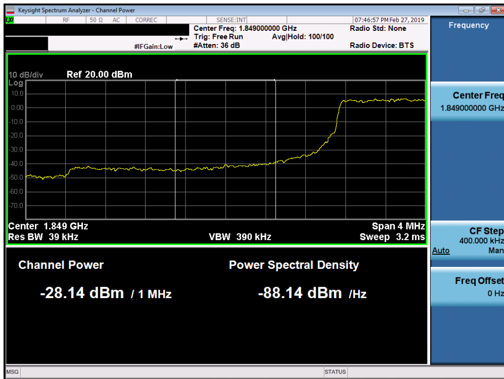
Plot 7-270. Lower Extended Band Edge Plot (Band 25/2 - 3.0MHz QPSK - Full RB Configuration)
