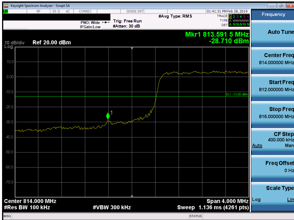
Plot 7-223. Lower Band Edge Plot (Band 26/5 - 10.0MHz QPSK - Full RB Configuration)
