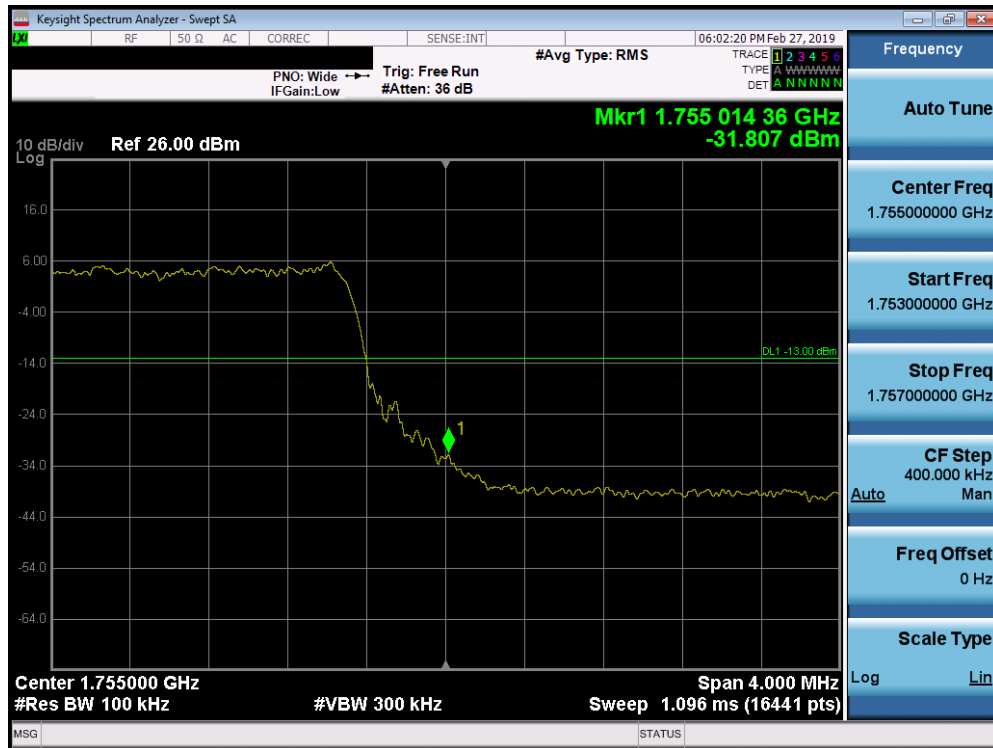
Plot 7-247. Upper Band Edge Plot (Band 4 – 10.0MHz QPSK - Full RB Configuration)
