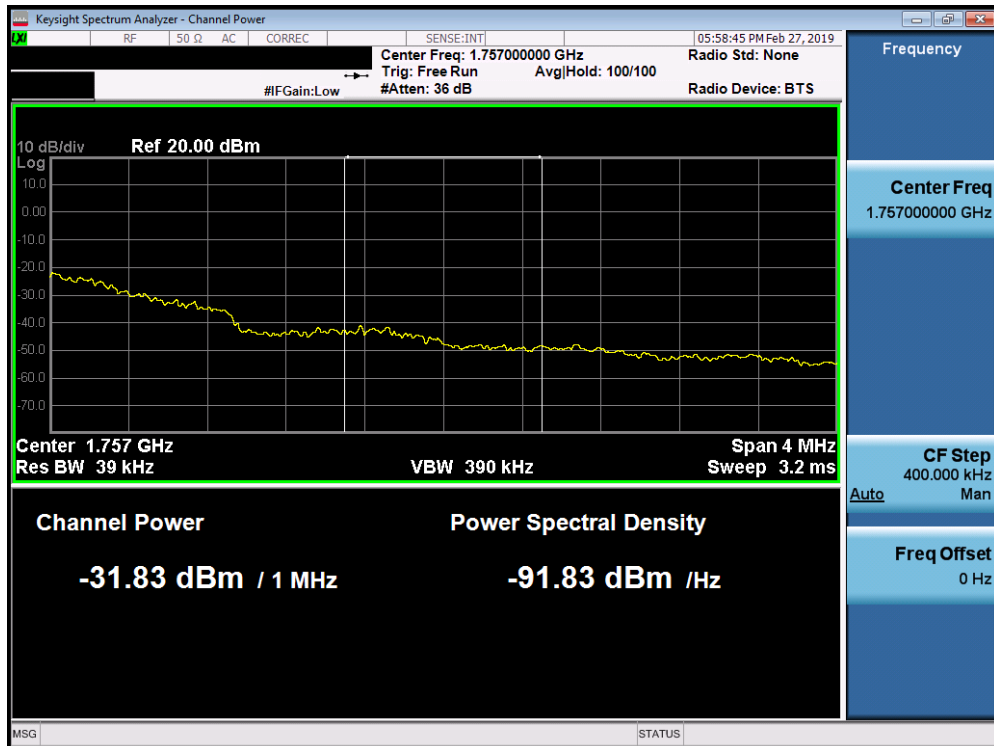
Plot 7-230. Upper Extended Band Edge Plot (Band 4 - 1.4MHz QPSK - Full RB Configuration)
