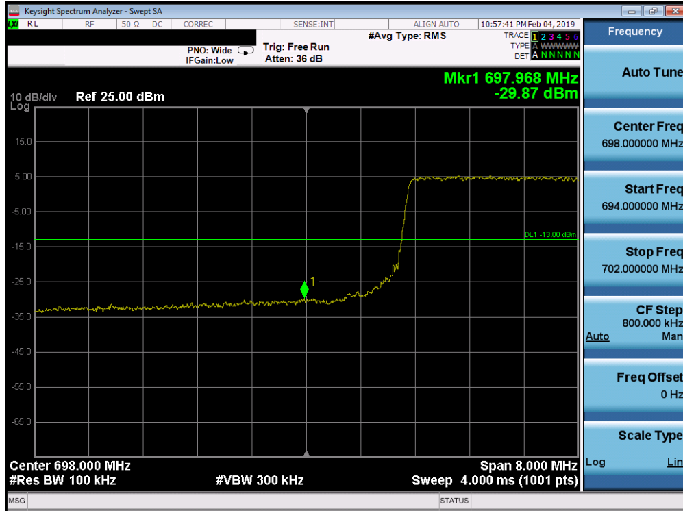
Plot 7-207. Lower Band Edge Plot (Band 12 - 10.0MHz QPSK - Full RB Configuration)
