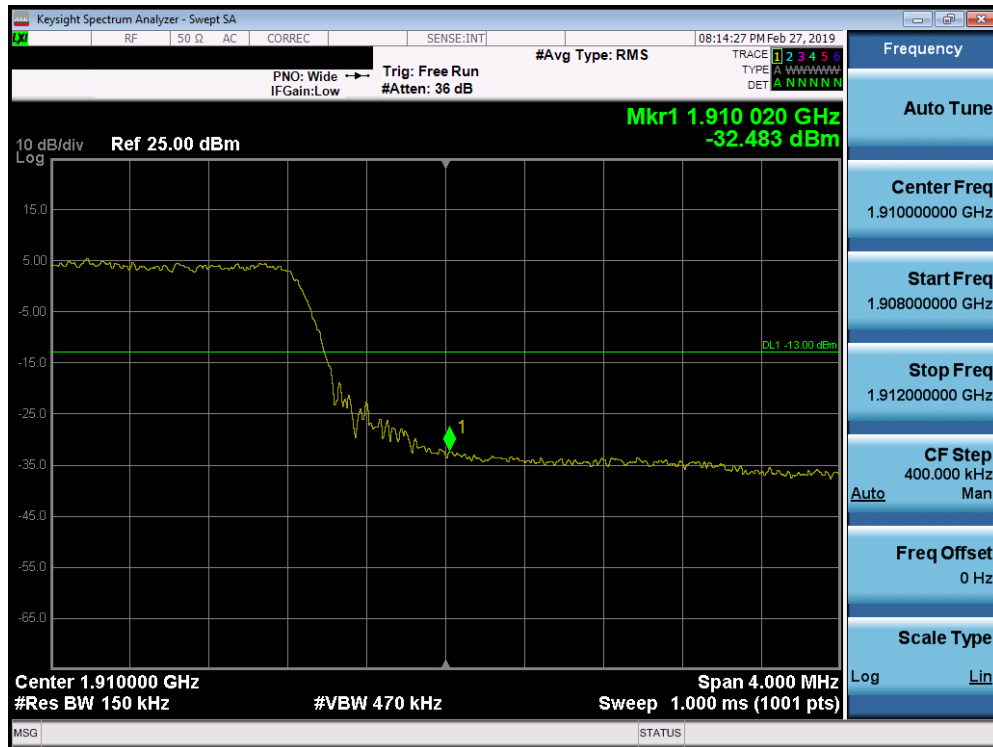
Plot 7-289. Upper Band Edge Plot (Band 2 – 15.0MHz QPSK - Full RB Configuration)
