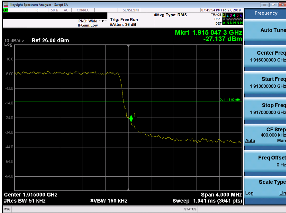
Plot 7-273. Upper Band Edge Plot (Band 25 - 3.0MHz QPSK - Full RB Configuration)
