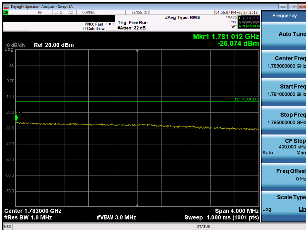
Plot 7-256. Upper Extended Band Edge Plot (Band 66 - 15.0MHz QPSK - Full RB Configuration)
