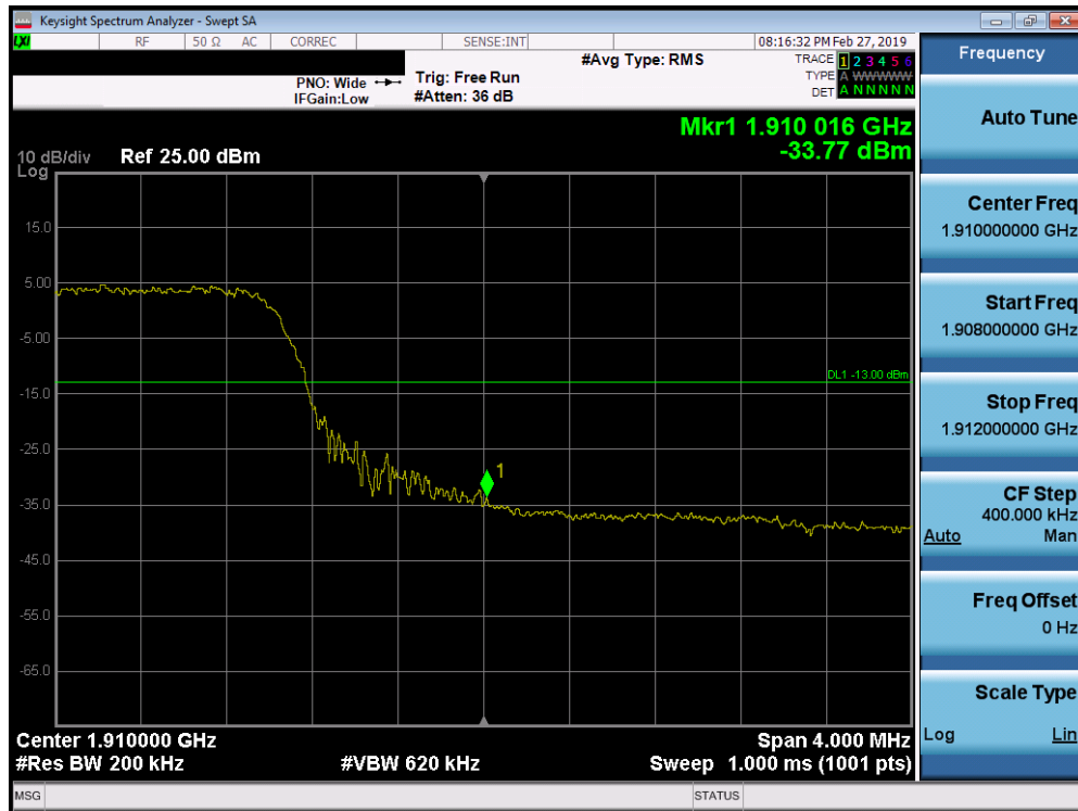
Plot 7-295. Upper Band Edge Plot (Band 2 – 20.0MHz QPSK - Full RB Configuration)
