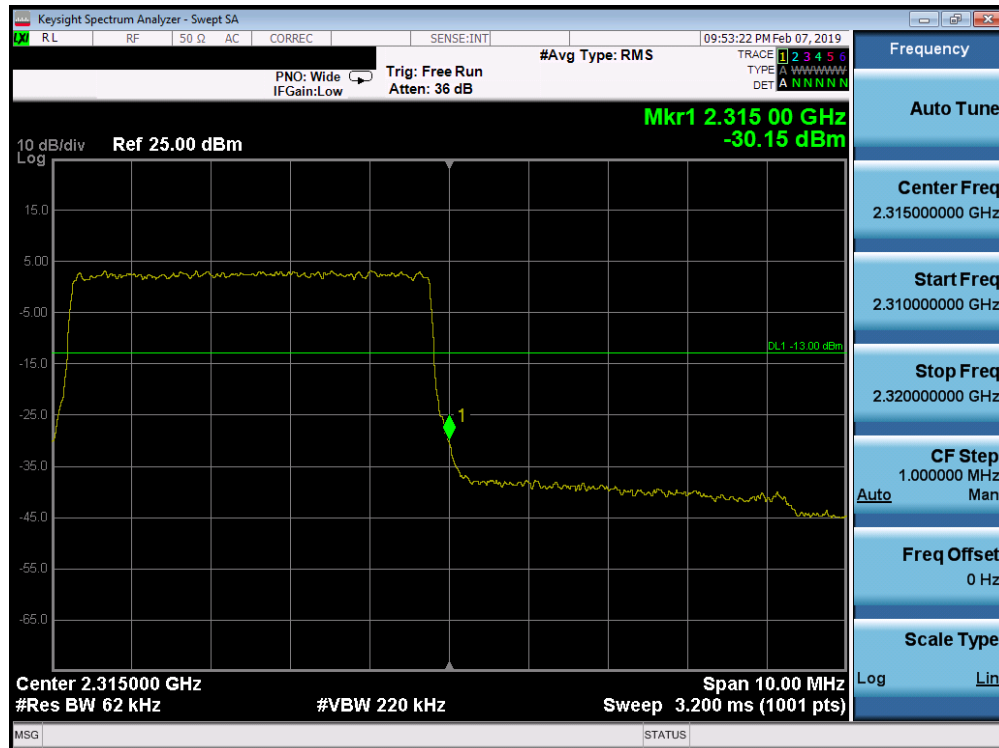
Plot 7-301. Upper Band Edge Plot (Band 30 - 5.0MHz QPSK - Full RB Configuration)
