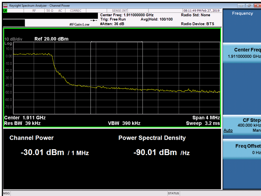
Plot 7-278. Upper Extended Band Edge Plot (Band 2 – 5.0MHz QPSK - Full RB Configuration)
