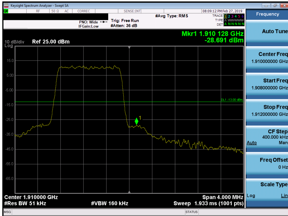
Plot 7-265. Upper Band Edge Plot (Band 2 - 1.4MHz QPSK - Full RB Configuration)
