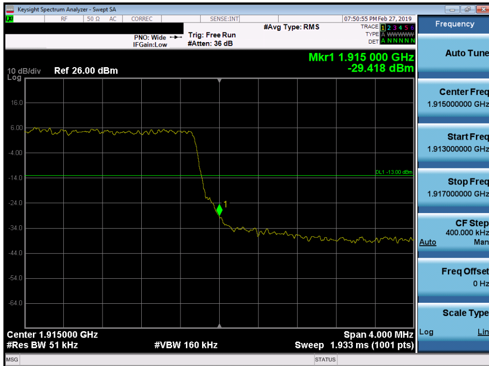
Plot 7-279. Upper Band Edge Plot (Band 25 - 5.0MHz QPSK - Full RB Configuration)
