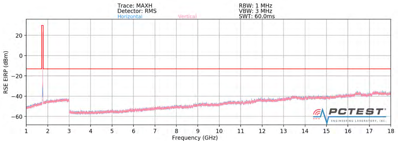
Plot 7-439. Radiated Spurious Plot (ULCA 66B PCC: RB 1 Offset 0, SCC: RB 1 Offset 24 – High Channel - OPEN)
