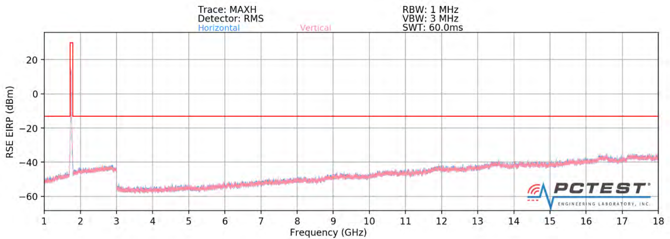
Plot 7-441. Radiated Spurious Plot (ULCA 66B PCC: RB 75 Offset 0, SCC: RB 25 Offset 0 – Mid Channel - OPEN)
