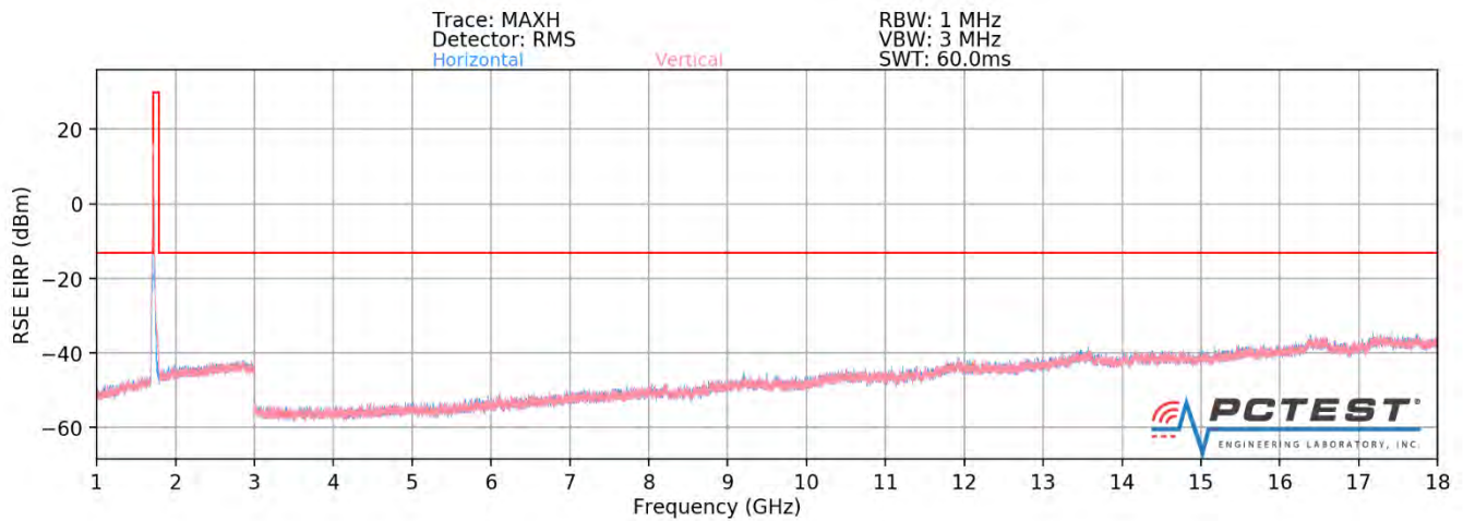
Plot 7-440. Radiated Spurious Plot (ULCA 66B PCC: RB 75 Offset 0, SCC: RB 25 Offset 0 – Low Channel - OPEN)
