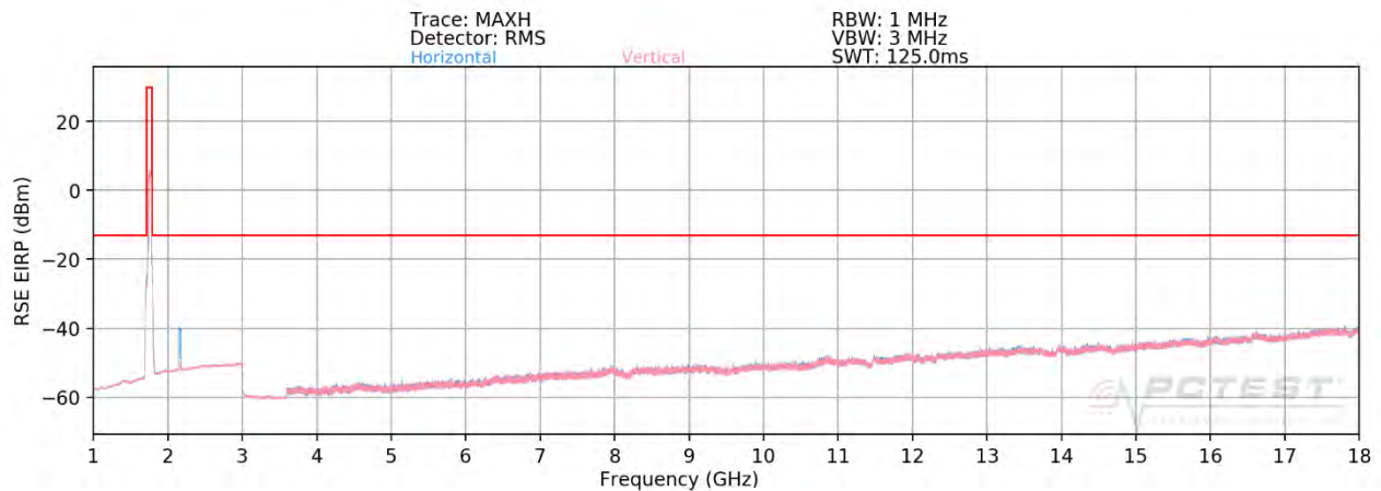
Plot 7-448. Radiated Spurious Plot (ULCA 66C PCC: RB 100 Offset 0, SCC: RB 100 Offset 0 - High Channel - OPEN)
