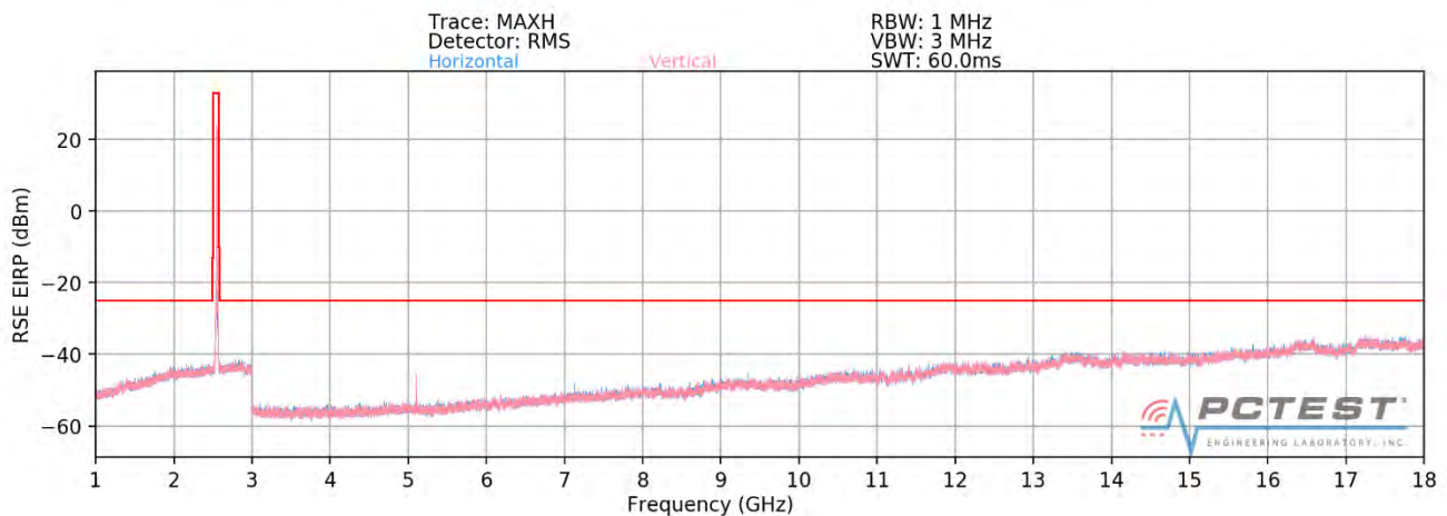
Plot 7-433. Radiated Spurious Plot (ULCA 7C PCC: RB 1 Offset 0, SCC: RB 1 Offset 99 – High Channel - CLOSED)
