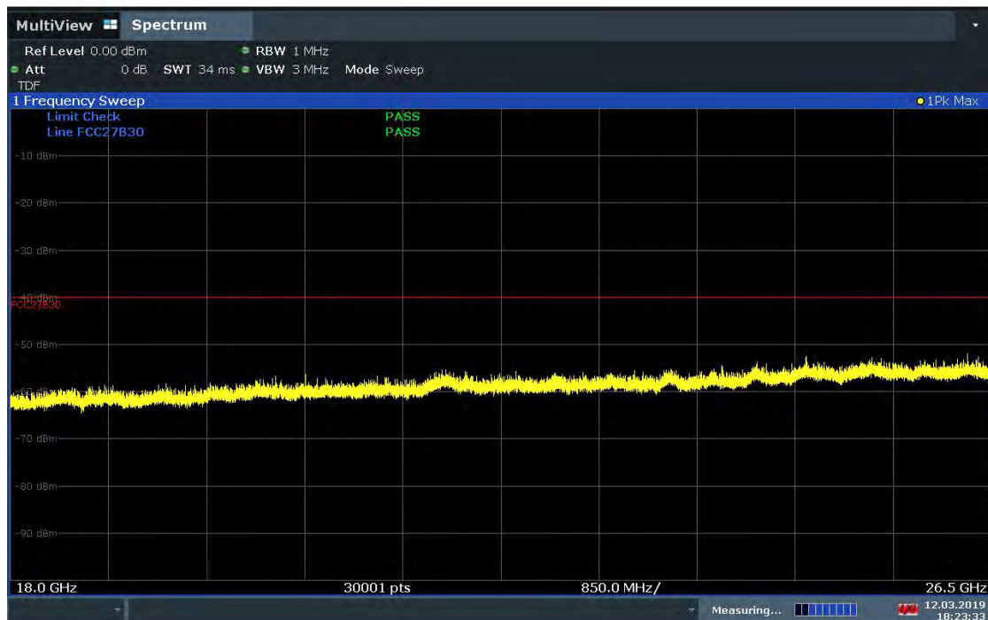
Plot 7-416. Radiated Spurious Plot 18GHz – 26.5GHz (Band 30 – V - CLOSED)
