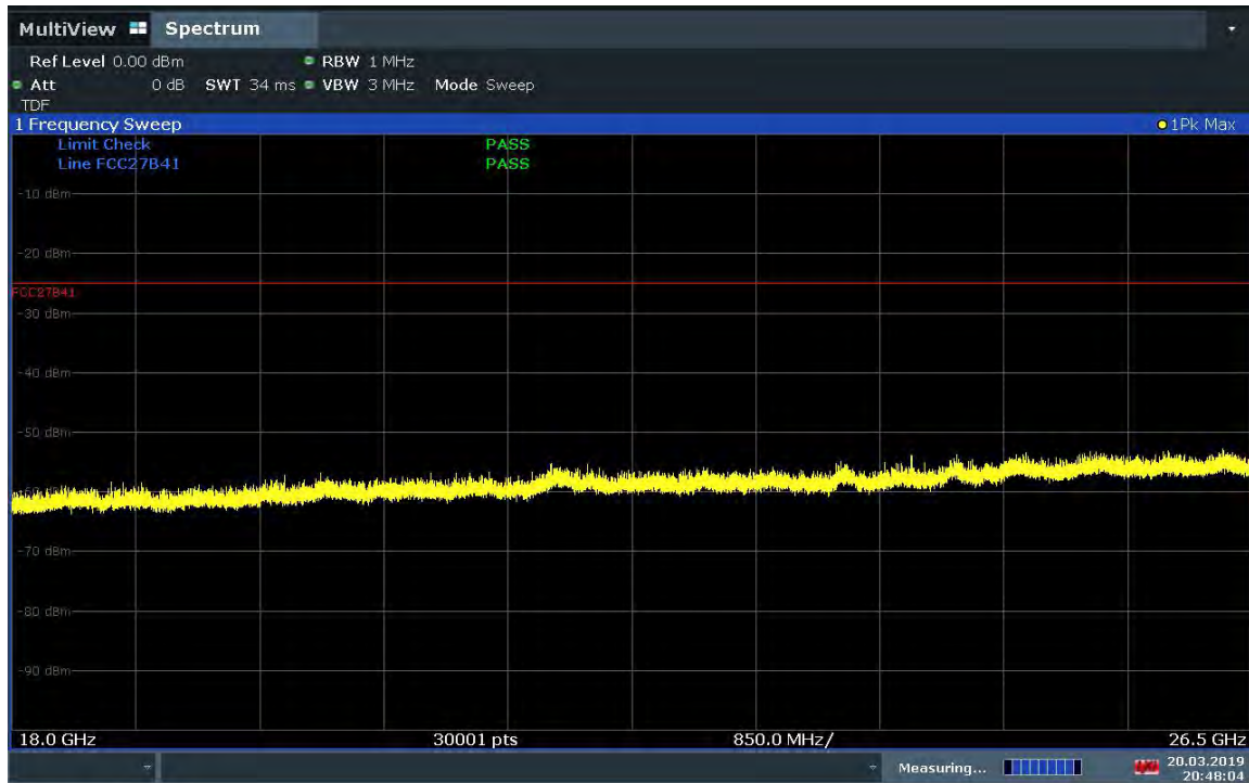
Plot 7-427. Radiated Spurious Plot 18GHz – 26.5GHz (Band 41 PC3 – H - CLOSED)
