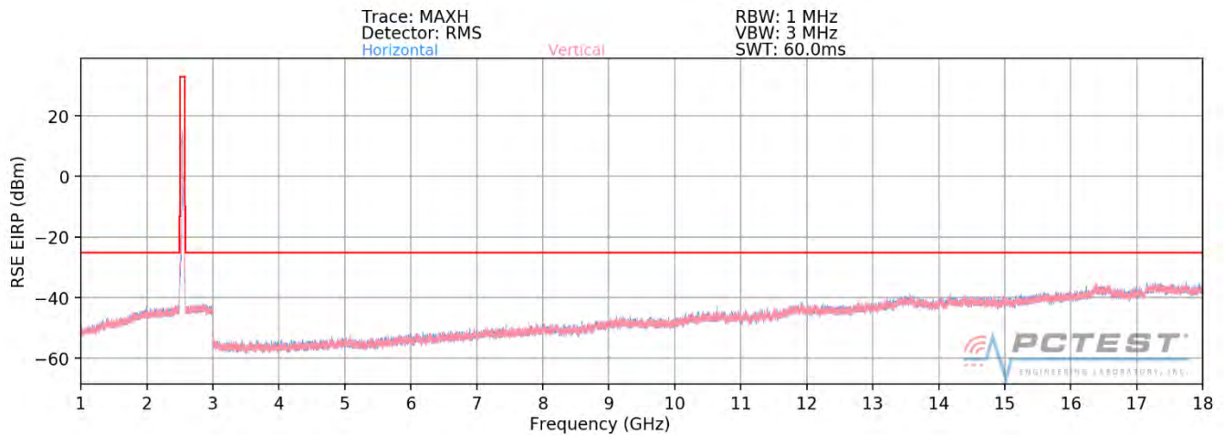
Plot 7-435. Radiated Spurious Plot (ULCA 7C PCC: RB 100 Offset 0, SCC: RB 100 Offset 0 – Mid Channel - CLOSED)
