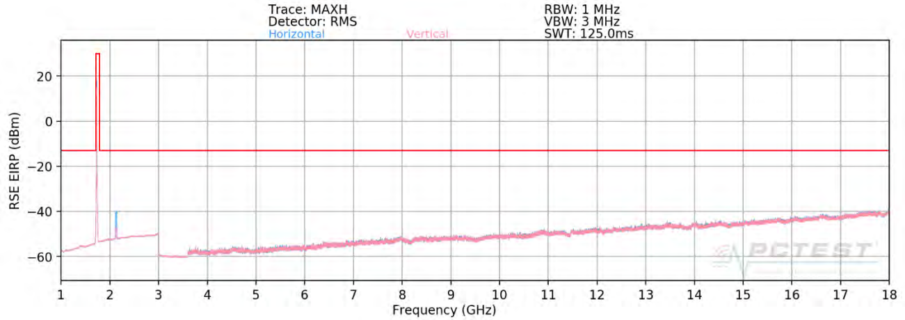
Plot 7-443. Radiated Spurious Plot (ULCA 66C PCC: RB 1 Offset 99, SCC: RB 1 Offset 0 – Low Channel - OPEN)
