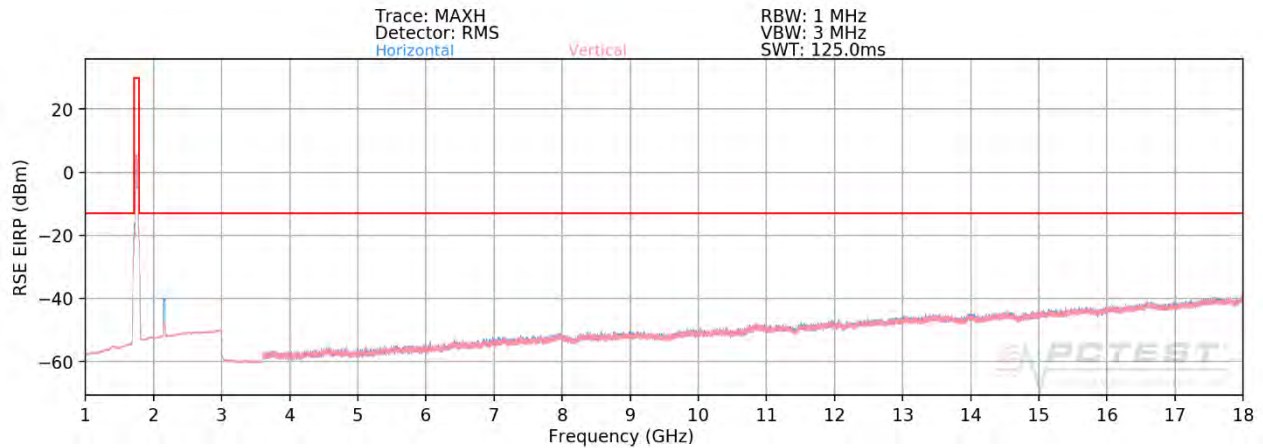
Plot 7-447. Radiated Spurious Plot (ULCA 66C PCC: RB 100 Offset 0, SCC: RB 100 Offset 0 - Mid Channel - OPEN)
