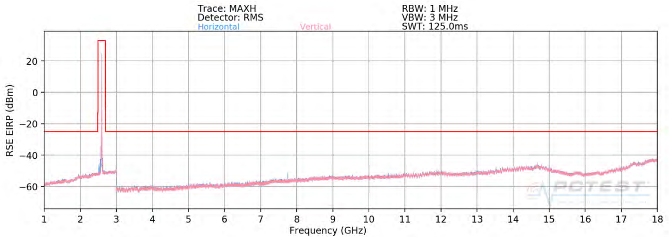
Plot 7-426. Radiated Spurious Plot 1GHz - 18GHz (Band 41 PC3 - OPEN)
