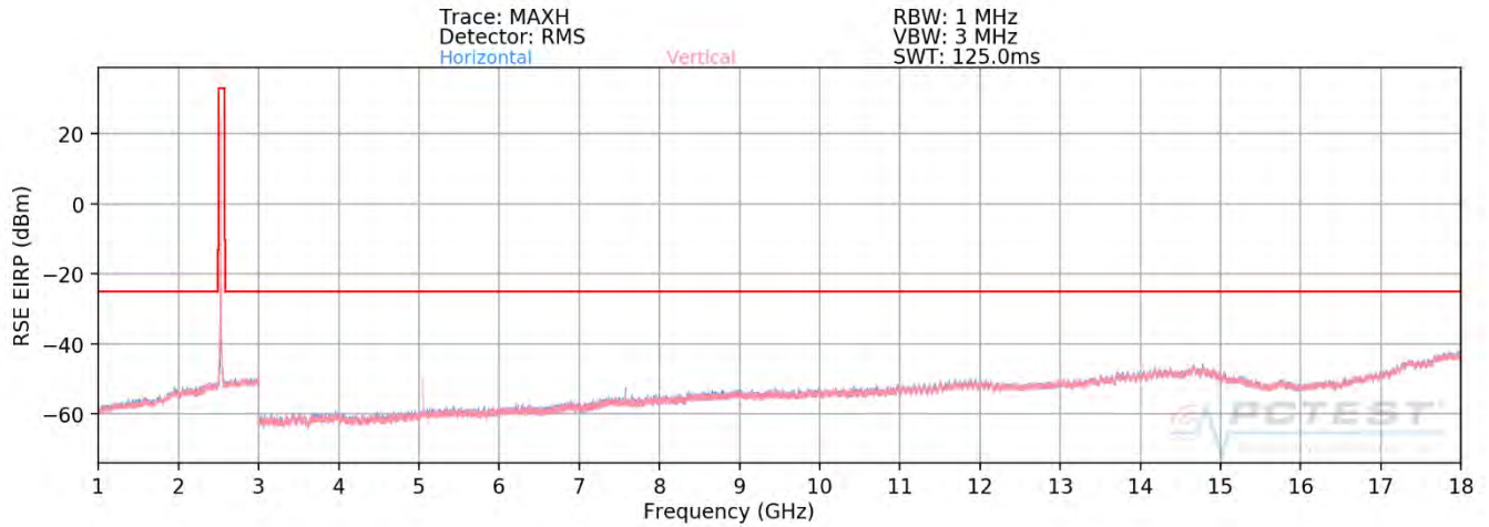
Plot 7-419. Radiated Spurious Plot 1GHz - 18GHz (Band 7 - CLOSED)
