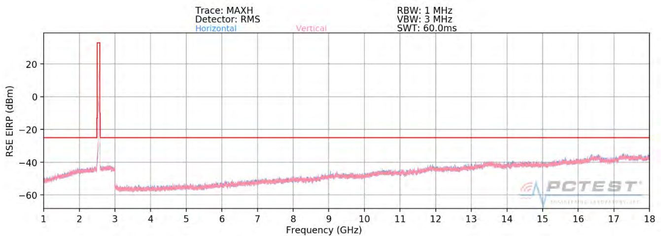
Plot 7-436. Radiated Spurious Plot (ULCA 7C PCC: RB 100 Offset 0, SCC: RB 100 Offset 0 – High Channel - CLOSED)
