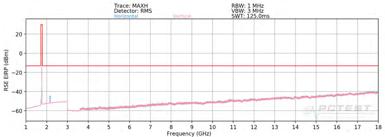
Plot 7-445. Radiated Spurious Plot (ULCA 66C PCC: RB 1 Offset 0, SCC: RB 1 Offset 99 – High Channel - OPEN)
