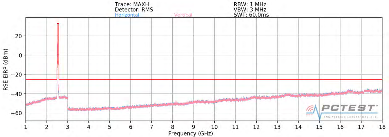
Plot 7-434. Radiated Spurious Plot (ULCA 7C PCC: RB 100 Offset 0, SCC: RB 100 Offset 0 – Low Channel - CLOSED)
