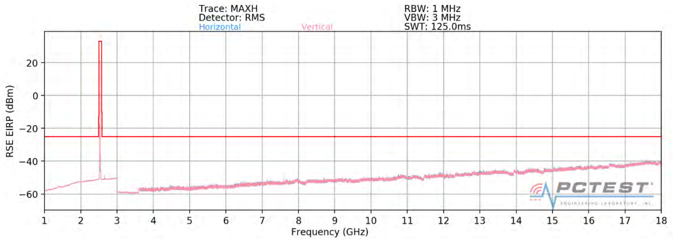
Plot 7-425. Radiated Spurious Plot 1GHz - 18GHz (Band 41 PC3 - CLOSED)
