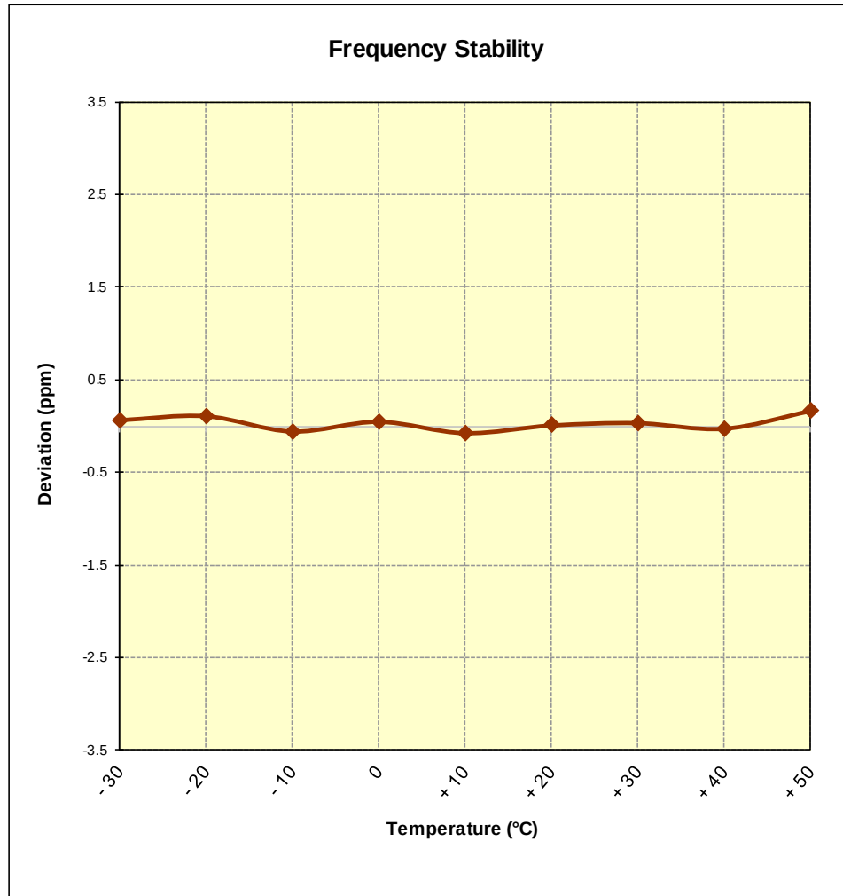
Figure 7-18. Frequency Stability Graph (Band 41/38)
