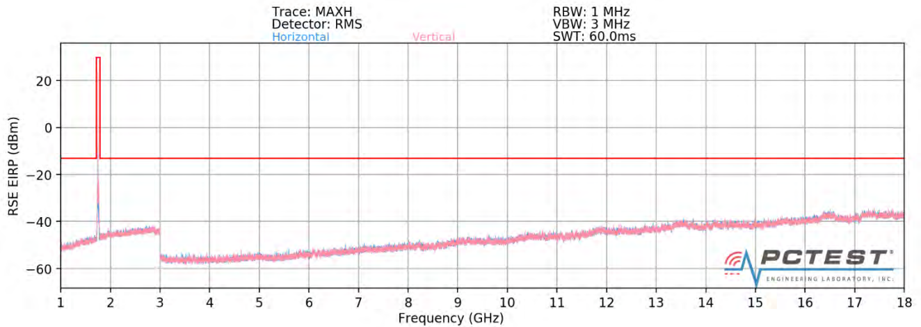
Plot 7-438. Radiated Spurious Plot (ULCA 66B PCC: RB 1 Offset 74, SCC: RB 1 Offset 0 – Mid Channel - OPEN)
