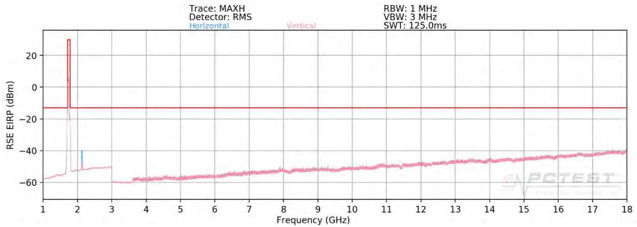
Plot 7-446. Radiated Spurious Plot (ULCA 66C PCC: RB 100 Offset 0, SCC: RB 100 Offset 0 - Low Channel - OPEN)
