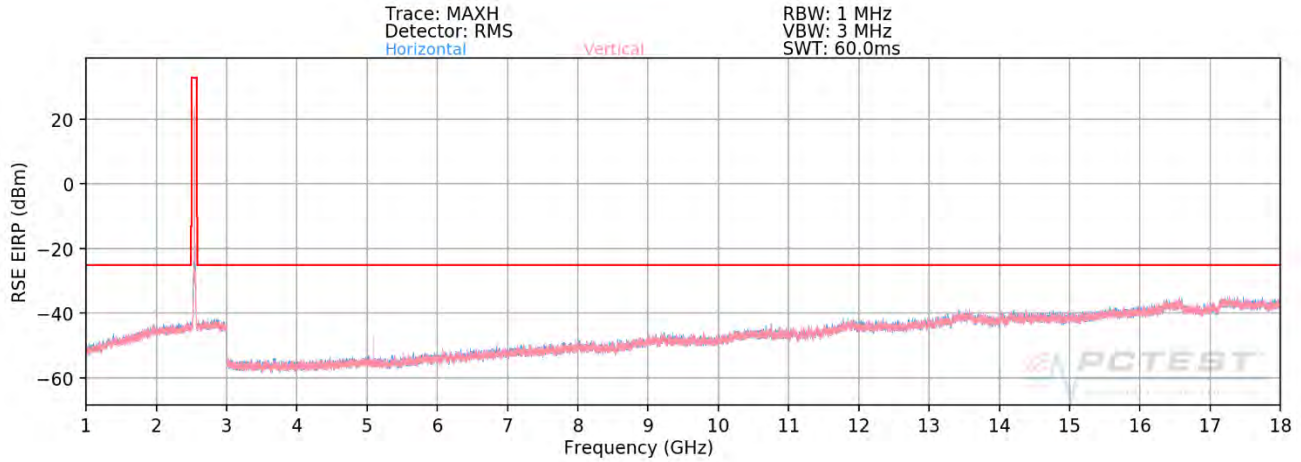
Plot 7-431. Radiated Spurious Plot (ULCA 7C PCC: RB 1 Offset 99, SCC: RB 1 Offset 0 – Low Channel - CLOSED)
