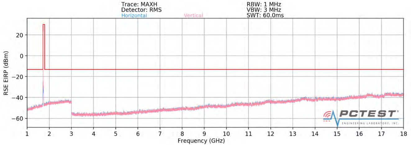
Plot 7-437. Radiated Spurious Plot (ULCA 66B PCC: RB 1 Offset 74, SCC: RB 1 Offset 0 – Low Channel – OPEN)
