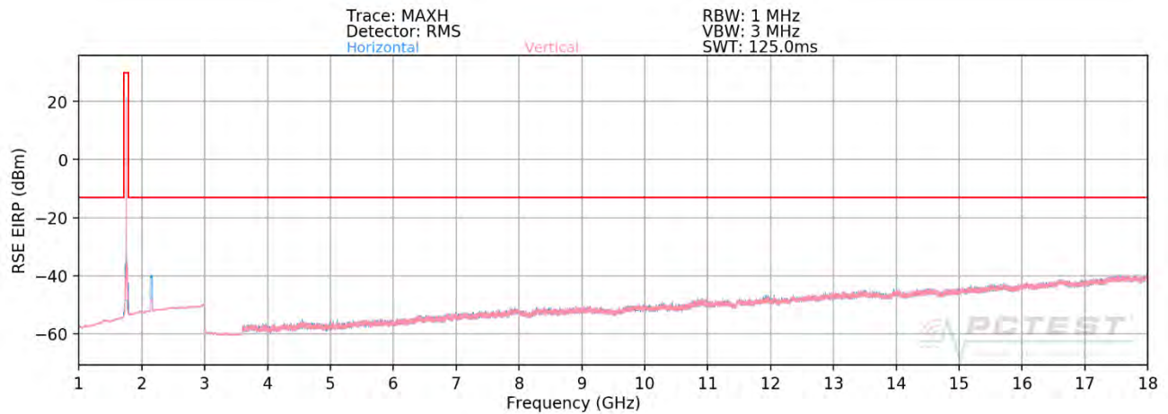
Plot 7-444. Radiated Spurious Plot (ULCA 66C PCC: RB 1 Offset 99, SCC: RB 1 Offset 0 – Mid Channel - OPEN)
