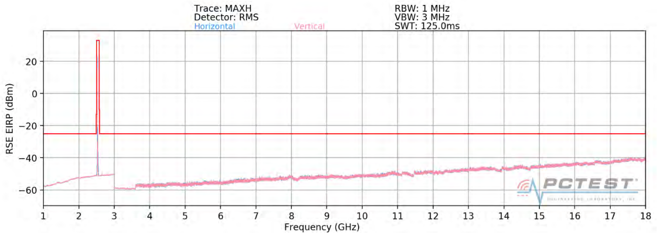
Plot 7-420. Radiated Spurious Plot 1GHz - 18GHz (Band 7 - OPEN)
