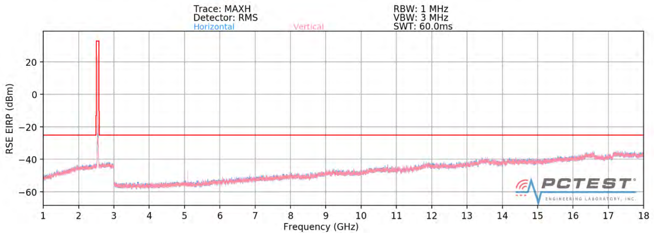
Plot 7-432. Radiated Spurious Plot (ULCA 7C PCC: RB 1 Offset 99, SCC: RB 1 Offset 0 – Mid Channel - CLOSED)
