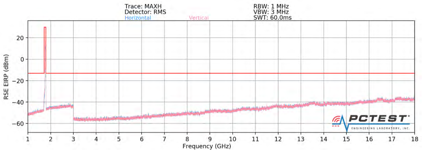
Plot 7-442. Radiated Spurious Plot (ULCA 66B PCC: RB 75 Offset 0, SCC: RB 25 Offset 0 – High Channel - OPEN)
