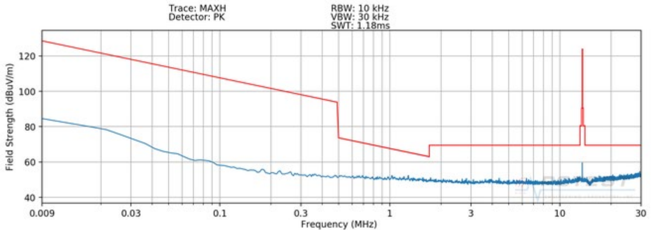
Plot 7-4. Radiated Spurious Plot 9kHz – 30MHz (Pol. Y - OPEN)
