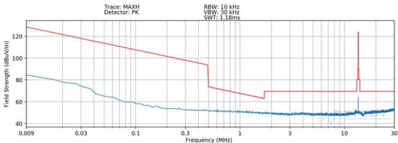
Plot 7-2. Radiated Spurious Plot 9kHz – 30MHz (Pol. X - OPEN)
