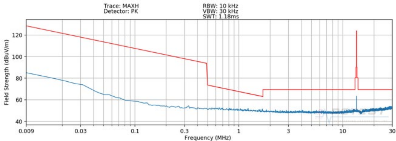
Plot 7-1. Radiated Spurious Plot 9kHz – 30MHz (Pol. X - CLOSED)
