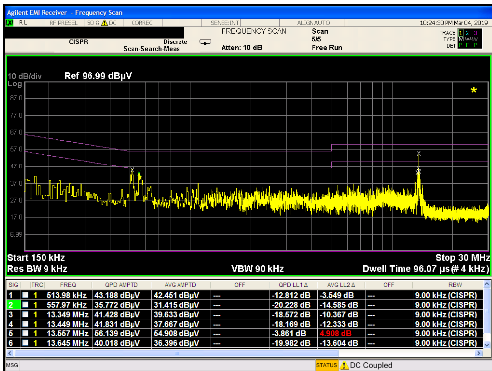
Plot 7-10. Line-Conducted Test Plot (N)
