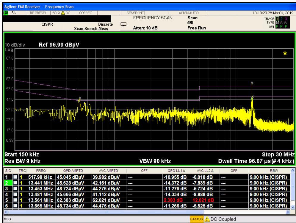
Plot 7-9. Line-Conducted Test Plot (L1)
