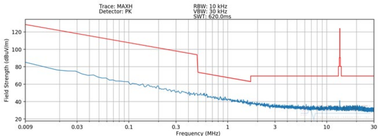
Plot 7-3. Radiated Spurious Plot 9kHz – 30MHz (Pol. Y - CLOSED)
