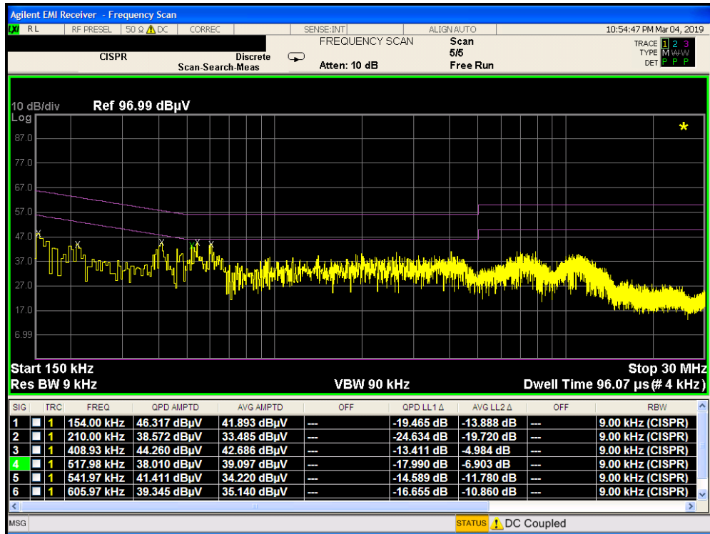
Plot 7-11. Line-Conducted Test Plot Terminated at 50 Ohms(L1)
