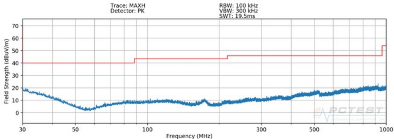
Plot 7-7. Radiated Spurious Plot 30MHz – 1GHz (Pol. H)
