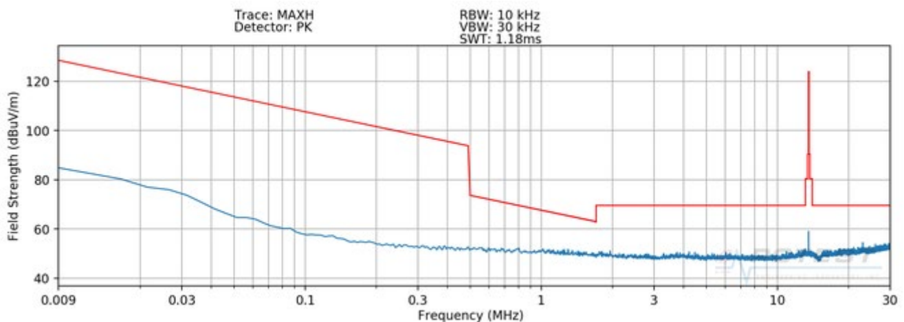
Plot 7-6. Radiated Spurious Plot 9kHz – 30MHz (Pol. Z - OPEN)
