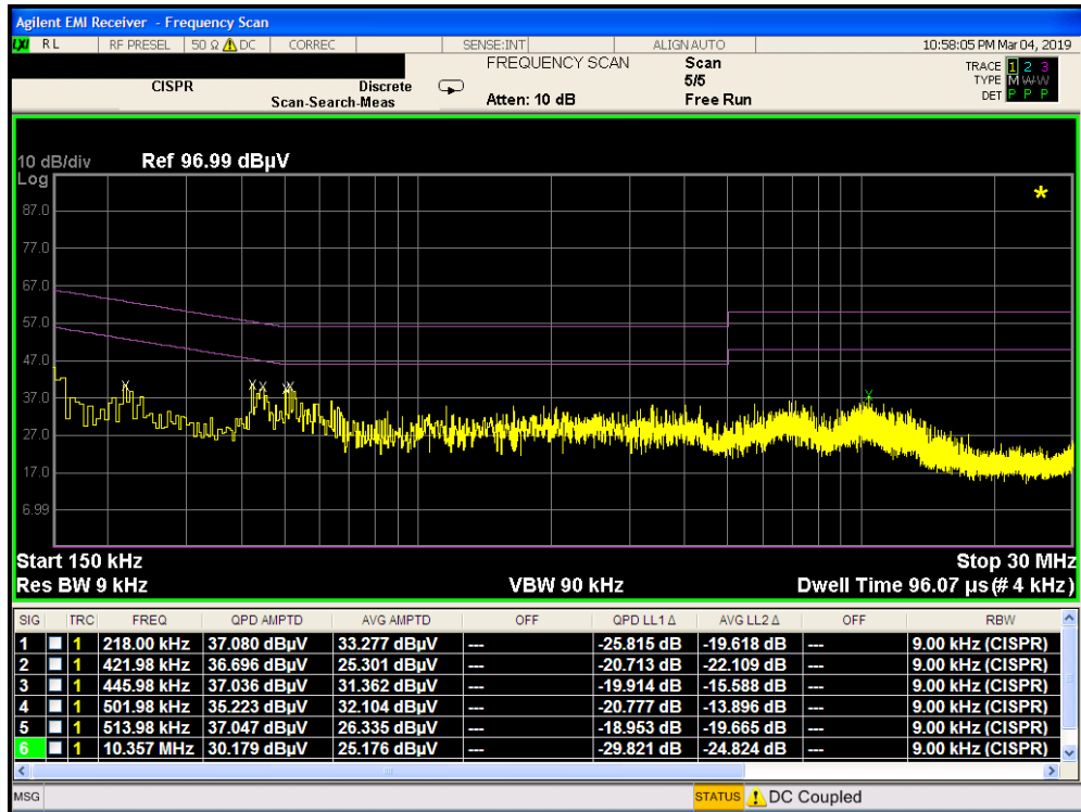
Plot 7-12. Line-Conducted Test Plot Terminated at 50 Ohms (N)
