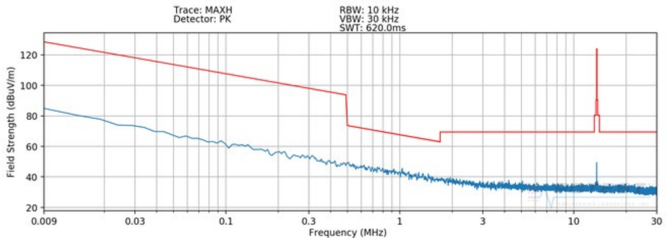
Plot 7-5. Radiated Spurious Plot 9kHz – 30MHz (Pol. Z - CLOSED)
