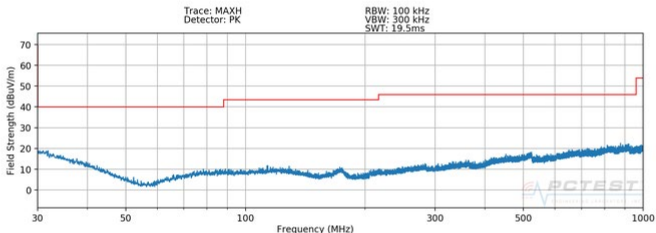
Plot 7-8. Radiated Spurious Plot 30MHz – 1GHz (Pol. V)
