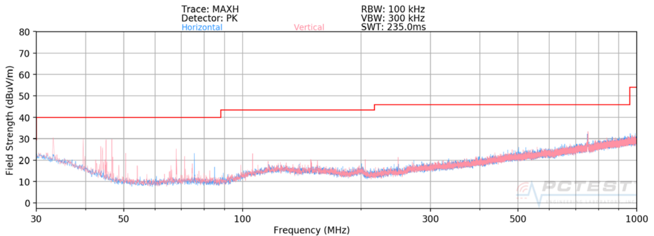
Plot 7-1. Radiated Spurious Plot below 1GHz - OPEN
