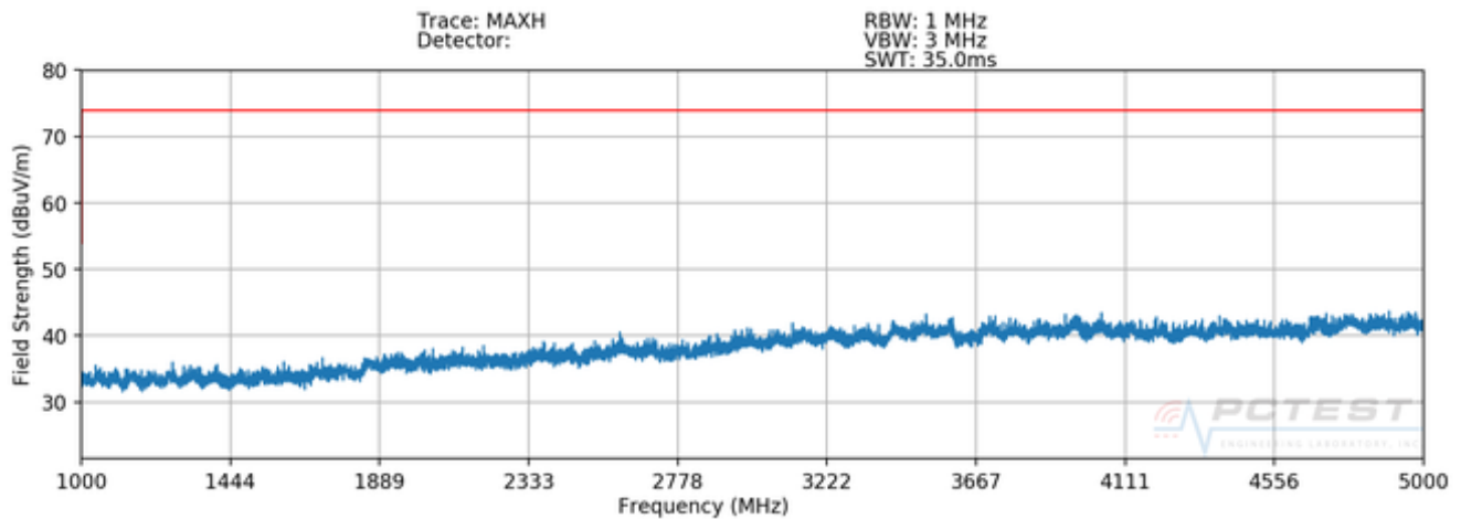
Plot 7-2. Radiated Spurious Plot above 1GHz - H - OPEN
