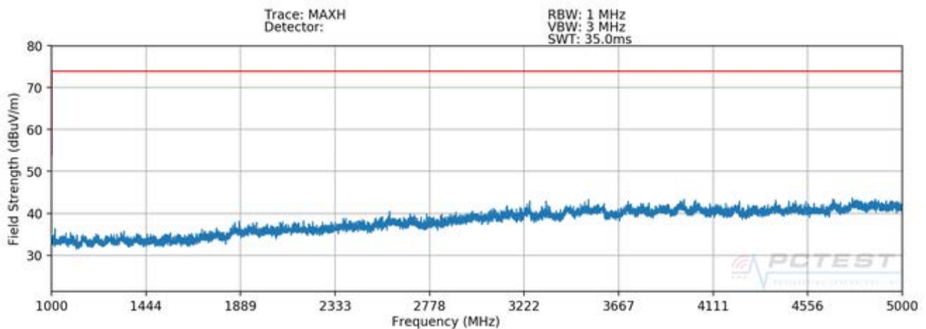
Plot 7-3. Radiated Spurious Plot above 1GHz - V - OPEN
