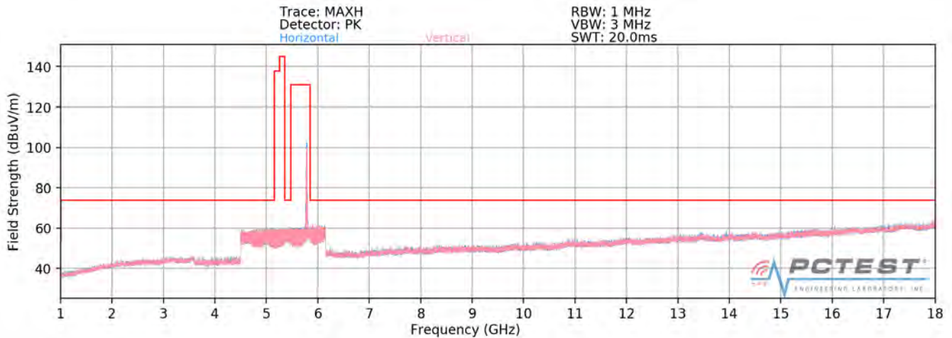
Plot 7-283. Radiated Spurious Plot above 1GHz SISO ANT2 (802.11a – U3 Ch. 157 - CLOSED)
