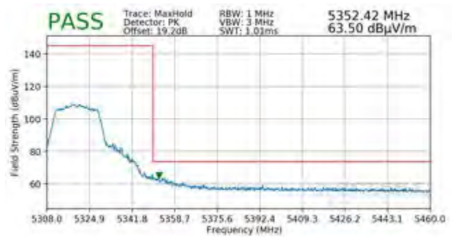
Plot 7-367. Radiated Band Edge Plot MIMO (Peak – WCP)
