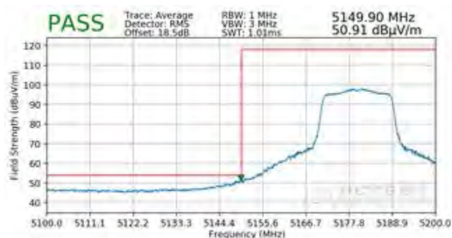
Plot 7-343. Radiated Band Edge Plot SISO ANT2 (Average – WCP)
