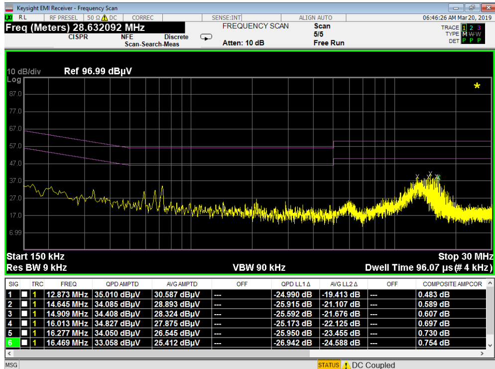
Plot 7-386. Line Conducted Plot with 802.11a UNII Band 1 (N)
