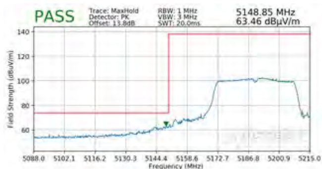
Plot 7-369. Radiated Lower Band Edge Plot MIMO (Peak – UNII Band 1)
