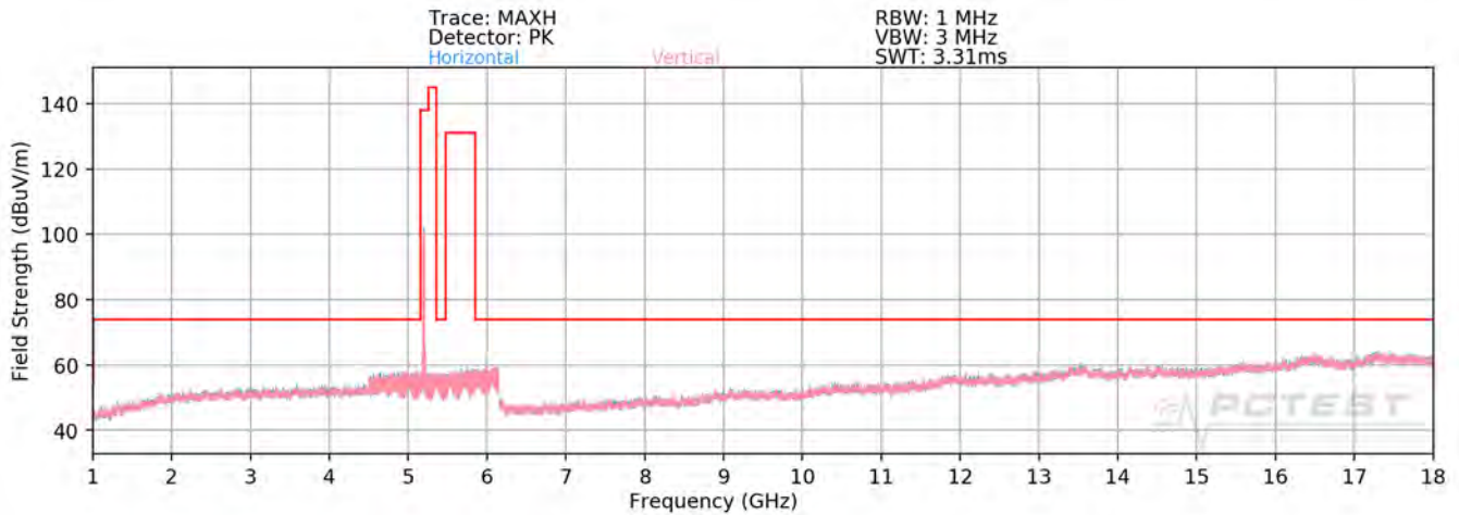
Plot 7-290. Radiated Spurious Plot above 1GHz MIMO/CDD (802.11a – U1 Ch. 40 - OPEN)
