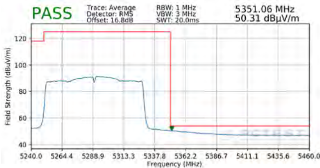
Plot 7-331. Radiated Upper Band Edge Plot SISO ANT1 (Average - UNII Band 2A)
