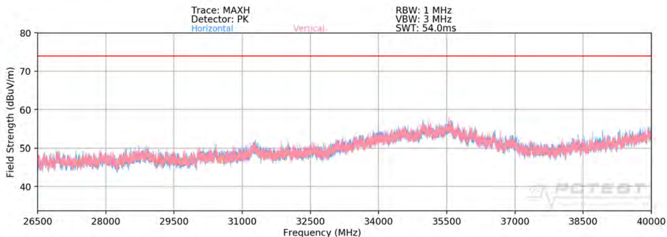
Plot 7-308. Radiated Spurious Plot above 26.5GHz (5GHz – 2.4 GHz - CLOSED)
