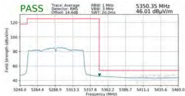
Plot 7-377. Radiated Upper Band Edge Plot MIMO (Average – UNII Band 2A)
