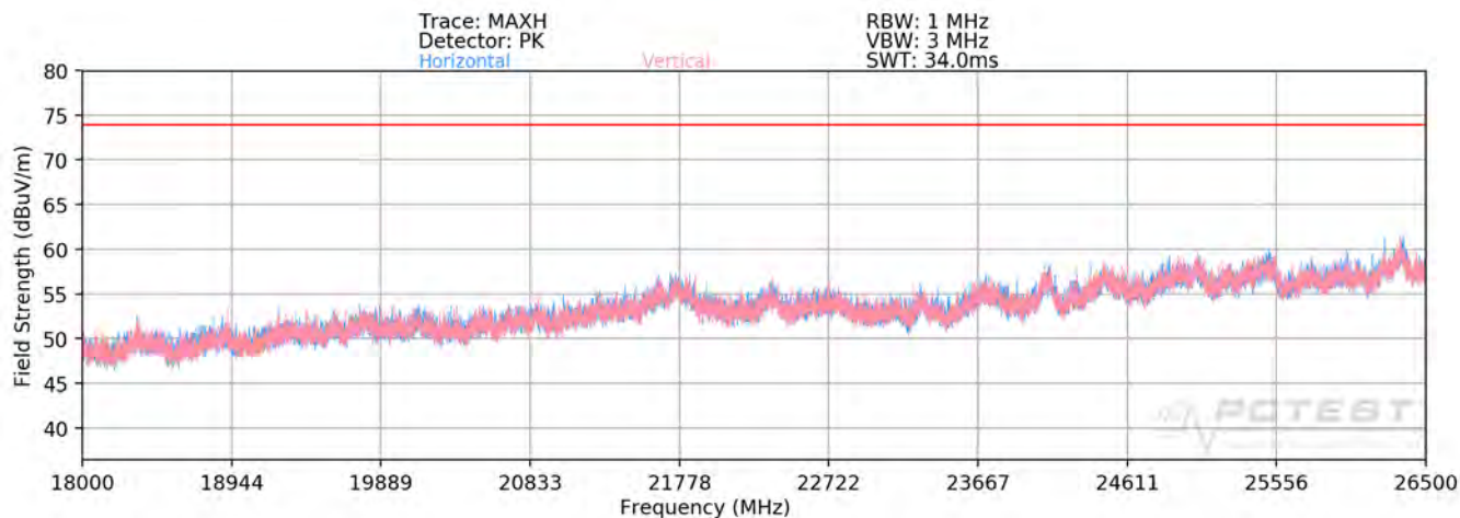
Plot 7-307. Radiated Spurious Plot 18GHz – 26.5GHz (5GHz – 2.4 GHz - CLOSED)
