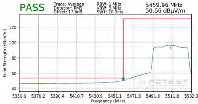
Plot 7-326. Radiated Lower Band Edge Plot SISO ANT1 (Average - UNII Band 2C)
