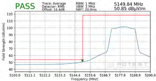
Plot 7-313. Radiated Lower Band Edge Plot SISO ANT1 (Average - UNII Band 1)
