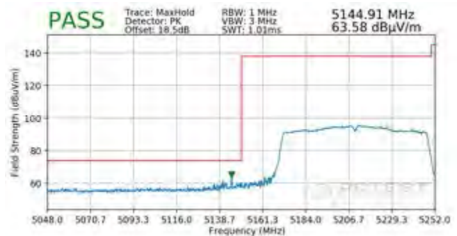
Plot 7-353. Radiated Lower Band Edge Plot SISO ANT2 (Peak - UNII Band 1)
