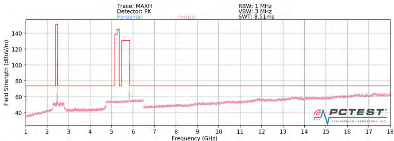
Plot 7-306. Radiated Spurious Plot above 1GHz (5GHz – 2.4 GHz - OPEN)
