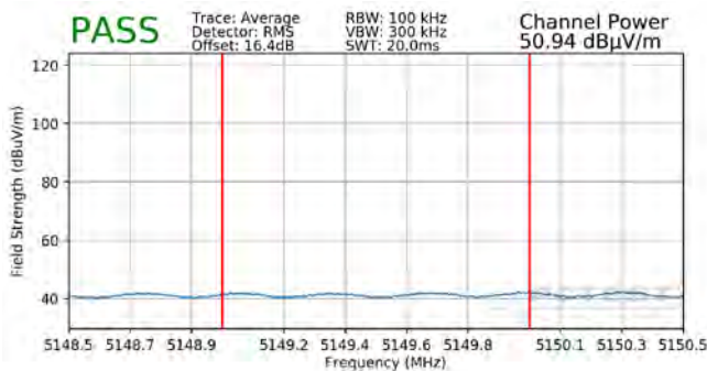
Plot 7-329. Radiated Lower Band Edge Plot SISO ANT1 (Average - UNII Band 1)
