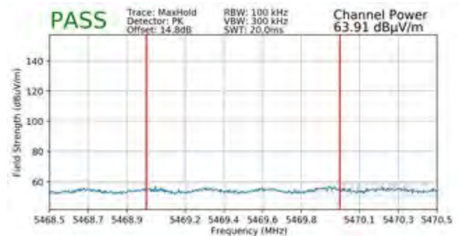
Plot 7-373. Radiated Lower Band Edge Plot MIMO (Peak – UNII Band 2C)
