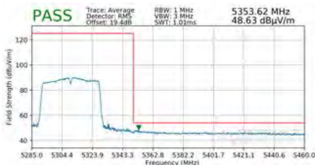
Plot 7-347. Radiated Upper Band Edge Plot SISO ANT2 (Average - UNII Band 2A)
