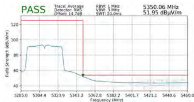
Plot 7-370. Radiated Upper Band Edge Plot MIMO (Average – UNII Band 2A)
