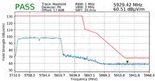
Plot 7-335. Radiated Upper Band Edge Plot SISO ANT1 (Peak - UNII Band 3)
