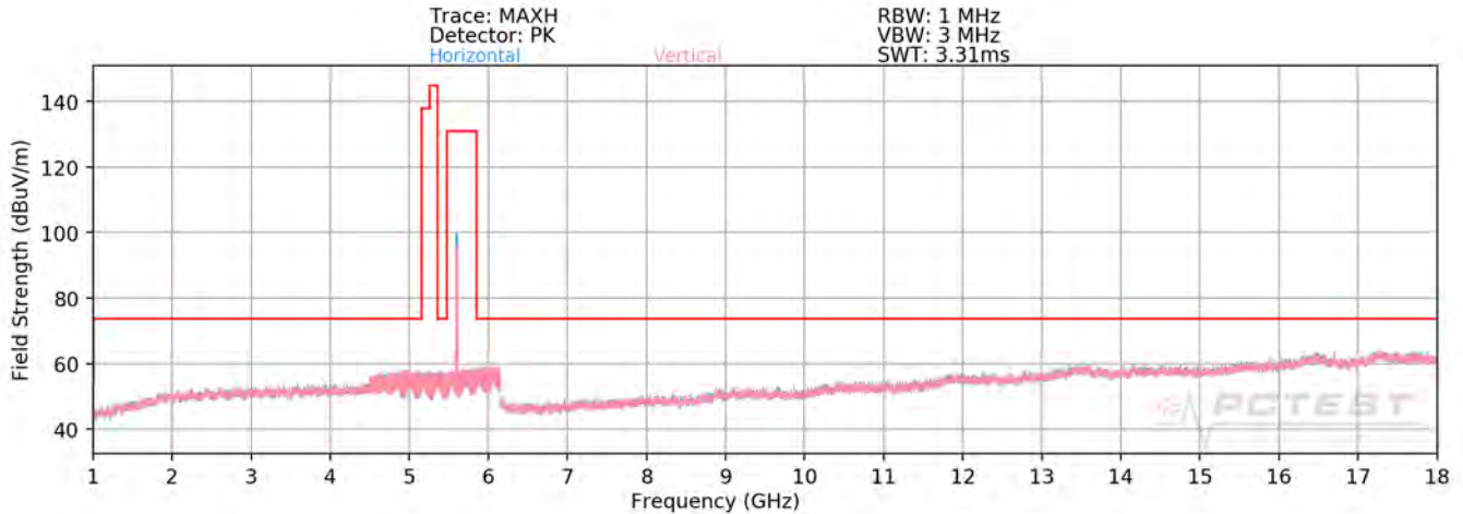
Plot 7-282. Radiated Spurious Plot above 1GHz SISO ANT2 (802.11a – U2C Ch. 120 - OPEN)
