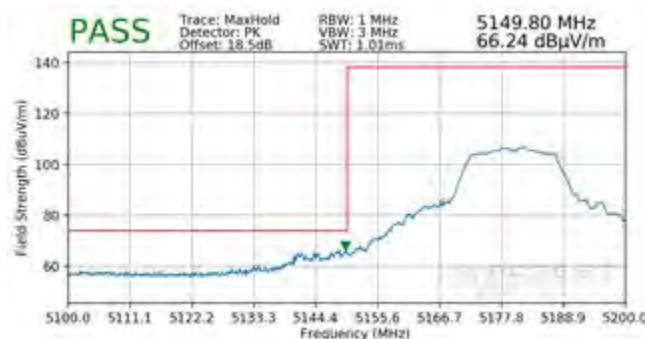
Plot 7-337. Radiated Lower Band Edge Plot SISO ANT2 (Peak – UNII Band 1)
