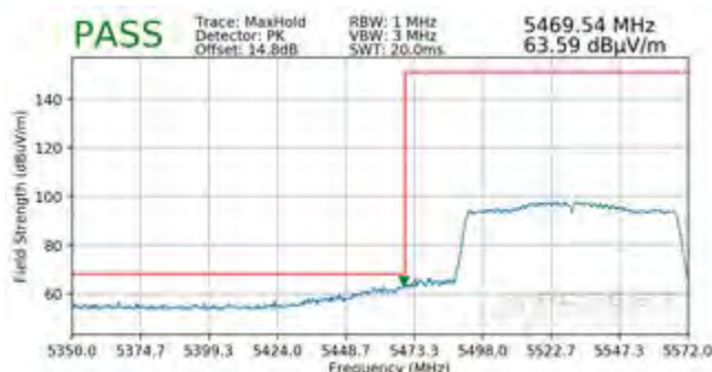
Plot 7-380. Radiated Lower Band Edge Plot MIMO (Peak – UNII Band 2C)
