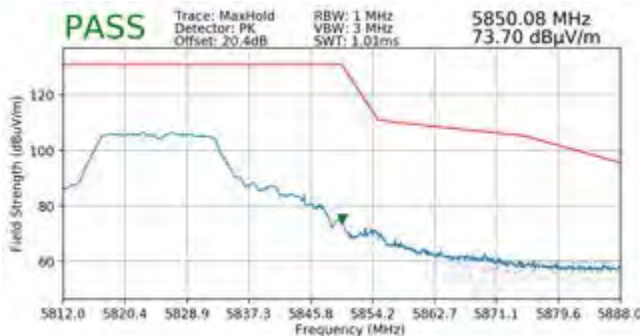
Plot 7-342. Radiated Upper Band Edge Plot SISO ANT2 (Peak - UNII Band 3)
