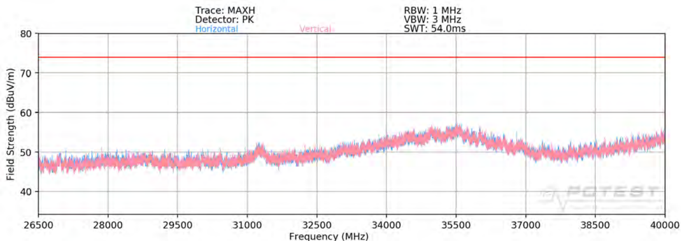
Plot 7-312. Radiated Spurious Plot above 26.5GHz (Dual Band Simult. Tx - CLOSED)
