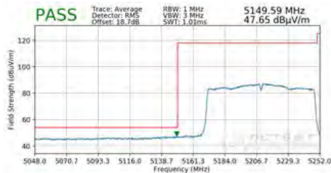
Plot 7-352. Radiated Lower Band Edge Plot SISO ANT2 (Average - UNII Band 1)
