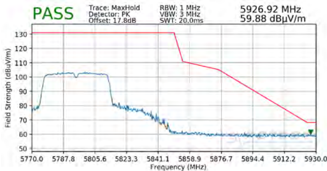
Plot 7-328. Radiated Upper Band Edge Plot SISO ANT1 (Peak - UNII Band 3)
