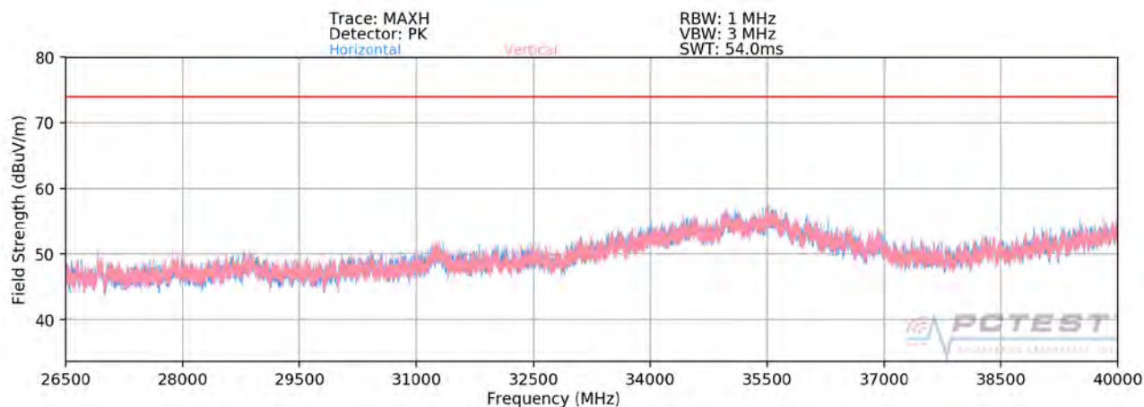
Plot 7-299. Radiated Spurious Plot 26.5GHz - 40GHz MIMO/CDD (802.11a - CLOSED)
