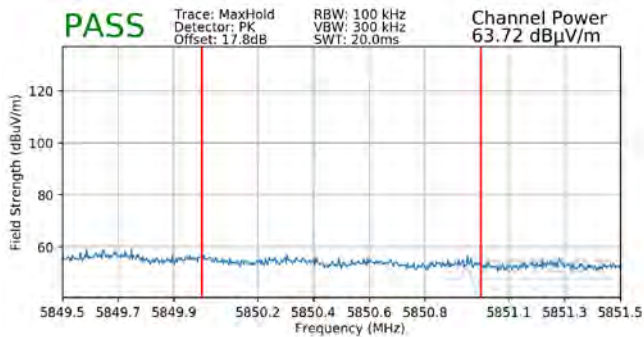
Plot 7-319. Radiated Upper Band Edge Plot SISO ANT1 (Peak – UNII Band 3)
