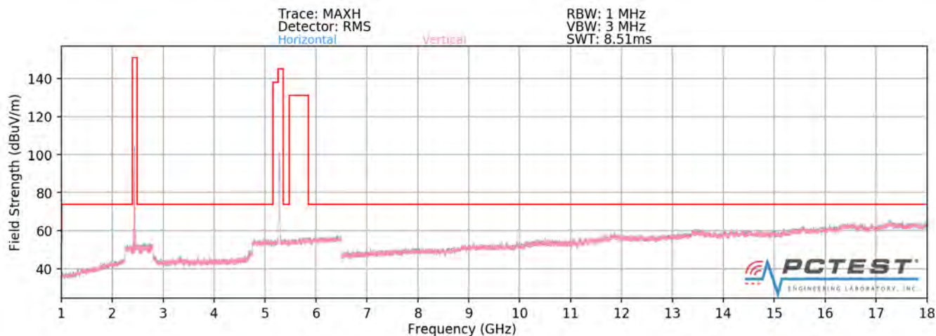
Plot 7-301. Radiated Spurious Plot above 1GHz (2.4GHz – 5GHz - CLOSED)
