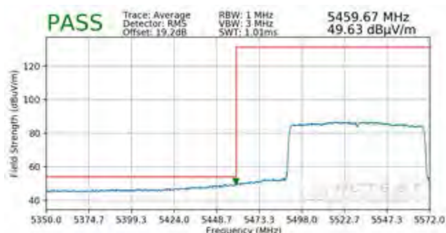
Plot 7-356. Radiated Lower Band Edge Plot SISO ANT2 (Average - UNII Band 2C)
