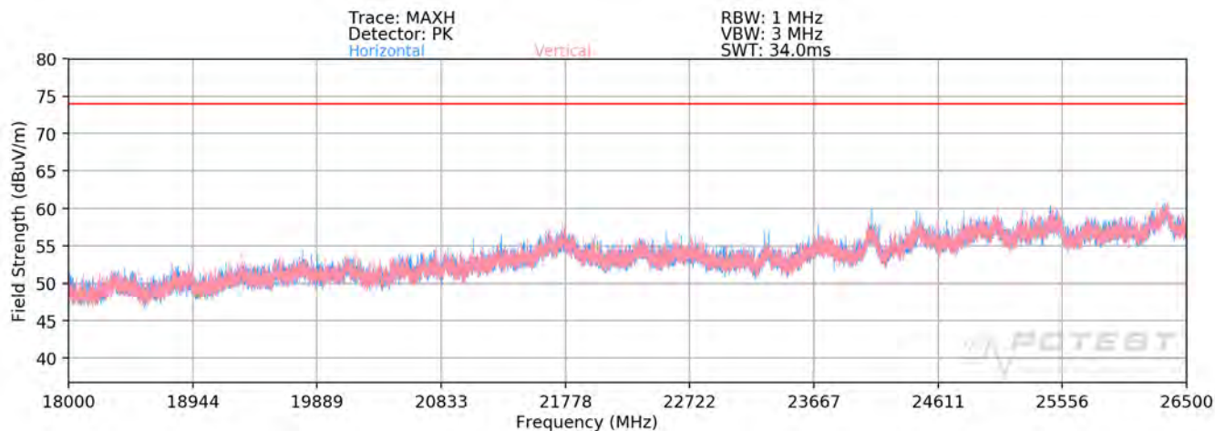
Plot 7-303. Radiated Spurious Plot 18GHz – 26.5GHz (2.4GHz – 5GHz - CLOSED)
