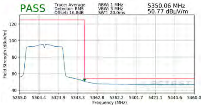
Plot 7-324. Radiated Upper Band Edge Plot SISO ANT1 (Average - UNII Band 2A)
