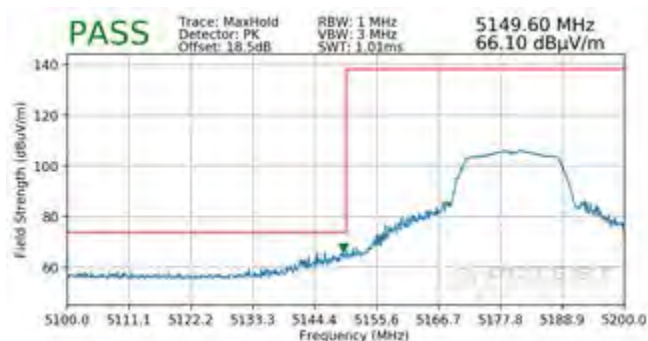
Plot 7-344. Radiated Band Edge Plot SISO ANT2 (Peak – WCP)
