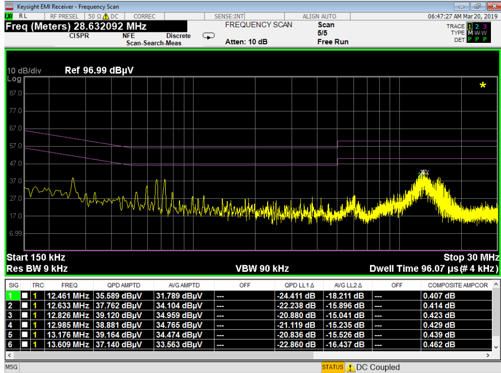
Plot 7-385. Line Conducted Plot with 802.11a UNII Band 1 (L1)
