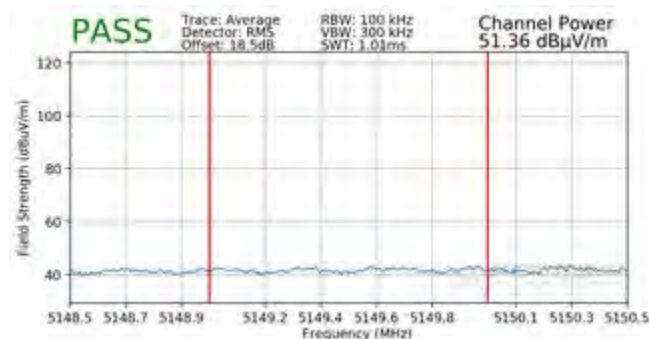
Plot 7-336. Radiated Lower Band Edge Plot SISO ANT2 (Average – UNII Band 1)
