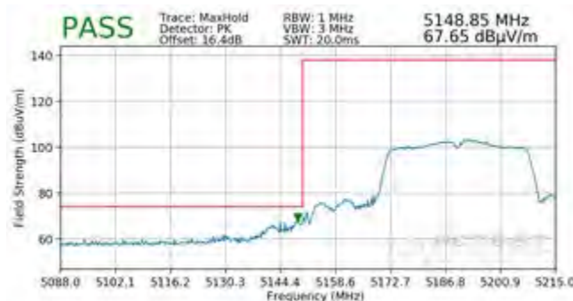
Plot 7-346. Radiated Lower Band Edge Plot SISO ANT2 (Peak - UNII Band 1)
