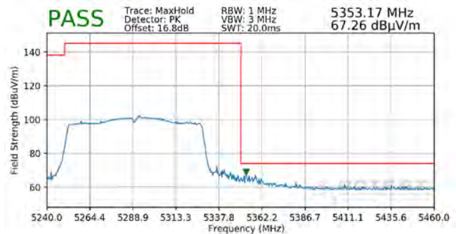
Plot 7-332. Radiated Upper Band Edge Plot SISO ANT1 (Peak - UNII Band 2A)
