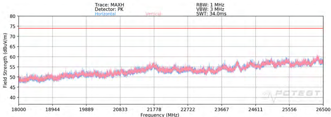
Plot 7-311. Radiated Spurious Plot 18GHz – 26.5GHz (Dual Band Simult. Tx - OPEN)
