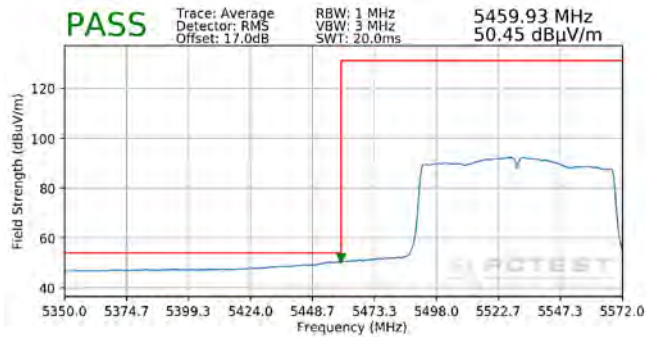
Plot 7-333. Radiated Lower Band Edge Plot SISO ANT1 (Average - UNII Band 2C)
