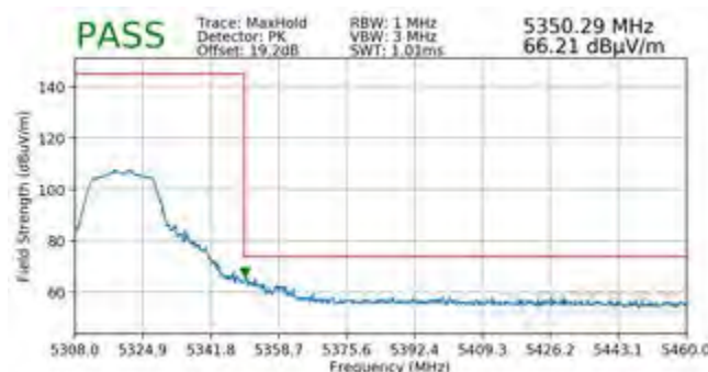
Plot 7-339. Radiated Upper Band Edge Plot SISO ANT2 (Peak – UNII Band 2A)
