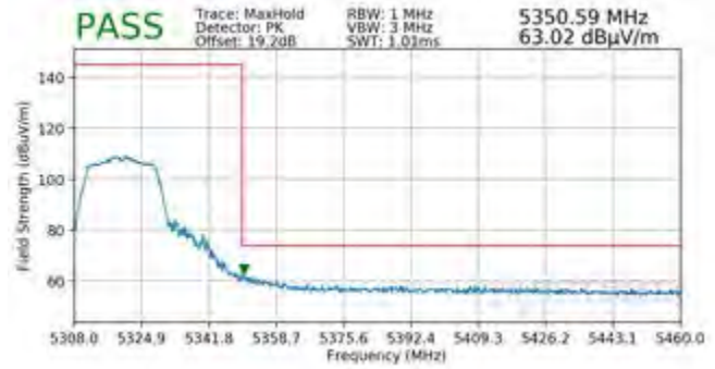
Plot 7-321. Radiated Band Edge Plot SISO ANT1 (Peak – WCP)
