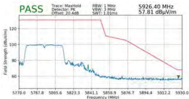
Plot 7-351. Radiated Upper Band Edge Plot SISO ANT2 (Peak - UNII Band 3)
