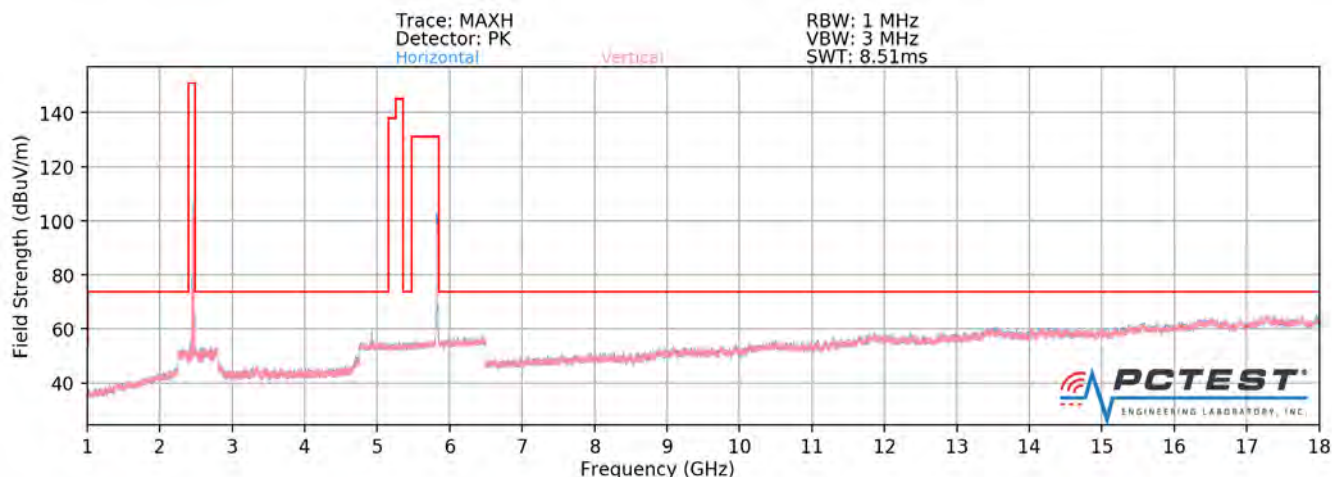
Plot 7-309. Radiated Spurious Plot above 1GHz (Dual Band Simult. Tx - CLOSED)
