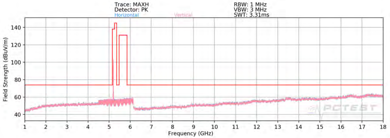
Plot 7-289. Radiated Spurious Plot above 1GHz MIMO/CDD (802.11a – U1 Ch. 40 - CLOSED)
