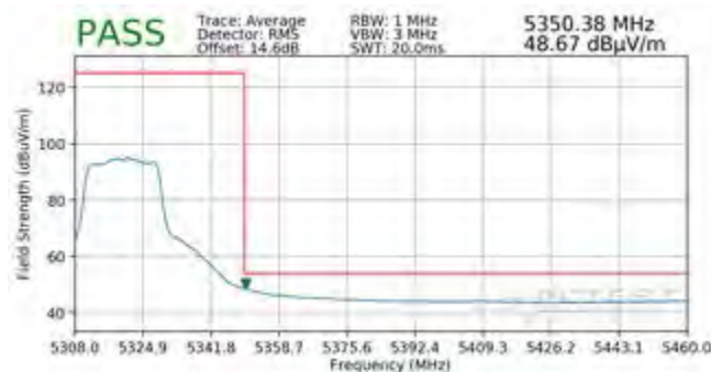
Plot 7-361. Radiated Upper Band Edge Plot MIMO (Average – UNII Band 2A)
