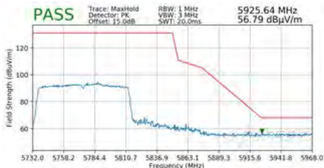
Plot 7-381. Radiated Upper Band Edge Plot MIMO (Peak – UNII Band 3)
