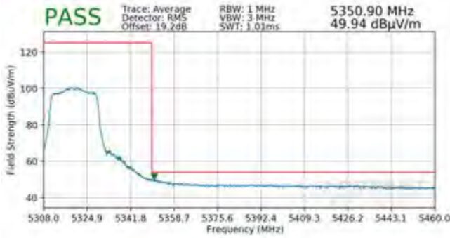
Plot 7-320. Radiated Band Edge Plot SISO ANT1 (Average – WCP)
