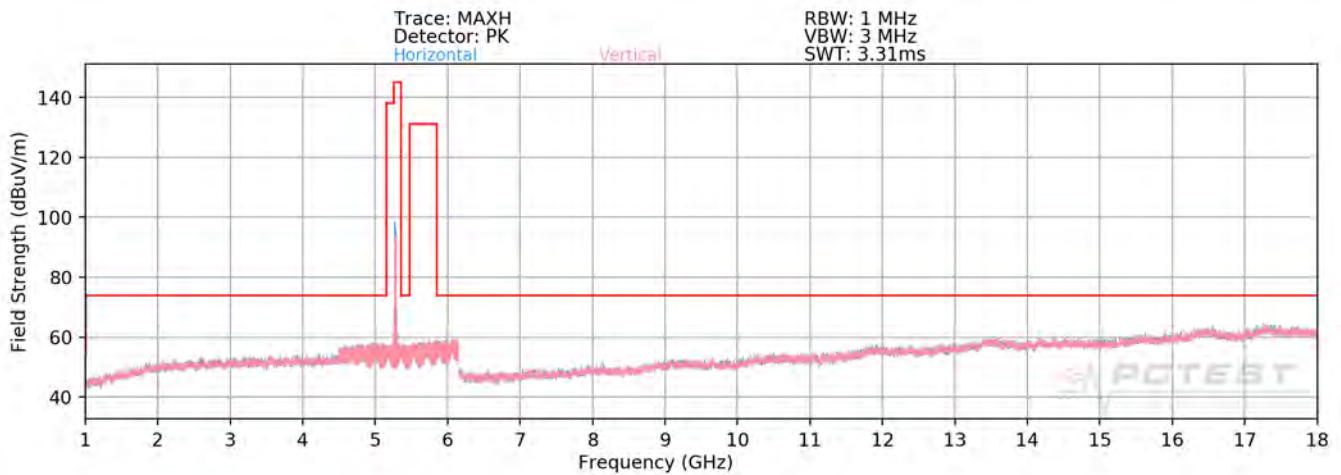
Plot 7-280. Radiated Spurious Plot above 1GHz SISO ANT2 (802.11a – U2A Ch. 56 - OPEN)
