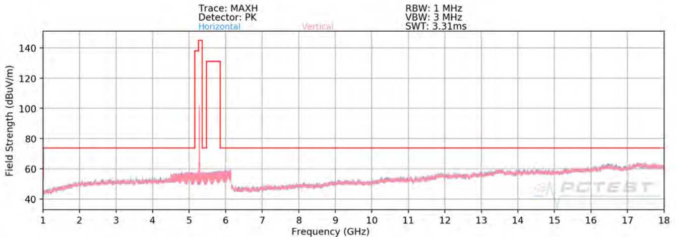
Plot 7-292. Radiated Spurious Plot above 1GHz MIMO/CDD (802.11a – U2A Ch. 56 - OPEN)
