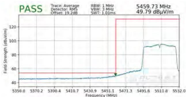
Plot 7-349. Radiated Lower Band Edge Plot SISO ANT2 (Average - UNII Band 2C)
