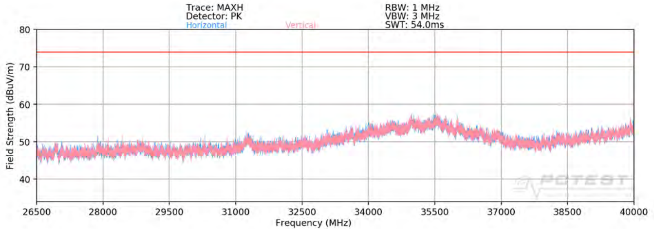
Plot 7-288. Radiated Spurious Plot 26.5GHz - 40GHz SISO ANT2 (802.11a - OPEN)
