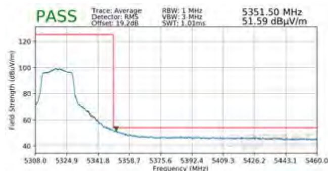
Plot 7-338. Radiated Upper Band Edge Plot SISO ANT2 (Average – UNII Band 2A)
