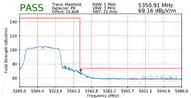
Plot 7-325. Radiated Upper Band Edge Plot SISO ANT1 (Peak - UNII Band 2A)
