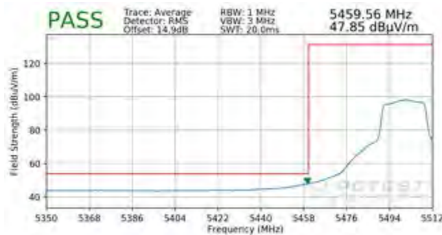
Plot 7-363. Radiated Lower Band Edge Plot MIMO (Average – UNII Band 2C)
