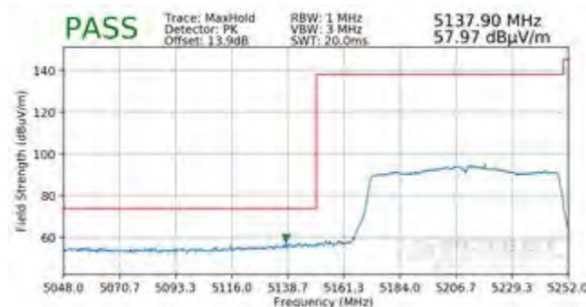
Plot 7-376. Radiated Lower Band Edge Plot MIMO (Peak – UNII Band 1)
