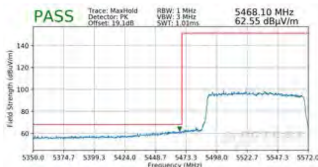
Plot 7-357. Radiated Lower Band Edge Plot SISO ANT2 (Peak - UNII Band 2C)
