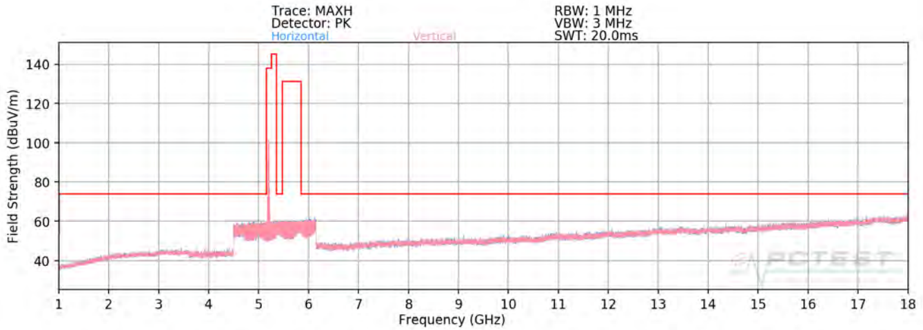
Plot 7-277. Radiated Spurious Plot above 1GHz SISO ANT2 (802.11a – U1 Ch. 40 - CLOSED)
