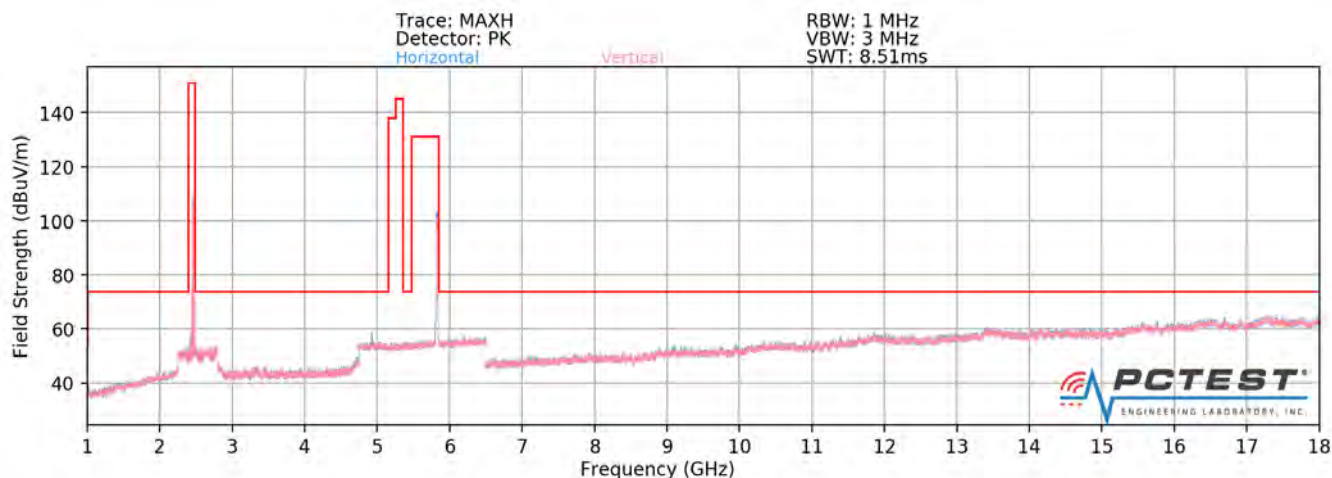
Plot 7-310. Radiated Spurious Plot above 1GHz (Dual Band Simult. Tx - OPEN)
