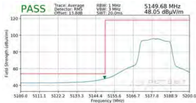
Plot 7-359. Radiated Lower Band Edge Plot MIMO (Average – UNII Band 1)
