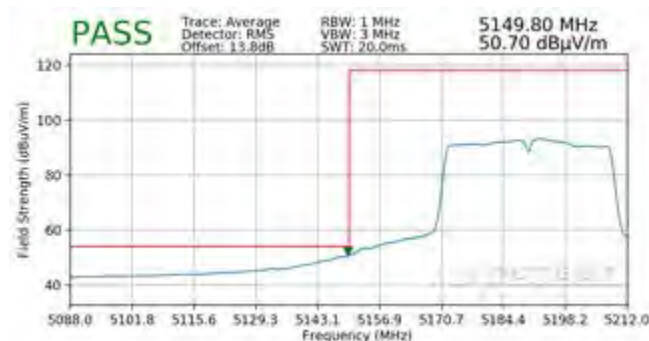
Plot 7-368. Radiated Lower Band Edge Plot MIMO (Average – UNII Band 1)
