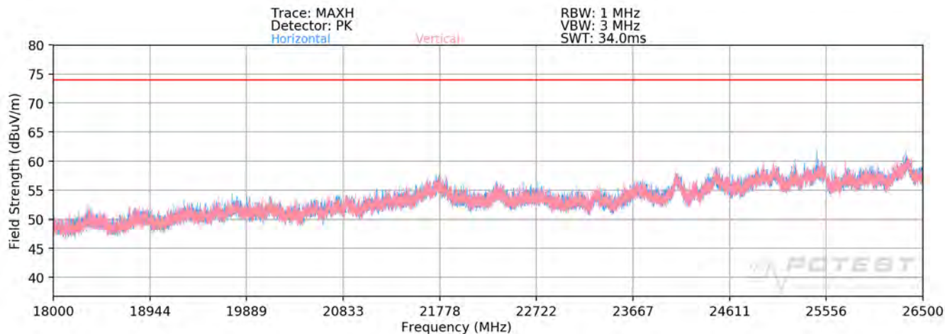
Plot 7-285. Radiated Spurious Plot above 18GHz - 26.5GHz SISO ANT2 (802.11a - CLOSED)
