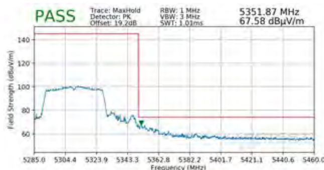
Plot 7-348. Radiated Upper Band Edge Plot SISO ANT2 (Peak - UNII Band 2A)
