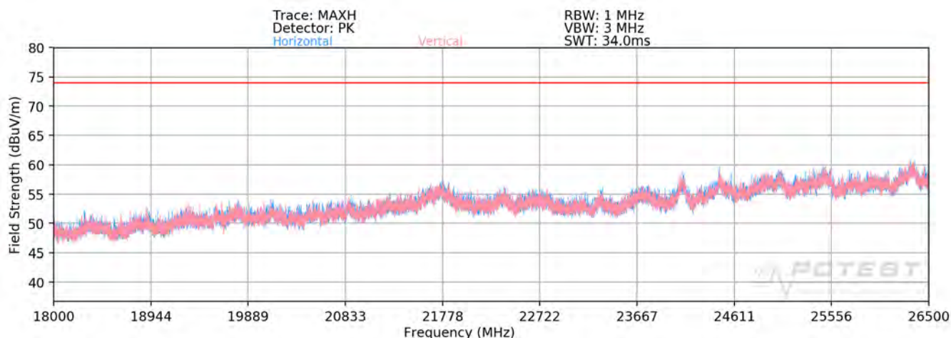
Plot 7-286. Radiated Spurious Plot above 18GHz - 26.5GHz SISO ANT2 (802.11a - OPEN)
