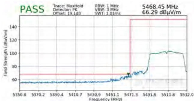
Plot 7-350. Radiated Lower Band Edge Plot SISO ANT2 (Peak - UNII Band 2C)
