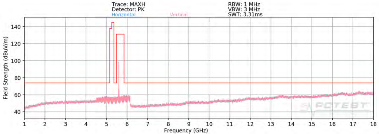
Plot 7-294. Radiated Spurious Plot above 1GHz MIMO/CDD (802.11a – U2C Ch. 120 - OPEN)
