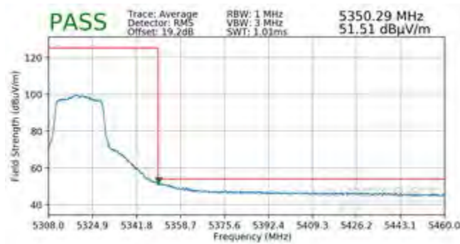
Plot 7-366. Radiated Band Edge Plot MIMO (Average – WCP)
