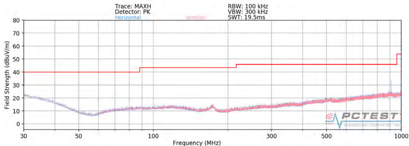
Plot 7-384. Radiated Spurious Plot below 1GHz (Dual Band Simult. Tx)
