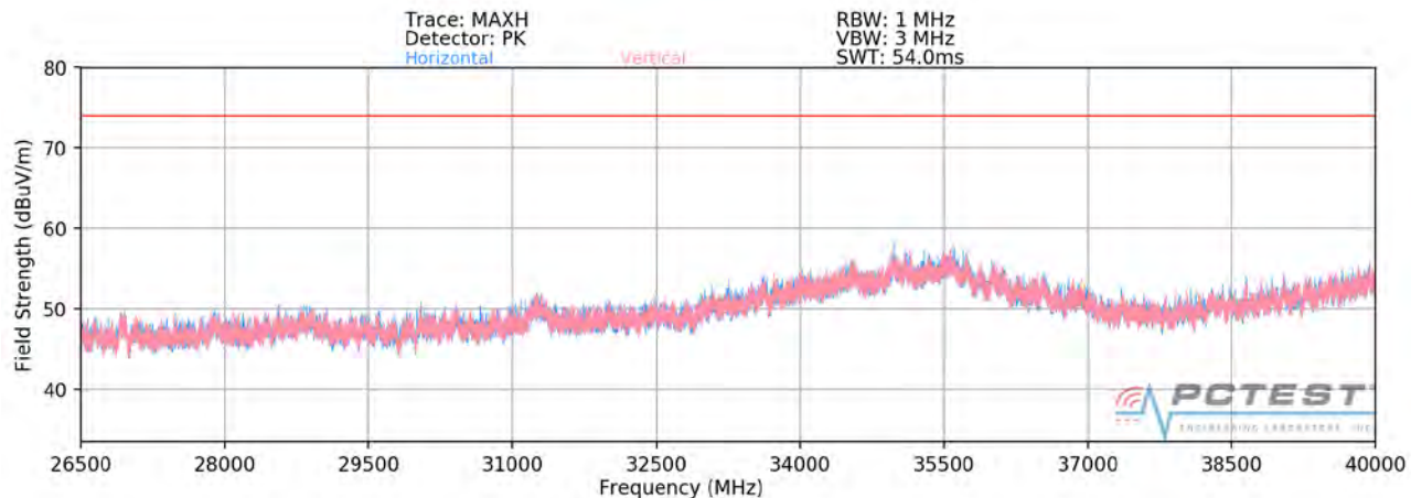
Plot 7-300. Radiated Spurious Plot 26.5GHz - 40GHz MIMO/CDD (802.11a - OPEN)
