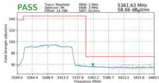
Plot 7-378. Radiated Upper Band Edge Plot MIMO (Peak – UNII Band 2A)
