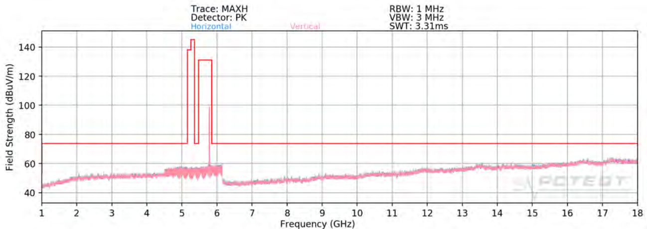
Plot 7-295. Radiated Spurious Plot above 1GHz MIMO/CDD (802.11a – U3 Ch. 157 - CLOSED)
