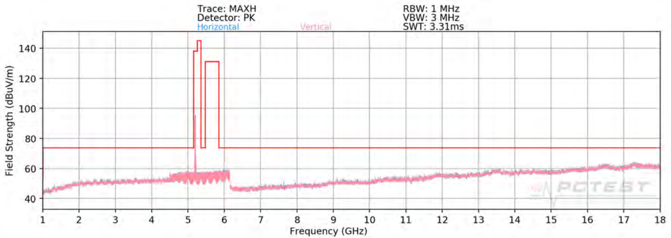
Plot 7-278. Radiated Spurious Plot above 1GHz SISO ANT2 (802.11a – U1 Ch. 40 - OPEN)
