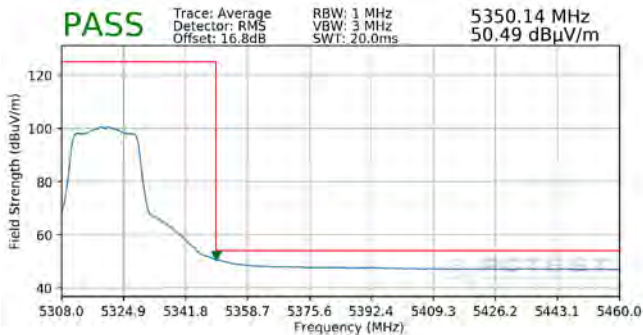
Plot 7-315. Radiated Upper Band Edge Plot SISO ANT1 (Average - UNII Band 2A)
