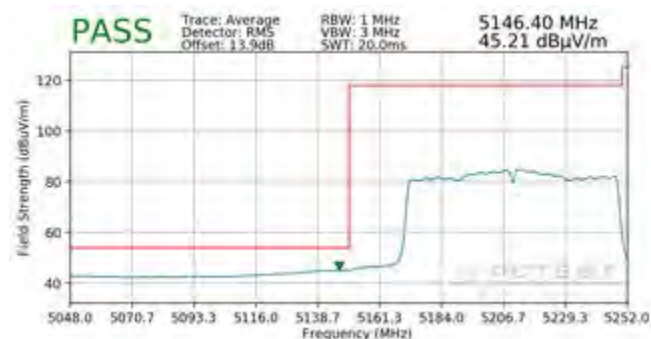
Plot 7-375. Radiated Lower Band Edge Plot MIMO (Average – UNII Band 1)
