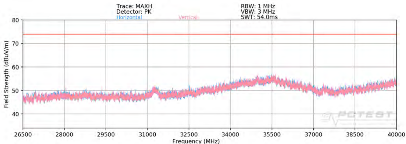
Plot 7-304. Radiated Spurious Plot above 26.5GHz (2.4GHz – 5GHz - CLOSED)
