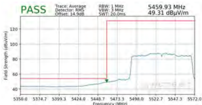
Plot 7-379. Radiated Lower Band Edge Plot MIMO (Average – UNII Band 2C)
