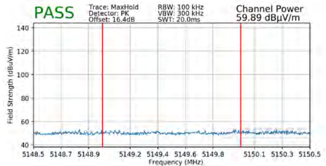
Plot 7-314. Radiated Lower Band Edge Plot SISO ANT1 (Peak - UNII Band 1)
