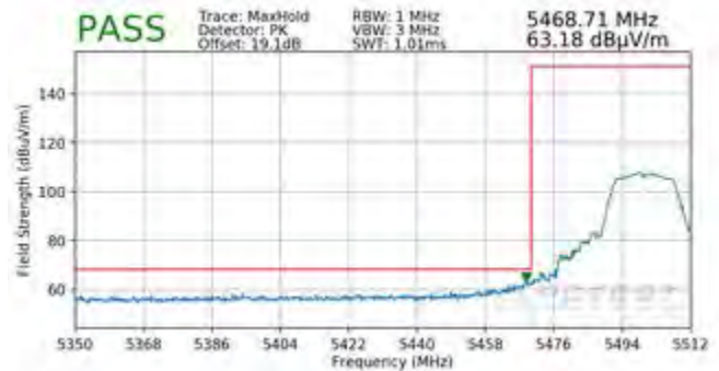
Plot 7-341. Radiated Lower Band Edge Plot SISO ANT2 (Peak - UNII Band 2C)
