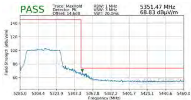
Plot 7-371. Radiated Upper Band Edge Plot MIMO (Peak – UNII Band 2A)
