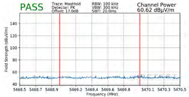
Plot 7-334. Radiated Lower Band Edge Plot SISO ANT1 (Peak - UNII Band 2C)
