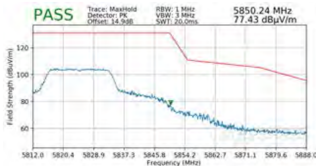
Plot 7-365. Radiated Upper Band Edge Plot MIMO (Peak – UNII Band 3)
