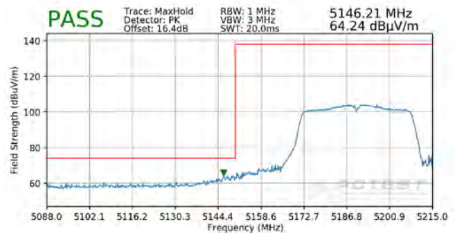
Plot 7-323. Radiated Lower Band Edge Plot SISO ANT1 (Peak - UNII Band 1)
