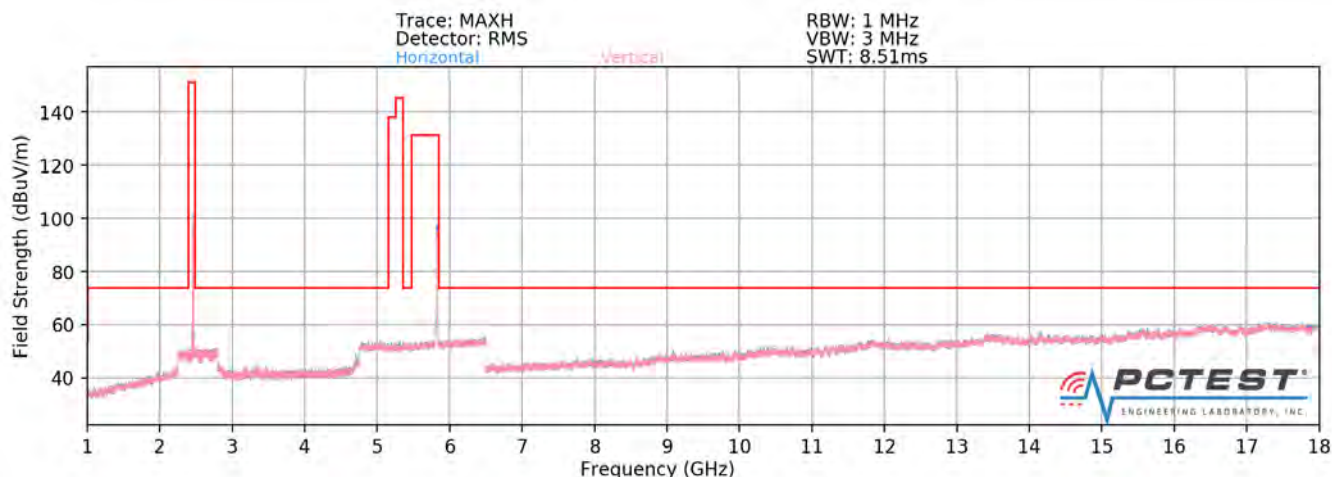
Plot 7-305. Radiated Spurious Plot above 1GHz (5GHz – 2.4 GHz - CLOSED)
