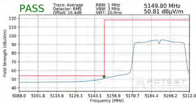
Plot 7-322. Radiated Lower Band Edge Plot SISO ANT1 (Average - UNII Band 1)
