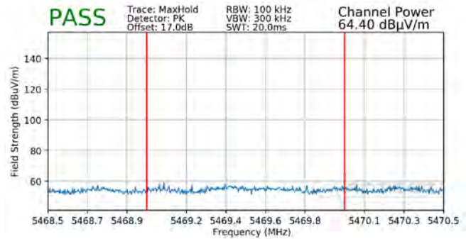
Plot 7-327. Radiated Lower Band Edge Plot SISO ANT1 (Peak - UNII Band 2C)
