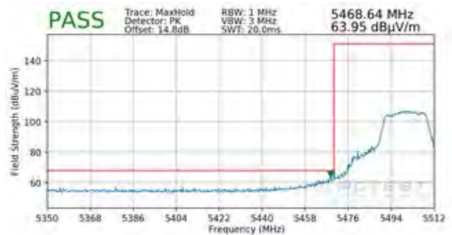
Plot 7-364. Radiated Lower Band Edge Plot MIMO (Peak – UNII Band 2C)
