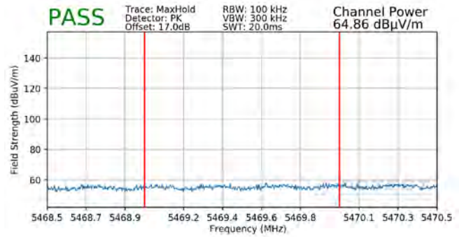
Plot 7-318. Radiated Lower Band Edge Plot SISO ANT1 (Peak – UNII Band 2C)
