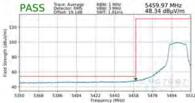
Plot 7-340. Radiated Lower Band Edge Plot SISO ANT2 (Average - UNII Band 2C)
