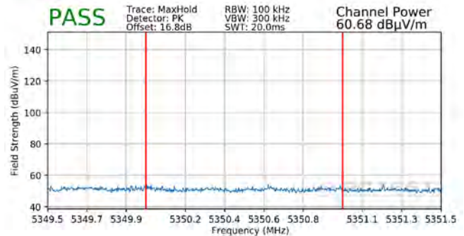
Plot 7-316. Radiated Upper Band Edge Plot SISO ANT1 (Peak - UNII Band 2A)
