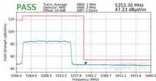
Plot 7-354. Radiated Upper Band Edge Plot SISO ANT2 (Average - UNII Band 2A)
