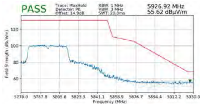
Plot 7-374. Radiated Upper Band Edge Plot MIMO (Peak – UNII Band 3)
