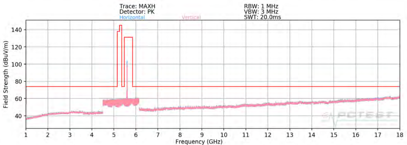
Plot 7-281. Radiated Spurious Plot above 1GHz SISO ANT2 (802.11a – U2C Ch. 120 - CLOSED)
