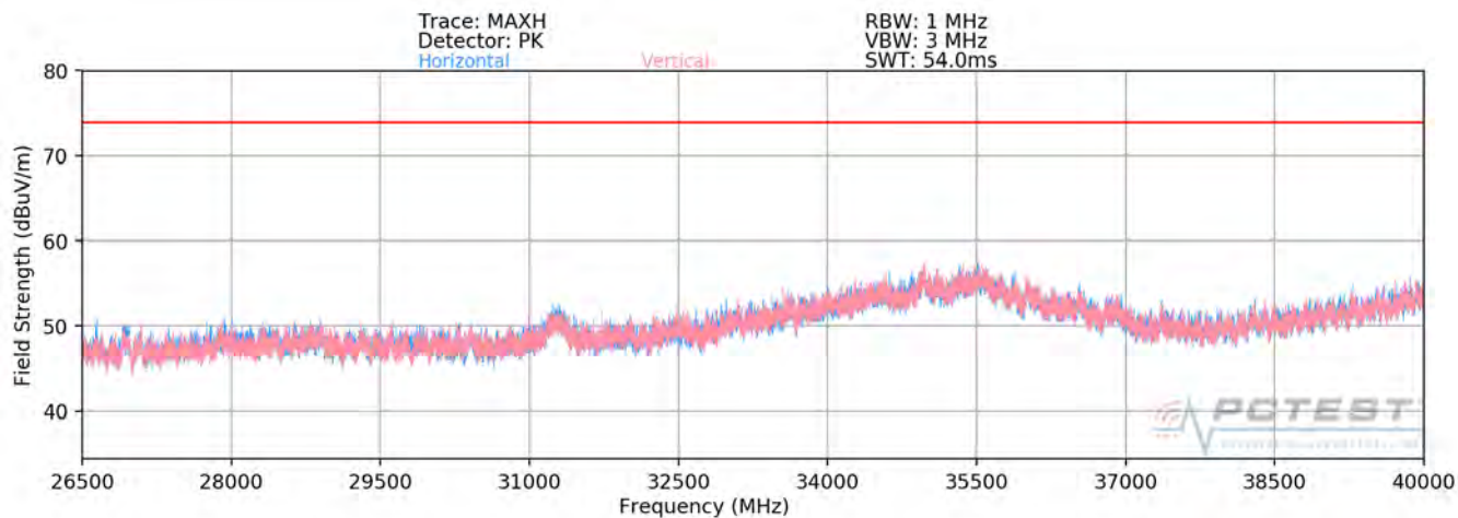
Plot 7-276. Radiated Spurious Plot 26.5GHz - 40GHz SISO ANT1 (802.11a - OPEN)
