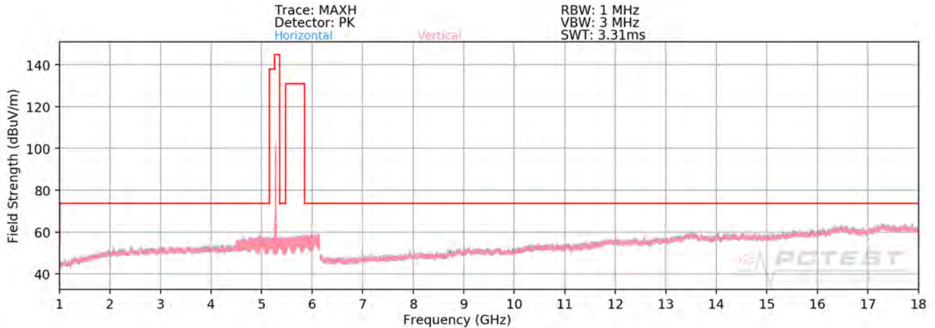
Plot 7-291. Radiated Spurious Plot above 1GHz MIMO/CDD (802.11a – U2A Ch. 56 - CLOSED)
