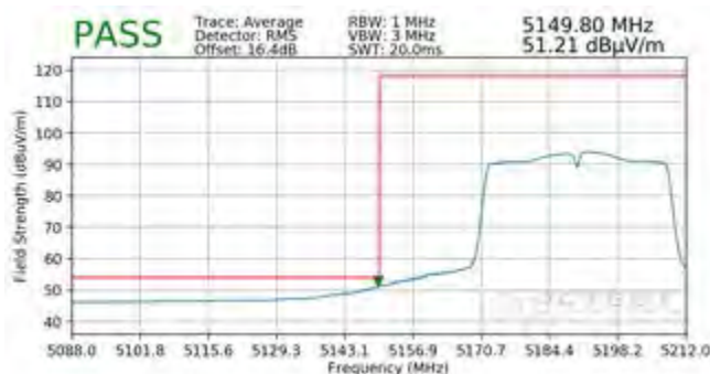
Plot 7-345. Radiated Lower Band Edge Plot SISO ANT2 (Average - UNII Band 1)
