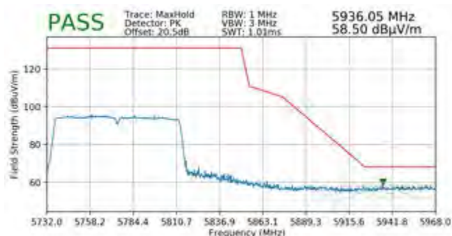
Plot 7-358. Radiated Upper Band Edge Plot SISO ANT2 (Peak - UNII Band 3)
