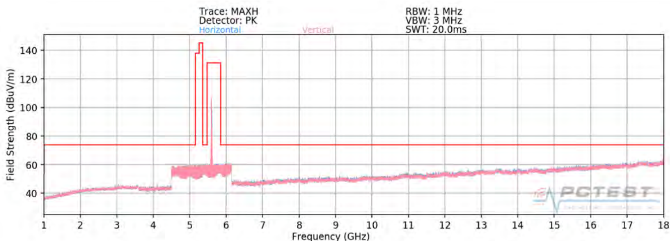
Plot 7-269. Radiated Spurious Plot above 1GHz SISO ANT1 (802.11a – U2C Ch. 120 - CLOSED)
