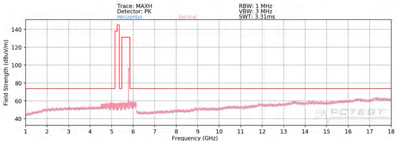
Plot 7-296. Radiated Spurious Plot above 1GHz MIMO/CDD (802.11a – U3 Ch. 157 - OPEN)
