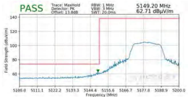
Plot 7-360. Radiated Lower Band Edge Plot MIMO (Peak – UNII Band 1)
