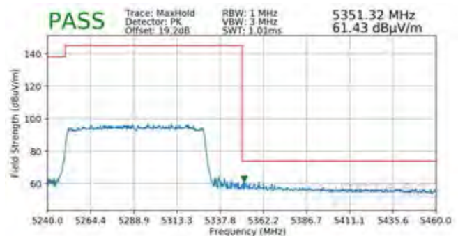
Plot 7-355. Radiated Upper Band Edge Plot SISO ANT2 (Peak - UNII Band 2A)
