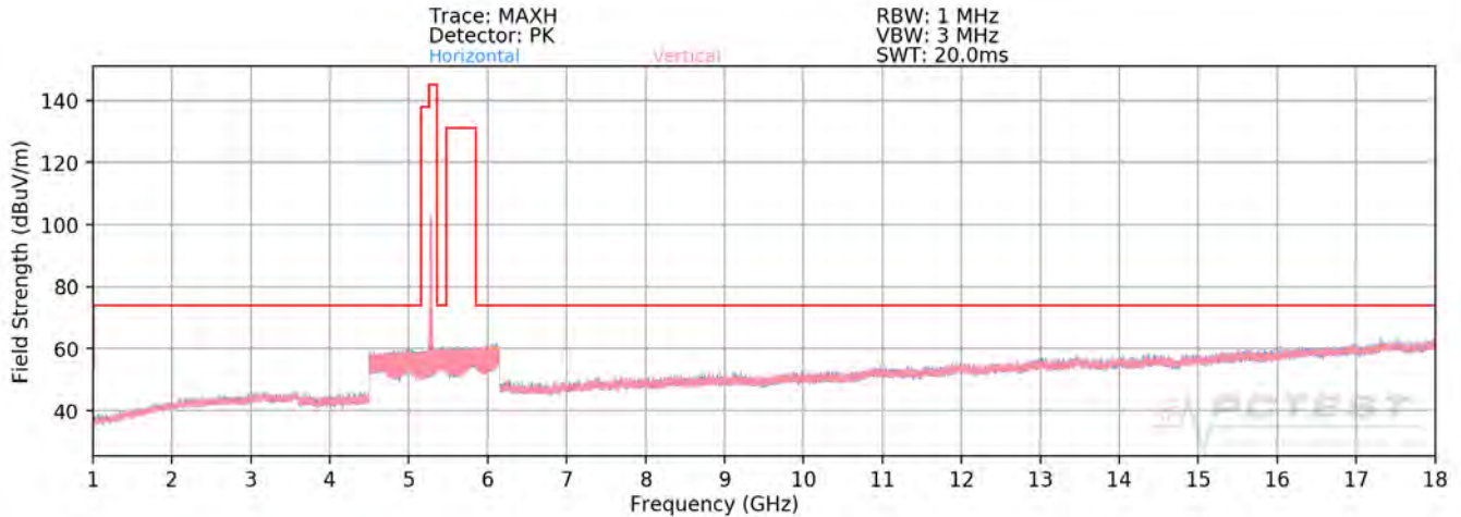
Plot 7-279. Radiated Spurious Plot above 1GHz SISO ANT2 (802.11a – U2A Ch. 56 - CLOSED)
