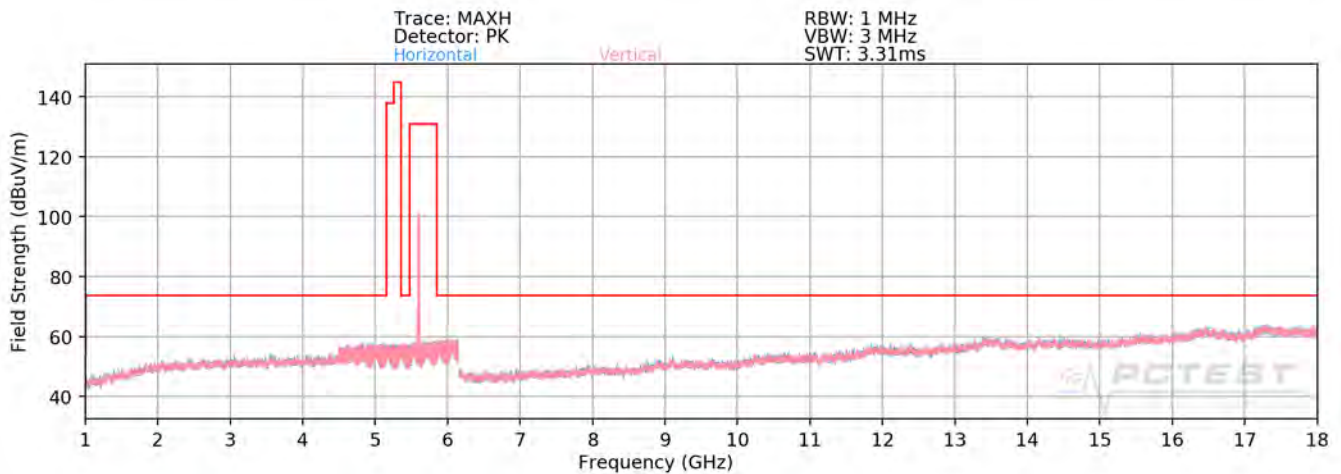
Plot 7-293. Radiated Spurious Plot above 1GHz MIMO/CDD (802.11a – U2C Ch. 120 - CLOSED)
