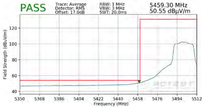
Plot 7-317. Radiated Lower Band Edge Plot SISO ANT1 (Average – UNII Band 2C)
