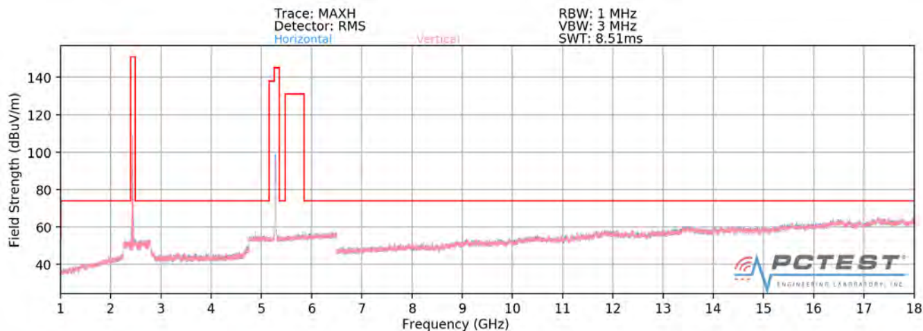
Plot 7-302. Radiated Spurious Plot above 1GHz (2.4GHz – 5GHz - OPEN)
