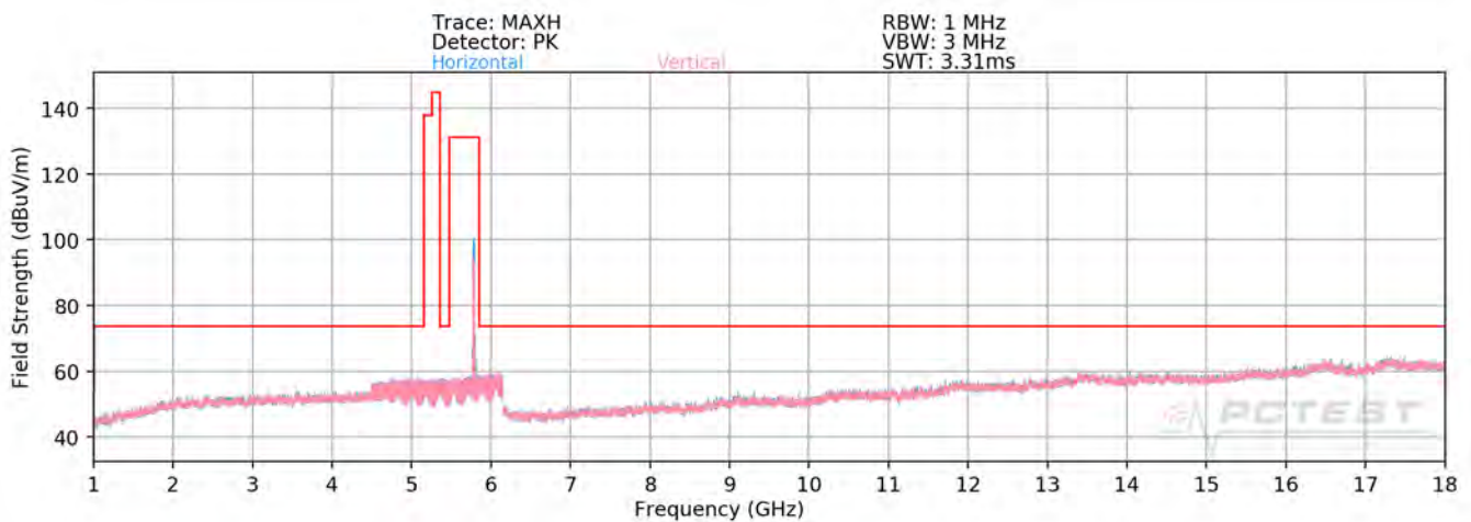
Plot 7-284. Radiated Spurious Plot above 1GHz SISO ANT2 (802.11a – U3 Ch. 157 - OPEN)
