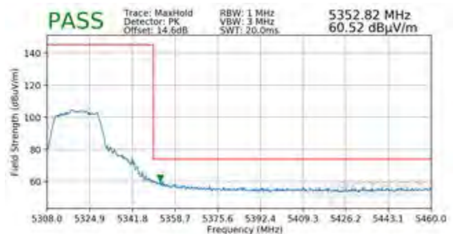
Plot 7-362. Radiated Upper Band Edge Plot MIMO (Peak – UNII Band 2A)
