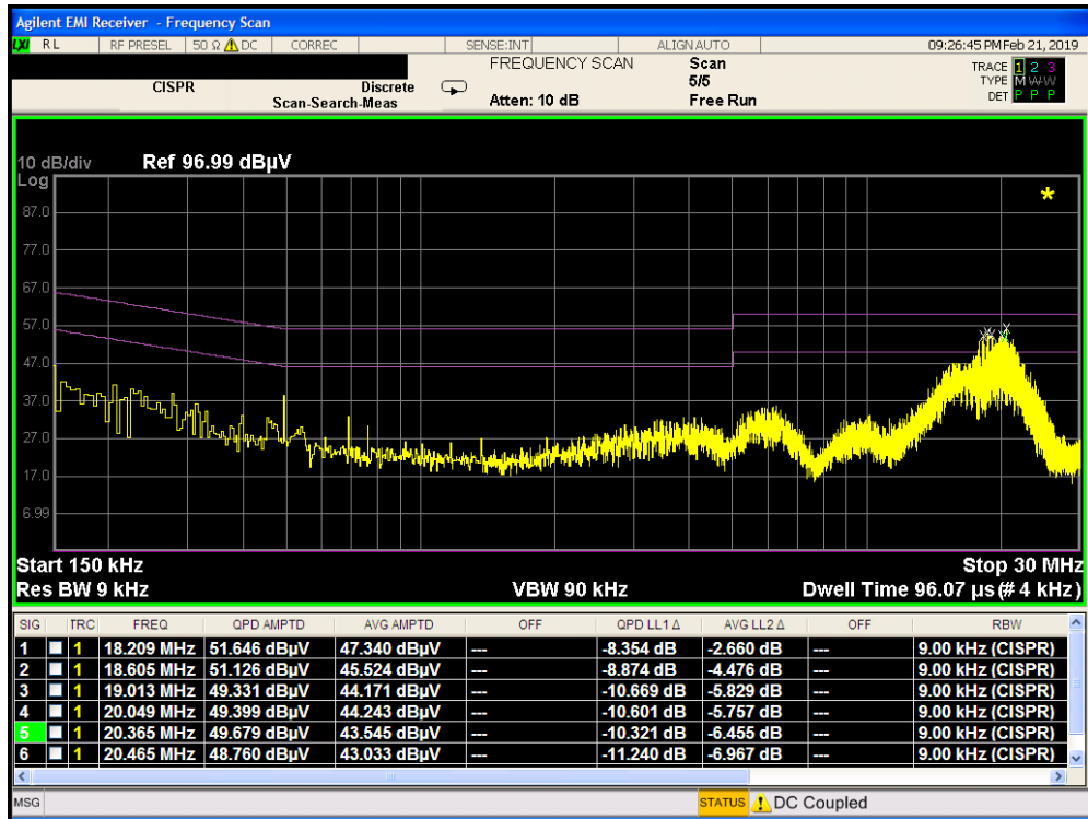
Plot 7-389. Line Conducted Plot with 802.11a UNII Band 2C (L1)
