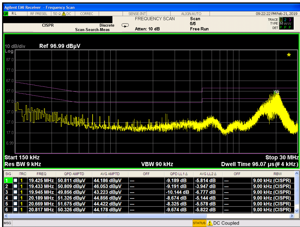
Plot 7-387. Line Conducted Plot with 802.11a UNII Band 2A (L1)
