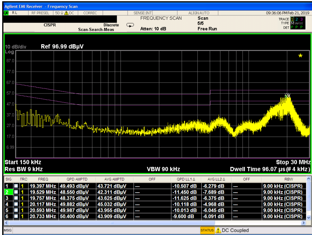
Plot 7-391. Line Conducted Plot with 802.11a UNII Band 3 (L1)
