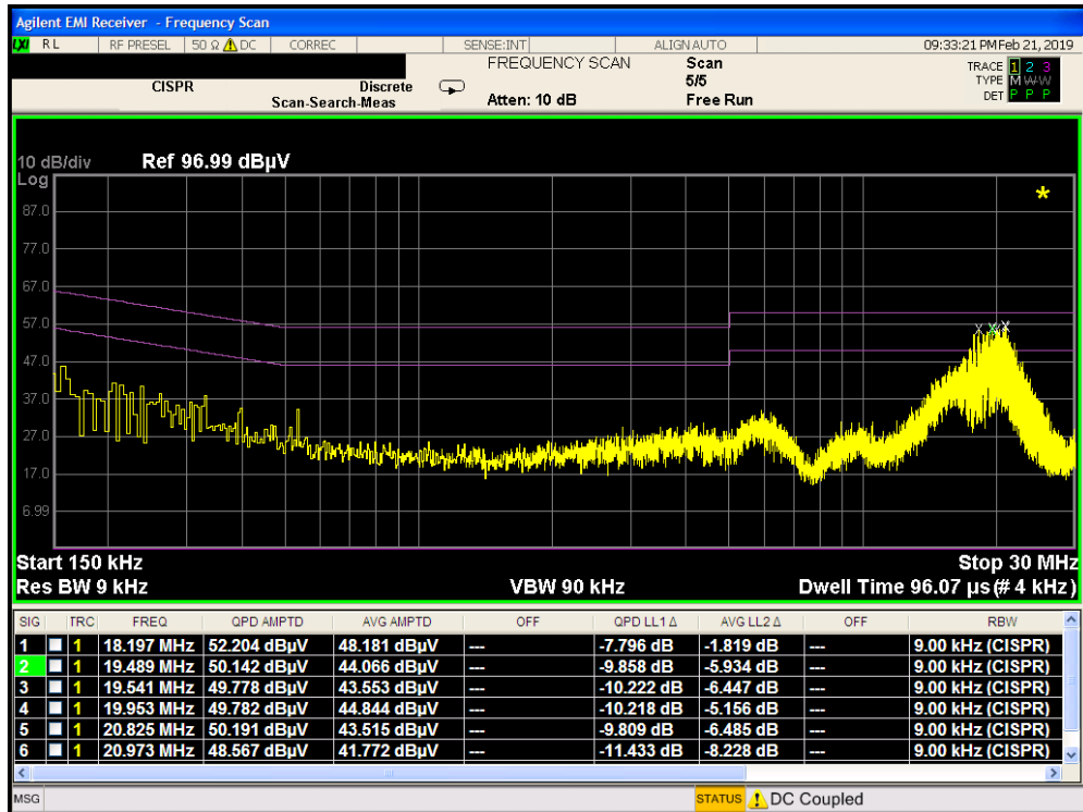
Plot 7-392. Line Conducted Plot with 802.11a UNII Band 3 (N)
