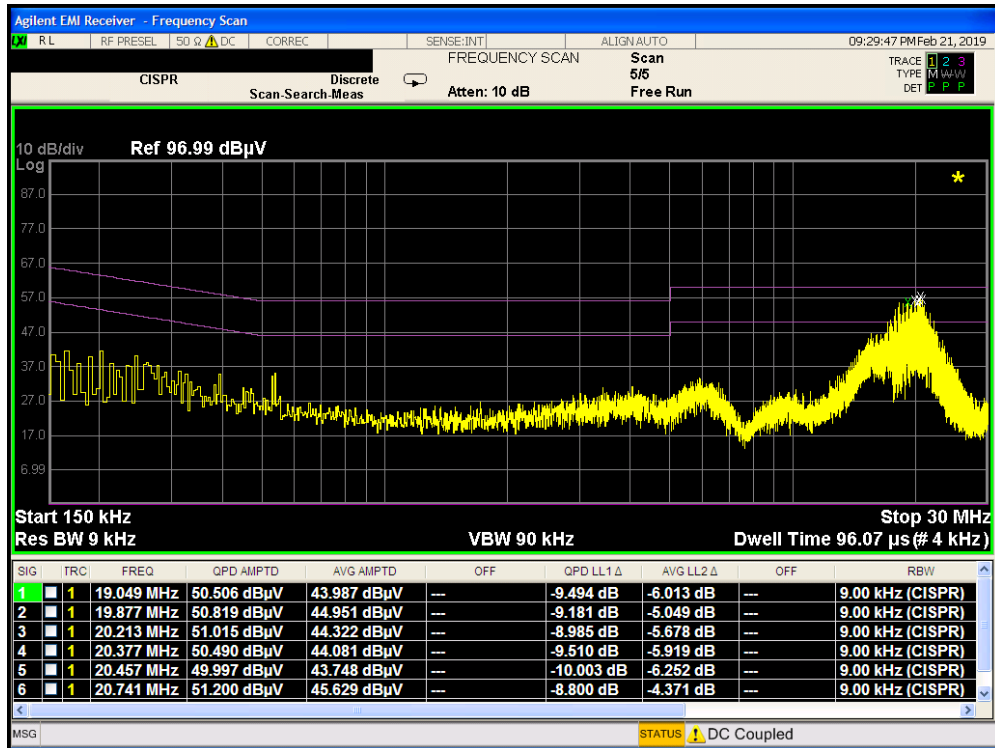
Plot 7-390. Line Conducted Plot with 802.11a UNII Band 2C (N)
