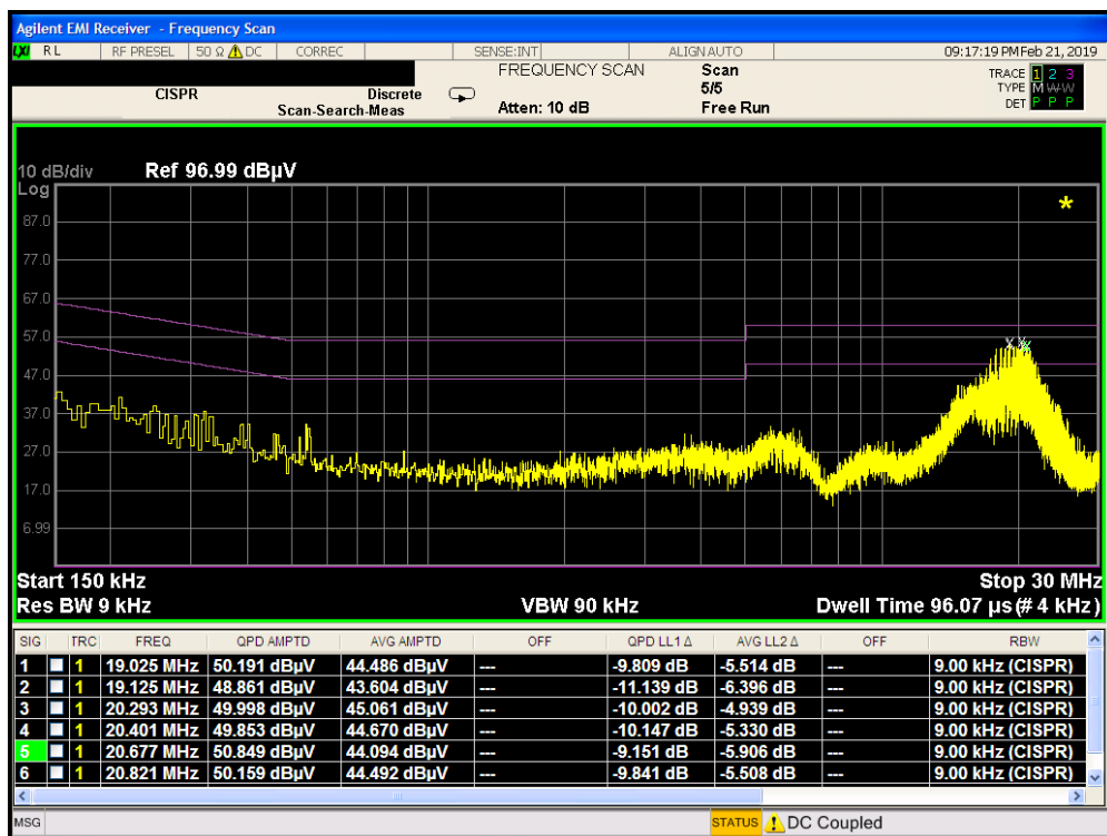
Plot 7-388. Line Conducted Plot with 802.11a UNII Band 2A (N)
