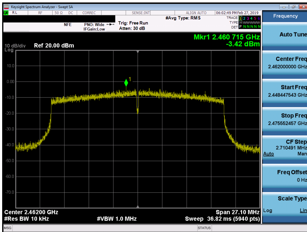
Plot 7-48. Power Spectral Density Plot SISO ANT2 (802.11ax – Ch. 11)
