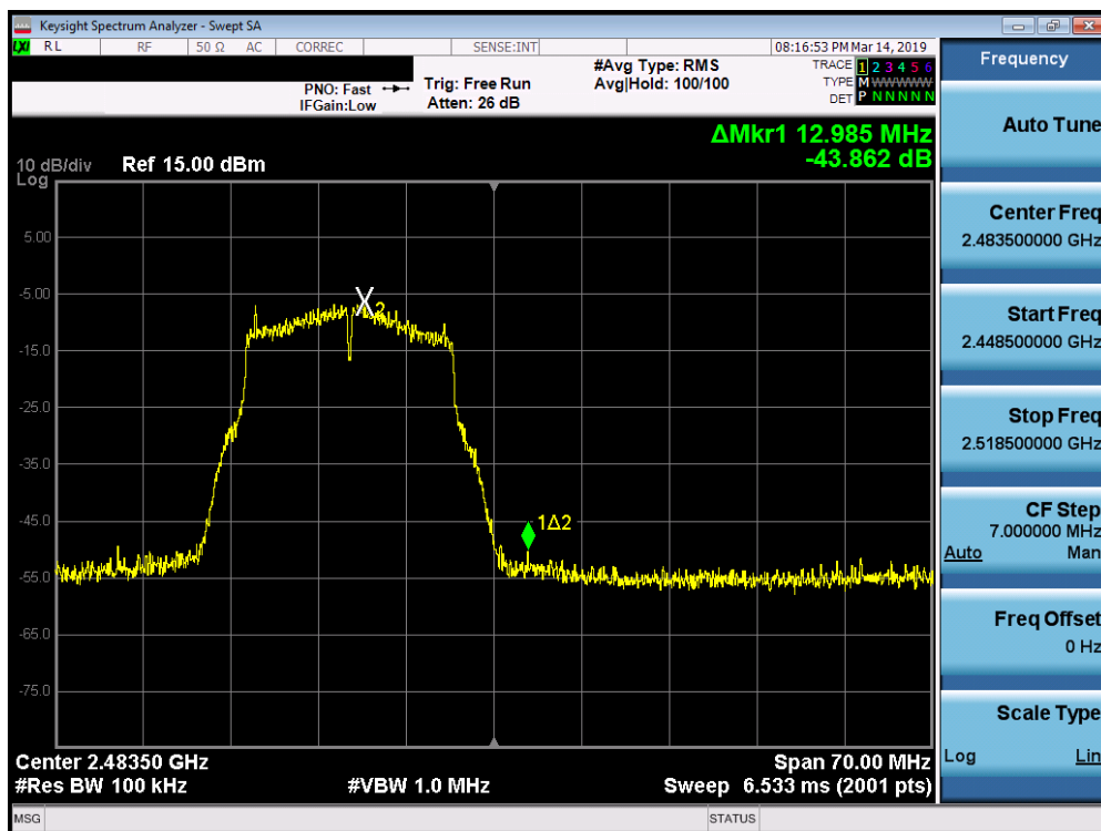
Plot 7-62. Band Edge Plot SISO ANT1 (802.11g – Ch. 13)
