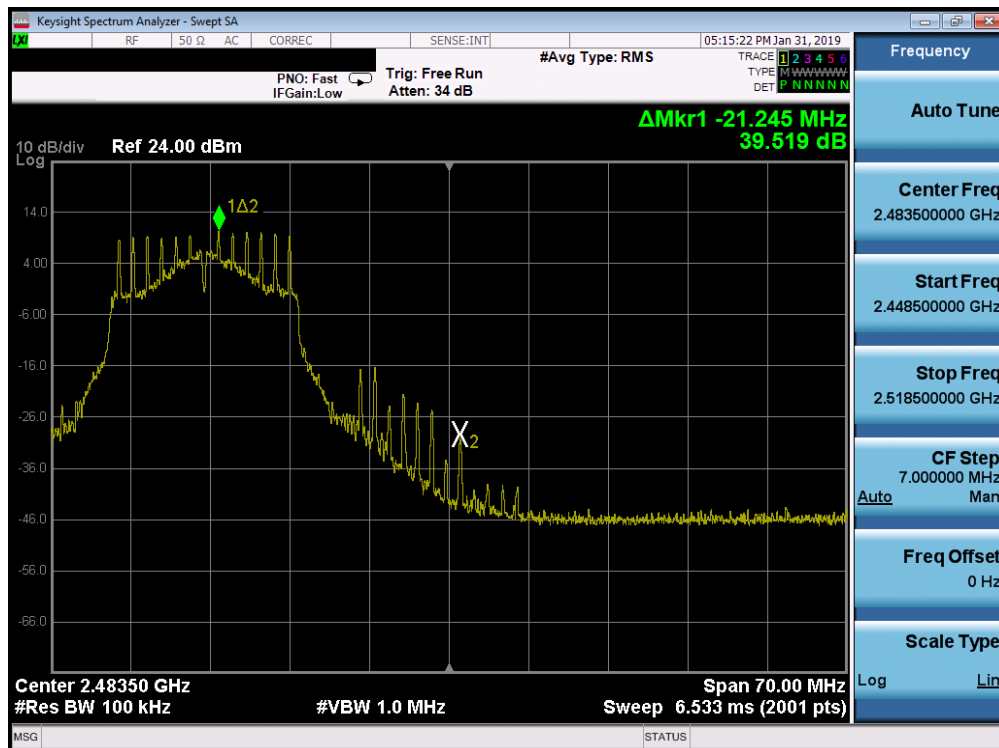
Plot 7-60. Band Edge Plot SISO ANT1 (802.11g - Ch. 11)
