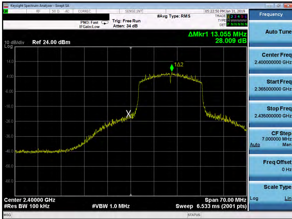
Plot 7-67. Band Edge Plot SISO ANT1 (802.11ax (2.4GHz) – Ch. 1)
