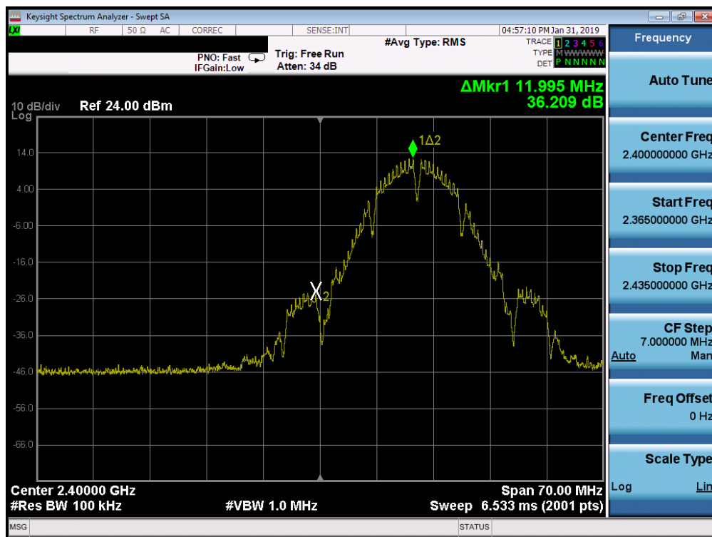
Plot 7-55. Band Edge Plot SISO ANT1 (802.11b - Ch. 1)
