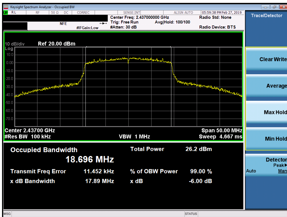
Plot 7-23. 6dB Bandwidth Plot SISO ANT2 (802.11ax - Ch. 6)
