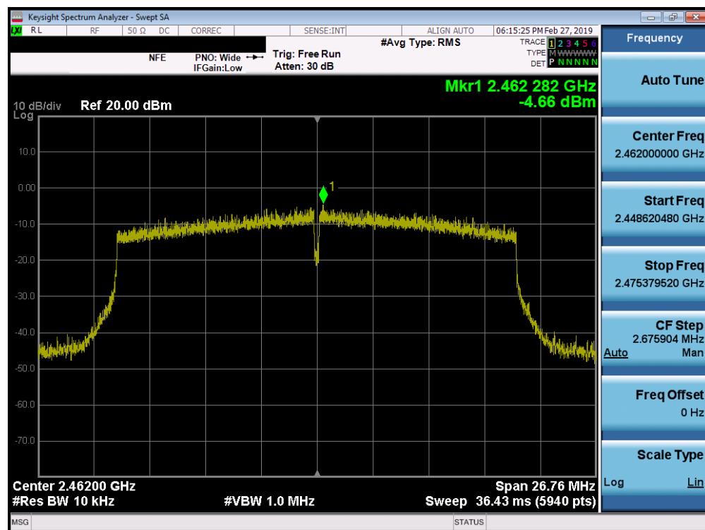
Plot 7-54. Power Spectral Density Plot MIMO ANT2 (802.11ax – Ch. 11)
