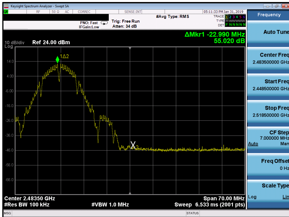
Plot 7-56. Band Edge Plot SISO ANT1 (802.11b - Ch. 11)
