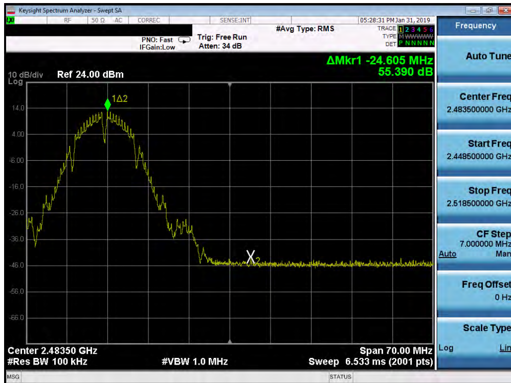
Plot 7-72. Band Edge Plot SISO ANT2 (802.11b - Ch. 11)
