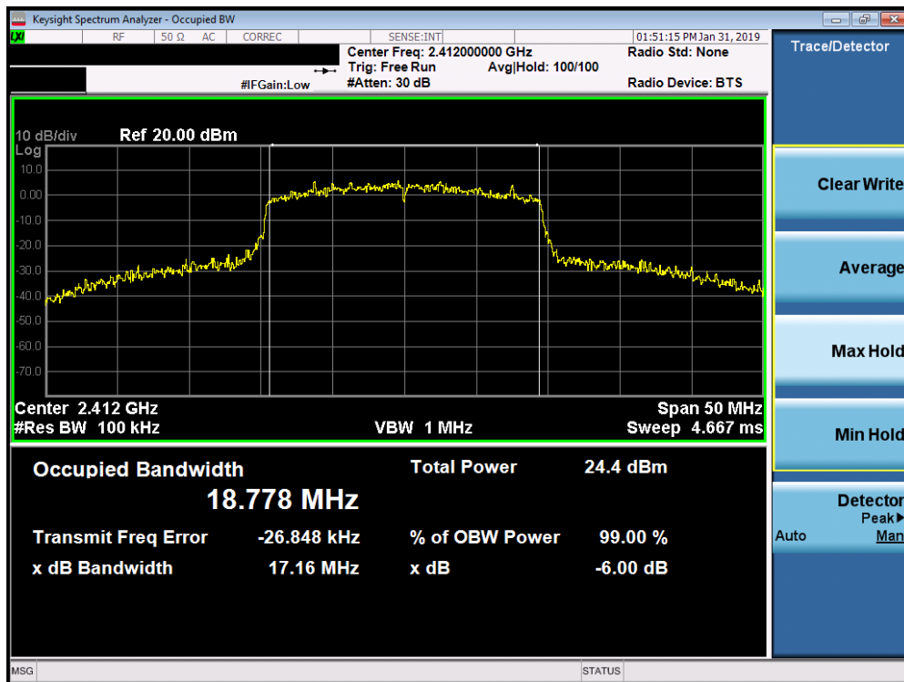
Plot 7-10. 6dB Bandwidth Plot SISO ANT1 (802.11ax - Ch. 1)
