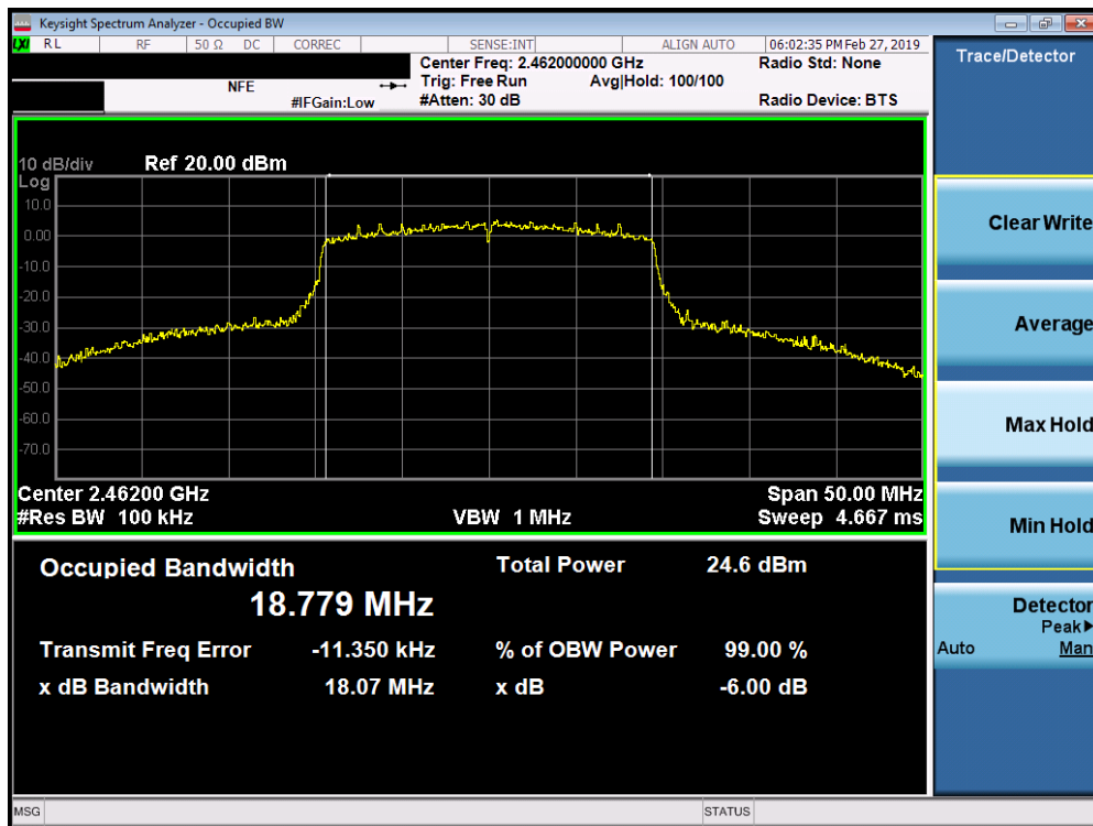
Plot 7-24. 6dB Bandwidth Plot SISO ANT2 (802.11ax – Ch. 11)
