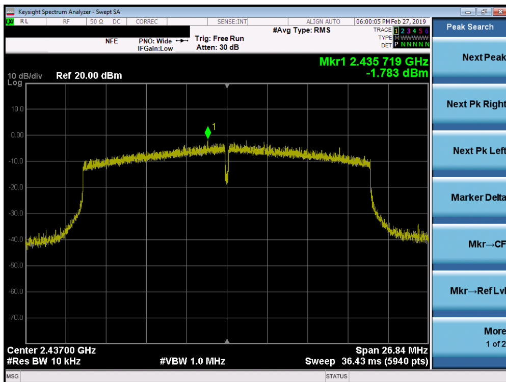
Plot 7-47. Power Spectral Density Plot SISO ANT2 (802.11ax – Ch. 6)
