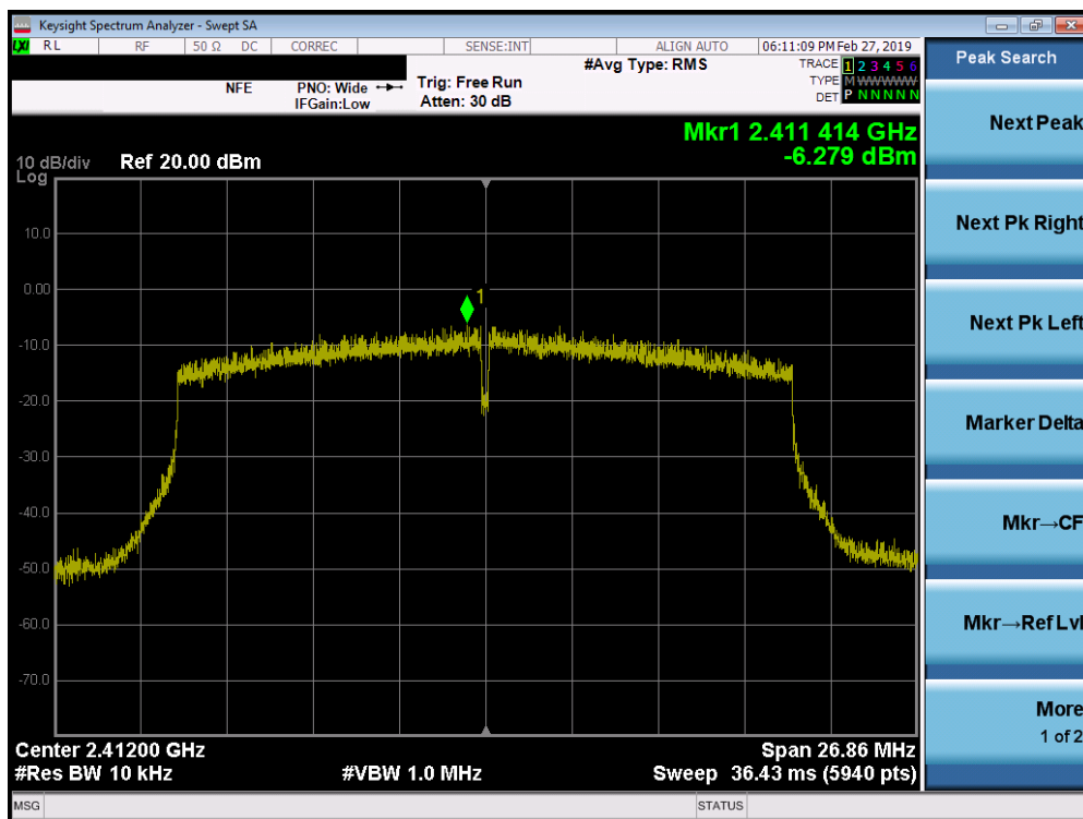
Plot 7-52. Power Spectral Density Plot MIMO ANT2 (802.11ax – Ch. 1)
