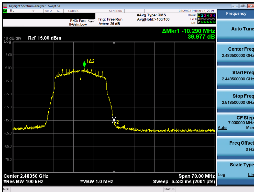
Plot 7-66. Band Edge Plot SISO ANT1 (802.11n (2.4GHz) – Ch. 13)
