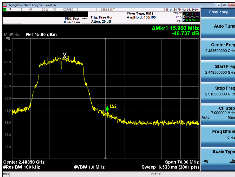
Plot 7-61. Band Edge Plot SISO ANT1 (802.11g – Ch. 12)
