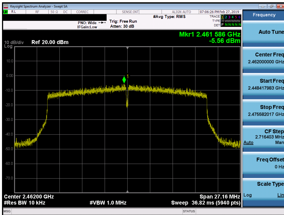
Plot 7-51. Power Spectral Density Plot MIMO ANT1 (802.11ax – Ch. 11)
