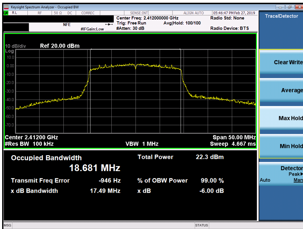
Plot 7-22. 6dB Bandwidth Plot SISO ANT2 (802.11ax - Ch. 1)
