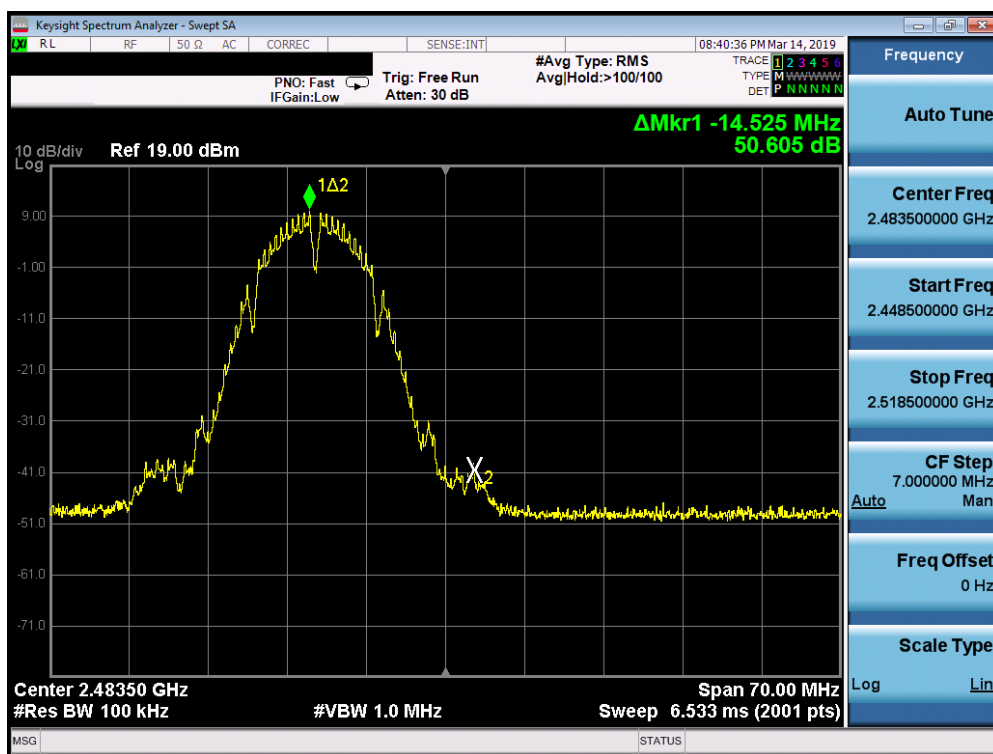
Plot 7-74. Band Edge Plot SISO ANT2 (802.11b - Ch. 13)
