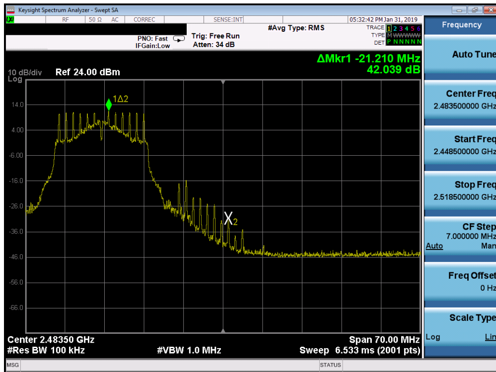
Plot 7-76. Band Edge Plot SISO ANT2 (802.11g - Ch. 11)
