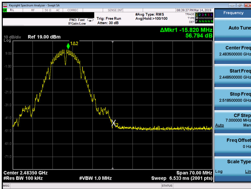
Plot 7-73. Band Edge Plot SISO ANT2 (802.11b - Ch. 12)
