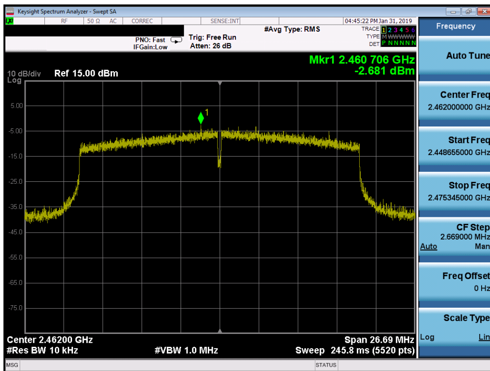
Plot 7-36. Power Spectral Density Plot SISO ANT1 (802.11ax – Ch. 11)
