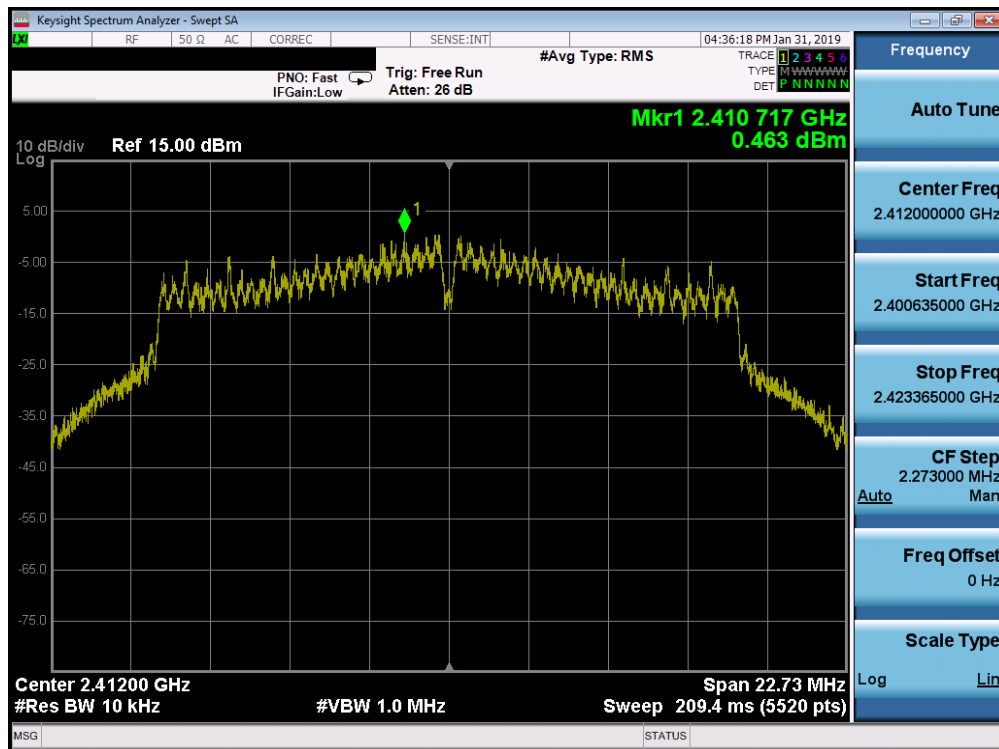
Plot 7-28. Power Spectral Density Plot SISO ANT1 (802.11g – Ch. 1)
