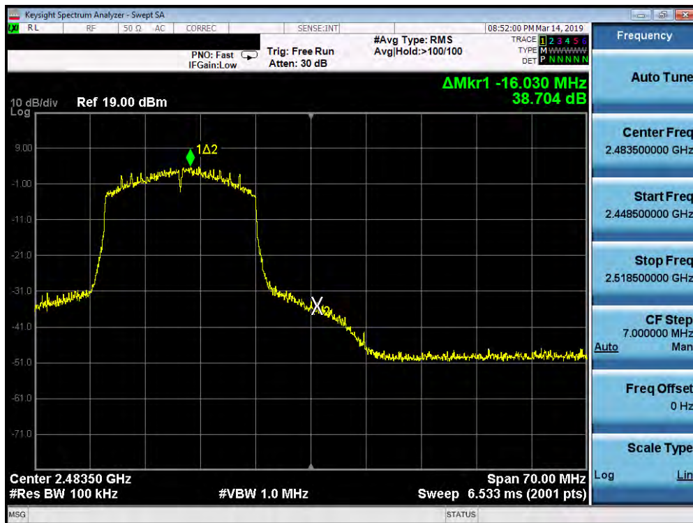
Plot 7-69. Band Edge Plot SISO ANT1 (802.11ax (2.4GHz) – Ch. 12)
