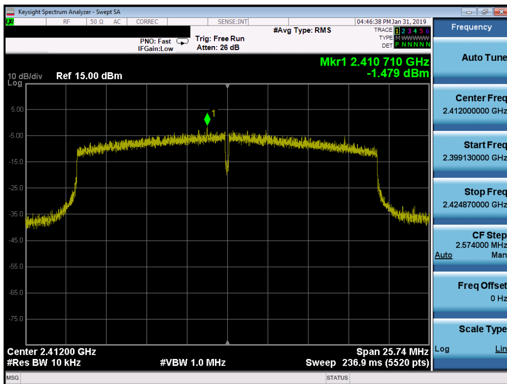
Plot 7-34. Power Spectral Density Plot SISO ANT1 (802.11ax – Ch. 1)
