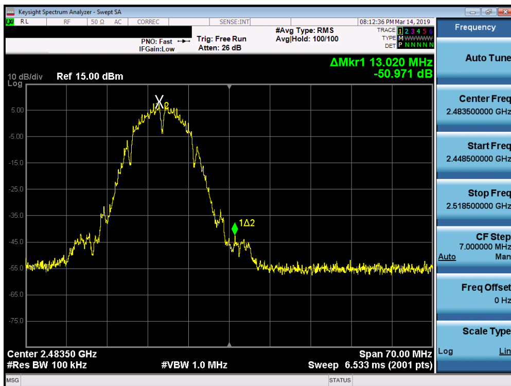
Plot 7-58. Band Edge Plot SISO ANT1 (802.11b – Ch. 13)
