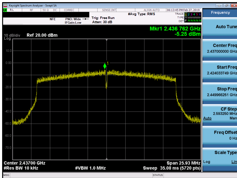
Plot 7-53. Power Spectral Density Plot MIMO ANT2 (802.11ax – Ch. 6)
