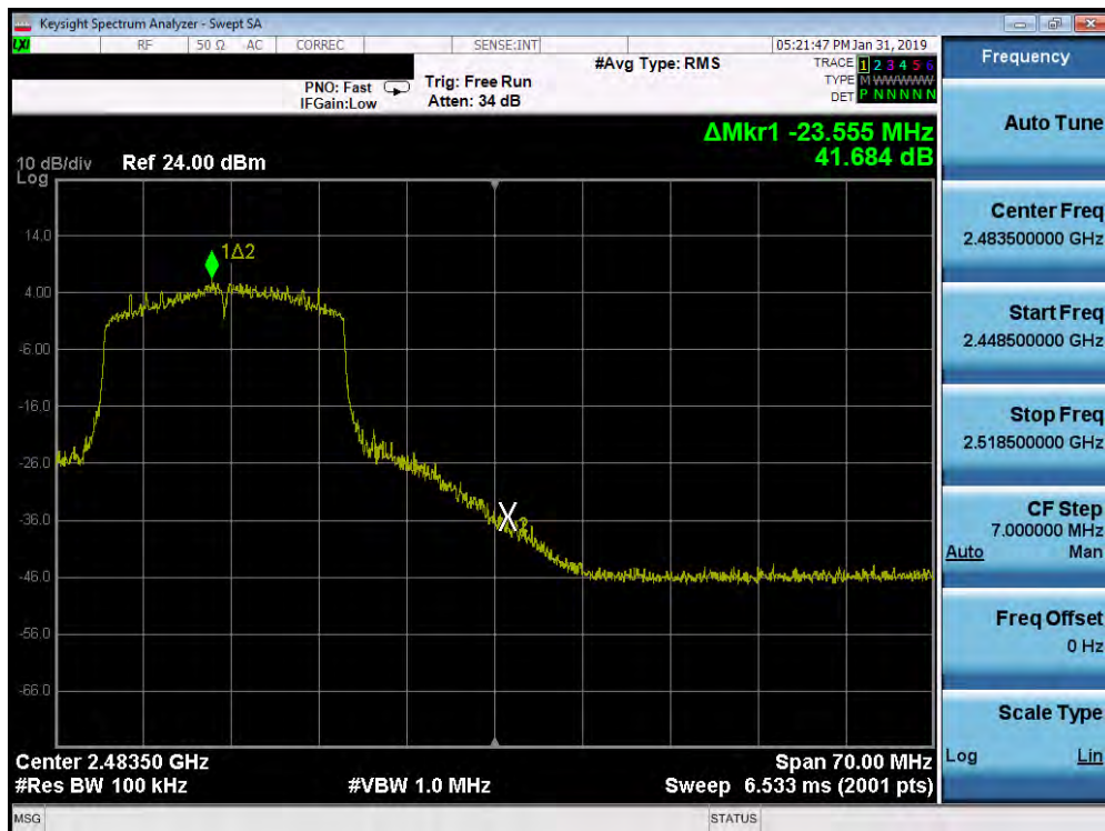
Plot 7-68. Band Edge Plot SISO ANT1 (802.11ax (2.4GHz) – Ch. 11)
