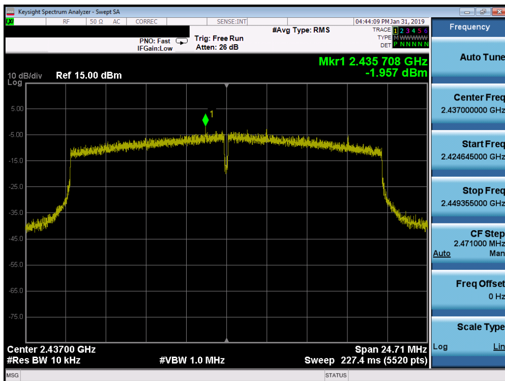
Plot 7-35. Power Spectral Density Plot SISO ANT1 (802.11ax – Ch. 6)
