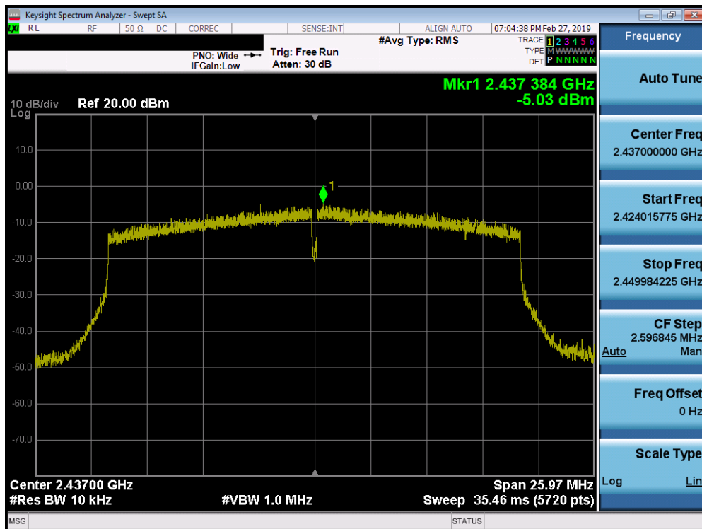
Plot 7-50. Power Spectral Density Plot MIMO ANT1 (802.11ax – Ch. 6)
