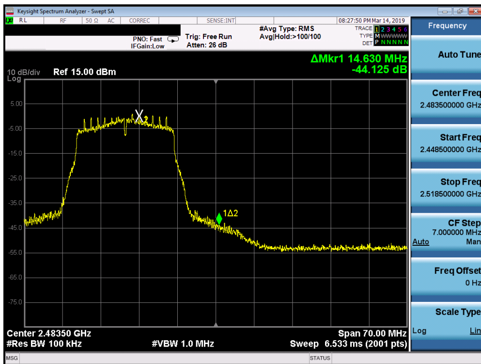
Plot 7-65. Band Edge Plot SISO ANT1 (802.11n (2.4GHz) – Ch. 12)
