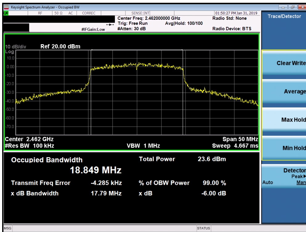
Plot 7-12. 6dB Bandwidth Plot SISO ANT1 (802.11ax – Ch. 11)
