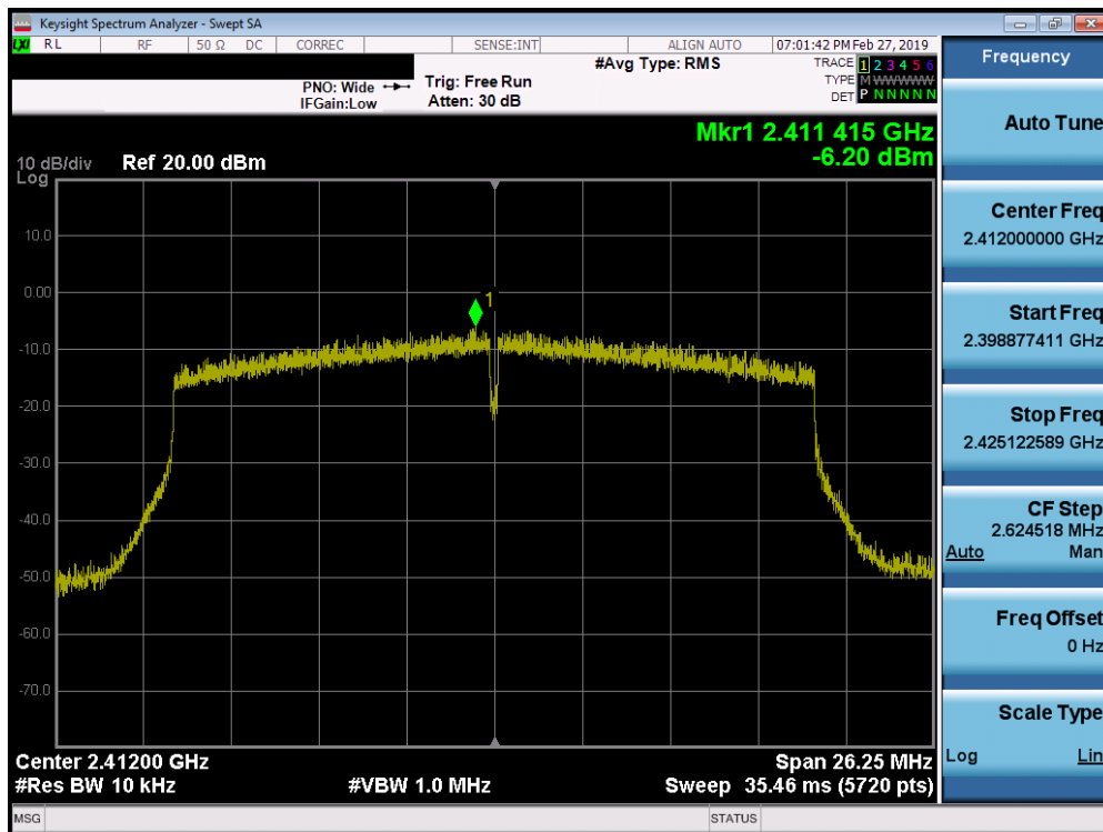
Plot 7-49. Power Spectral Density Plot MIMO ANT1 (802.11ax – Ch. 1)
