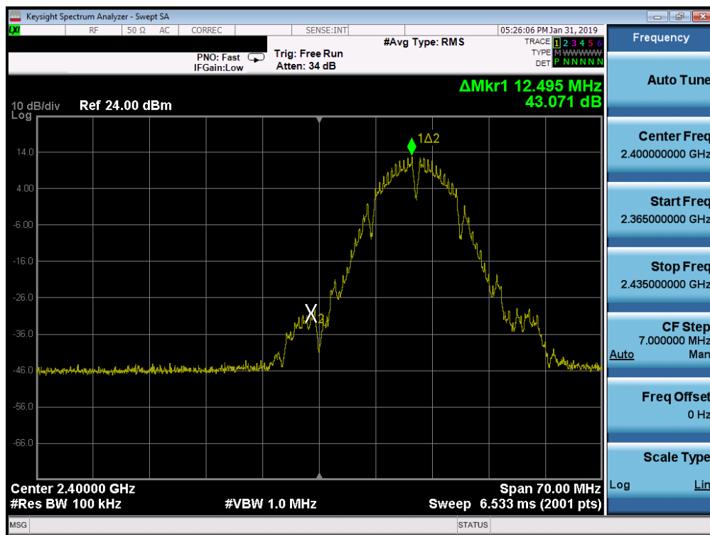
Plot 7-71. Band Edge Plot SISO ANT2 (802.11b - Ch. 1)
