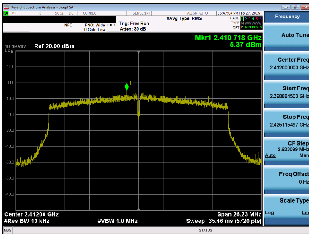
Plot 7-46. Power Spectral Density Plot SISO ANT2 (802.11ax – Ch. 1)
