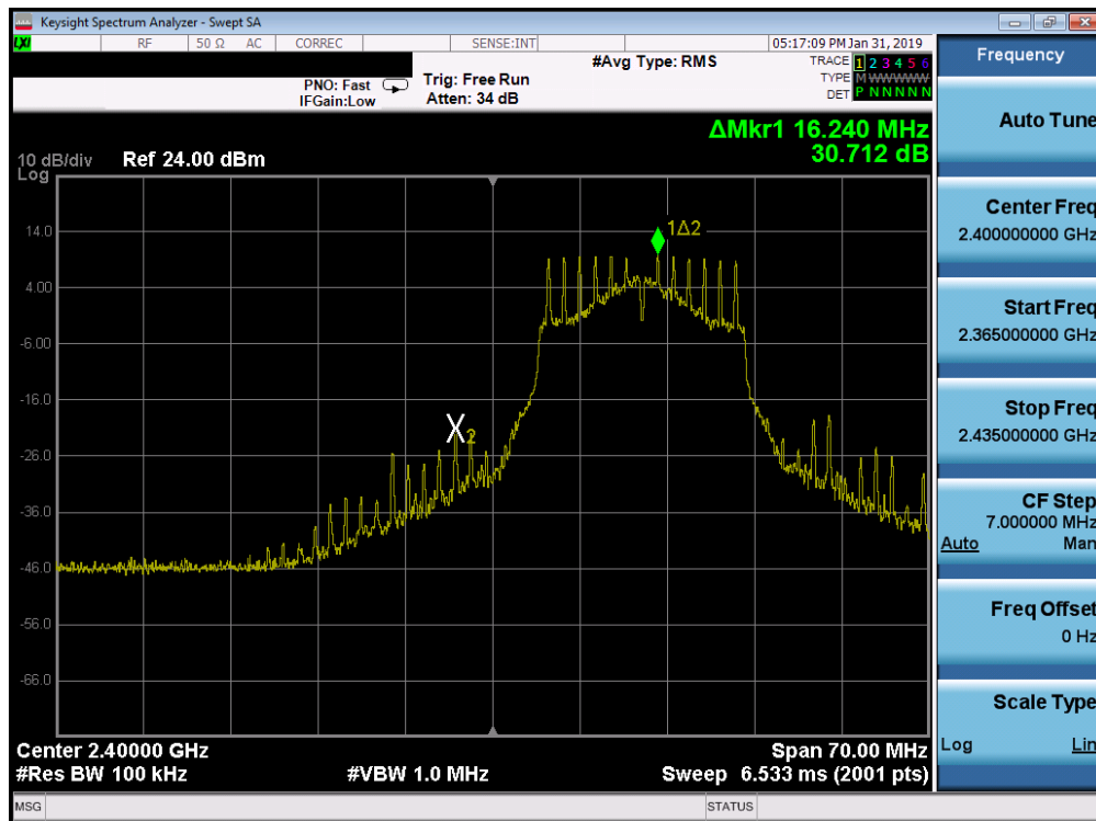
Plot 7-59. Band Edge Plot SISO ANT1 (802.11g- Ch. 1)
