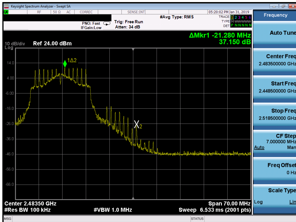
Plot 7-64. Band Edge Plot SISO ANT1 (802.11n (2.4GHz) – Ch. 11)
