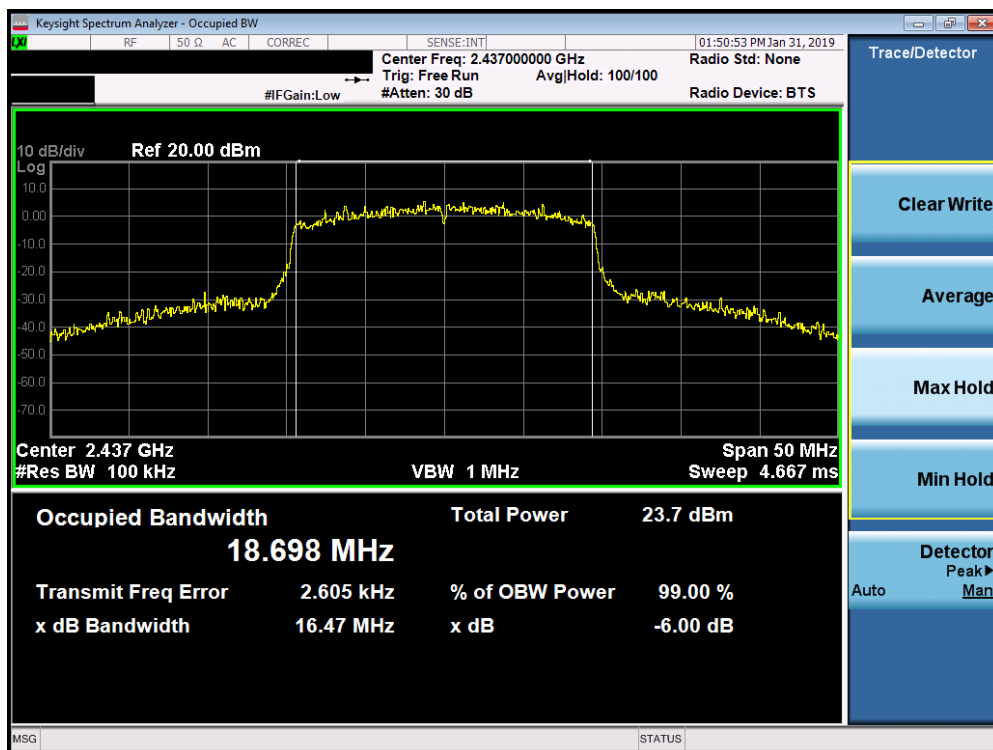
Plot 7-11. 6dB Bandwidth Plot SISO ANT1 (802.11ax - Ch. 6)
