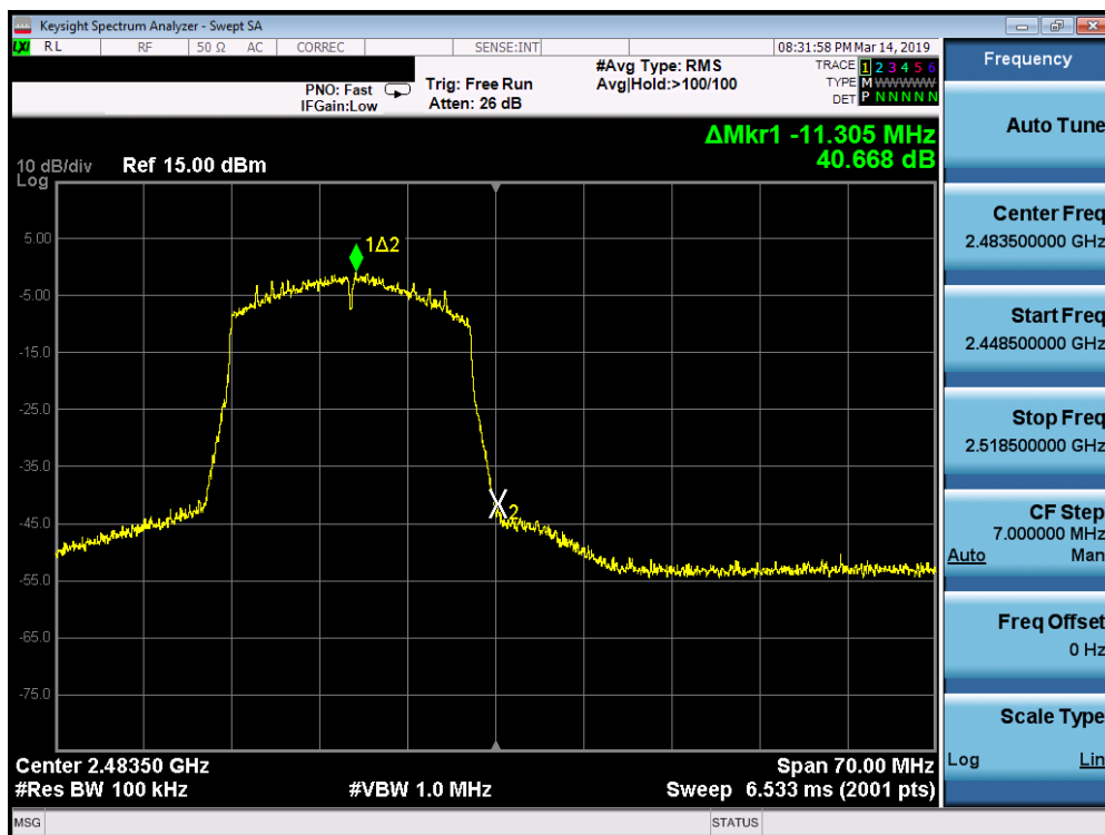
Plot 7-70. Band Edge Plot SISO ANT1 (802.11ax (2.4GHz) – Ch. 13)
