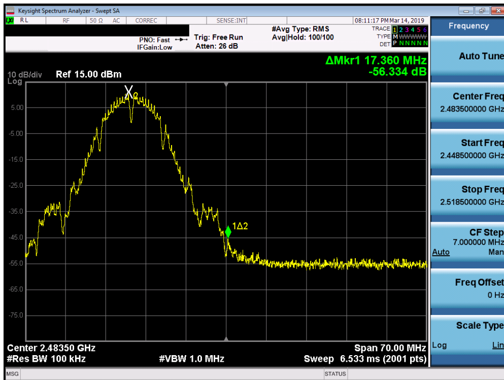
Plot 7-57. Band Edge Plot SISO ANT1 (802.11b – Ch. 12)
