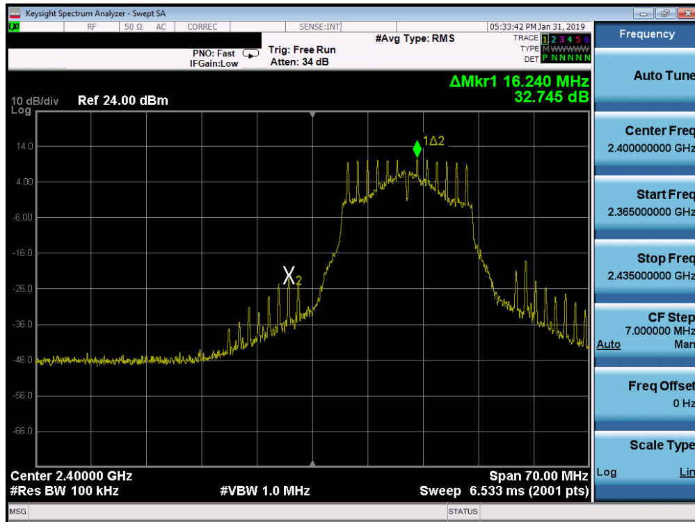
Plot 7-75. Band Edge Plot SISO ANT2 (802.11g- Ch. 1)
