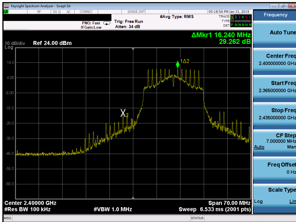
Plot 7-63. Band Edge Plot SISO ANT1 (802.11n (2.4GHz) – Ch. 1)
