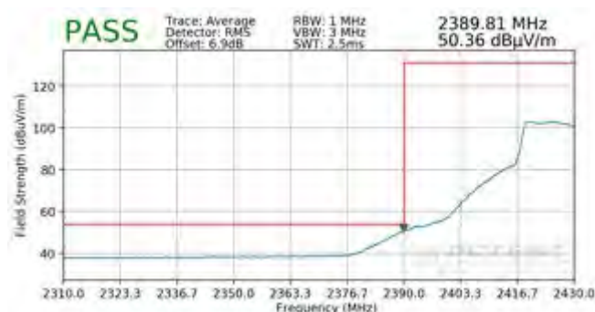
Plot 7-153. Radiated Restricted Lower Band Edge Measurement MIMO (Average)
