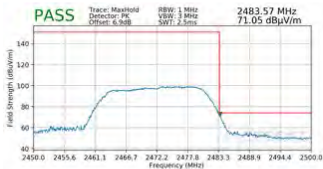
Plot 7-166. Radiated Restricted Band Edge Measurement MIMO with WCP (Peak)
