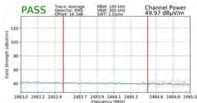
Plot 7-141. Radiated Restricted Upper Band Edge Measurement SISO ANT1 (Average)
