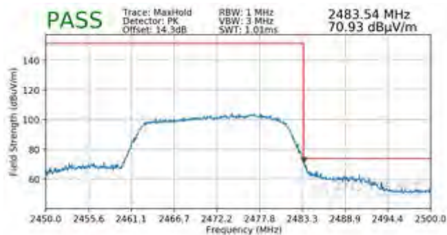
Plot 7-164. Radiated Restricted Upper Band Edge Measurement SISO ANT1 (Peak)
