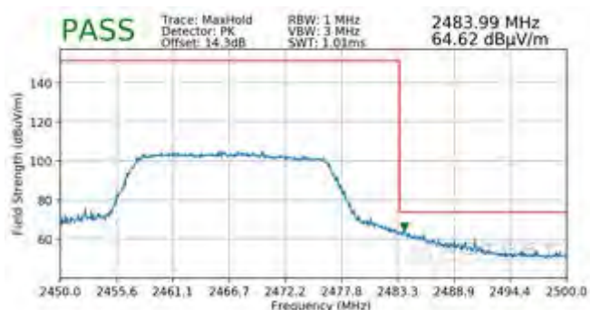
Plot 7-162. Radiated Restricted Upper Band Edge Measurement SISO ANT1 (Peak)
