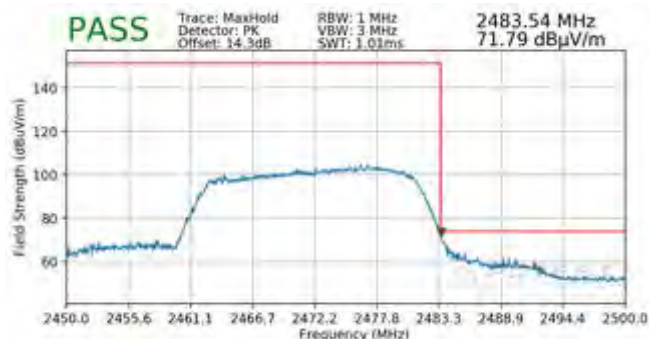
Plot 7-128. Radiated Restricted Upper Band Edge Measurement SISO ANT1 (Peak)
