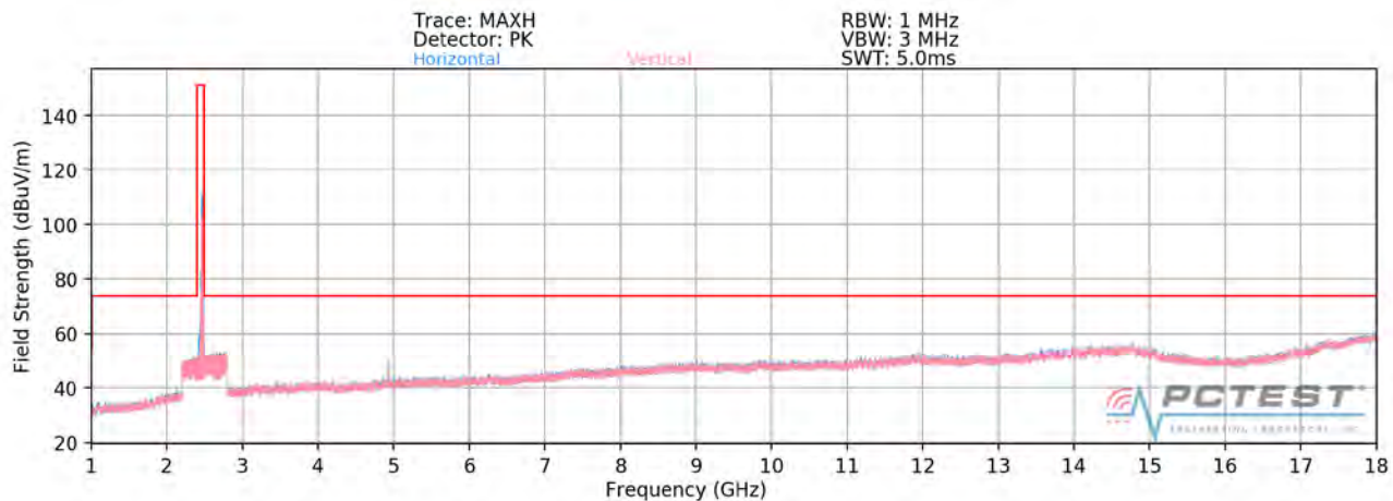
Plot 7-109. Radiated Spurious Plot above 1GHz MIMO/CDD (802.11g – Ch. 11 – CLOSED)
