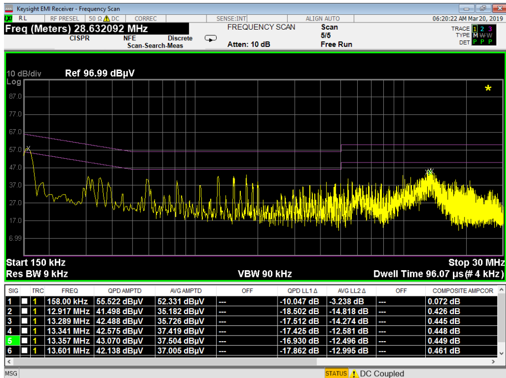
Plot 7-171. Line Conducted Plot with 802.11b and WCP (L1)
