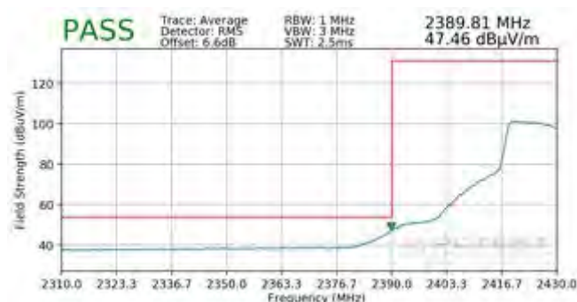
Plot 7-117. Radiated Restricted Lower Band Edge Measurement SISO ANT1 (Average)
