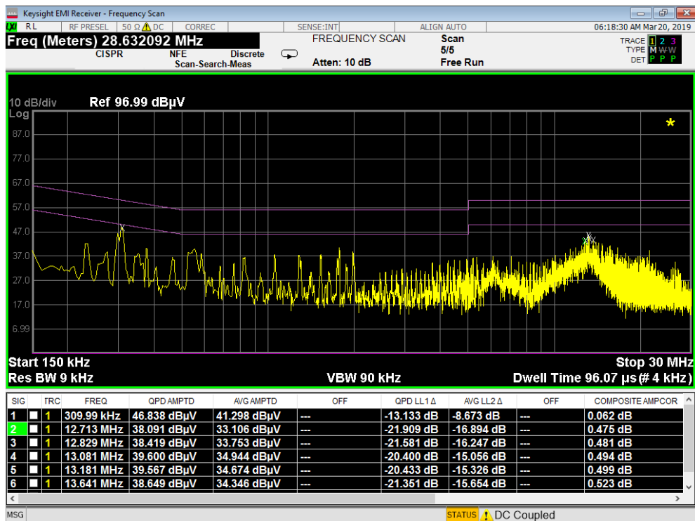
Plot 7-172. Line Conducted Plot with 802.11b and WCP (N)
