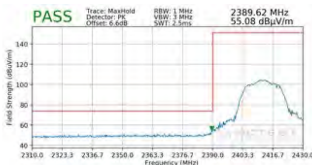
Plot 7-132. Radiated Restricted Lower Band Edge Measurement SISO ANT2 (Peak)
