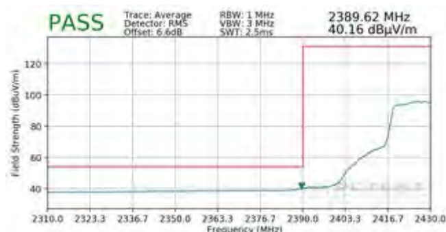
Plot 7-137. Radiated Restricted Lower Band Edge Measurement SISO ANT2 (Average)
