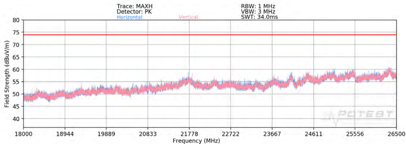
Plot 7-110. Radiated Spurious Plot above 18GHz MIMO/CDD – CLOSED
