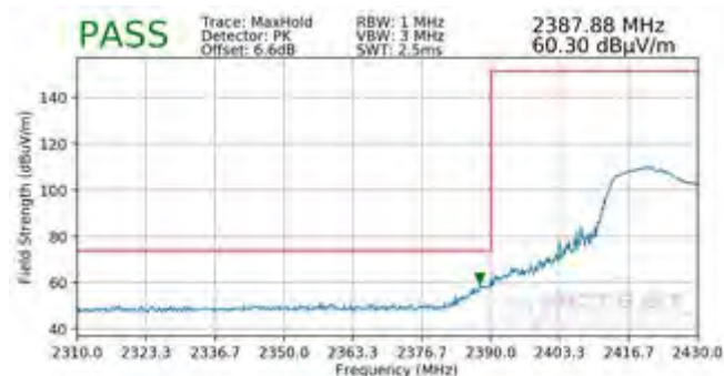
Plot 7-116. Radiated Restricted Lower Band Edge Measurement SISO ANT1 (Peak)
