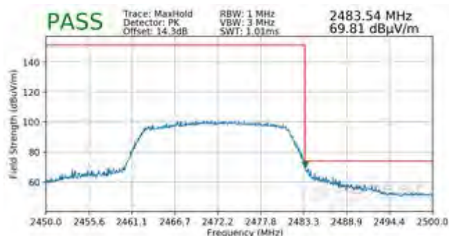
Plot 7-144. Radiated Restricted Upper Band Edge Measurement SISO ANT1 (Peak)
