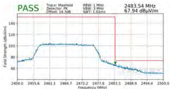
Plot 7-126. Radiated Restricted Upper Band Edge Measurement SISO ANT1 (Peak)
