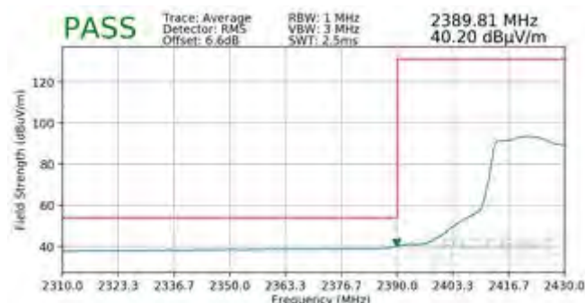
Plot 7-135. Radiated Restricted Lower Band Edge Measurement SISO ANT2 (Average)
