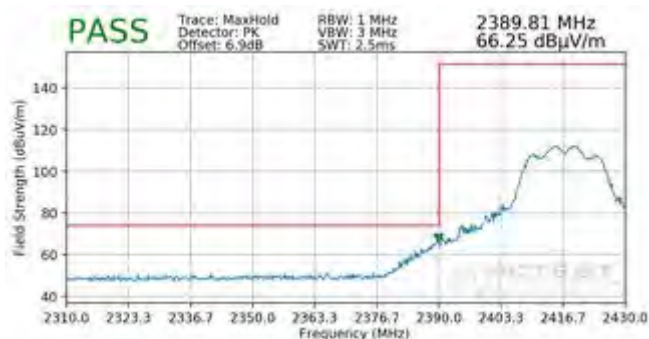
Plot 7-150. Radiated Restricted Lower Band Edge Measurement MIMO (Peak)
