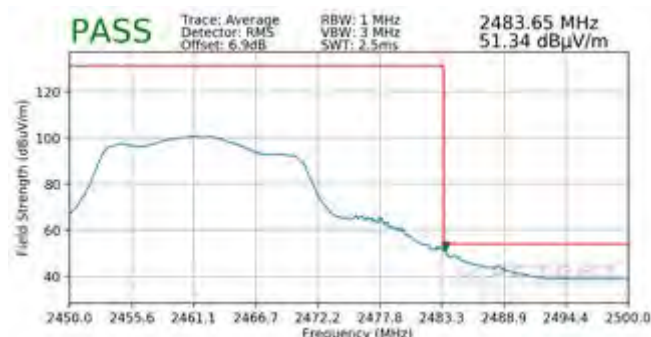
Plot 7-159. Radiated Restricted Upper Band Edge Measurement MIMO (Average)
