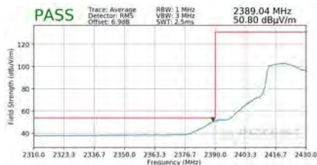
Plot 7-151. Radiated Restricted Lower Band Edge Measurement MIMO (Average)
