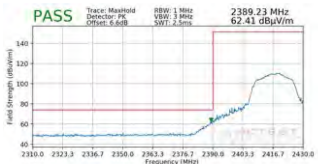
Plot 7-114. Radiated Restricted Lower Band Edge Measurement SISO ANT1 (Peak)
