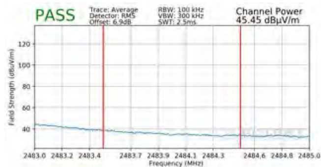
Plot 7-165. Radiated Restricted Band Edge Measurement MIMO with WCP (Average)
