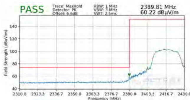
Plot 7-134. Radiated Restricted Lower Band Edge Measurement SISO ANT2 (Peak)
