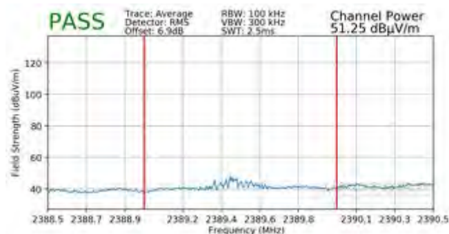
Plot 7-147. Radiated Restricted Lower Band Edge Measurement MIMO (Average)
