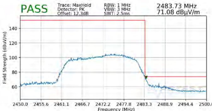
Plot 7-130. Radiated Restricted Band Edge Measurement SISO ANT1 with WCP (Peak)
