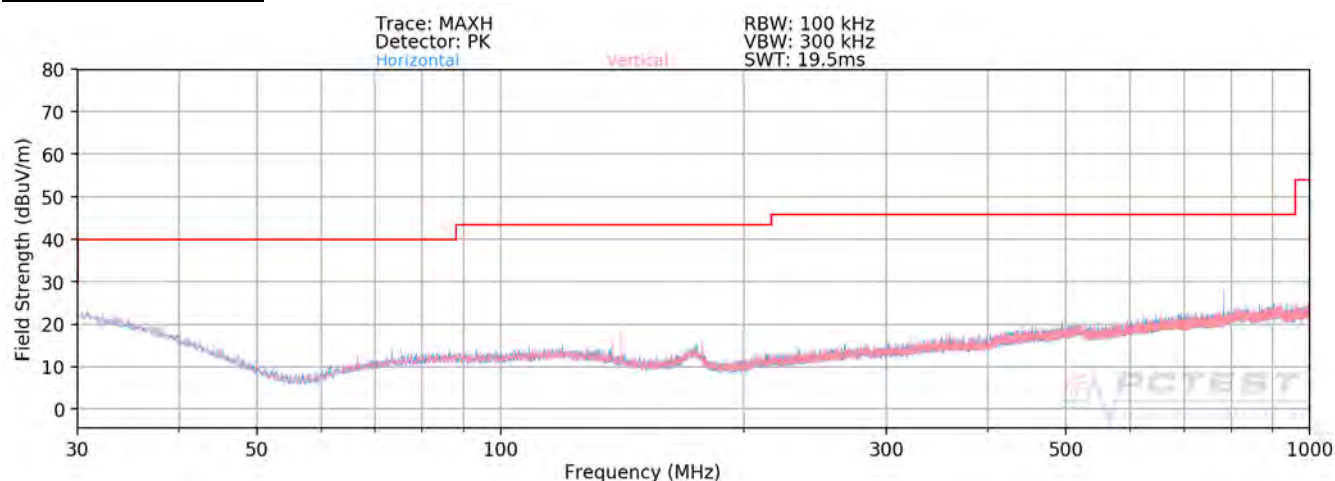
Plot 7-168. Radiated Spurious Plot below 1GHz SISO ANT2 - CLOSED
