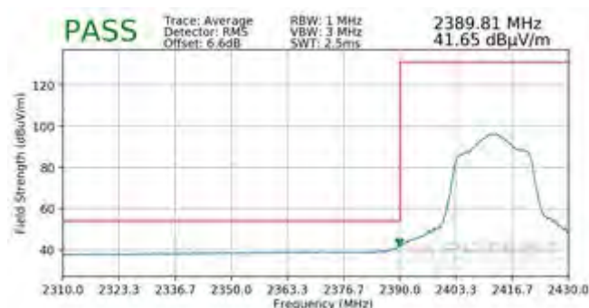
Plot 7-131. Radiated Restricted Lower Band Edge Measurement SISO ANT2 (Average)
