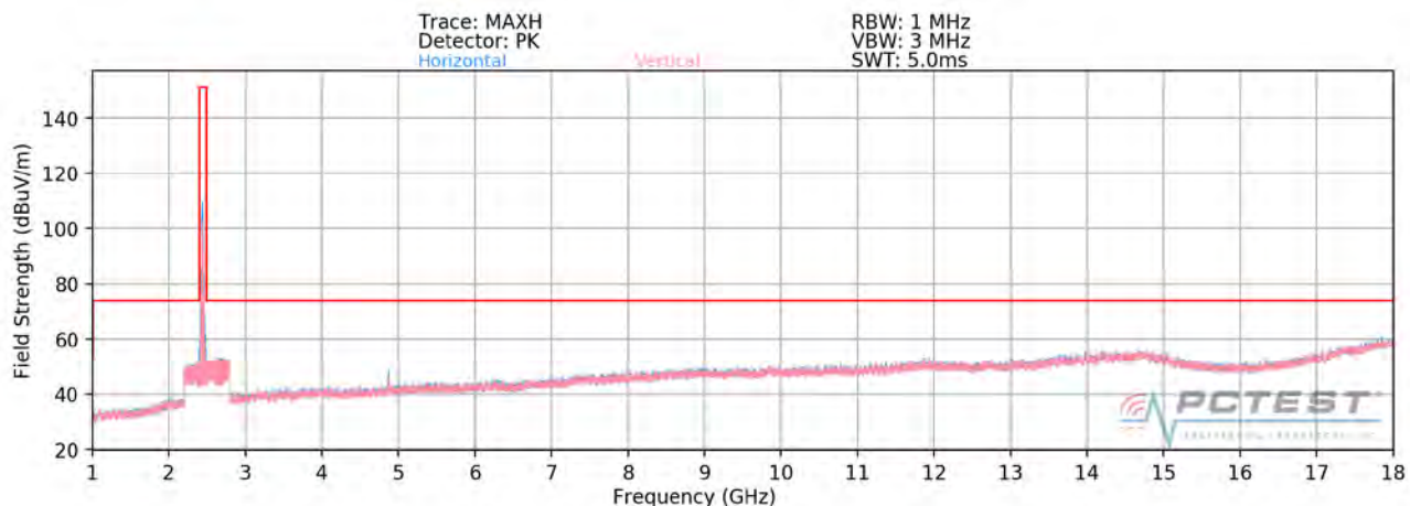
Plot 7-108. Radiated Spurious Plot above 1GHz MIMO/CDD (802.11g – Ch. 6 – CLOSED)
