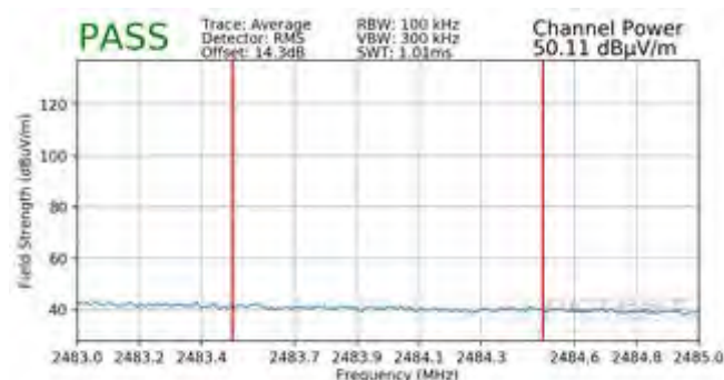
Plot 7-161. Radiated Restricted Upper Band Edge Measurement SISO ANT1 (Average)
