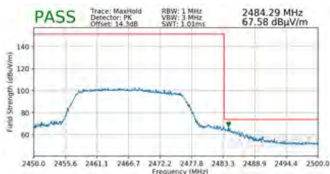
Plot 7-142. Radiated Restricted Upper Band Edge Measurement SISO ANT1 (Peak)
