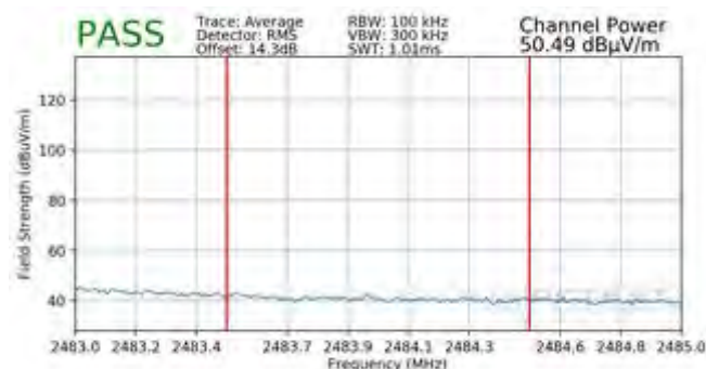
Plot 7-143. Radiated Restricted Upper Band Edge Measurement SISO ANT1 (Average)
