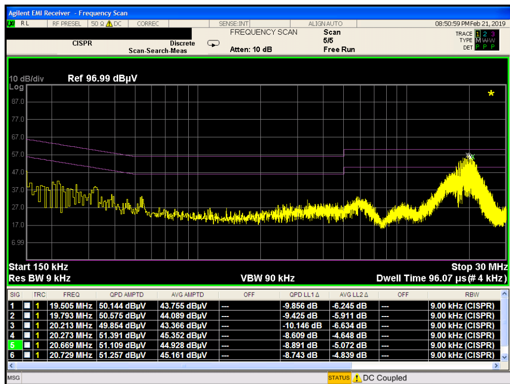
Plot 7-170. Line Conducted Plot with 802.11b (N)
