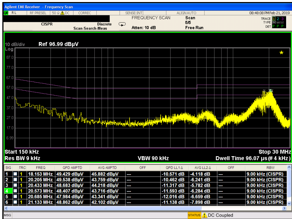
Plot 7-169. Line Conducted Plot with 802.11b (L1)
