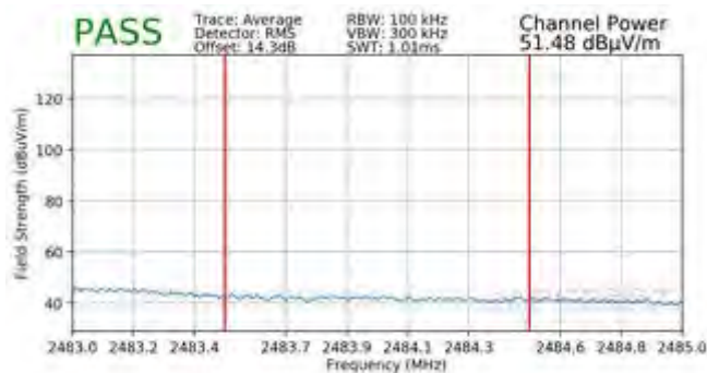
Plot 7-163. Radiated Restricted Upper Band Edge Measurement SISO ANT1 (Average)
