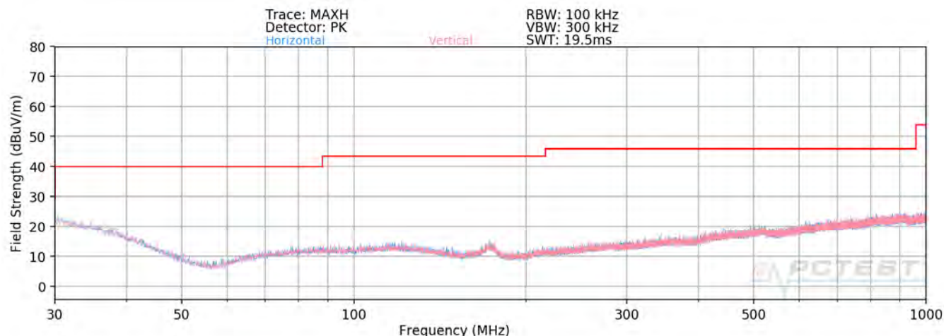
Plot 7-167. Radiated Spurious Plot below 1GHz SISO ANT1 - CLOSED
