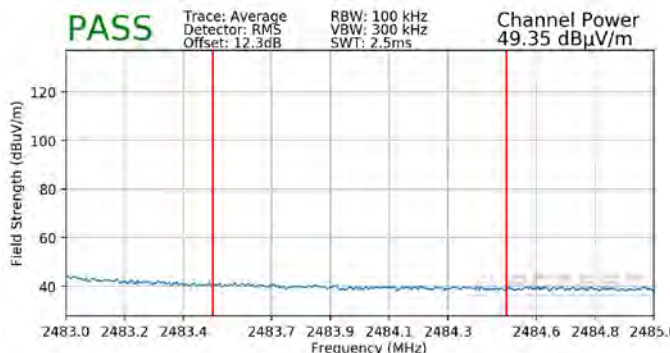
Plot 7-129. Radiated Restricted Band Edge Measurement SISO ANT1 with WCP (Average)
