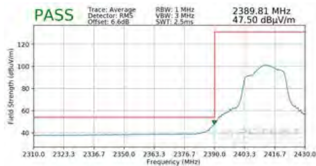
Plot 7-111. Radiated Restricted Lower Band Edge Measurement SISO ANT1 (Average)
