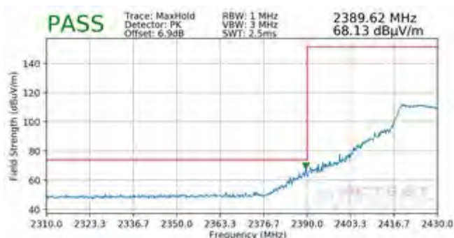
Plot 7-154. Radiated Restricted Lower Band Edge Measurement MIMO (Peak)
