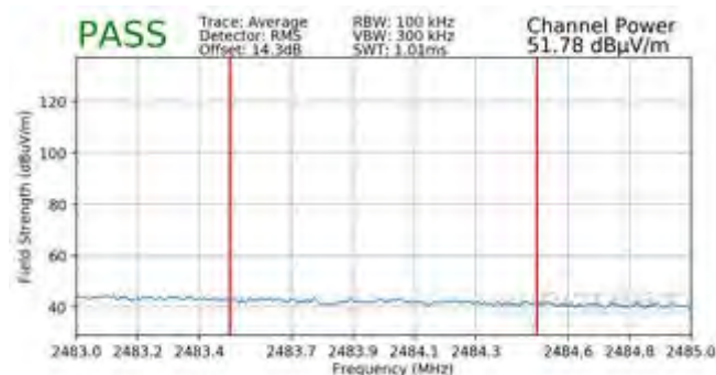
Plot 7-125. Radiated Restricted Upper Band Edge Measurement SISO ANT1 (Average)
