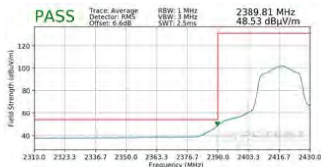
Plot 7-113. Radiated Restricted Lower Band Edge Measurement SISO ANT1 (Average)
