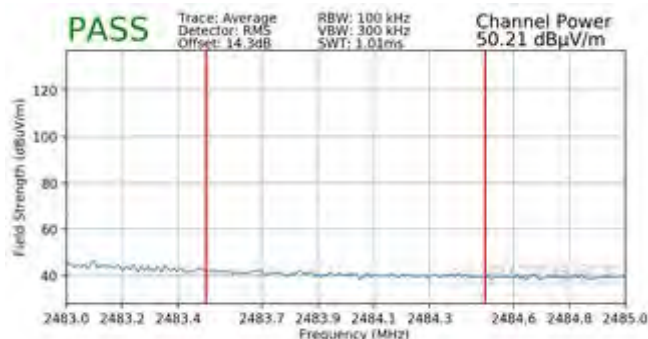
Plot 7-127. Radiated Restricted Upper Band Edge Measurement SISO ANT1 (Average)
