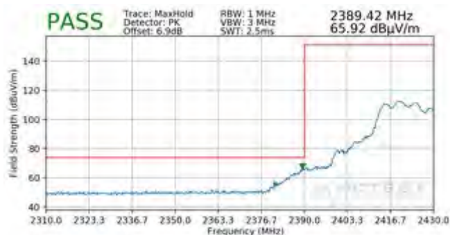
Plot 7-152. Radiated Restricted Lower Band Edge Measurement MIMO (Peak)
