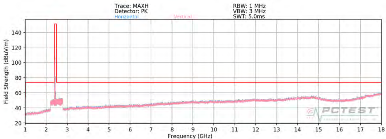
Plot 7-107. Radiated Spurious Plot above 1GHz MIMO/CDD (802.11g – Ch. 1 – CLOSED)
