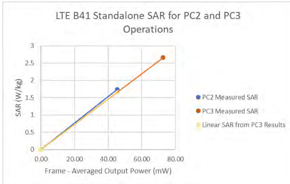
Figure 14-5 LTE Band 41 Standalone 10g Linearity
