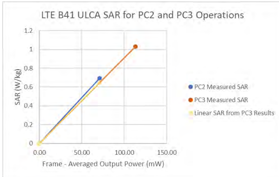
Figure 14-4 LTE Band 41 ULCA 1g Body Linearity
