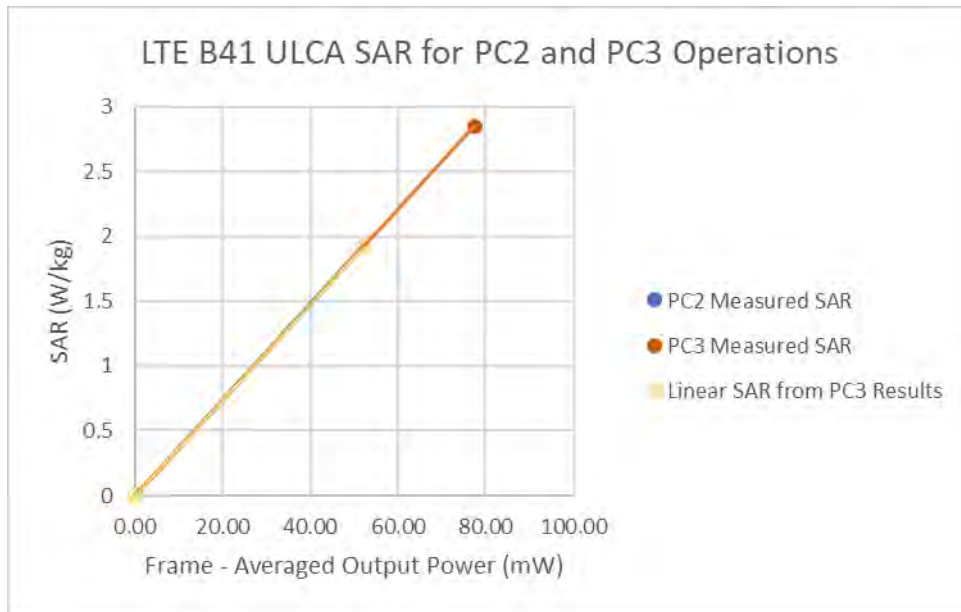
Figure 14-6 LTE Band 41 ULCA 10g Linearity
