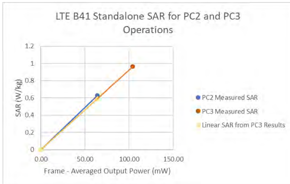
Figure 14-3 LTE Band 41 Standalone 1g Body Linearity
