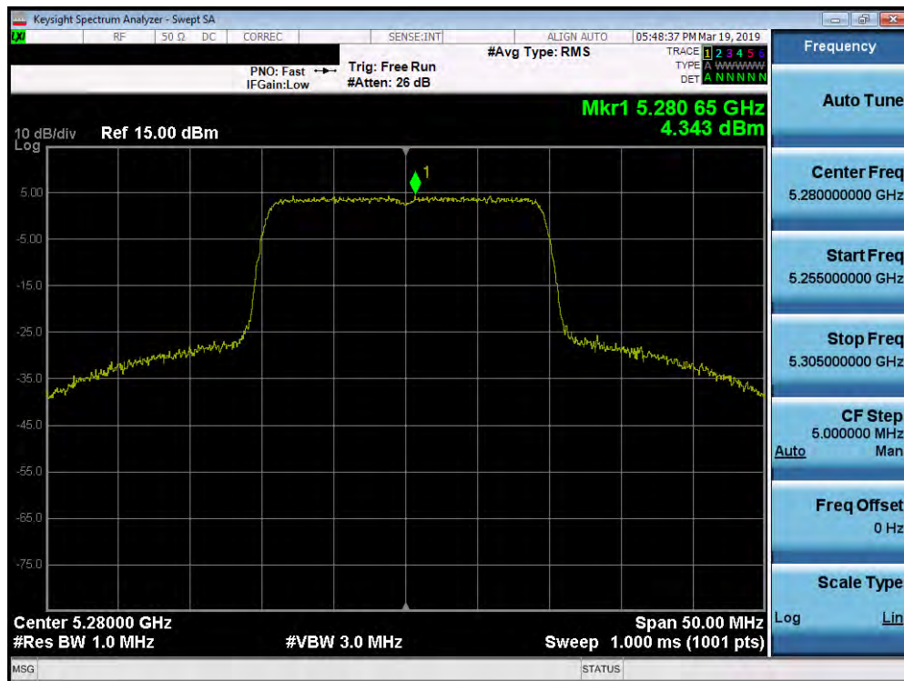
Plot 7-143. Power Spectral Density Plot SISO ANT1 (20MHz BW 802.11ax – 242 Tones (UNII Band 2A) – Ch. 56)
