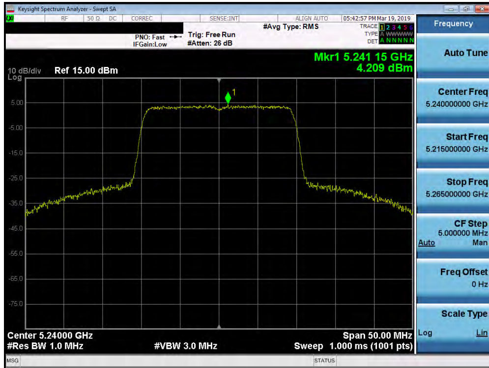
Plot 7-138. Power Spectral Density Plot SISO ANT1 (20MHz BW 802.11ax – 242 Tones (UNII Band 1) – Ch. 48)
