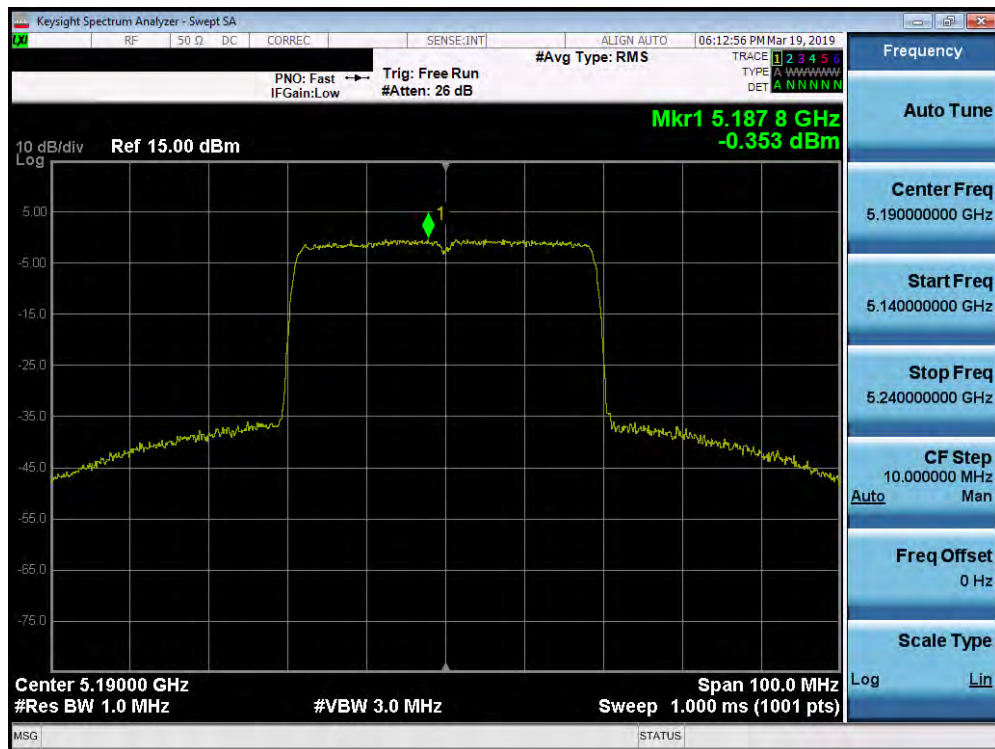
Plot 7-139. Power Spectral Density Plot SISO ANT1 (40MHz BW 802.11ax – 484 Tones (UNII Band 1) – Ch. 38)
