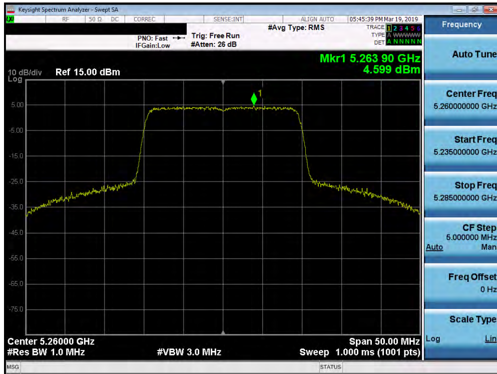
Plot 7-142. Power Spectral Density Plot SISO ANT1 (20MHz BW 802.11ax – 242 Tones (UNII Band 2A) – Ch. 52)
