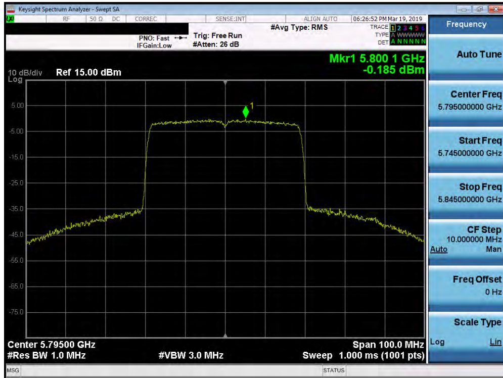
Plot 7-161. Power Spectral Density Plot SISO ANT1 (40MHz BW 802.11ax – 484 Tones (UNII Band 3) – Ch. 159)
