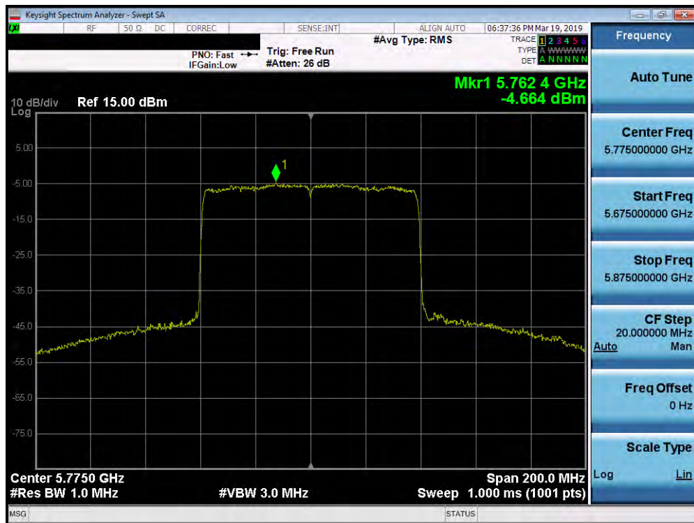
Plot 7-162. Power Spectral Density Plot SISO ANT1 (80MHz BW 802.11ax – 996 Tones (UNII Band 3) – Ch. 155)
