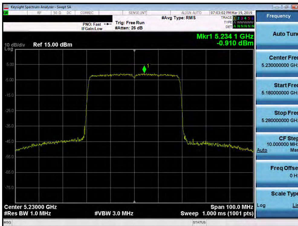
Plot 7-194. Power Spectral Density Plot SISO ANT2 (40MHz BW 802.11ax – 484 Tones (UNII Band 1) – Ch. 46)
