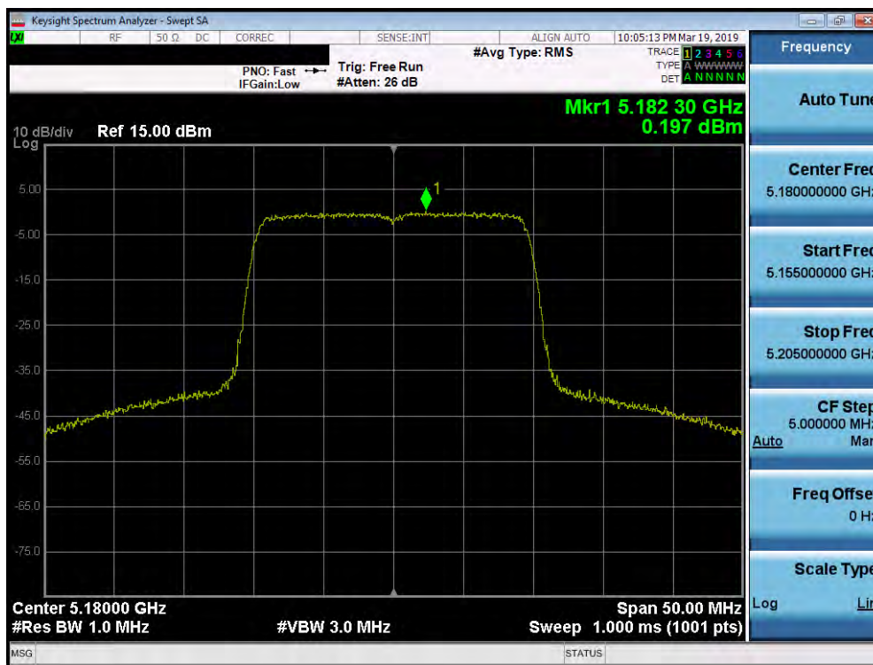
Plot 7-271. Power Spectral Density Plot MIMO ANT1 (20MHz BW 802.11ax – 242 Tones (UNII Band 1) – Ch. 36)
