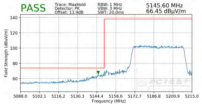
Plot 7-412. Radiated Lower Band Edge Plot SISO ANT1 (Peak - UNII Band 1 - 484 Tones)
