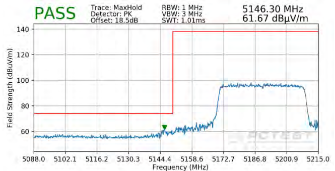
Plot 7-454. Radiated Lower Band Edge Plot SISO ANT2 (Peak - UNII Band 1 - 484 Tones)
