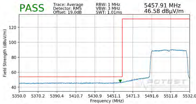
Plot 7-457. Radiated Lower Band Edge Plot SISO ANT2 (Average – UNII Band 2C – 484 Tones)
