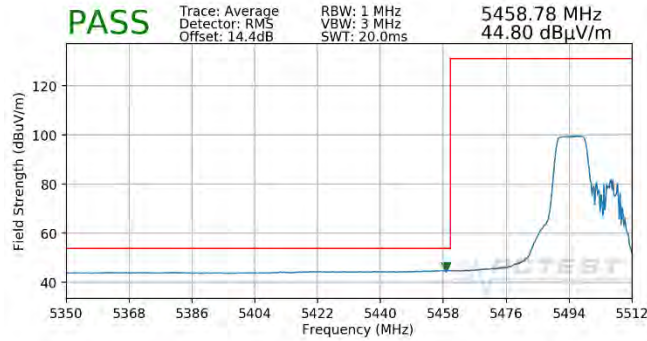
Plot 7-408. Radiated Lower Band Edge Plot SISO ANT1 (Average - UNII Band 2C - 106 Tones)
