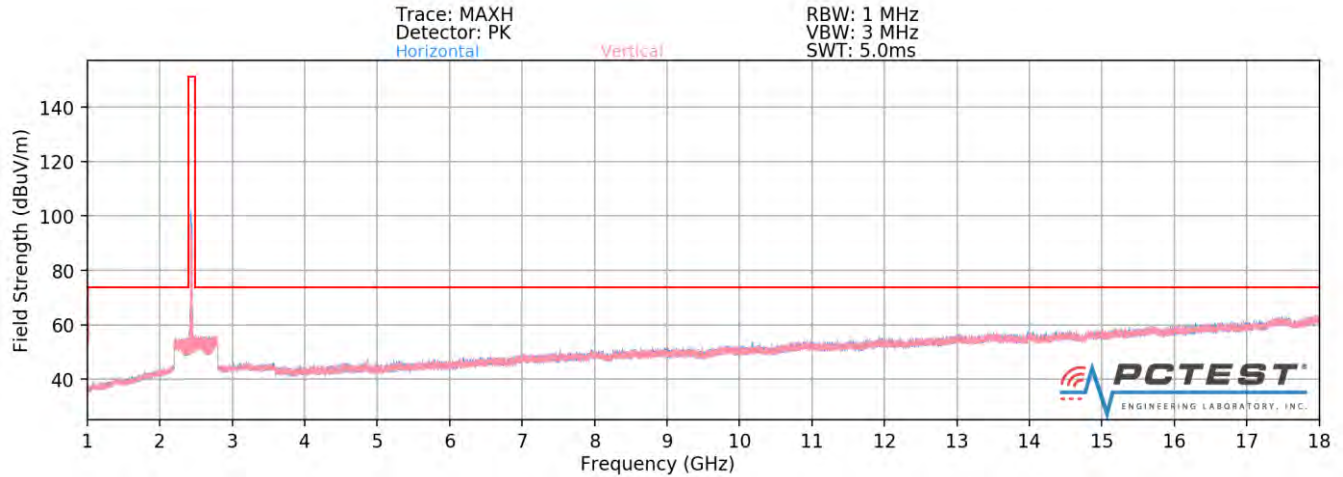
Plot 7-74. Radiated Spurious Plot above 1GHz SISO ANT2 (802.11ax OFDMA – 106 Tones – Ch. 6 – CLOSED)
