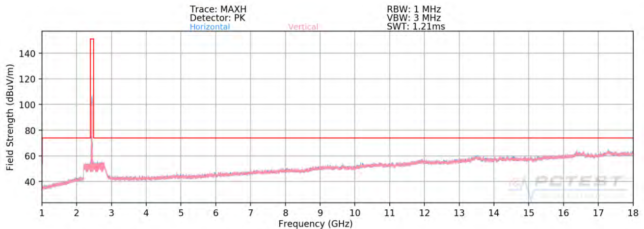
Plot 7-85. Radiated Spurious Plot above 1GHz MIMO (802.11ax OFDMA – 242 Tones – Ch. 6 – CLOSED)
