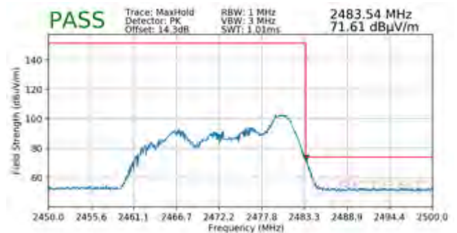
Plot 7-152. Radiated Restricted Upper Band Edge Measurement MIMO (Peak – 26 Tones)
