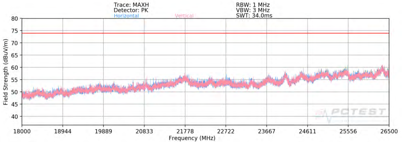
Plot 7-71. Radiated Spurious Plot above 18GHz SISO ANT1 (802.11ax OFDMA – 106 Tones – CLOSED)
