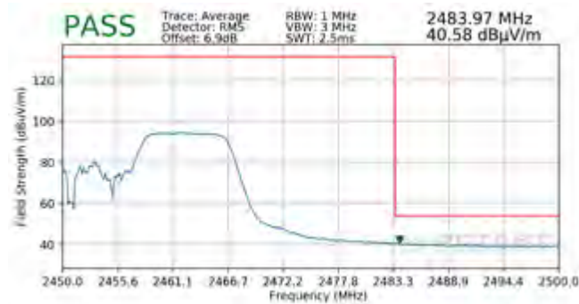
Plot 7-145. Radiated Restricted Upper Band Edge Measurement MIMO (Average – 106 Tones)
