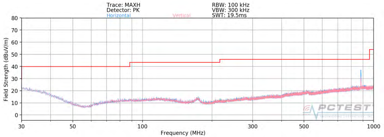
Plot 7-171. Radiated Spurious Plot below 1GHz MIMO (106 Tones - CLOSED)
