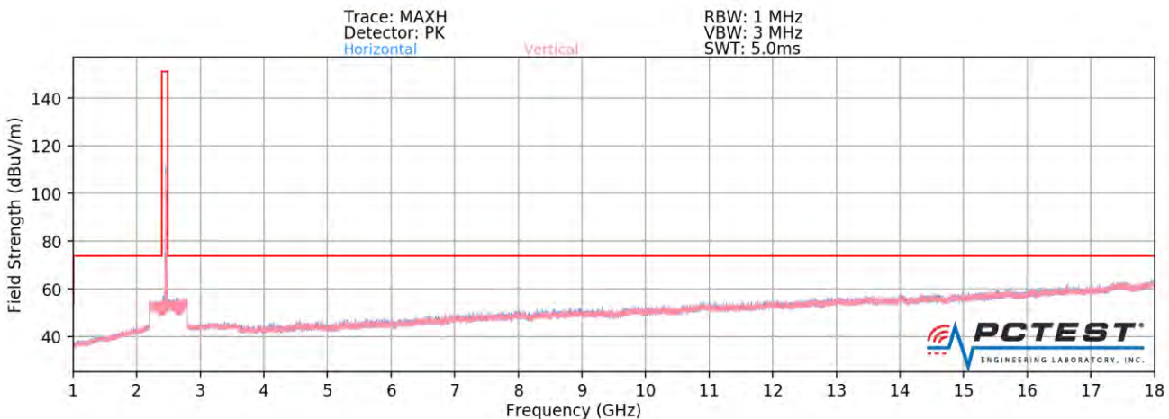
Plot 7-83. Radiated Spurious Plot above 1GHz MIMO (802.11ax OFDMA – 106 Tones – Ch. 11 – CLOSED)
