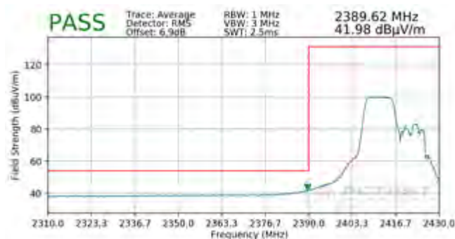
Plot 7-91. Radiated Restricted Lower Band Edge Measurement SISO ANT1 (Average – 106 Tones)
