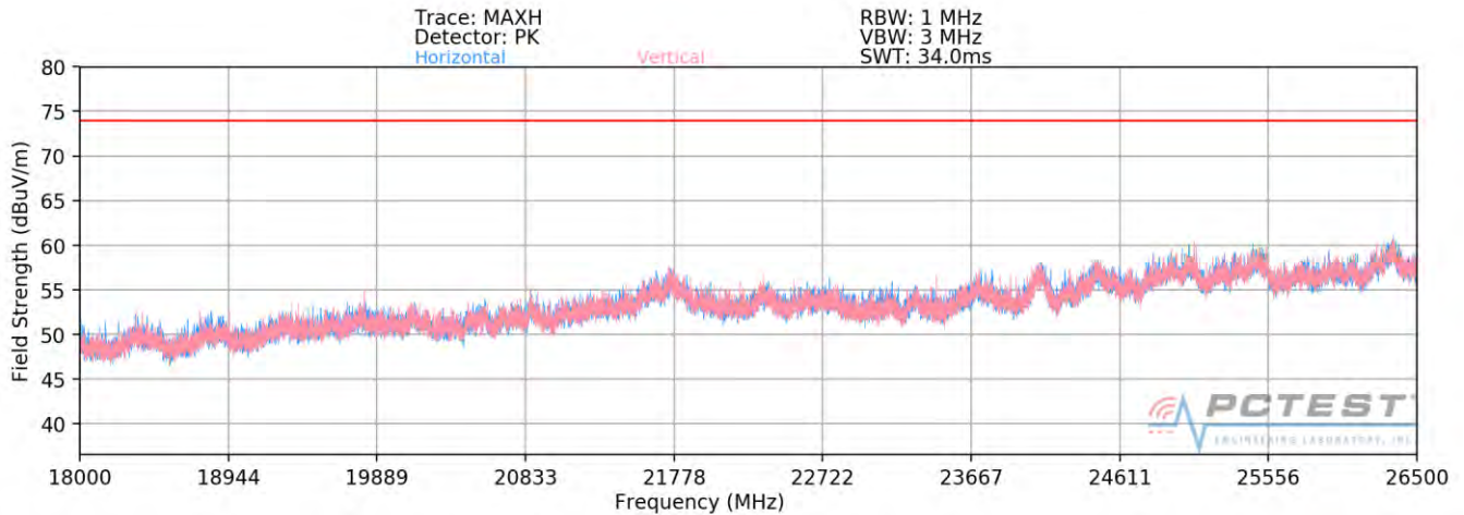
Plot 7-87. Radiated Spurious Plot above 18GHz MIMO (802.11ax OFDMA – 106 Tones – CLOSED)
