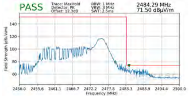
Plot 7-98. Radiated Restricted Upper Band Edge Measurement SISO ANT1 (Peak – 26 Tones)
