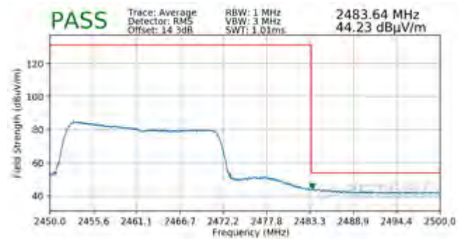
Plot 7-139. Radiated Restricted Band Edge Measurement SISO ANT2 with WCP (Average – 242 Tones)
