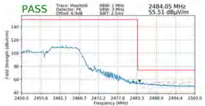
Plot 7-94. Radiated Restricted Upper Band Edge Measurement SISO ANT1 (Peak – 106 Tones)
