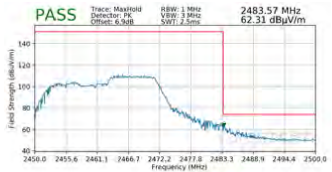
Plot 7-96. Radiated Restricted Upper Band Edge Measurement SISO ANT1 (Peak – 106 Tones)
