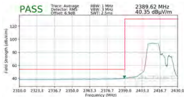
Plot 7-143. Radiated Restricted Lower Band Edge Measurement MIMO (Average – 106 Tones)
