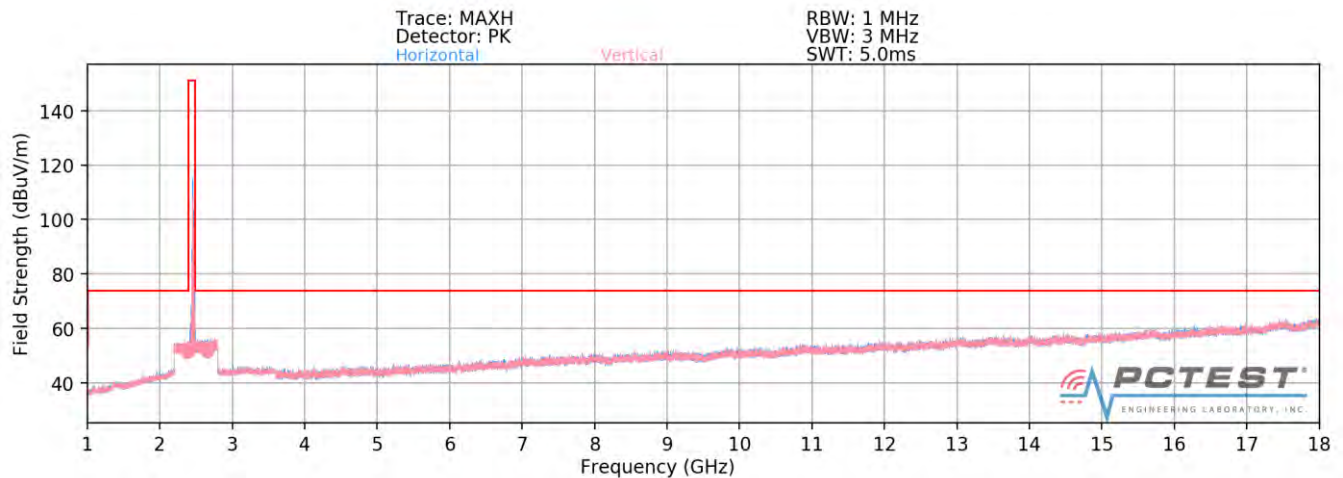
Plot 7-67. Radiated Spurious Plot above 1GHz SISO ANT1 (802.11ax OFDMA – 106 Tones – Ch. 11 – CLOSED)
