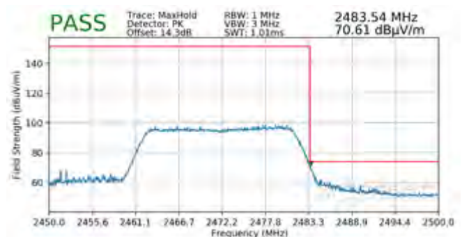
Plot 7-164. Radiated Restricted Upper Band Edge Measurement MIMO (Peak – 242 Tones)
