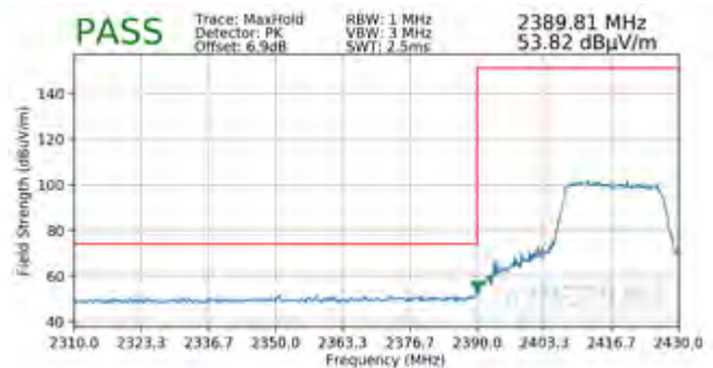
Plot 7-130. Radiated Restricted Lower Band Edge Measurement SISO ANT2 (Peak – 242 Tones)
