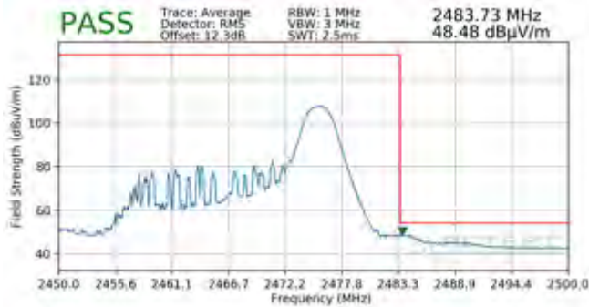
Plot 7-97. Radiated Restricted Upper Band Edge Measurement SISO ANT1 (Average – 26 Tones)
