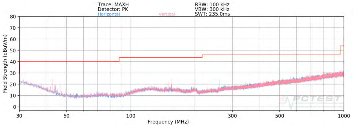
Plot 7-168. Radiated Spurious Plot below 1GHz SISO ANT1 (242 Tones - CLOSED)
