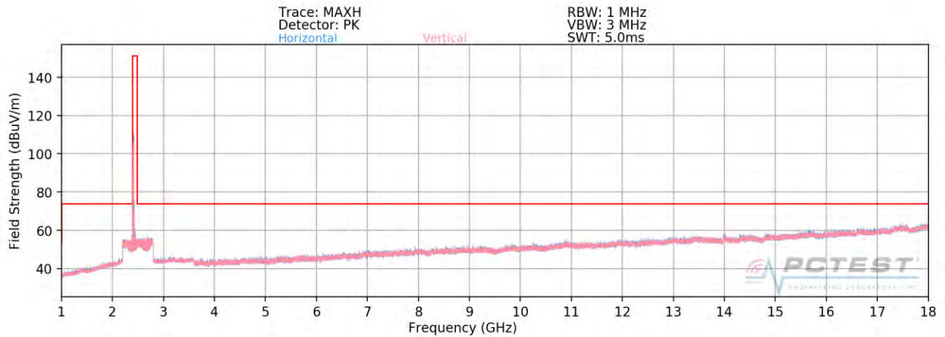
Plot 7-65. Radiated Spurious Plot above 1GHz SISO ANT1 (802.11ax OFDMA – 106 Tones – Ch. 1 – CLOSED)
