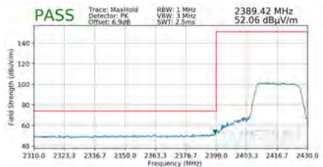
Plot 7-156. Radiated Restricted Lower Band Edge Measurement MIMO (Peak – 242 Tones)
