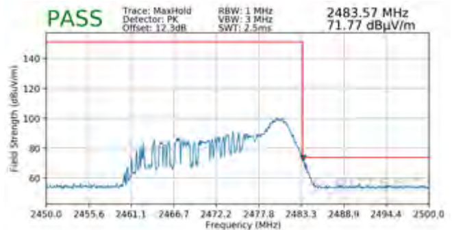
Plot 7-100. Radiated Restricted Upper Band Edge Measurement SISO ANT1 (Peak – 26 Tones)
