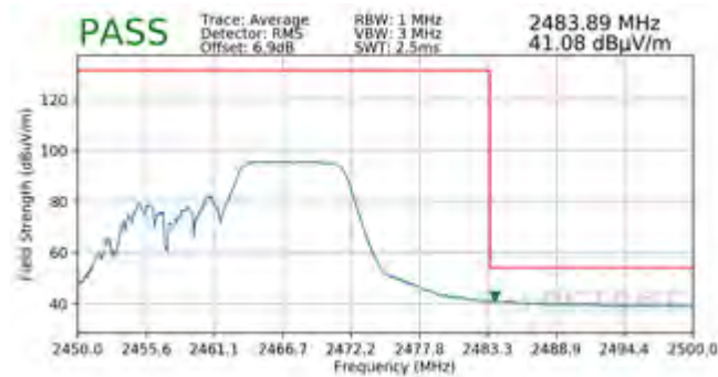
Plot 7-147. Radiated Restricted Upper Band Edge Measurement MIMO (Average – 106 Tones)
