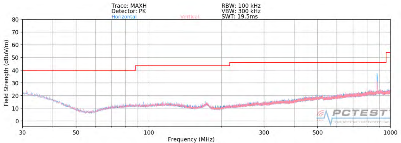
Plot 7-172. Radiated Spurious Plot below 1GHz MIMO (242 Tones - CLOSED)
