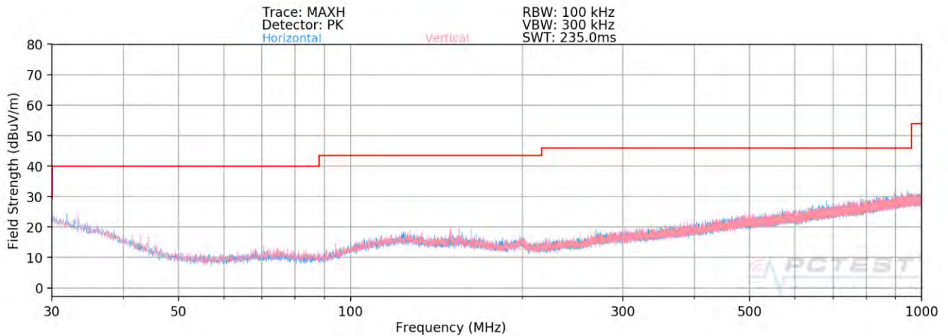
Plot 7-170. Radiated Spurious Plot below 1GHz SISO ANT2 (242 Tones - CLOSED)
