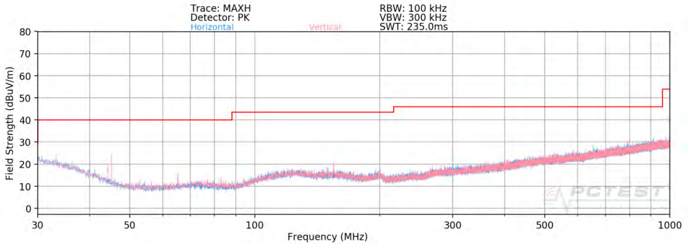
Plot 7-167. Radiated Spurious Plot below 1GHz SISO ANT1 (106 Tones - CLOSED)
