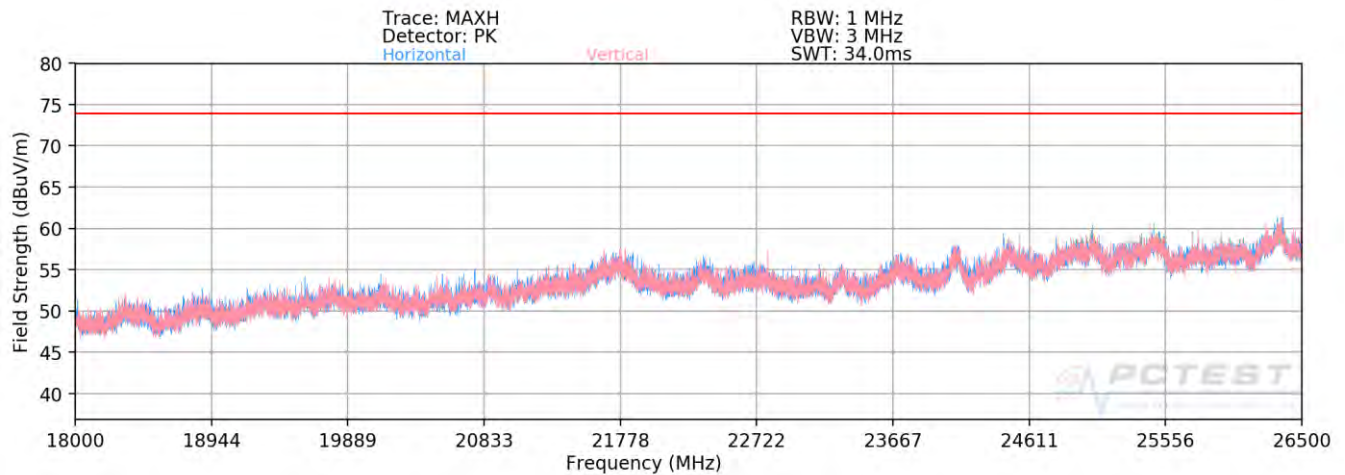
Plot 7-79. Radiated Spurious Plot above 18GHz SISO ANT2 (802.11ax OFDMA – 106 Tones – CLOSED)
