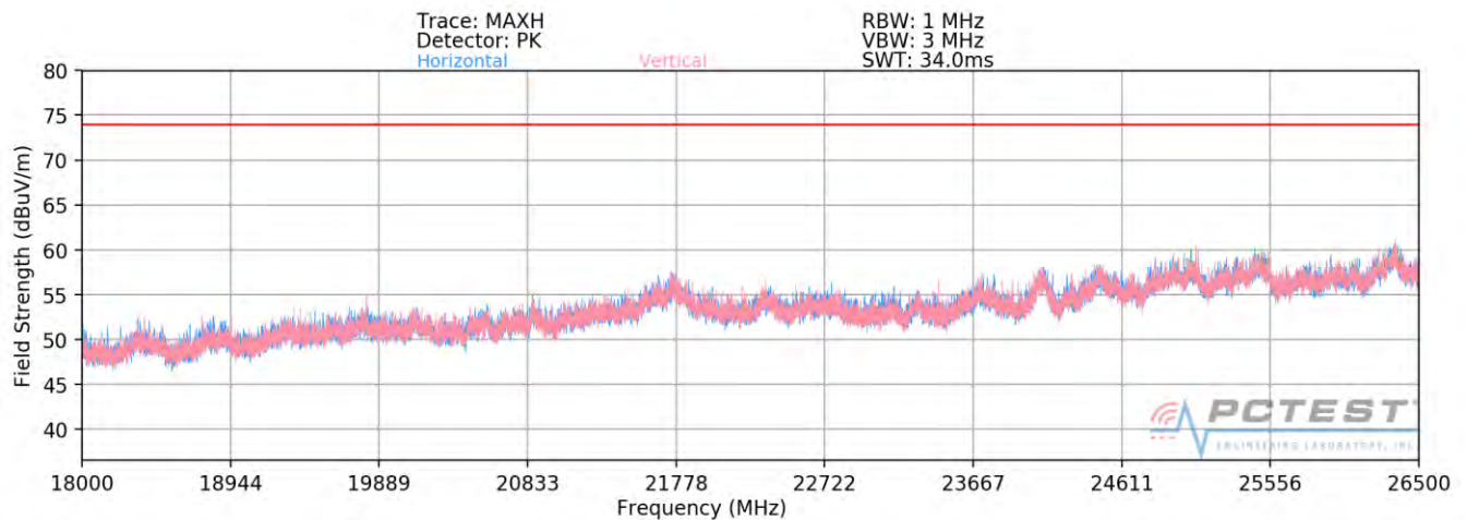
Plot 7-80. Radiated Spurious Plot above 18GHz SISO ANT2 (802.11ax OFDMA – 242 Tones – CLOSED)
