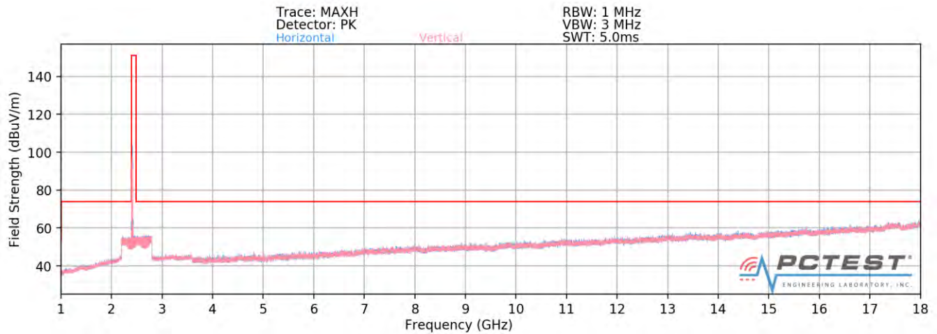
Plot 7-73. Radiated Spurious Plot above 1GHz SISO ANT2 (802.11ax OFDMA – 106 Tones – Ch. 1 – CLOSED)
