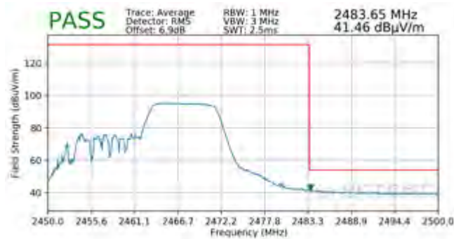
Plot 7-121. Radiated Restricted Upper Band Edge Measurement SISO ANT2 (Average – 106 Tones)
