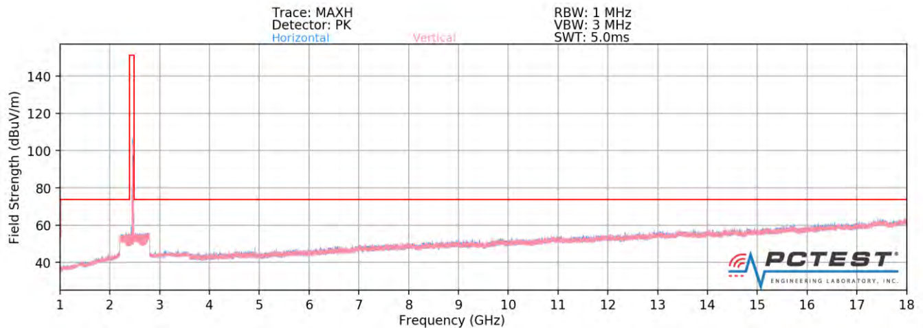
Plot 7-75. Radiated Spurious Plot above 1GHz SISO ANT2 (802.11ax OFDMA – 106 Tones – Ch. 11 – CLOSED)
