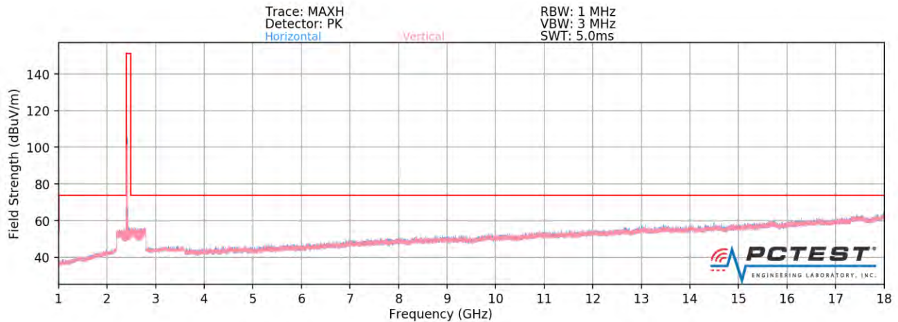
Plot 7-81. Radiated Spurious Plot above 1GHz MIMO (802.11ax OFDMA – 106 Tones – Ch. 1 – CLOSED)
