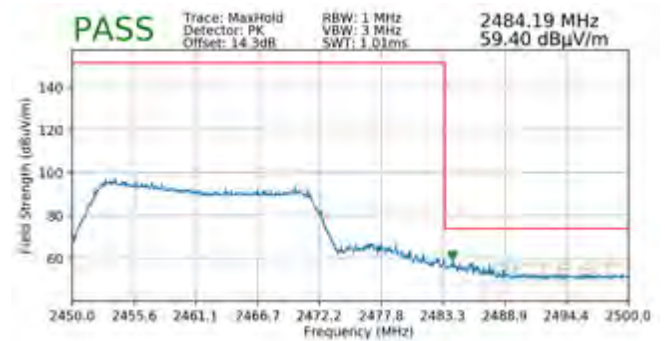
Plot 7-140. Radiated Restricted Band Edge Measurement SISO ANT2 with WCP (Peak – 242 Tones)
