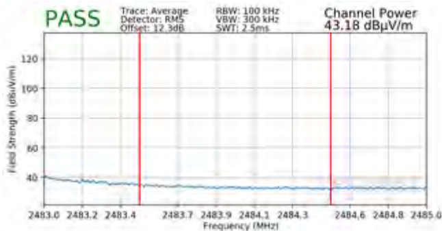
Plot 7-99. Radiated Restricted Upper Band Edge Measurement SISO ANT1 (Average – 26 Tones)
