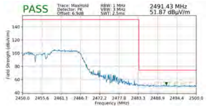
Plot 7-120. Radiated Restricted Upper Band Edge Measurement SISO ANT2 (Peak – 106 Tones)
