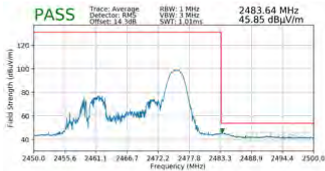
Plot 7-123. Radiated Restricted Upper Band Edge Measurement SISO ANT2 (Average – 26 Tones)
