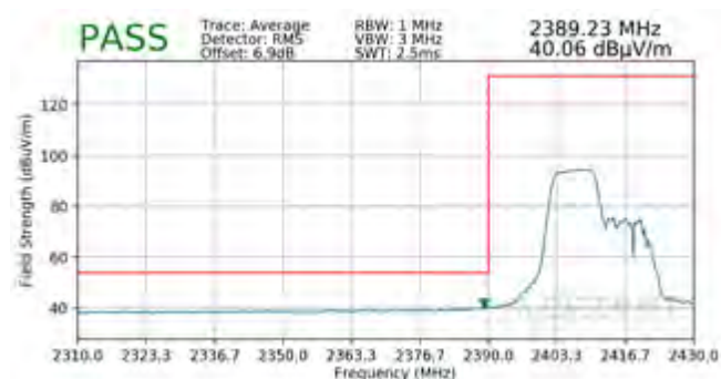
Plot 7-115. Radiated Restricted Lower Band Edge Measurement SISO ANT2 (Average – 106 Tones)
