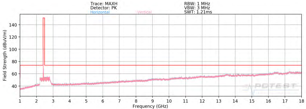
Plot 7-84. Radiated Spurious Plot above 1GHz MIMO (802.11ax OFDMA – 242 Tones – Ch. 1 – CLOSED)
