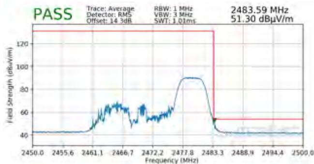
Plot 7-125. Radiated Restricted Upper Band Edge Measurement SISO ANT2 (Average – 52 Tones)
