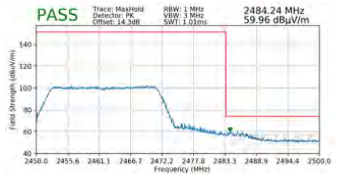
Plot 7-166. Radiated Restricted Band Edge Measurement MIMO with WCP (Peak – 242 Tones)
