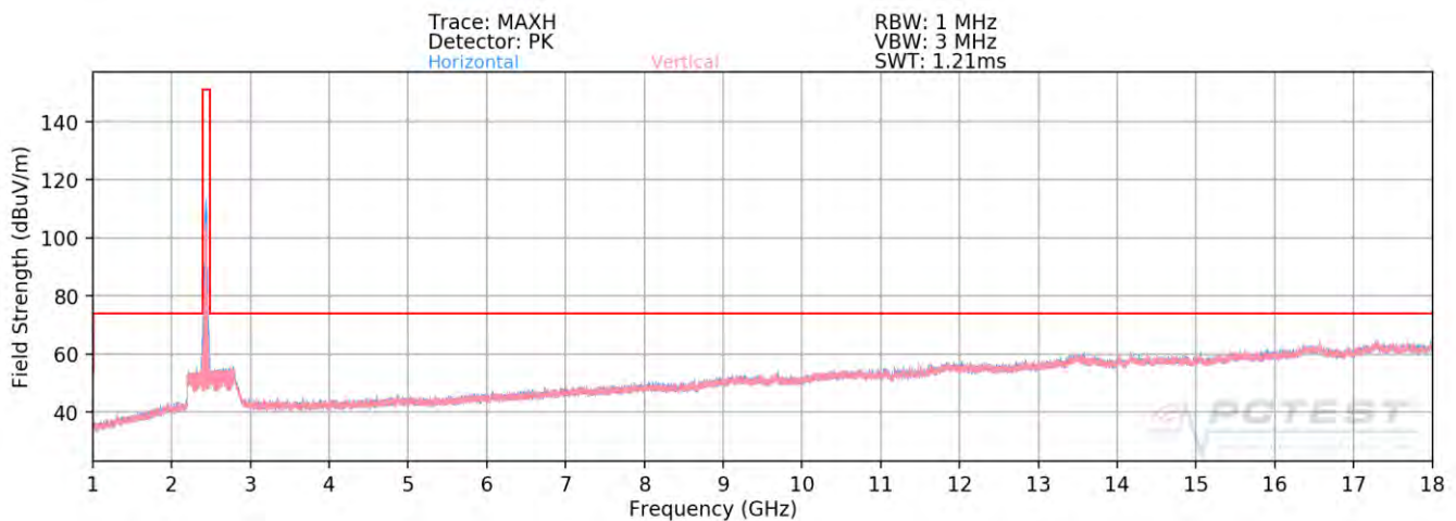
Plot 7-69. Radiated Spurious Plot above 1GHz SISO ANT1 (802.11ax OFDMA – 242 Tones – Ch. 6 – CLOSED)
