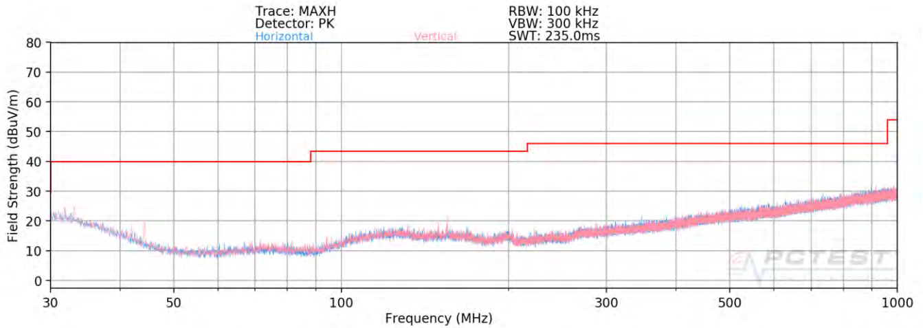
Plot 7-169. Radiated Spurious Plot below 1GHz SISO ANT2 (106 Tones - CLOSED)
