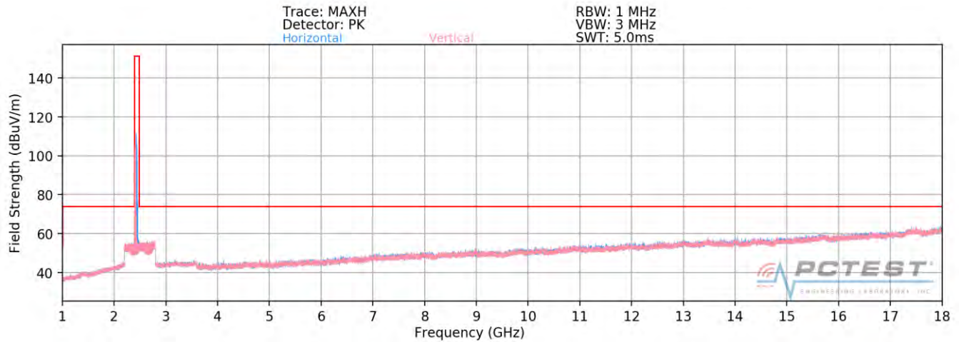
Plot 7-66. Radiated Spurious Plot above 1GHz SISO ANT1 (802.11ax OFDMA – 106 Tones – Ch. 6 – CLOSED)
