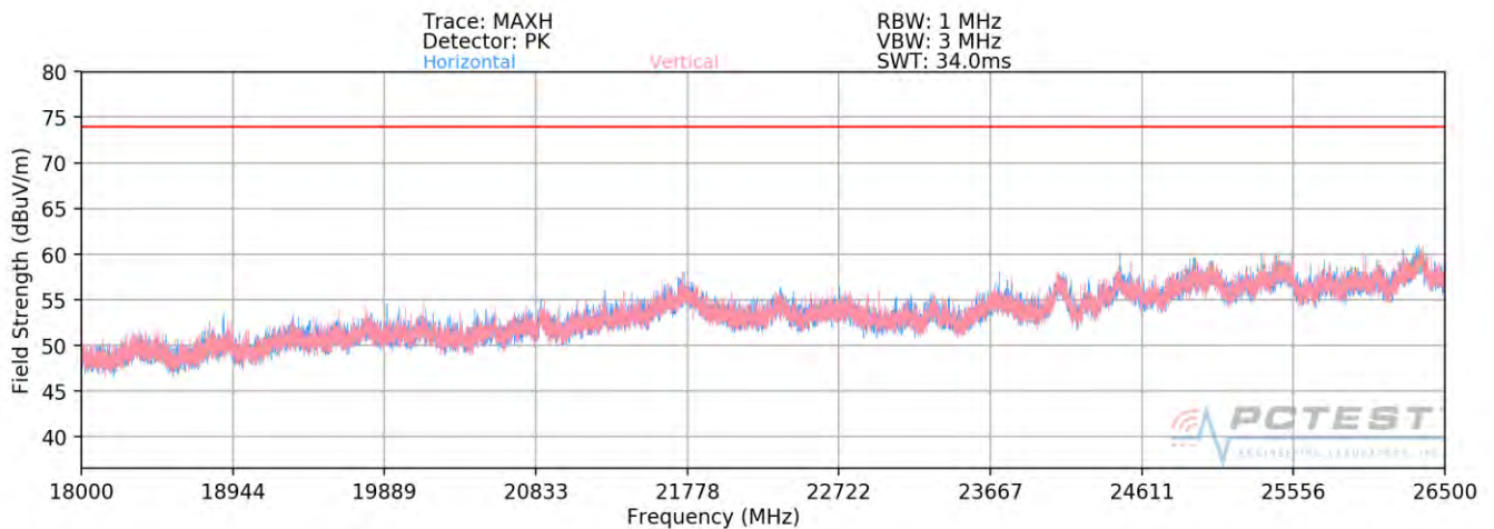
Plot 7-72. Radiated Spurious Plot above 18GHz SISO ANT1 (802.11ax OFDMA – 242 Tones – CLOSED)
