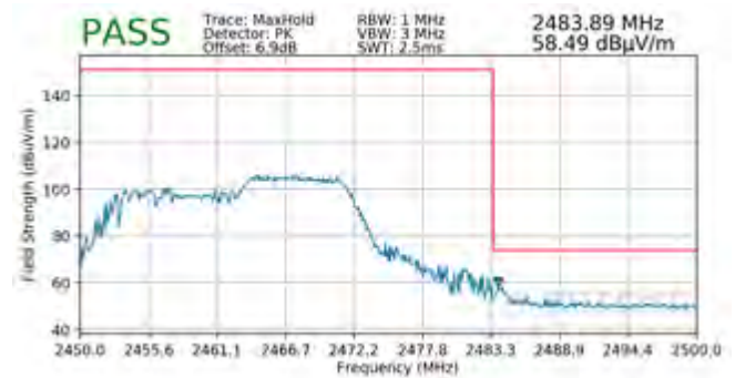
Plot 7-122. Radiated Restricted Upper Band Edge Measurement SISO ANT2 (Peak – 106 Tones)
