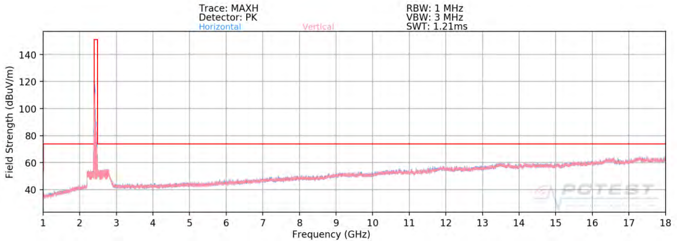
Plot 7-68. Radiated Spurious Plot above 1GHz SISO ANT1 (802.11ax OFDMA – 242 Tones – Ch. 1 – CLOSED)
