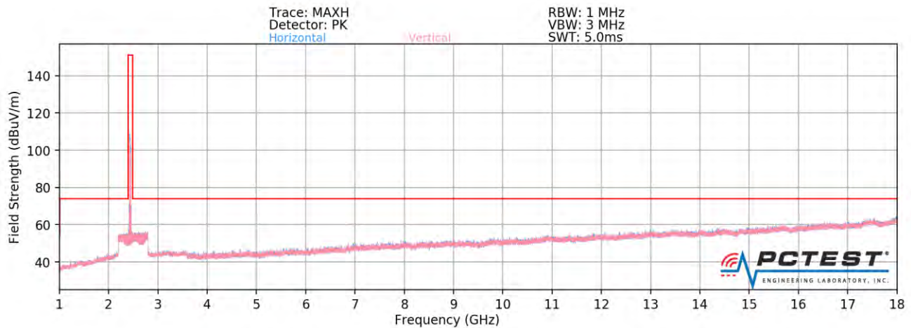
Plot 7-82. Radiated Spurious Plot above 1GHz MIMO (802.11ax OFDMA – 106 Tones – Ch. 6 – CLOSED)
