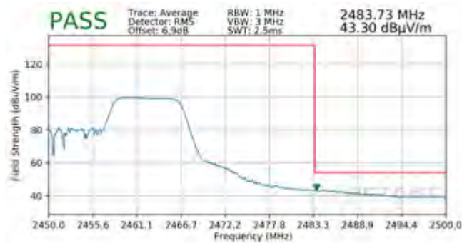
Plot 7-93. Radiated Restricted Upper Band Edge Measurement SISO ANT1 (Average – 106 Tones)
