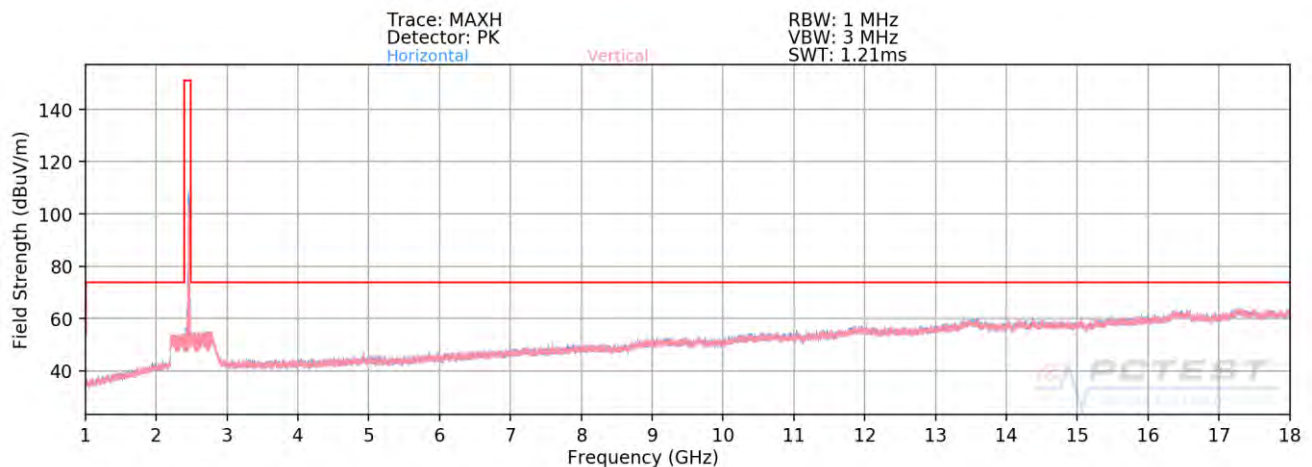
Plot 7-86. Radiated Spurious Plot above 1GHz MIMO (802.11ax OFDMA – 242 Tones – Ch. 11 – CLOSED)
