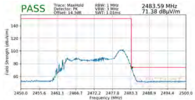
Plot 7-126. Radiated Restricted Upper Band Edge Measurement SISO ANT2 (Peak – 26 Tones)
