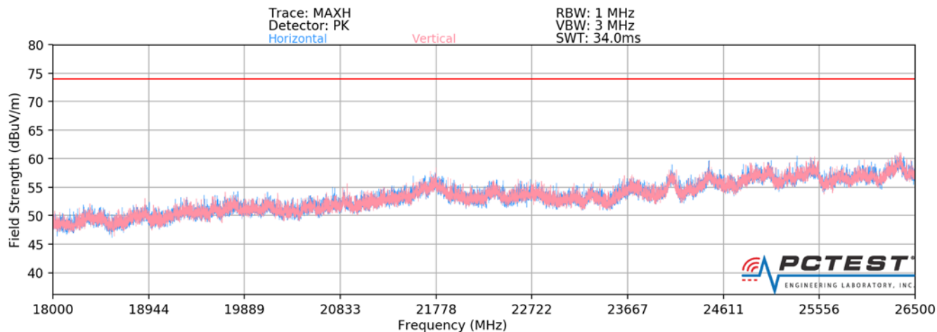
Plot 7-48. Radiated Spurious Plot above 18GHz – CLOSED
