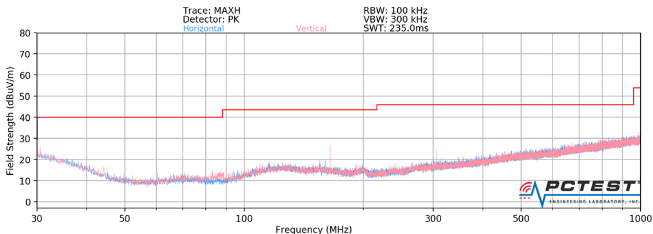
Plot 7-57. Radiated Spurious Plot below 1GHz - CLOSED
