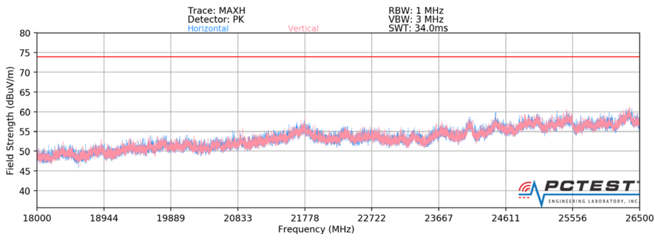
Plot 7-49. Radiated Spurious Plot above 18GHz - OPEN
