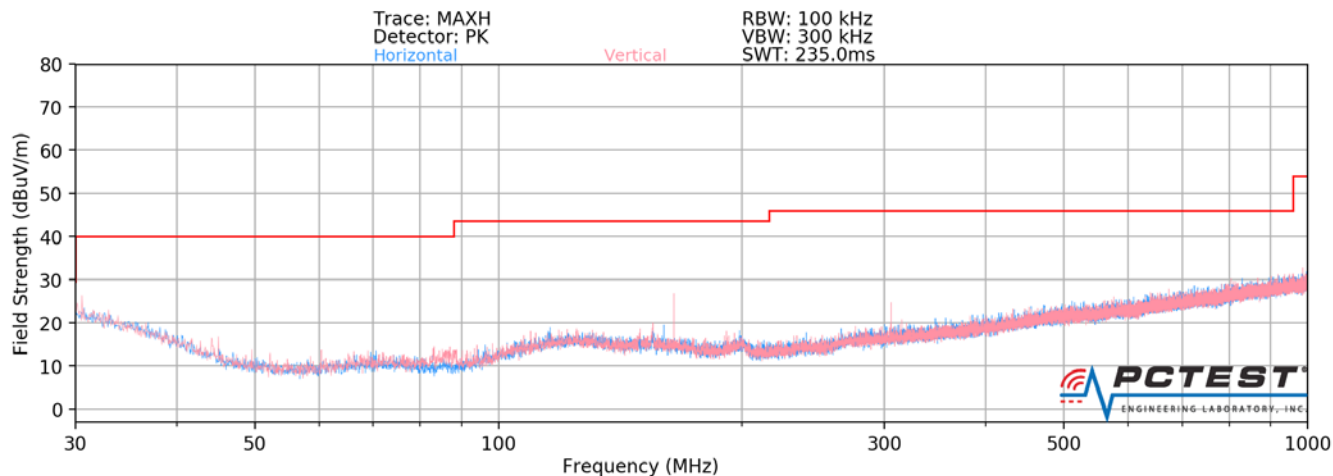
Plot 7-56. Radiated Spurious Plot below 1GHz – OPEN
