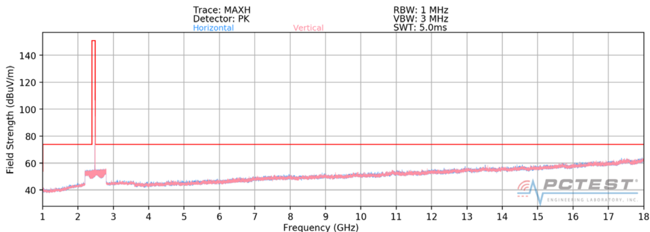
Plot 7-46. Radiated Spurious Plot above 1GHz (BT- Ch. 78 - OPEN)
