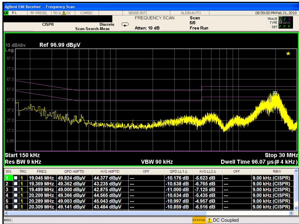
Plot 7-58. Line-Conducted Test Plot (L1)
