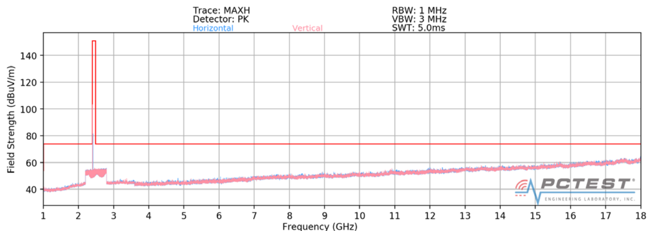
Plot 7-43. Radiated Spurious Plot above 1GHz (BT- Ch. 0 - CLOSED)
