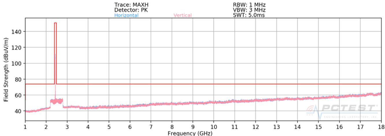
Plot 7-44. Radiated Spurious Plot above 1GHz (BT- Ch. 39 - OPEN)
