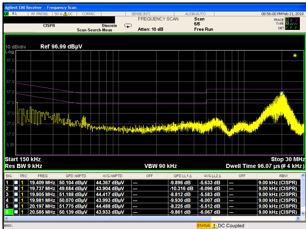
Plot 7-59. Line-Conducted Test Plot (N)
