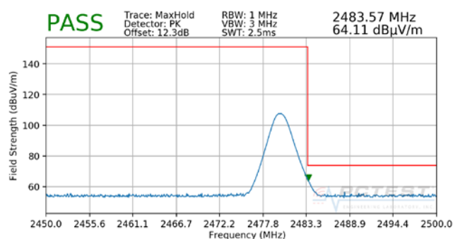
Plot 7-51. Radiated Restricted Upper Band Edge Measurement (Peak - OPEN)
