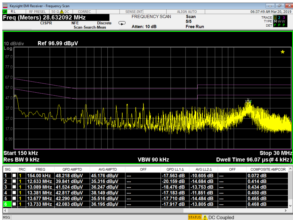
Plot 7-60. Line-Conducted Test Plot (L1 with WCP)
