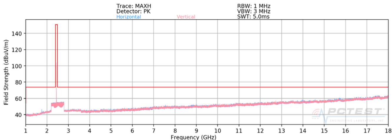
Plot 7-45. Radiated Spurious Plot above 1GHz (BT- Ch. 39 - CLOSED)
