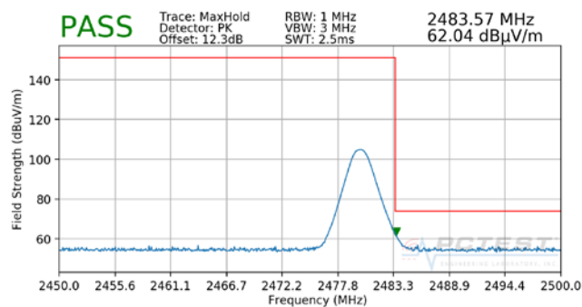
Plot 7-53. Radiated Restricted Upper Band Edge Measurement (Peak - CLOSED)
