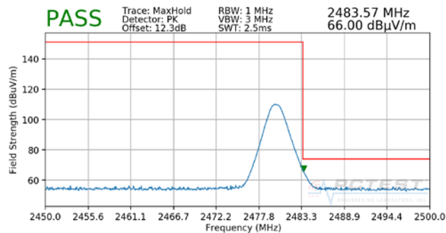
Plot 7-55. Radiated Restricted Upper Band Edge Measurement with WCP (Peak)
