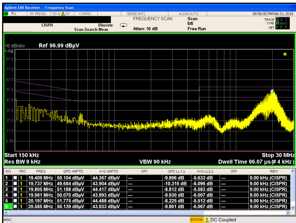
Plot 7-61. Line-Conducted Test Plot (N with WCP)
